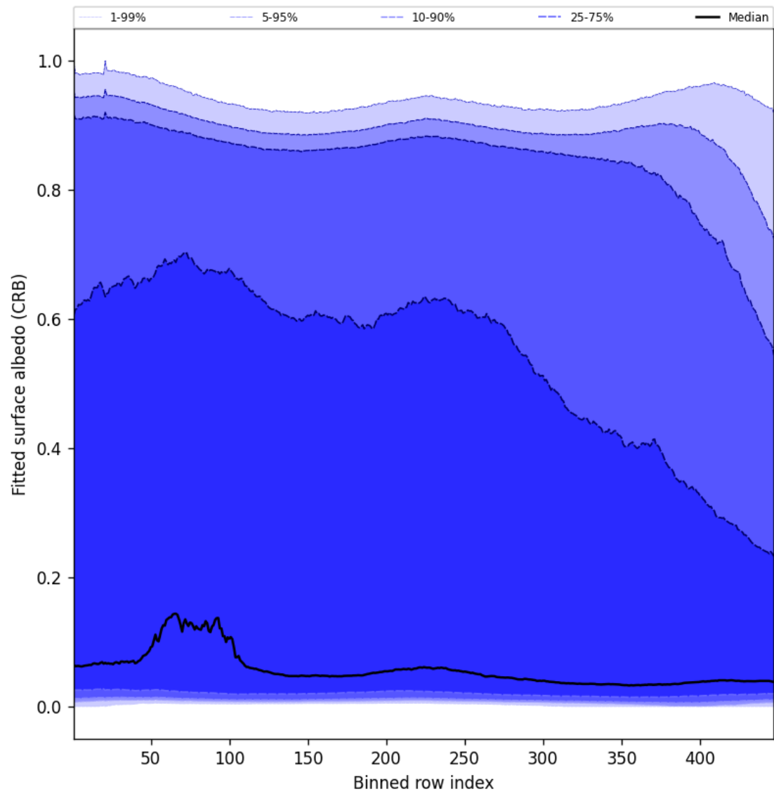
Figure 60: Along track statistics of “Fitted surface albedo (CRB)” for 2025-02-03 to 2025-02-04
