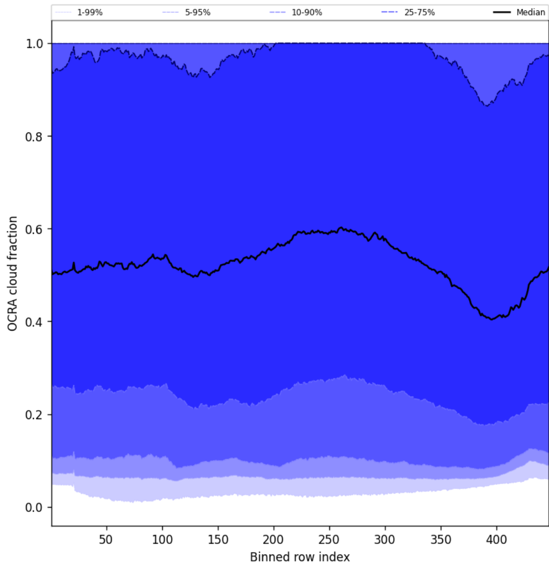
Figure 64: Along track statistics of “OCRA cloud fraction” for 2025-02-03 to 2025-02-04
