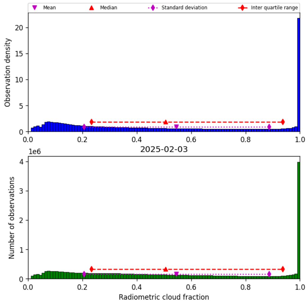
Figure 37: Histogram of “Radiometric cloud fraction” for 2025-02-03 to 2025-02-04
