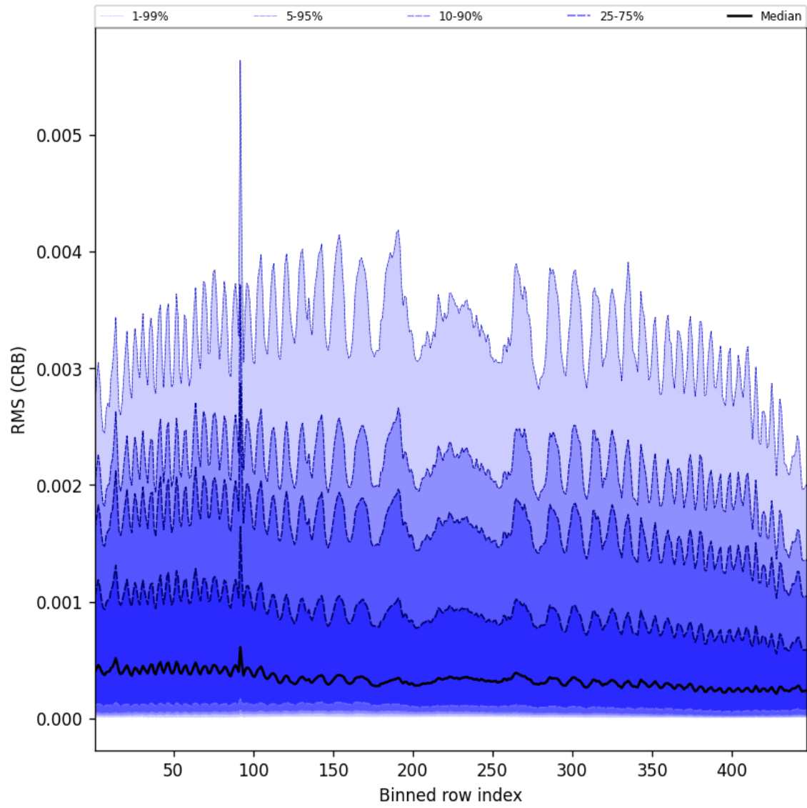
Figure 62: Along track statistics of “RMS (CRB)” for 2025-02-03 to 2025-02-04
