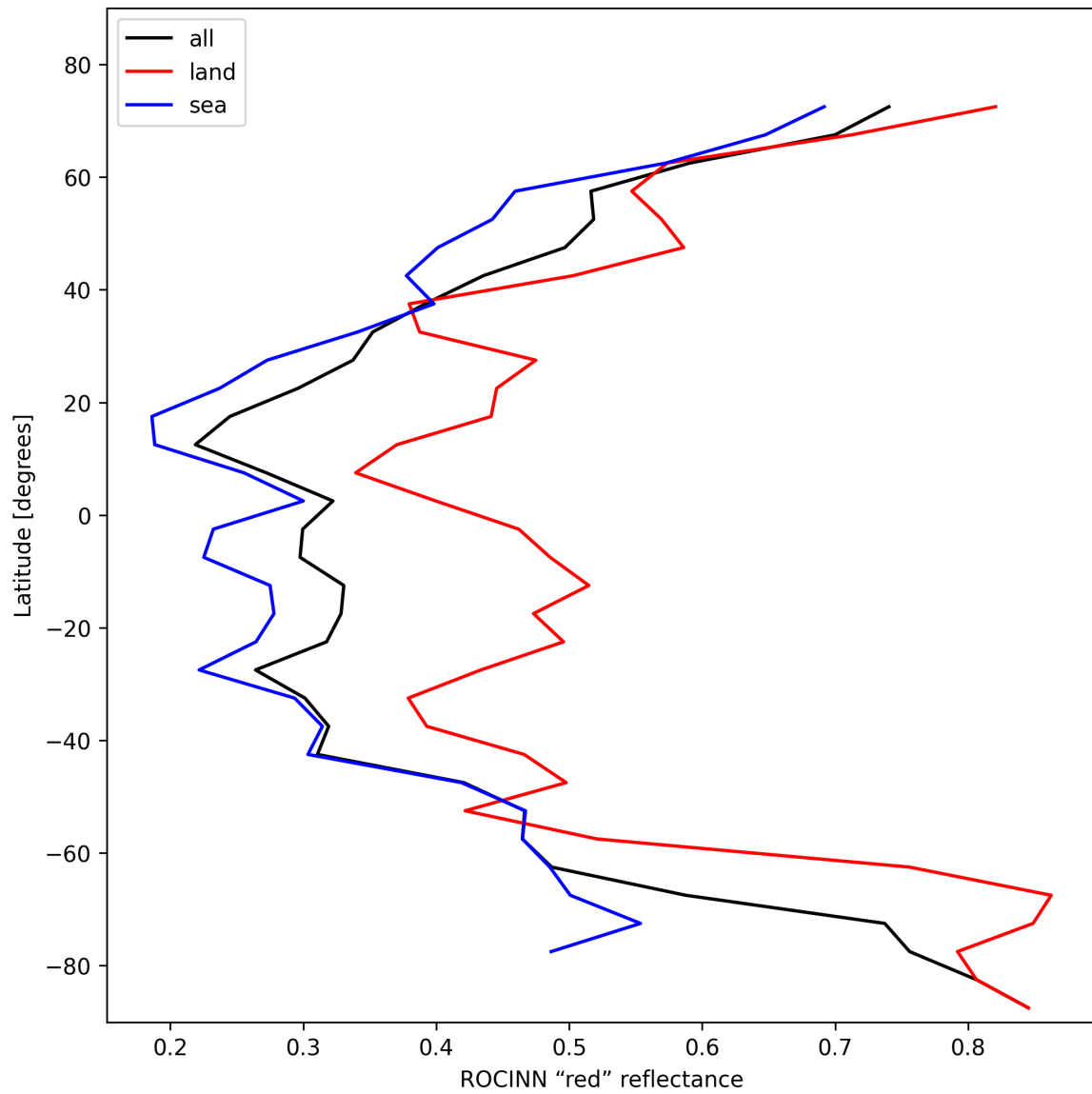
Figure 35: Zonal average of “ROCINN “red” reflectance” for 2025-02-03 to 2025-02-04.
