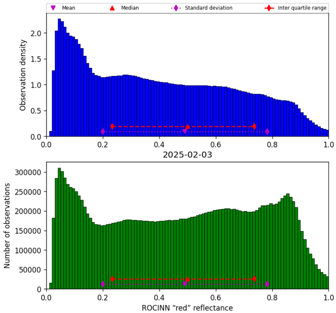
Figure 51: Histogram of “ROCINN “red” reflectance” for 2025-02-03 to 2025-02-04
