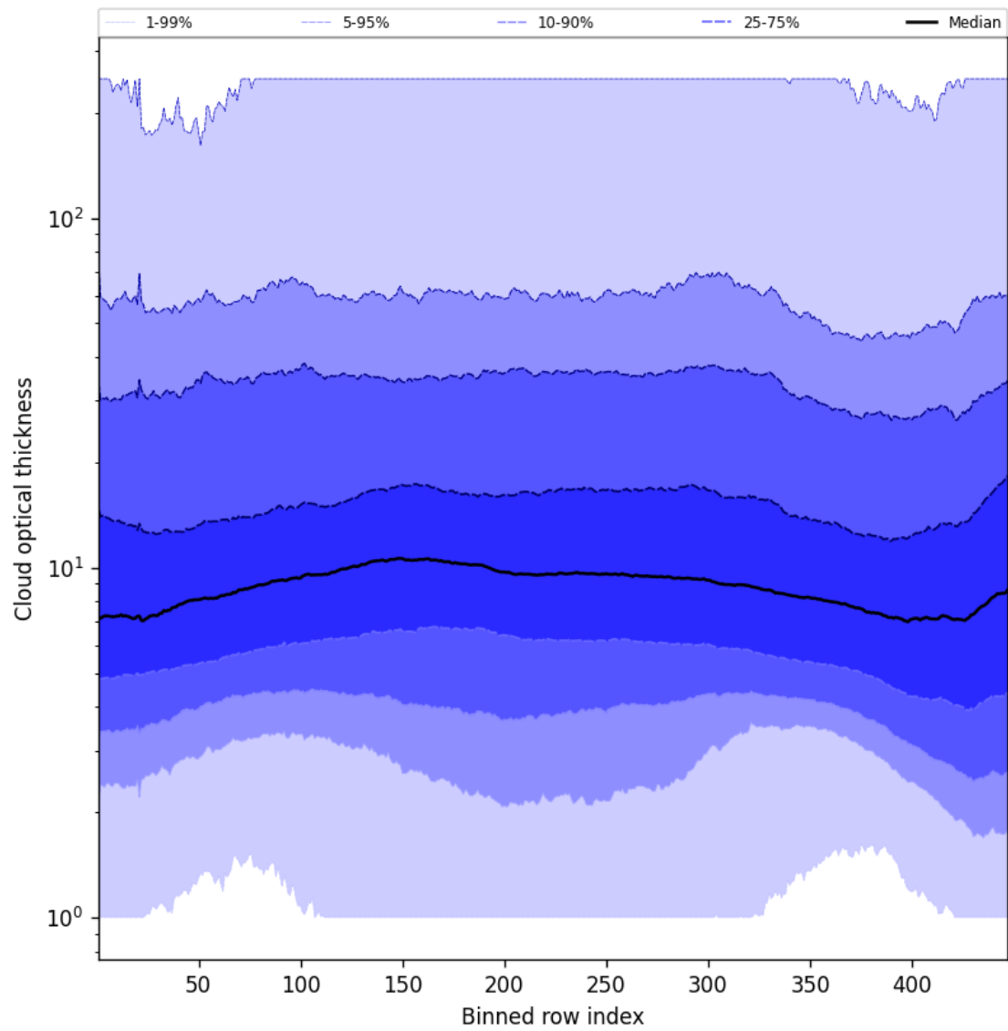
Figure 55: Along track statistics of “Cloud optical thickness” for 2025-02-03 to 2025-02-04
