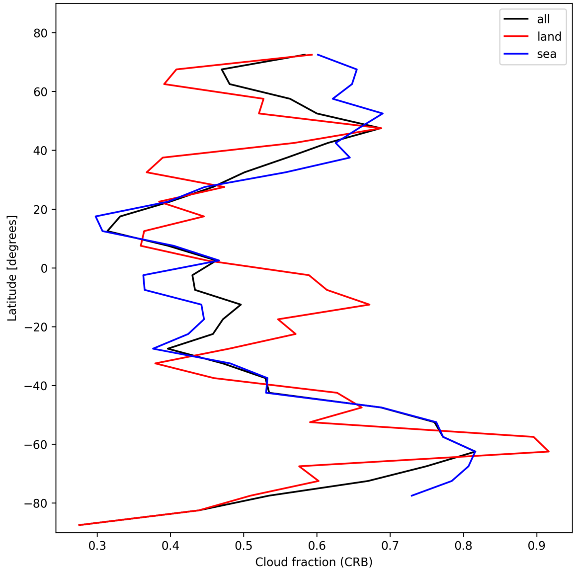
Figure 24: Zonal average of “Cloud fraction (CRB)” for 2025-02-03 to 2025-02-04.
