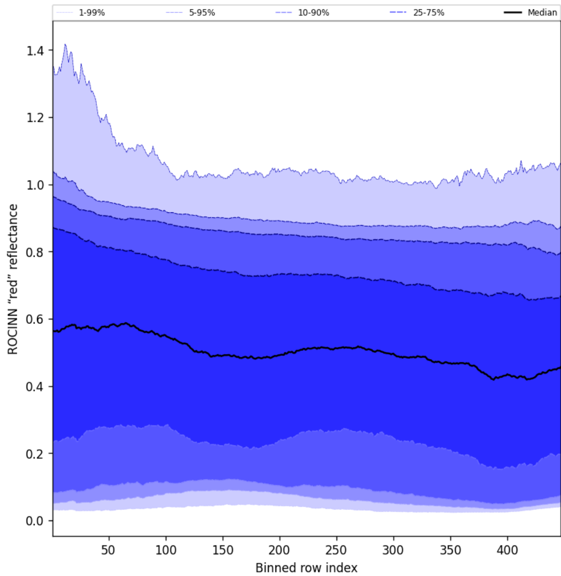
Figure 67: Along track statistics of "ROCINN "red" reflectance" for 2025-02-03 to 2025-02-04
