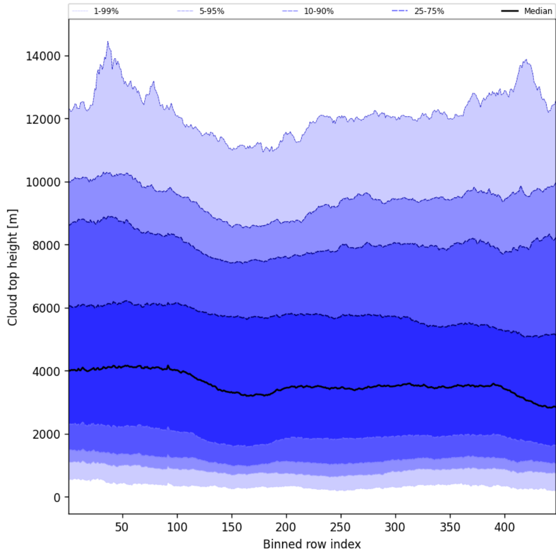
Figure 54: Along track statistics of “Cloud top height” for 2025-02-03 to 2025-02-04
