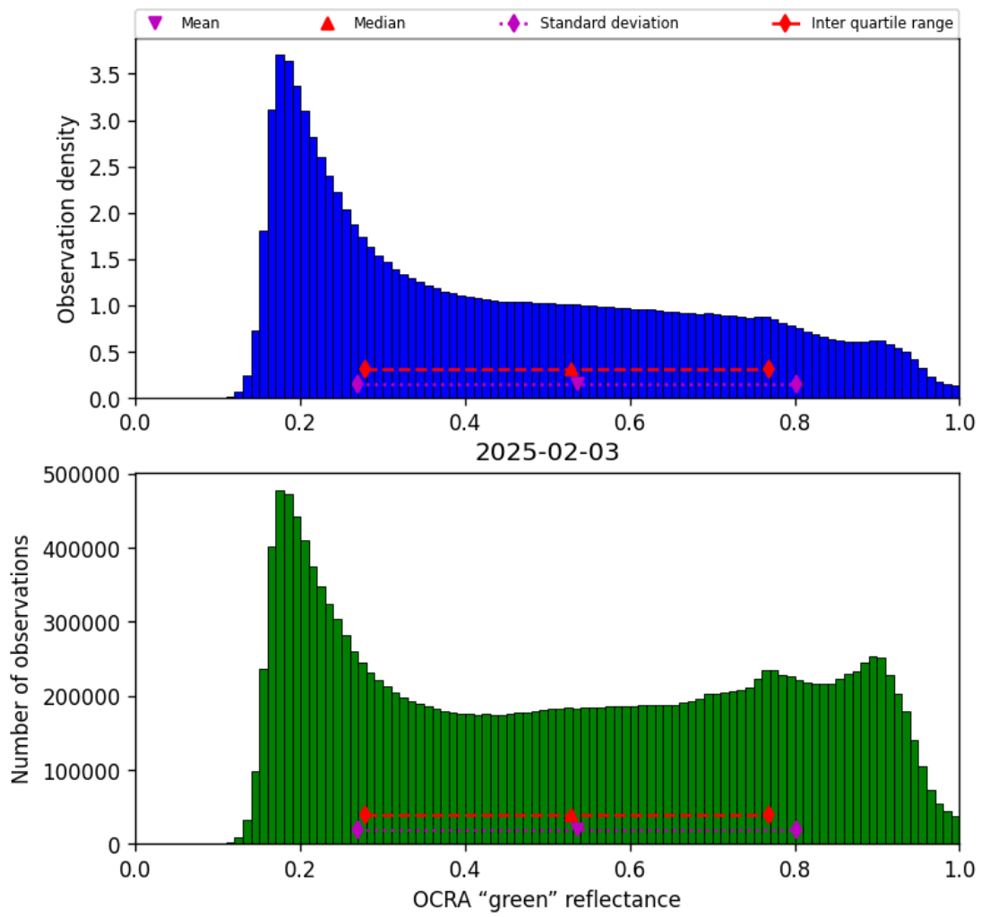
Figure 50: Histogram of “OCRA “green” reflectance” for 2025-02-03 to 2025-02-04
