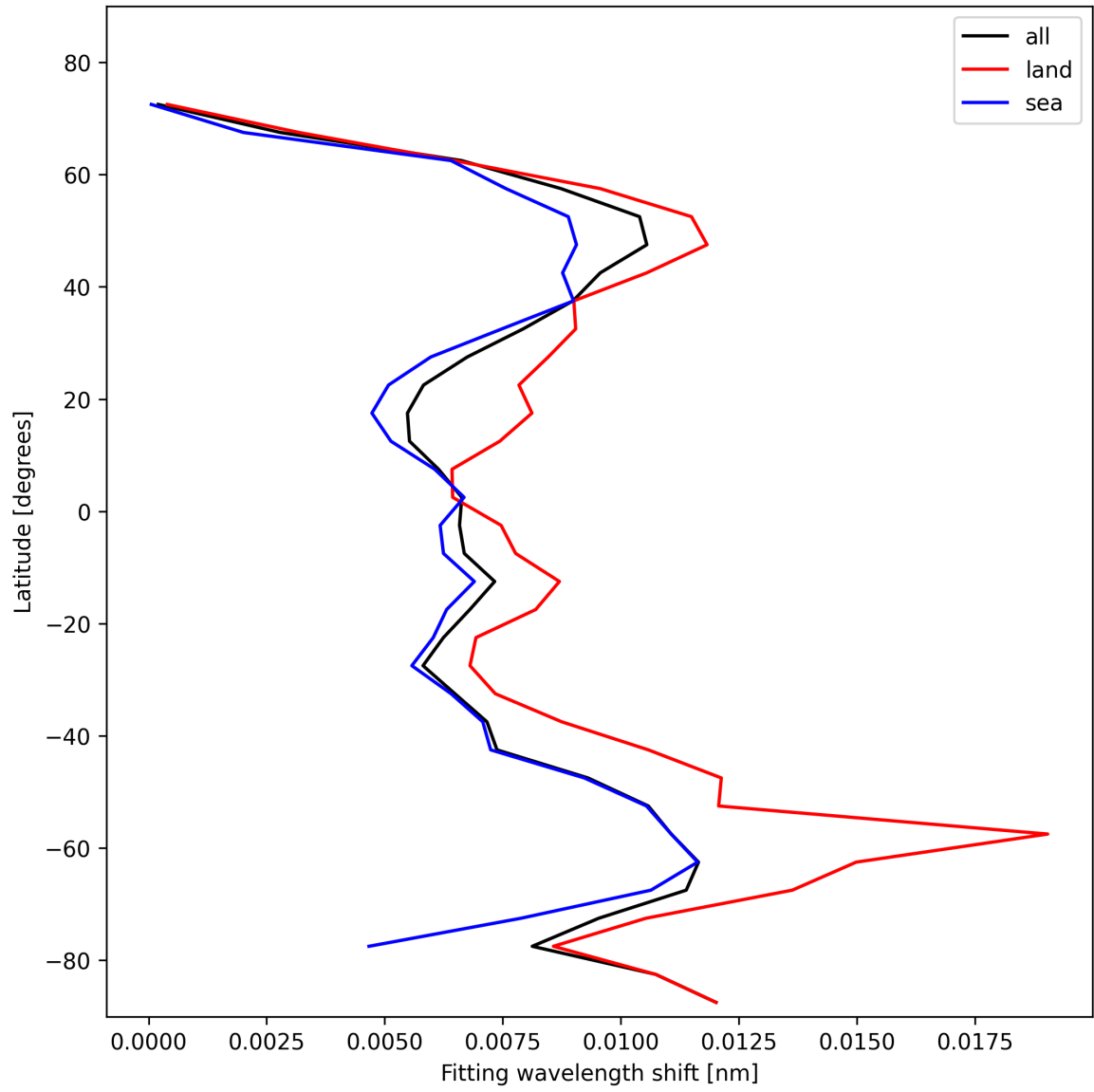
Figure 31: Zonal average of “Fitting wavelength shift” for 2025-02-03 to 2025-02-04.
