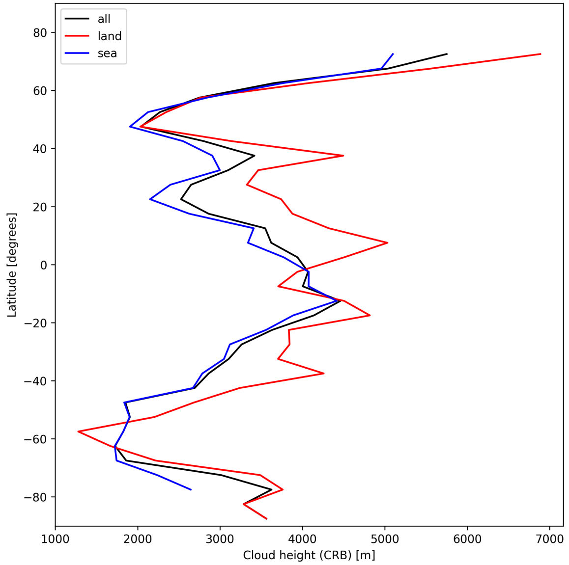
Figure 25: Zonal average of “Cloud height (CRB)” for 2025-02-03 to 2025-02-04.
