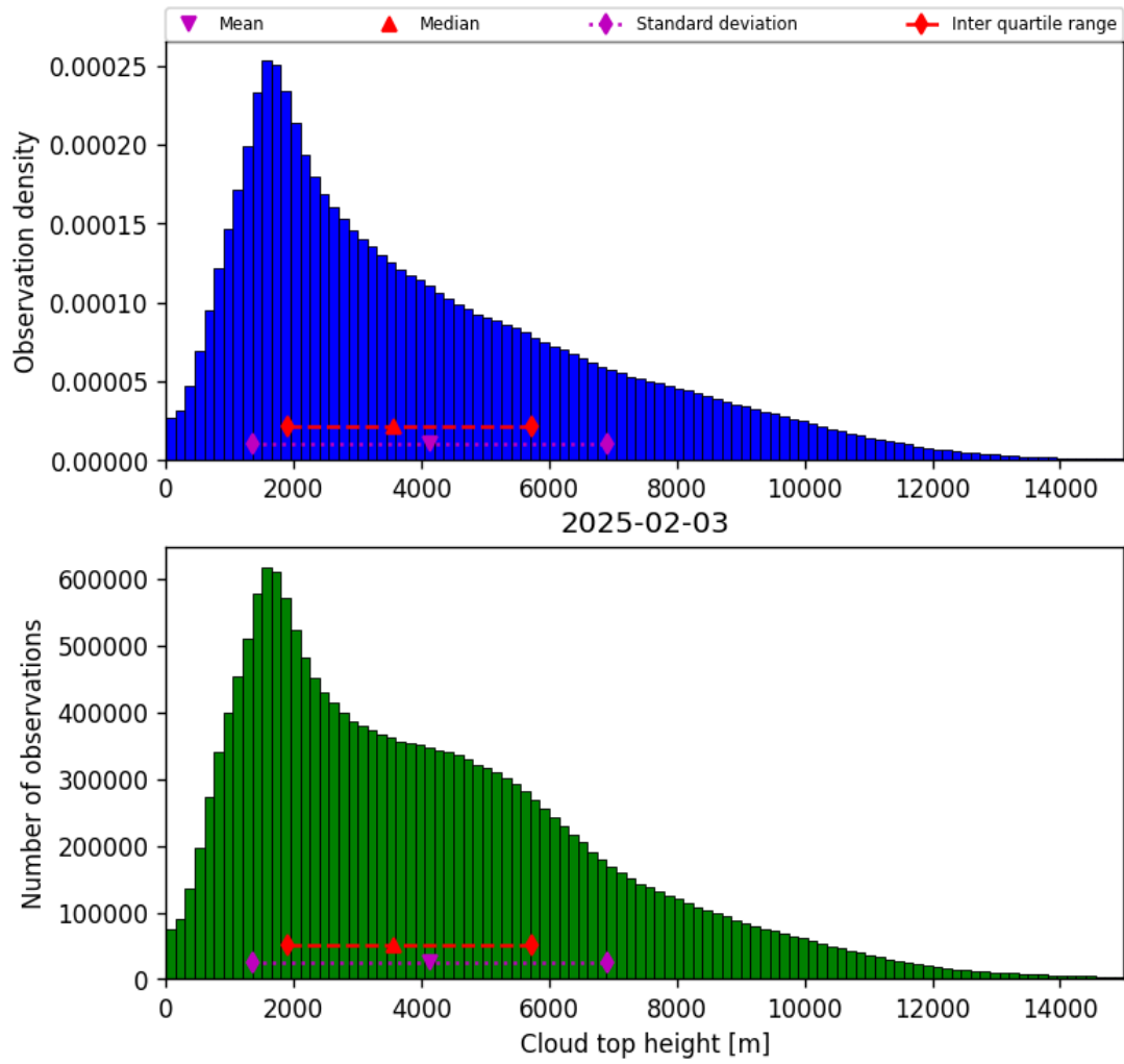
Figure 38: Histogram of “Cloud top height” for 2025-02-03 to 2025-02-04
