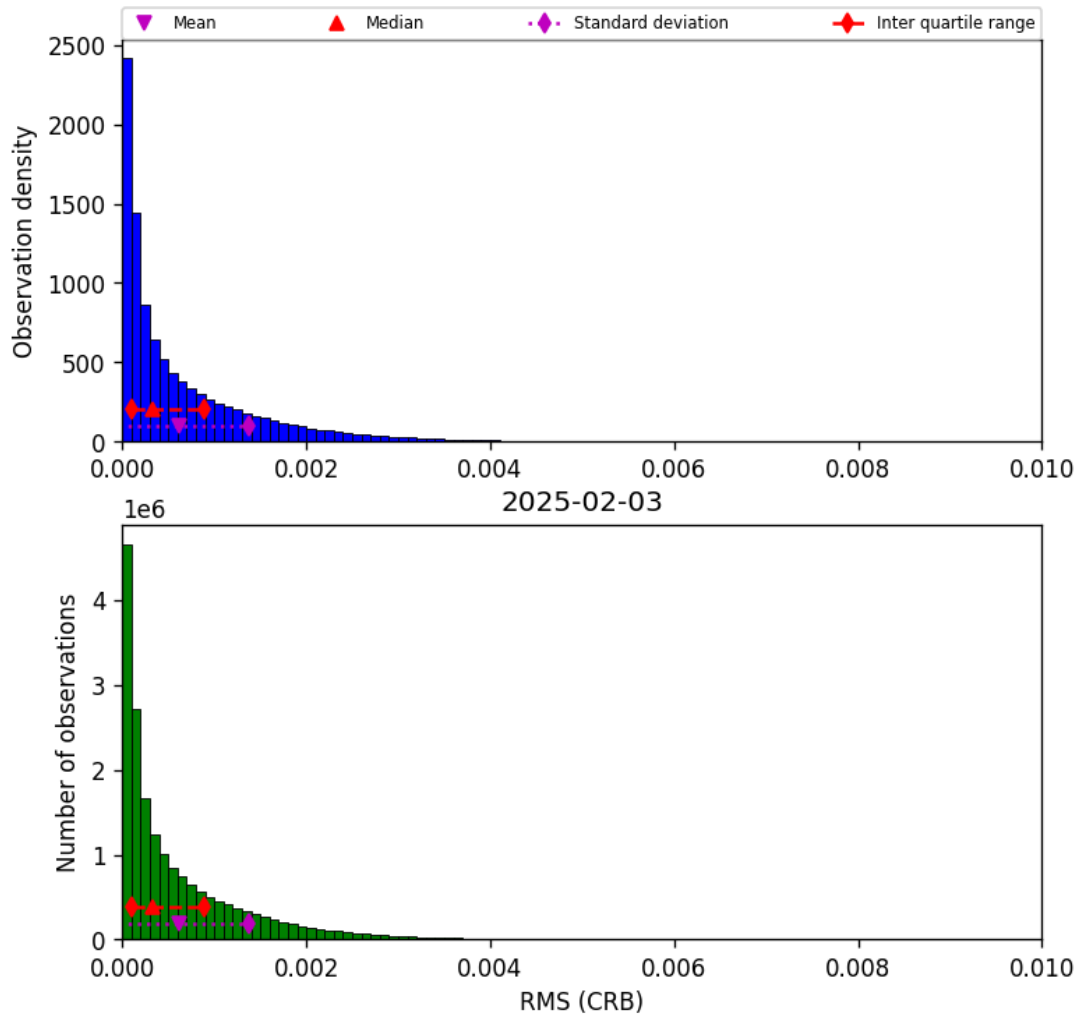
Figure 46: Histogram of “RMS (CRB)” for 2025-02-03 to 2025-02-04
