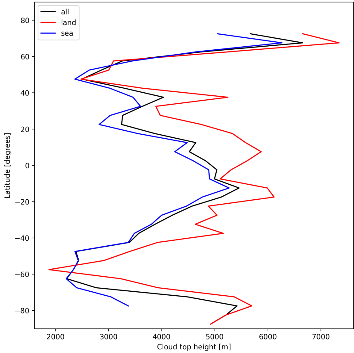
Figure 22: Zonal average of “Cloud top height” for 2025-02-03 to 2025-02-04.
