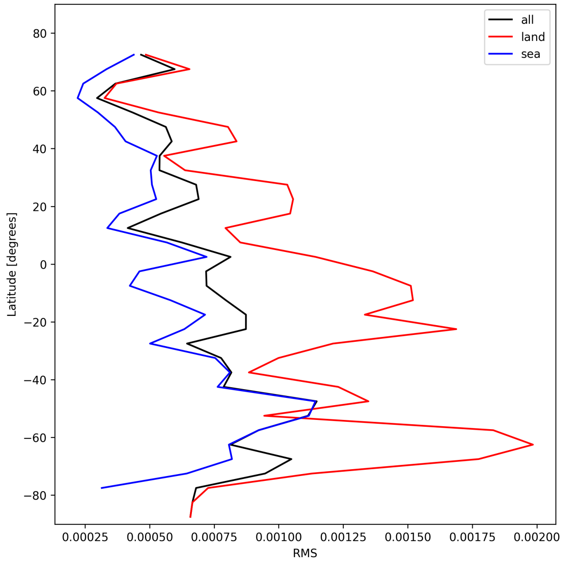
Figure 29: Zonal average of “RMS” for 2025-02-03 to 2025-02-04.
