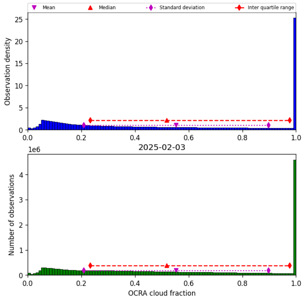
Figure 48: Histogram of “OCRA cloud fraction” for 2025-02-03 to 2025-02-04
