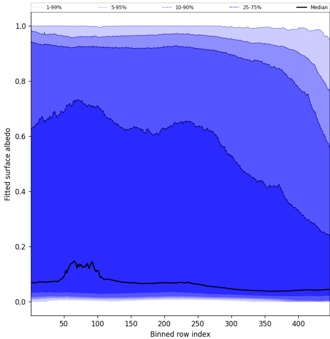
Figure 59: Along track statistics of “Fitted surface albedo” for 2025-02-03 to 2025-02-04
