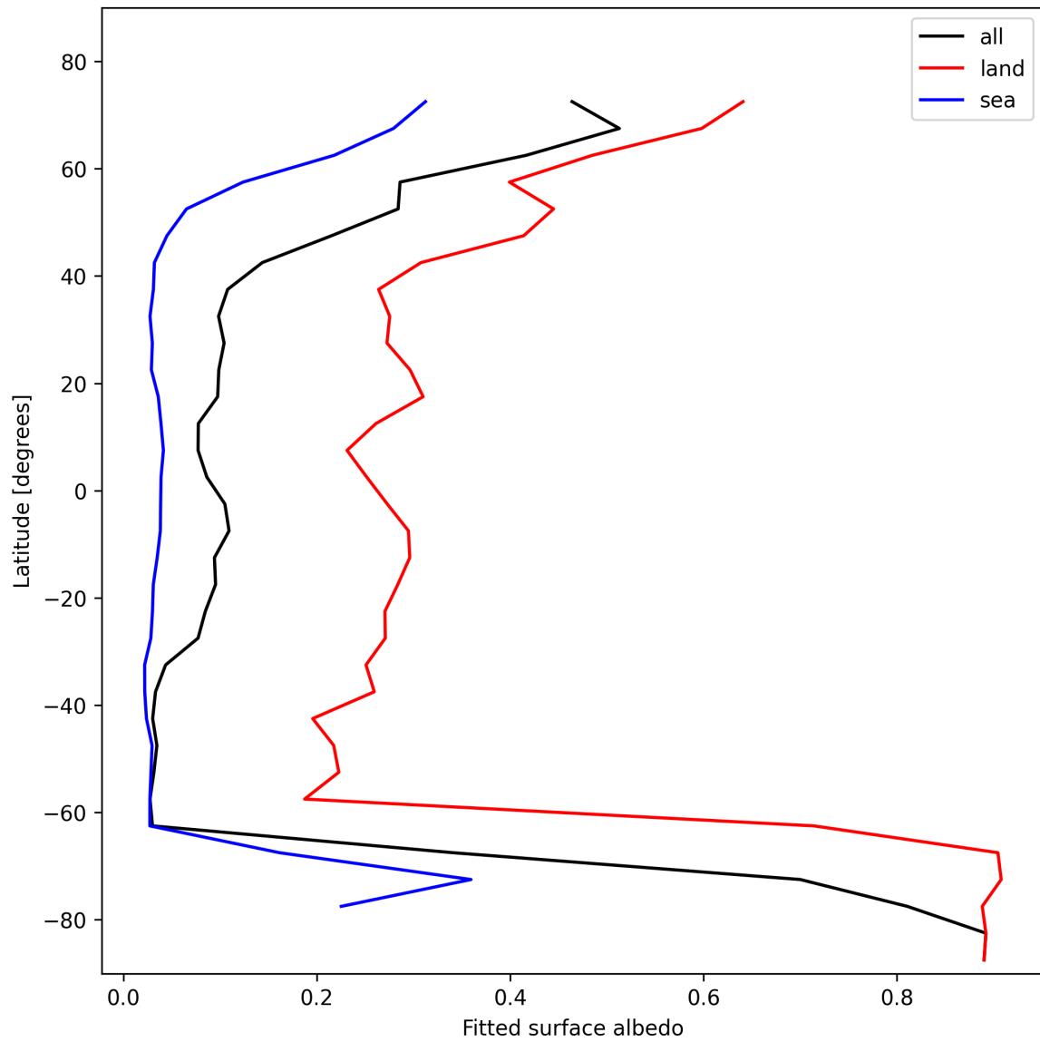
Figure 27: Zonal average of “Fitted surface albedo” for 2025-02-03 to 2025-02-04.
