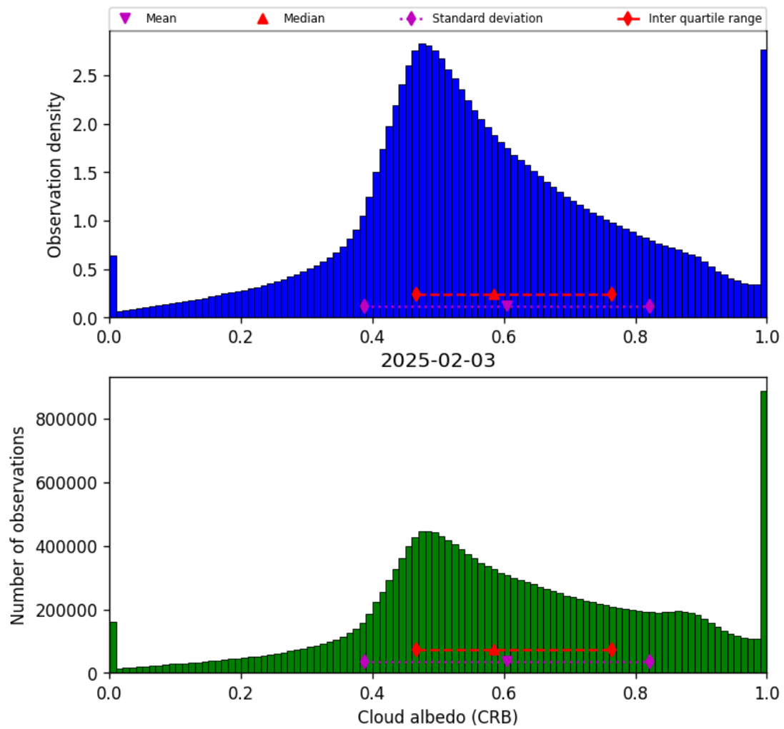
Figure 42: Histogram of “Cloud albedo (CRB)” for 2025-02-03 to 2025-02-04
