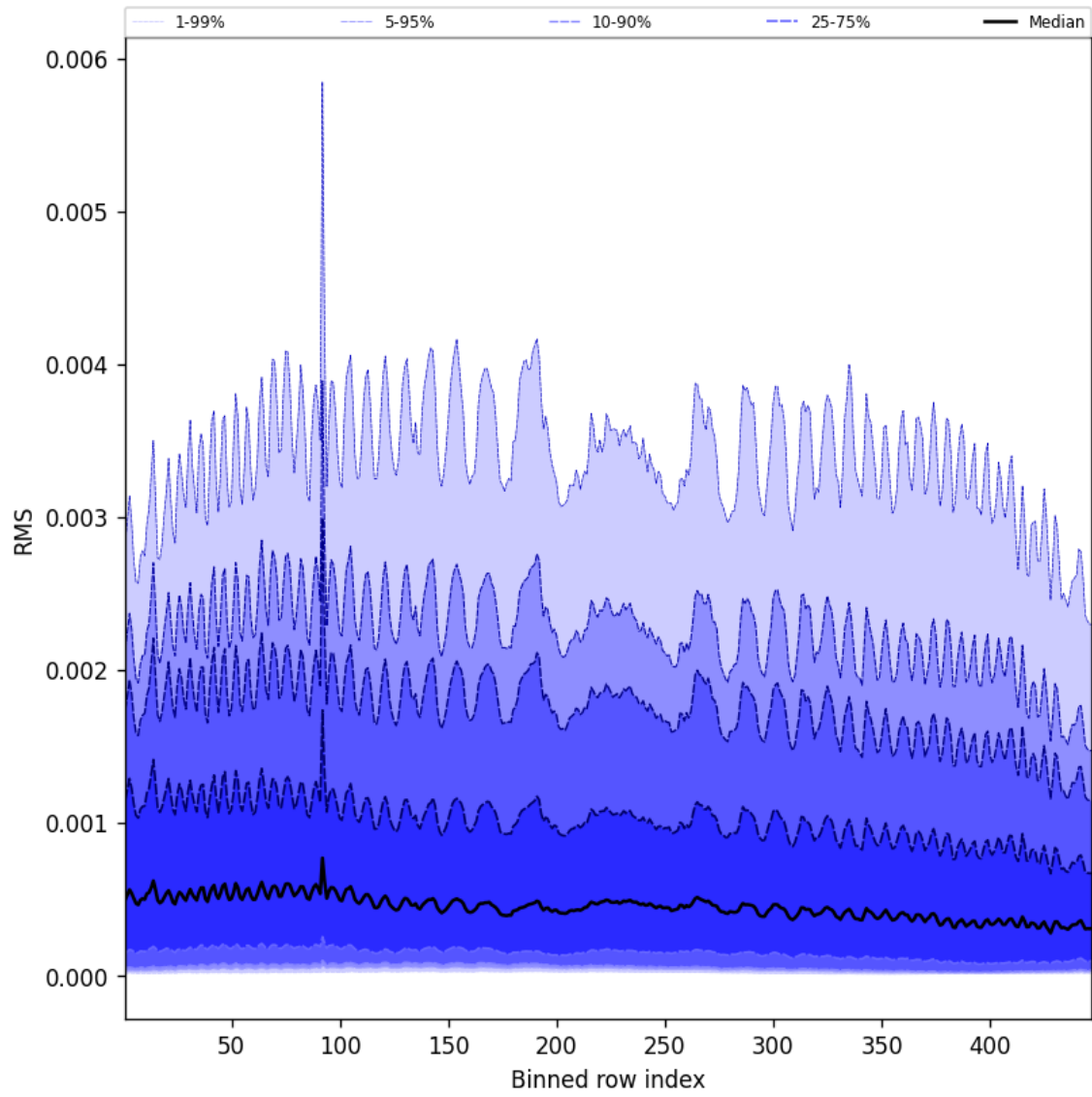
Figure 61: Along track statistics of “RMS” for 2025-02-03 to 2025-02-04
