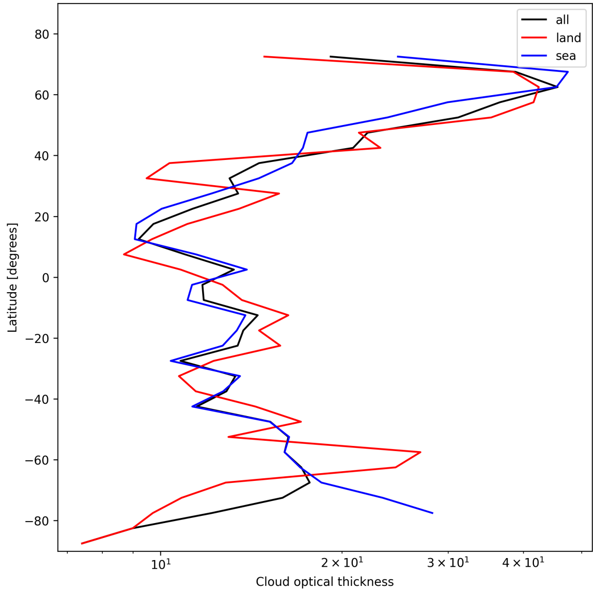
Figure 23: Zonal average of “Cloud optical thickness” for 2025-02-03 to 2025-02-04.
