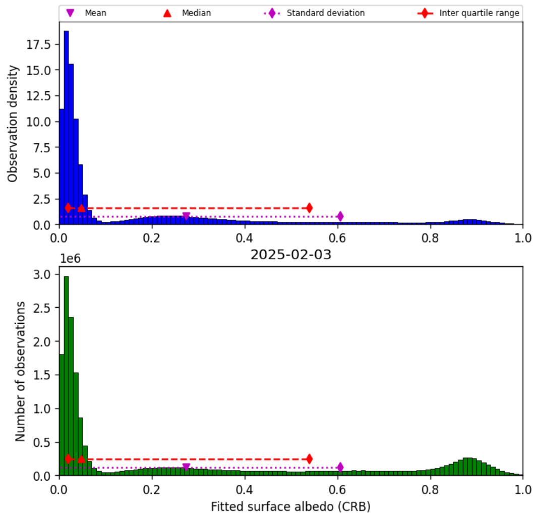
Figure 44: Histogram of “Fitted surface albedo (CRB)” for 2025-02-03 to 2025-02-04
