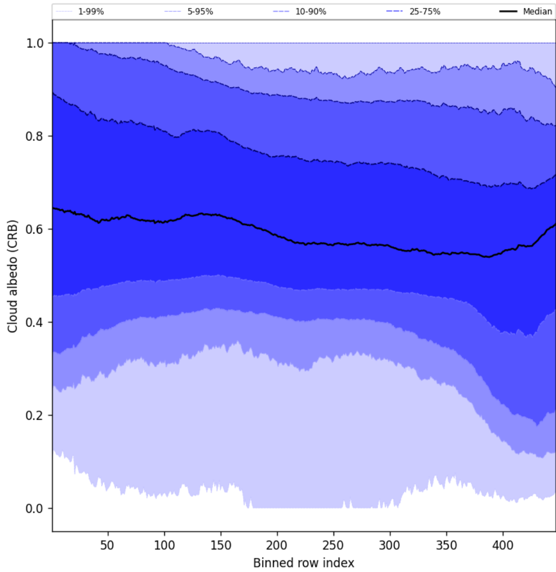
Figure 58: Along track statistics of “Cloud albedo (CRB)” for 2025-02-03 to 2025-02-04
