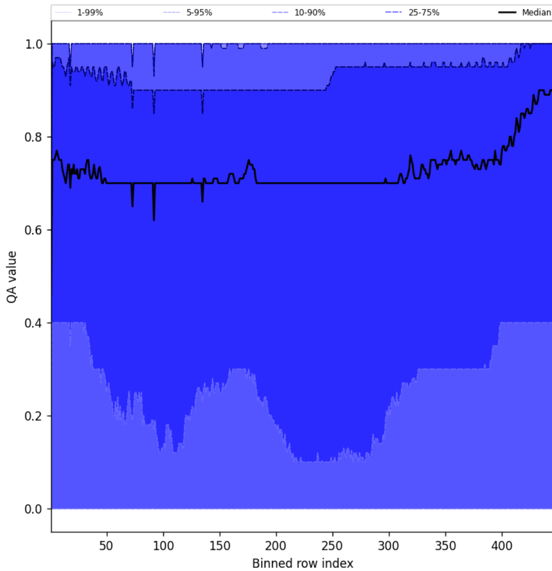
Figure 52: Along track statistics of “QA value” for 2025-02-03 to 2025-02-04
