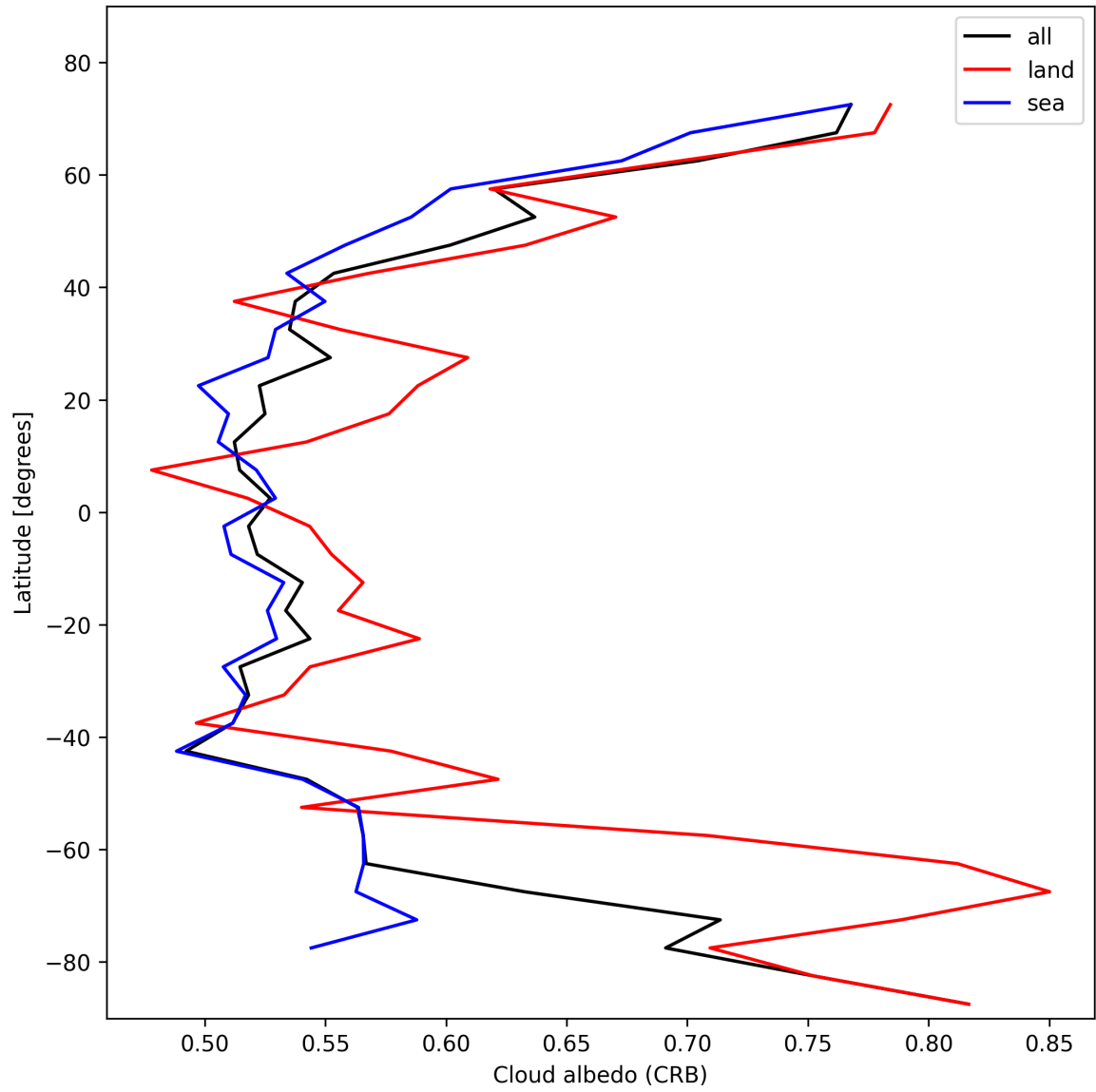
Figure 26: Zonal average of “Cloud albedo (CRB)” for 2025-02-03 to 2025-02-04.
