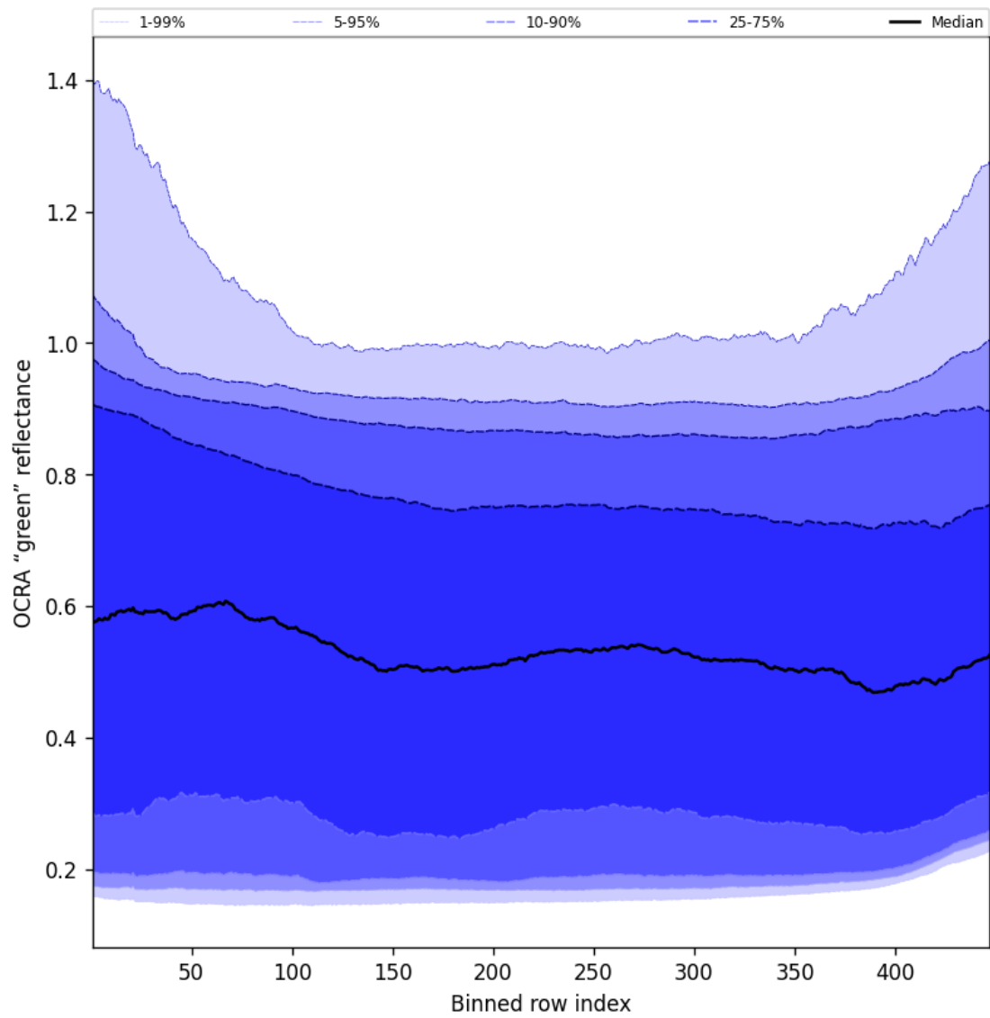
Figure 66: Along track statistics of “OCRA “green” reflectance” for 2025-02-03 to 2025-02-04
