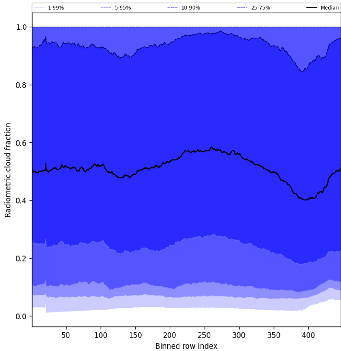
Figure 53: Along track statistics of “Radiometric cloud fraction” for 2025-02-03 to 2025-02-04
