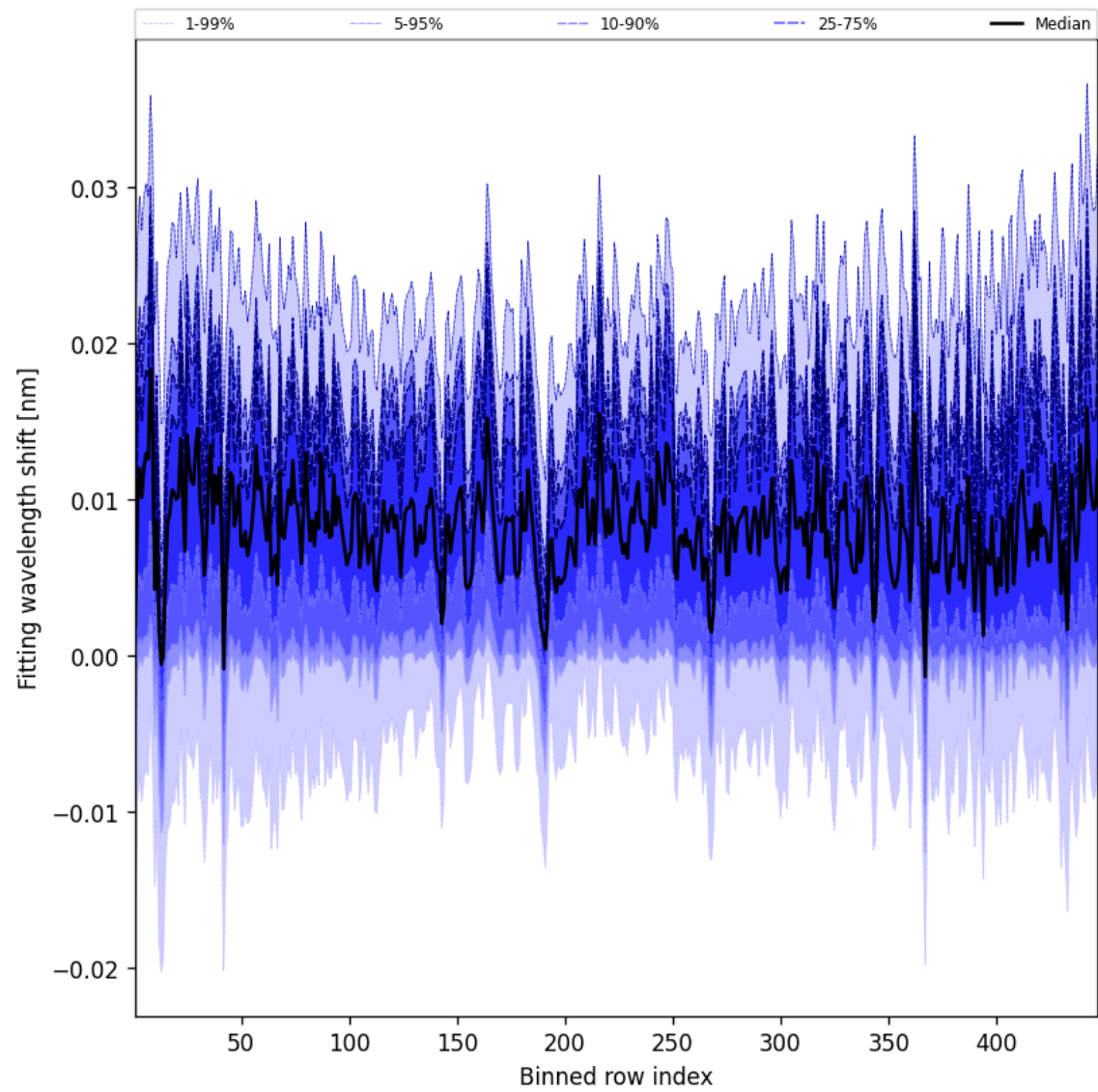
Figure 63: Along track statistics of “Fitting wavelength shift” for 2025-02-03 to 2025-02-04
