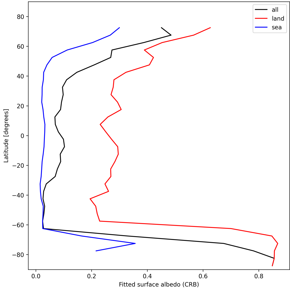
Figure 28: Zonal average of “Fitted surface albedo (CRB)” for 2025-02-03 to 2025-02-04.
