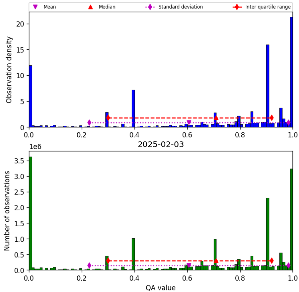
Figure 36: Histogram of “QA value” for 2025-02-03 to 2025-02-04
