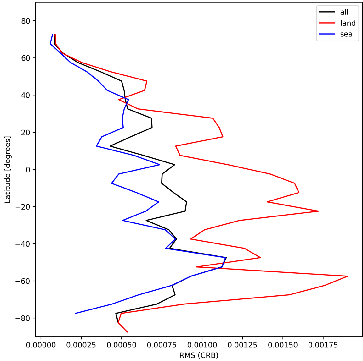
Figure 30: Zonal average of “RMS (CRB)” for 2025-02-03 to 2025-02-04.
