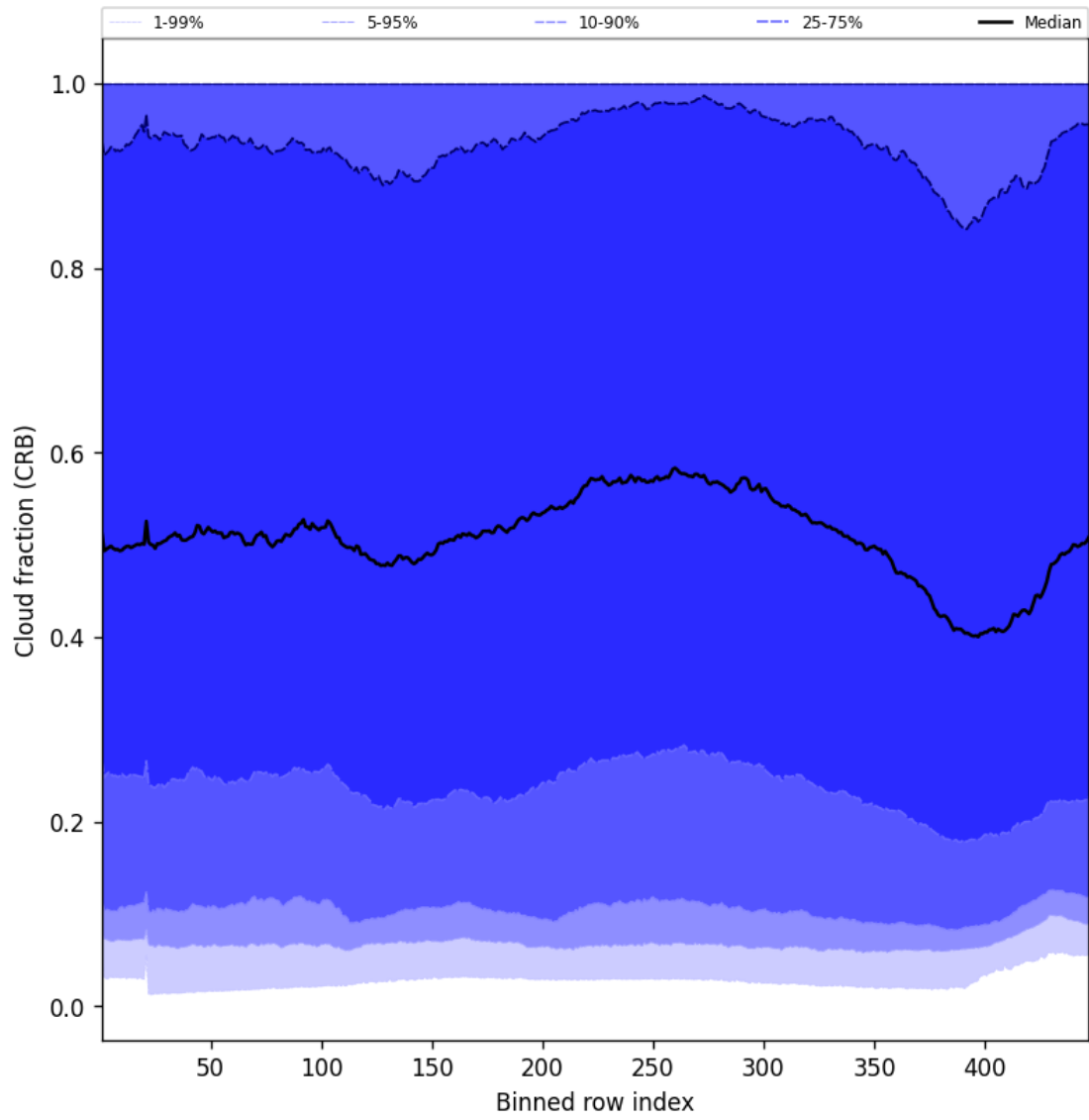
Figure 56: Along track statistics of “Cloud fraction (CRB)” for 2025-02-03 to 2025-02-04
