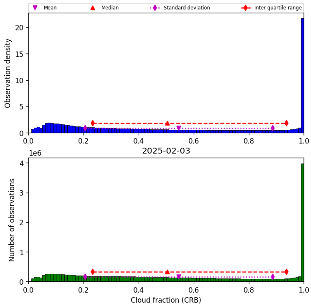
Figure 40: Histogram of “Cloud fraction (CRB)” for 2025-02-03 to 2025-02-04
