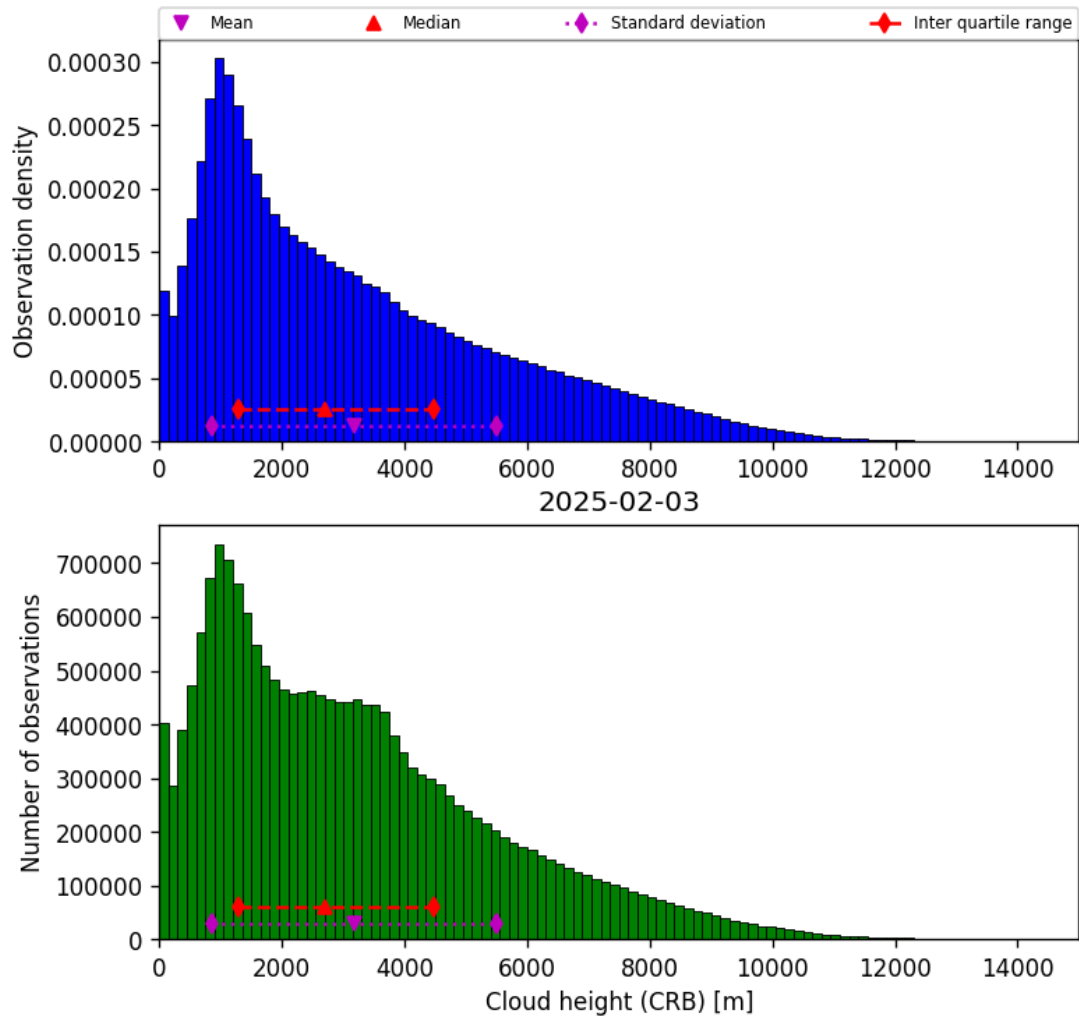
Figure 41: Histogram of “Cloud height (CRB)” for 2025-02-03 to 2025-02-04
