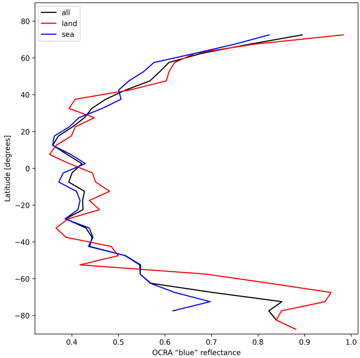
Figure 33: Zonal average of “OCRA “blue” reflectance” for 2025-02-03 to 2025-02-04.
