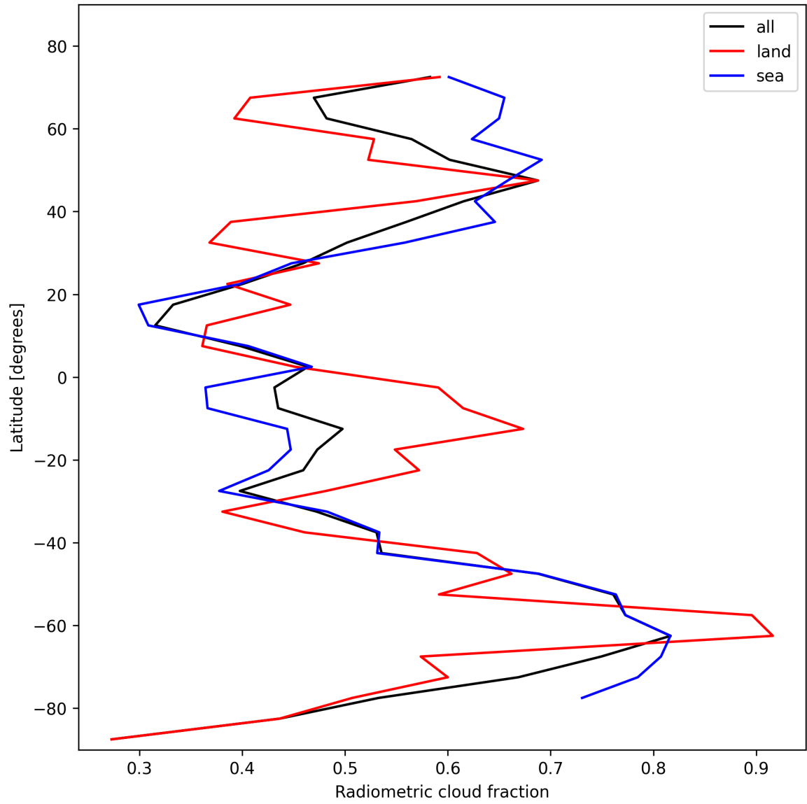
Figure 21: Zonal average of “Radiometric cloud fraction” for 2025-02-03 to 2025-02-04.
