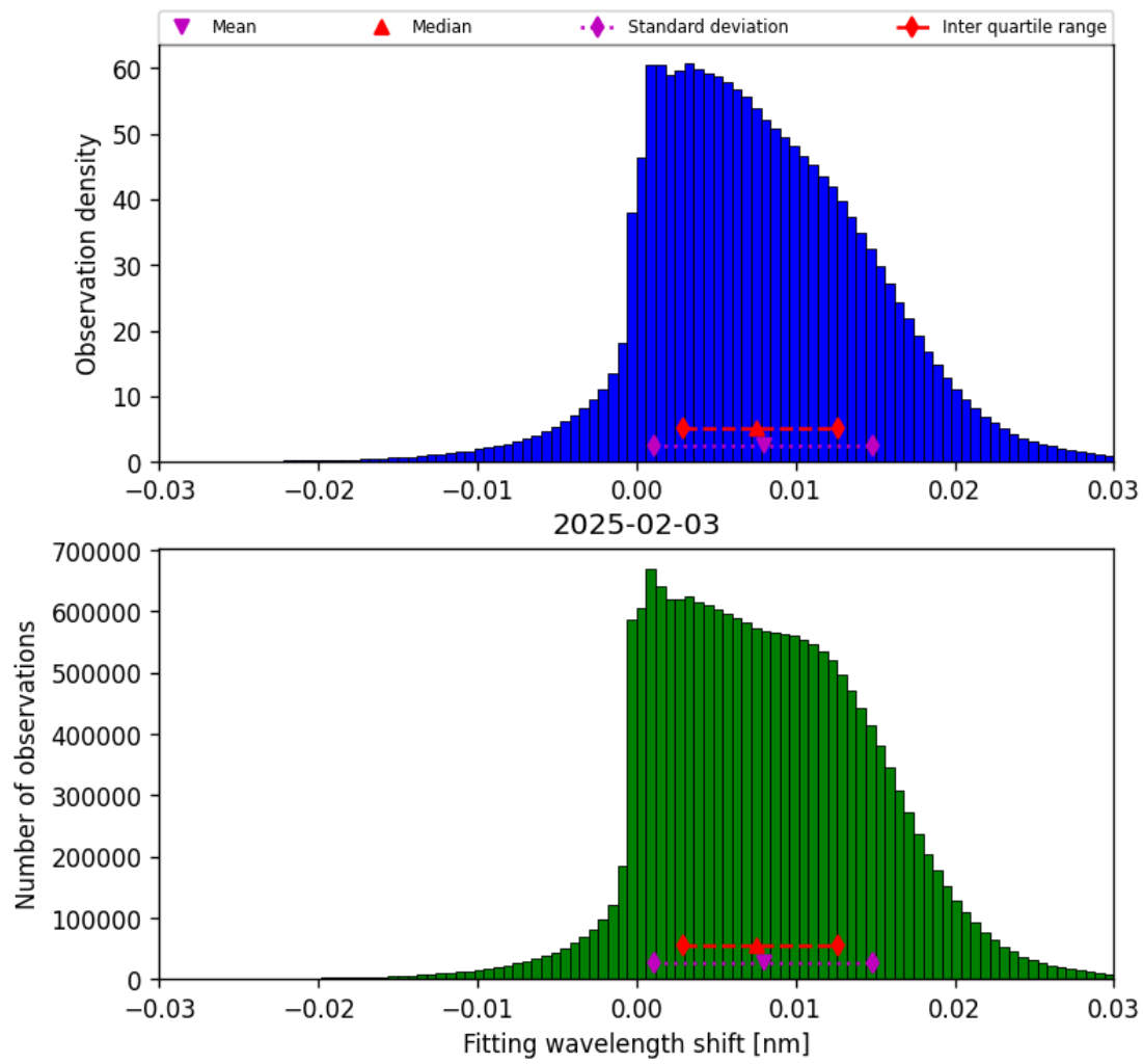
Figure 47: Histogram of “Fitting wavelength shift” for 2025-02-03 to 2025-02-04
