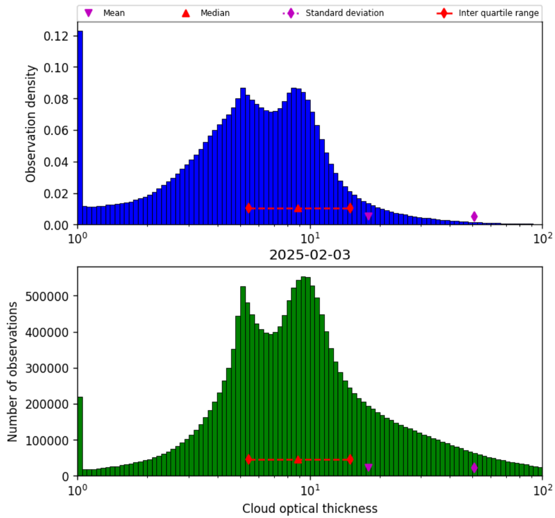
Figure 39: Histogram of “Cloud optical thickness” for 2025-02-03 to 2025-02-04
