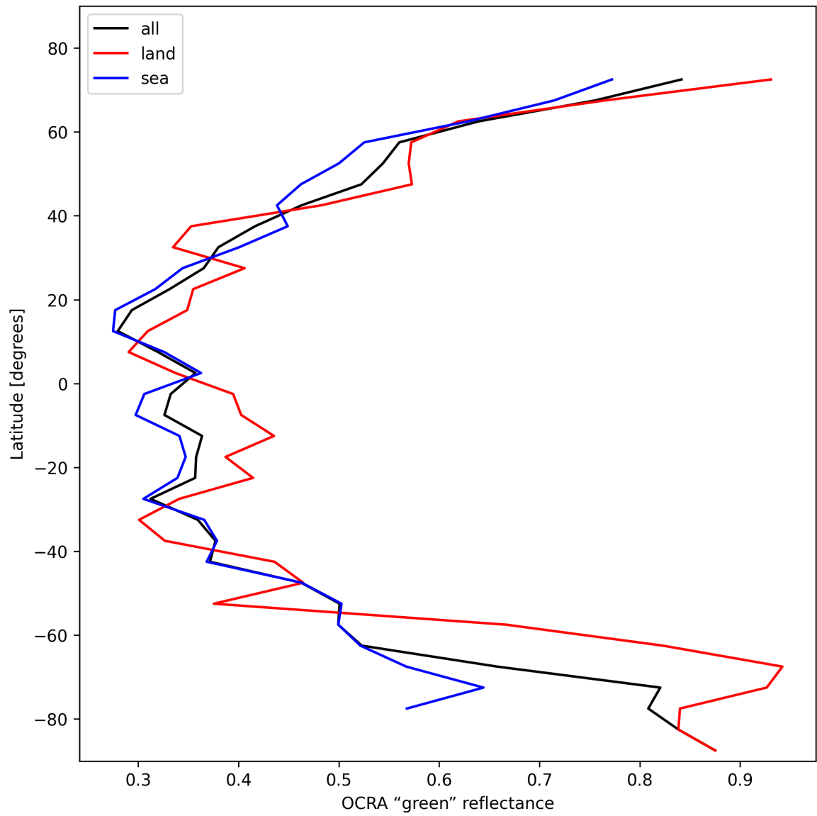
Figure 34: Zonal average of “OCRA “green” reflectance” for 2025-02-03 to 2025-02-04.
