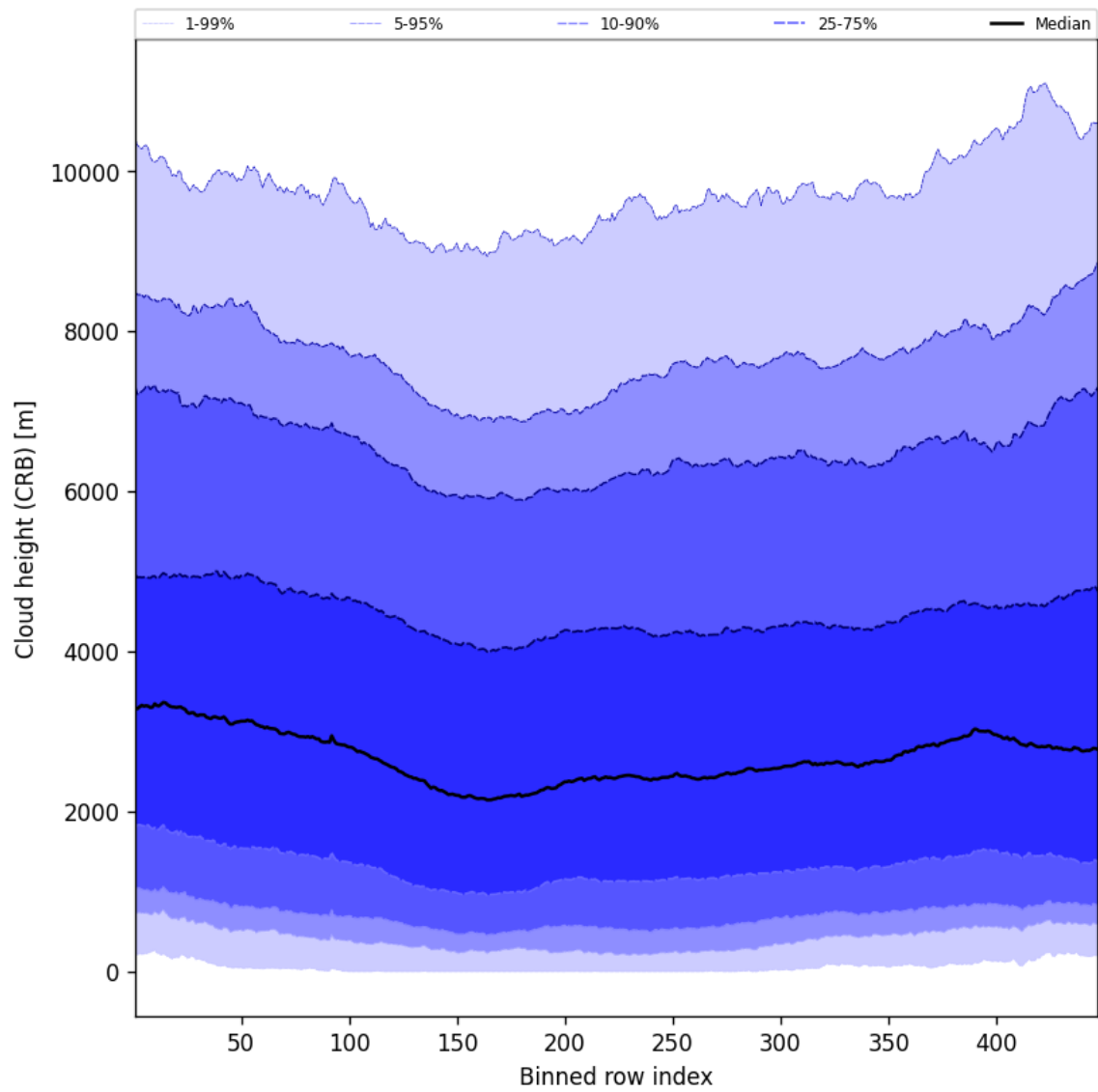
Figure 57: Along track statistics of “Cloud height (CRB)” for 2025-02-03 to 2025-02-04
