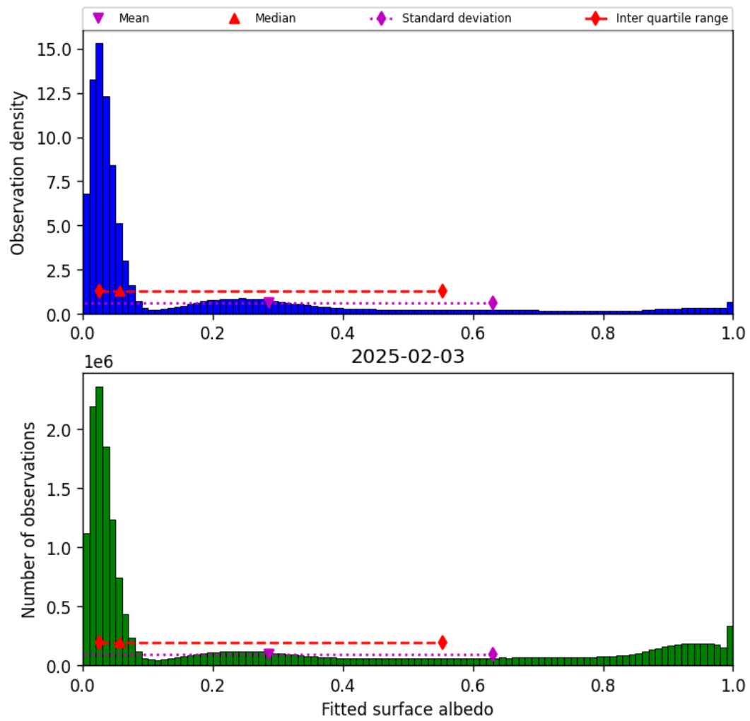
Figure 43: Histogram of “Fitted surface albedo” for 2025-02-03 to 2025-02-04
