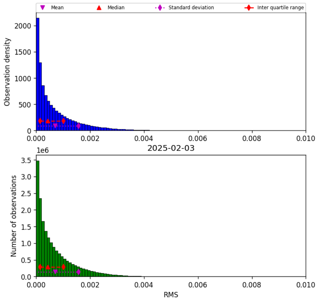
Figure 45: Histogram of “RMS” for 2025-02-03 to 2025-02-04
