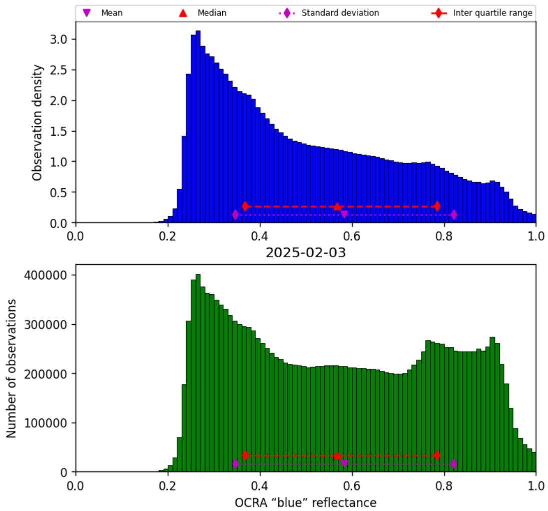
Figure 49: Histogram of “OCRA “blue” reflectance” for 2025-02-03 to 2025-02-04
