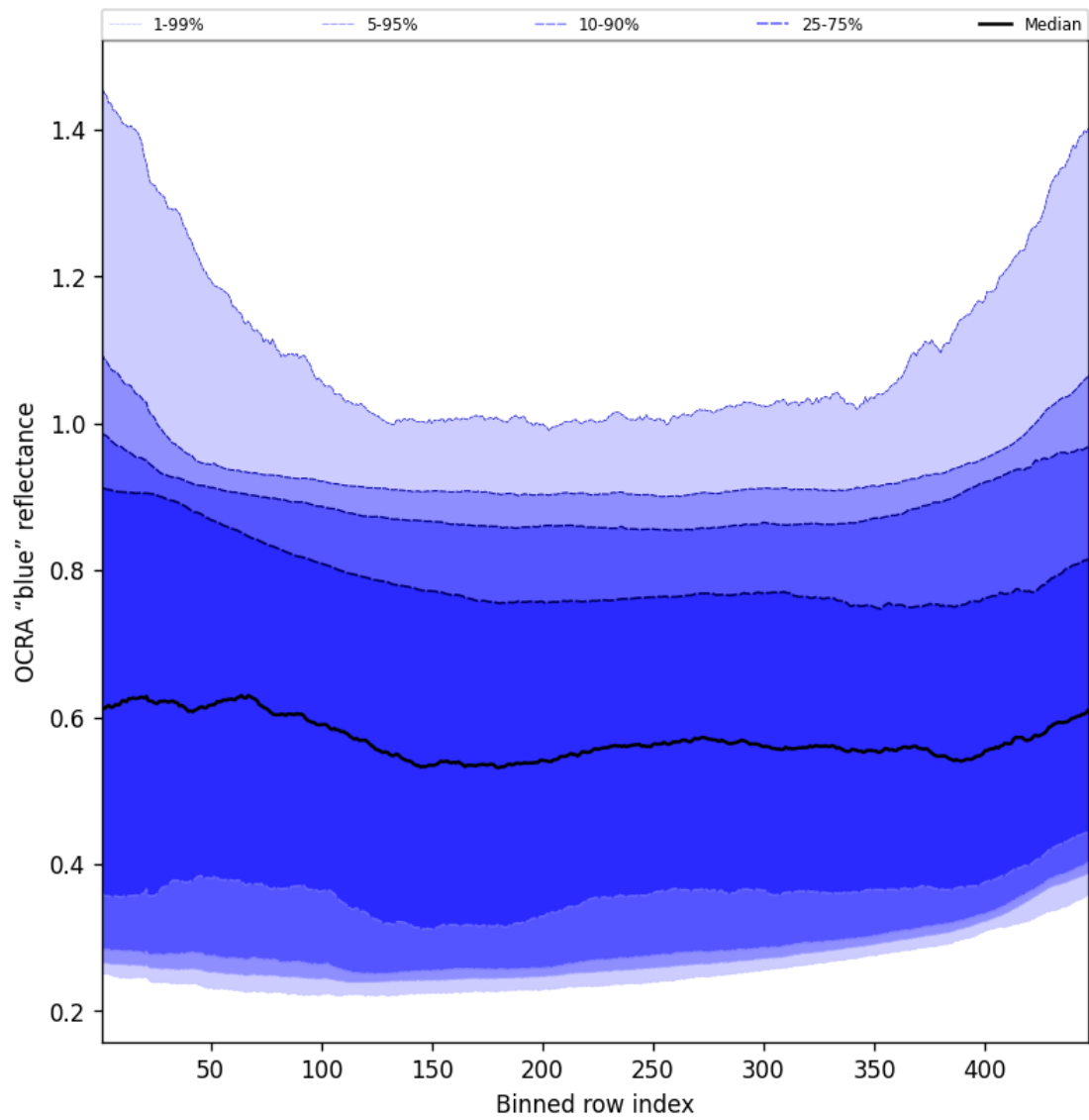
Figure 65: Along track statistics of “OCRA “blue” reflectance” for 2025-02-03 to 2025-02-04
