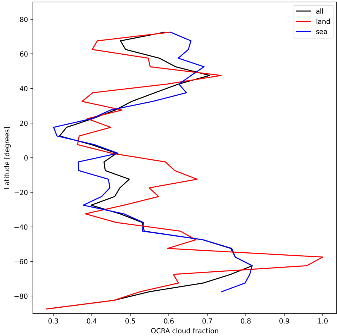
Figure 32: Zonal average of “OCRA cloud fraction” for 2025-02-03 to 2025-02-04.
