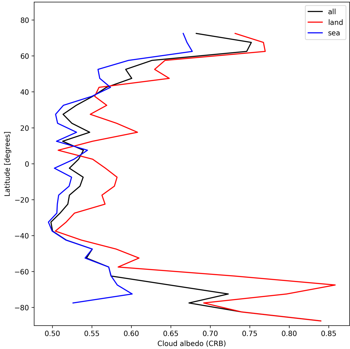
Figure 26: Zonal average of “Cloud albedo (CRB)” for 2025-02-04 to 2025-02-05.
