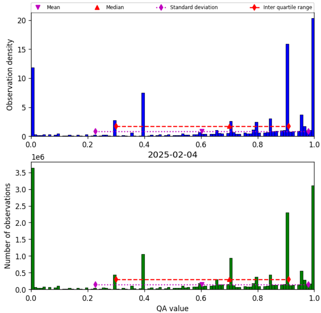
Figure 36: Histogram of “QA value” for 2025-02-04 to 2025-02-05
