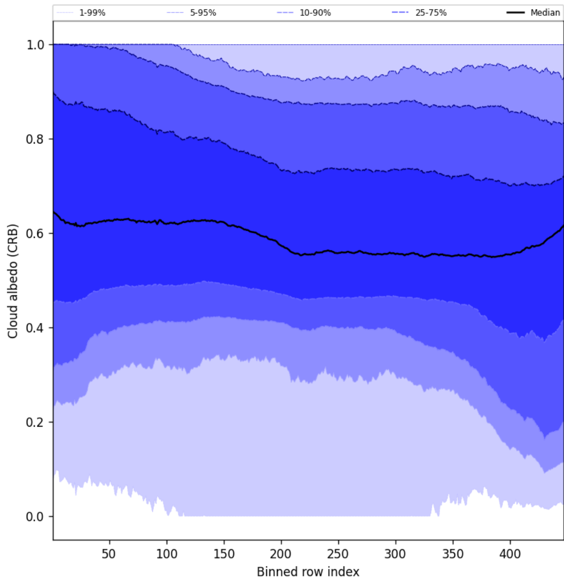
Figure 58: Along track statistics of “Cloud albedo (CRB)” for 2025-02-04 to 2025-02-05
