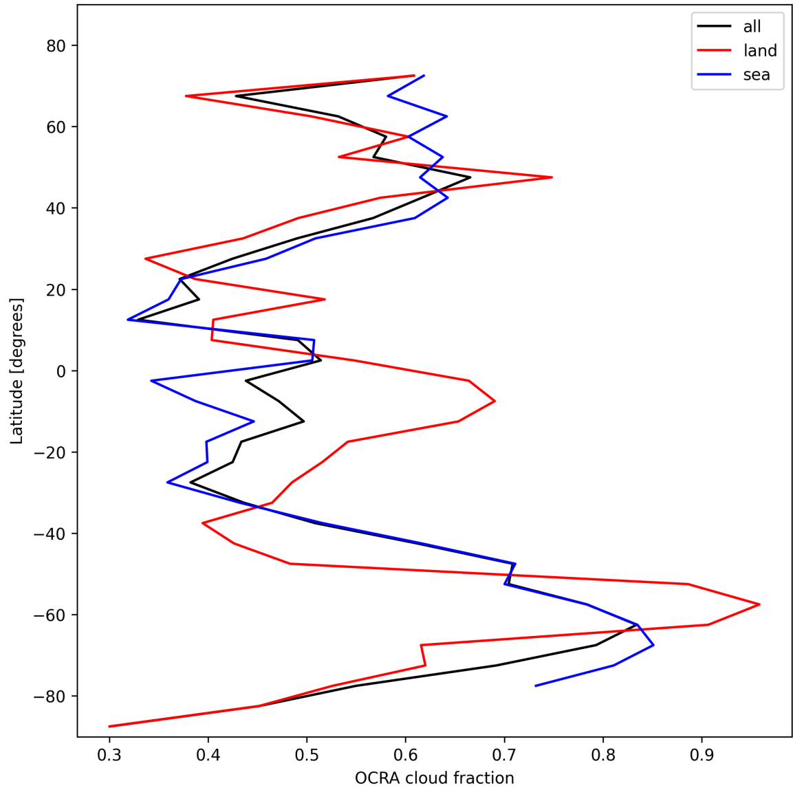
Figure 32: Zonal average of “OCRA cloud fraction” for 2025-02-04 to 2025-02-05.
