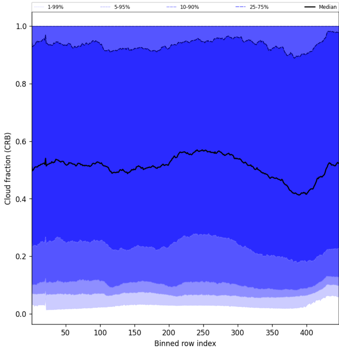
Figure 56: Along track statistics of “Cloud fraction (CRB)” for 2025-02-04 to 2025-02-05
