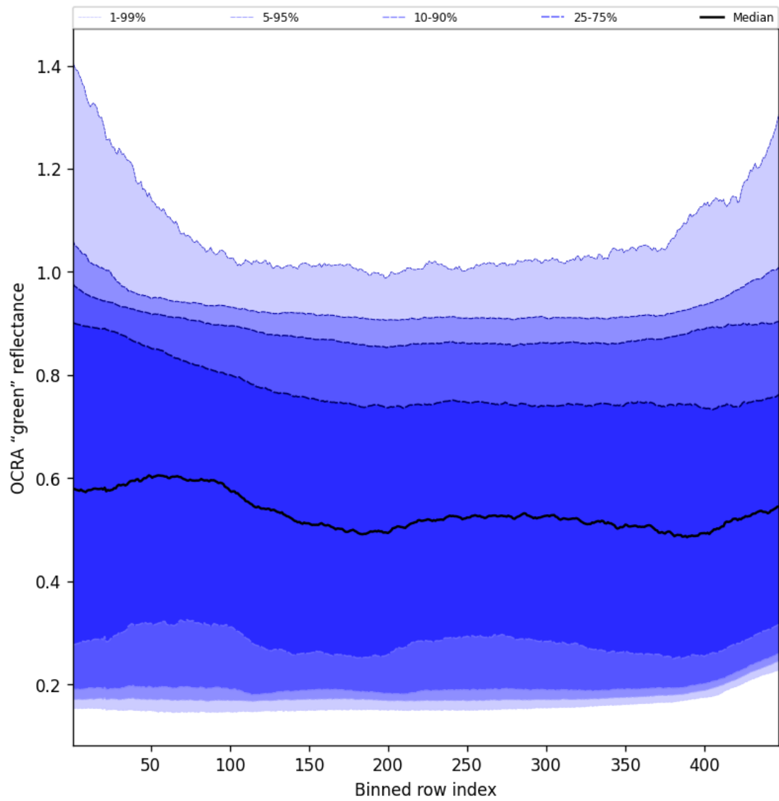
Figure 66: Along track statistics of “OCRA “green” reflectance” for 2025-02-04 to 2025-02-05
