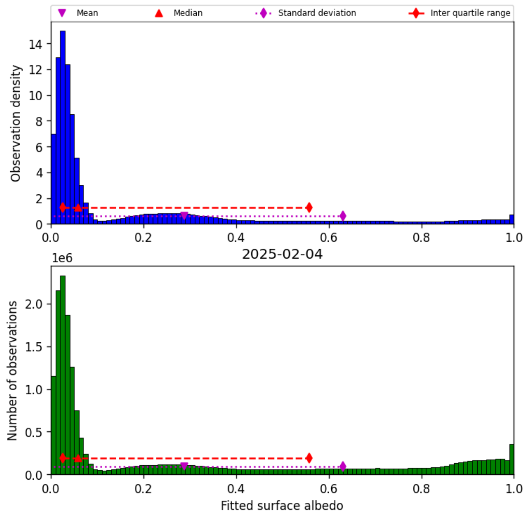
Figure 43: Histogram of “Fitted surface albedo” for 2025-02-04 to 2025-02-05
