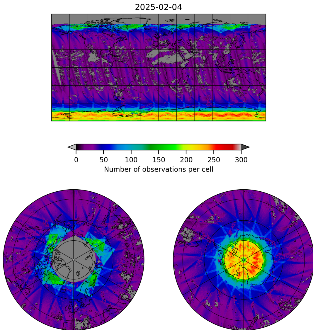
Figure 19: Map of the number of observations for 2025-02-04 to 2025-02-05
