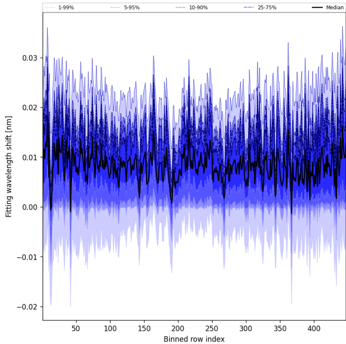
Figure 63: Along track statistics of “Fitting wavelength shift” for 2025-02-04 to 2025-02-05
