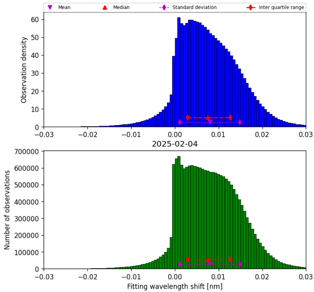
Figure 47: Histogram of “Fitting wavelength shift” for 2025-02-04 to 2025-02-05
