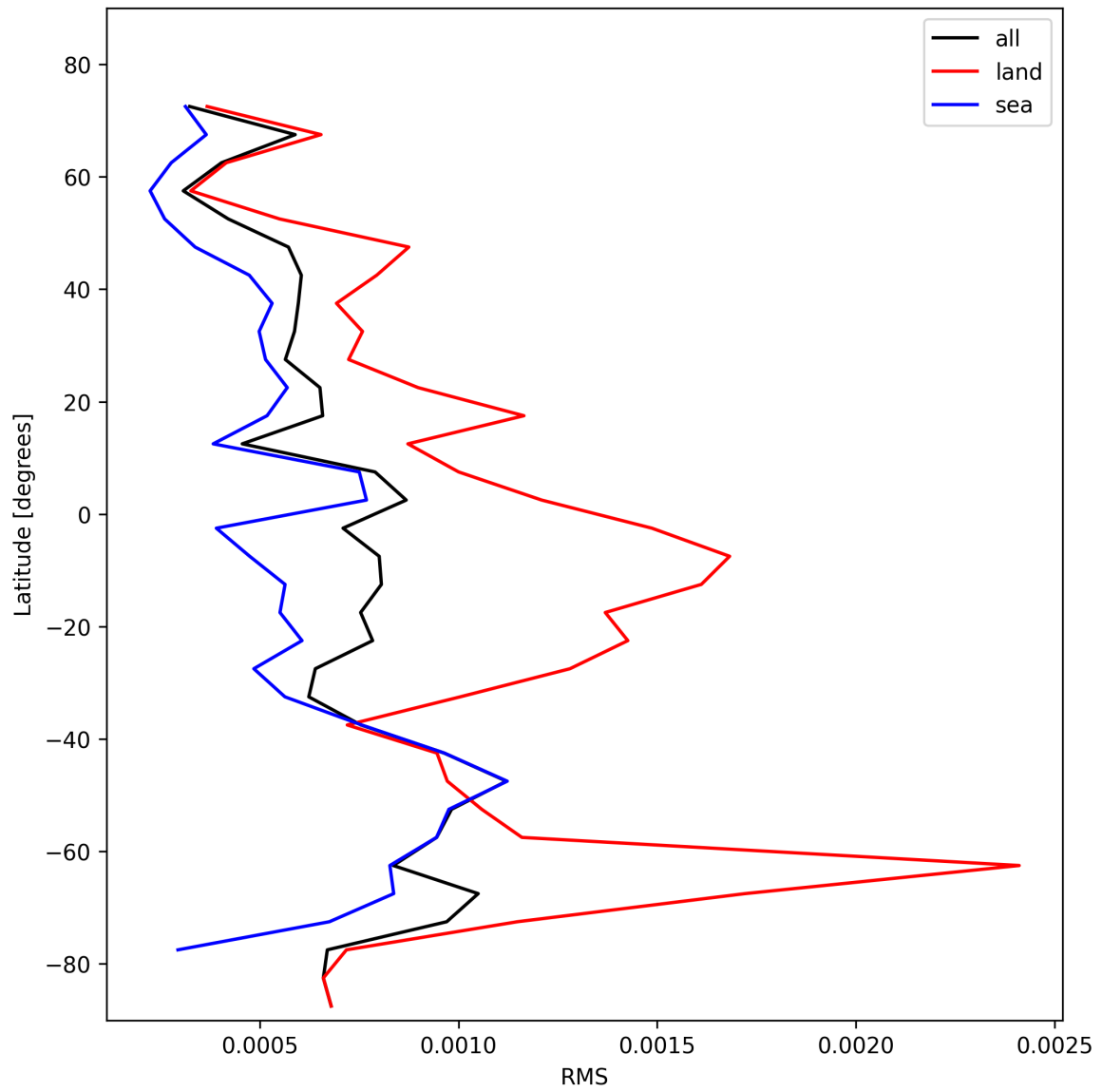
Figure 29: Zonal average of “RMS” for 2025-02-04 to 2025-02-05.
