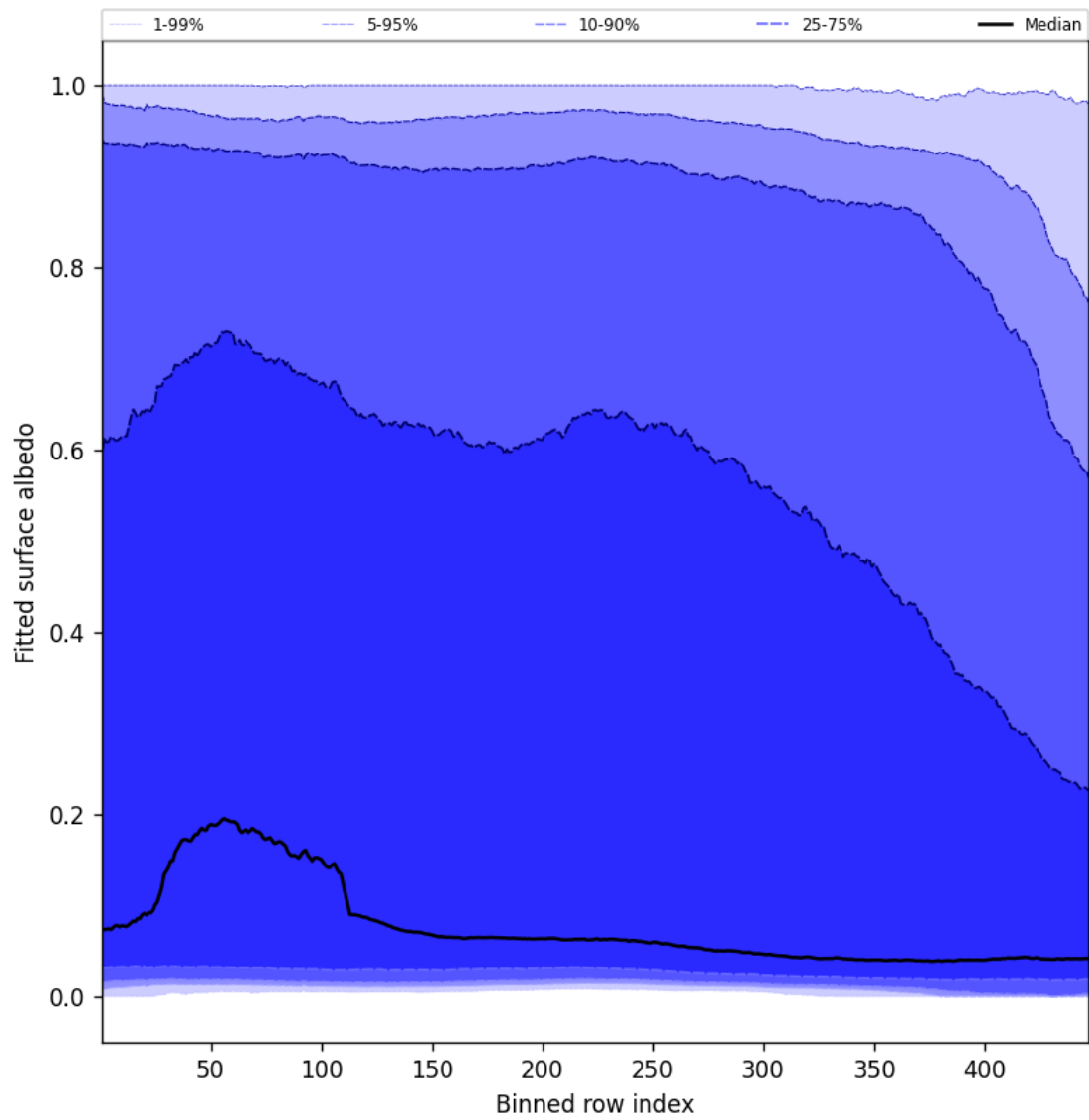
Figure 59: Along track statistics of “Fitted surface albedo” for 2025-02-04 to 2025-02-05
