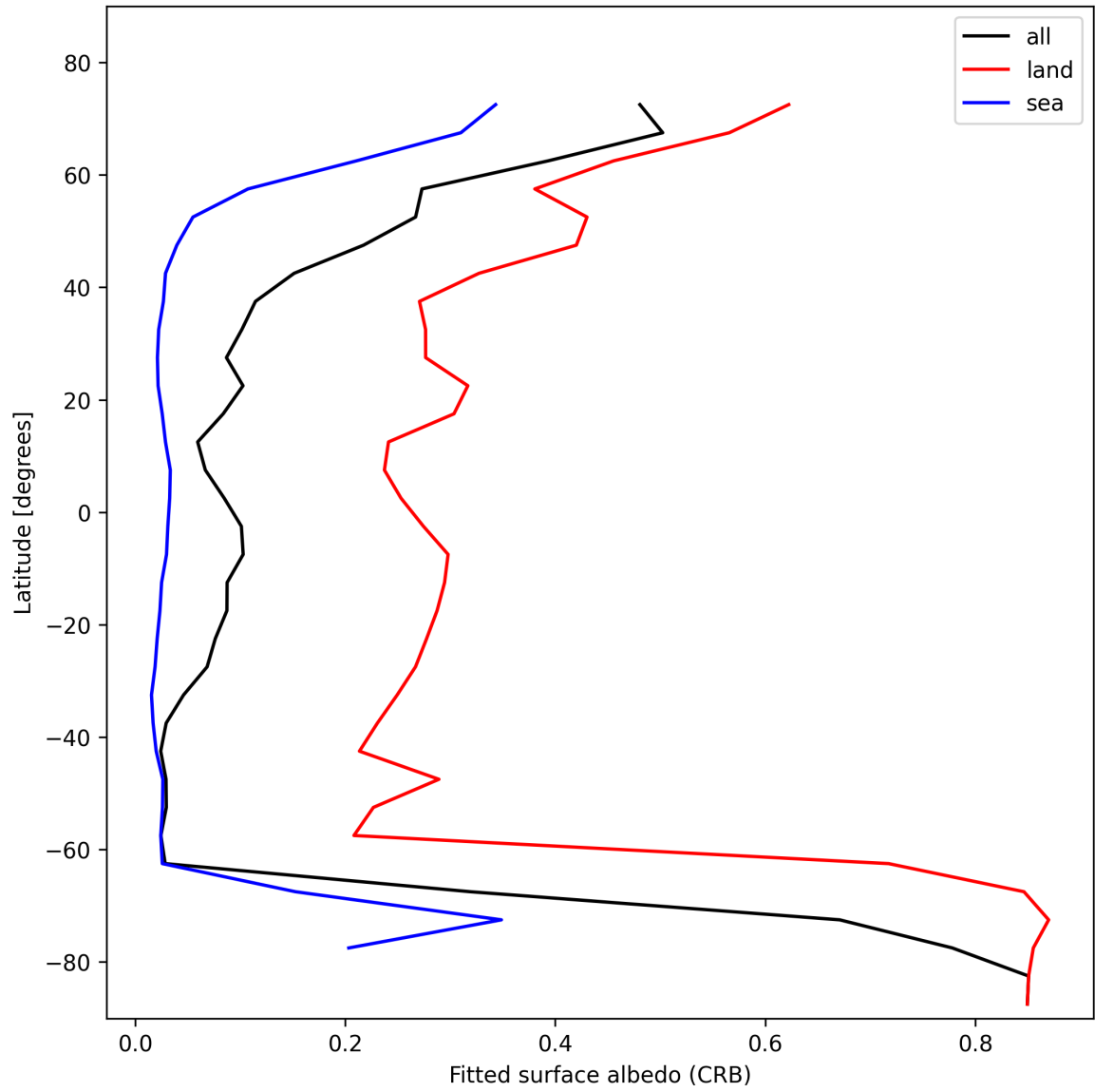
Figure 28: Zonal average of “Fitted surface albedo (CRB)” for 2025-02-04 to 2025-02-05.
