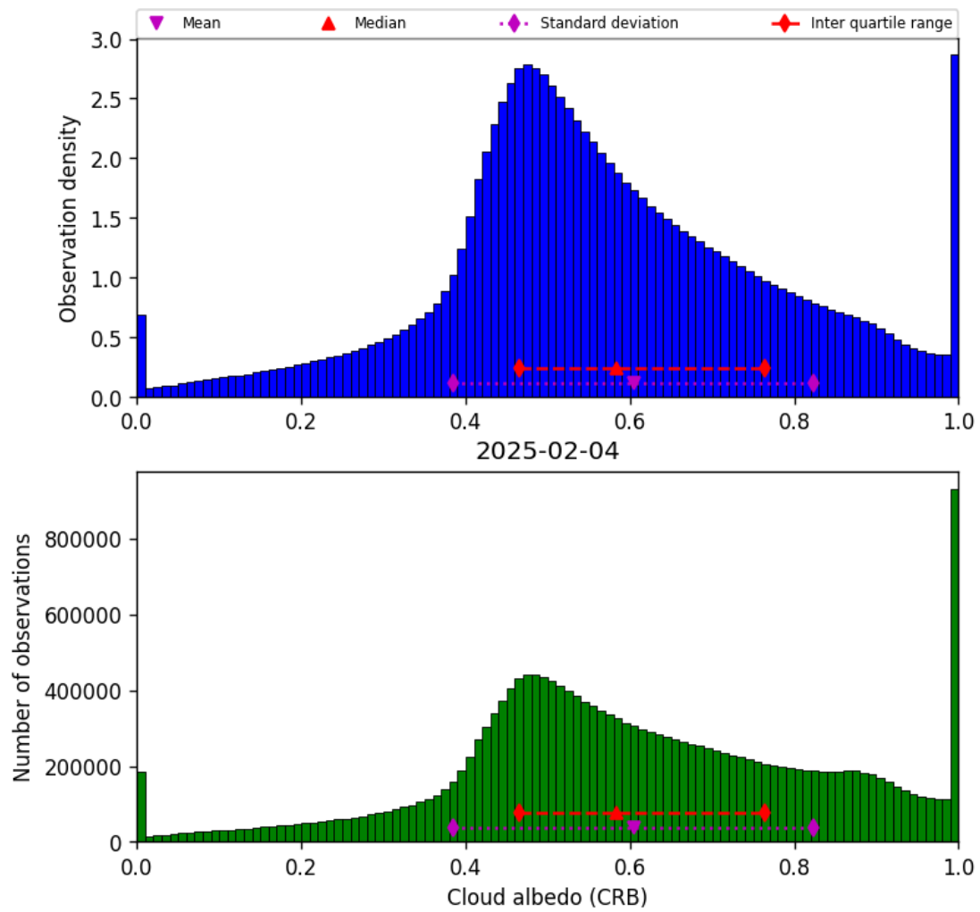
Figure 42: Histogram of “Cloud albedo (CRB)” for 2025-02-04 to 2025-02-05
