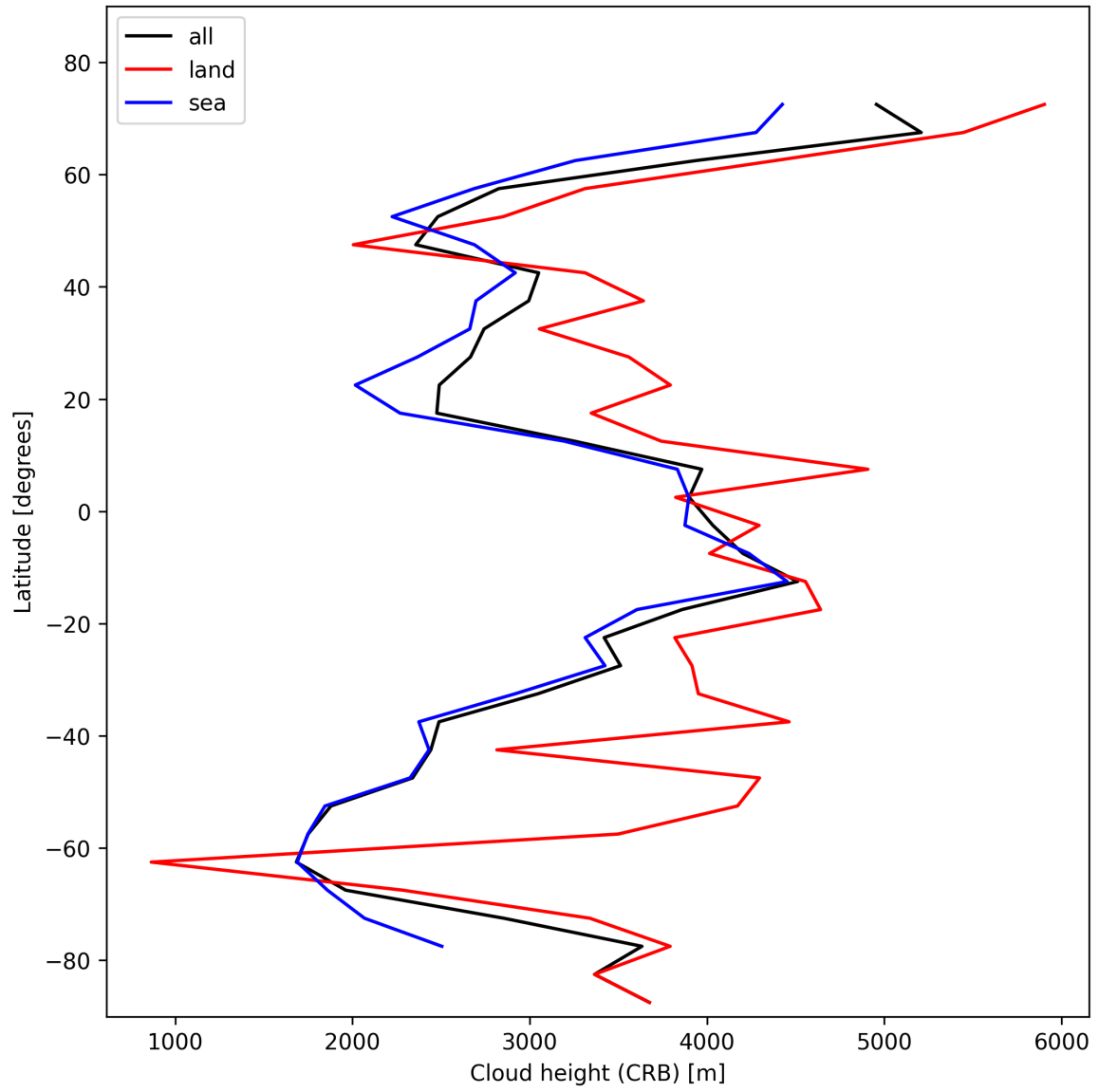
Figure 25: Zonal average of “Cloud height (CRB)” for 2025-02-04 to 2025-02-05.
