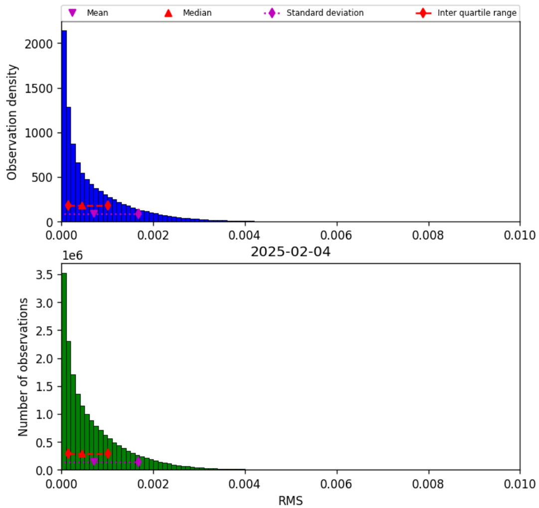
Figure 45: Histogram of “RMS” for 2025-02-04 to 2025-02-05
