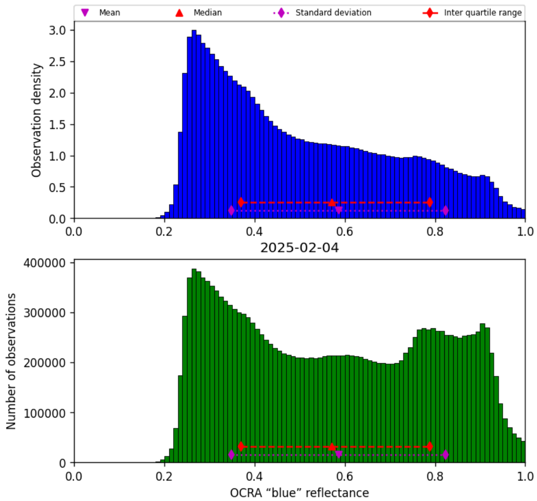
Figure 49: Histogram of “OCRA “blue” reflectance” for 2025-02-04 to 2025-02-05
