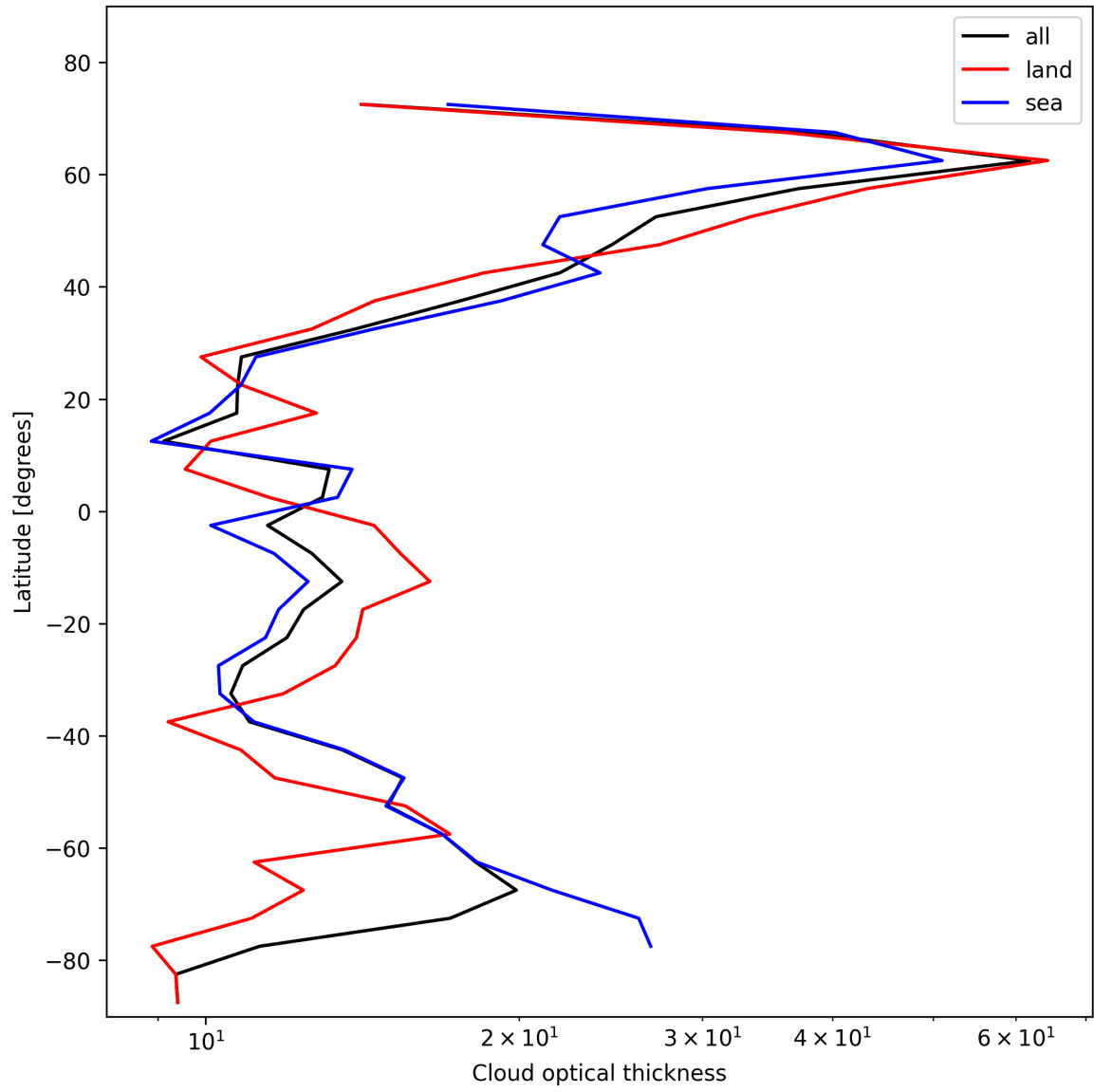
Figure 23: Zonal average of “Cloud optical thickness” for 2025-02-04 to 2025-02-05.
