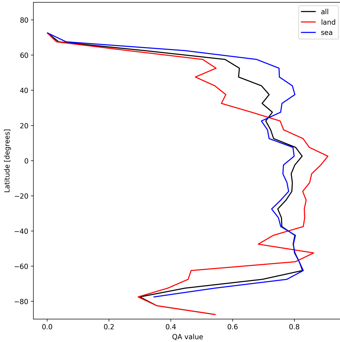
Figure 20: Zonal average of “QA value” for 2025-02-04 to 2025-02-05.
