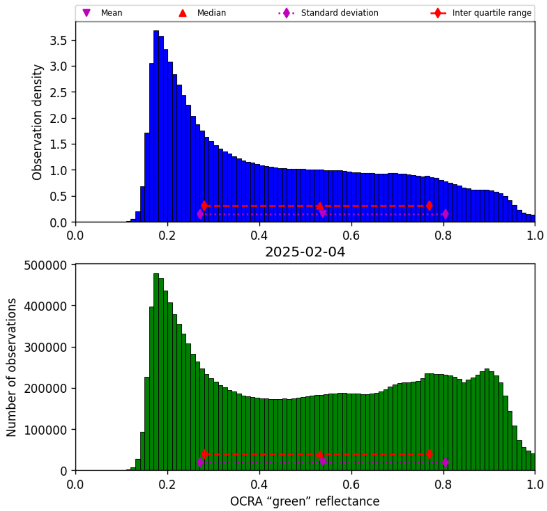
Figure 50: Histogram of “OCRA “green” reflectance” for 2025-02-04 to 2025-02-05
