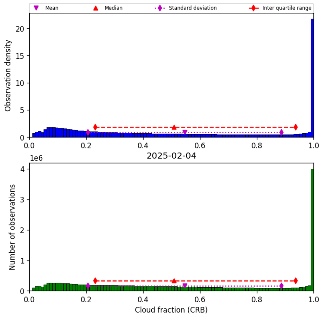
Figure 40: Histogram of “Cloud fraction (CRB)” for 2025-02-04 to 2025-02-05
