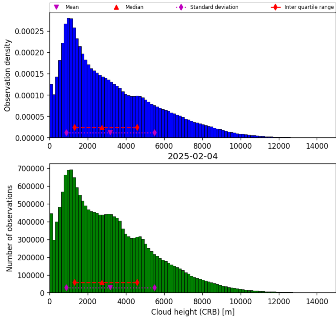
Figure 41: Histogram of “Cloud height (CRB)” for 2025-02-04 to 2025-02-05
