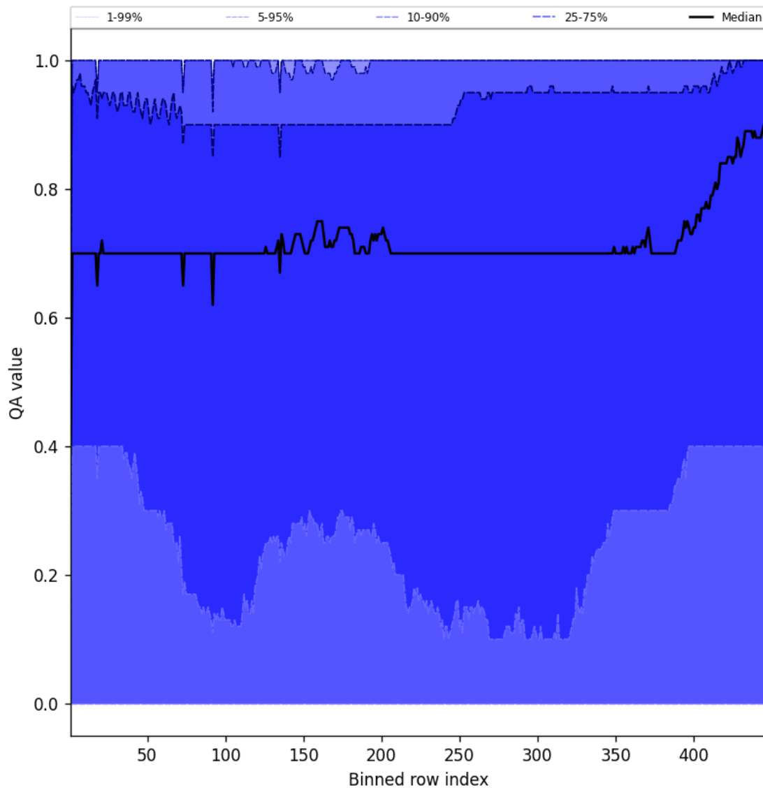
Figure 52: Along track statistics of “QA value” for 2025-02-04 to 2025-02-05
