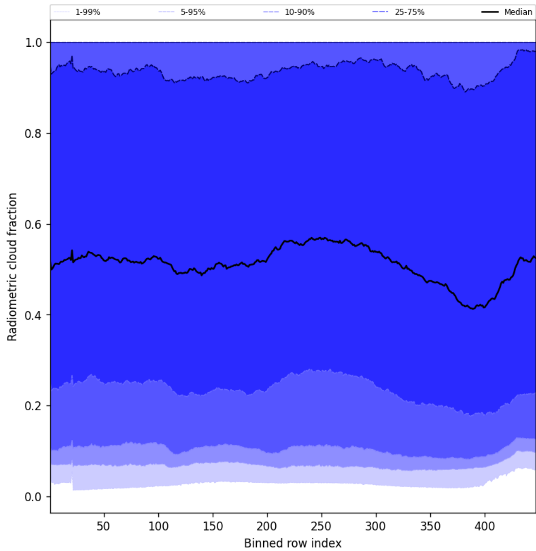
Figure 53: Along track statistics of “Radiometric cloud fraction” for 2025-02-04 to 2025-02-05
