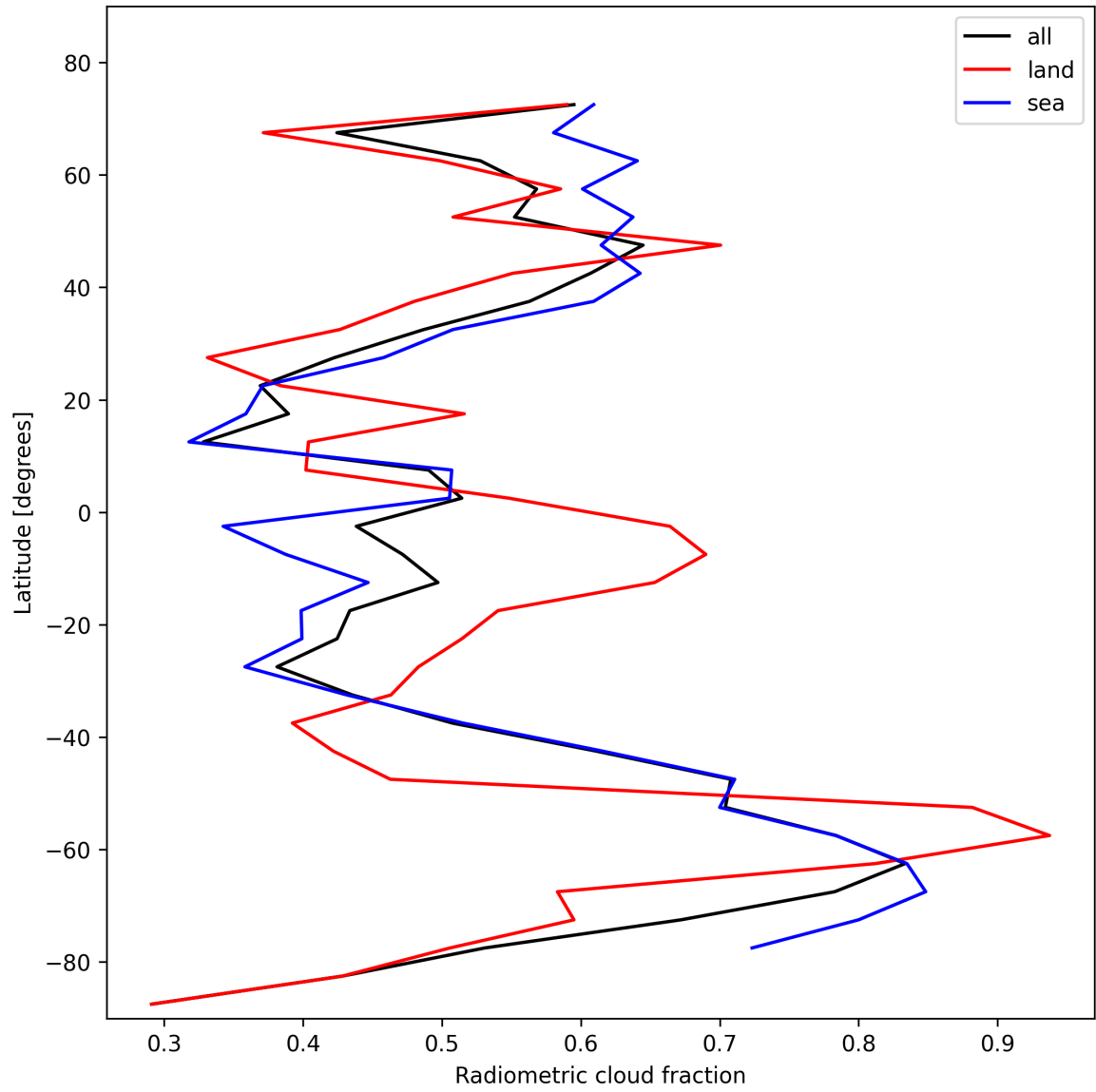
Figure 21: Zonal average of “Radiometric cloud fraction” for 2025-02-04 to 2025-02-05.
