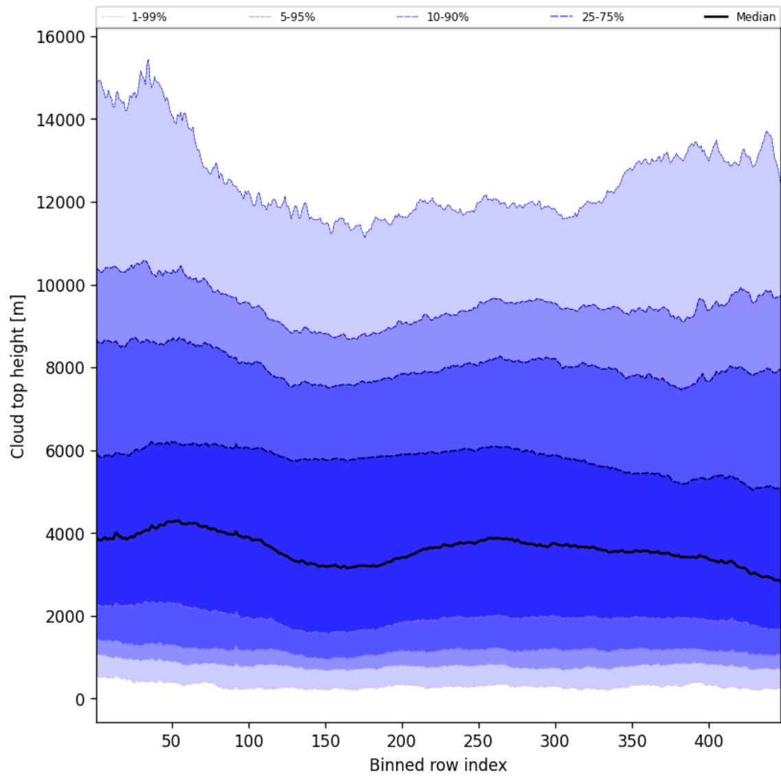
Figure 54: Along track statistics of “Cloud top height” for 2025-02-04 to 2025-02-05
