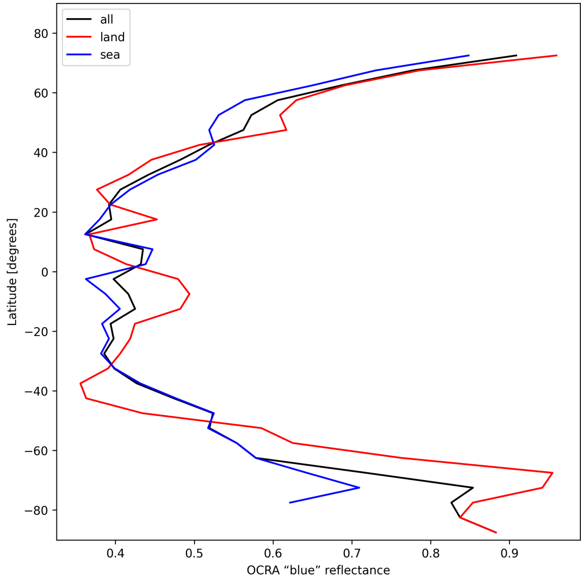
Figure 33: Zonal average of “OCRA “blue” reflectance” for 2025-02-04 to 2025-02-05.
