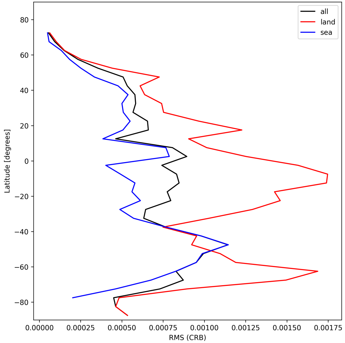
Figure 30: Zonal average of “RMS (CRB)” for 2025-02-04 to 2025-02-05.
