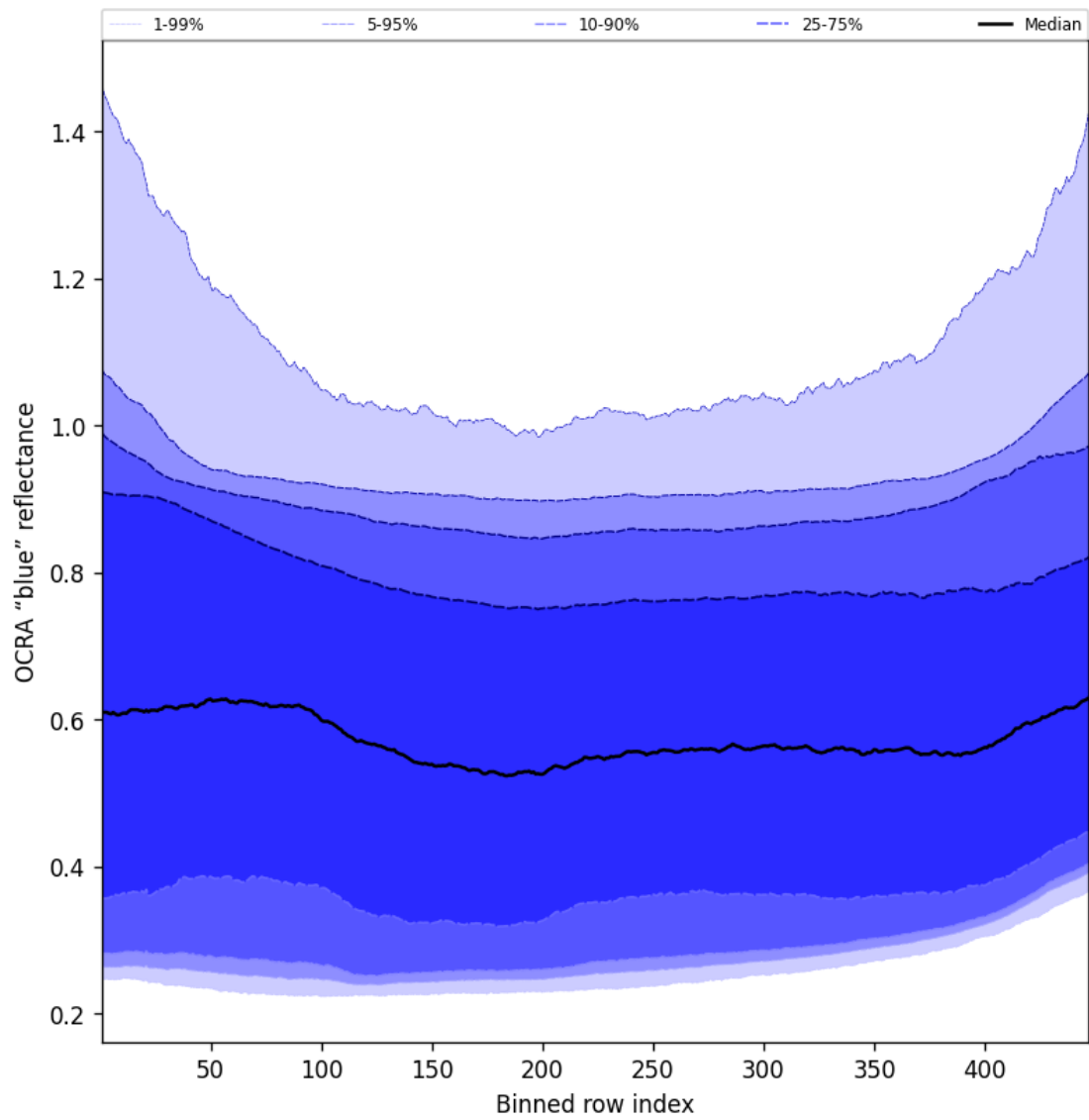
Figure 65: Along track statistics of "OCRA "blue" reflectance" for 2025-02-04 to 2025-02-05
