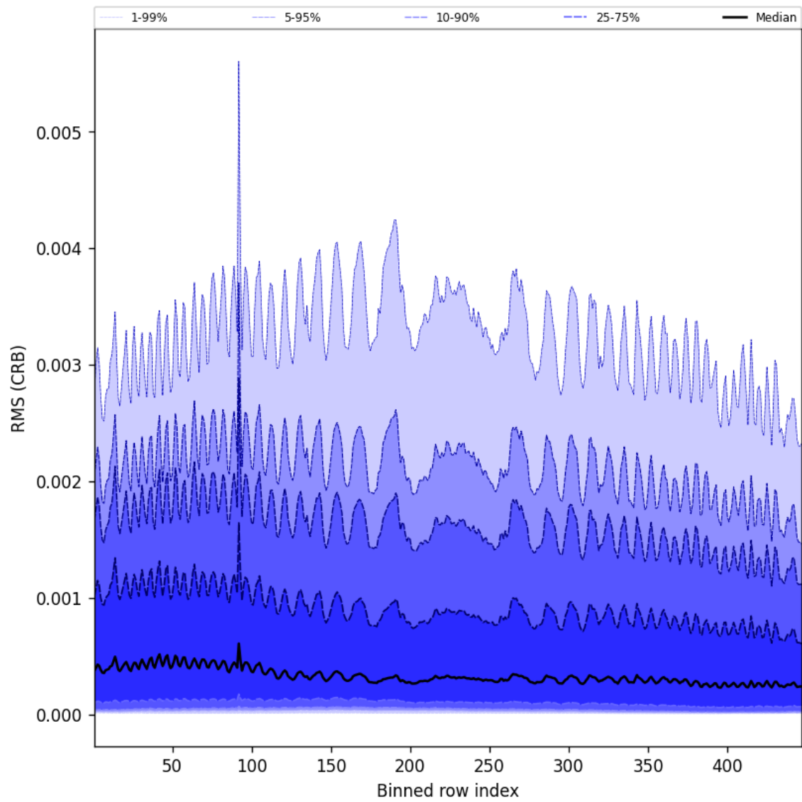
Figure 62: Along track statistics of “RMS (CRB)” for 2025-02-04 to 2025-02-05
