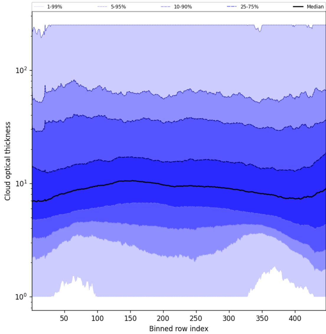
Figure 55: Along track statistics of “Cloud optical thickness” for 2025-02-04 to 2025-02-05
