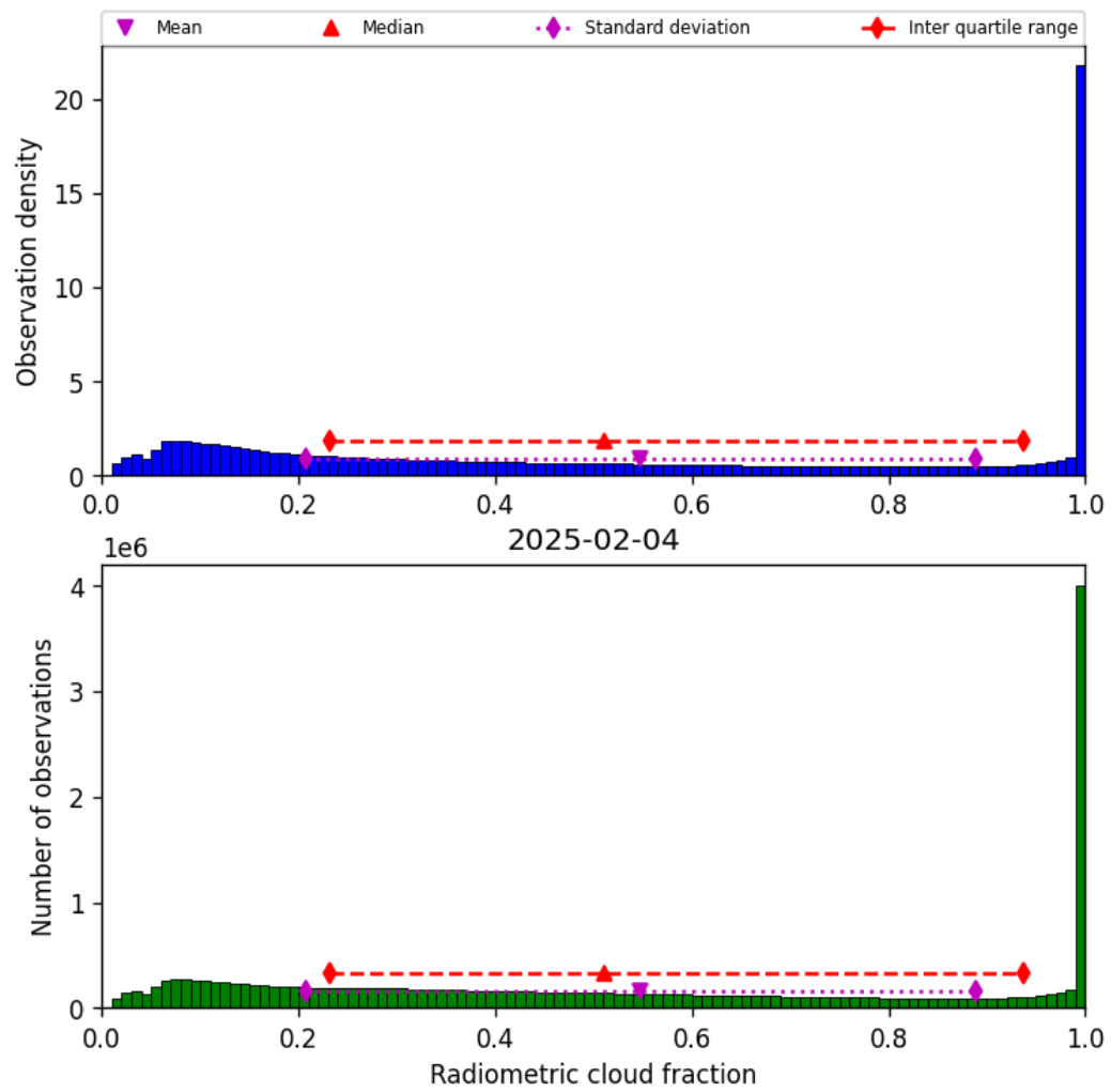
Figure 37: Histogram of “Radiometric cloud fraction” for 2025-02-04 to 2025-02-05
