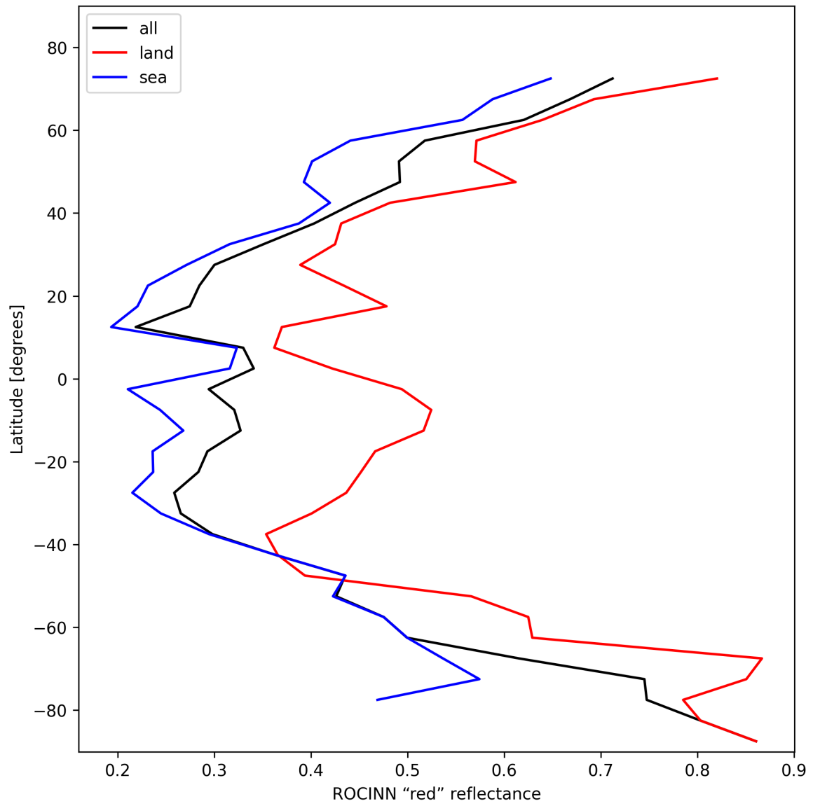
Figure 35: Zonal average of “ROCINN “red” reflectance” for 2025-02-04 to 2025-02-05.
