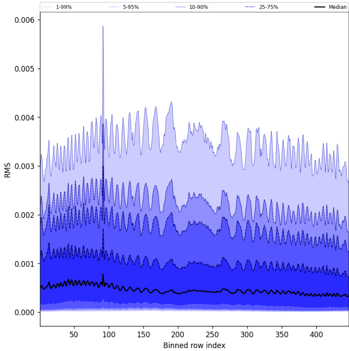
Figure 61: Along track statistics of “RMS” for 2025-02-04 to 2025-02-05
