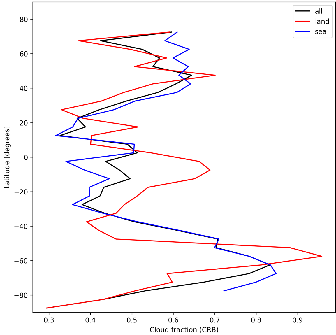
Figure 24: Zonal average of “Cloud fraction (CRB)” for 2025-02-04 to 2025-02-05.
