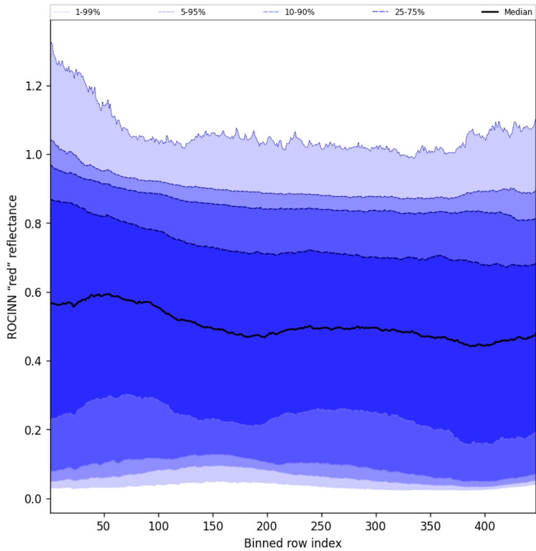
Figure 67: Along track statistics of "ROCINN "red" reflectance" for 2025-02-04 to 2025-02-05
