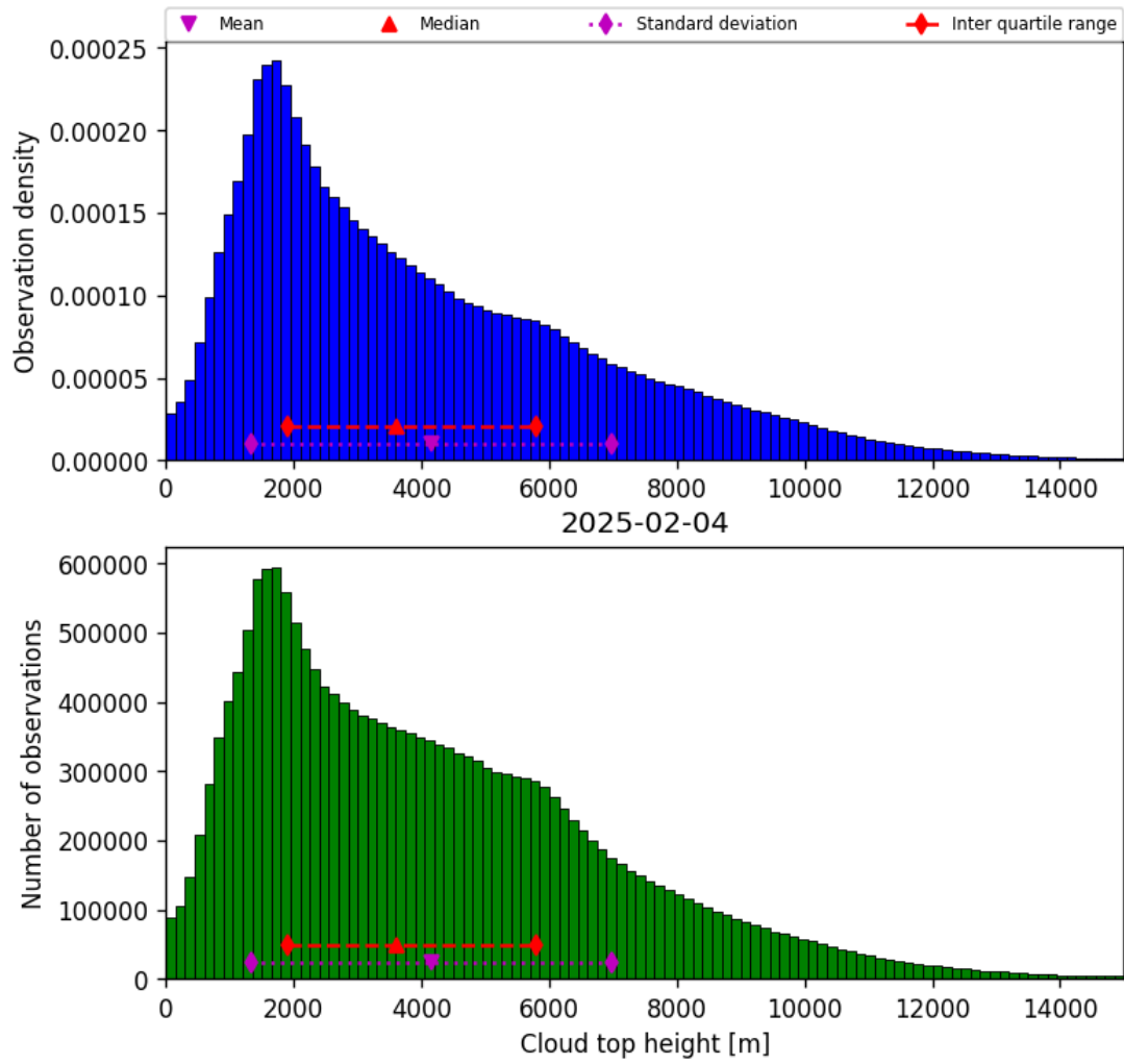
Figure 38: Histogram of “Cloud top height” for 2025-02-04 to 2025-02-05
