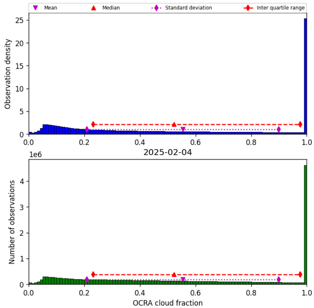
Figure 48: Histogram of “OCRA cloud fraction” for 2025-02-04 to 2025-02-05
