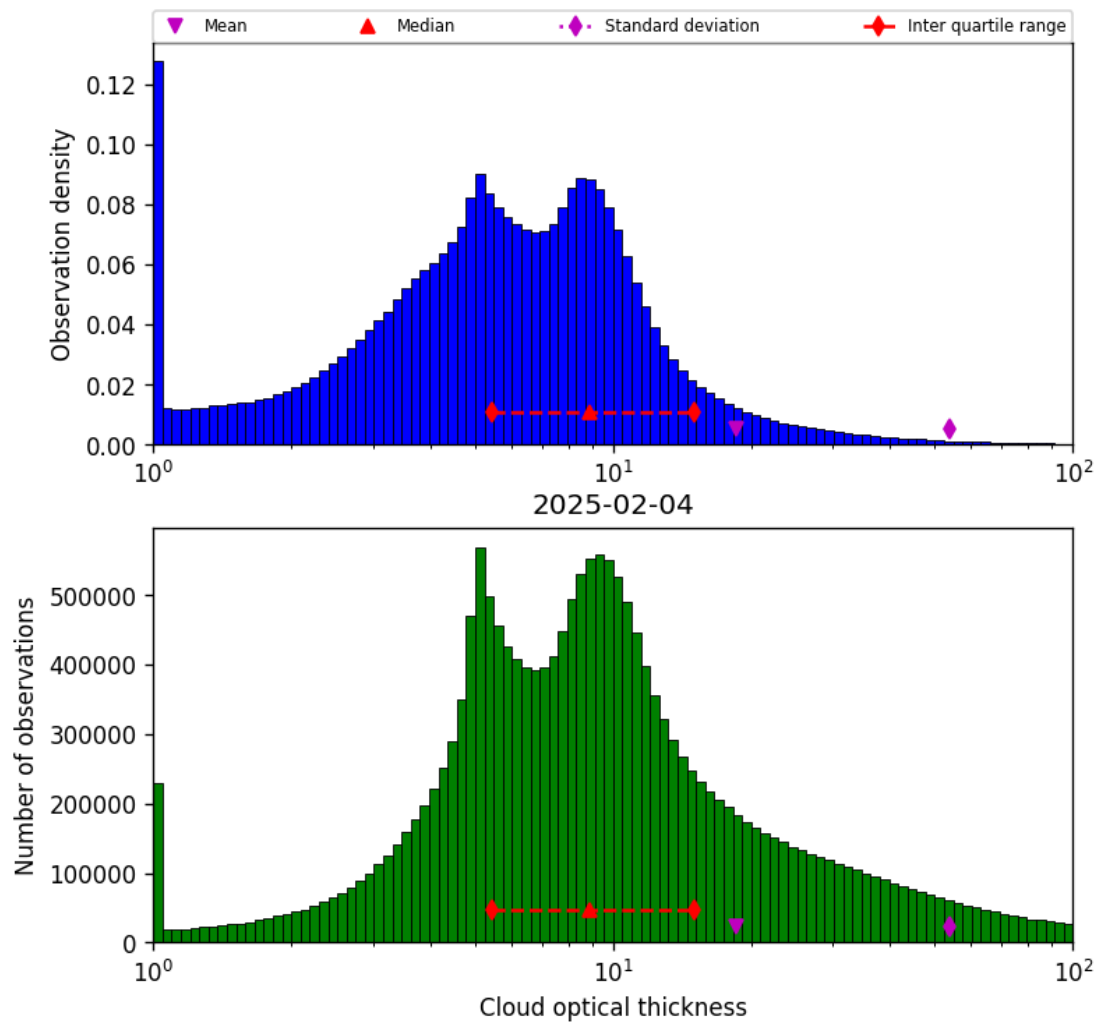
Figure 39: Histogram of “Cloud optical thickness” for 2025-02-04 to 2025-02-05
