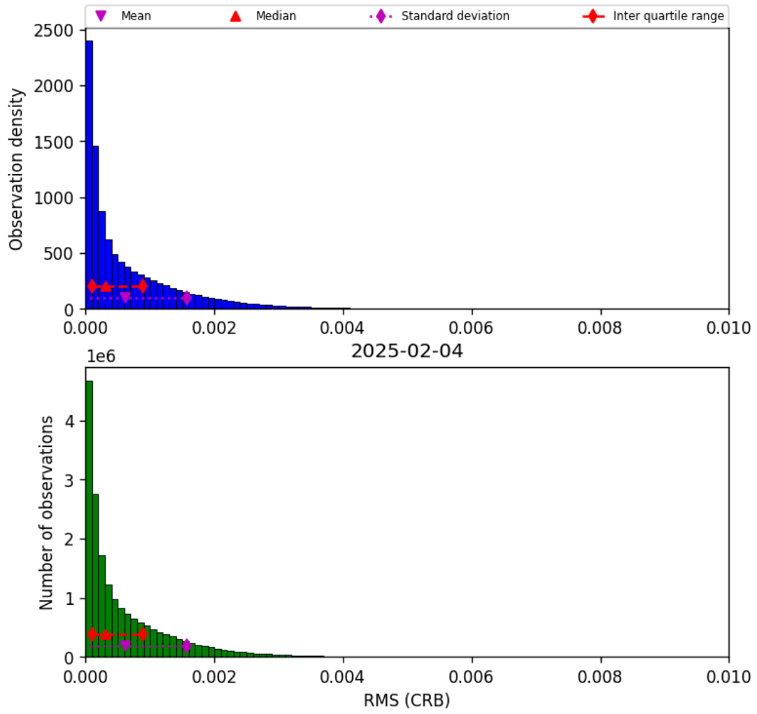
Figure 46: Histogram of “RMS (CRB)” for 2025-02-04 to 2025-02-05
