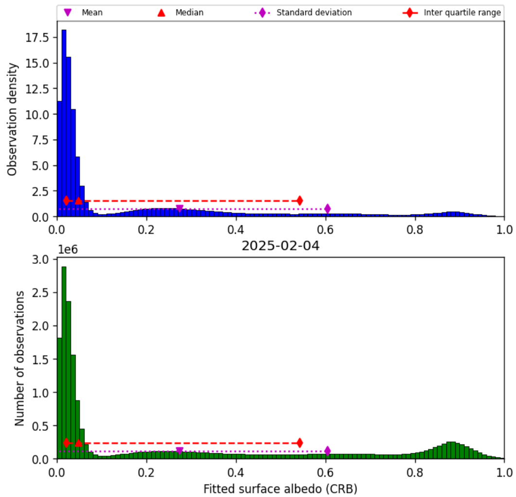
Figure 44: Histogram of “Fitted surface albedo (CRB)” for 2025-02-04 to 2025-02-05
