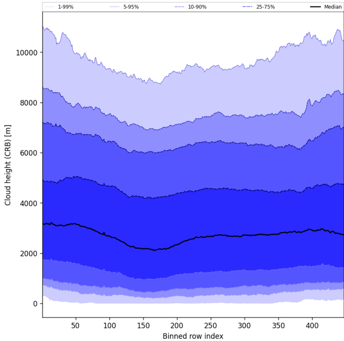
Figure 57: Along track statistics of “Cloud height (CRB)” for 2025-02-04 to 2025-02-05
