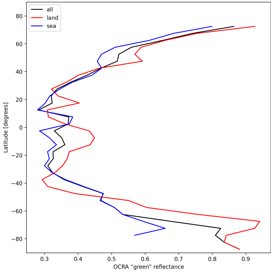
Figure 34: Zonal average of “OCRA “green” reflectance” for 2025-02-04 to 2025-02-05.
