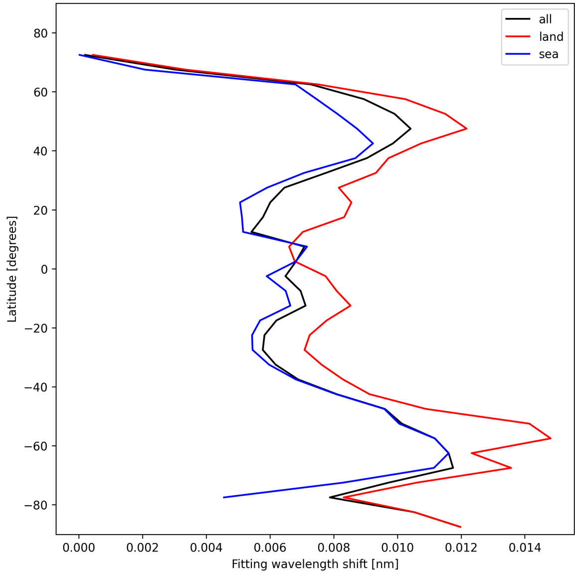
Figure 31: Zonal average of “Fitting wavelength shift” for 2025-02-04 to 2025-02-05.
