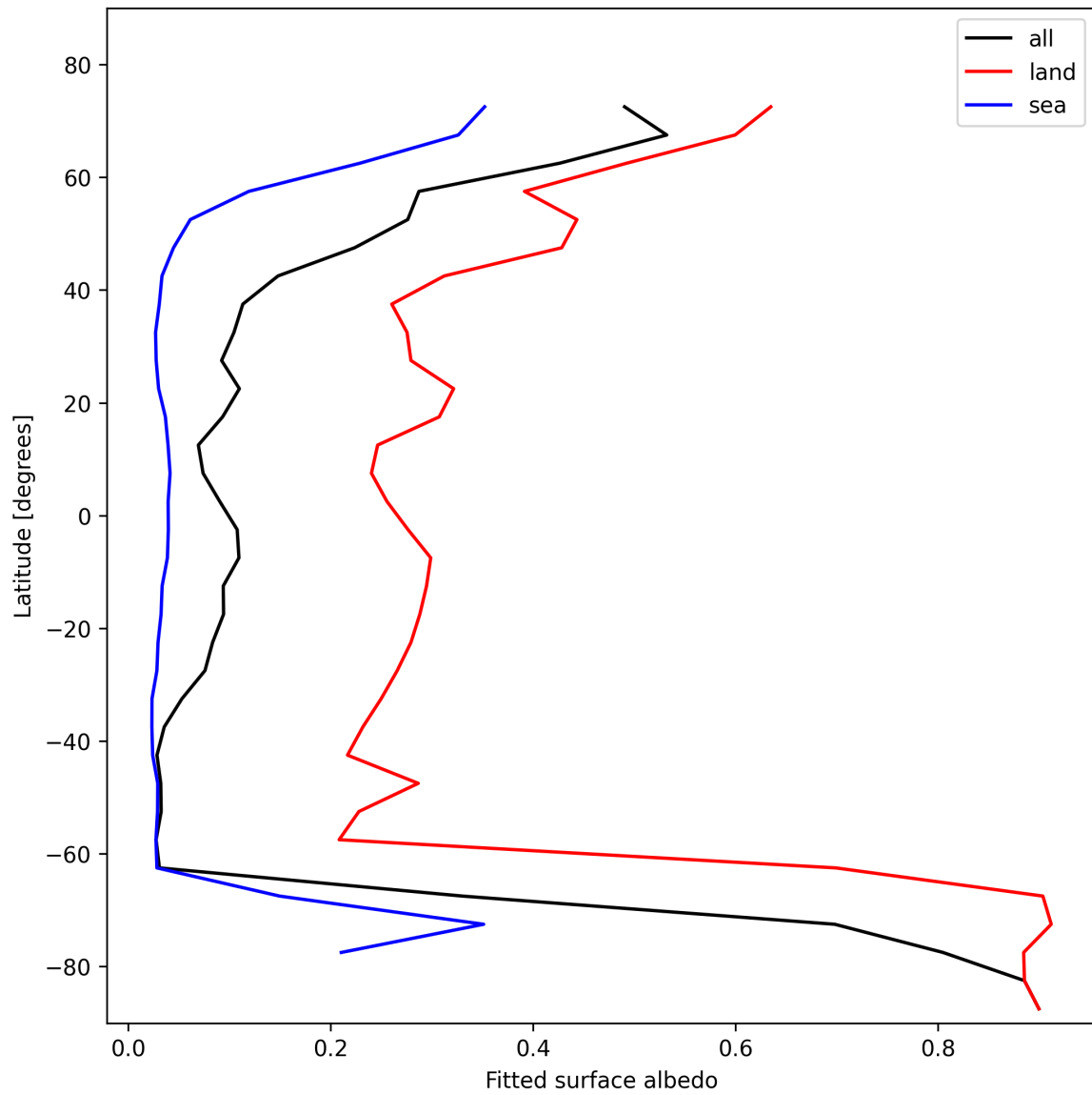
Figure 27: Zonal average of “Fitted surface albedo” for 2025-02-04 to 2025-02-05.
