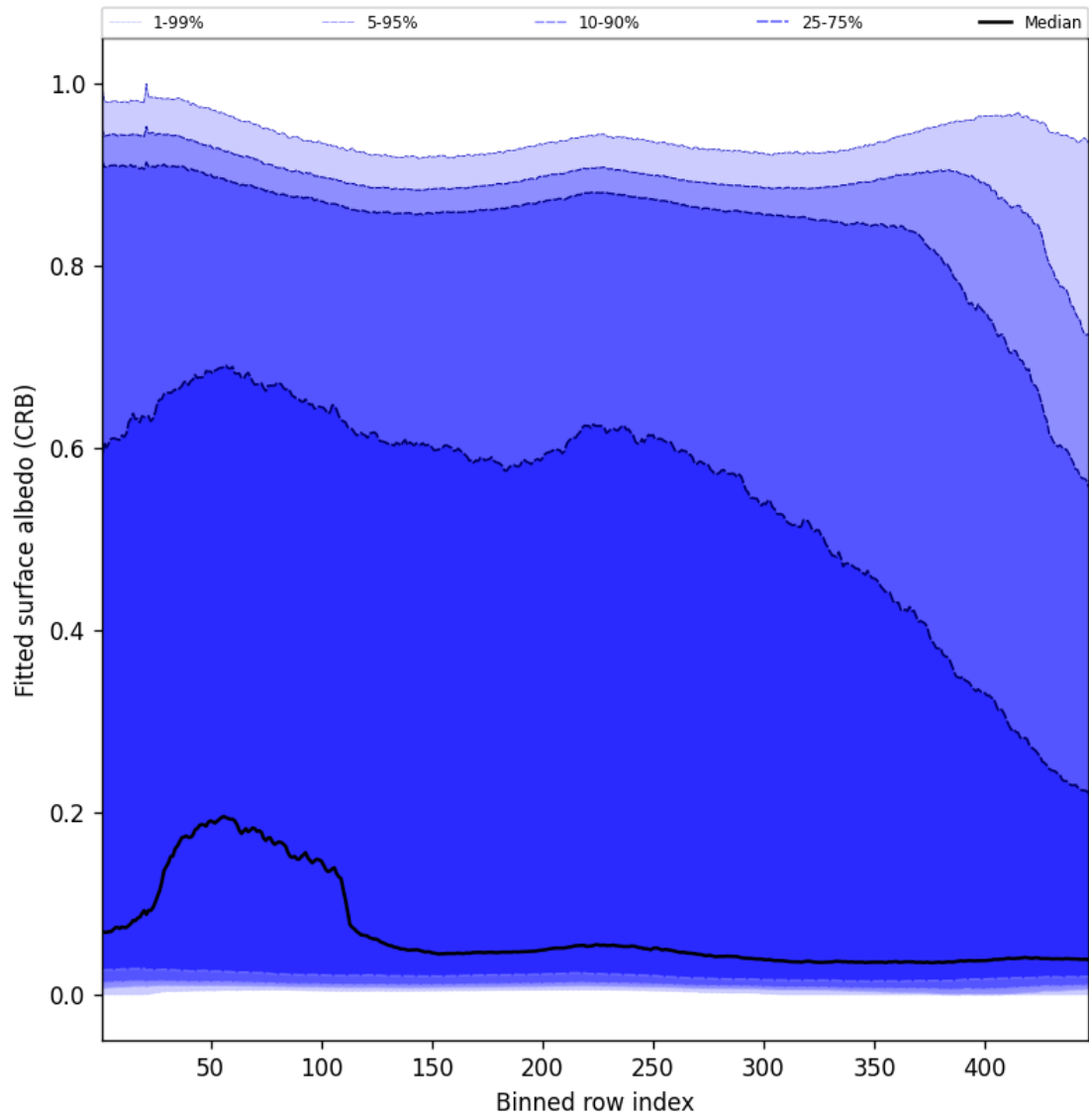
Figure 60: Along track statistics of “Fitted surface albedo (CRB)” for 2025-02-04 to 2025-02-05
