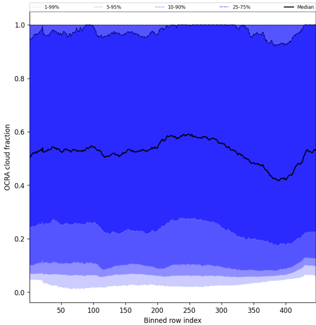
Figure 64: Along track statistics of “OCRA cloud fraction” for 2025-02-04 to 2025-02-05
