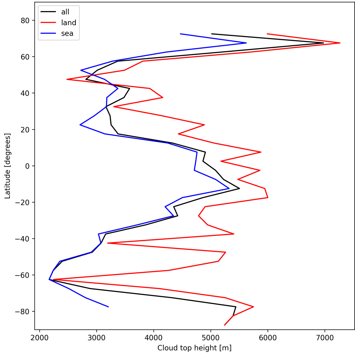
Figure 22: Zonal average of “Cloud top height” for 2025-02-04 to 2025-02-05.
