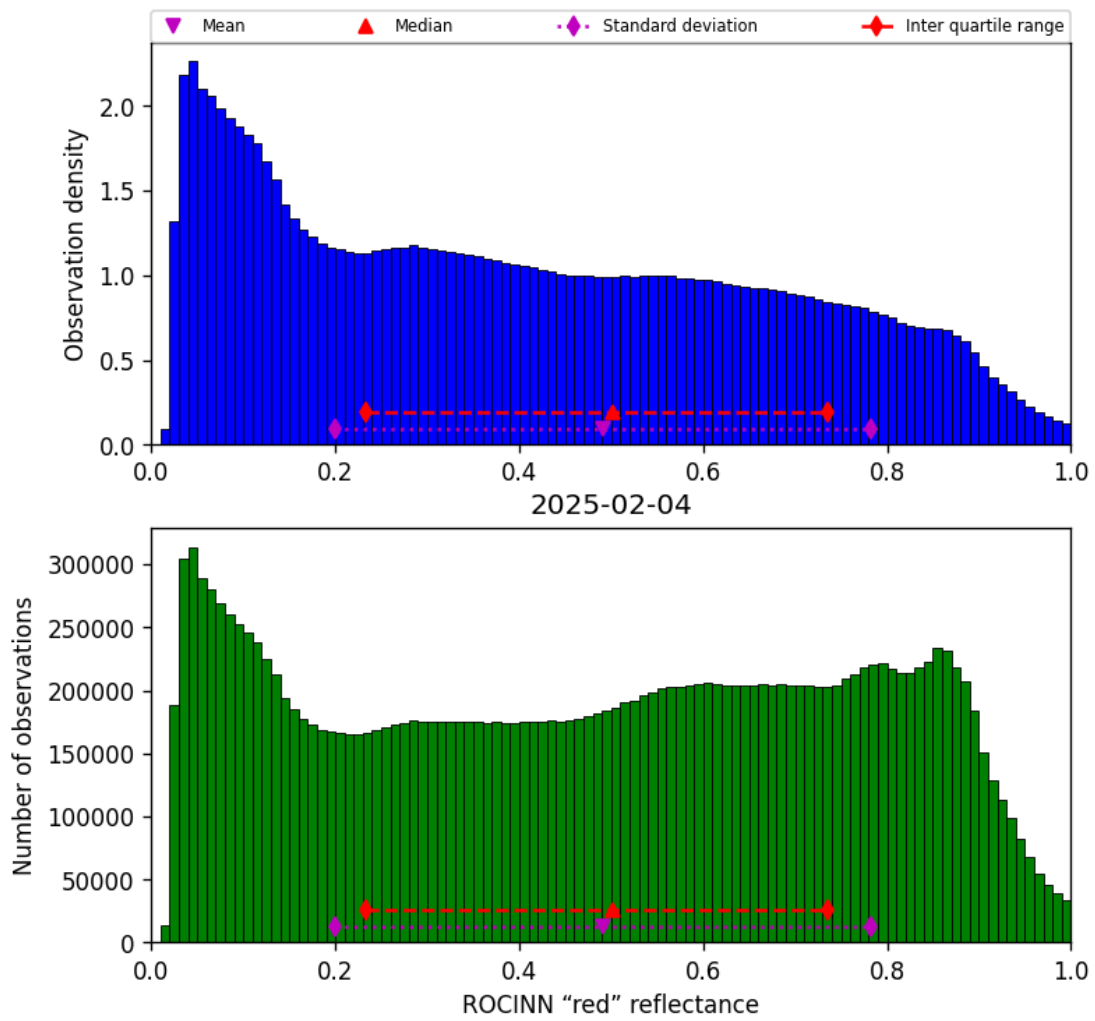
Figure 51: Histogram of “ROCINN “red” reflectance” for 2025-02-04 to 2025-02-05
