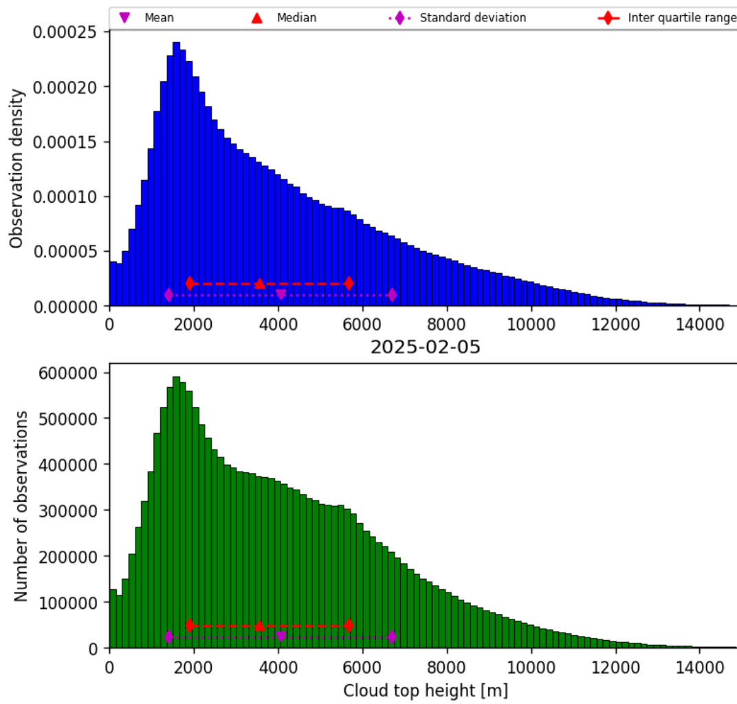
Figure 38: Histogram of “Cloud top height” for 2025-02-05 to 2025-02-06
