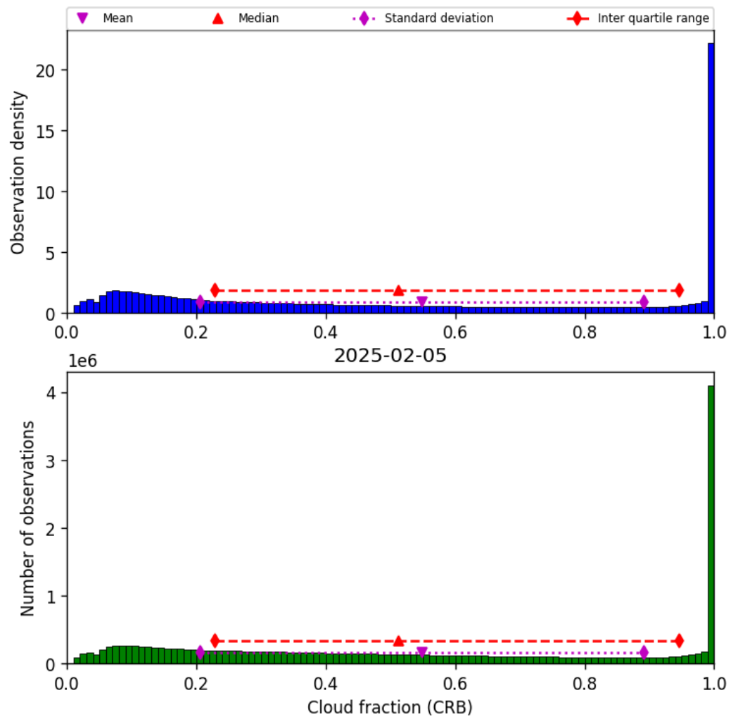
Figure 40: Histogram of “Cloud fraction (CRB)” for 2025-02-05 to 2025-02-06
