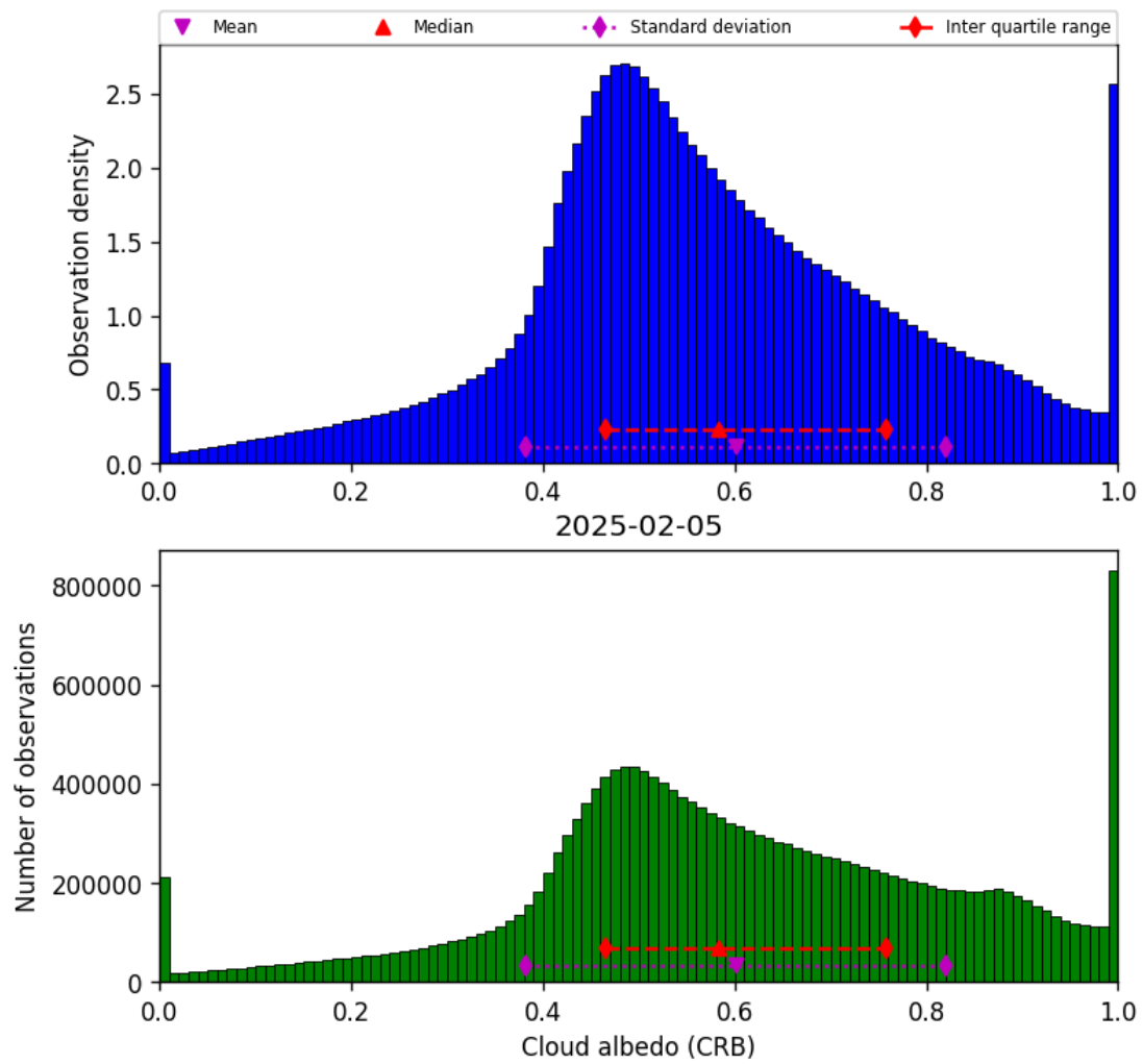
Figure 42: Histogram of “Cloud albedo (CRB)” for 2025-02-05 to 2025-02-06
