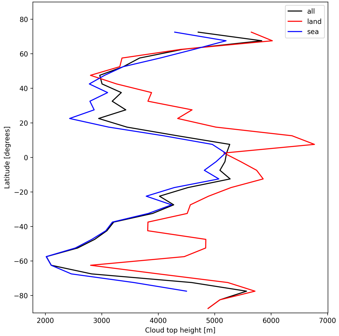
Figure 22: Zonal average of “Cloud top height” for 2025-02-05 to 2025-02-06.
