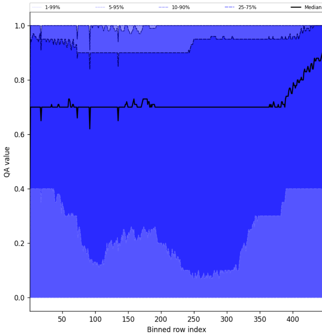
Figure 52: Along track statistics of “QA value” for 2025-02-05 to 2025-02-06
