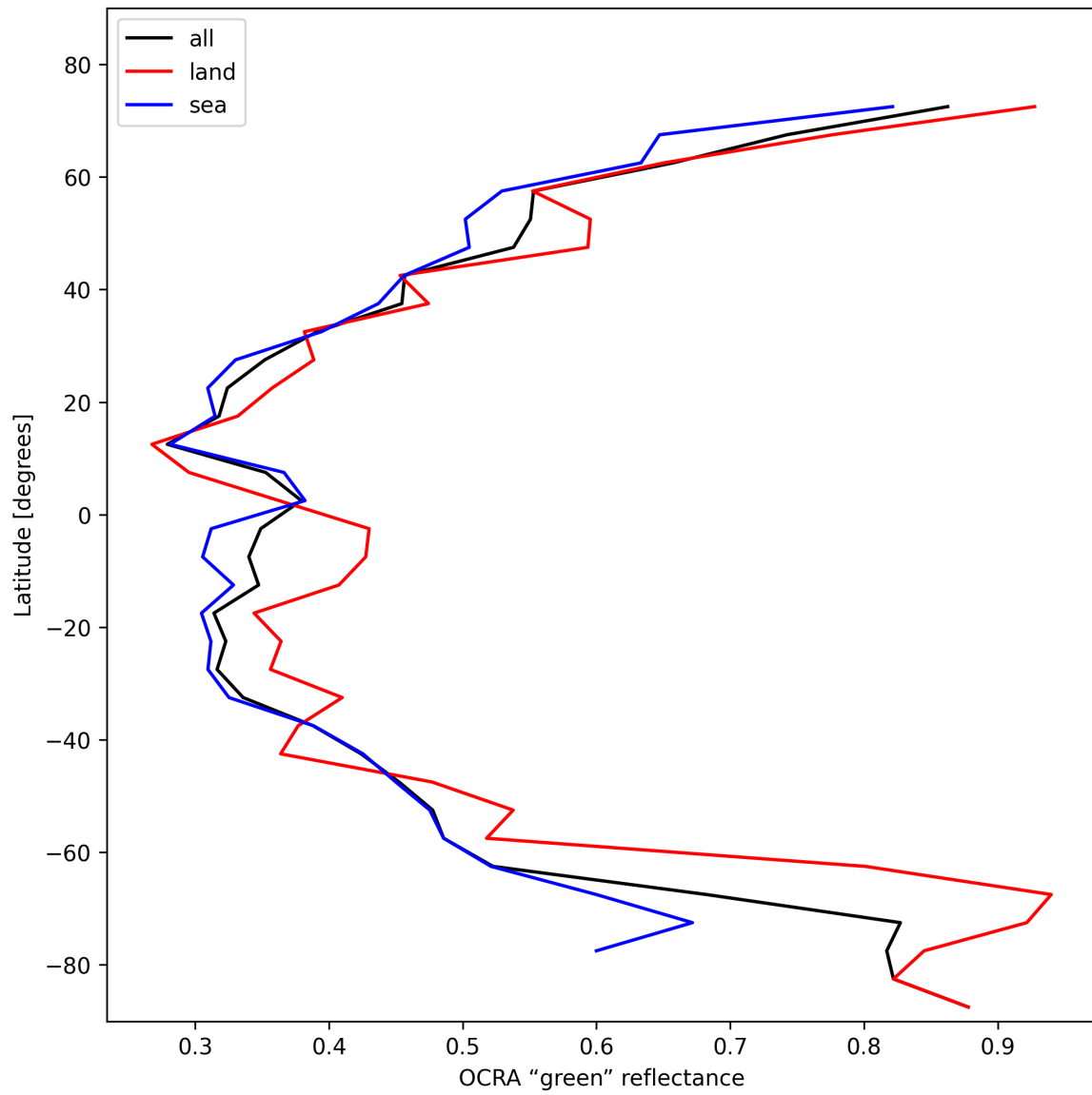
Figure 34: Zonal average of “OCRA “green” reflectance” for 2025-02-05 to 2025-02-06.
