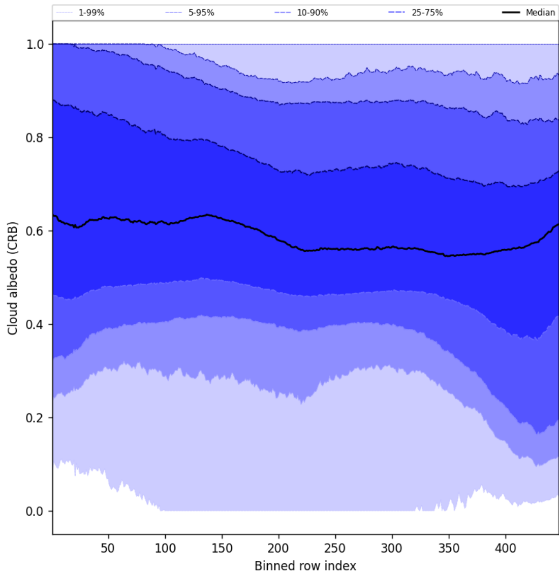
Figure 58: Along track statistics of “Cloud albedo (CRB)” for 2025-02-05 to 2025-02-06
