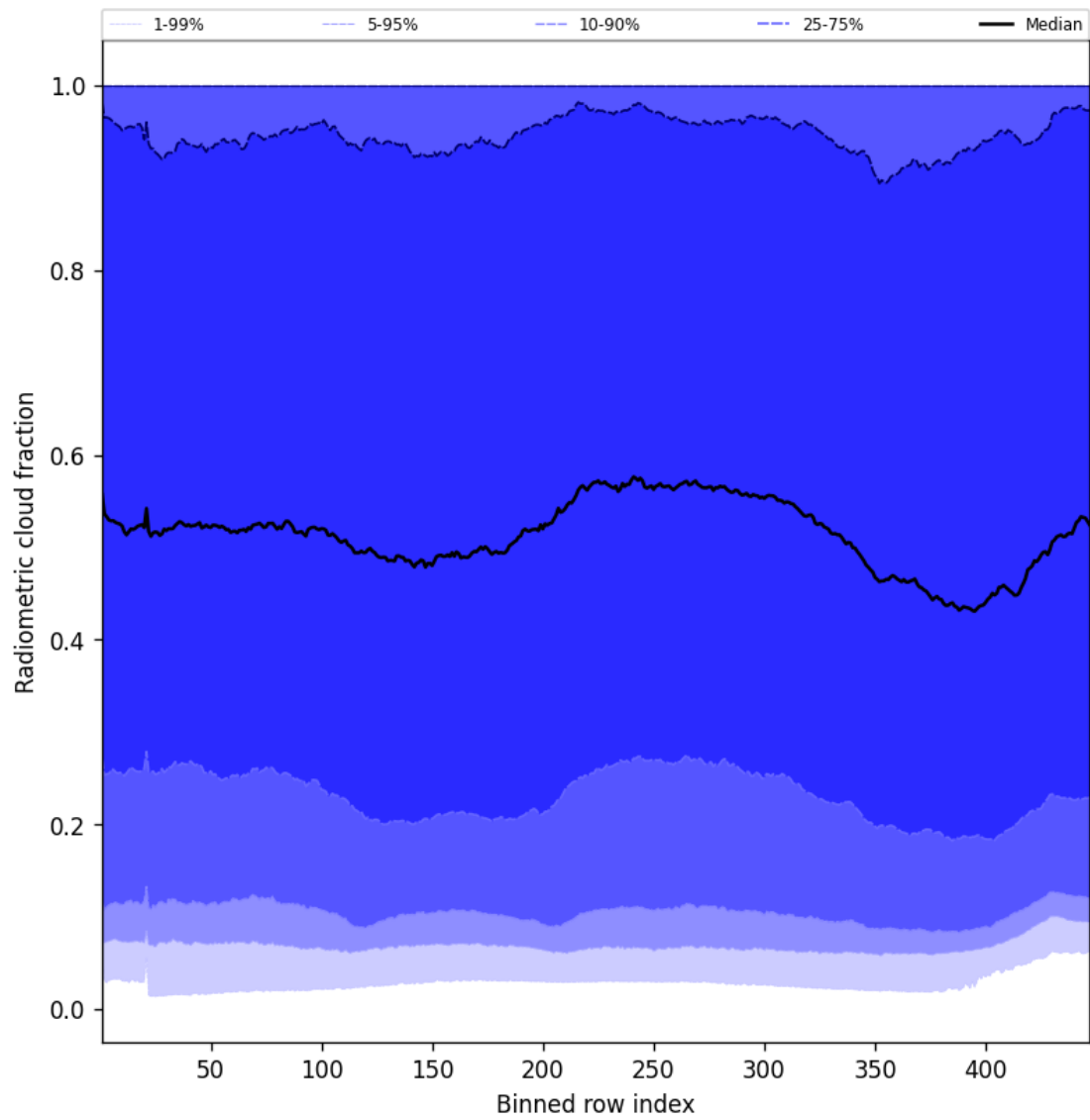
Figure 53: Along track statistics of “Radiometric cloud fraction” for 2025-02-05 to 2025-02-06
