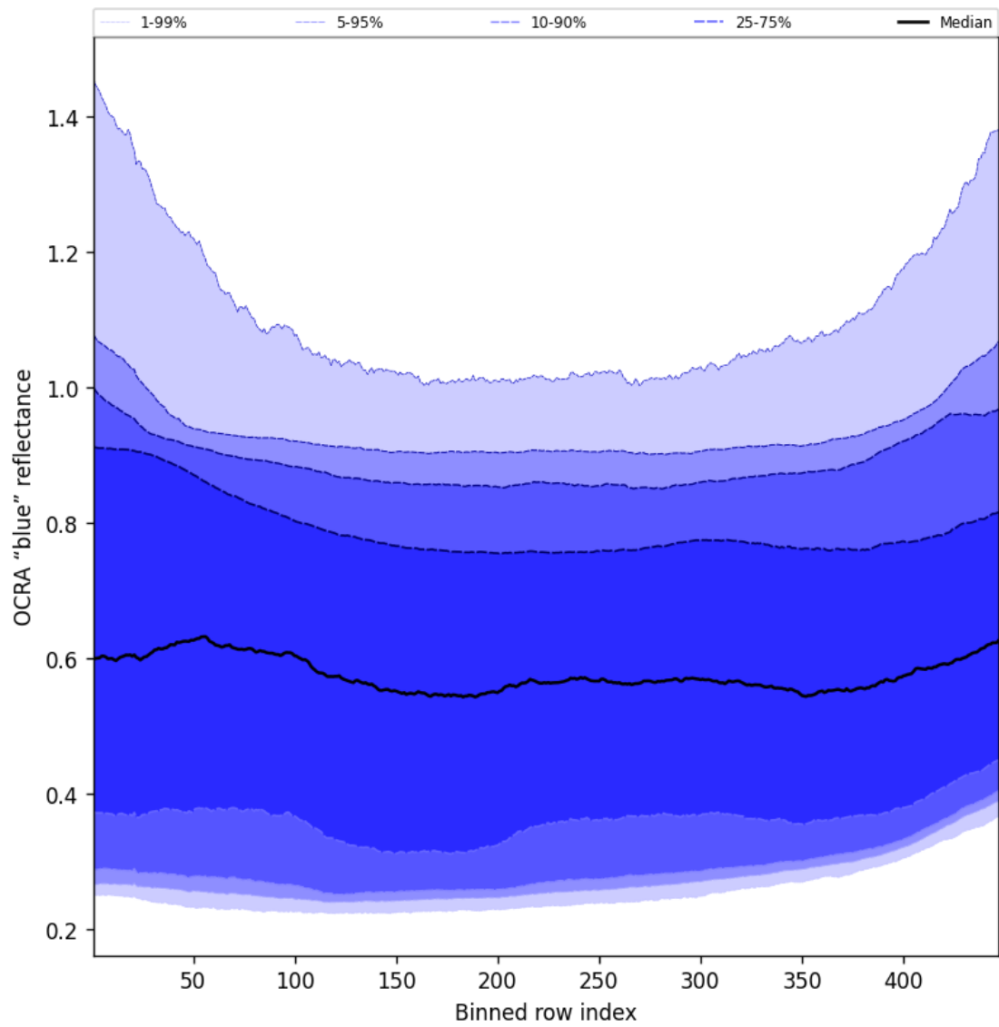
Figure 65: Along track statistics of “OCRA “blue” reflectance” for 2025-02-05 to 2025-02-06
