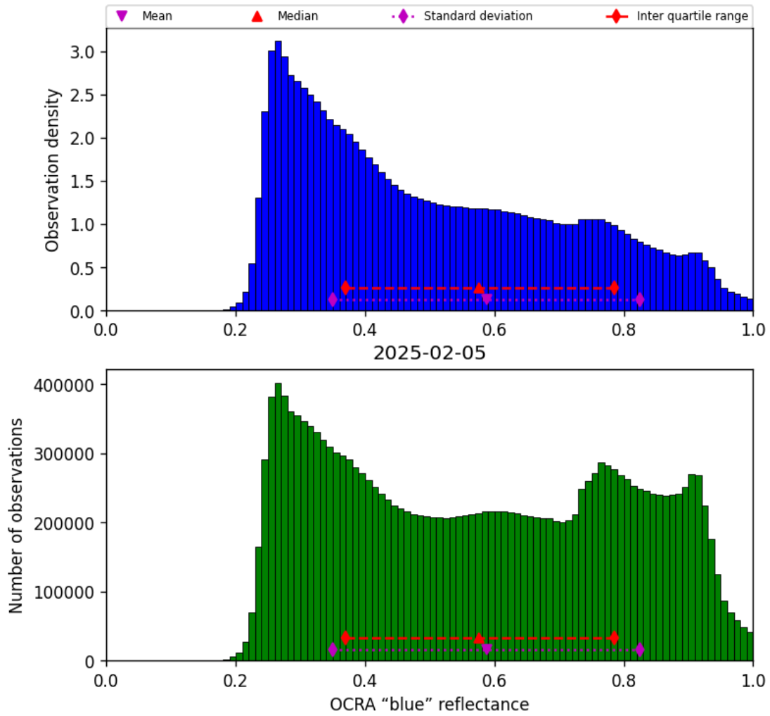
Figure 49: Histogram of “OCRA “blue” reflectance” for 2025-02-05 to 2025-02-06
