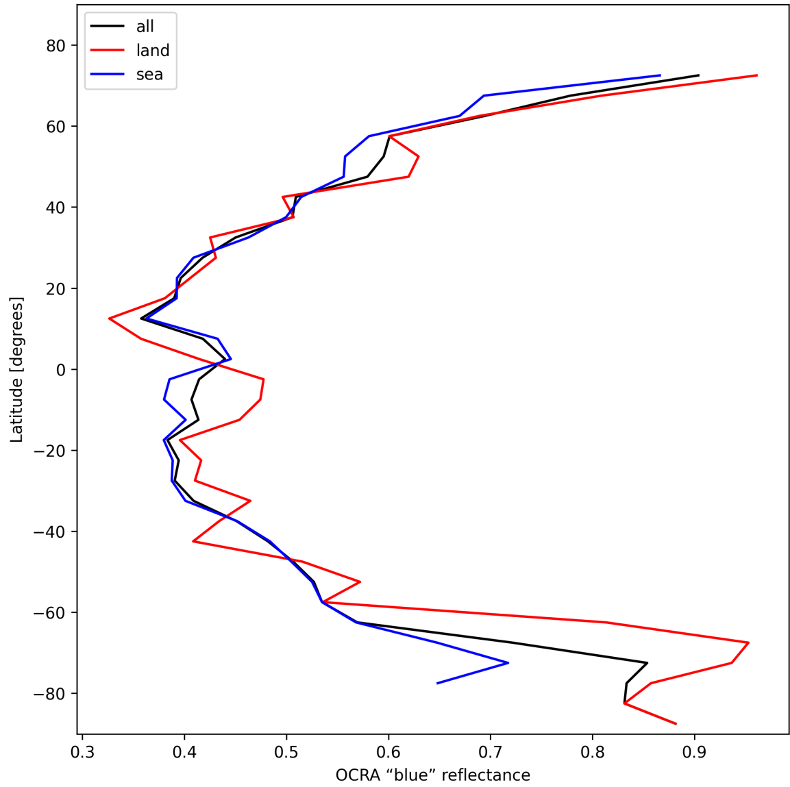
Figure 33: Zonal average of “OCRA “blue” reflectance” for 2025-02-05 to 2025-02-06.
