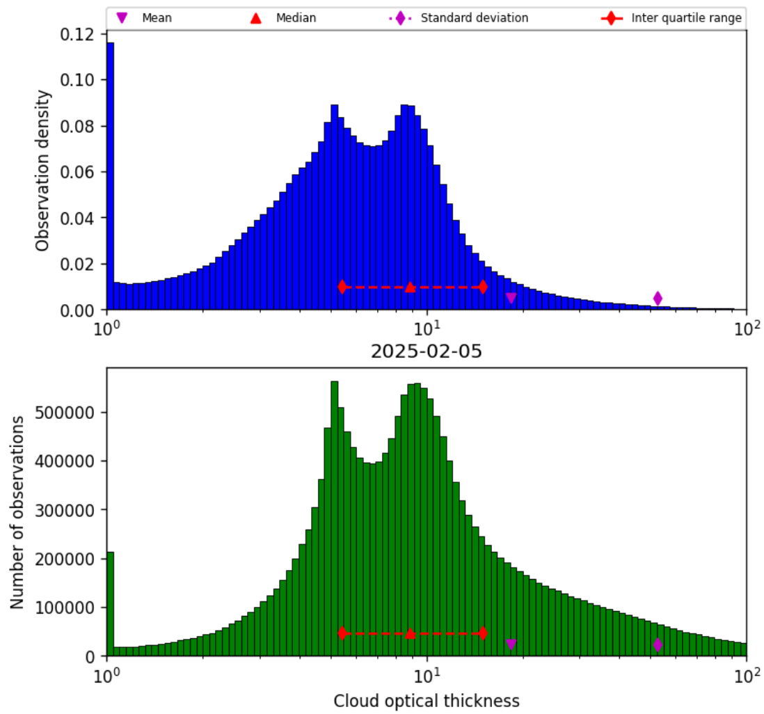
Figure 39: Histogram of “Cloud optical thickness” for 2025-02-05 to 2025-02-06
