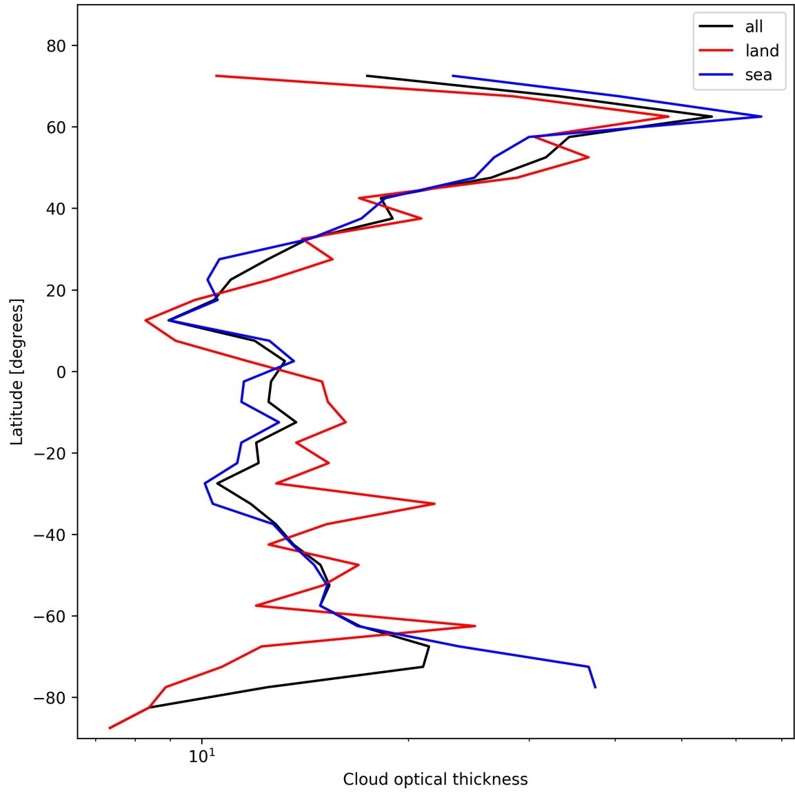
Figure 23: Zonal average of “Cloud optical thickness” for 2025-02-05 to 2025-02-06.
