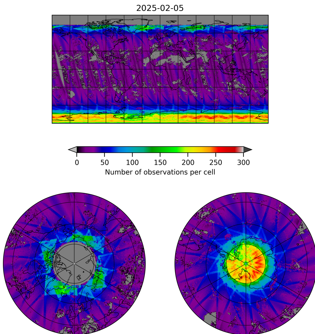
Figure 19: Map of the number of observations for 2025-02-05 to 2025-02-06
