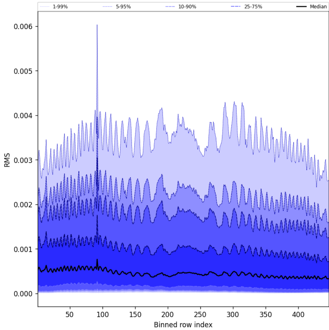
Figure 61: Along track statistics of “RMS” for 2025-02-05 to 2025-02-06
