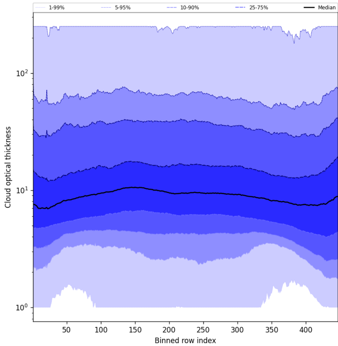
Figure 55: Along track statistics of “Cloud optical thickness” for 2025-02-05 to 2025-02-06
