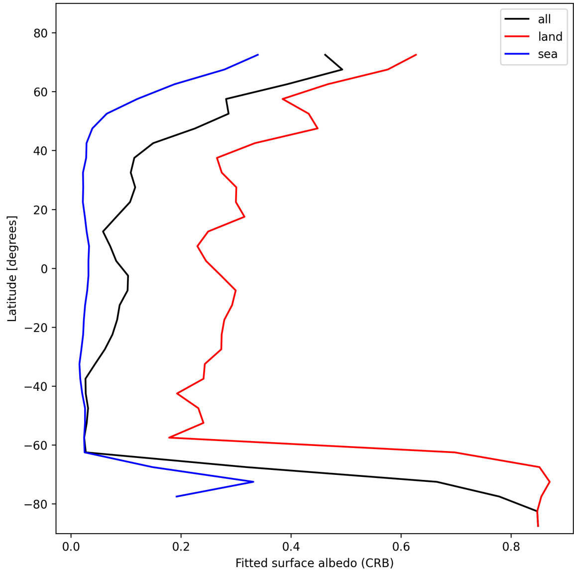
Figure 28: Zonal average of “Fitted surface albedo (CRB)” for 2025-02-05 to 2025-02-06.
