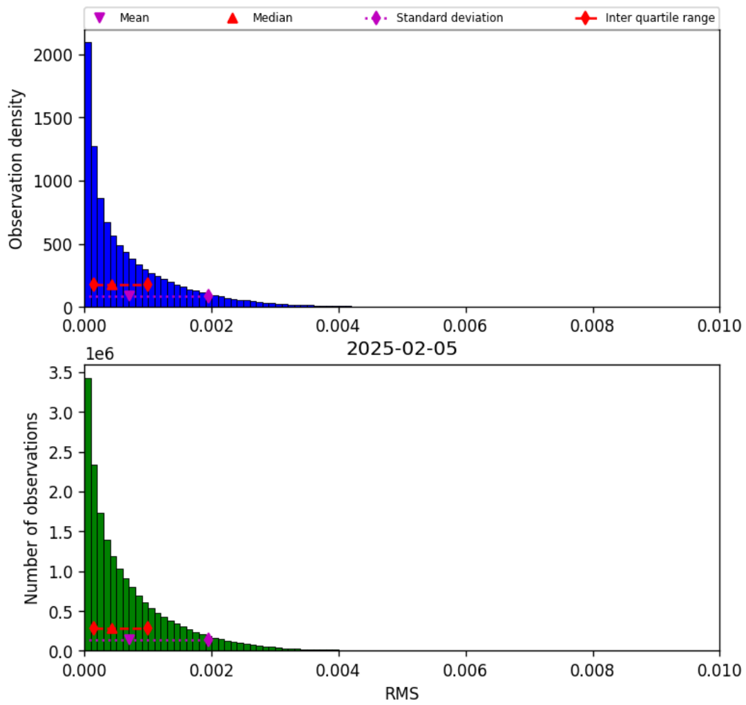
Figure 45: Histogram of “RMS” for 2025-02-05 to 2025-02-06
