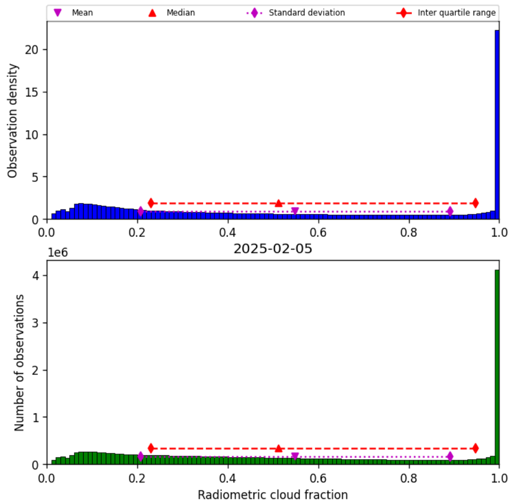
Figure 37: Histogram of “Radiometric cloud fraction” for 2025-02-05 to 2025-02-06
