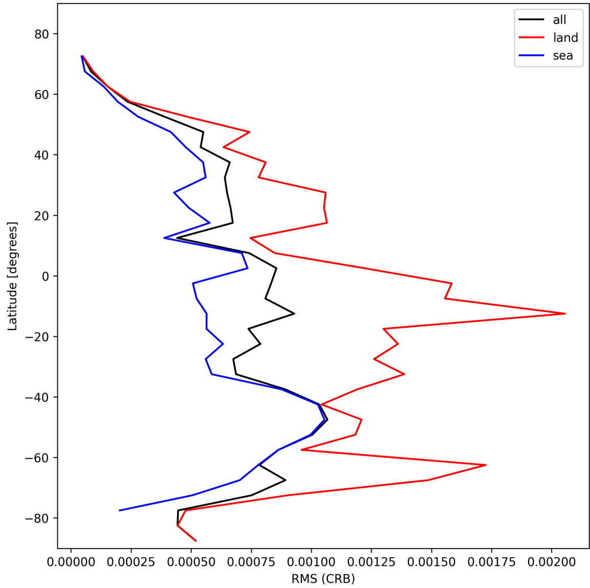
Figure 30: Zonal average of “RMS (CRB)” for 2025-02-05 to 2025-02-06.
