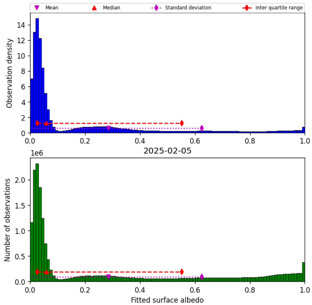
Figure 43: Histogram of “Fitted surface albedo” for 2025-02-05 to 2025-02-06
