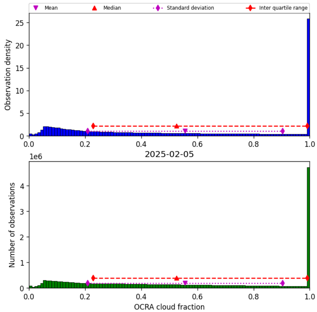
Figure 48: Histogram of “OCRA cloud fraction” for 2025-02-05 to 2025-02-06
