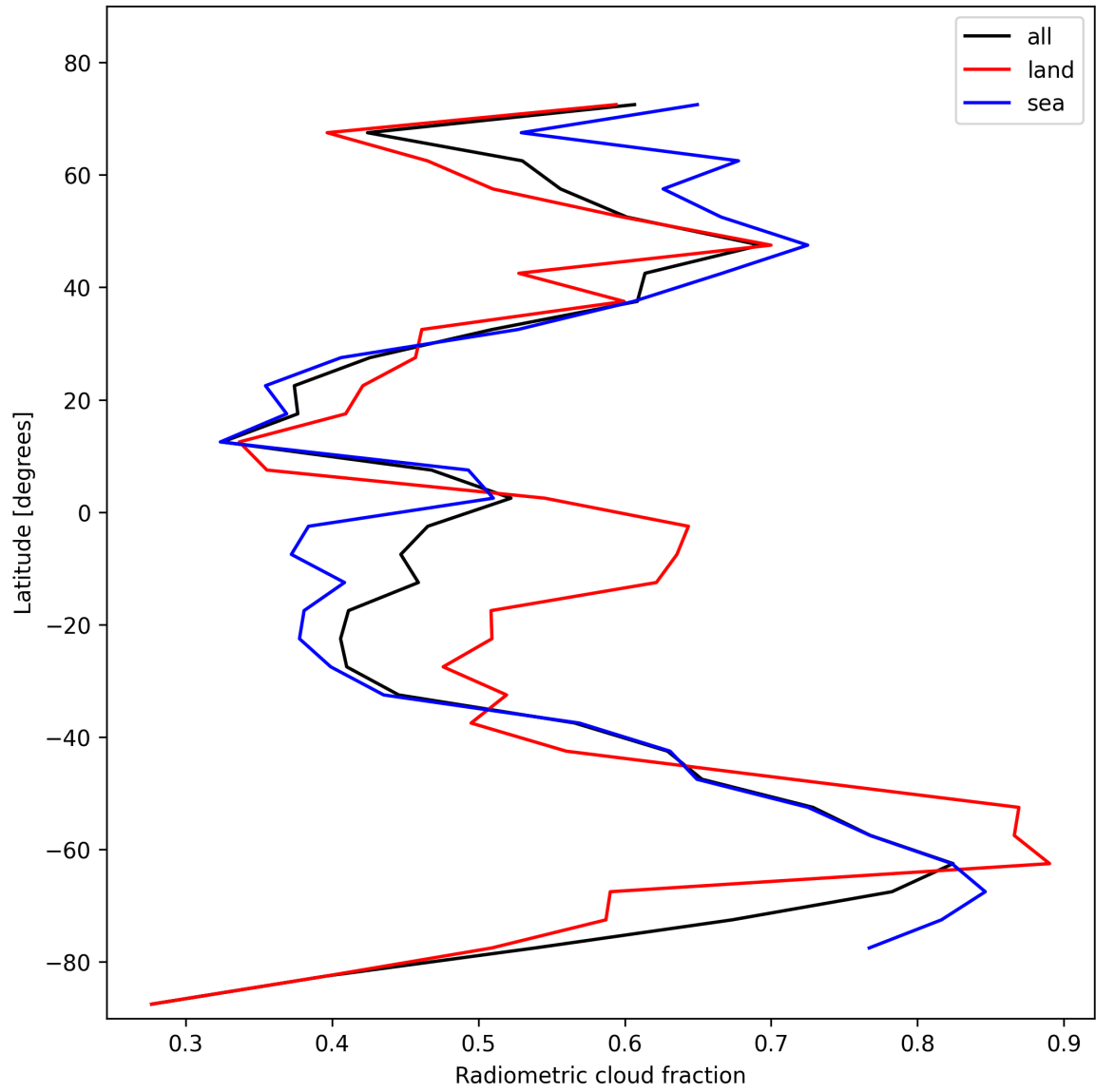
Figure 21: Zonal average of “Radiometric cloud fraction” for 2025-02-05 to 2025-02-06.
