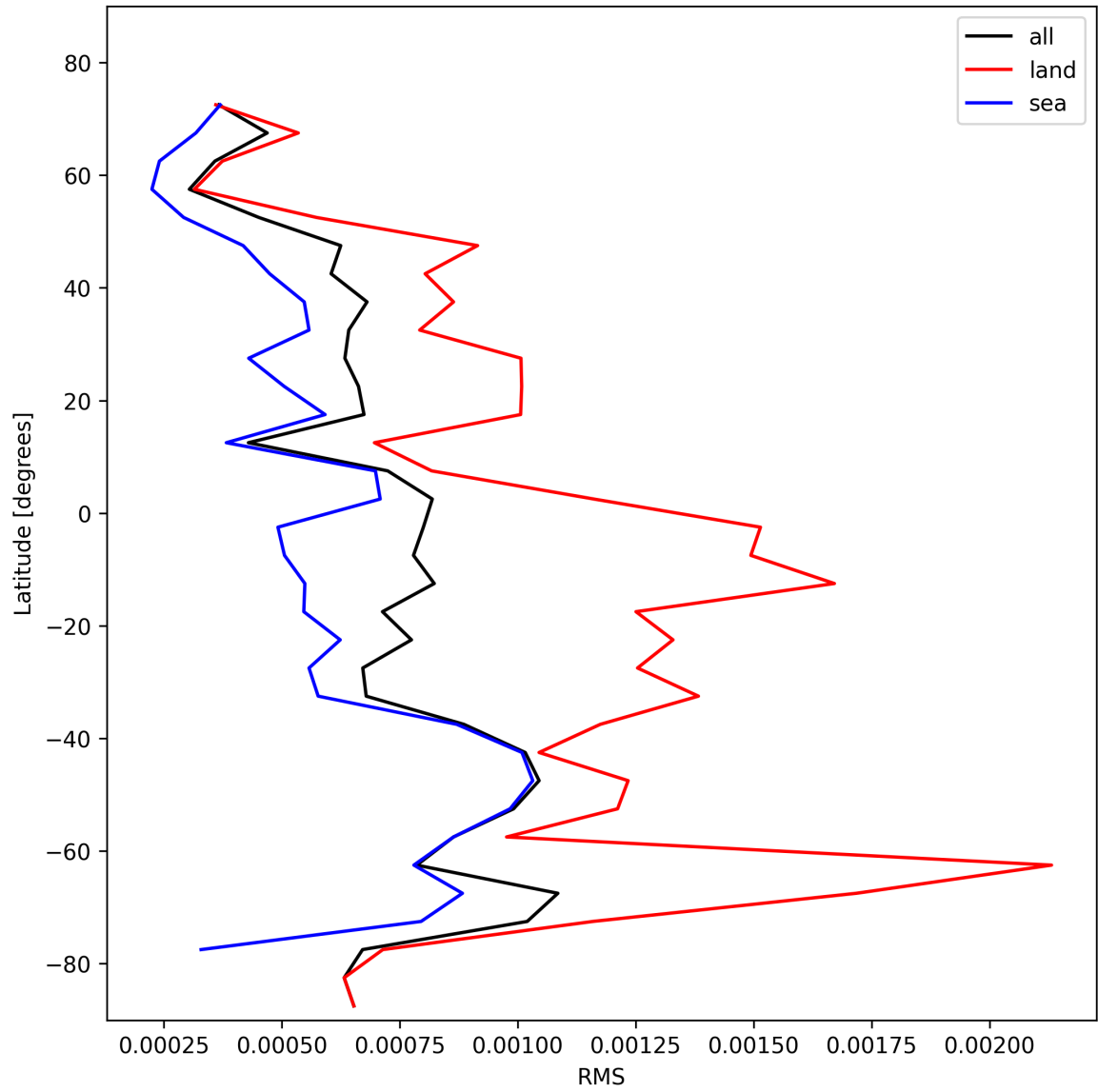
Figure 29: Zonal average of “RMS” for 2025-02-05 to 2025-02-06.
