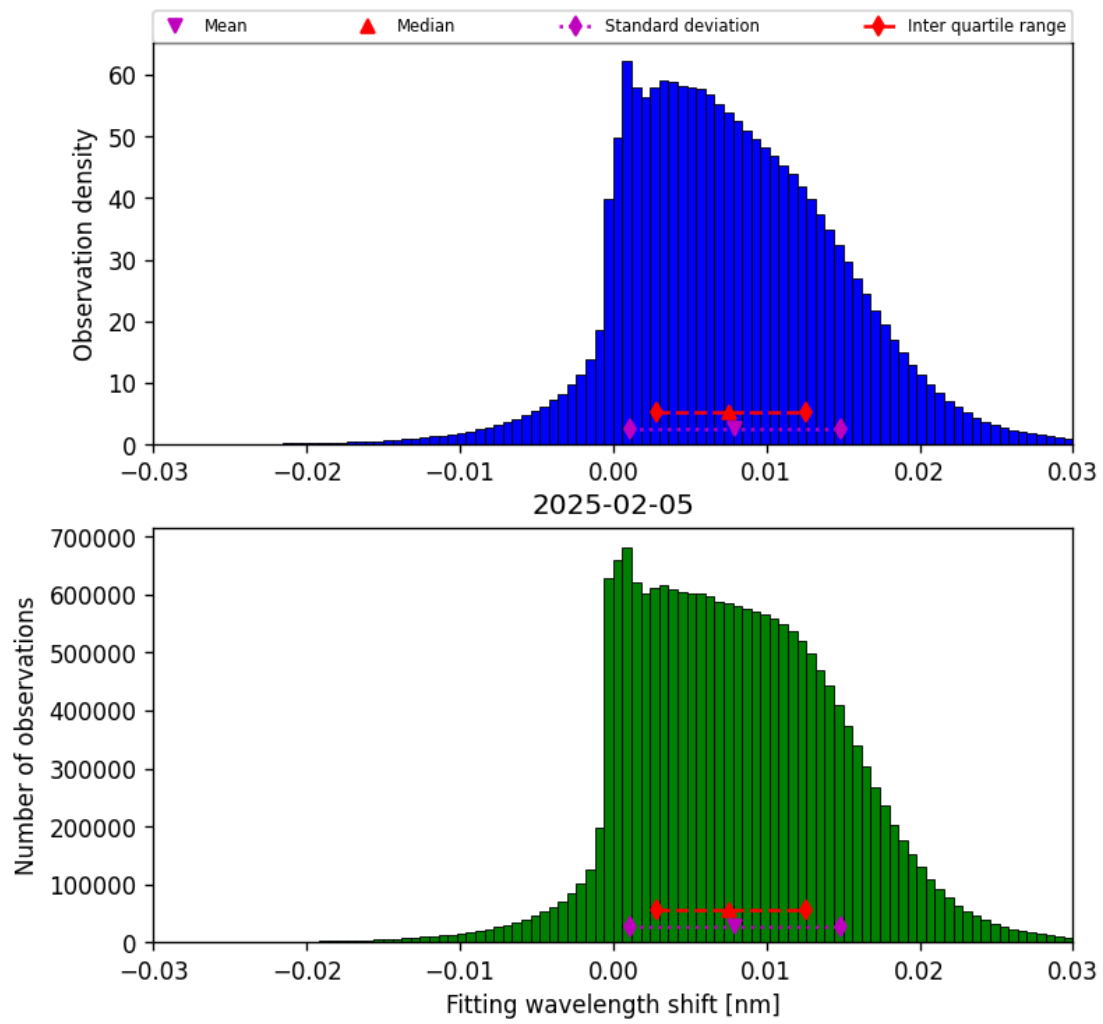
Figure 47: Histogram of “Fitting wavelength shift” for 2025-02-05 to 2025-02-06
