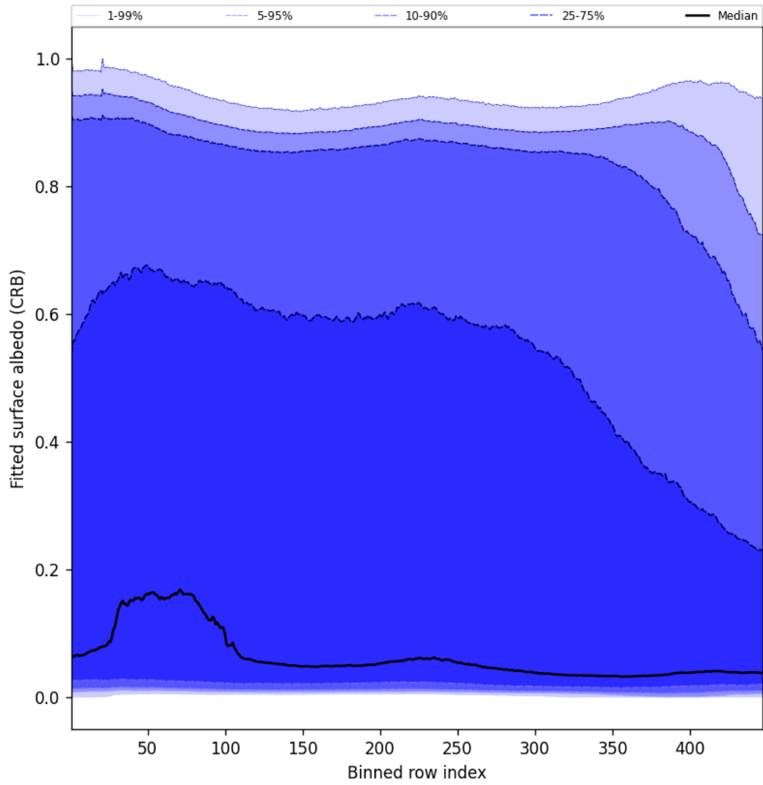
Figure 60: Along track statistics of “Fitted surface albedo (CRB)” for 2025-02-05 to 2025-02-06
