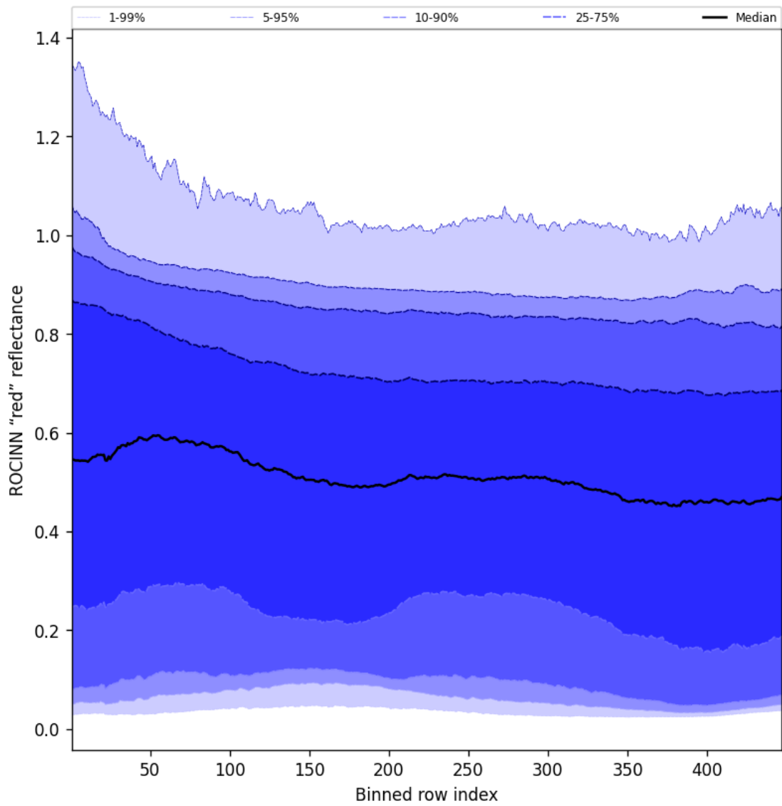
Figure 67: Along track statistics of “ROCINN “red” reflectance” for 2025-02-05 to 2025-02-06
