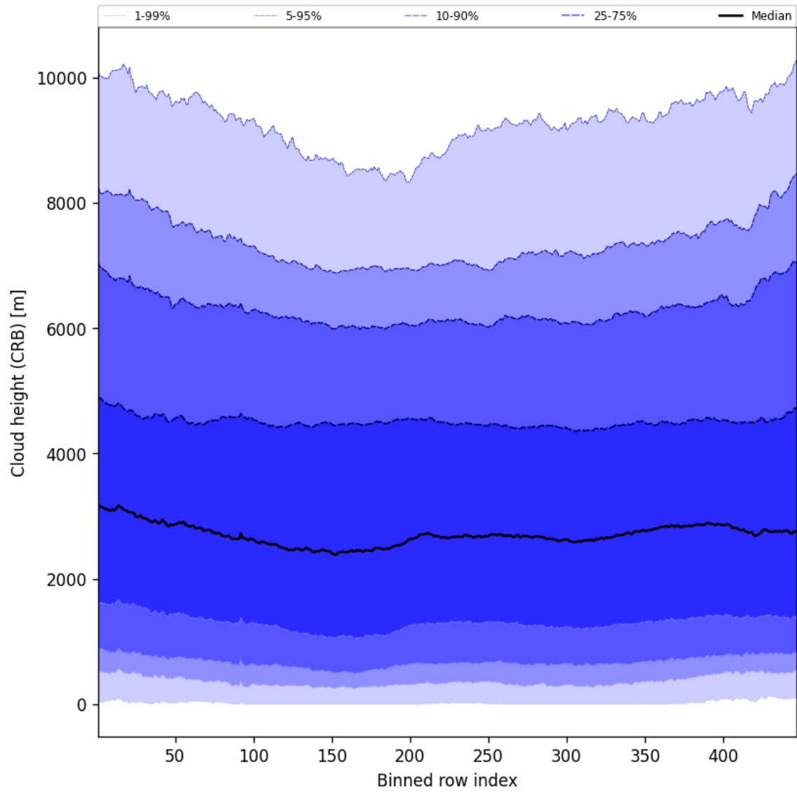
Figure 57: Along track statistics of “Cloud height (CRB)” for 2025-02-05 to 2025-02-06
