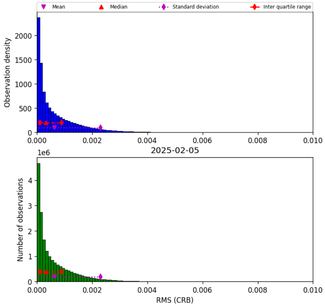
Figure 46: Histogram of "RMS (CRB)" for 2025-02-05 to 2025-02-06
