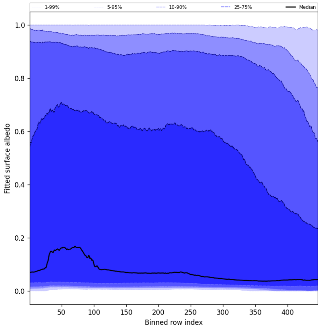
Figure 59: Along track statistics of “Fitted surface albedo” for 2025-02-05 to 2025-02-06
