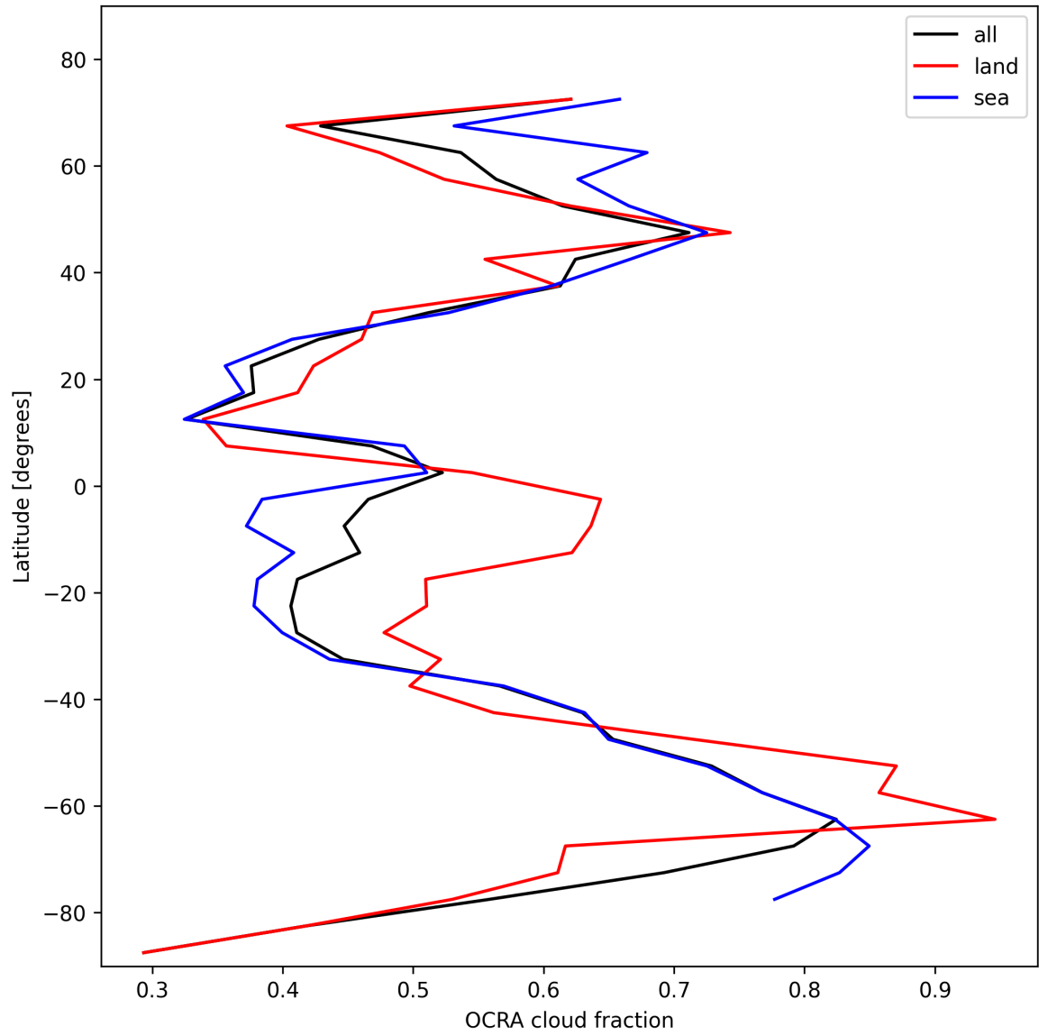
Figure 32: Zonal average of “OCRA cloud fraction” for 2025-02-05 to 2025-02-06.
