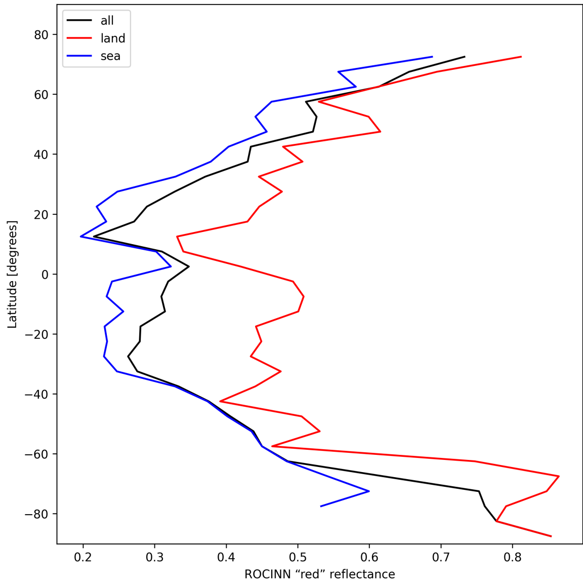
Figure 35: Zonal average of “ROCINN “red” reflectance” for 2025-02-05 to 2025-02-06.
