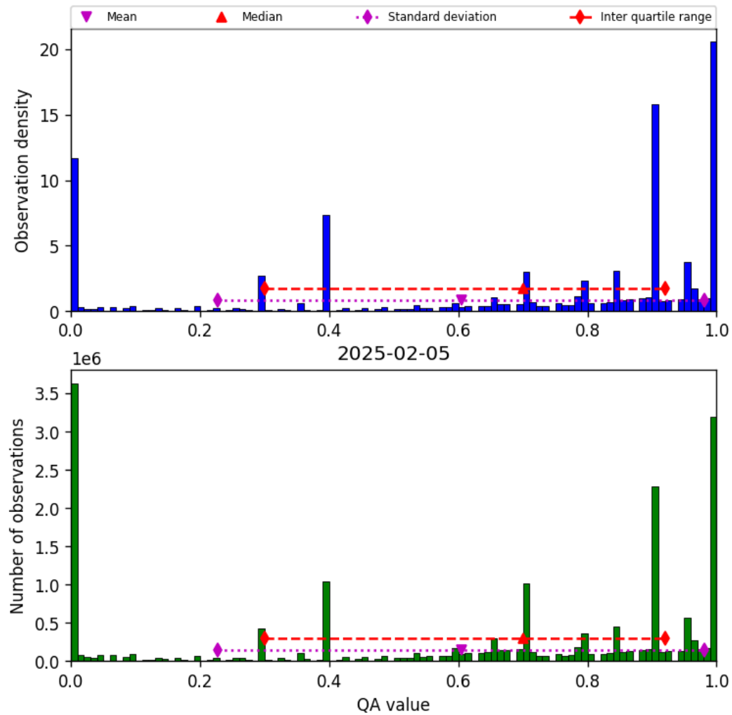
Figure 36: Histogram of “QA value” for 2025-02-05 to 2025-02-06
