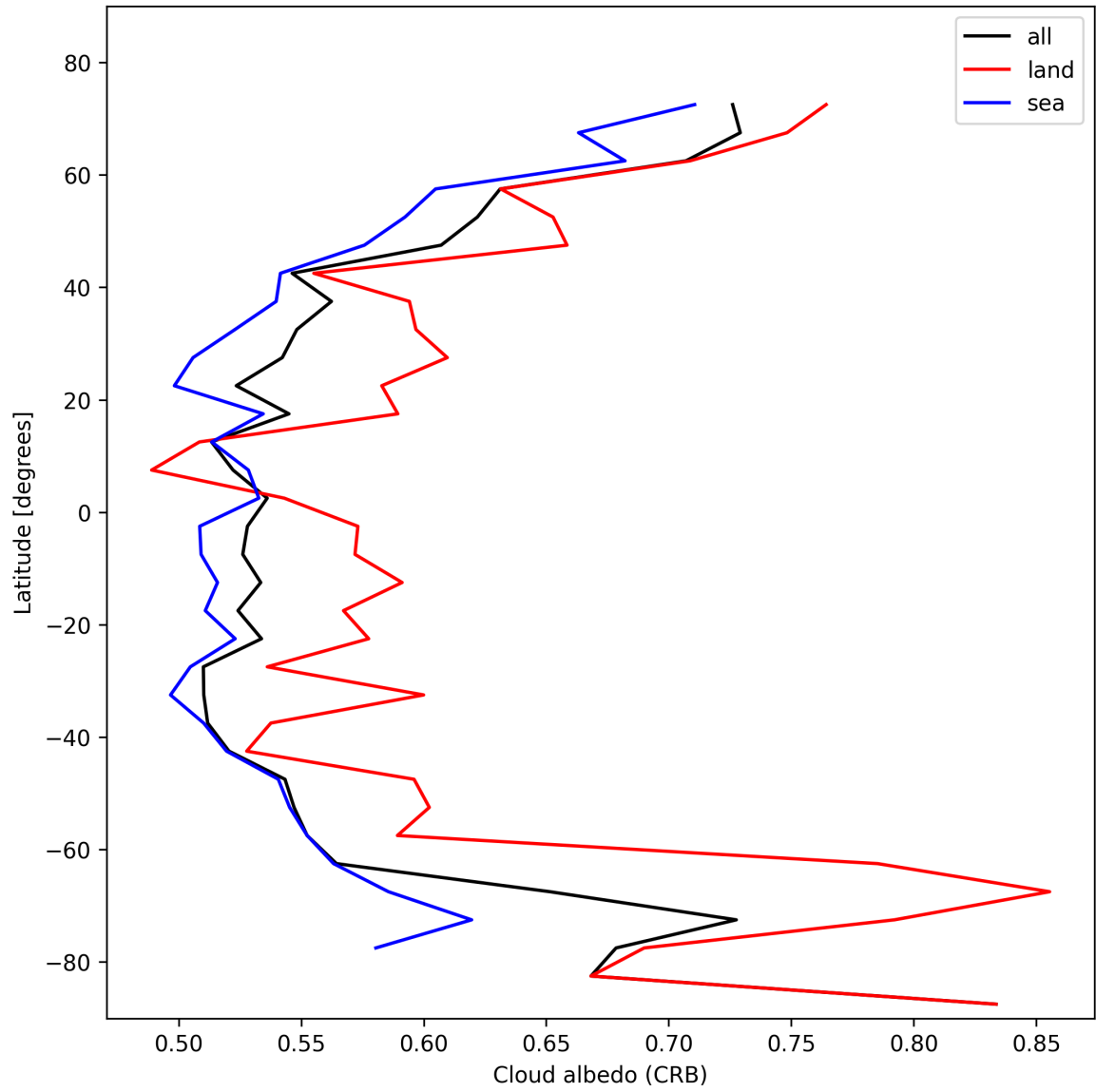
Figure 26: Zonal average of “Cloud albedo (CRB)” for 2025-02-05 to 2025-02-06.
