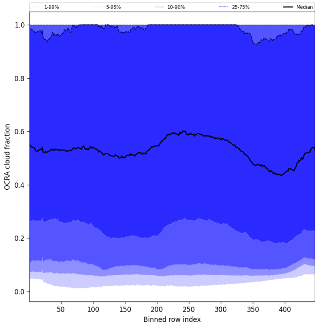
Figure 64: Along track statistics of “OCRA cloud fraction” for 2025-02-05 to 2025-02-06
