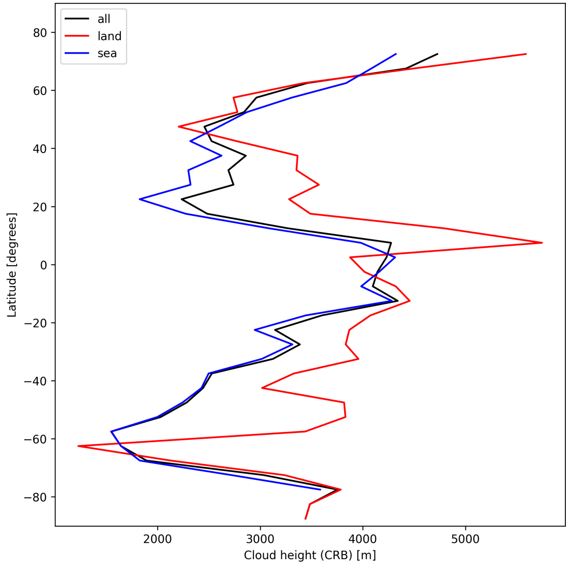
Figure 25: Zonal average of “Cloud height (CRB)” for 2025-02-05 to 2025-02-06.
