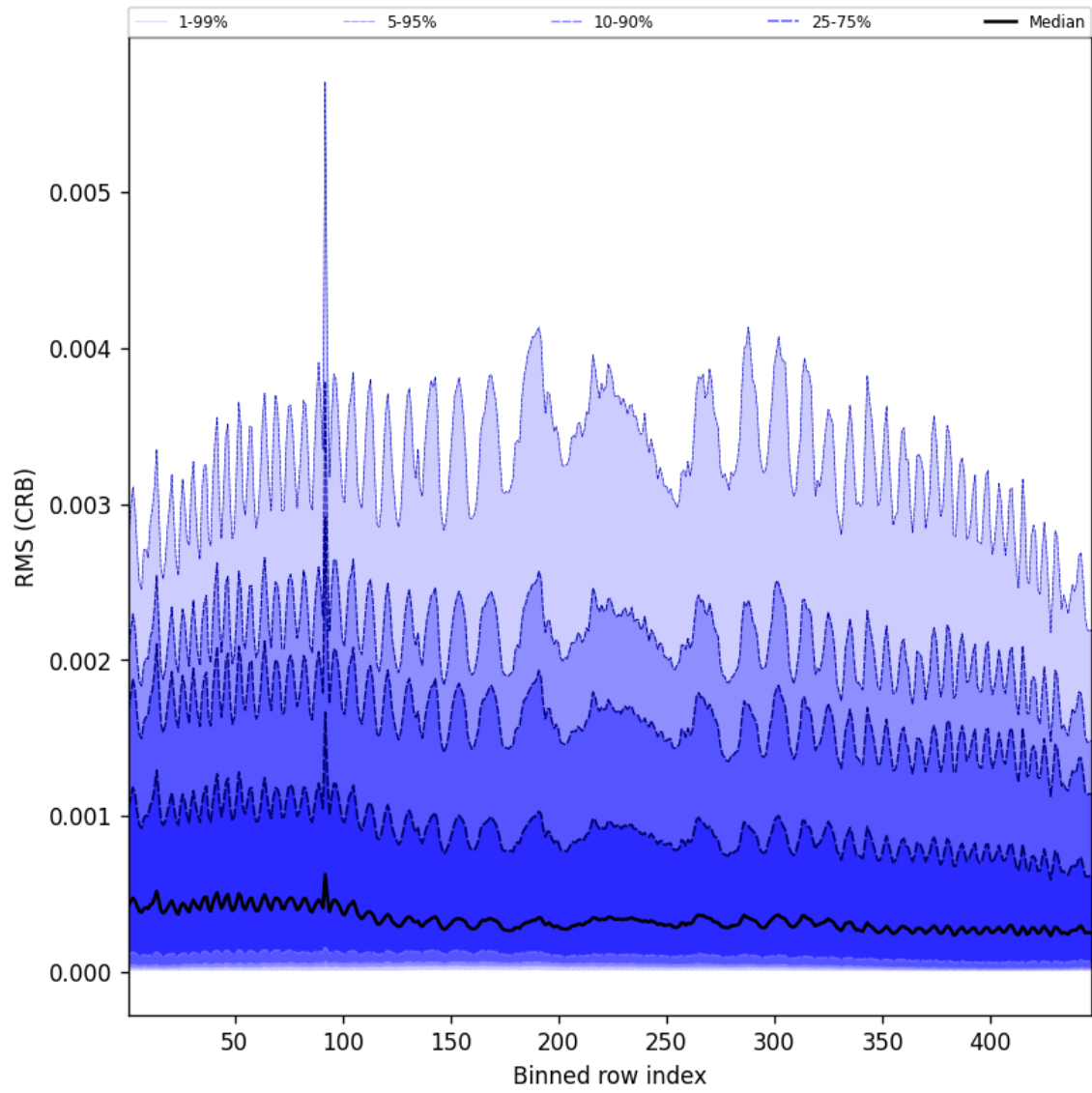
Figure 62: Along track statistics of “RMS (CRB)” for 2025-02-05 to 2025-02-06
