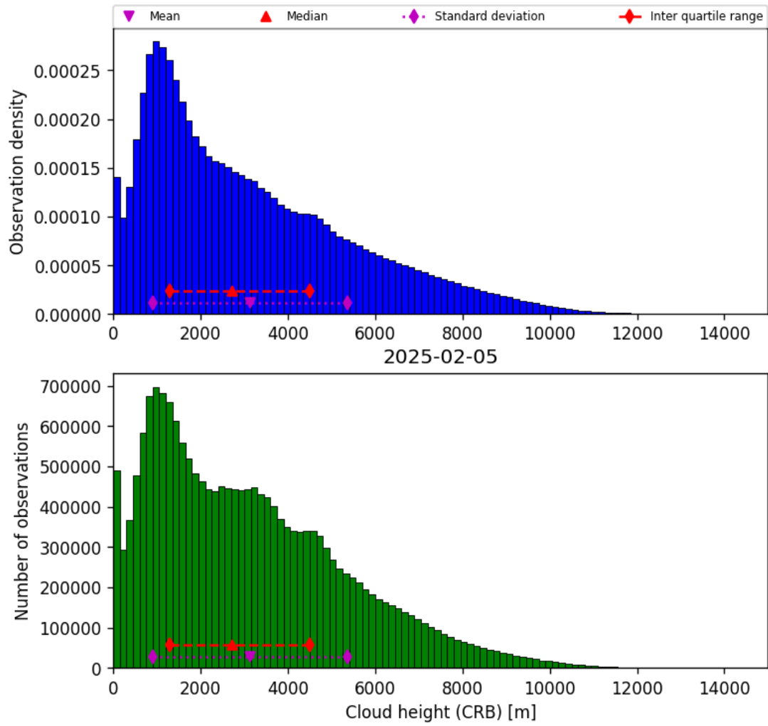
Figure 41: Histogram of “Cloud height (CRB)” for 2025-02-05 to 2025-02-06
