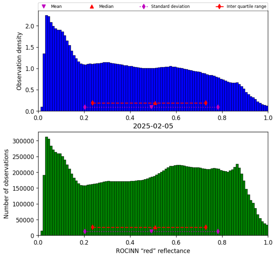
Figure 51: Histogram of “ROCINN “red” reflectance” for 2025-02-05 to 2025-02-06
