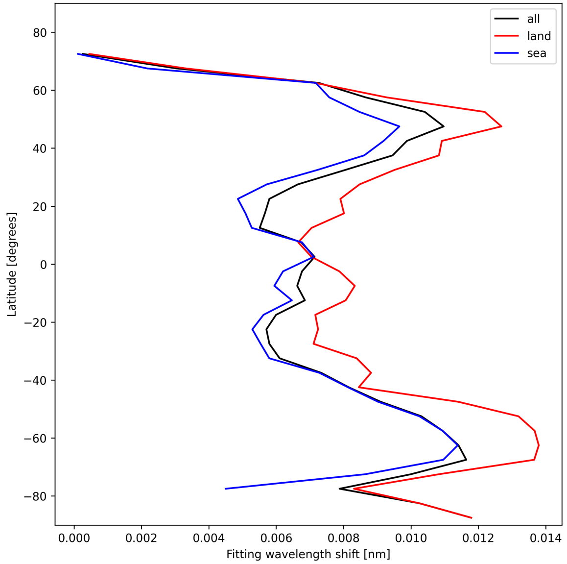
Figure 31: Zonal average of “Fitting wavelength shift” for 2025-02-05 to 2025-02-06.
