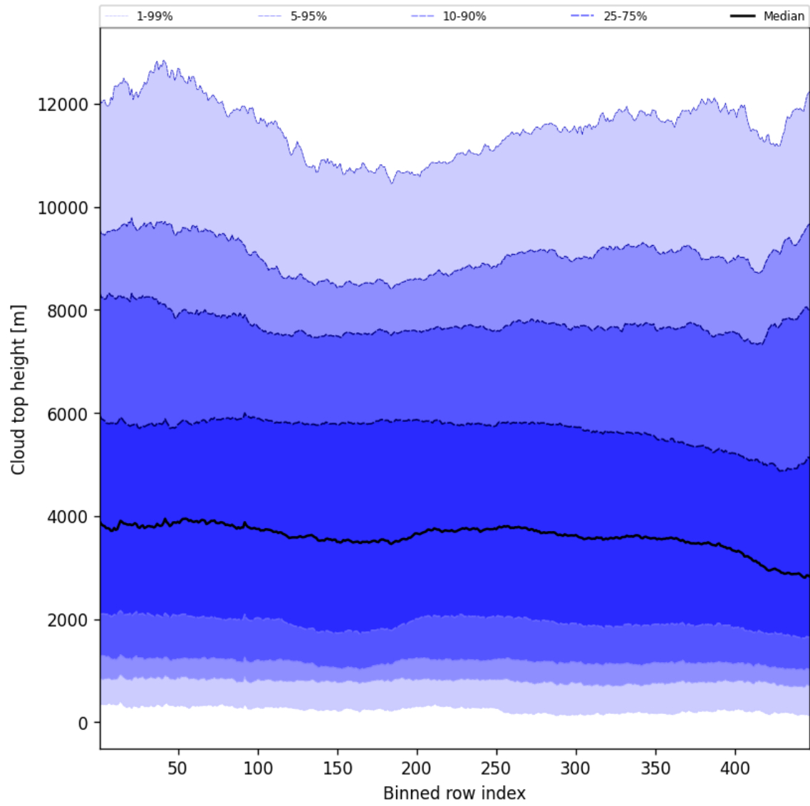
Figure 54: Along track statistics of “Cloud top height” for 2025-02-05 to 2025-02-06
