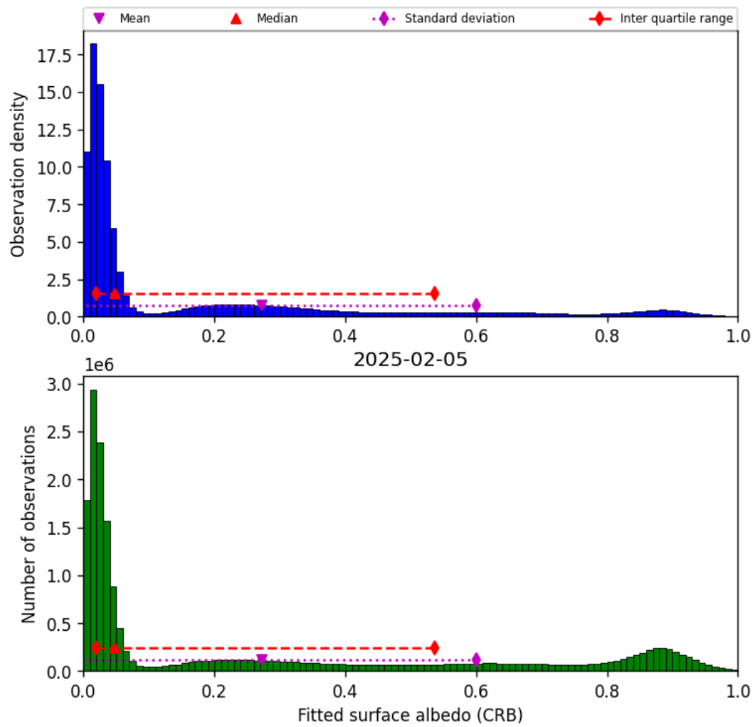
Figure 44: Histogram of “Fitted surface albedo (CRB)” for 2025-02-05 to 2025-02-06
