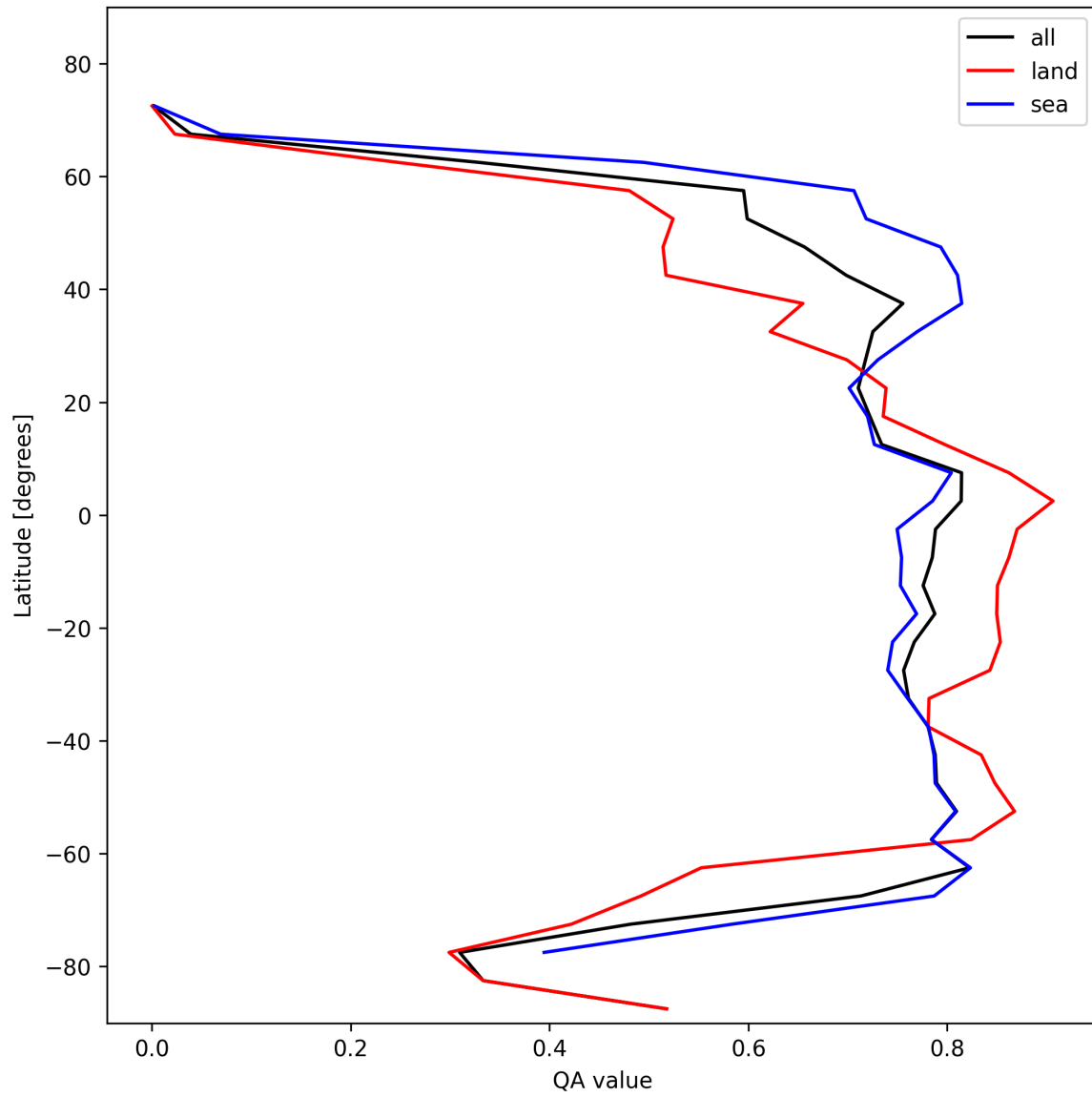
Figure 20: Zonal average of “QA value” for 2025-02-05 to 2025-02-06.
