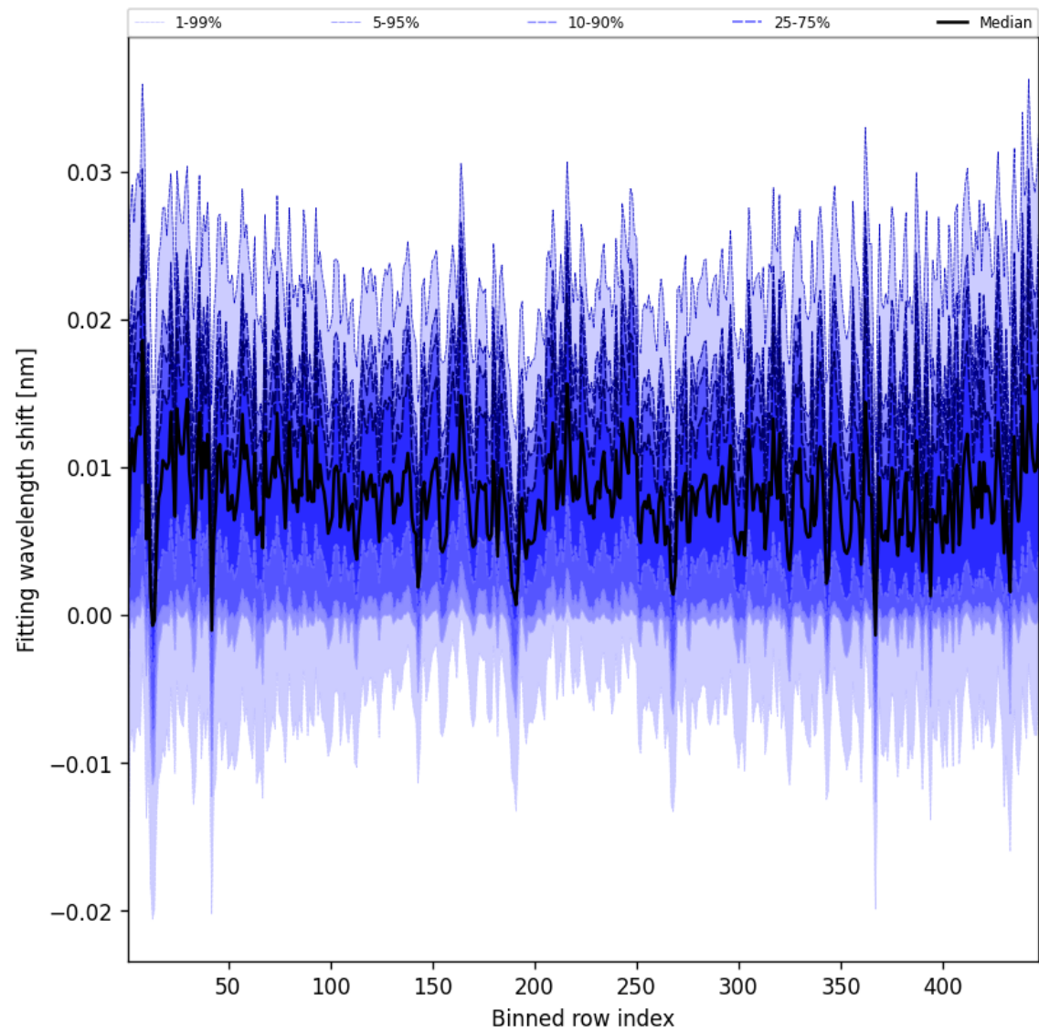
Figure 63: Along track statistics of “Fitting wavelength shift” for 2025-02-05 to 2025-02-06
