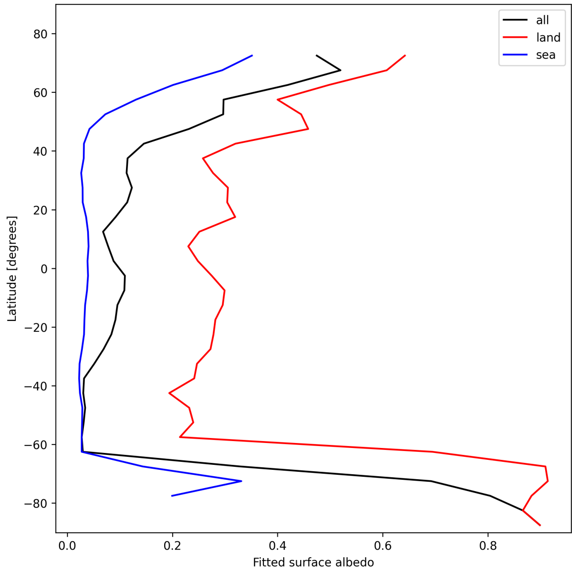
Figure 27: Zonal average of “Fitted surface albedo” for 2025-02-05 to 2025-02-06.
