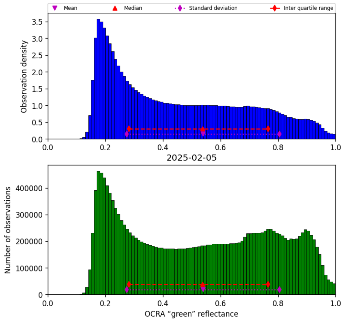
Figure 50: Histogram of “OCRA “green” reflectance” for 2025-02-05 to 2025-02-06
