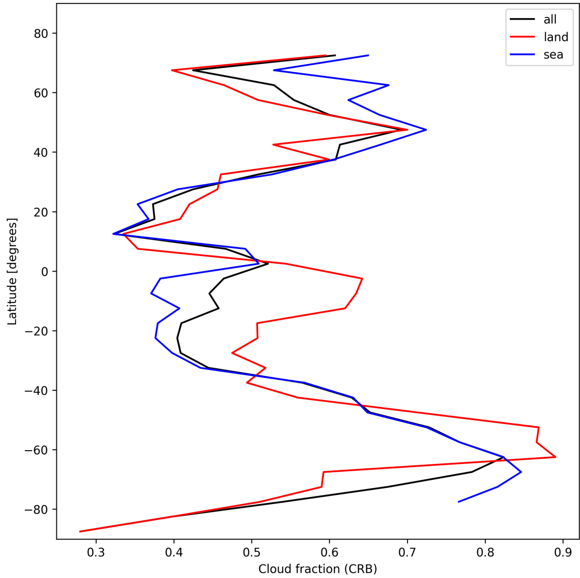
Figure 24: Zonal average of “Cloud fraction (CRB)” for 2025-02-05 to 2025-02-06.
