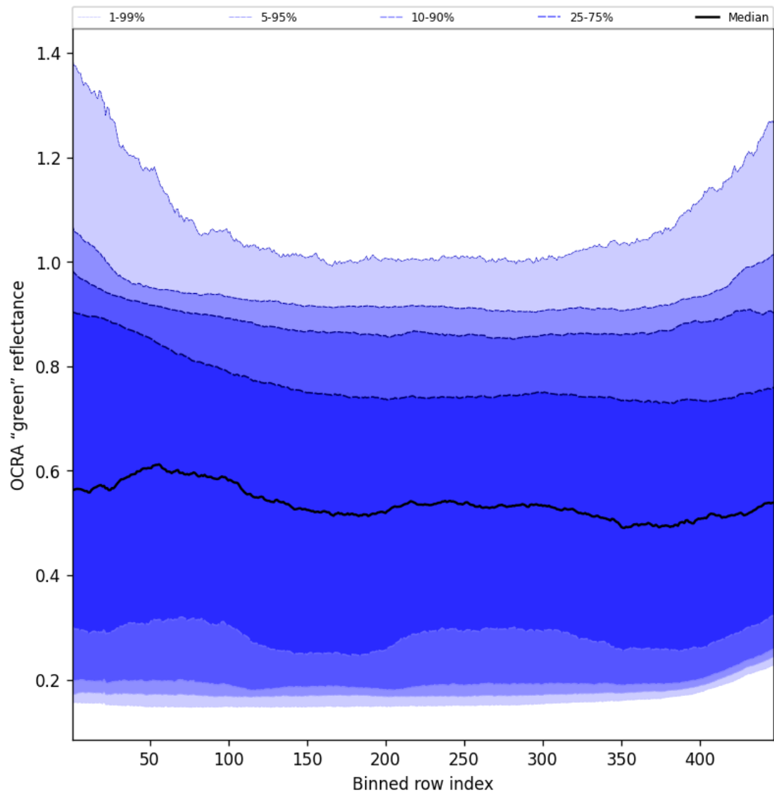
Figure 66: Along track statistics of “OCRA “green” reflectance” for 2025-02-05 to 2025-02-06
