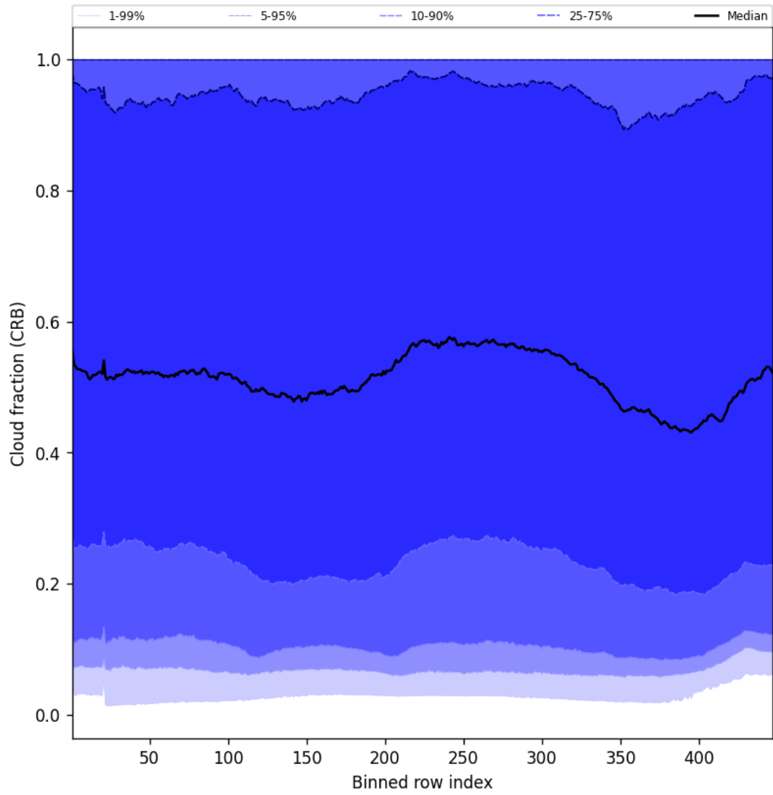
Figure 56: Along track statistics of “Cloud fraction (CRB)” for 2025-02-05 to 2025-02-06
