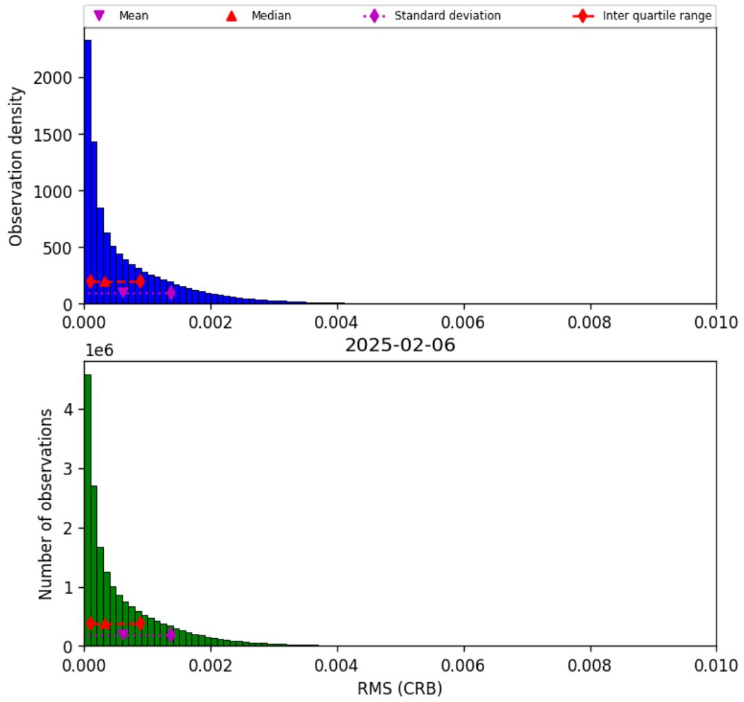
Figure 46: Histogram of “RMS (CRB)” for 2025-02-06 to 2025-02-06
