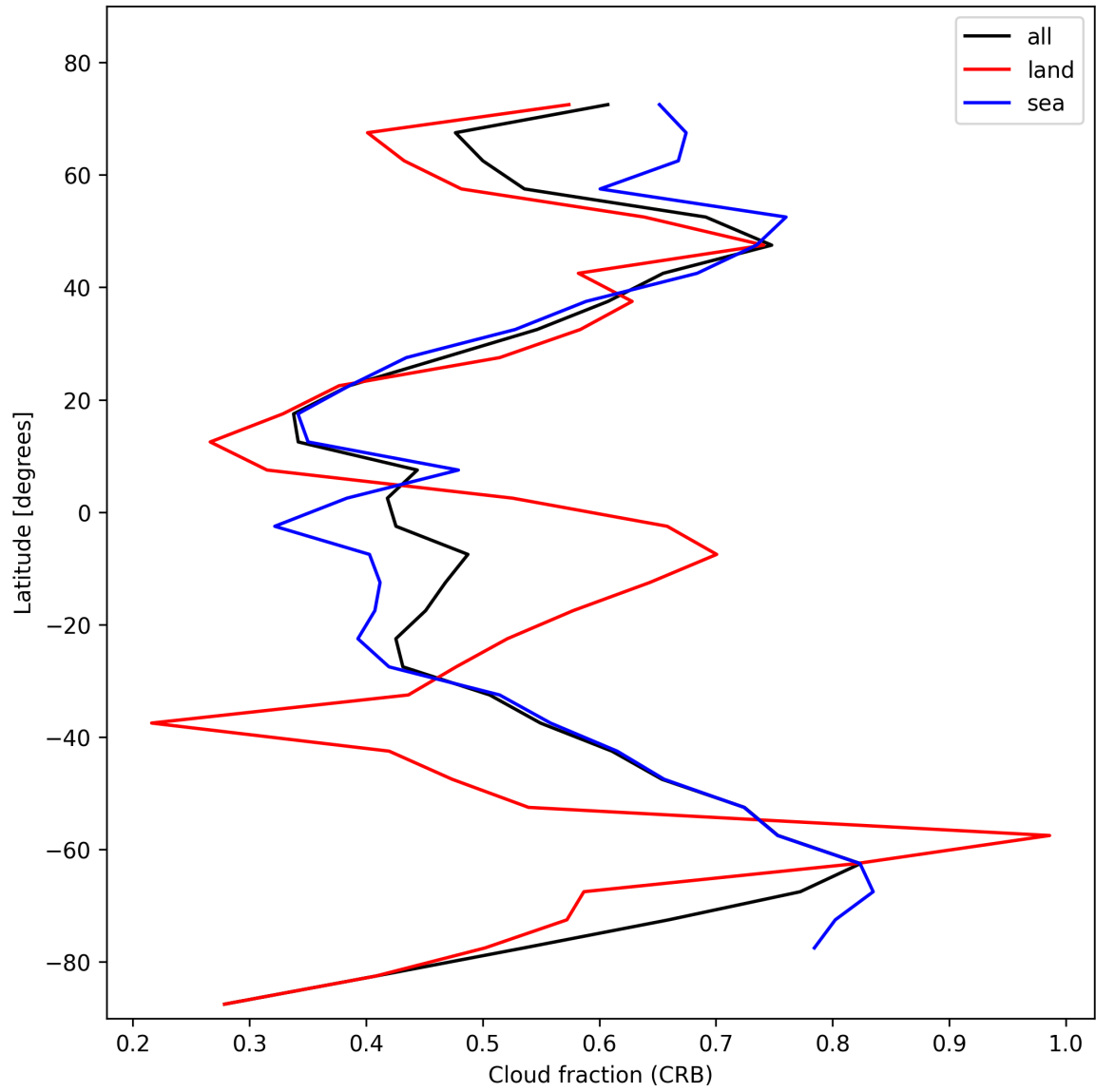
Figure 24: Zonal average of “Cloud fraction (CRB)” for 2025-02-06 to 2025-02-06.
