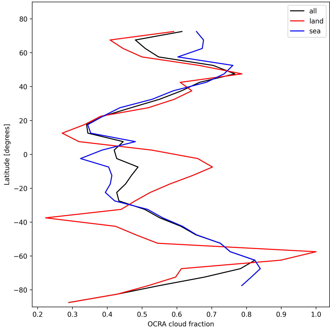
Figure 32: Zonal average of “OCRA cloud fraction” for 2025-02-06 to 2025-02-06.
