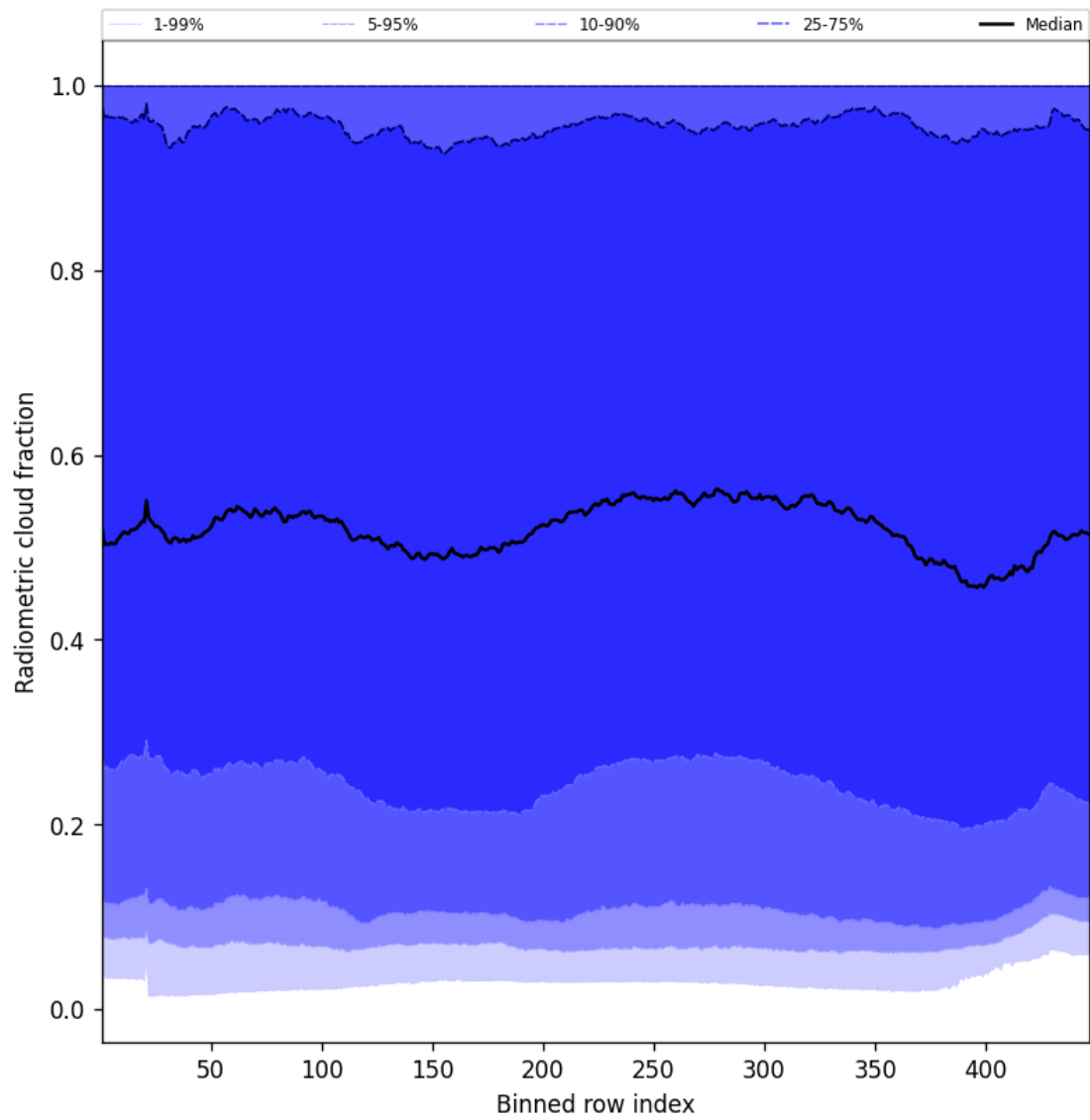
Figure 53: Along track statistics of “Radiometric cloud fraction” for 2025-02-06 to 2025-02-06
