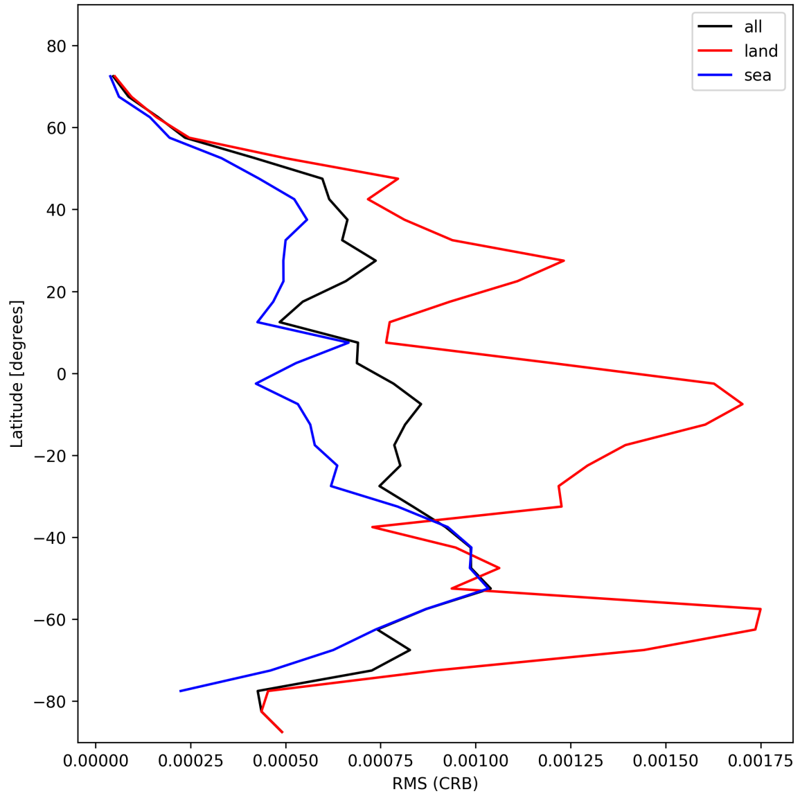
Figure 30: Zonal average of “RMS (CRB)” for 2025-02-06 to 2025-02-06.
