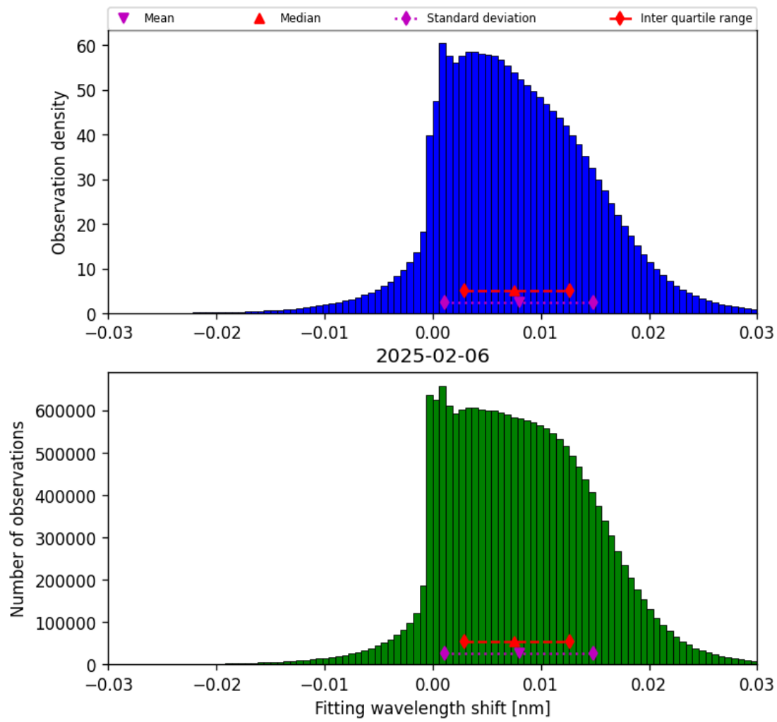
Figure 47: Histogram of “Fitting wavelength shift” for 2025-02-06 to 2025-02-06
