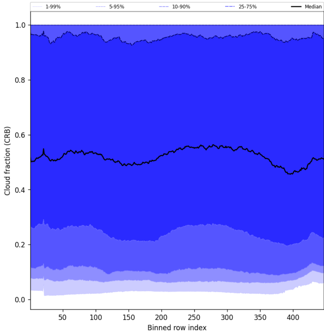
Figure 56: Along track statistics of “Cloud fraction (CRB)” for 2025-02-06 to 2025-02-06
