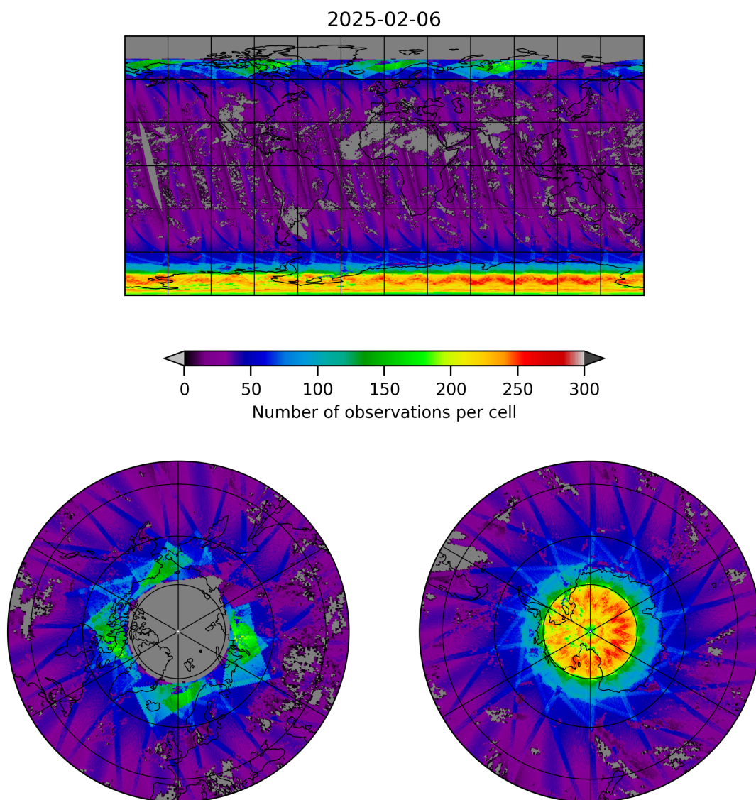
Figure 19: Map of the number of observations for 2025-02-06 to 2025-02-06
