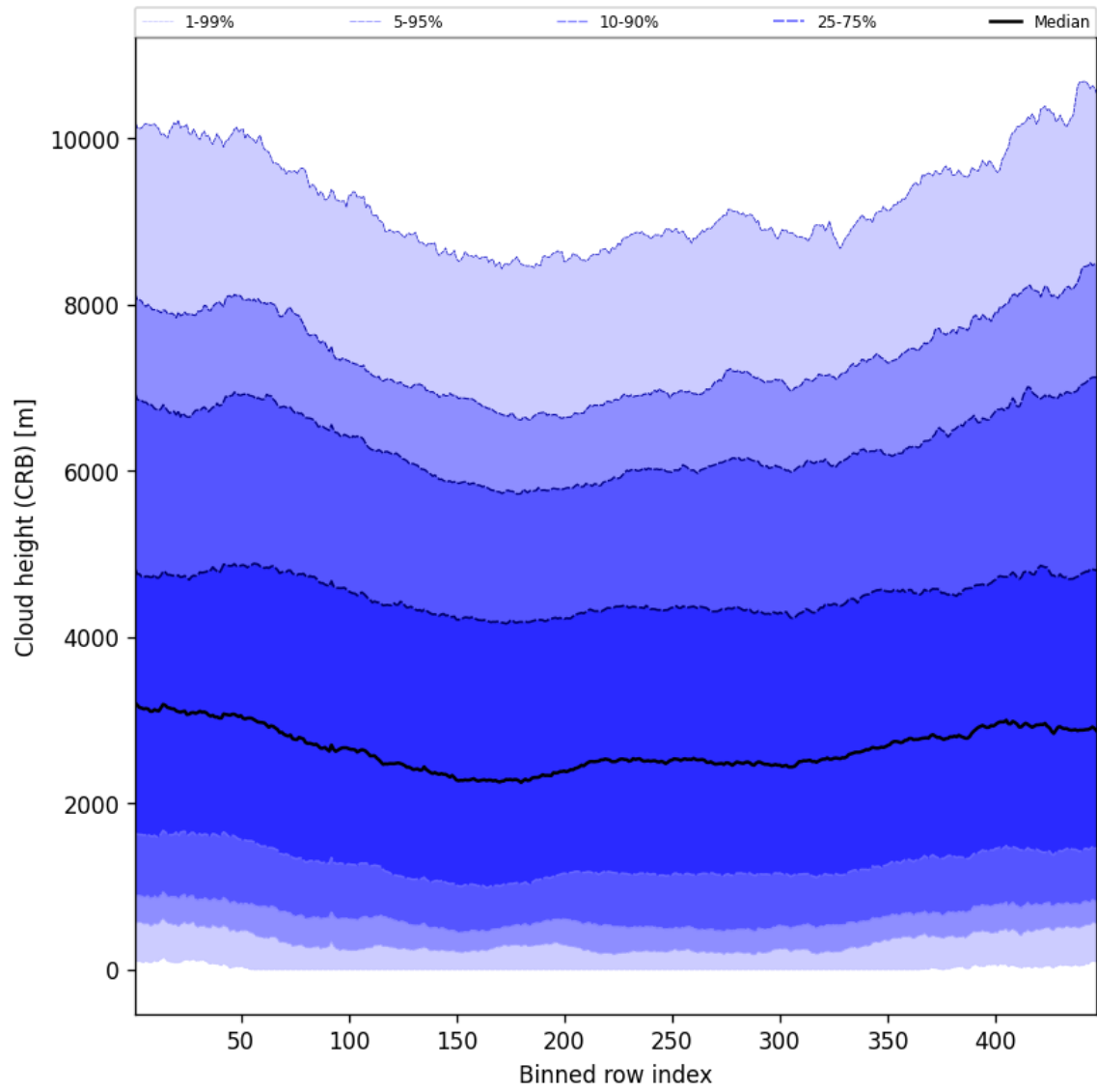
Figure 57: Along track statistics of “Cloud height (CRB)” for 2025-02-06 to 2025-02-06
