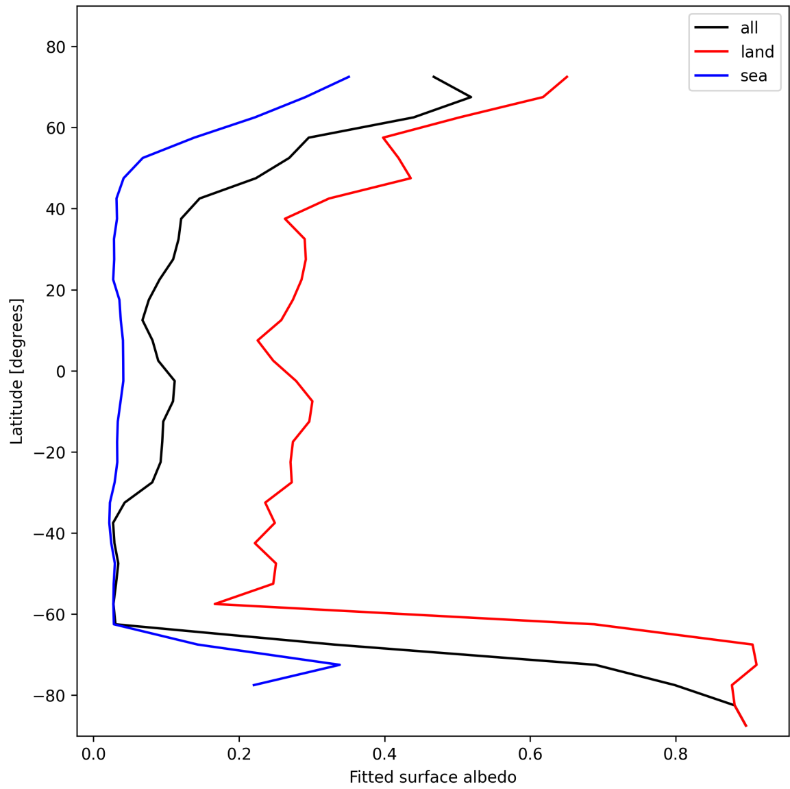
Figure 27: Zonal average of “Fitted surface albedo” for 2025-02-06 to 2025-02-06.
