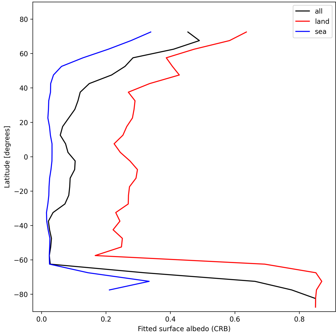
Figure 28: Zonal average of “Fitted surface albedo (CRB)” for 2025-02-06 to 2025-02-06.
