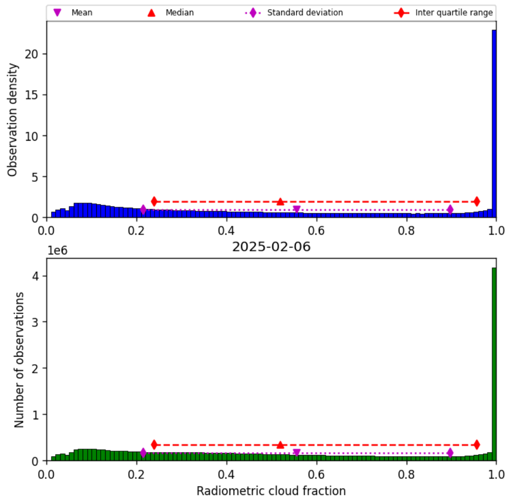
Figure 37: Histogram of “Radiometric cloud fraction” for 2025-02-06 to 2025-02-06
