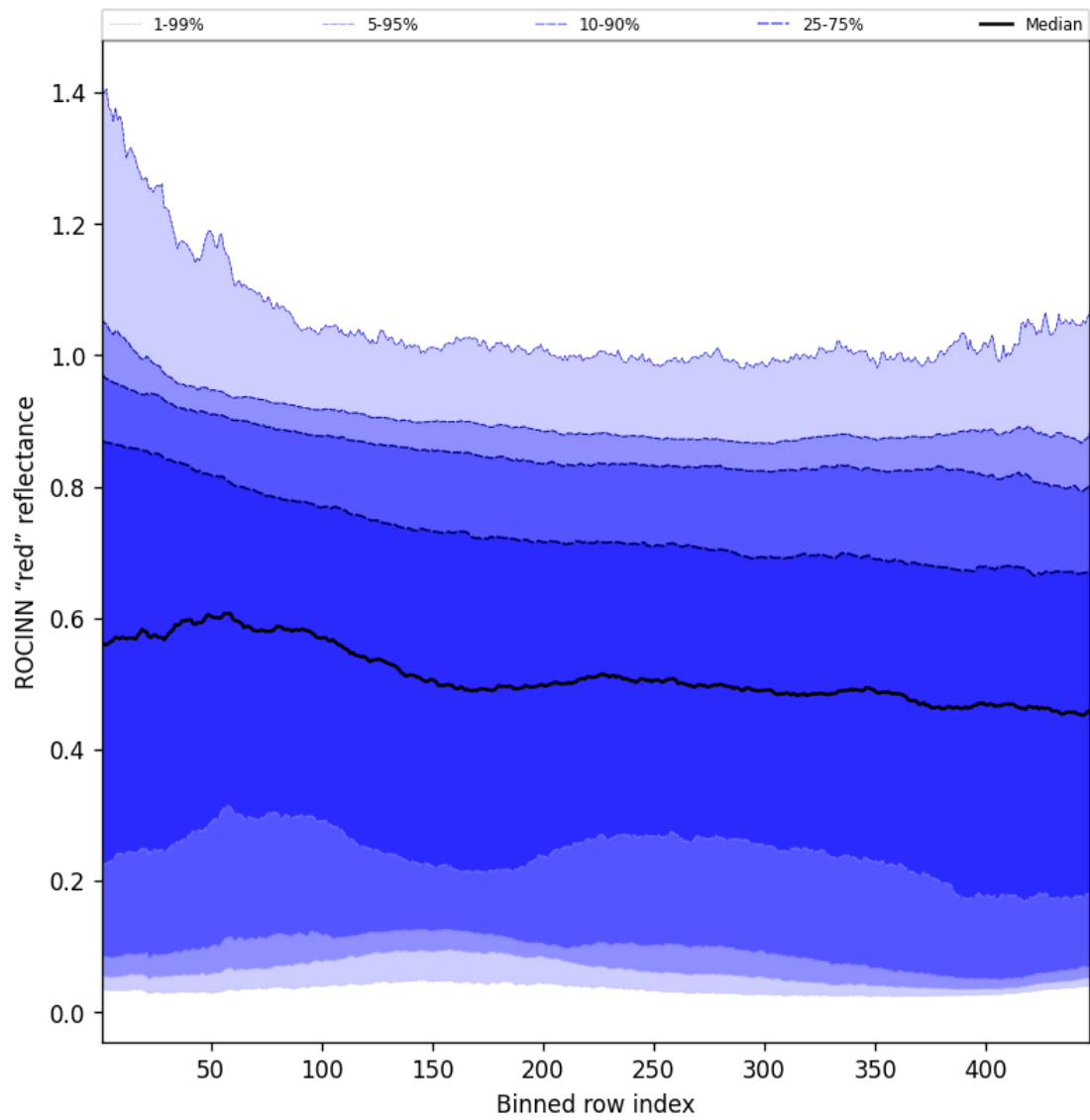
Figure 67: Along track statistics of "ROCINN "red" reflectance" for 2025-02-06 to 2025-02-06
