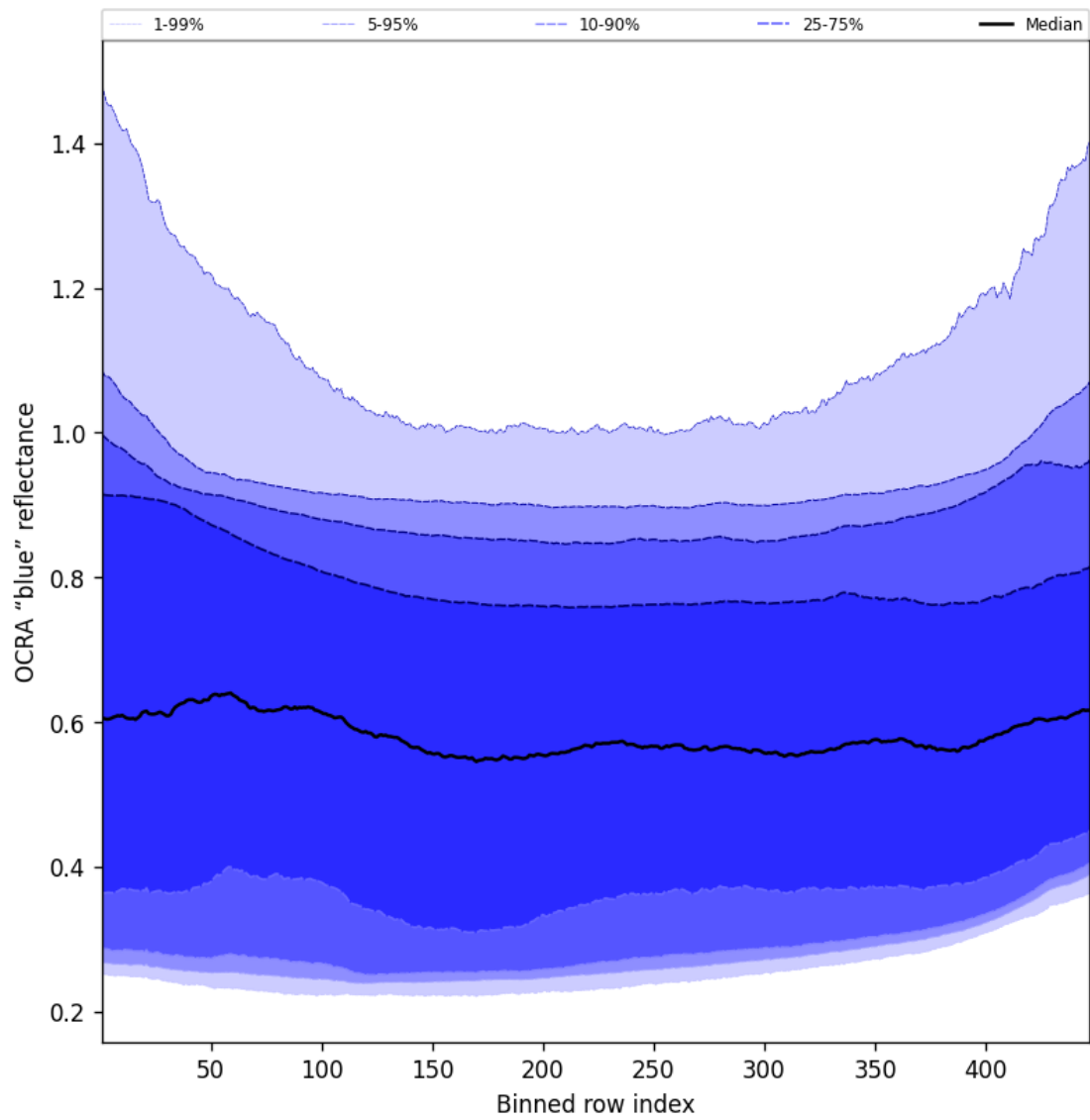
Figure 65: Along track statistics of “OCRA “blue” reflectance” for 2025-02-06 to 2025-02-06
