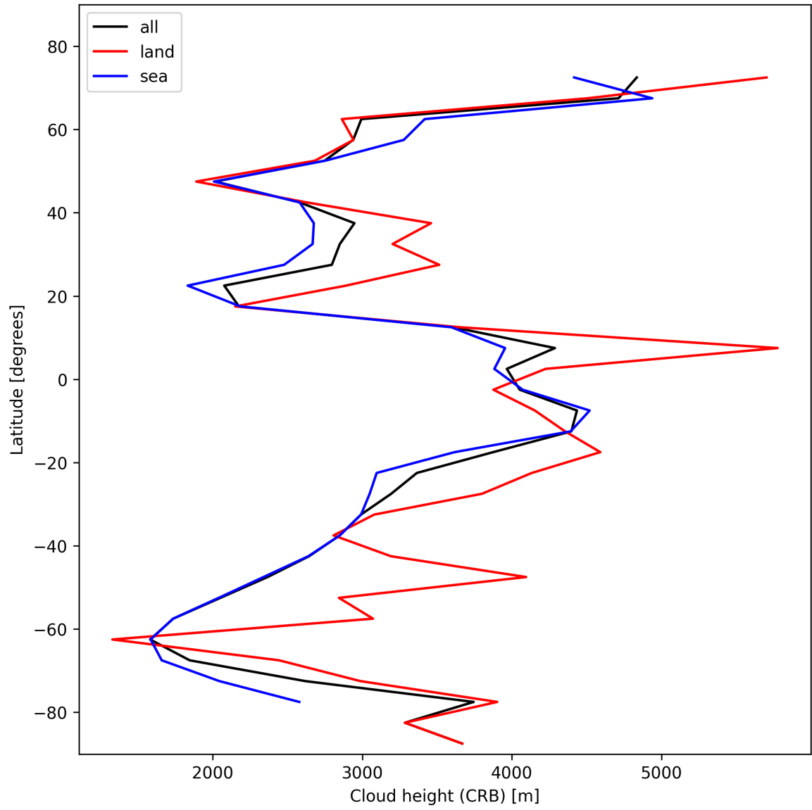
Figure 25: Zonal average of “Cloud height (CRB)” for 2025-02-06 to 2025-02-06.
