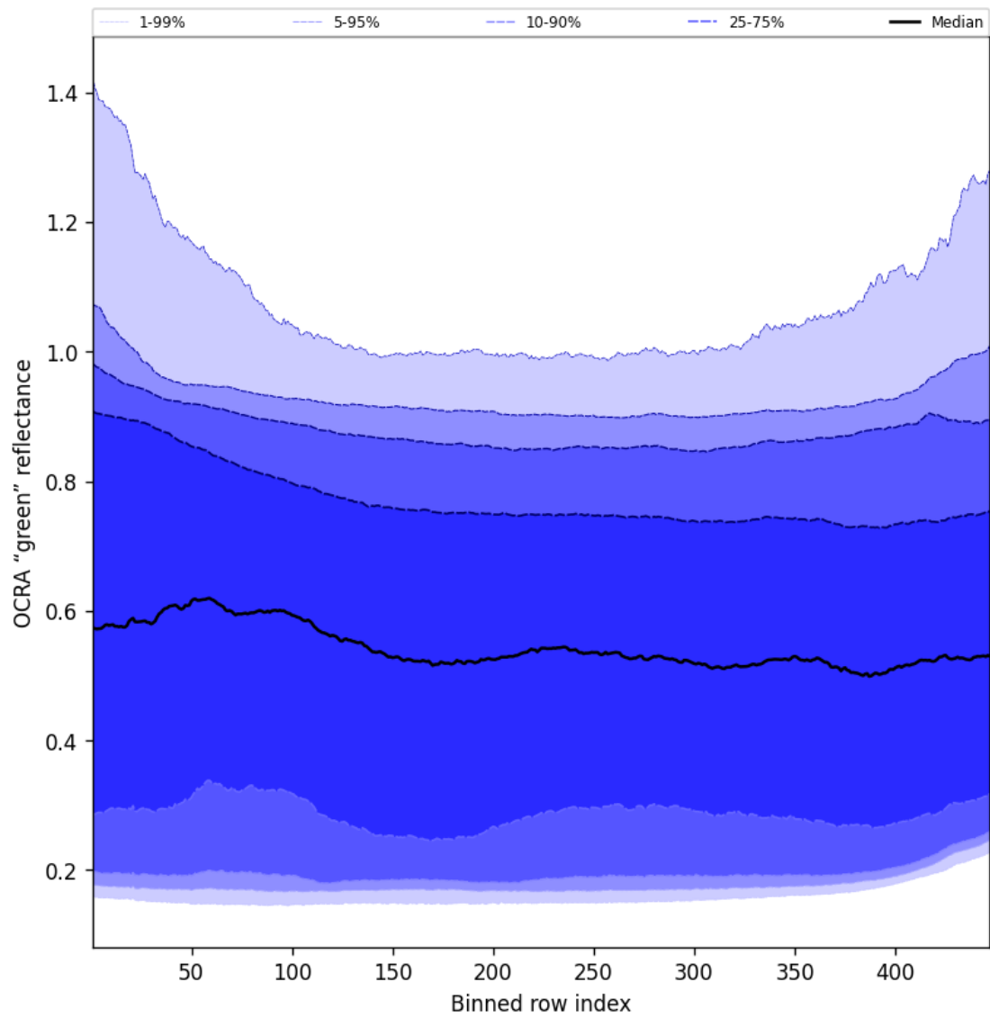
Figure 66: Along track statistics of "OCRA "green" reflectance" for 2025-02-06 to 2025-02-06
