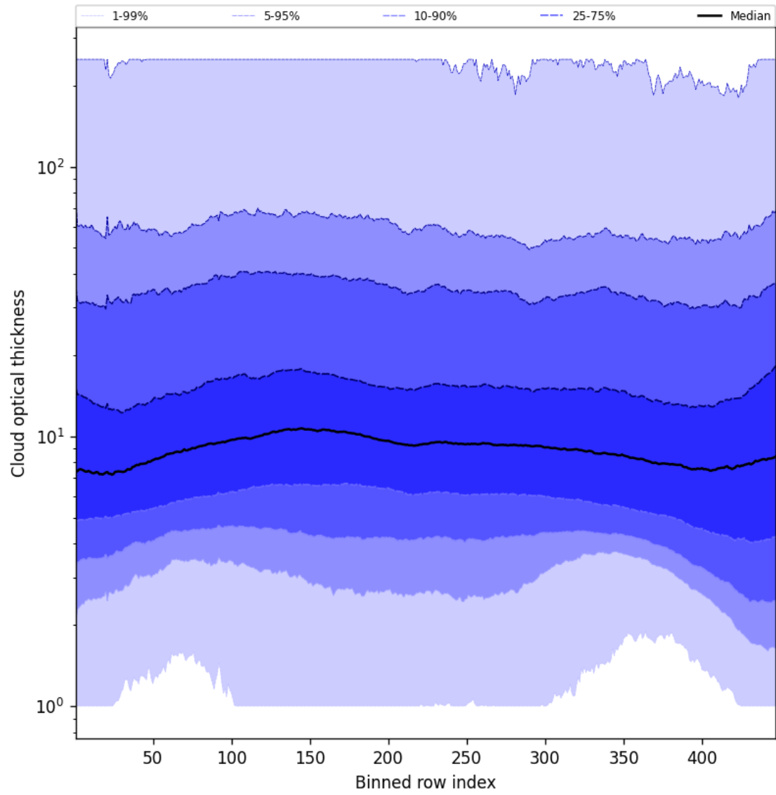
Figure 55: Along track statistics of “Cloud optical thickness” for 2025-02-06 to 2025-02-06
