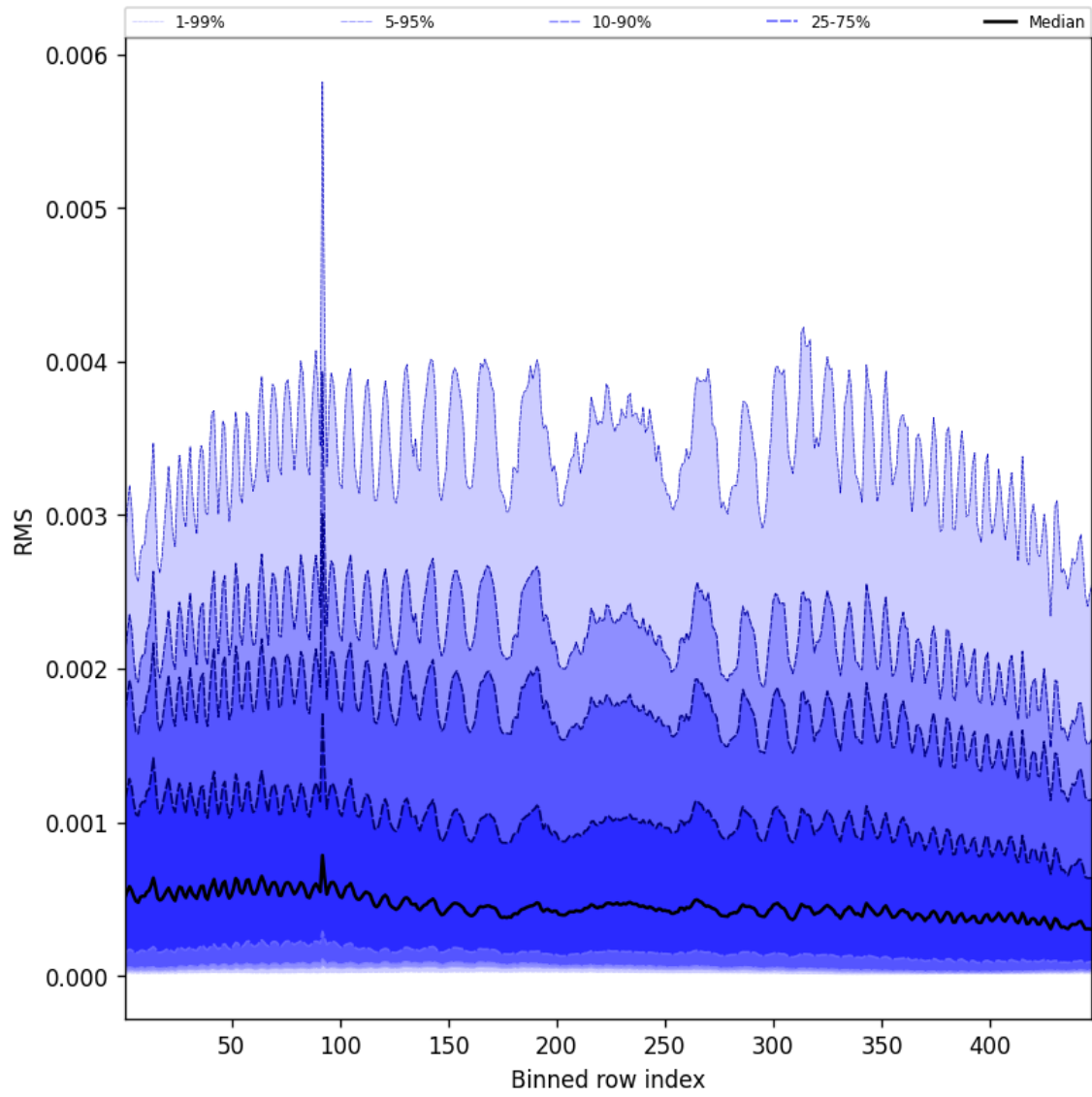
Figure 61: Along track statistics of “RMS” for 2025-02-06 to 2025-02-06
