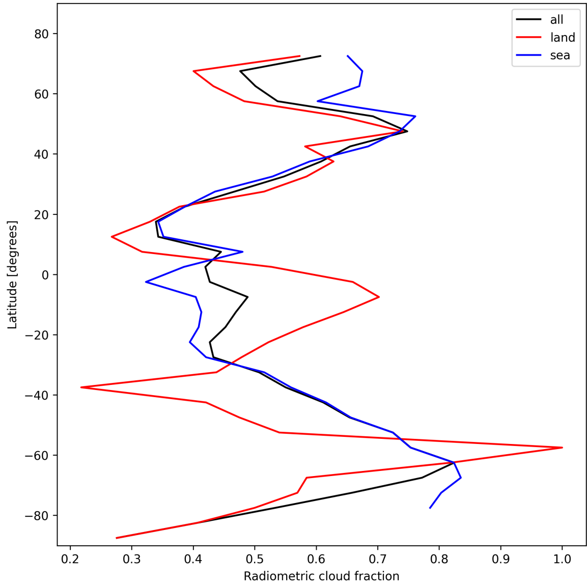
Figure 21: Zonal average of “Radiometric cloud fraction” for 2025-02-06 to 2025-02-06.
