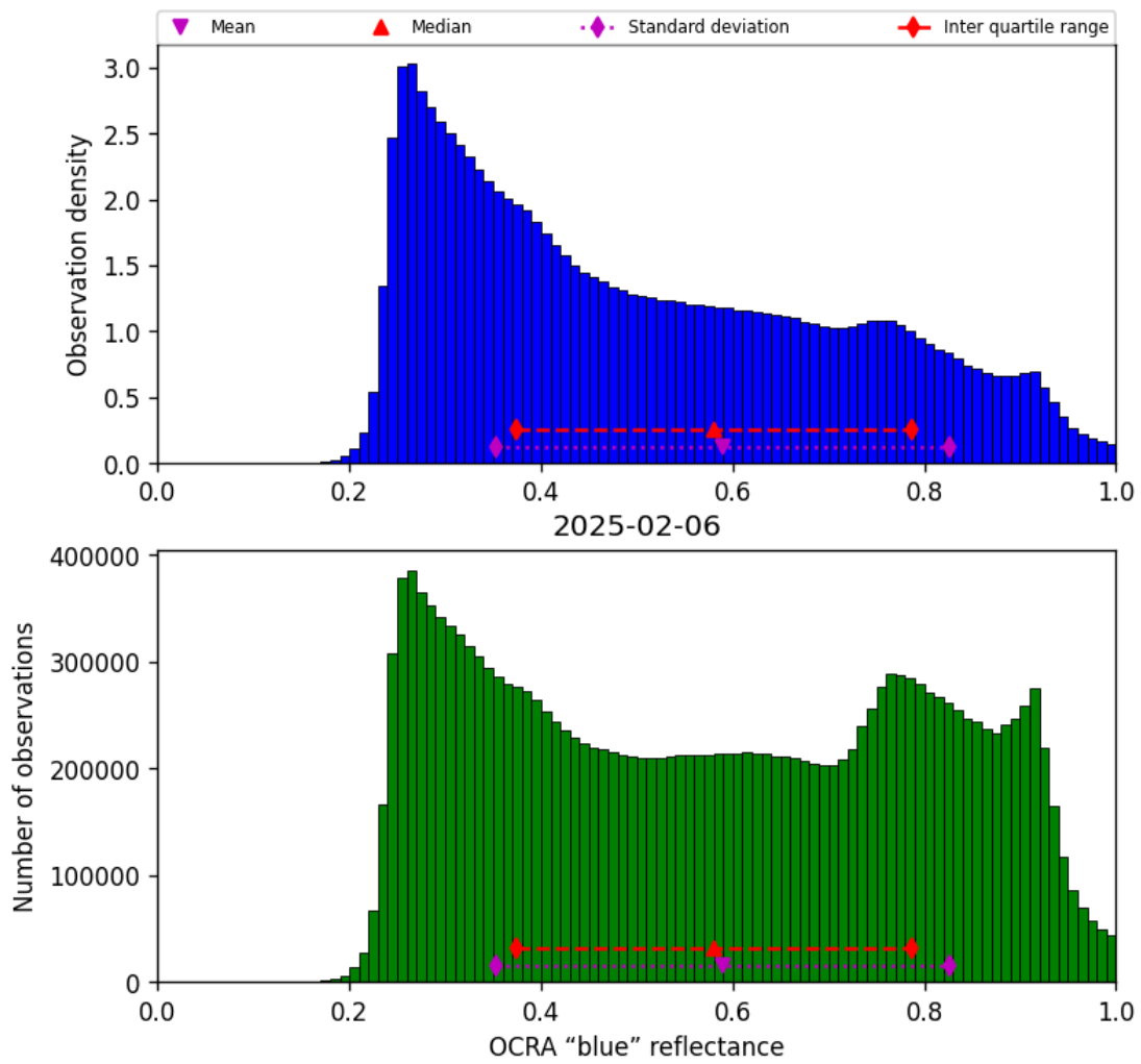
Figure 49: Histogram of “OCRA “blue” reflectance” for 2025-02-06 to 2025-02-06
