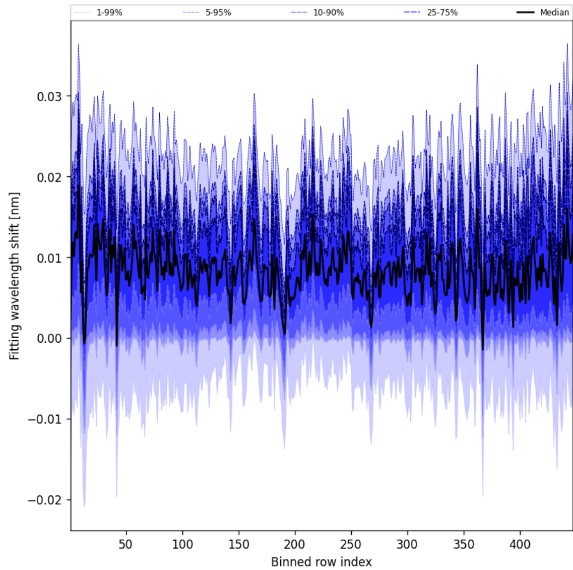
Figure 63: Along track statistics of “Fitting wavelength shift” for 2025-02-06 to 2025-02-06
