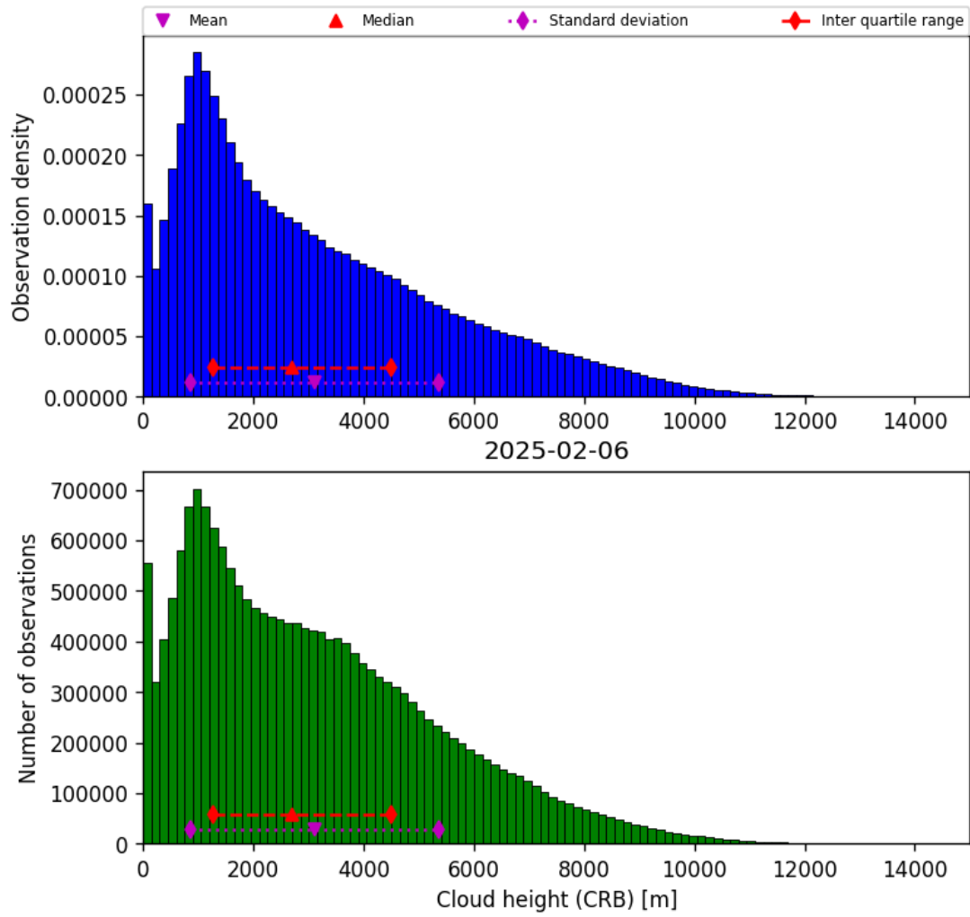
Figure 41: Histogram of “Cloud height (CRB)” for 2025-02-06 to 2025-02-06
