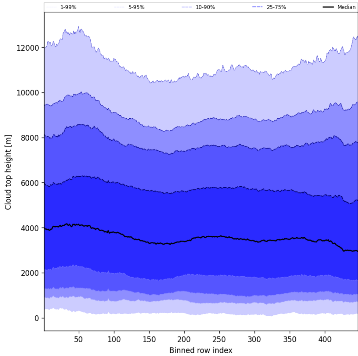
Figure 54: Along track statistics of “Cloud top height” for 2025-02-06 to 2025-02-06
