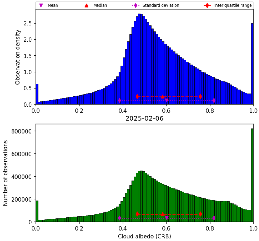
Figure 42: Histogram of “Cloud albedo (CRB)” for 2025-02-06 to 2025-02-06
