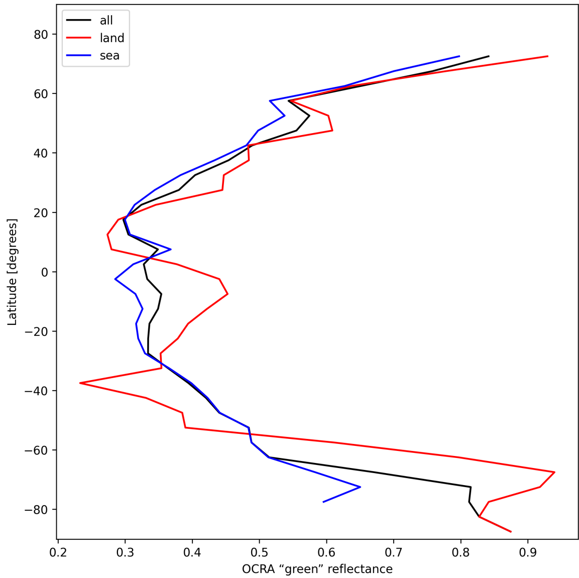
Figure 34: Zonal average of “OCRA “green” reflectance” for 2025-02-06 to 2025-02-06.
