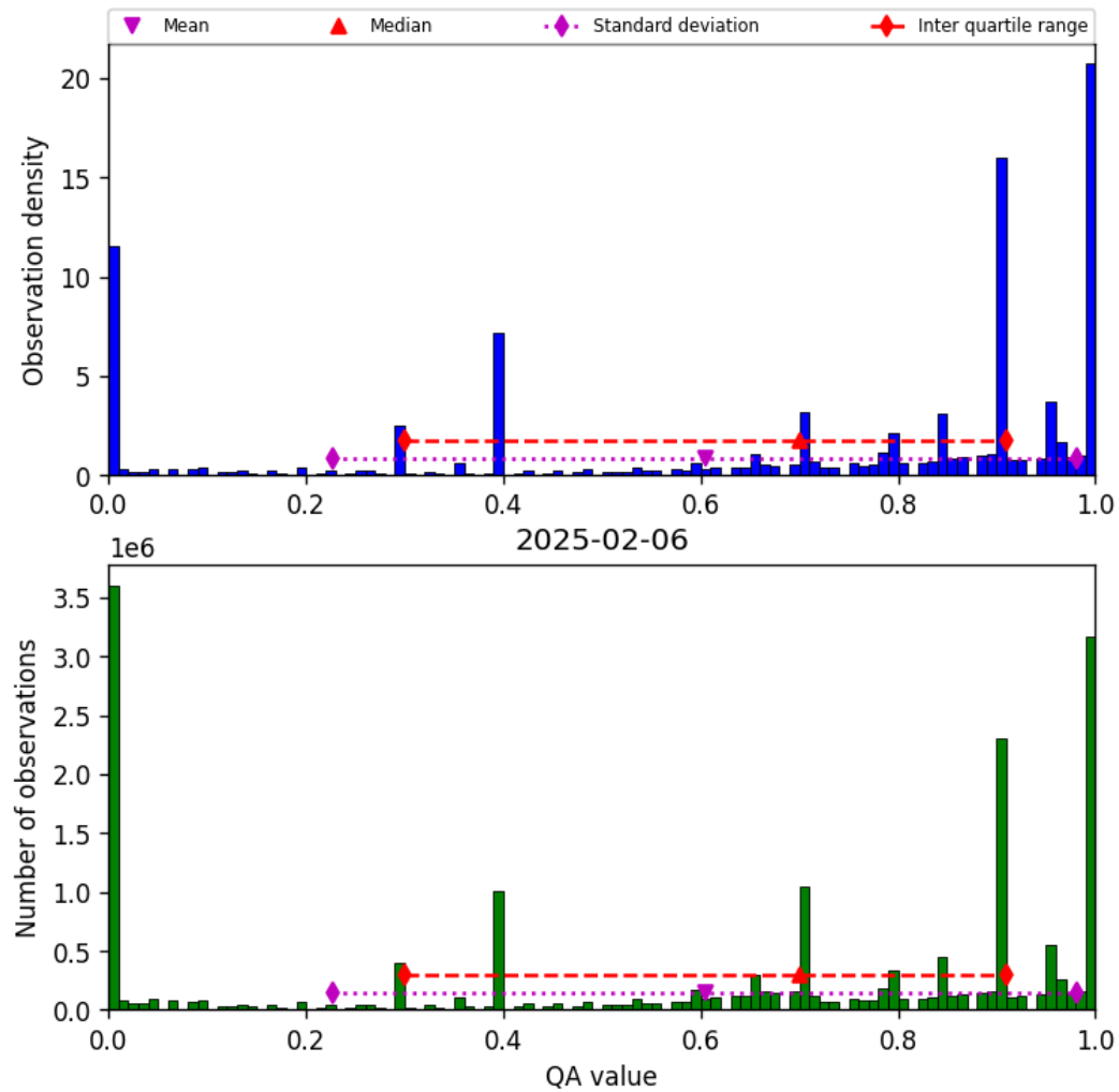
Figure 36: Histogram of “QA value” for 2025-02-06 to 2025-02-06
