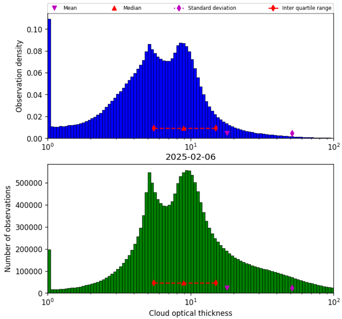
Figure 39: Histogram of “Cloud optical thickness” for 2025-02-06 to 2025-02-06
