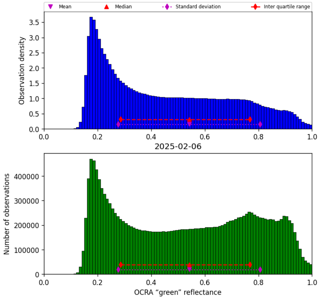
Figure 50: Histogram of “OCRA “green” reflectance” for 2025-02-06 to 2025-02-06
