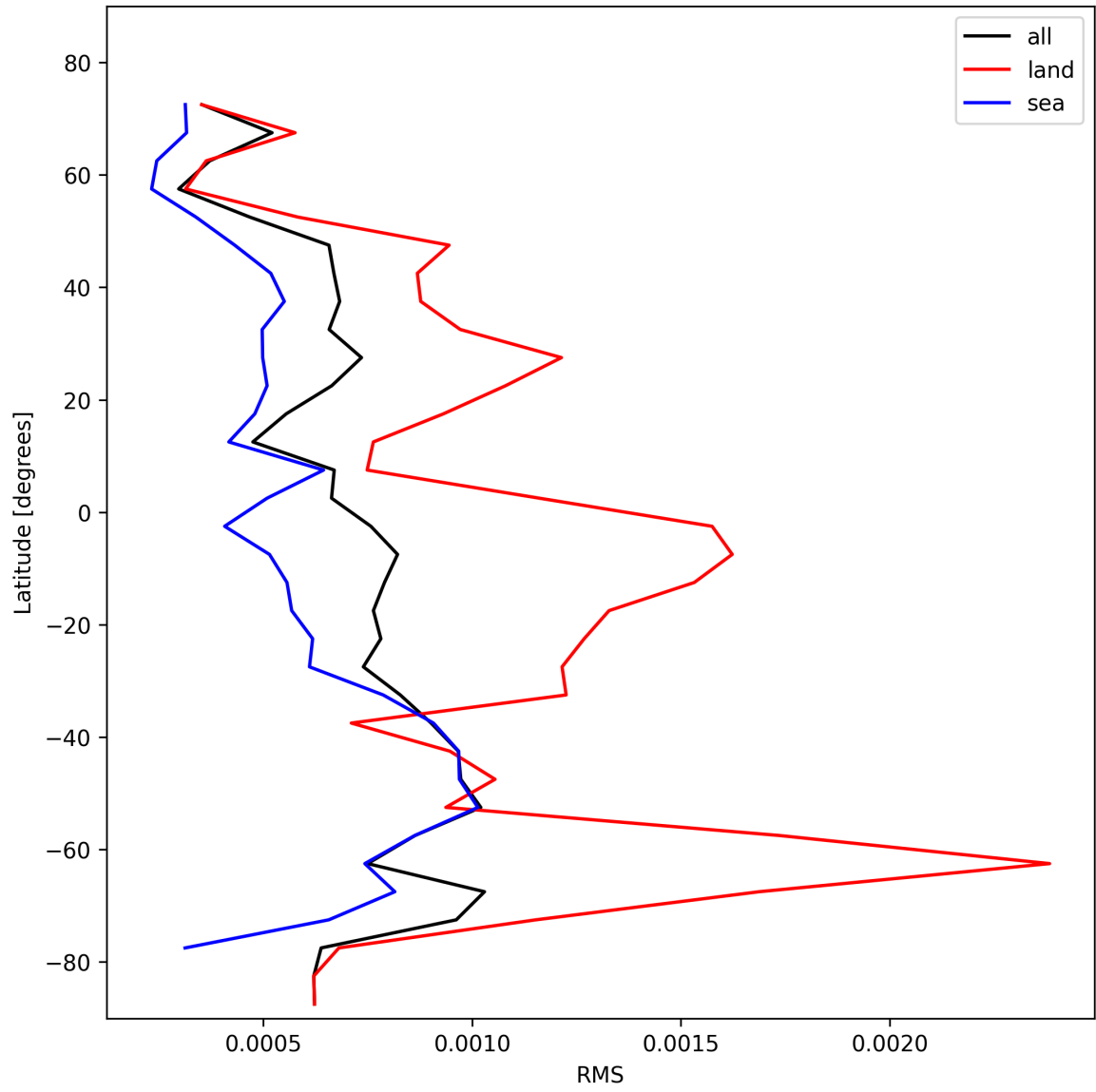
Figure 29: Zonal average of “RMS” for 2025-02-06 to 2025-02-06.
