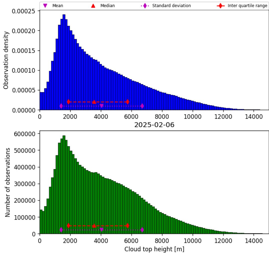
Figure 38: Histogram of “Cloud top height” for 2025-02-06 to 2025-02-06
