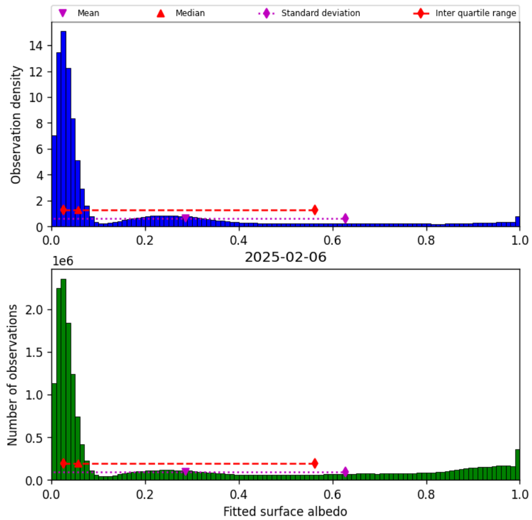
Figure 43: Histogram of “Fitted surface albedo” for 2025-02-06 to 2025-02-06
