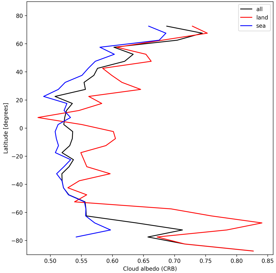
Figure 26: Zonal average of “Cloud albedo (CRB)” for 2025-02-06 to 2025-02-06.
