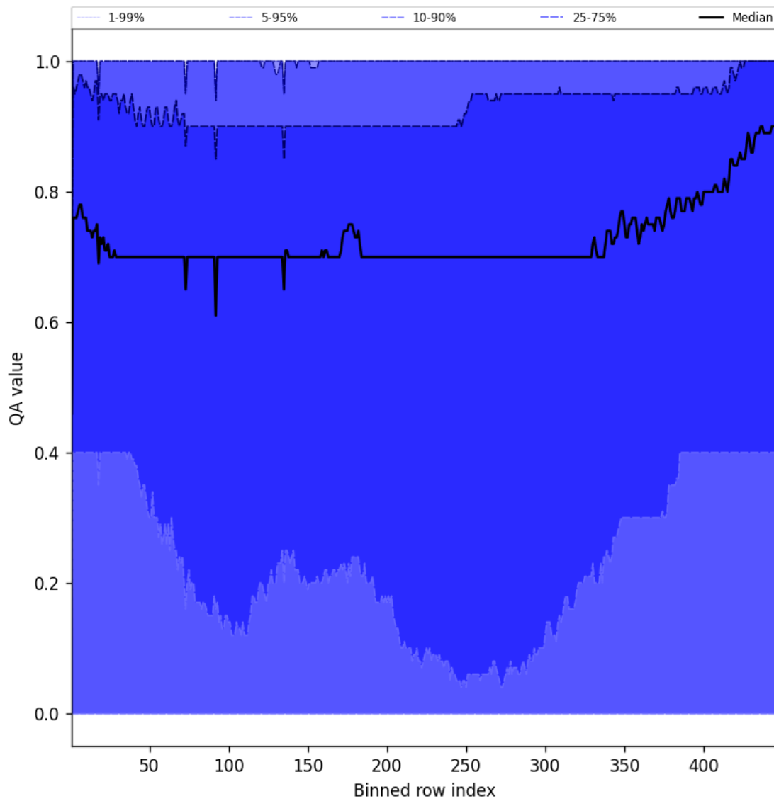
Figure 52: Along track statistics of “QA value” for 2025-02-06 to 2025-02-06
