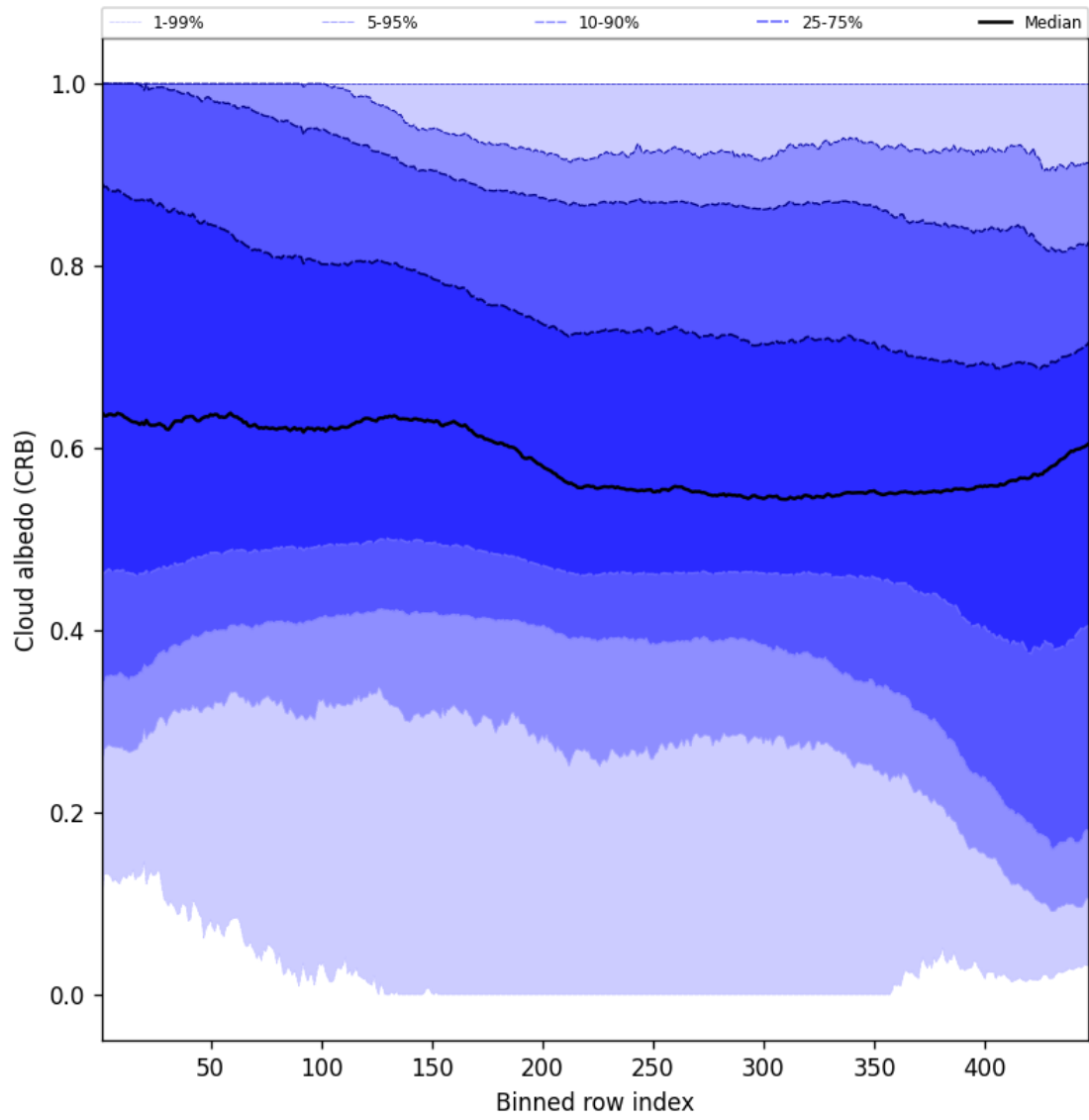
Figure 58: Along track statistics of “Cloud albedo (CRB)” for 2025-02-06 to 2025-02-06
