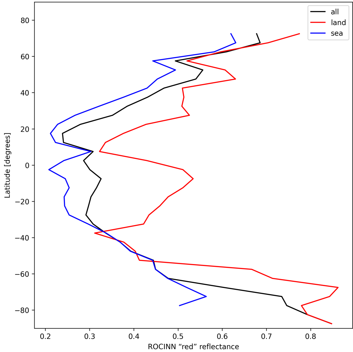
Figure 35: Zonal average of “ROCINN “red” reflectance” for 2025-02-06 to 2025-02-06.
