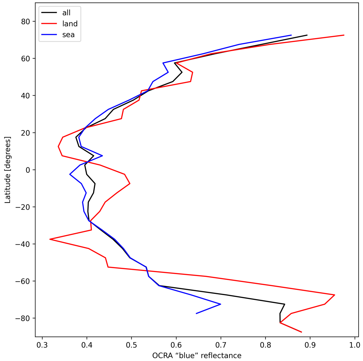
Figure 33: Zonal average of “OCRA “blue” reflectance” for 2025-02-06 to 2025-02-06.
