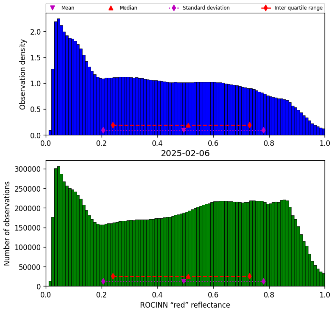
Figure 51: Histogram of “ROCINN “red” reflectance” for 2025-02-06 to 2025-02-06
