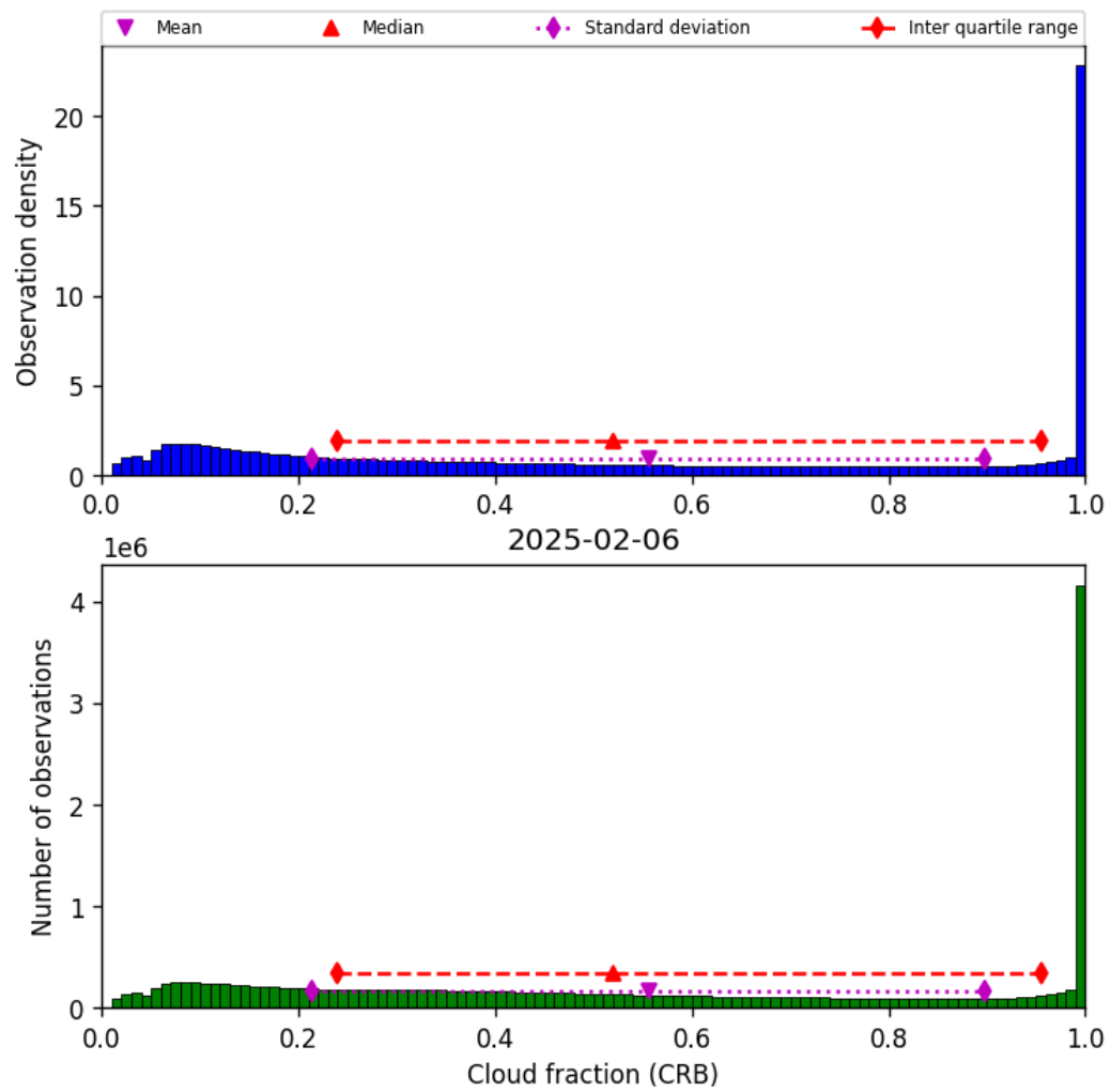
Figure 40: Histogram of “Cloud fraction (CRB)” for 2025-02-06 to 2025-02-06
