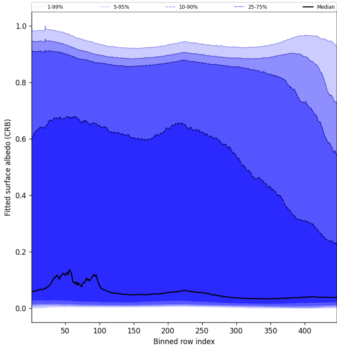
Figure 60: Along track statistics of “Fitted surface albedo (CRB)” for 2025-02-06 to 2025-02-06
