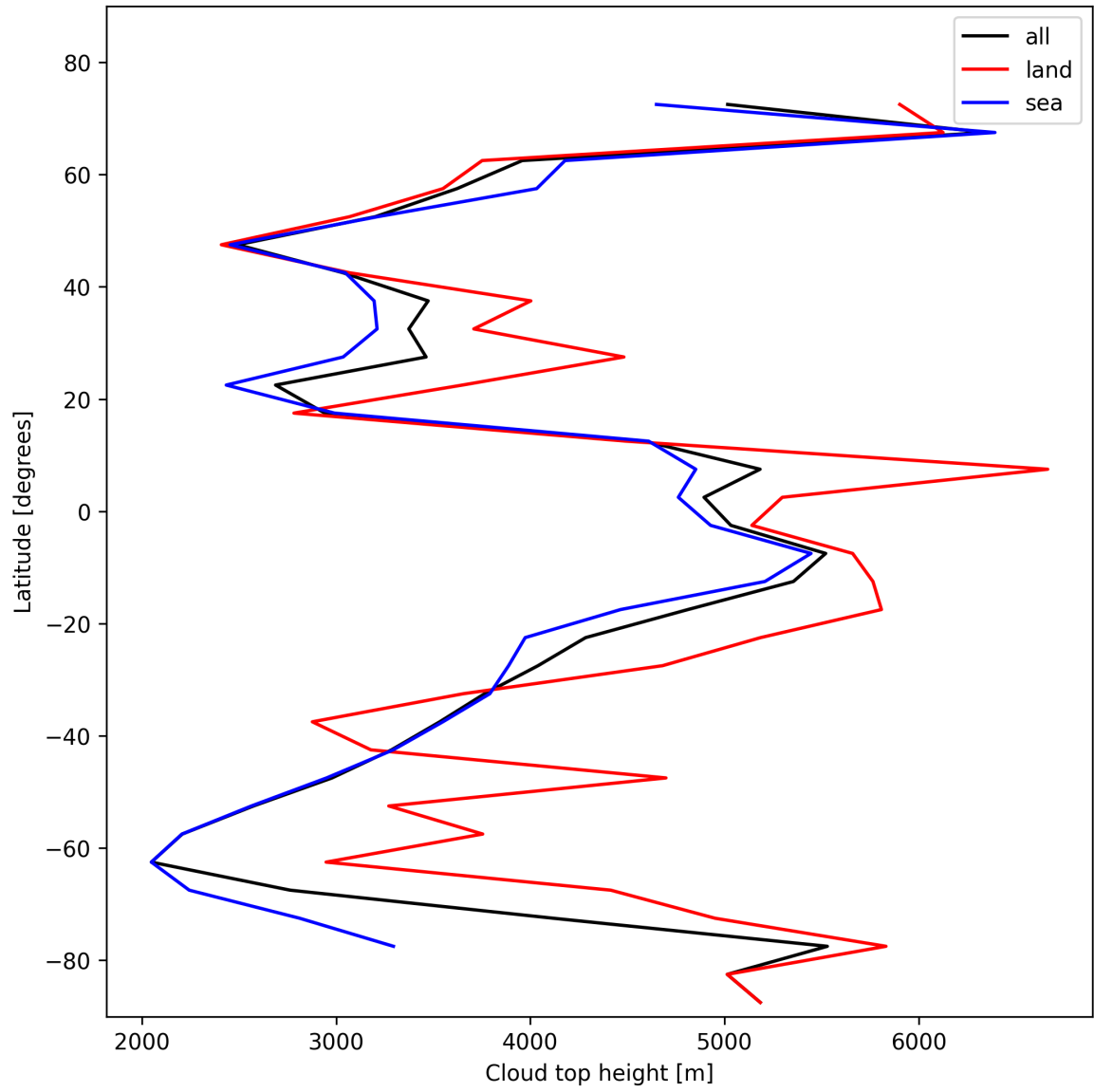
Figure 22: Zonal average of “Cloud top height” for 2025-02-06 to 2025-02-06.
