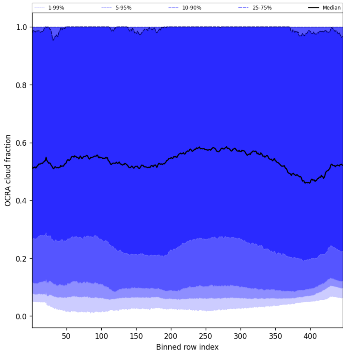
Figure 64: Along track statistics of “OCRA cloud fraction” for 2025-02-06 to 2025-02-06
