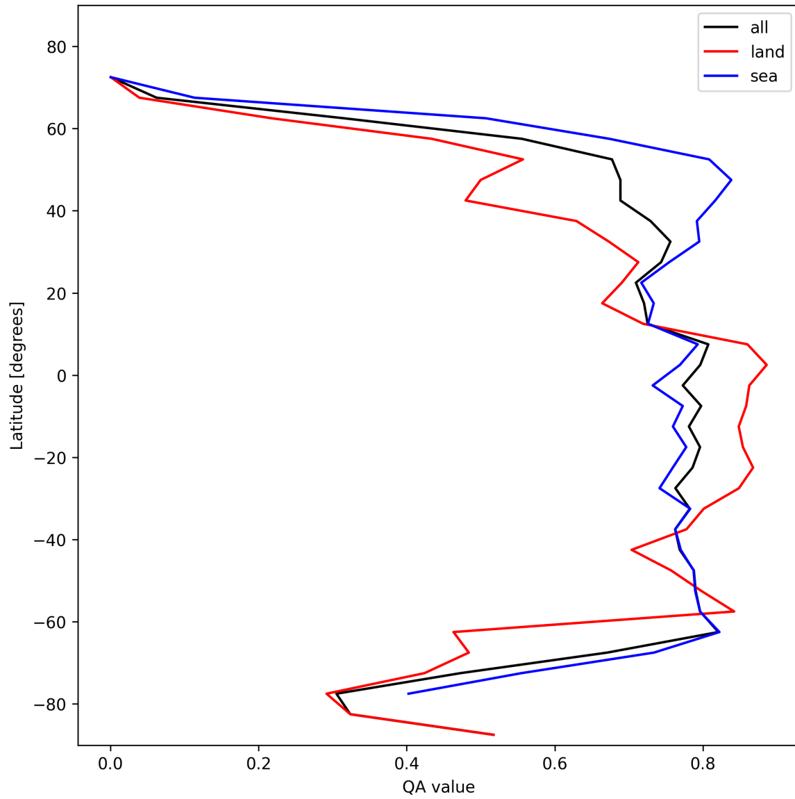
Figure 20: Zonal average of “QA value” for 2025-02-06 to 2025-02-06.
