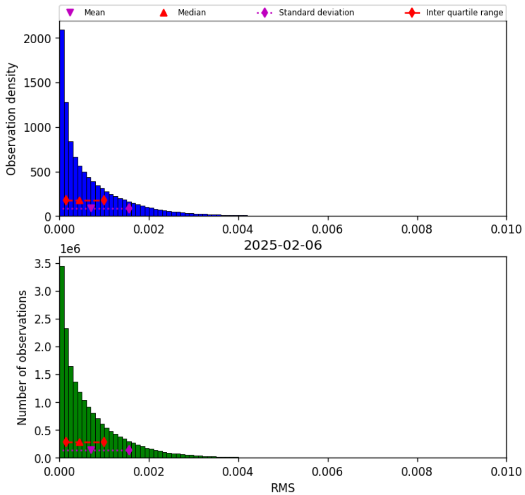
Figure 45: Histogram of “RMS” for 2025-02-06 to 2025-02-06
