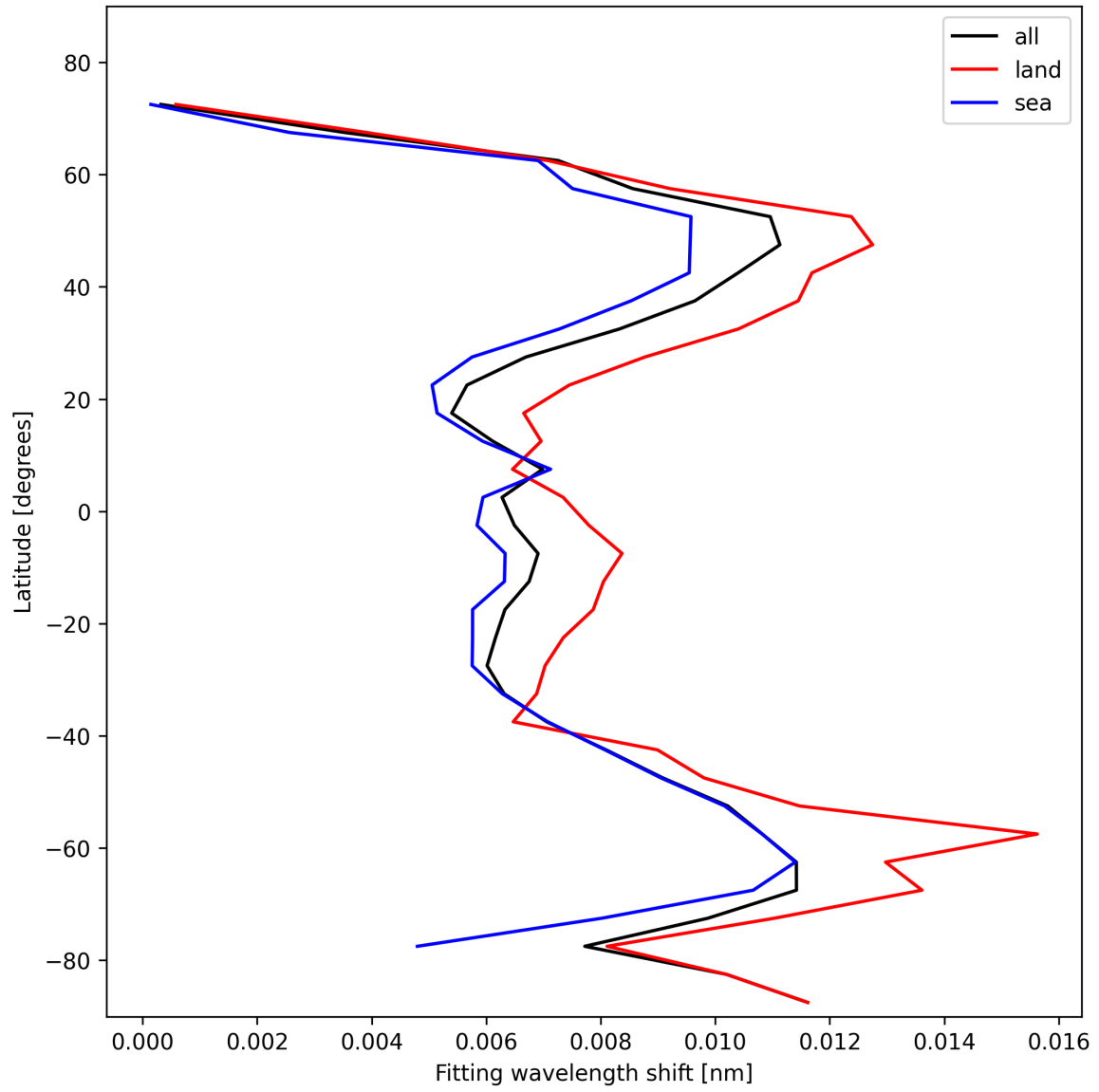
Figure 31: Zonal average of “Fitting wavelength shift” for 2025-02-06 to 2025-02-06.
