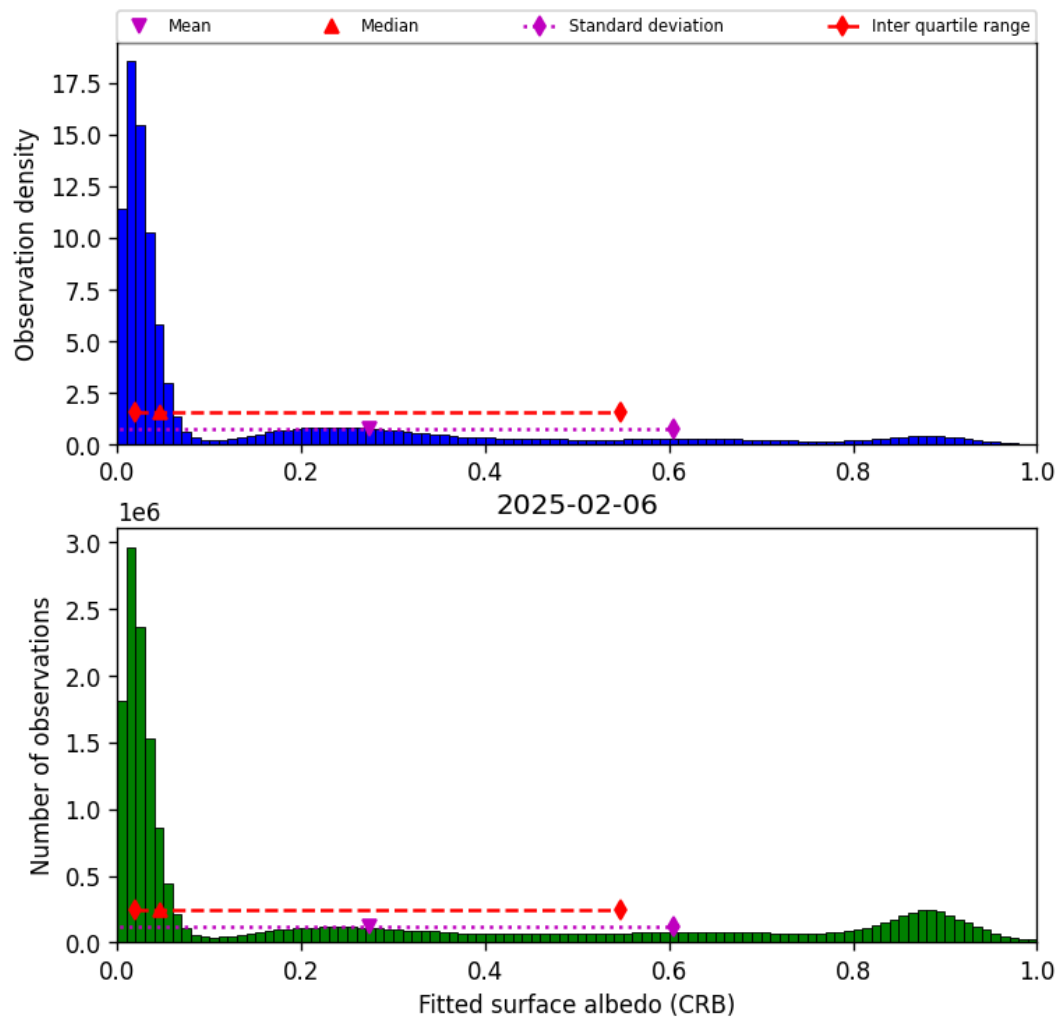
Figure 44: Histogram of “Fitted surface albedo (CRB)” for 2025-02-06 to 2025-02-06
