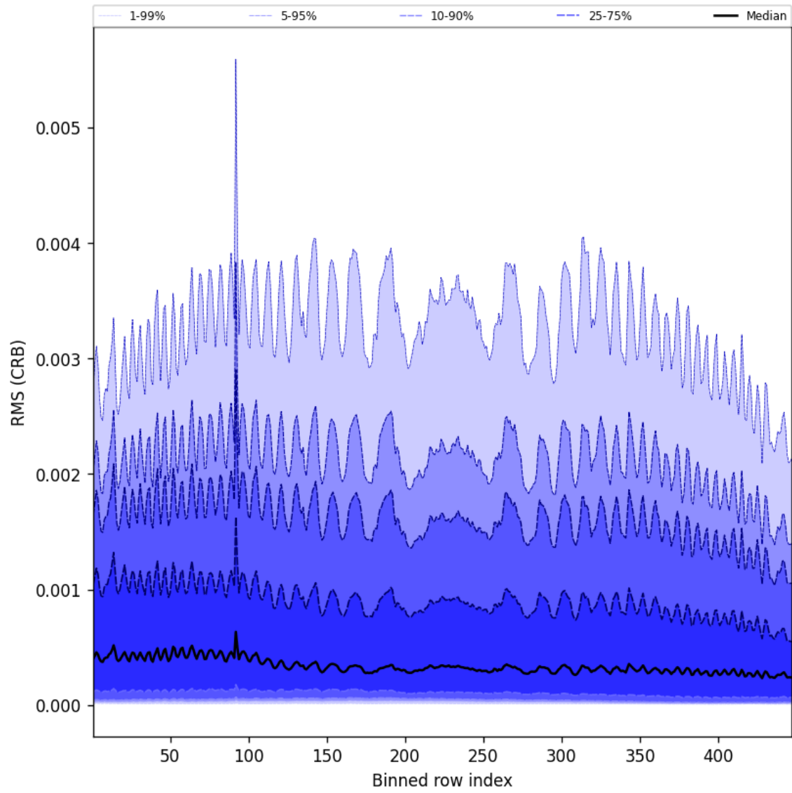
Figure 62: Along track statistics of “RMS (CRB)” for 2025-02-06 to 2025-02-06
