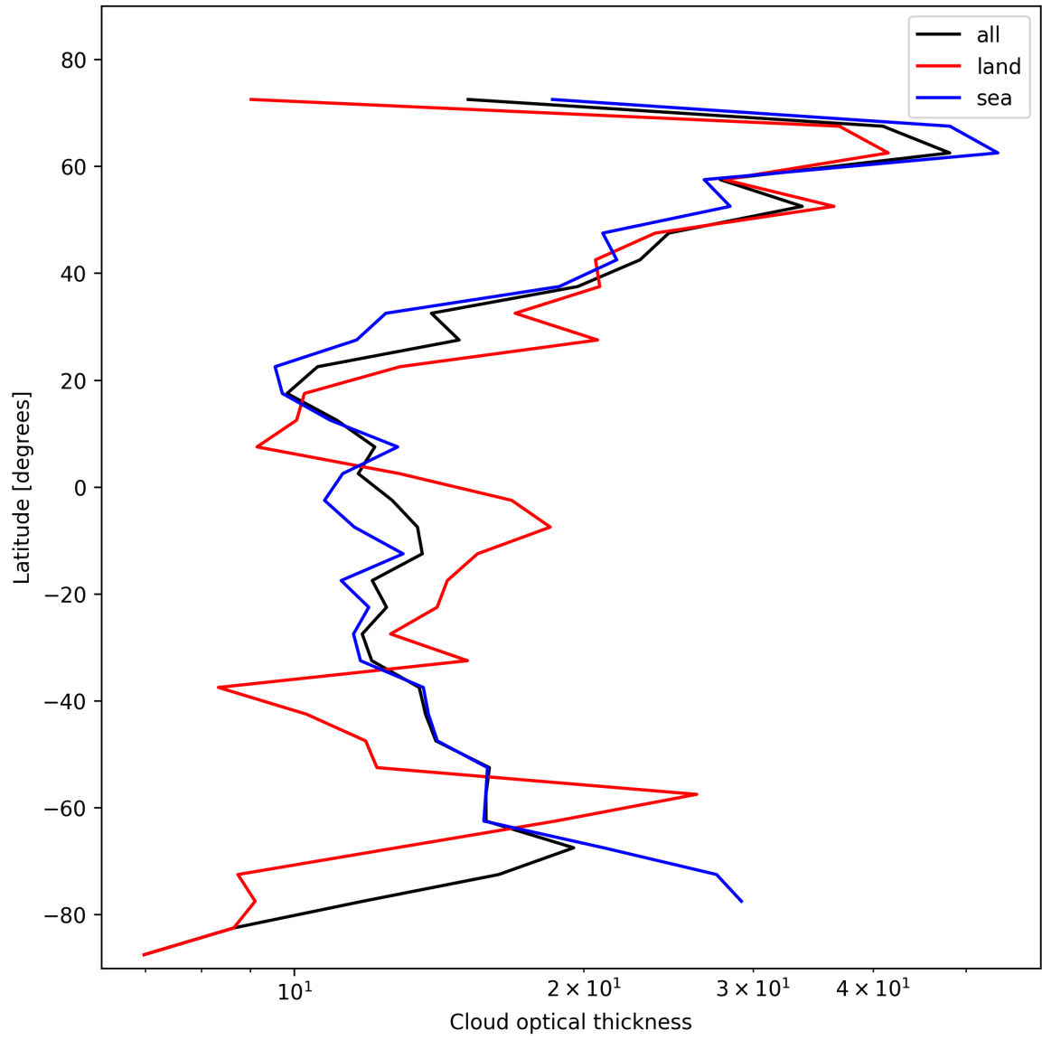
Figure 23: Zonal average of “Cloud optical thickness” for 2025-02-06 to 2025-02-06.
