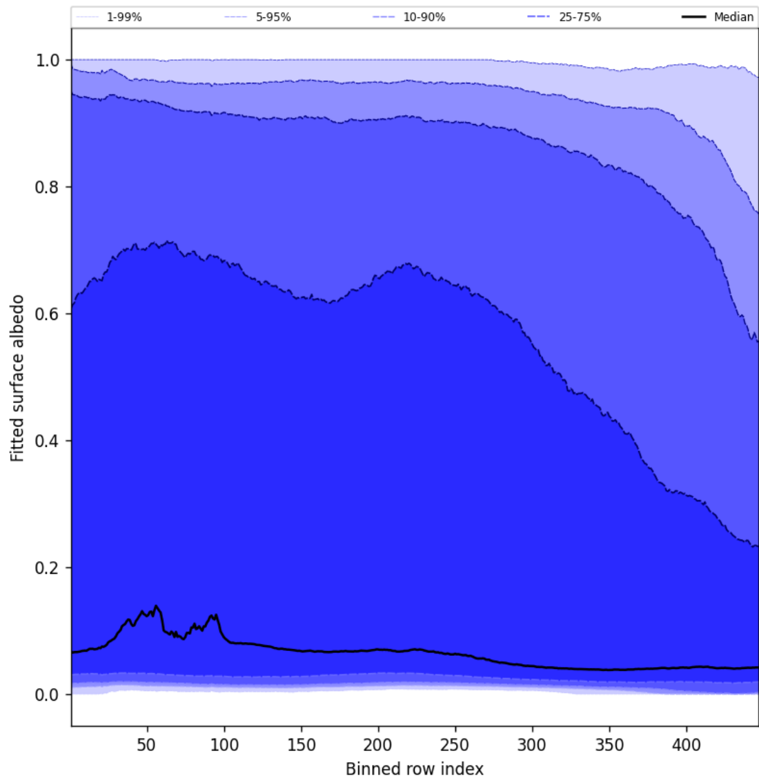
Figure 59: Along track statistics of “Fitted surface albedo” for 2025-02-06 to 2025-02-06
