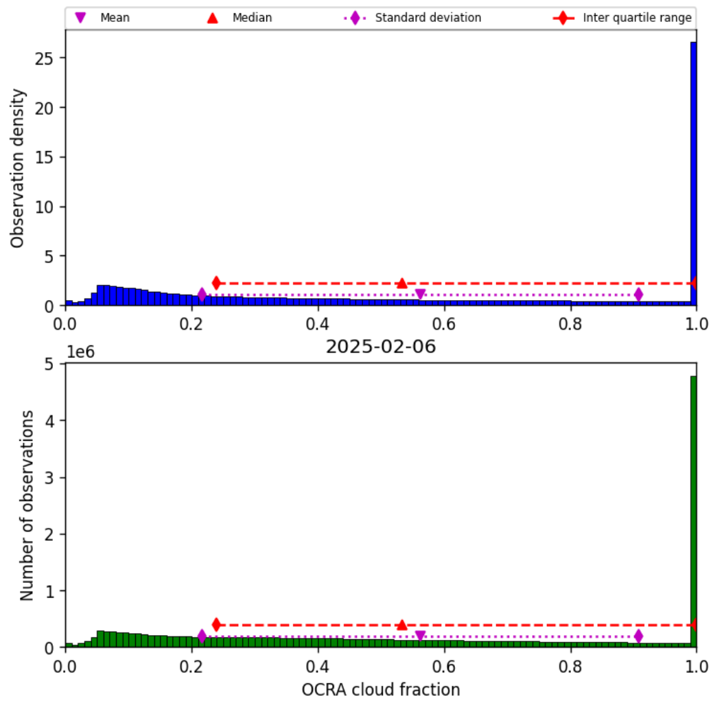
Figure 48: Histogram of “OCRA cloud fraction” for 2025-02-06 to 2025-02-06
