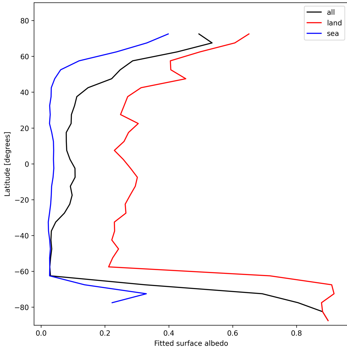
Figure 27: Zonal average of “Fitted surface albedo” for 2025-02-08 to 2025-02-09.
