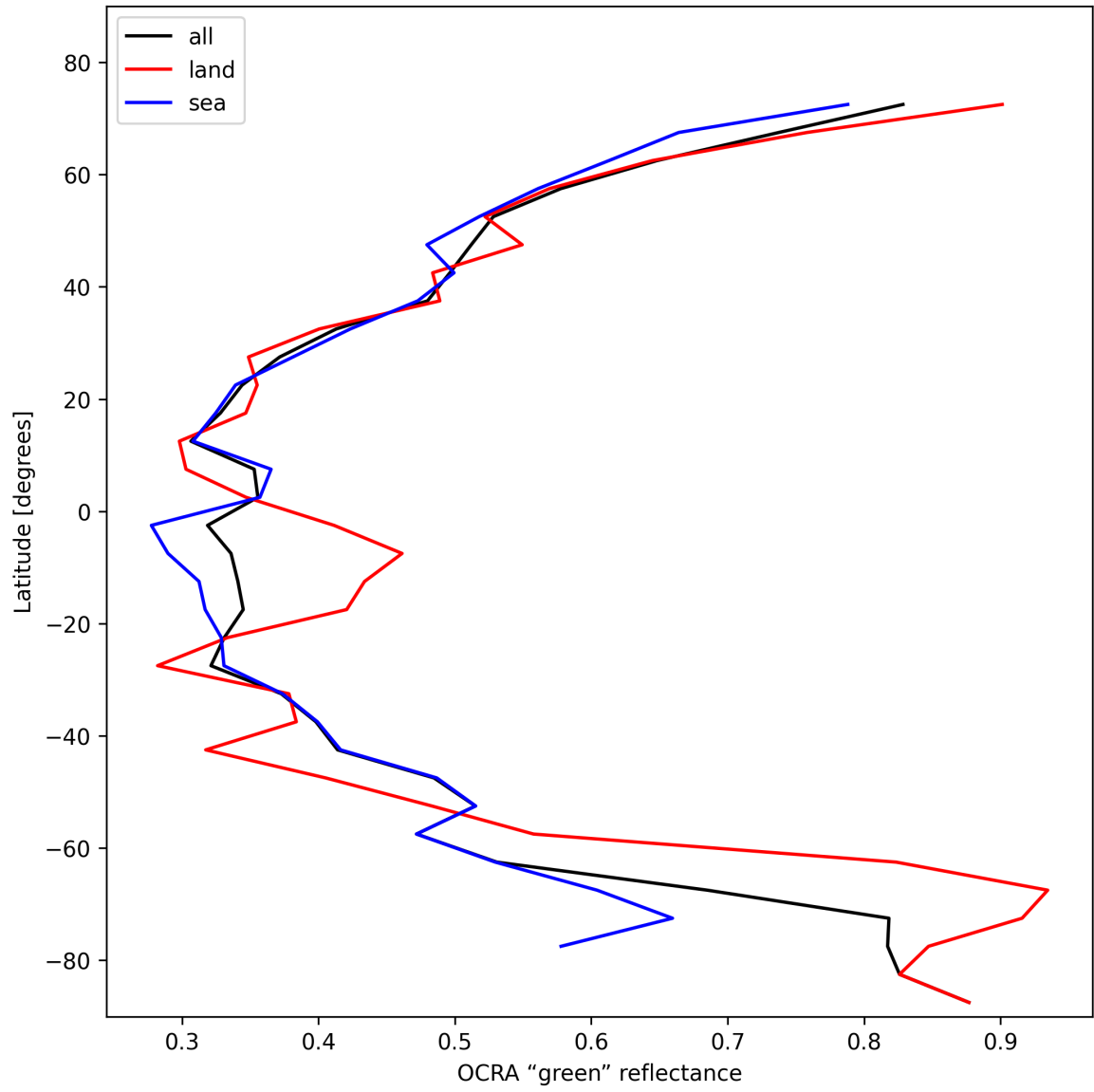
Figure 34: Zonal average of “OCRA “green” reflectance” for 2025-02-08 to 2025-02-09.
