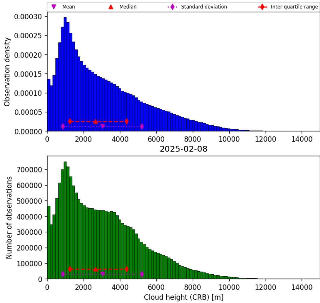
Figure 41: Histogram of “Cloud height (CRB)” for 2025-02-08 to 2025-02-09
