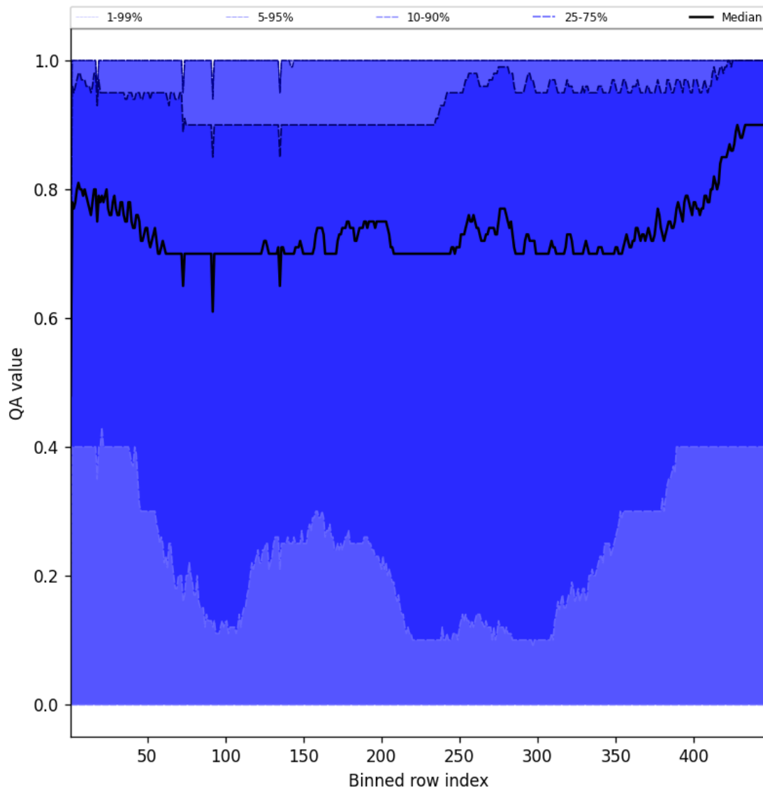
Figure 52: Along track statistics of “QA value” for 2025-02-08 to 2025-02-09
