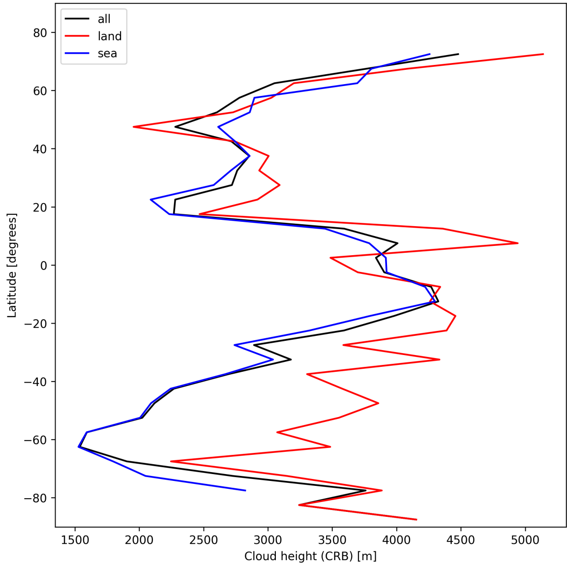
Figure 25: Zonal average of “Cloud height (CRB)” for 2025-02-08 to 2025-02-09.
