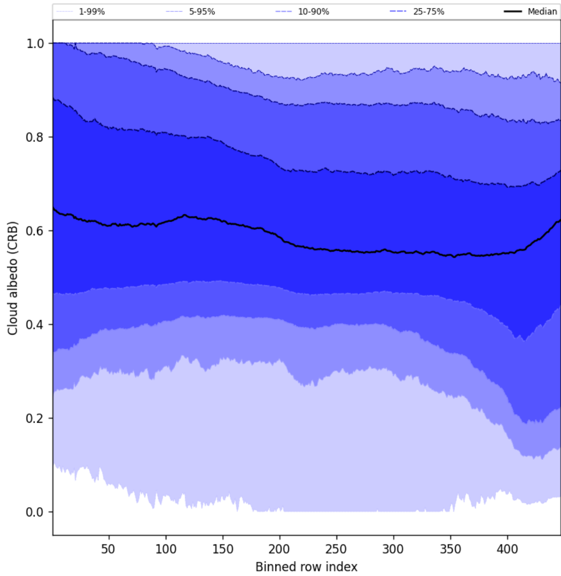
Figure 58: Along track statistics of “Cloud albedo (CRB)” for 2025-02-08 to 2025-02-09
