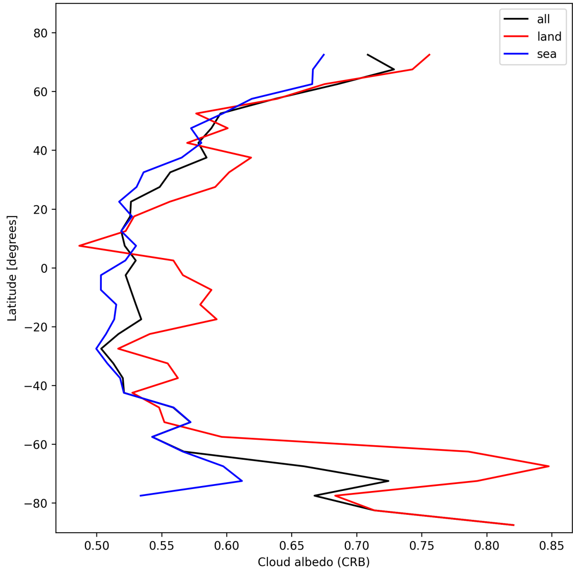
Figure 26: Zonal average of “Cloud albedo (CRB)” for 2025-02-08 to 2025-02-09.
