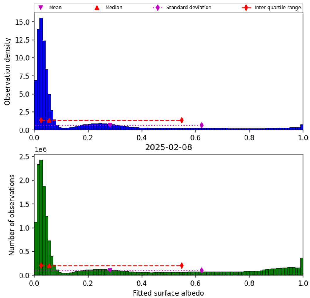
Figure 43: Histogram of “Fitted surface albedo” for 2025-02-08 to 2025-02-09
