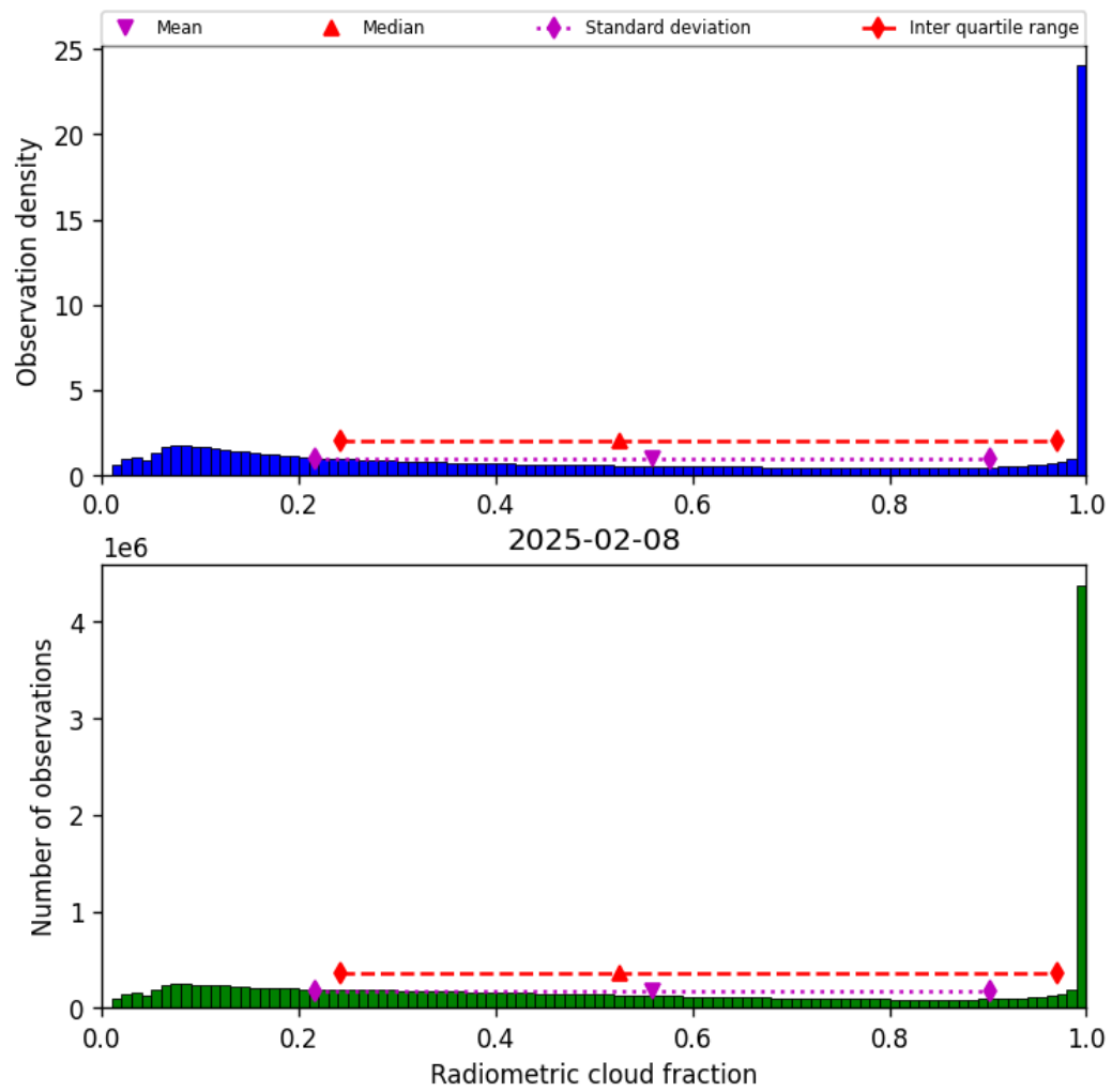
Figure 37: Histogram of “Radiometric cloud fraction” for 2025-02-08 to 2025-02-09
