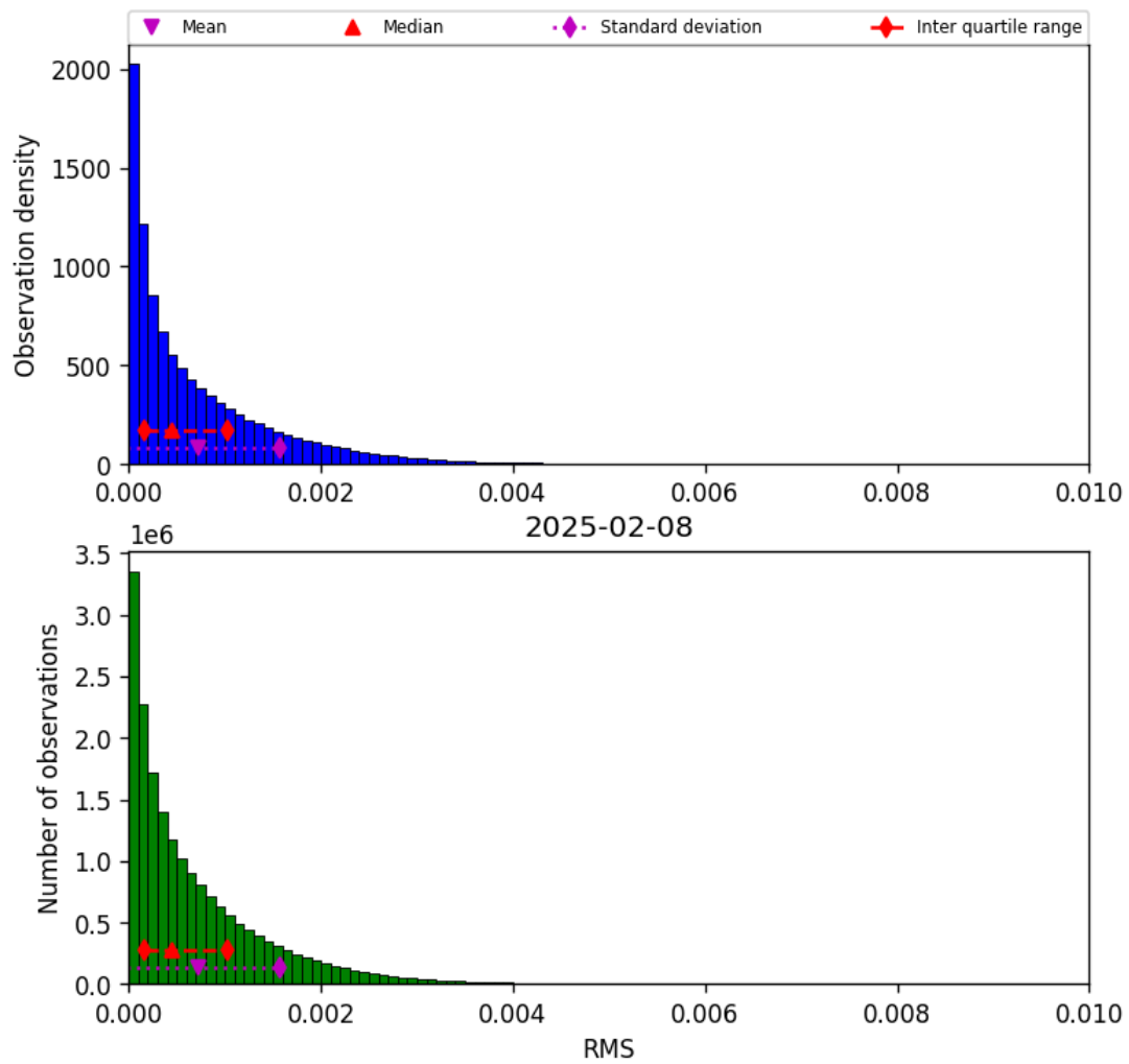
Figure 45: Histogram of “RMS” for 2025-02-08 to 2025-02-09
