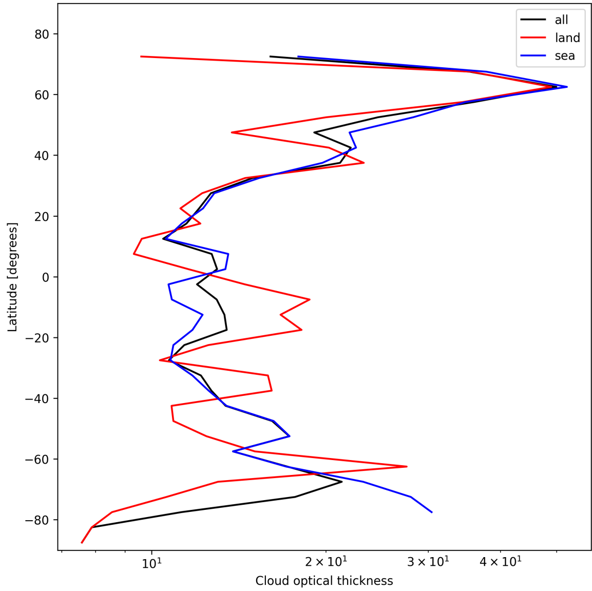
Figure 23: Zonal average of “Cloud optical thickness” for 2025-02-08 to 2025-02-09.
