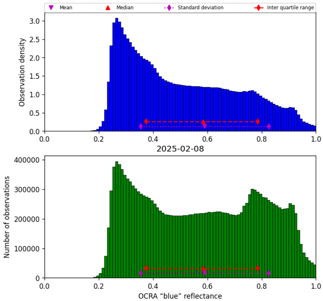
Figure 49: Histogram of “OCRA “blue” reflectance” for 2025-02-08 to 2025-02-09
