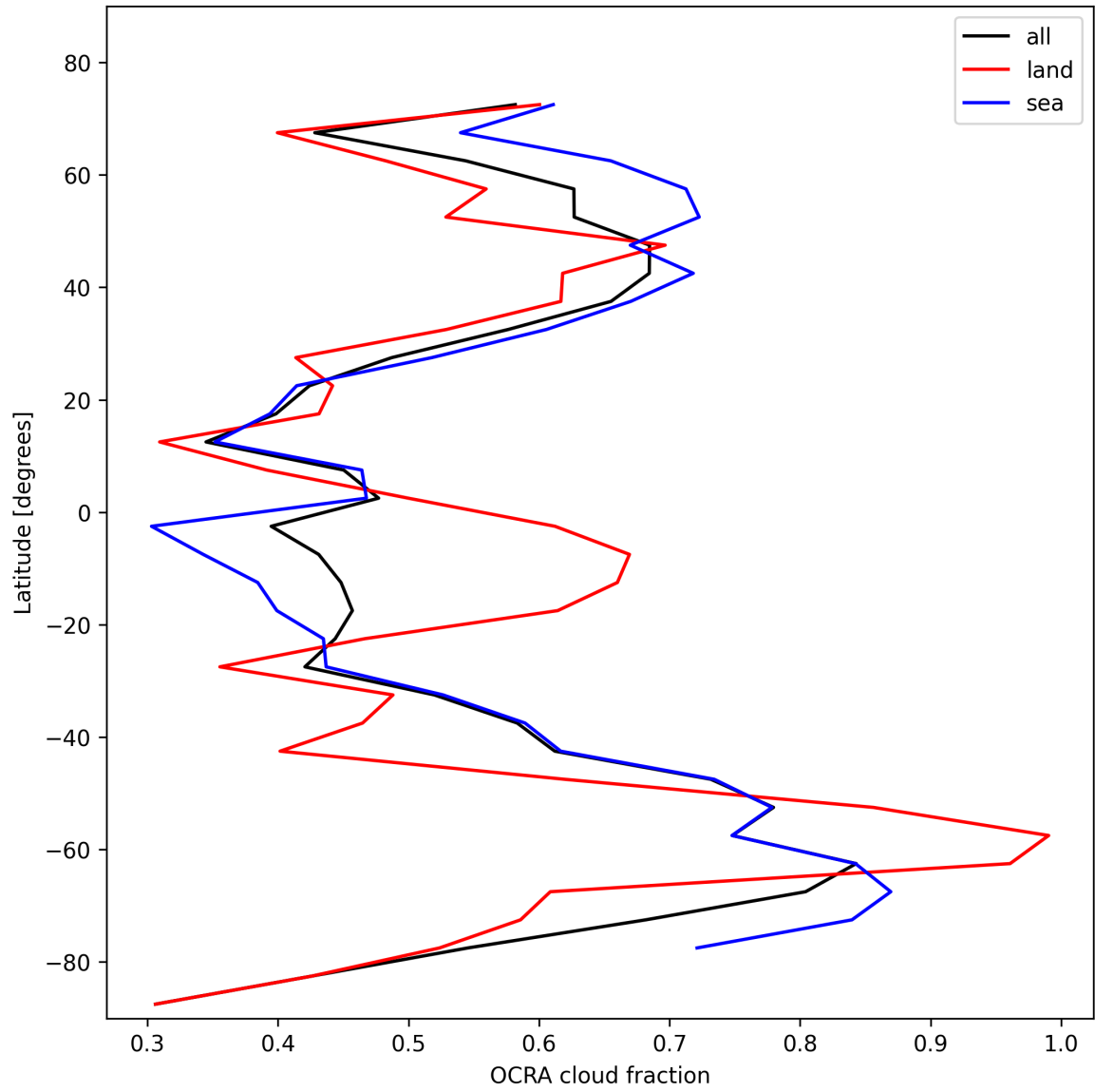
Figure 32: Zonal average of “OCRA cloud fraction” for 2025-02-08 to 2025-02-09.
