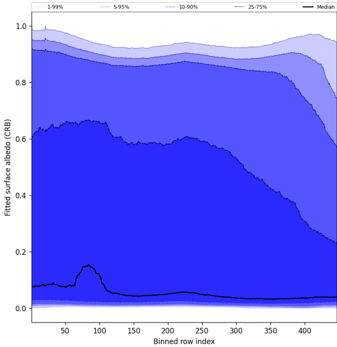
Figure 60: Along track statistics of “Fitted surface albedo (CRB)” for 2025-02-08 to 2025-02-09
