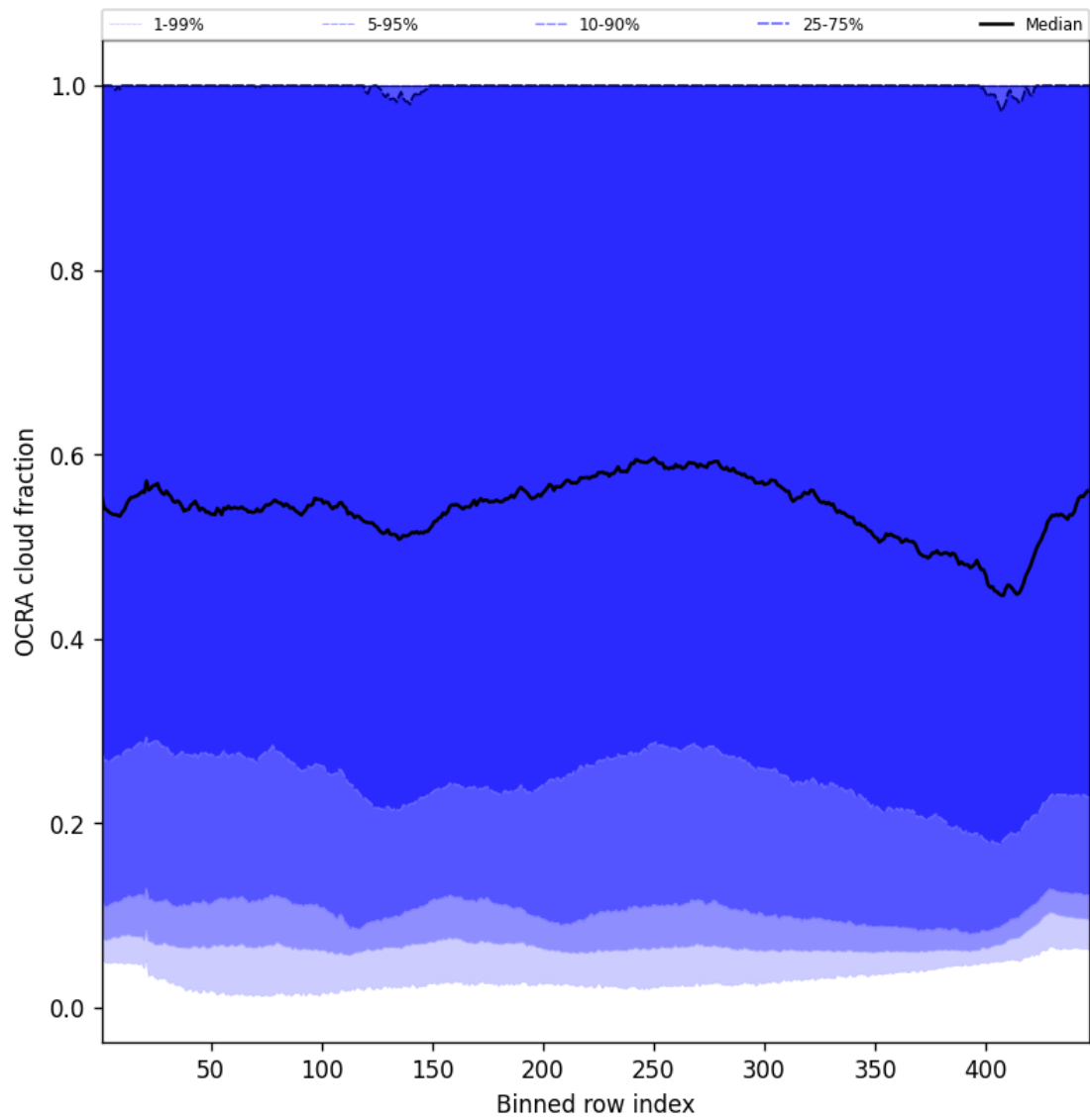
Figure 64: Along track statistics of “OCRA cloud fraction” for 2025-02-08 to 2025-02-09
