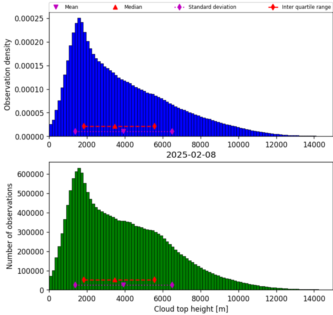
Figure 38: Histogram of “Cloud top height” for 2025-02-08 to 2025-02-09
