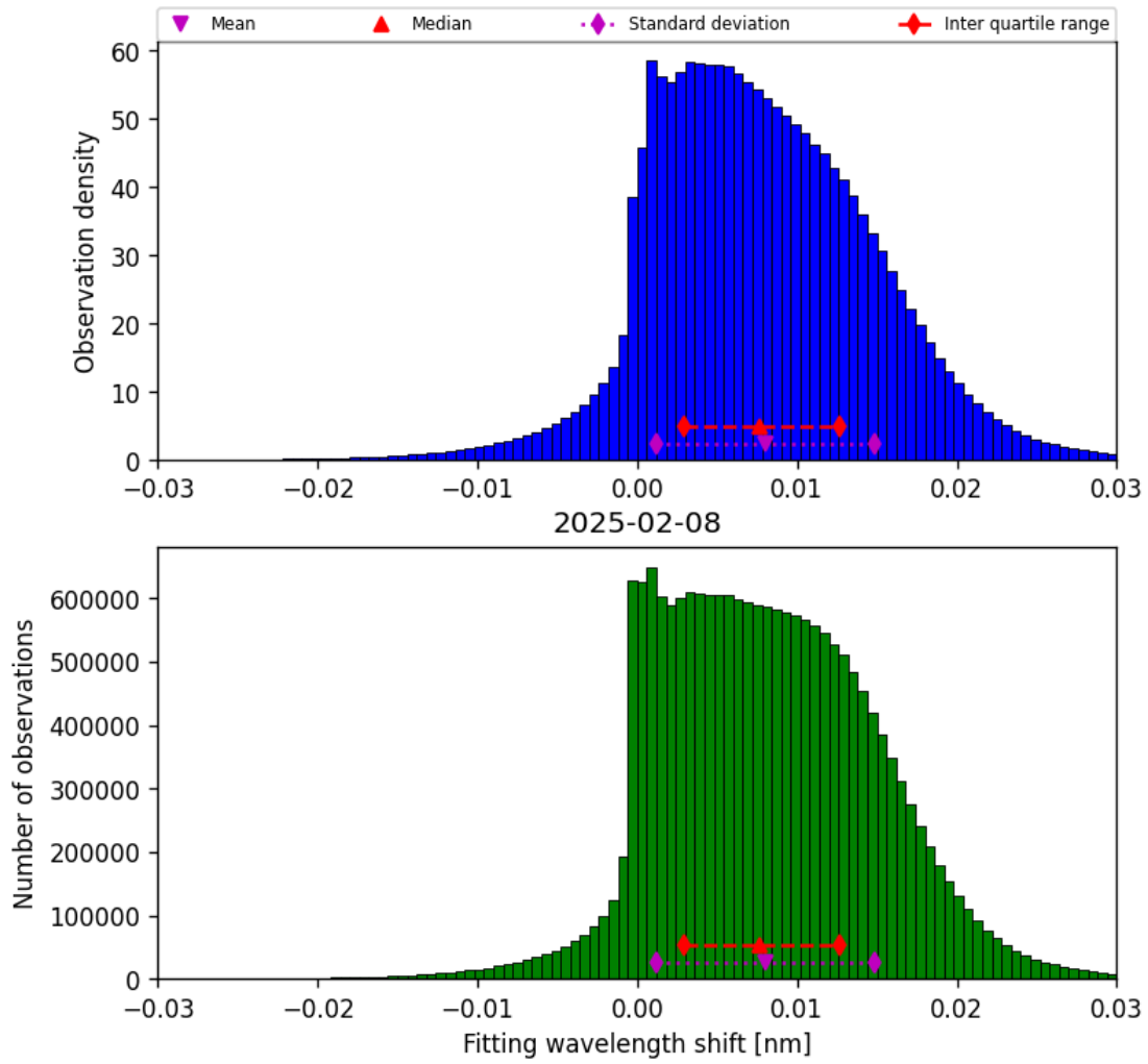
Figure 47: Histogram of “Fitting wavelength shift” for 2025-02-08 to 2025-02-09
