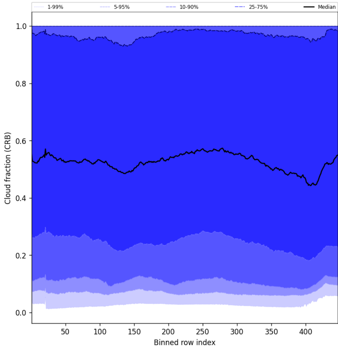
Figure 56: Along track statistics of “Cloud fraction (CRB)” for 2025-02-08 to 2025-02-09
