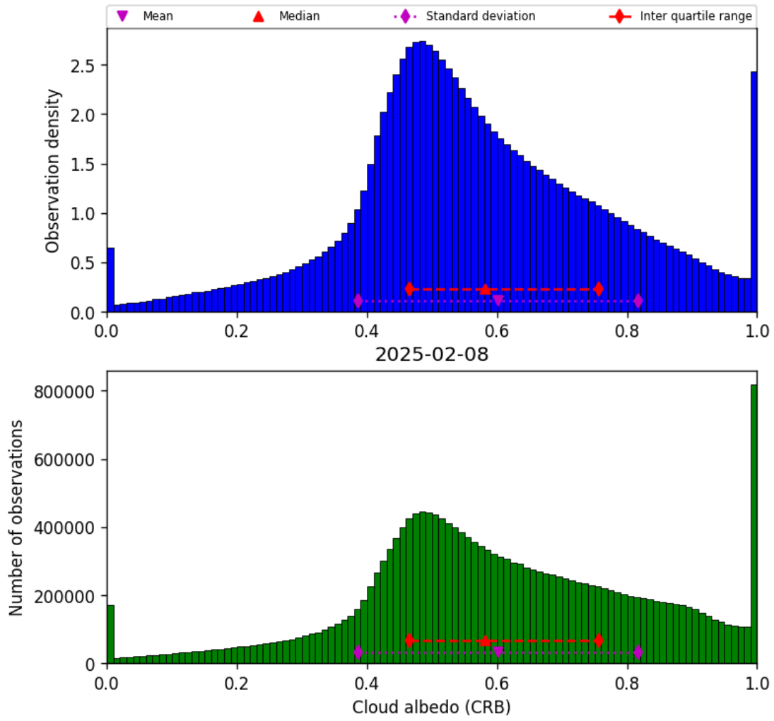
Figure 42: Histogram of “Cloud albedo (CRB)” for 2025-02-08 to 2025-02-09
