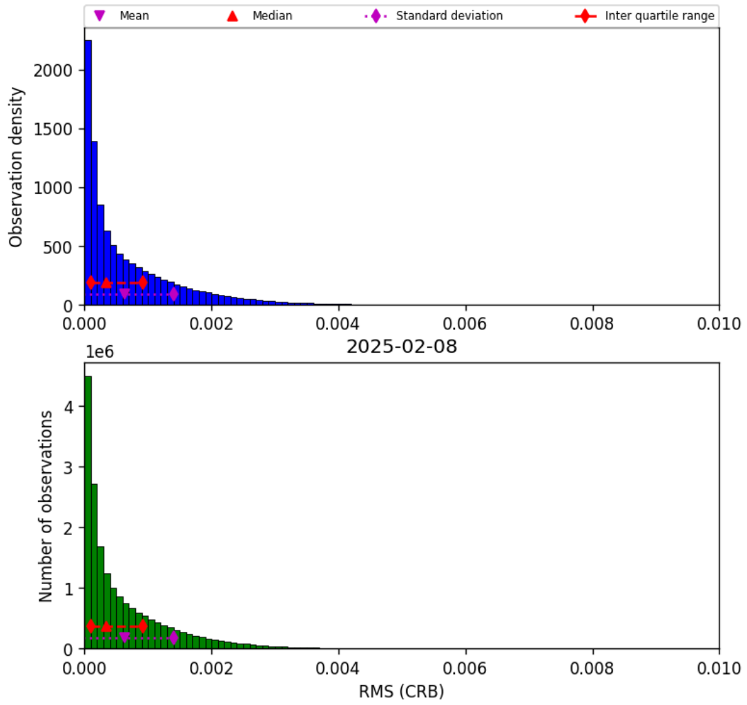
Figure 46: Histogram of “RMS (CRB)” for 2025-02-08 to 2025-02-09
