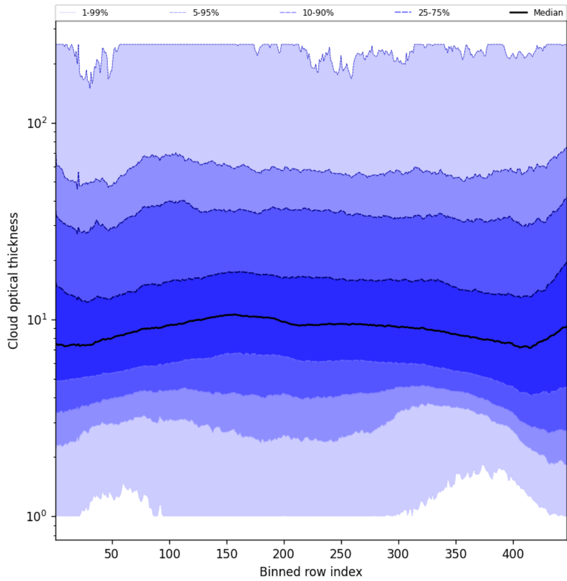
Figure 55: Along track statistics of “Cloud optical thickness” for 2025-02-08 to 2025-02-09
