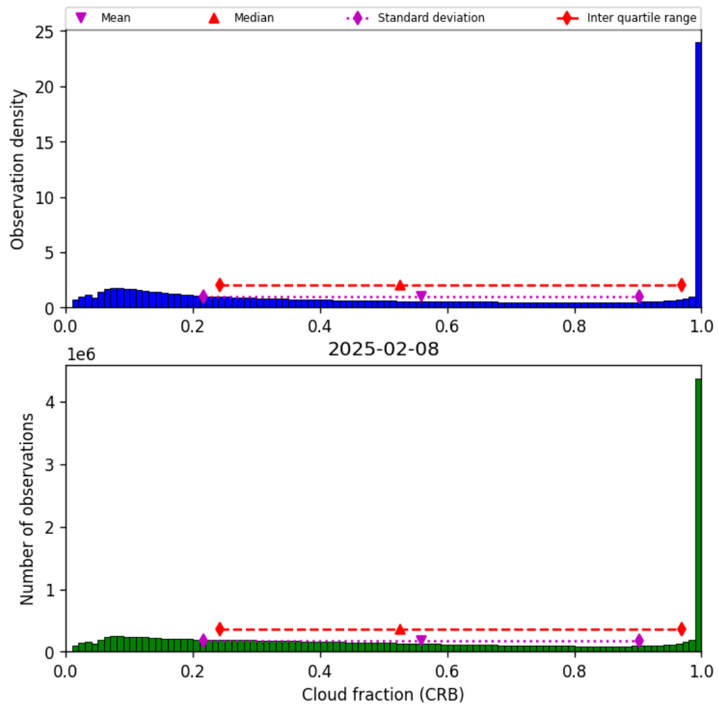
Figure 40: Histogram of “Cloud fraction (CRB)” for 2025-02-08 to 2025-02-09
