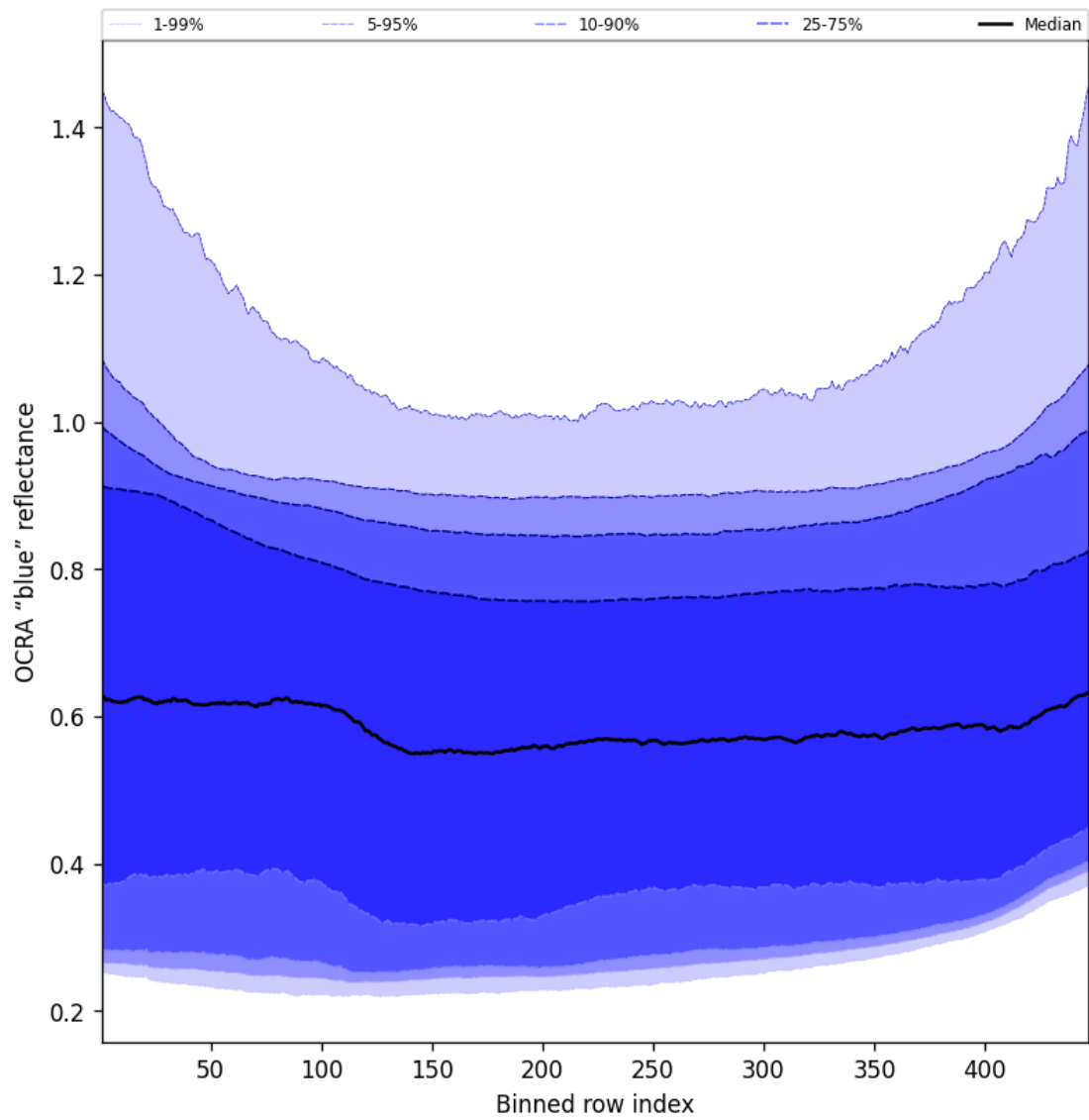
Figure 65: Along track statistics of "OCRA "blue" reflectance" for 2025-02-08 to 2025-02-09
