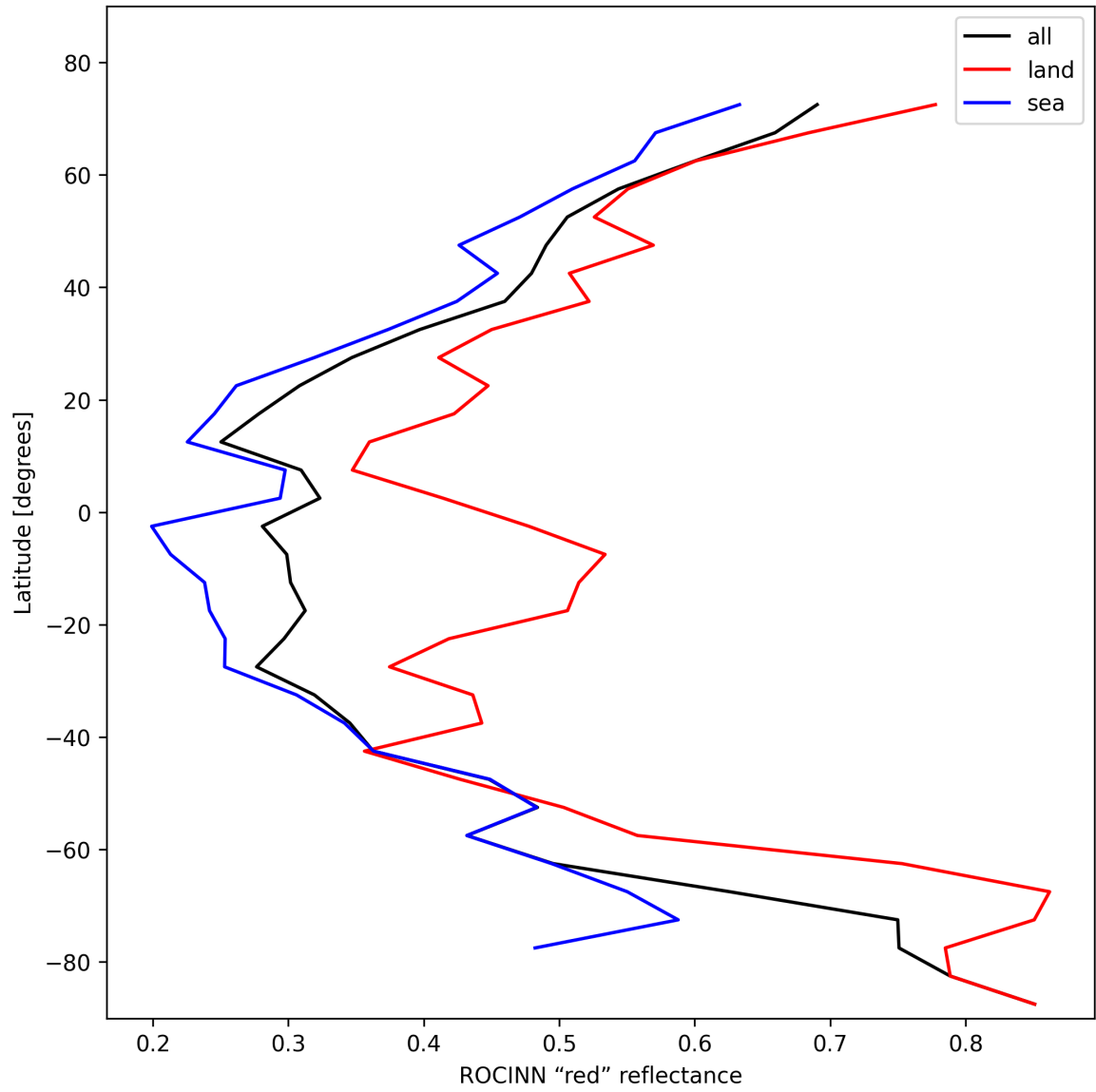
Figure 35: Zonal average of "ROCINN "red" reflectance" for 2025-02-08 to 2025-02-09.
