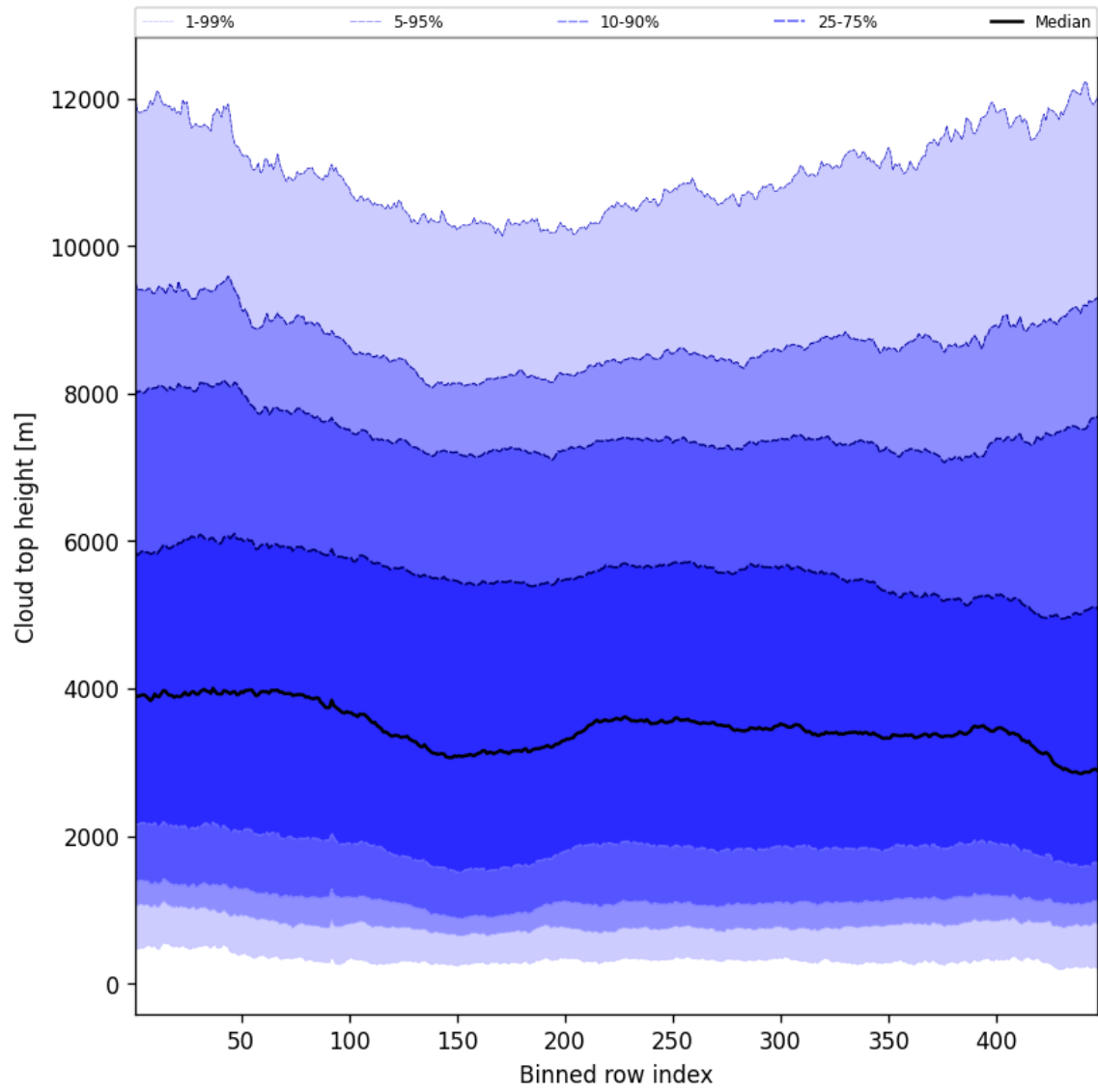
Figure 54: Along track statistics of “Cloud top height” for 2025-02-08 to 2025-02-09
