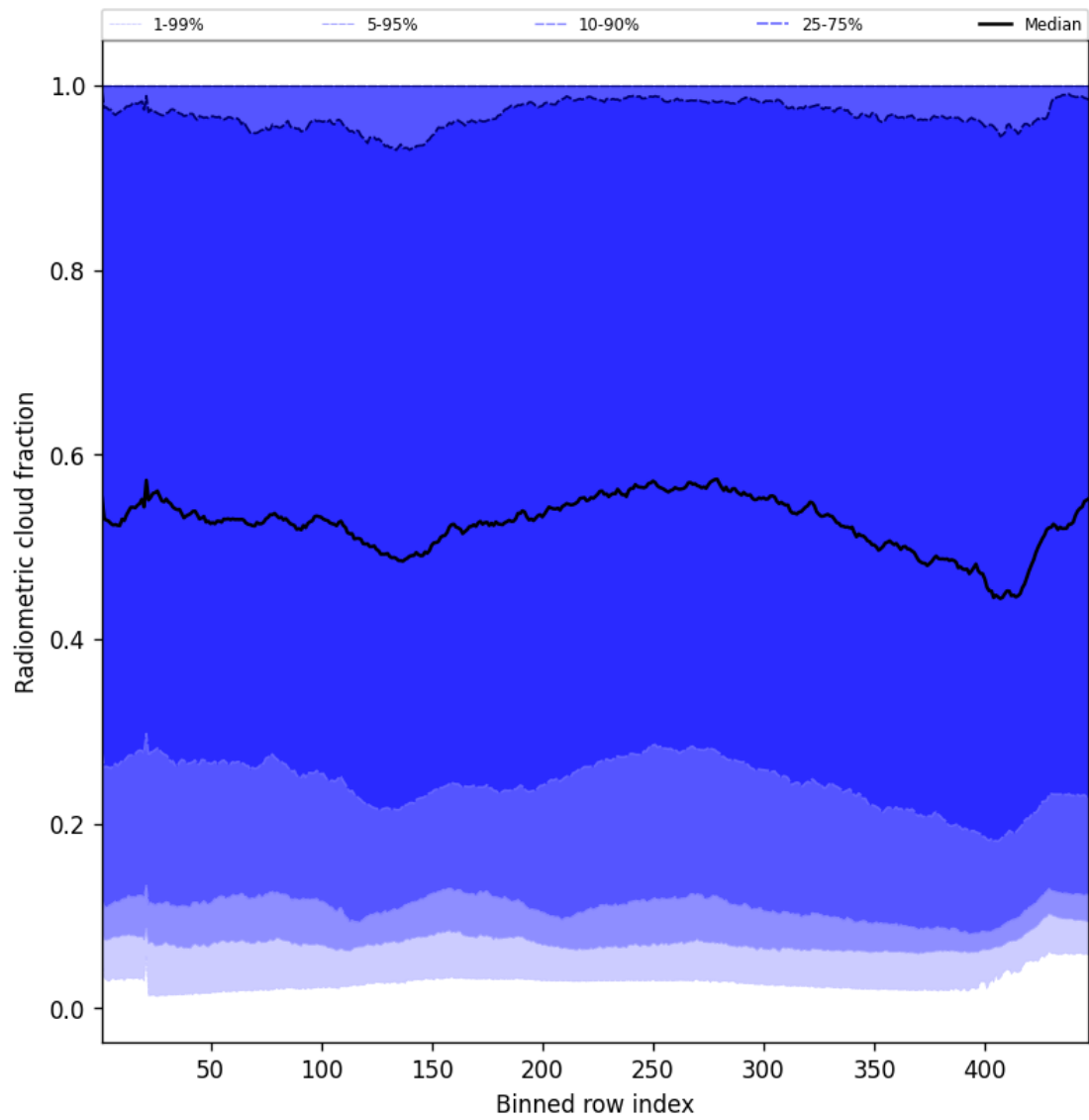
Figure 53: Along track statistics of “Radiometric cloud fraction” for 2025-02-08 to 2025-02-09
