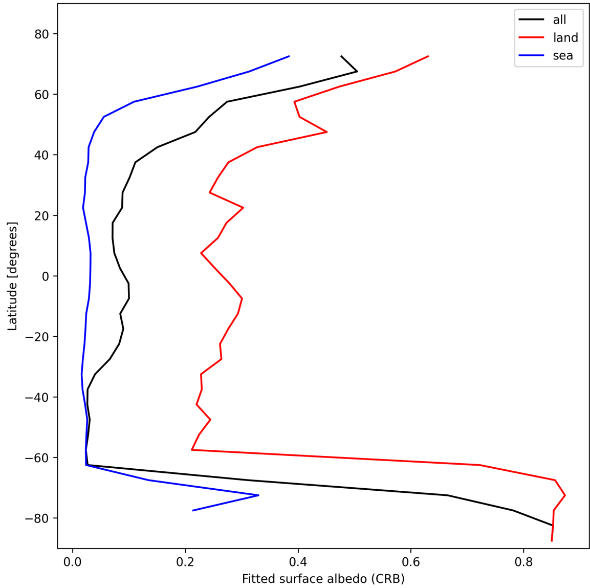
Figure 28: Zonal average of “Fitted surface albedo (CRB)” for 2025-02-08 to 2025-02-09.
