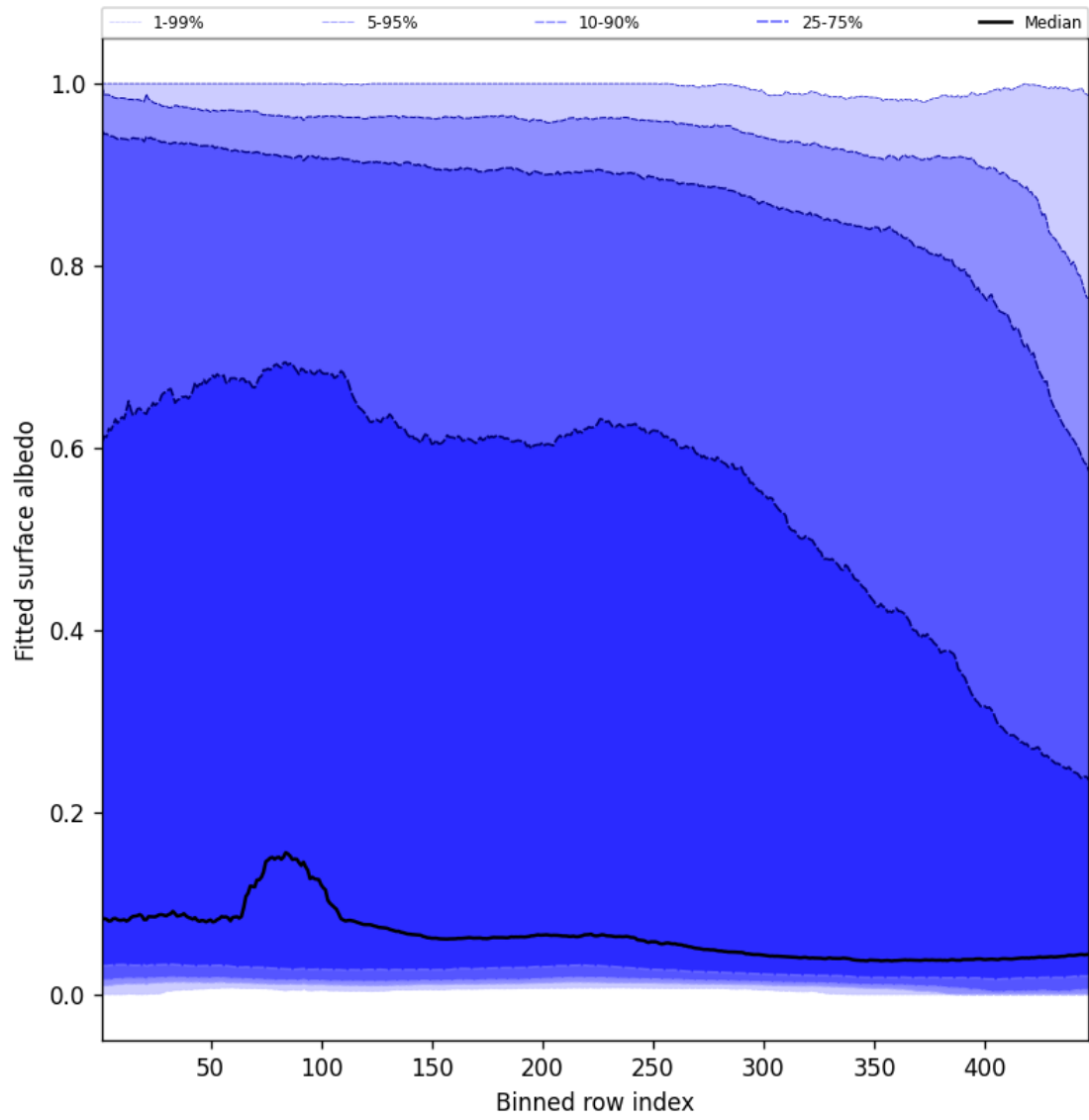
Figure 59: Along track statistics of “Fitted surface albedo” for 2025-02-08 to 2025-02-09
