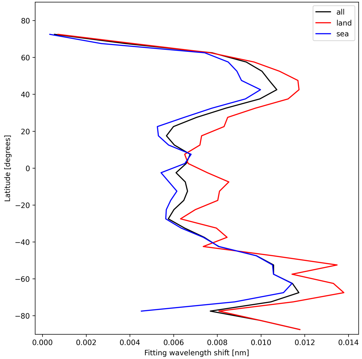
Figure 31: Zonal average of “Fitting wavelength shift” for 2025-02-08 to 2025-02-09.
