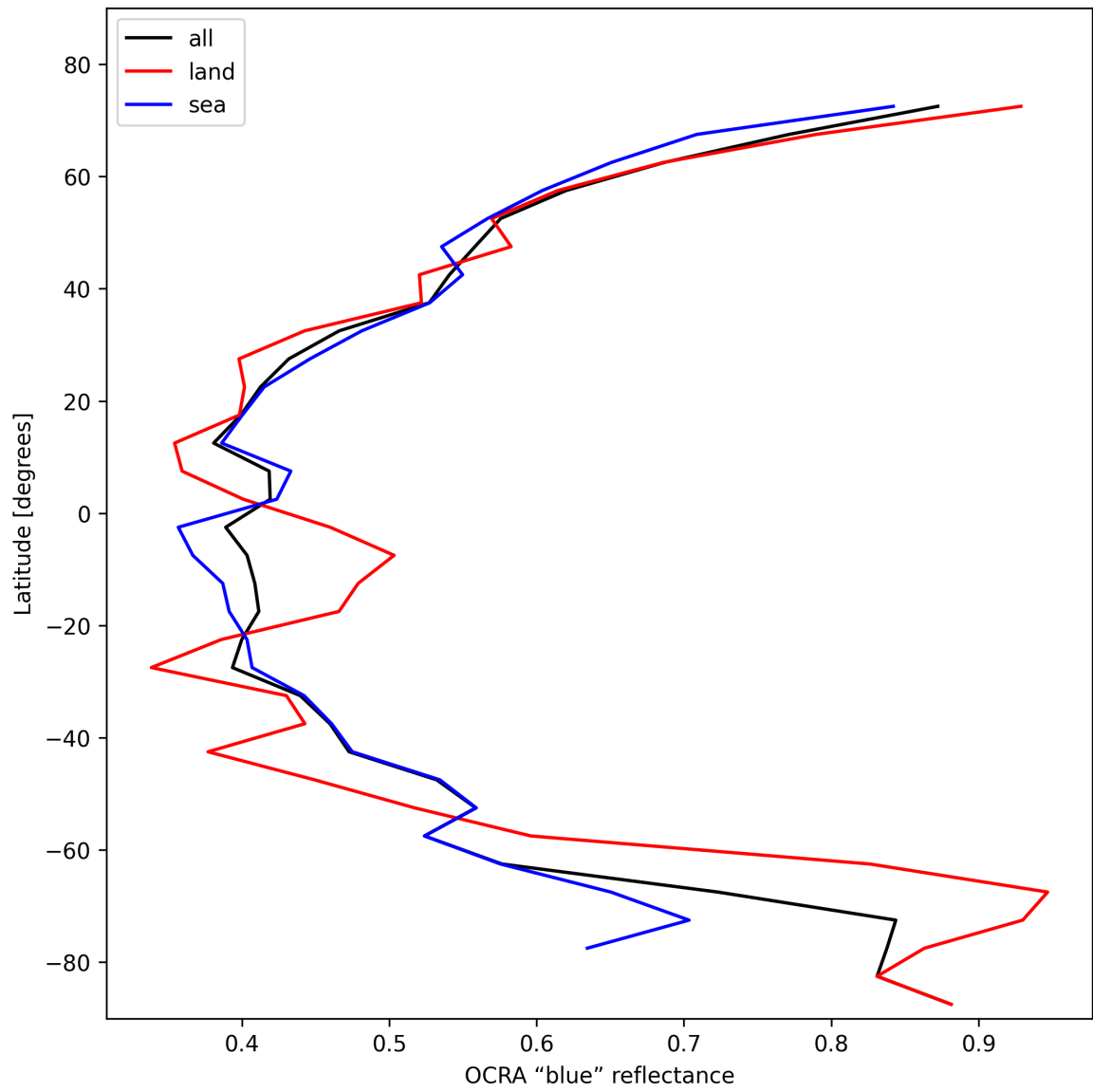
Figure 33: Zonal average of “OCRA “blue” reflectance” for 2025-02-08 to 2025-02-09.
