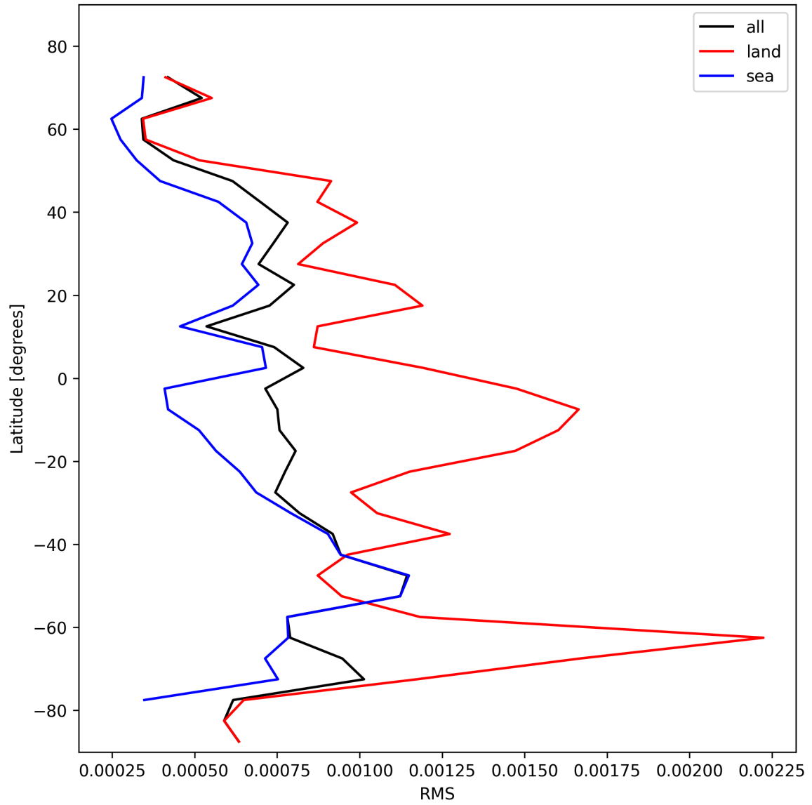
Figure 29: Zonal average of “RMS” for 2025-02-08 to 2025-02-09.
