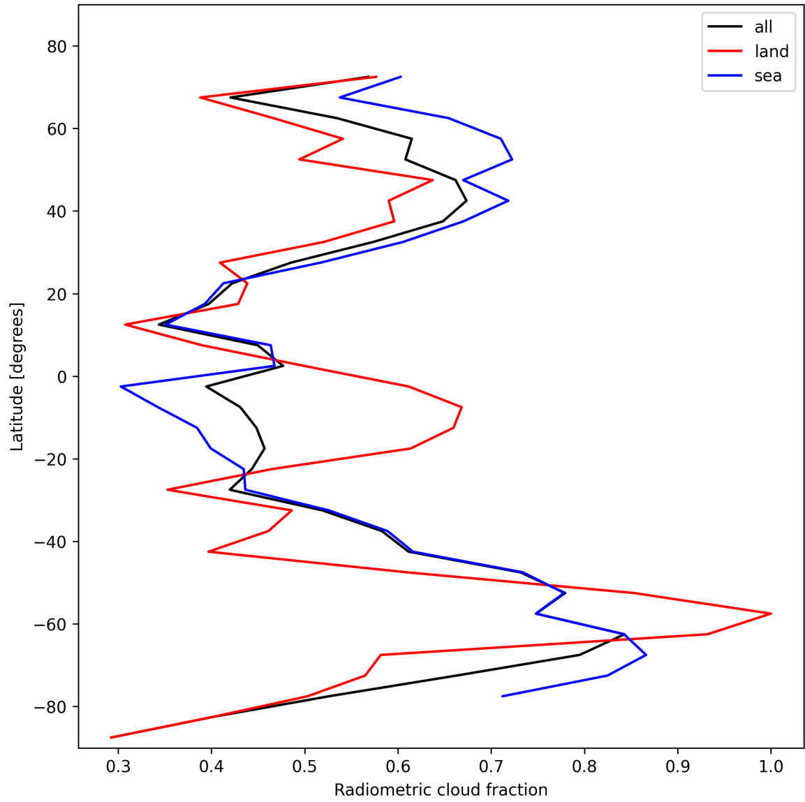
Figure 21: Zonal average of “Radiometric cloud fraction” for 2025-02-08 to 2025-02-09.
