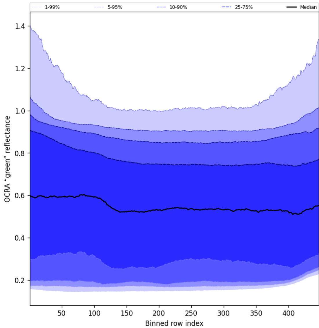
Figure 66: Along track statistics of "OCRA "green" reflectance" for 2025-02-08 to 2025-02-09
