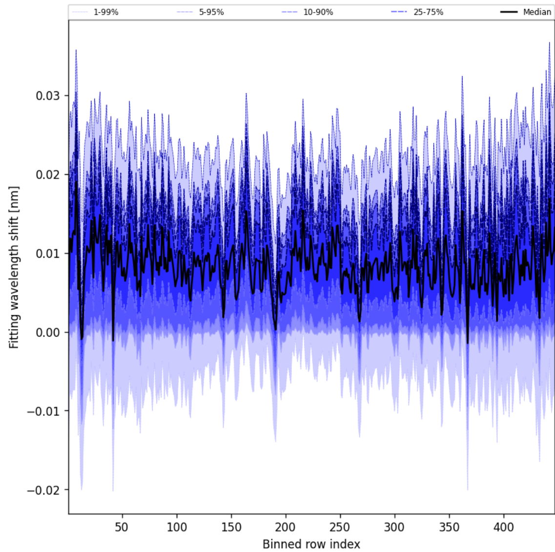
Figure 63: Along track statistics of “Fitting wavelength shift” for 2025-02-08 to 2025-02-09
