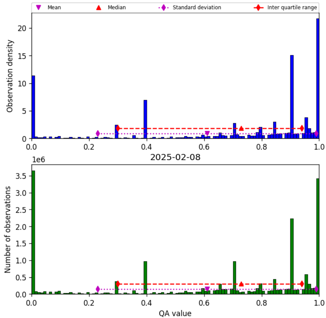
Figure 36: Histogram of “QA value” for 2025-02-08 to 2025-02-09
