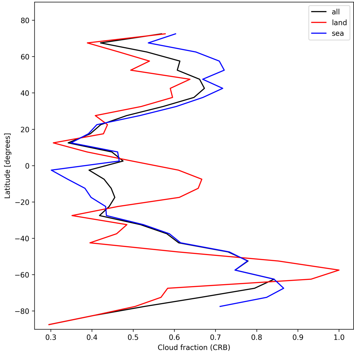
Figure 24: Zonal average of “Cloud fraction (CRB)” for 2025-02-08 to 2025-02-09.
