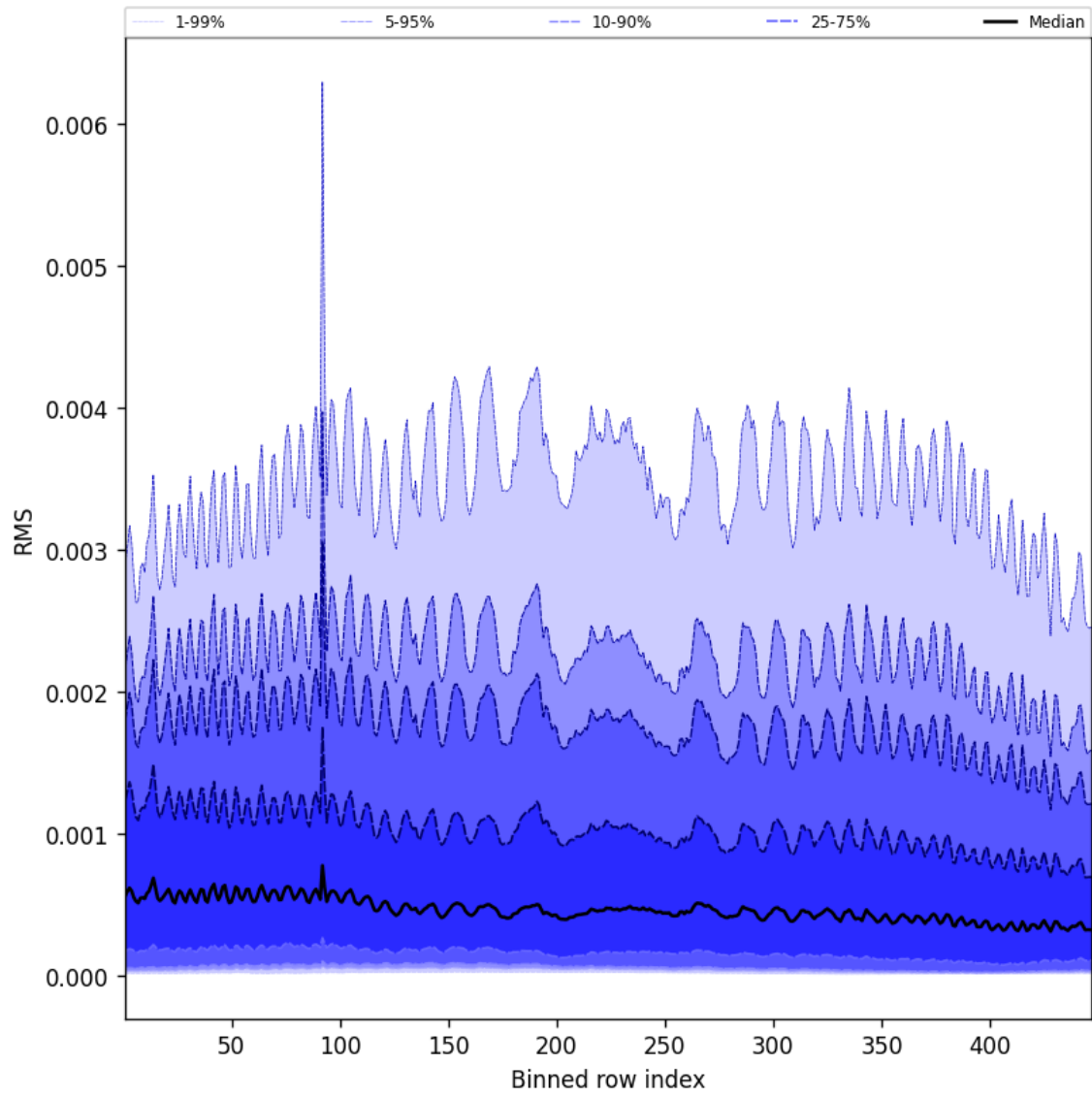
Figure 61: Along track statistics of “RMS” for 2025-02-08 to 2025-02-09
