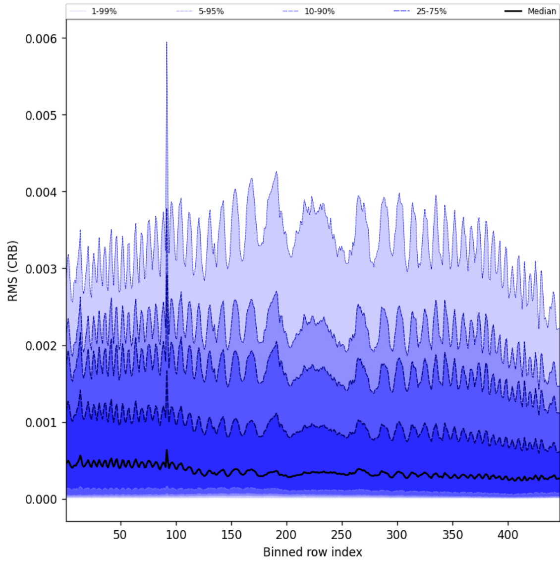
Figure 62: Along track statistics of “RMS (CRB)” for 2025-02-08 to 2025-02-09
