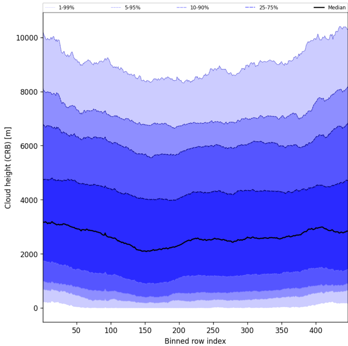
Figure 57: Along track statistics of “Cloud height (CRB)” for 2025-02-08 to 2025-02-09
