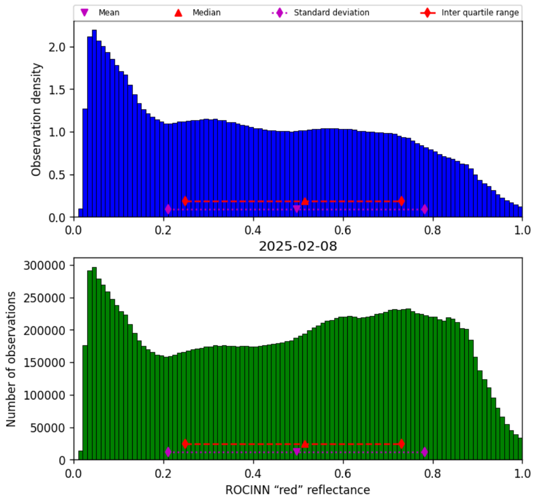
Figure 51: Histogram of “ROCINN “red” reflectance” for 2025-02-08 to 2025-02-09
