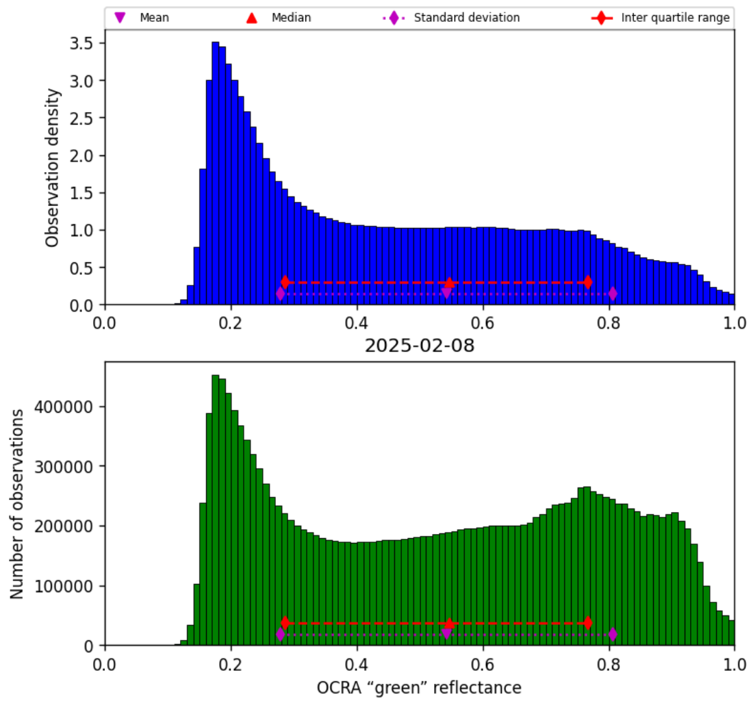
Figure 50: Histogram of “OCRA “green” reflectance” for 2025-02-08 to 2025-02-09
