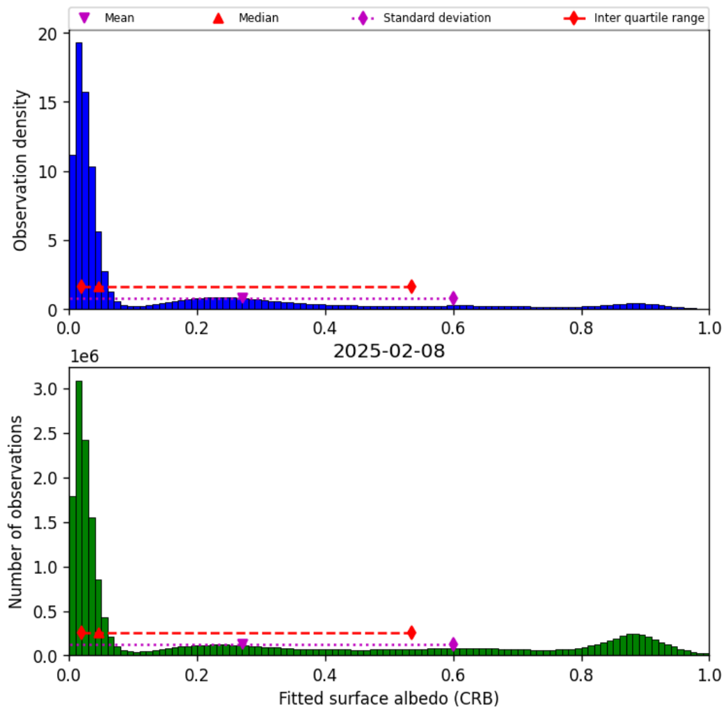
Figure 44: Histogram of “Fitted surface albedo (CRB)” for 2025-02-08 to 2025-02-09
