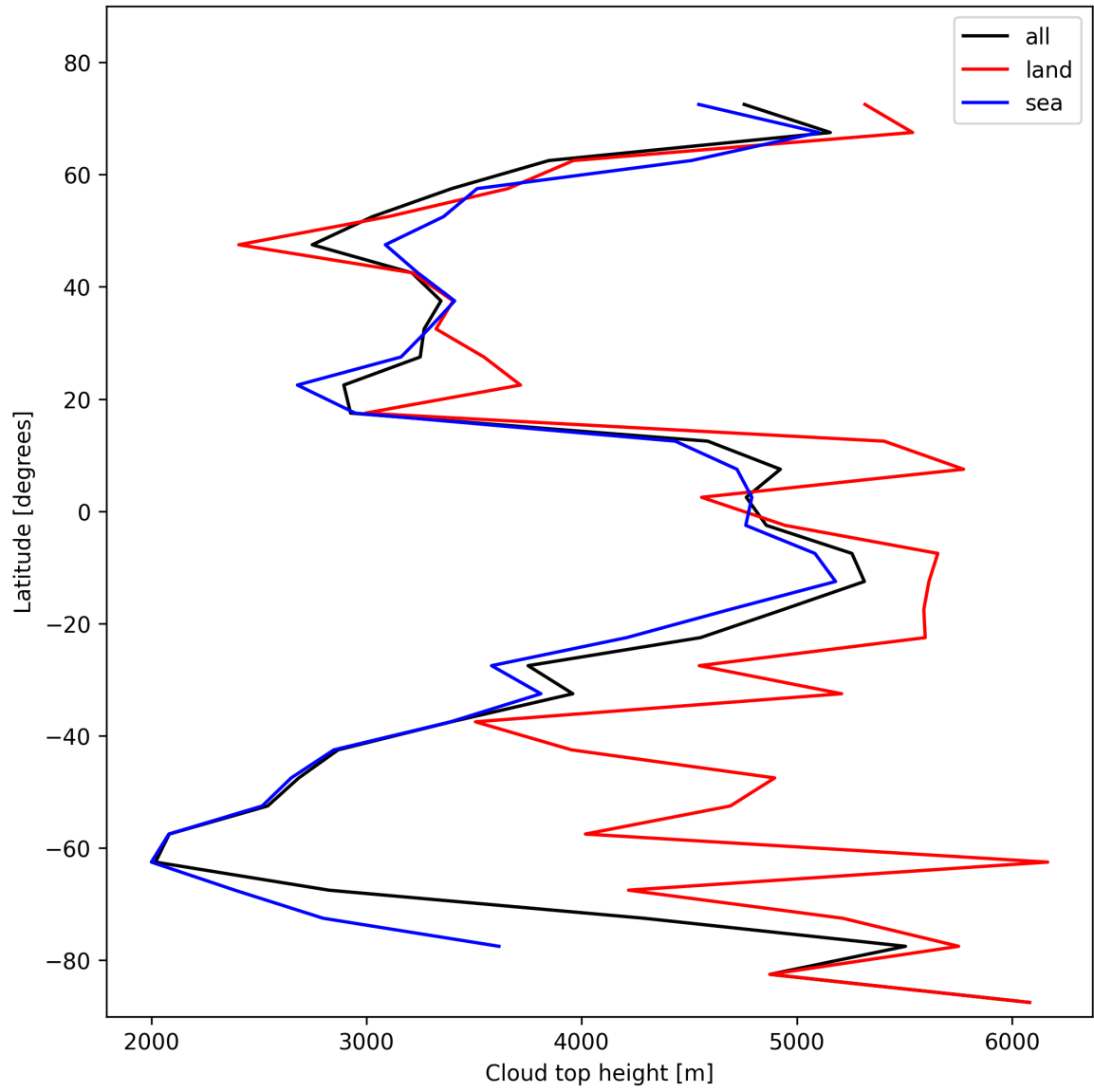
Figure 22: Zonal average of “Cloud top height” for 2025-02-08 to 2025-02-09.
