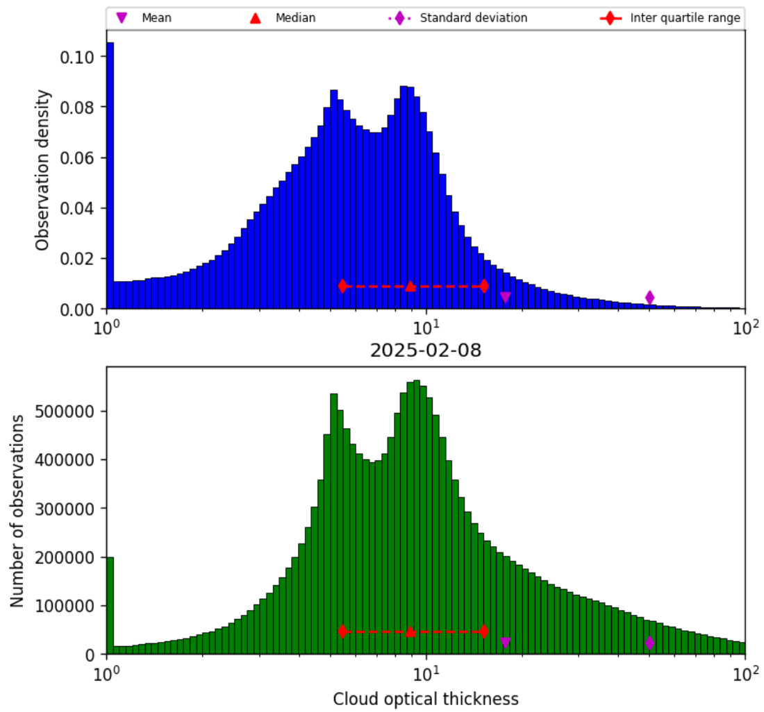
Figure 39: Histogram of “Cloud optical thickness” for 2025-02-08 to 2025-02-09
