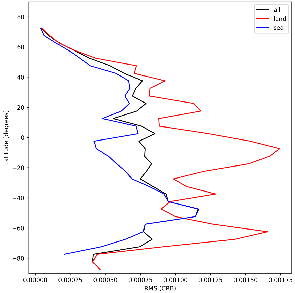
Figure 30: Zonal average of “RMS (CRB)” for 2025-02-08 to 2025-02-09.
