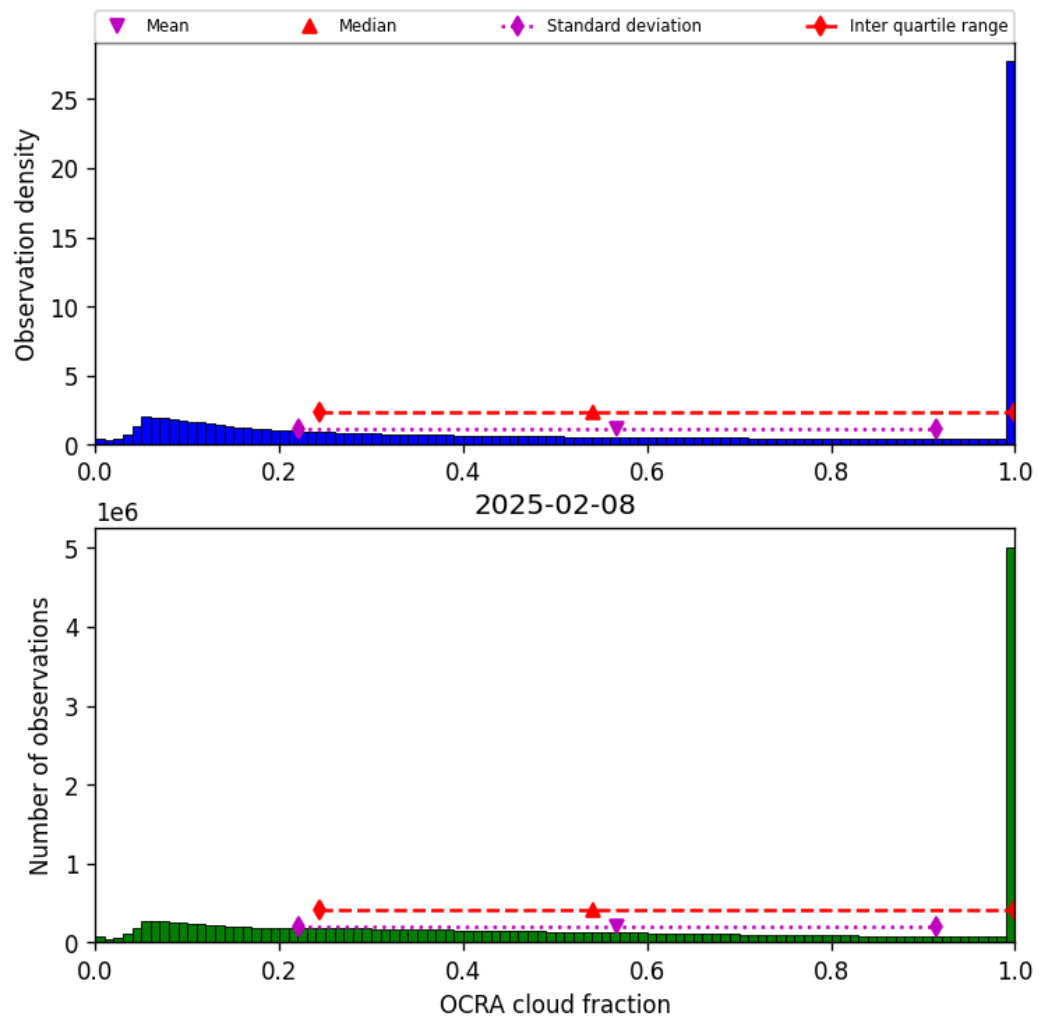
Figure 48: Histogram of “OCRA cloud fraction” for 2025-02-08 to 2025-02-09
