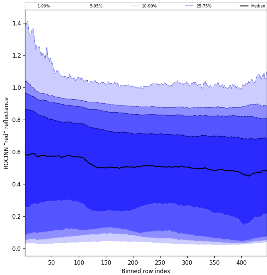
Figure 67: Along track statistics of “ROCINN “red” reflectance” for 2025-02-08 to 2025-02-09
