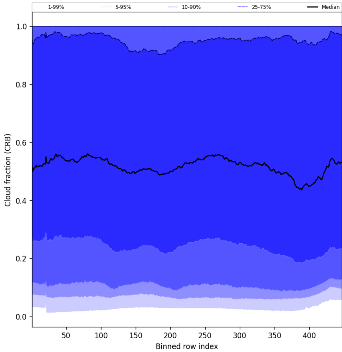
Figure 56: Along track statistics of “Cloud fraction (CRB)” for 2025-02-09 to 2025-02-10
