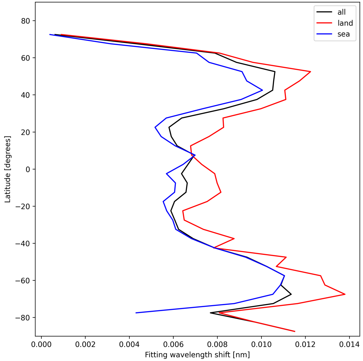
Figure 31: Zonal average of “Fitting wavelength shift” for 2025-02-09 to 2025-02-10.
