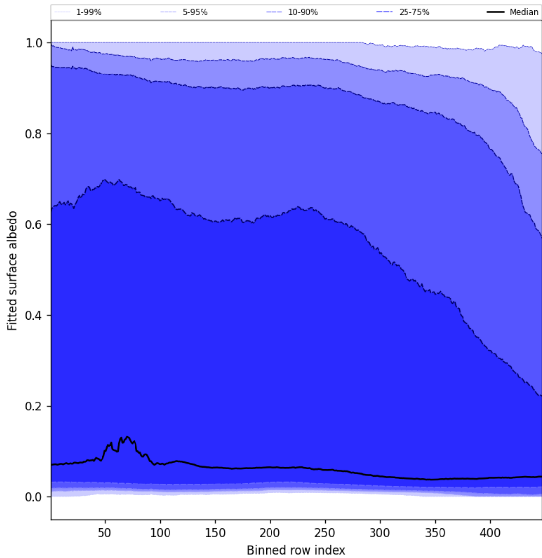
Figure 59: Along track statistics of “Fitted surface albedo” for 2025-02-09 to 2025-02-10
