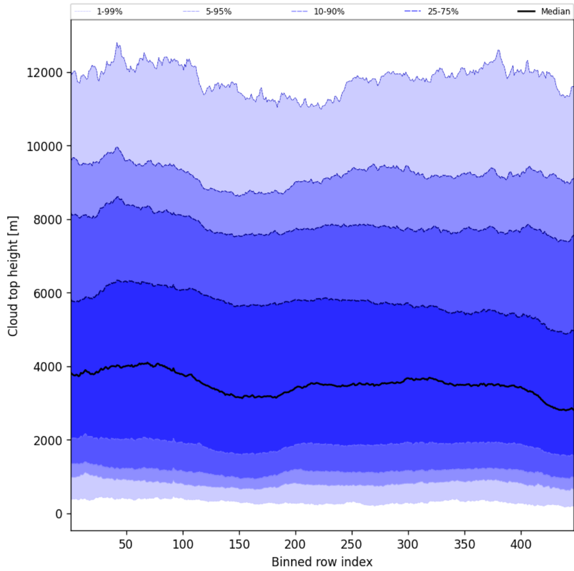
Figure 54: Along track statistics of “Cloud top height” for 2025-02-09 to 2025-02-10
