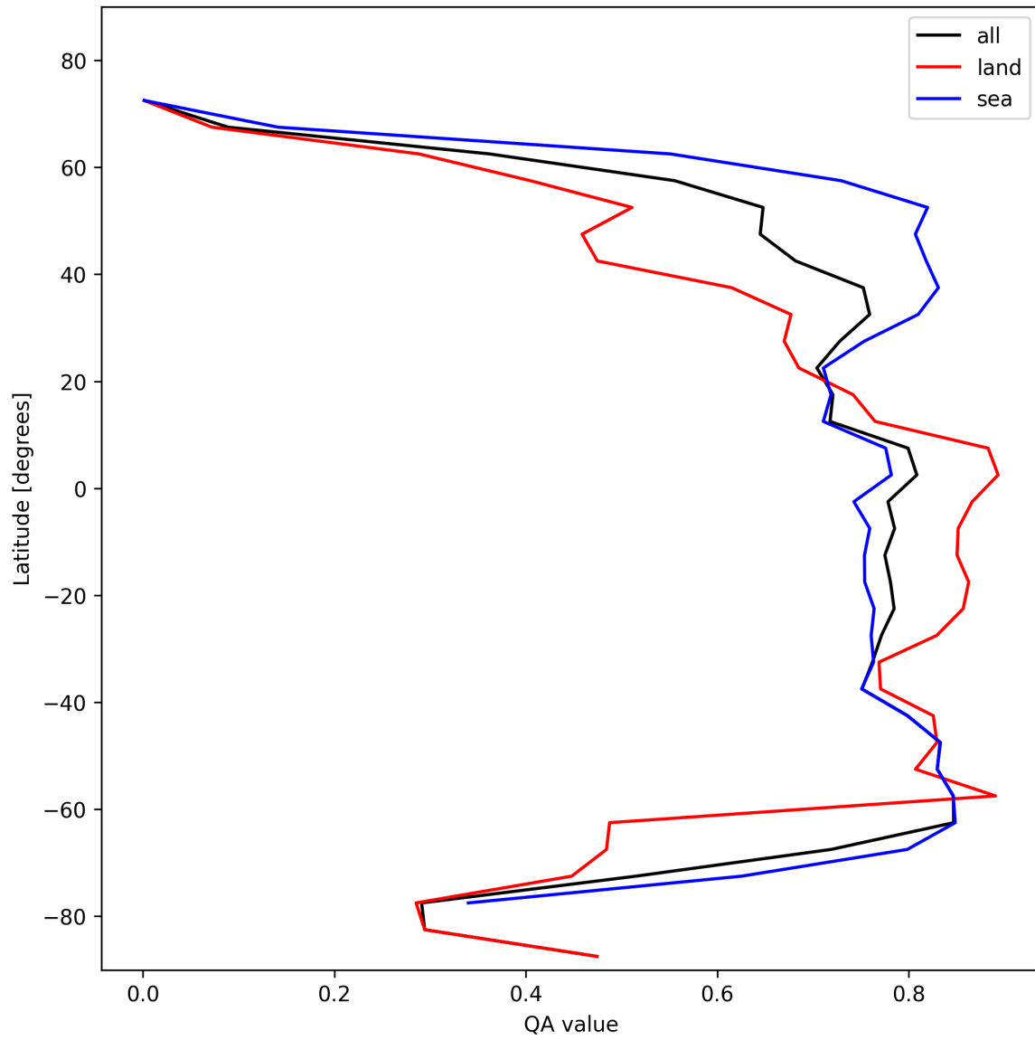
Figure 20: Zonal average of “QA value” for 2025-02-09 to 2025-02-10.
