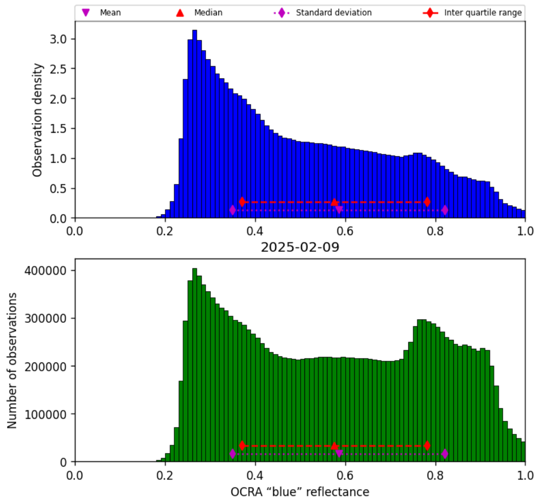
Figure 49: Histogram of “OCRA “blue” reflectance” for 2025-02-09 to 2025-02-10
