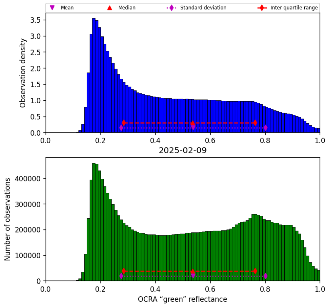
Figure 50: Histogram of “OCRA “green” reflectance” for 2025-02-09 to 2025-02-10
