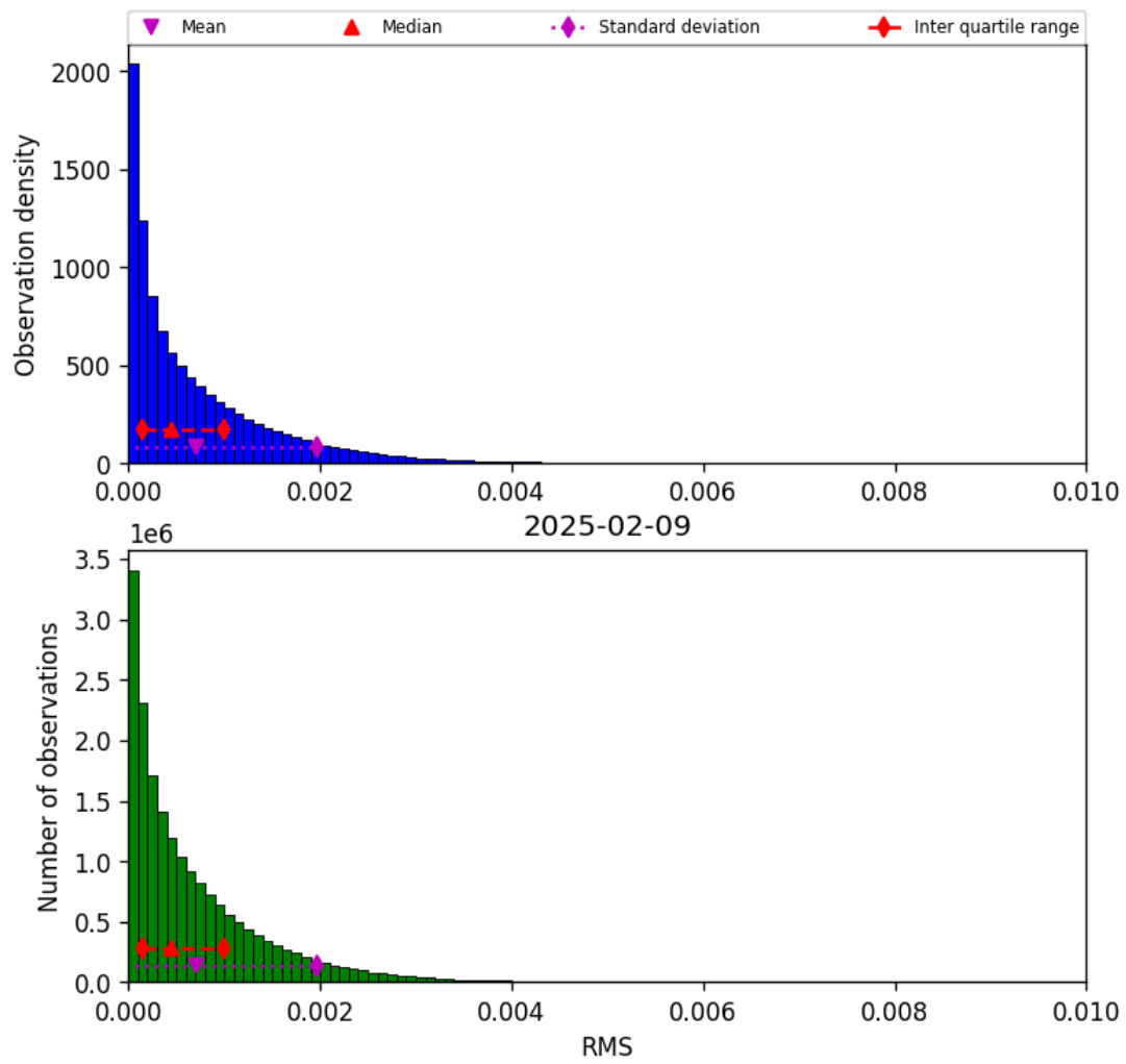
Figure 45: Histogram of “RMS” for 2025-02-09 to 2025-02-10
