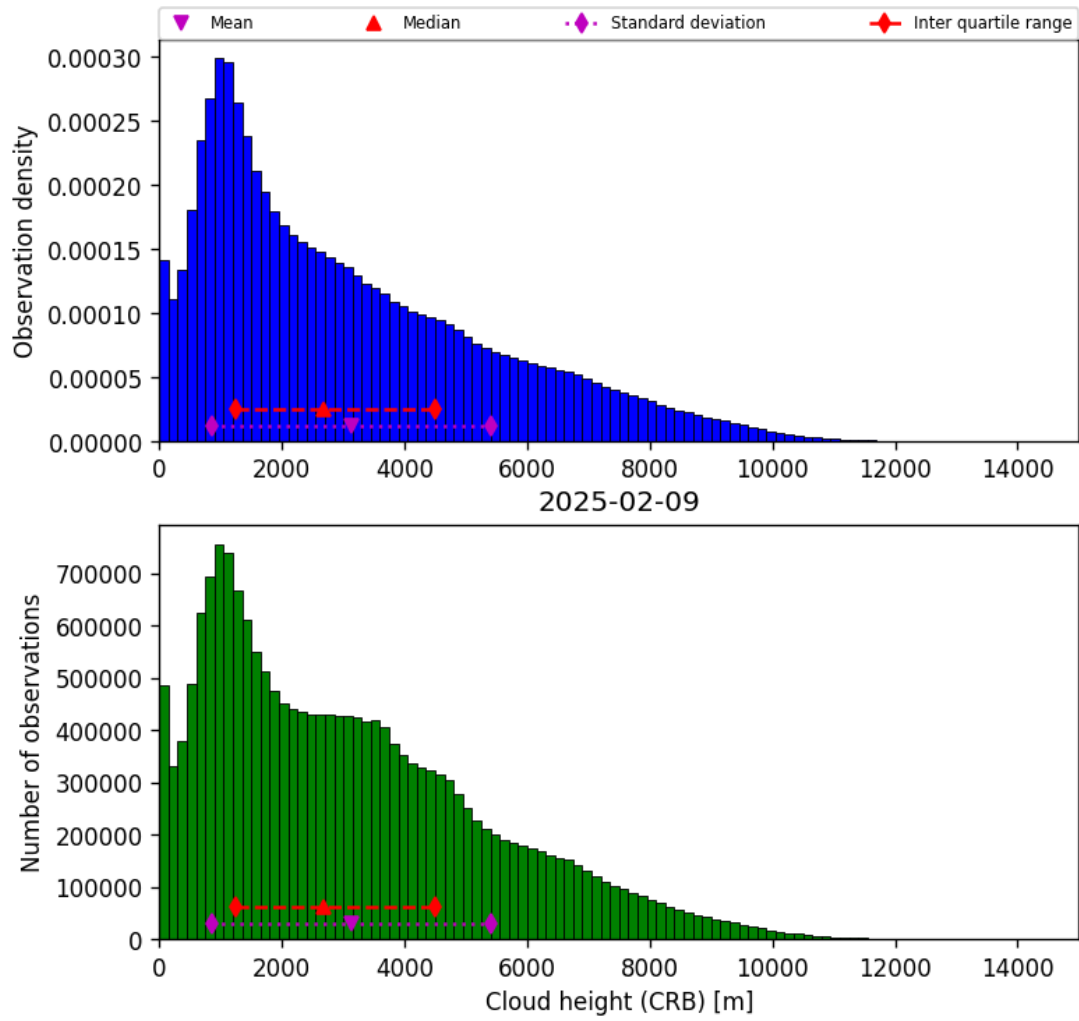
Figure 41: Histogram of “Cloud height (CRB)” for 2025-02-09 to 2025-02-10
