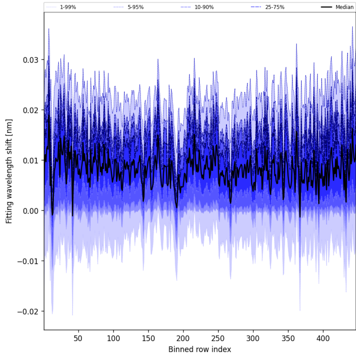
Figure 63: Along track statistics of “Fitting wavelength shift” for 2025-02-09 to 2025-02-10
