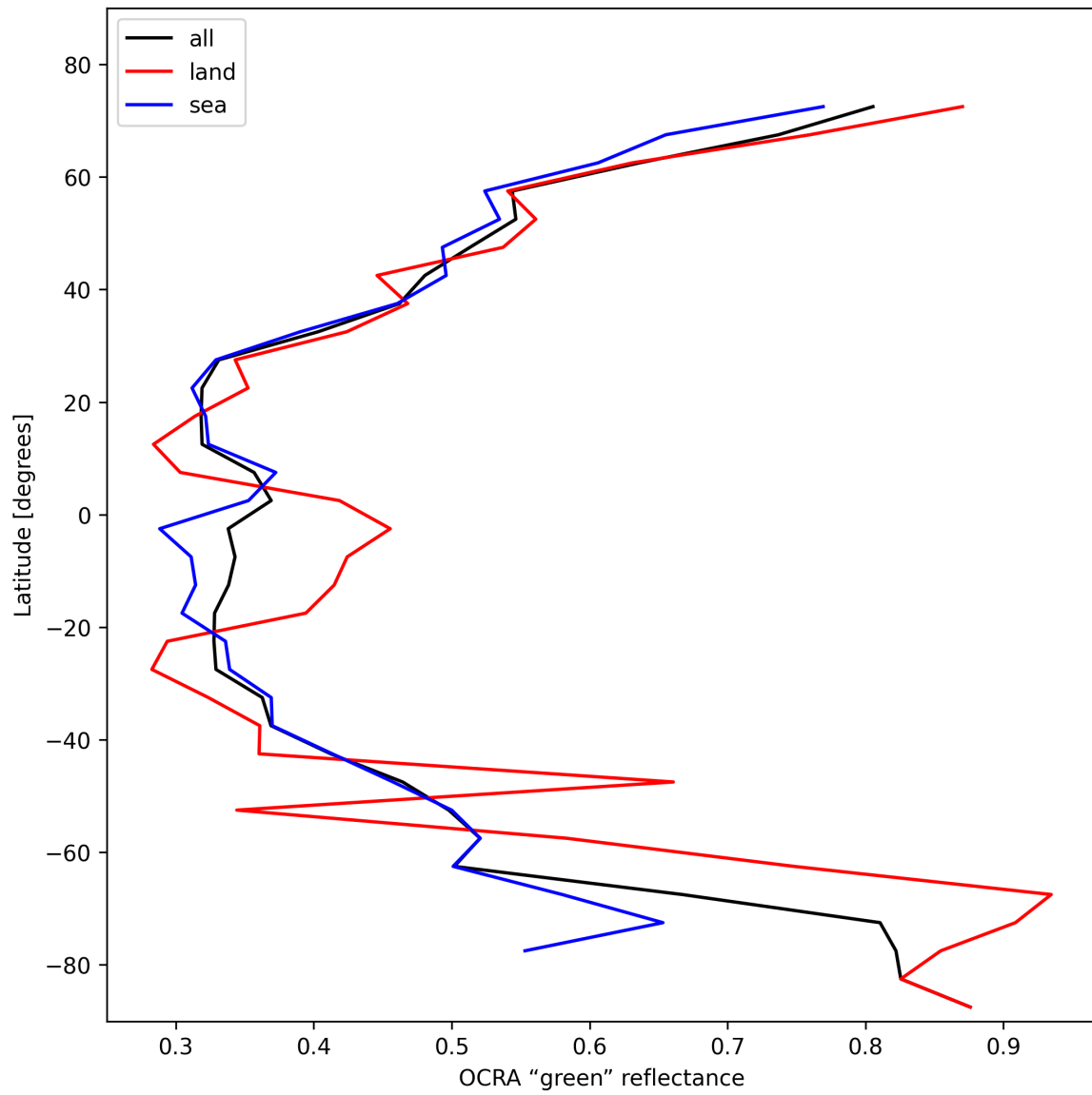
Figure 34: Zonal average of “OCRA “green” reflectance” for 2025-02-09 to 2025-02-10.
