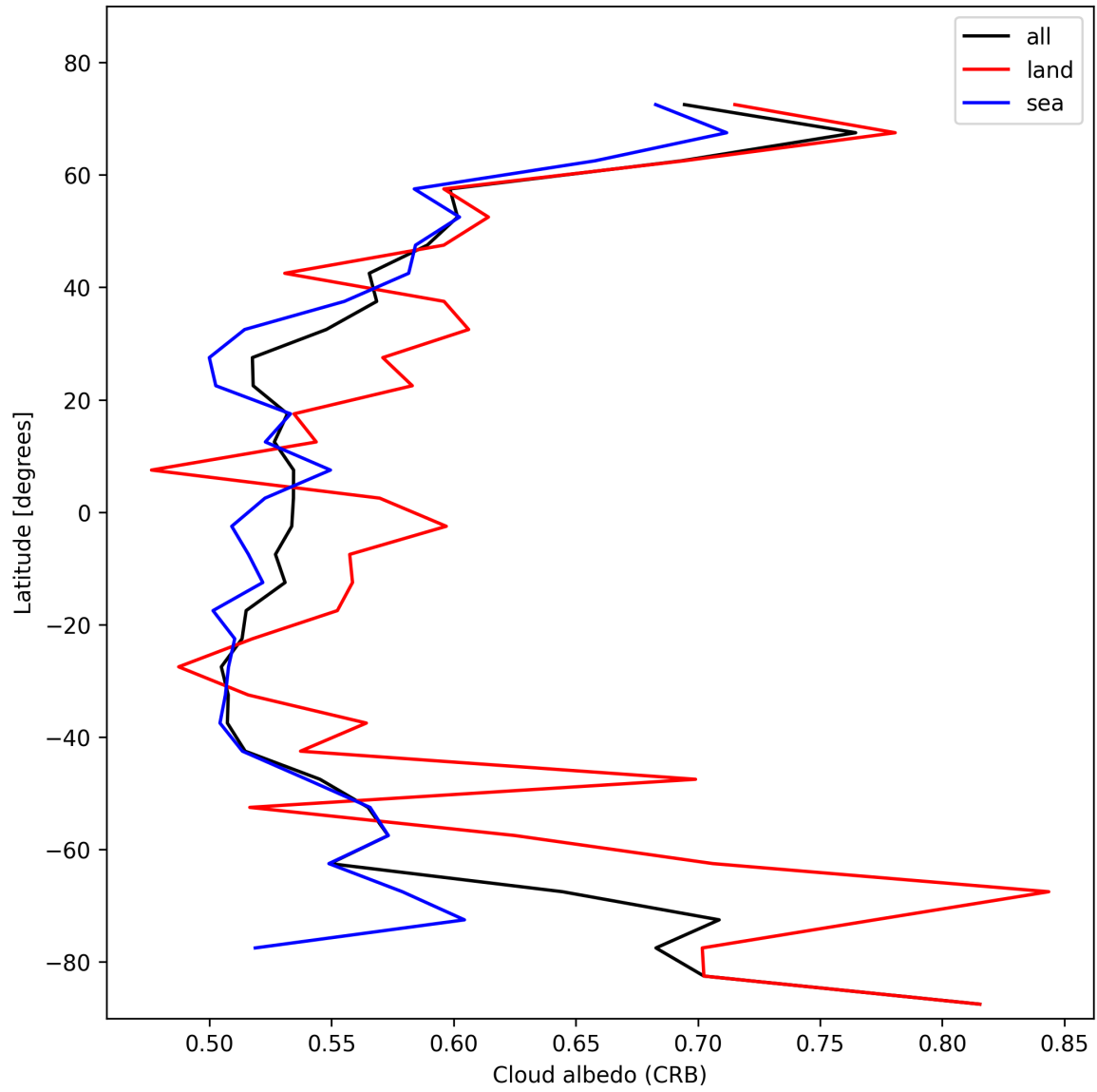
Figure 26: Zonal average of “Cloud albedo (CRB)” for 2025-02-09 to 2025-02-10.
