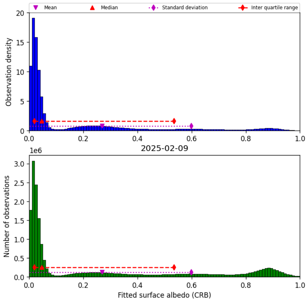
Figure 44: Histogram of “Fitted surface albedo (CRB)” for 2025-02-09 to 2025-02-10
