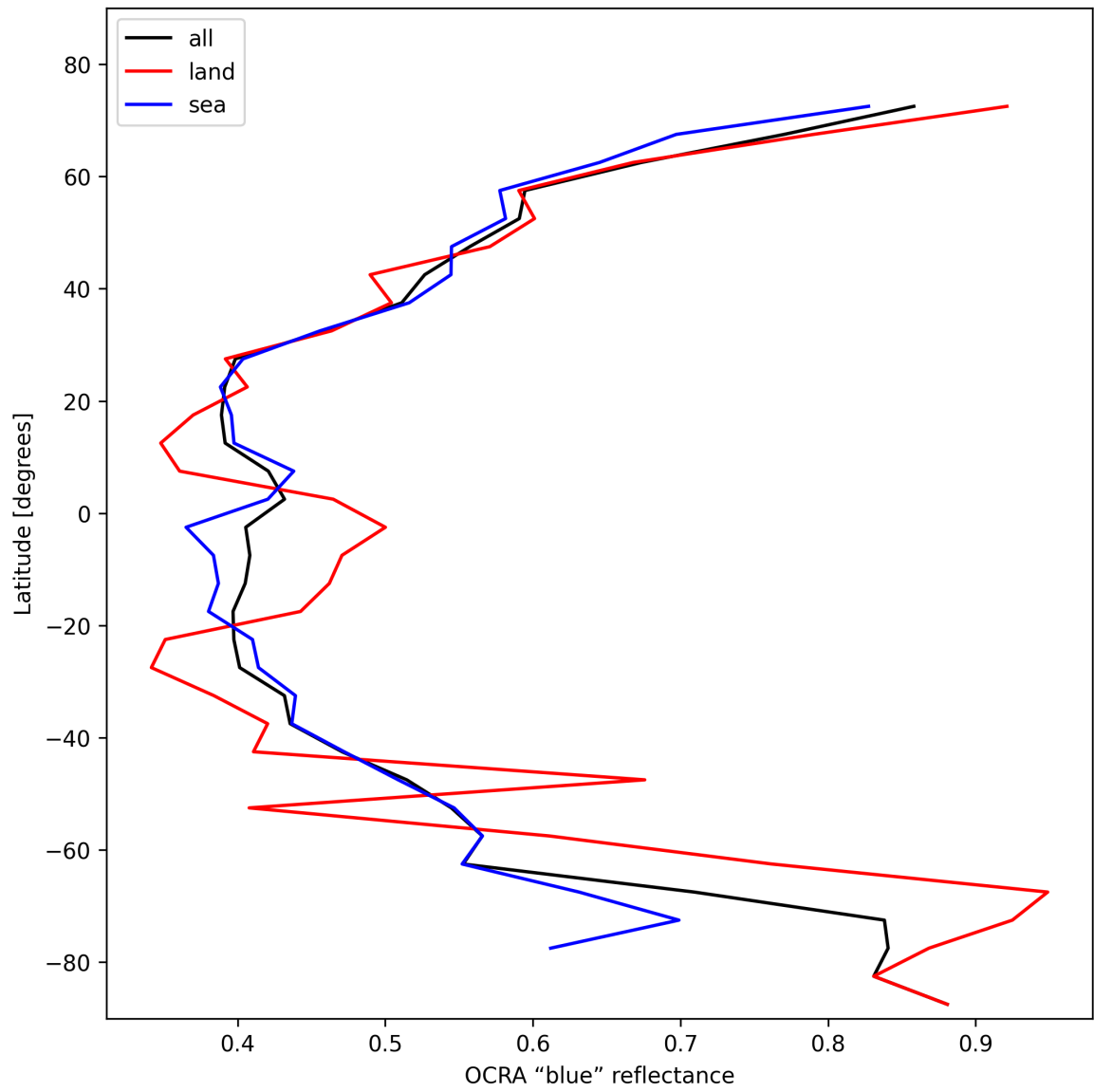
Figure 33: Zonal average of “OCRA “blue” reflectance” for 2025-02-09 to 2025-02-10.
