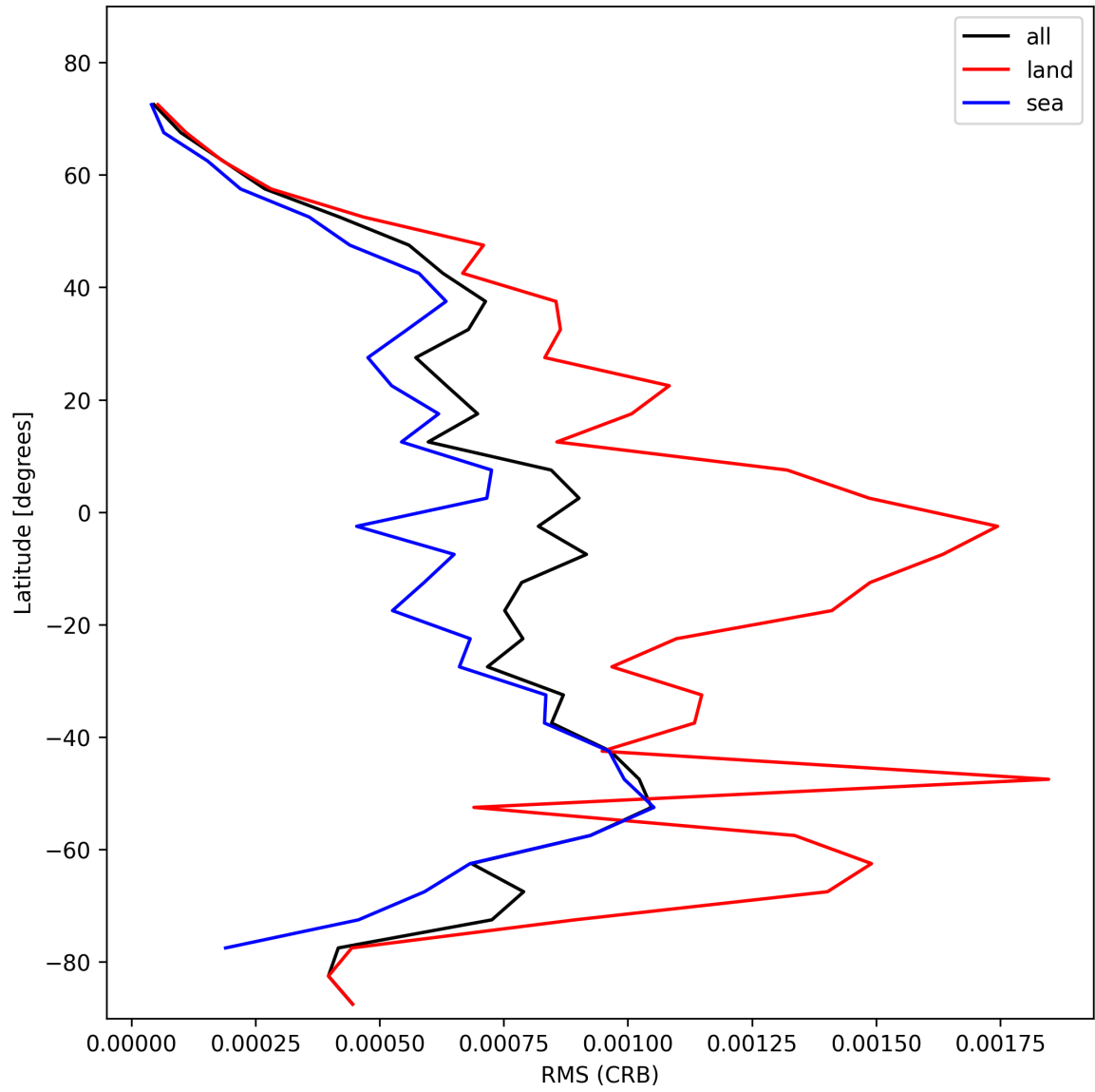
Figure 30: Zonal average of “RMS (CRB)” for 2025-02-09 to 2025-02-10.
