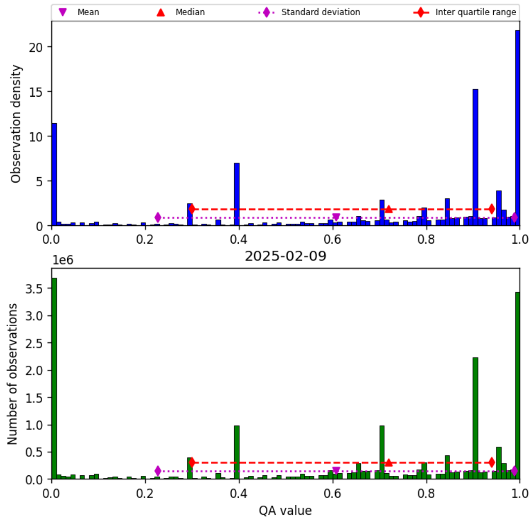
Figure 36: Histogram of “QA value” for 2025-02-09 to 2025-02-10
