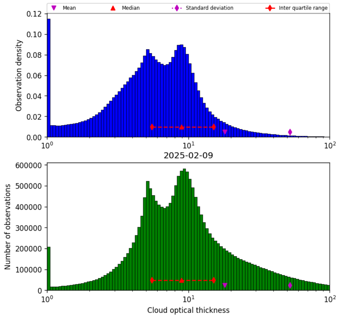
Figure 39: Histogram of “Cloud optical thickness” for 2025-02-09 to 2025-02-10
