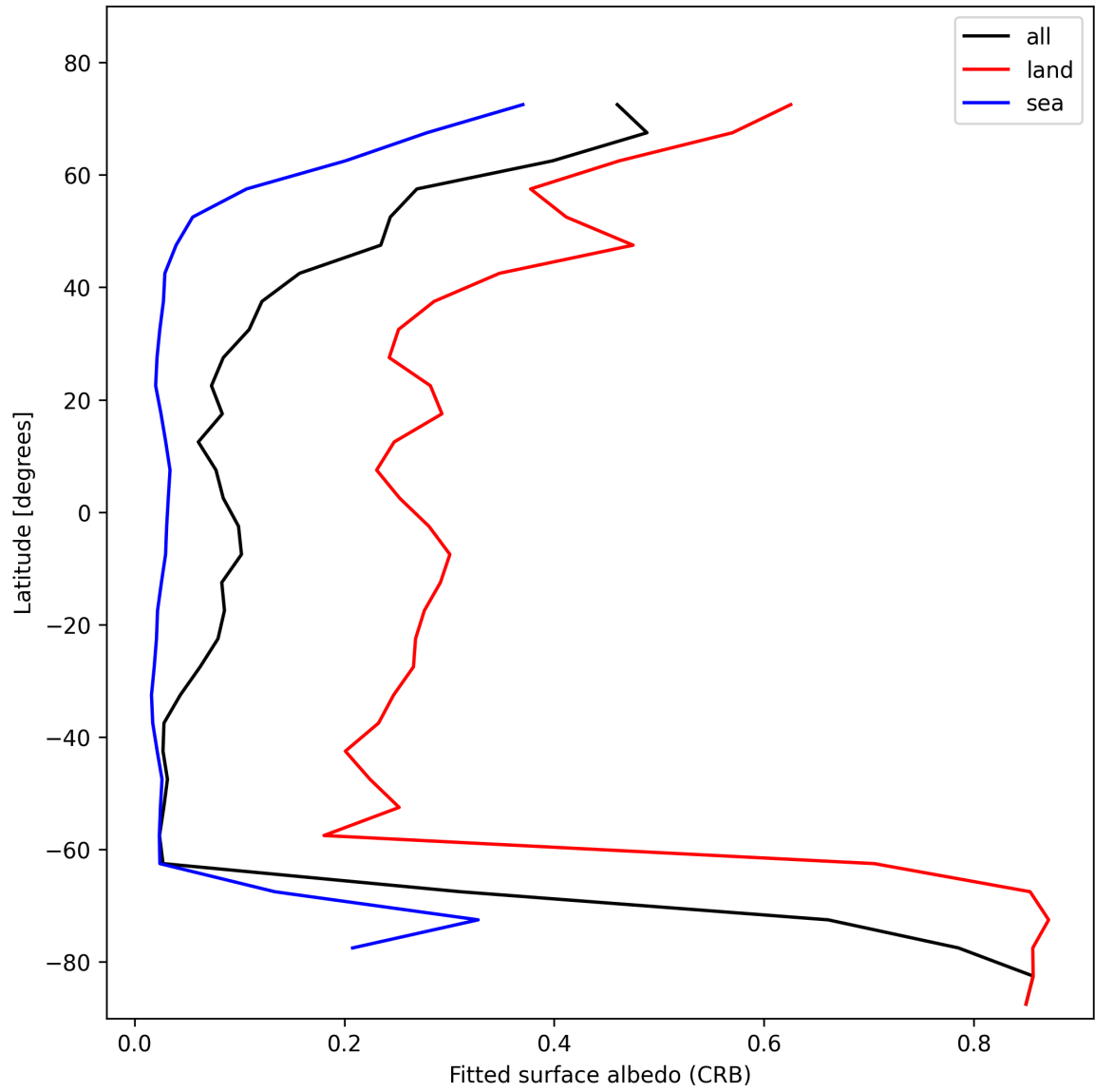
Figure 28: Zonal average of “Fitted surface albedo (CRB)” for 2025-02-09 to 2025-02-10.
