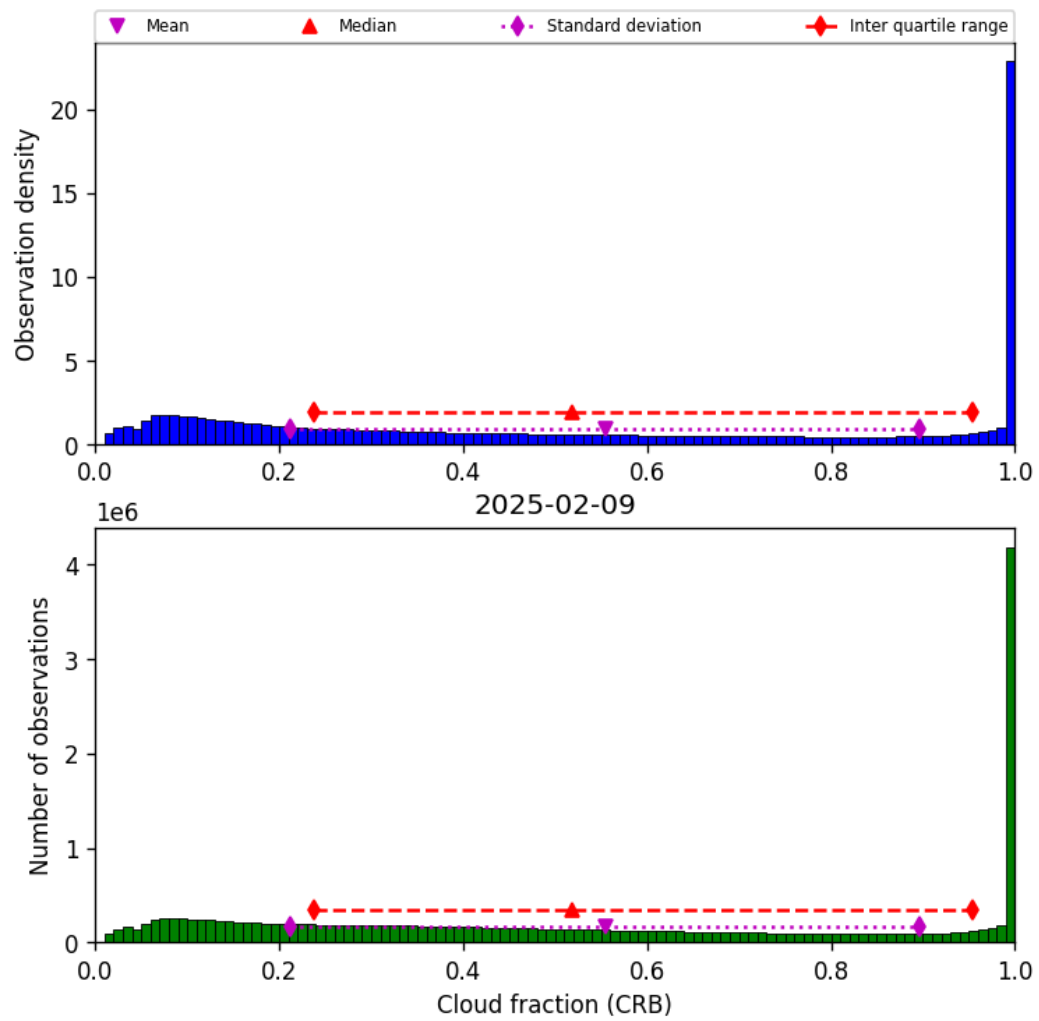
Figure 40: Histogram of “Cloud fraction (CRB)” for 2025-02-09 to 2025-02-10
