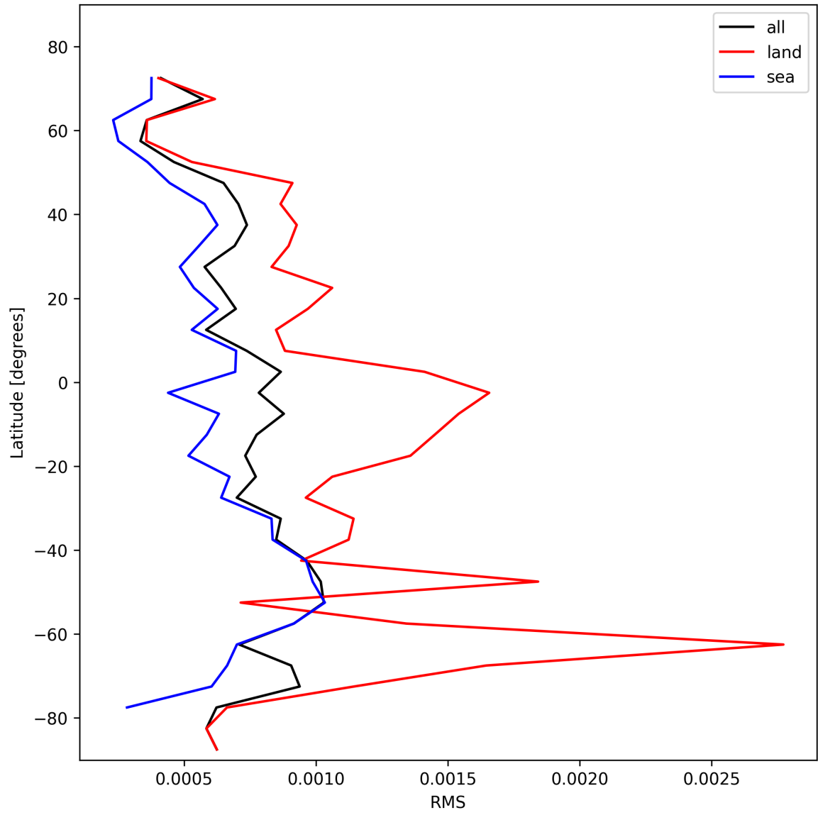
Figure 29: Zonal average of “RMS” for 2025-02-09 to 2025-02-10.
