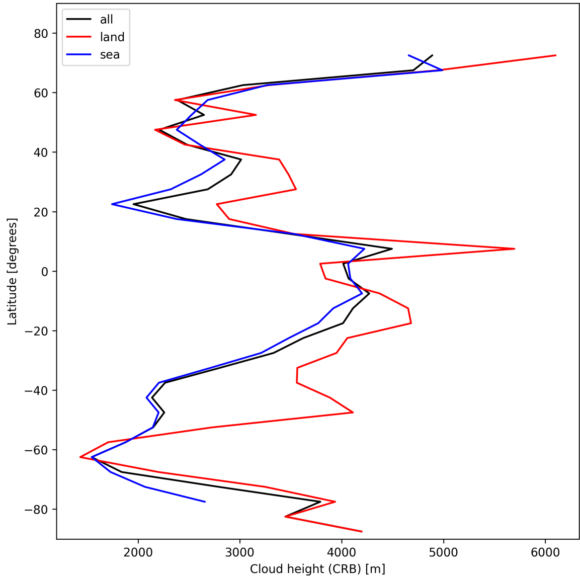
Figure 25: Zonal average of “Cloud height (CRB)” for 2025-02-09 to 2025-02-10.
