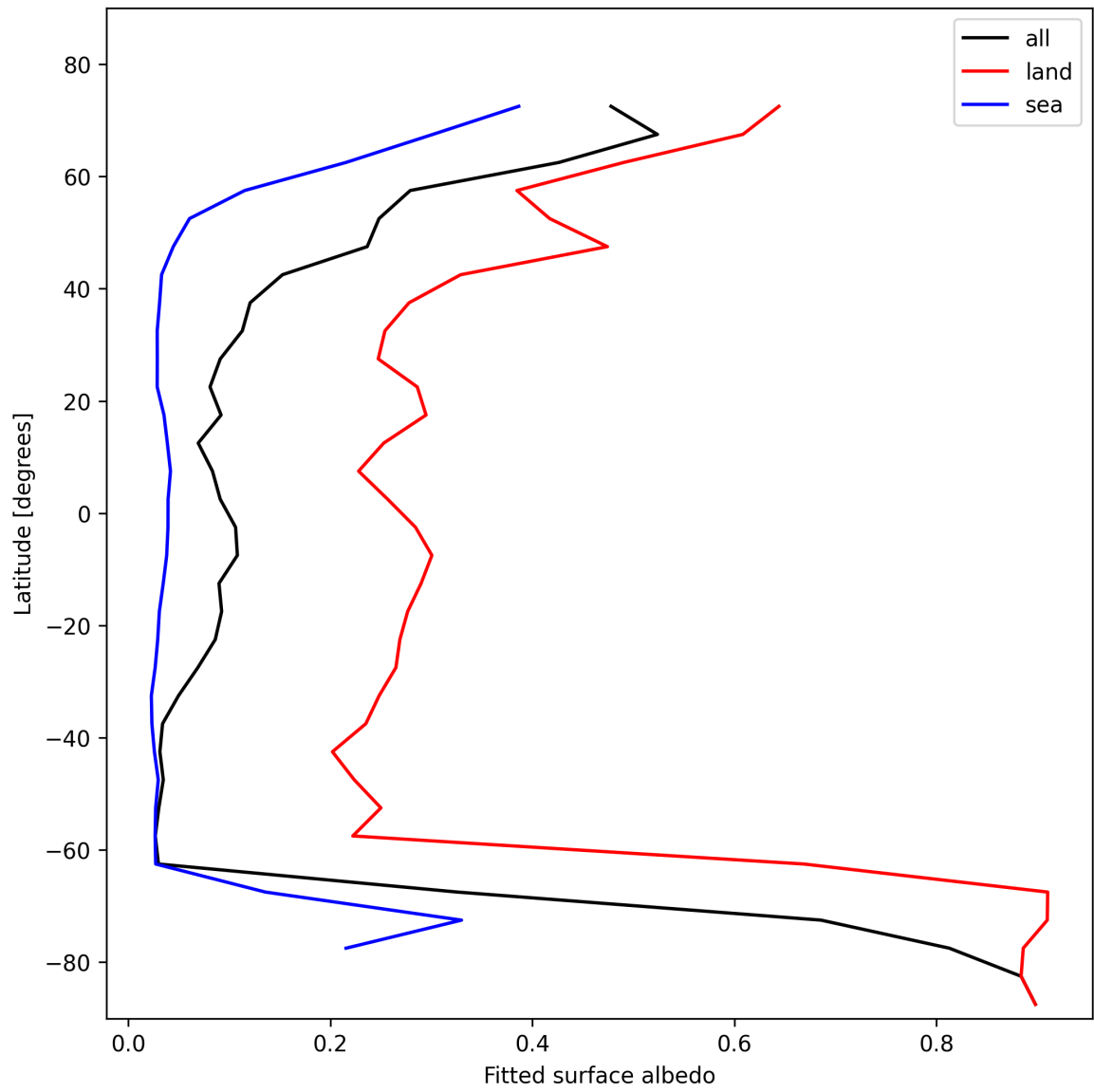
Figure 27: Zonal average of “Fitted surface albedo” for 2025-02-09 to 2025-02-10.
