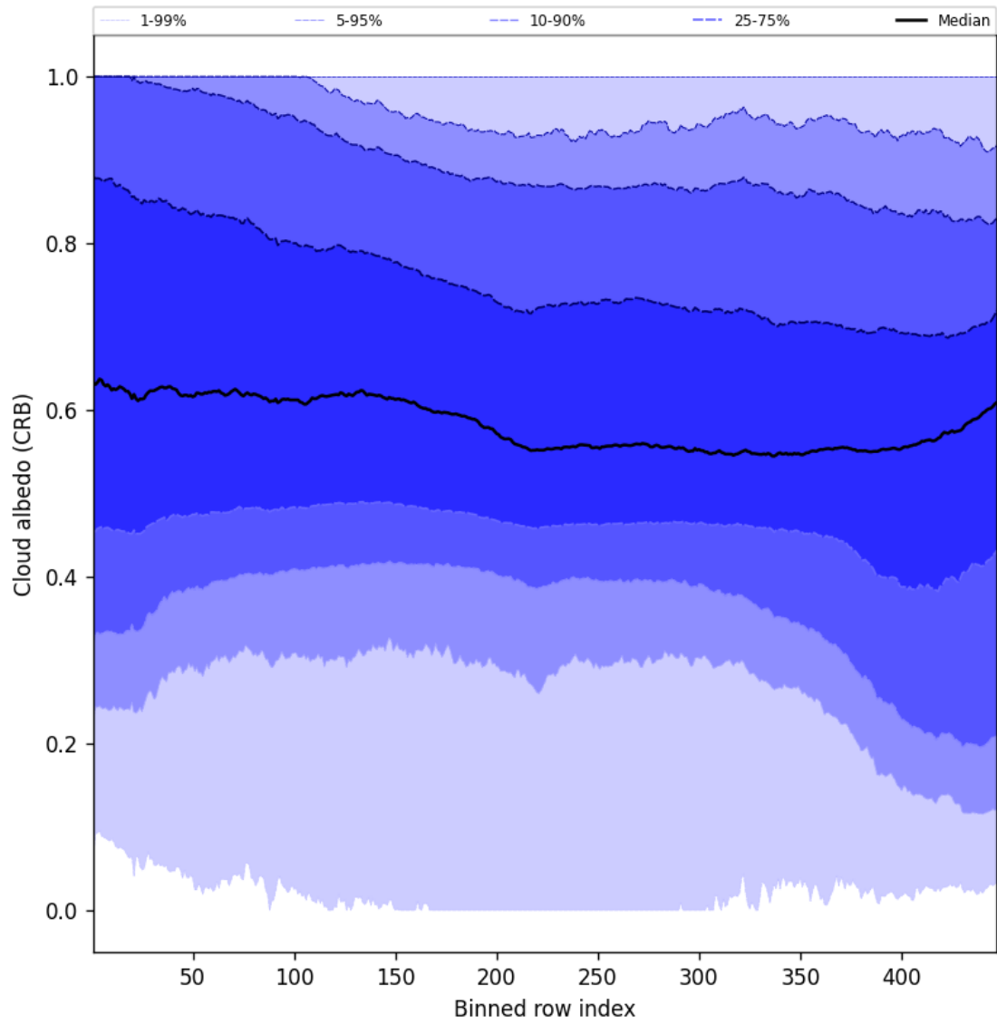
Figure 58: Along track statistics of “Cloud albedo (CRB)” for 2025-02-09 to 2025-02-10
