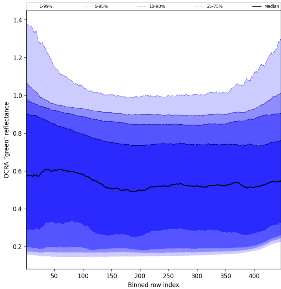
Figure 66: Along track statistics of “OCRA “green” reflectance” for 2025-02-09 to 2025-02-10
