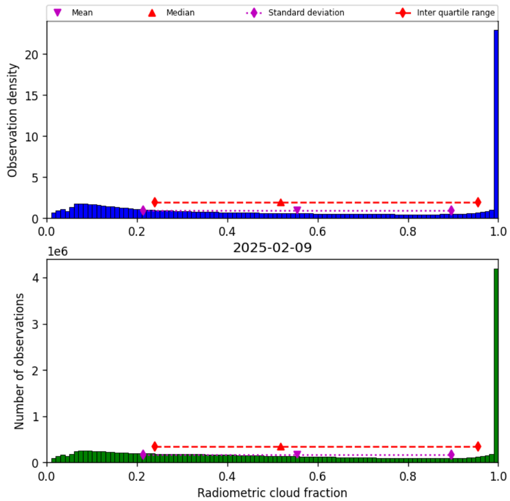
Figure 37: Histogram of “Radiometric cloud fraction” for 2025-02-09 to 2025-02-10
