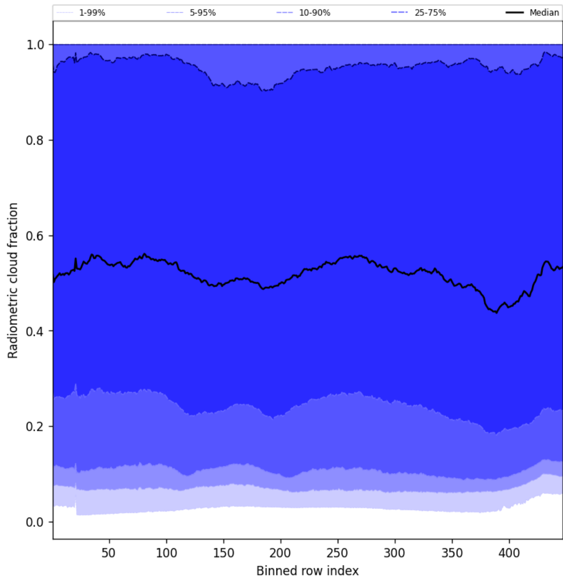
Figure 53: Along track statistics of “Radiometric cloud fraction” for 2025-02-09 to 2025-02-10
