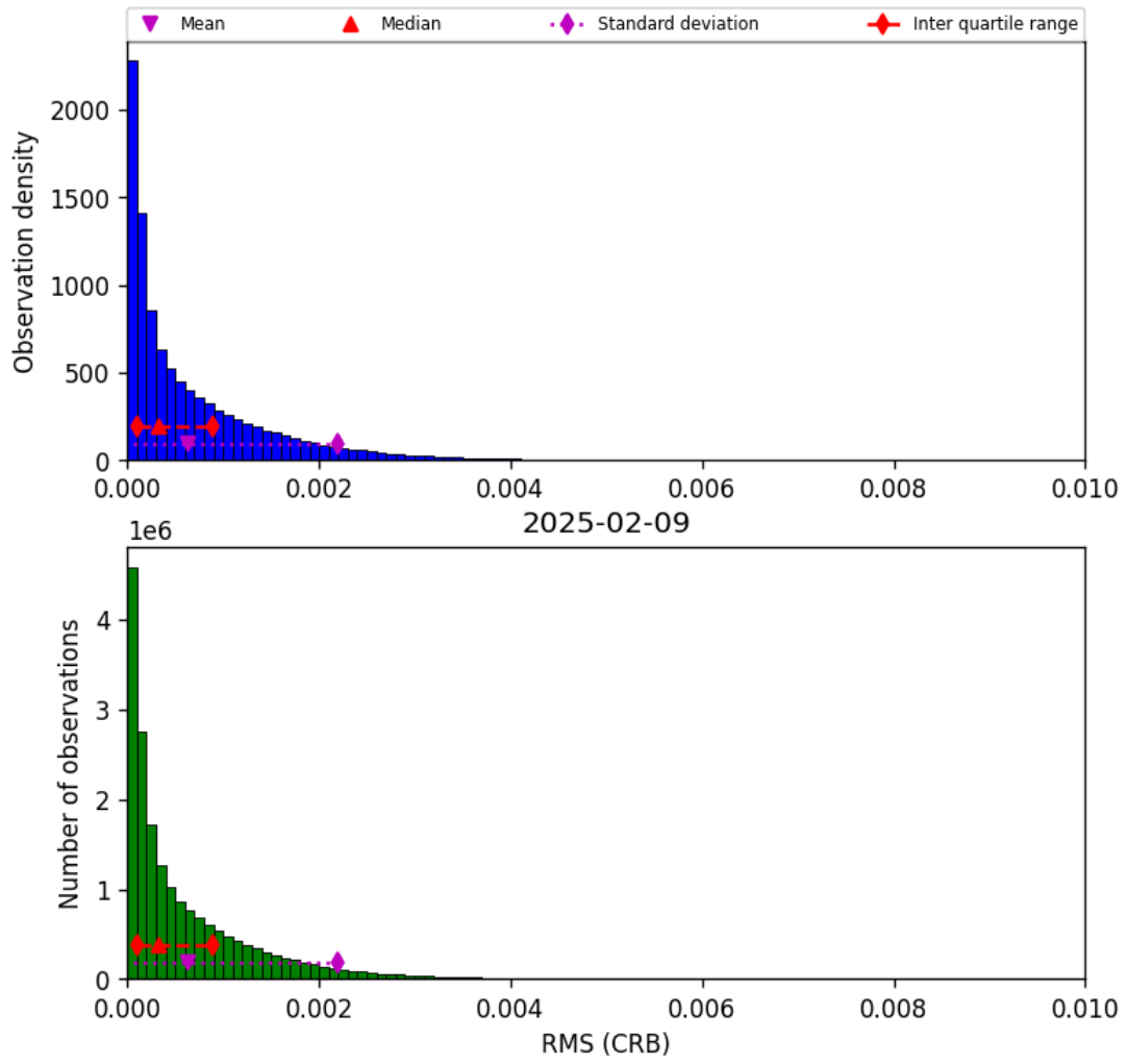
Figure 46: Histogram of "RMS (CRB)" for 2025-02-09 to 2025-02-10
