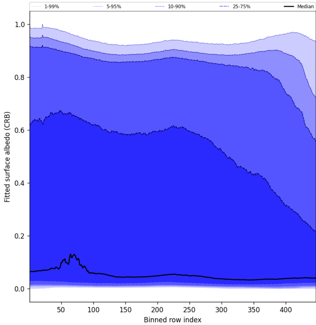
Figure 60: Along track statistics of “Fitted surface albedo (CRB)” for 2025-02-09 to 2025-02-10
