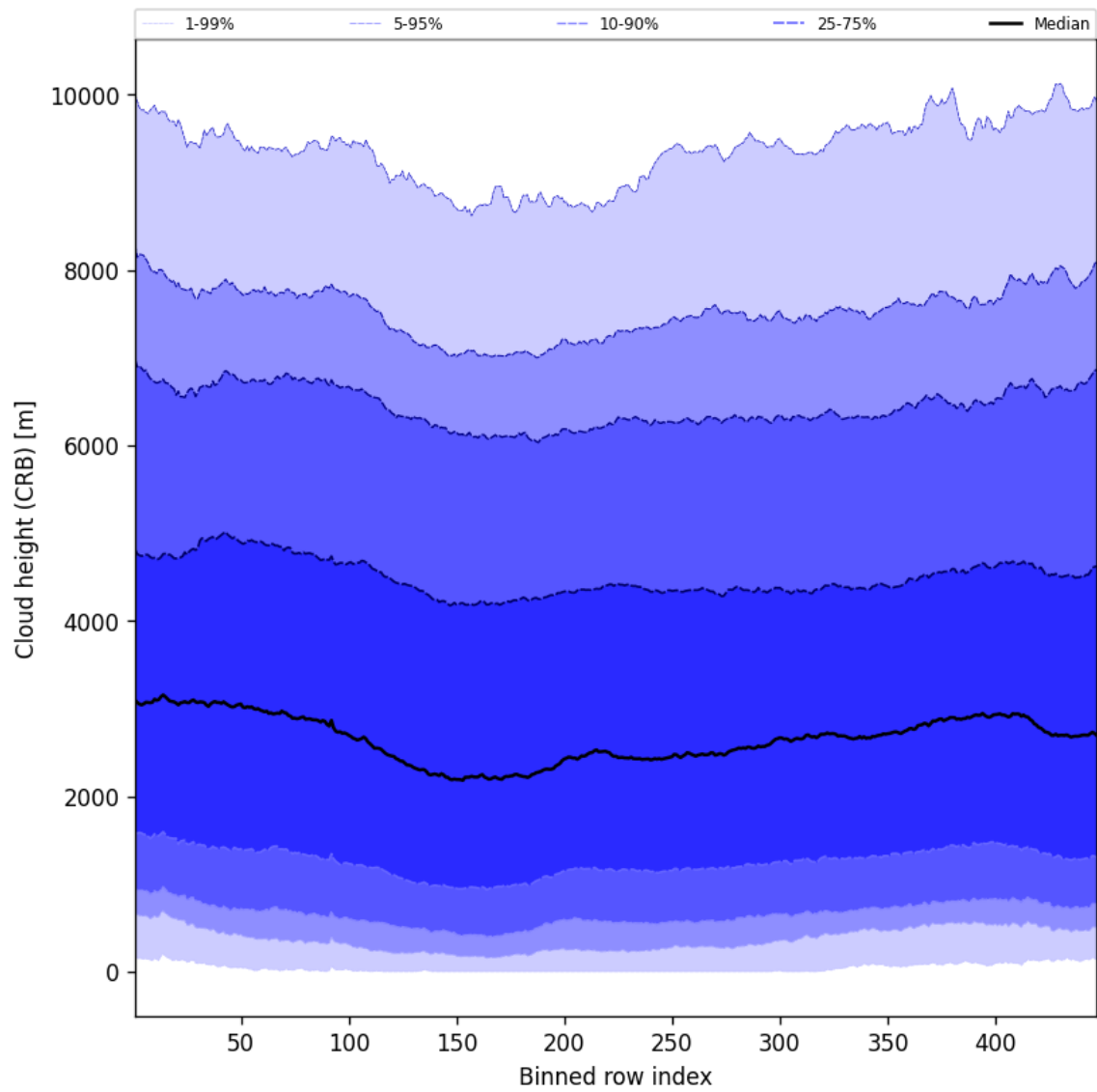
Figure 57: Along track statistics of “Cloud height (CRB)” for 2025-02-09 to 2025-02-10
