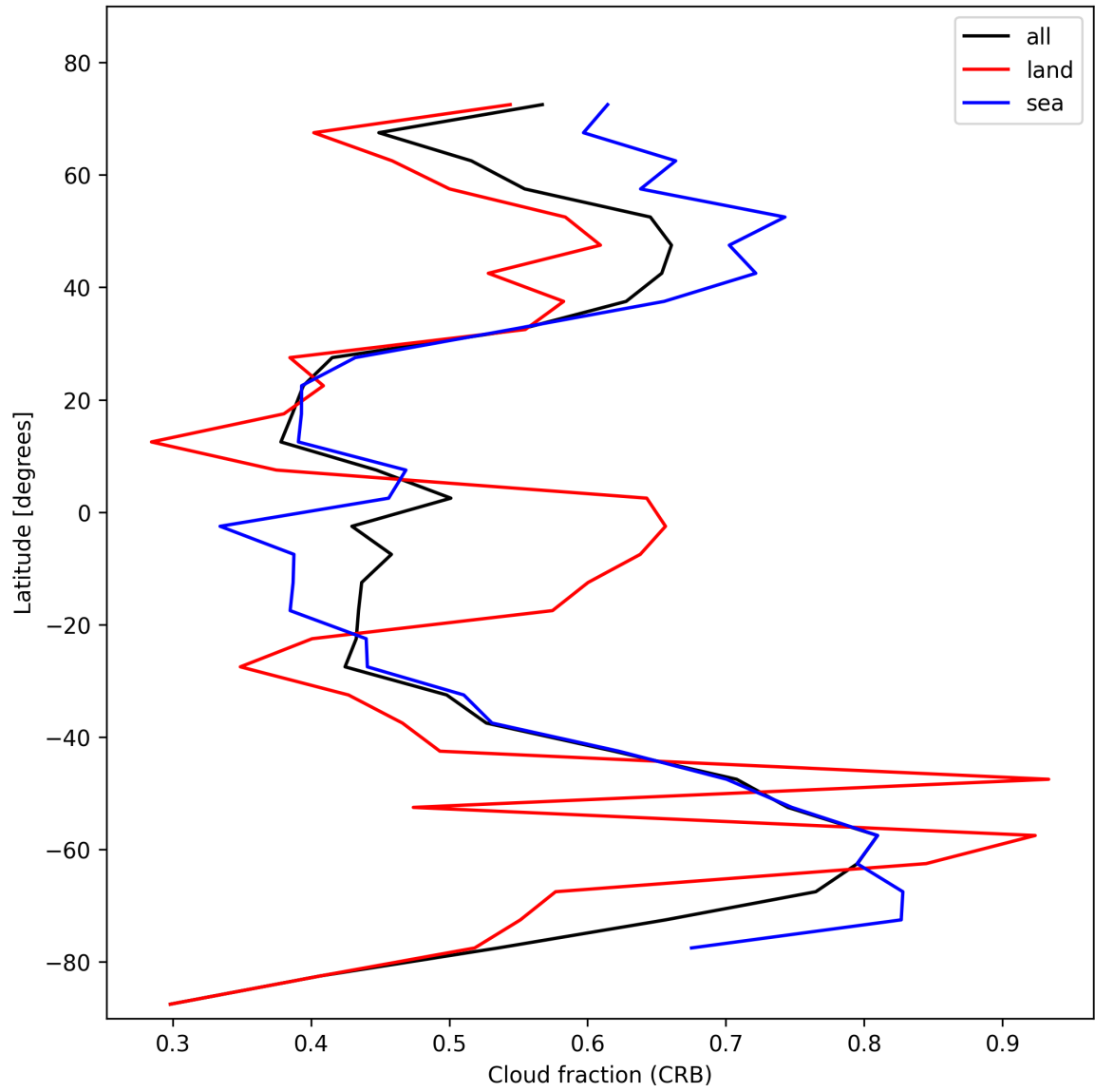
Figure 24: Zonal average of “Cloud fraction (CRB)” for 2025-02-09 to 2025-02-10.
