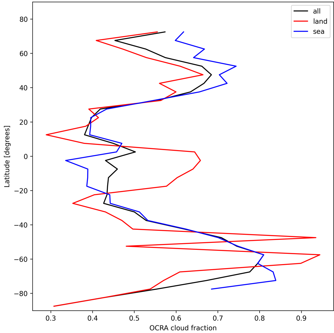
Figure 32: Zonal average of “OCRA cloud fraction” for 2025-02-09 to 2025-02-10.
