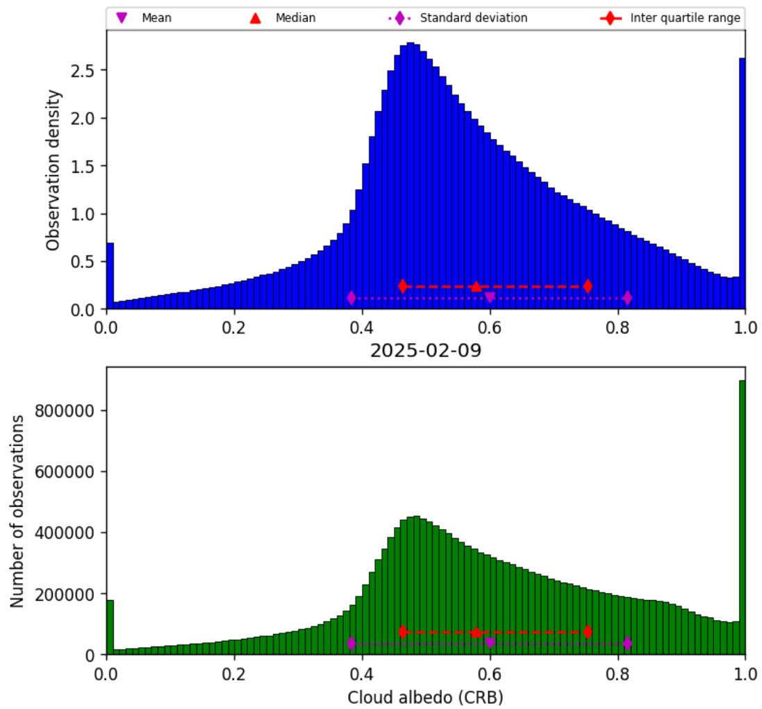
Figure 42: Histogram of “Cloud albedo (CRB)” for 2025-02-09 to 2025-02-10
