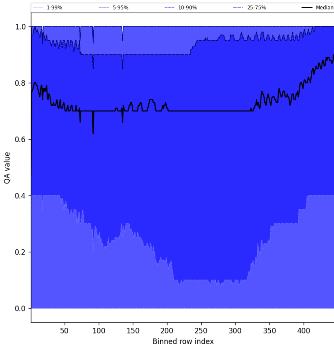
Figure 52: Along track statistics of “QA value” for 2025-02-09 to 2025-02-10
