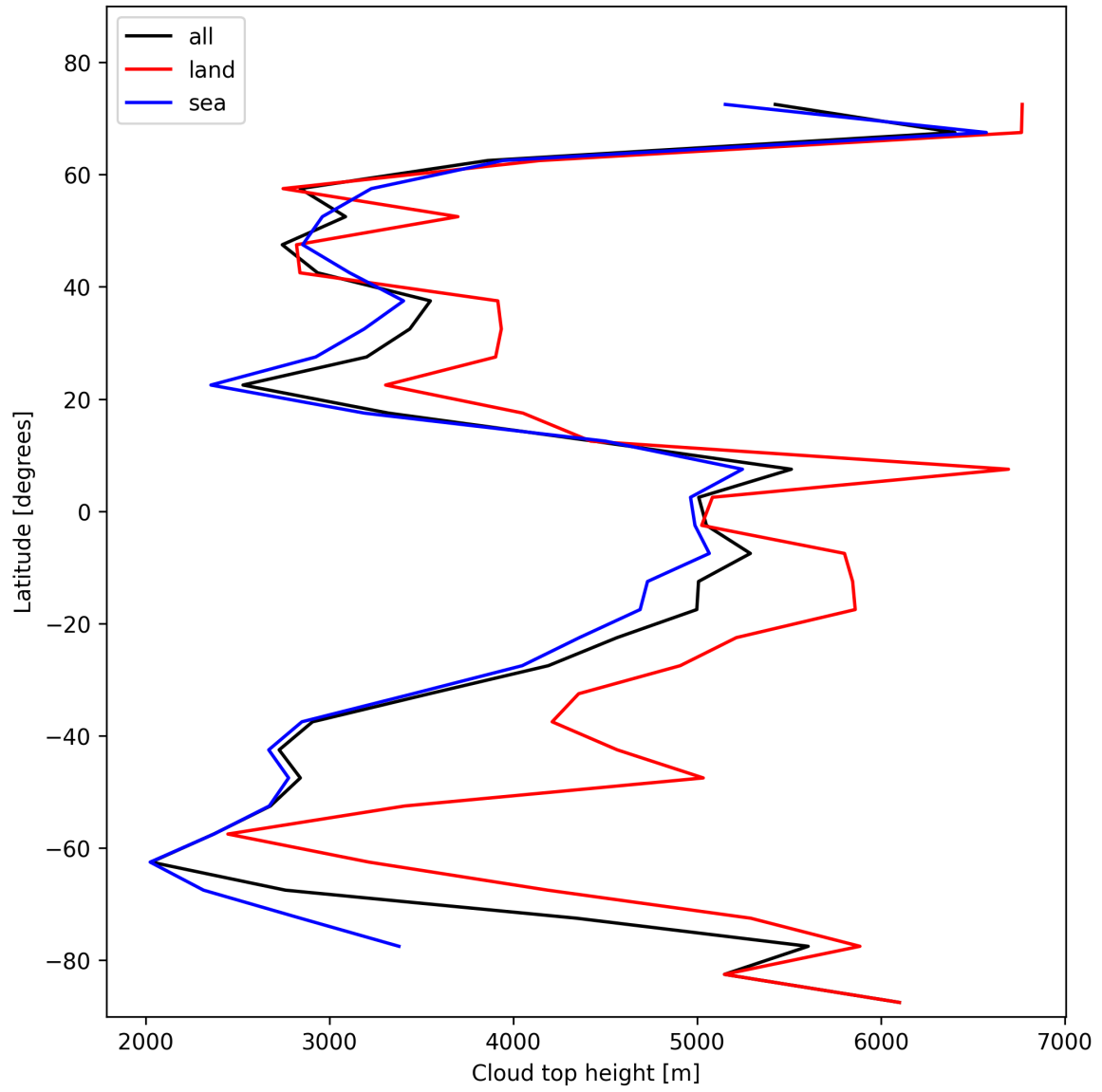
Figure 22: Zonal average of “Cloud top height” for 2025-02-09 to 2025-02-10.
