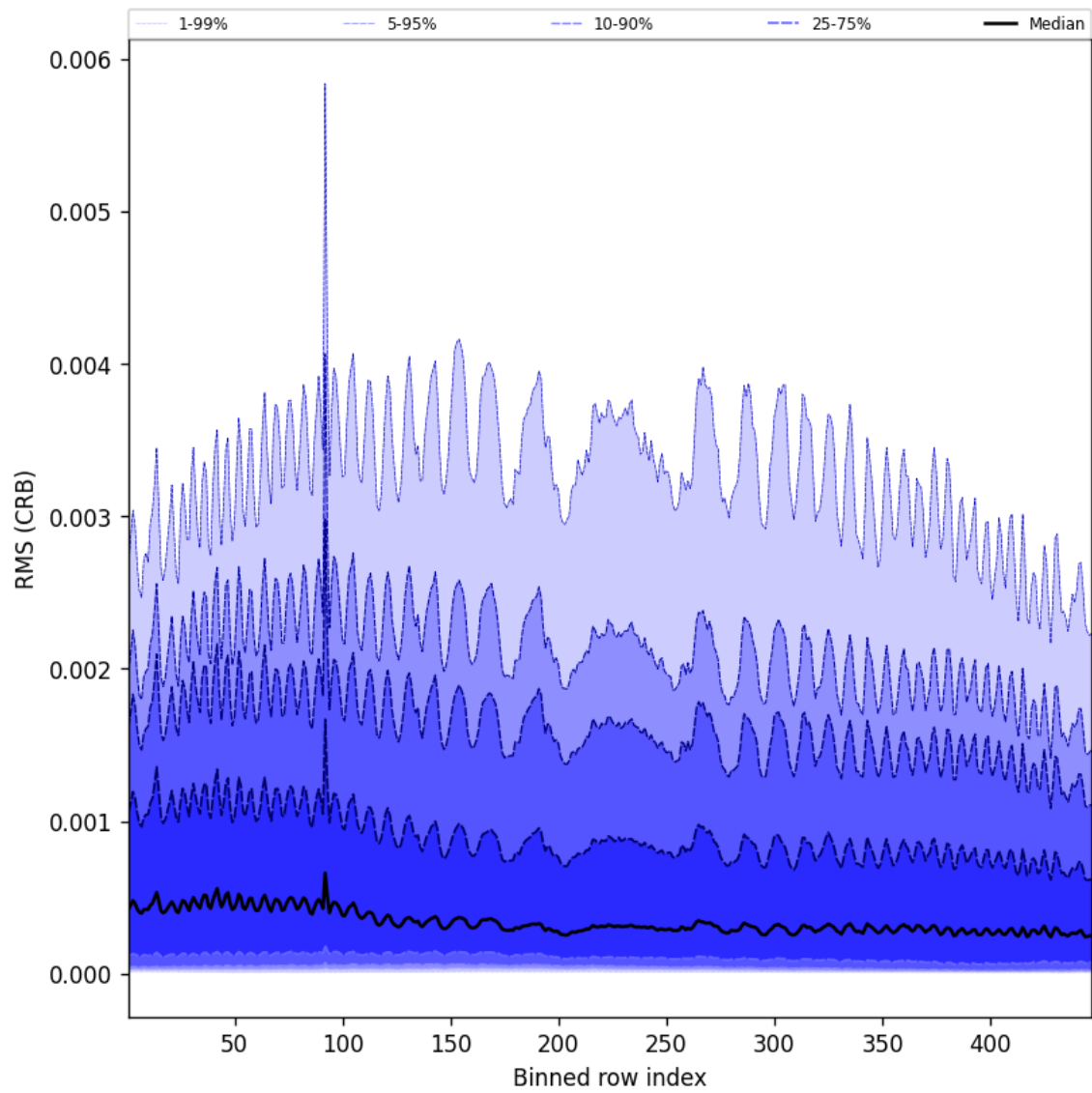
Figure 62: Along track statistics of “RMS (CRB)” for 2025-02-09 to 2025-02-10
