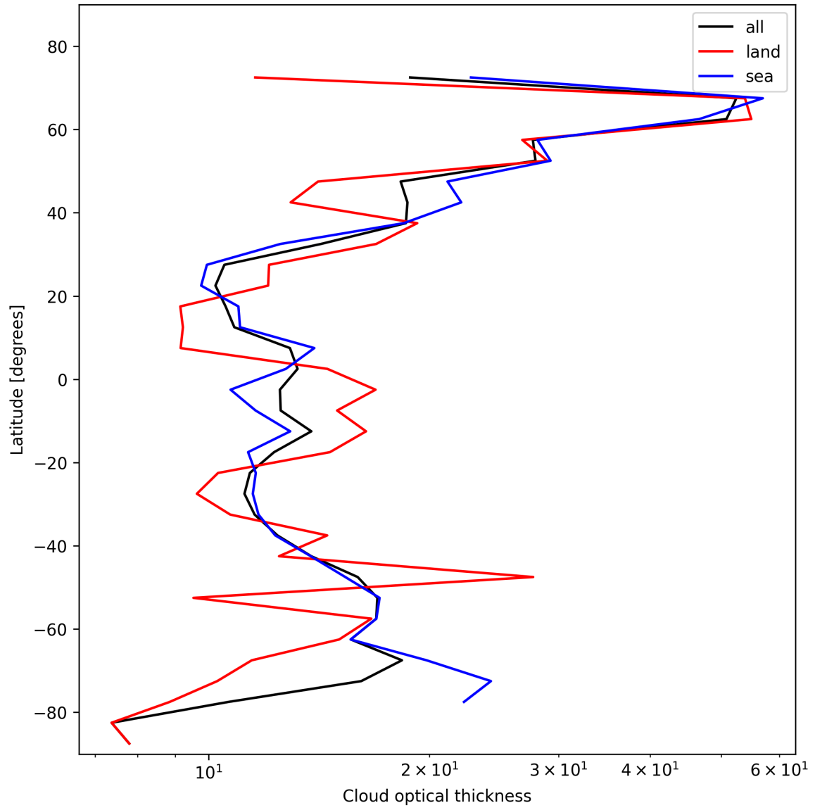
Figure 23: Zonal average of “Cloud optical thickness” for 2025-02-09 to 2025-02-10.
