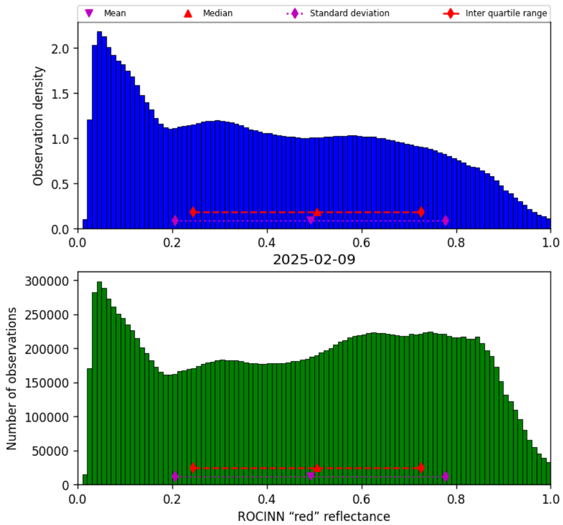
Figure 51: Histogram of “ROCINN “red” reflectance” for 2025-02-09 to 2025-02-10
