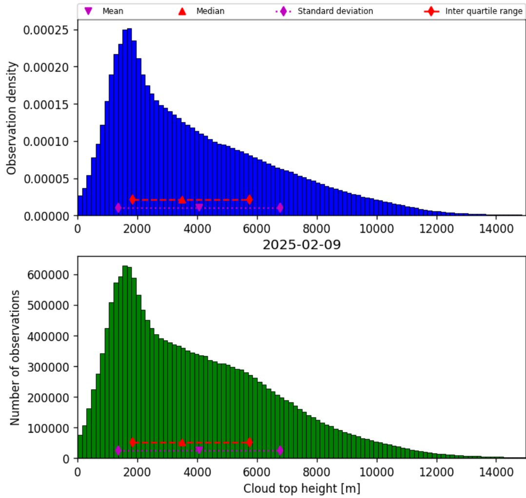
Figure 38: Histogram of “Cloud top height” for 2025-02-09 to 2025-02-10
