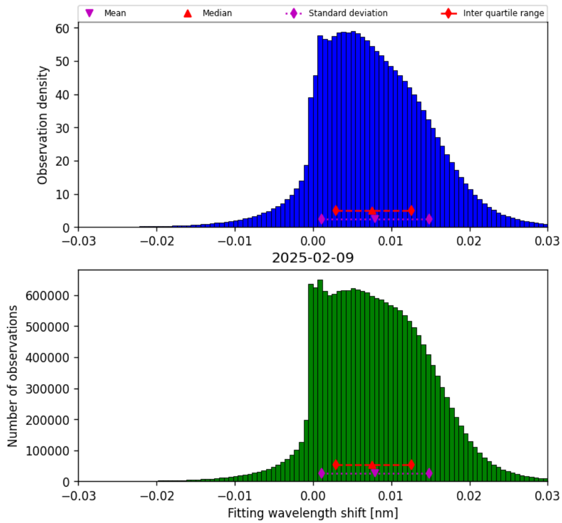
Figure 47: Histogram of “Fitting wavelength shift” for 2025-02-09 to 2025-02-10
