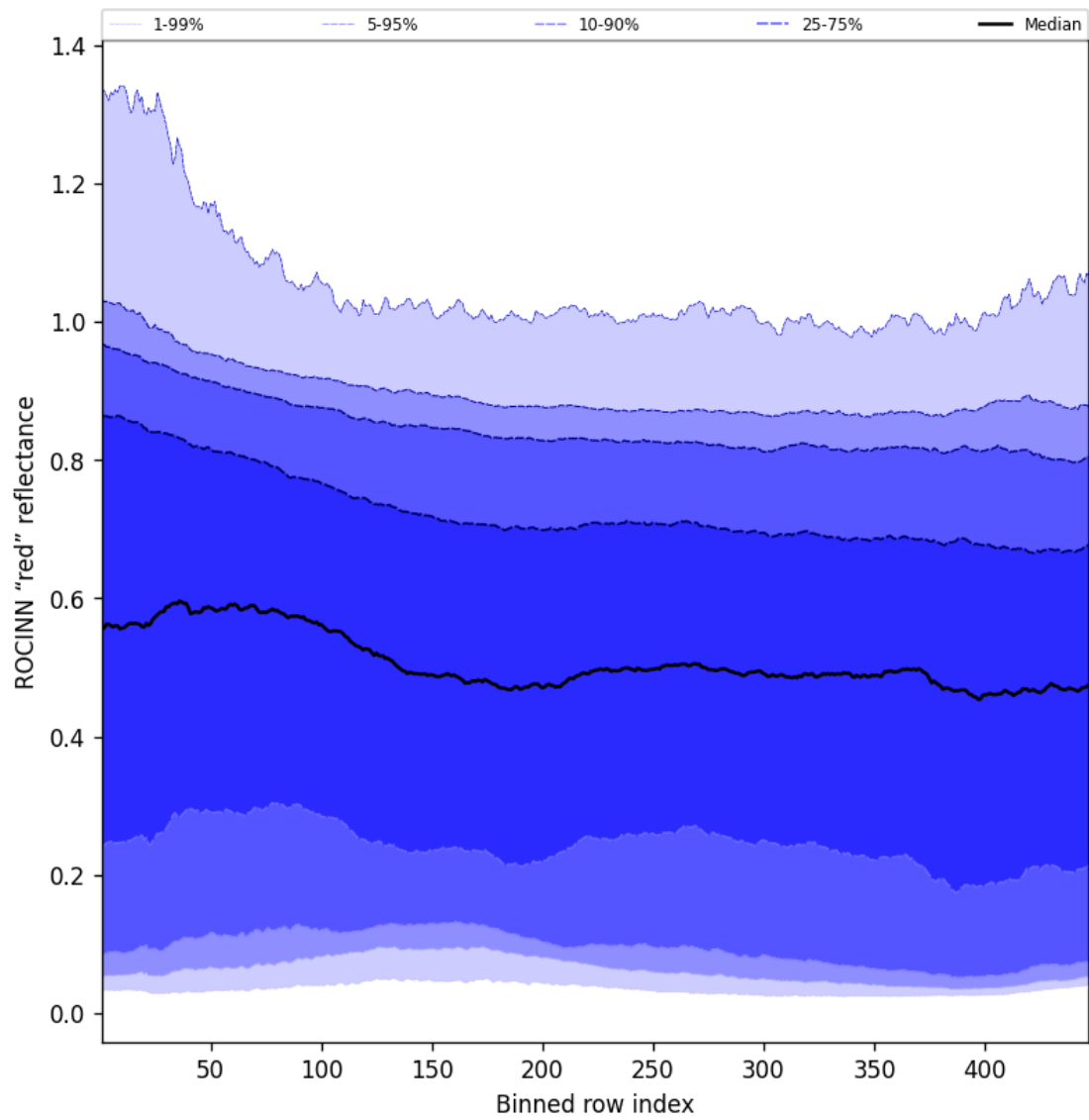
Figure 67: Along track statistics of “ROCINN “red” reflectance” for 2025-02-09 to 2025-02-10
