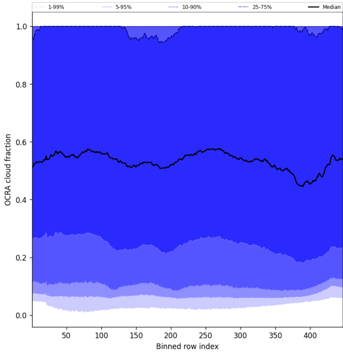
Figure 64: Along track statistics of “OCRA cloud fraction” for 2025-02-09 to 2025-02-10
