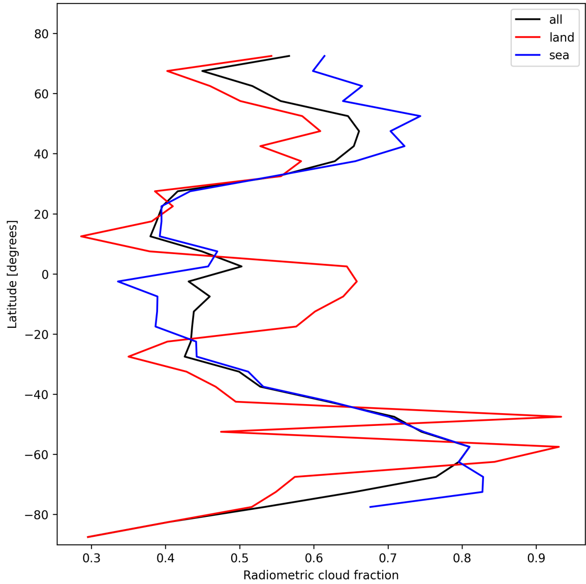
Figure 21: Zonal average of “Radiometric cloud fraction” for 2025-02-09 to 2025-02-10.
