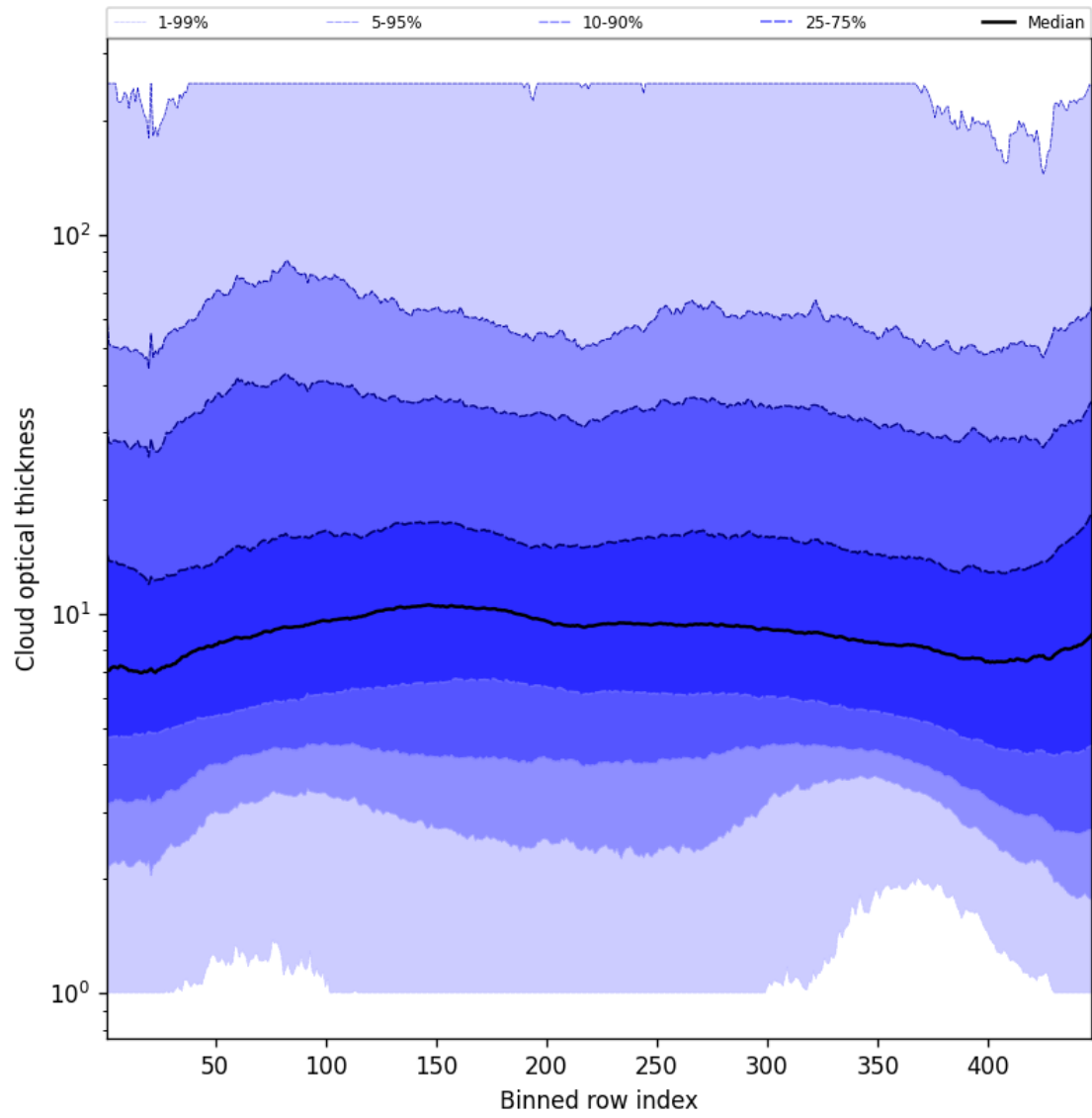
Figure 55: Along track statistics of “Cloud optical thickness” for 2025-02-09 to 2025-02-10
