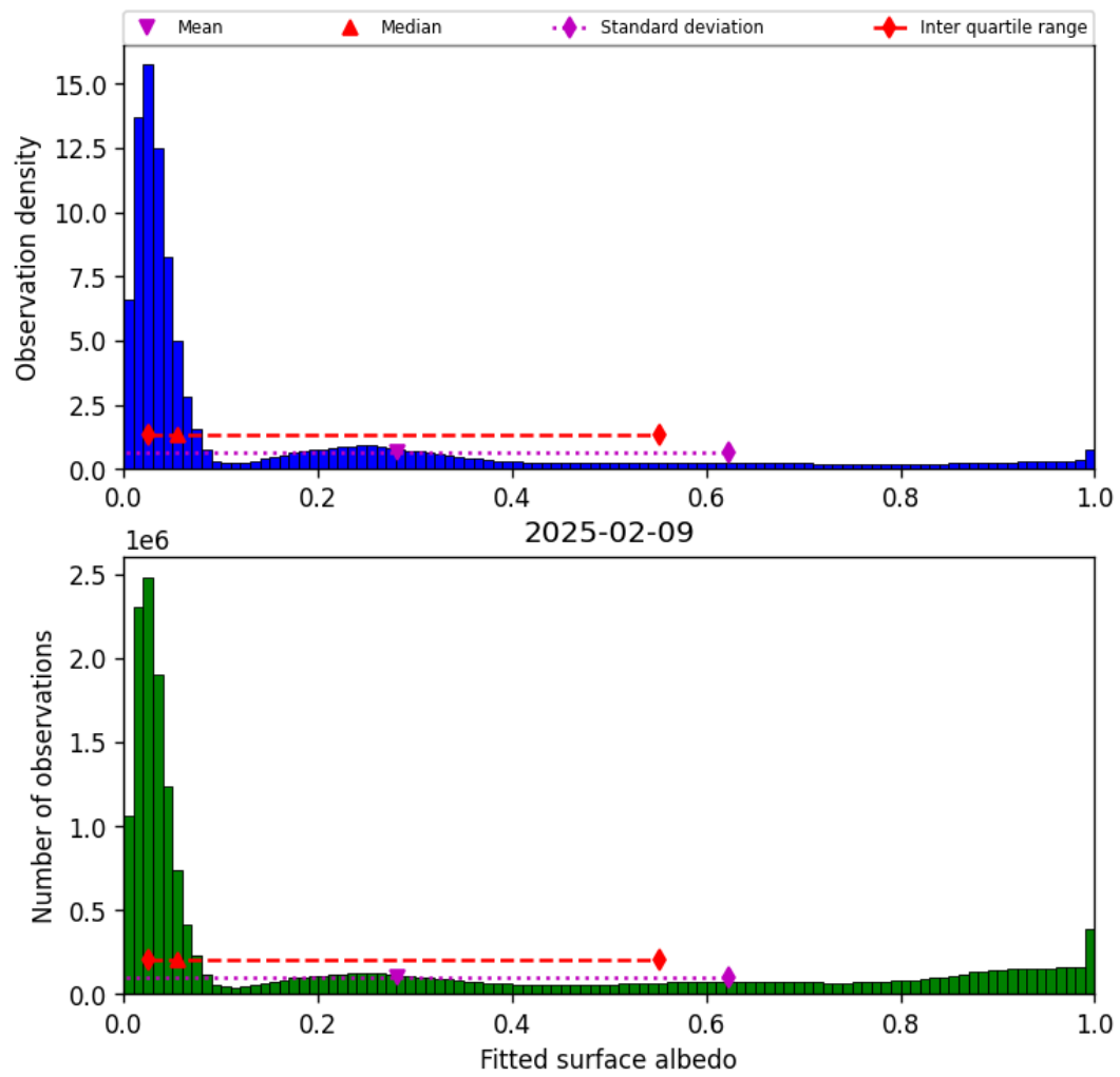
Figure 43: Histogram of “Fitted surface albedo” for 2025-02-09 to 2025-02-10
