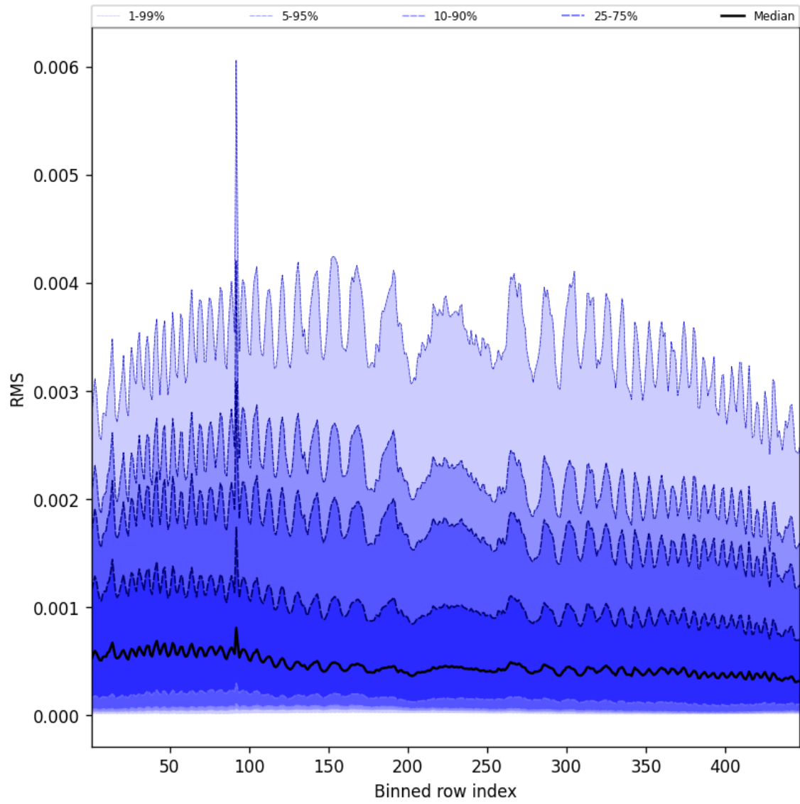
Figure 61: Along track statistics of “RMS” for 2025-02-09 to 2025-02-10
