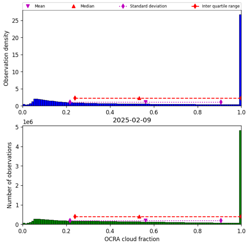
Figure 48: Histogram of “OCRA cloud fraction” for 2025-02-09 to 2025-02-10
