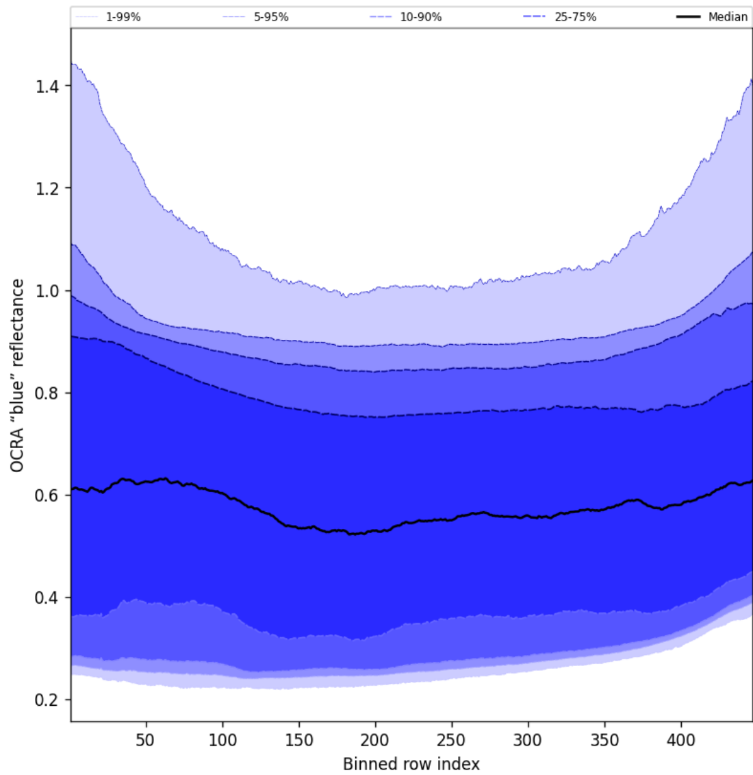
Figure 65: Along track statistics of “OCRA “blue” reflectance” for 2025-02-09 to 2025-02-10
