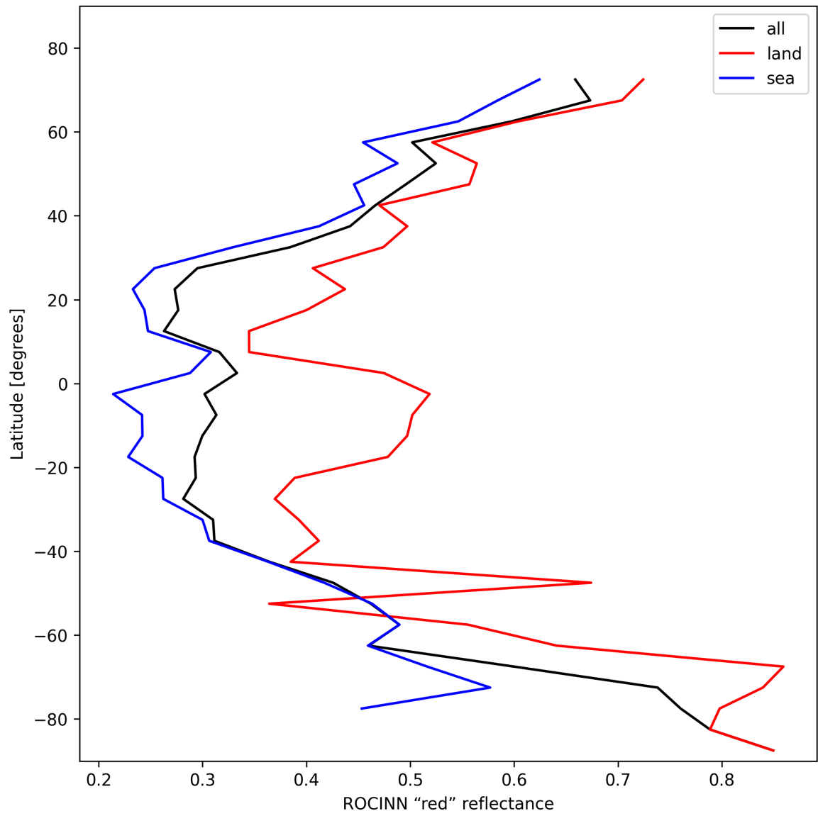
Figure 35: Zonal average of “ROCINN “red” reflectance” for 2025-02-09 to 2025-02-10.
