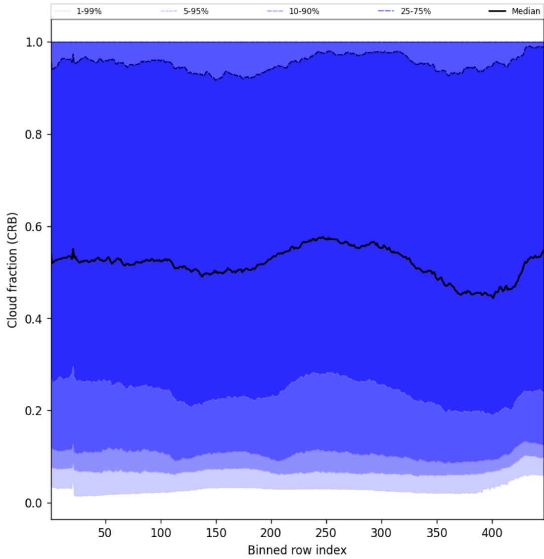
Figure 56: Along track statistics of “Cloud fraction (CRB)” for 2025-02-10 to 2025-02-11
