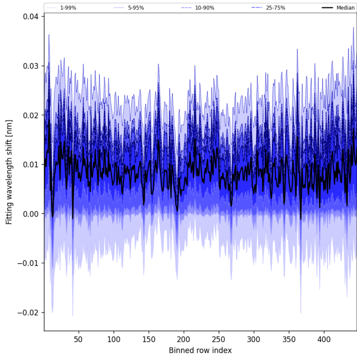
Figure 63: Along track statistics of “Fitting wavelength shift” for 2025-02-10 to 2025-02-11
