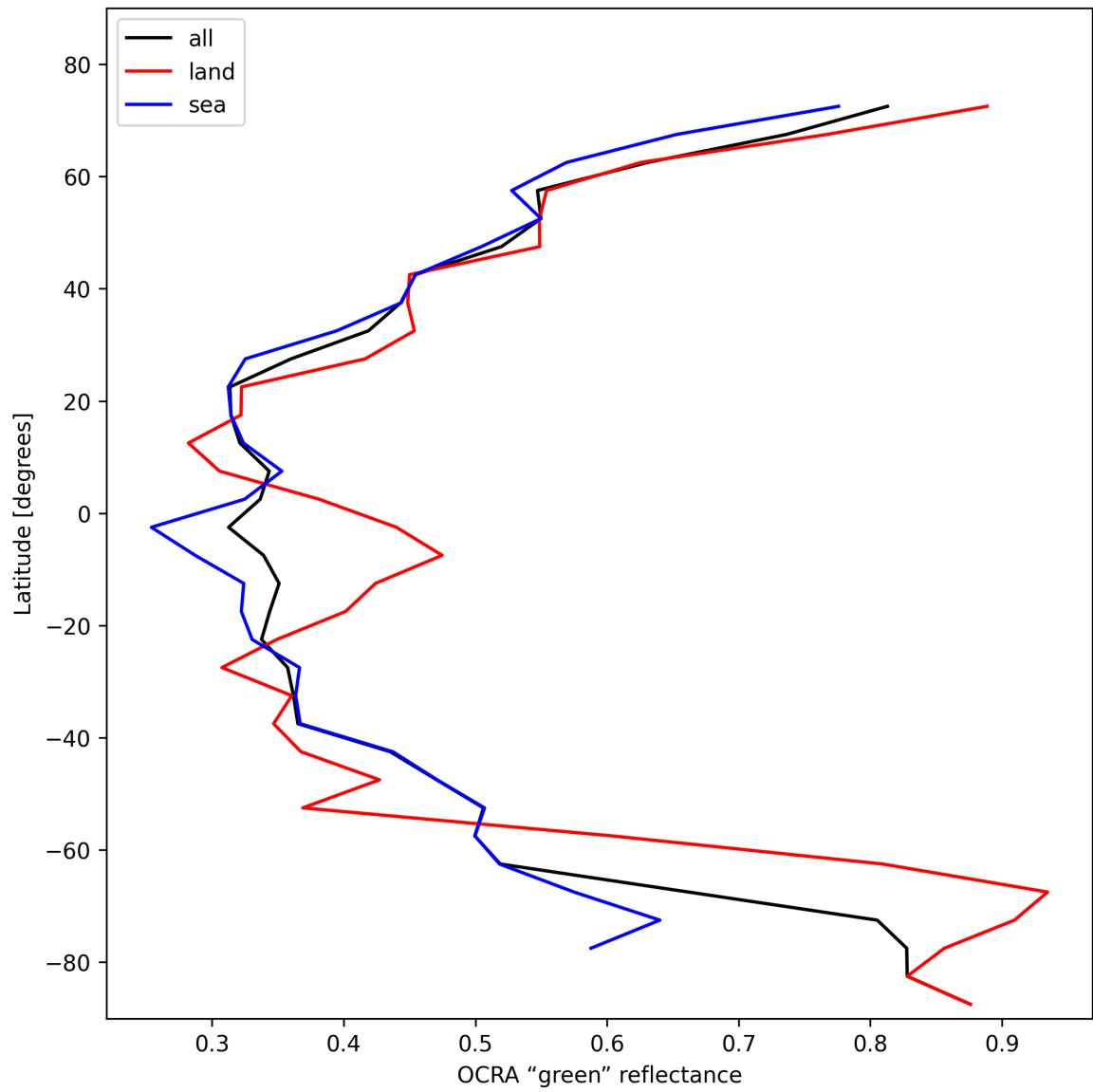
Figure 34: Zonal average of “OCRA “green” reflectance” for 2025-02-10 to 2025-02-11.
