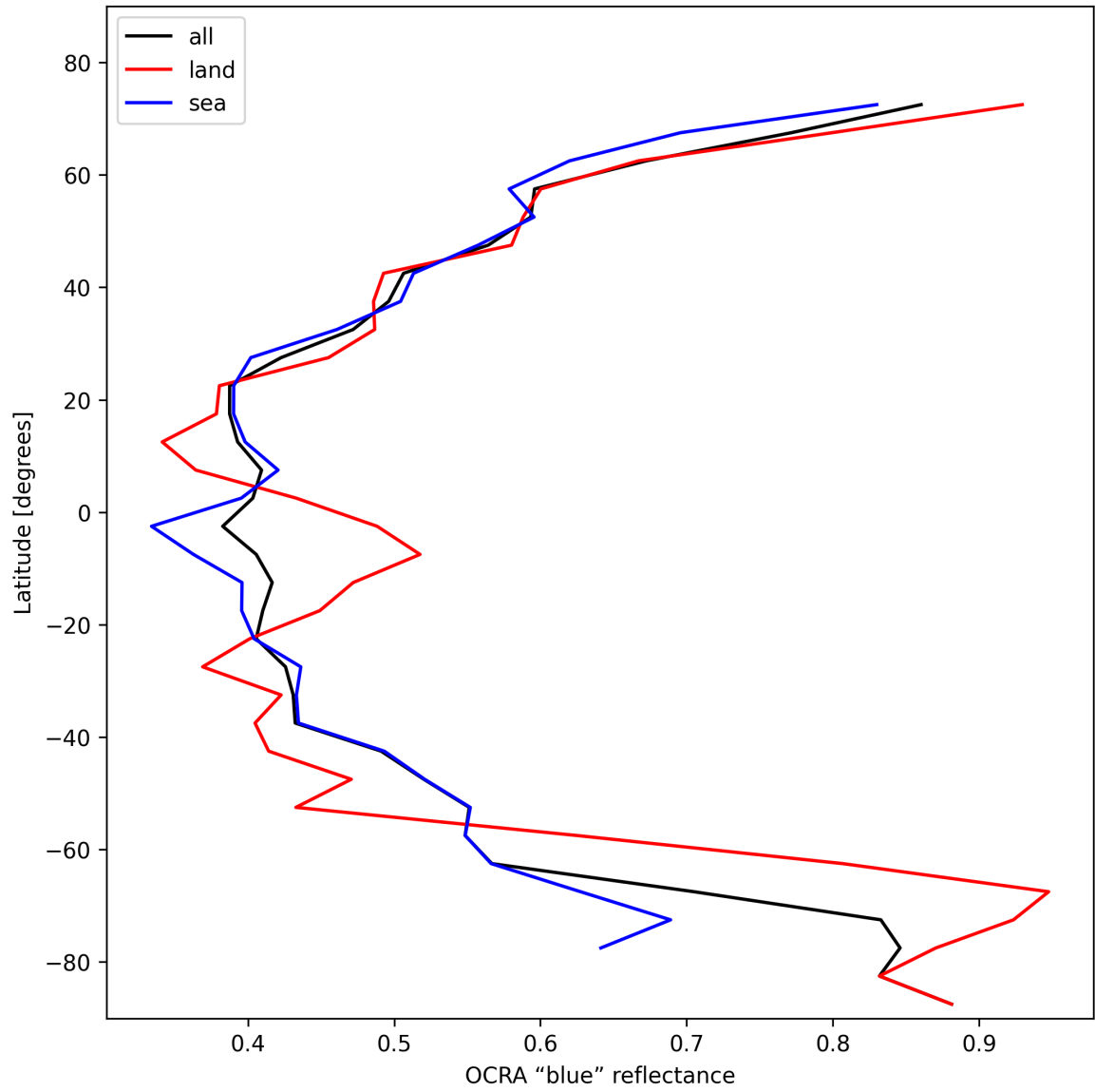
Figure 33: Zonal average of “OCRA “blue” reflectance” for 2025-02-10 to 2025-02-11.
