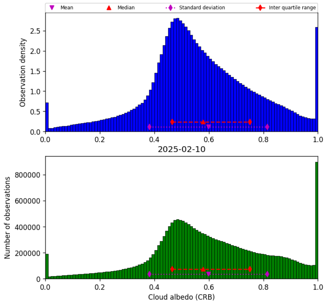
Figure 42: Histogram of “Cloud albedo (CRB)” for 2025-02-10 to 2025-02-11
