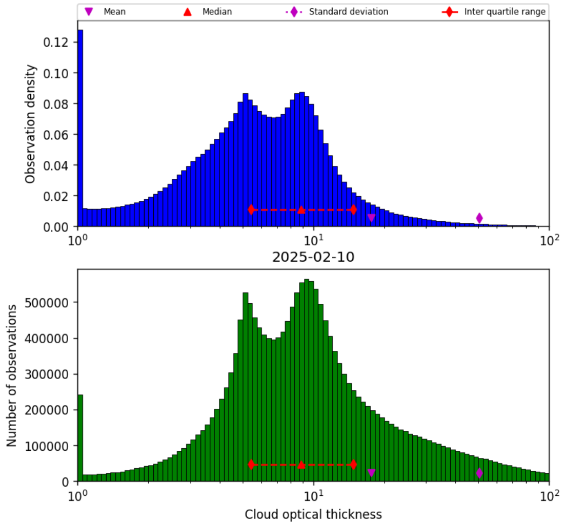
Figure 39: Histogram of “Cloud optical thickness” for 2025-02-10 to 2025-02-11
