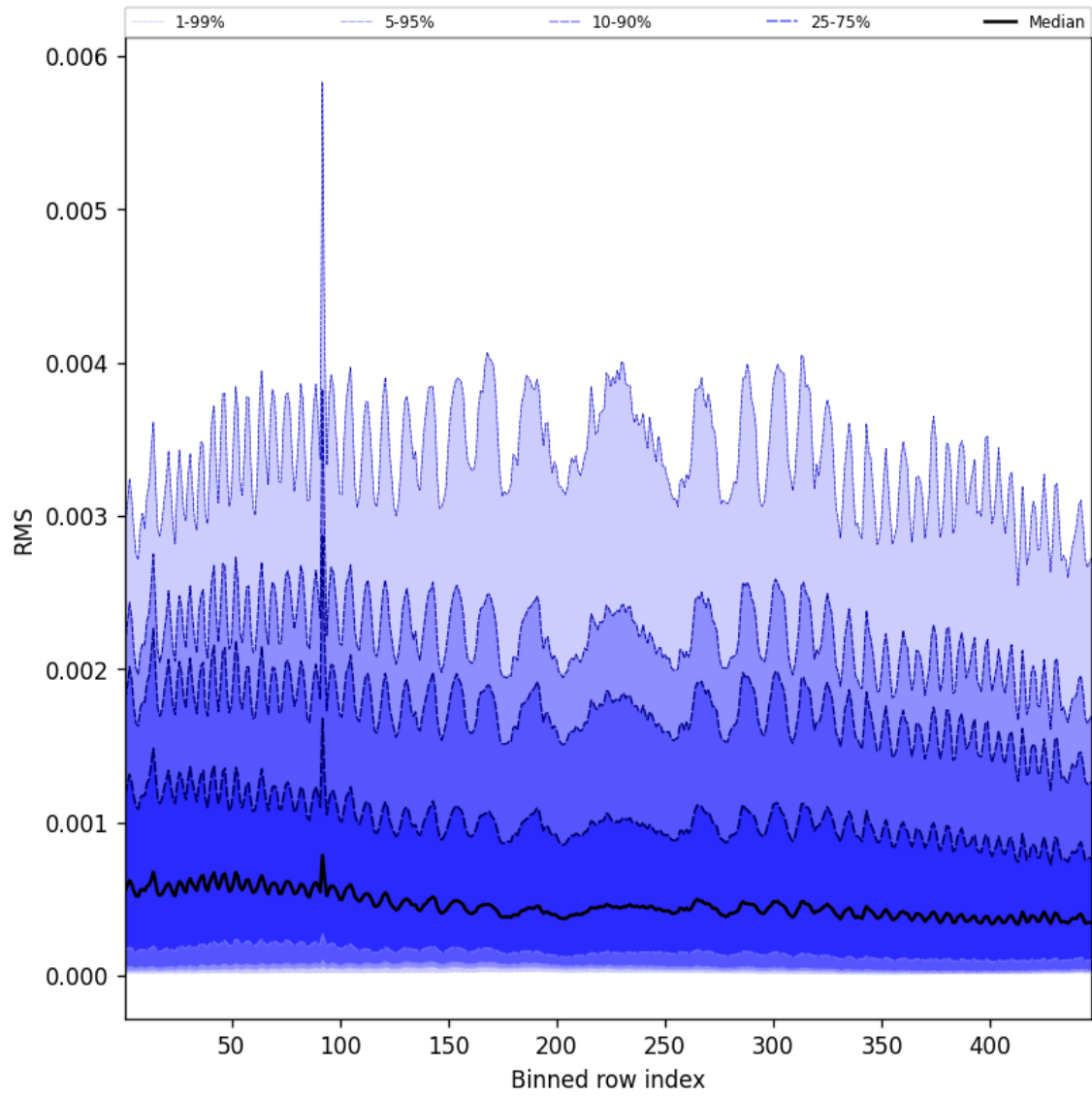
Figure 61: Along track statistics of “RMS” for 2025-02-10 to 2025-02-11
