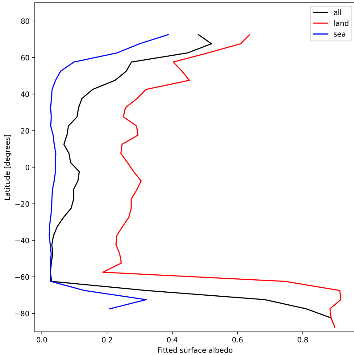
Figure 27: Zonal average of “Fitted surface albedo” for 2025-02-10 to 2025-02-11.
