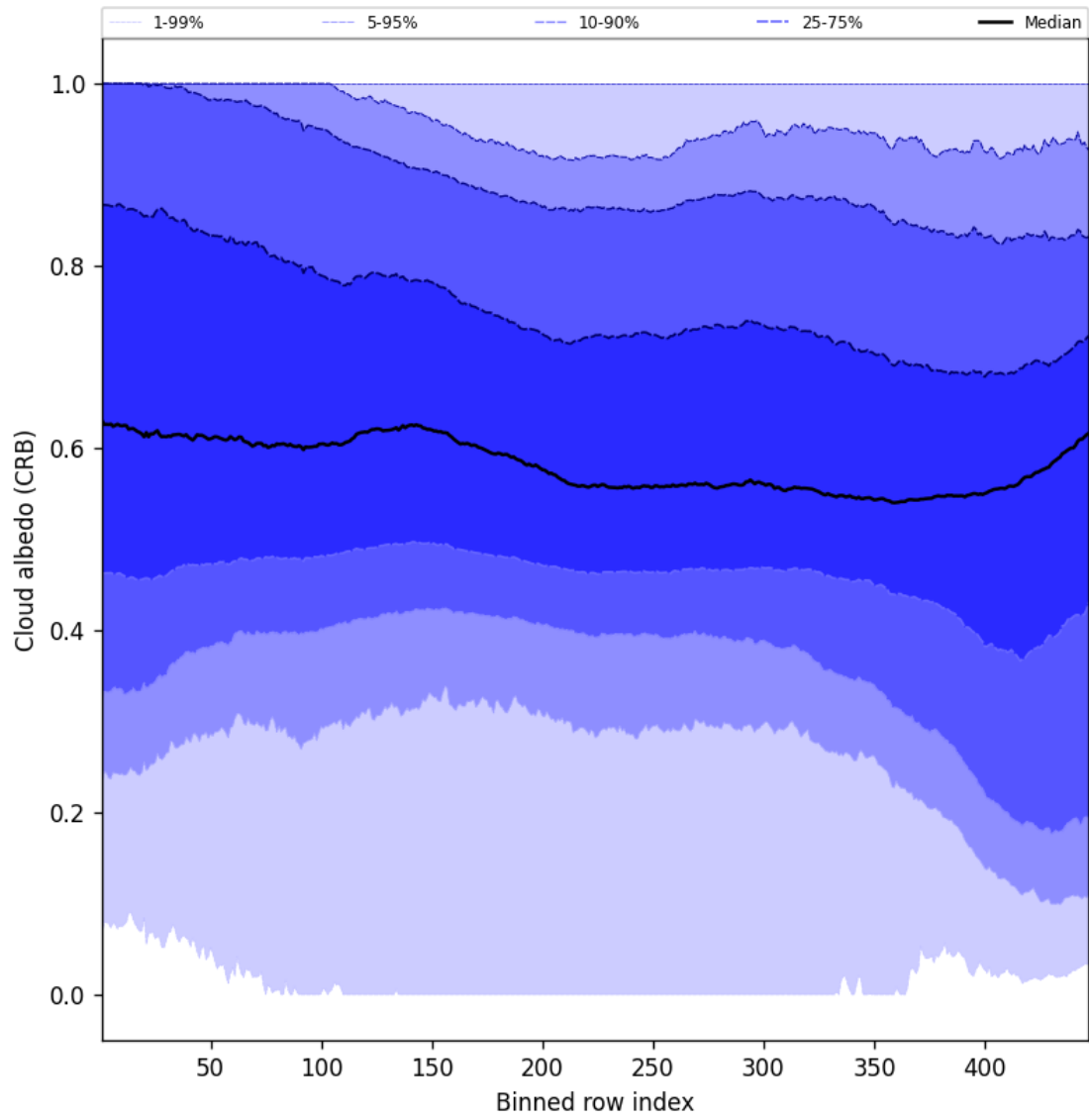
Figure 58: Along track statistics of “Cloud albedo (CRB)” for 2025-02-10 to 2025-02-11
