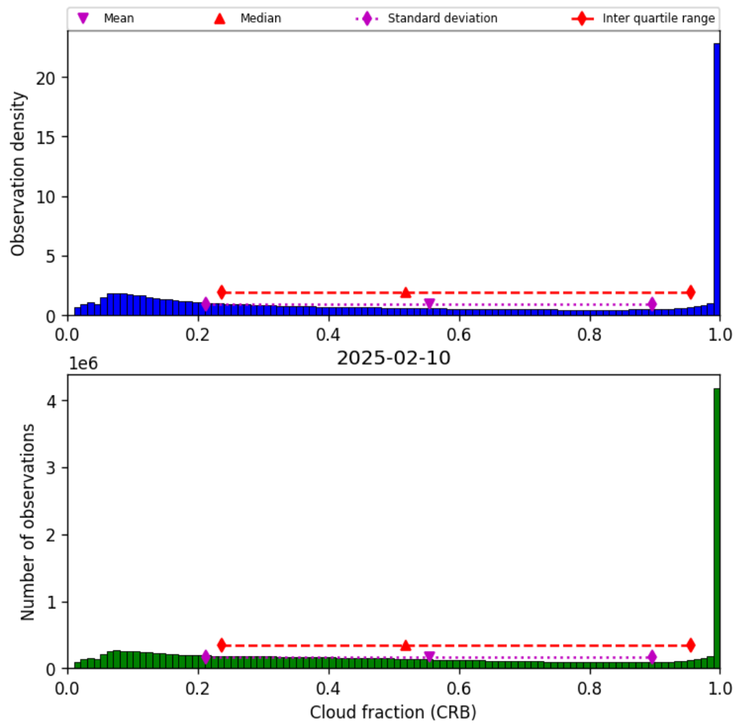
Figure 40: Histogram of “Cloud fraction (CRB)” for 2025-02-10 to 2025-02-11
