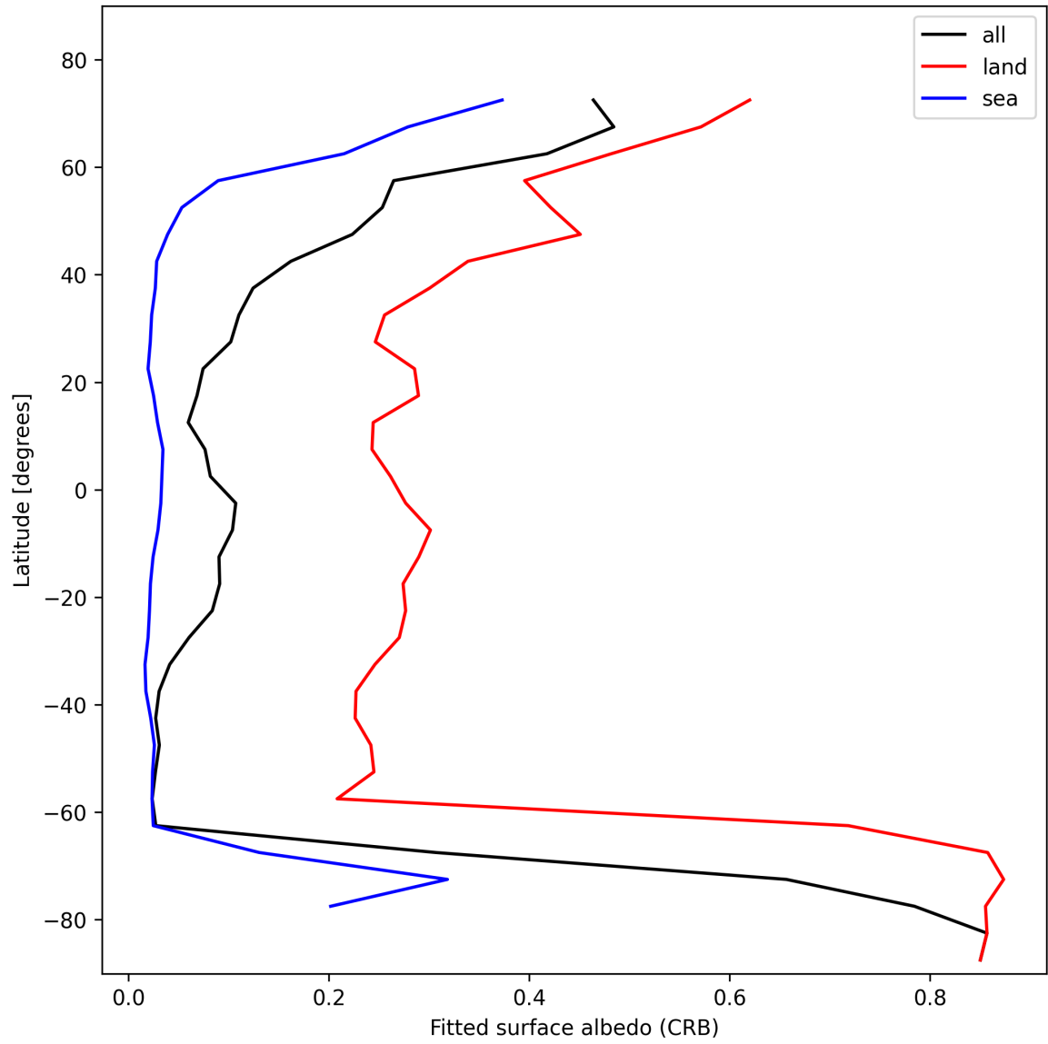
Figure 28: Zonal average of “Fitted surface albedo (CRB)” for 2025-02-10 to 2025-02-11.
