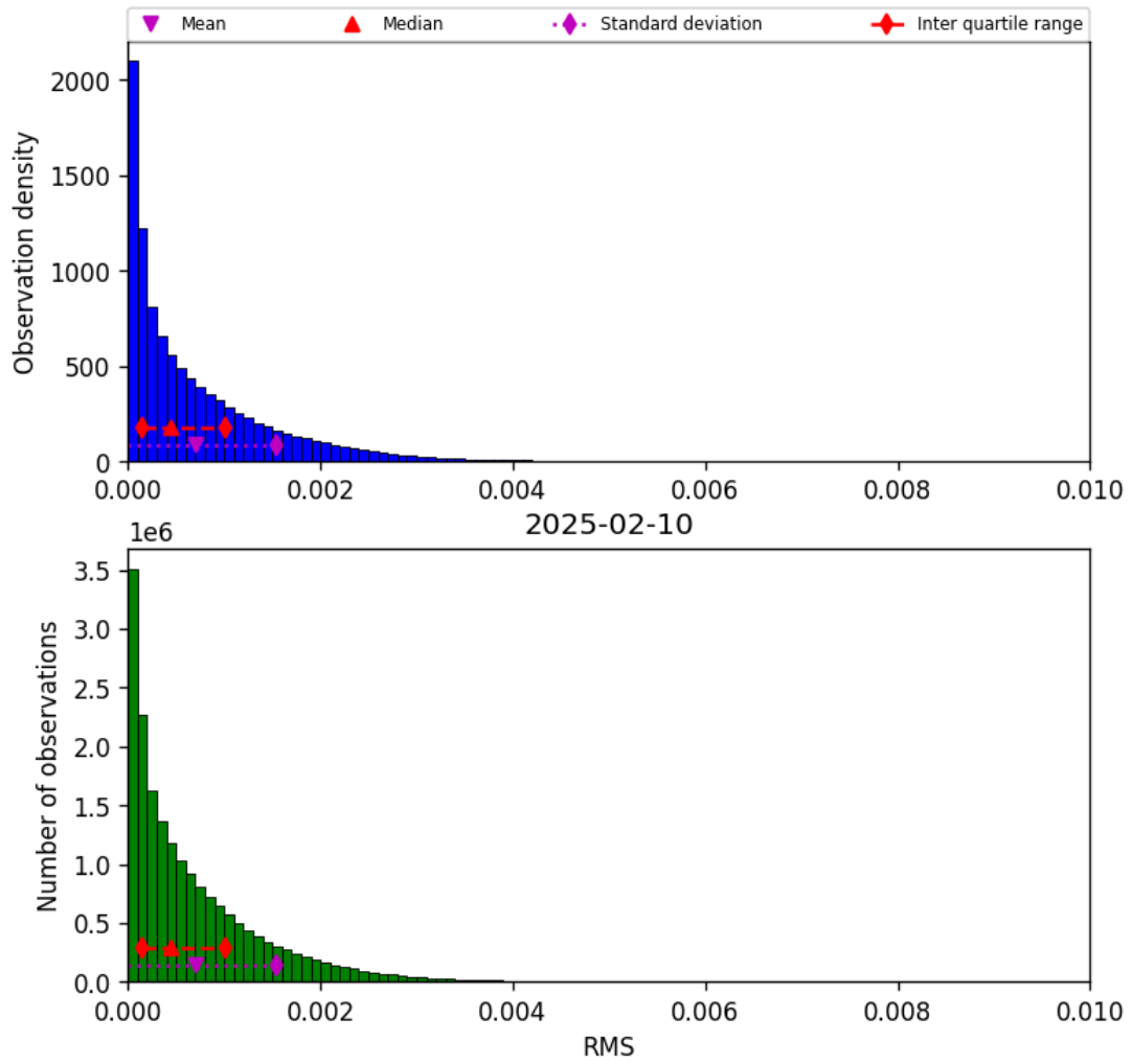
Figure 45: Histogram of “RMS” for 2025-02-10 to 2025-02-11
