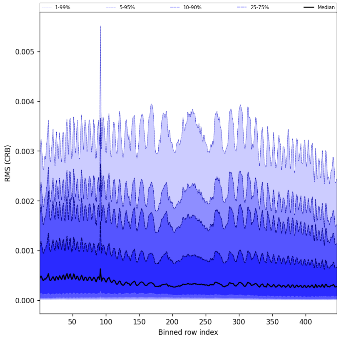
Figure 62: Along track statistics of “RMS (CRB)” for 2025-02-10 to 2025-02-11
