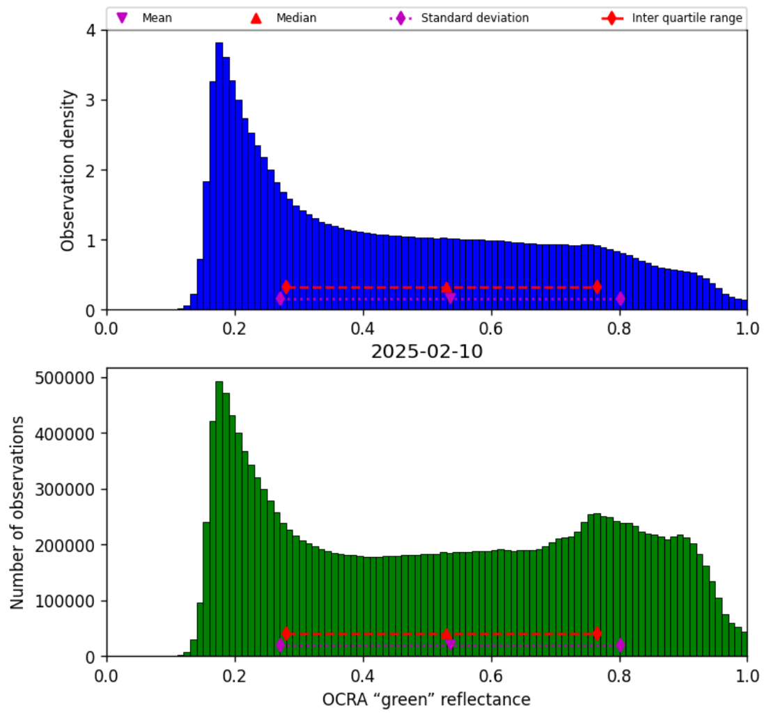
Figure 50: Histogram of “OCRA “green” reflectance” for 2025-02-10 to 2025-02-11
