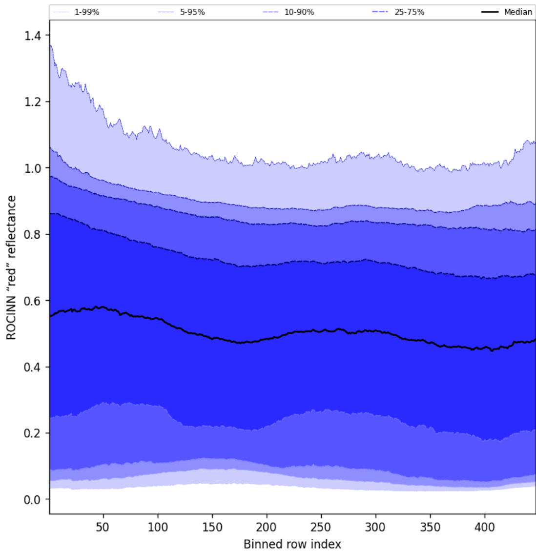
Figure 67: Along track statistics of “ROCINN “red” reflectance” for 2025-02-10 to 2025-02-11
