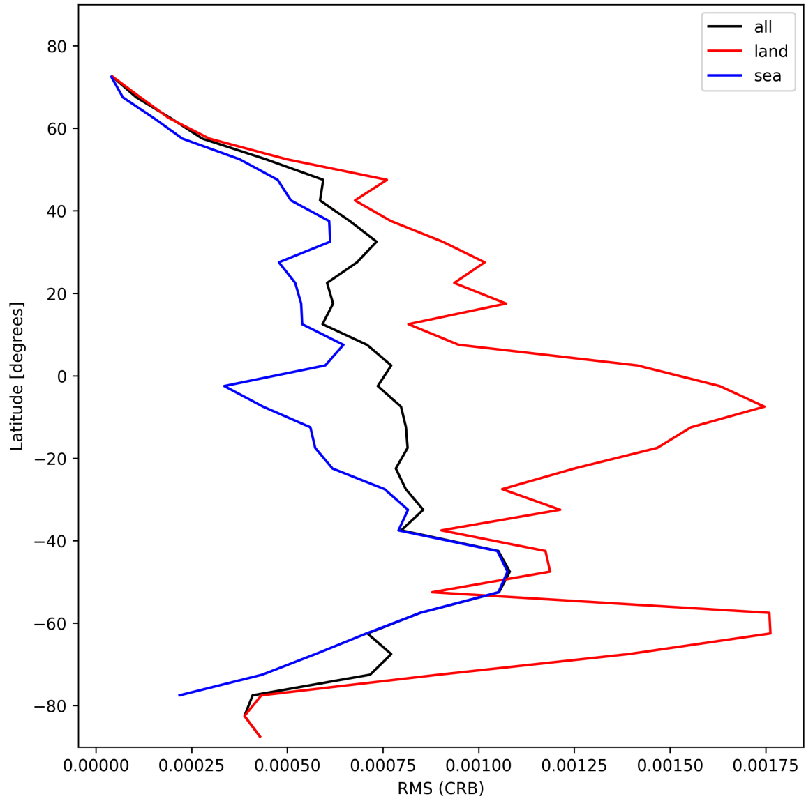
Figure 30: Zonal average of “RMS (CRB)” for 2025-02-10 to 2025-02-11.
