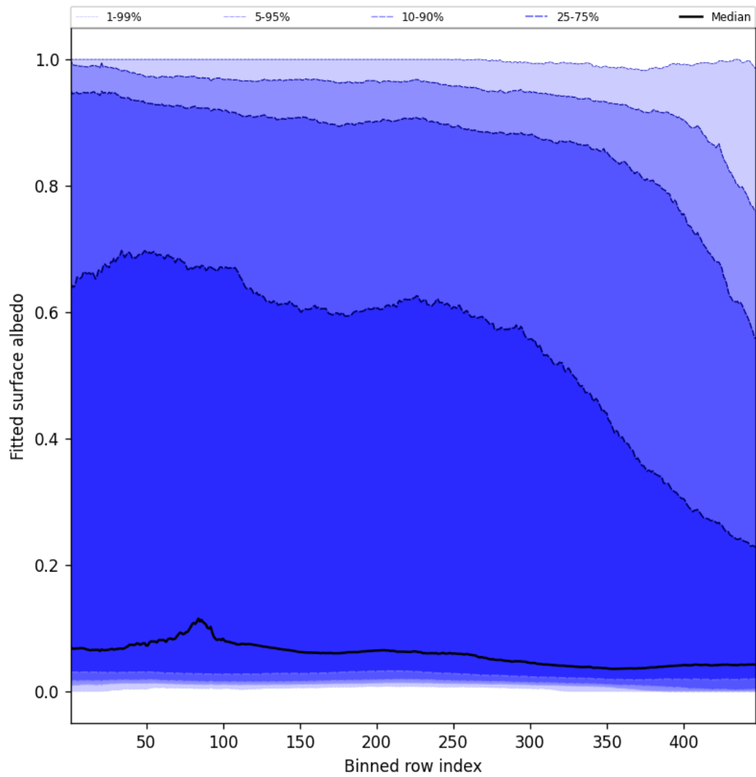
Figure 59: Along track statistics of “Fitted surface albedo” for 2025-02-10 to 2025-02-11
