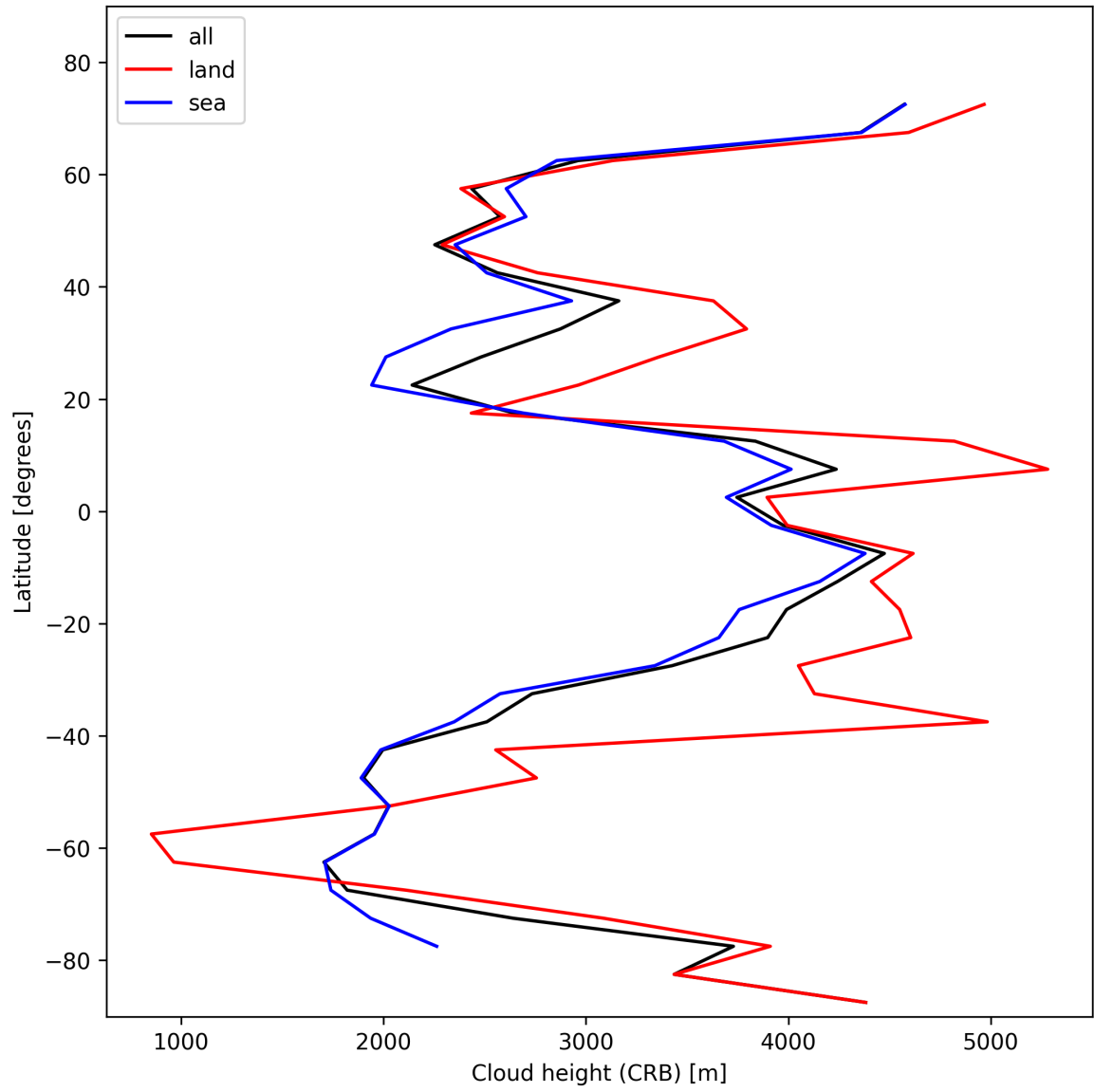
Figure 25: Zonal average of “Cloud height (CRB)” for 2025-02-10 to 2025-02-11.
