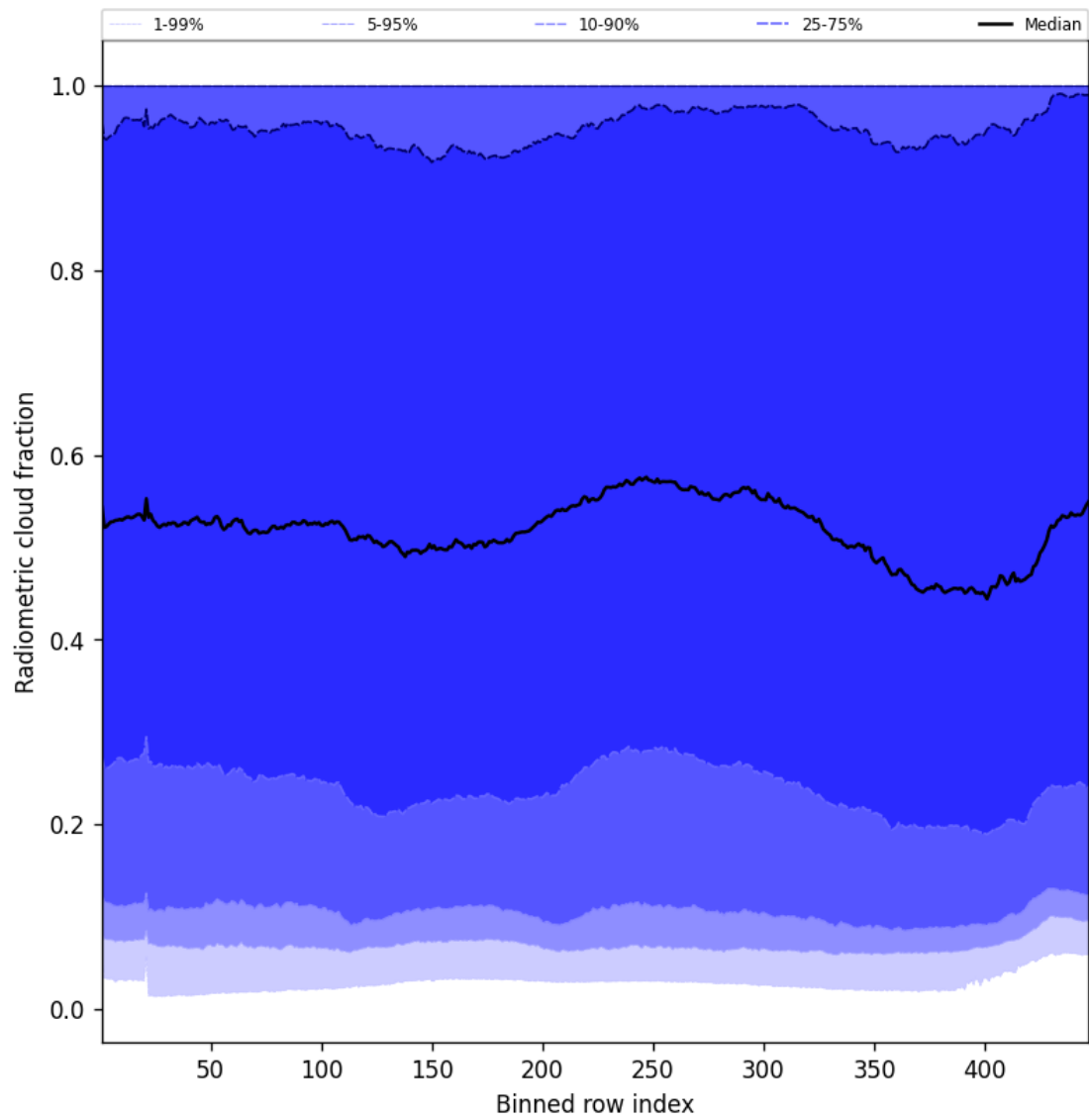
Figure 53: Along track statistics of “Radiometric cloud fraction” for 2025-02-10 to 2025-02-11
