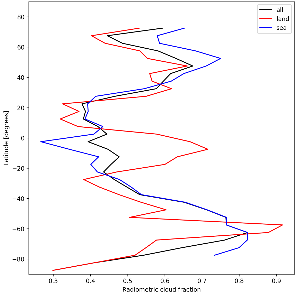
Figure 21: Zonal average of “Radiometric cloud fraction” for 2025-02-10 to 2025-02-11.
