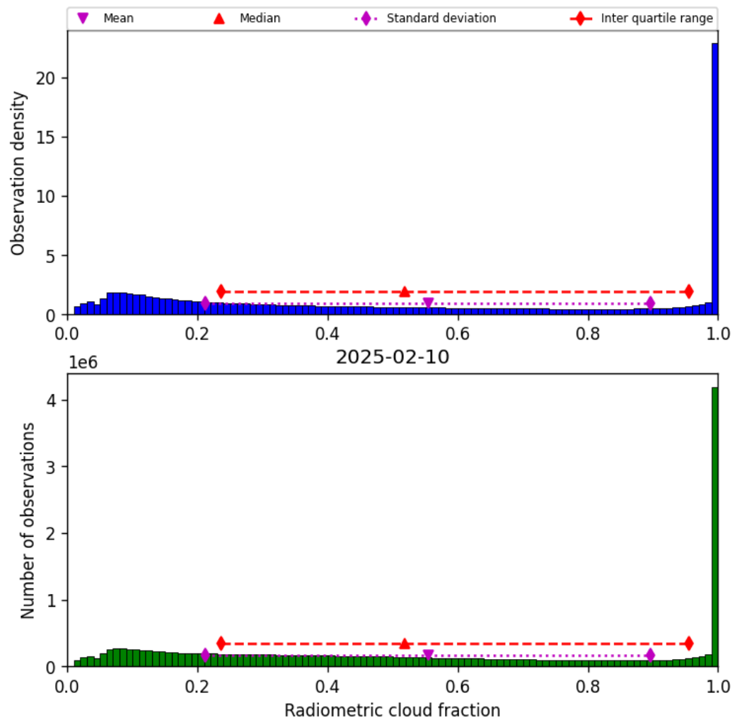
Figure 37: Histogram of “Radiometric cloud fraction” for 2025-02-10 to 2025-02-11
