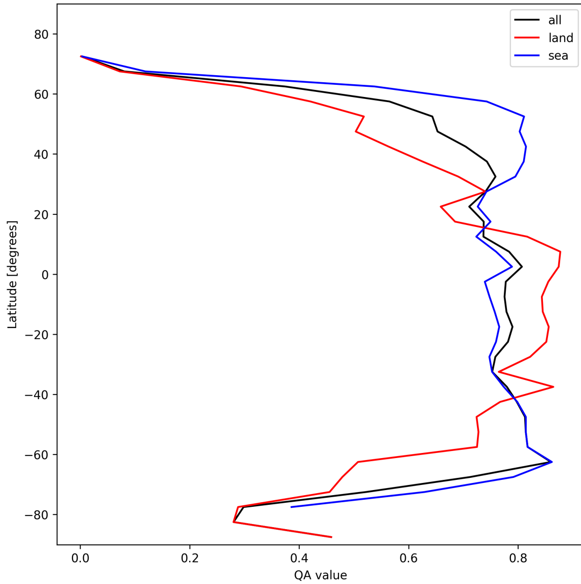
Figure 20: Zonal average of “QA value” for 2025-02-10 to 2025-02-11.
