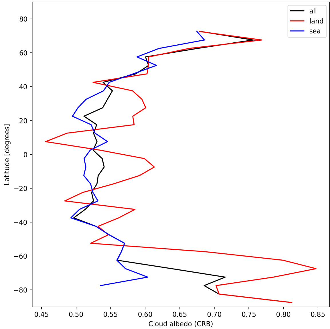
Figure 26: Zonal average of “Cloud albedo (CRB)” for 2025-02-10 to 2025-02-11.
