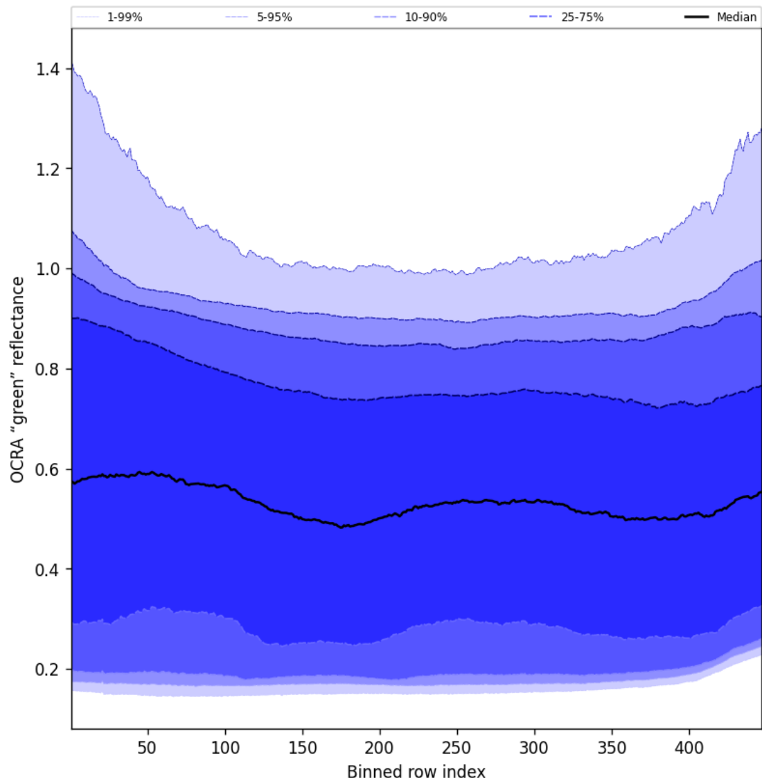
Figure 66: Along track statistics of “OCRA “green” reflectance” for 2025-02-10 to 2025-02-11
