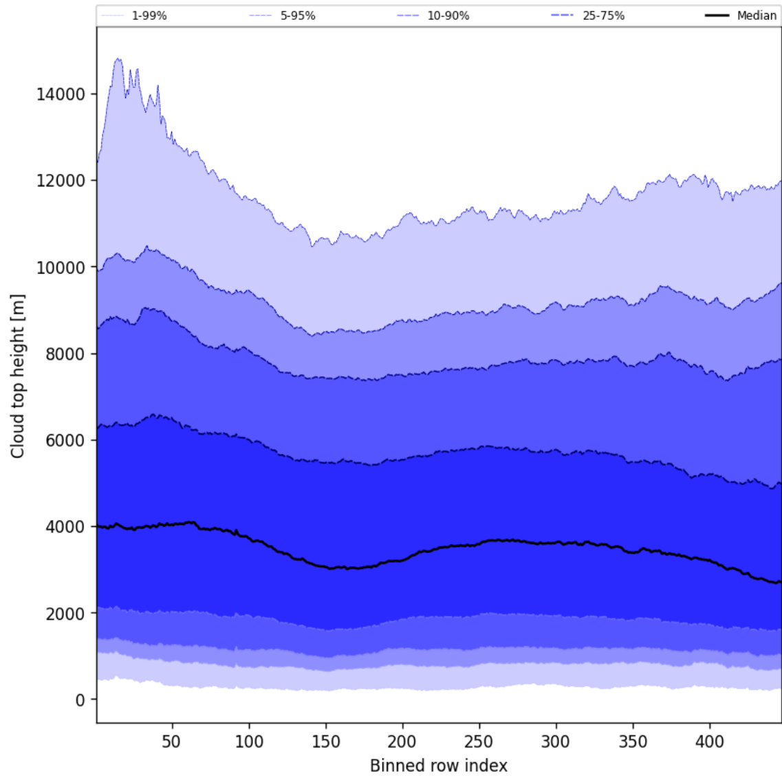
Figure 54: Along track statistics of “Cloud top height” for 2025-02-10 to 2025-02-11
