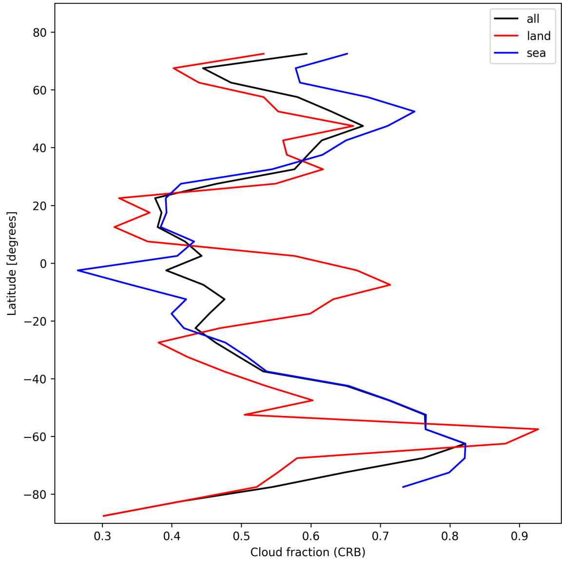
Figure 24: Zonal average of “Cloud fraction (CRB)” for 2025-02-10 to 2025-02-11.
