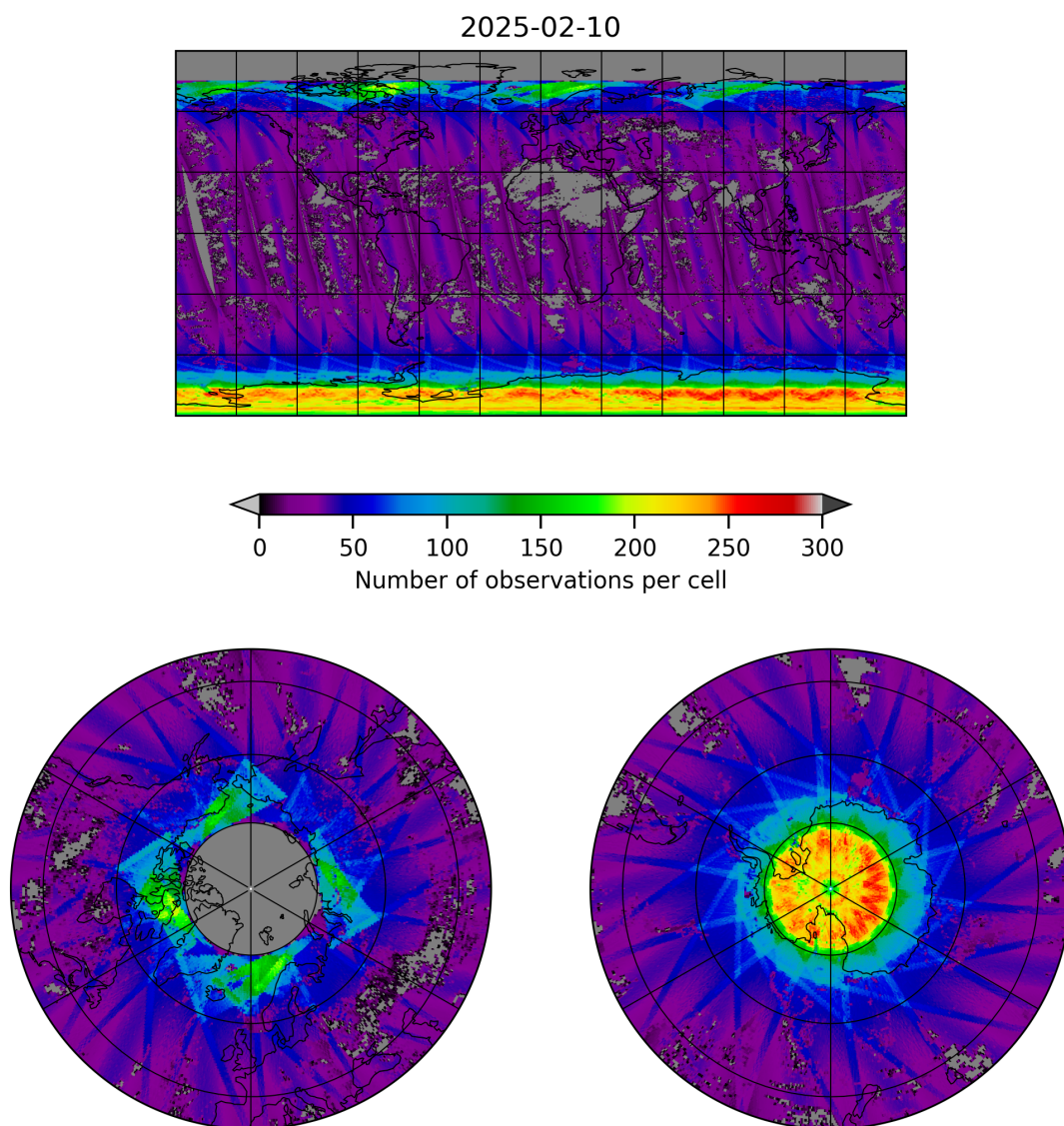
Figure 19: Map of the number of observations for 2025-02-10 to 2025-02-11
