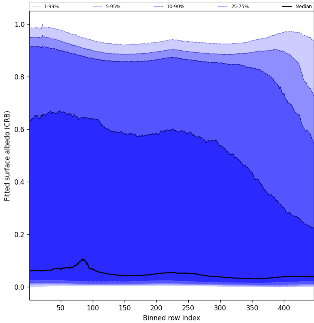
Figure 60: Along track statistics of “Fitted surface albedo (CRB)” for 2025-02-10 to 2025-02-11
