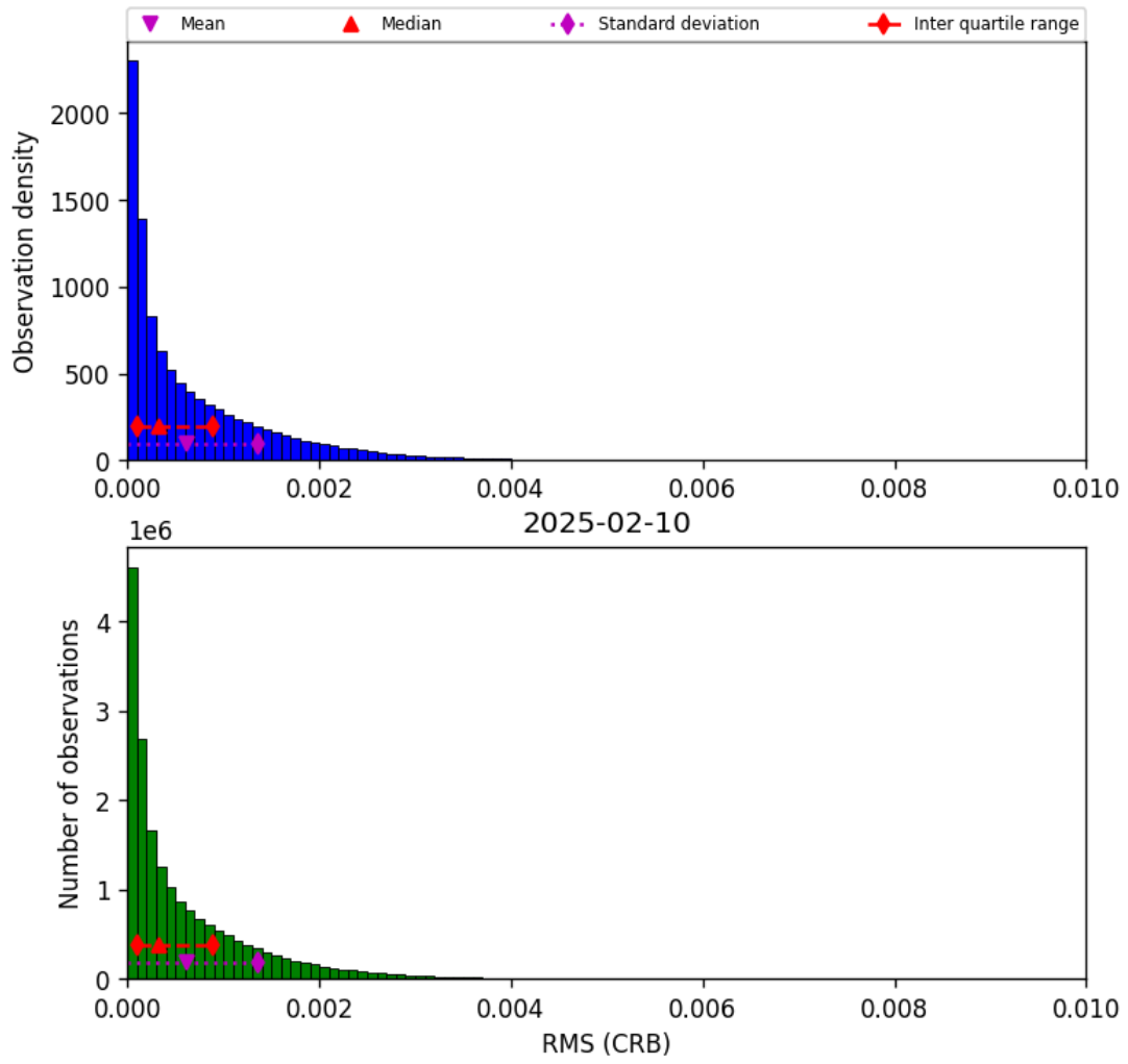
Figure 46: Histogram of “RMS (CRB)” for 2025-02-10 to 2025-02-11
