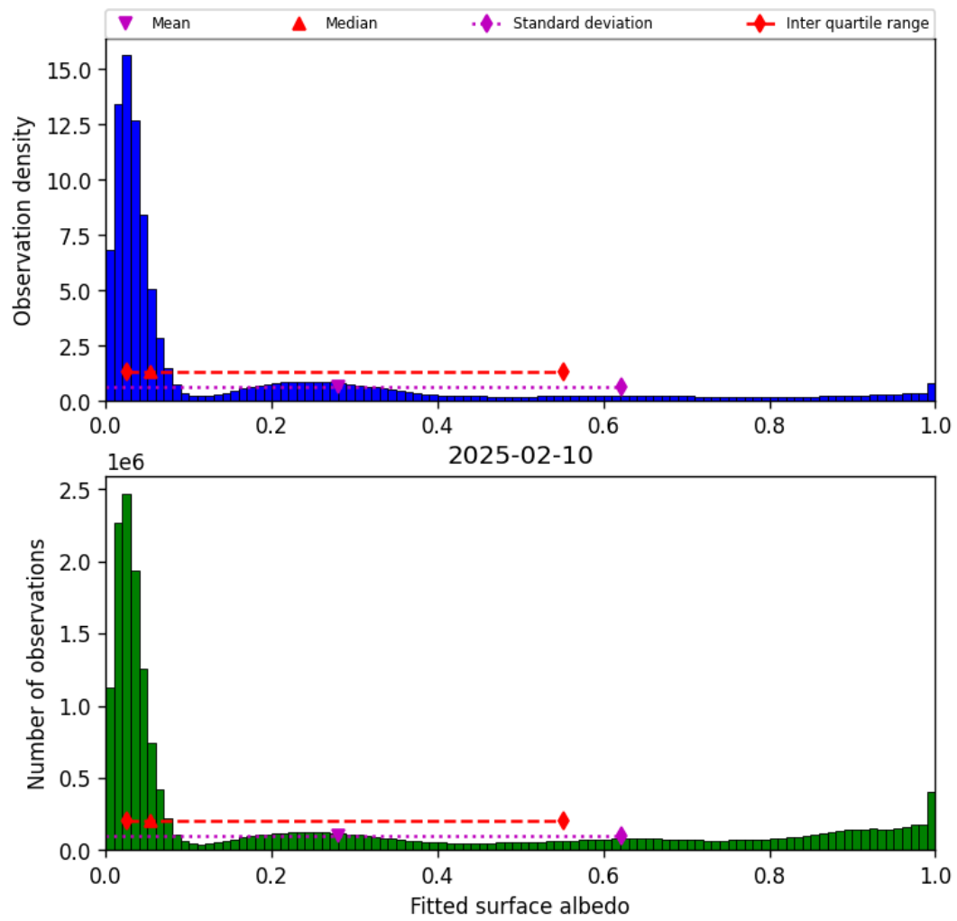
Figure 43: Histogram of “Fitted surface albedo” for 2025-02-10 to 2025-02-11
