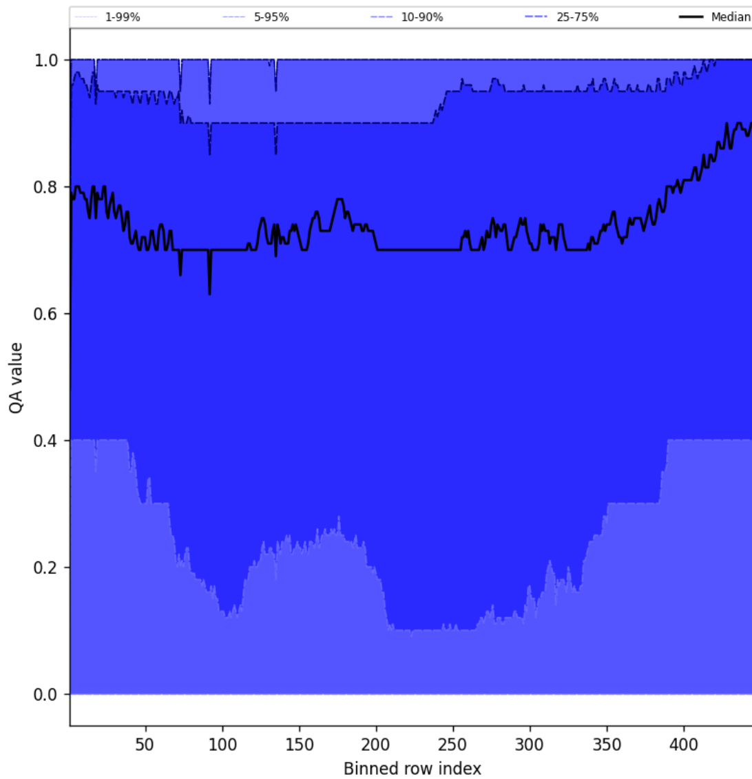
Figure 52: Along track statistics of “QA value” for 2025-02-10 to 2025-02-11
