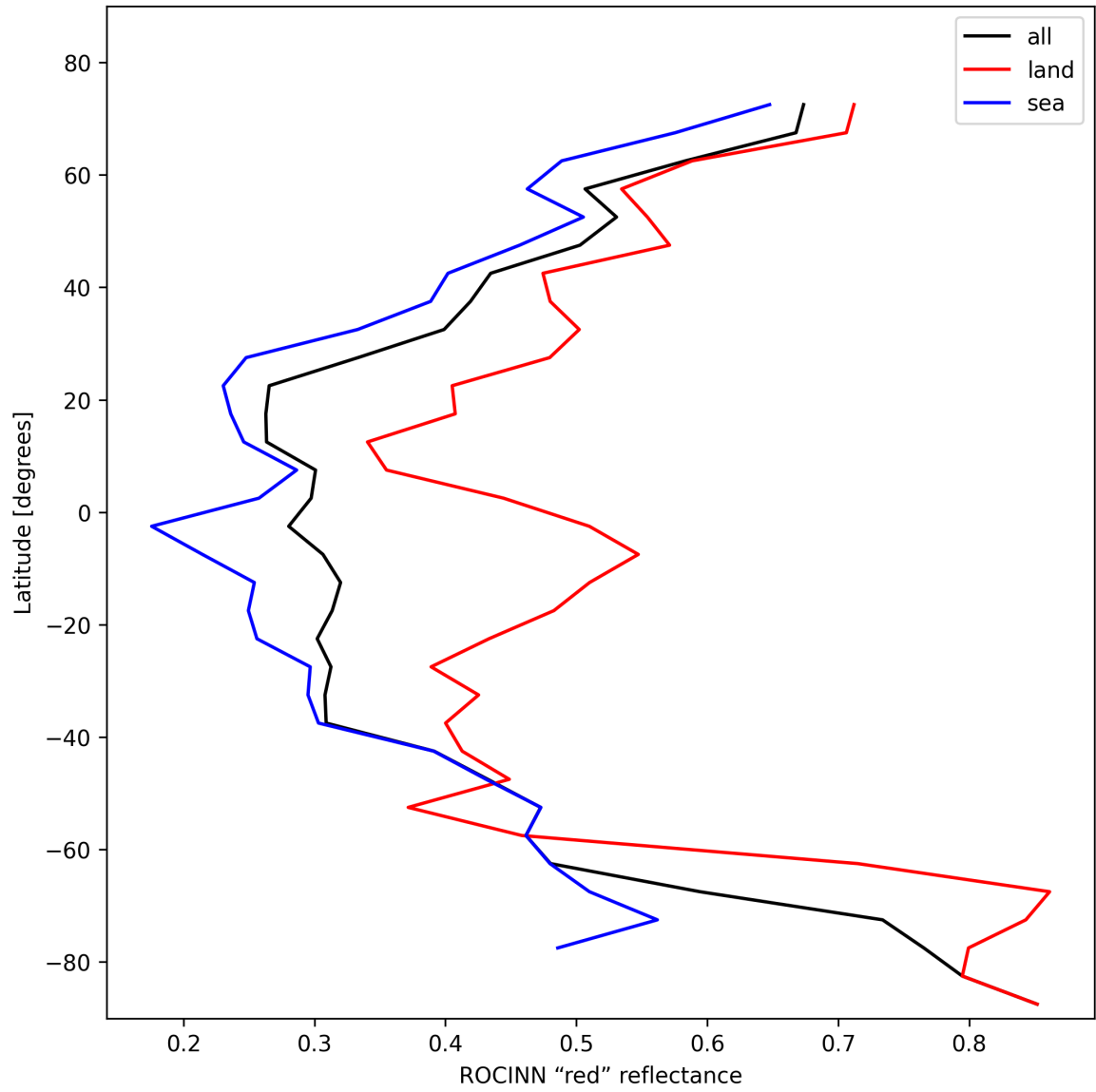
Figure 35: Zonal average of “ROCINN “red” reflectance” for 2025-02-10 to 2025-02-11.
