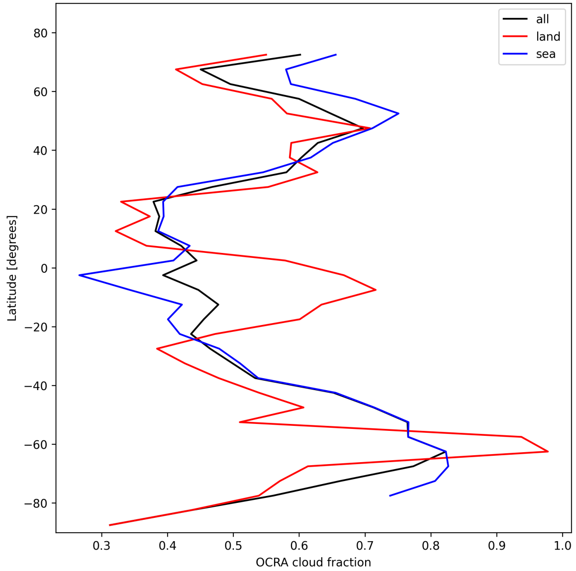
Figure 32: Zonal average of “OCRA cloud fraction” for 2025-02-10 to 2025-02-11.
