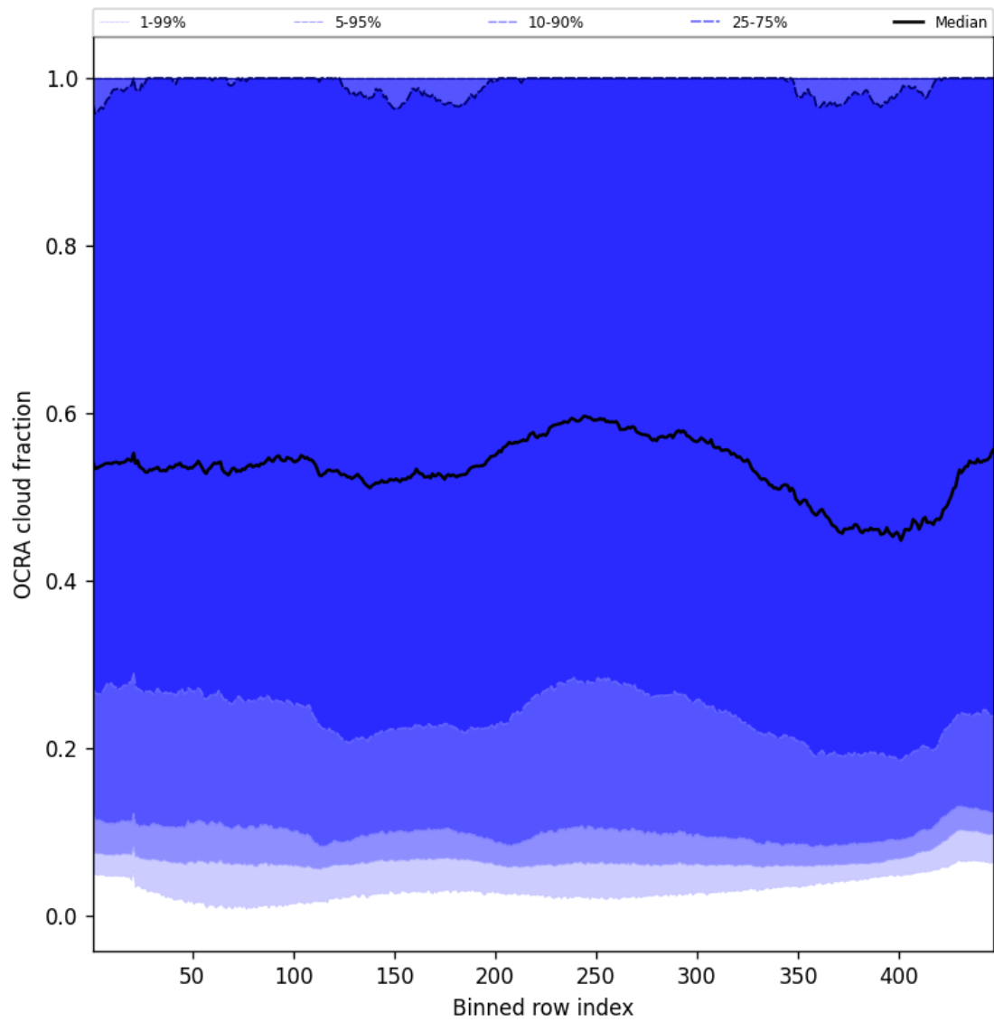
Figure 64: Along track statistics of “OCRA cloud fraction” for 2025-02-10 to 2025-02-11
