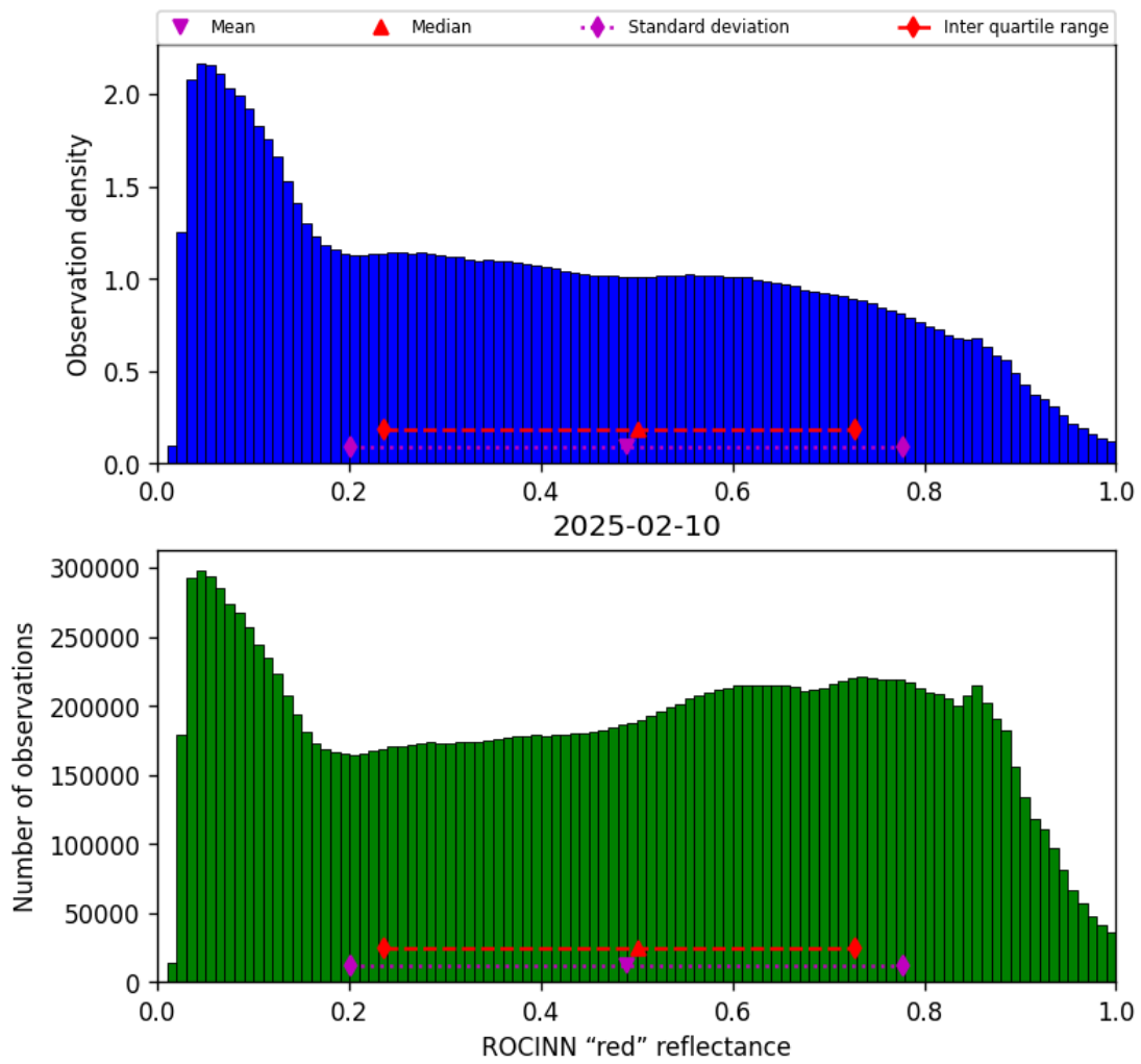
Figure 51: Histogram of “ROCINN “red” reflectance” for 2025-02-10 to 2025-02-11
