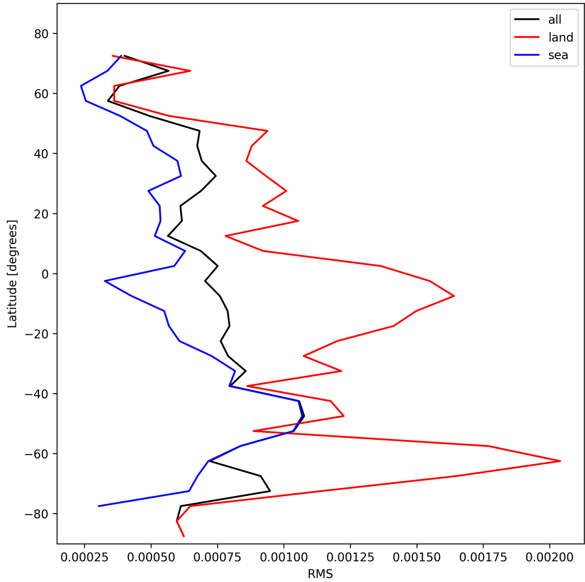
Figure 29: Zonal average of “RMS” for 2025-02-10 to 2025-02-11.
