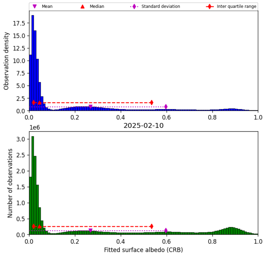
Figure 44: Histogram of “Fitted surface albedo (CRB)” for 2025-02-10 to 2025-02-11
