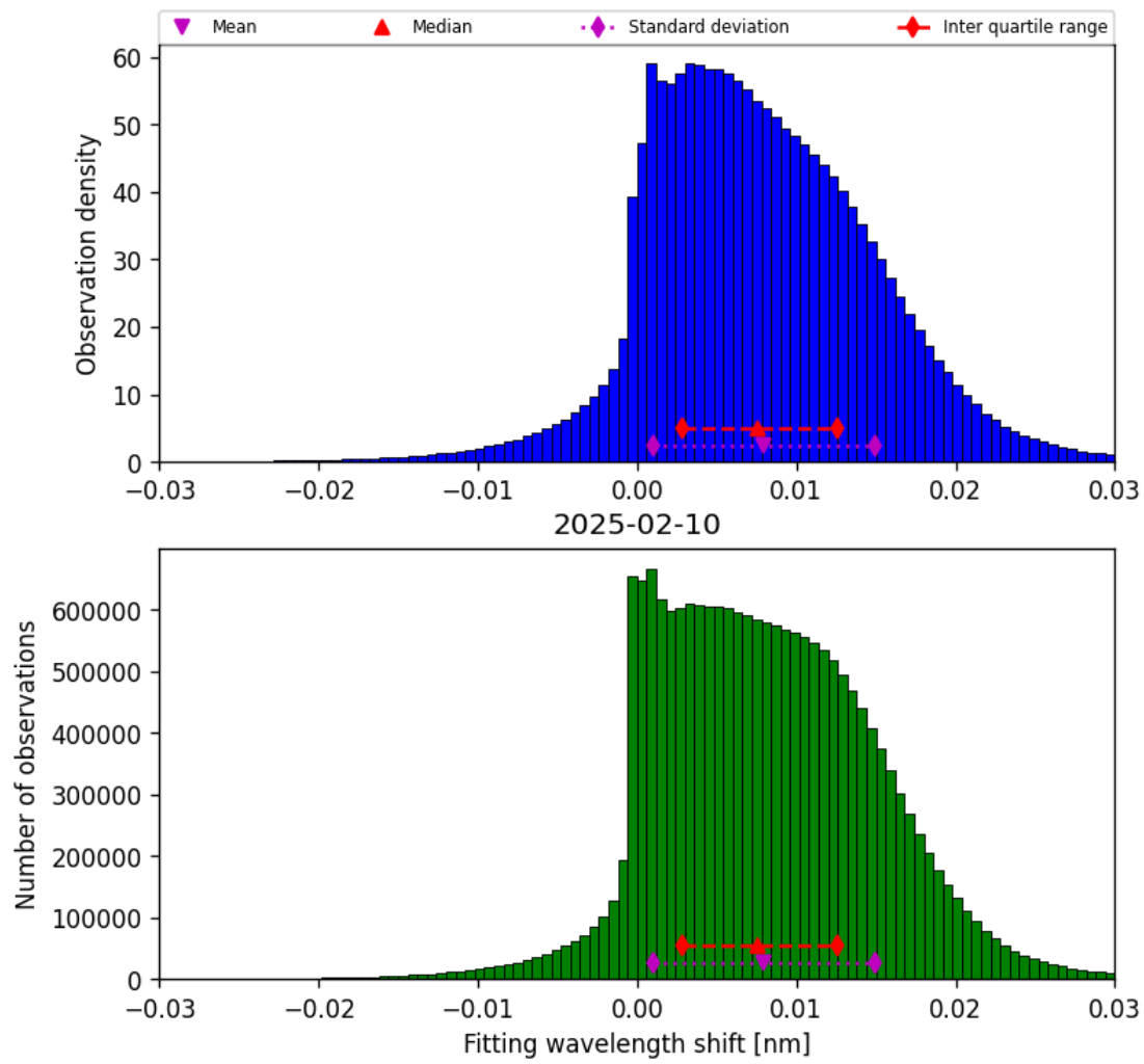
Figure 47: Histogram of “Fitting wavelength shift” for 2025-02-10 to 2025-02-11
