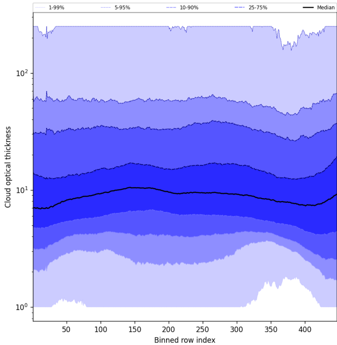
Figure 55: Along track statistics of “Cloud optical thickness” for 2025-02-10 to 2025-02-11
