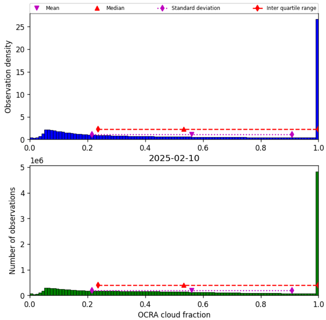
Figure 48: Histogram of “OCRA cloud fraction” for 2025-02-10 to 2025-02-11
