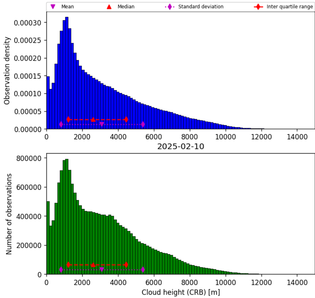
Figure 41: Histogram of “Cloud height (CRB)” for 2025-02-10 to 2025-02-11
