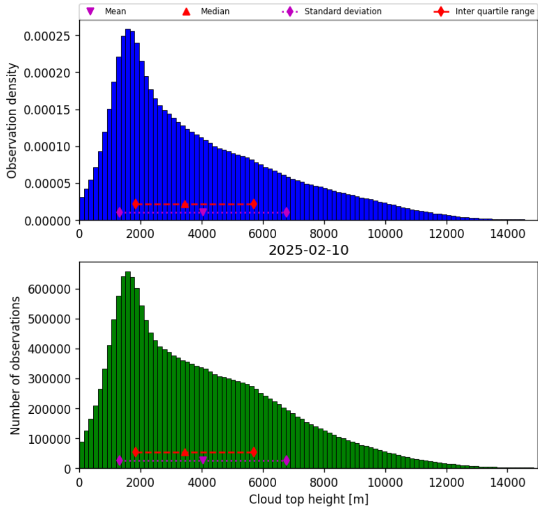
Figure 38: Histogram of “Cloud top height” for 2025-02-10 to 2025-02-11
