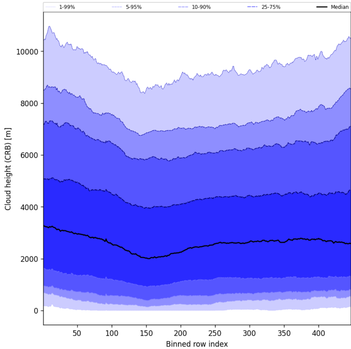
Figure 57: Along track statistics of “Cloud height (CRB)” for 2025-02-10 to 2025-02-11
