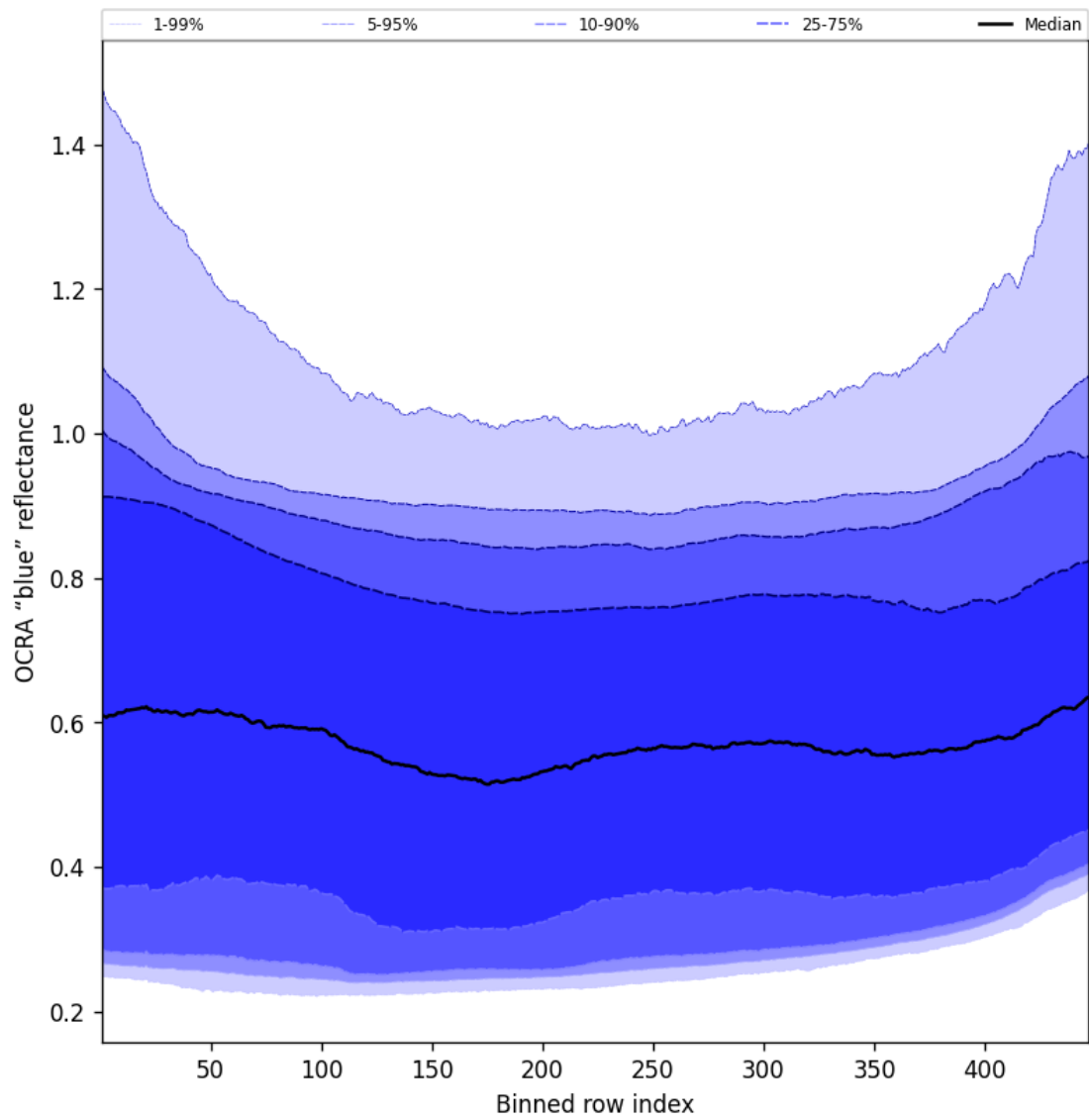
Figure 65: Along track statistics of “OCRA “blue” reflectance” for 2025-02-10 to 2025-02-11
