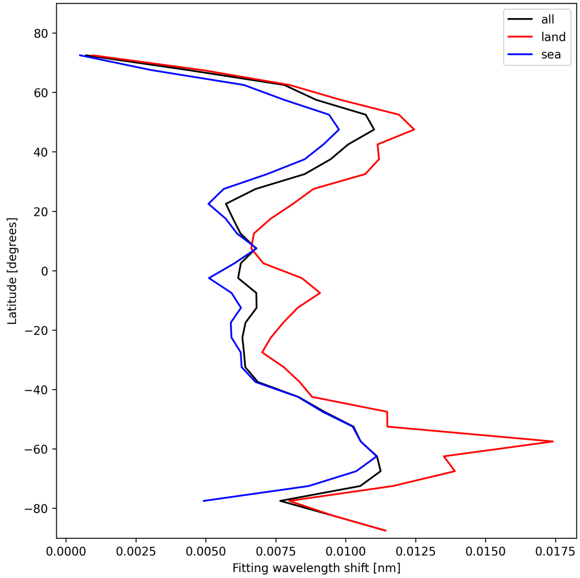
Figure 31: Zonal average of “Fitting wavelength shift” for 2025-02-10 to 2025-02-11.
