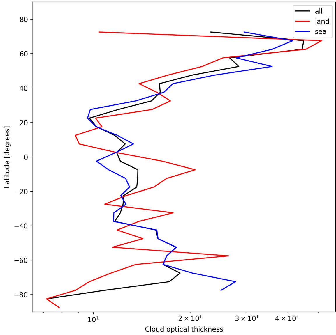
Figure 23: Zonal average of “Cloud optical thickness” for 2025-02-10 to 2025-02-11.
