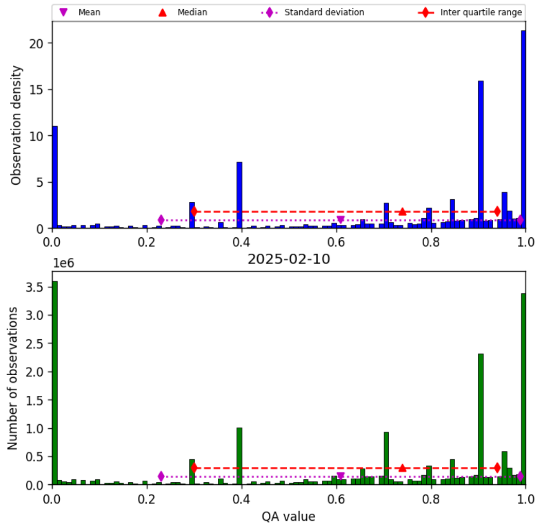
Figure 36: Histogram of “QA value” for 2025-02-10 to 2025-02-11
