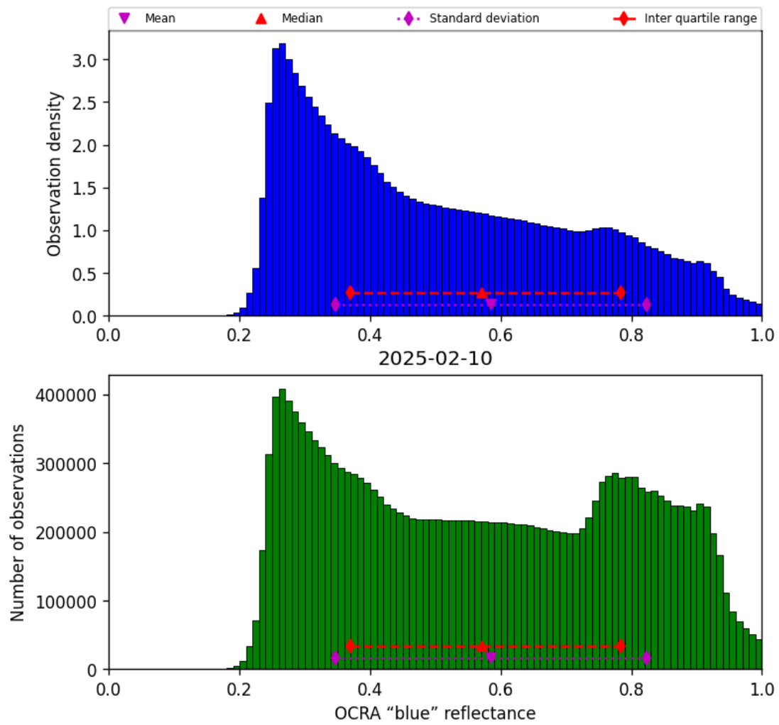
Figure 49: Histogram of “OCRA “blue” reflectance” for 2025-02-10 to 2025-02-11
