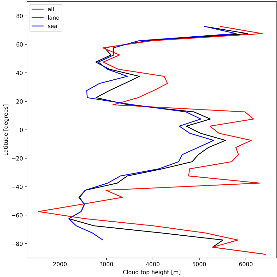
Figure 22: Zonal average of “Cloud top height” for 2025-02-10 to 2025-02-11.
