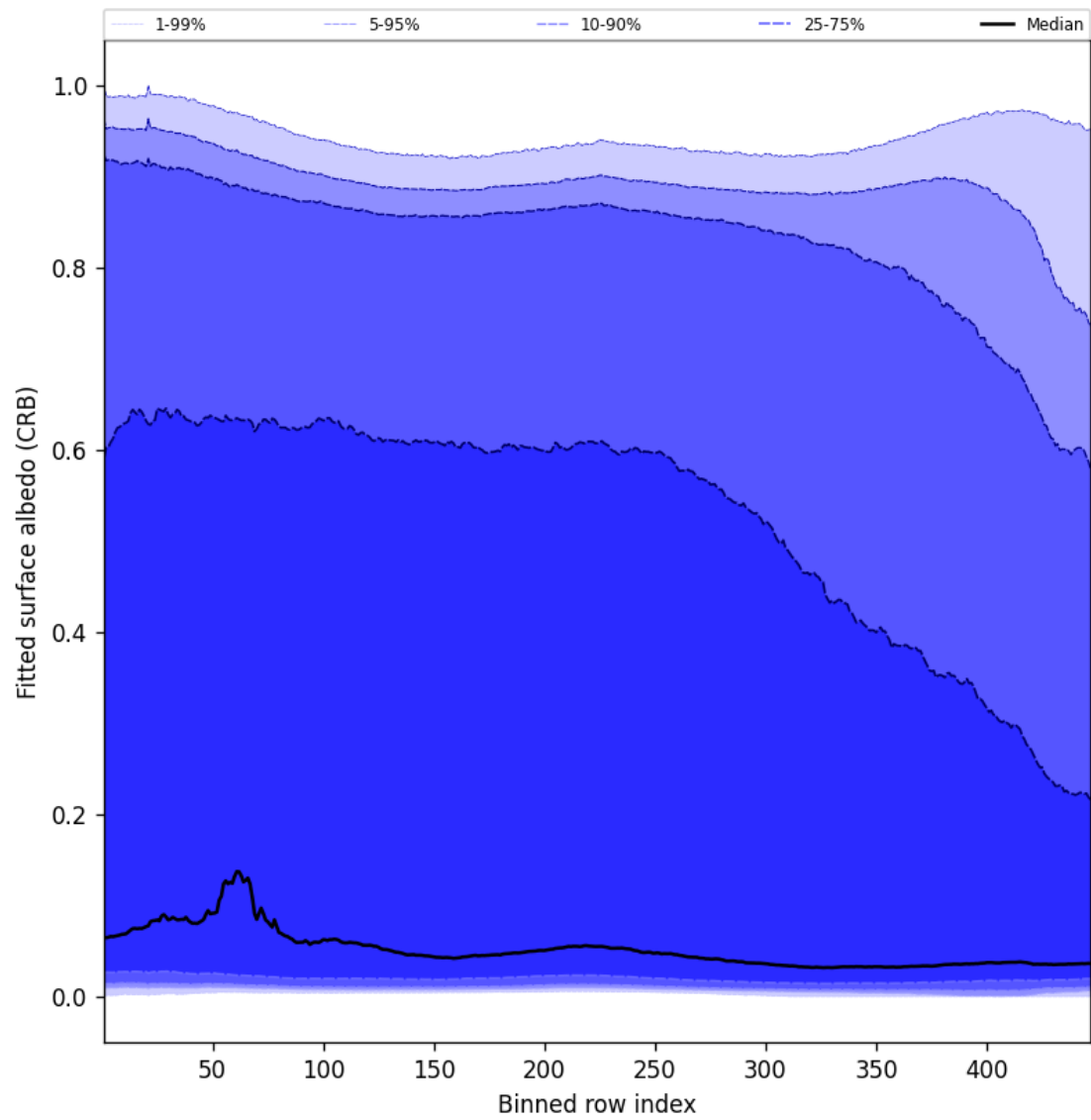
Figure 60: Along track statistics of “Fitted surface albedo (CRB)” for 2025-02-12 to 2025-02-13
