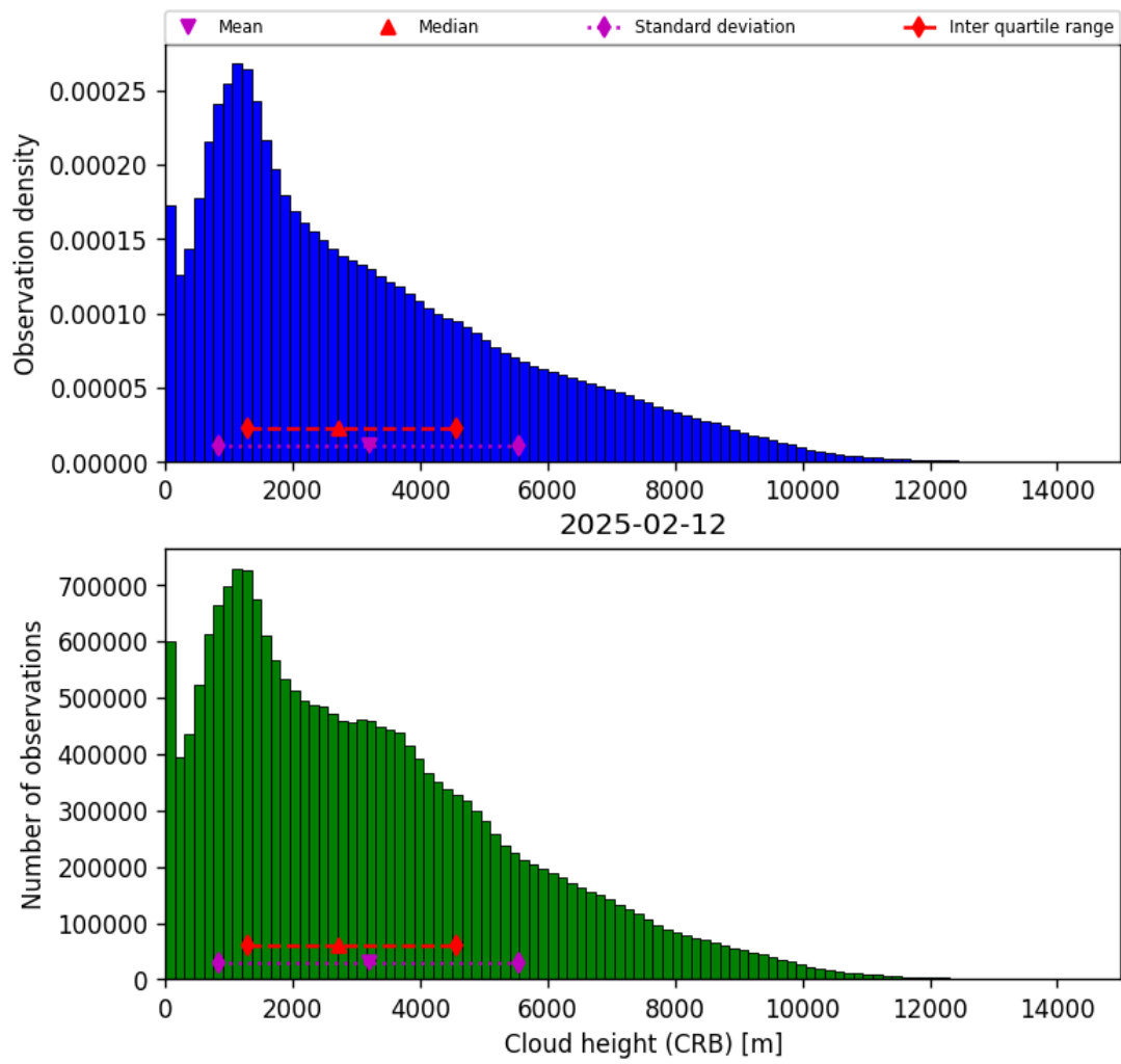
Figure 41: Histogram of “Cloud height (CRB)” for 2025-02-12 to 2025-02-13
