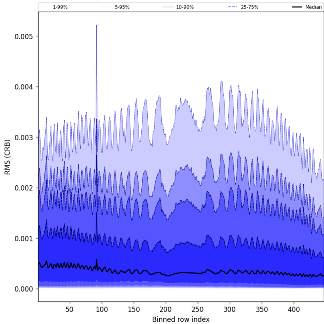
Figure 62: Along track statistics of “RMS (CRB)” for 2025-02-12 to 2025-02-13
