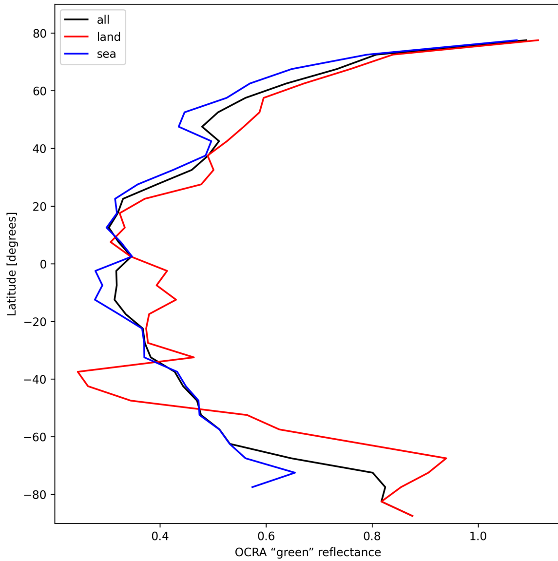
Figure 34: Zonal average of “OCRA “green” reflectance” for 2025-02-12 to 2025-02-13.
