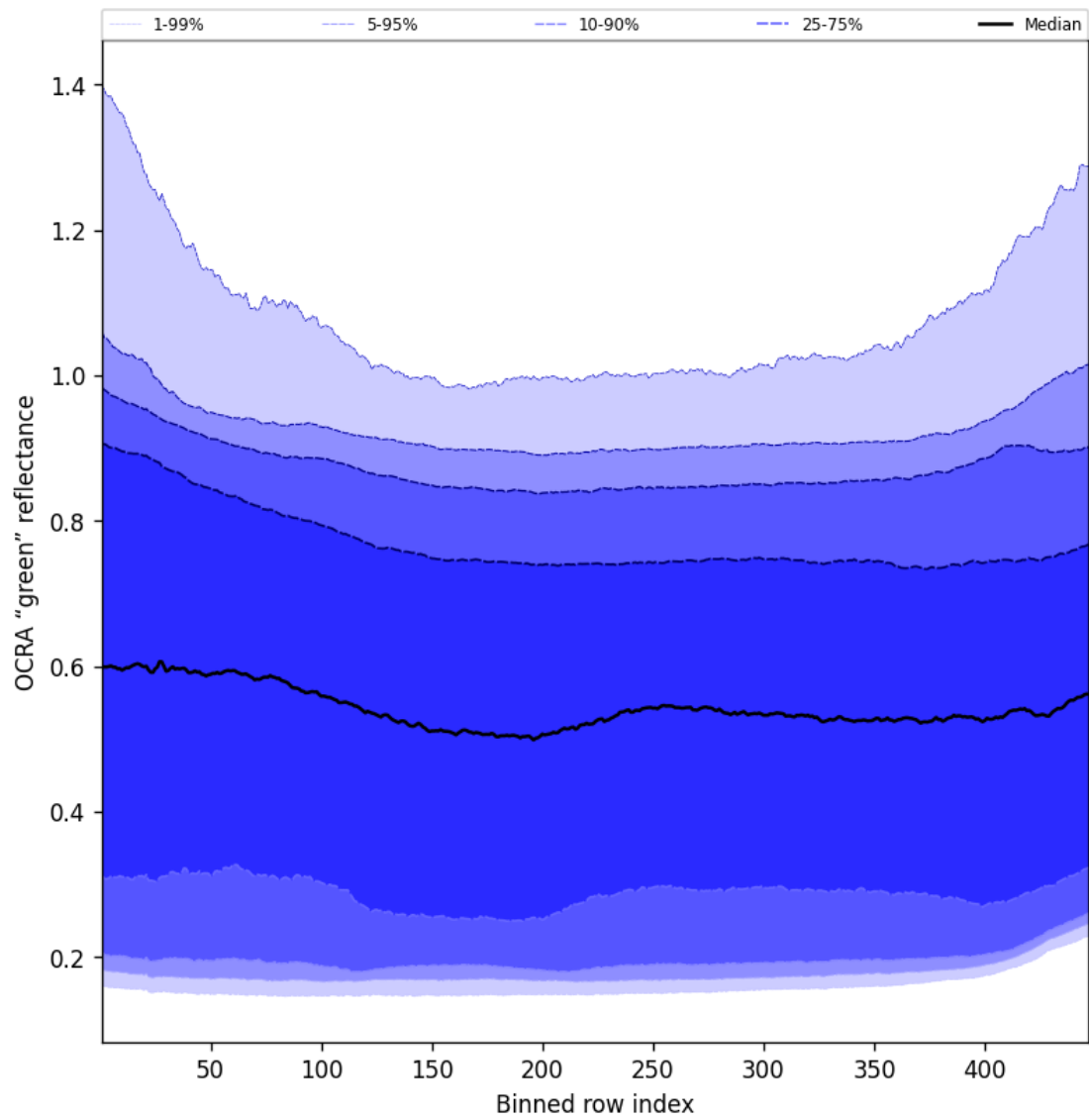
Figure 66: Along track statistics of "OCRA "green" reflectance" for 2025-02-12 to 2025-02-13
