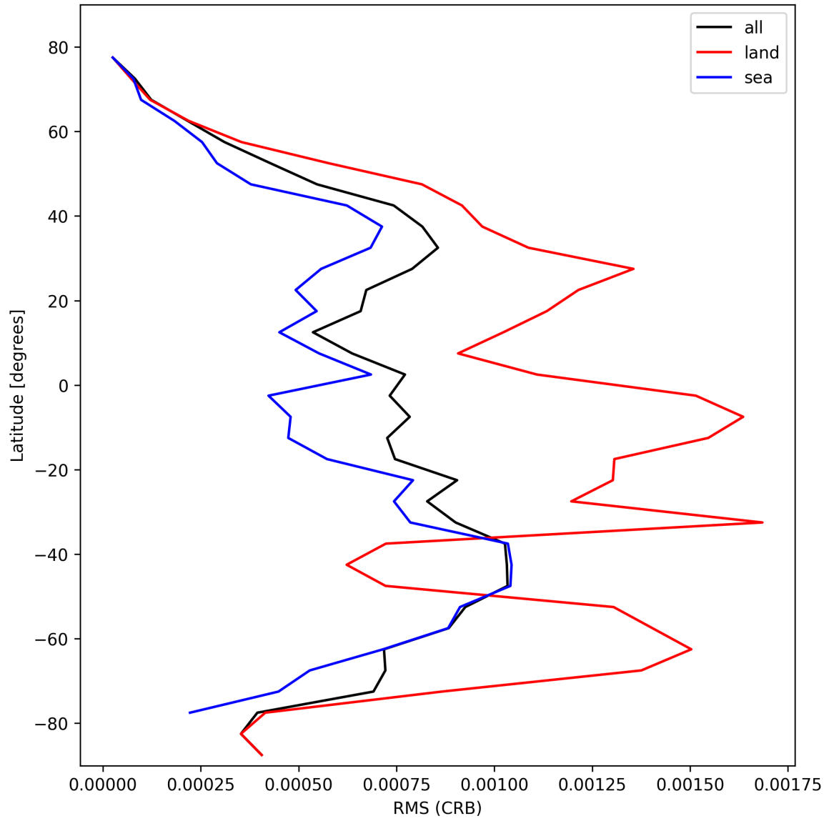
Figure 30: Zonal average of “RMS (CRB)” for 2025-02-12 to 2025-02-13.
