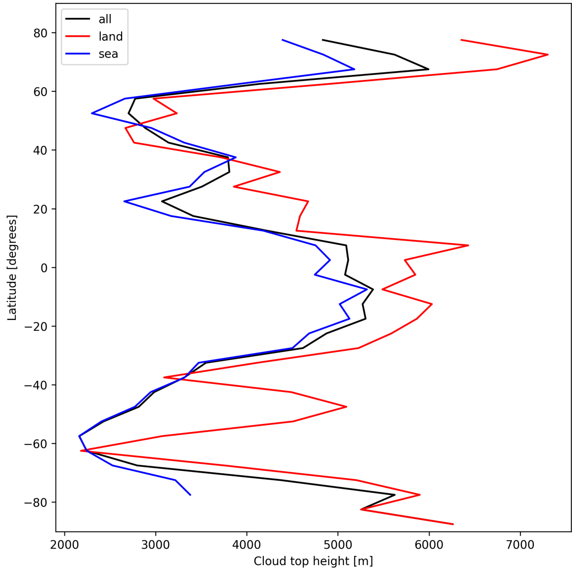
Figure 22: Zonal average of “Cloud top height” for 2025-02-12 to 2025-02-13.
