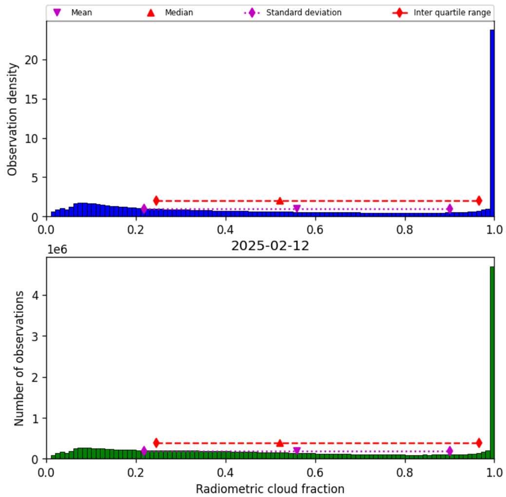
Figure 37: Histogram of “Radiometric cloud fraction” for 2025-02-12 to 2025-02-13
