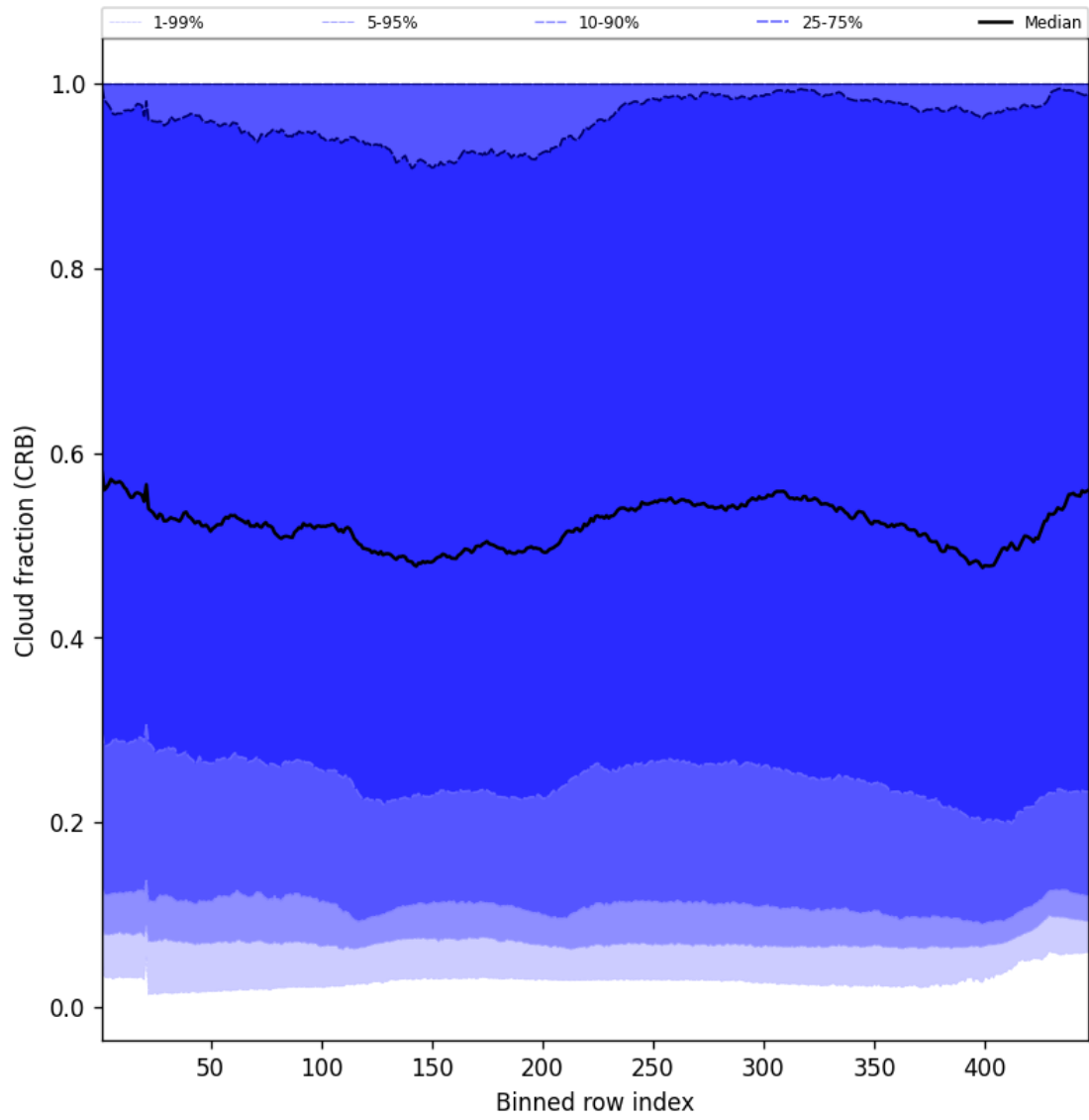
Figure 56: Along track statistics of “Cloud fraction (CRB)” for 2025-02-12 to 2025-02-13
