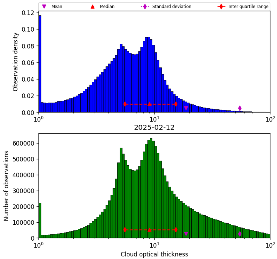
Figure 39: Histogram of “Cloud optical thickness” for 2025-02-12 to 2025-02-13
