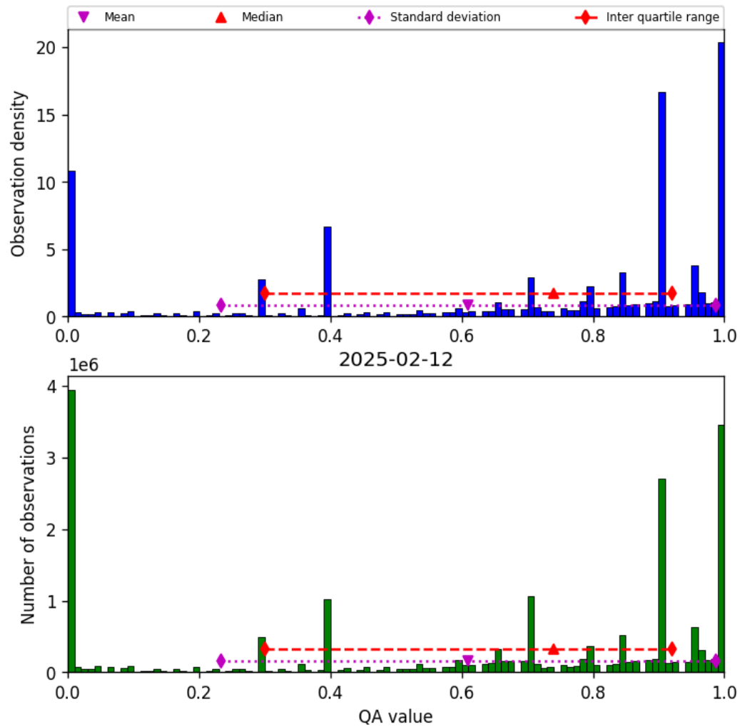
Figure 36: Histogram of “QA value” for 2025-02-12 to 2025-02-13
