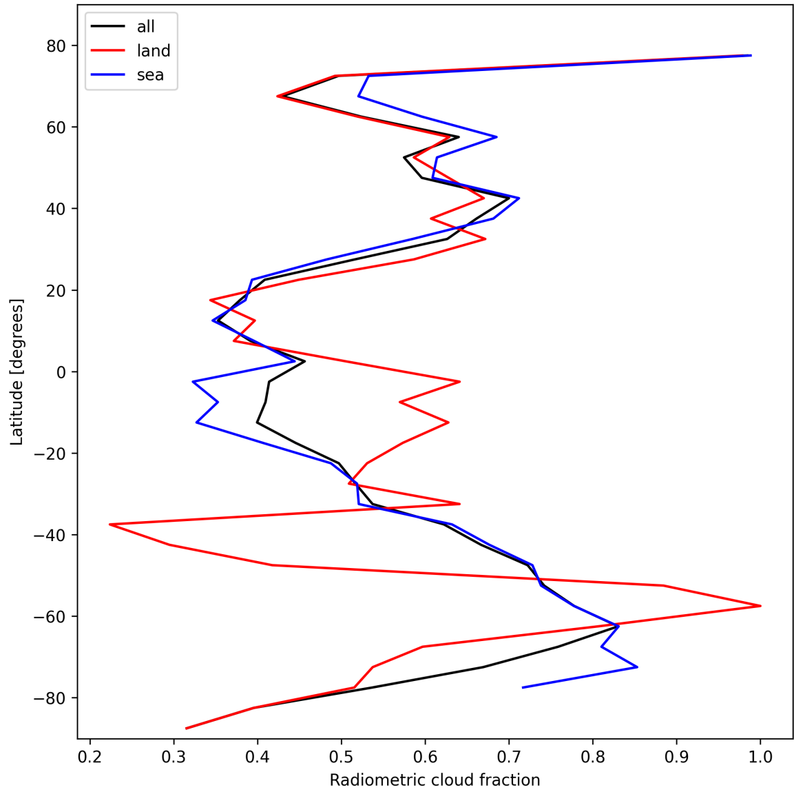
Figure 21: Zonal average of “Radiometric cloud fraction” for 2025-02-12 to 2025-02-13.
