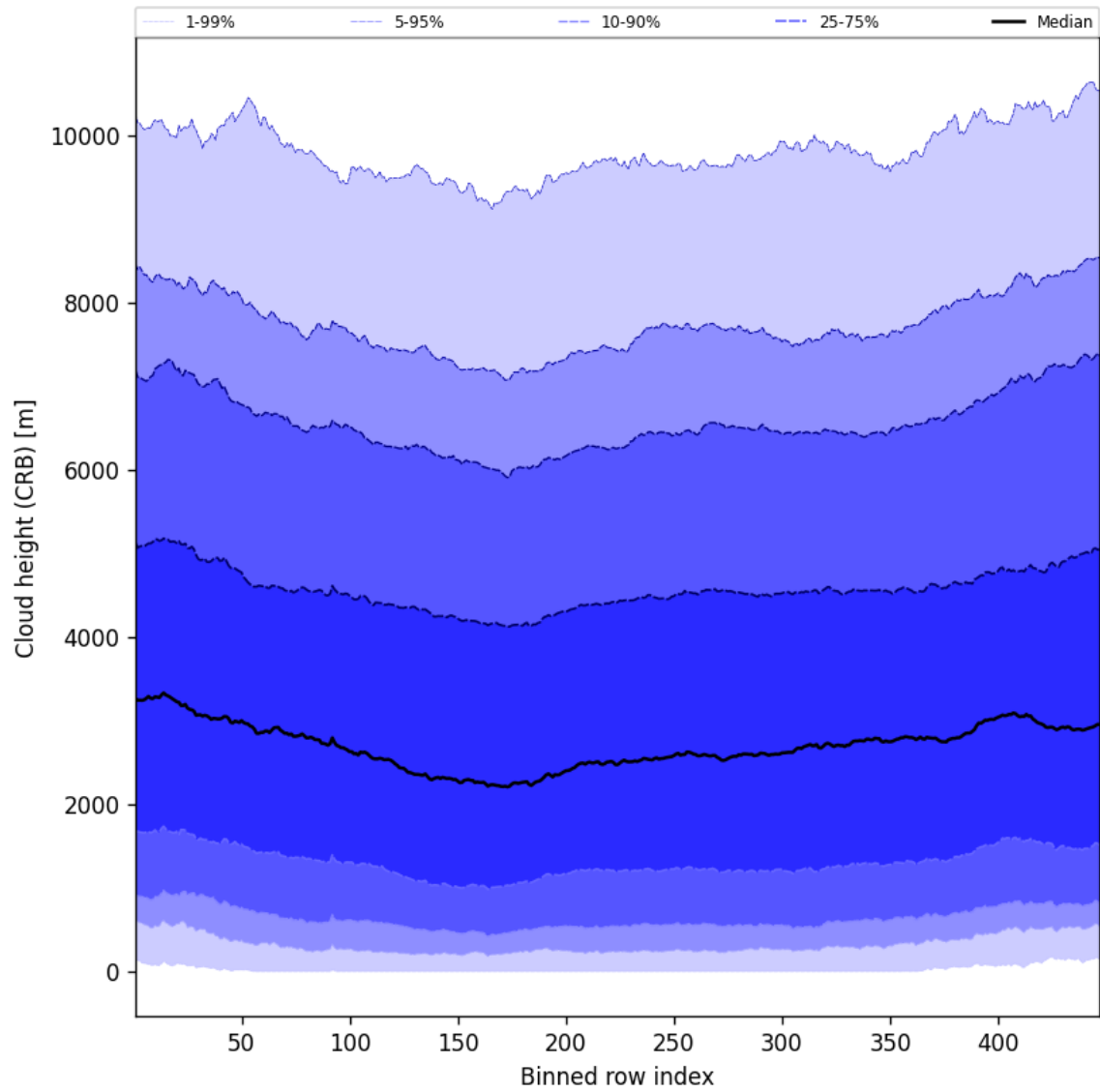
Figure 57: Along track statistics of “Cloud height (CRB)” for 2025-02-12 to 2025-02-13
