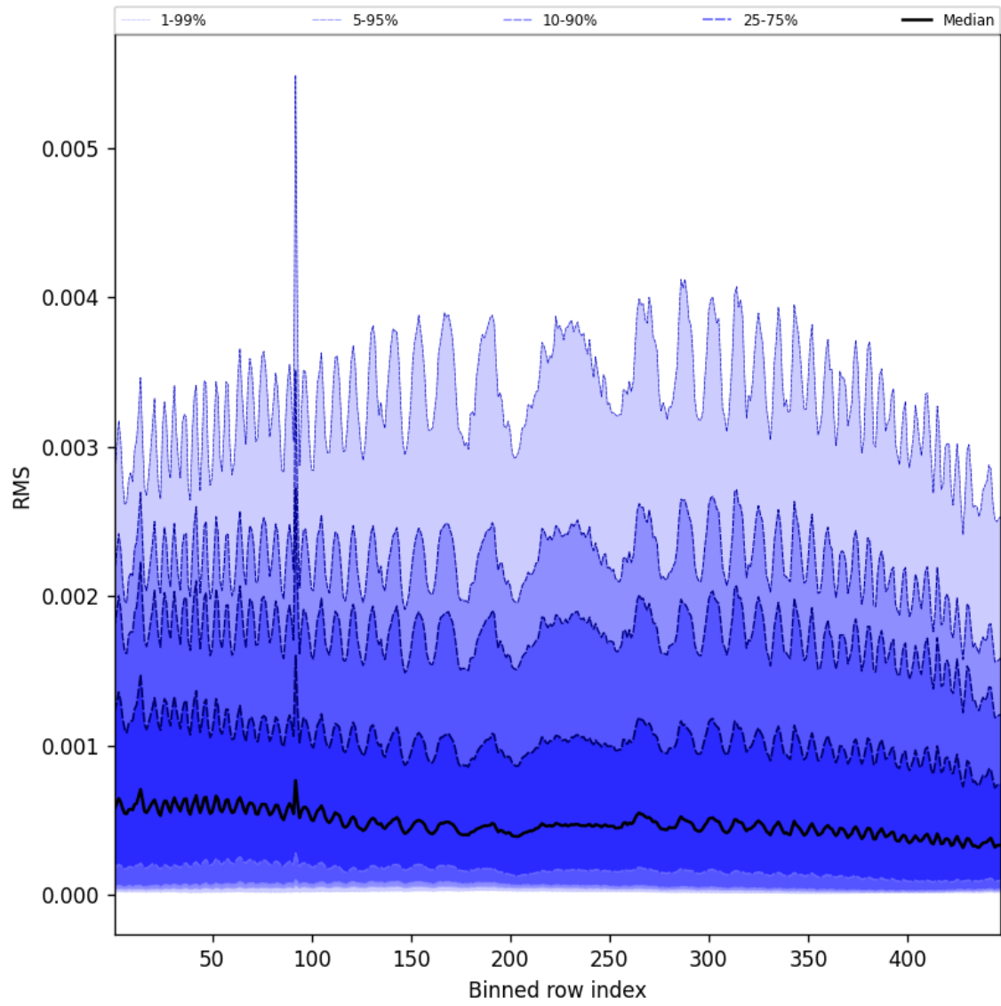
Figure 61: Along track statistics of “RMS” for 2025-02-12 to 2025-02-13
