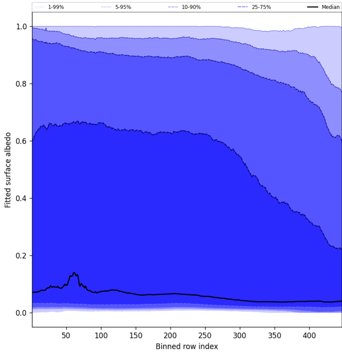
Figure 59: Along track statistics of “Fitted surface albedo” for 2025-02-12 to 2025-02-13
