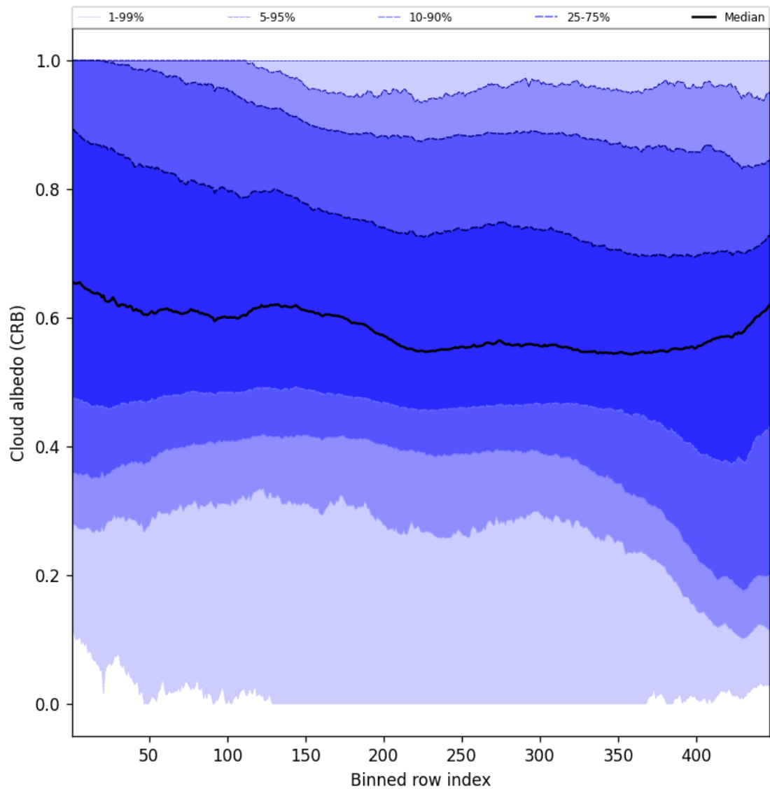
Figure 58: Along track statistics of “Cloud albedo (CRB)” for 2025-02-12 to 2025-02-13
