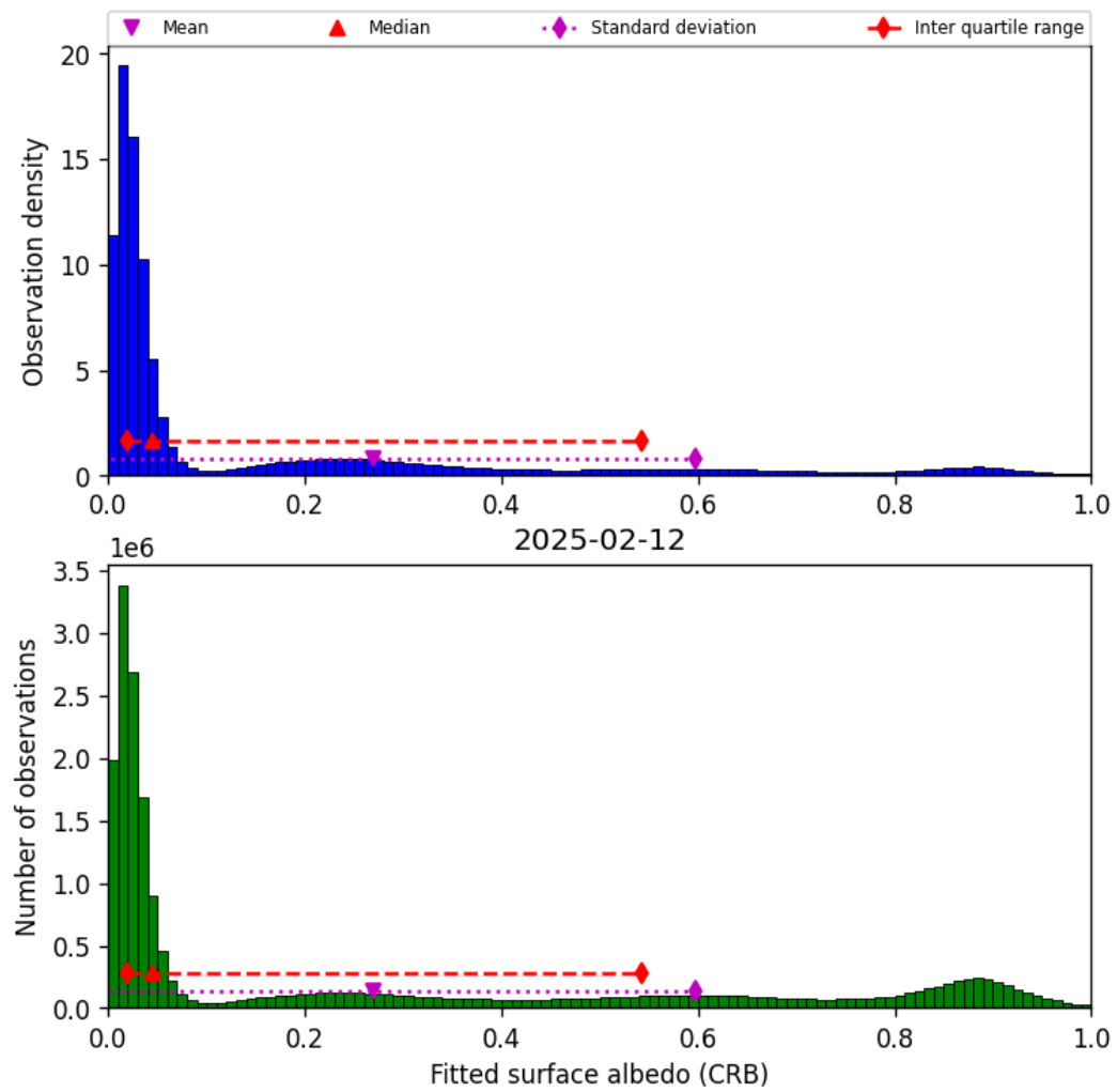
Figure 44: Histogram of “Fitted surface albedo (CRB)” for 2025-02-12 to 2025-02-13
