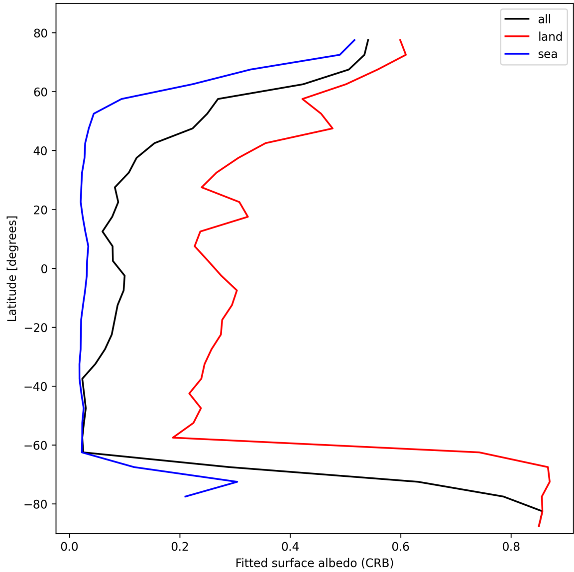
Figure 28: Zonal average of “Fitted surface albedo (CRB)” for 2025-02-12 to 2025-02-13.
