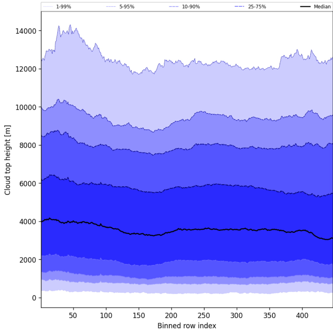
Figure 54: Along track statistics of “Cloud top height” for 2025-02-12 to 2025-02-13
