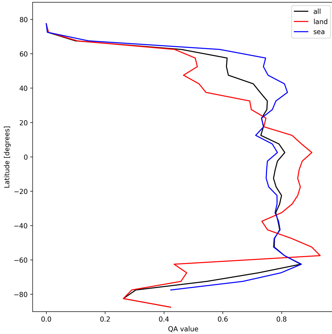
Figure 20: Zonal average of “QA value” for 2025-02-12 to 2025-02-13.
