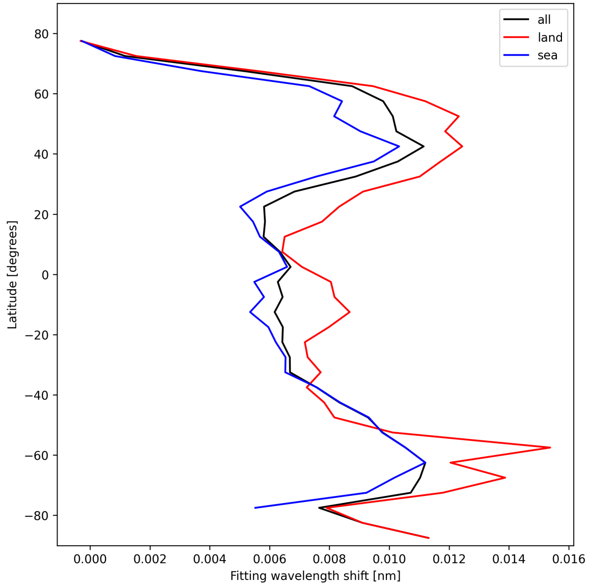
Figure 31: Zonal average of “Fitting wavelength shift” for 2025-02-12 to 2025-02-13.
