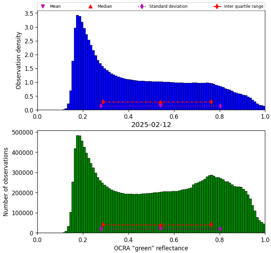
Figure 50: Histogram of “OCRA “green” reflectance” for 2025-02-12 to 2025-02-13
