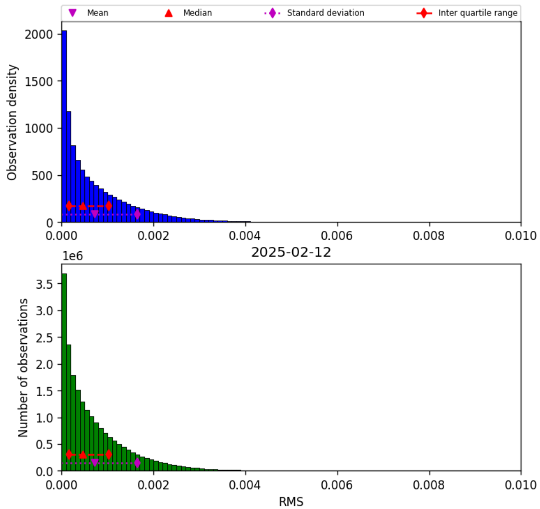
Figure 45: Histogram of “RMS” for 2025-02-12 to 2025-02-13
