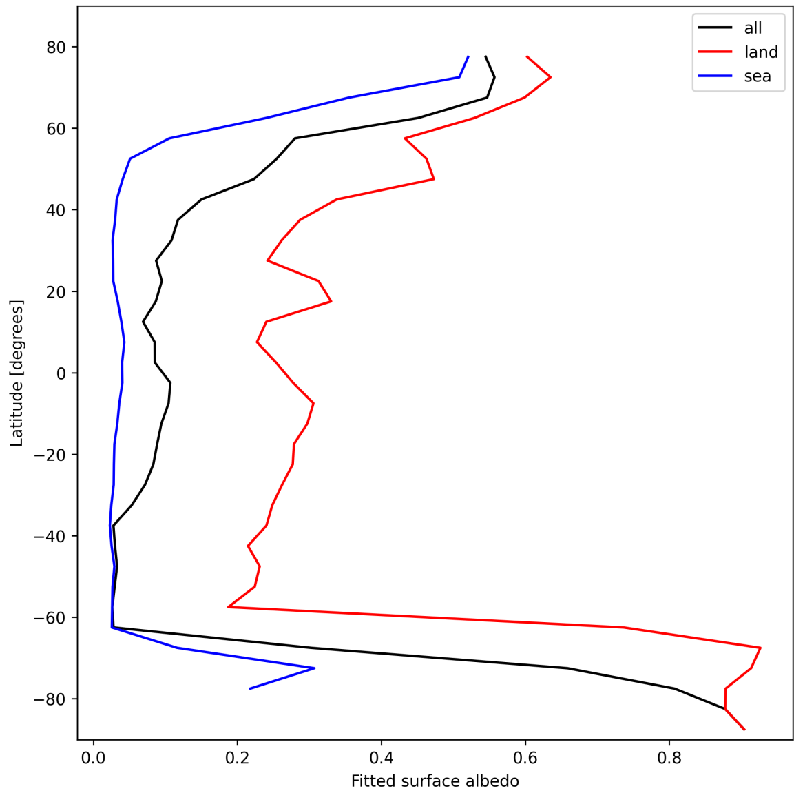
Figure 27: Zonal average of “Fitted surface albedo” for 2025-02-12 to 2025-02-13.
