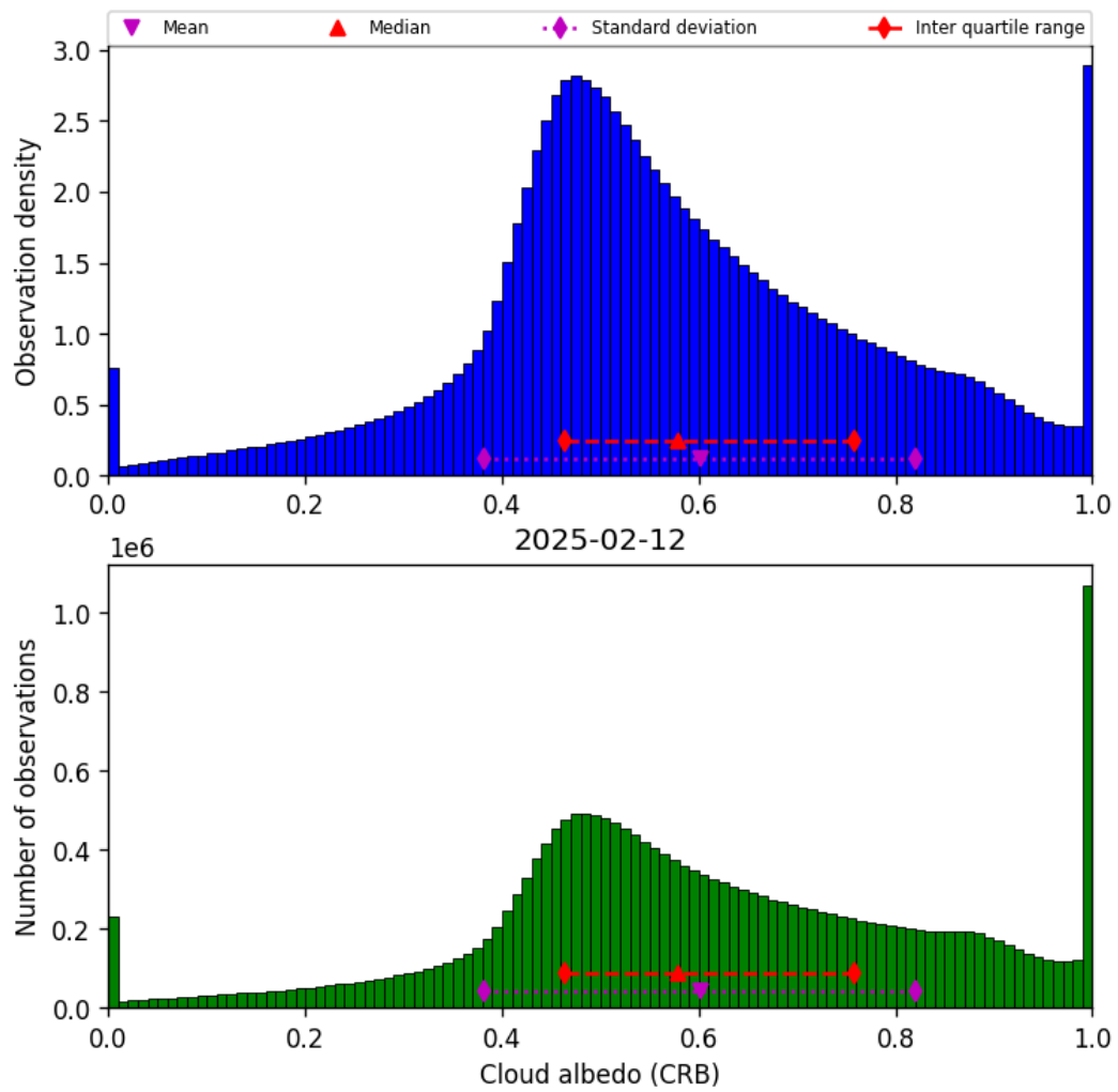
Figure 42: Histogram of “Cloud albedo (CRB)” for 2025-02-12 to 2025-02-13
