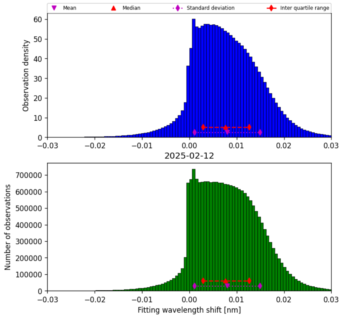
Figure 47: Histogram of “Fitting wavelength shift” for 2025-02-12 to 2025-02-13
