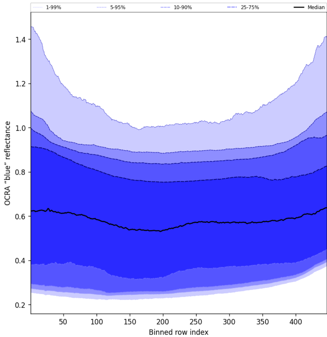
Figure 65: Along track statistics of "OCRA "blue" reflectance" for 2025-02-12 to 2025-02-13
