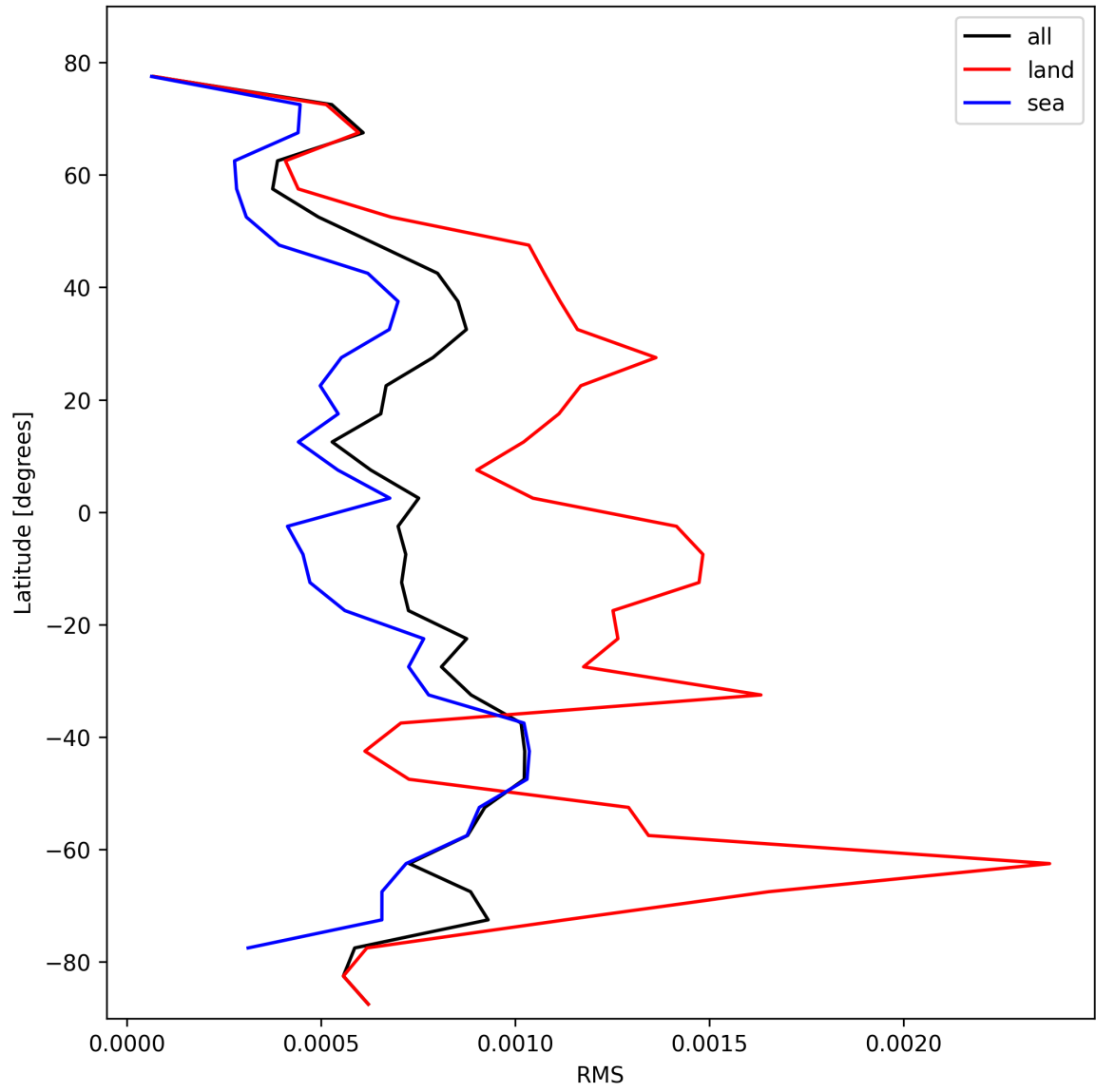
Figure 29: Zonal average of “RMS” for 2025-02-12 to 2025-02-13.
