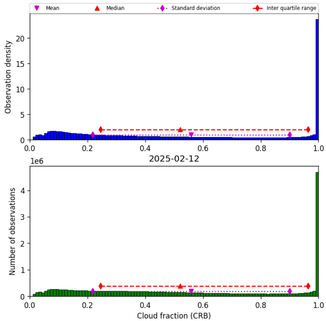
Figure 40: Histogram of “Cloud fraction (CRB)” for 2025-02-12 to 2025-02-13
