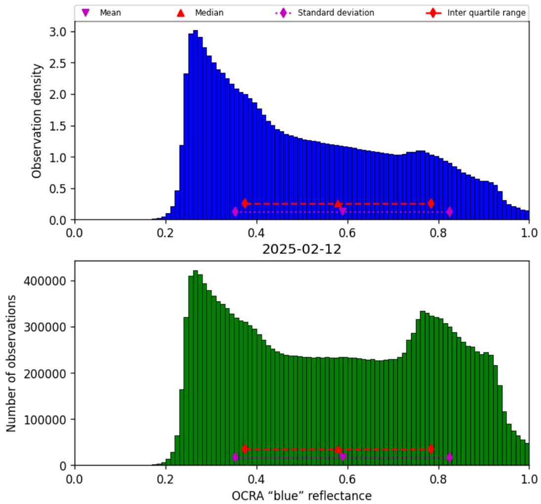
Figure 49: Histogram of "OCRA "blue" reflectance" for 2025-02-12 to 2025-02-13
