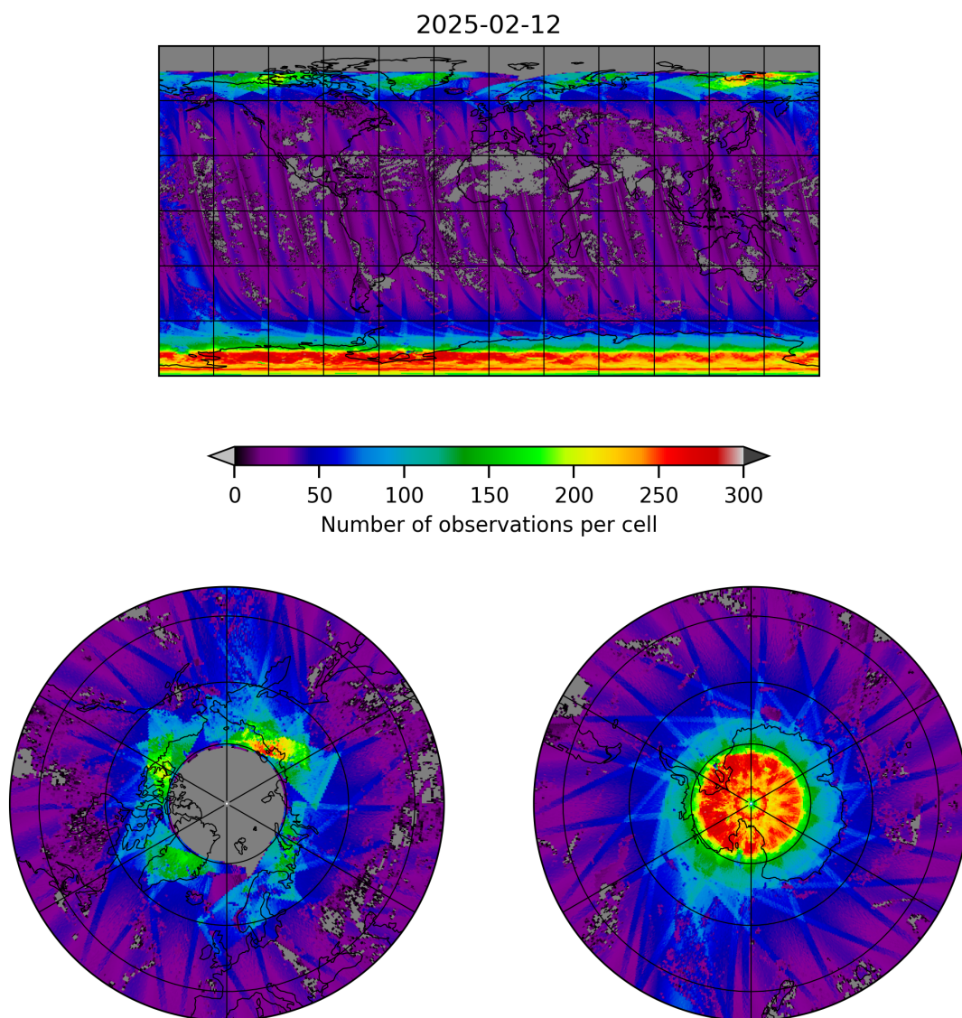
Figure 19: Map of the number of observations for 2025-02-12 to 2025-02-13
