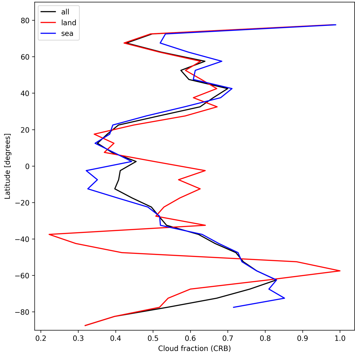
Figure 24: Zonal average of “Cloud fraction (CRB)” for 2025-02-12 to 2025-02-13.
