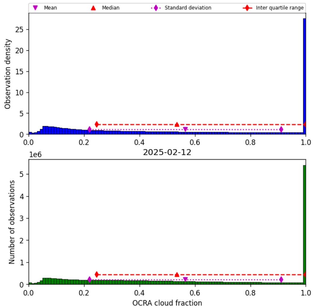
Figure 48: Histogram of “OCRA cloud fraction” for 2025-02-12 to 2025-02-13
