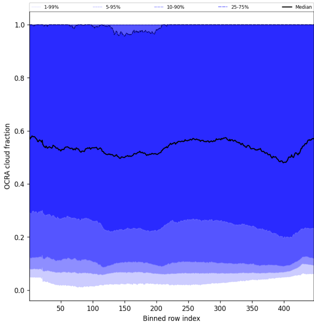
Figure 64: Along track statistics of “OCRA cloud fraction” for 2025-02-12 to 2025-02-13
