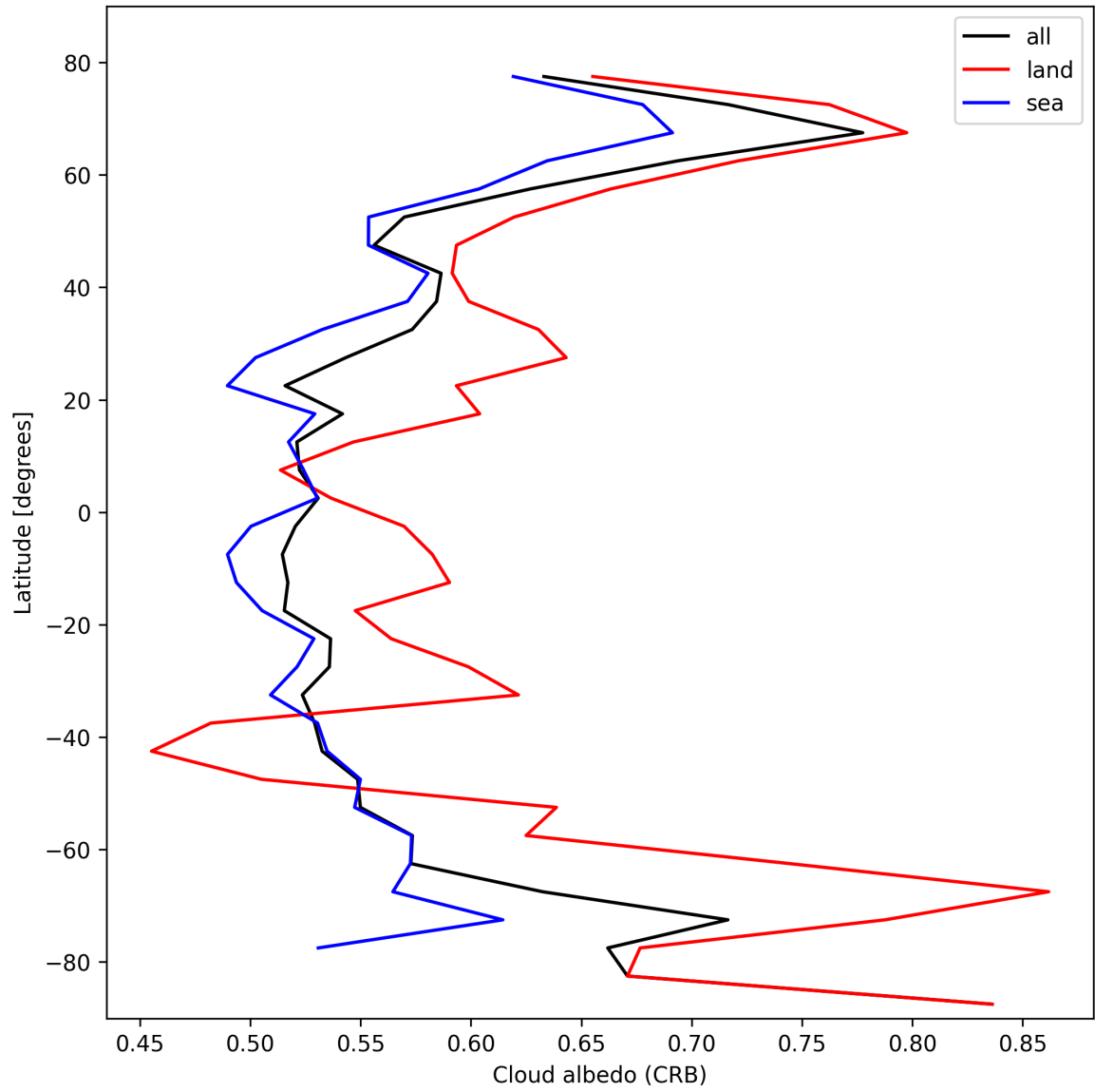
Figure 26: Zonal average of “Cloud albedo (CRB)” for 2025-02-12 to 2025-02-13.
