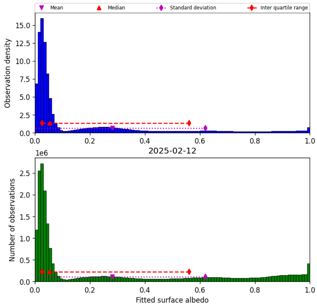
Figure 43: Histogram of “Fitted surface albedo” for 2025-02-12 to 2025-02-13
