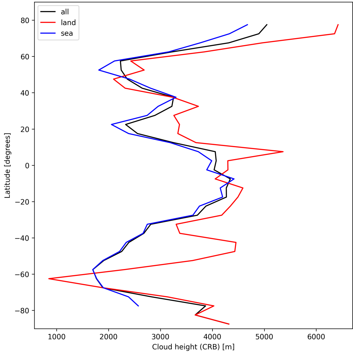
Figure 25: Zonal average of “Cloud height (CRB)” for 2025-02-12 to 2025-02-13.
