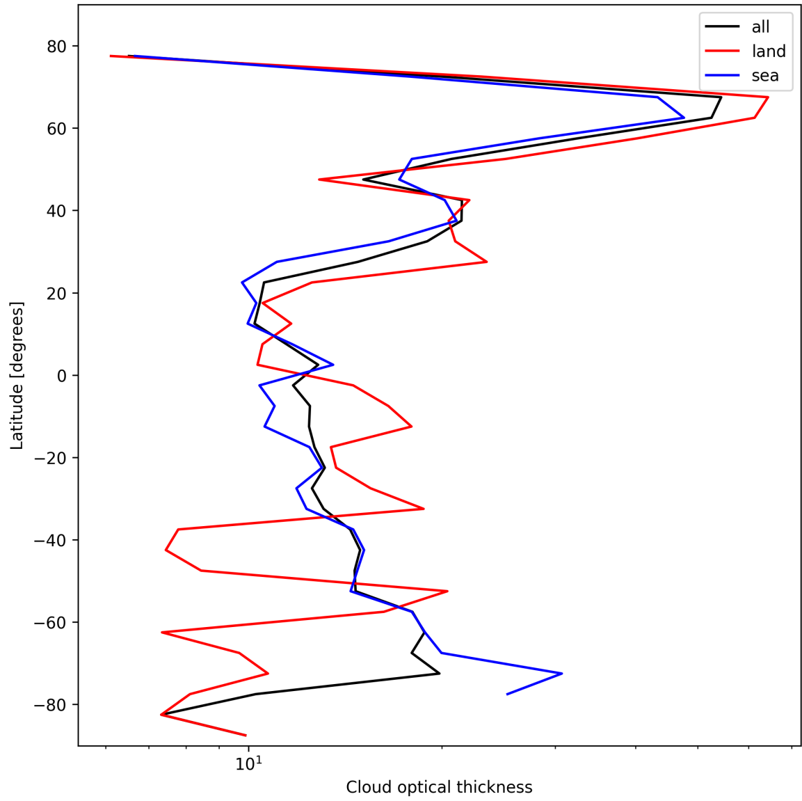
Figure 23: Zonal average of “Cloud optical thickness” for 2025-02-12 to 2025-02-13.
