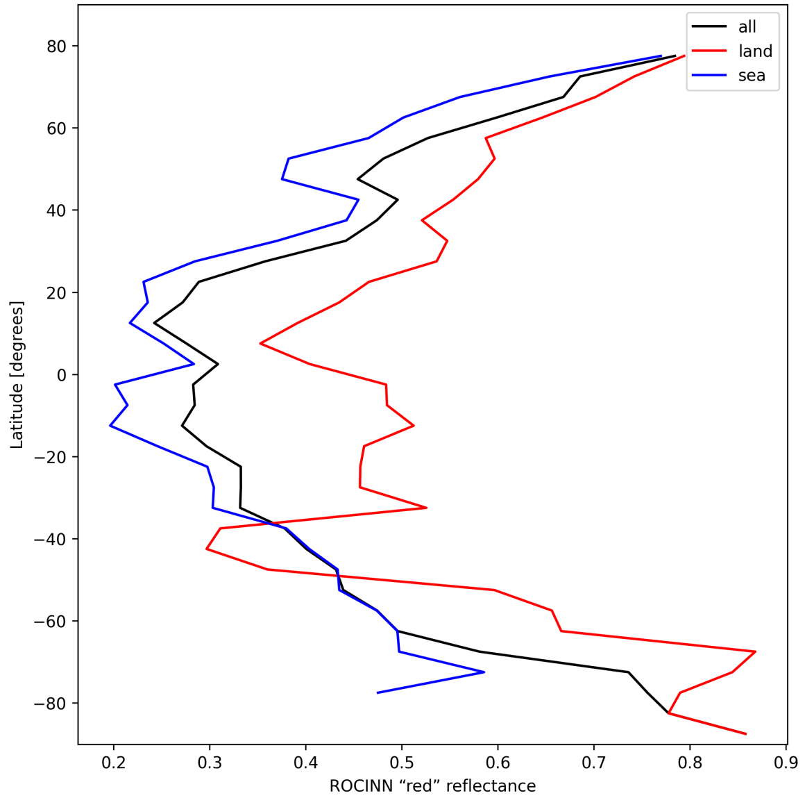
Figure 35: Zonal average of “ROCINN “red” reflectance” for 2025-02-12 to 2025-02-13.
