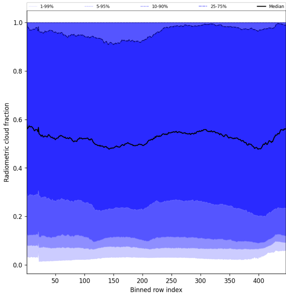
Figure 53: Along track statistics of “Radiometric cloud fraction” for 2025-02-12 to 2025-02-13
