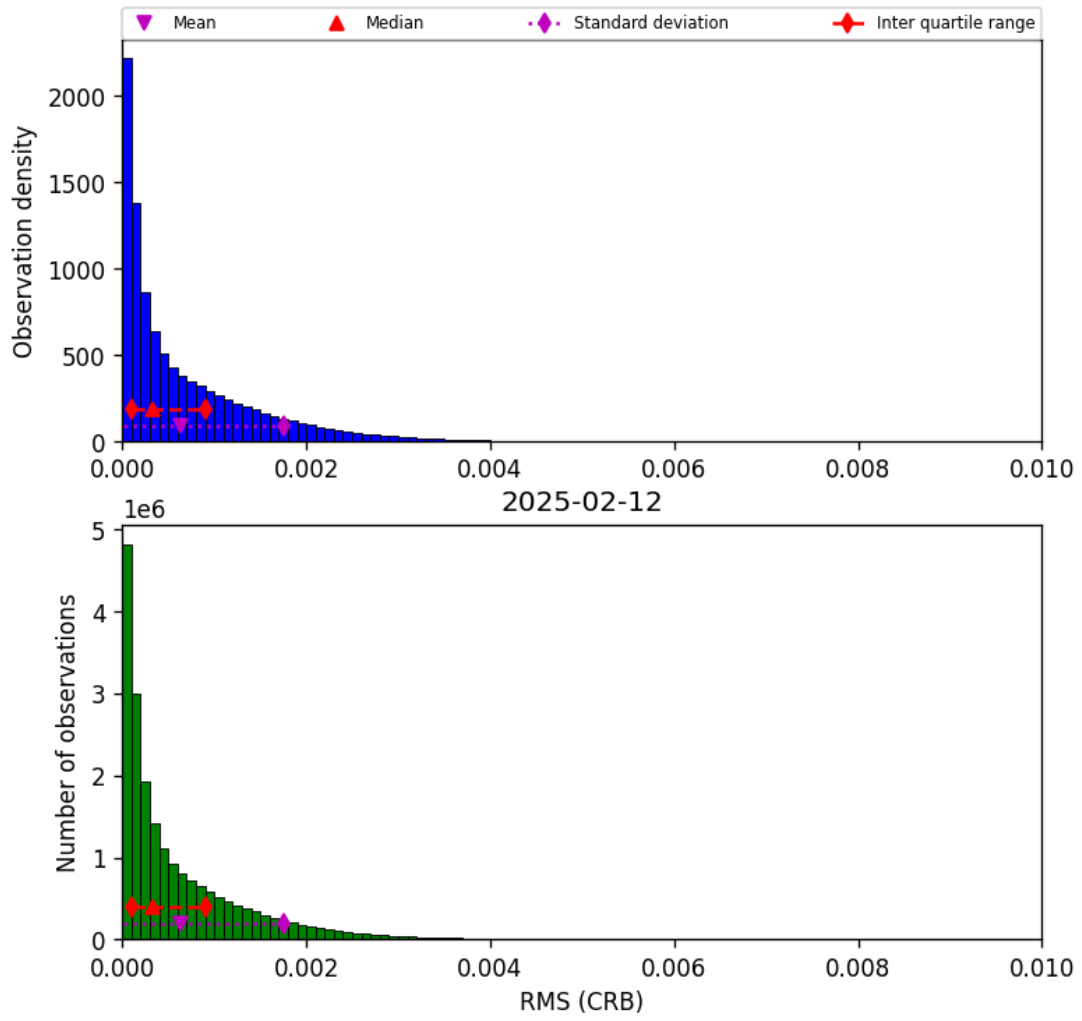
Figure 46: Histogram of "RMS (CRB)" for 2025-02-12 to 2025-02-13
