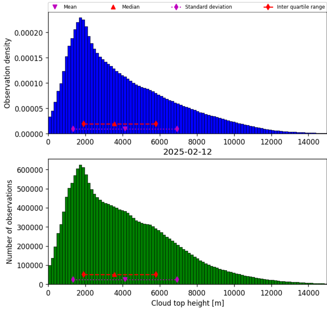
Figure 38: Histogram of “Cloud top height” for 2025-02-12 to 2025-02-13
