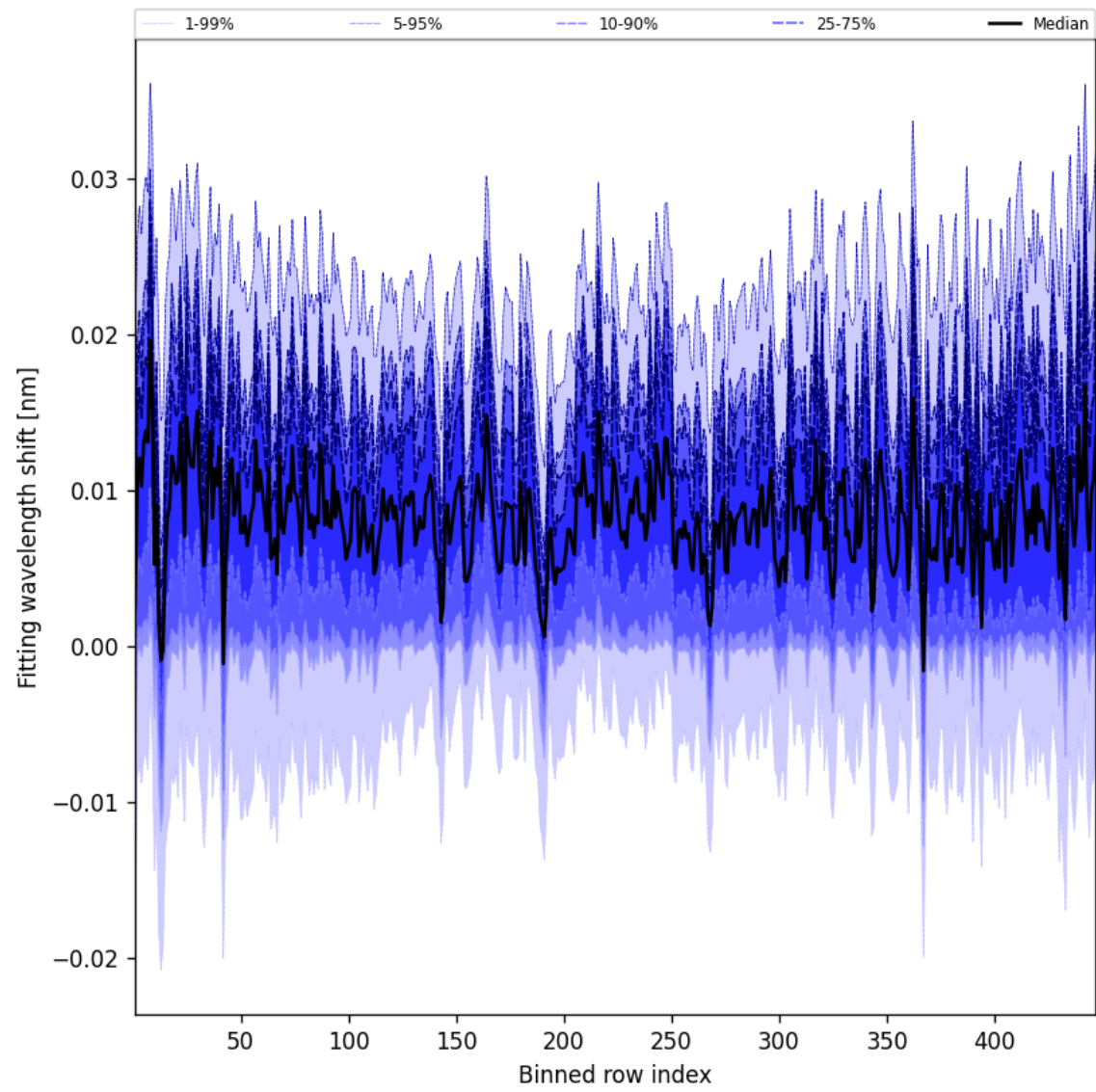
Figure 63: Along track statistics of “Fitting wavelength shift” for 2025-02-12 to 2025-02-13
