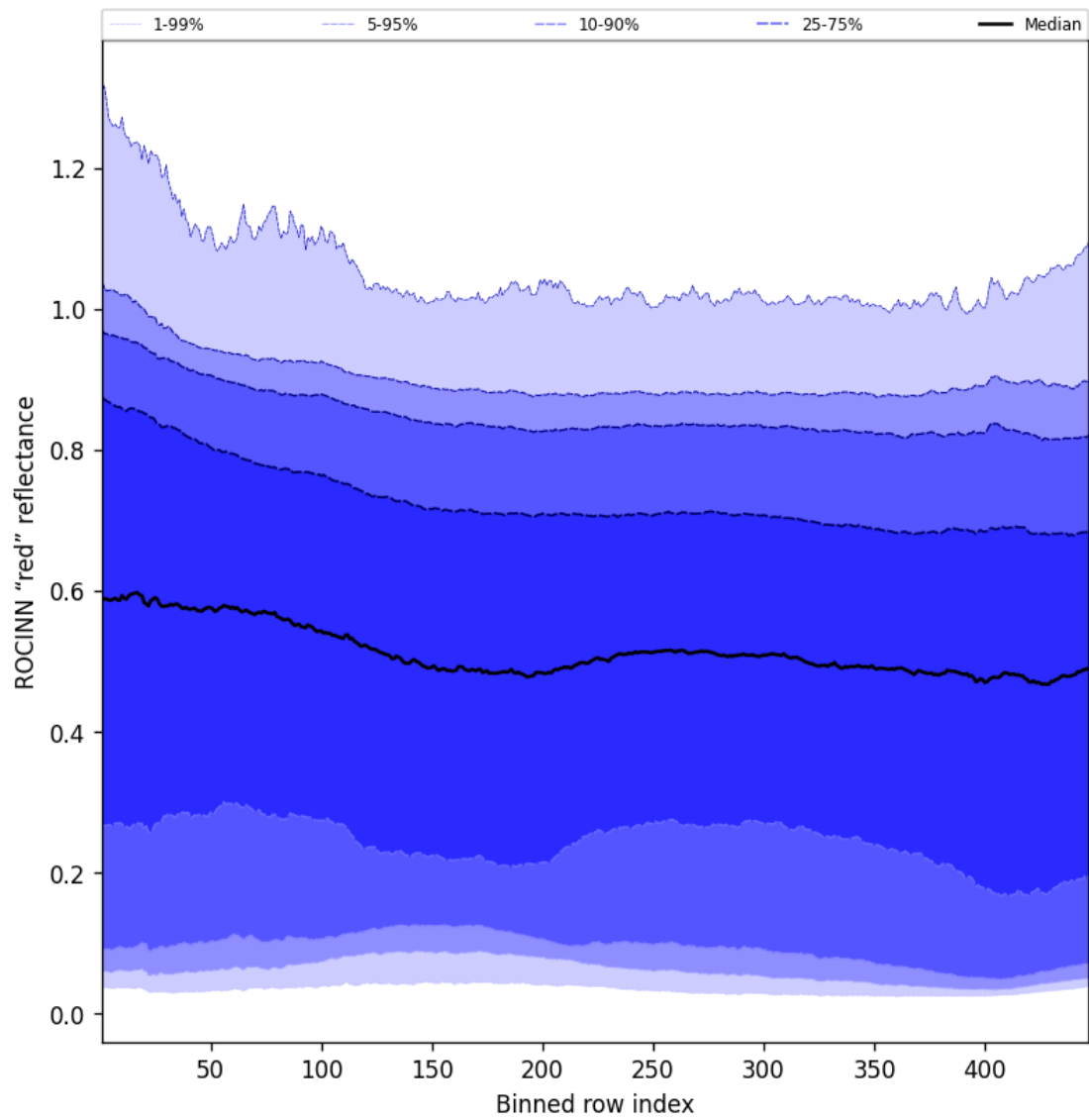
Figure 67: Along track statistics of "ROCINN "red" reflectance" for 2025-02-12 to 2025-02-13
