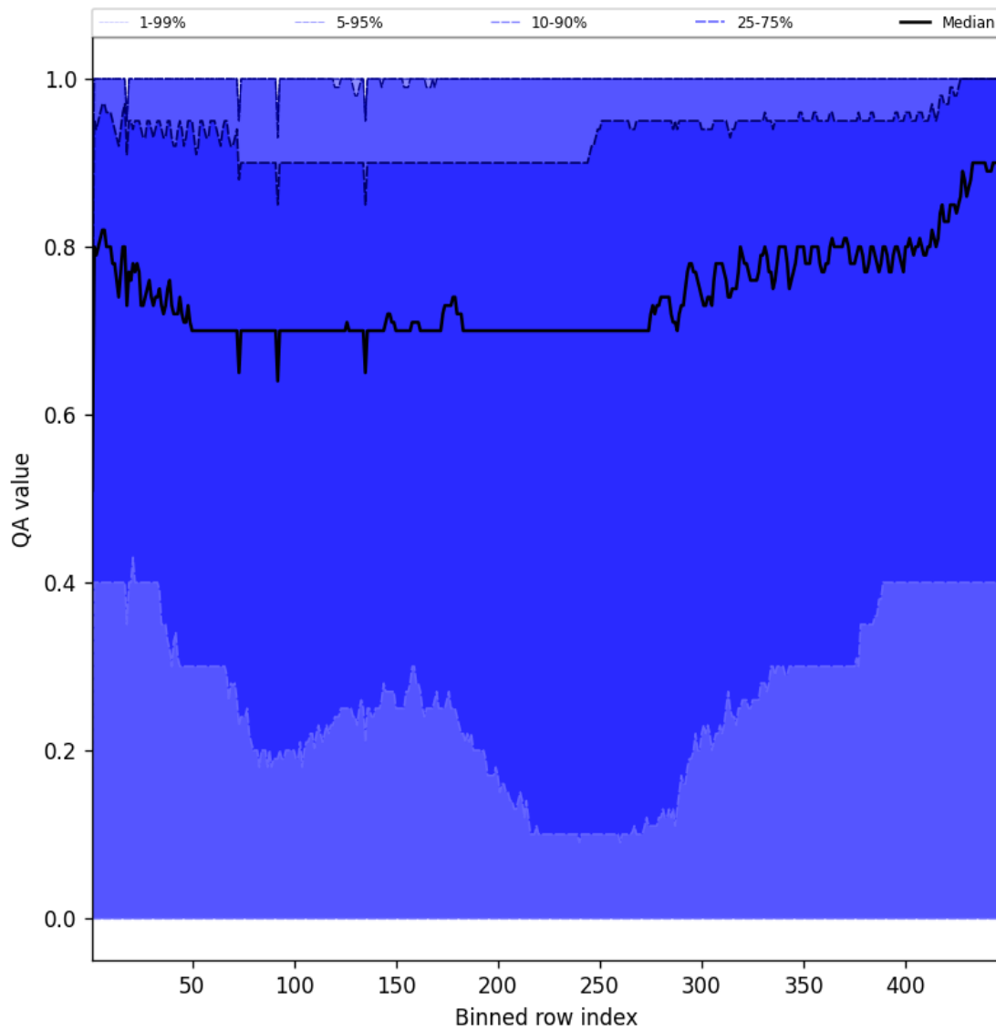
Figure 52: Along track statistics of “QA value” for 2025-02-12 to 2025-02-13
