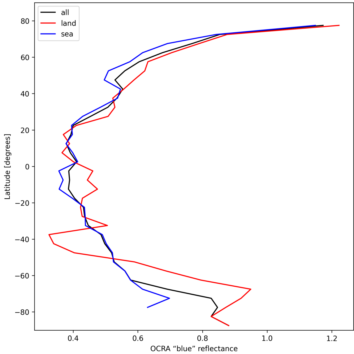
Figure 33: Zonal average of “OCRA “blue” reflectance” for 2025-02-12 to 2025-02-13.
