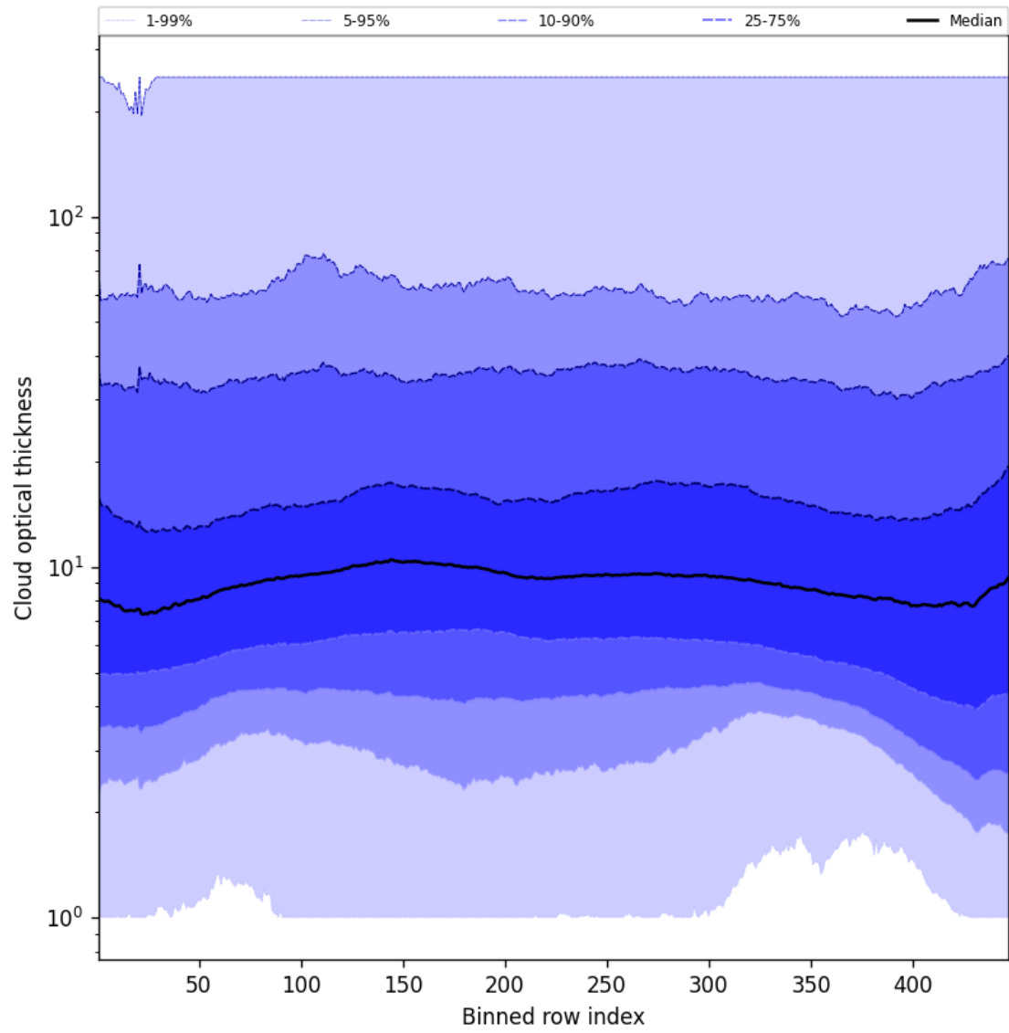
Figure 55: Along track statistics of “Cloud optical thickness” for 2025-02-12 to 2025-02-13
