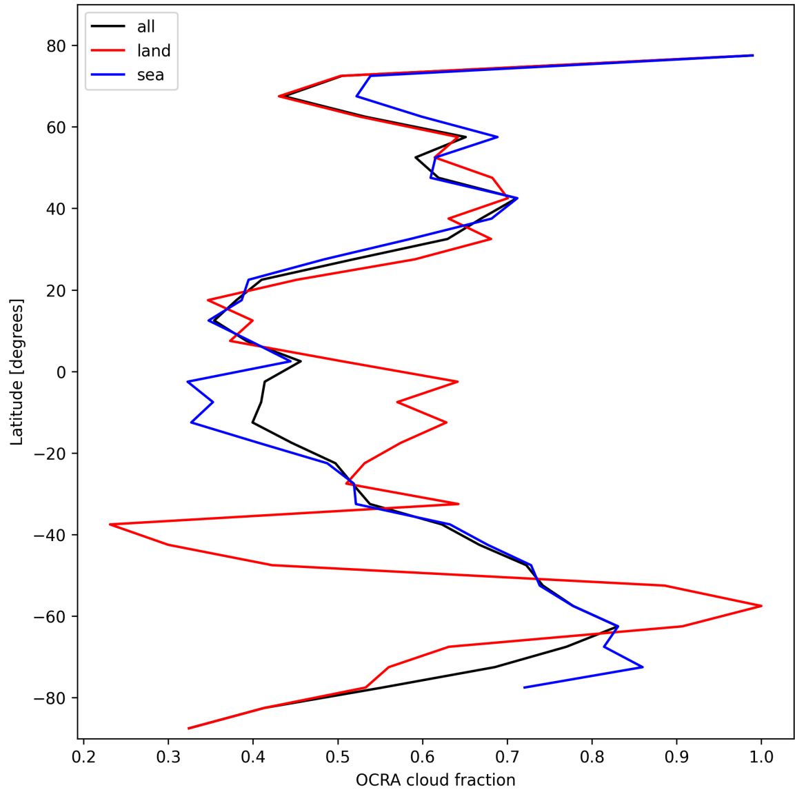
Figure 32: Zonal average of “OCRA cloud fraction” for 2025-02-12 to 2025-02-13.
