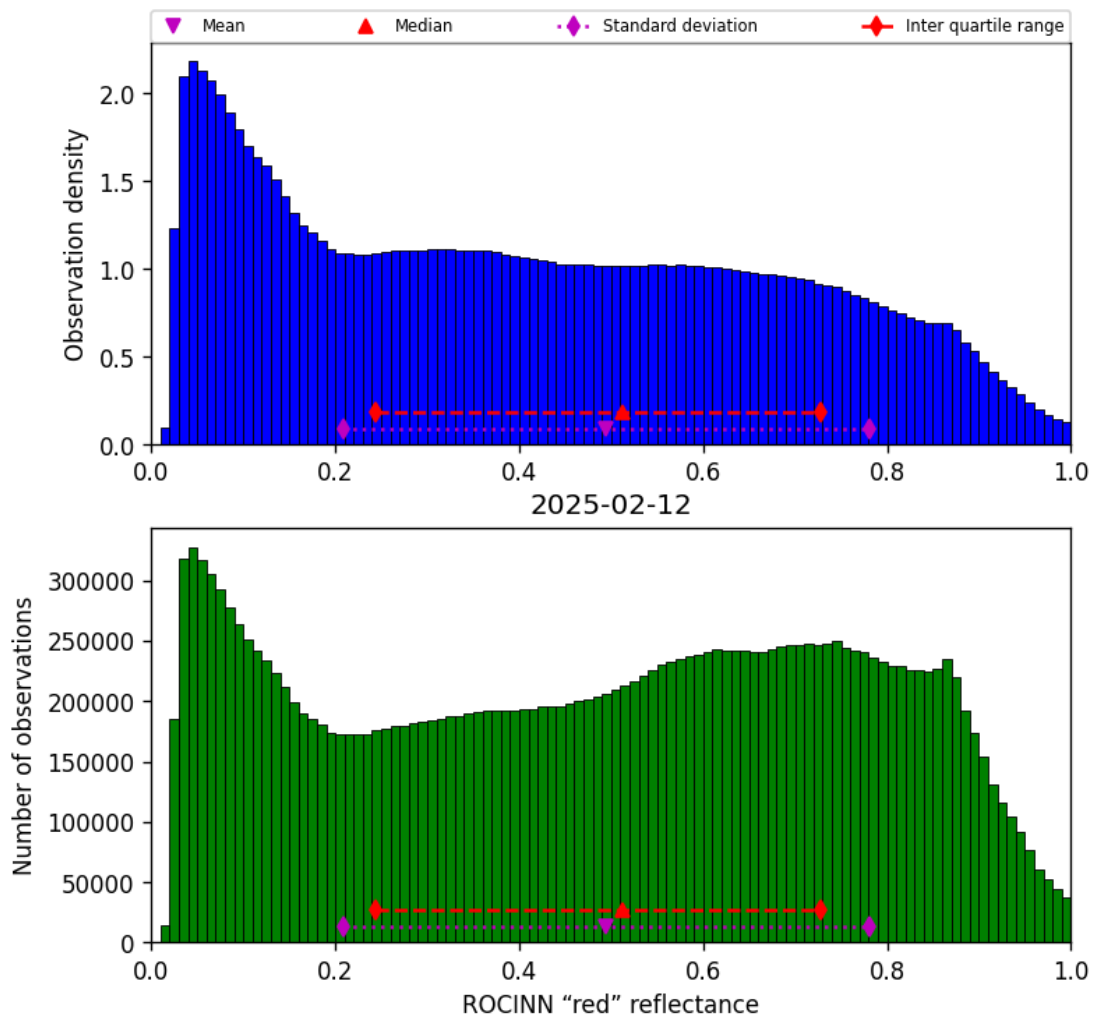
Figure 51: Histogram of “ROCINN “red” reflectance” for 2025-02-12 to 2025-02-13
