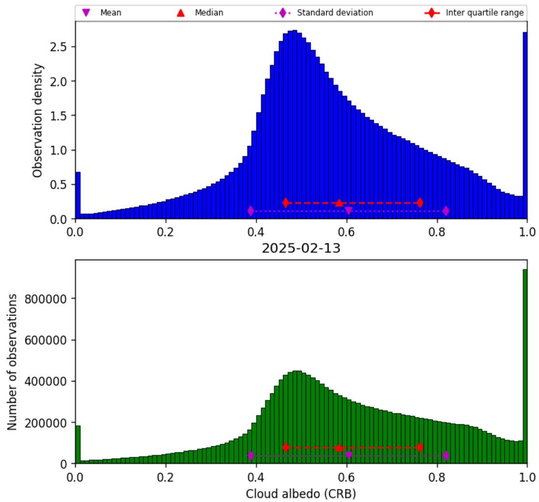
Figure 42: Histogram of “Cloud albedo (CRB)” for 2025-02-13 to 2025-02-14
