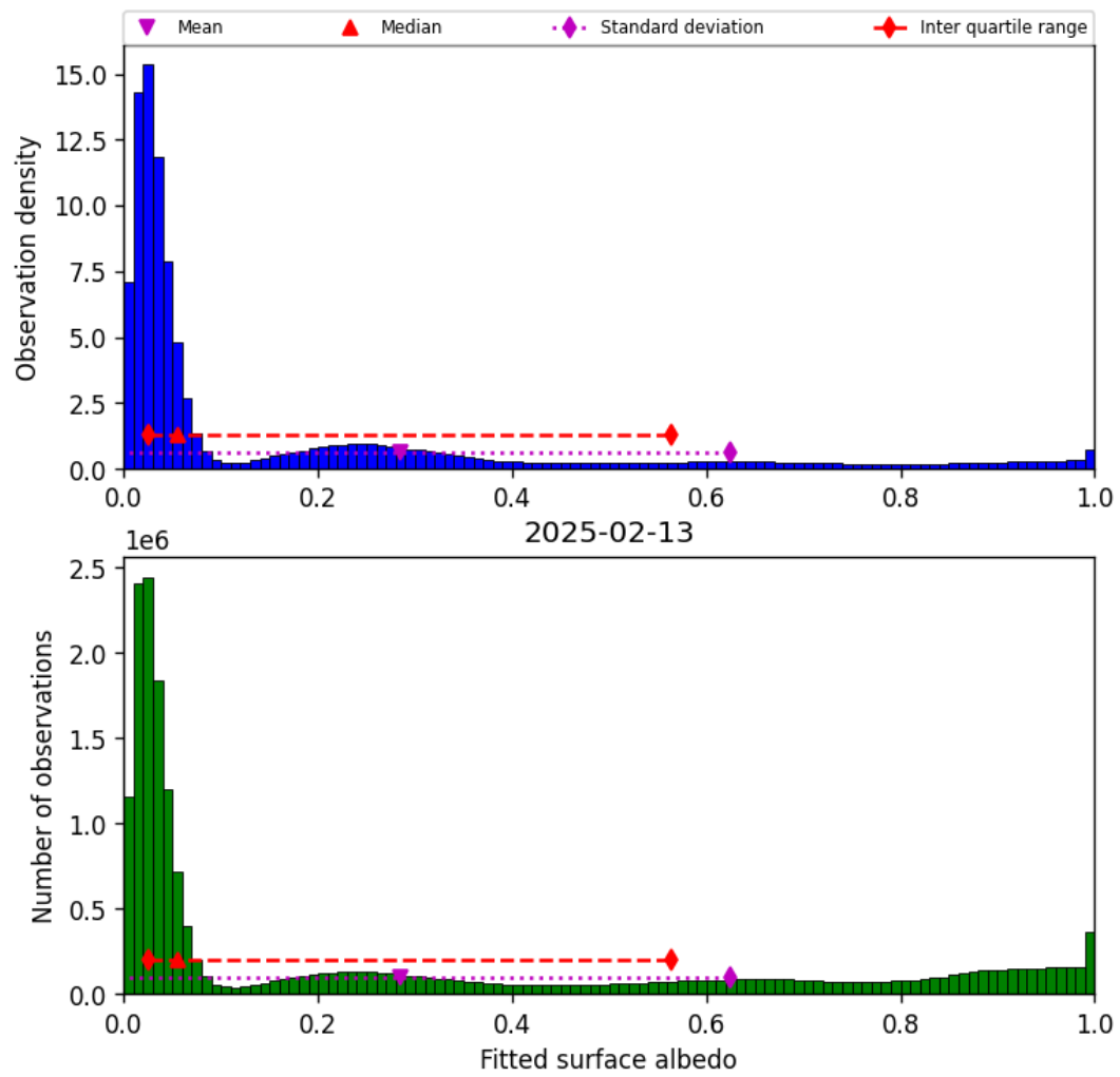
Figure 43: Histogram of “Fitted surface albedo” for 2025-02-13 to 2025-02-14
