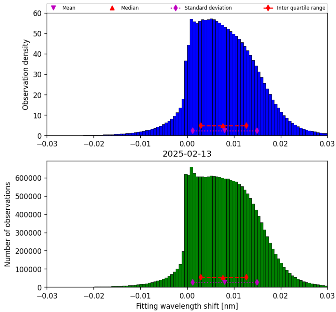
Figure 47: Histogram of “Fitting wavelength shift” for 2025-02-13 to 2025-02-14
