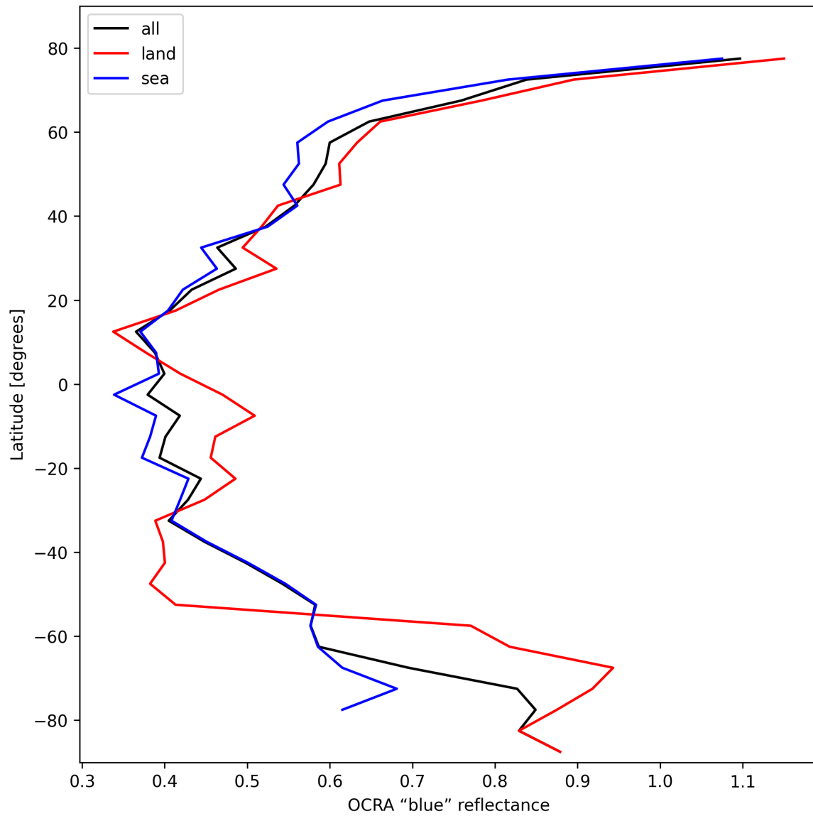
Figure 33: Zonal average of “OCRA “blue” reflectance” for 2025-02-13 to 2025-02-14.
