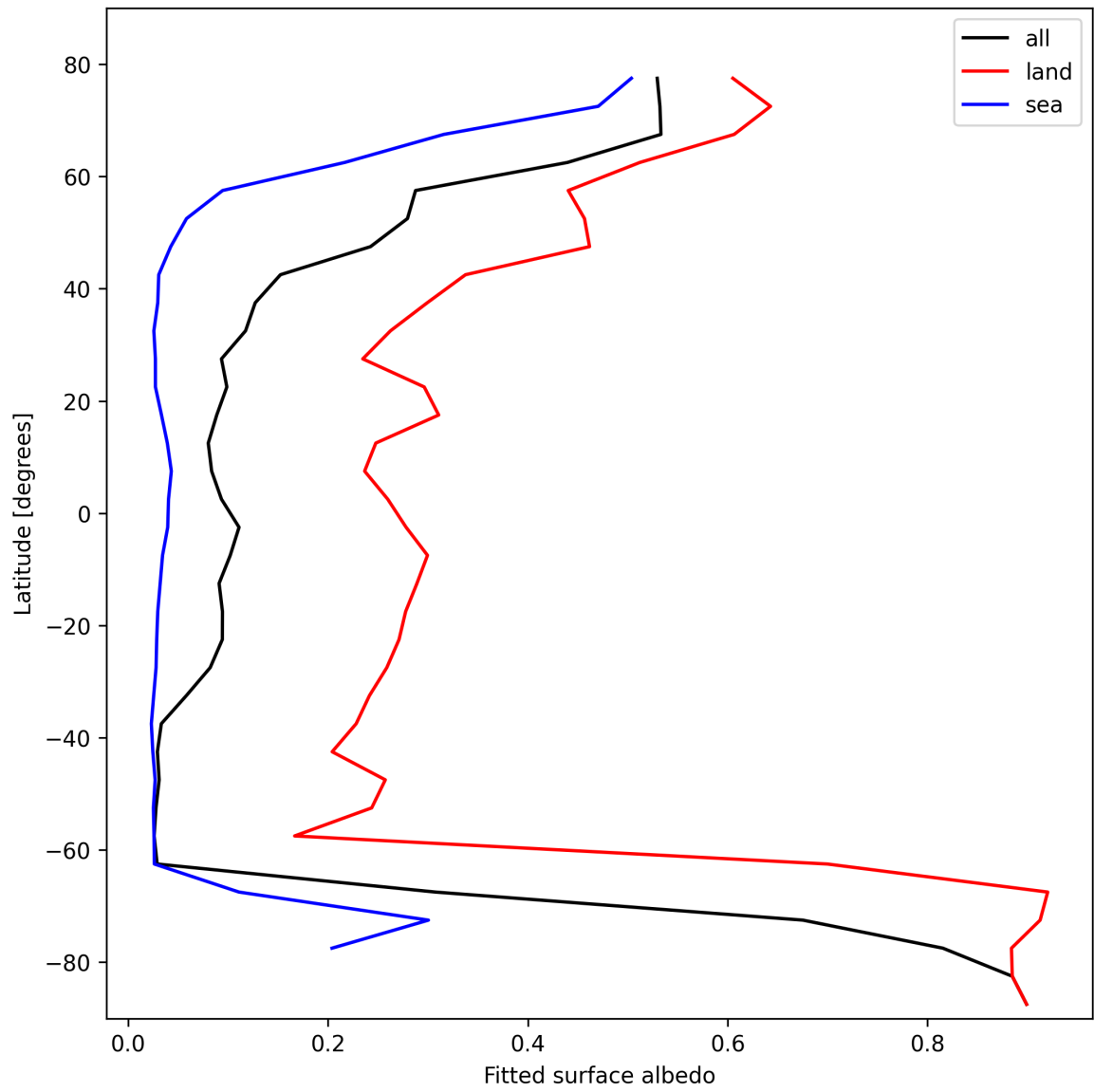
Figure 27: Zonal average of “Fitted surface albedo” for 2025-02-13 to 2025-02-14.
