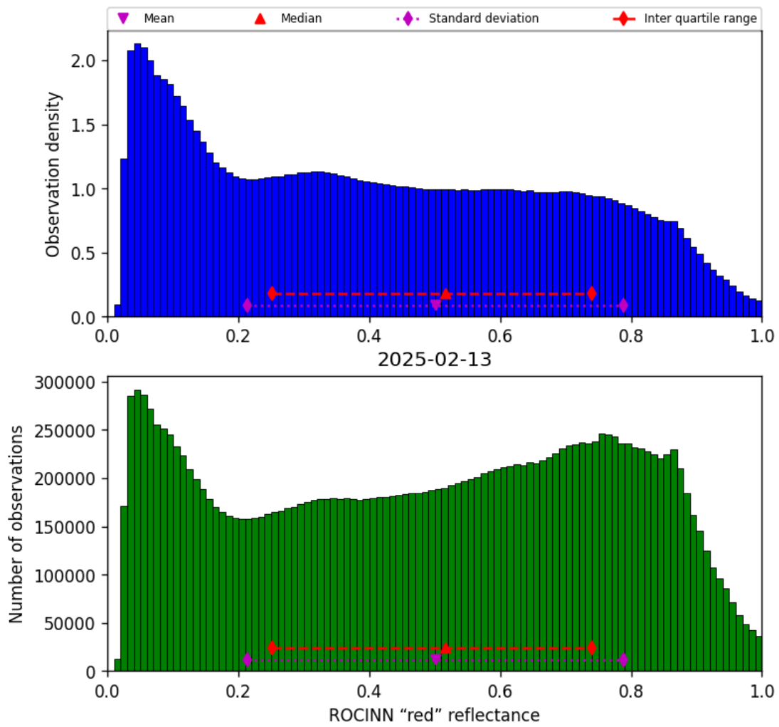
Figure 51: Histogram of “ROCINN “red” reflectance” for 2025-02-13 to 2025-02-14
