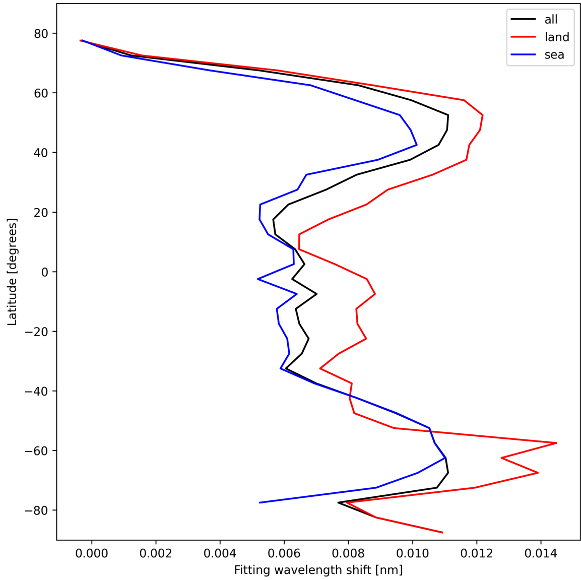
Figure 31: Zonal average of “Fitting wavelength shift” for 2025-02-13 to 2025-02-14.
