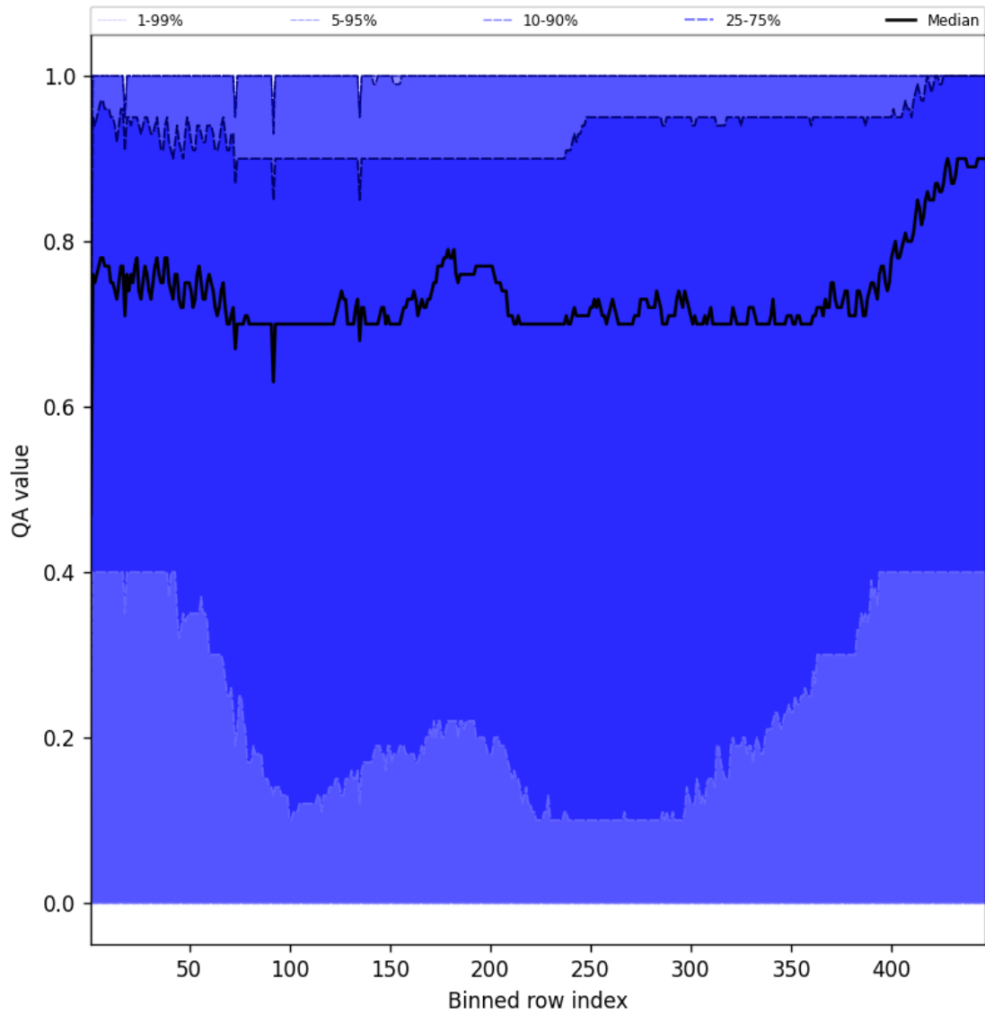
Figure 52: Along track statistics of “QA value” for 2025-02-13 to 2025-02-14
