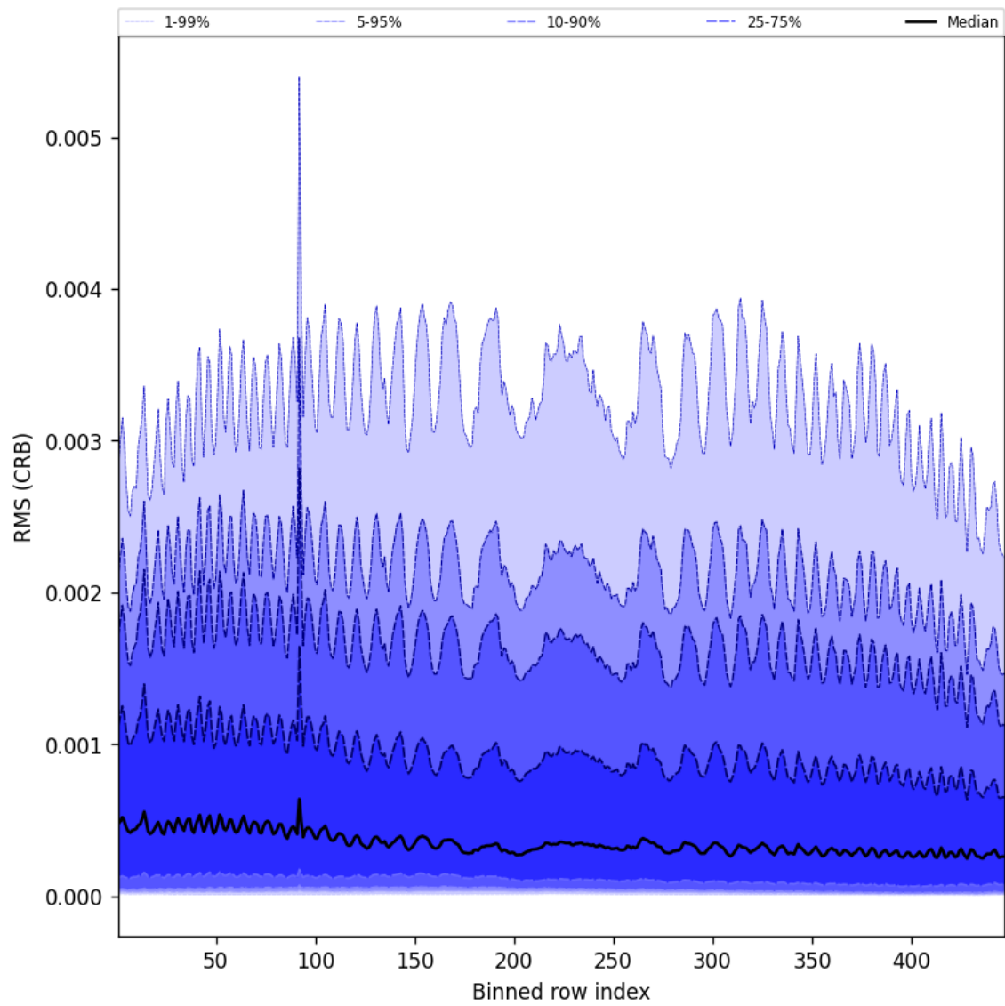
Figure 62: Along track statistics of “RMS (CRB)” for 2025-02-13 to 2025-02-14
