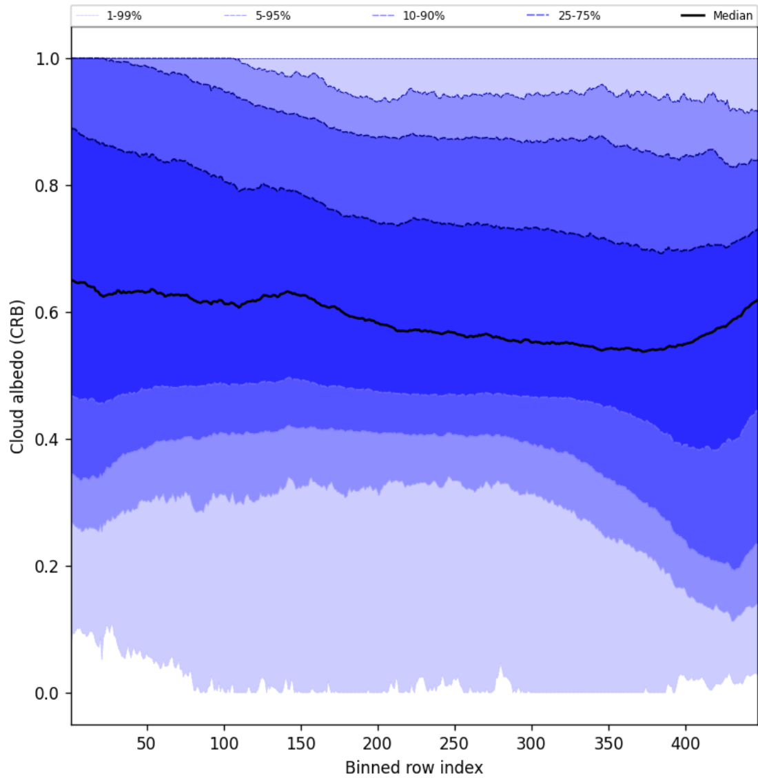
Figure 58: Along track statistics of “Cloud albedo (CRB)” for 2025-02-13 to 2025-02-14
