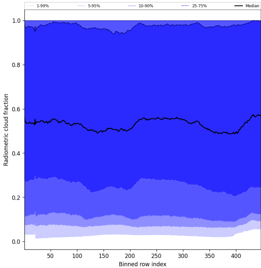
Figure 53: Along track statistics of “Radiometric cloud fraction” for 2025-02-13 to 2025-02-14
