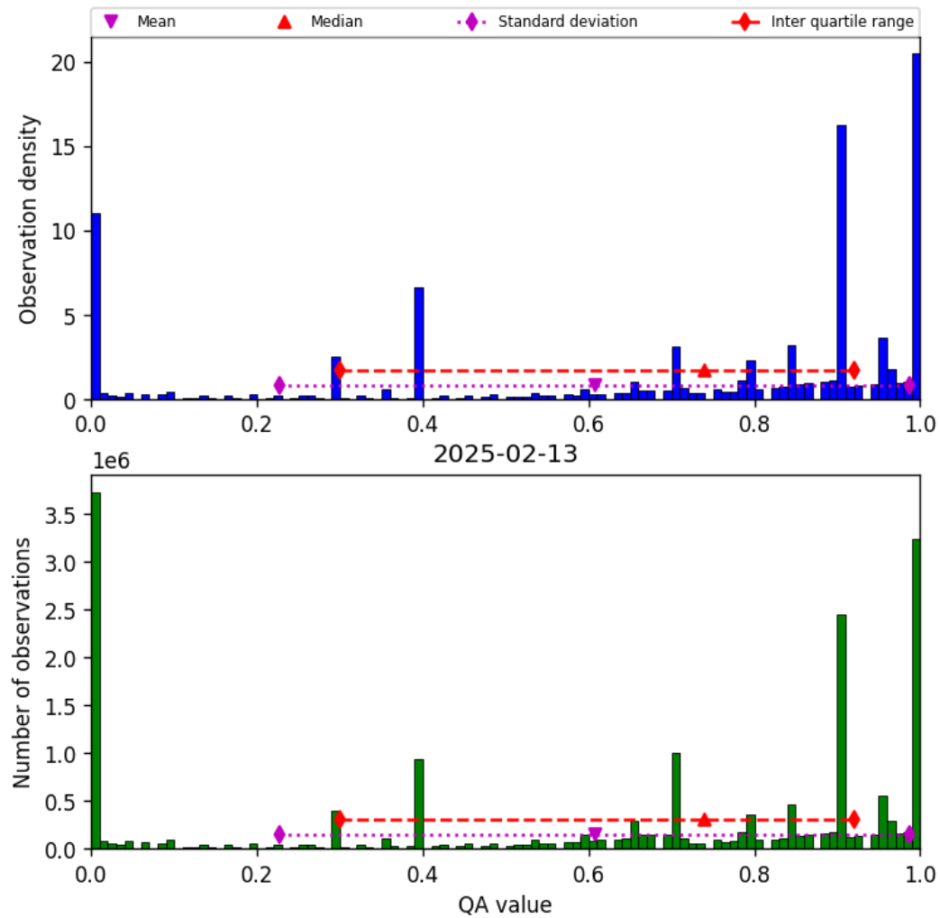
Figure 36: Histogram of “QA value” for 2025-02-13 to 2025-02-14
