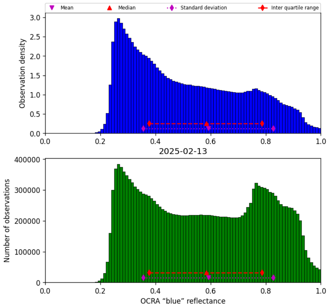
Figure 49: Histogram of “OCRA “blue” reflectance” for 2025-02-13 to 2025-02-14
