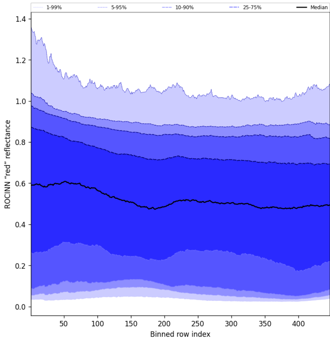
Figure 67: Along track statistics of “ROCINN “red” reflectance” for 2025-02-13 to 2025-02-14
