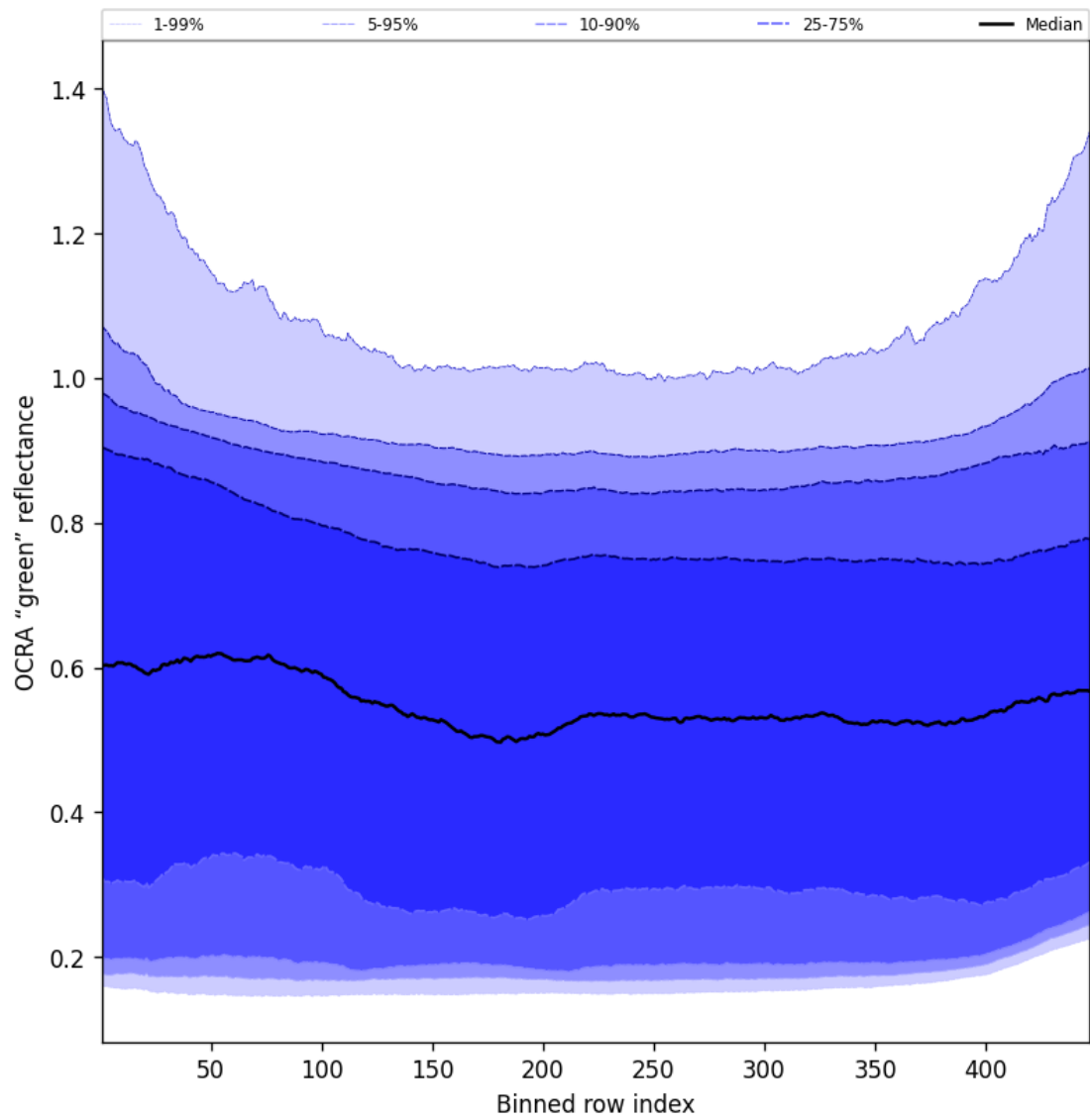
Figure 66: Along track statistics of "OCRA "green" reflectance" for 2025-02-13 to 2025-02-14
