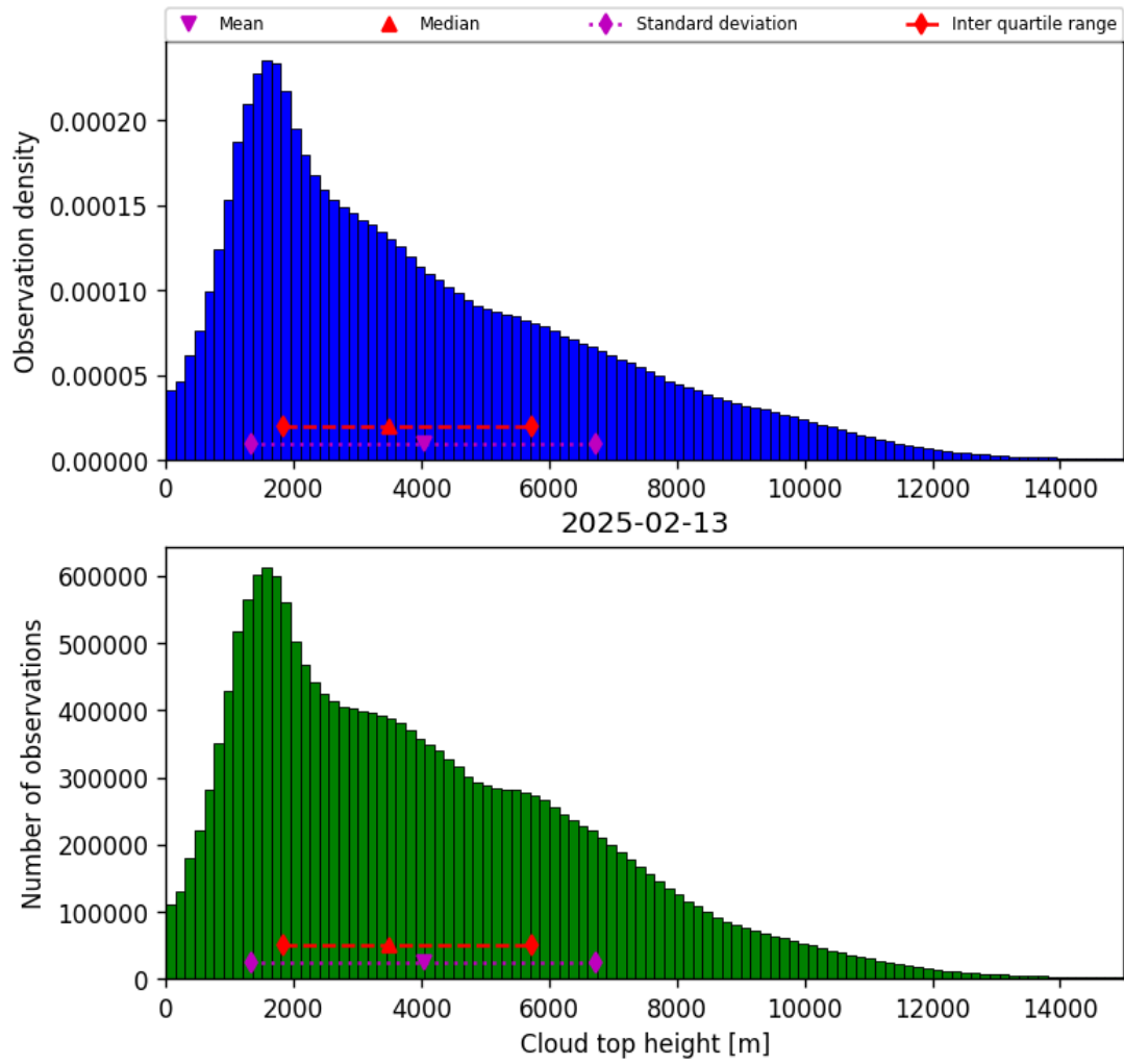
Figure 38: Histogram of “Cloud top height” for 2025-02-13 to 2025-02-14
