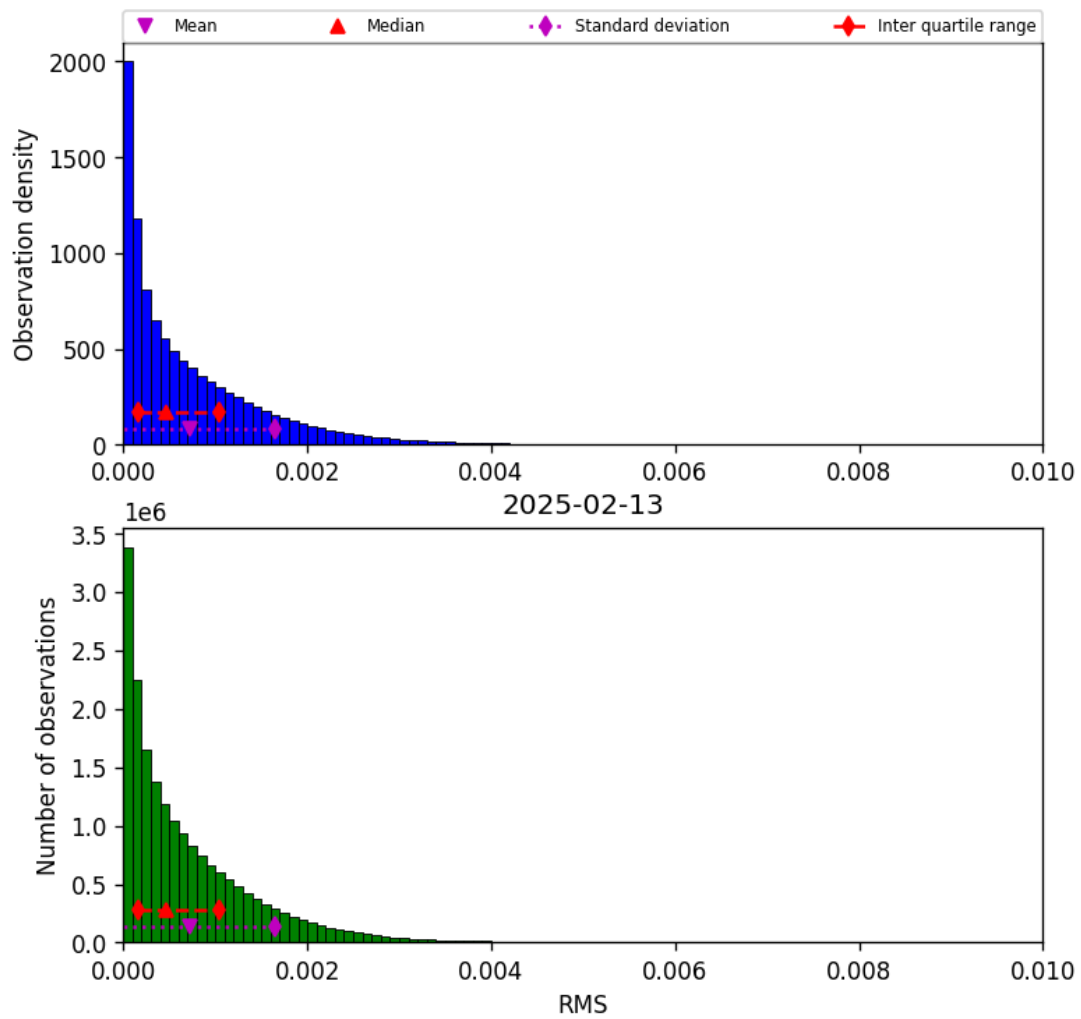
Figure 45: Histogram of “RMS” for 2025-02-13 to 2025-02-14
