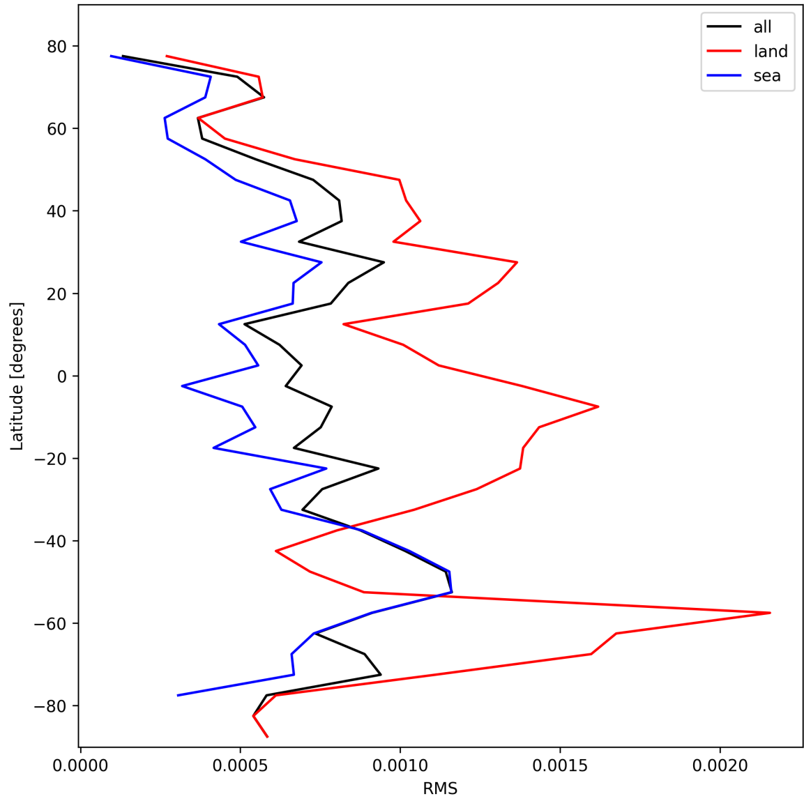
Figure 29: Zonal average of “RMS” for 2025-02-13 to 2025-02-14.
