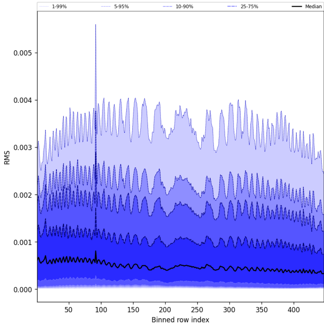
Figure 61: Along track statistics of “RMS” for 2025-02-13 to 2025-02-14
