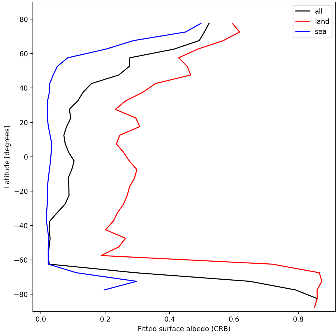
Figure 28: Zonal average of “Fitted surface albedo (CRB)” for 2025-02-13 to 2025-02-14.
