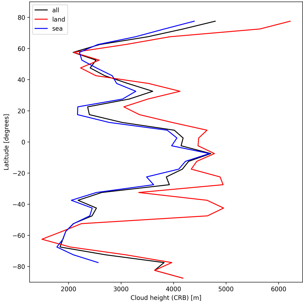
Figure 25: Zonal average of “Cloud height (CRB)” for 2025-02-13 to 2025-02-14.
