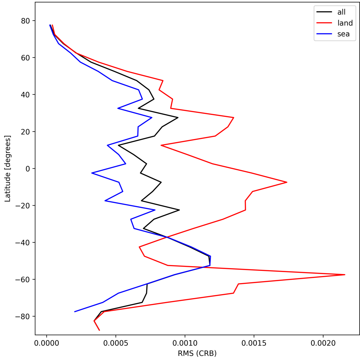
Figure 30: Zonal average of “RMS (CRB)” for 2025-02-13 to 2025-02-14.
