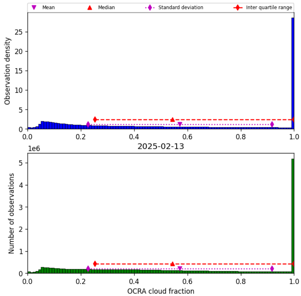
Figure 48: Histogram of “OCRA cloud fraction” for 2025-02-13 to 2025-02-14
