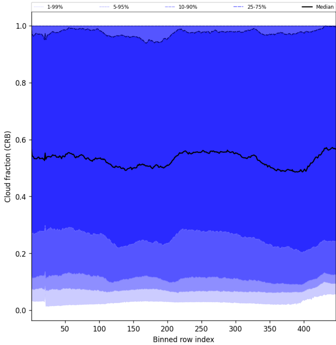
Figure 56: Along track statistics of “Cloud fraction (CRB)” for 2025-02-13 to 2025-02-14
