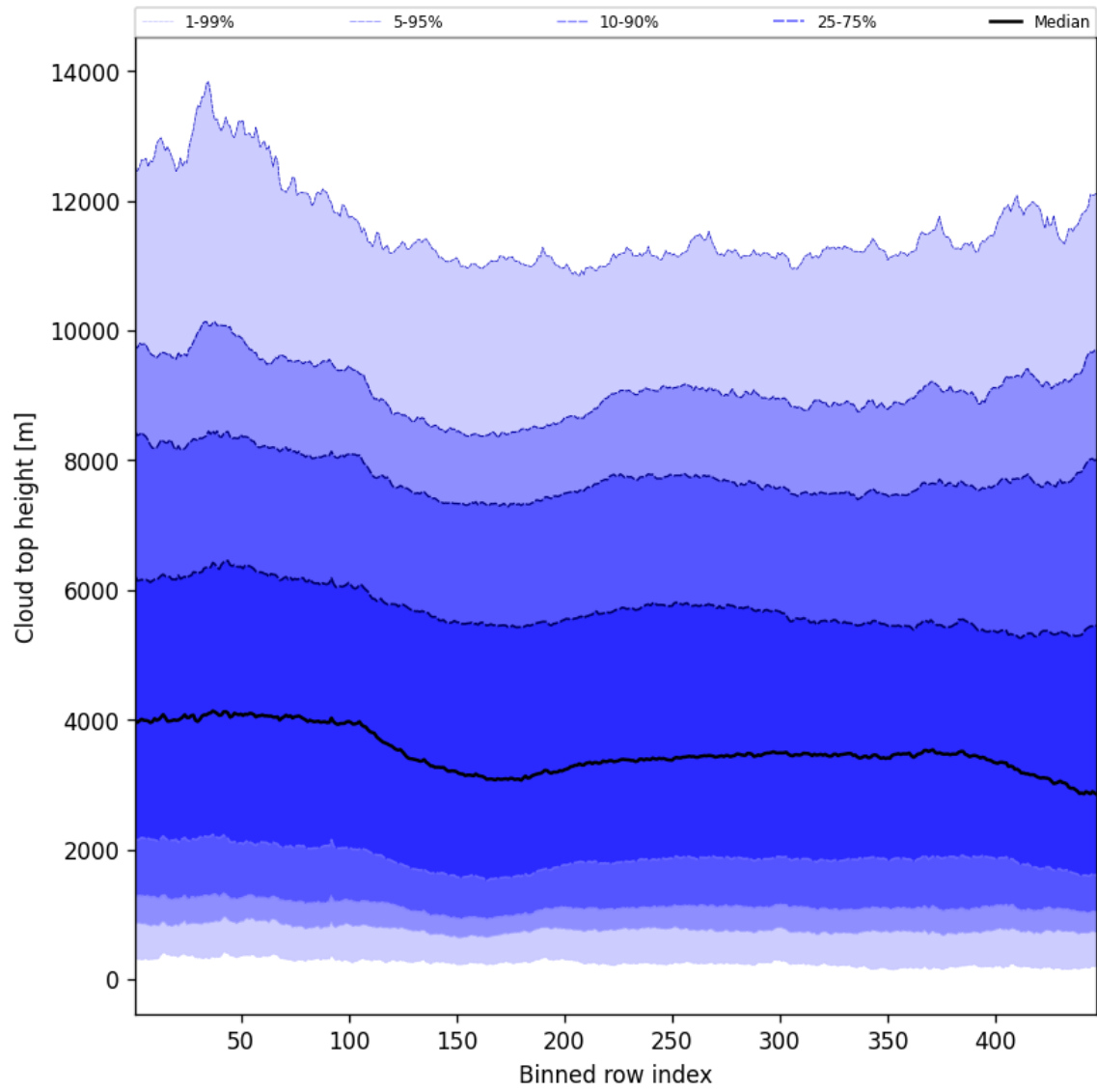
Figure 54: Along track statistics of “Cloud top height” for 2025-02-13 to 2025-02-14
