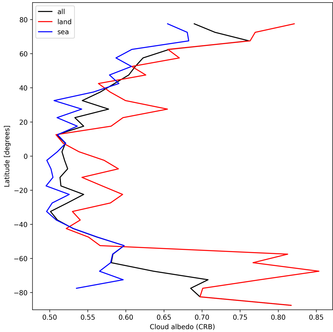
Figure 26: Zonal average of “Cloud albedo (CRB)” for 2025-02-13 to 2025-02-14.
