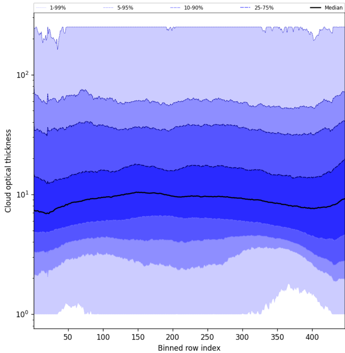
Figure 55: Along track statistics of “Cloud optical thickness” for 2025-02-13 to 2025-02-14
