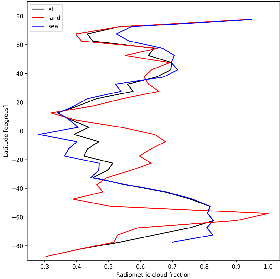
Figure 21: Zonal average of “Radiometric cloud fraction” for 2025-02-13 to 2025-02-14.
