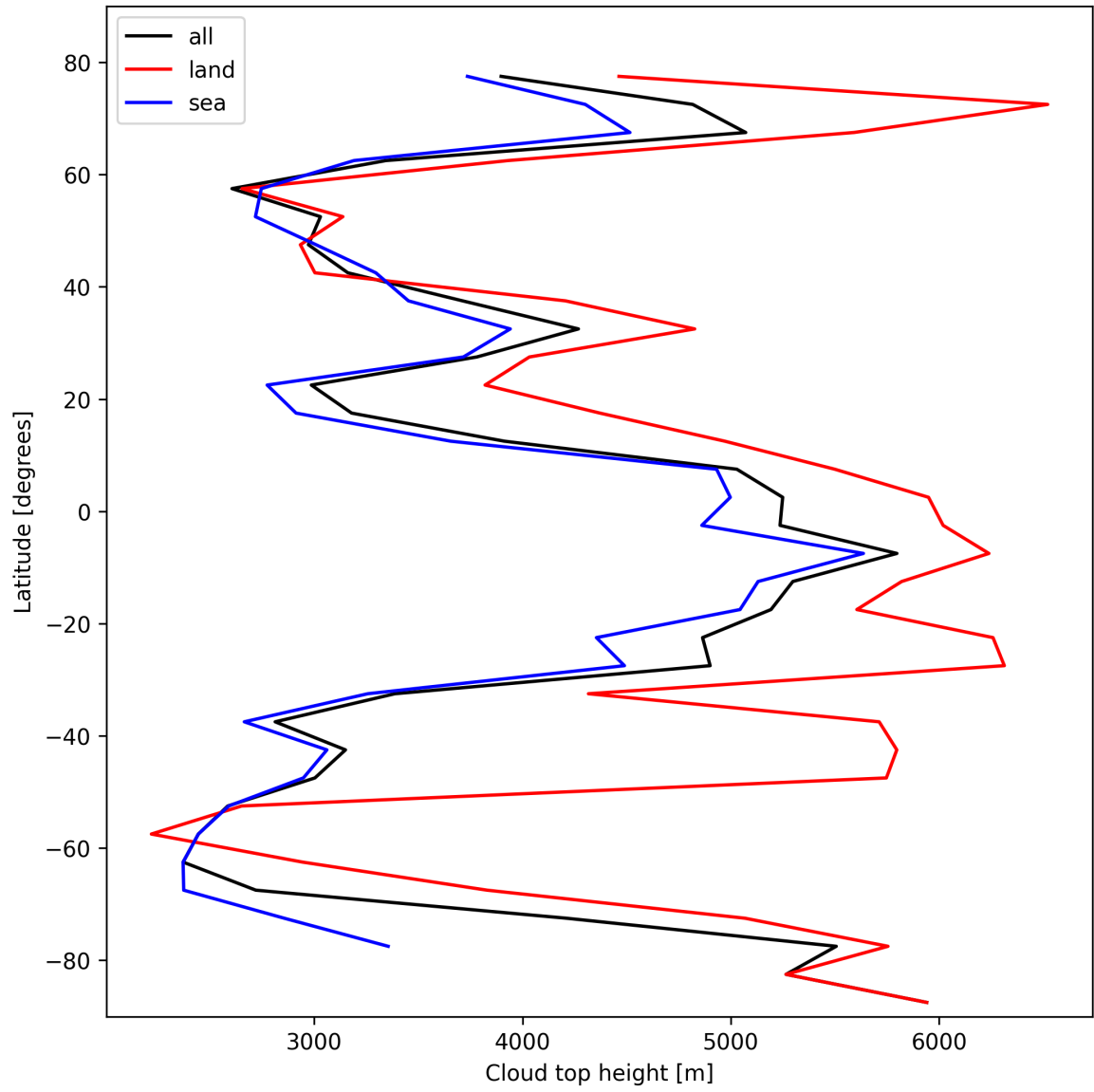
Figure 22: Zonal average of “Cloud top height” for 2025-02-13 to 2025-02-14.
