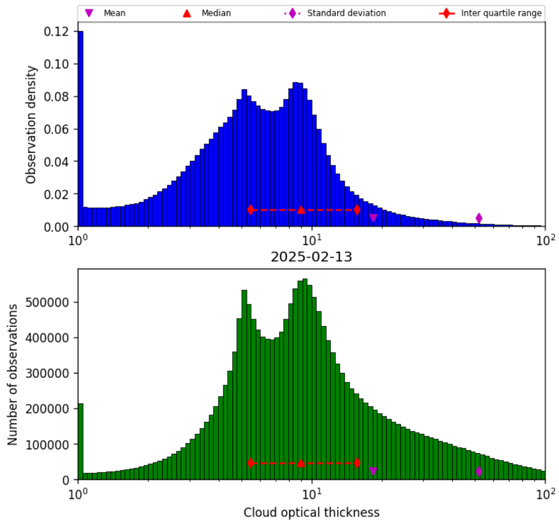
Figure 39: Histogram of “Cloud optical thickness” for 2025-02-13 to 2025-02-14
