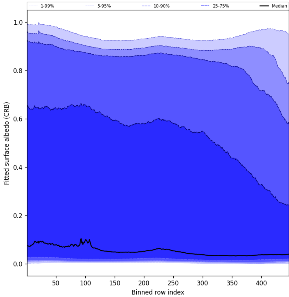
Figure 60: Along track statistics of “Fitted surface albedo (CRB)” for 2025-02-13 to 2025-02-14
