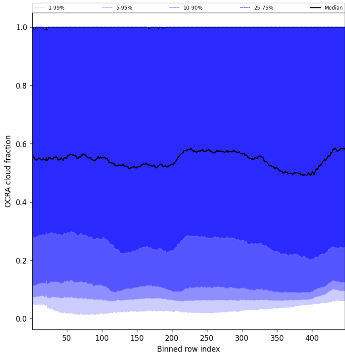
Figure 64: Along track statistics of “OCRA cloud fraction” for 2025-02-13 to 2025-02-14
