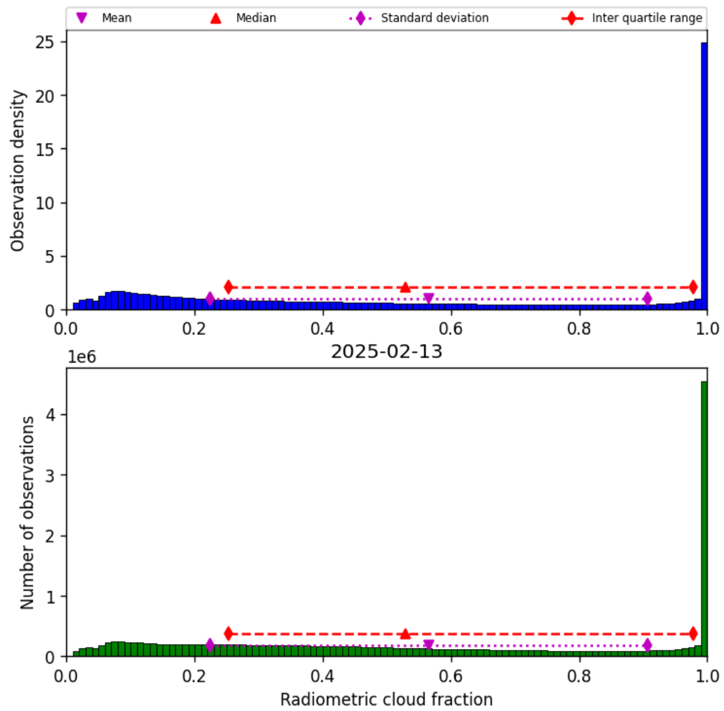
Figure 37: Histogram of “Radiometric cloud fraction” for 2025-02-13 to 2025-02-14
