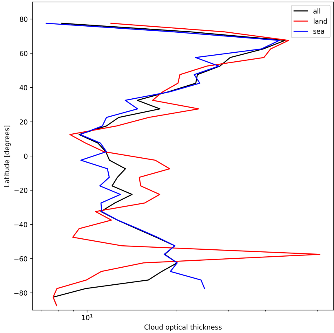
Figure 23: Zonal average of “Cloud optical thickness” for 2025-02-13 to 2025-02-14.
