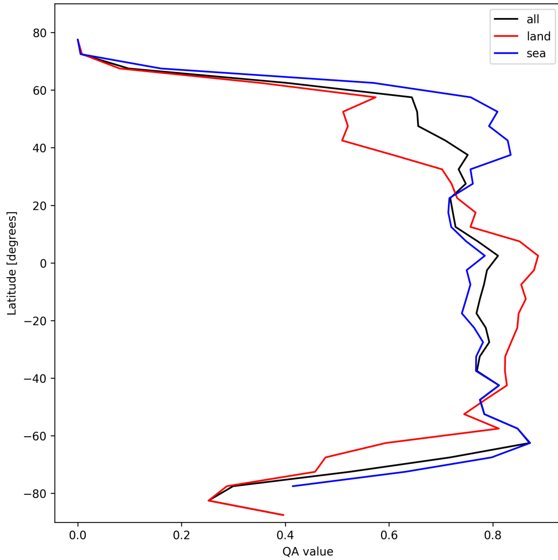
Figure 20: Zonal average of “QA value” for 2025-02-13 to 2025-02-14.
