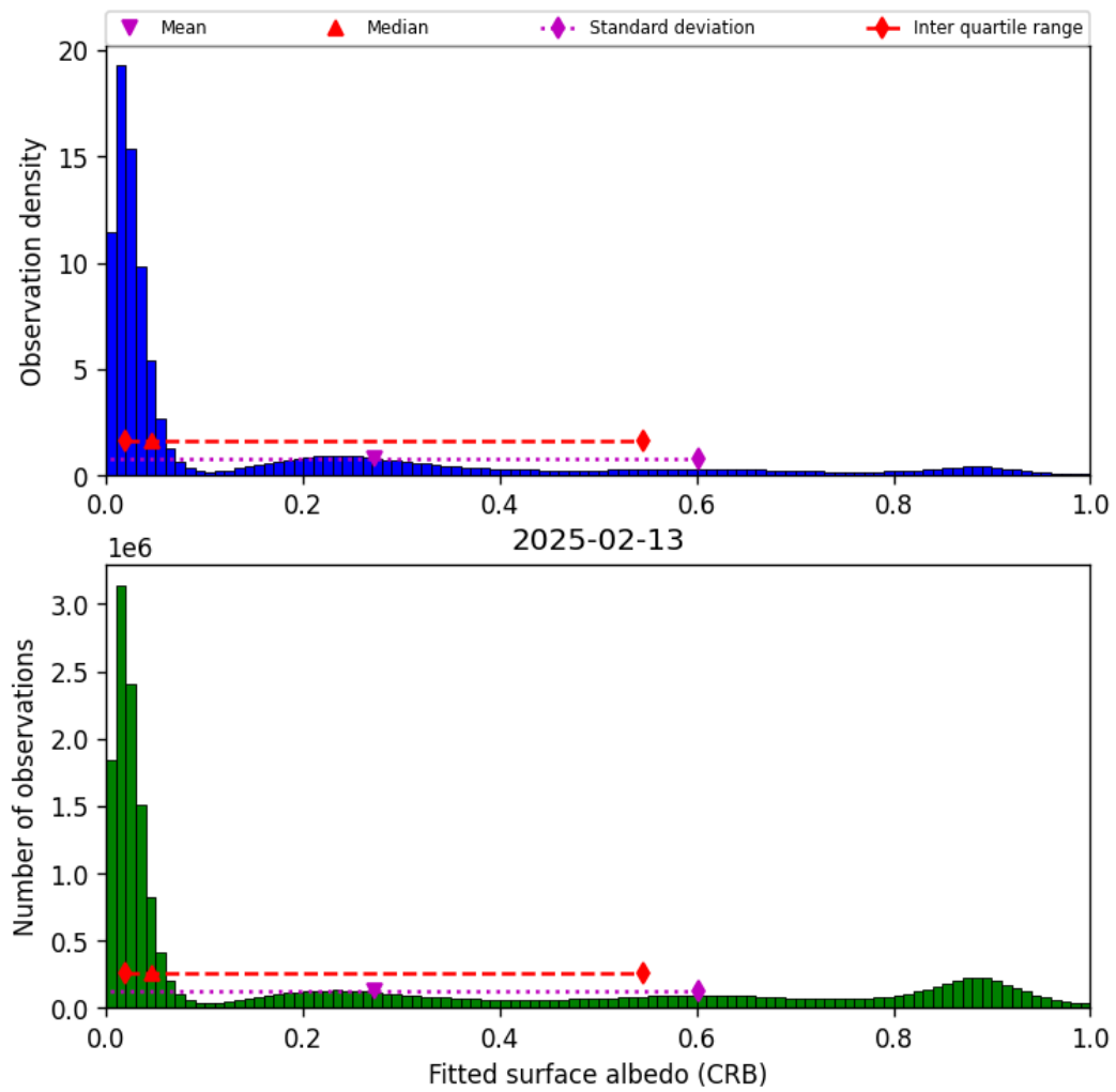
Figure 44: Histogram of “Fitted surface albedo (CRB)” for 2025-02-13 to 2025-02-14
