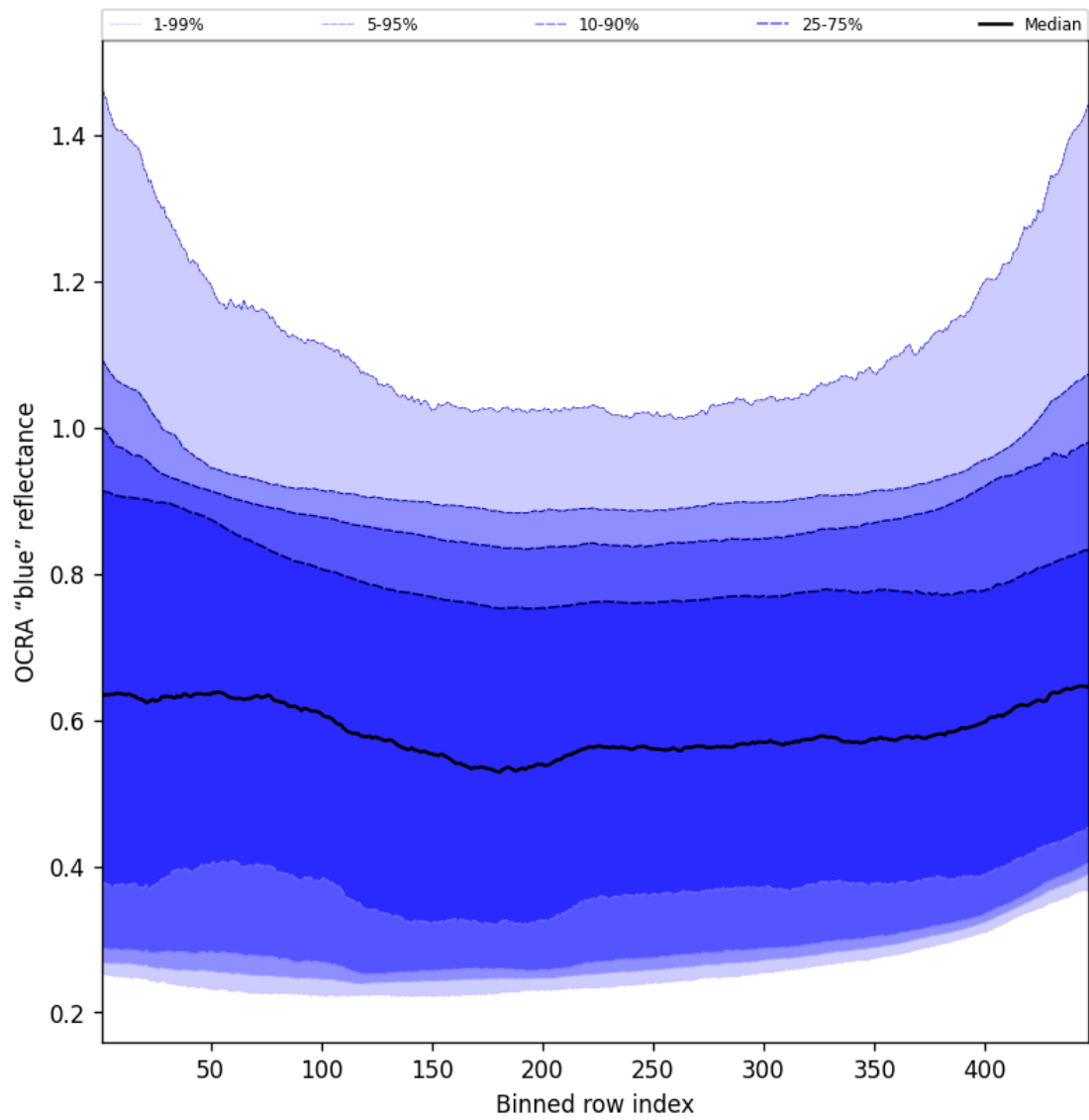
Figure 65: Along track statistics of "OCRA "blue" reflectance" for 2025-02-13 to 2025-02-14
