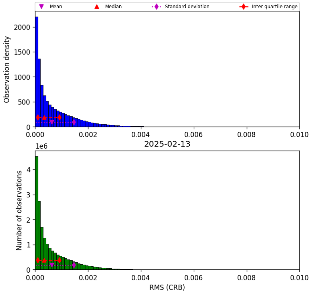
Figure 46: Histogram of “RMS (CRB)” for 2025-02-13 to 2025-02-14
