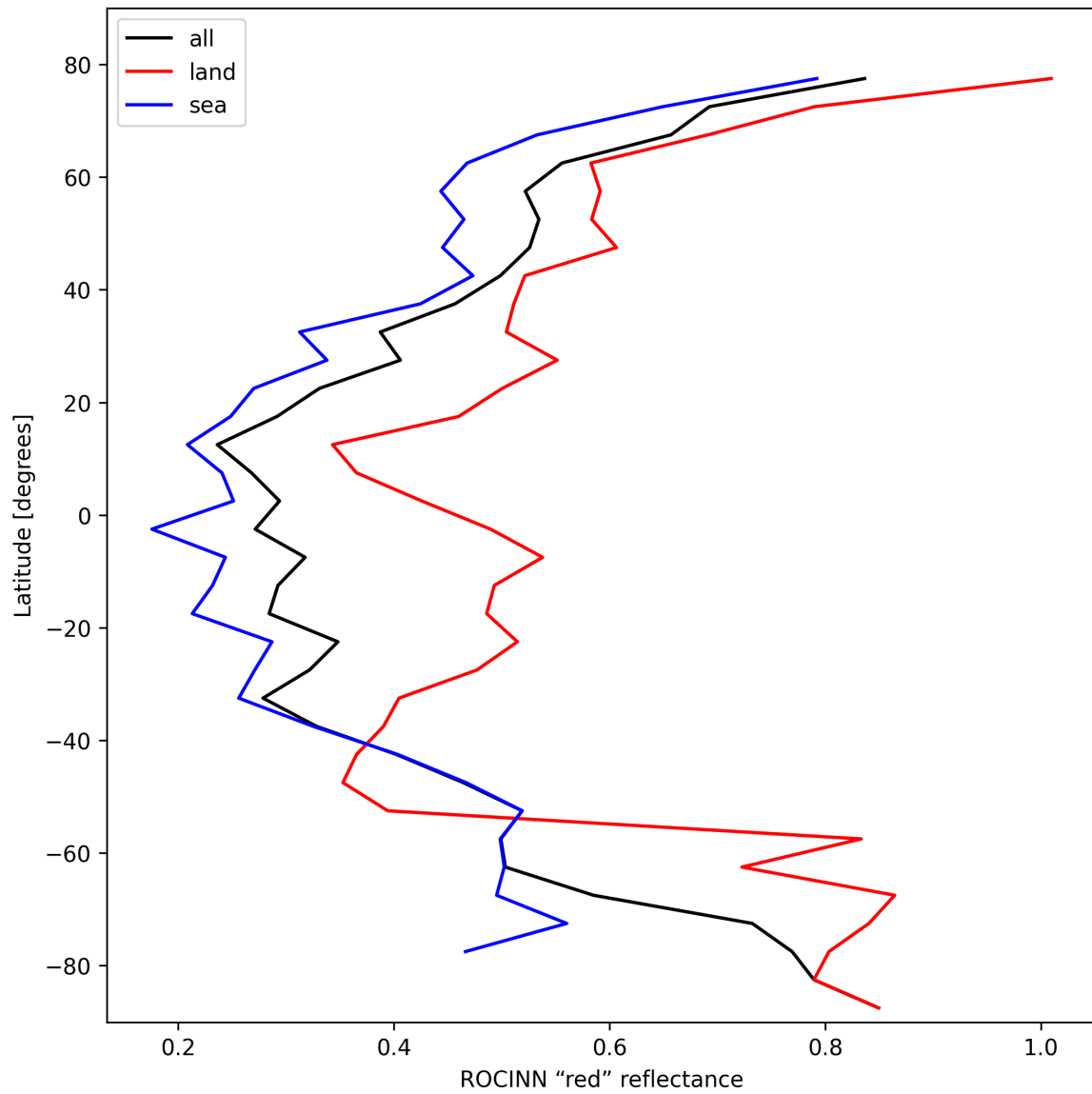
Figure 35: Zonal average of “ROCINN “red” reflectance” for 2025-02-13 to 2025-02-14.
