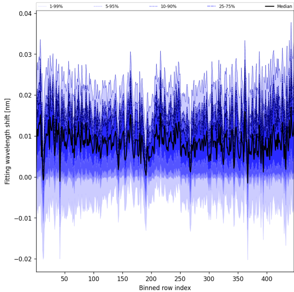
Figure 63: Along track statistics of “Fitting wavelength shift” for 2025-02-13 to 2025-02-14
