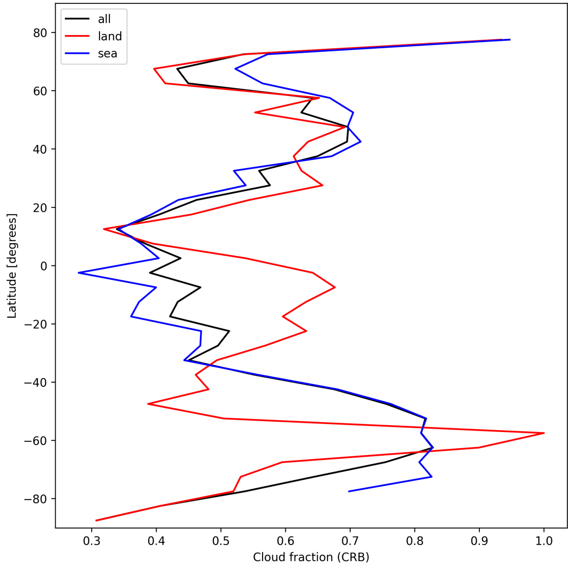
Figure 24: Zonal average of “Cloud fraction (CRB)” for 2025-02-13 to 2025-02-14.
