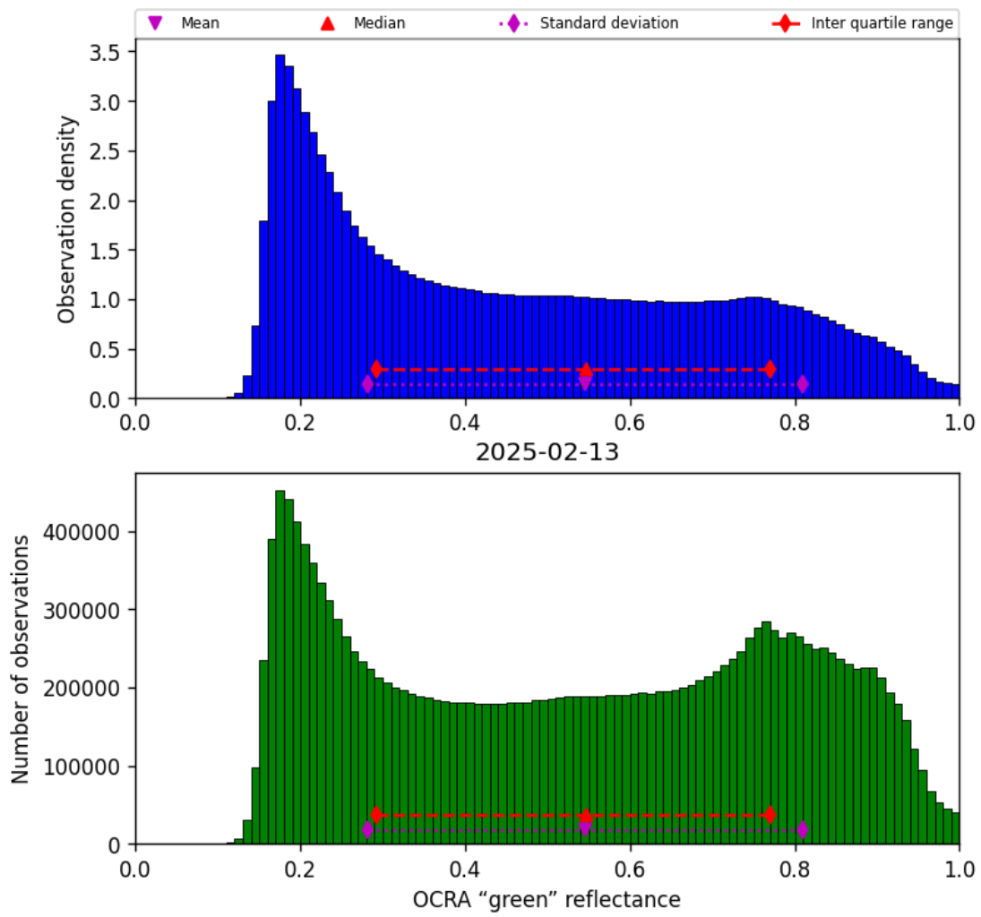
Figure 50: Histogram of “OCRA “green” reflectance” for 2025-02-13 to 2025-02-14
