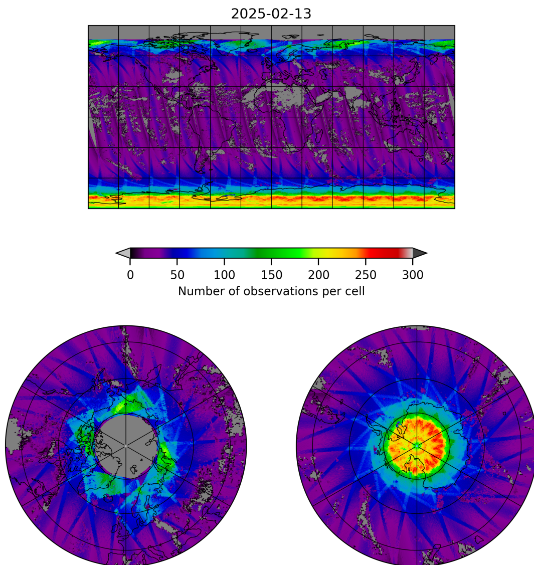
Figure 19: Map of the number of observations for 2025-02-13 to 2025-02-14
