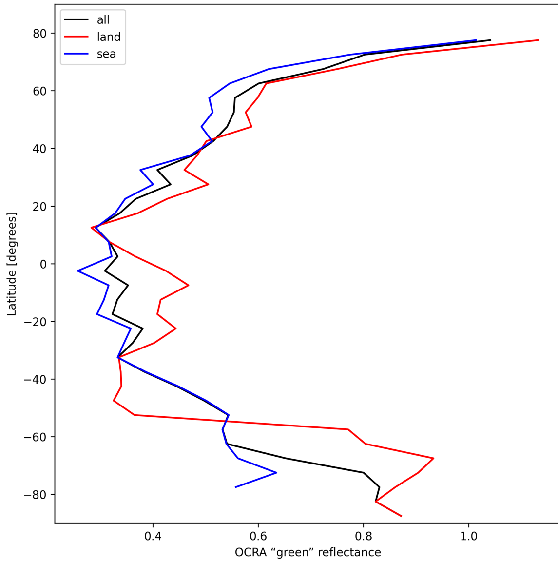
Figure 34: Zonal average of “OCRA “green” reflectance” for 2025-02-13 to 2025-02-14.
