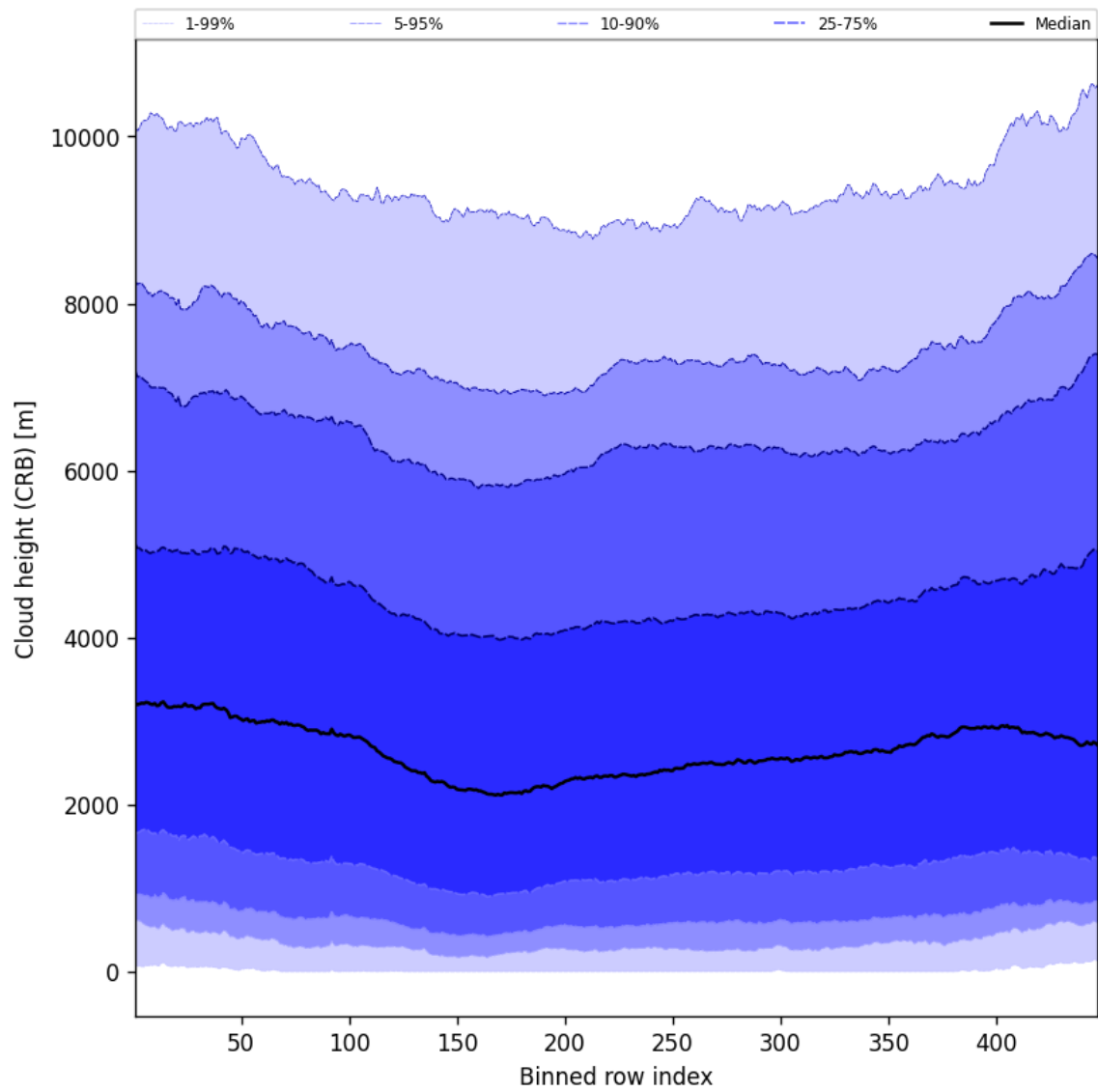
Figure 57: Along track statistics of “Cloud height (CRB)” for 2025-02-13 to 2025-02-14
