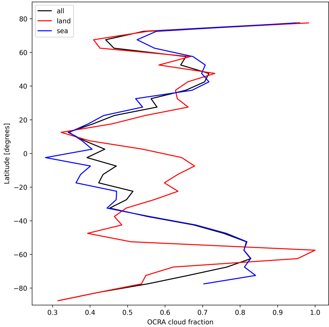
Figure 32: Zonal average of “OCRA cloud fraction” for 2025-02-13 to 2025-02-14.
