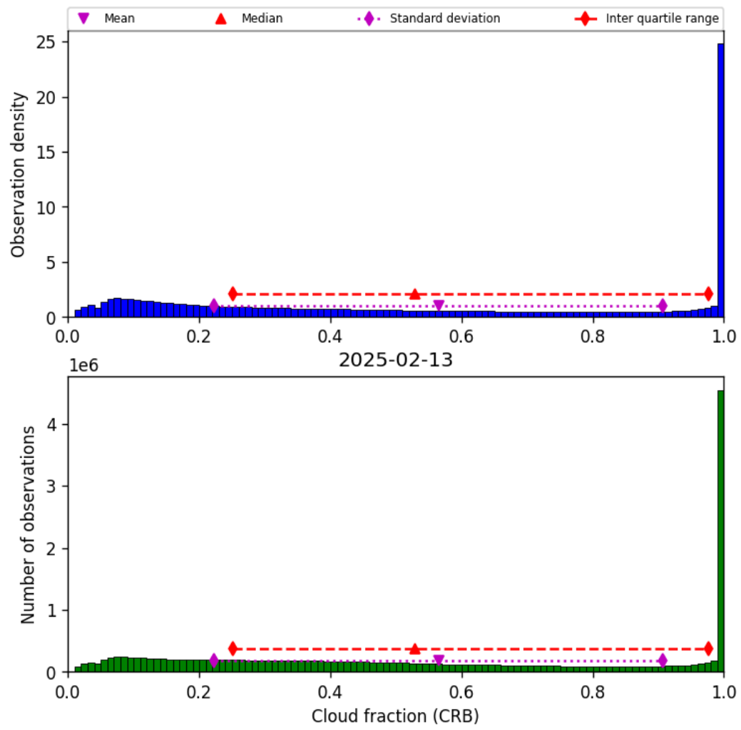
Figure 40: Histogram of “Cloud fraction (CRB)” for 2025-02-13 to 2025-02-14
