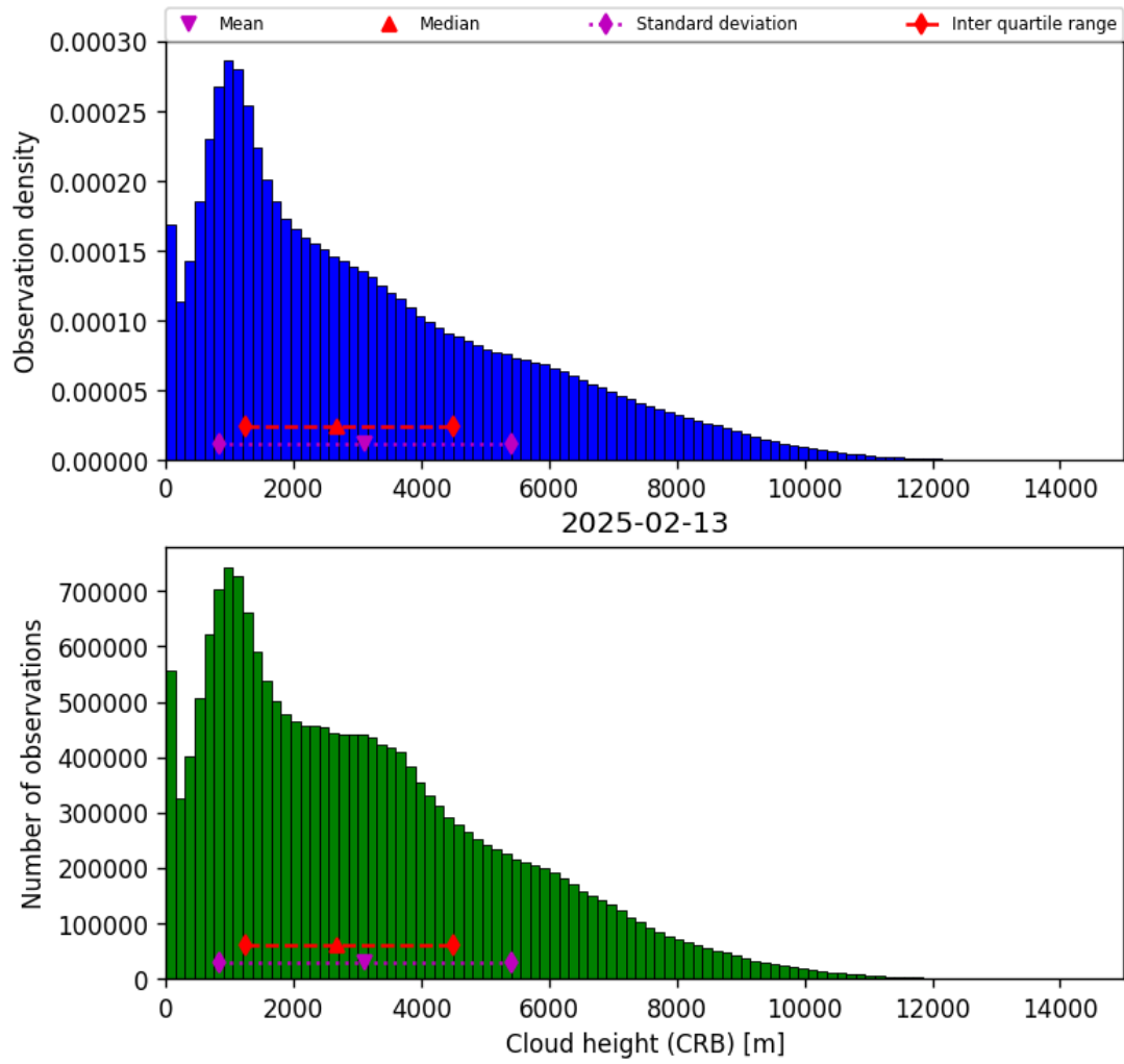
Figure 41: Histogram of “Cloud height (CRB)” for 2025-02-13 to 2025-02-14
