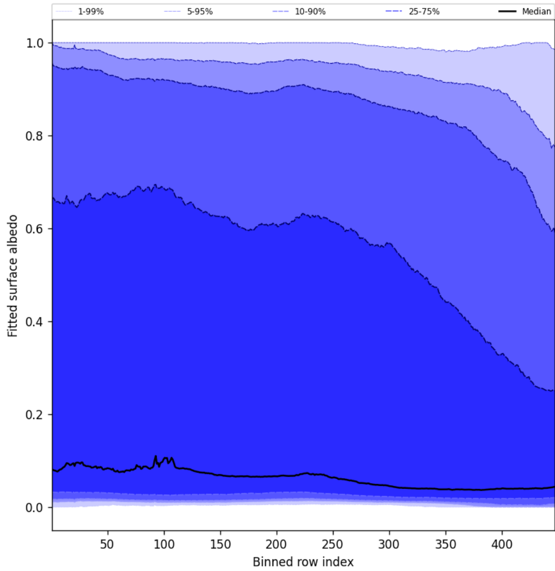
Figure 59: Along track statistics of “Fitted surface albedo” for 2025-02-13 to 2025-02-14
