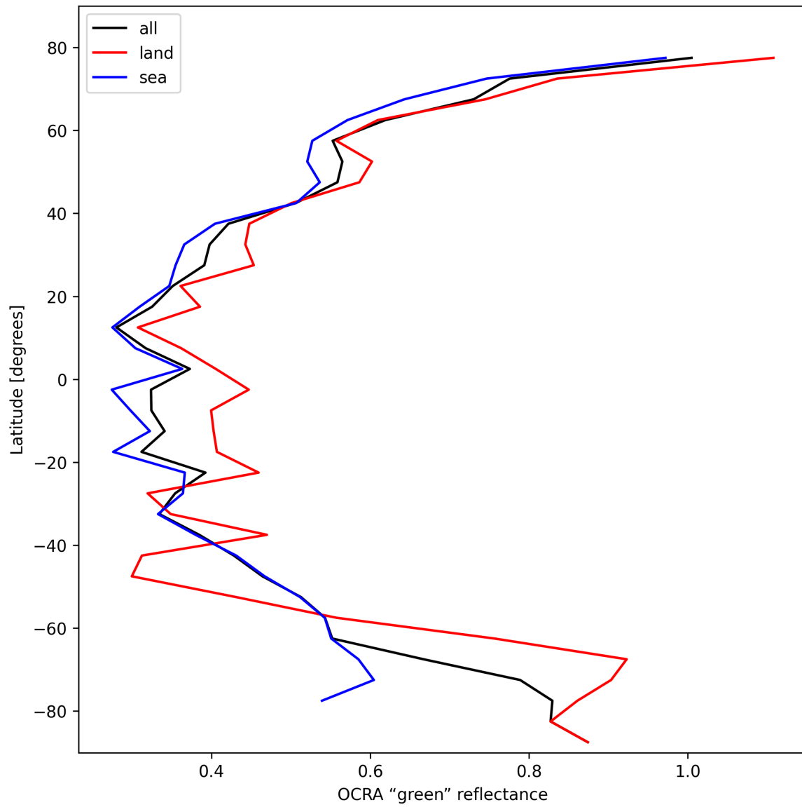
Figure 34: Zonal average of “OCRA “green” reflectance” for 2025-02-14 to 2025-02-15.
