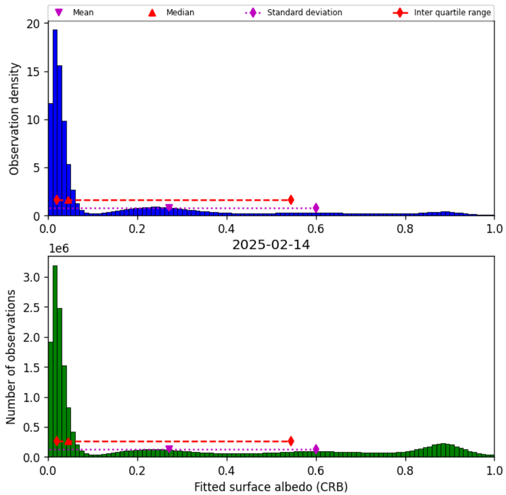
Figure 44: Histogram of “Fitted surface albedo (CRB)” for 2025-02-14 to 2025-02-15
