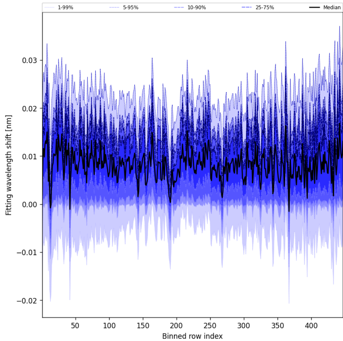
Figure 63: Along track statistics of “Fitting wavelength shift” for 2025-02-14 to 2025-02-15
