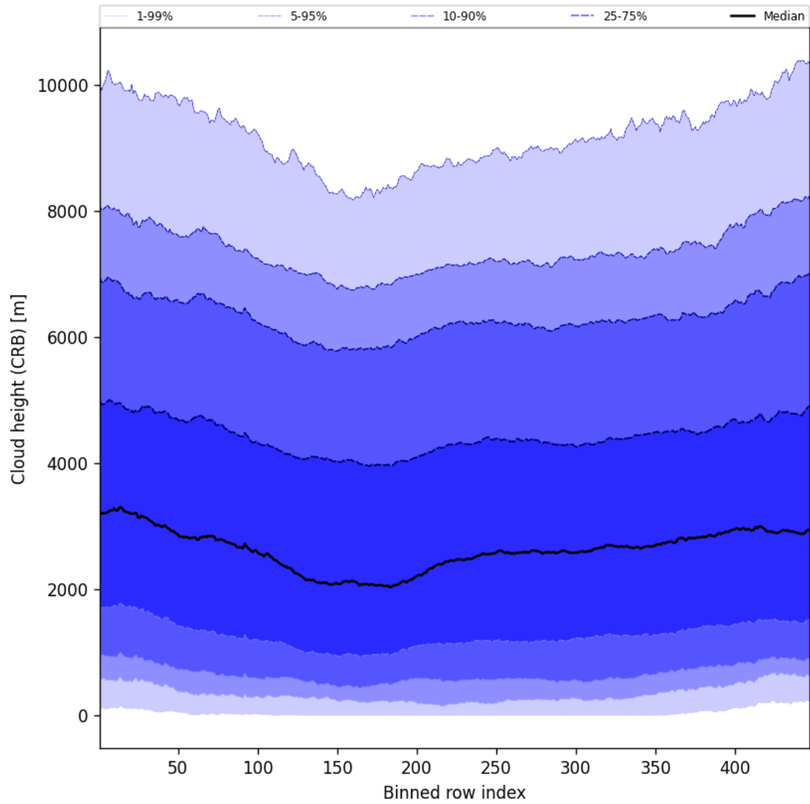
Figure 57: Along track statistics of “Cloud height (CRB)” for 2025-02-14 to 2025-02-15
