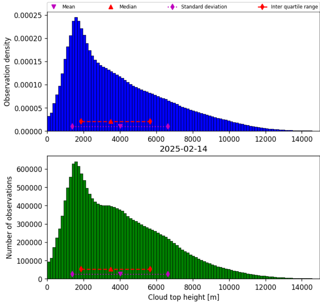
Figure 38: Histogram of “Cloud top height” for 2025-02-14 to 2025-02-15
