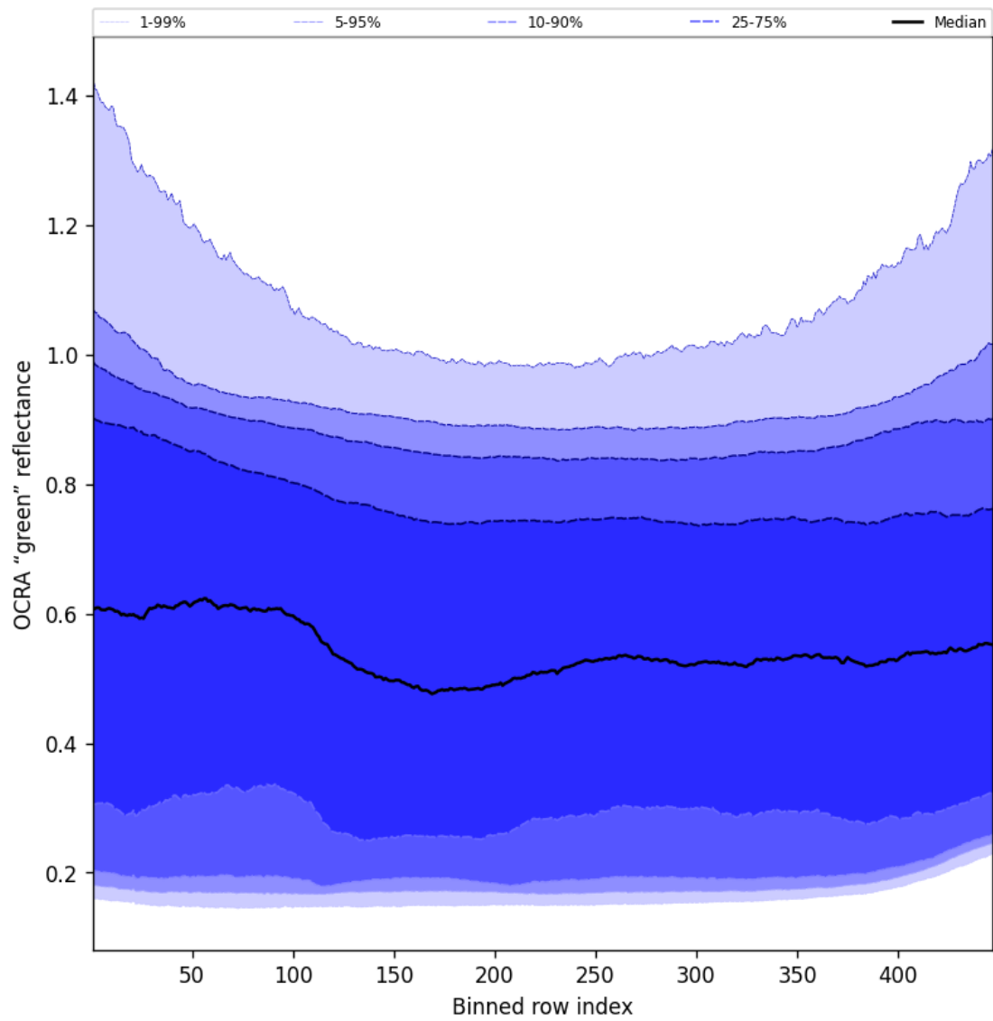
Figure 66: Along track statistics of “OCRA “green” reflectance” for 2025-02-14 to 2025-02-15
