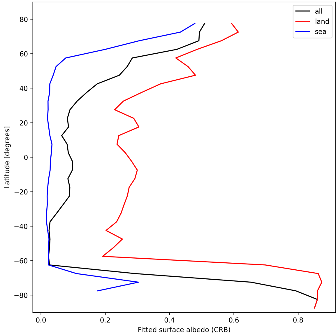
Figure 28: Zonal average of “Fitted surface albedo (CRB)” for 2025-02-14 to 2025-02-15.
