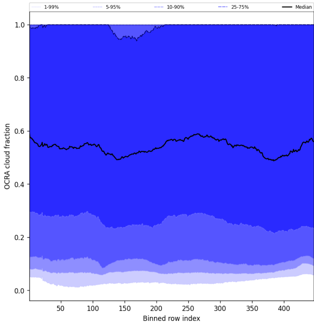
Figure 64: Along track statistics of “OCRA cloud fraction” for 2025-02-14 to 2025-02-15
