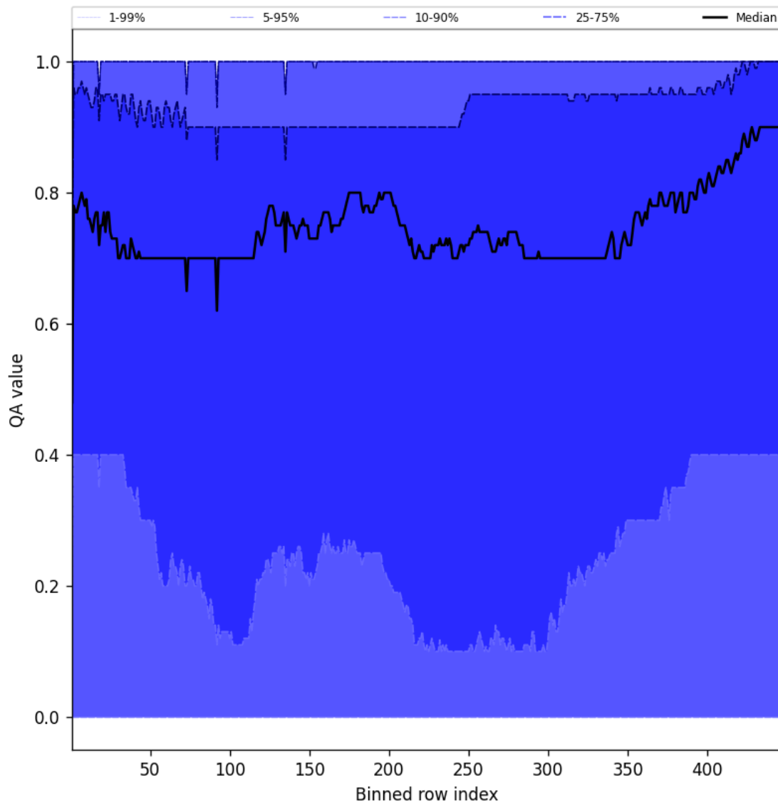
Figure 52: Along track statistics of “QA value” for 2025-02-14 to 2025-02-15
