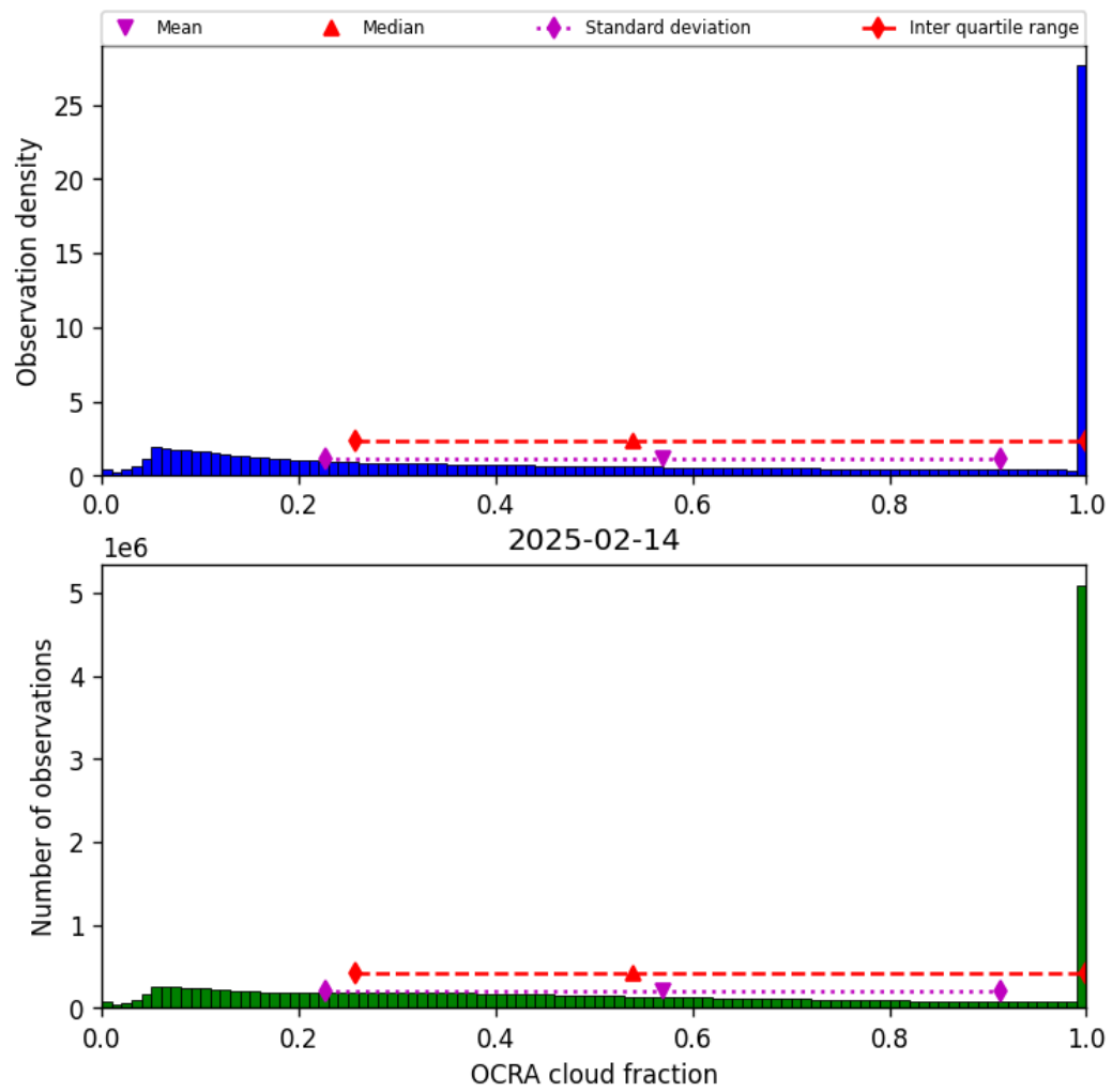
Figure 48: Histogram of “OCRA cloud fraction” for 2025-02-14 to 2025-02-15
