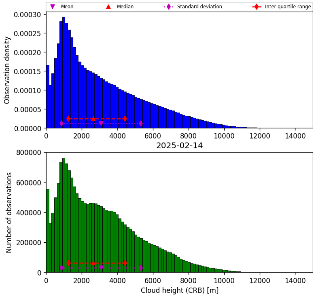
Figure 41: Histogram of “Cloud height (CRB)” for 2025-02-14 to 2025-02-15
