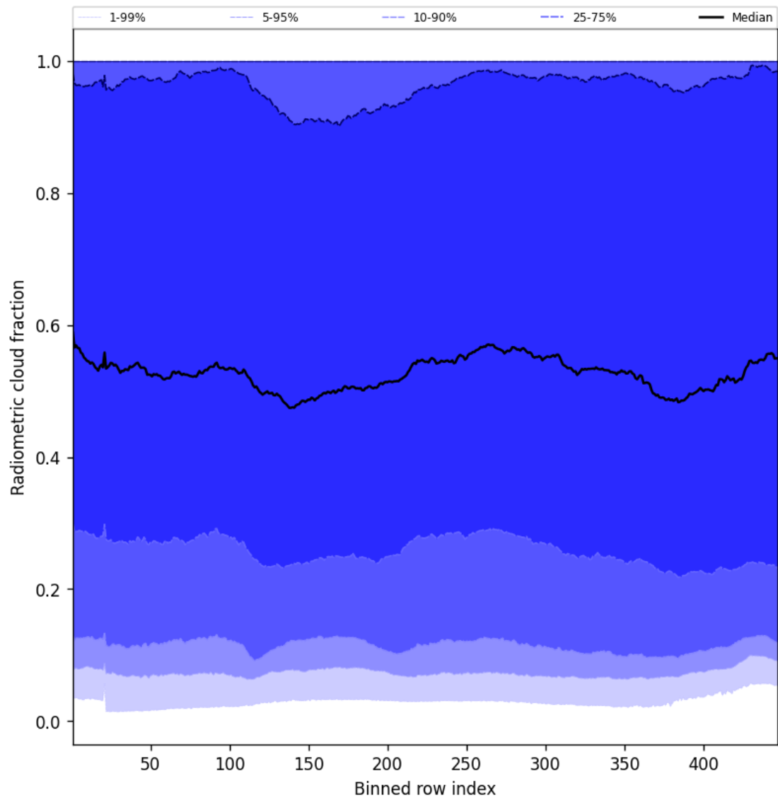
Figure 53: Along track statistics of “Radiometric cloud fraction” for 2025-02-14 to 2025-02-15
