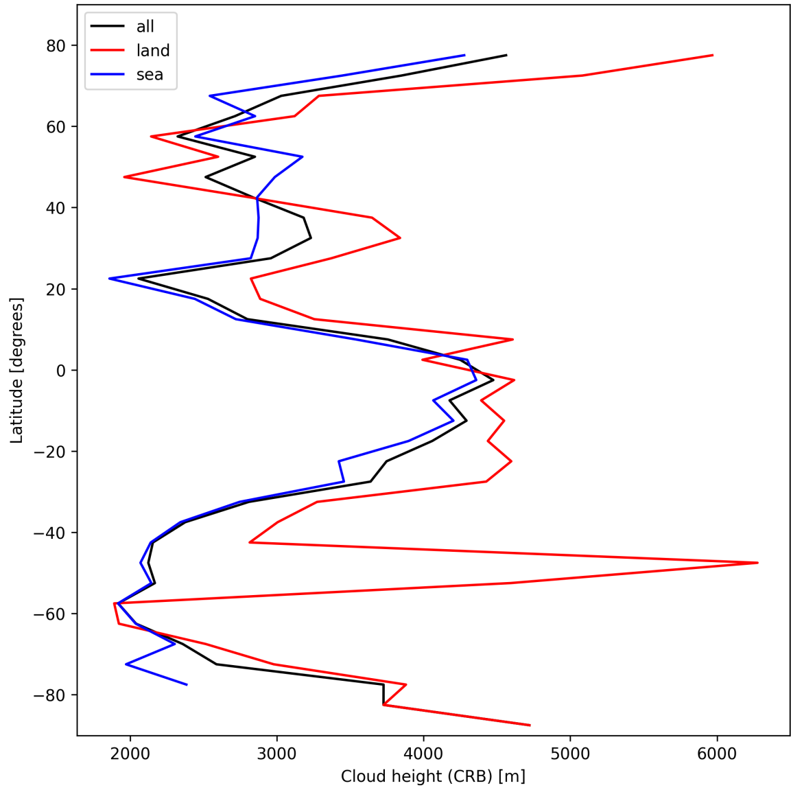
Figure 25: Zonal average of “Cloud height (CRB)” for 2025-02-14 to 2025-02-15.
