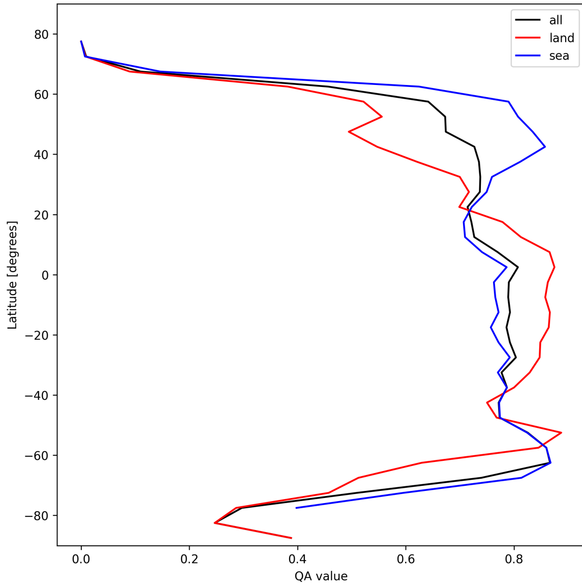
Figure 20: Zonal average of “QA value” for 2025-02-14 to 2025-02-15.
