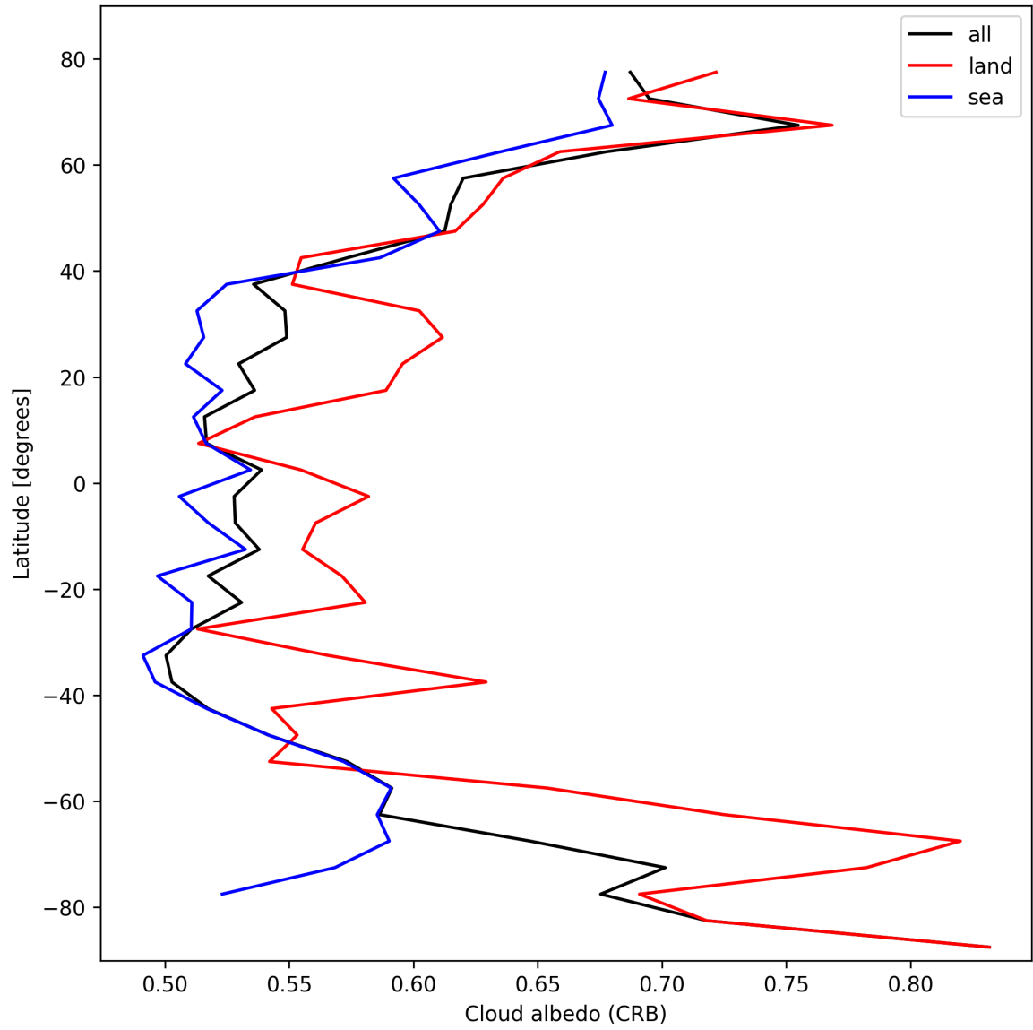
Figure 26: Zonal average of “Cloud albedo (CRB)” for 2025-02-14 to 2025-02-15.
