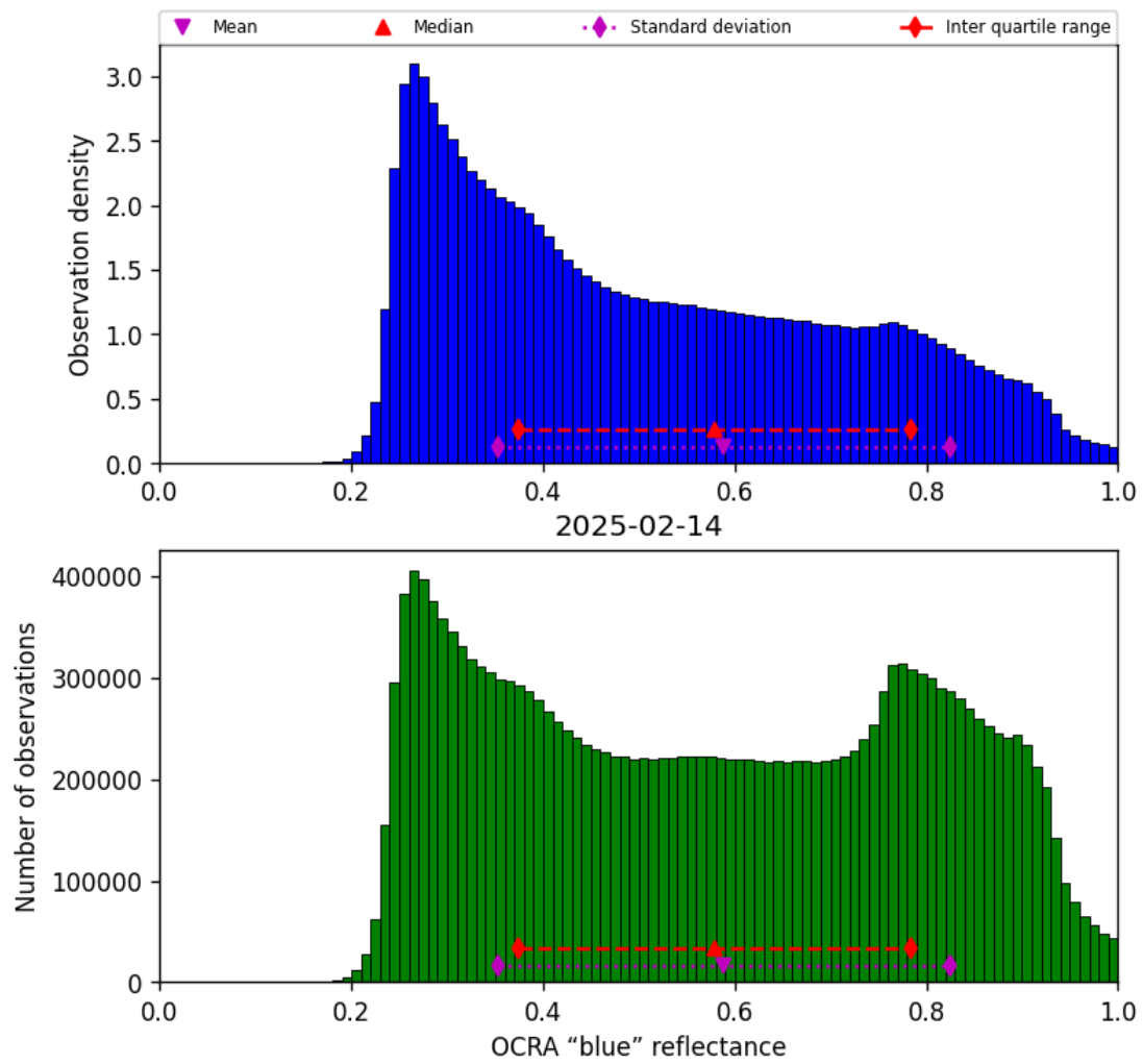
Figure 49: Histogram of “OCRA “blue” reflectance” for 2025-02-14 to 2025-02-15
