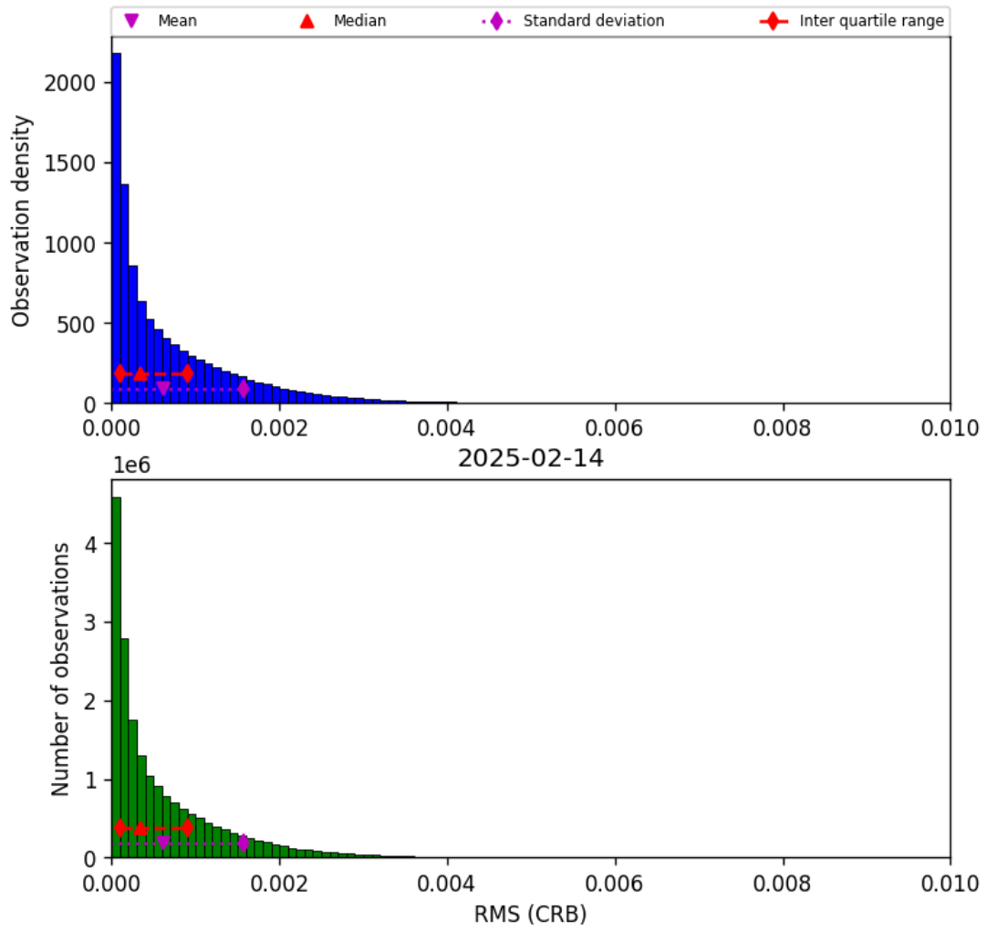
Figure 46: Histogram of “RMS (CRB)” for 2025-02-14 to 2025-02-15
