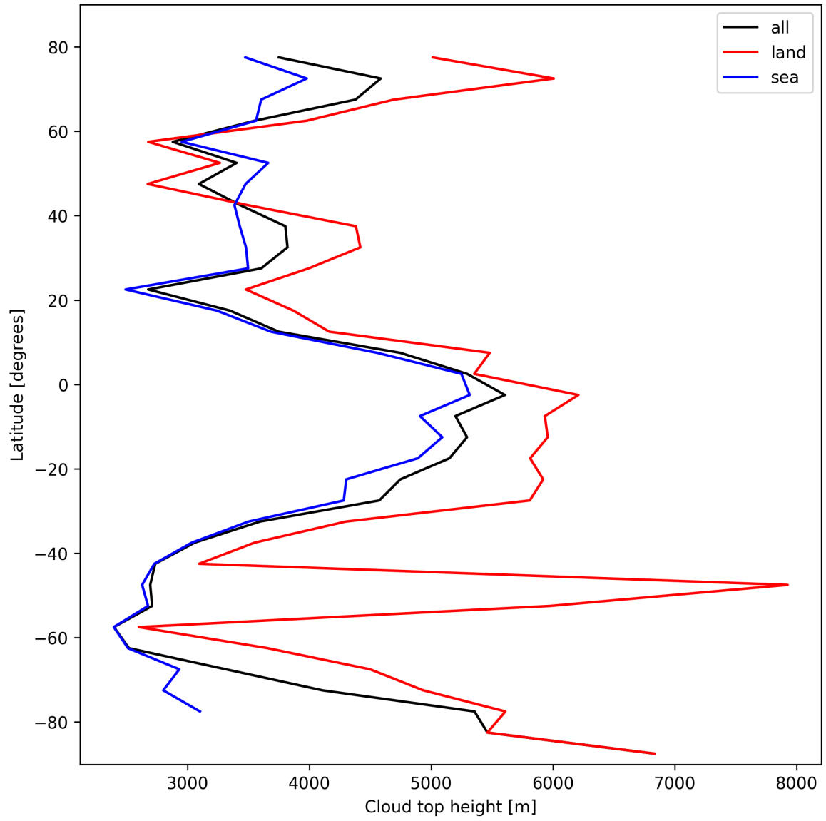
Figure 22: Zonal average of “Cloud top height” for 2025-02-14 to 2025-02-15.
