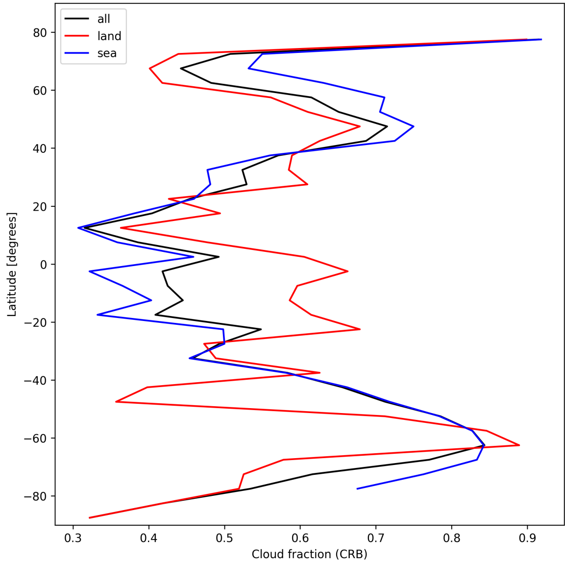
Figure 24: Zonal average of “Cloud fraction (CRB)” for 2025-02-14 to 2025-02-15.
