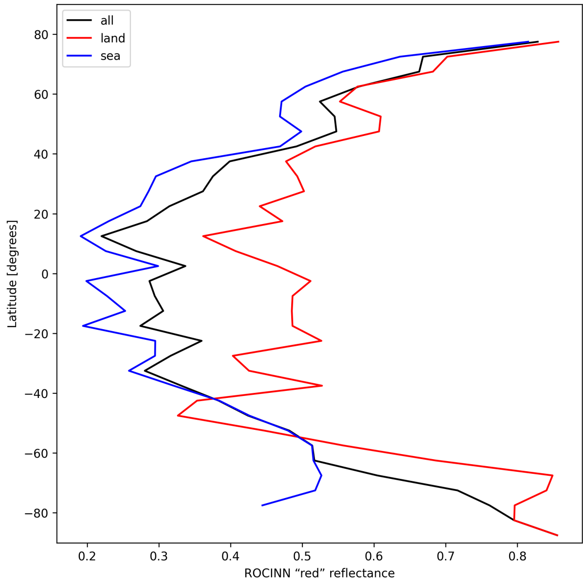
Figure 35: Zonal average of “ROCINN “red” reflectance” for 2025-02-14 to 2025-02-15.
