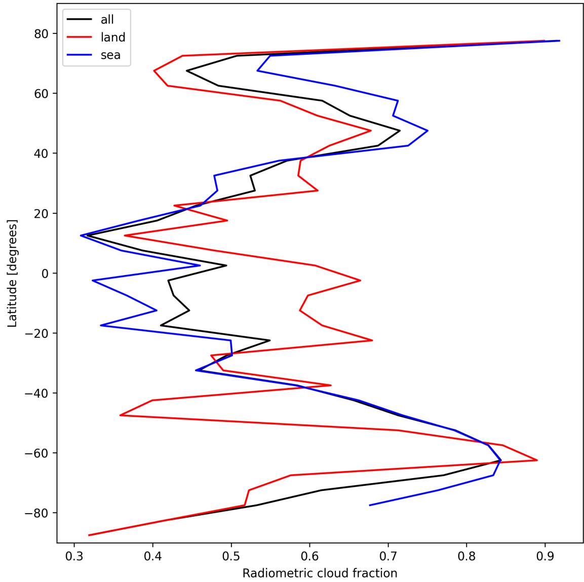
Figure 21: Zonal average of “Radiometric cloud fraction” for 2025-02-14 to 2025-02-15.
