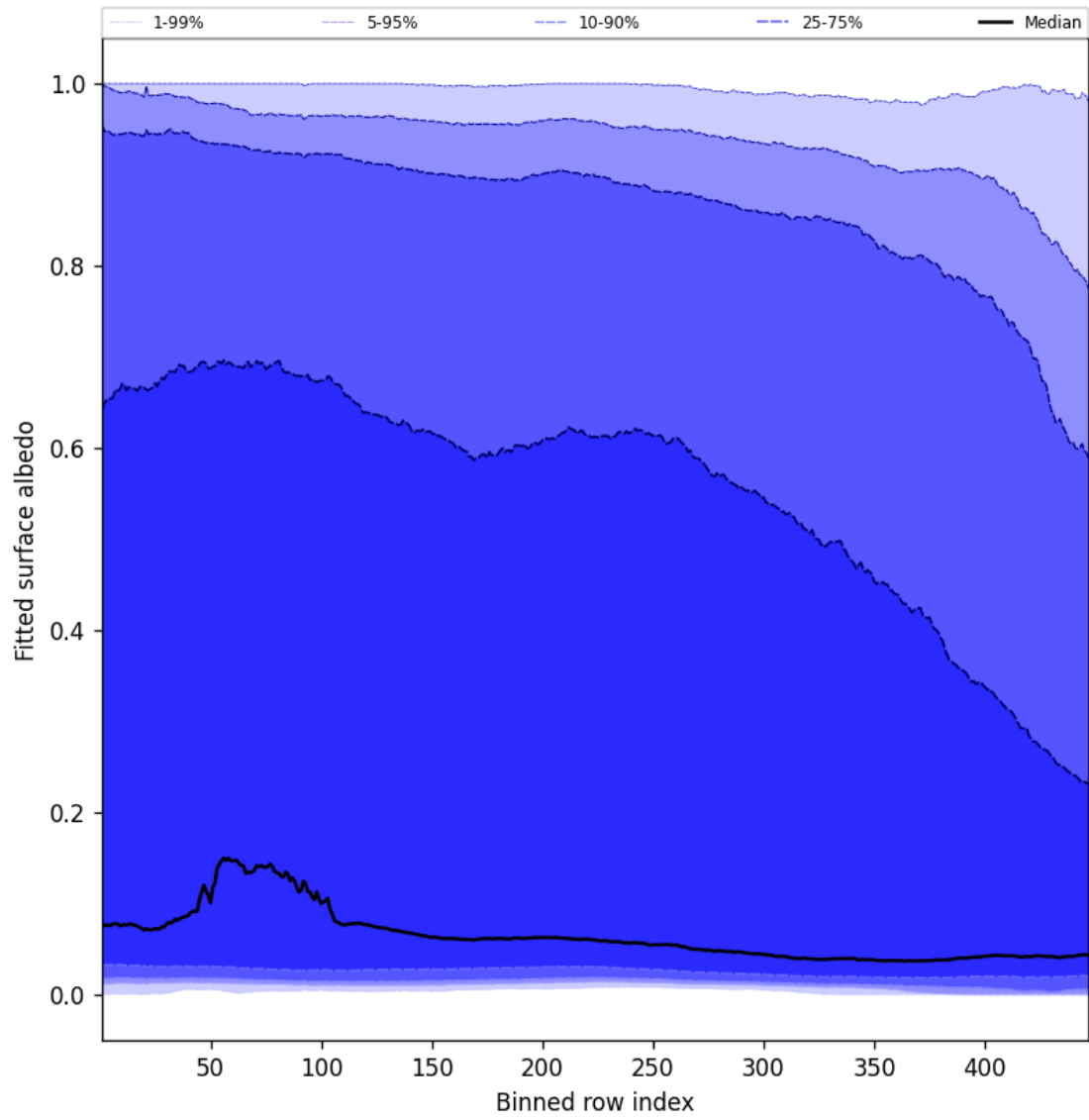
Figure 59: Along track statistics of “Fitted surface albedo” for 2025-02-14 to 2025-02-15
