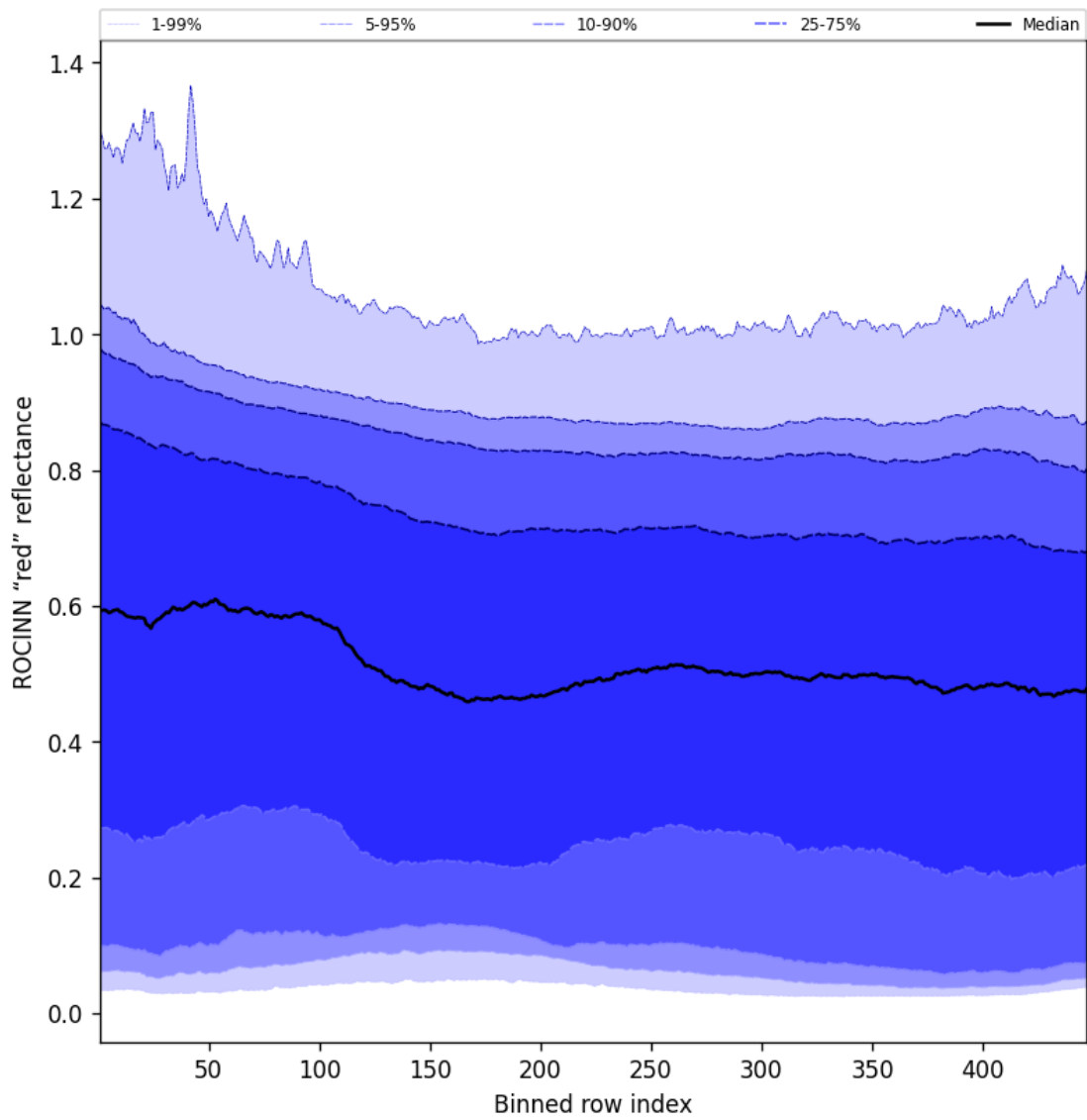
Figure 67: Along track statistics of “ROCINN “red” reflectance” for 2025-02-14 to 2025-02-15
