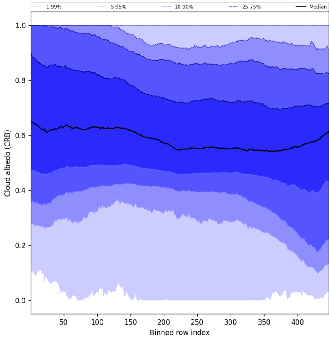
Figure 58: Along track statistics of “Cloud albedo (CRB)” for 2025-02-14 to 2025-02-15
