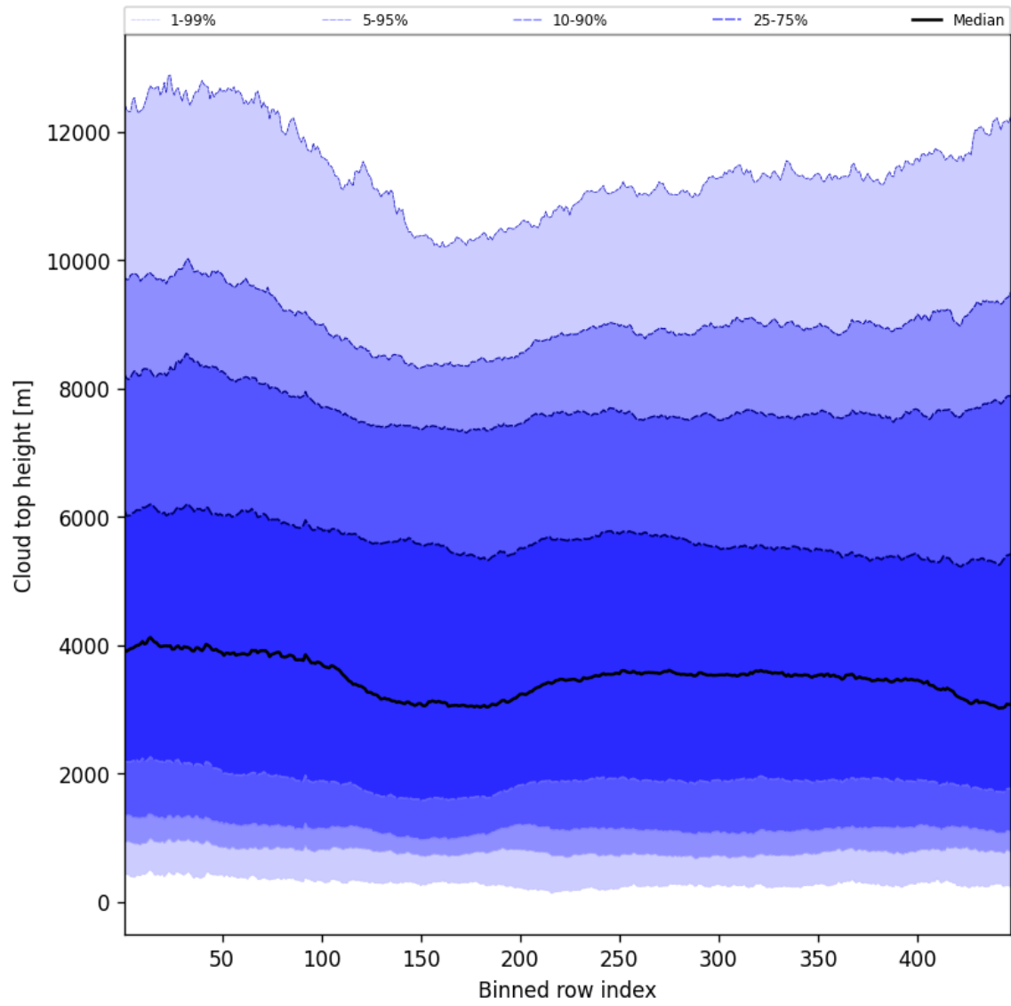
Figure 54: Along track statistics of “Cloud top height” for 2025-02-14 to 2025-02-15
