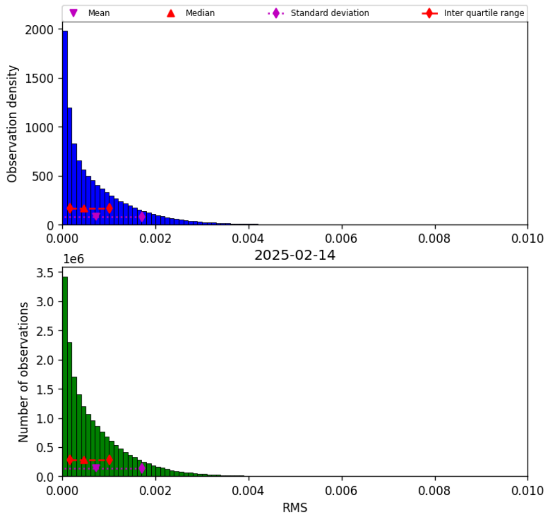
Figure 45: Histogram of “RMS” for 2025-02-14 to 2025-02-15
