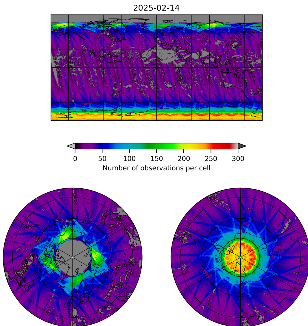
Figure 19: Map of the number of observations for 2025-02-14 to 2025-02-15
