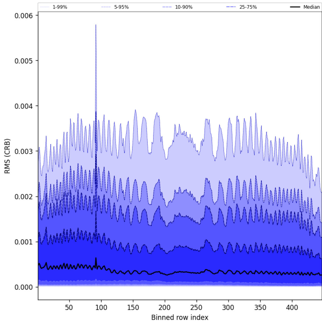
Figure 62: Along track statistics of “RMS (CRB)” for 2025-02-14 to 2025-02-15
