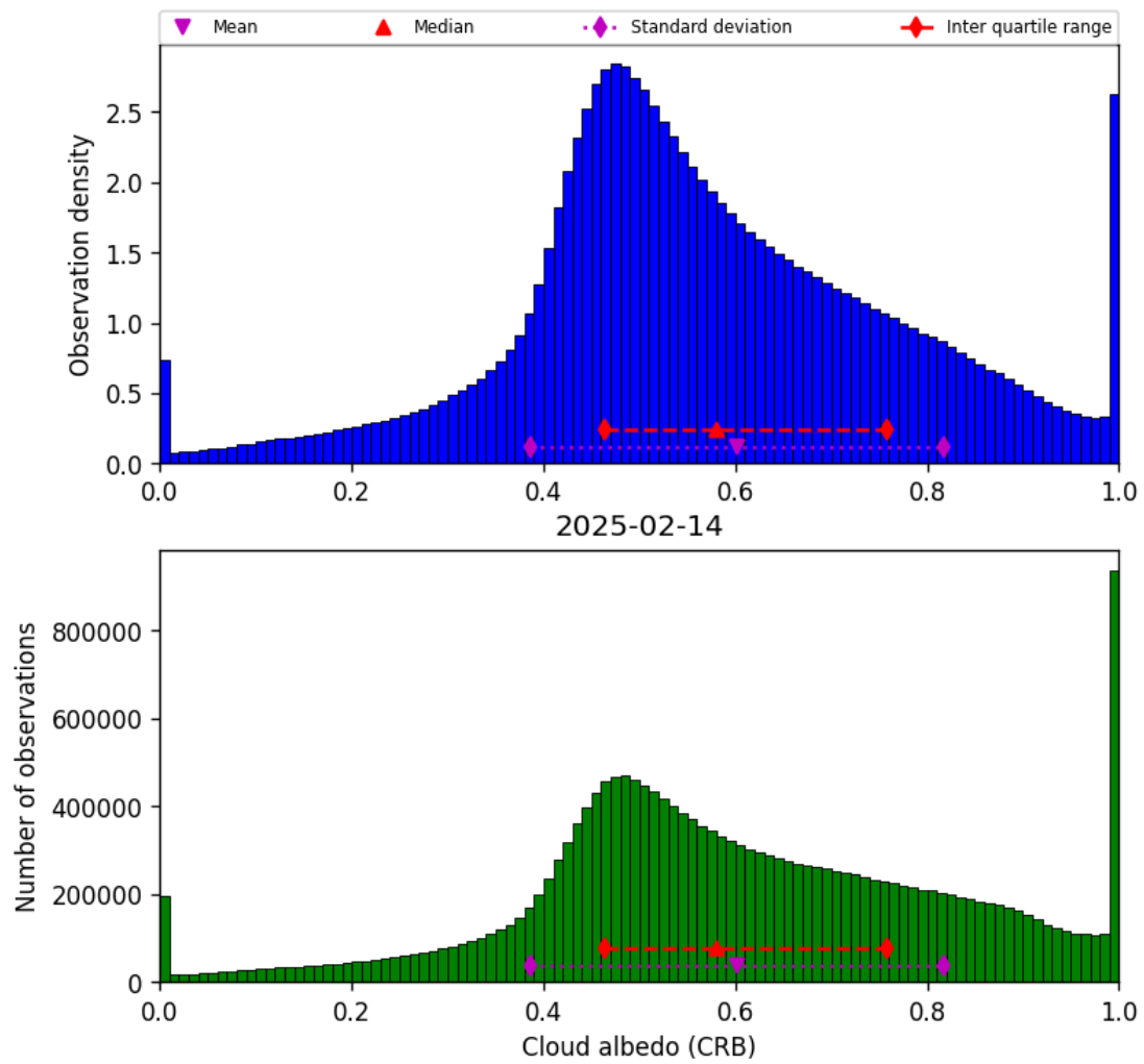
Figure 42: Histogram of “Cloud albedo (CRB)” for 2025-02-14 to 2025-02-15
