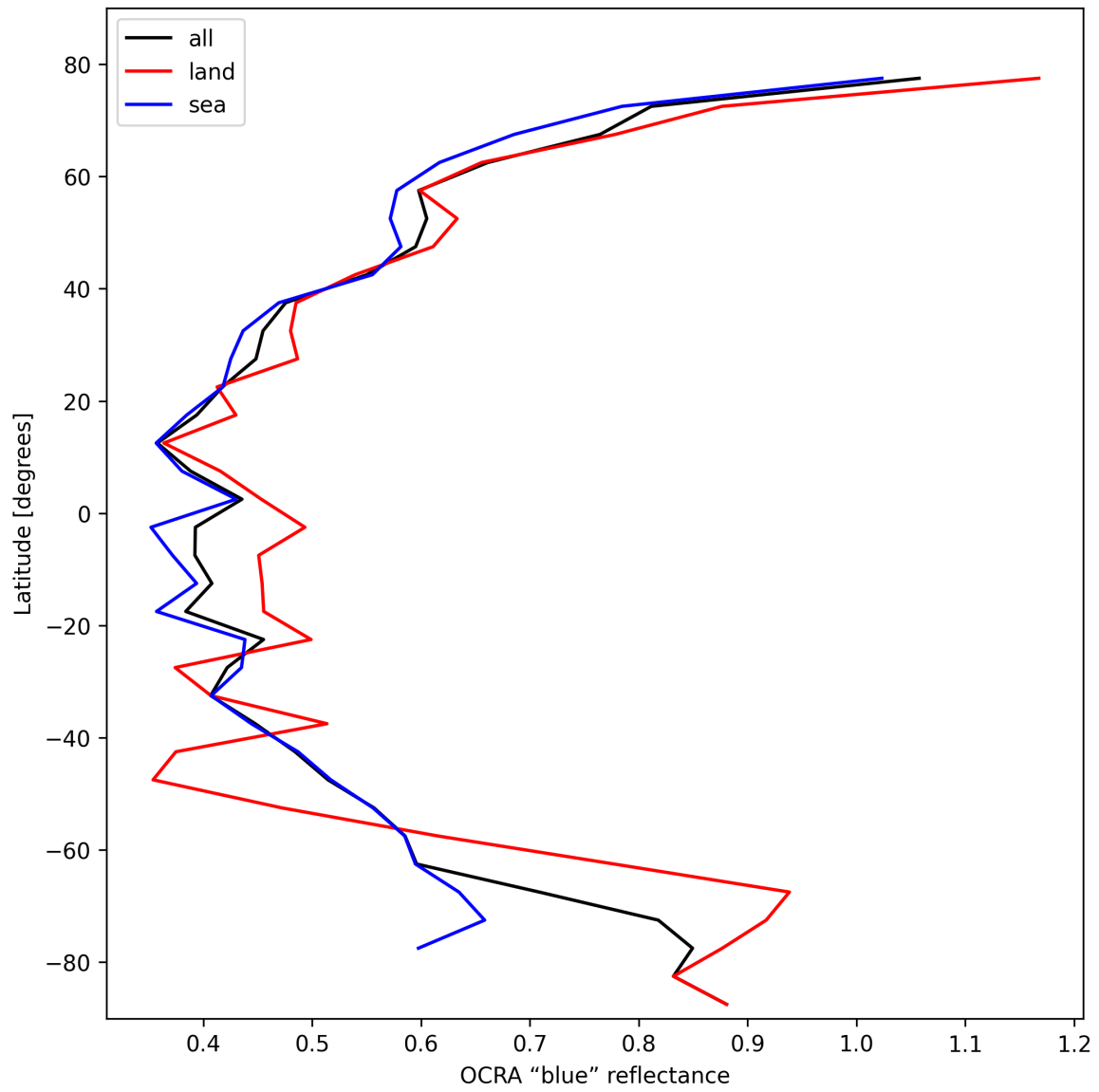
Figure 33: Zonal average of “OCRA “blue” reflectance” for 2025-02-14 to 2025-02-15.
