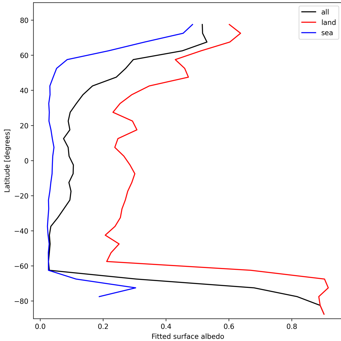
Figure 27: Zonal average of “Fitted surface albedo” for 2025-02-14 to 2025-02-15.
