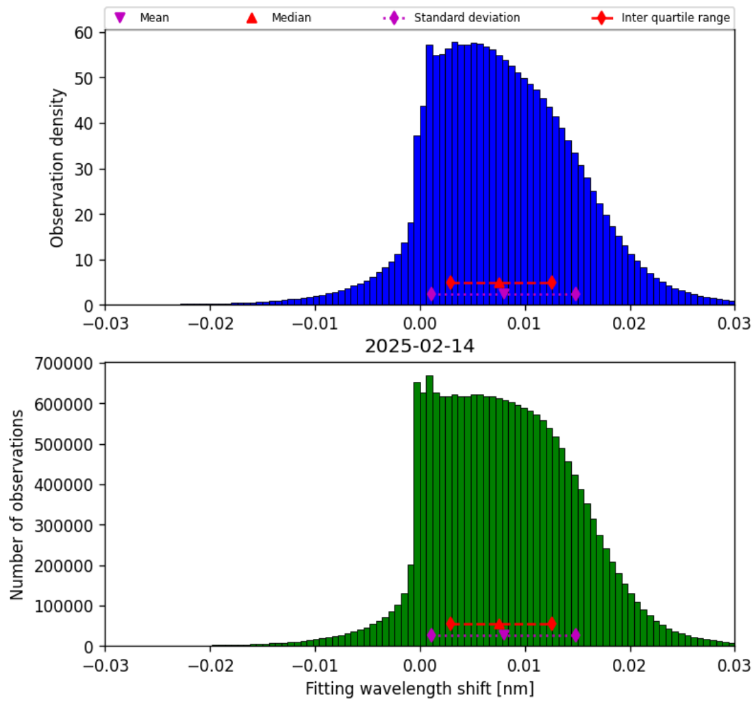
Figure 47: Histogram of “Fitting wavelength shift” for 2025-02-14 to 2025-02-15
