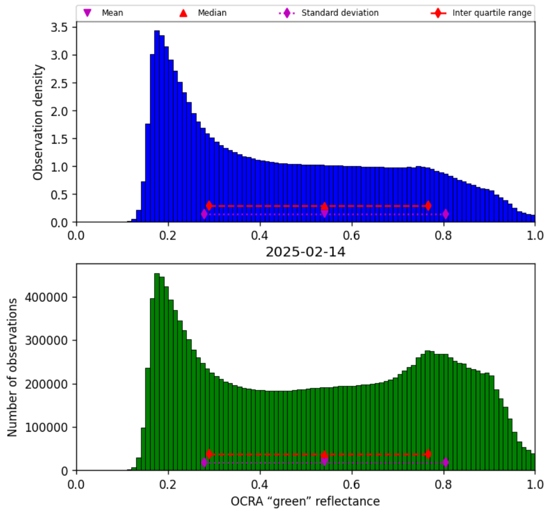
Figure 50: Histogram of “OCRA “green” reflectance” for 2025-02-14 to 2025-02-15
