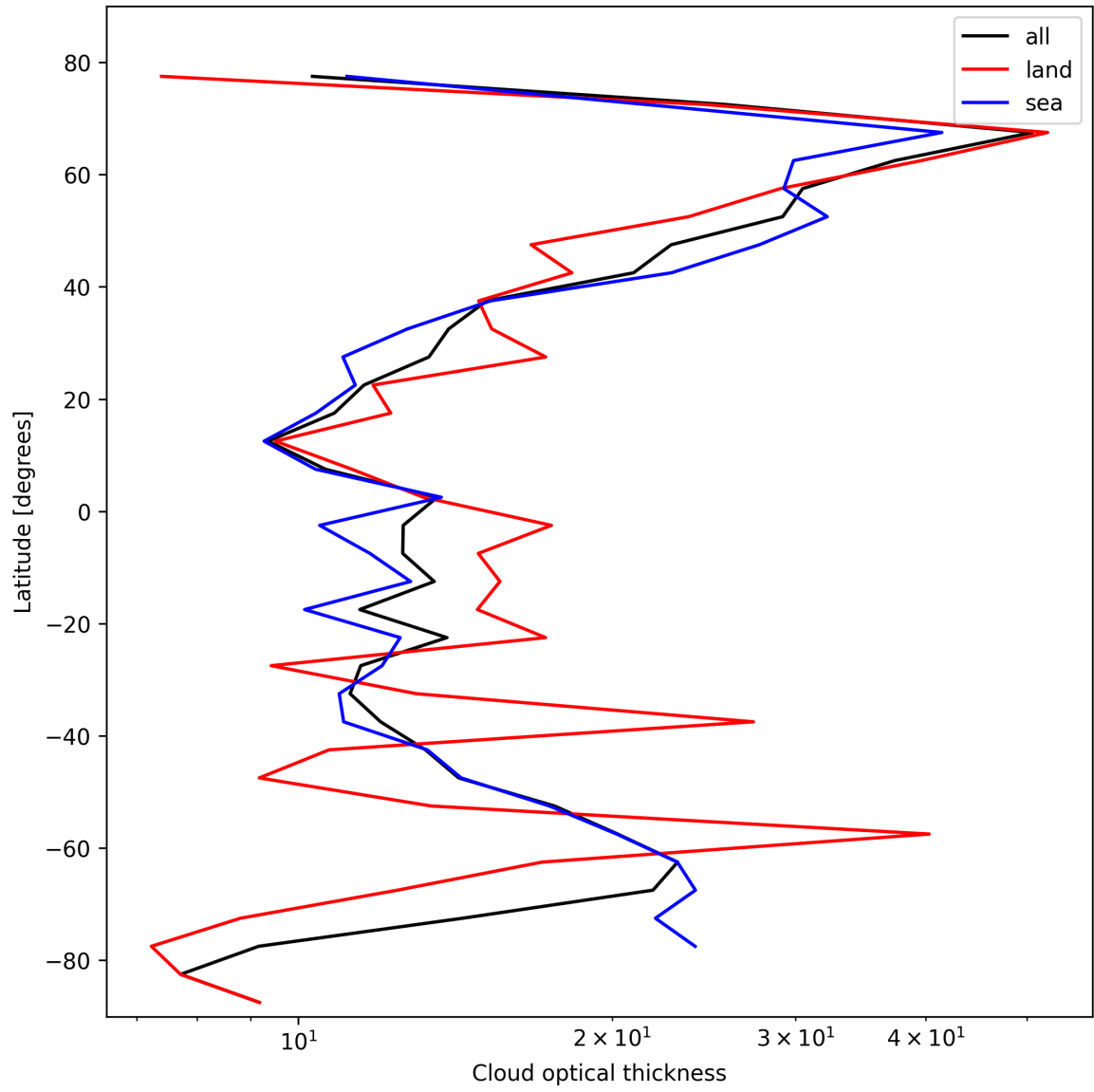
Figure 23: Zonal average of “Cloud optical thickness” for 2025-02-14 to 2025-02-15.
