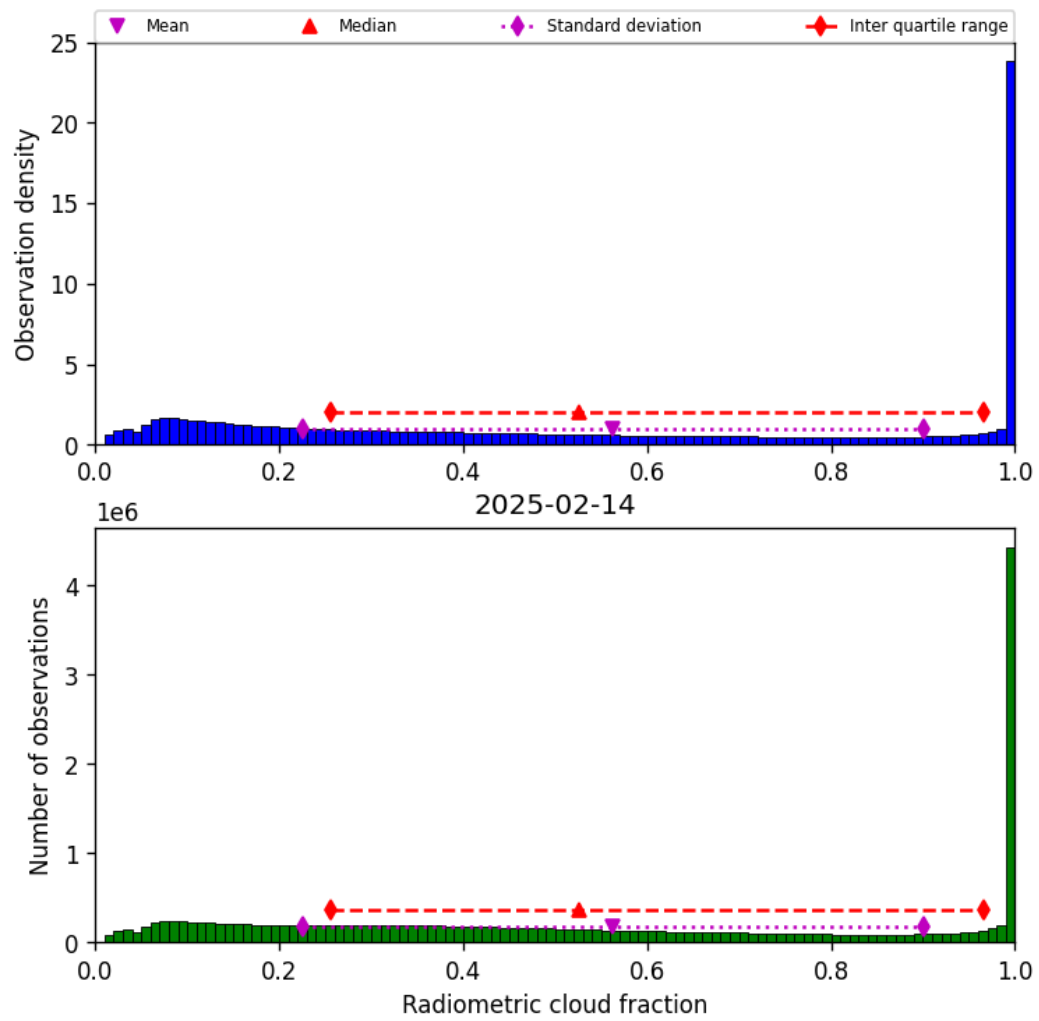
Figure 37: Histogram of “Radiometric cloud fraction” for 2025-02-14 to 2025-02-15
