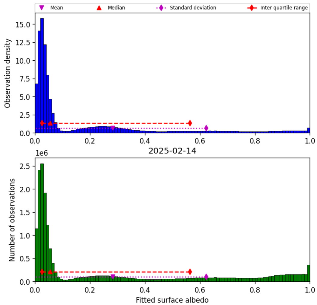
Figure 43: Histogram of “Fitted surface albedo” for 2025-02-14 to 2025-02-15
