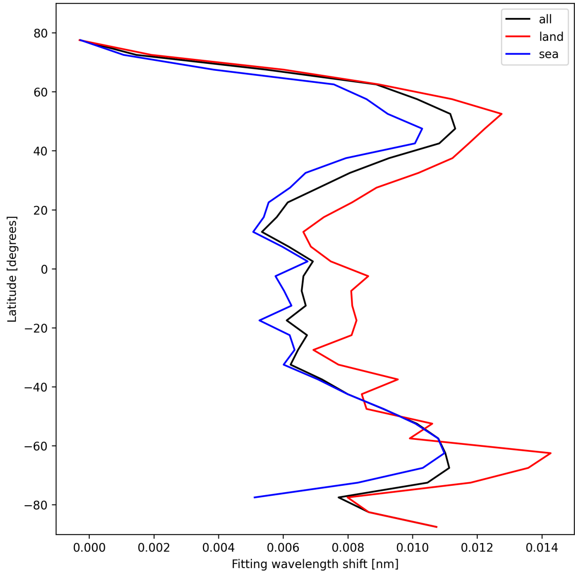
Figure 31: Zonal average of “Fitting wavelength shift” for 2025-02-14 to 2025-02-15.
