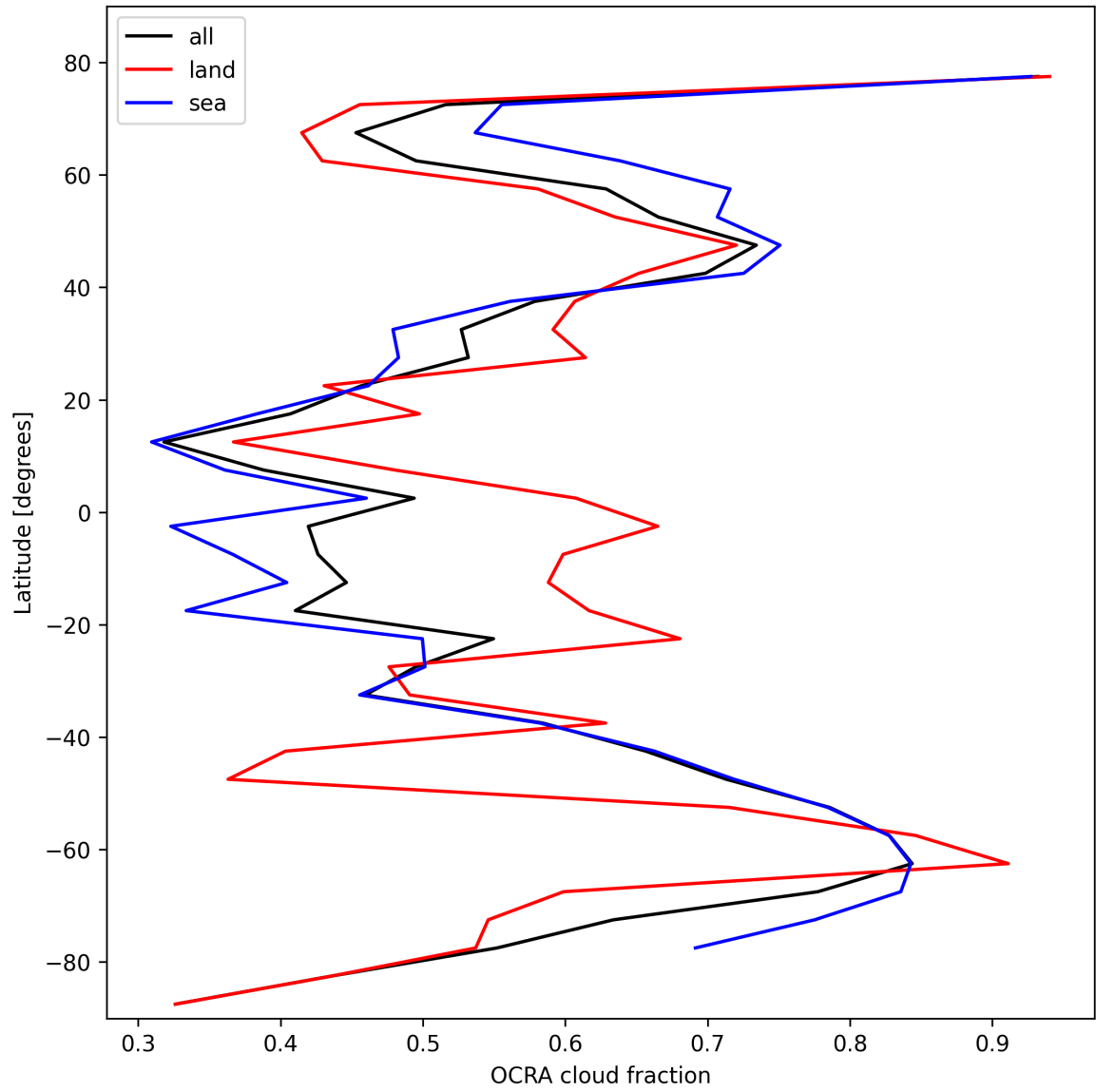
Figure 32: Zonal average of “OCRA cloud fraction” for 2025-02-14 to 2025-02-15.
