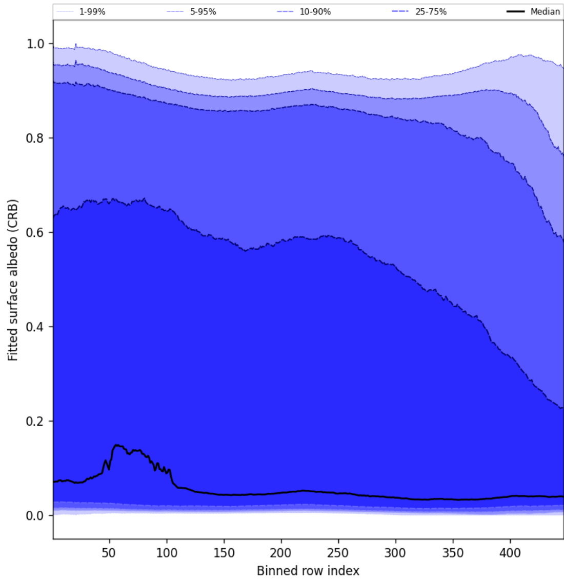
Figure 60: Along track statistics of “Fitted surface albedo (CRB)” for 2025-02-14 to 2025-02-15
