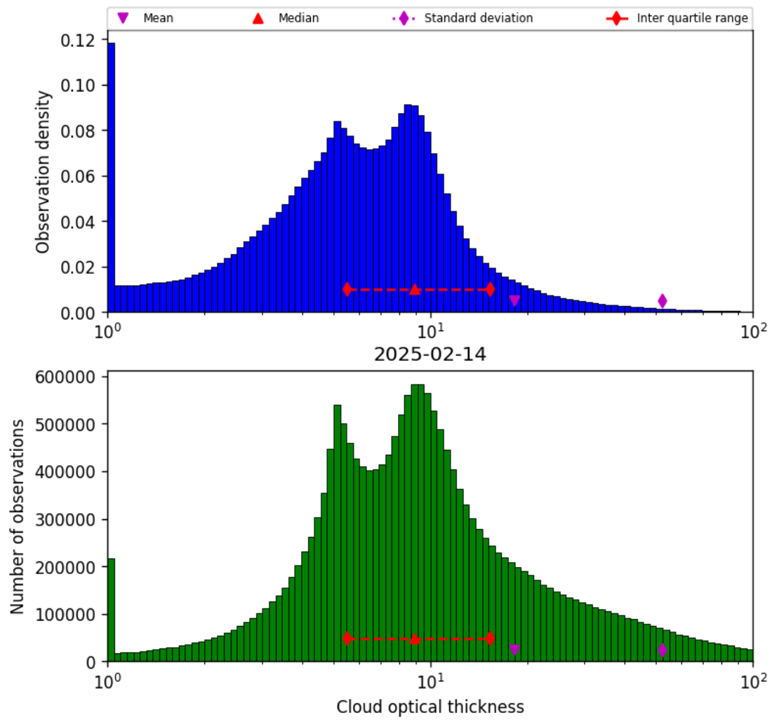
Figure 39: Histogram of “Cloud optical thickness” for 2025-02-14 to 2025-02-15
