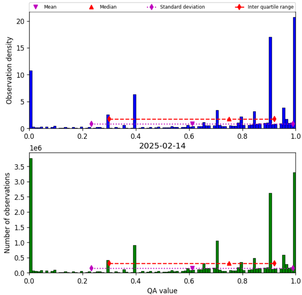
Figure 36: Histogram of “QA value” for 2025-02-14 to 2025-02-15
