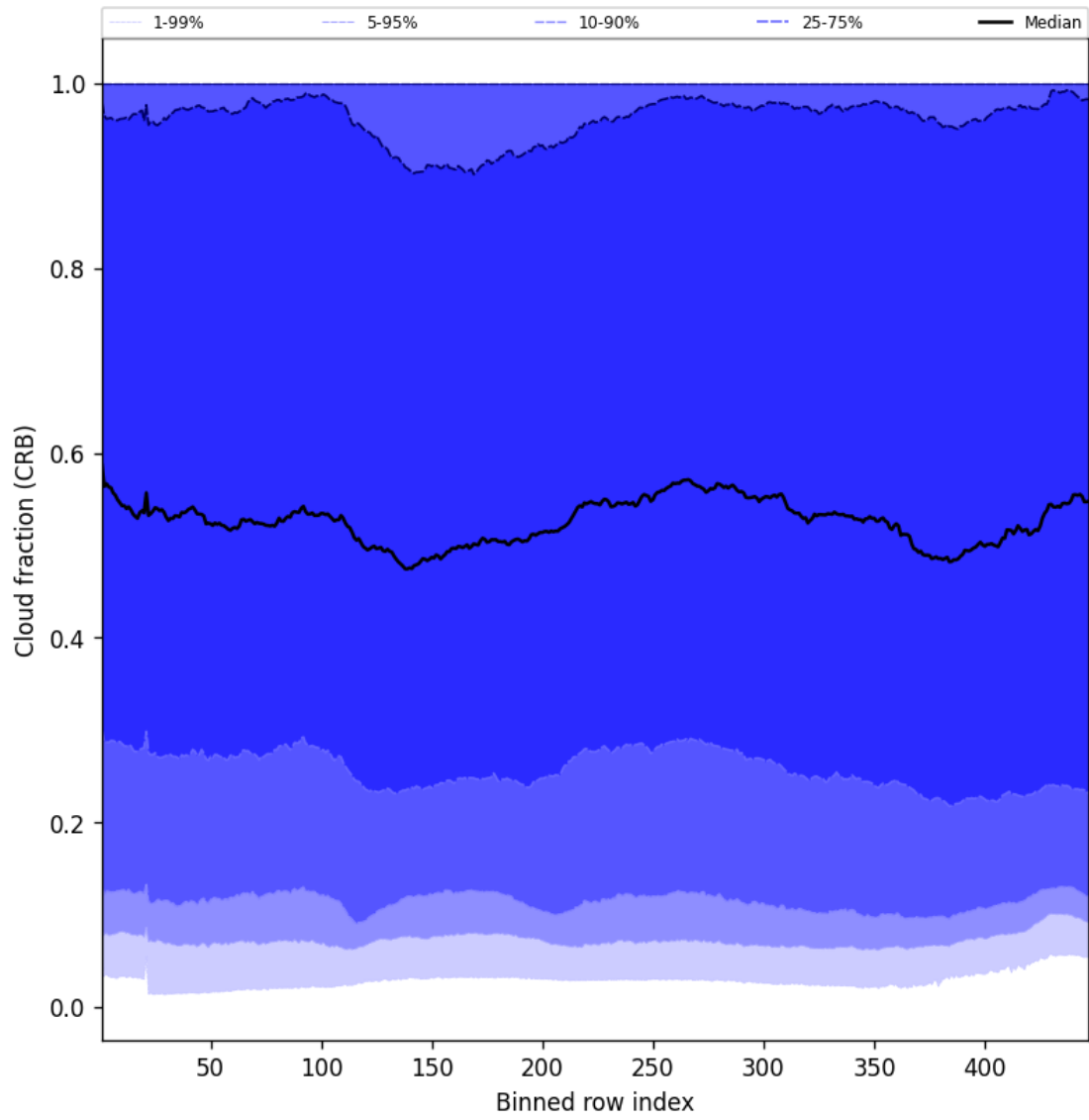
Figure 56: Along track statistics of “Cloud fraction (CRB)” for 2025-02-14 to 2025-02-15
