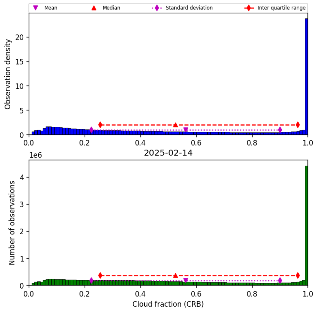
Figure 40: Histogram of “Cloud fraction (CRB)” for 2025-02-14 to 2025-02-15
