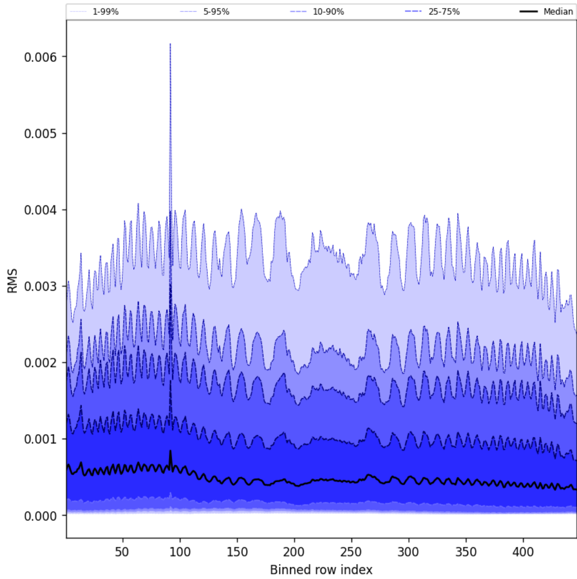
Figure 61: Along track statistics of “RMS” for 2025-02-14 to 2025-02-15
