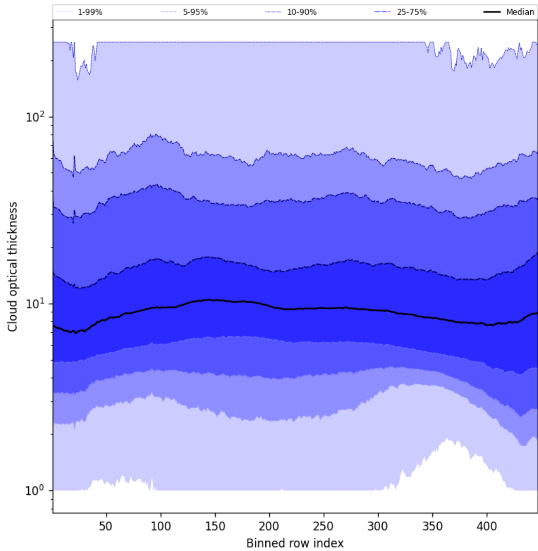
Figure 55: Along track statistics of “Cloud optical thickness” for 2025-02-14 to 2025-02-15
