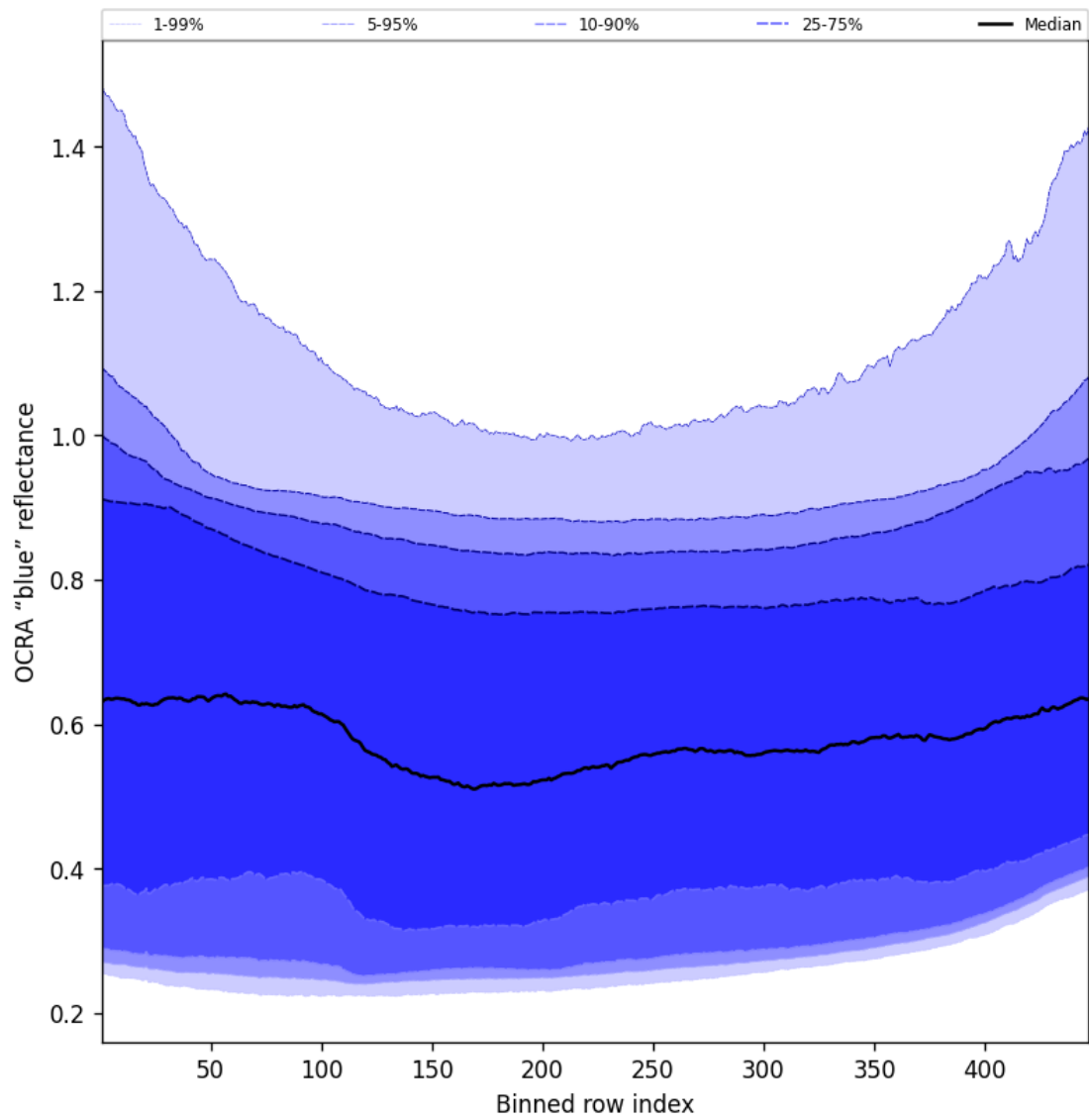
Figure 65: Along track statistics of “OCRA “blue” reflectance” for 2025-02-14 to 2025-02-15
