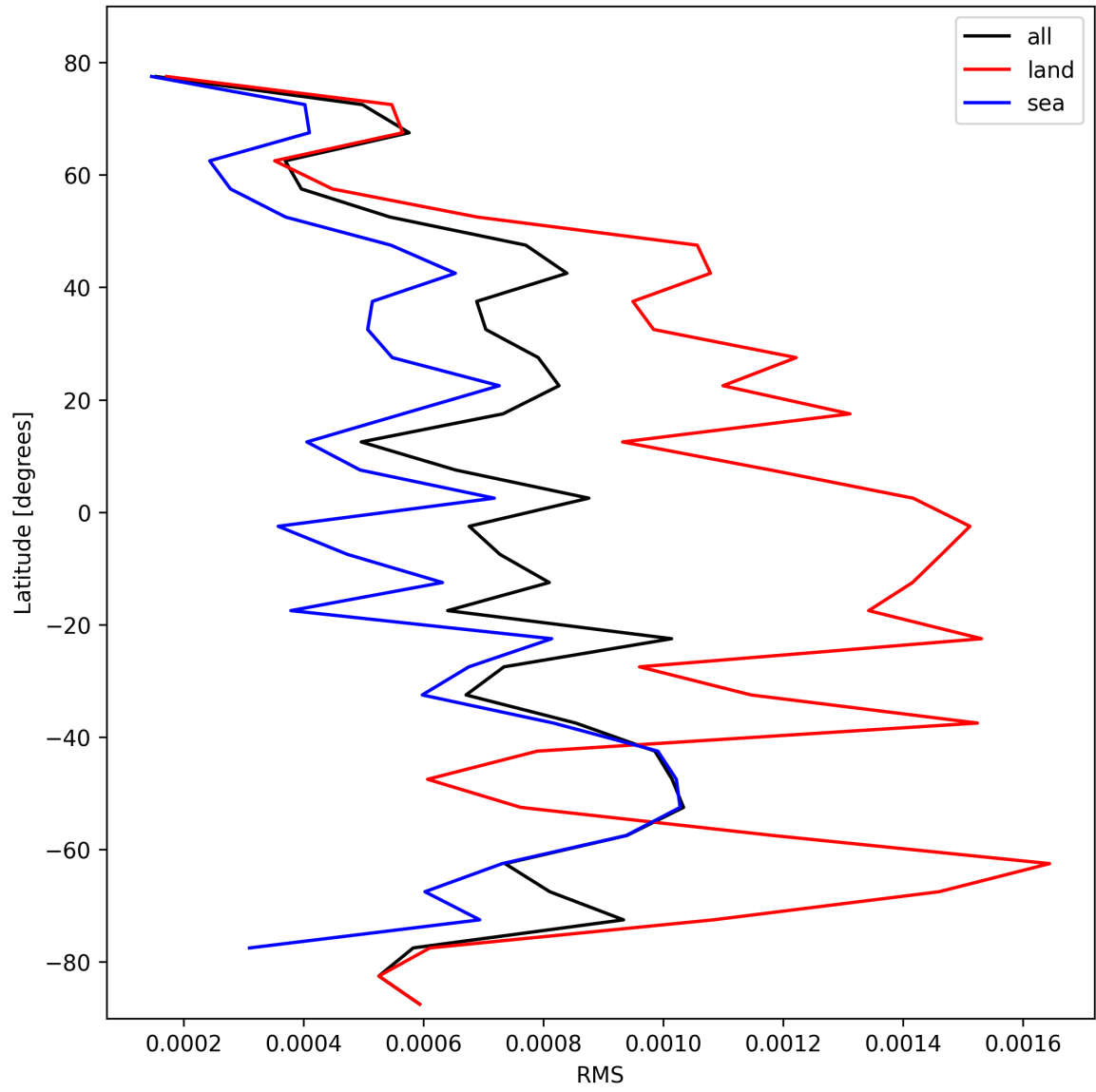
Figure 29: Zonal average of “RMS” for 2025-02-14 to 2025-02-15.
