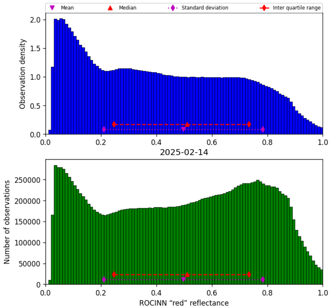
Figure 51: Histogram of “ROCINN “red” reflectance” for 2025-02-14 to 2025-02-15
