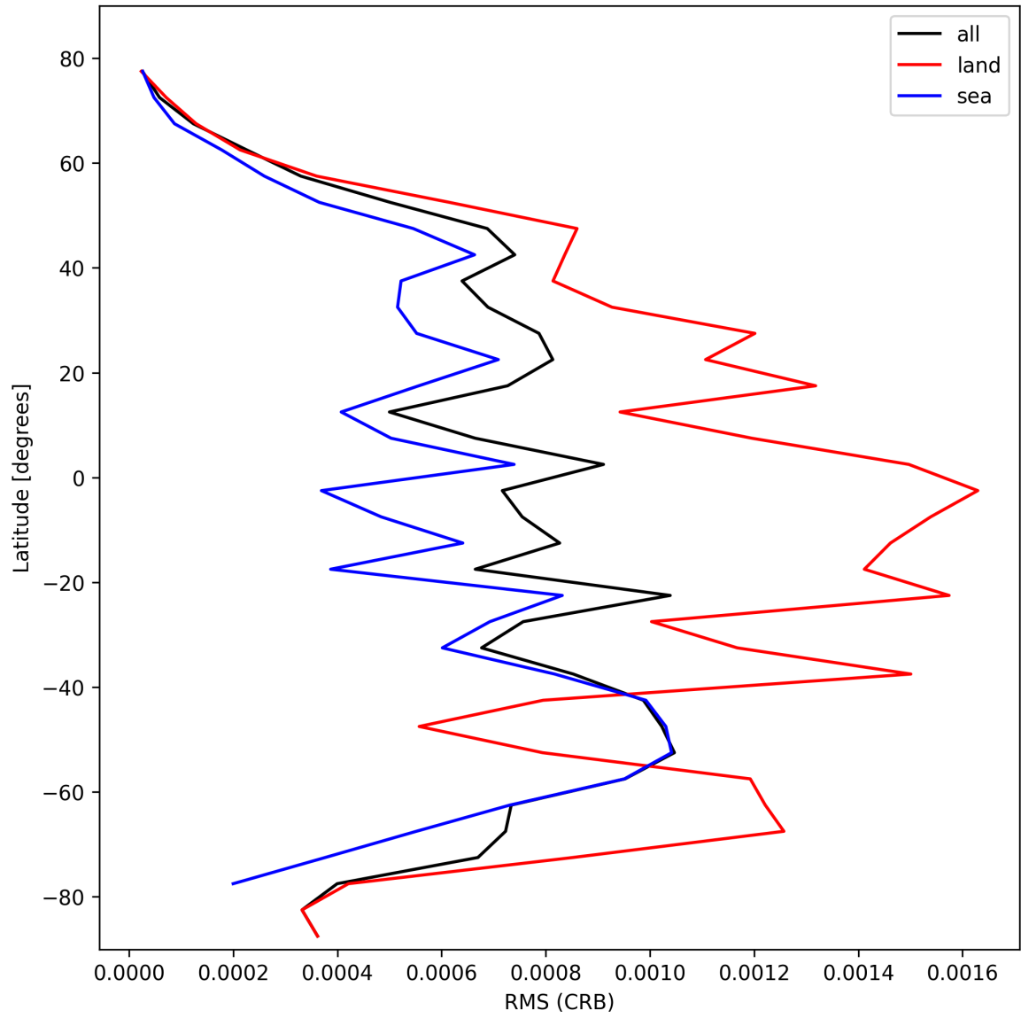
Figure 30: Zonal average of “RMS (CRB)” for 2025-02-14 to 2025-02-15.
