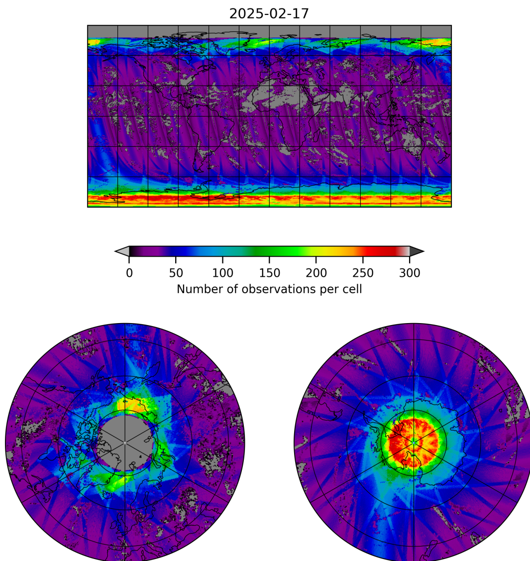
Figure 19: Map of the number of observations for 2025-02-17 to 2025-02-18
