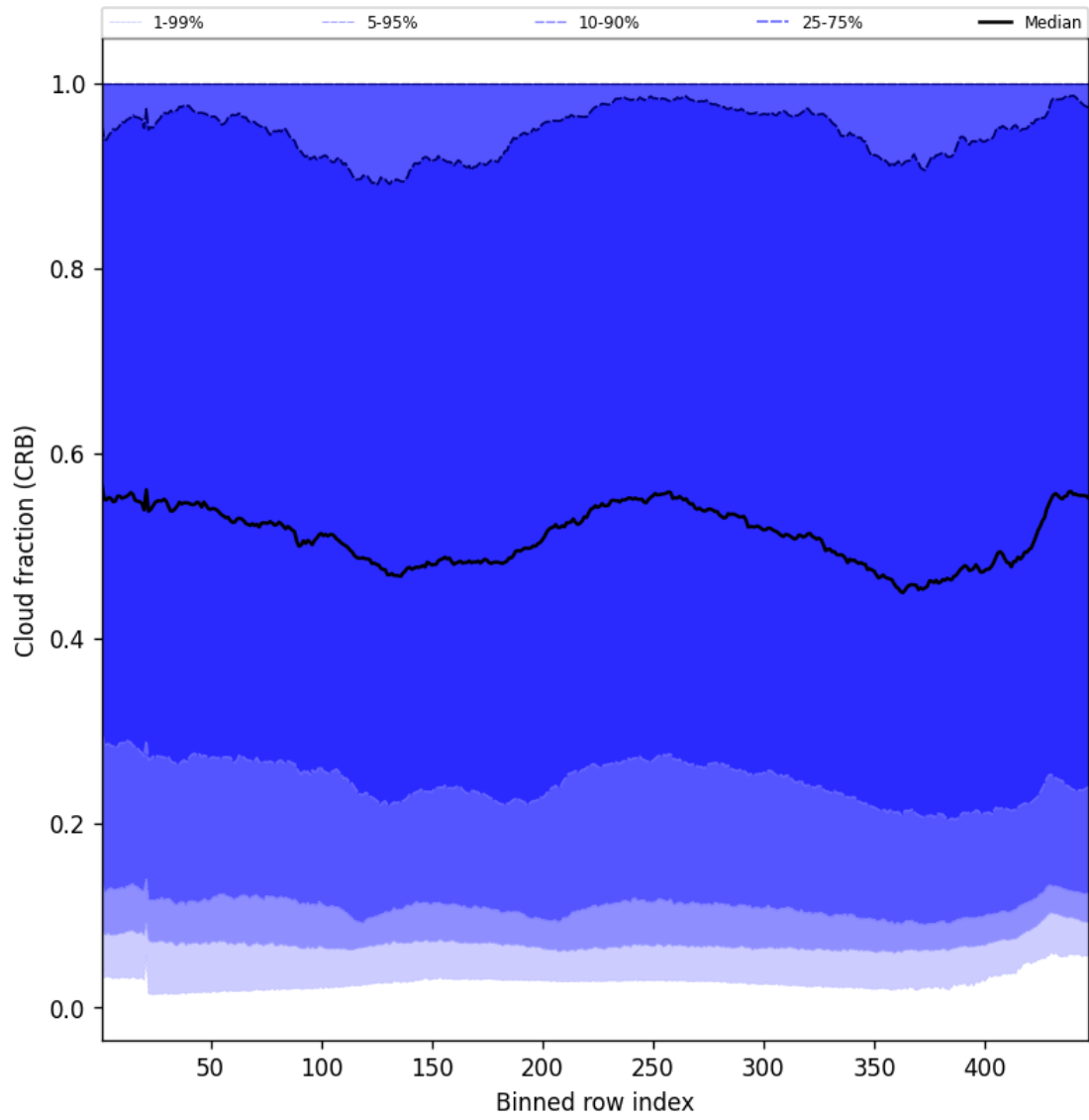
Figure 56: Along track statistics of “Cloud fraction (CRB)” for 2025-02-17 to 2025-02-18
