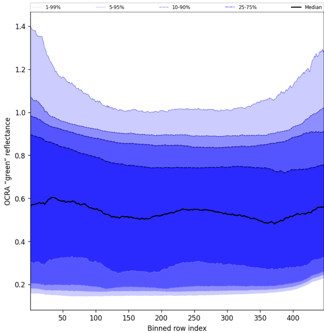
Figure 66: Along track statistics of "OCRA "green" reflectance" for 2025-02-17 to 2025-02-18
