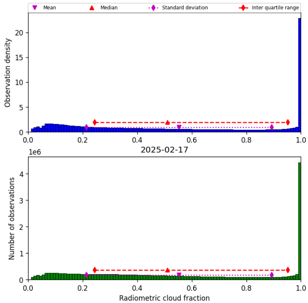
Figure 37: Histogram of “Radiometric cloud fraction” for 2025-02-17 to 2025-02-18
