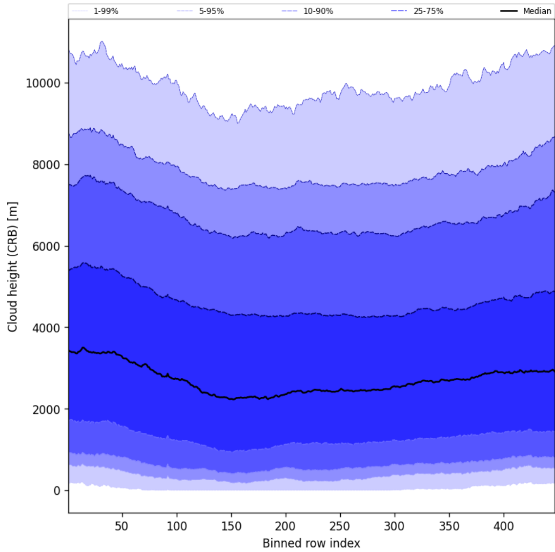
Figure 57: Along track statistics of “Cloud height (CRB)” for 2025-02-17 to 2025-02-18
