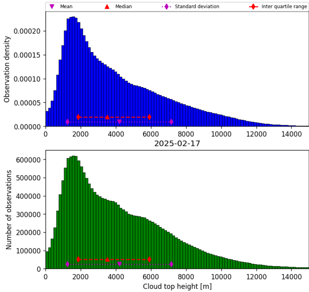
Figure 38: Histogram of “Cloud top height” for 2025-02-17 to 2025-02-18
