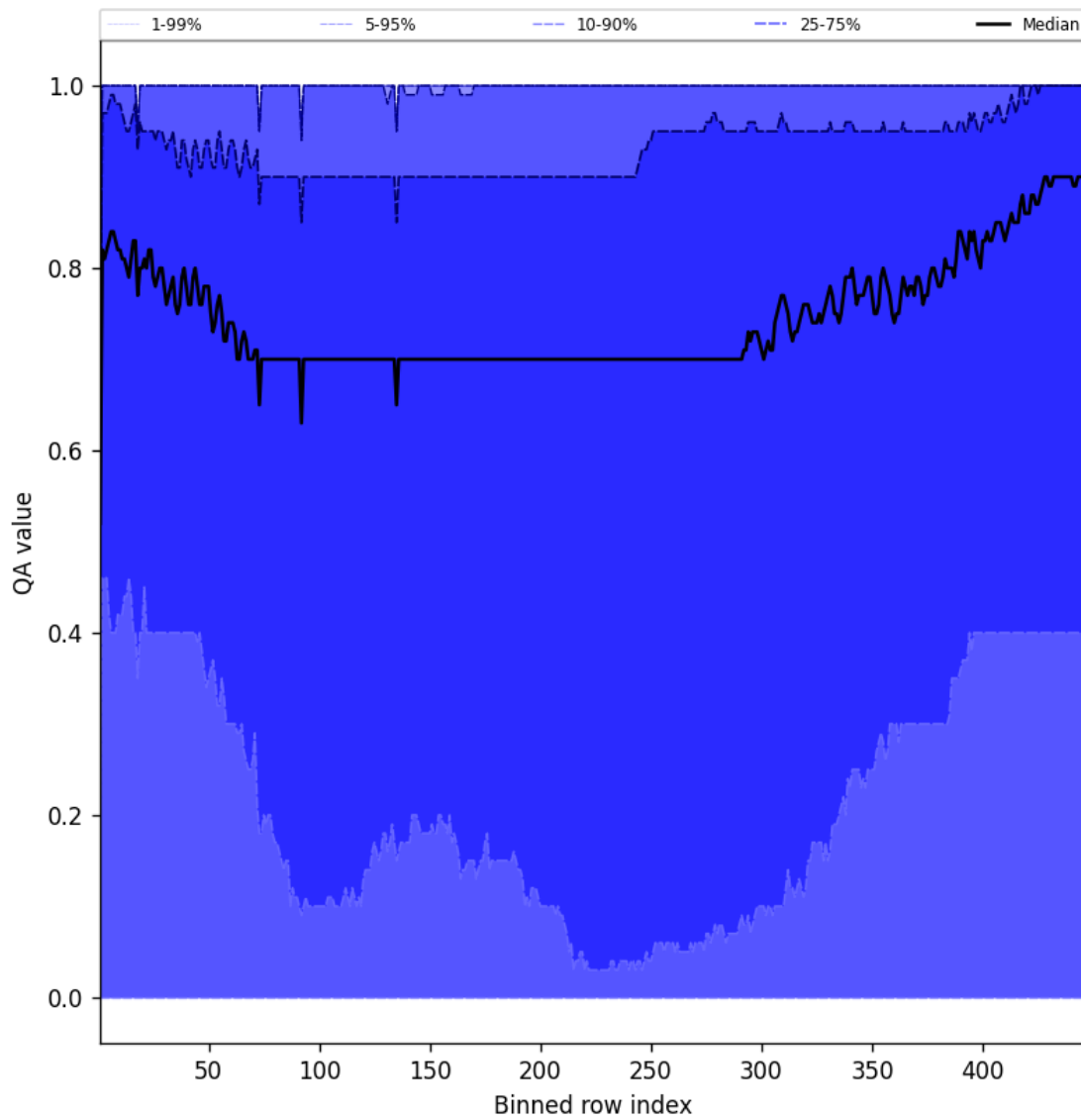
Figure 52: Along track statistics of “QA value” for 2025-02-17 to 2025-02-18
