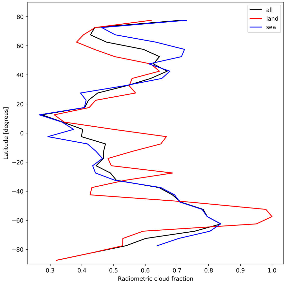
Figure 21: Zonal average of “Radiometric cloud fraction” for 2025-02-17 to 2025-02-18.
