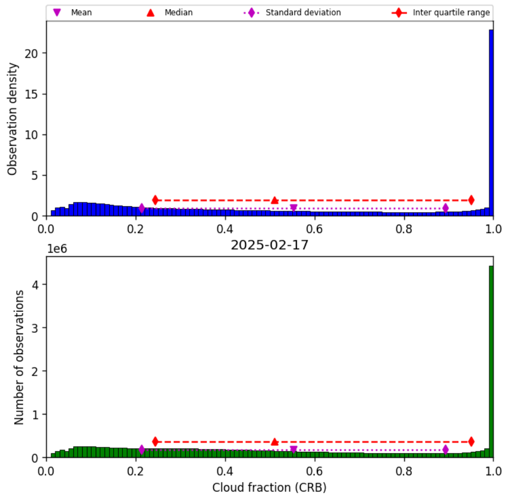
Figure 40: Histogram of “Cloud fraction (CRB)” for 2025-02-17 to 2025-02-18
