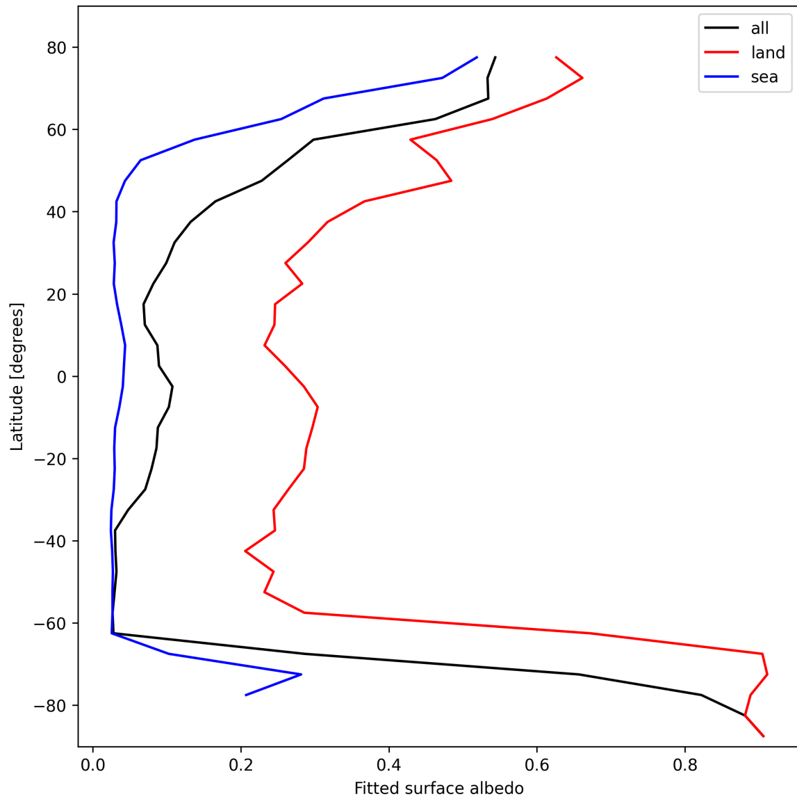
Figure 27: Zonal average of “Fitted surface albedo” for 2025-02-17 to 2025-02-18.
