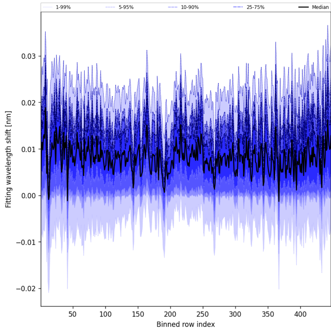
Figure 63: Along track statistics of “Fitting wavelength shift” for 2025-02-17 to 2025-02-18
