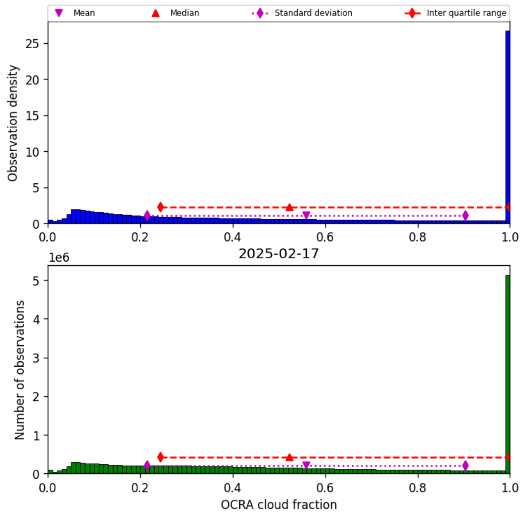
Figure 48: Histogram of “OCRA cloud fraction” for 2025-02-17 to 2025-02-18
