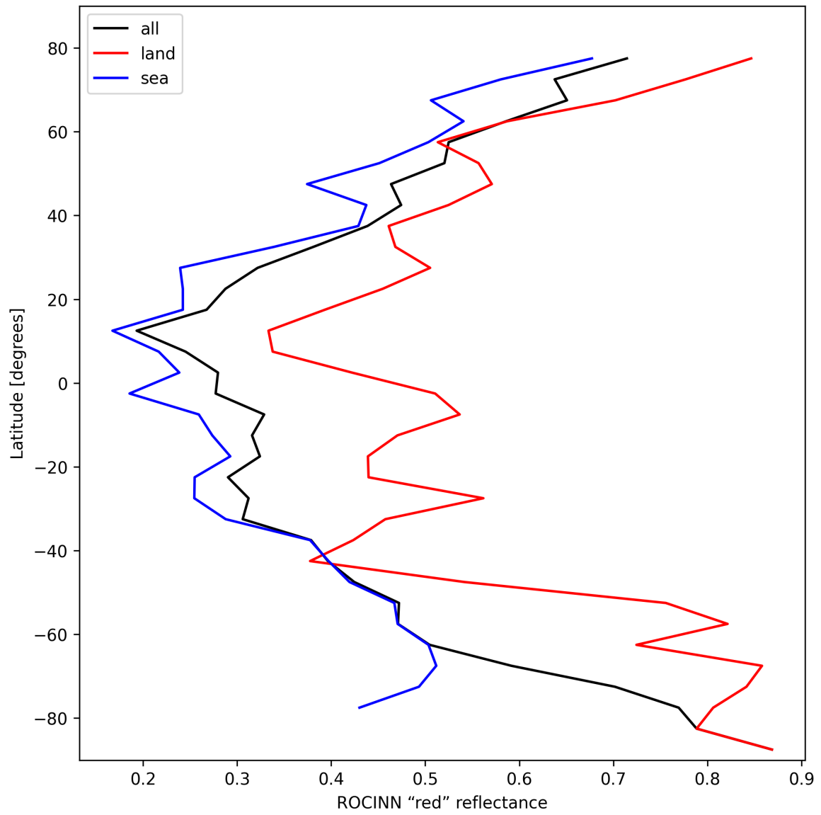
Figure 35: Zonal average of “ROCINN “red” reflectance” for 2025-02-17 to 2025-02-18.
