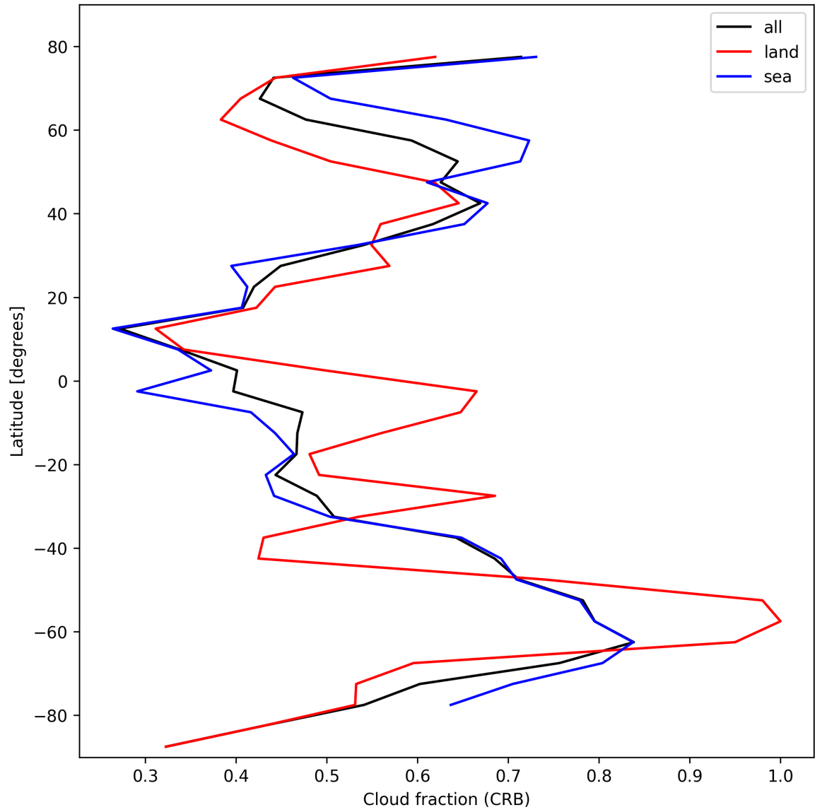
Figure 24: Zonal average of “Cloud fraction (CRB)” for 2025-02-17 to 2025-02-18.
