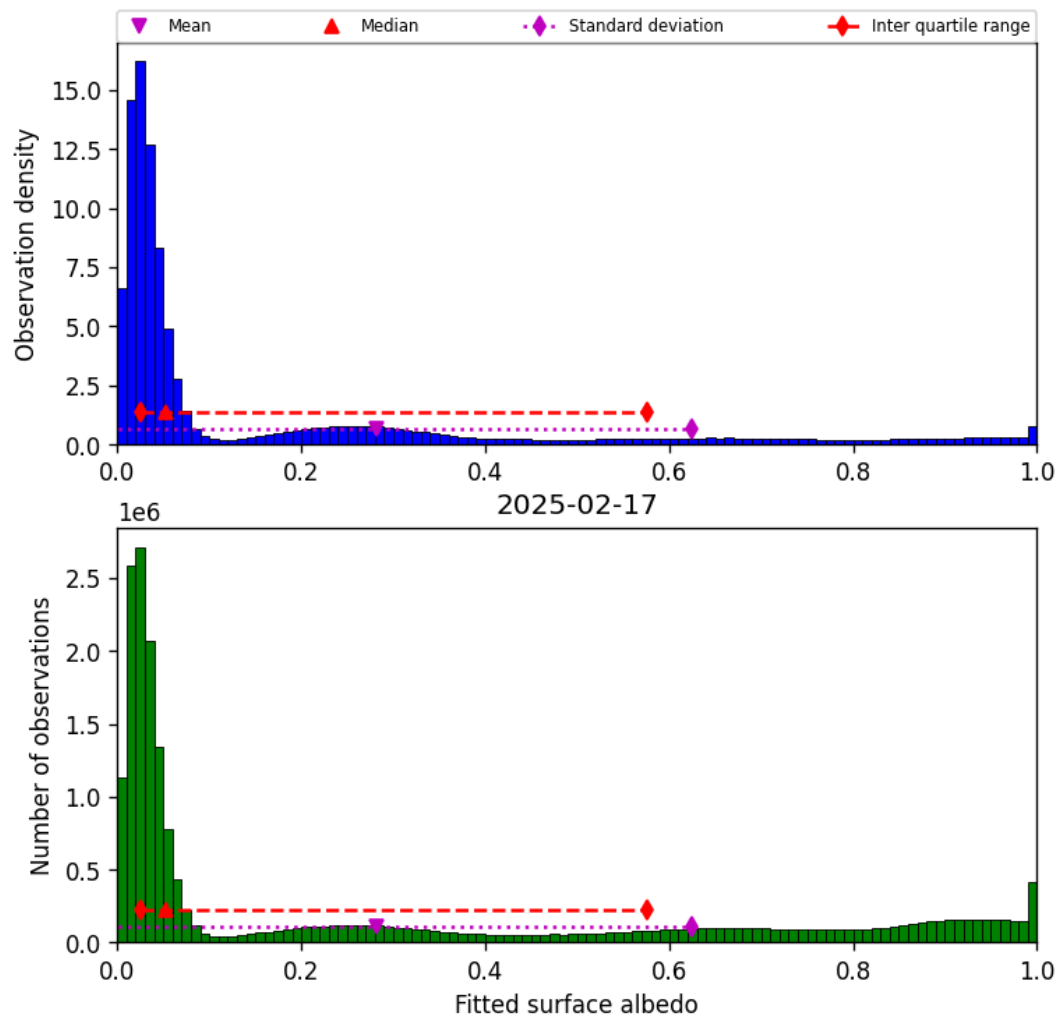
Figure 43: Histogram of “Fitted surface albedo” for 2025-02-17 to 2025-02-18
