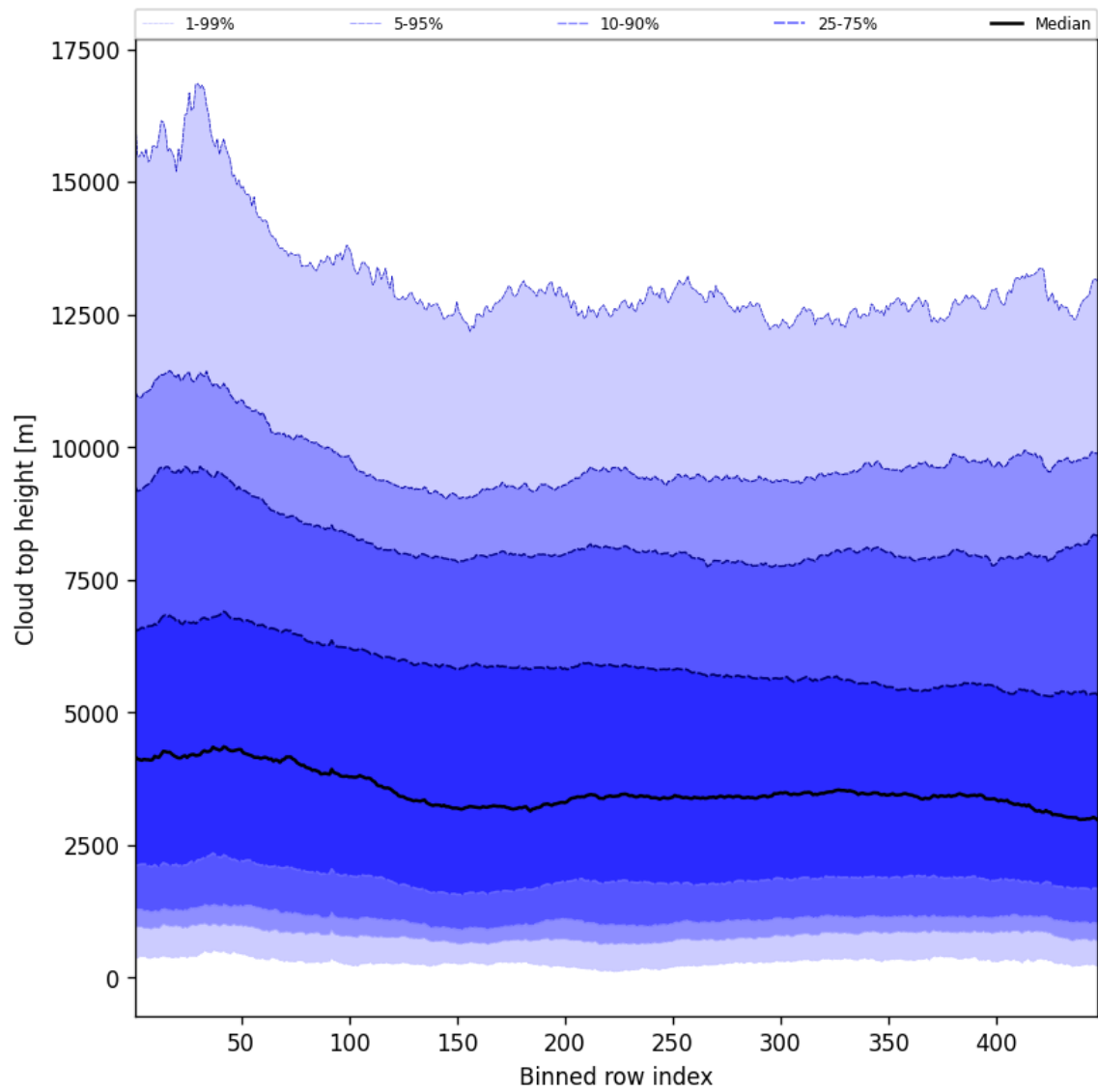
Figure 54: Along track statistics of “Cloud top height” for 2025-02-17 to 2025-02-18
