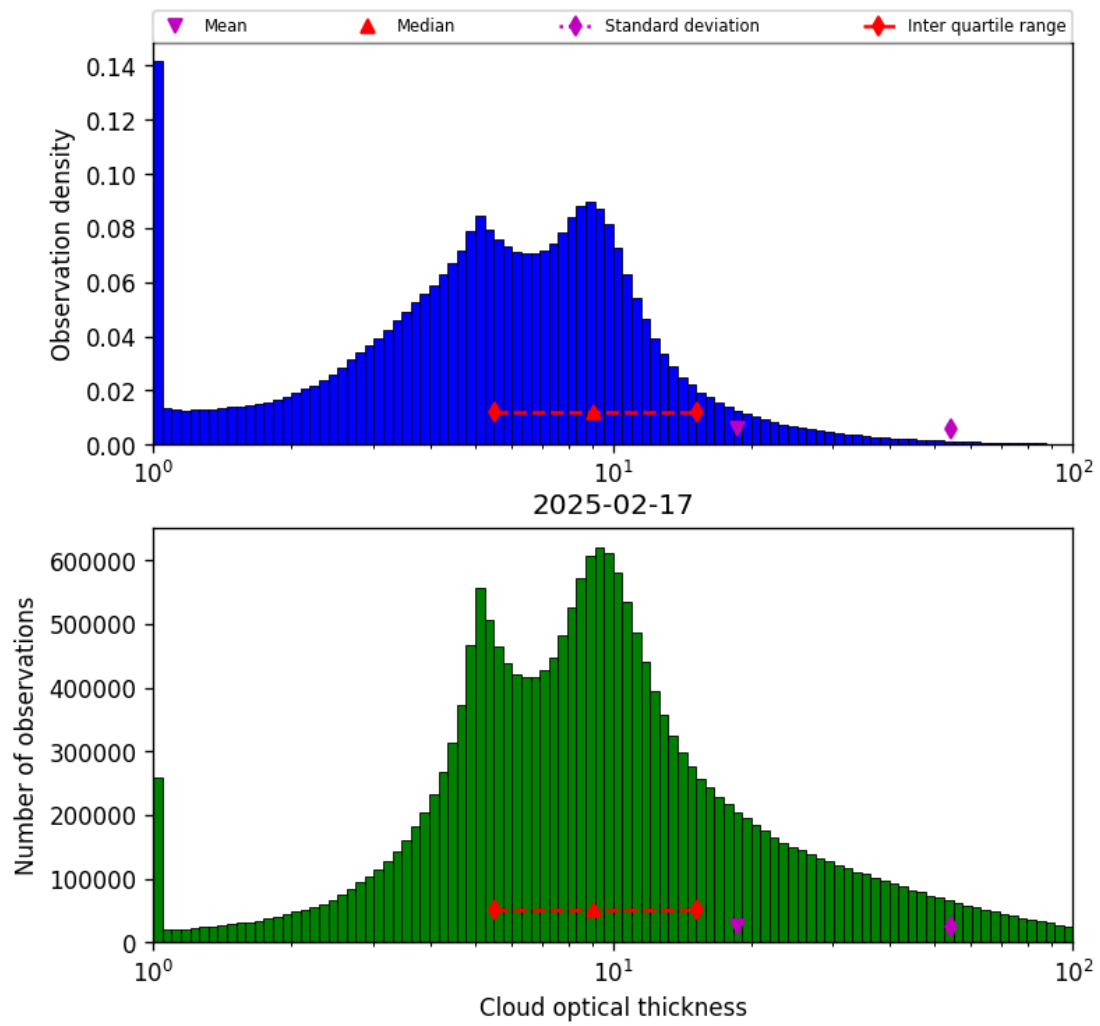
Figure 39: Histogram of “Cloud optical thickness” for 2025-02-17 to 2025-02-18
