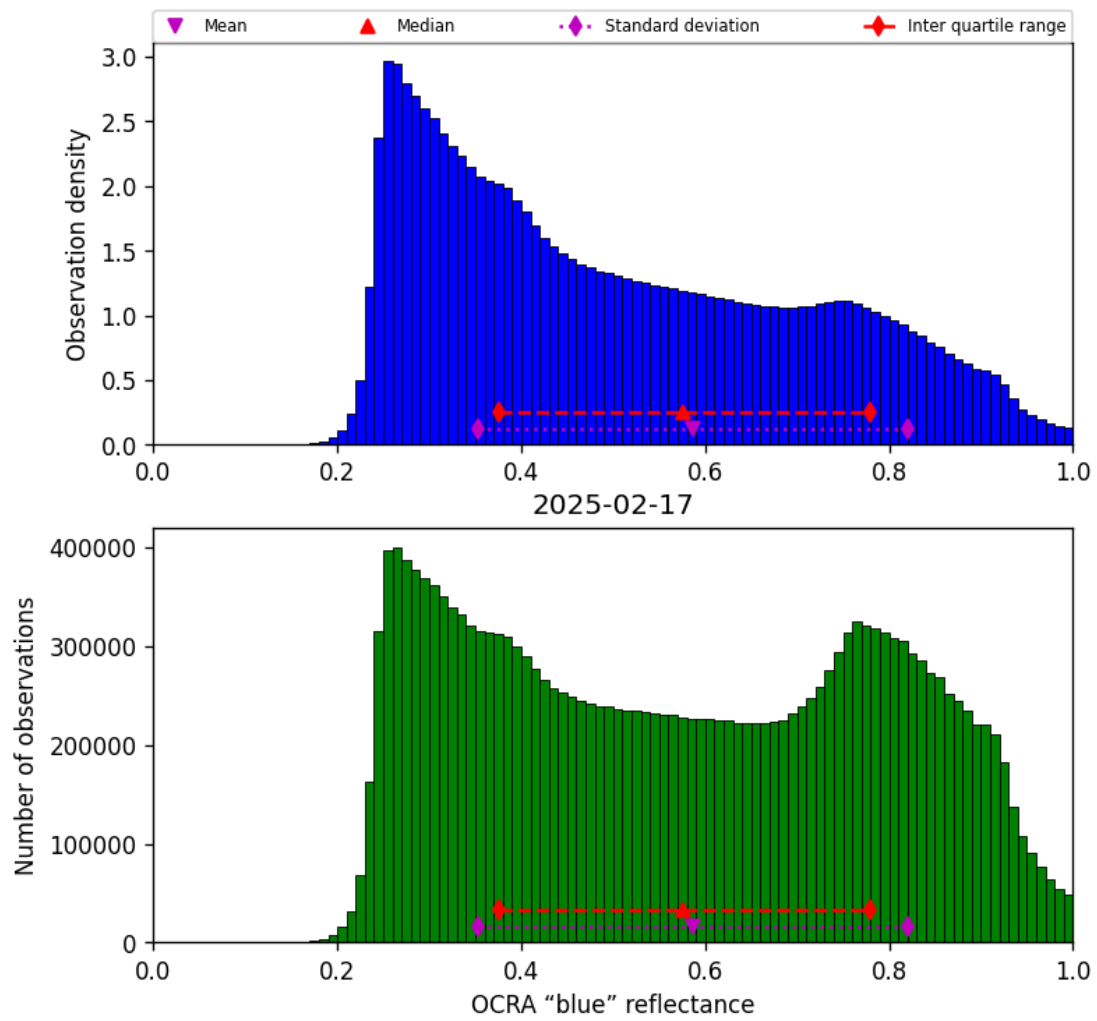
Figure 49: Histogram of “OCRA “blue” reflectance” for 2025-02-17 to 2025-02-18
