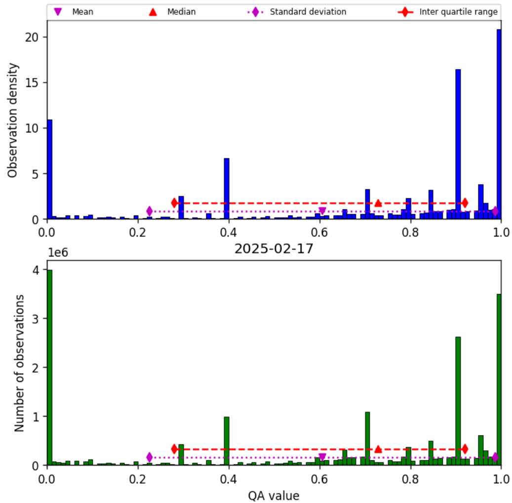
Figure 36: Histogram of “QA value” for 2025-02-17 to 2025-02-18
