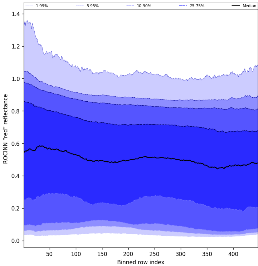
Figure 67: Along track statistics of “ROCINN “red” reflectance” for 2025-02-17 to 2025-02-18
