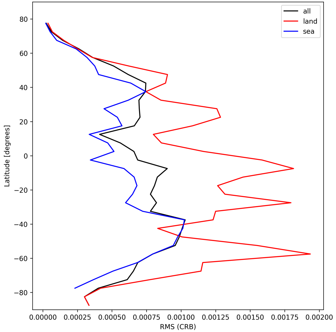
Figure 30: Zonal average of “RMS (CRB)” for 2025-02-17 to 2025-02-18.
