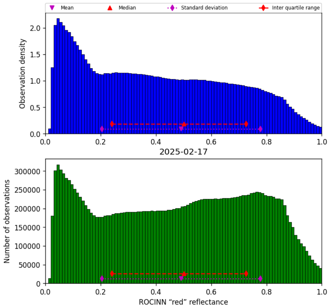
Figure 51: Histogram of “ROCINN “red” reflectance” for 2025-02-17 to 2025-02-18
