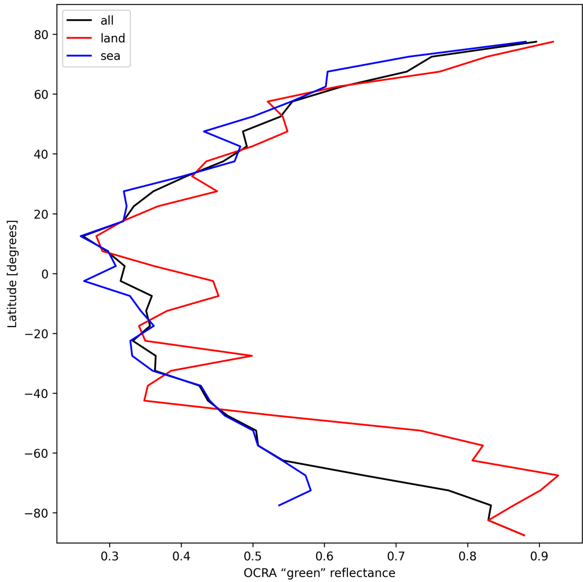
Figure 34: Zonal average of “OCRA “green” reflectance” for 2025-02-17 to 2025-02-18.
