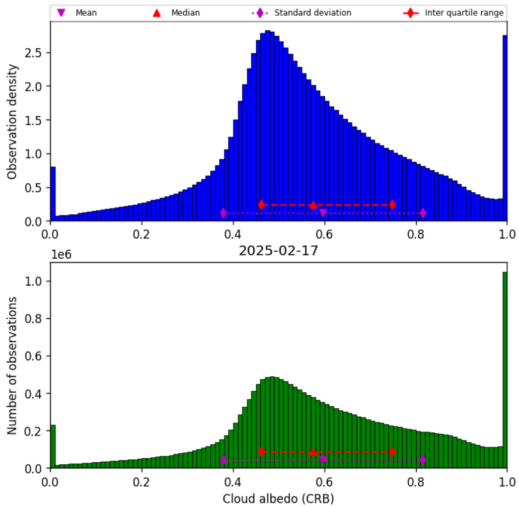
Figure 42: Histogram of “Cloud albedo (CRB)” for 2025-02-17 to 2025-02-18
