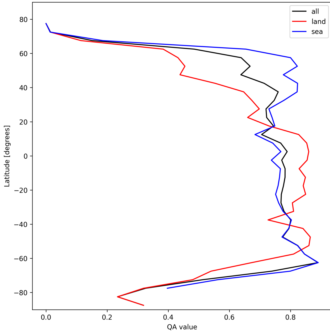
Figure 20: Zonal average of “QA value” for 2025-02-17 to 2025-02-18.
