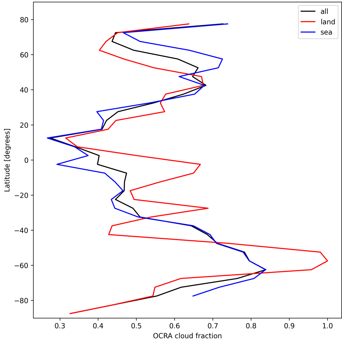
Figure 32: Zonal average of “OCRA cloud fraction” for 2025-02-17 to 2025-02-18.
