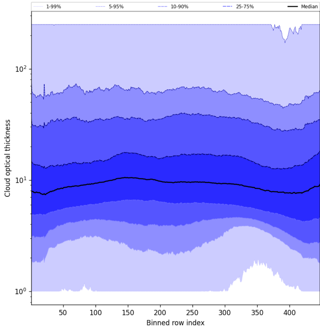
Figure 55: Along track statistics of “Cloud optical thickness” for 2025-02-17 to 2025-02-18
