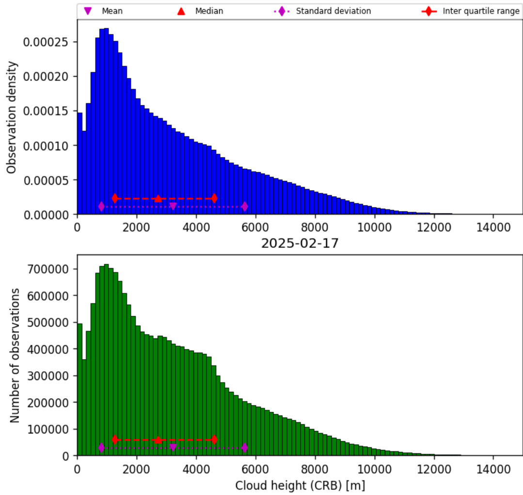
Figure 41: Histogram of “Cloud height (CRB)” for 2025-02-17 to 2025-02-18
