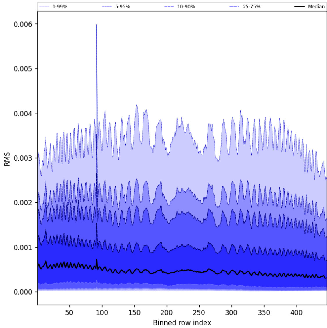
Figure 61: Along track statistics of “RMS” for 2025-02-17 to 2025-02-18
