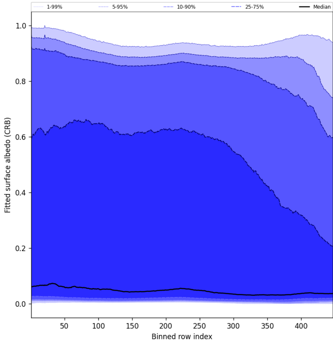
Figure 60: Along track statistics of “Fitted surface albedo (CRB)” for 2025-02-17 to 2025-02-18
