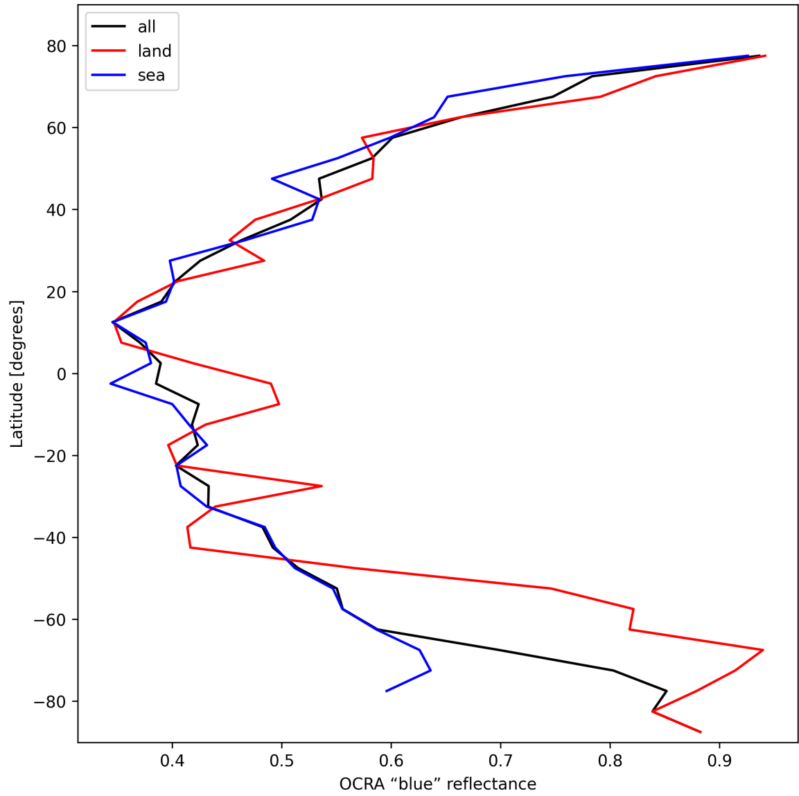
Figure 33: Zonal average of “OCRA “blue” reflectance” for 2025-02-17 to 2025-02-18.
