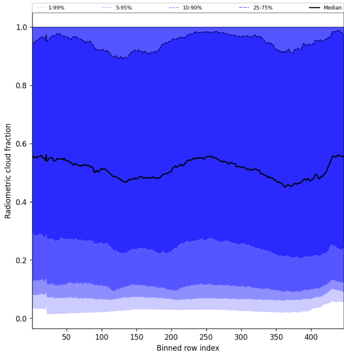
Figure 53: Along track statistics of “Radiometric cloud fraction” for 2025-02-17 to 2025-02-18
