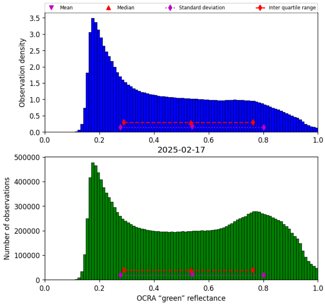
Figure 50: Histogram of “OCRA “green” reflectance” for 2025-02-17 to 2025-02-18
