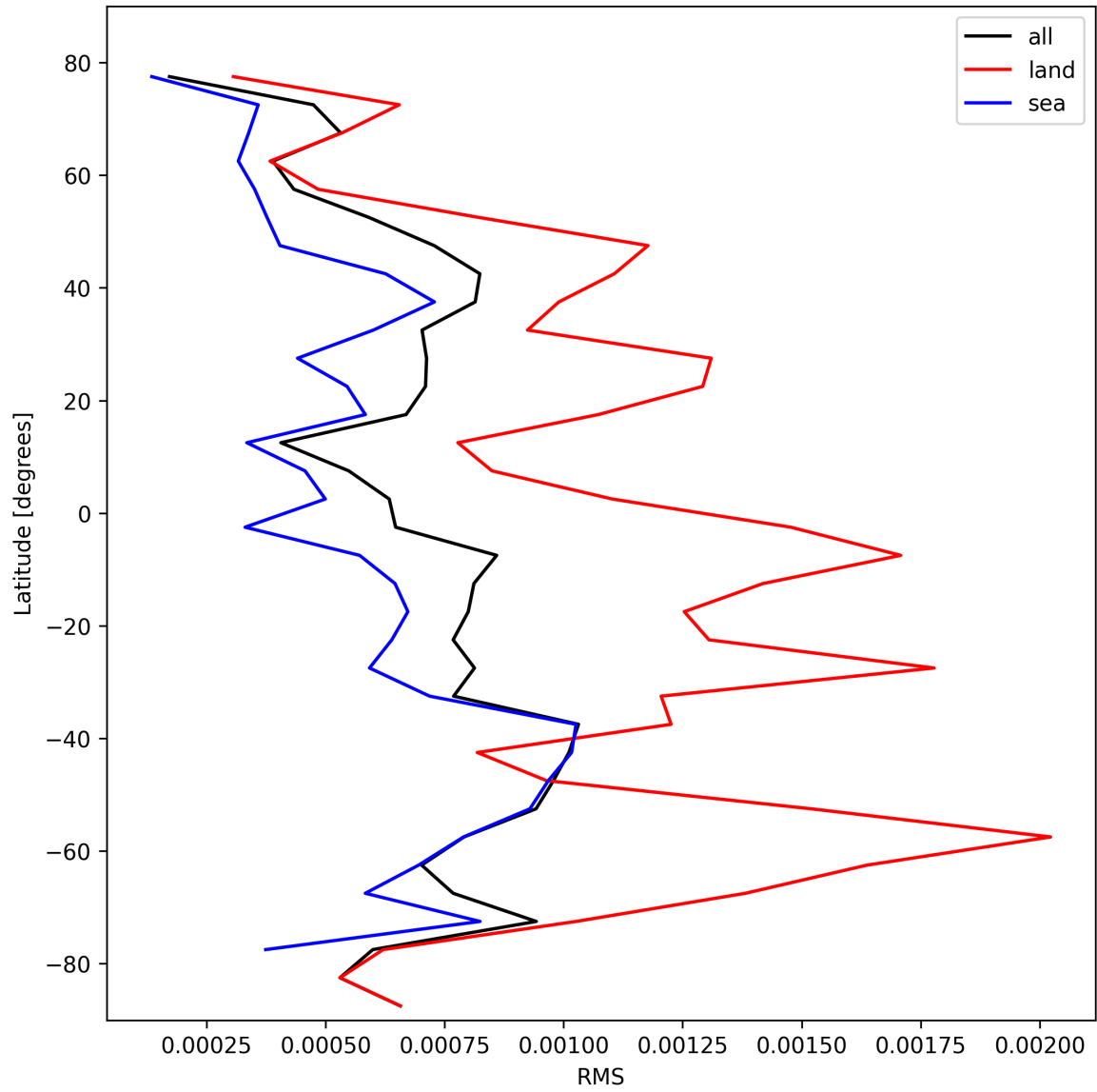
Figure 29: Zonal average of “RMS” for 2025-02-17 to 2025-02-18.
