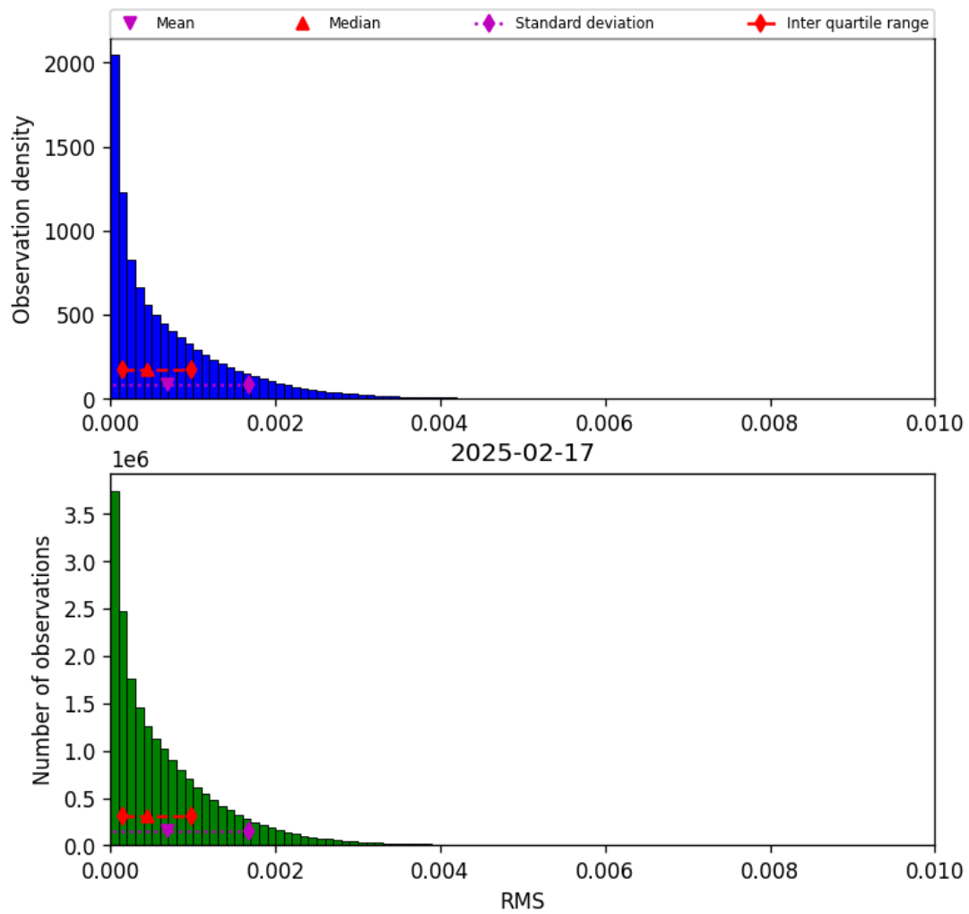
Figure 45: Histogram of “RMS” for 2025-02-17 to 2025-02-18
