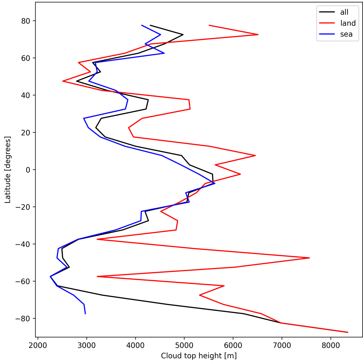
Figure 22: Zonal average of “Cloud top height” for 2025-02-17 to 2025-02-18.
