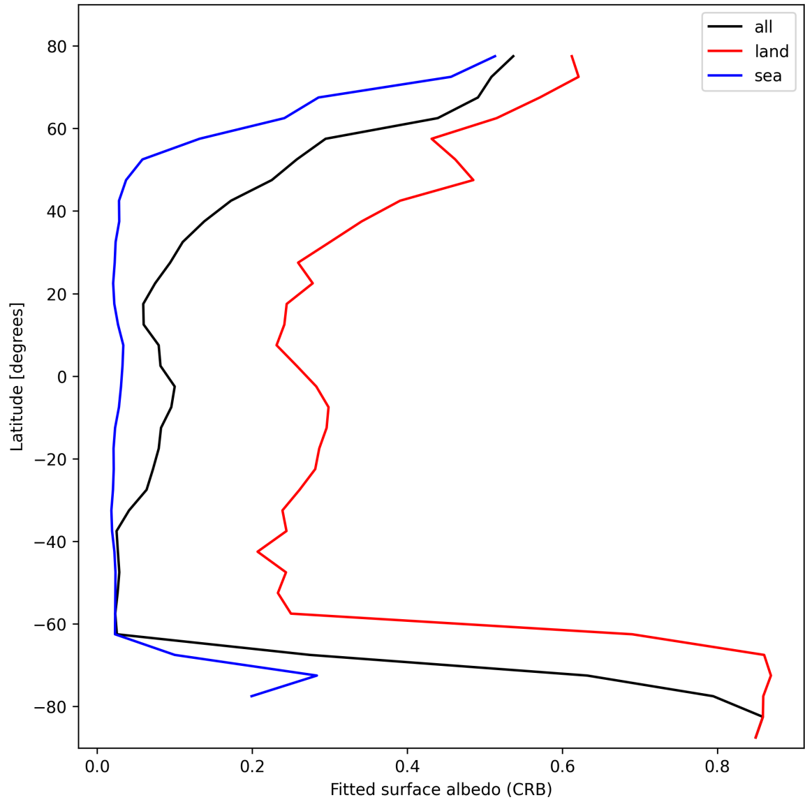
Figure 28: Zonal average of “Fitted surface albedo (CRB)” for 2025-02-17 to 2025-02-18.
