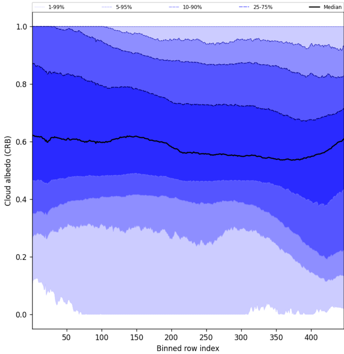
Figure 58: Along track statistics of “Cloud albedo (CRB)” for 2025-02-17 to 2025-02-18
