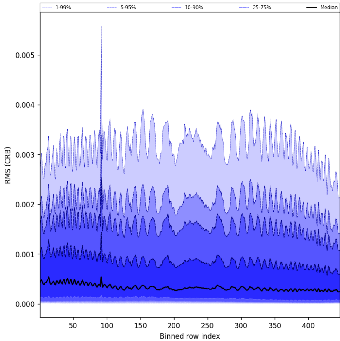
Figure 62: Along track statistics of “RMS (CRB)” for 2025-02-17 to 2025-02-18
