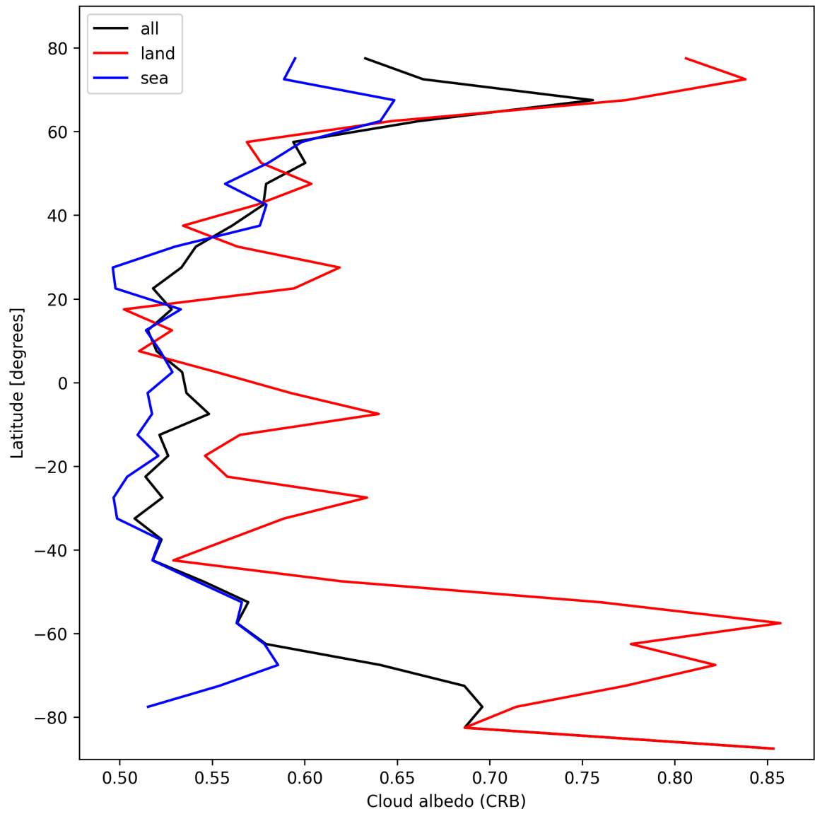
Figure 26: Zonal average of “Cloud albedo (CRB)” for 2025-02-17 to 2025-02-18.
