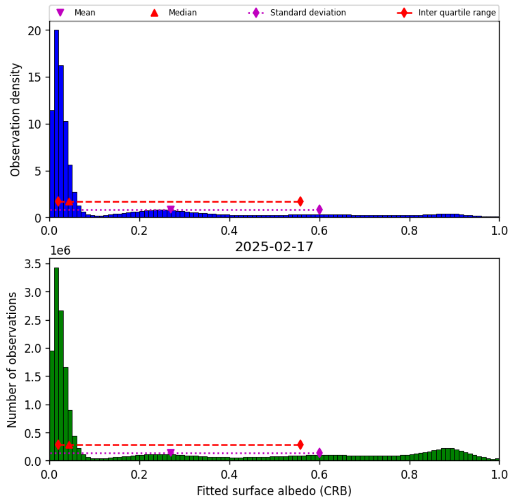
Figure 44: Histogram of “Fitted surface albedo (CRB)” for 2025-02-17 to 2025-02-18
