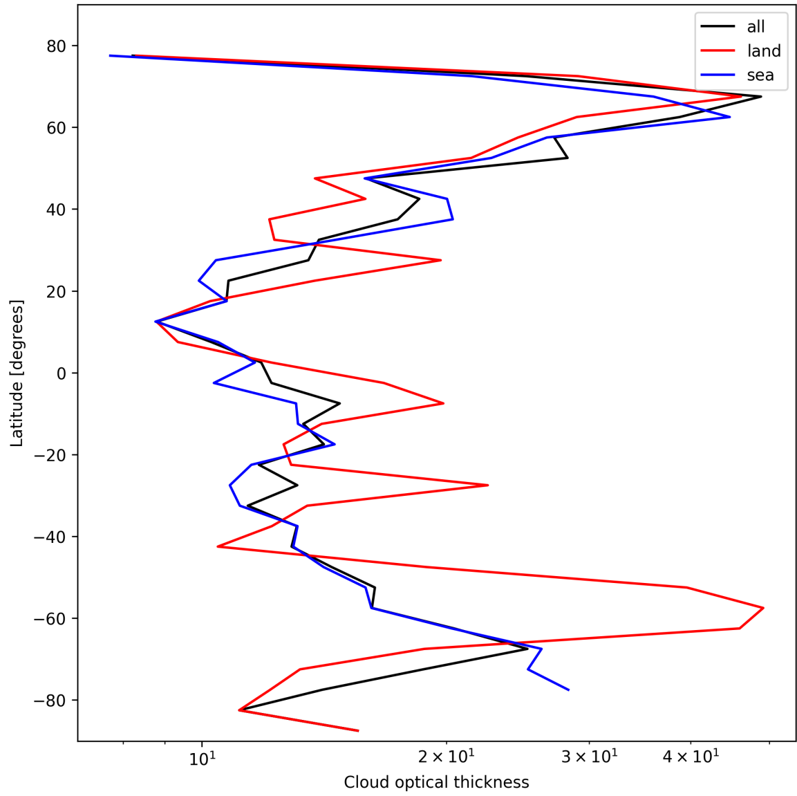
Figure 23: Zonal average of “Cloud optical thickness” for 2025-02-17 to 2025-02-18.
