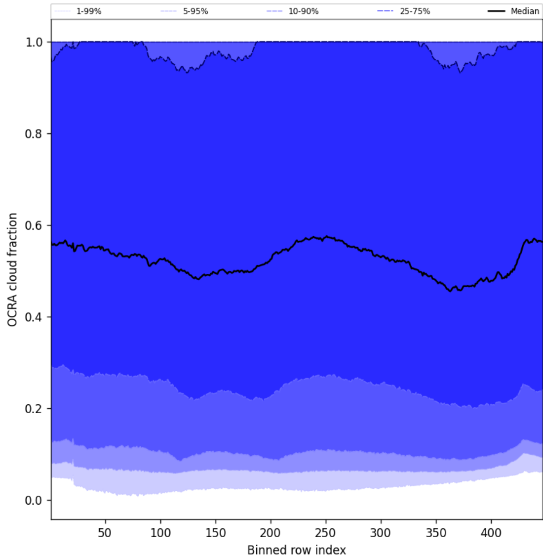
Figure 64: Along track statistics of “OCRA cloud fraction” for 2025-02-17 to 2025-02-18
