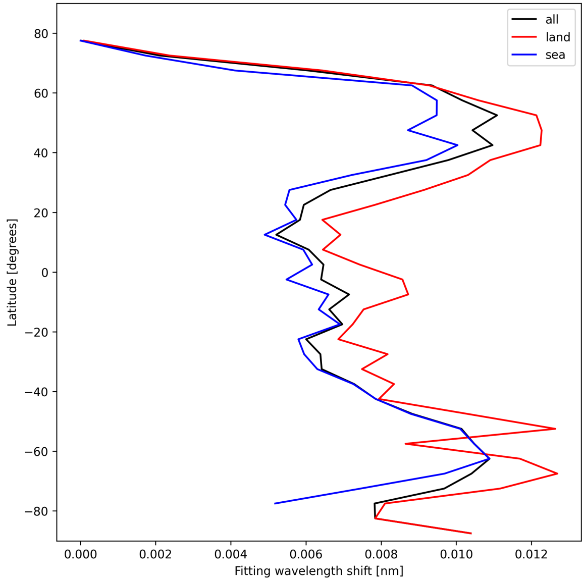
Figure 31: Zonal average of “Fitting wavelength shift” for 2025-02-17 to 2025-02-18.
