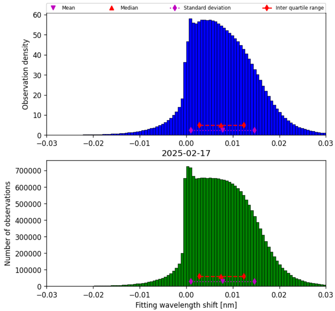
Figure 47: Histogram of “Fitting wavelength shift” for 2025-02-17 to 2025-02-18
