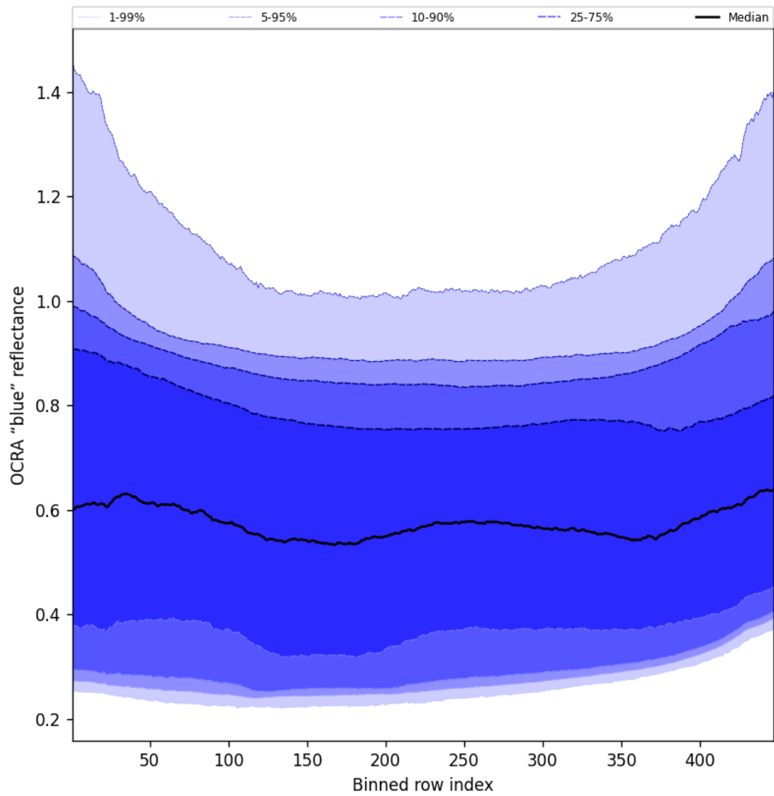
Figure 65: Along track statistics of “OCRA “blue” reflectance” for 2025-02-17 to 2025-02-18
