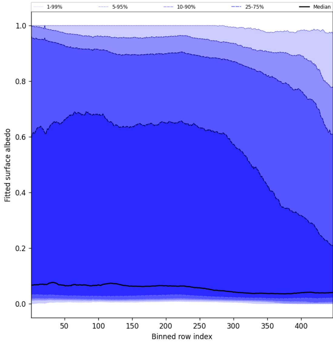
Figure 59: Along track statistics of “Fitted surface albedo” for 2025-02-17 to 2025-02-18
