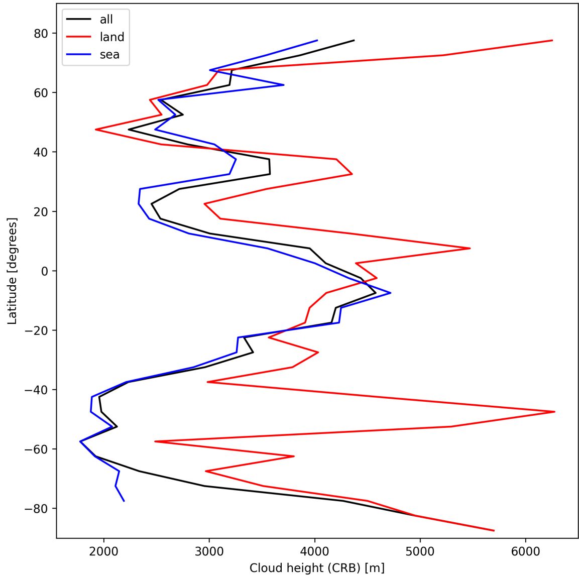
Figure 25: Zonal average of “Cloud height (CRB)” for 2025-02-17 to 2025-02-18.
