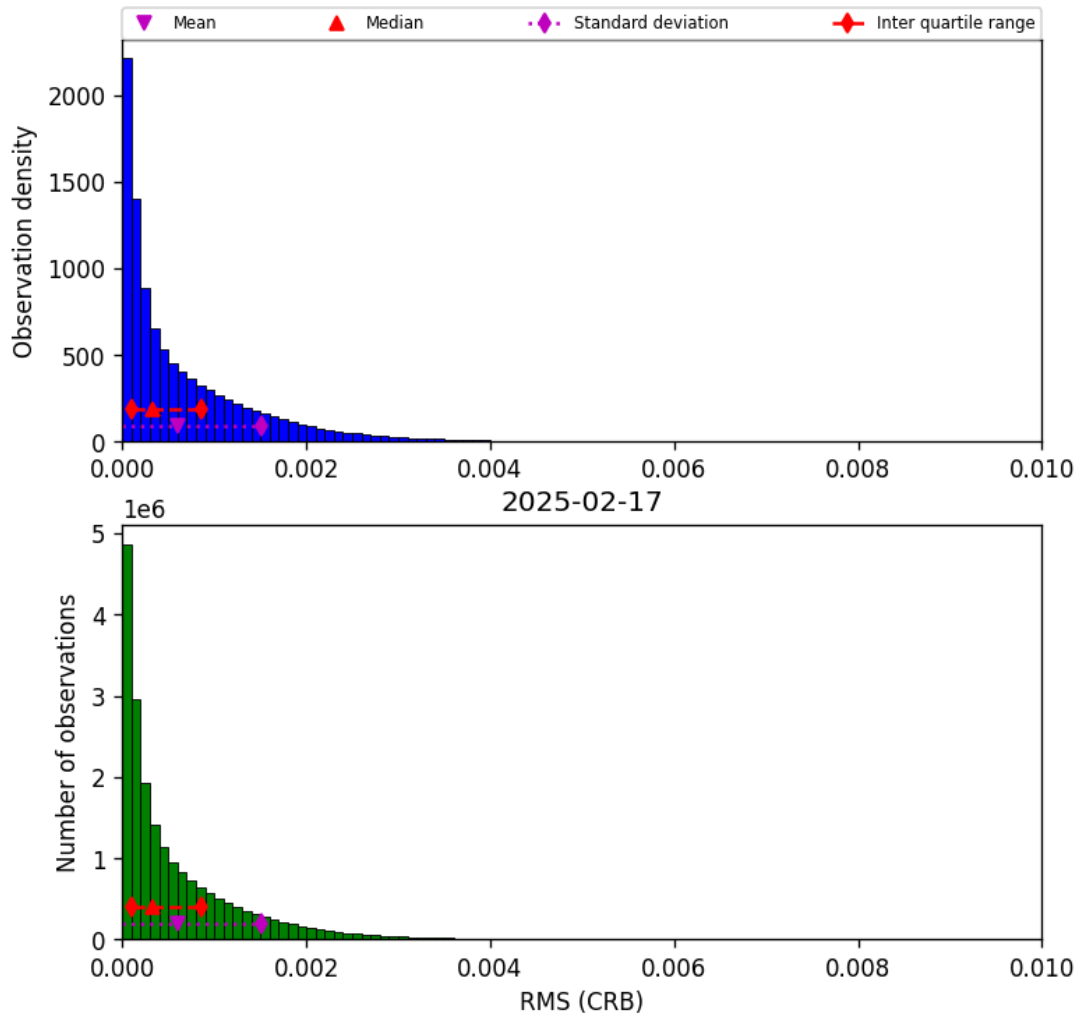
Figure 46: Histogram of "RMS (CRB)" for 2025-02-17 to 2025-02-18
