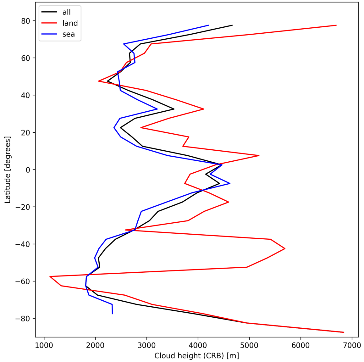
Figure 25: Zonal average of “Cloud height (CRB)” for 2025-02-18 to 2025-02-19.
