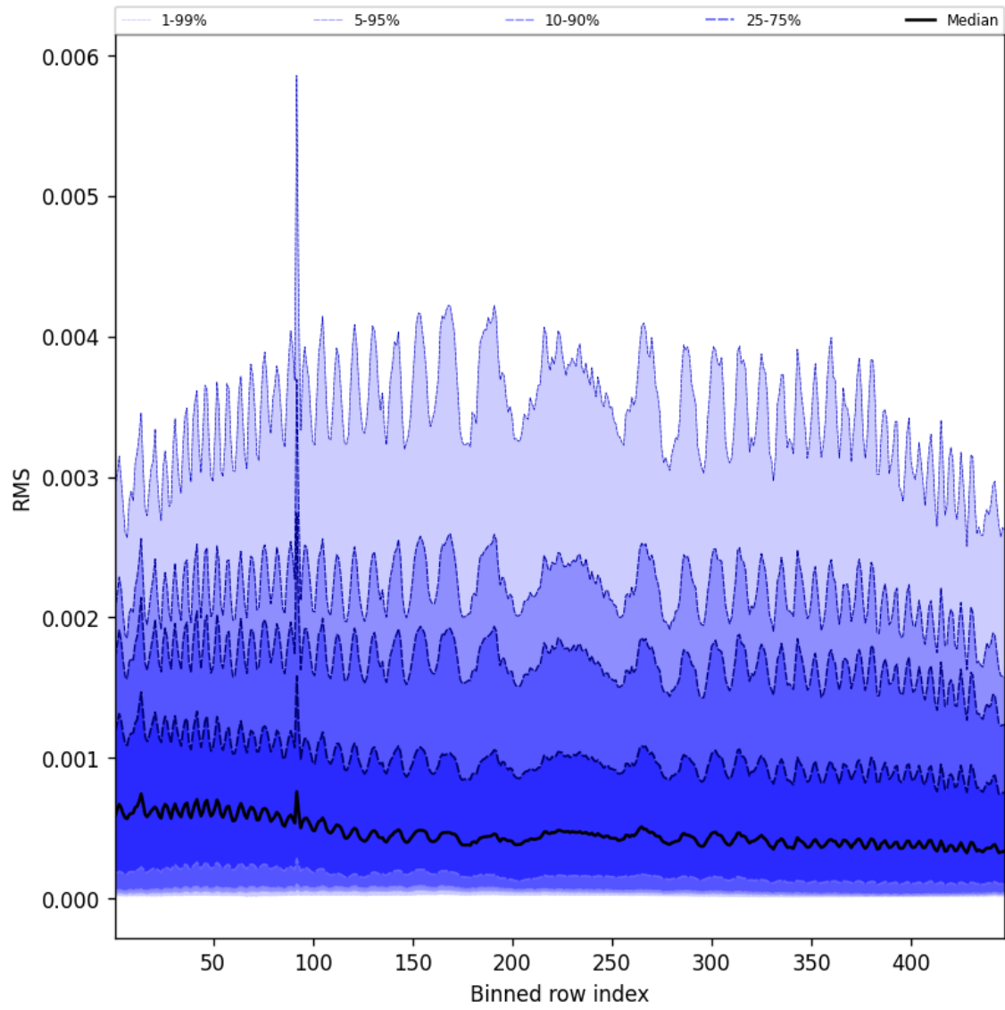
Figure 61: Along track statistics of “RMS” for 2025-02-18 to 2025-02-19
