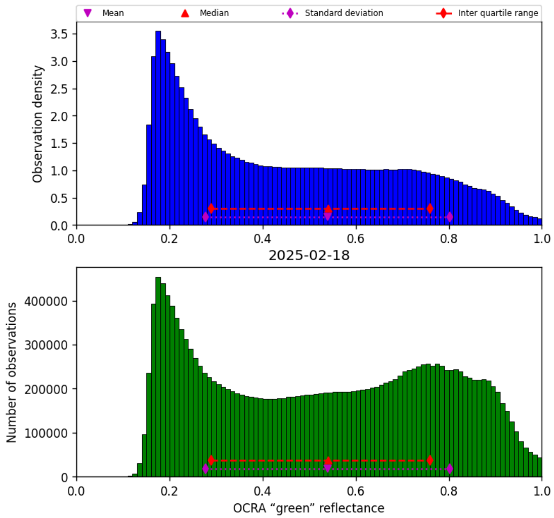
Figure 50: Histogram of “OCRA “green” reflectance” for 2025-02-18 to 2025-02-19
