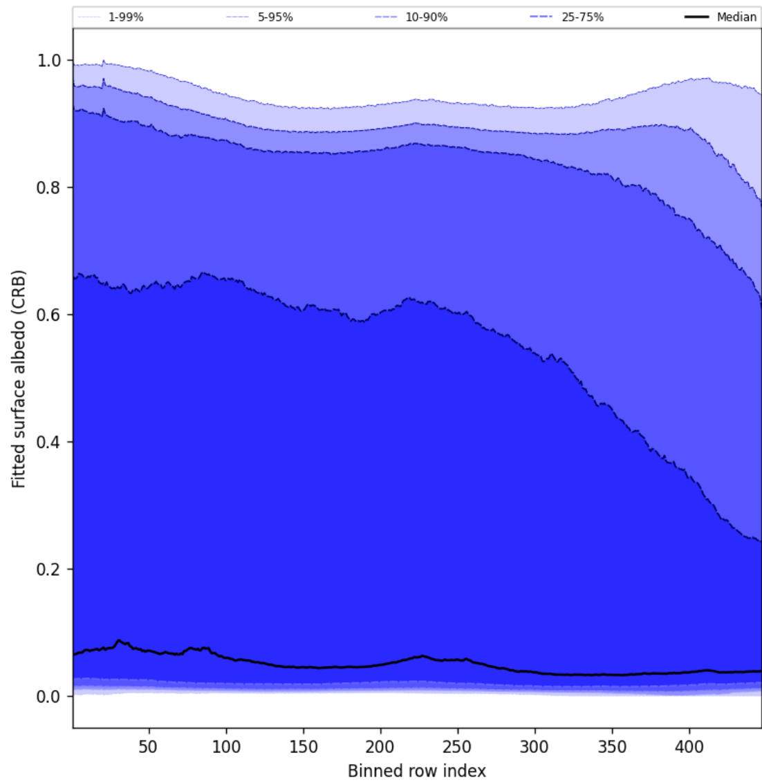
Figure 60: Along track statistics of “Fitted surface albedo (CRB)” for 2025-02-18 to 2025-02-19
