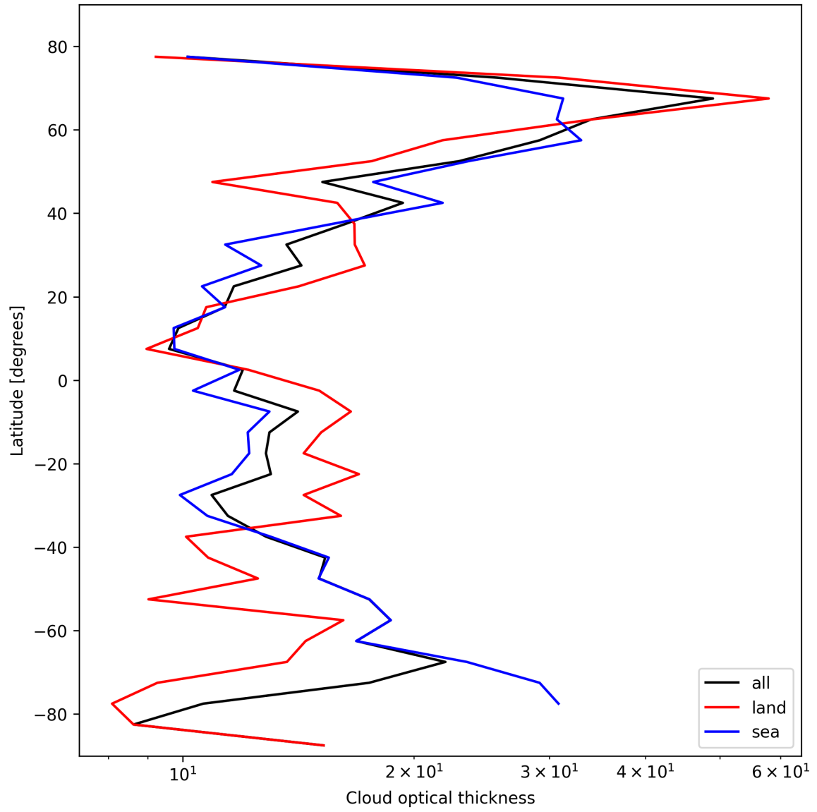
Figure 23: Zonal average of “Cloud optical thickness” for 2025-02-18 to 2025-02-19.
