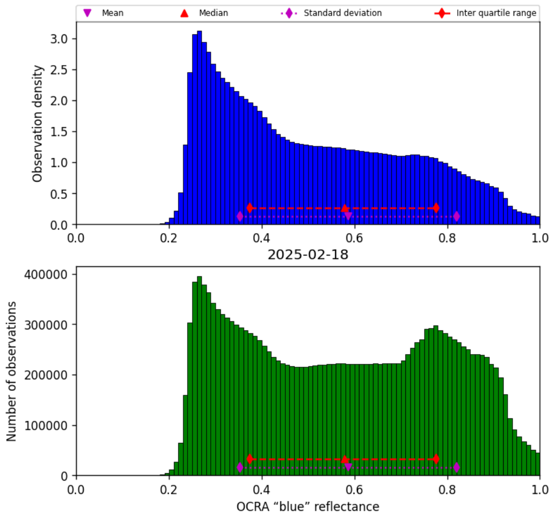
Figure 49: Histogram of “OCRA “blue” reflectance” for 2025-02-18 to 2025-02-19
