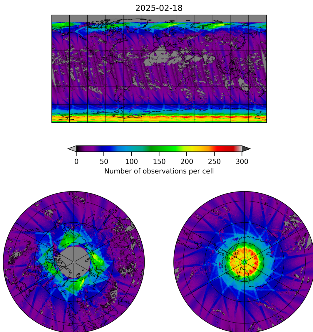
Figure 19: Map of the number of observations for 2025-02-18 to 2025-02-19
