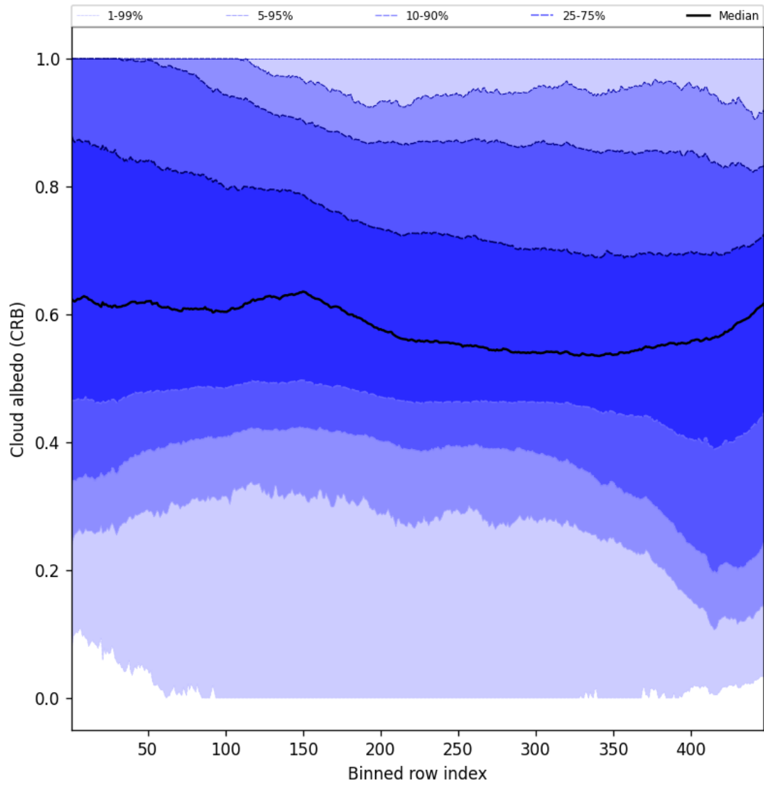
Figure 58: Along track statistics of “Cloud albedo (CRB)” for 2025-02-18 to 2025-02-19
