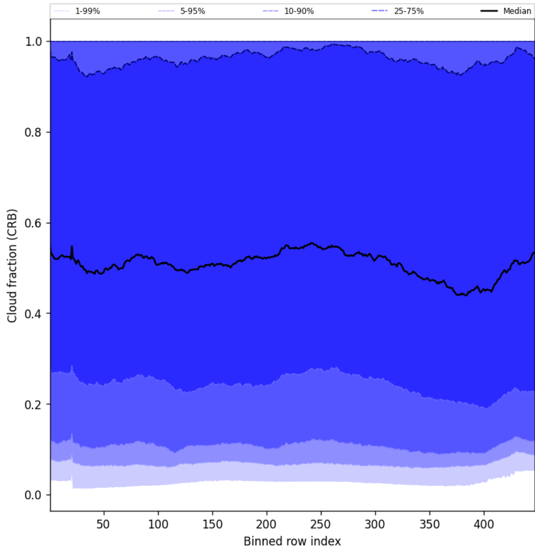
Figure 56: Along track statistics of “Cloud fraction (CRB)” for 2025-02-19 to 2025-02-20
