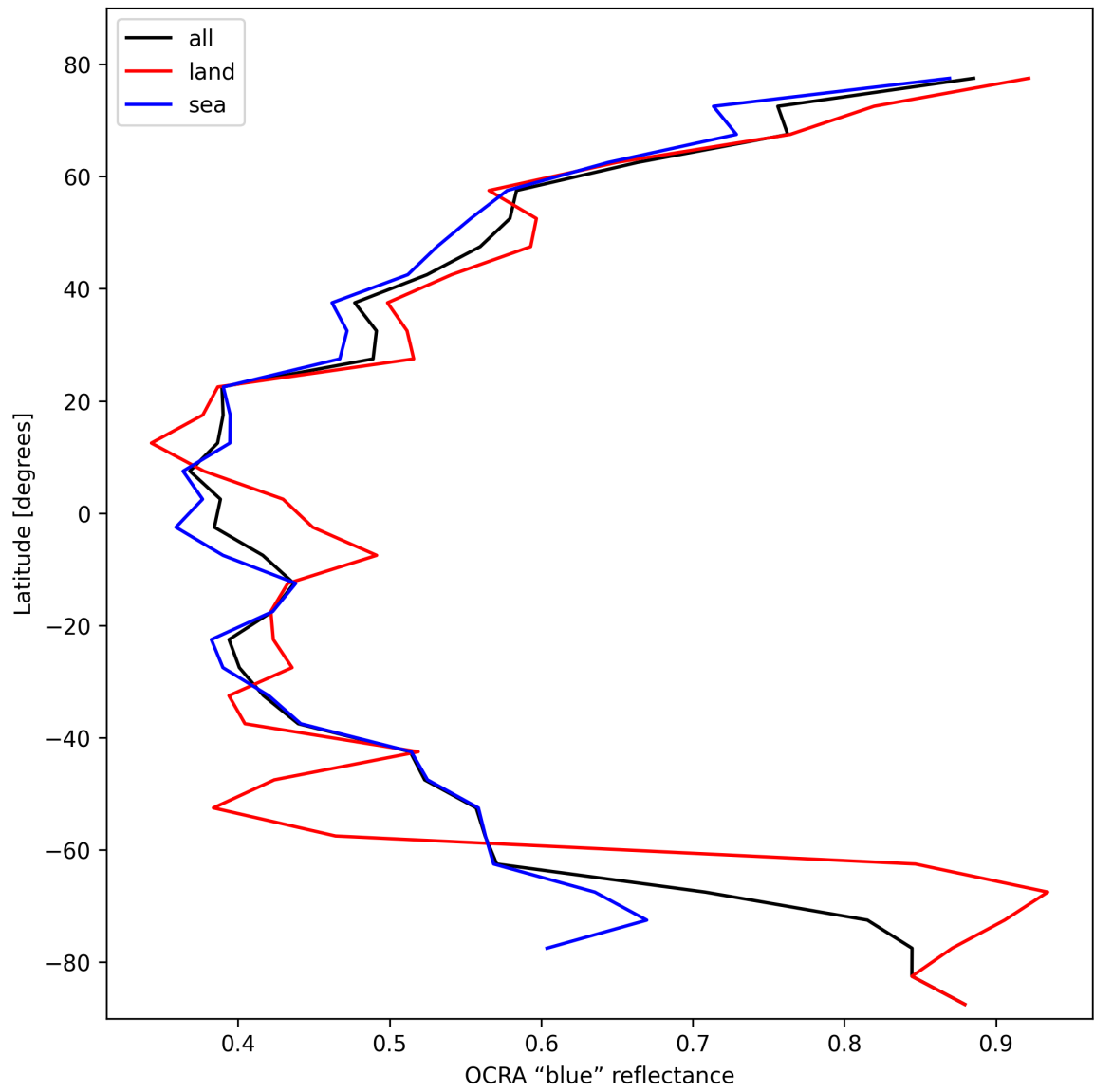
Figure 33: Zonal average of “OCRA “blue” reflectance” for 2025-02-19 to 2025-02-20.
