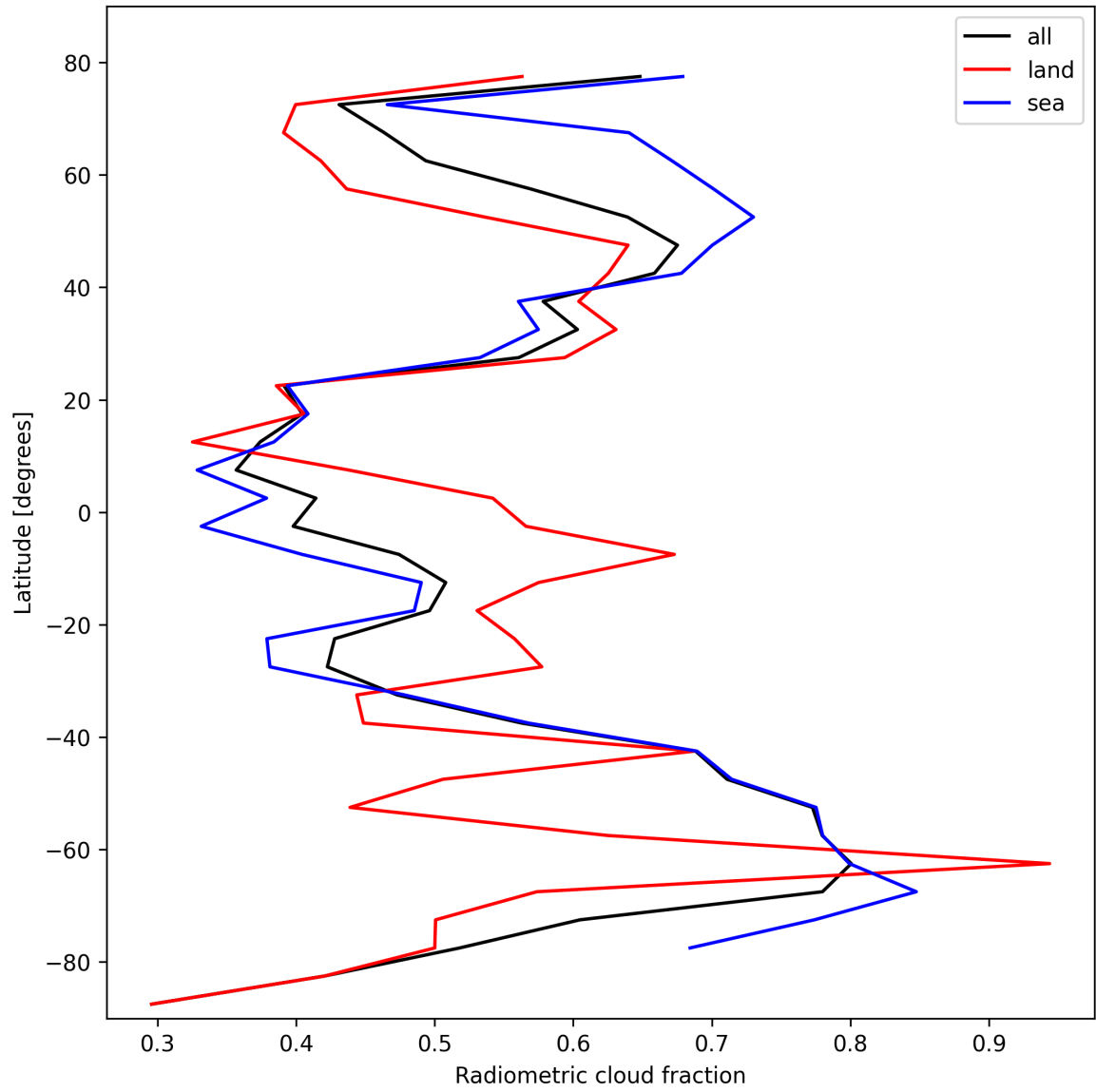
Figure 21: Zonal average of “Radiometric cloud fraction” for 2025-02-19 to 2025-02-20.
