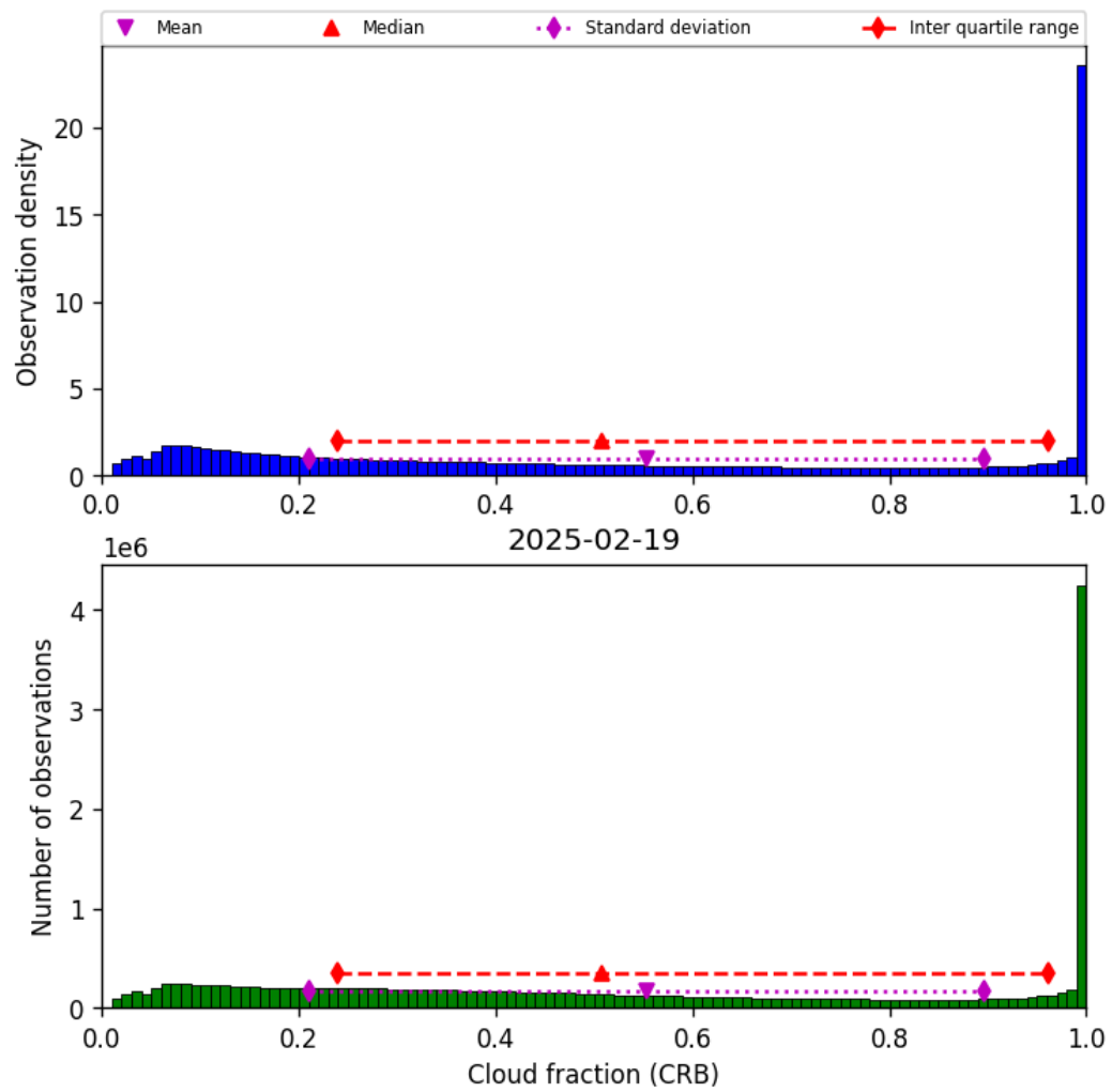
Figure 40: Histogram of “Cloud fraction (CRB)” for 2025-02-19 to 2025-02-20
