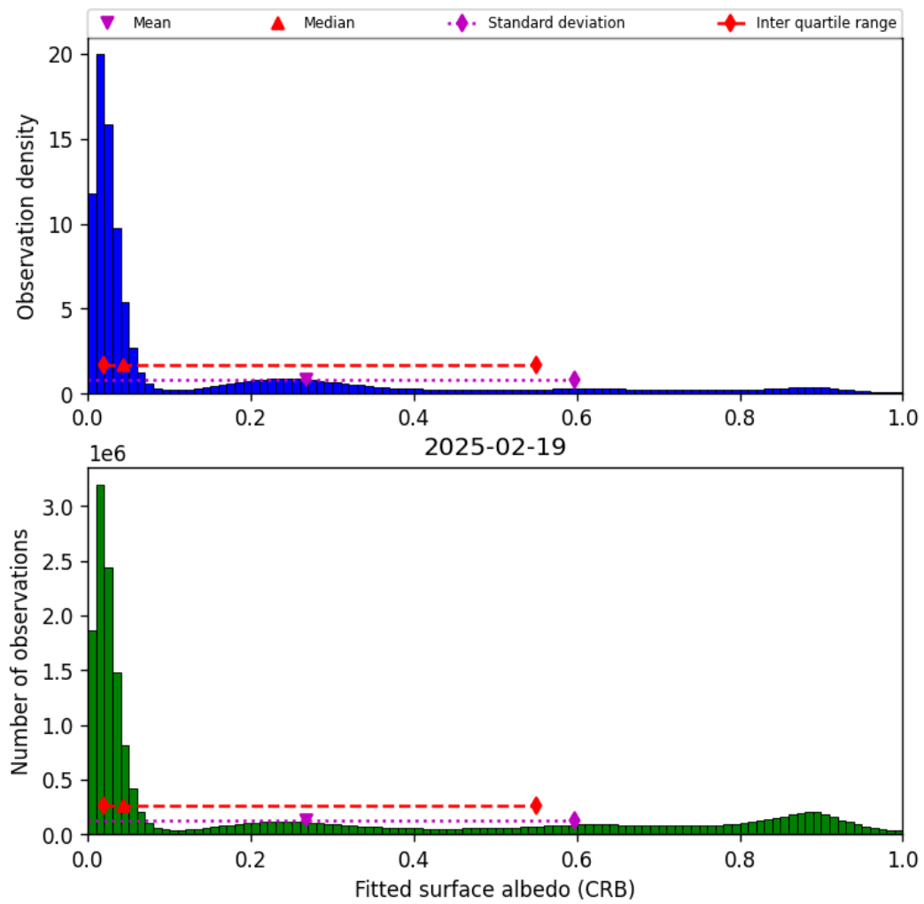
Figure 44: Histogram of “Fitted surface albedo (CRB)” for 2025-02-19 to 2025-02-20
