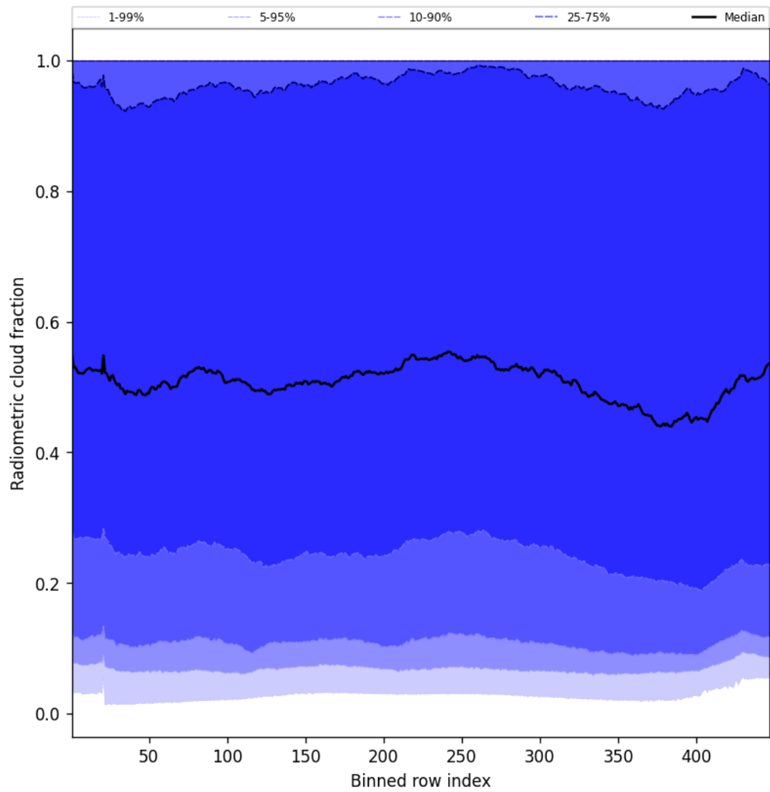
Figure 53: Along track statistics of “Radiometric cloud fraction” for 2025-02-19 to 2025-02-20
