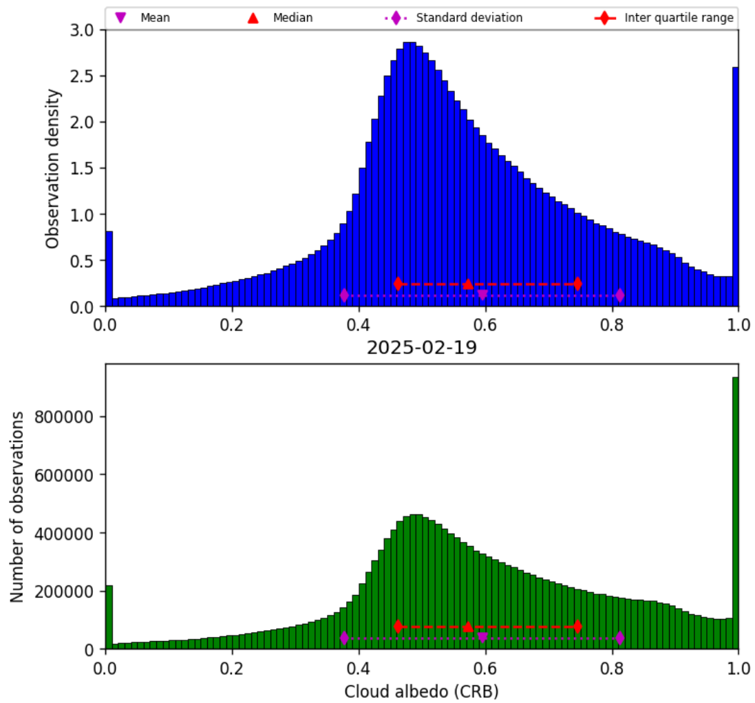
Figure 42: Histogram of “Cloud albedo (CRB)” for 2025-02-19 to 2025-02-20
