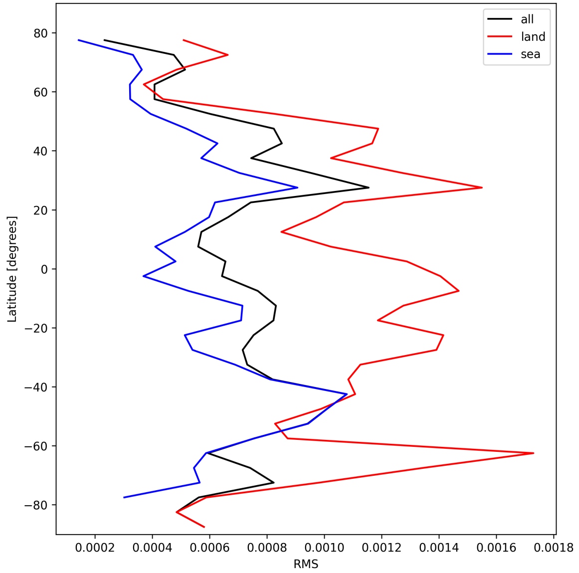
Figure 29: Zonal average of “RMS” for 2025-02-19 to 2025-02-20.
