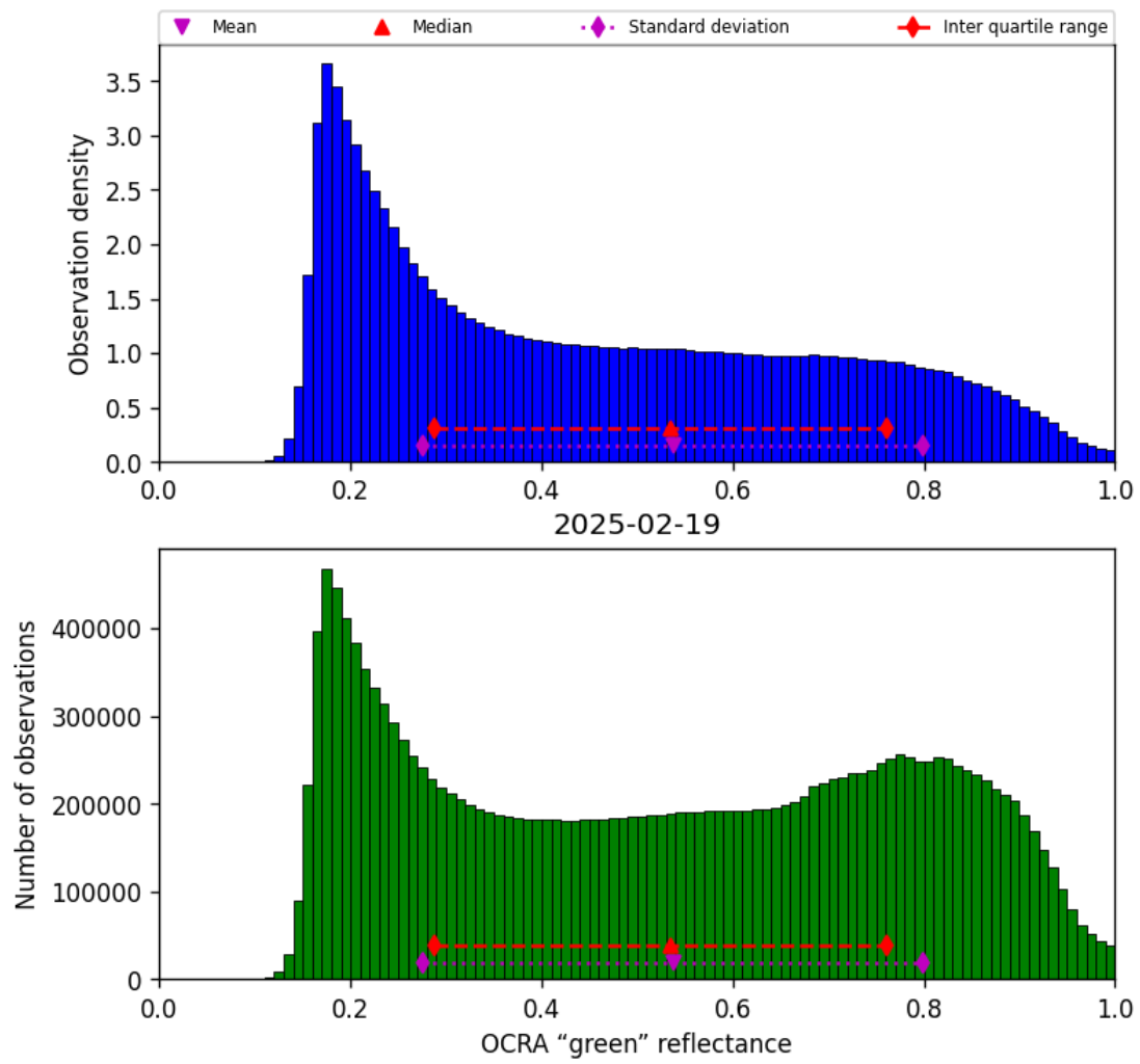
Figure 50: Histogram of “OCRA “green” reflectance” for 2025-02-19 to 2025-02-20
