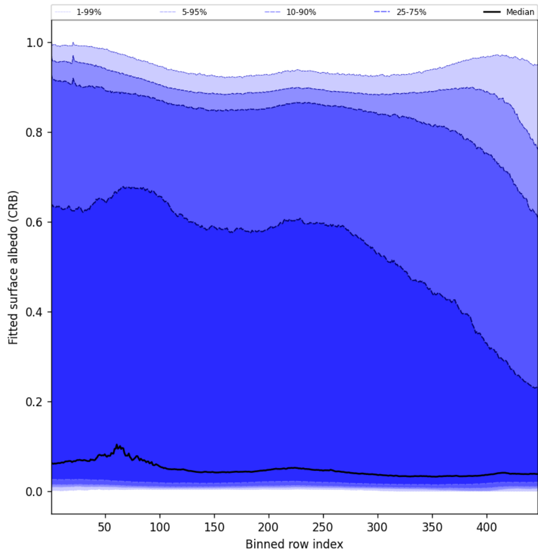
Figure 60: Along track statistics of “Fitted surface albedo (CRB)” for 2025-02-19 to 2025-02-20
