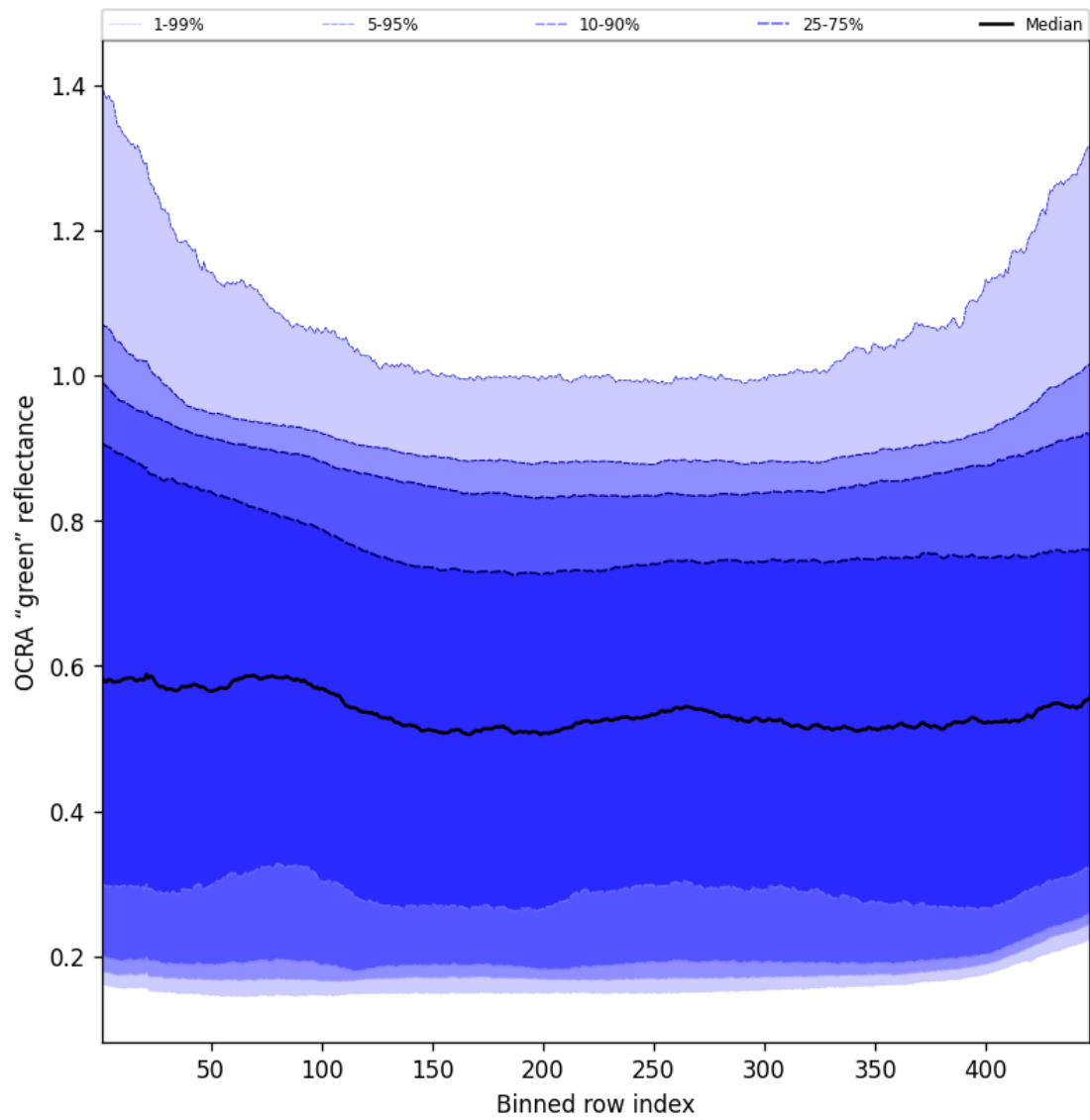
Figure 66: Along track statistics of “OCRA “green” reflectance” for 2025-02-19 to 2025-02-20
