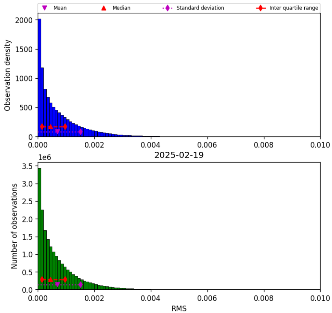
Figure 45: Histogram of “RMS” for 2025-02-19 to 2025-02-20
