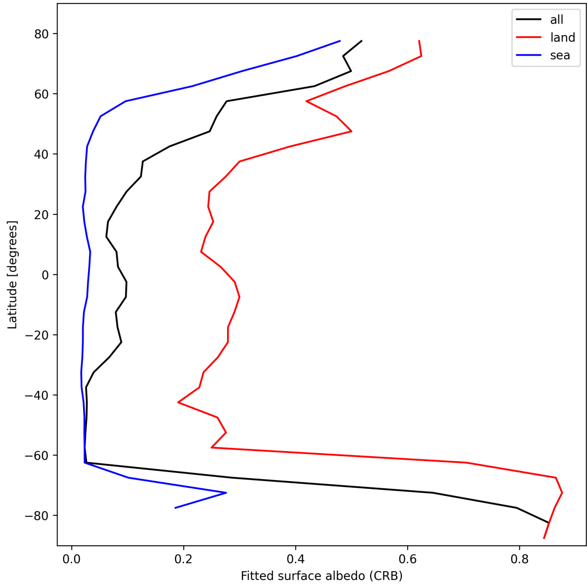
Figure 28: Zonal average of “Fitted surface albedo (CRB)” for 2025-02-19 to 2025-02-20.
