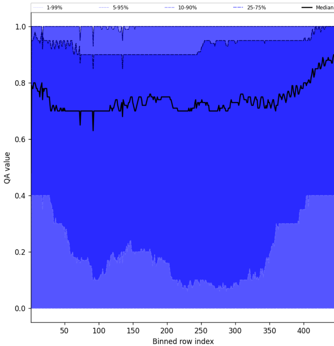
Figure 52: Along track statistics of “QA value” for 2025-02-19 to 2025-02-20
