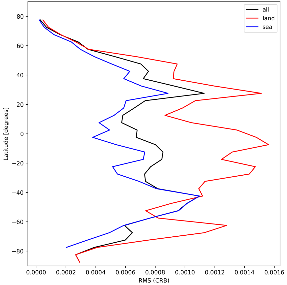
Figure 30: Zonal average of “RMS (CRB)” for 2025-02-19 to 2025-02-20.
