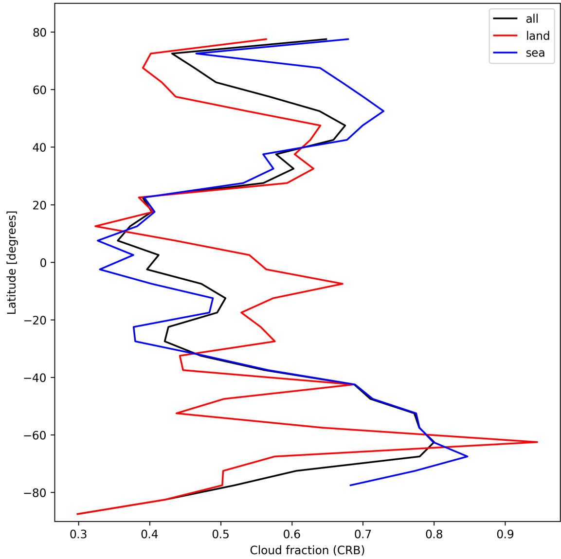
Figure 24: Zonal average of “Cloud fraction (CRB)” for 2025-02-19 to 2025-02-20.
