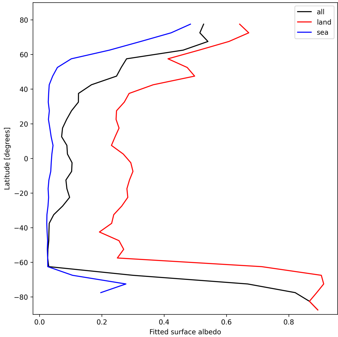
Figure 27: Zonal average of “Fitted surface albedo” for 2025-02-19 to 2025-02-20.
