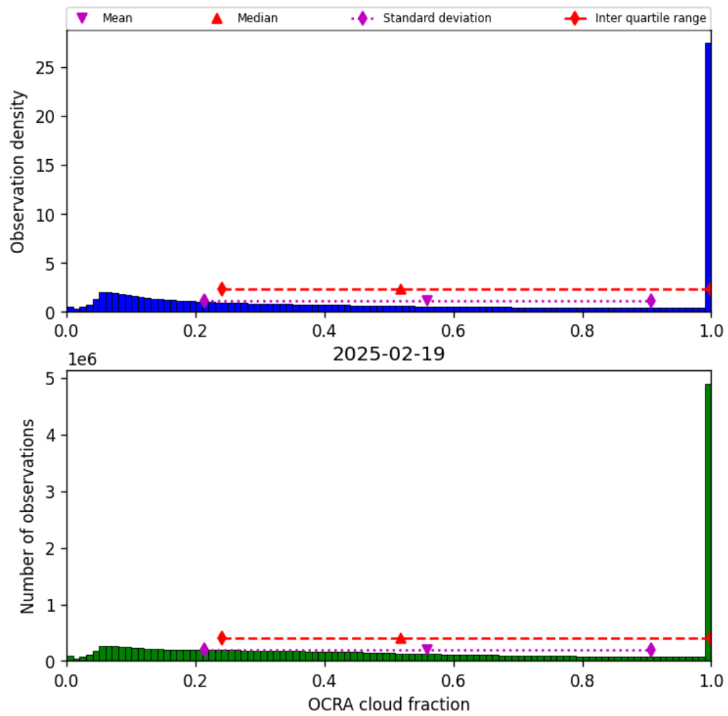
Figure 48: Histogram of “OCRA cloud fraction” for 2025-02-19 to 2025-02-20
