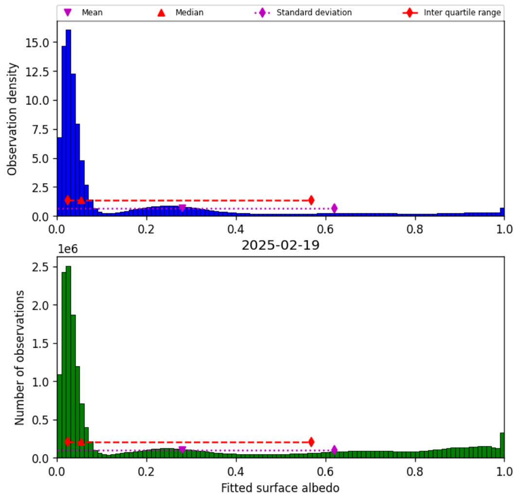
Figure 43: Histogram of “Fitted surface albedo” for 2025-02-19 to 2025-02-20
