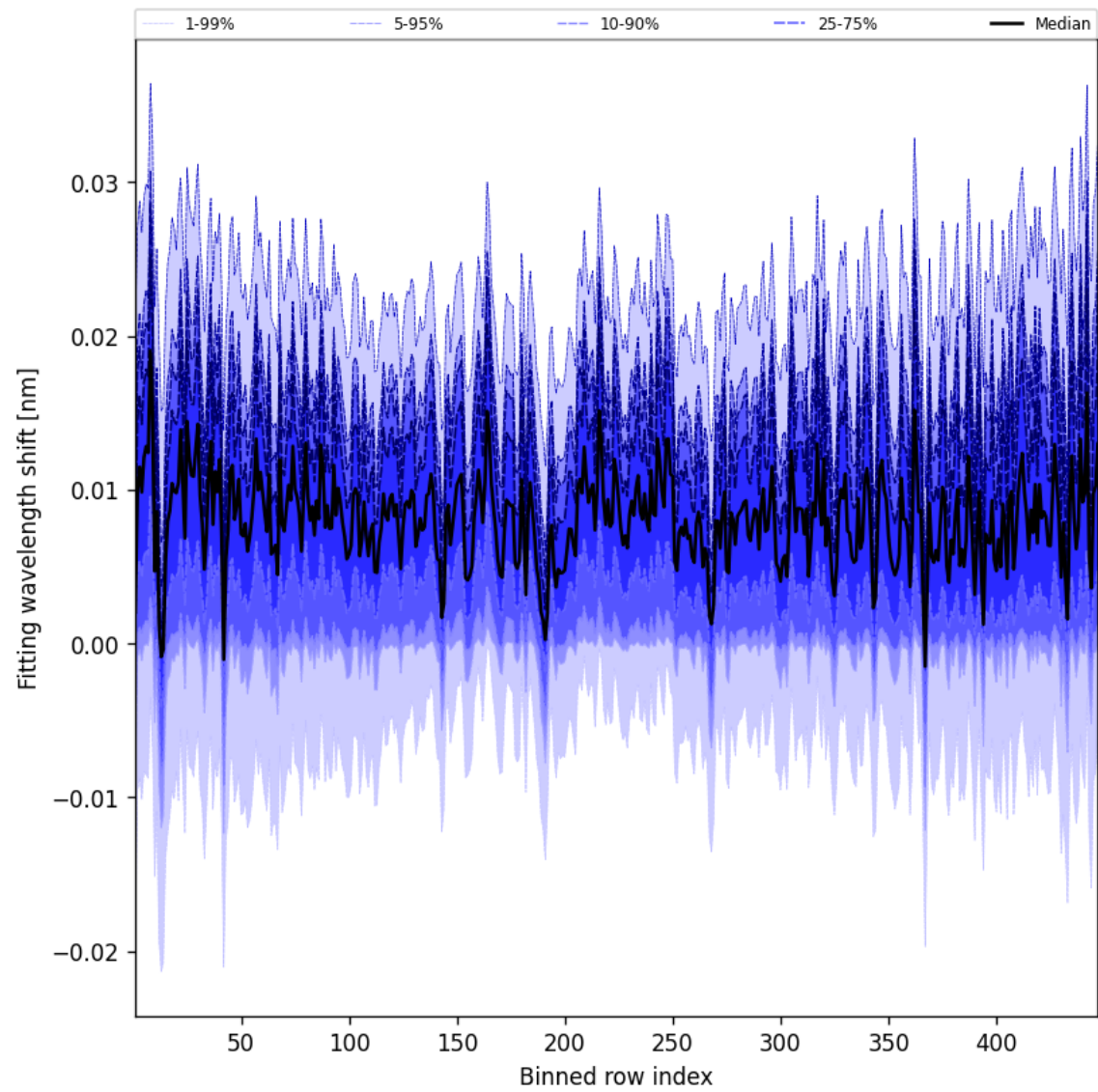
Figure 63: Along track statistics of “Fitting wavelength shift” for 2025-02-19 to 2025-02-20
