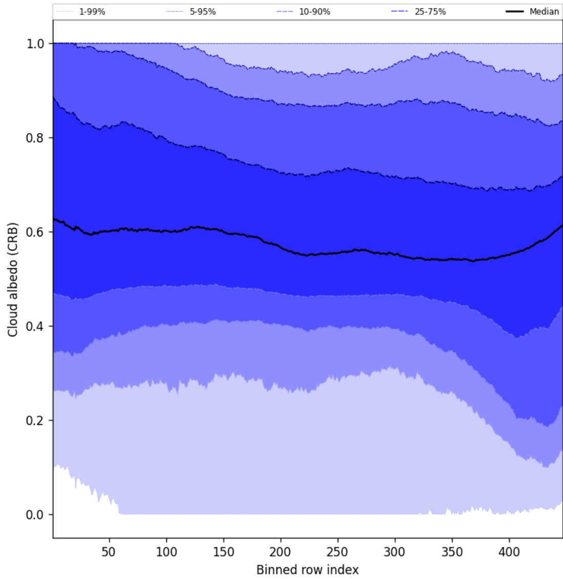
Figure 58: Along track statistics of “Cloud albedo (CRB)” for 2025-02-19 to 2025-02-20
