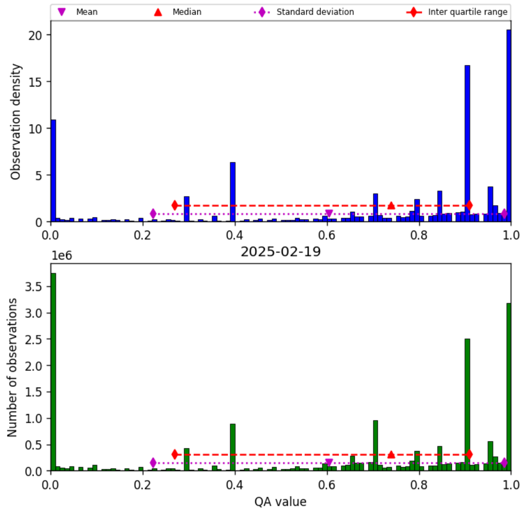
Figure 36: Histogram of “QA value” for 2025-02-19 to 2025-02-20
