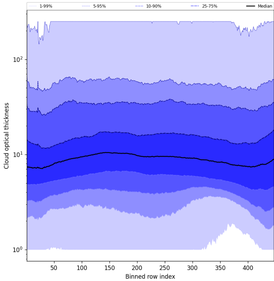
Figure 55: Along track statistics of “Cloud optical thickness” for 2025-02-19 to 2025-02-20
