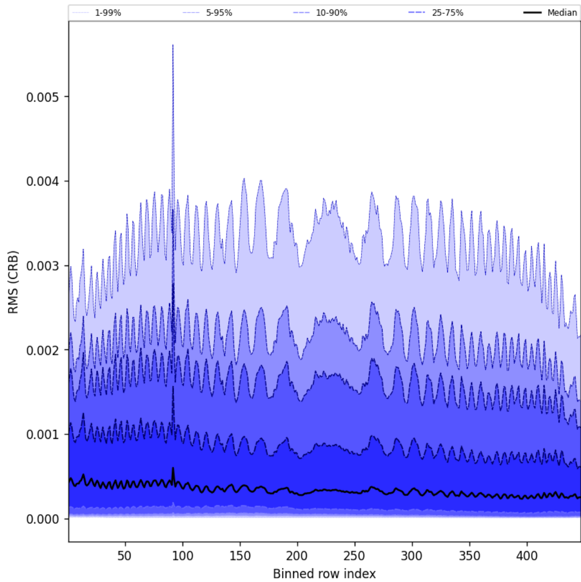
Figure 62: Along track statistics of “RMS (CRB)” for 2025-02-19 to 2025-02-20
