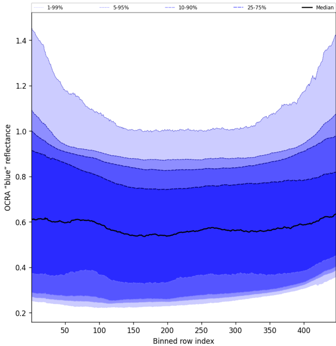
Figure 65: Along track statistics of “OCRA “blue” reflectance” for 2025-02-19 to 2025-02-20
