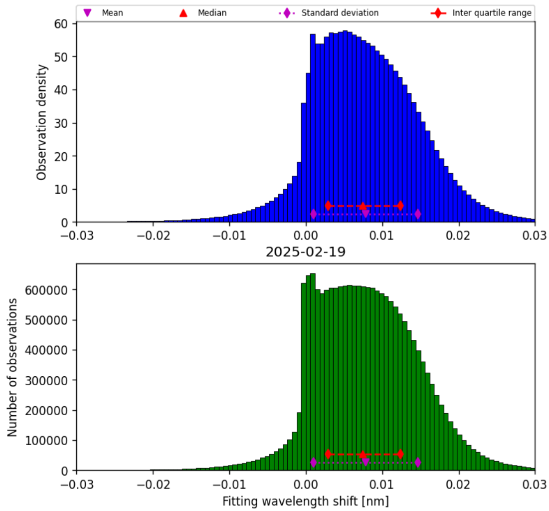
Figure 47: Histogram of “Fitting wavelength shift” for 2025-02-19 to 2025-02-20
