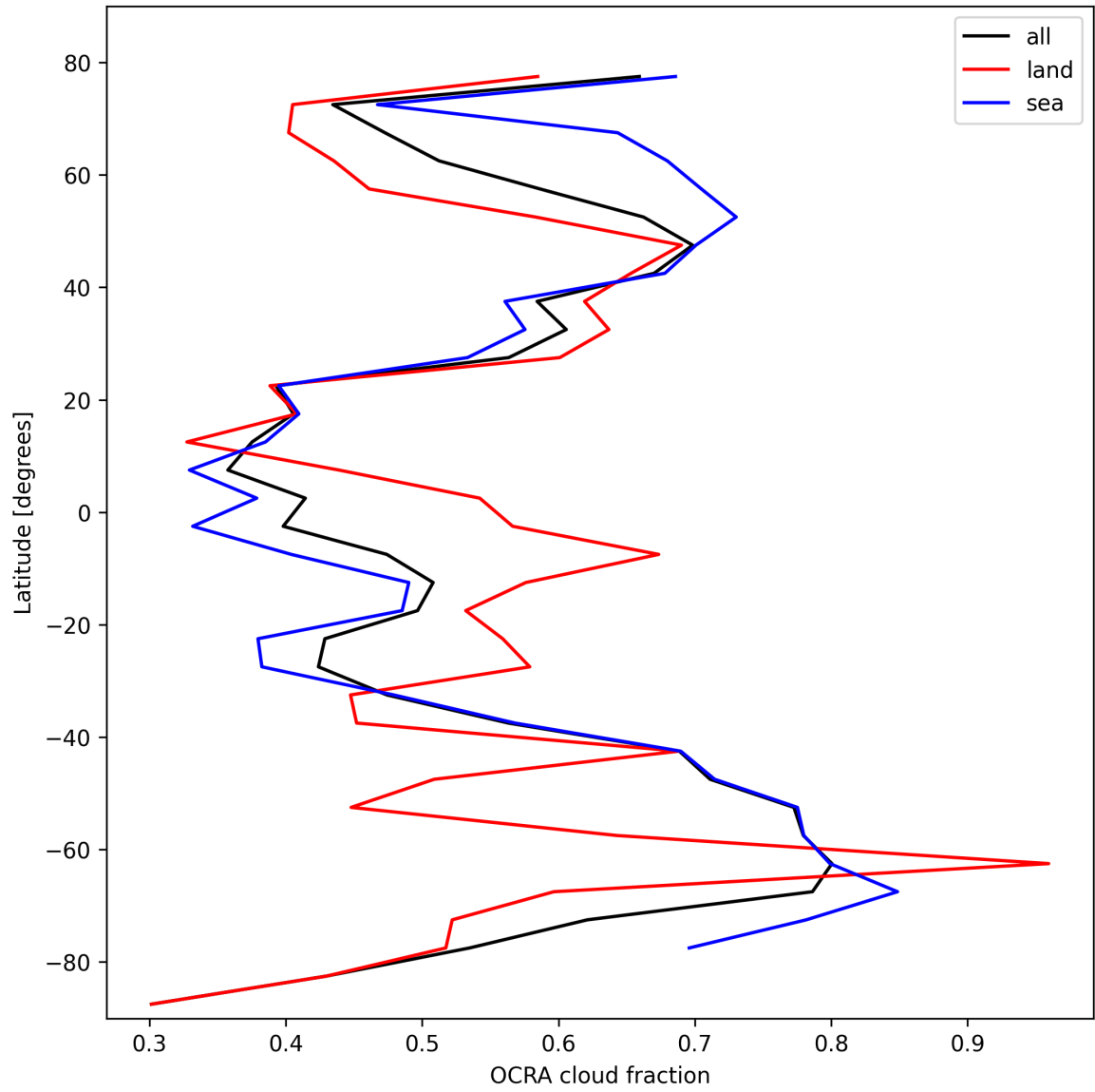
Figure 32: Zonal average of “OCRA cloud fraction” for 2025-02-19 to 2025-02-20.
