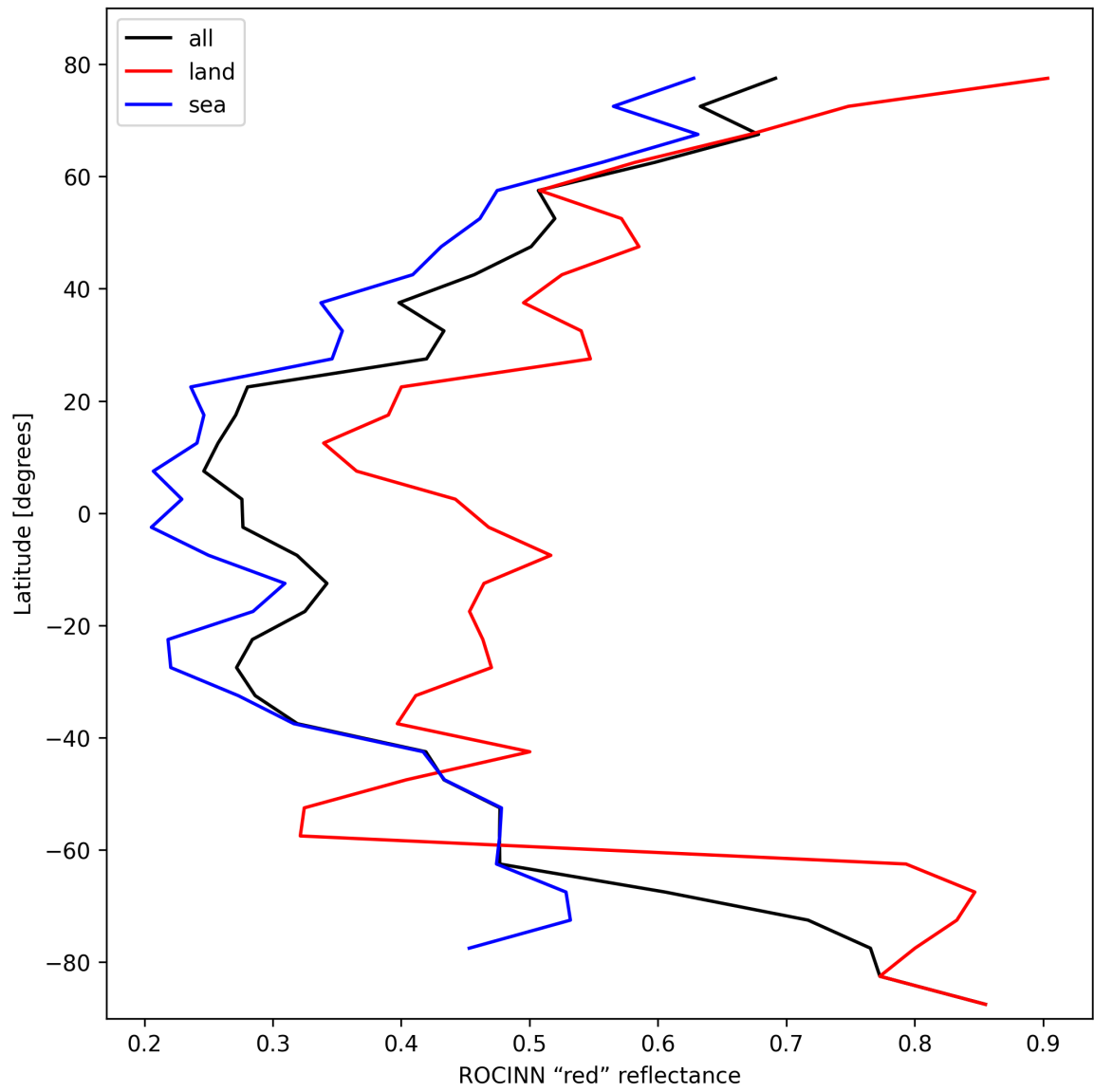
Figure 35: Zonal average of “ROCINN “red” reflectance” for 2025-02-19 to 2025-02-20.
