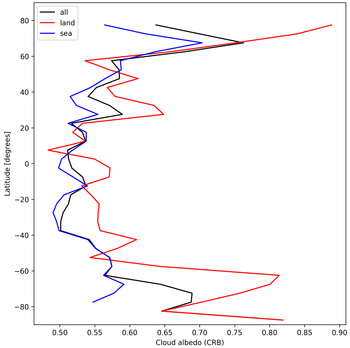
Figure 26: Zonal average of “Cloud albedo (CRB)” for 2025-02-19 to 2025-02-20.
