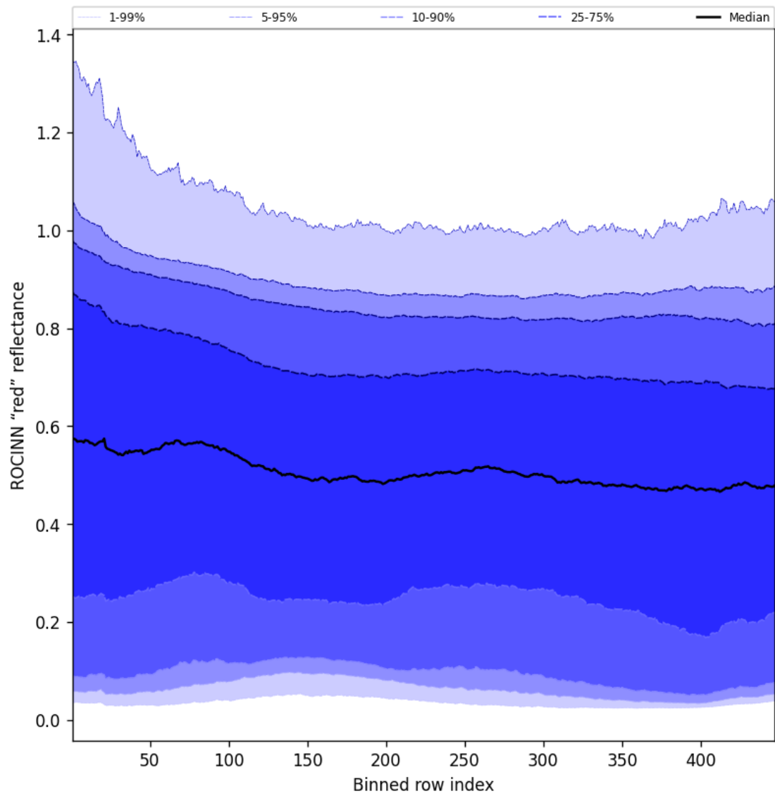
Figure 67: Along track statistics of “ROCINN “red” reflectance” for 2025-02-19 to 2025-02-20
