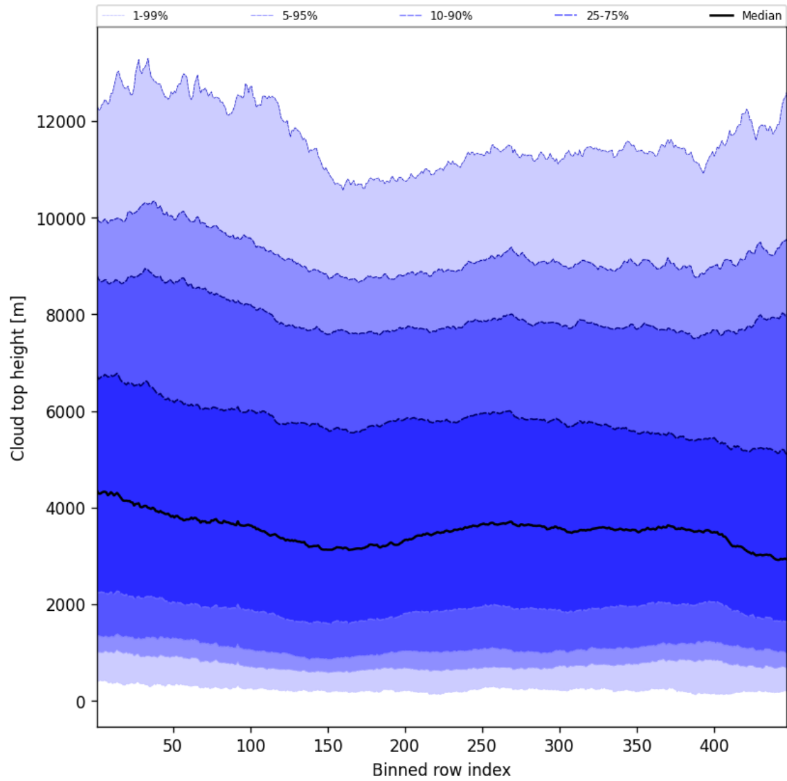
Figure 54: Along track statistics of “Cloud top height” for 2025-02-19 to 2025-02-20
