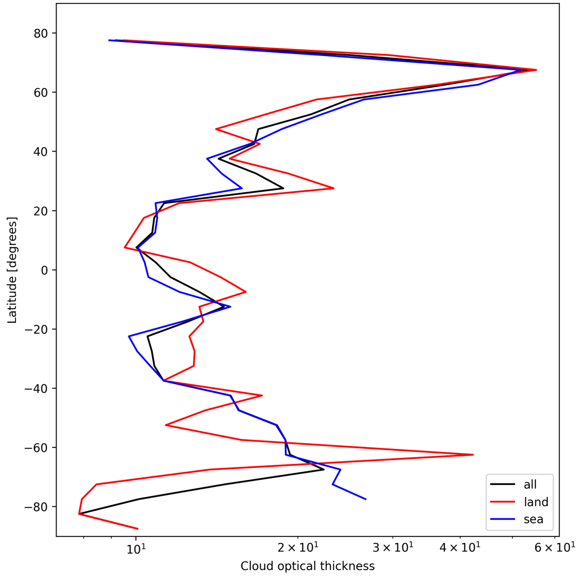
Figure 23: Zonal average of “Cloud optical thickness” for 2025-02-19 to 2025-02-20.
