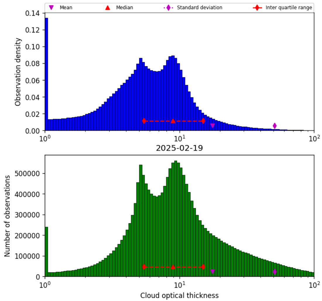
Figure 39: Histogram of “Cloud optical thickness” for 2025-02-19 to 2025-02-20
