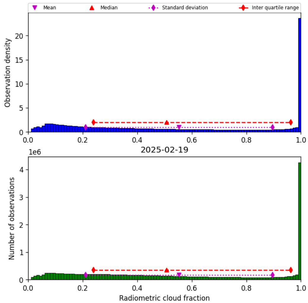
Figure 37: Histogram of “Radiometric cloud fraction” for 2025-02-19 to 2025-02-20
