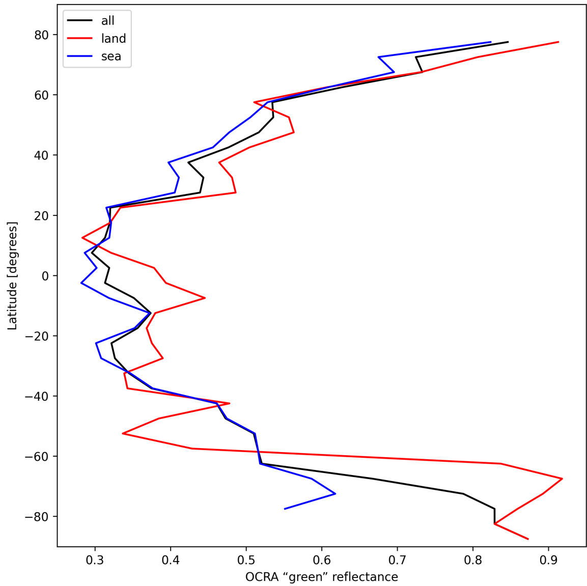
Figure 34: Zonal average of “OCRA “green” reflectance” for 2025-02-19 to 2025-02-20.
