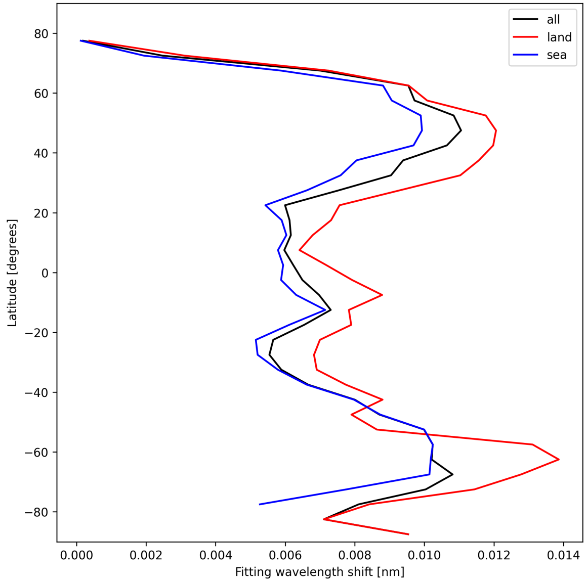
Figure 31: Zonal average of “Fitting wavelength shift” for 2025-02-19 to 2025-02-20.
