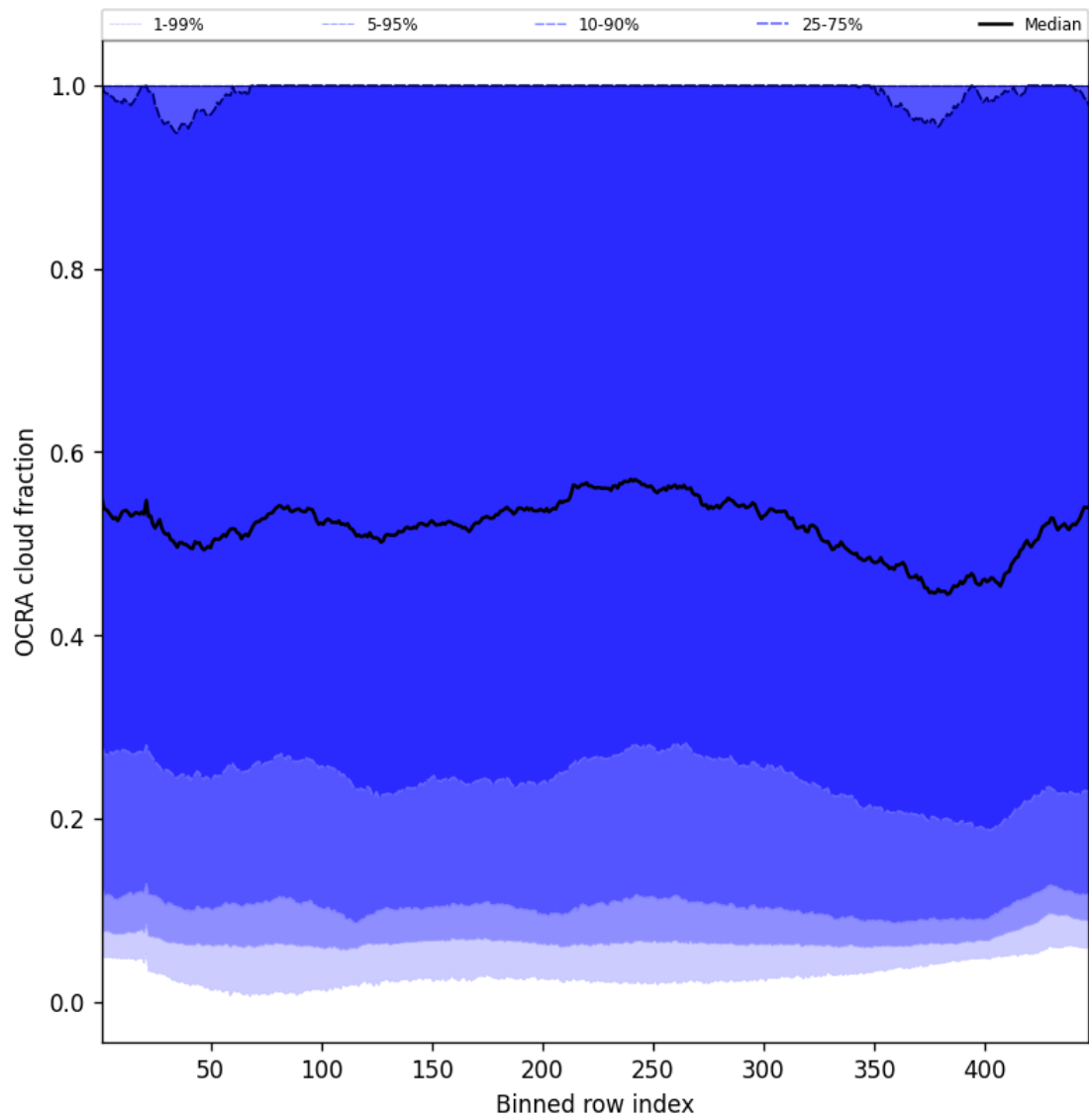
Figure 64: Along track statistics of “OCRA cloud fraction” for 2025-02-19 to 2025-02-20
