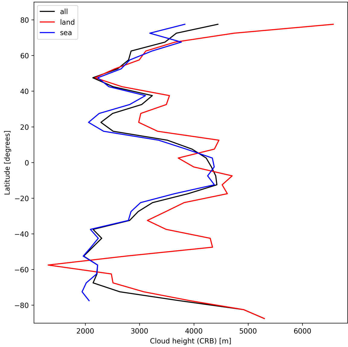
Figure 25: Zonal average of “Cloud height (CRB)” for 2025-02-19 to 2025-02-20.
