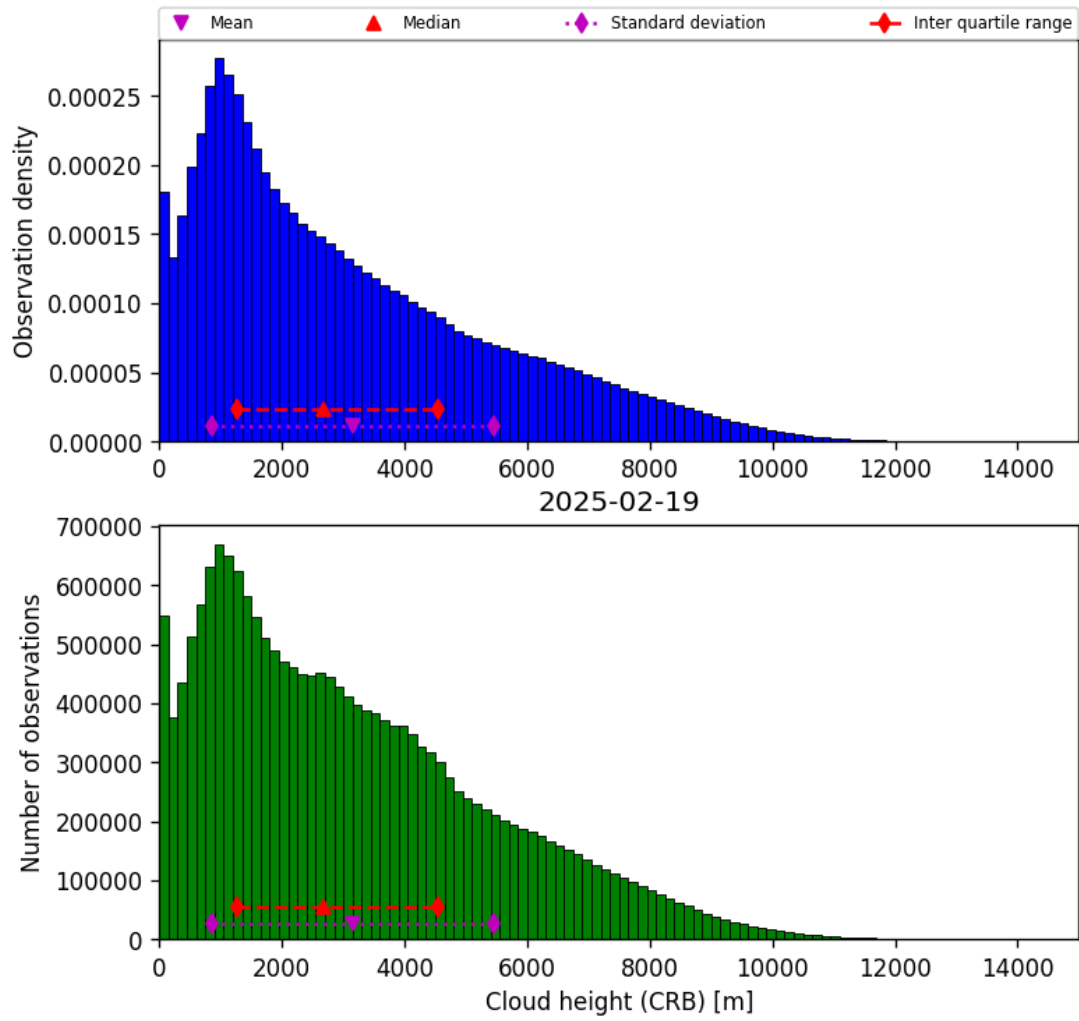
Figure 41: Histogram of “Cloud height (CRB)” for 2025-02-19 to 2025-02-20
