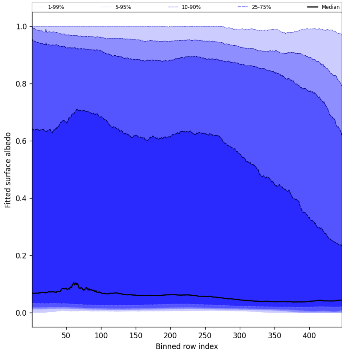
Figure 59: Along track statistics of “Fitted surface albedo” for 2025-02-19 to 2025-02-20
