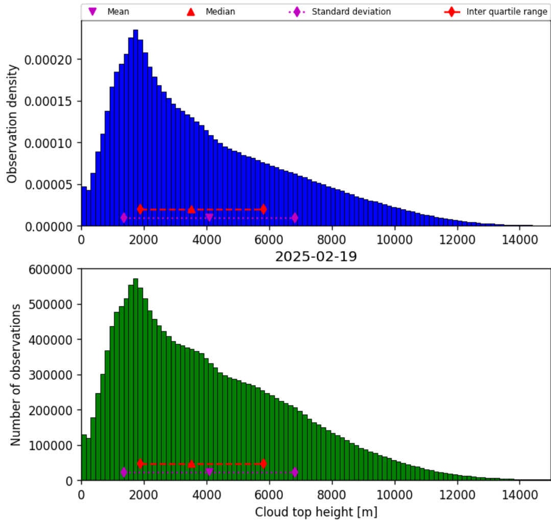
Figure 38: Histogram of “Cloud top height” for 2025-02-19 to 2025-02-20
