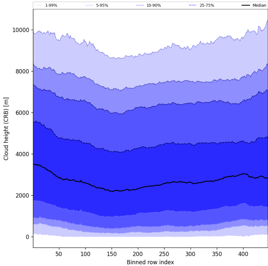
Figure 57: Along track statistics of “Cloud height (CRB)” for 2025-02-19 to 2025-02-20
