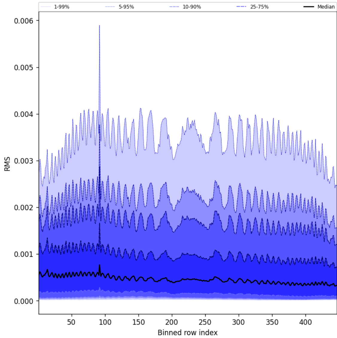
Figure 61: Along track statistics of “RMS” for 2025-02-19 to 2025-02-20
