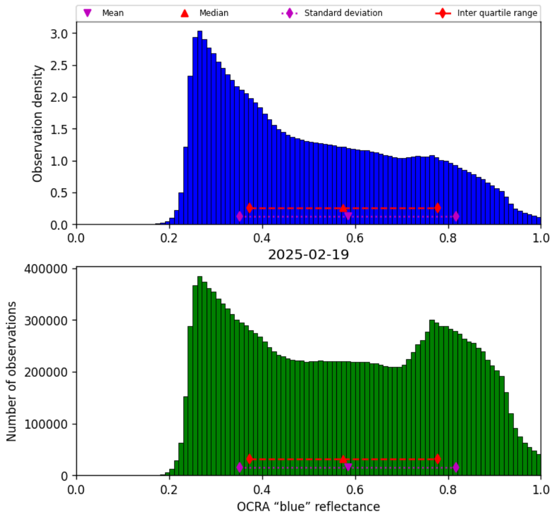
Figure 49: Histogram of “OCRA “blue” reflectance” for 2025-02-19 to 2025-02-20
