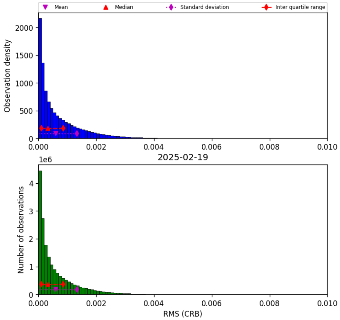
Figure 46: Histogram of “RMS (CRB)” for 2025-02-19 to 2025-02-20
