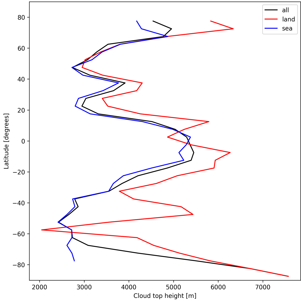
Figure 22: Zonal average of “Cloud top height” for 2025-02-19 to 2025-02-20.
