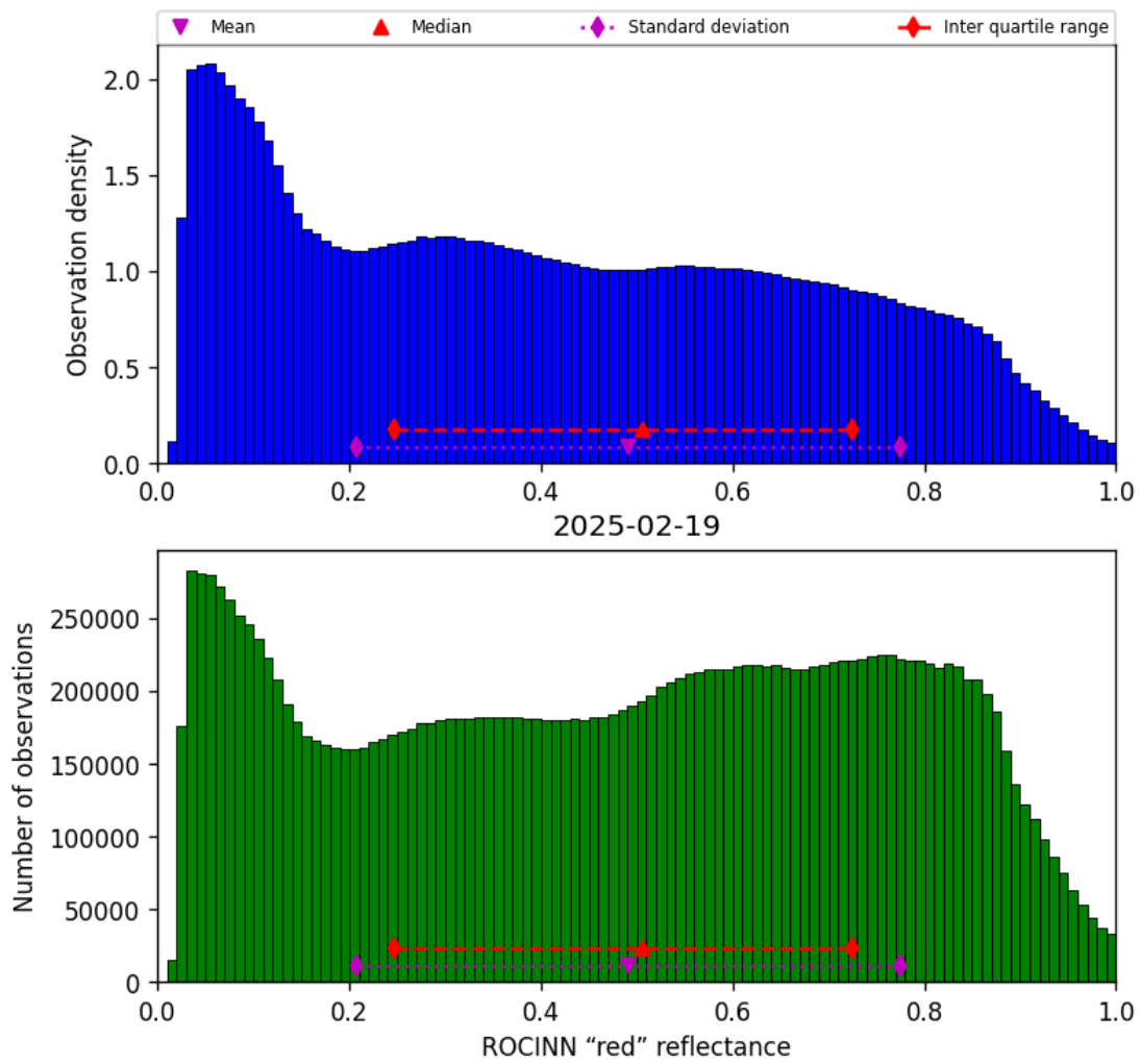
Figure 51: Histogram of “ROCINN “red” reflectance” for 2025-02-19 to 2025-02-20
