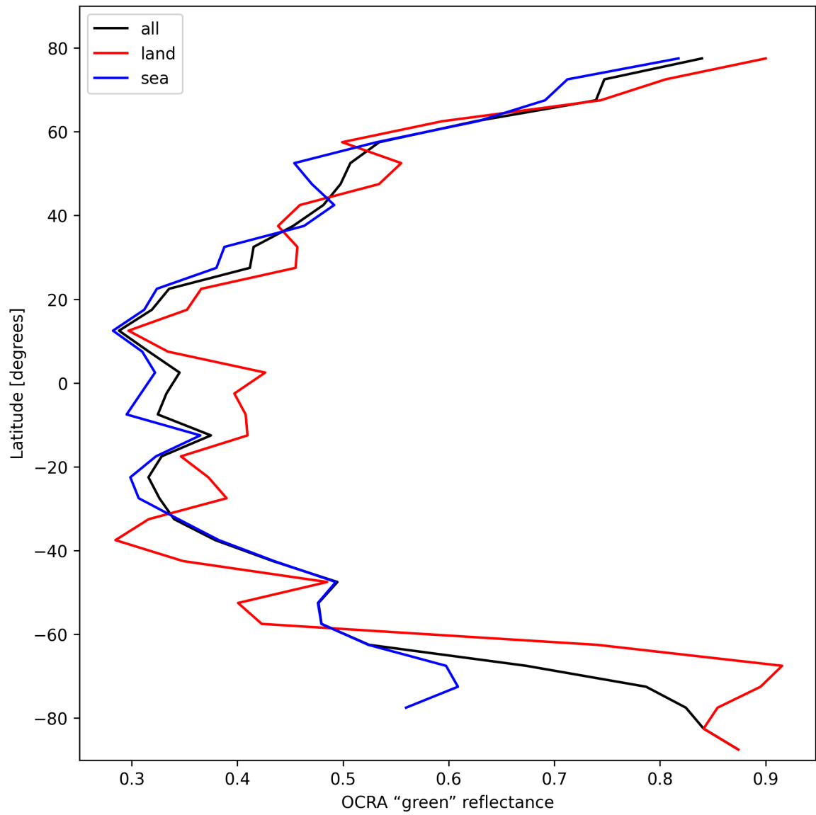
Figure 34: Zonal average of “OCRA “green” reflectance” for 2025-02-20 to 2025-02-21.
