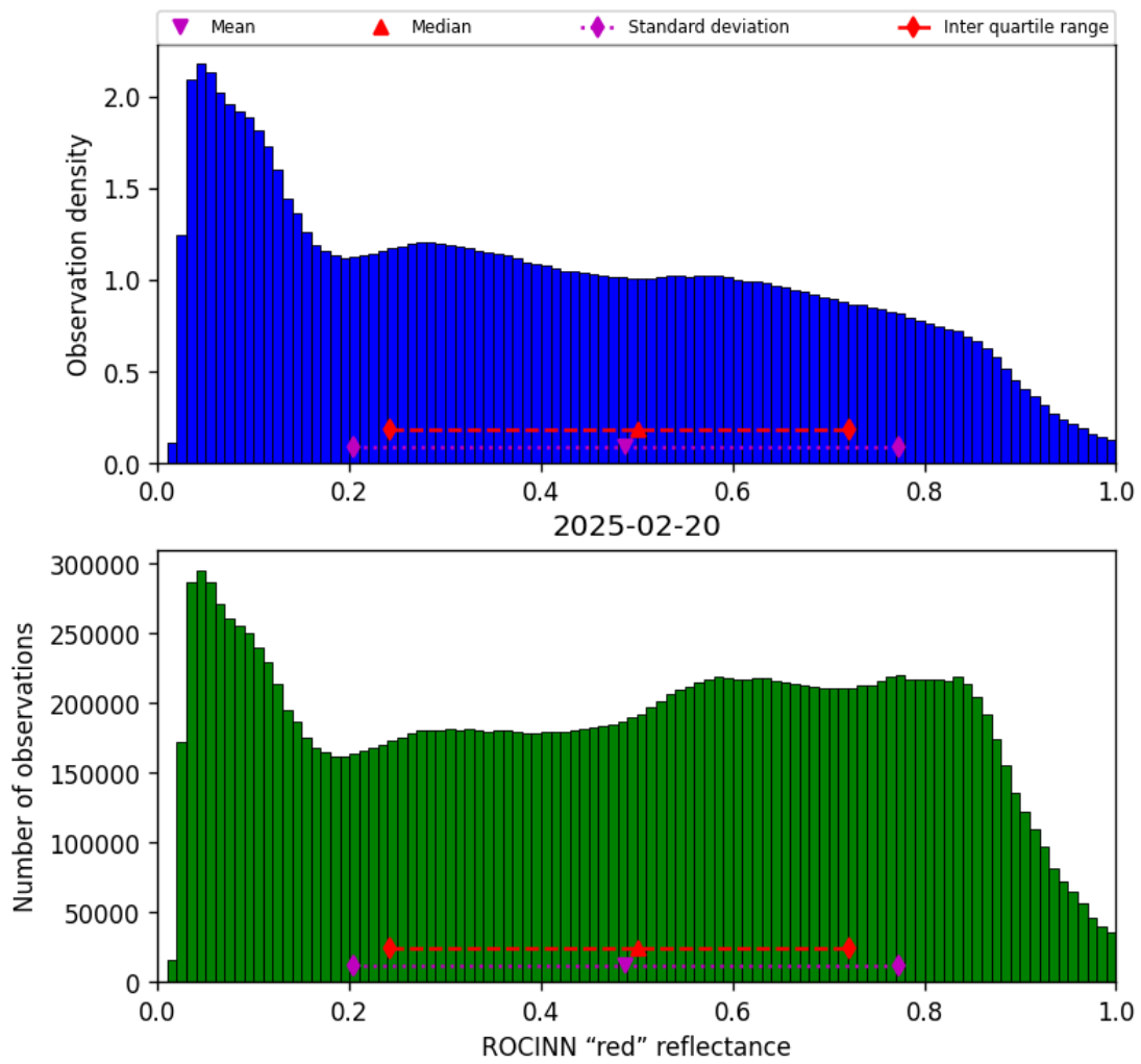
Figure 51: Histogram of “ROCINN “red” reflectance” for 2025-02-20 to 2025-02-21
