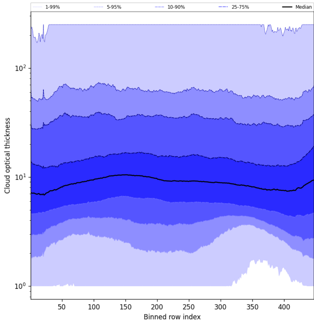
Figure 55: Along track statistics of “Cloud optical thickness” for 2025-02-20 to 2025-02-21
