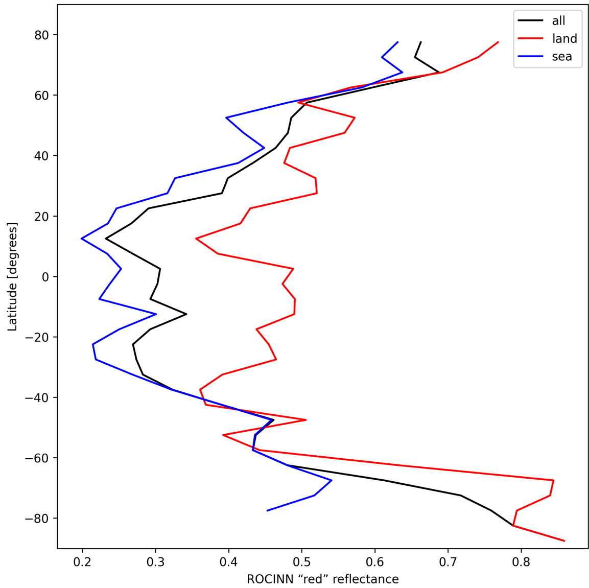
Figure 35: Zonal average of "ROCINN "red" reflectance" for 2025-02-20 to 2025-02-21.
