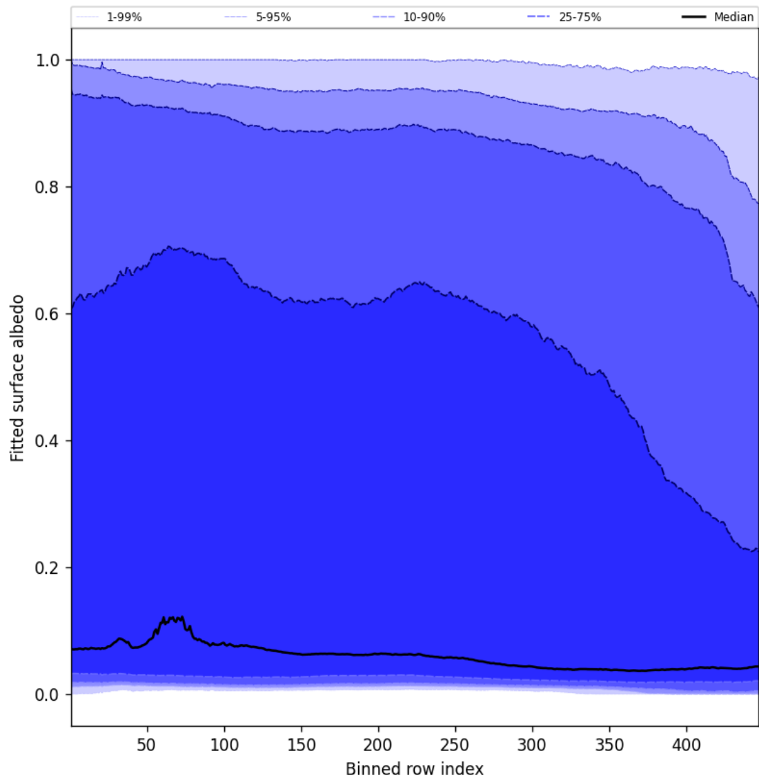
Figure 59: Along track statistics of “Fitted surface albedo” for 2025-02-20 to 2025-02-21
