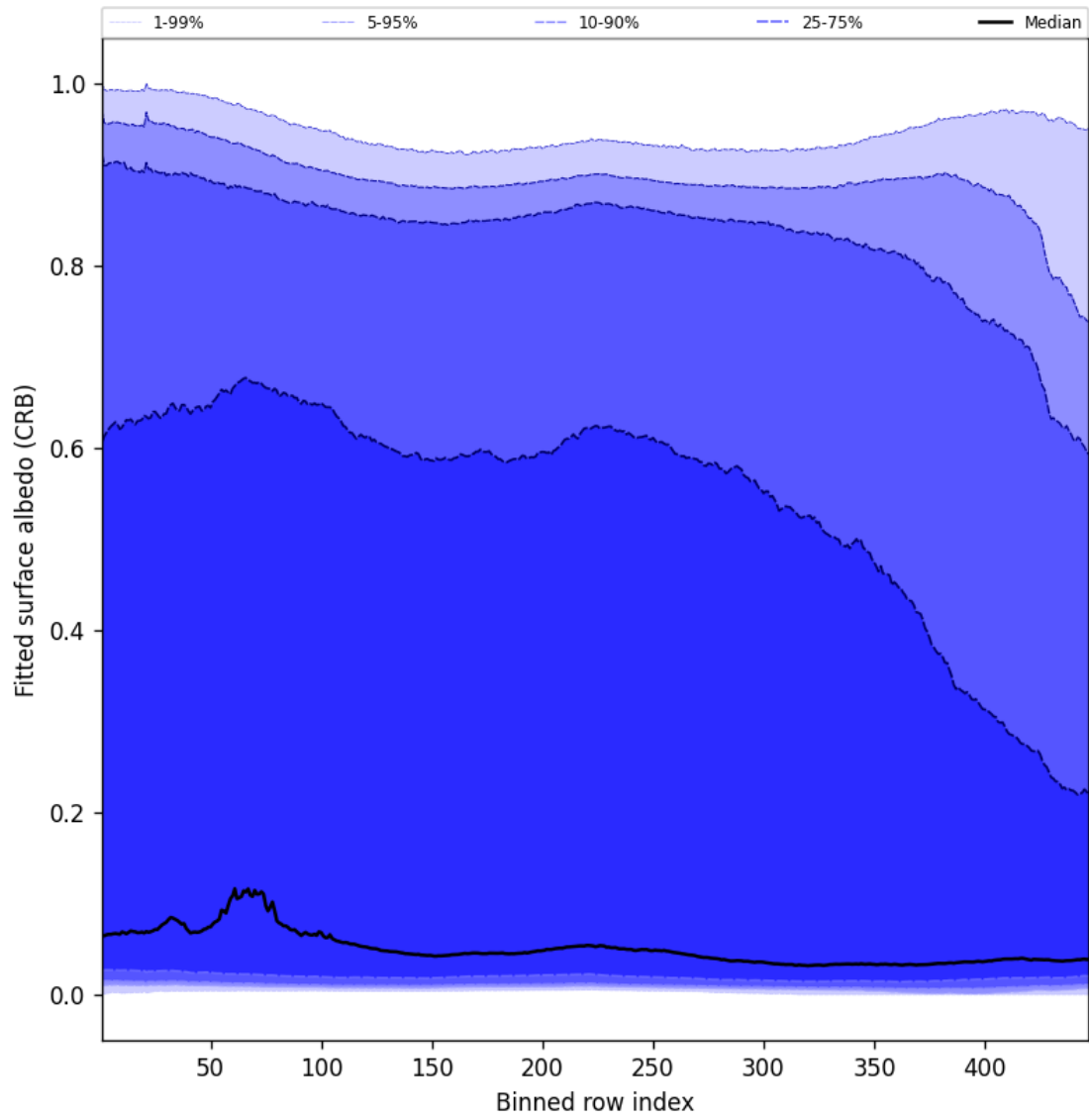
Figure 60: Along track statistics of “Fitted surface albedo (CRB)” for 2025-02-20 to 2025-02-21
