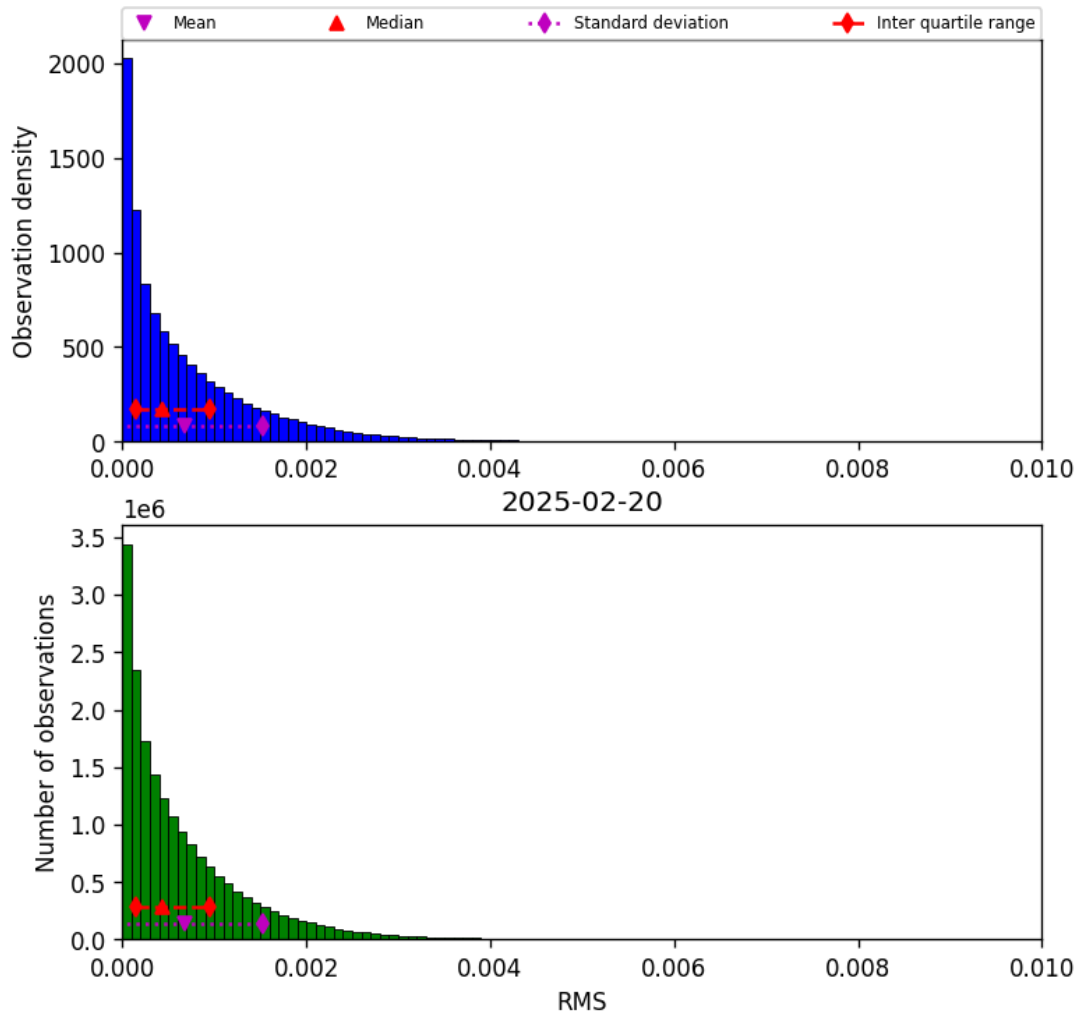
Figure 45: Histogram of “RMS” for 2025-02-20 to 2025-02-21
