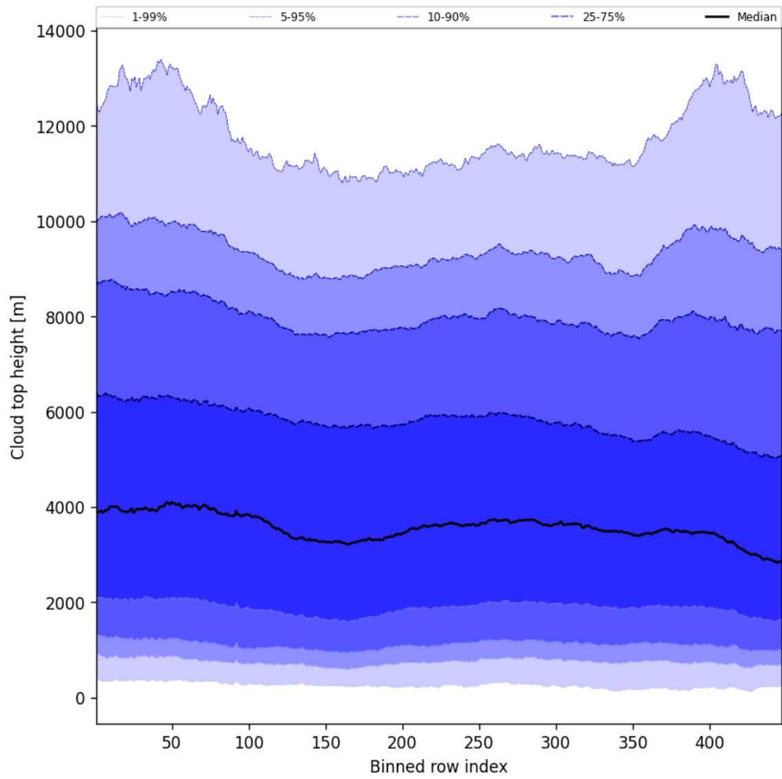
Figure 54: Along track statistics of “Cloud top height” for 2025-02-20 to 2025-02-21
