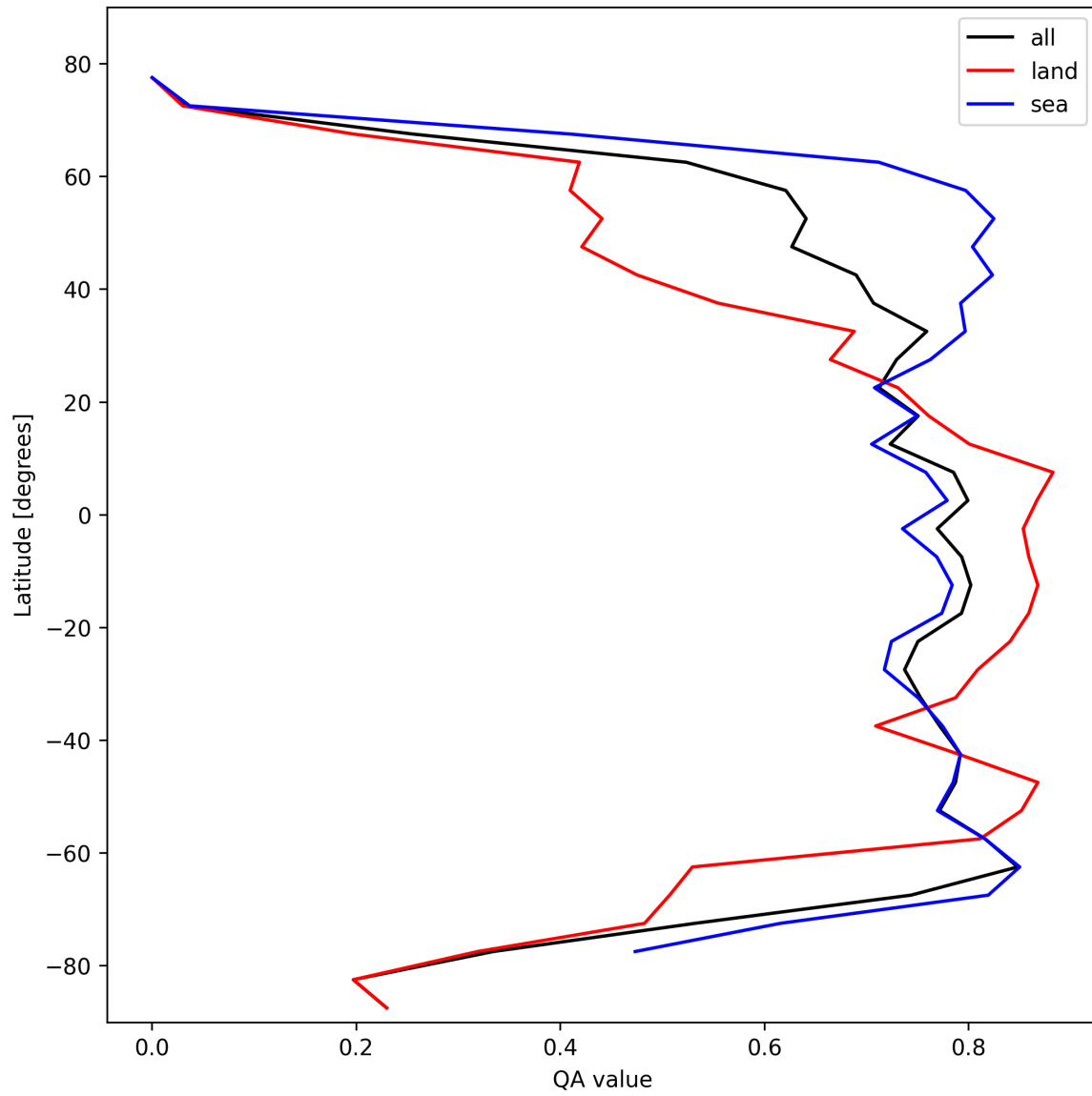
Figure 20: Zonal average of “QA value” for 2025-02-20 to 2025-02-21.
