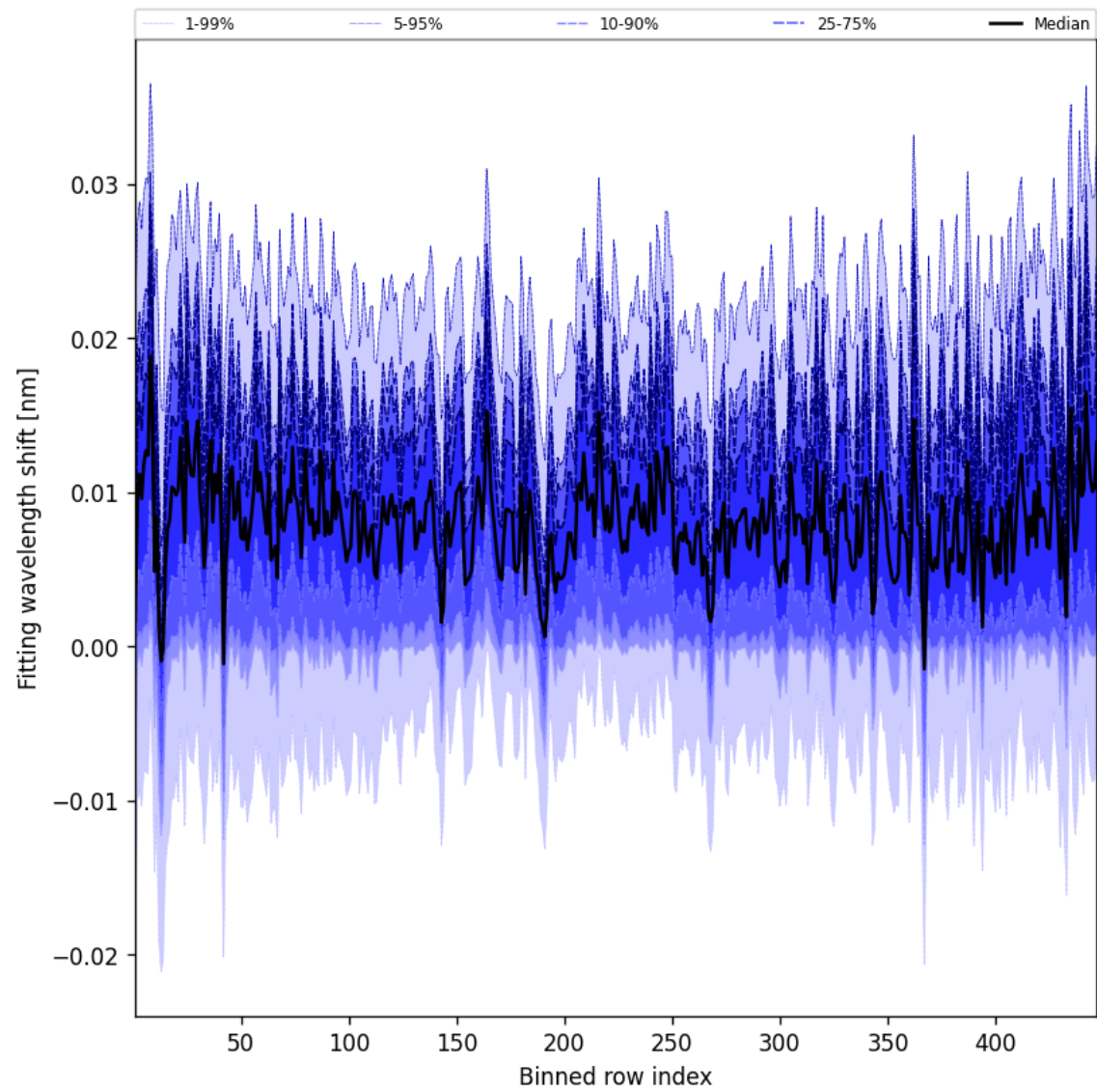
Figure 63: Along track statistics of “Fitting wavelength shift” for 2025-02-20 to 2025-02-21
