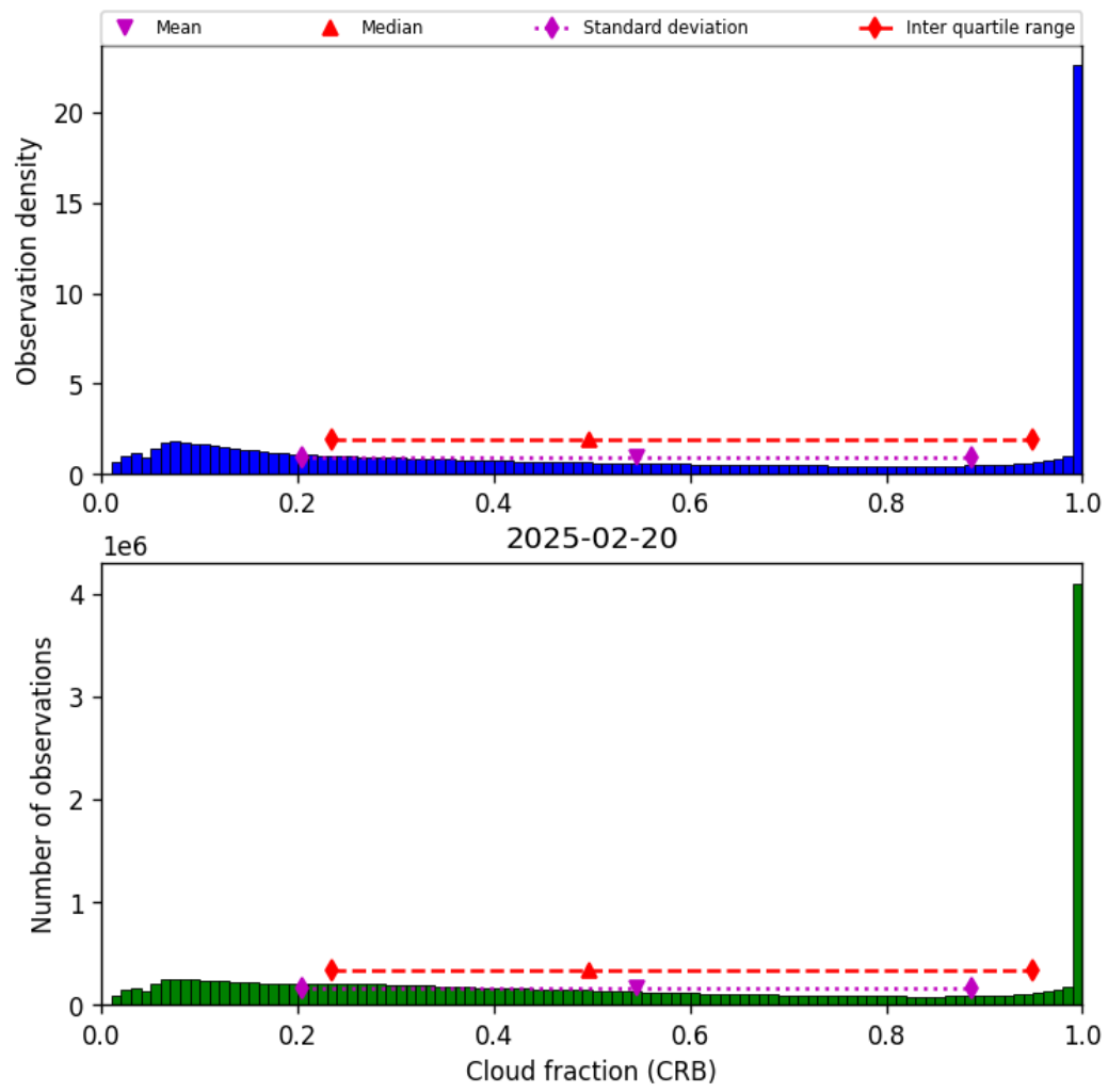
Figure 40: Histogram of “Cloud fraction (CRB)” for 2025-02-20 to 2025-02-21
