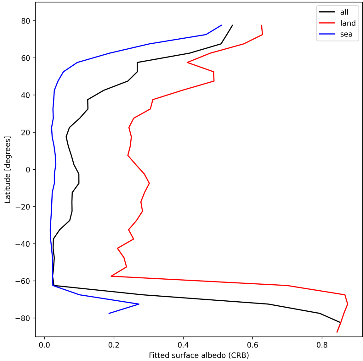
Figure 28: Zonal average of “Fitted surface albedo (CRB)” for 2025-02-20 to 2025-02-21.
