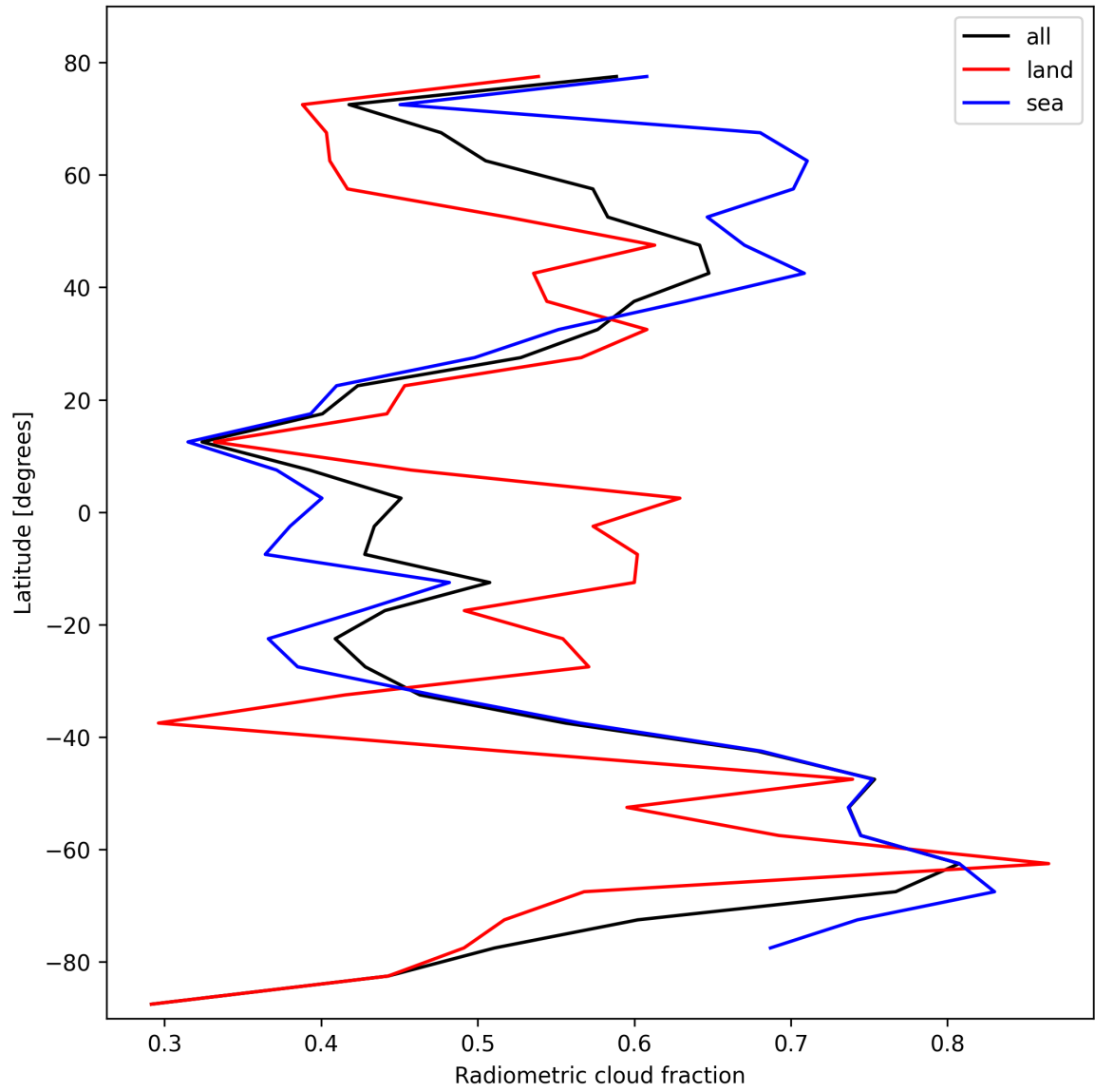
Figure 21: Zonal average of “Radiometric cloud fraction” for 2025-02-20 to 2025-02-21.
