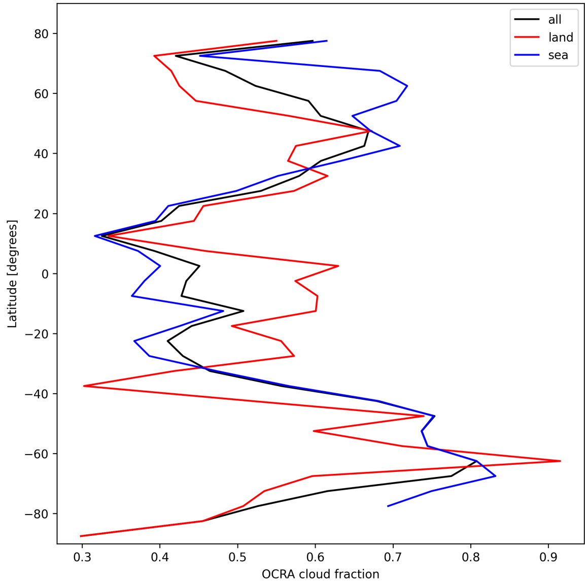
Figure 32: Zonal average of “OCRA cloud fraction” for 2025-02-20 to 2025-02-21.
