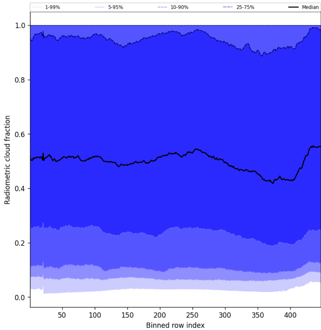
Figure 53: Along track statistics of “Radiometric cloud fraction” for 2025-02-20 to 2025-02-21
