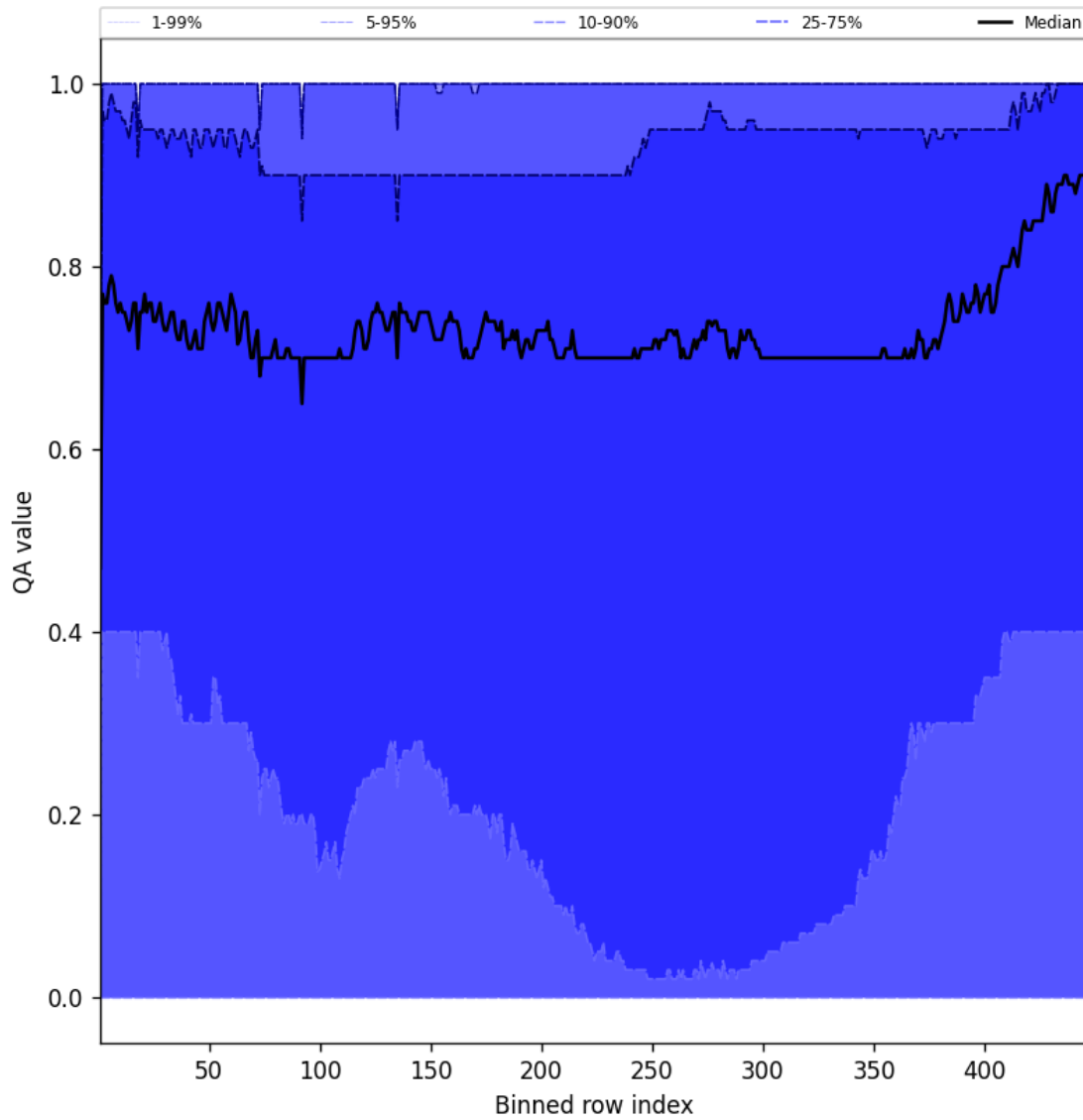
Figure 52: Along track statistics of “QA value” for 2025-02-20 to 2025-02-21
