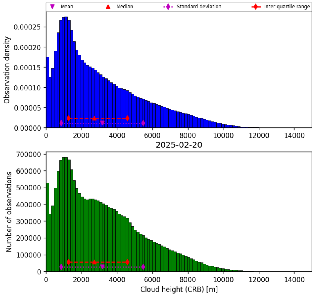
Figure 41: Histogram of “Cloud height (CRB)” for 2025-02-20 to 2025-02-21
