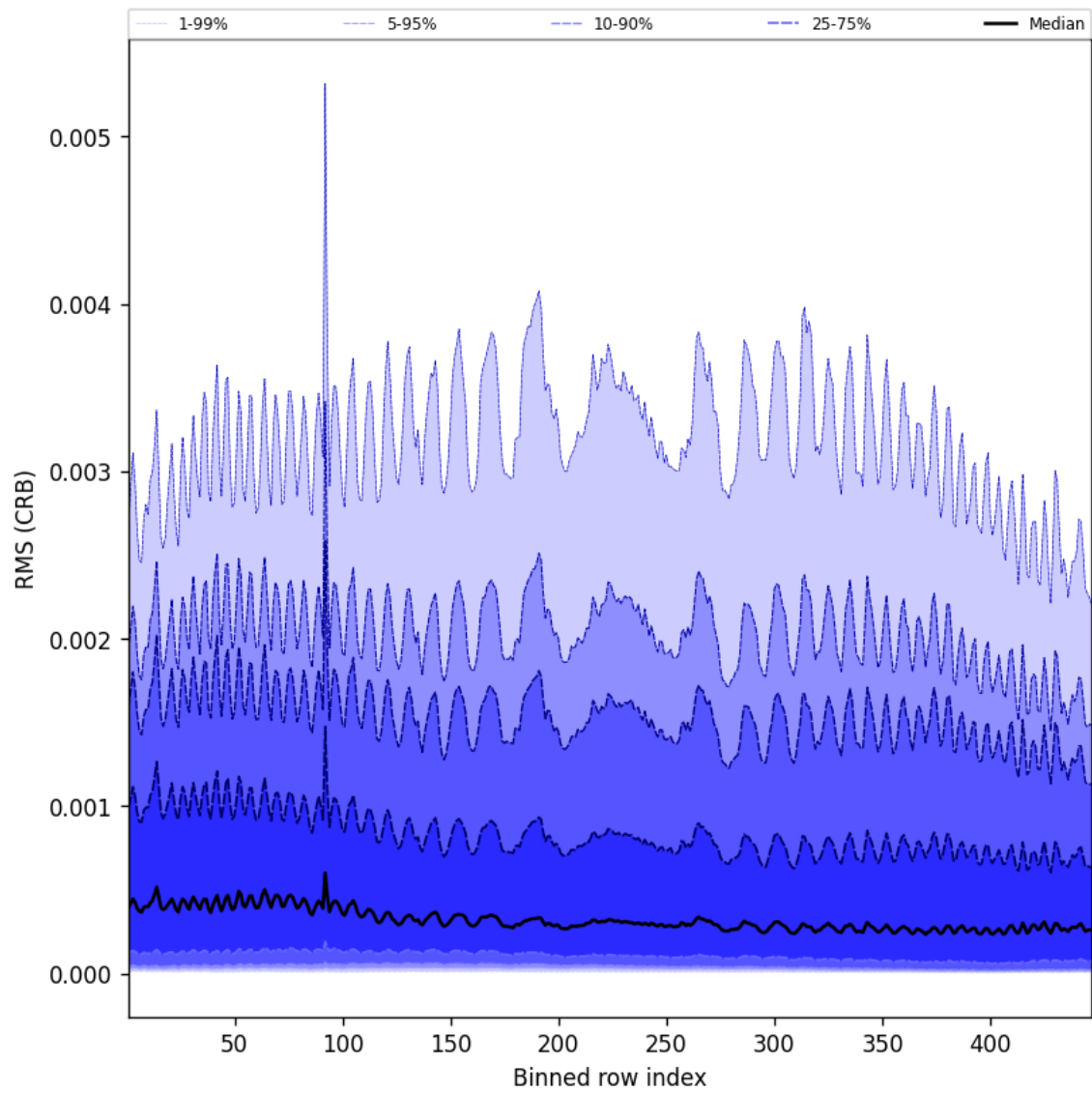
Figure 62: Along track statistics of “RMS (CRB)” for 2025-02-20 to 2025-02-21
