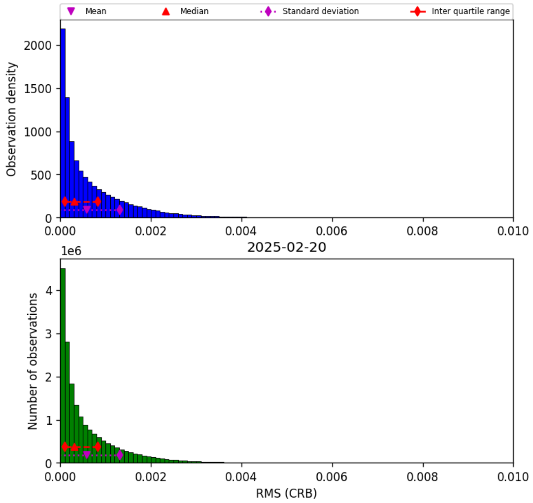
Figure 46: Histogram of "RMS (CRB)" for 2025-02-20 to 2025-02-21
