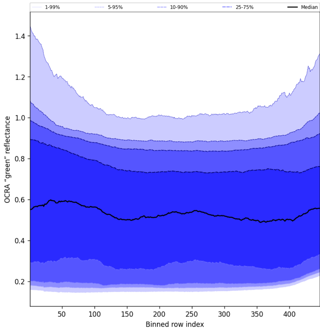
Figure 66: Along track statistics of “OCRA “green” reflectance” for 2025-02-20 to 2025-02-21
