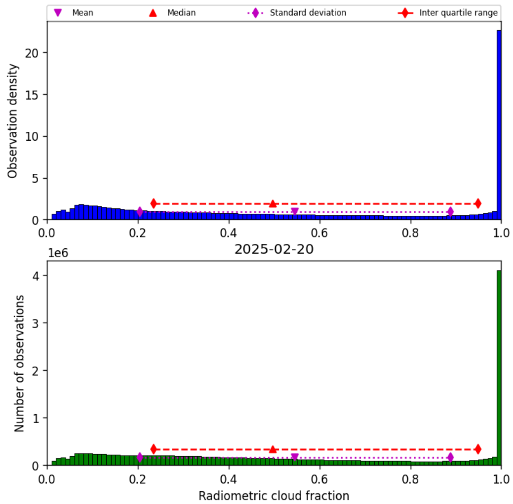
Figure 37: Histogram of “Radiometric cloud fraction” for 2025-02-20 to 2025-02-21
