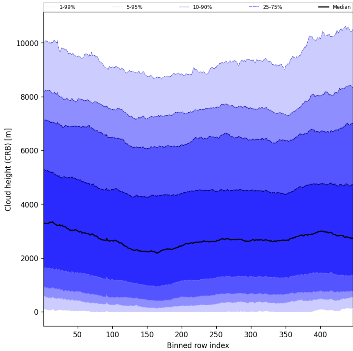
Figure 57: Along track statistics of “Cloud height (CRB)” for 2025-02-20 to 2025-02-21
