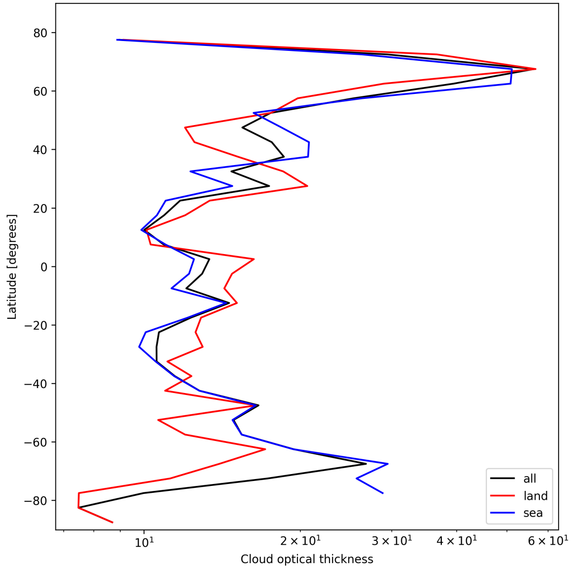
Figure 23: Zonal average of “Cloud optical thickness” for 2025-02-20 to 2025-02-21.
