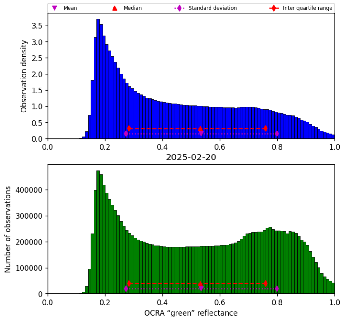
Figure 50: Histogram of “OCRA “green” reflectance” for 2025-02-20 to 2025-02-21
