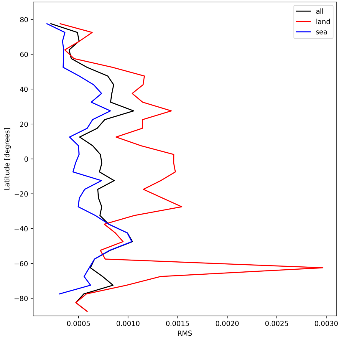
Figure 29: Zonal average of “RMS” for 2025-02-20 to 2025-02-21.
