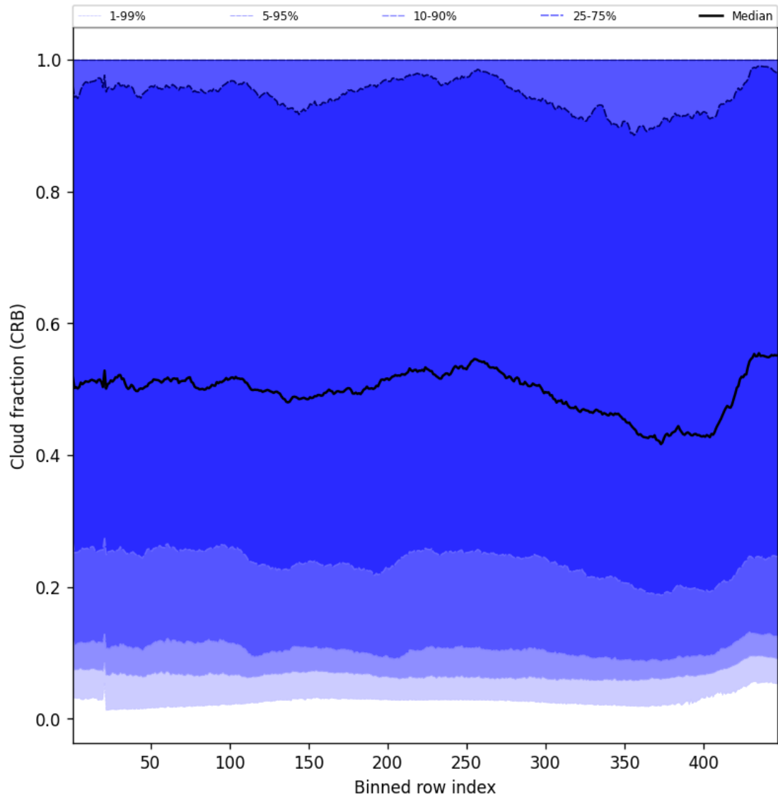
Figure 56: Along track statistics of “Cloud fraction (CRB)” for 2025-02-20 to 2025-02-21
