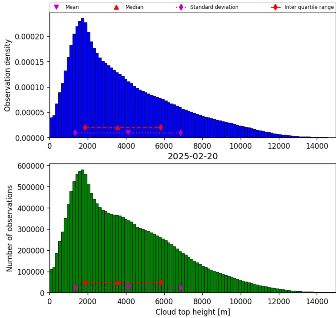
Figure 38: Histogram of “Cloud top height” for 2025-02-20 to 2025-02-21
