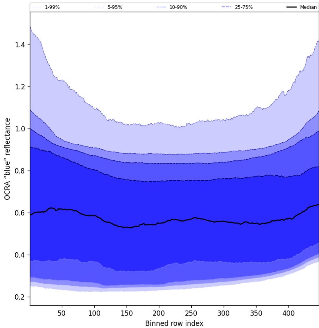
Figure 65: Along track statistics of “OCRA “blue” reflectance” for 2025-02-20 to 2025-02-21
