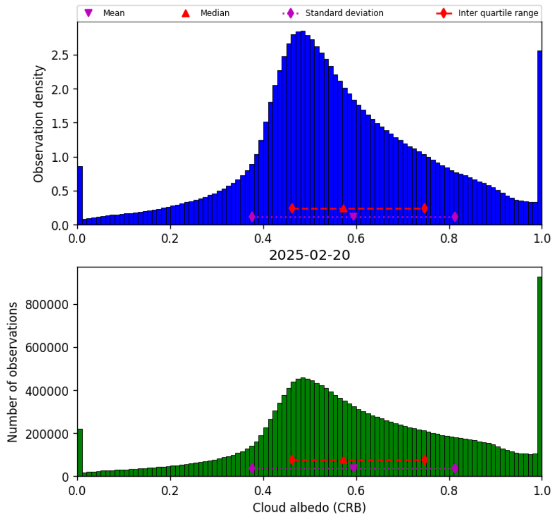
Figure 42: Histogram of “Cloud albedo (CRB)” for 2025-02-20 to 2025-02-21
