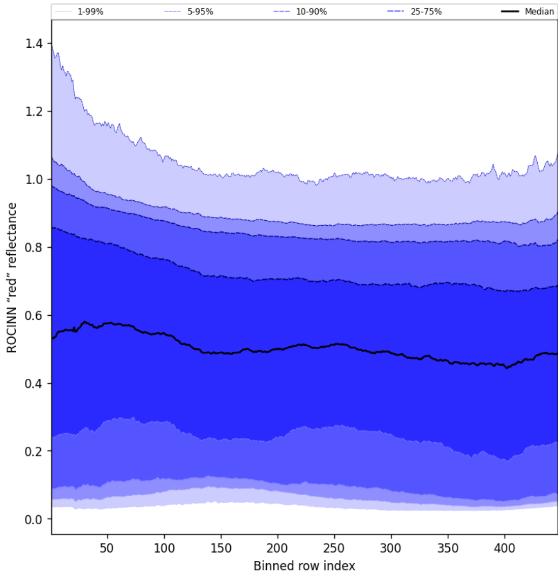
Figure 67: Along track statistics of “ROCINN “red” reflectance” for 2025-02-20 to 2025-02-21
