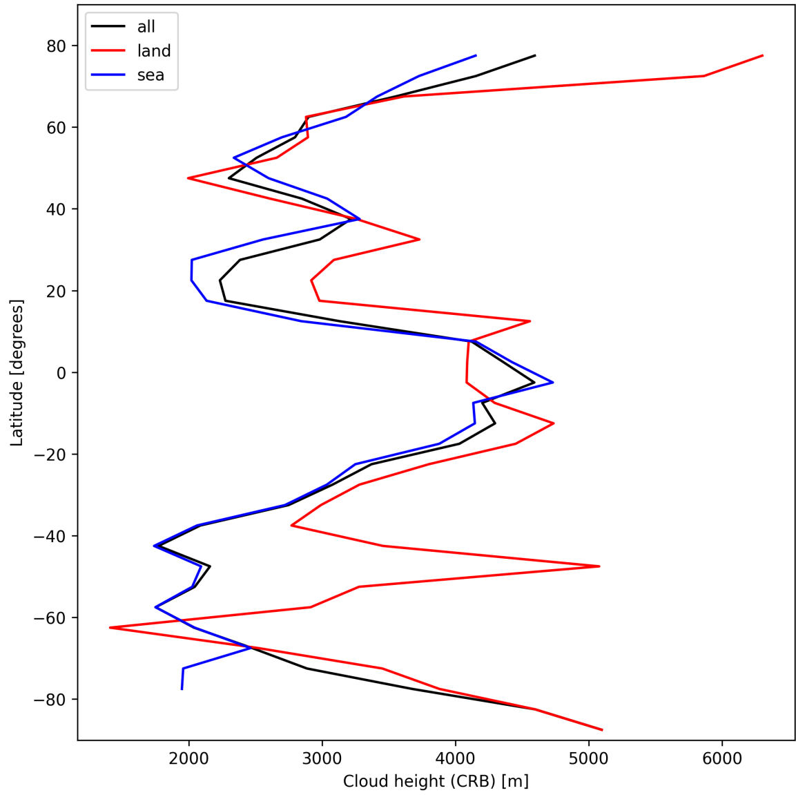
Figure 25: Zonal average of “Cloud height (CRB)” for 2025-02-20 to 2025-02-21.
