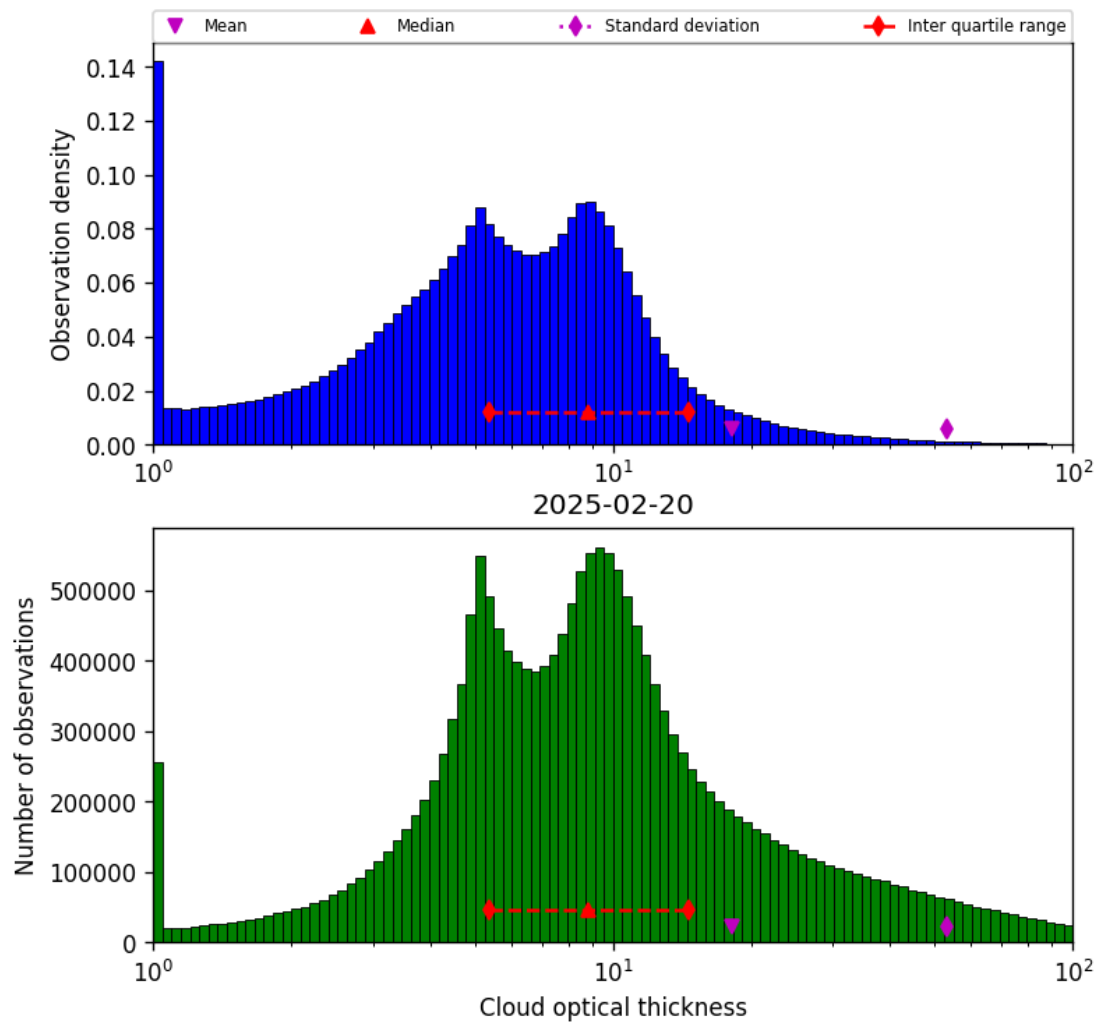
Figure 39: Histogram of “Cloud optical thickness” for 2025-02-20 to 2025-02-21
