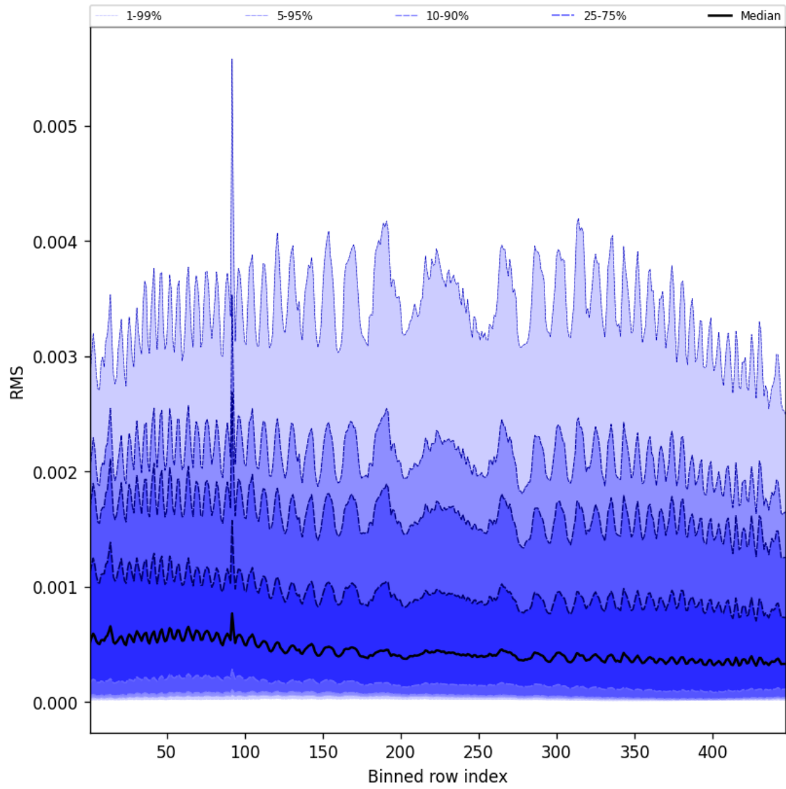
Figure 61: Along track statistics of “RMS” for 2025-02-20 to 2025-02-21
