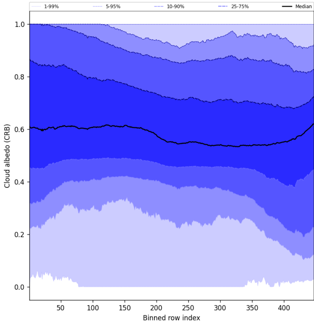
Figure 58: Along track statistics of “Cloud albedo (CRB)” for 2025-02-20 to 2025-02-21
