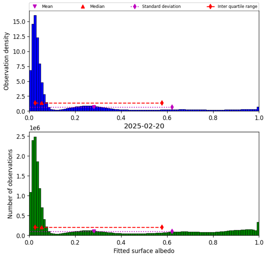
Figure 43: Histogram of “Fitted surface albedo” for 2025-02-20 to 2025-02-21
