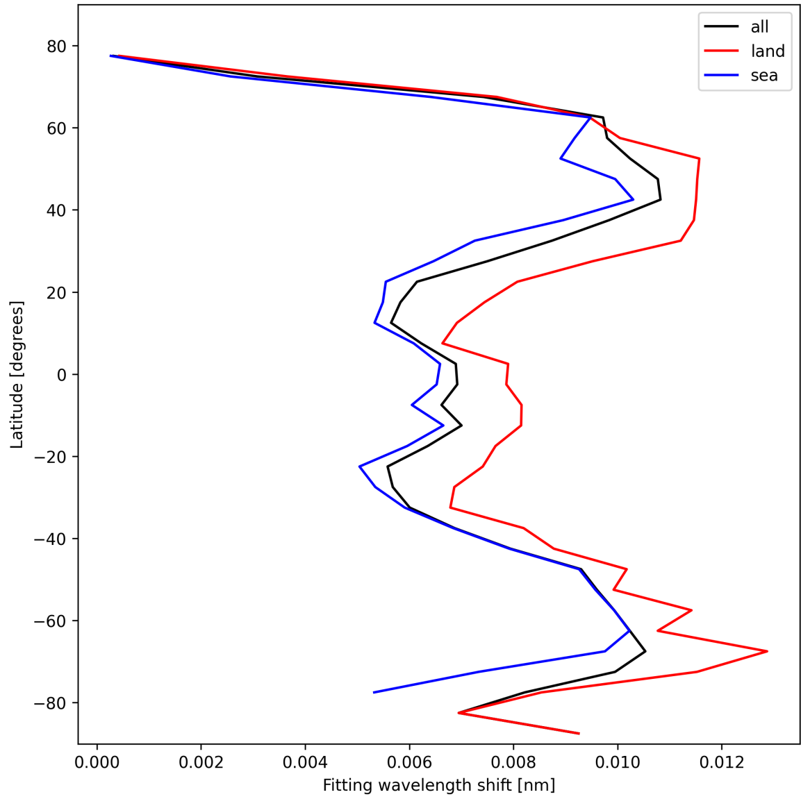
Figure 31: Zonal average of “Fitting wavelength shift” for 2025-02-20 to 2025-02-21.
