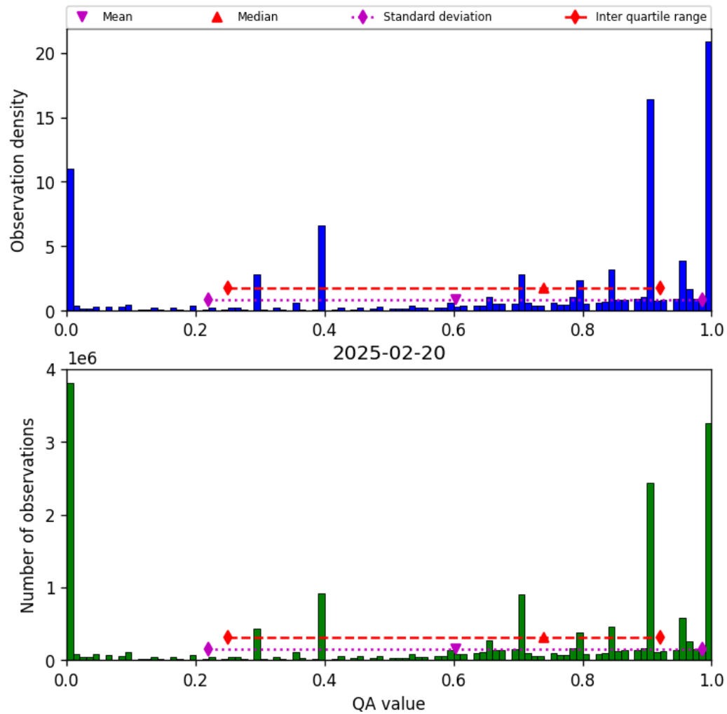
Figure 36: Histogram of “QA value” for 2025-02-20 to 2025-02-21
