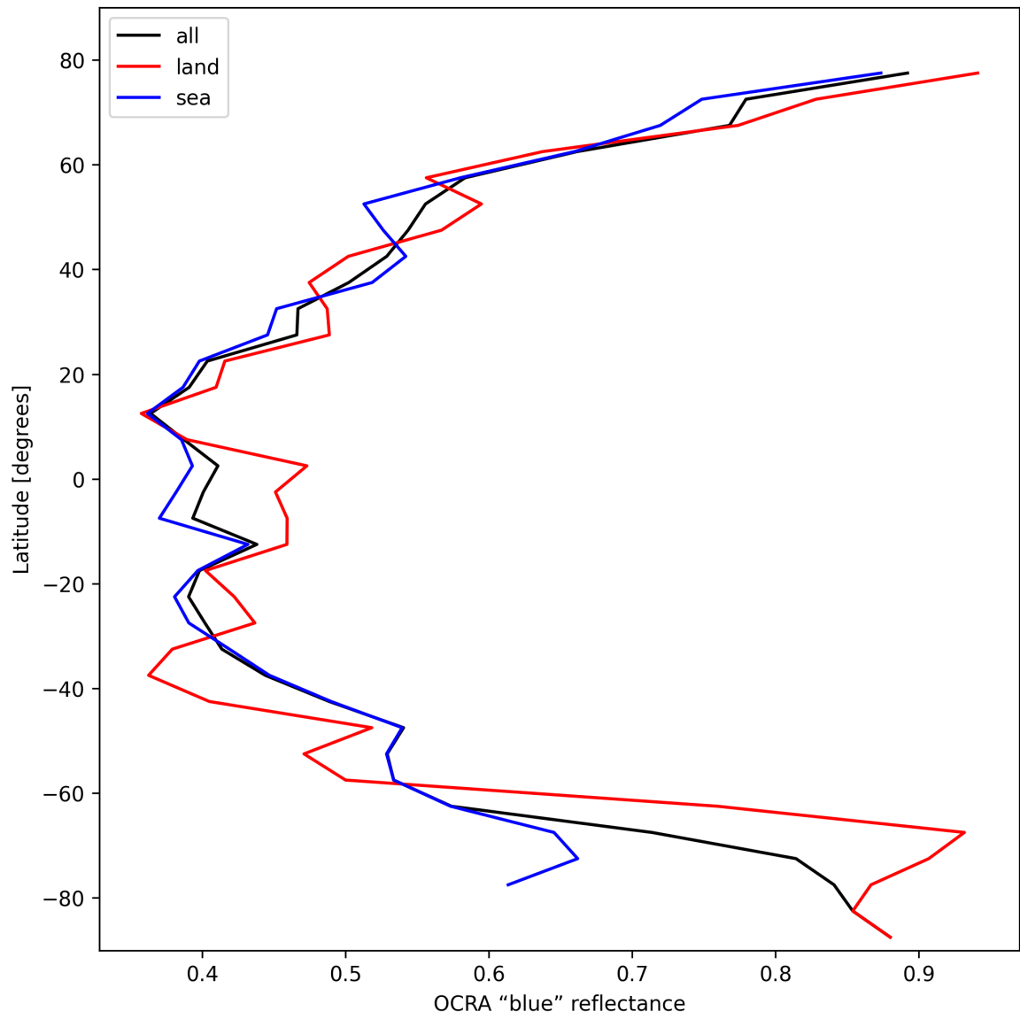
Figure 33: Zonal average of “OCRA “blue” reflectance” for 2025-02-20 to 2025-02-21.
