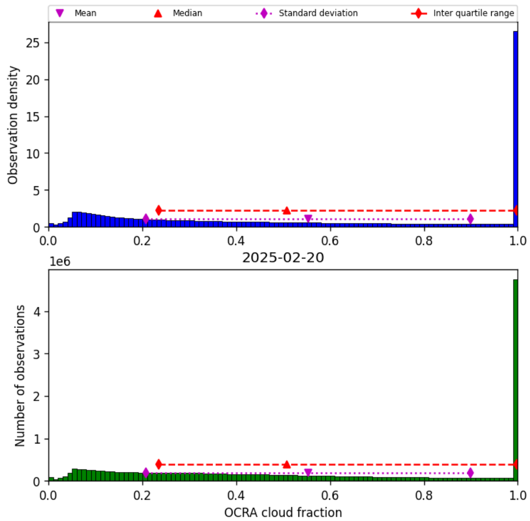
Figure 48: Histogram of “OCRA cloud fraction” for 2025-02-20 to 2025-02-21
