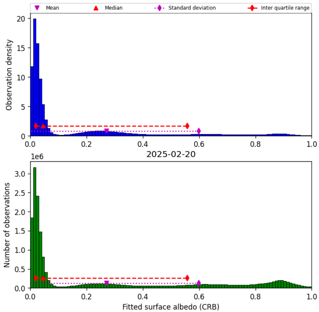
Figure 44: Histogram of “Fitted surface albedo (CRB)” for 2025-02-20 to 2025-02-21
