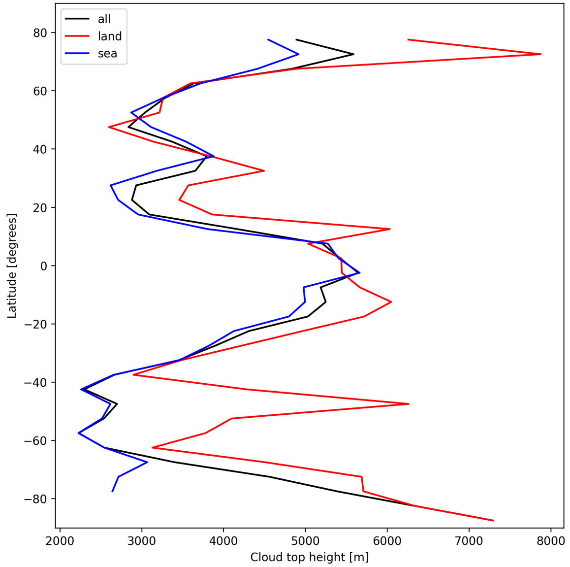
Figure 22: Zonal average of “Cloud top height” for 2025-02-20 to 2025-02-21.
