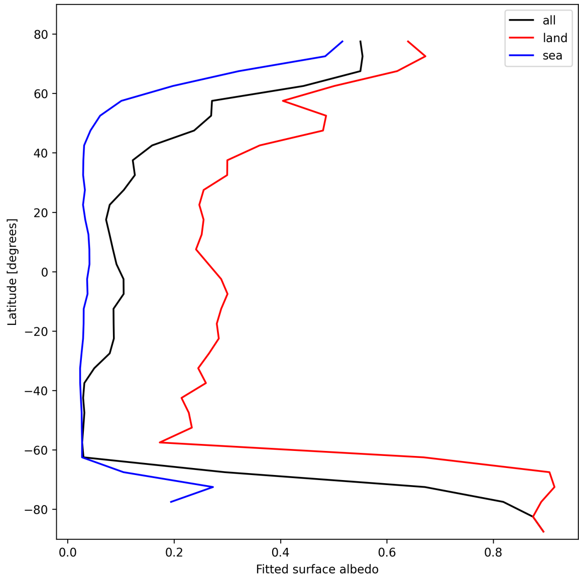
Figure 27: Zonal average of “Fitted surface albedo” for 2025-02-20 to 2025-02-21.
