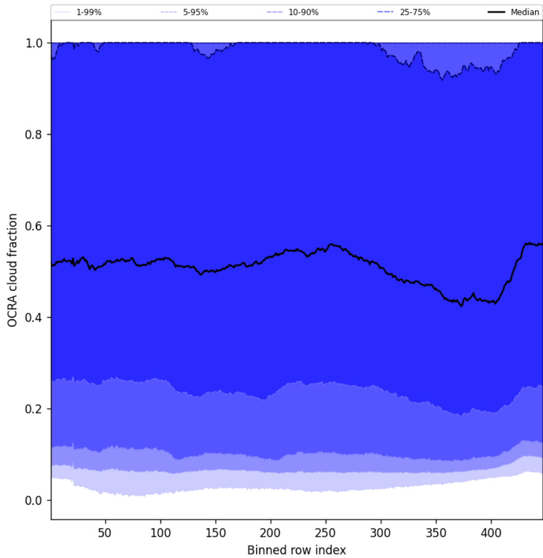
Figure 64: Along track statistics of “OCRA cloud fraction” for 2025-02-20 to 2025-02-21
