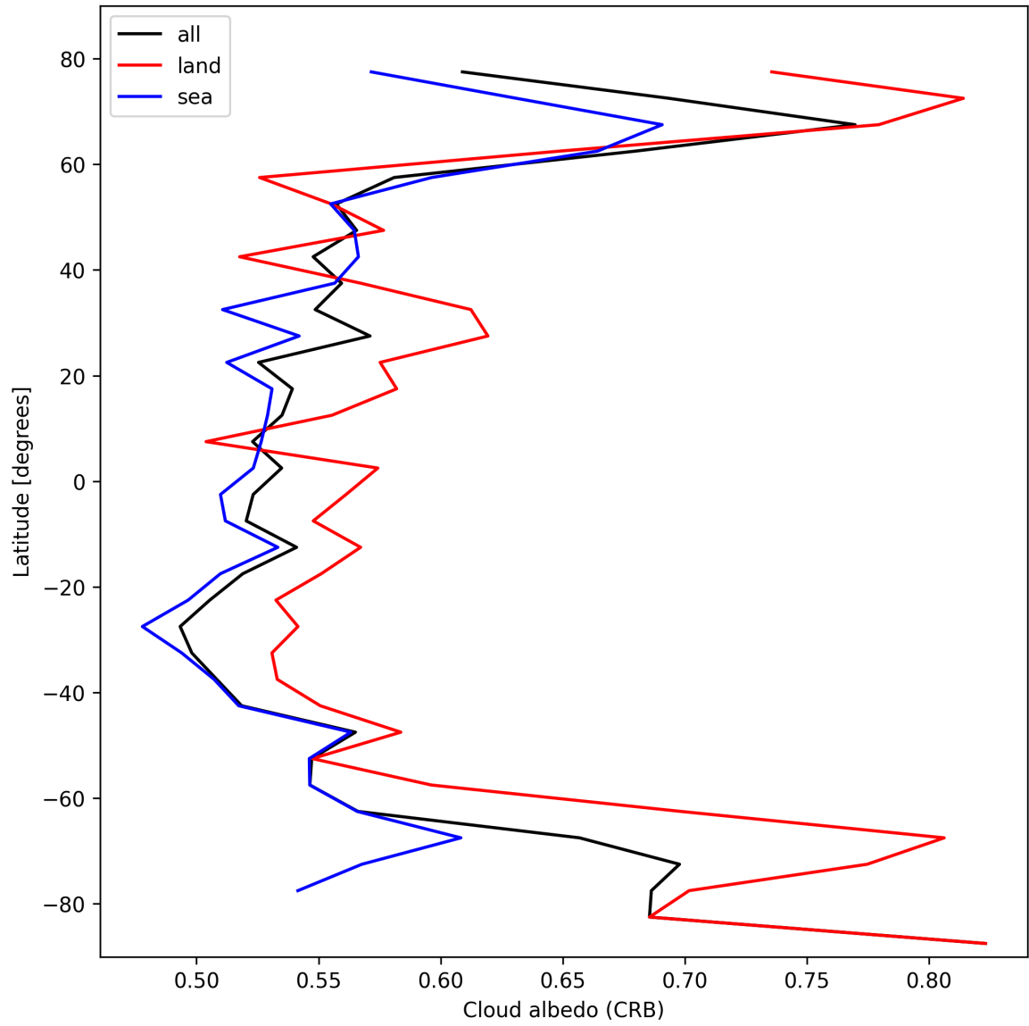
Figure 26: Zonal average of “Cloud albedo (CRB)” for 2025-02-20 to 2025-02-21.
