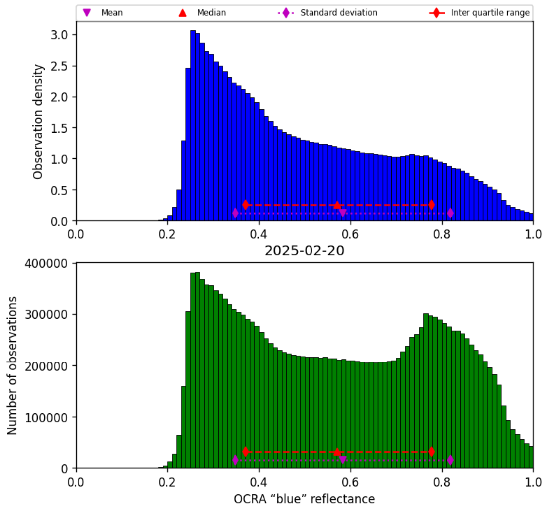
Figure 49: Histogram of “OCRA “blue” reflectance” for 2025-02-20 to 2025-02-21
