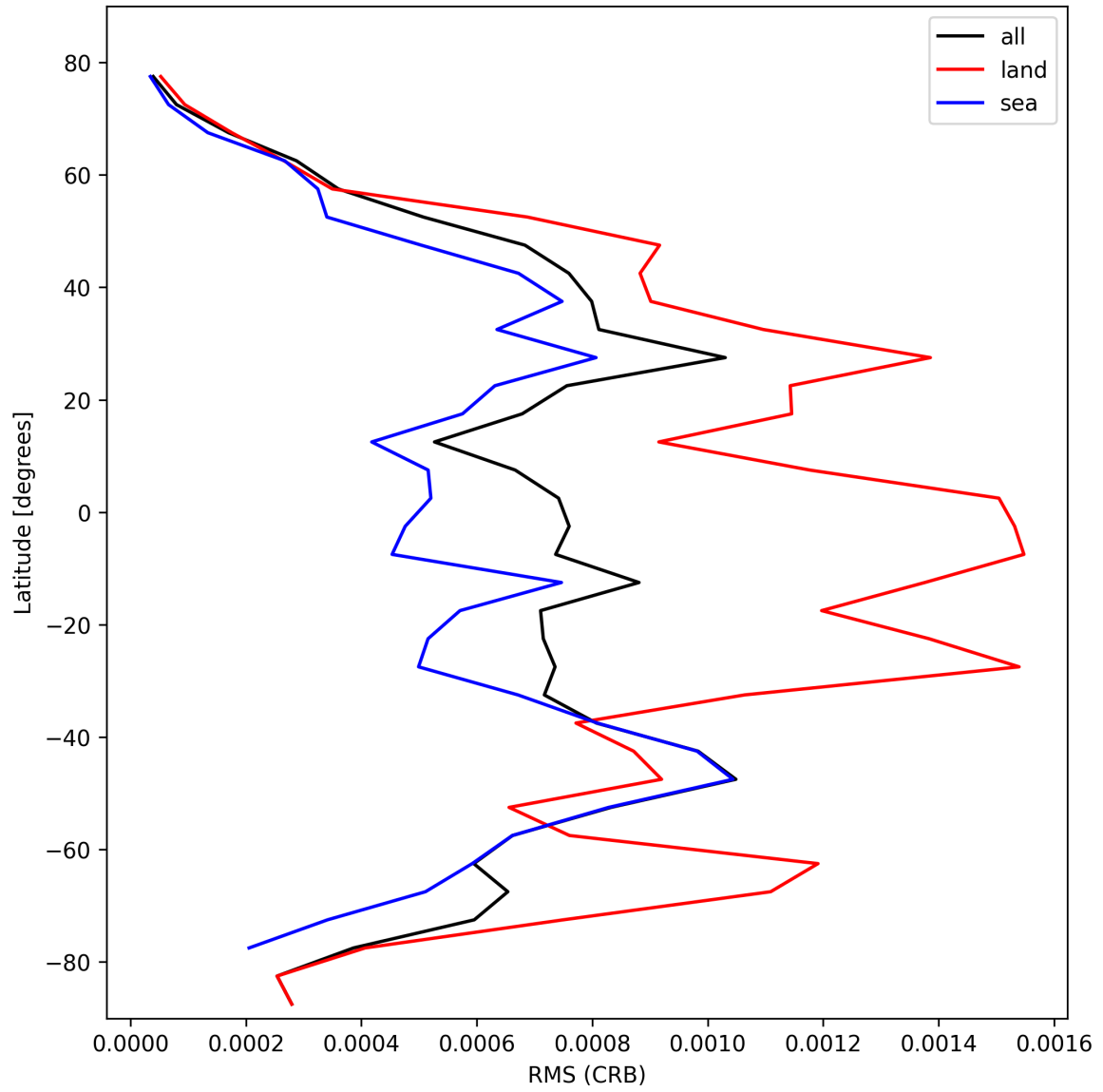
Figure 30: Zonal average of “RMS (CRB)” for 2025-02-20 to 2025-02-21.
