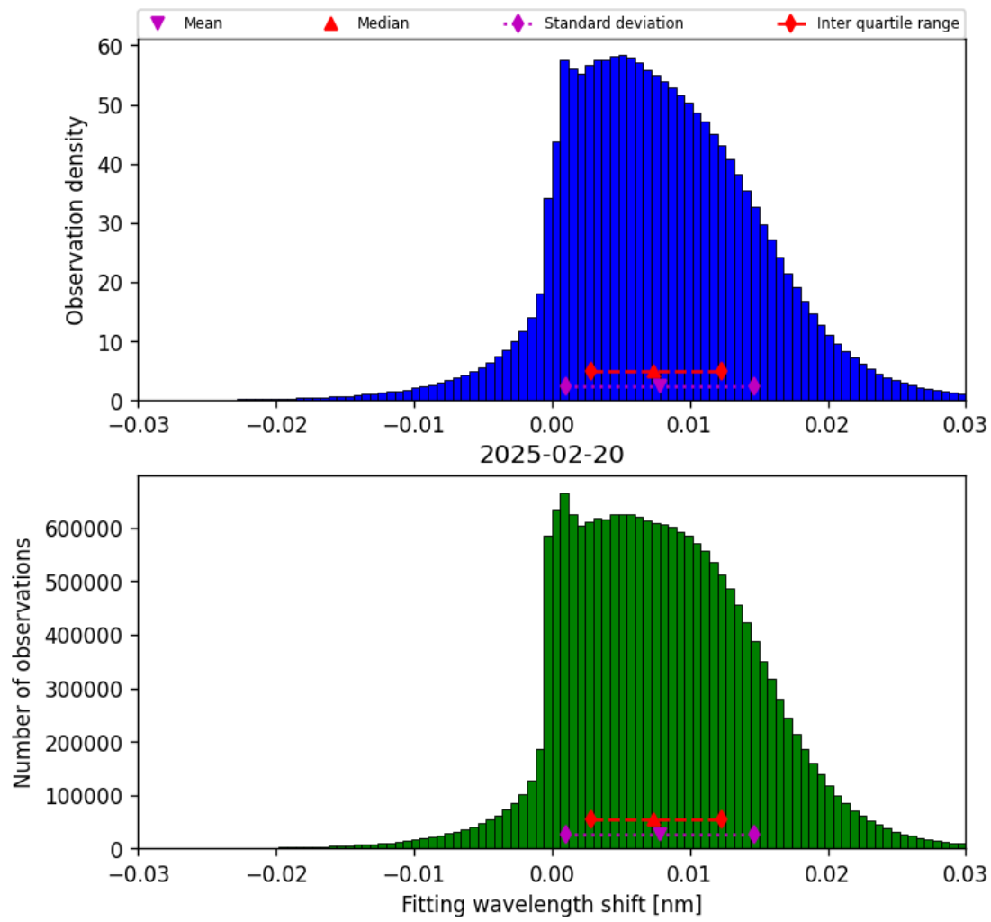
Figure 47: Histogram of “Fitting wavelength shift” for 2025-02-20 to 2025-02-21
