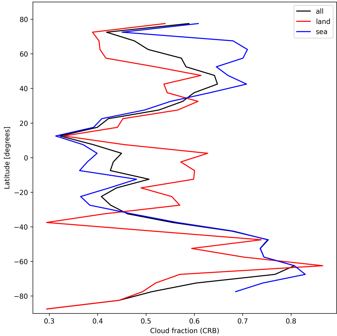
Figure 24: Zonal average of “Cloud fraction (CRB)” for 2025-02-20 to 2025-02-21.
