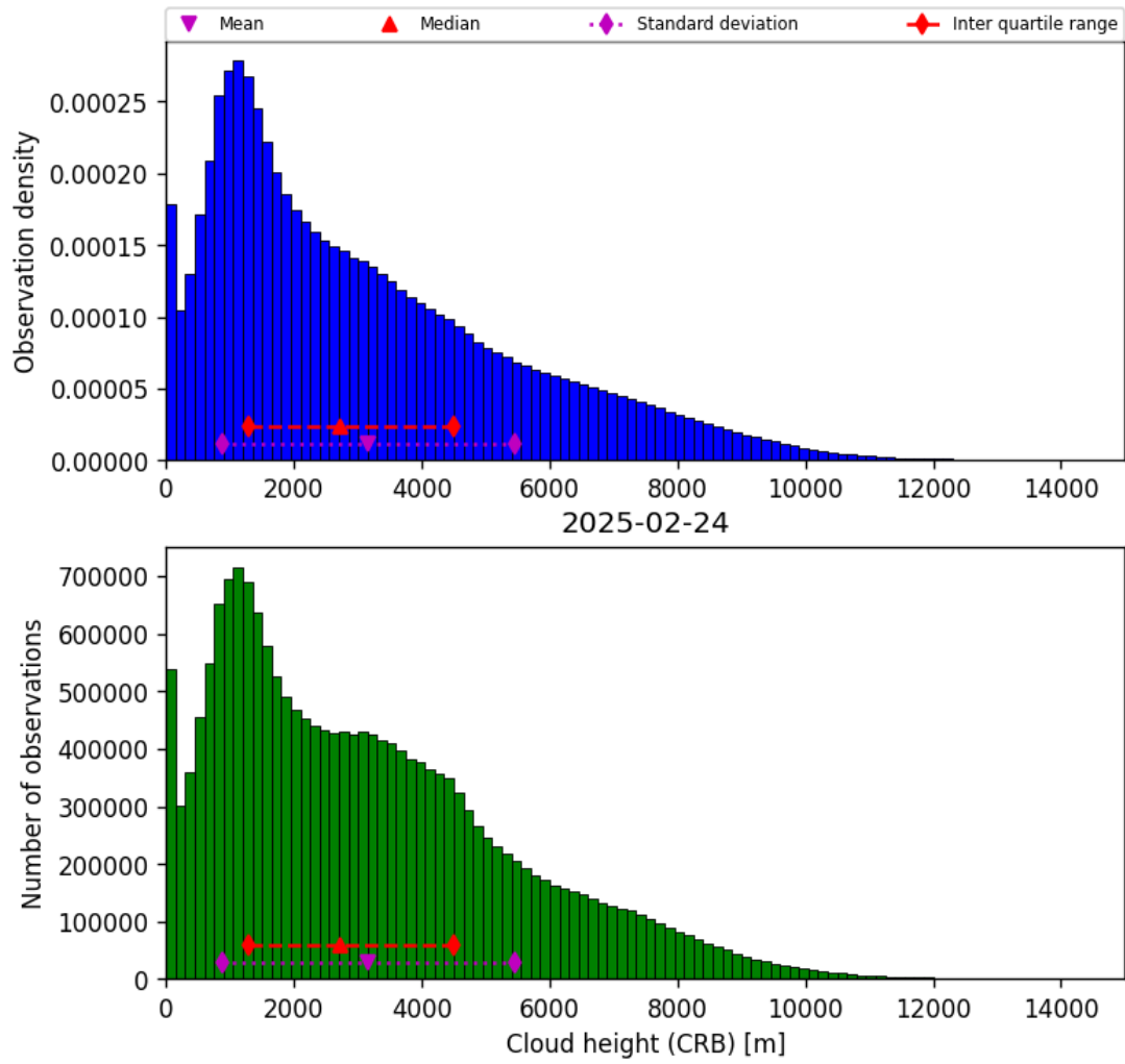
Figure 41: Histogram of “Cloud height (CRB)” for 2025-02-24 to 2025-02-25
