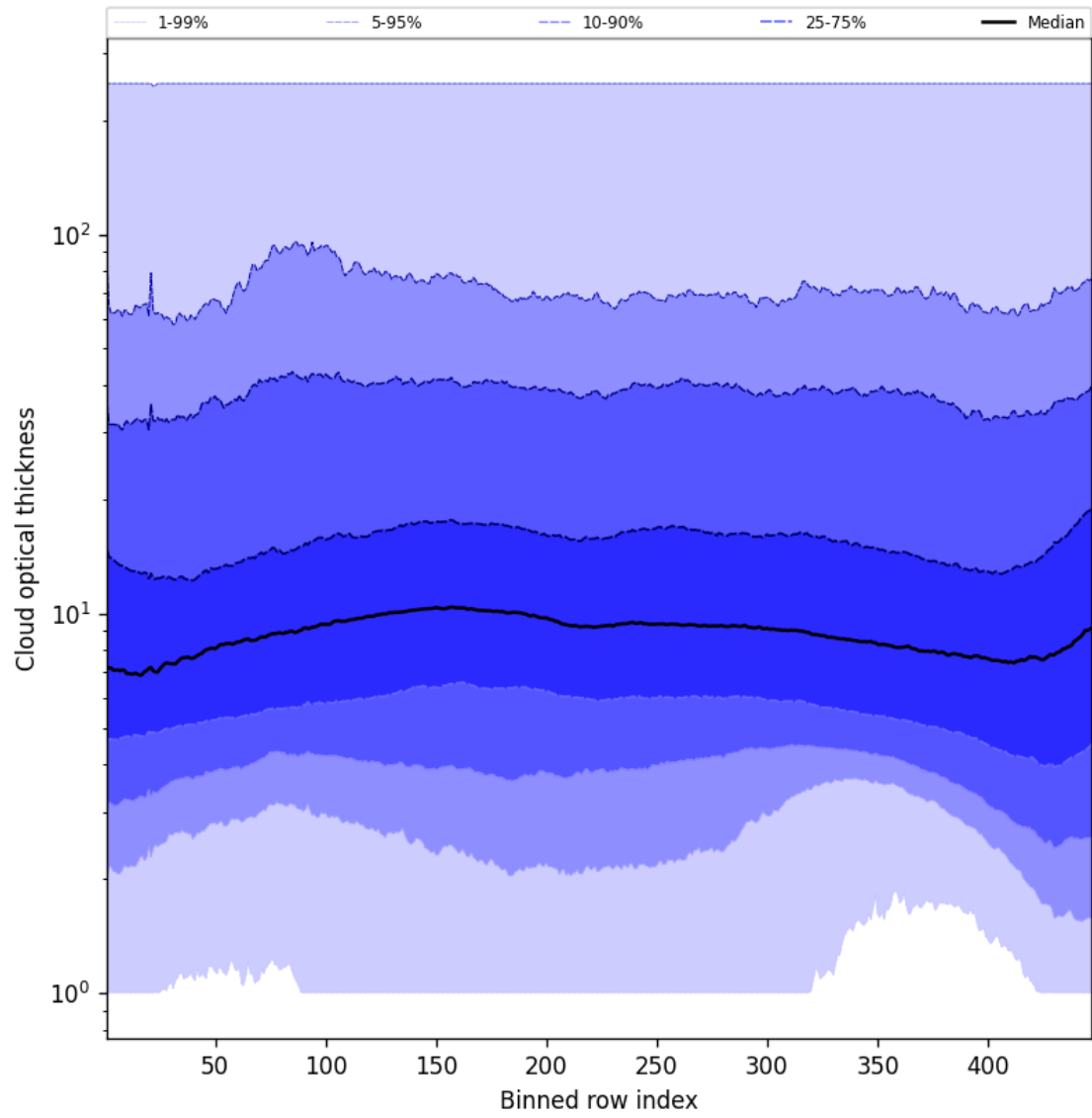
Figure 55: Along track statistics of “Cloud optical thickness” for 2025-02-24 to 2025-02-25
