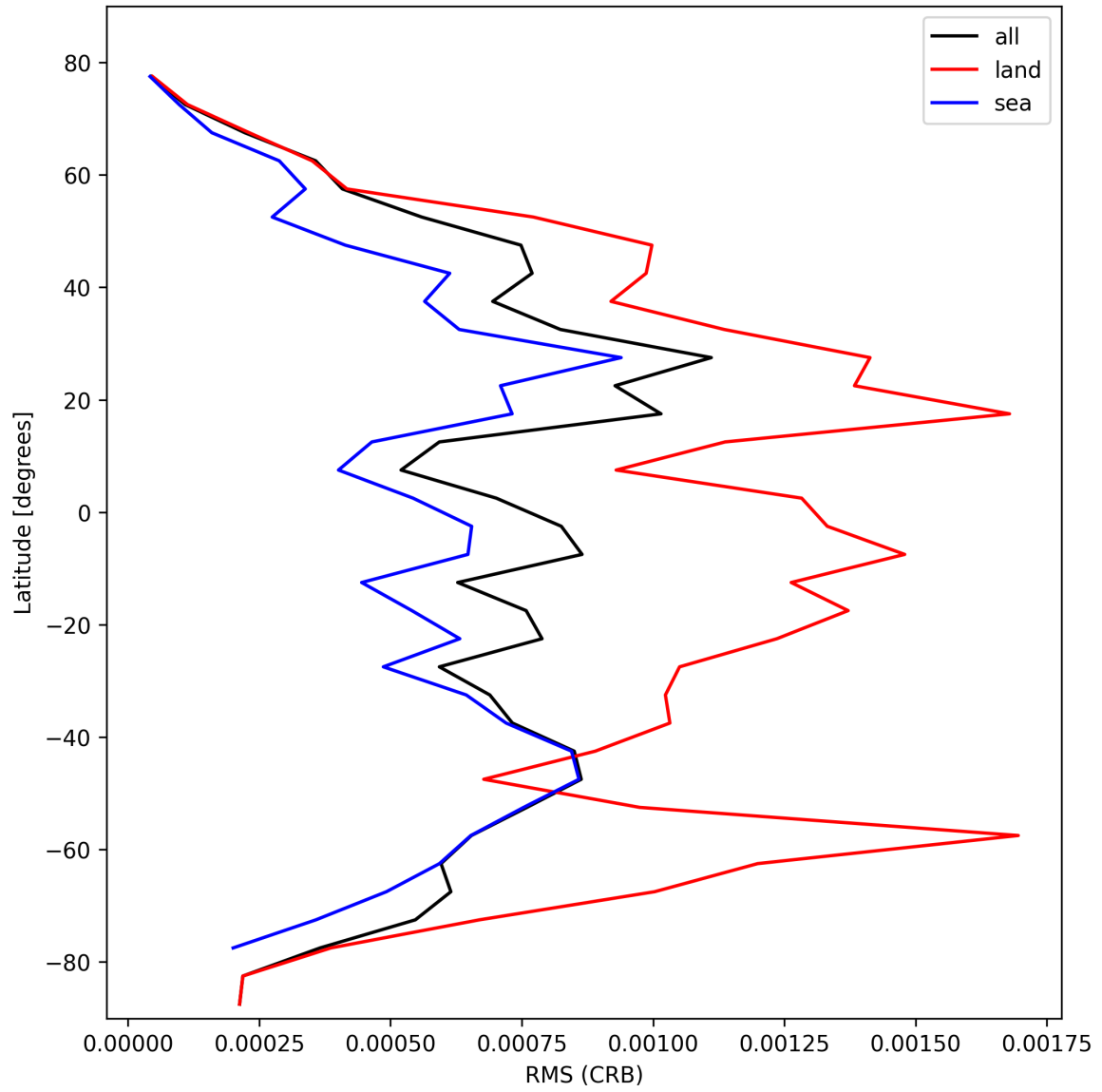
Figure 30: Zonal average of “RMS (CRB)” for 2025-02-24 to 2025-02-25.
