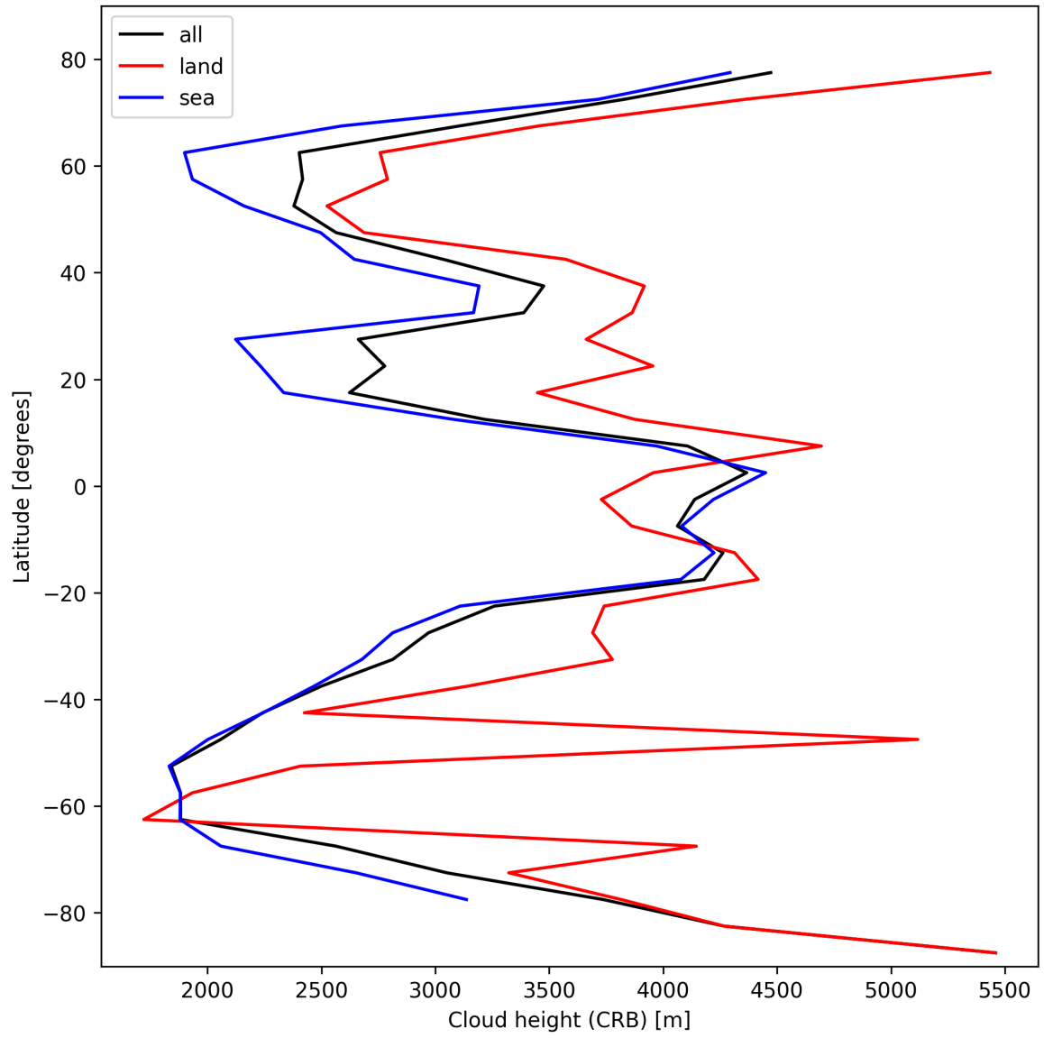
Figure 25: Zonal average of “Cloud height (CRB)” for 2025-02-24 to 2025-02-25.
