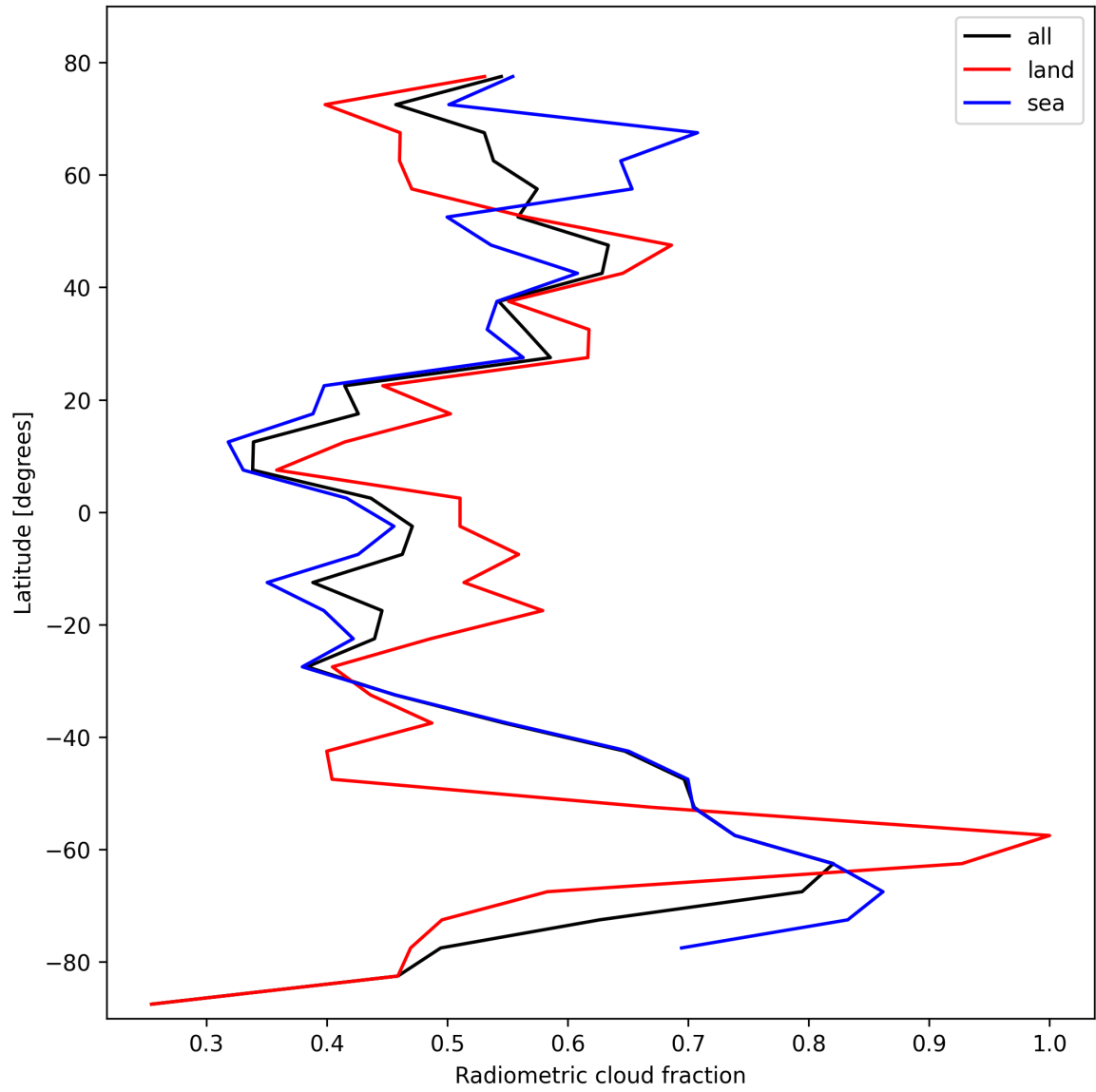
Figure 21: Zonal average of “Radiometric cloud fraction” for 2025-02-24 to 2025-02-25.
