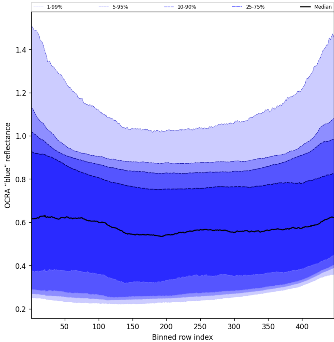
Figure 65: Along track statistics of “OCRA “blue” reflectance” for 2025-02-24 to 2025-02-25
