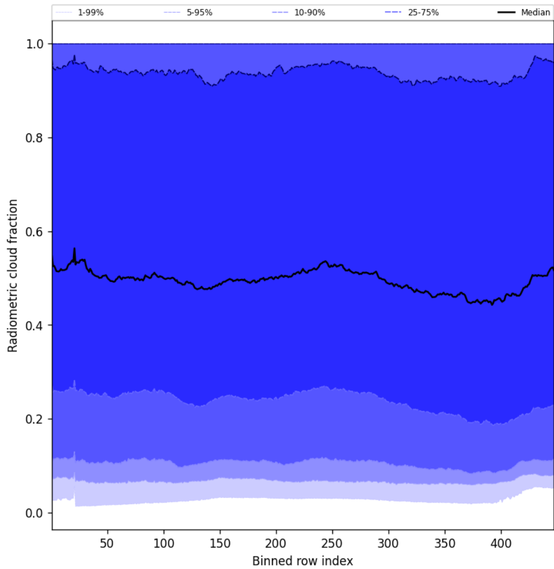
Figure 53: Along track statistics of “Radiometric cloud fraction” for 2025-02-24 to 2025-02-25
