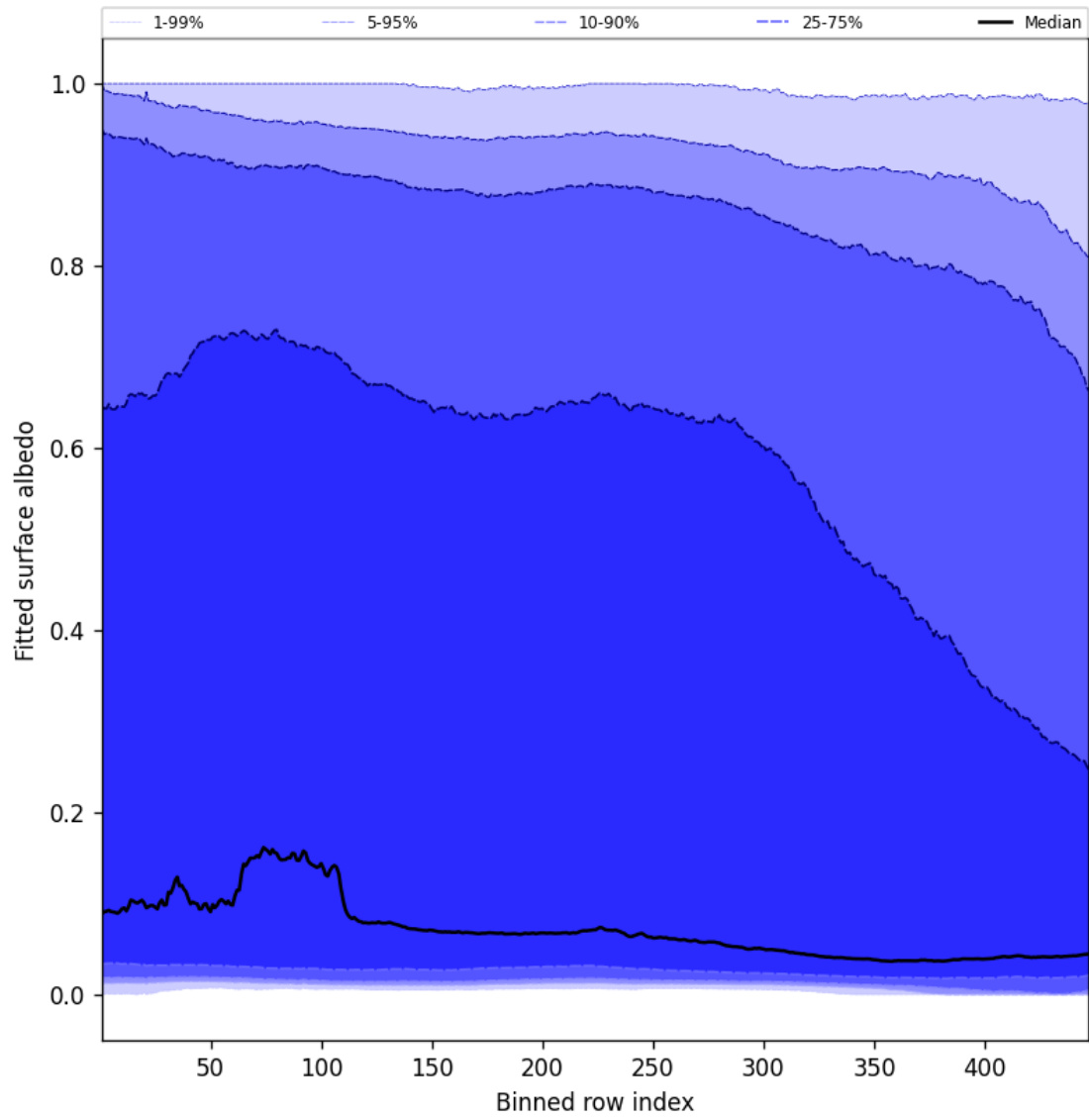
Figure 59: Along track statistics of “Fitted surface albedo” for 2025-02-24 to 2025-02-25
