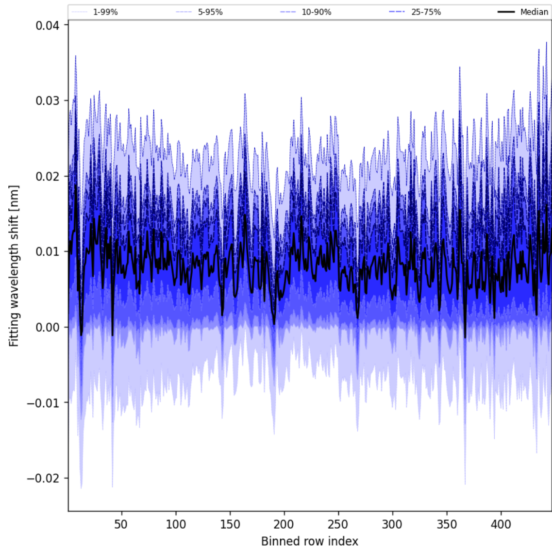
Figure 63: Along track statistics of “Fitting wavelength shift” for 2025-02-24 to 2025-02-25
