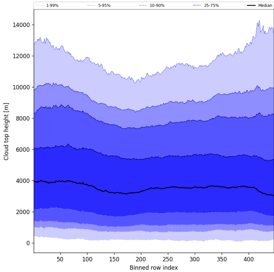
Figure 54: Along track statistics of “Cloud top height” for 2025-02-24 to 2025-02-25
