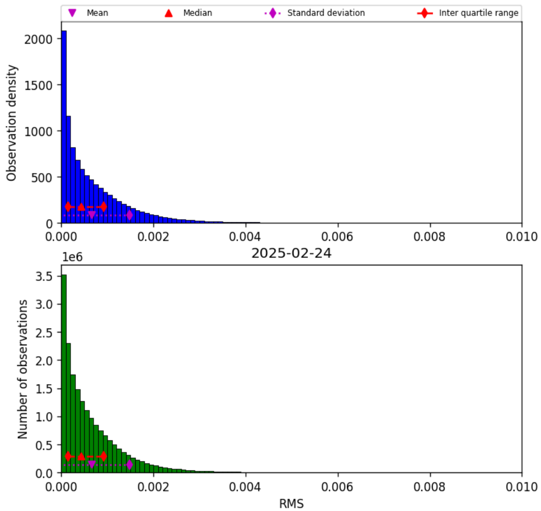
Figure 45: Histogram of “RMS” for 2025-02-24 to 2025-02-25
