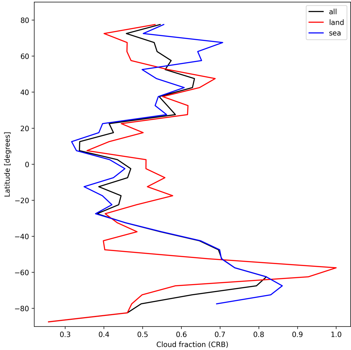
Figure 24: Zonal average of “Cloud fraction (CRB)” for 2025-02-24 to 2025-02-25.
