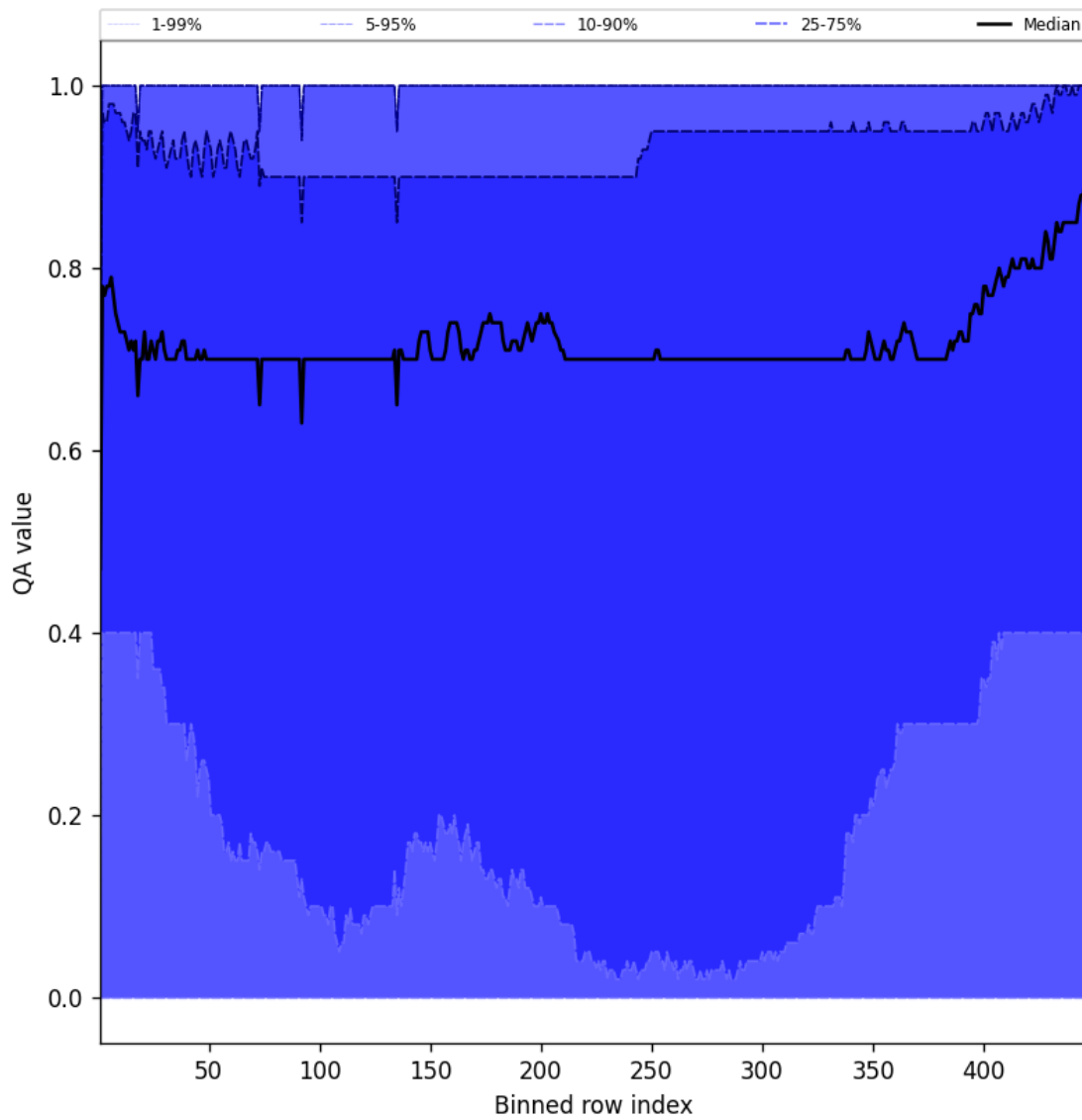
Figure 52: Along track statistics of “QA value” for 2025-02-24 to 2025-02-25
