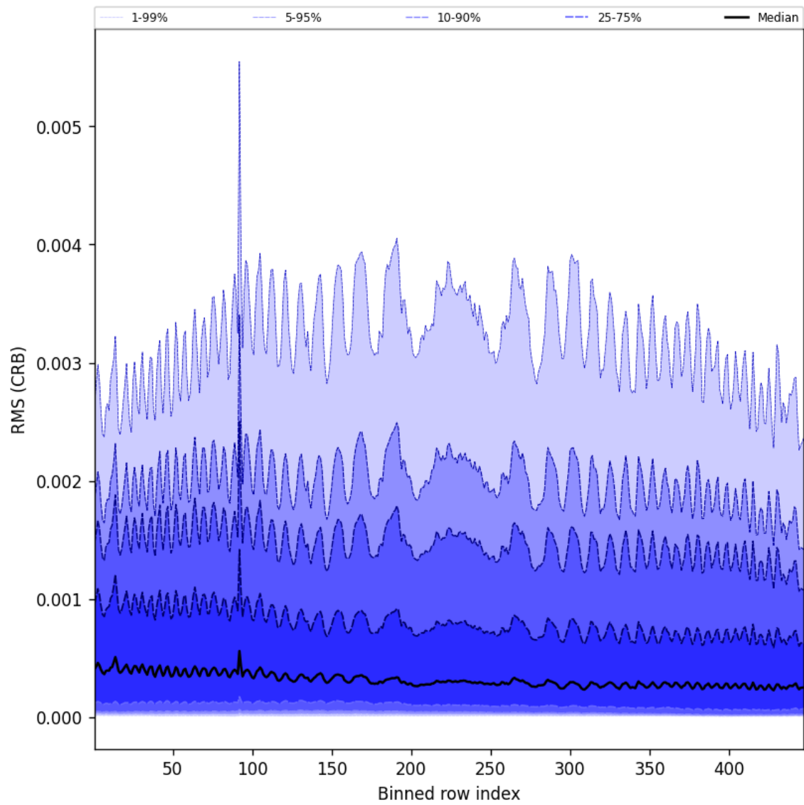
Figure 62: Along track statistics of “RMS (CRB)” for 2025-02-24 to 2025-02-25
