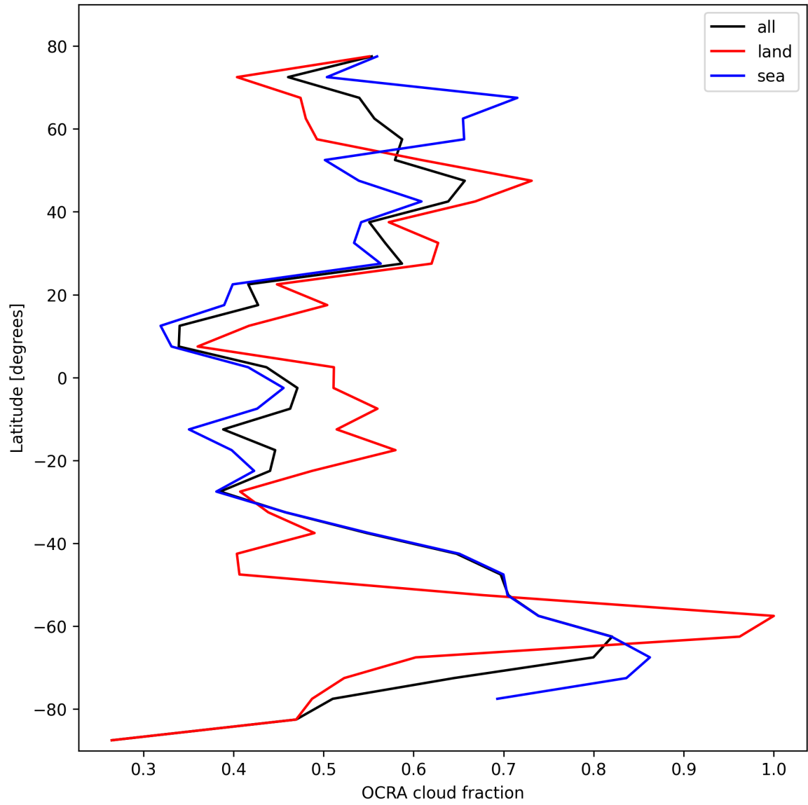
Figure 32: Zonal average of “OCRA cloud fraction” for 2025-02-24 to 2025-02-25.
