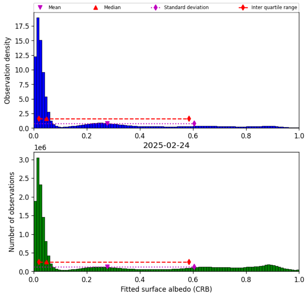
Figure 44: Histogram of “Fitted surface albedo (CRB)” for 2025-02-24 to 2025-02-25
