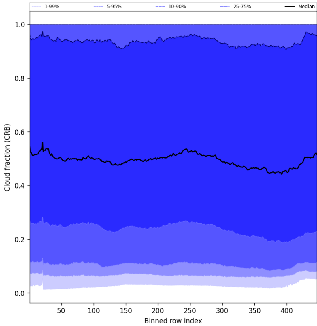
Figure 56: Along track statistics of “Cloud fraction (CRB)” for 2025-02-24 to 2025-02-25
