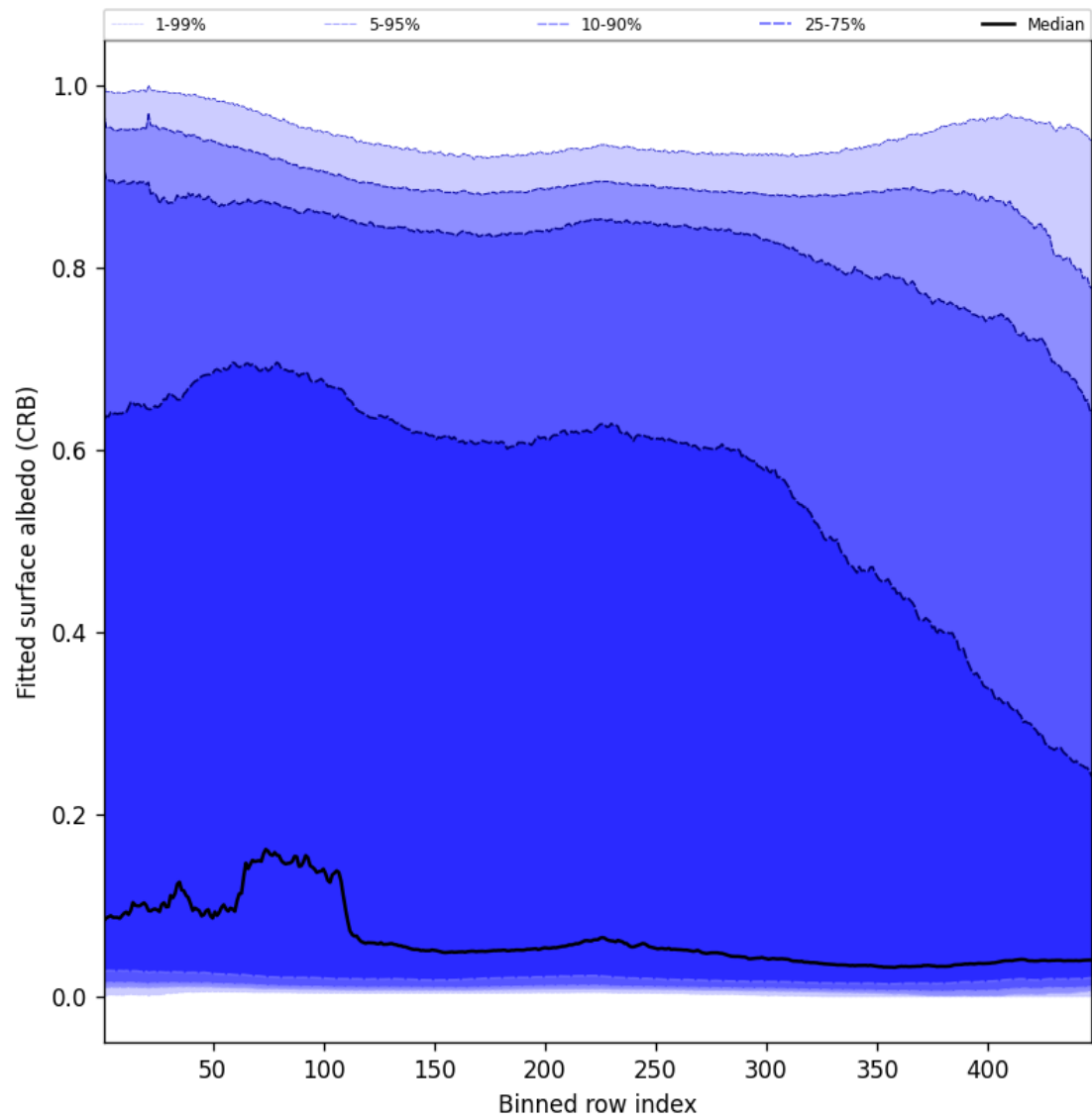
Figure 60: Along track statistics of “Fitted surface albedo (CRB)” for 2025-02-24 to 2025-02-25
