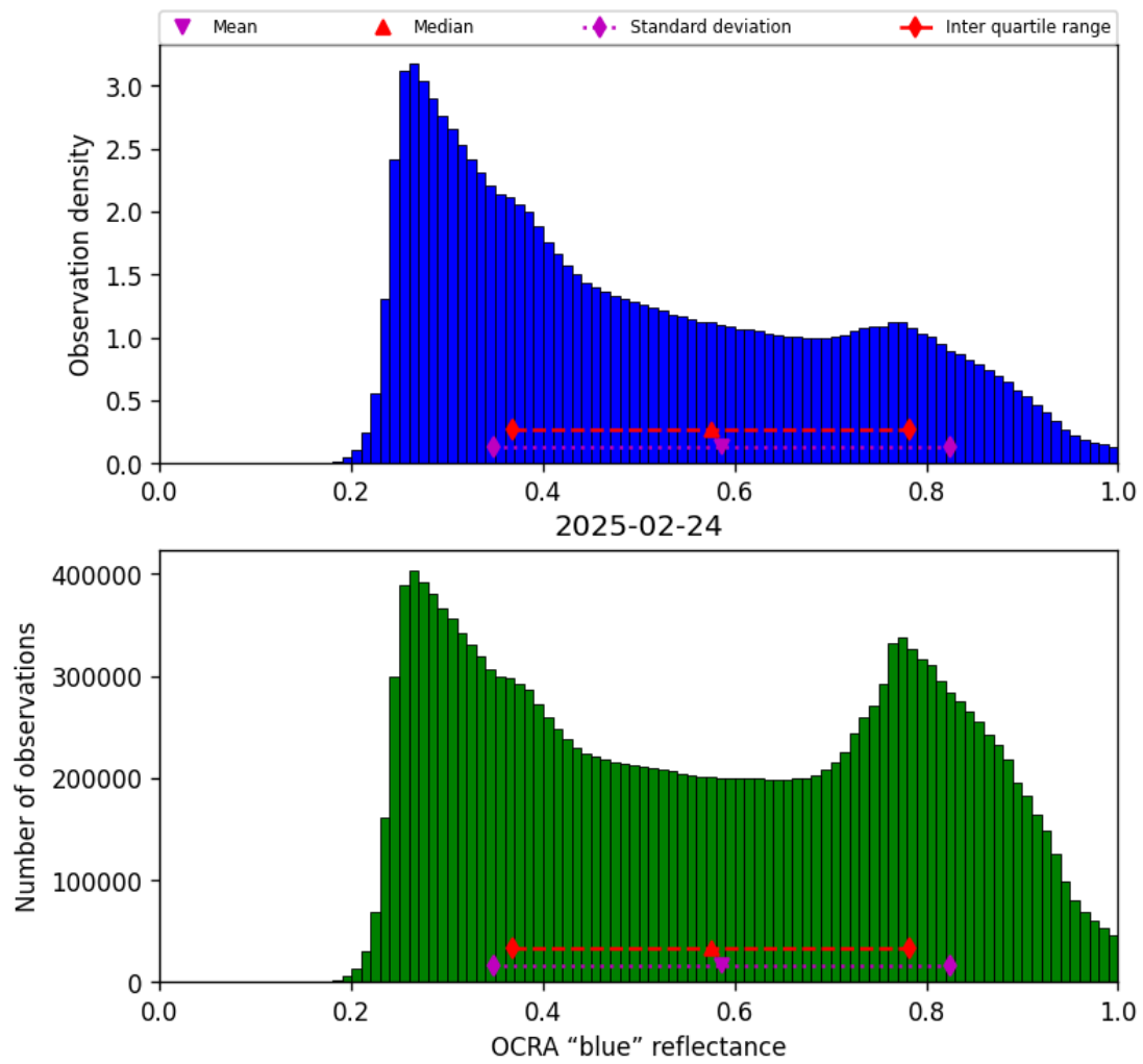
Figure 49: Histogram of “OCRA “blue” reflectance” for 2025-02-24 to 2025-02-25
