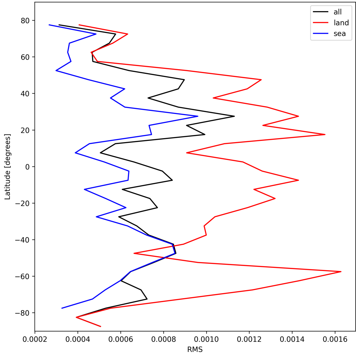
Figure 29: Zonal average of “RMS” for 2025-02-24 to 2025-02-25.
