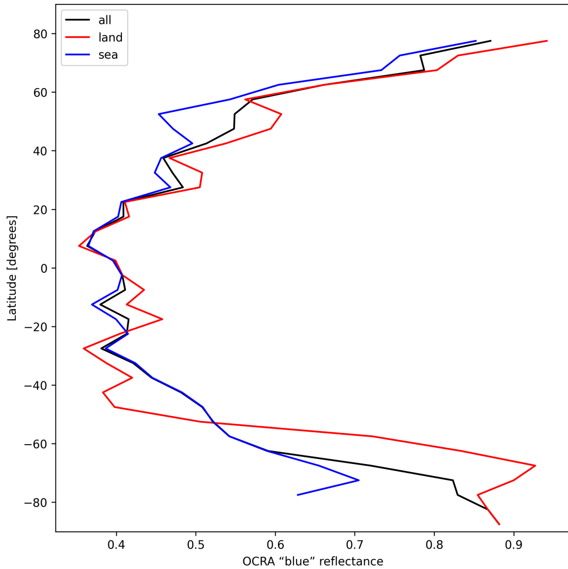
Figure 33: Zonal average of “OCRA “blue” reflectance” for 2025-02-24 to 2025-02-25.
