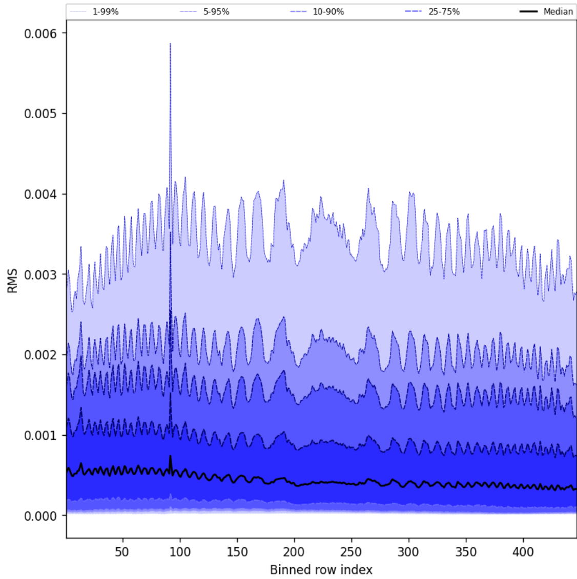
Figure 61: Along track statistics of “RMS” for 2025-02-24 to 2025-02-25
