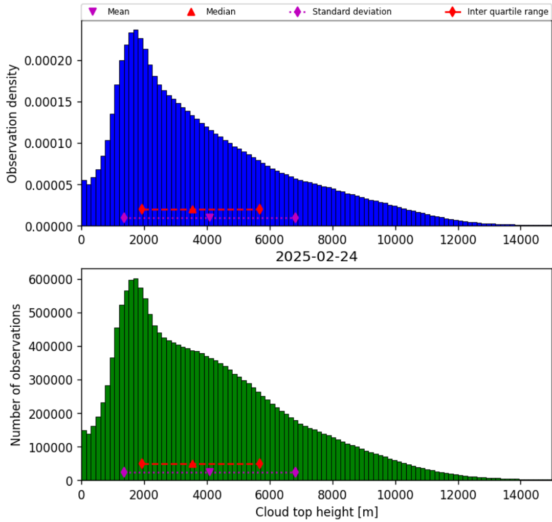
Figure 38: Histogram of “Cloud top height” for 2025-02-24 to 2025-02-25
