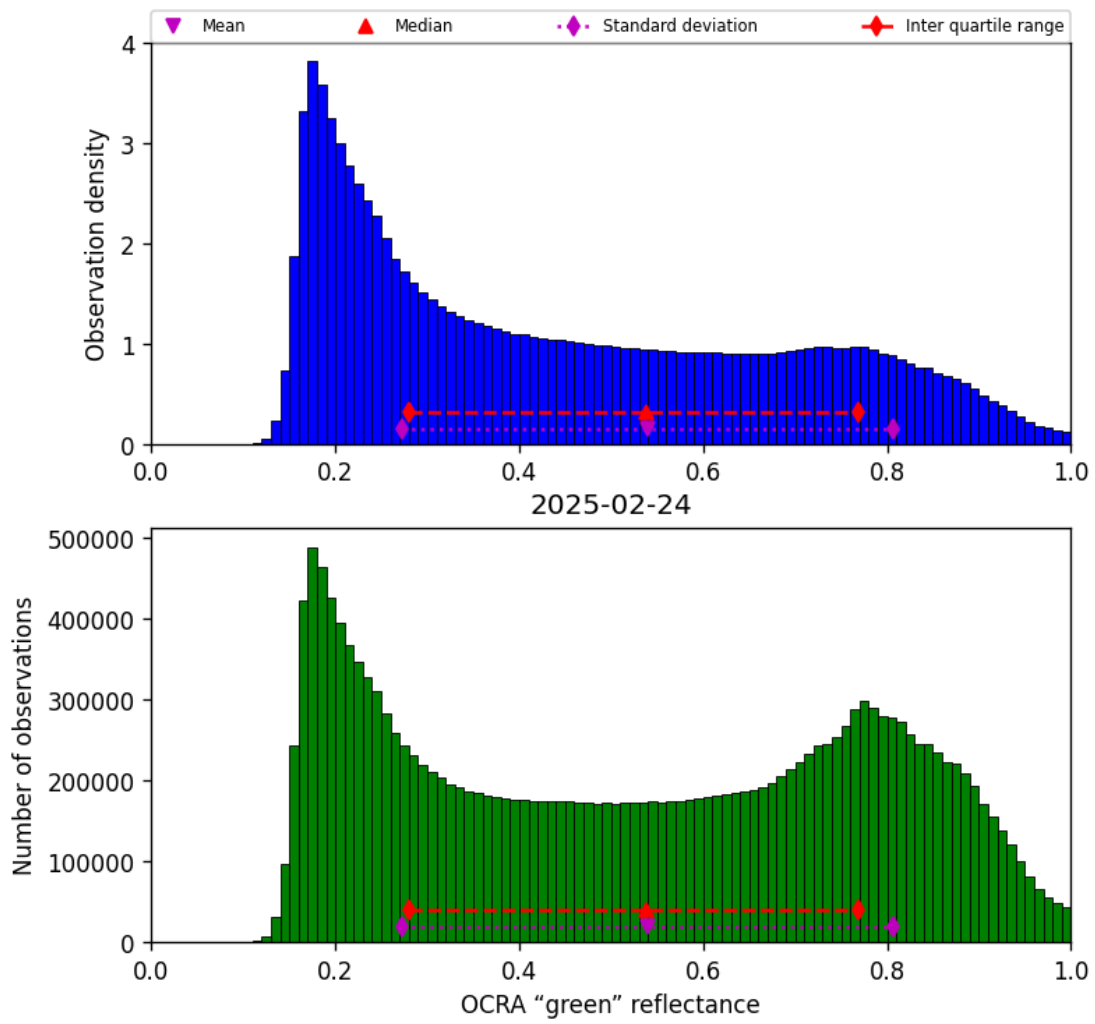
Figure 50: Histogram of “OCRA “green” reflectance” for 2025-02-24 to 2025-02-25
