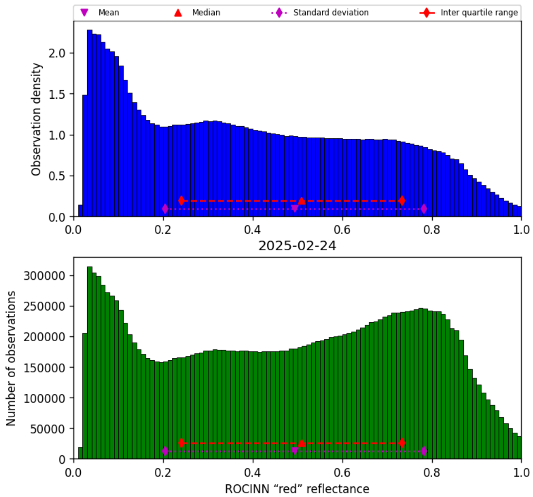
Figure 51: Histogram of “ROCINN “red” reflectance” for 2025-02-24 to 2025-02-25
