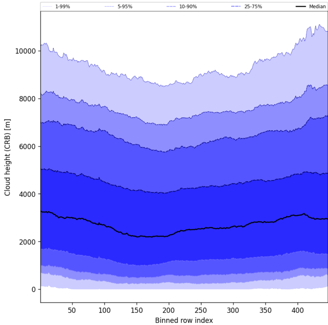
Figure 57: Along track statistics of “Cloud height (CRB)” for 2025-02-24 to 2025-02-25
