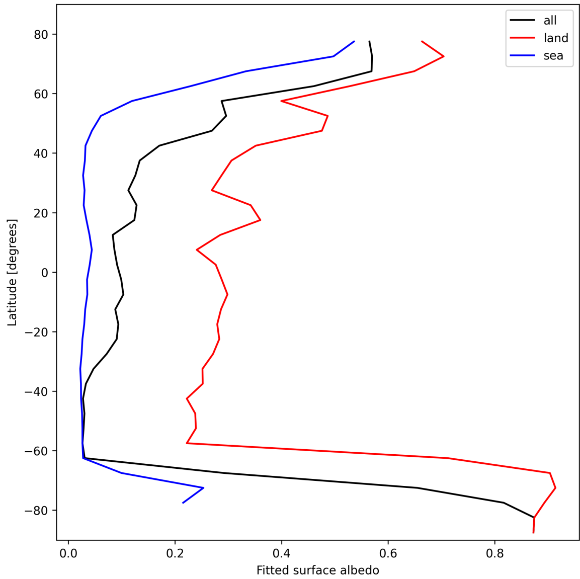
Figure 27: Zonal average of “Fitted surface albedo” for 2025-02-24 to 2025-02-25.
