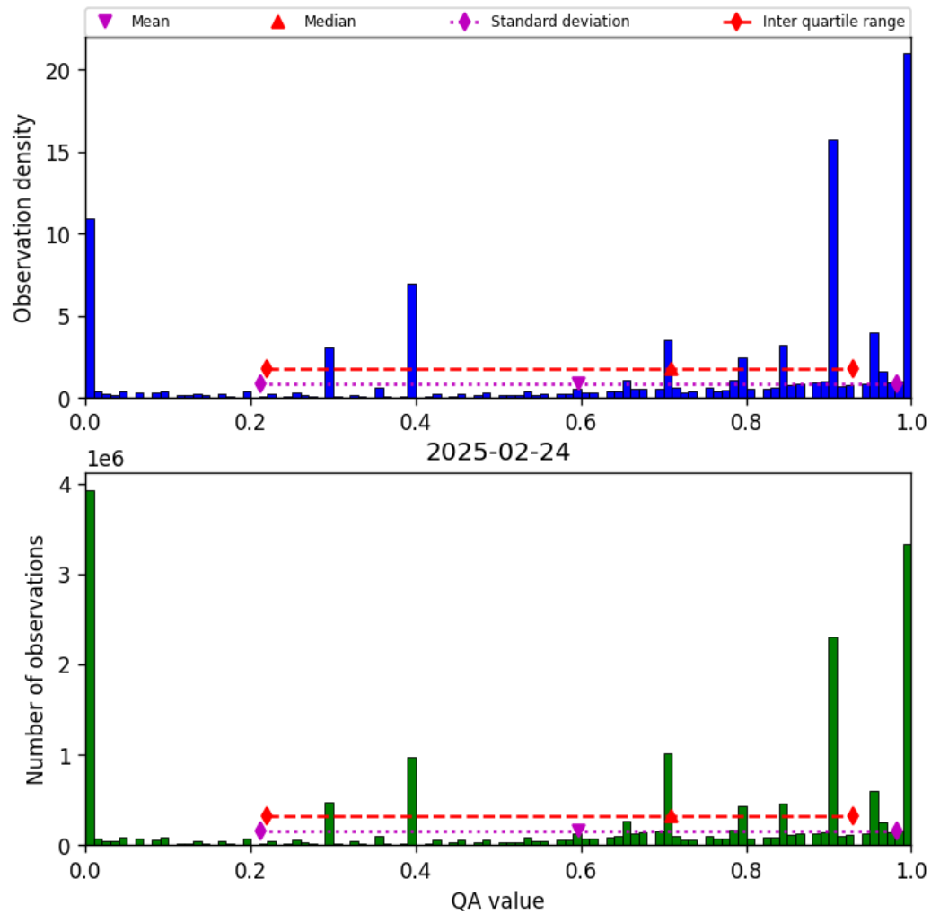
Figure 36: Histogram of “QA value” for 2025-02-24 to 2025-02-25
