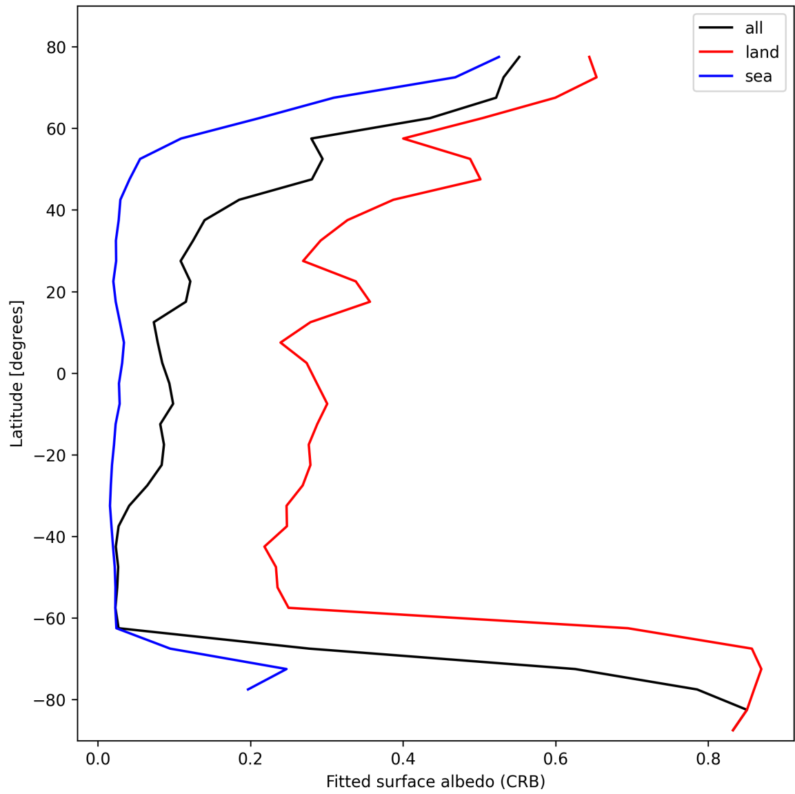
Figure 28: Zonal average of “Fitted surface albedo (CRB)” for 2025-02-24 to 2025-02-25.
