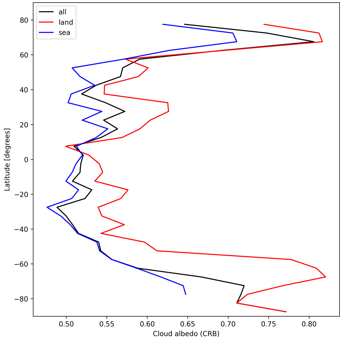
Figure 26: Zonal average of “Cloud albedo (CRB)” for 2025-02-24 to 2025-02-25.
