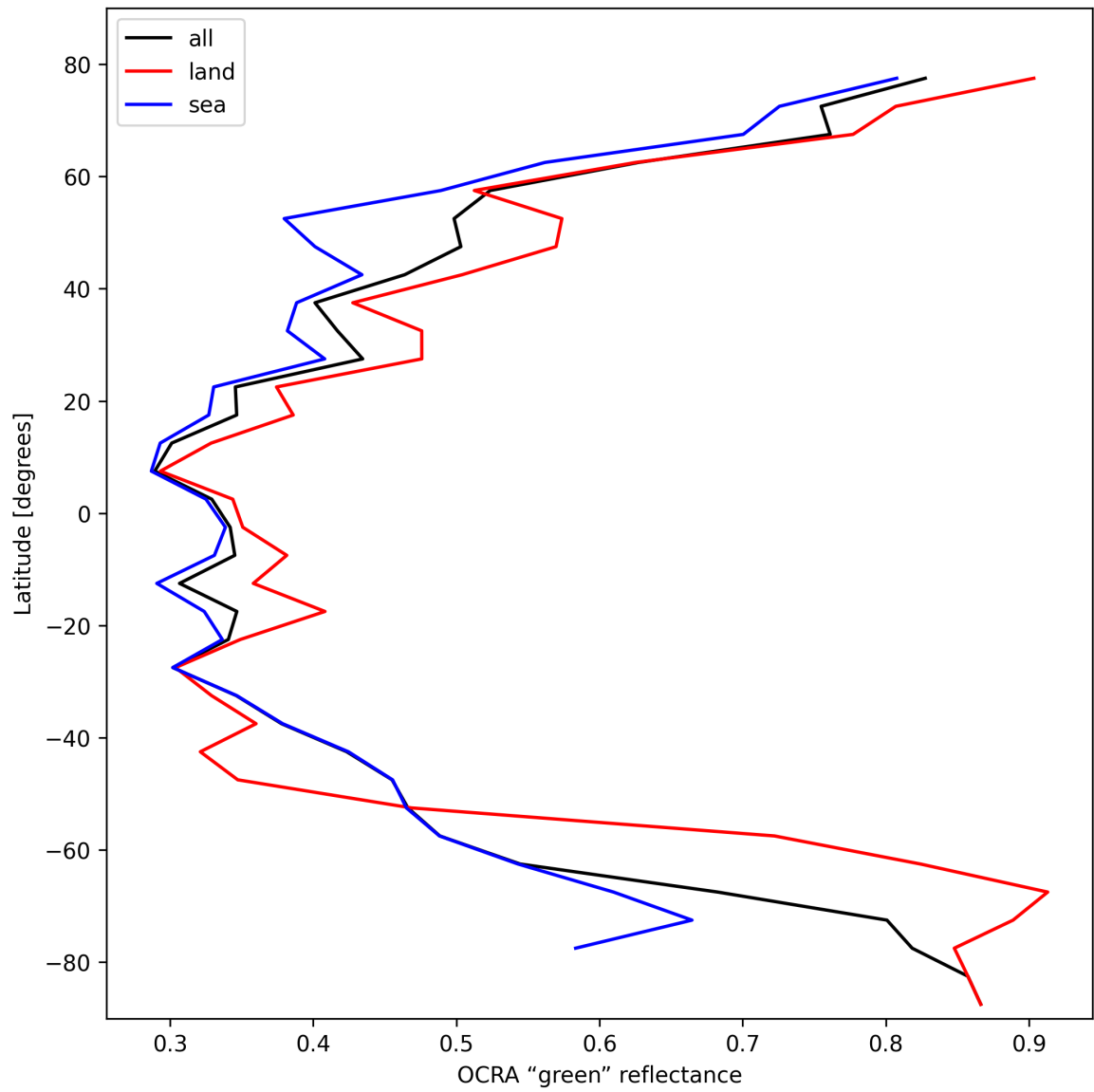
Figure 34: Zonal average of “OCRA “green” reflectance” for 2025-02-24 to 2025-02-25.
