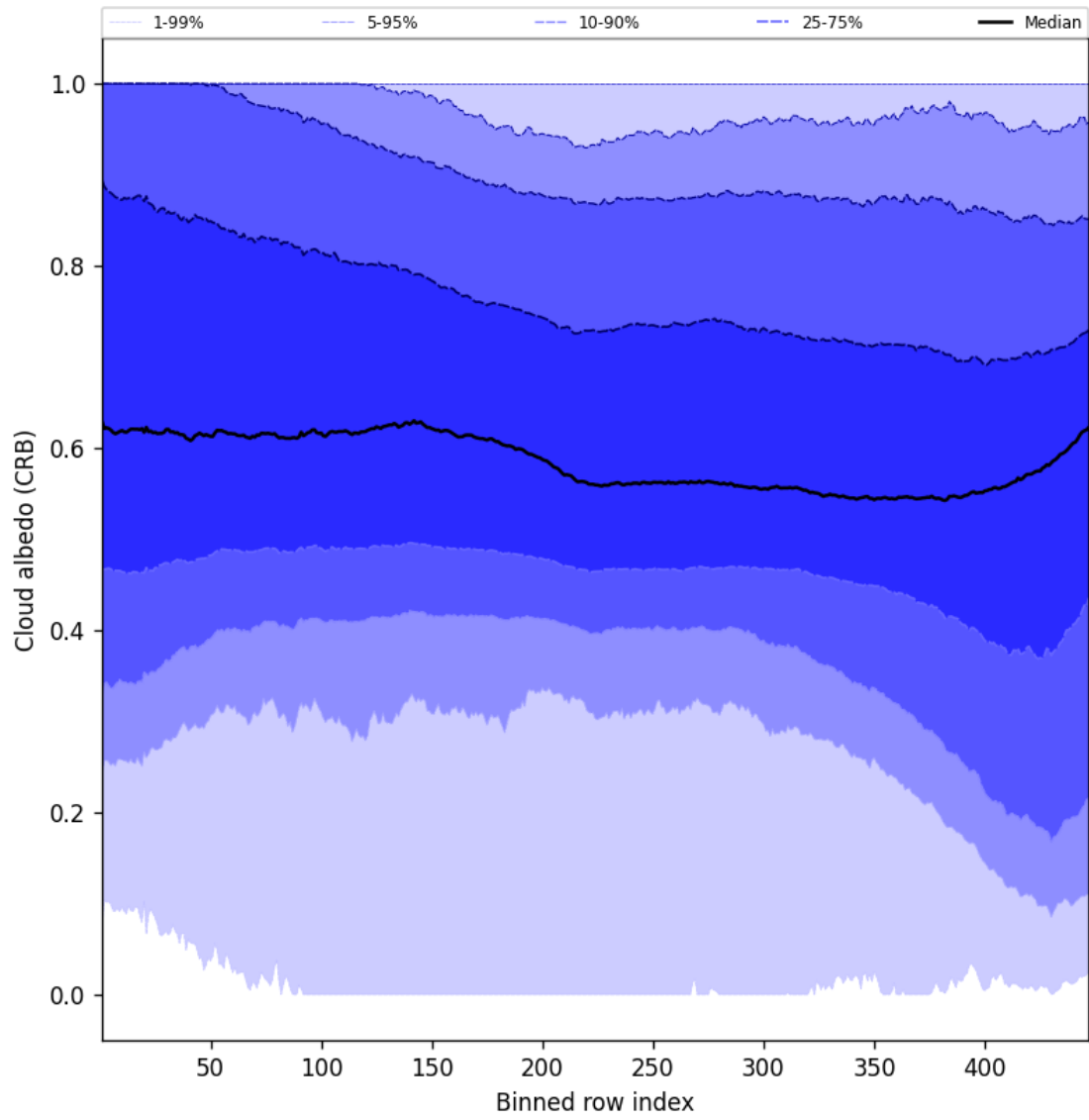
Figure 58: Along track statistics of “Cloud albedo (CRB)” for 2025-02-24 to 2025-02-25
