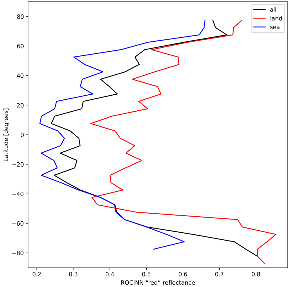
Figure 35: Zonal average of “ROCINN “red” reflectance” for 2025-02-24 to 2025-02-25.
