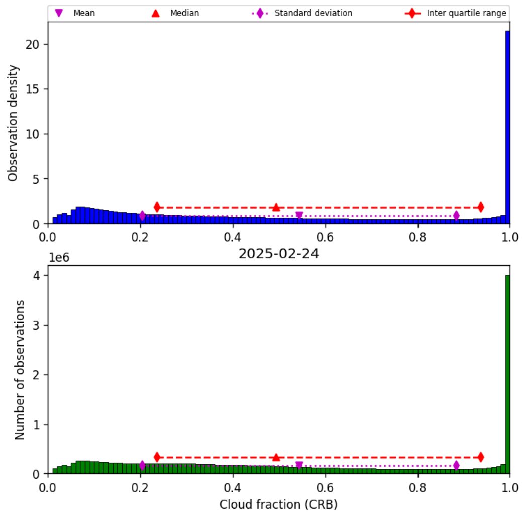
Figure 40: Histogram of “Cloud fraction (CRB)” for 2025-02-24 to 2025-02-25
