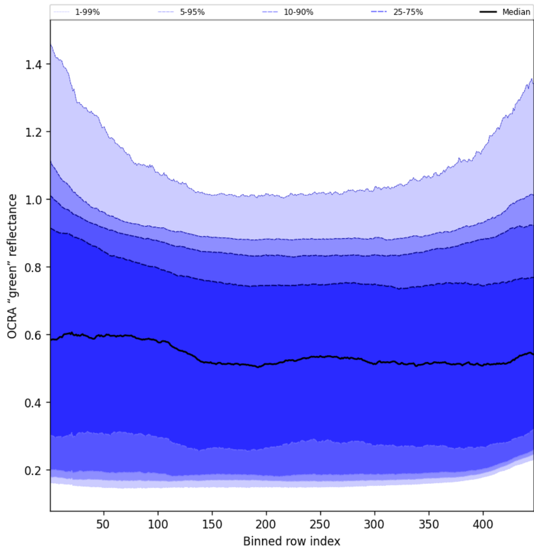
Figure 66: Along track statistics of “OCRA “green” reflectance” for 2025-02-24 to 2025-02-25
