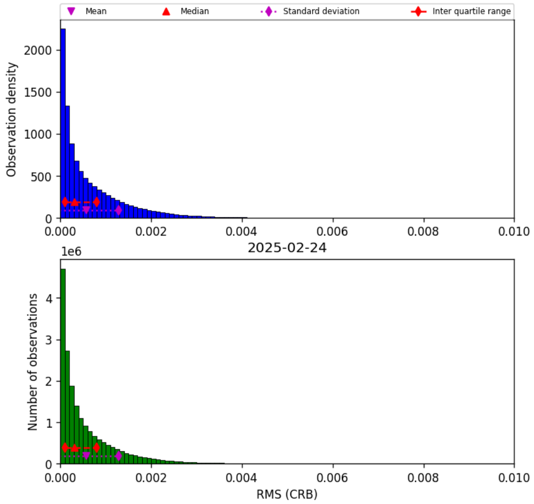
Figure 46: Histogram of “RMS (CRB)” for 2025-02-24 to 2025-02-25
