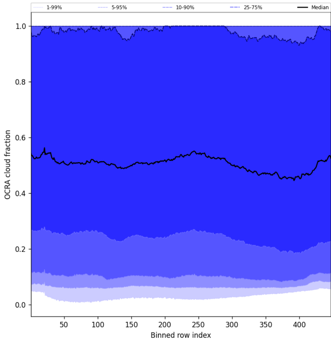
Figure 64: Along track statistics of “OCRA cloud fraction” for 2025-02-24 to 2025-02-25
