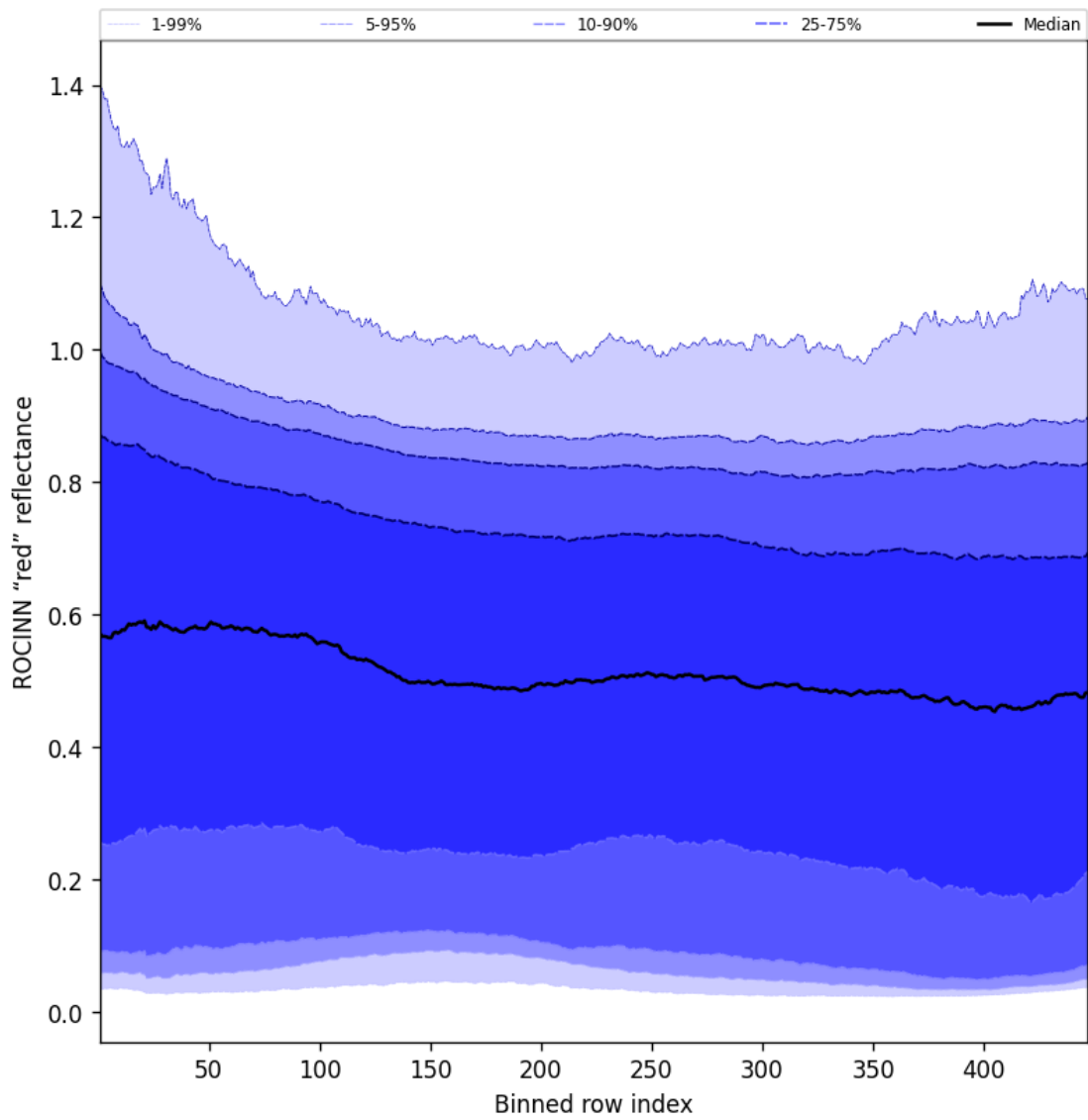
Figure 67: Along track statistics of "ROCINN "red" reflectance" for 2025-02-24 to 2025-02-25
