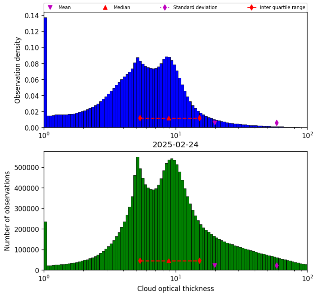
Figure 39: Histogram of “Cloud optical thickness” for 2025-02-24 to 2025-02-25
