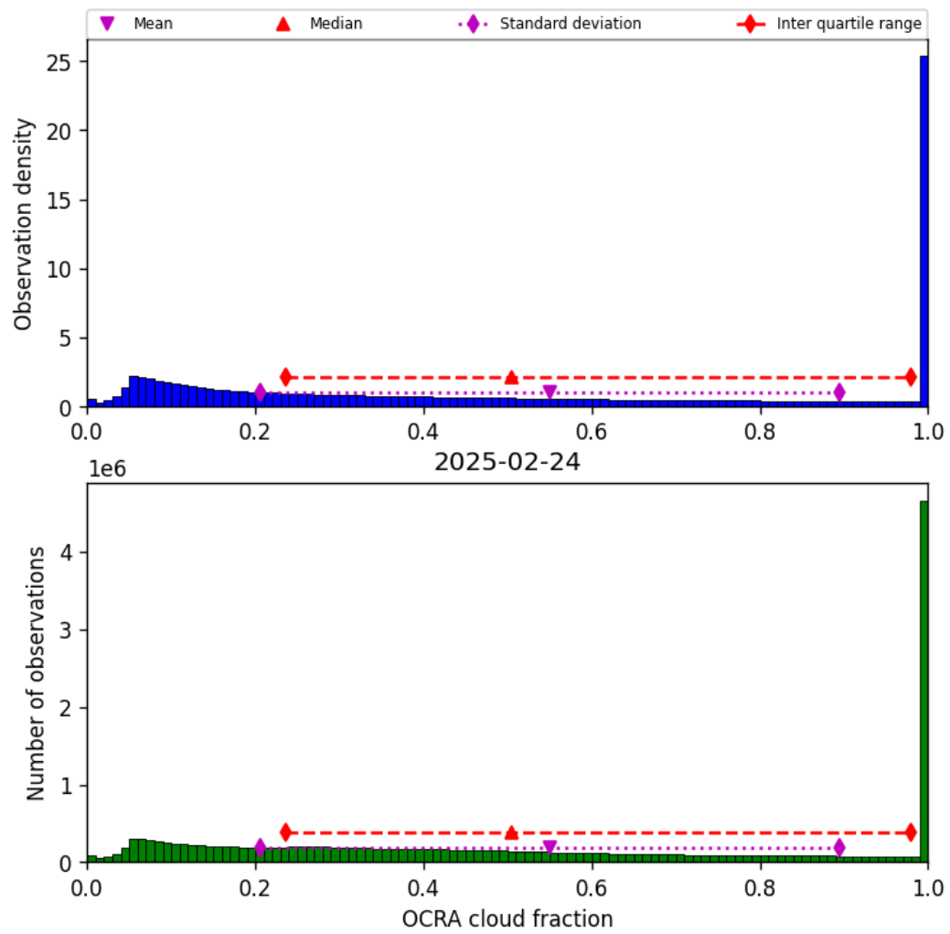
Figure 48: Histogram of “OCRA cloud fraction” for 2025-02-24 to 2025-02-25
