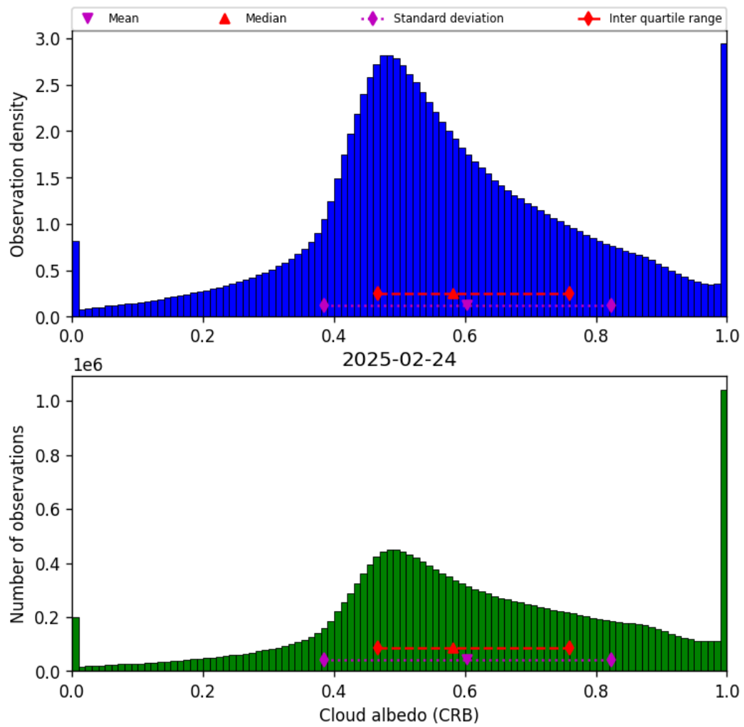
Figure 42: Histogram of “Cloud albedo (CRB)” for 2025-02-24 to 2025-02-25
