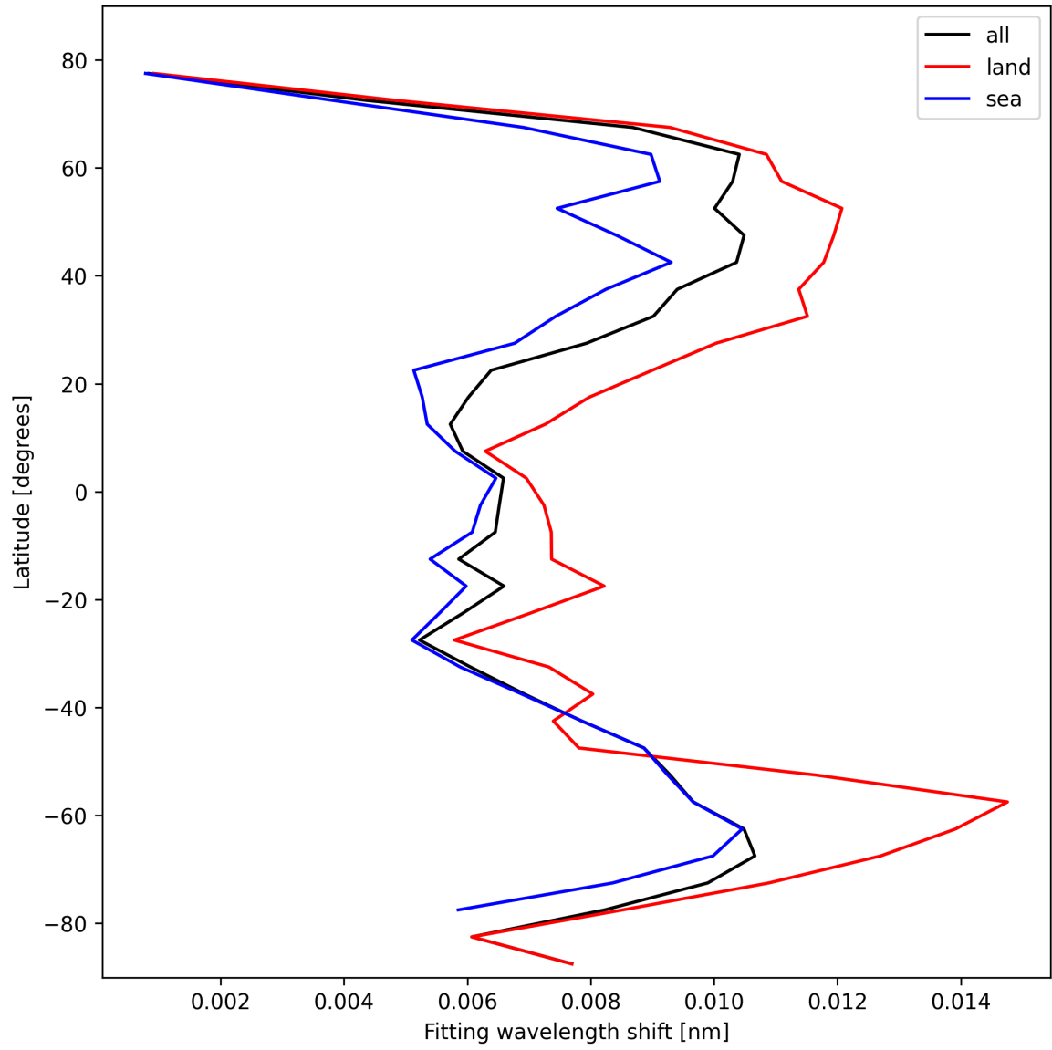
Figure 31: Zonal average of “Fitting wavelength shift” for 2025-02-24 to 2025-02-25.
