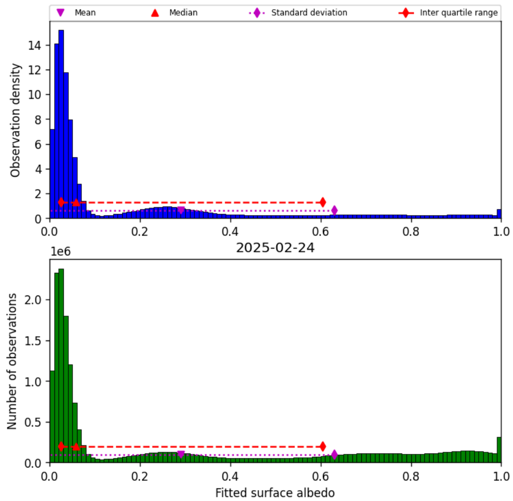
Figure 43: Histogram of “Fitted surface albedo” for 2025-02-24 to 2025-02-25
