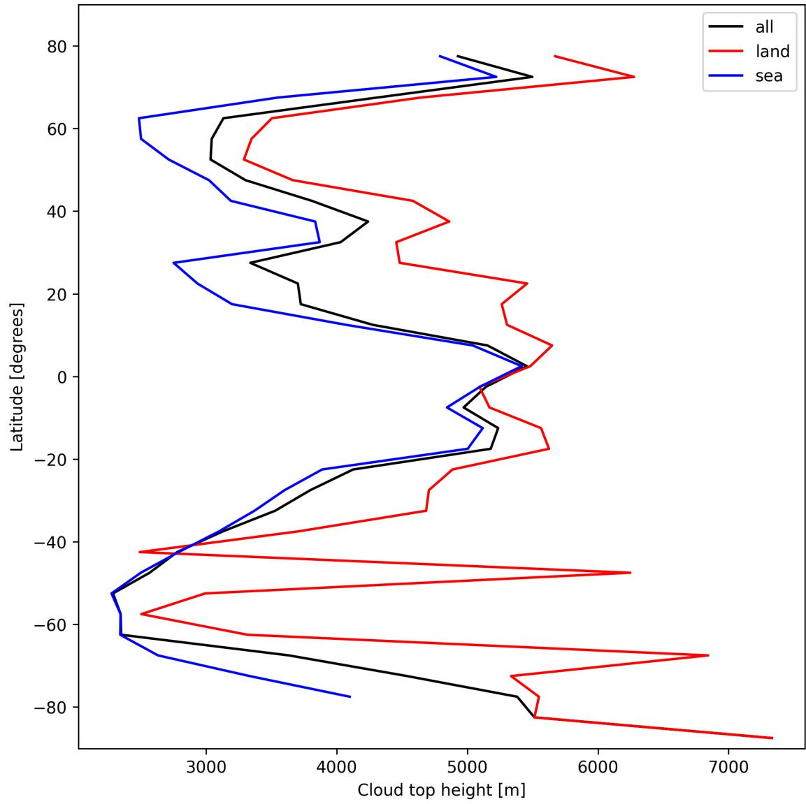
Figure 22: Zonal average of “Cloud top height” for 2025-02-24 to 2025-02-25.
