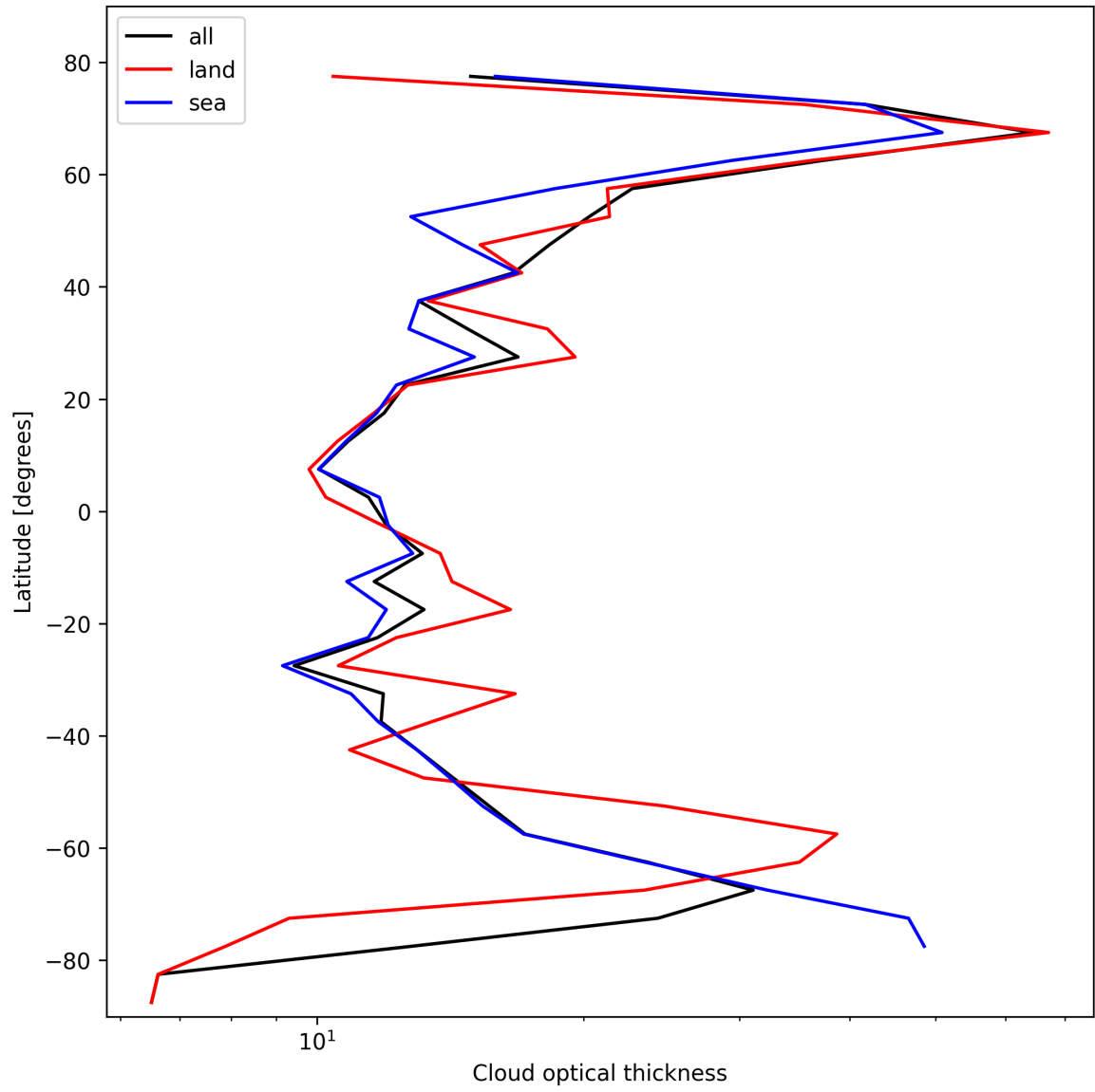
Figure 23: Zonal average of “Cloud optical thickness” for 2025-02-24 to 2025-02-25.
