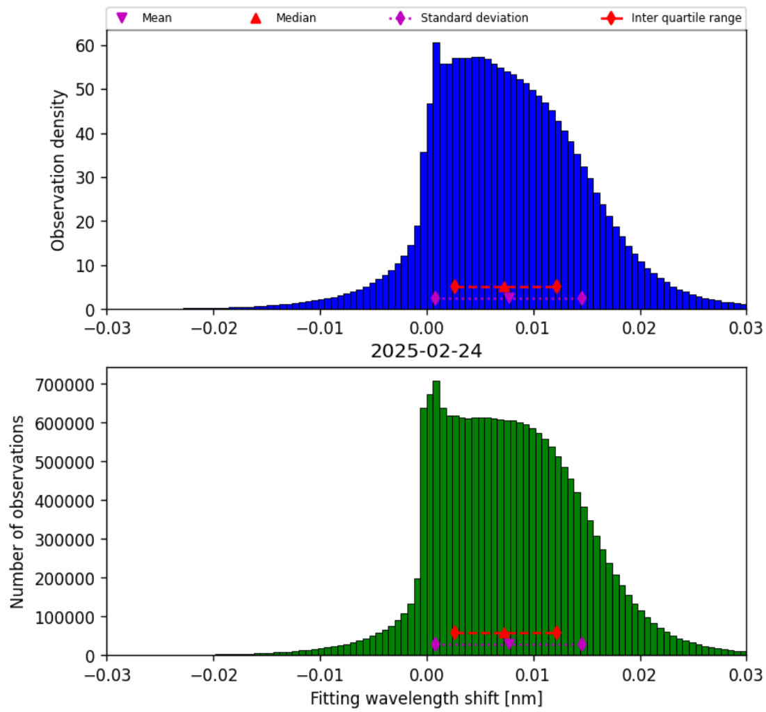
Figure 47: Histogram of “Fitting wavelength shift” for 2025-02-24 to 2025-02-25
