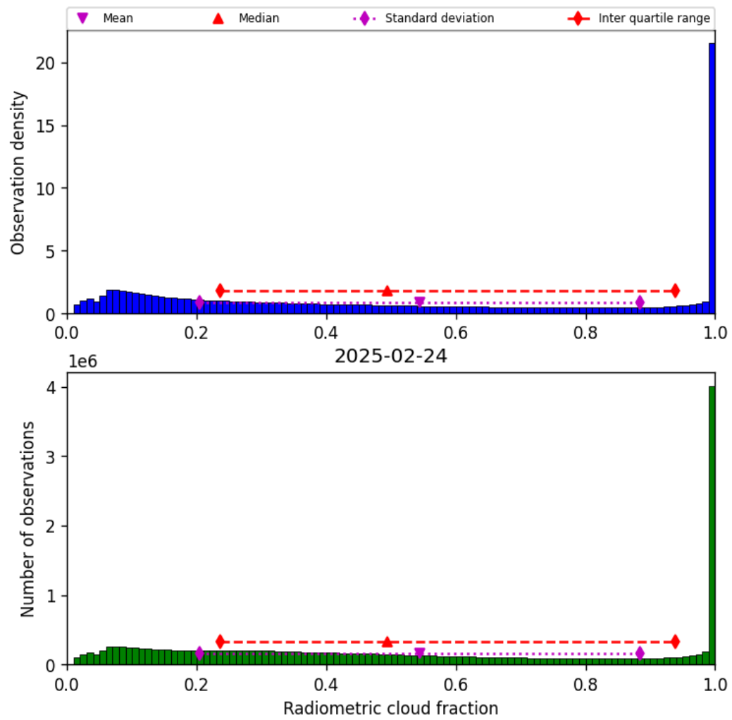
Figure 37: Histogram of “Radiometric cloud fraction” for 2025-02-24 to 2025-02-25
