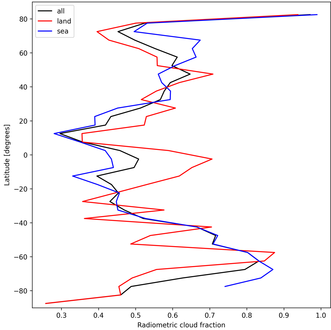
Figure 21: Zonal average of “Radiometric cloud fraction” for 2025-02-25 to 2025-02-26.
