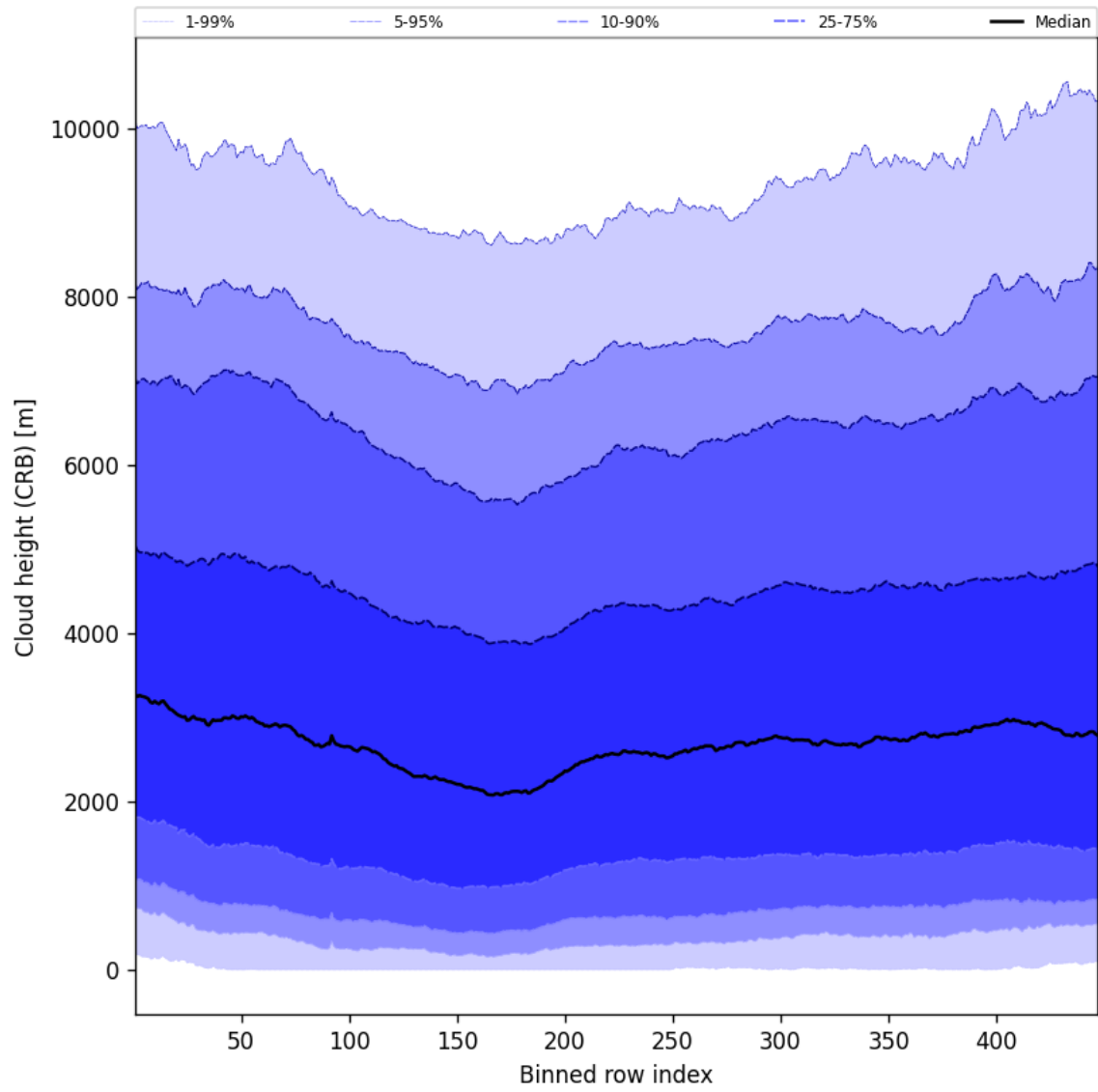
Figure 57: Along track statistics of “Cloud height (CRB)” for 2025-02-25 to 2025-02-26
