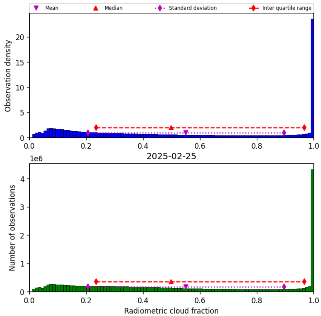
Figure 37: Histogram of “Radiometric cloud fraction” for 2025-02-25 to 2025-02-26
