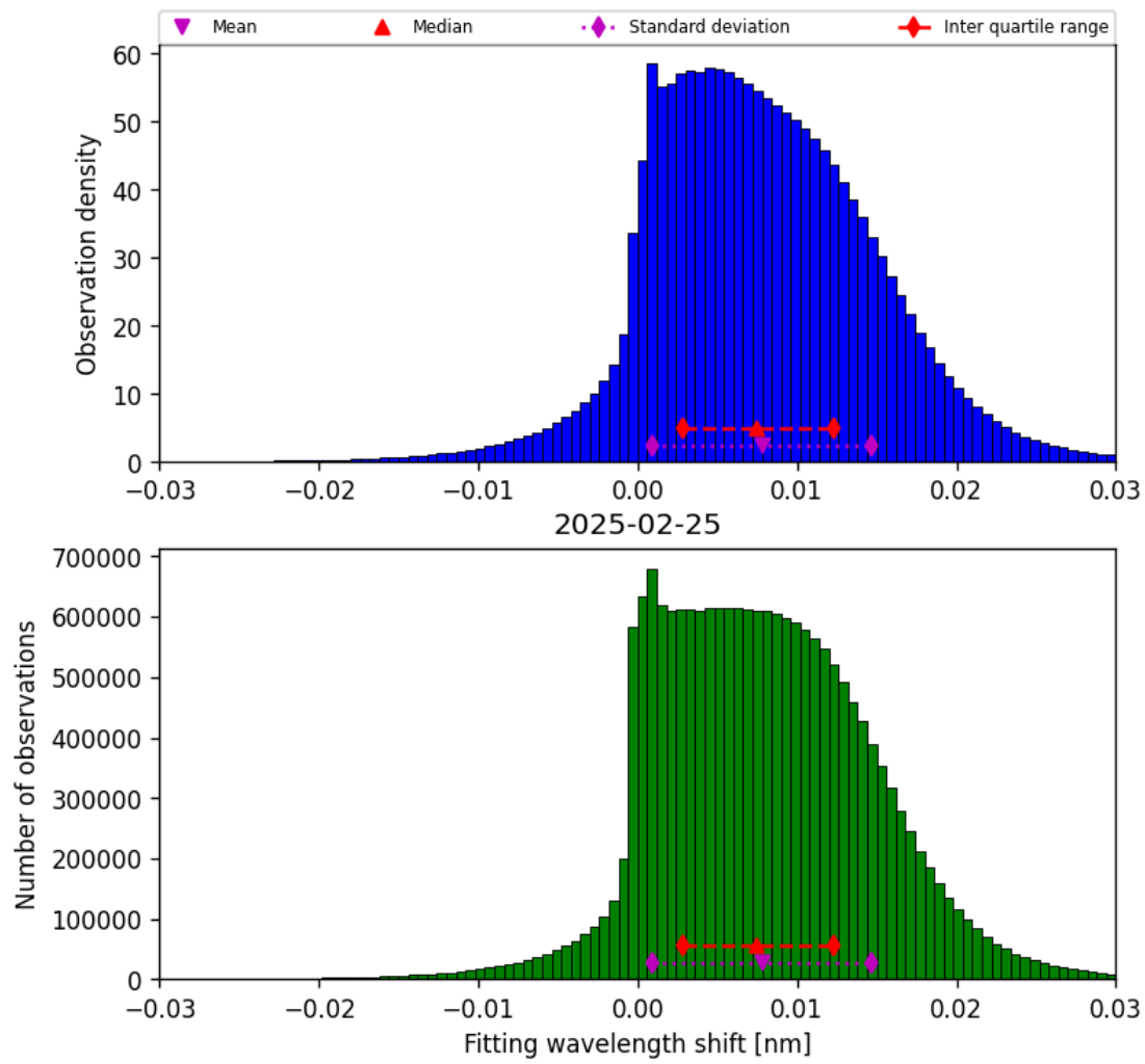
Figure 47: Histogram of “Fitting wavelength shift” for 2025-02-25 to 2025-02-26
