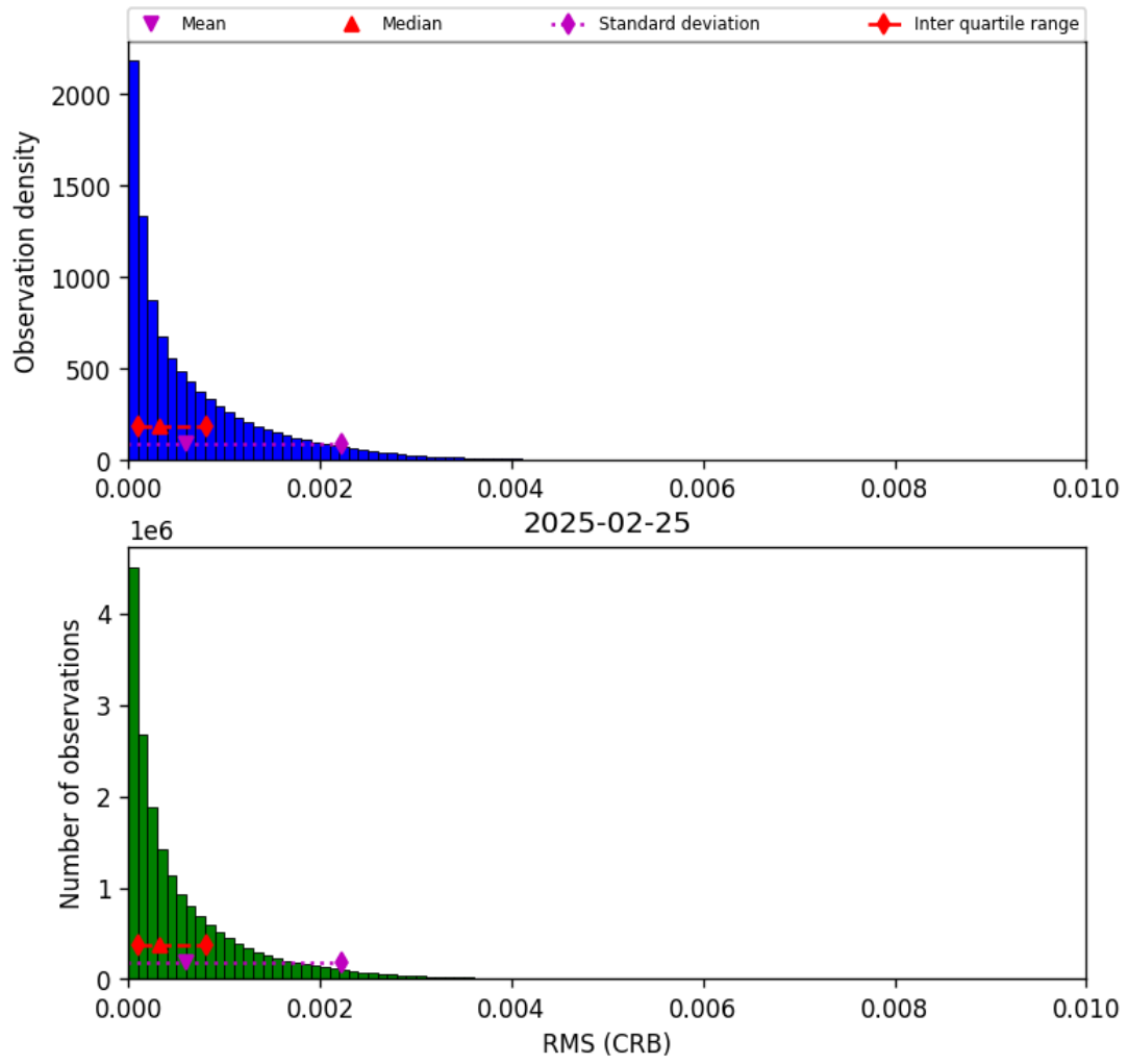
Figure 46: Histogram of “RMS (CRB)” for 2025-02-25 to 2025-02-26
