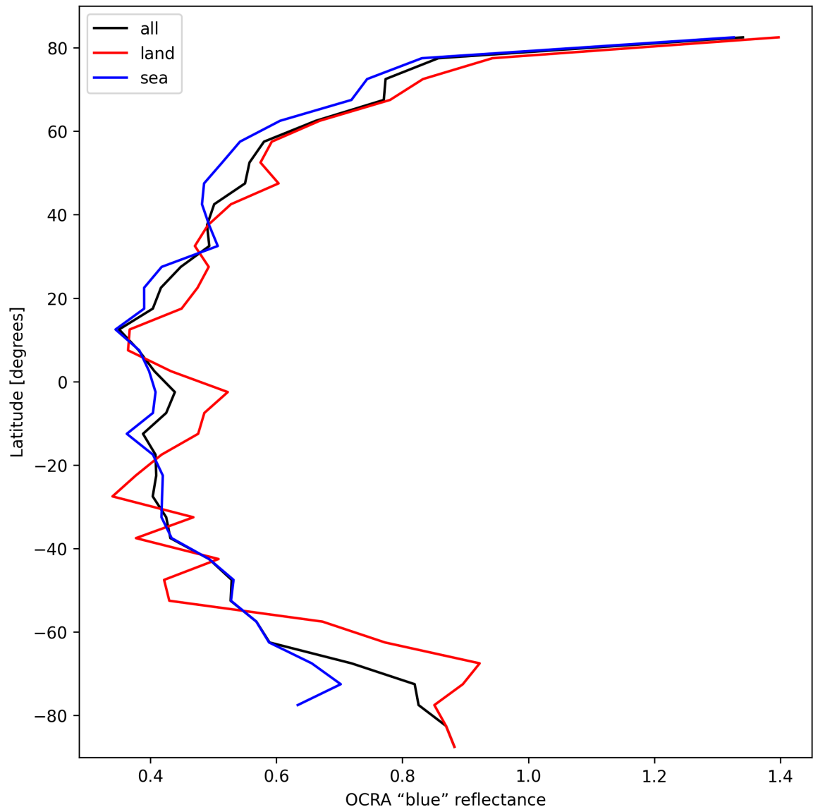
Figure 33: Zonal average of “OCRA “blue” reflectance” for 2025-02-25 to 2025-02-26.
