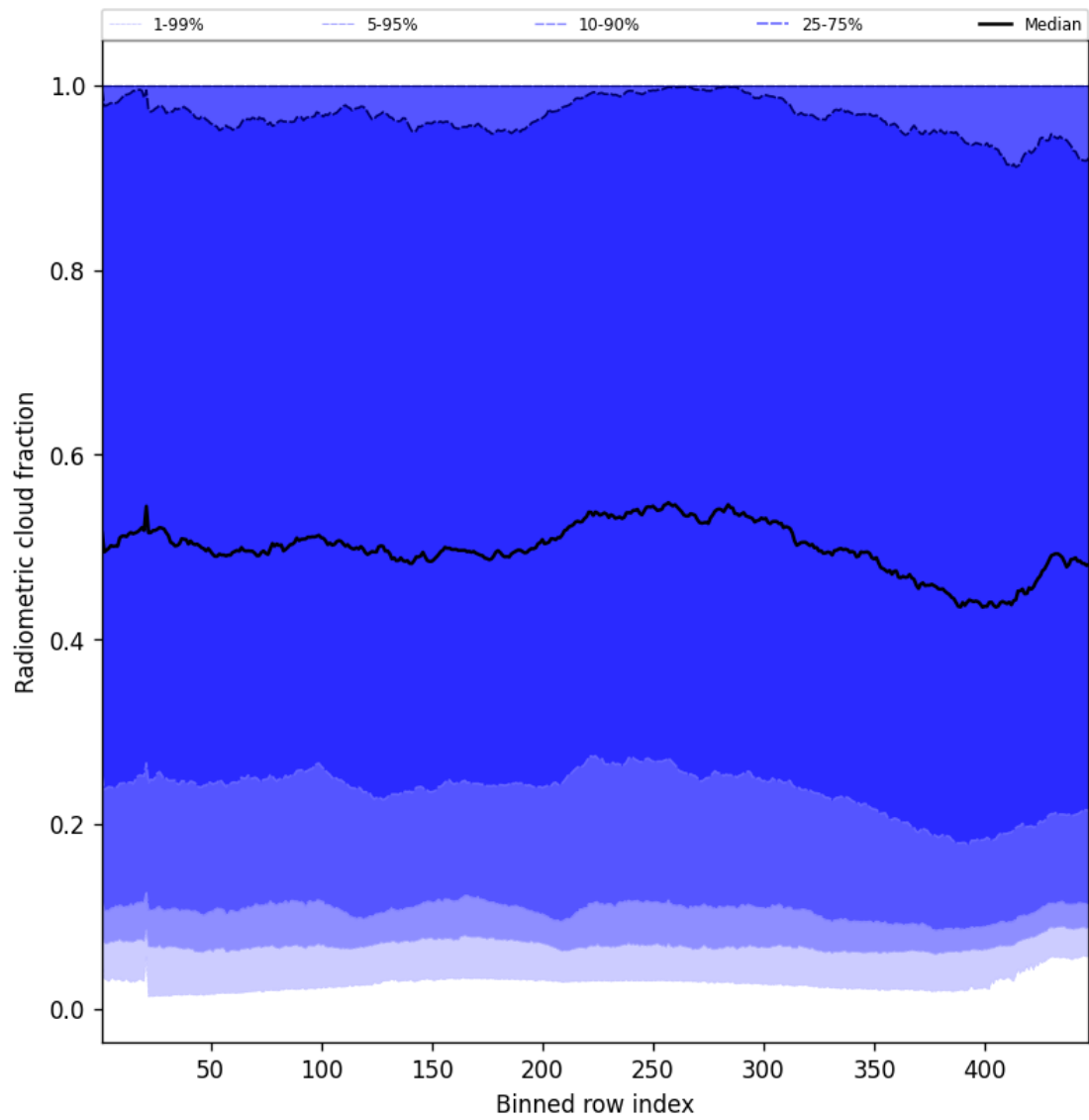
Figure 53: Along track statistics of “Radiometric cloud fraction” for 2025-02-25 to 2025-02-26
