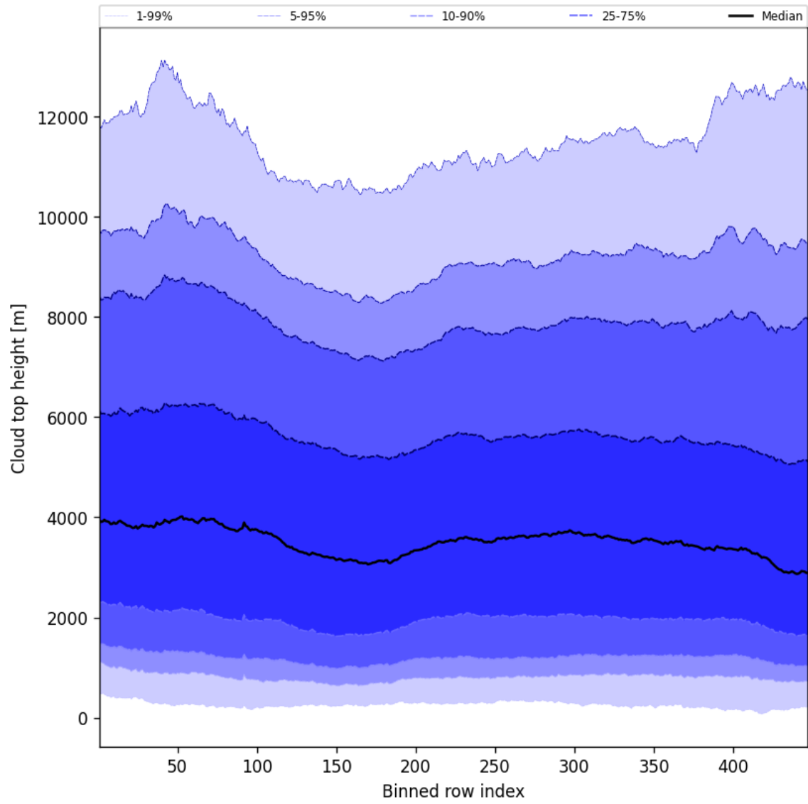
Figure 54: Along track statistics of “Cloud top height” for 2025-02-25 to 2025-02-26
