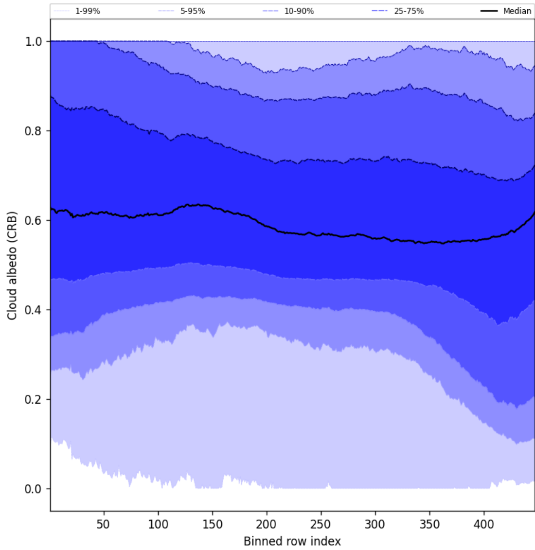
Figure 58: Along track statistics of “Cloud albedo (CRB)” for 2025-02-25 to 2025-02-26
