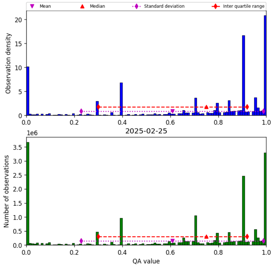
Figure 36: Histogram of “QA value” for 2025-02-25 to 2025-02-26
