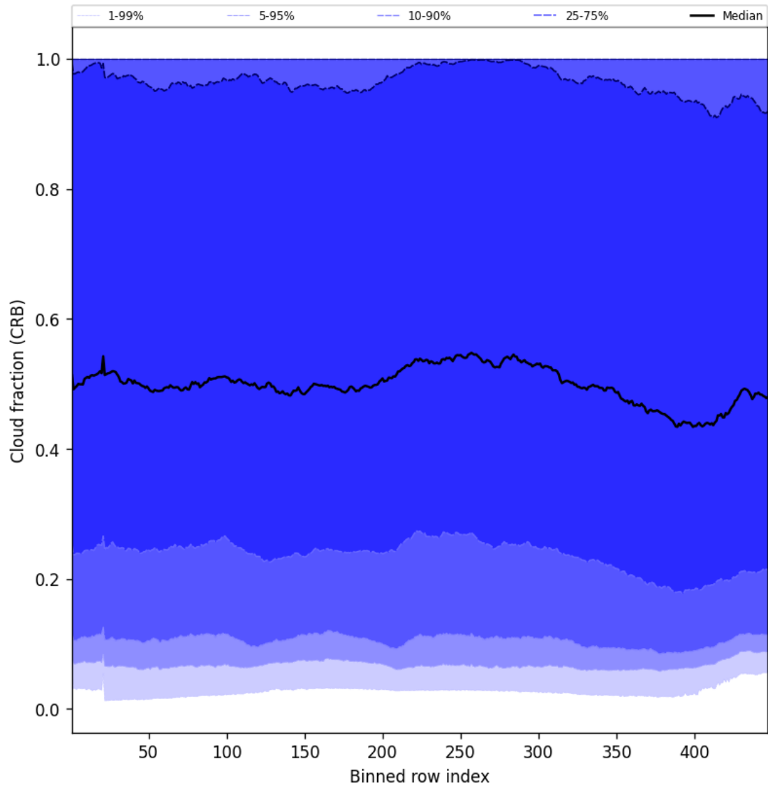
Figure 56: Along track statistics of “Cloud fraction (CRB)” for 2025-02-25 to 2025-02-26
