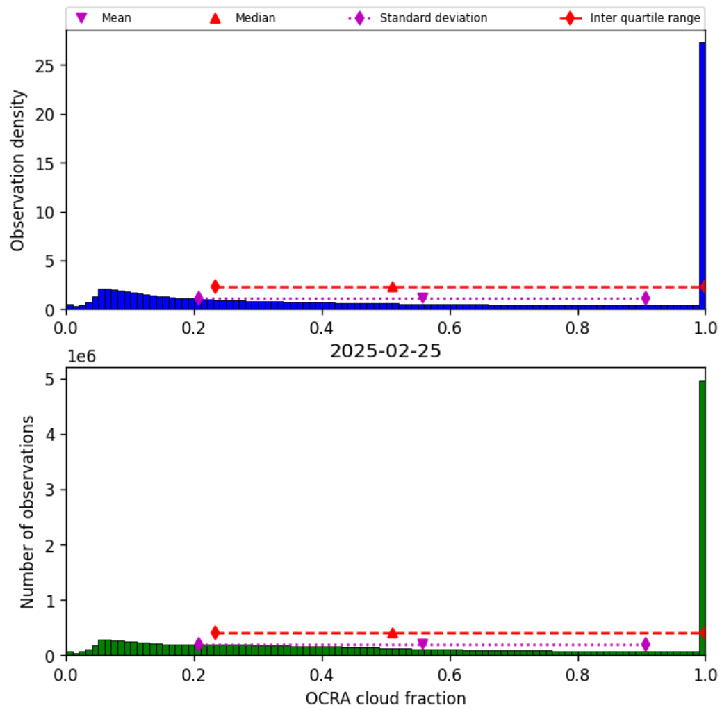
Figure 48: Histogram of “OCRA cloud fraction” for 2025-02-25 to 2025-02-26
