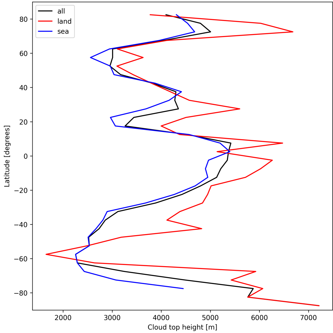
Figure 22: Zonal average of “Cloud top height” for 2025-02-25 to 2025-02-26.
