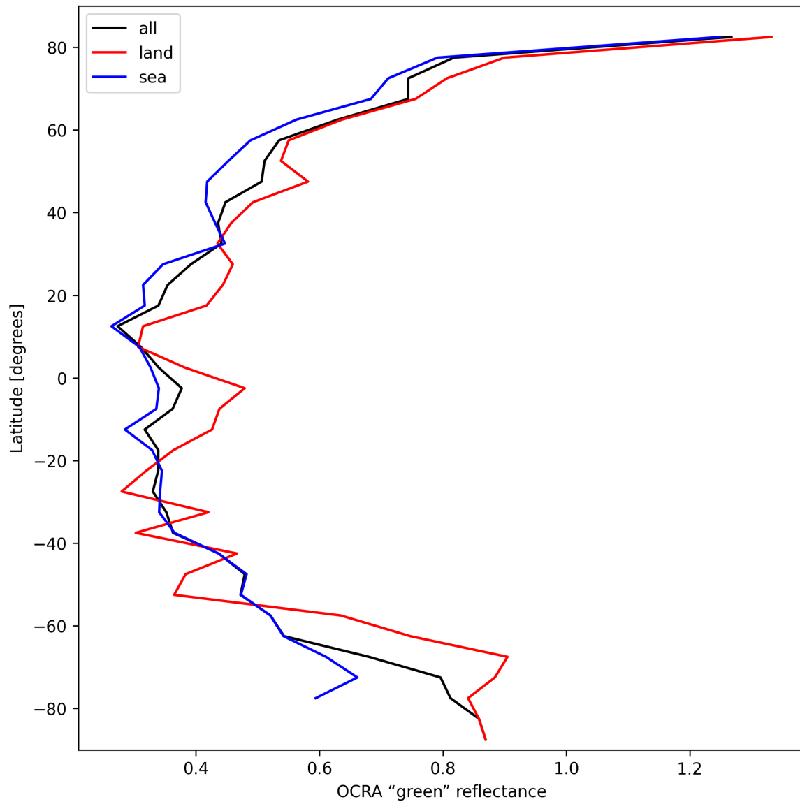
Figure 34: Zonal average of “OCRA “green” reflectance” for 2025-02-25 to 2025-02-26.
