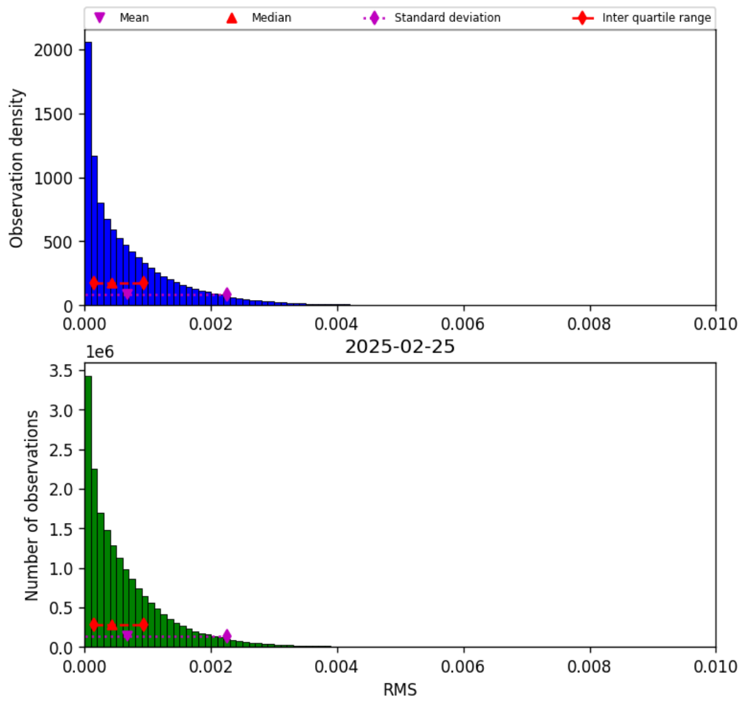
Figure 45: Histogram of “RMS” for 2025-02-25 to 2025-02-26
