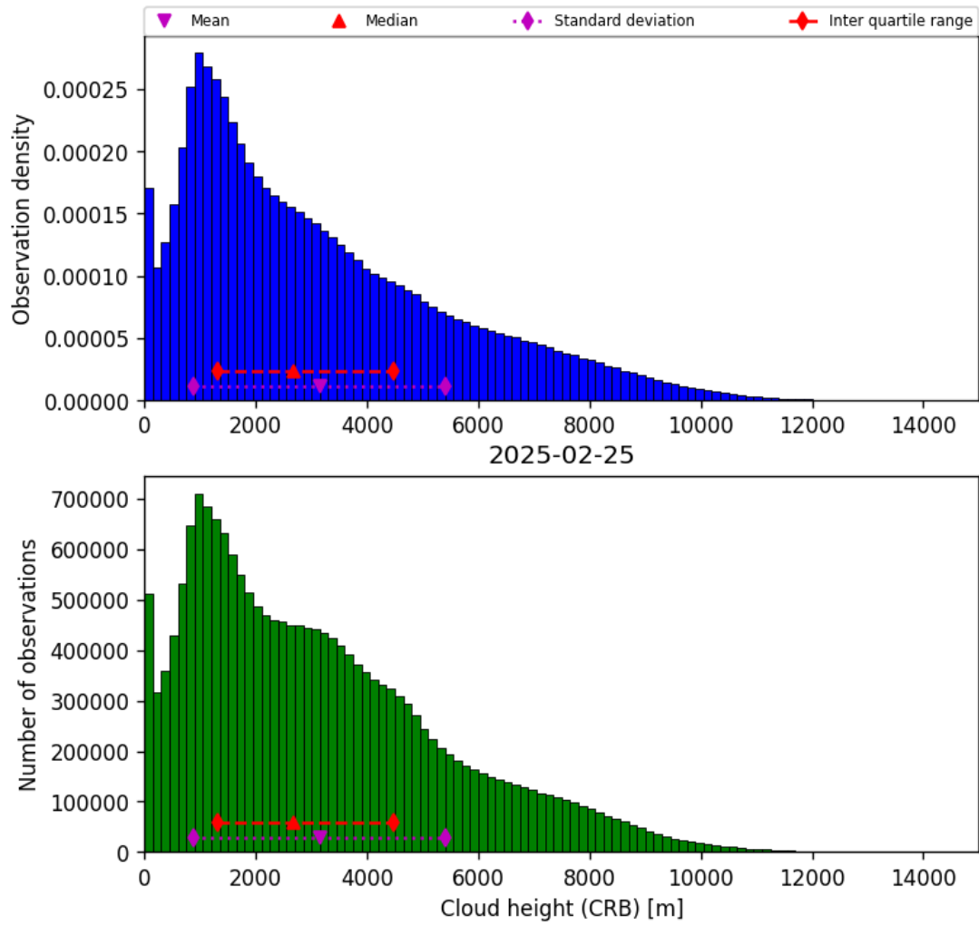
Figure 41: Histogram of “Cloud height (CRB)” for 2025-02-25 to 2025-02-26
