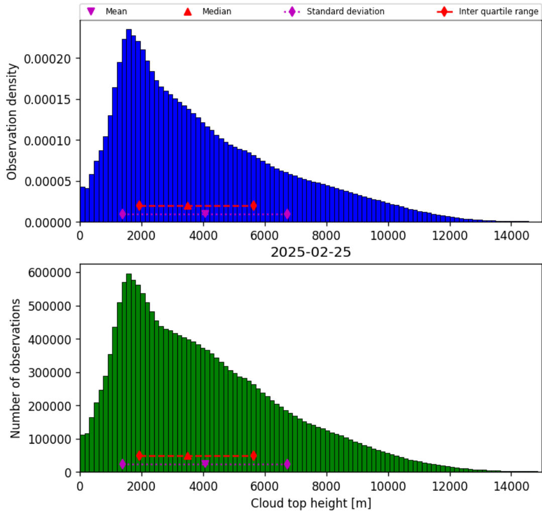
Figure 38: Histogram of “Cloud top height” for 2025-02-25 to 2025-02-26
