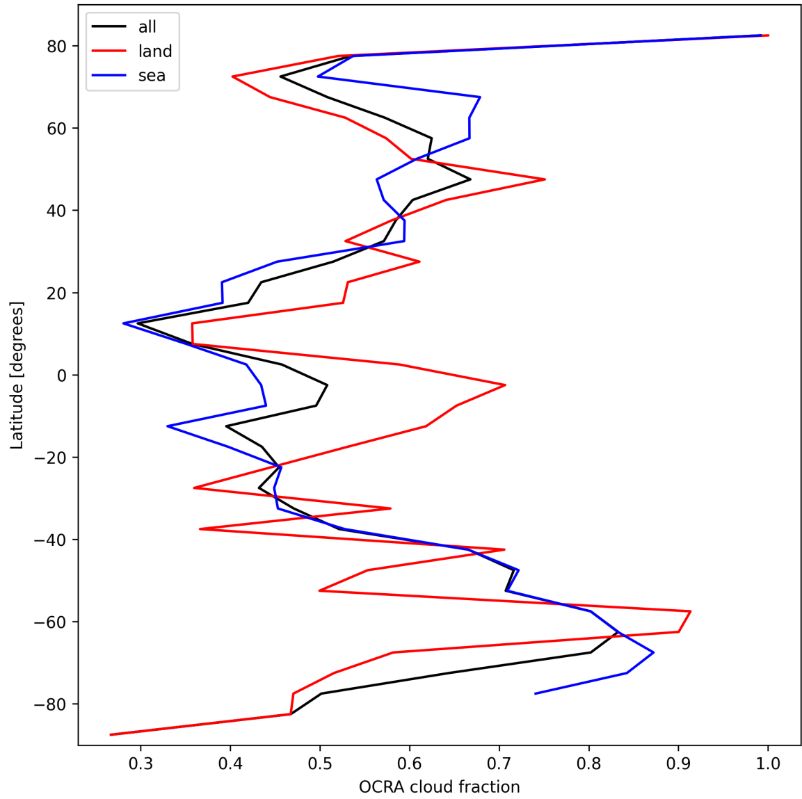
Figure 32: Zonal average of “OCRA cloud fraction” for 2025-02-25 to 2025-02-26.
