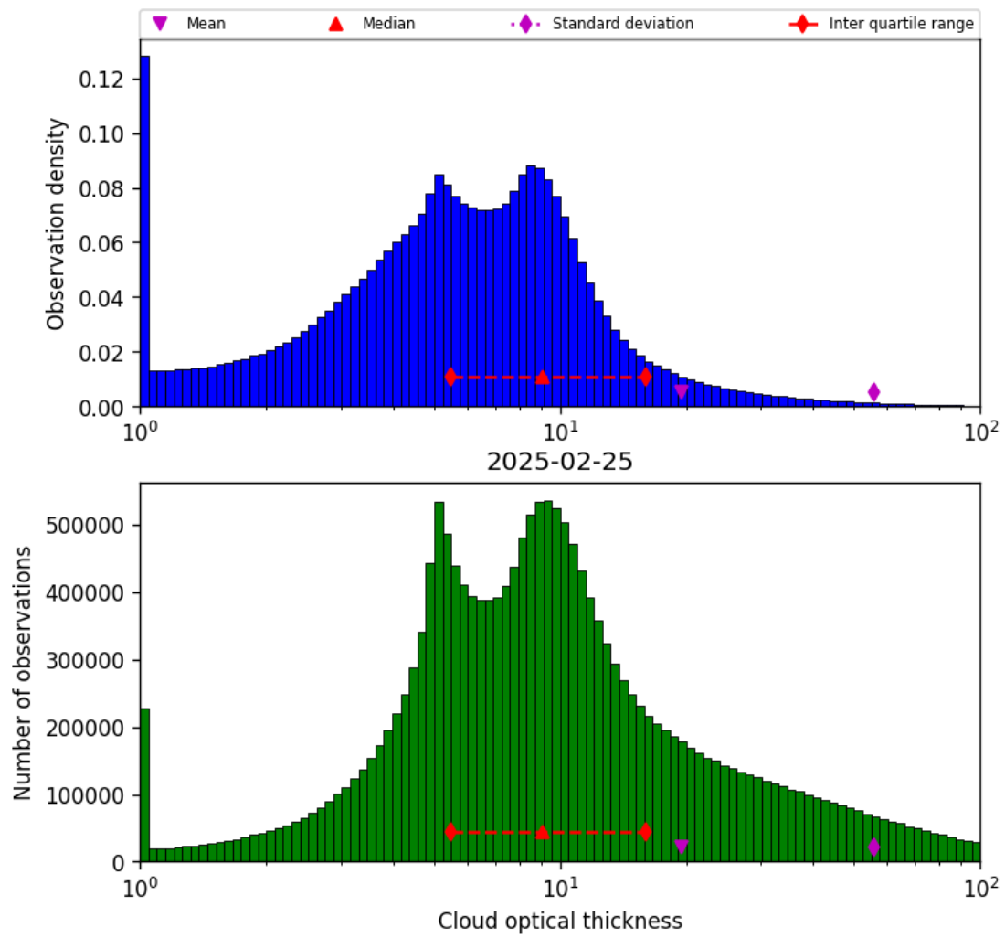
Figure 39: Histogram of “Cloud optical thickness” for 2025-02-25 to 2025-02-26
