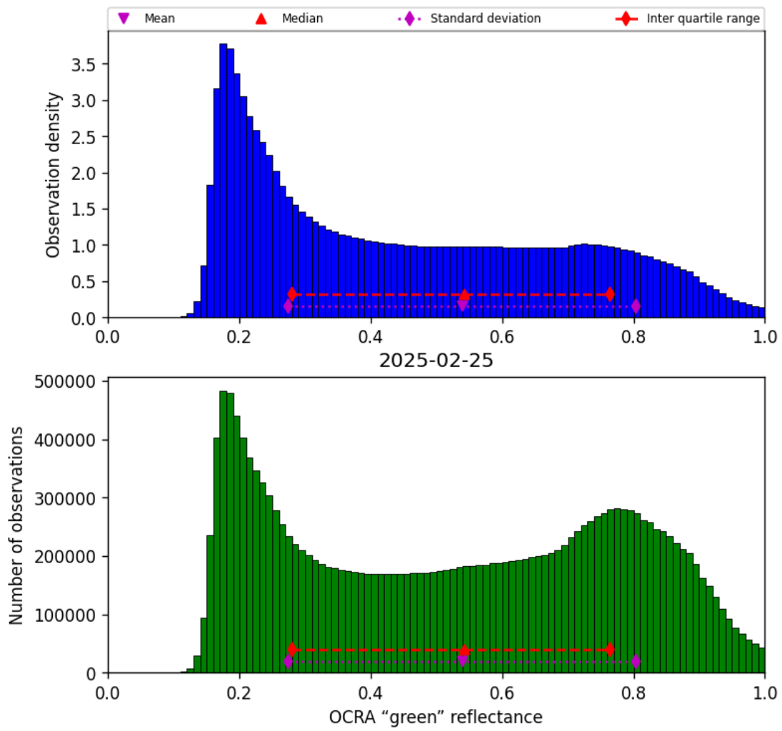
Figure 50: Histogram of “OCRA “green” reflectance” for 2025-02-25 to 2025-02-26
