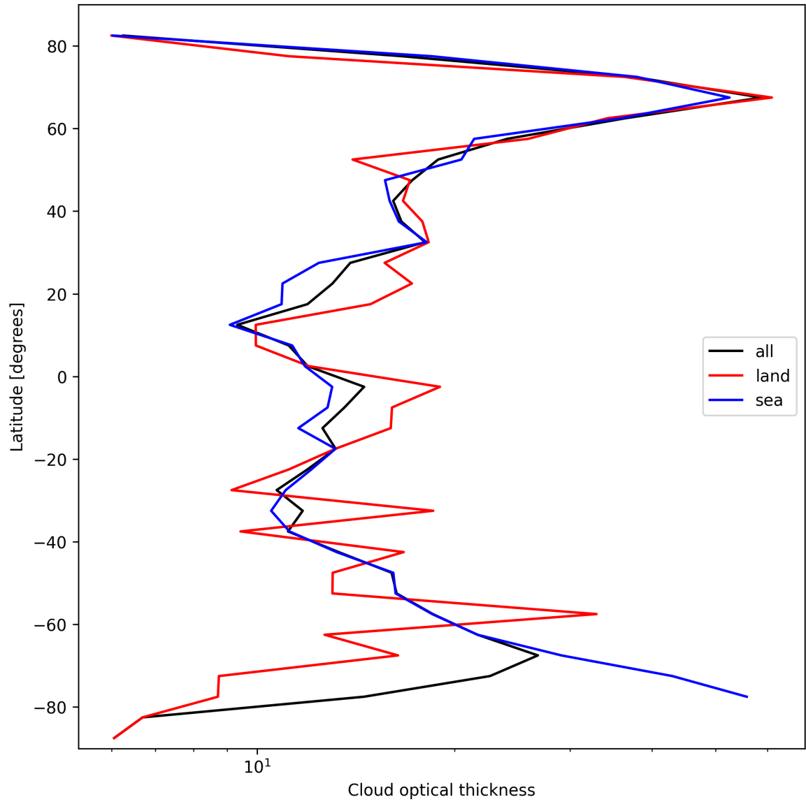
Figure 23: Zonal average of “Cloud optical thickness” for 2025-02-25 to 2025-02-26.
