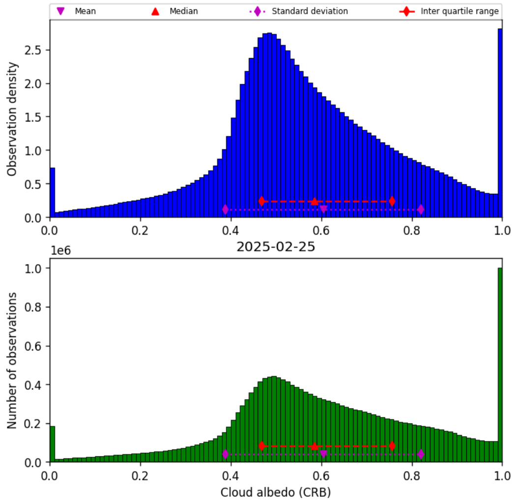
Figure 42: Histogram of “Cloud albedo (CRB)” for 2025-02-25 to 2025-02-26
