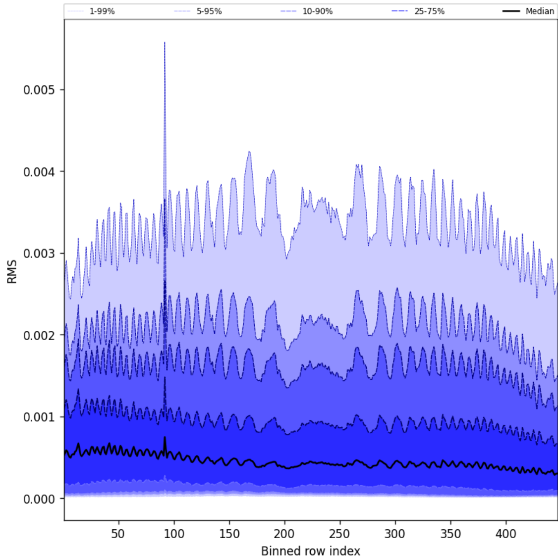
Figure 61: Along track statistics of “RMS” for 2025-02-25 to 2025-02-26
