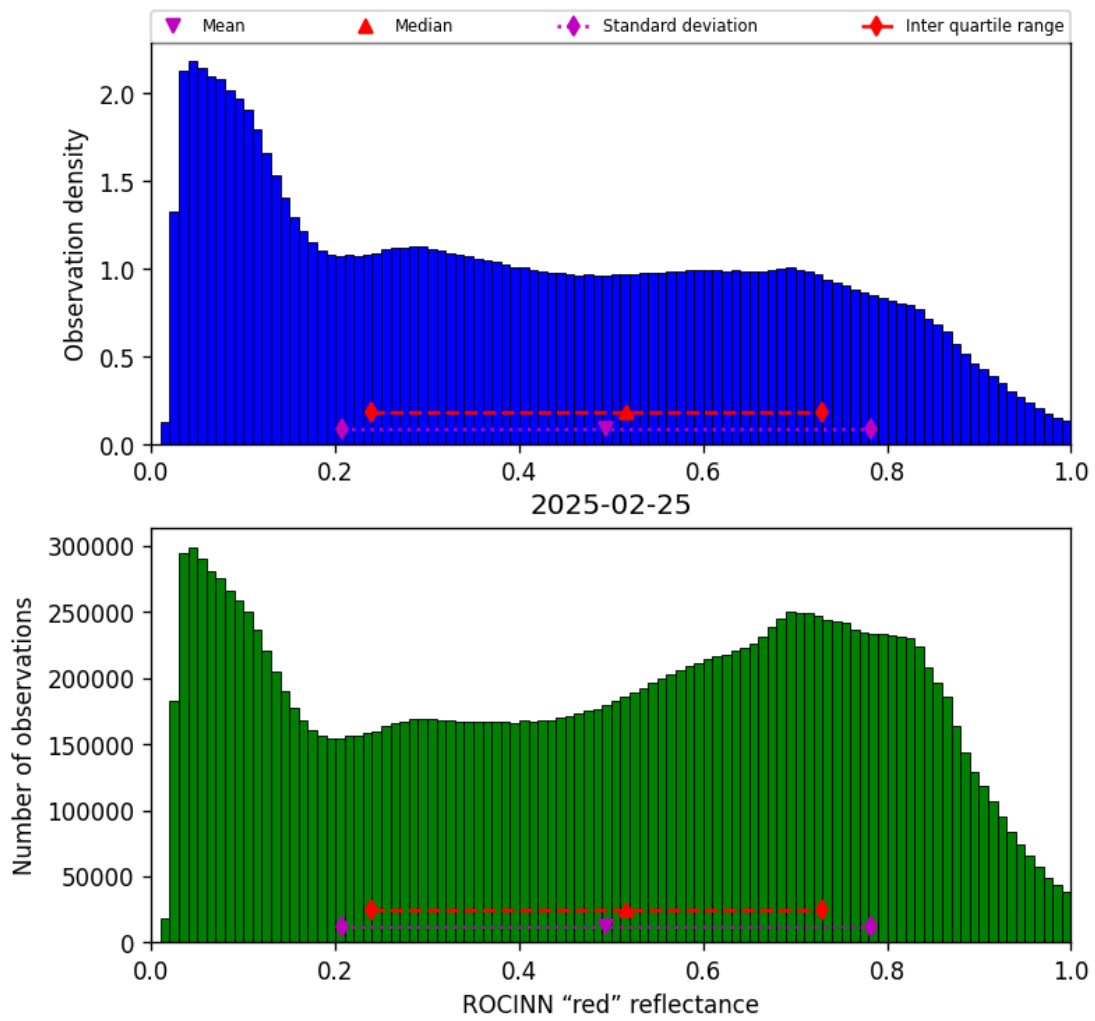
Figure 51: Histogram of “ROCINN “red” reflectance” for 2025-02-25 to 2025-02-26
