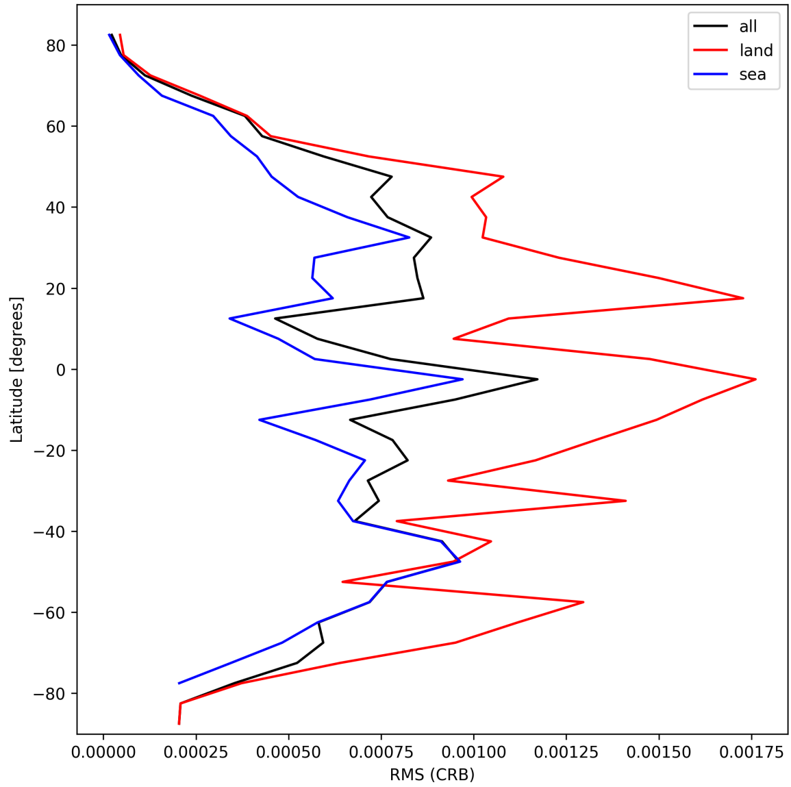
Figure 30: Zonal average of "RMS (CRB)" for 2025-02-25 to 2025-02-26.
