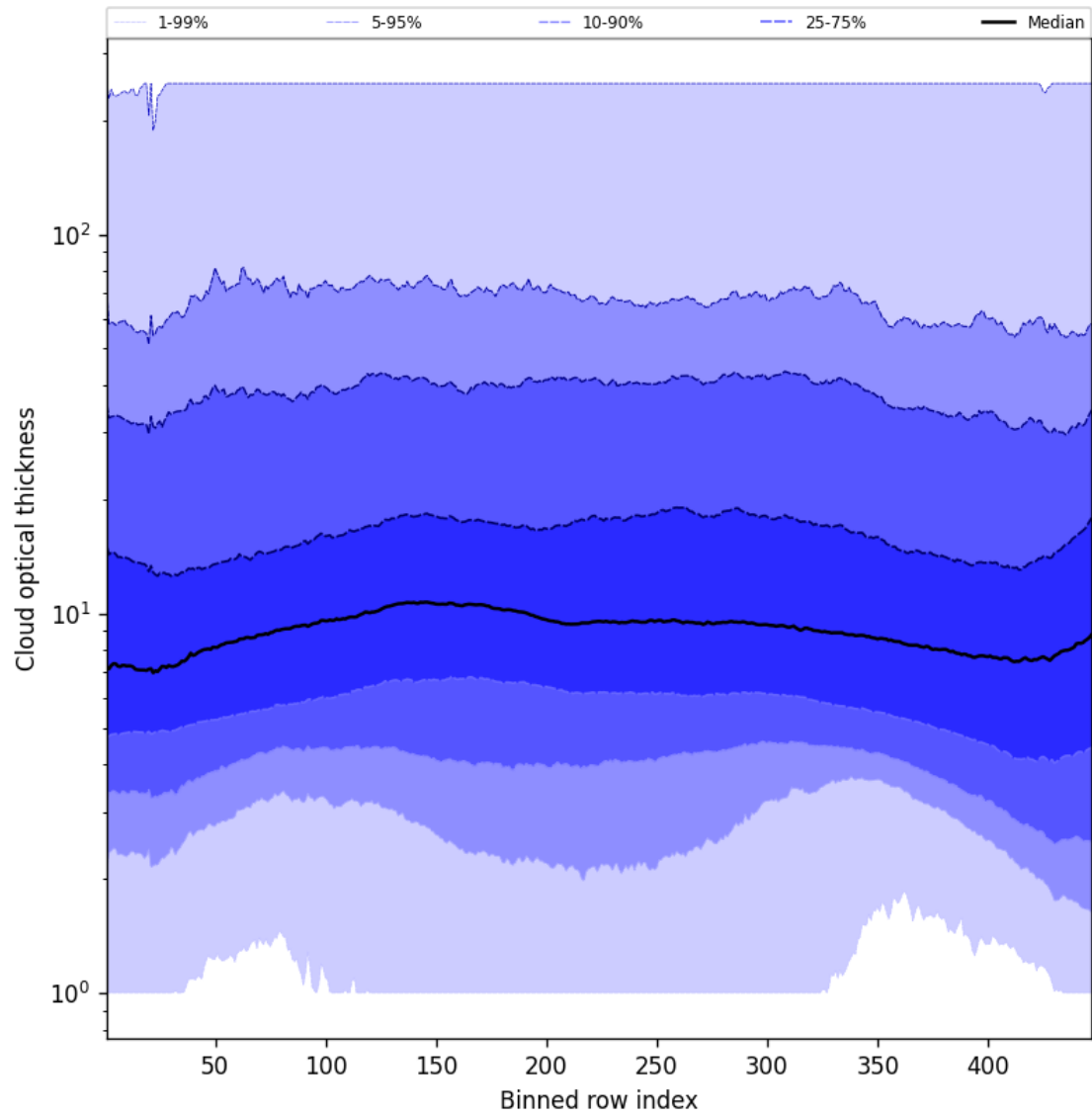
Figure 55: Along track statistics of “Cloud optical thickness” for 2025-02-25 to 2025-02-26
