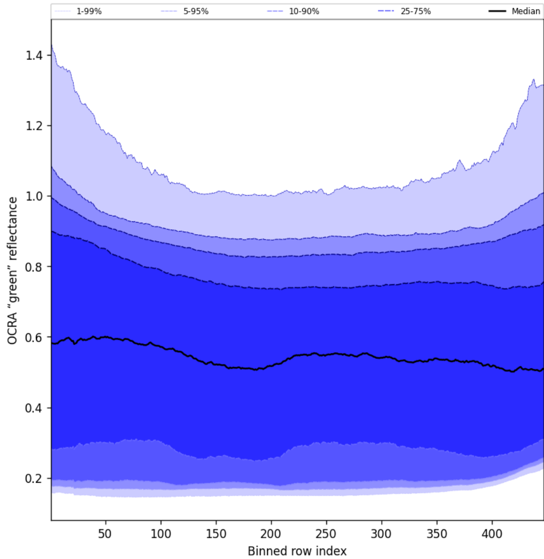
Figure 66: Along track statistics of “OCRA “green” reflectance” for 2025-02-25 to 2025-02-26
