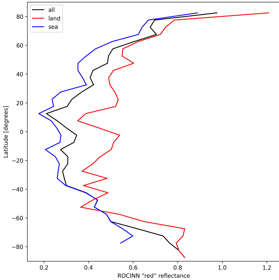
Figure 35: Zonal average of “ROCINN “red” reflectance” for 2025-02-25 to 2025-02-26.
