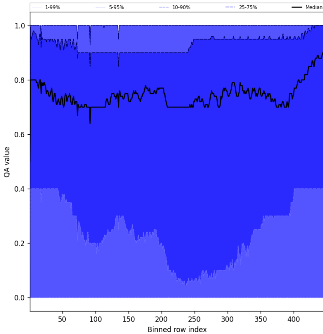
Figure 52: Along track statistics of “QA value” for 2025-02-25 to 2025-02-26
