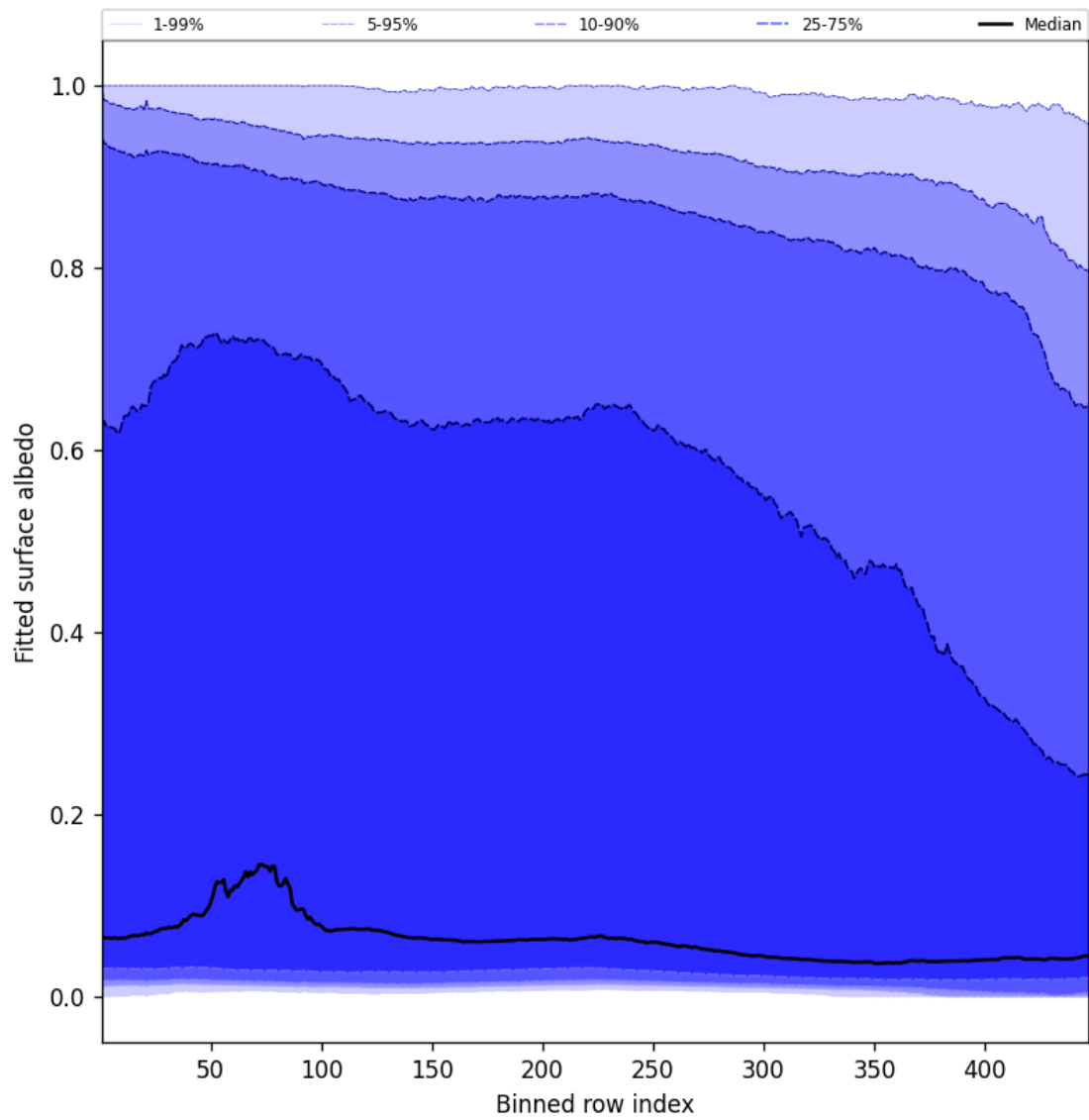
Figure 59: Along track statistics of “Fitted surface albedo” for 2025-02-25 to 2025-02-26
