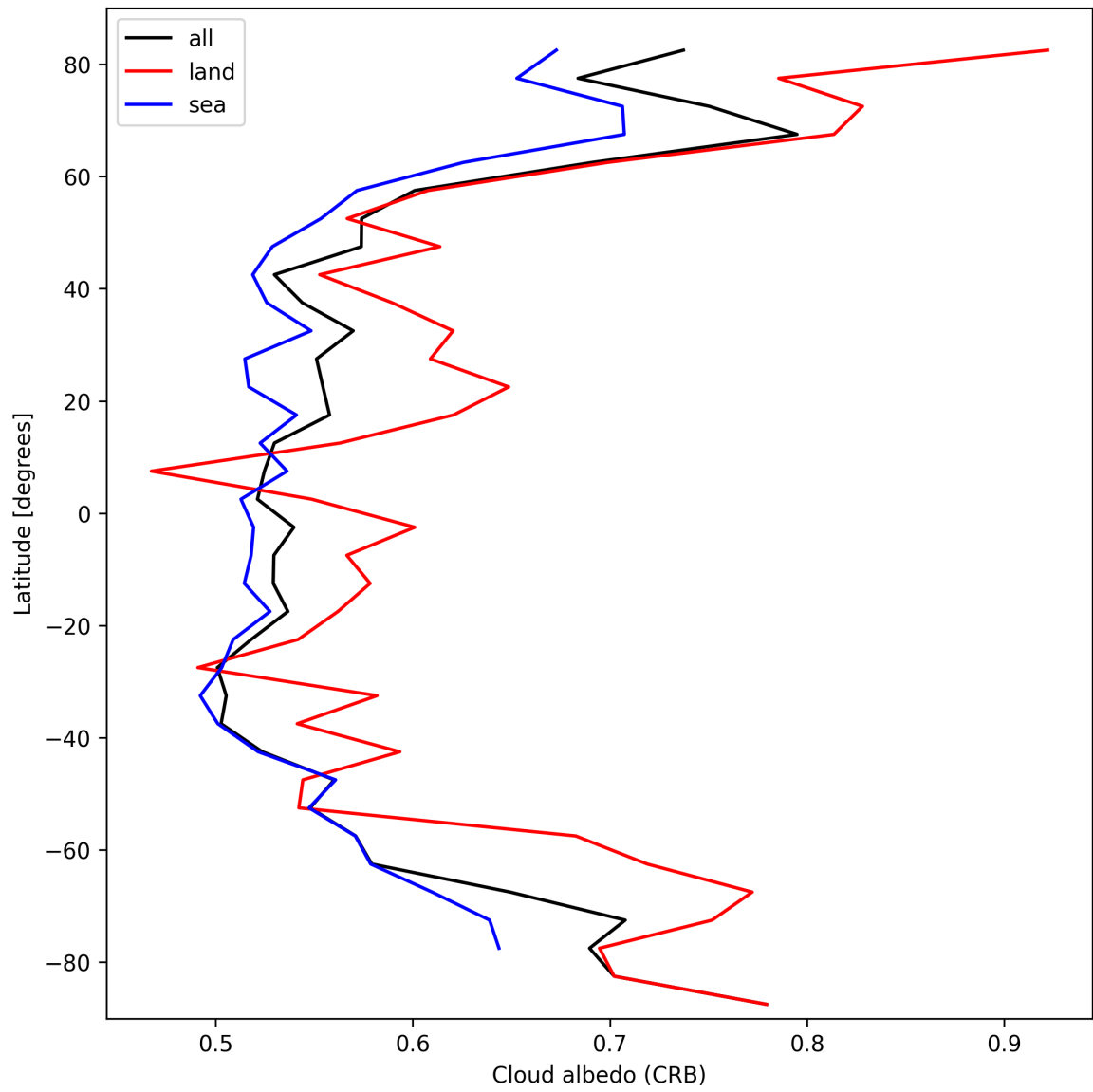
Figure 26: Zonal average of “Cloud albedo (CRB)” for 2025-02-25 to 2025-02-26.
