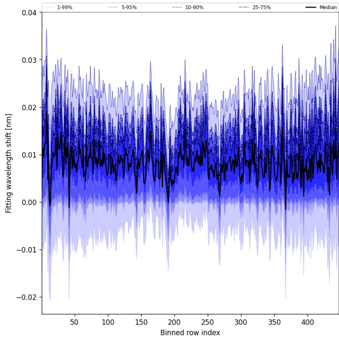
Figure 63: Along track statistics of “Fitting wavelength shift” for 2025-02-25 to 2025-02-26
