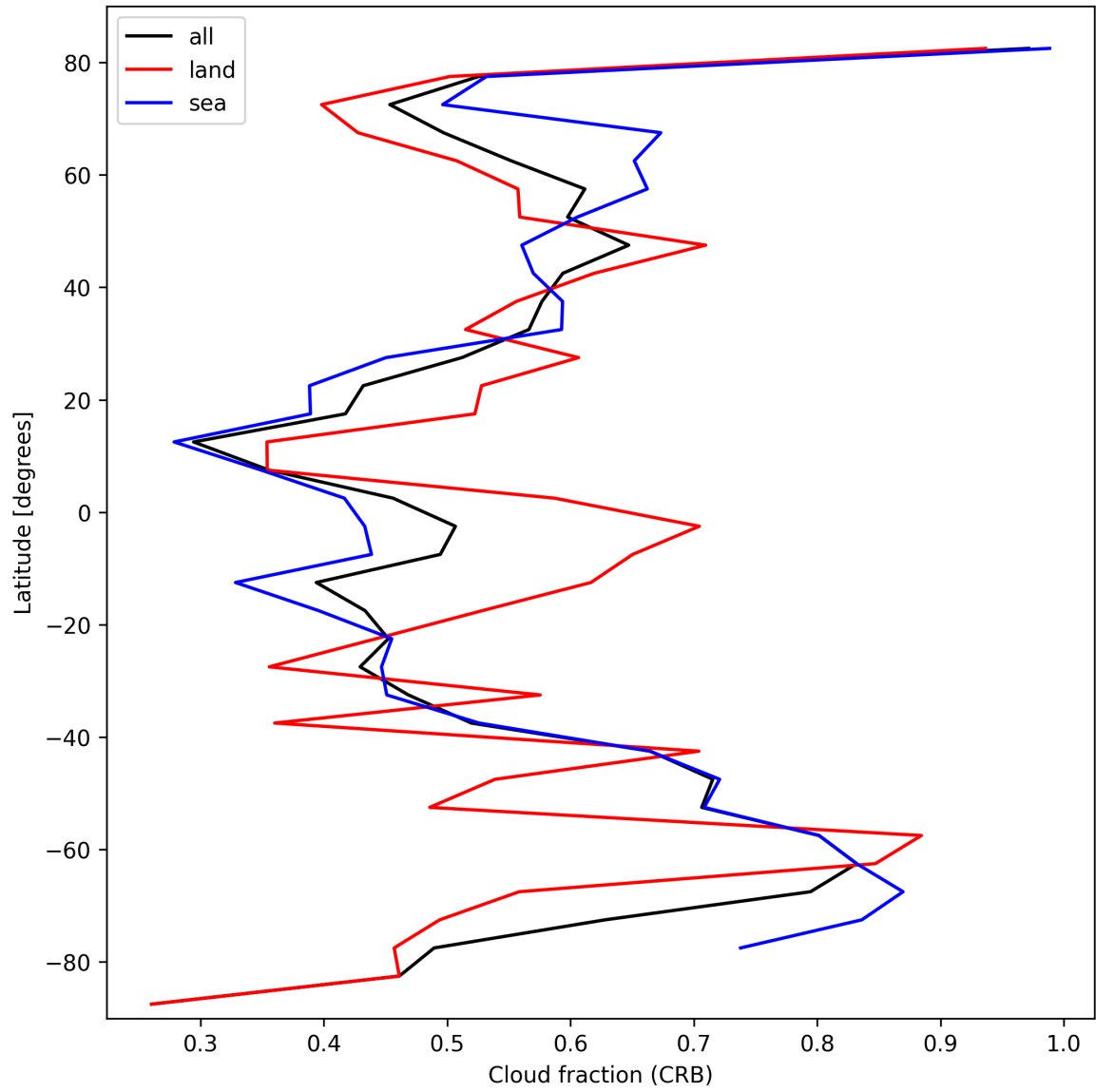
Figure 24: Zonal average of “Cloud fraction (CRB)” for 2025-02-25 to 2025-02-26.
