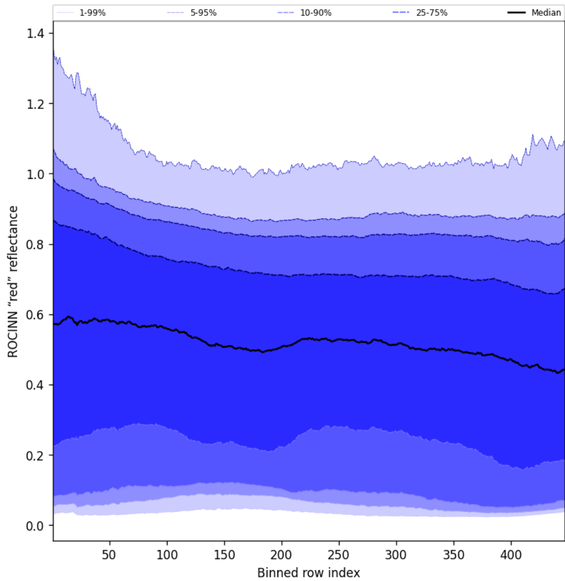
Figure 67: Along track statistics of “ROCINN “red” reflectance” for 2025-02-25 to 2025-02-26
