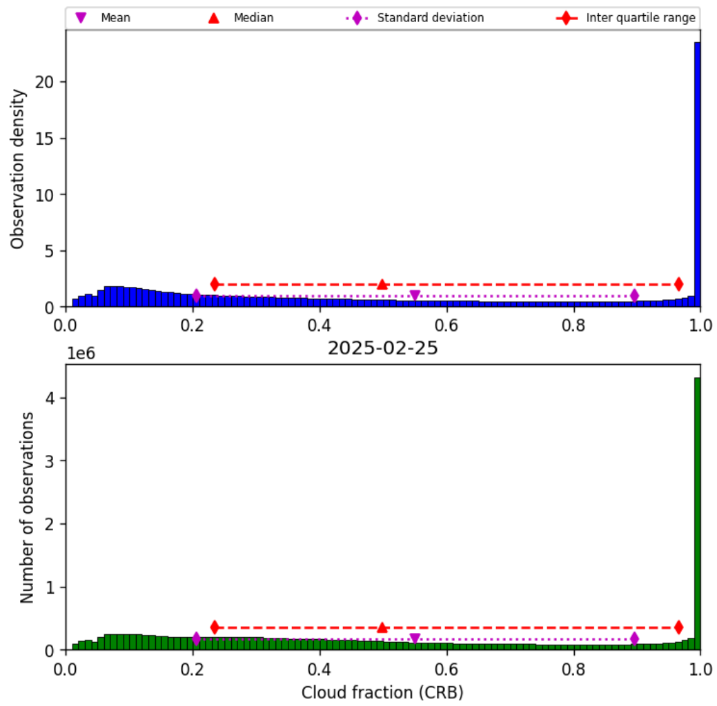
Figure 40: Histogram of “Cloud fraction (CRB)” for 2025-02-25 to 2025-02-26
