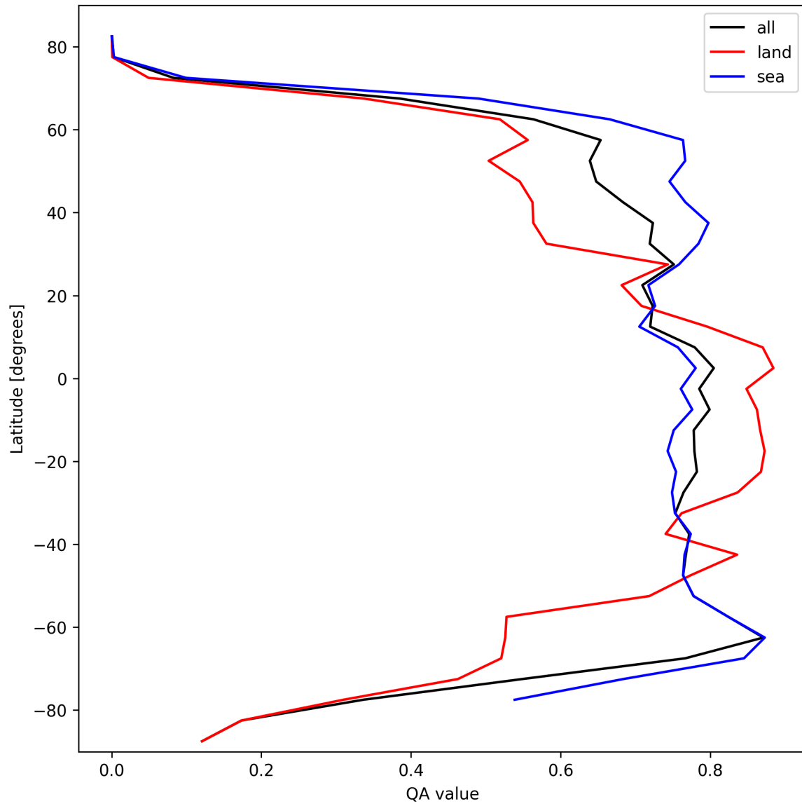
Figure 20: Zonal average of “QA value” for 2025-02-25 to 2025-02-26.
