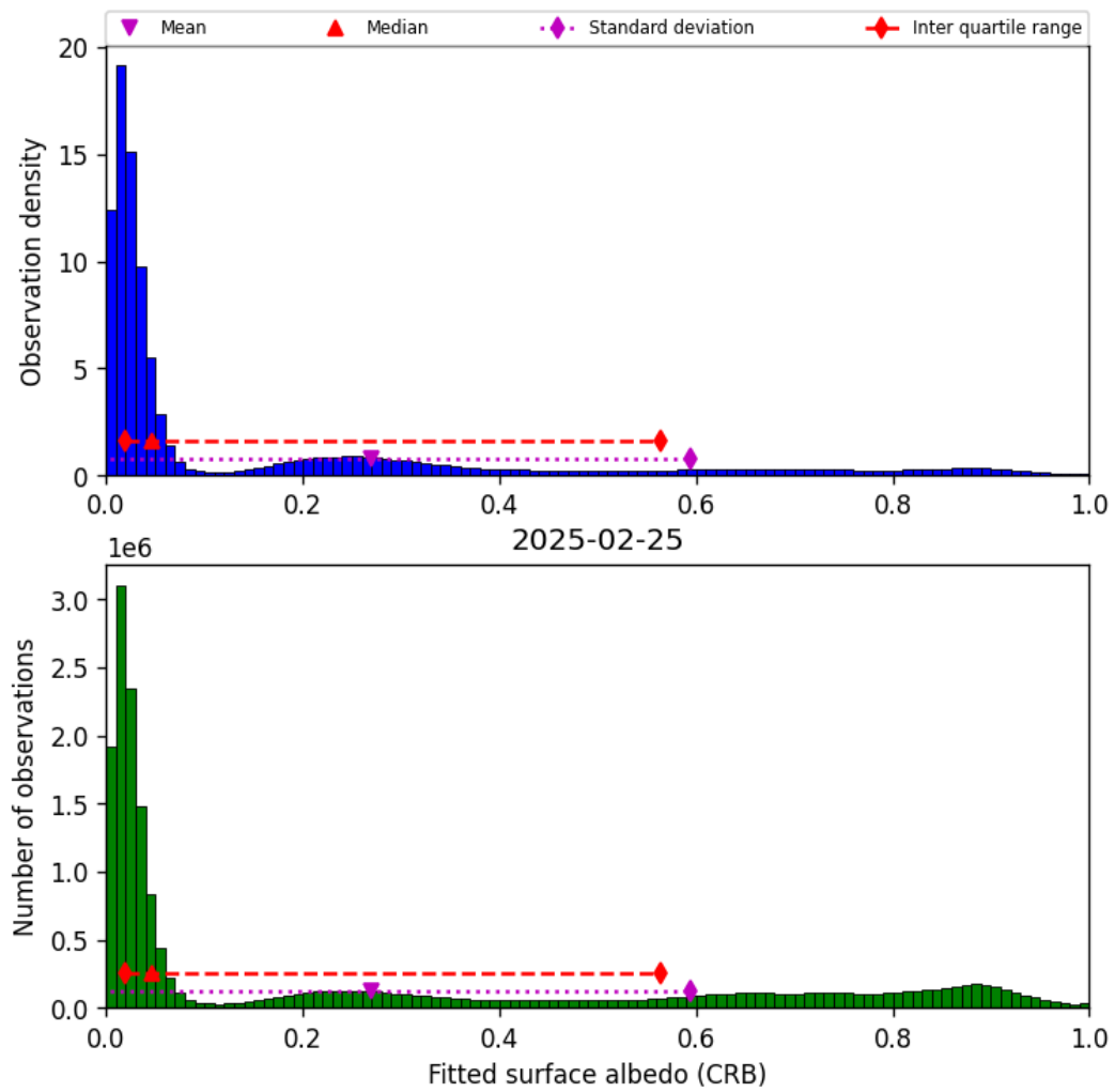
Figure 44: Histogram of “Fitted surface albedo (CRB)” for 2025-02-25 to 2025-02-26
