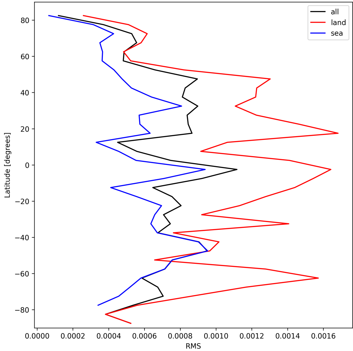
Figure 29: Zonal average of “RMS” for 2025-02-25 to 2025-02-26.
