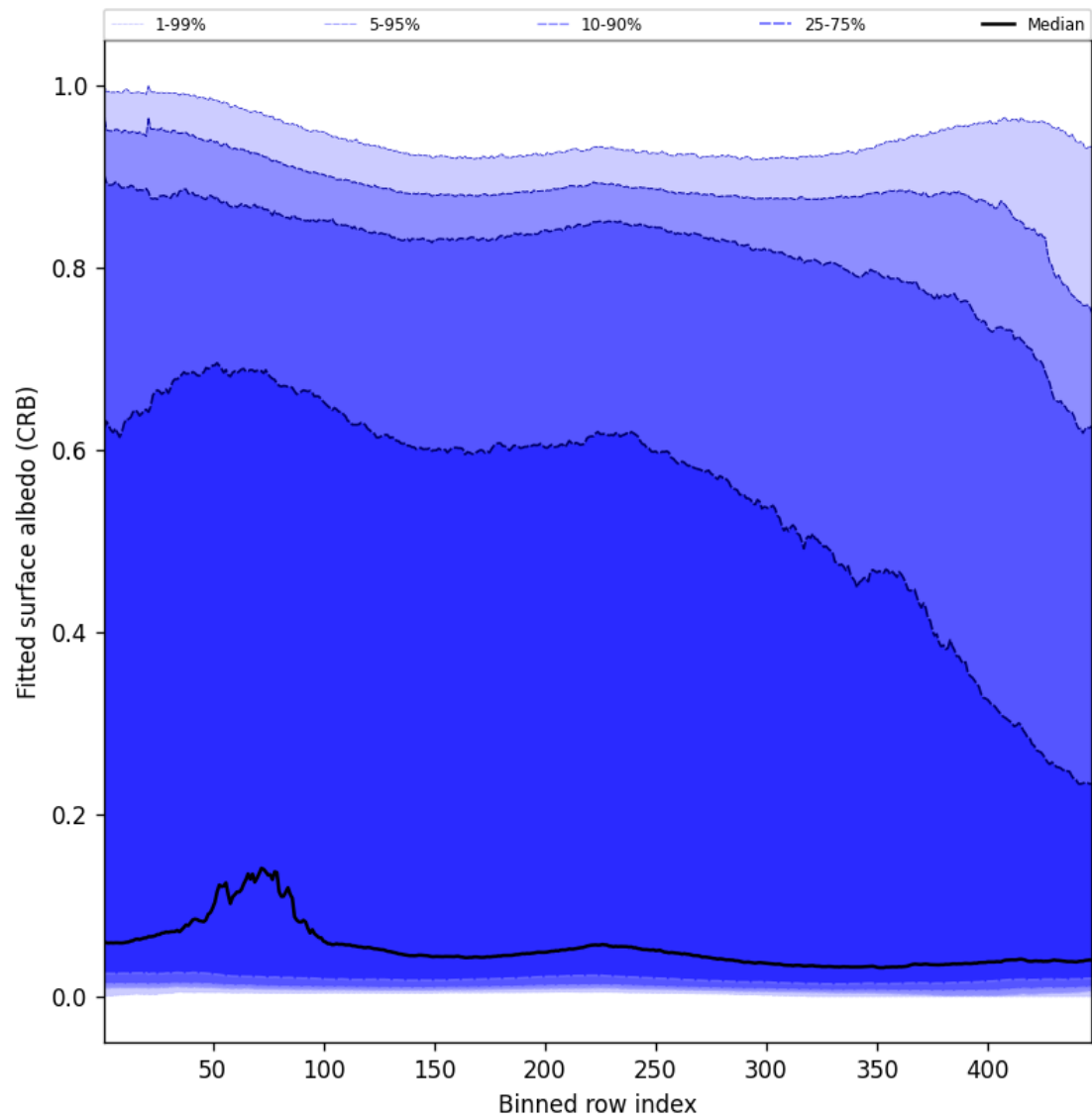
Figure 60: Along track statistics of “Fitted surface albedo (CRB)” for 2025-02-25 to 2025-02-26
