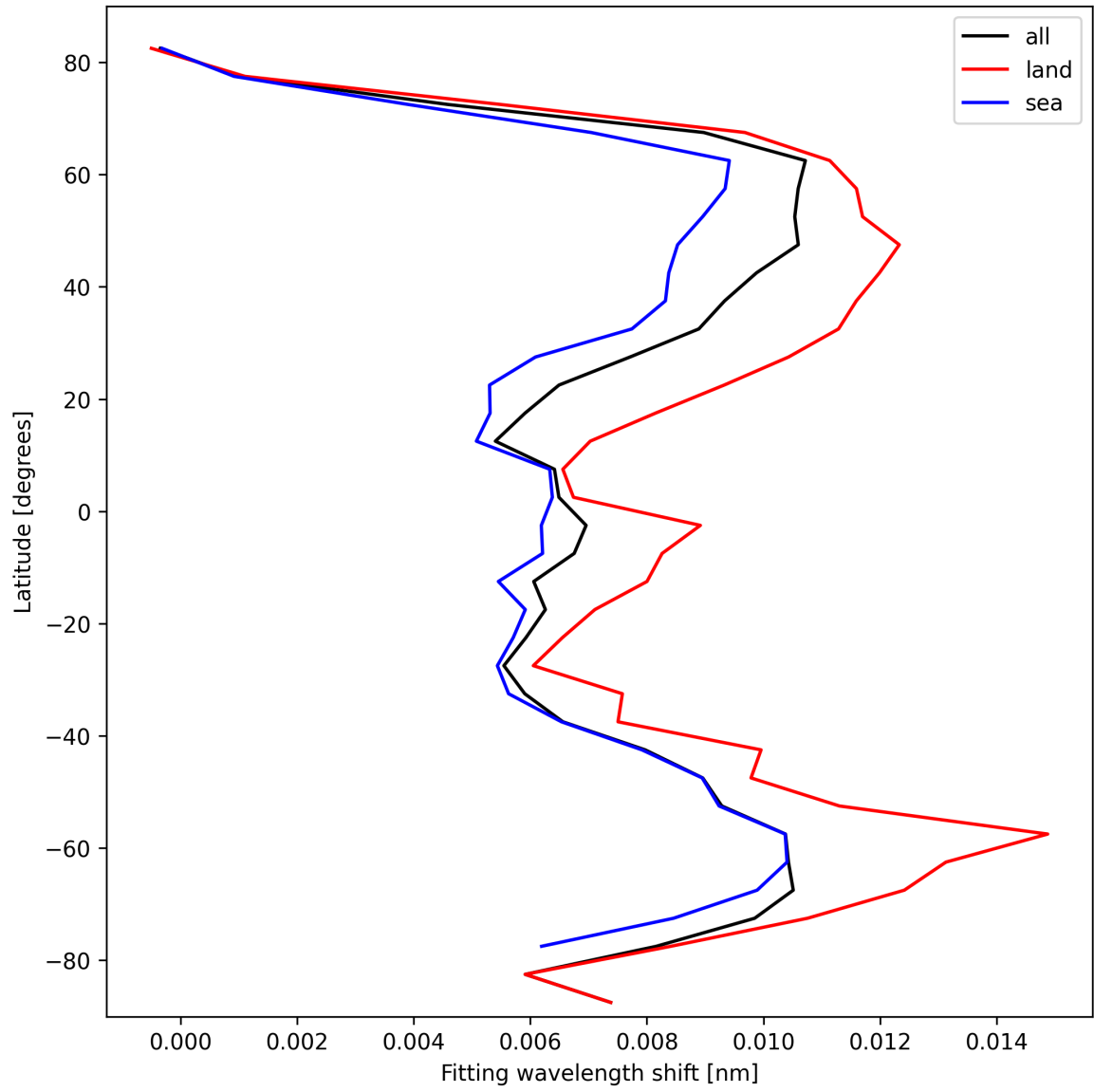
Figure 31: Zonal average of “Fitting wavelength shift” for 2025-02-25 to 2025-02-26.
