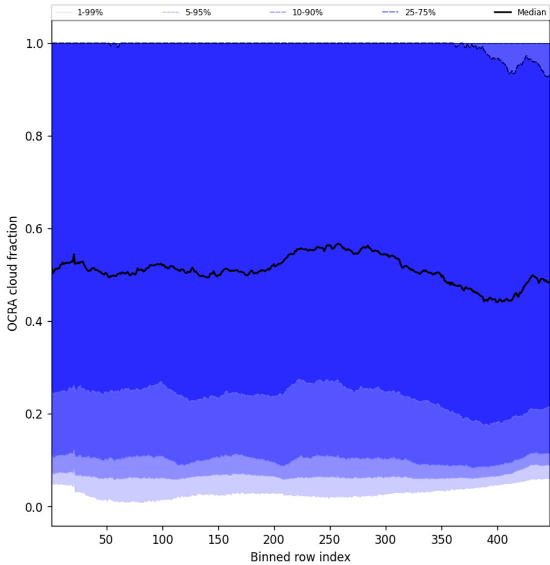
Figure 64: Along track statistics of “OCRA cloud fraction” for 2025-02-25 to 2025-02-26
