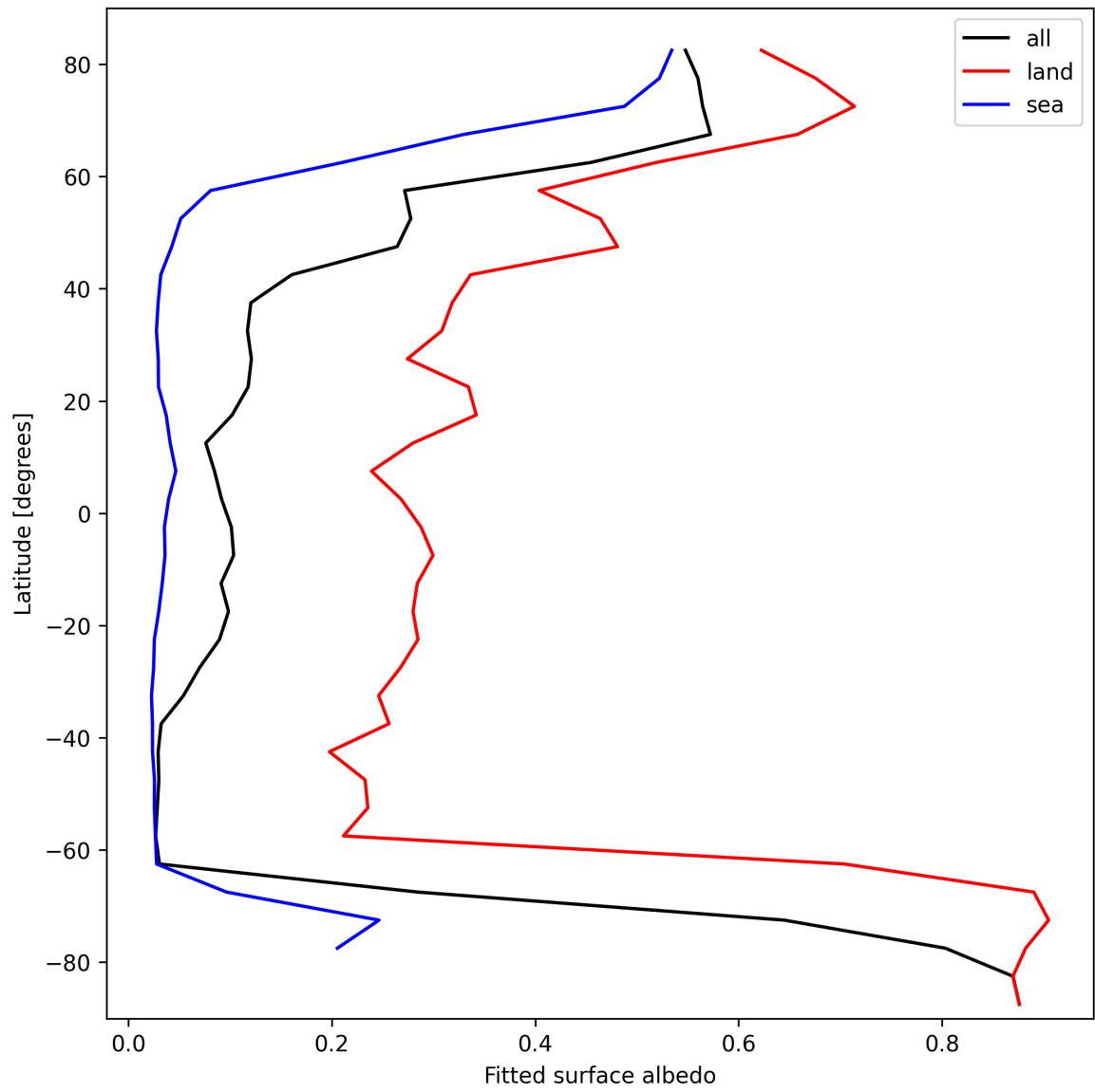
Figure 27: Zonal average of “Fitted surface albedo” for 2025-02-25 to 2025-02-26.
