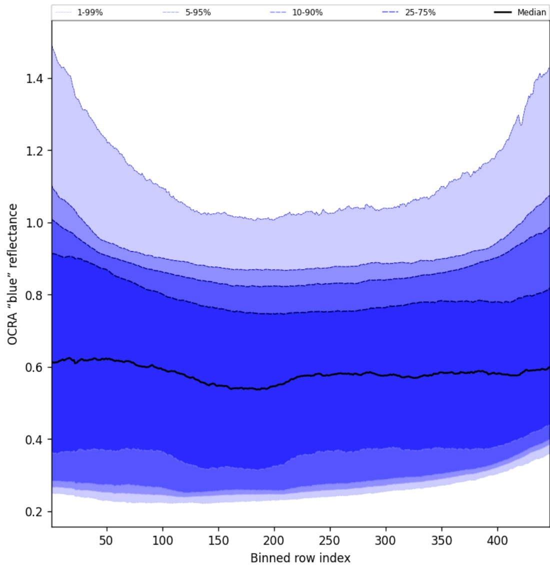
Figure 65: Along track statistics of “OCRA “blue” reflectance” for 2025-02-25 to 2025-02-26
