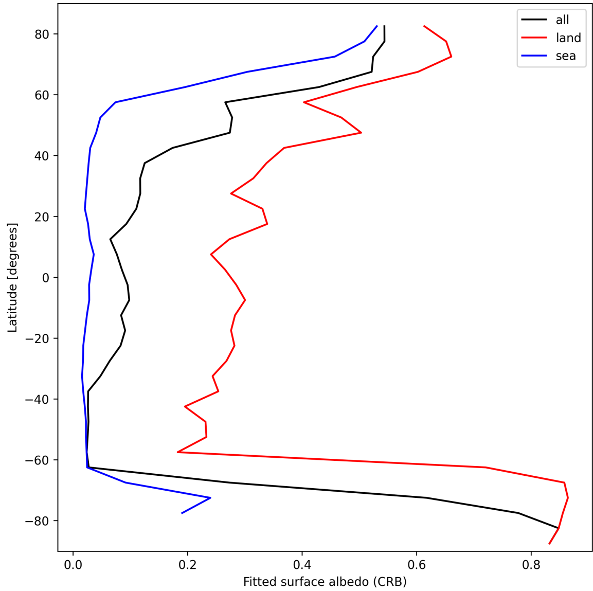
Figure 28: Zonal average of “Fitted surface albedo (CRB)” for 2025-02-25 to 2025-02-26.
