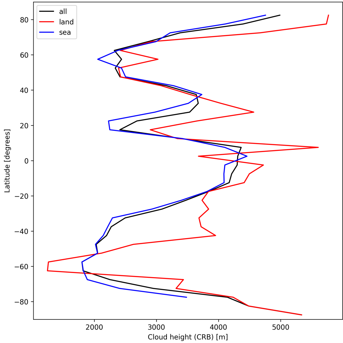
Figure 25: Zonal average of “Cloud height (CRB)” for 2025-02-25 to 2025-02-26.
