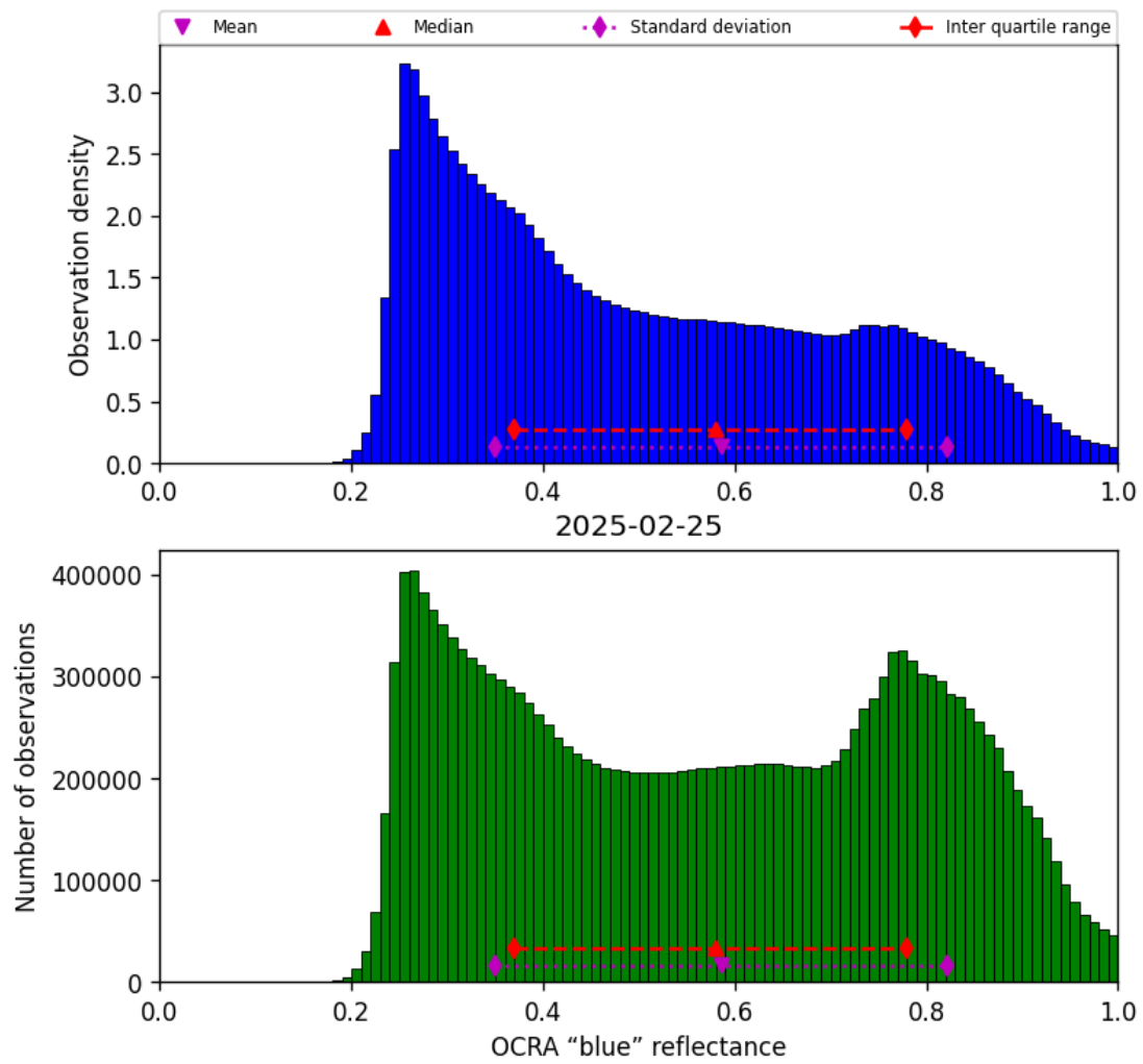
Figure 49: Histogram of “OCRA “blue” reflectance” for 2025-02-25 to 2025-02-26
