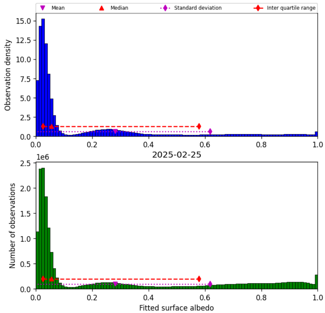
Figure 43: Histogram of “Fitted surface albedo” for 2025-02-25 to 2025-02-26
