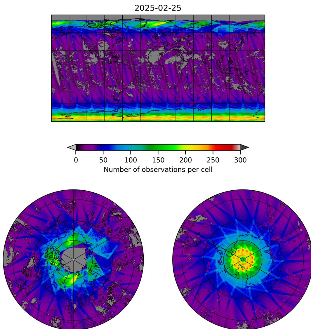
Figure 19: Map of the number of observations for 2025-02-25 to 2025-02-26
