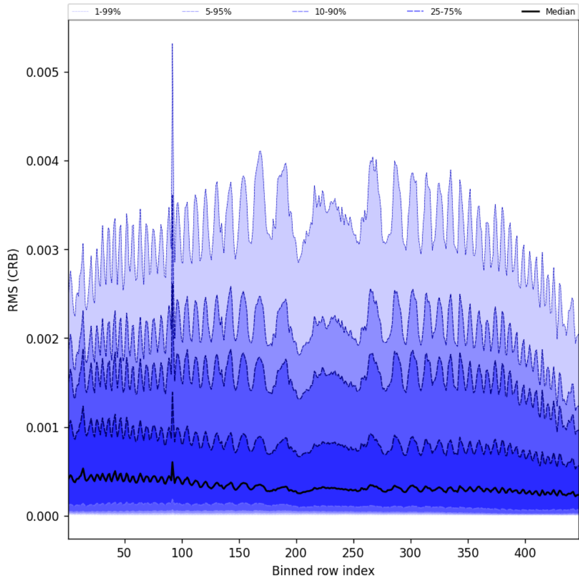
Figure 62: Along track statistics of “RMS (CRB)” for 2025-02-25 to 2025-02-26
