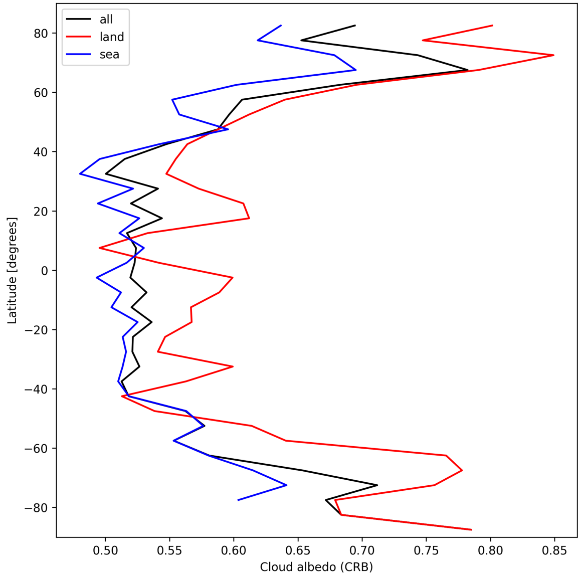
Figure 26: Zonal average of “Cloud albedo (CRB)” for 2025-02-26 to 2025-02-27.
