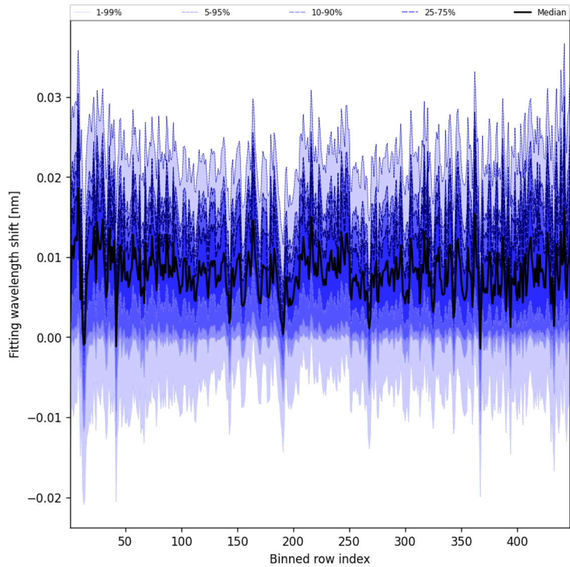
Figure 63: Along track statistics of “Fitting wavelength shift” for 2025-02-26 to 2025-02-27
