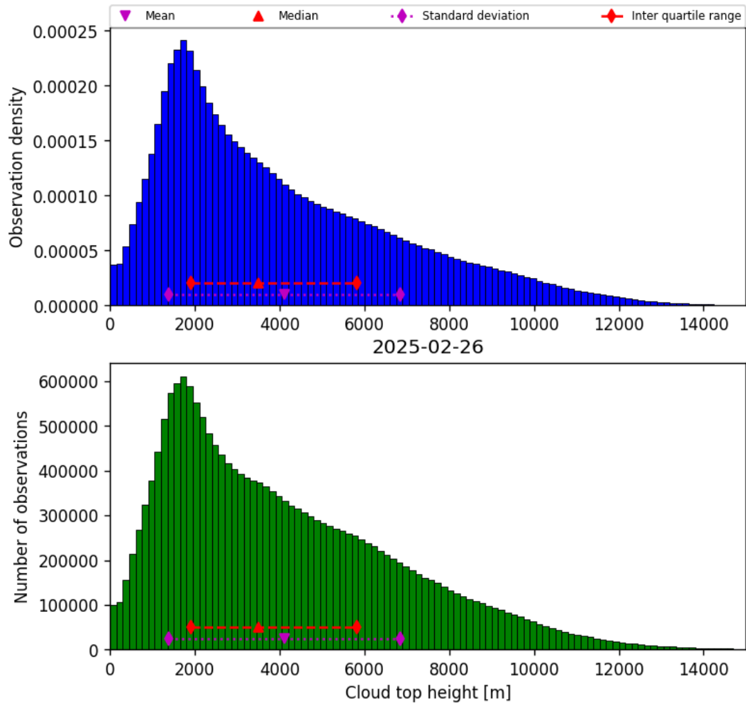
Figure 38: Histogram of “Cloud top height” for 2025-02-26 to 2025-02-27
