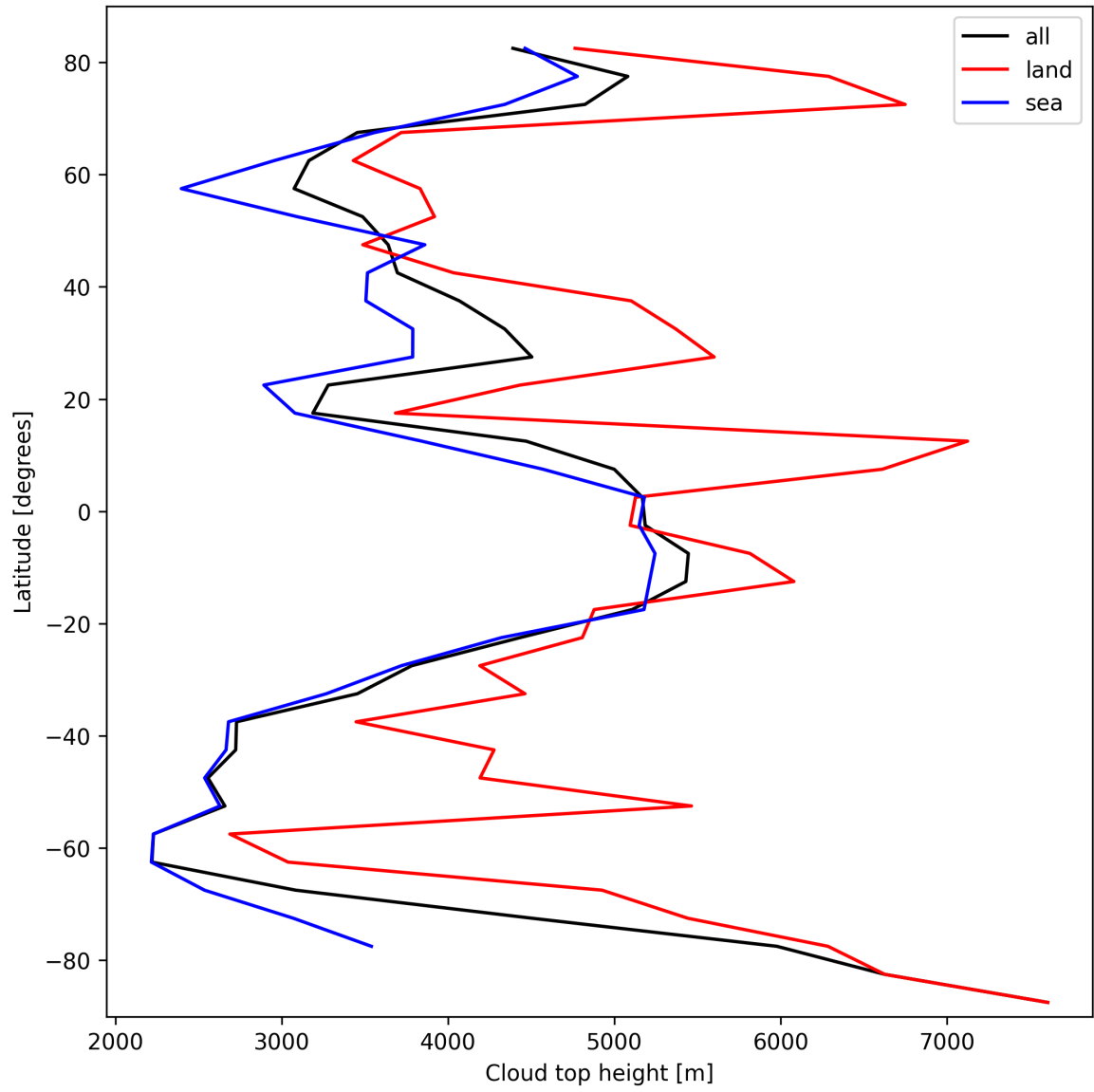
Figure 22: Zonal average of “Cloud top height” for 2025-02-26 to 2025-02-27.
