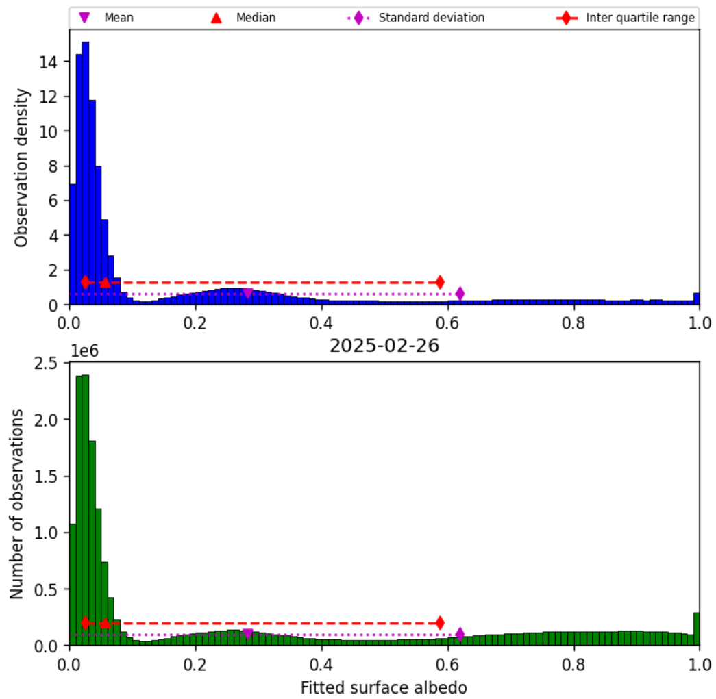
Figure 43: Histogram of “Fitted surface albedo” for 2025-02-26 to 2025-02-27
