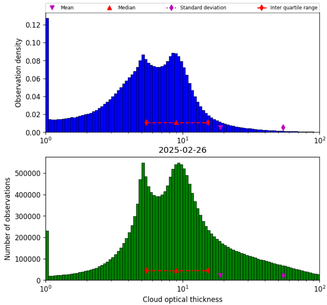
Figure 39: Histogram of “Cloud optical thickness” for 2025-02-26 to 2025-02-27
