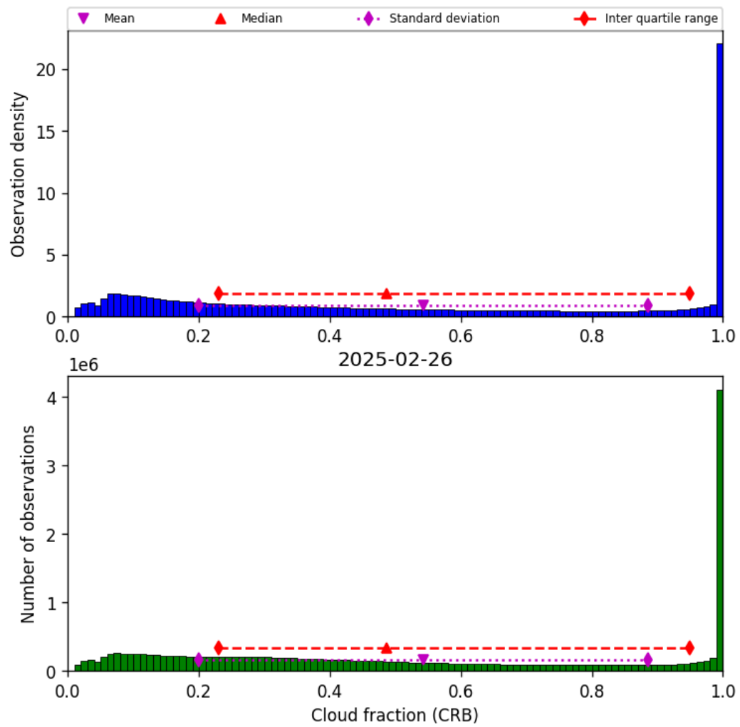
Figure 40: Histogram of “Cloud fraction (CRB)” for 2025-02-26 to 2025-02-27
