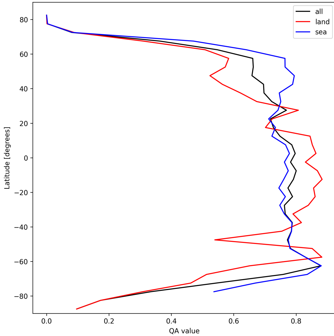
Figure 20: Zonal average of “QA value” for 2025-02-26 to 2025-02-27.
