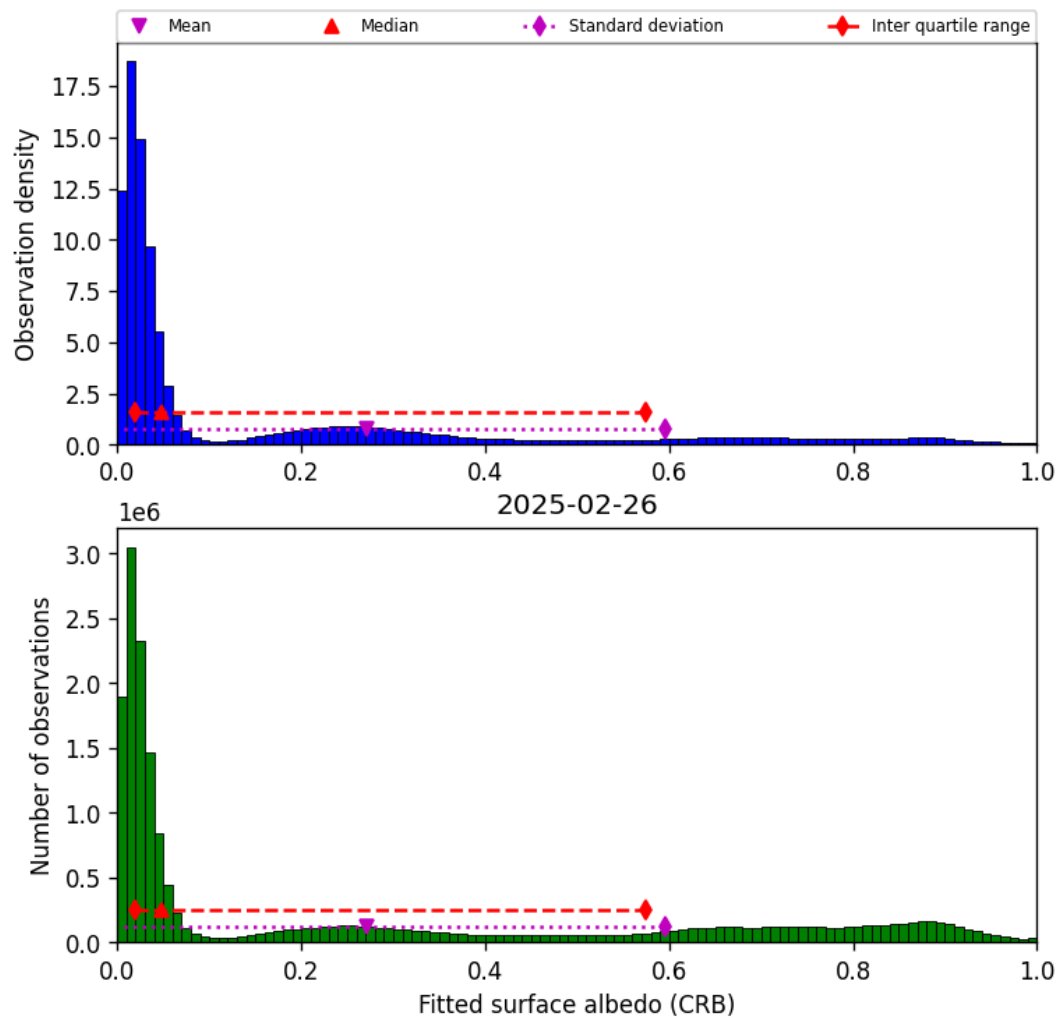
Figure 44: Histogram of “Fitted surface albedo (CRB)” for 2025-02-26 to 2025-02-27
