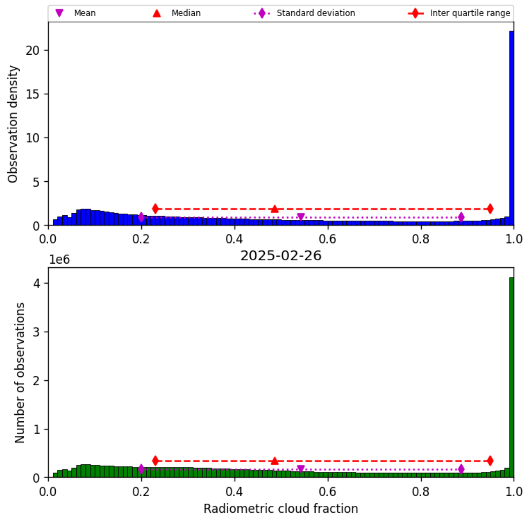
Figure 37: Histogram of “Radiometric cloud fraction” for 2025-02-26 to 2025-02-27
