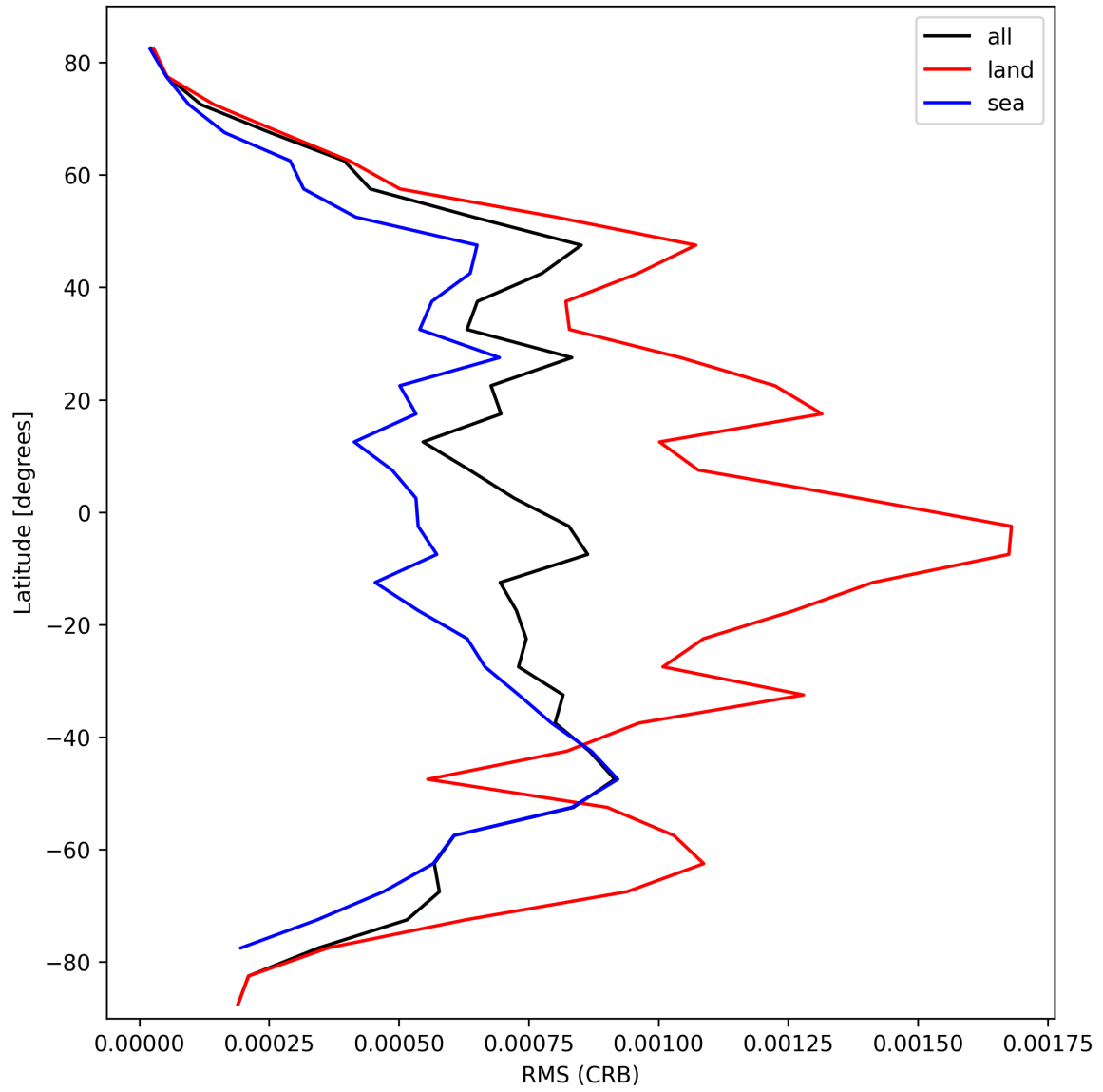
Figure 30: Zonal average of “RMS (CRB)” for 2025-02-26 to 2025-02-27.
