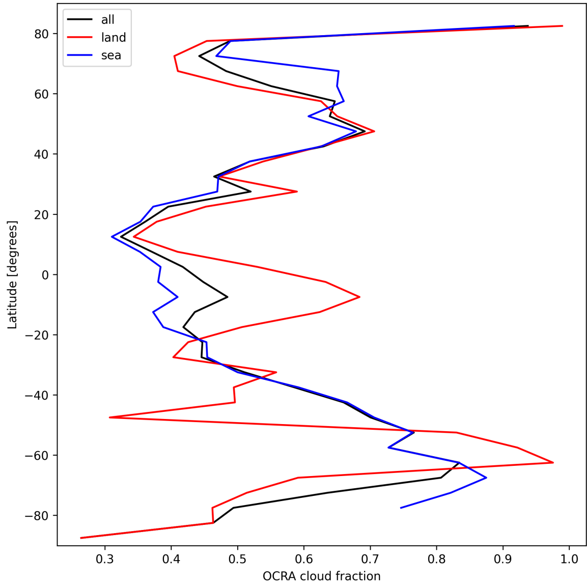
Figure 32: Zonal average of “OCRA cloud fraction” for 2025-02-26 to 2025-02-27.
