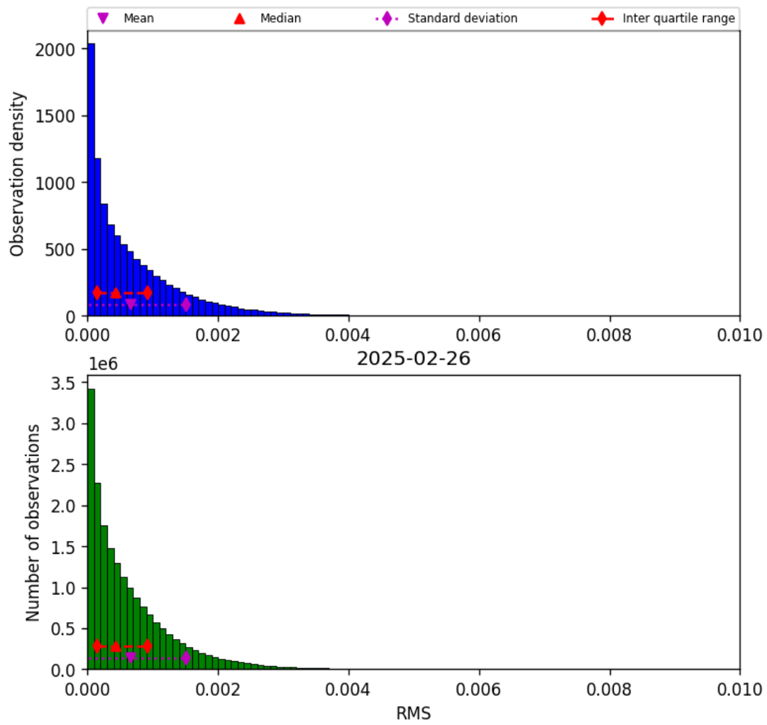
Figure 45: Histogram of “RMS” for 2025-02-26 to 2025-02-27
