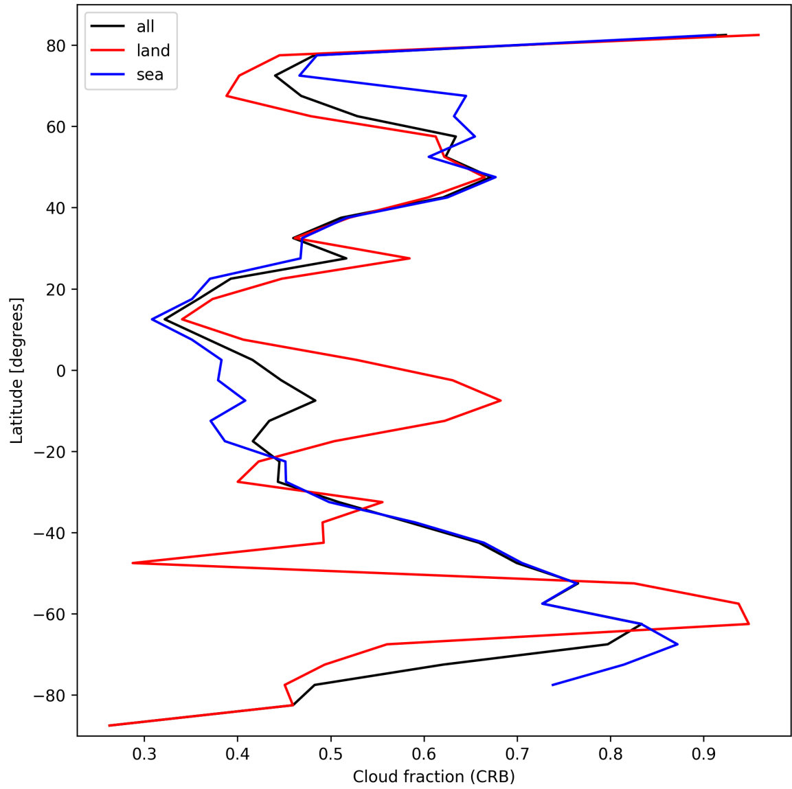
Figure 24: Zonal average of “Cloud fraction (CRB)” for 2025-02-26 to 2025-02-27.
