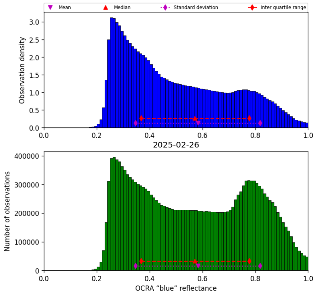
Figure 49: Histogram of “OCRA “blue” reflectance” for 2025-02-26 to 2025-02-27
