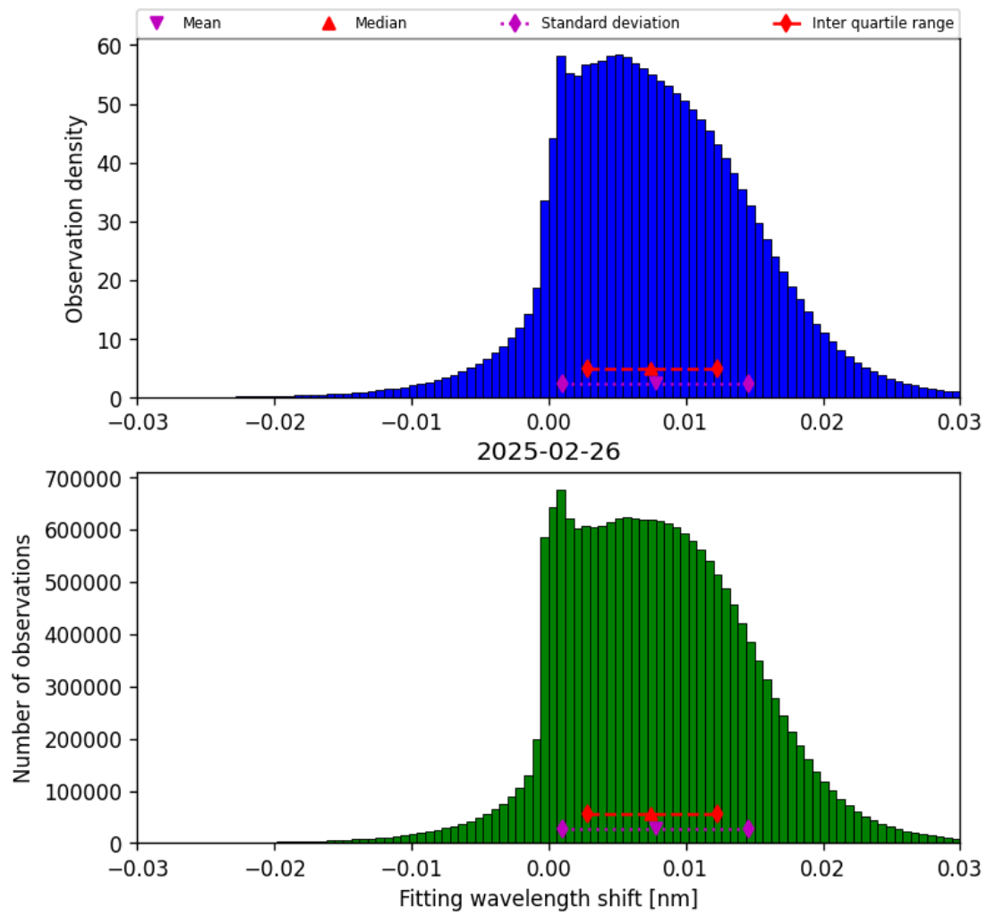
Figure 47: Histogram of “Fitting wavelength shift” for 2025-02-26 to 2025-02-27
