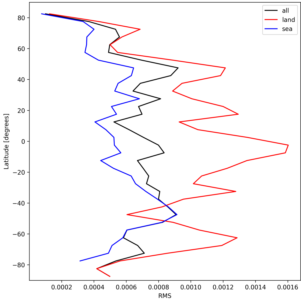
Figure 29: Zonal average of “RMS” for 2025-02-26 to 2025-02-27.
