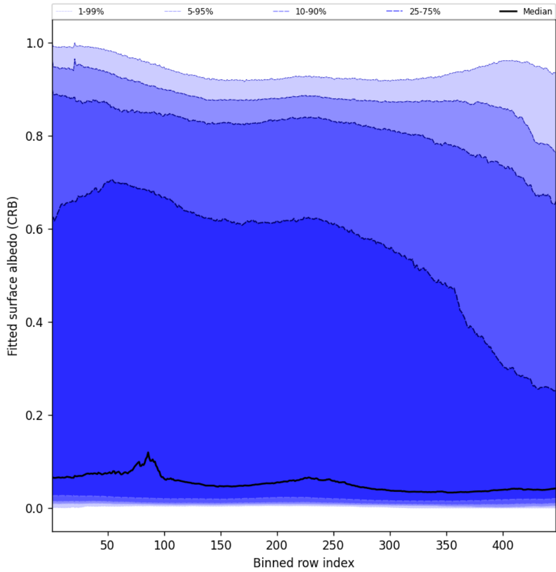
Figure 60: Along track statistics of “Fitted surface albedo (CRB)” for 2025-02-26 to 2025-02-27
