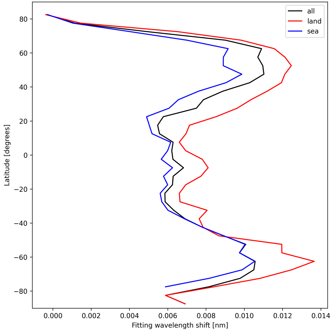
Figure 31: Zonal average of “Fitting wavelength shift” for 2025-02-26 to 2025-02-27.
