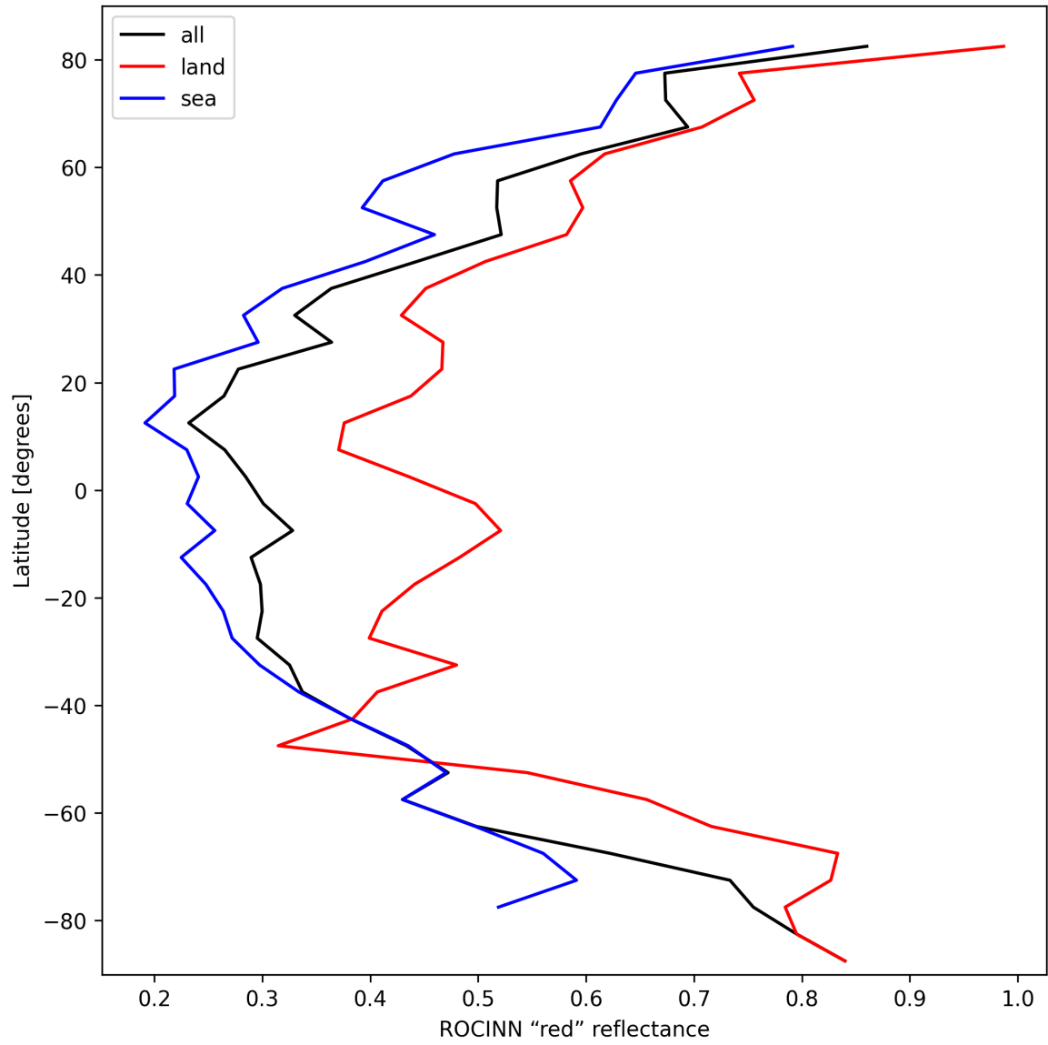
Figure 35: Zonal average of “ROCINN “red” reflectance” for 2025-02-26 to 2025-02-27.
