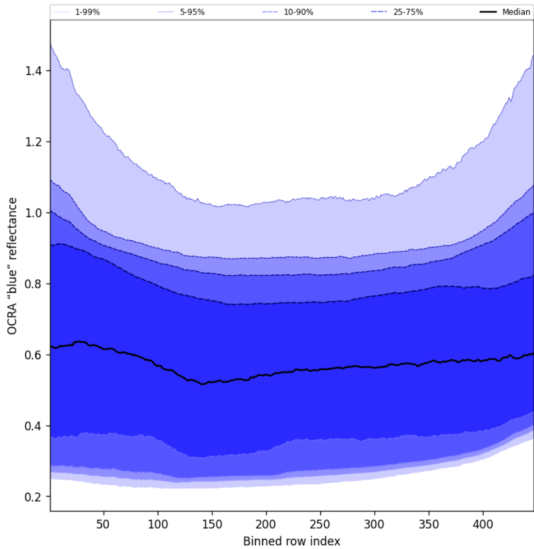
Figure 65: Along track statistics of “OCRA “blue” reflectance” for 2025-02-26 to 2025-02-27
