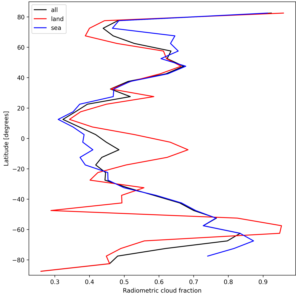
Figure 21: Zonal average of “Radiometric cloud fraction” for 2025-02-26 to 2025-02-27.
