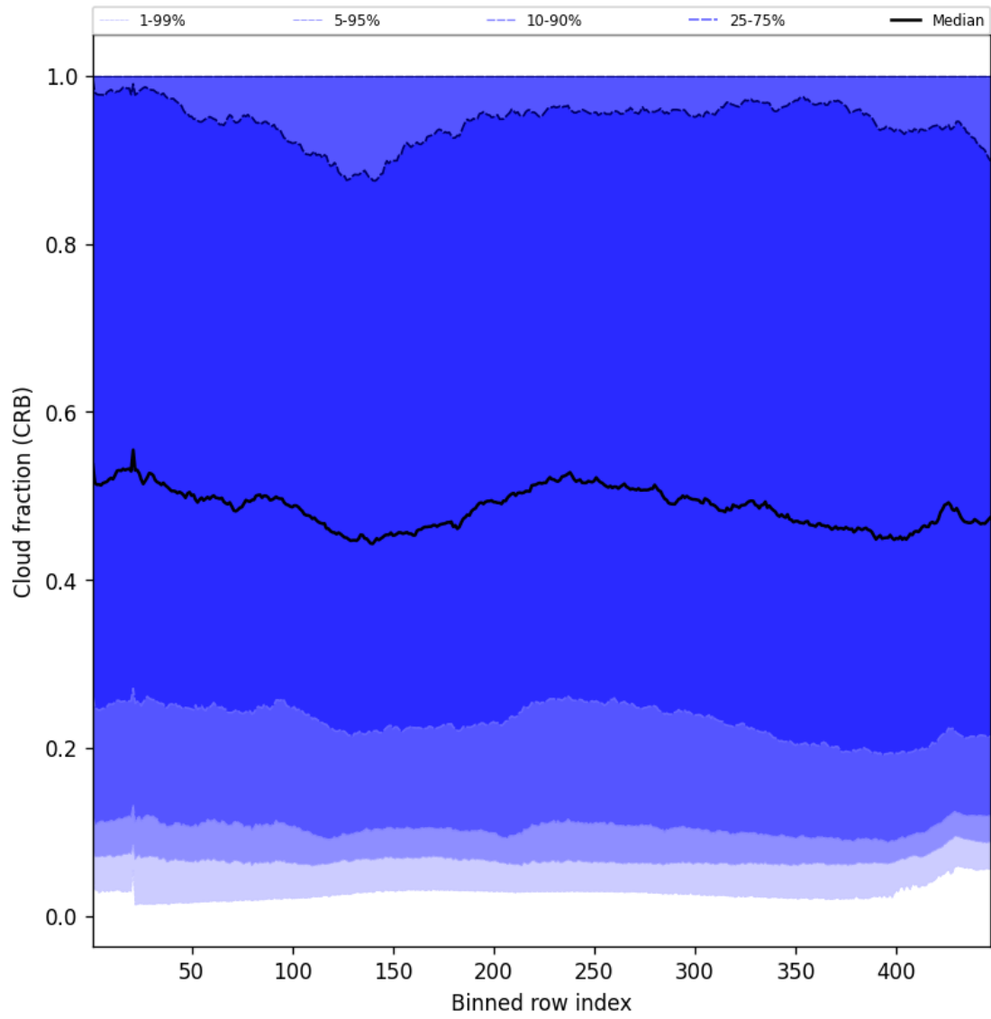
Figure 56: Along track statistics of “Cloud fraction (CRB)” for 2025-02-26 to 2025-02-27
