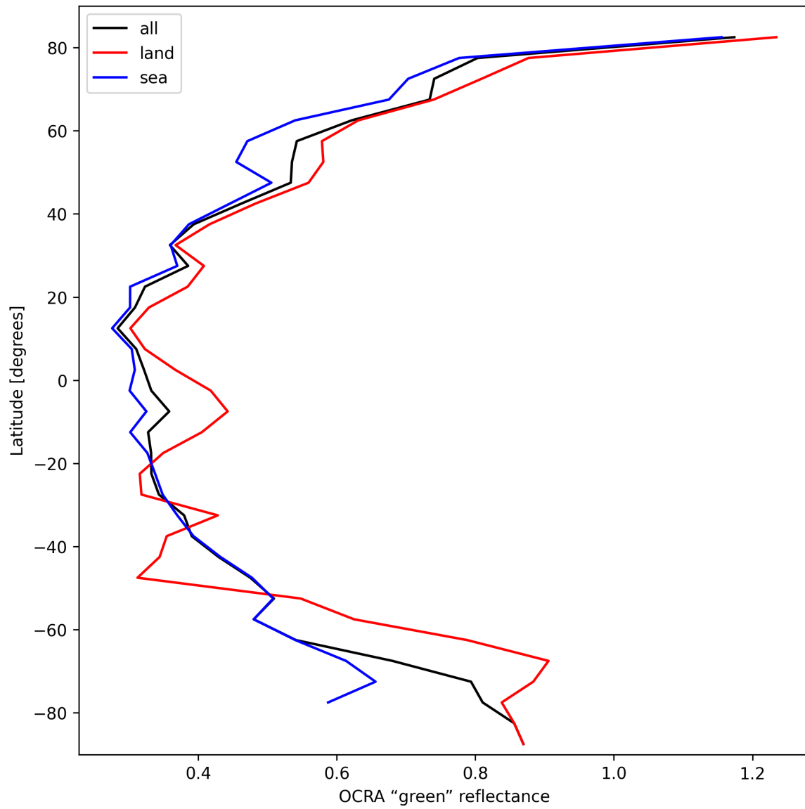
Figure 34: Zonal average of “OCRA “green” reflectance” for 2025-02-26 to 2025-02-27.
