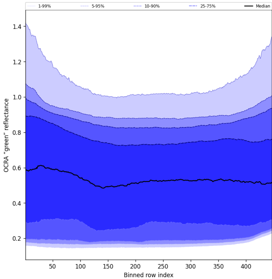
Figure 66: Along track statistics of “OCRA “green” reflectance” for 2025-02-26 to 2025-02-27
