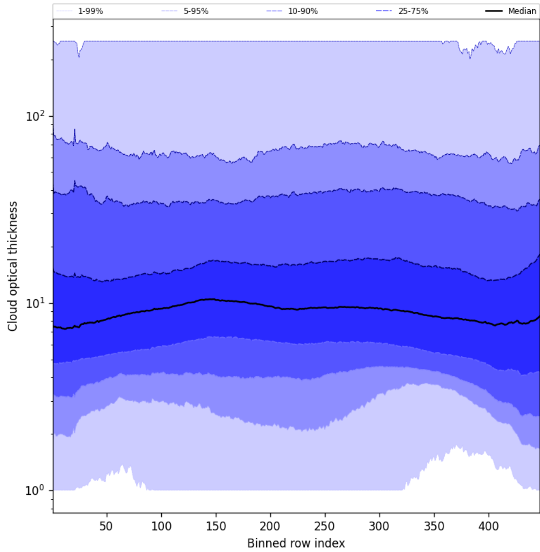
Figure 55: Along track statistics of “Cloud optical thickness” for 2025-02-26 to 2025-02-27
