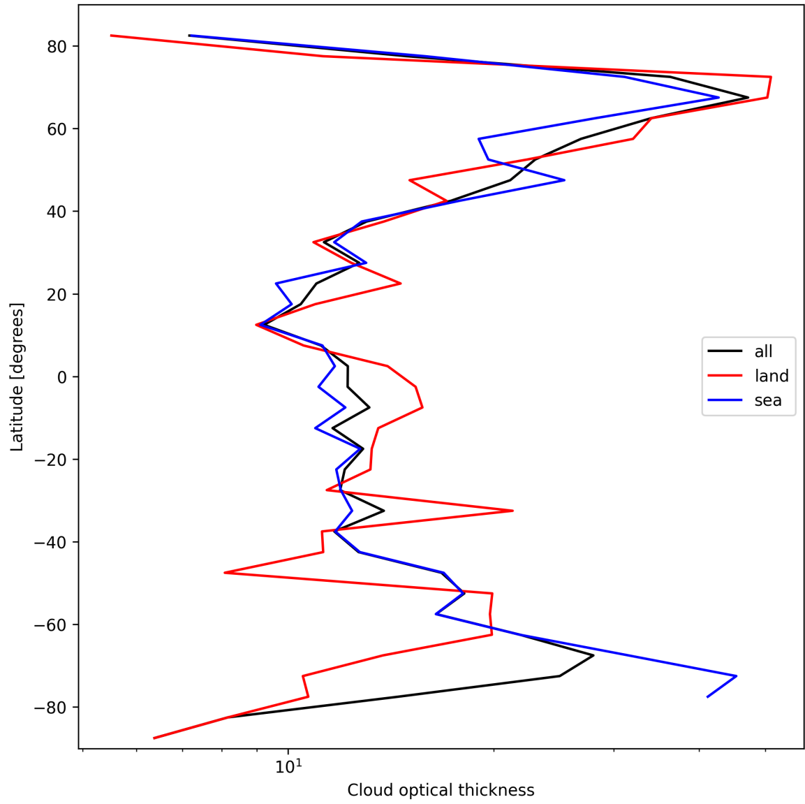
Figure 23: Zonal average of “Cloud optical thickness” for 2025-02-26 to 2025-02-27.
