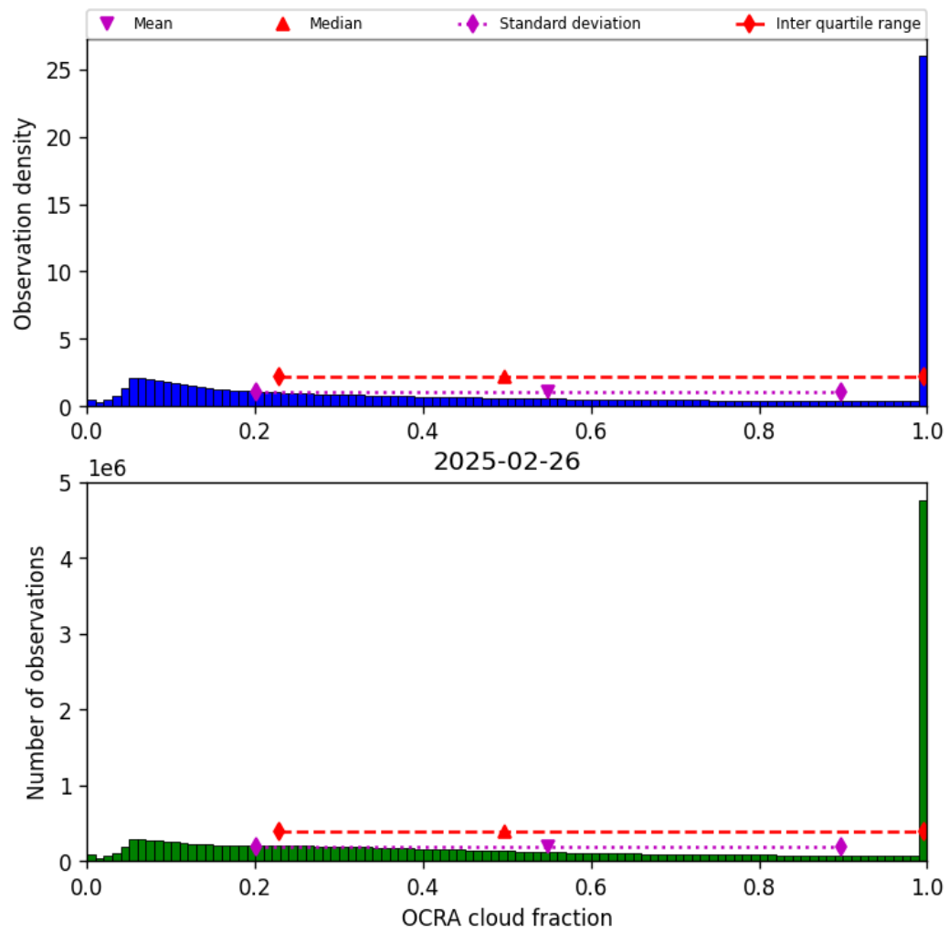
Figure 48: Histogram of “OCRA cloud fraction” for 2025-02-26 to 2025-02-27
