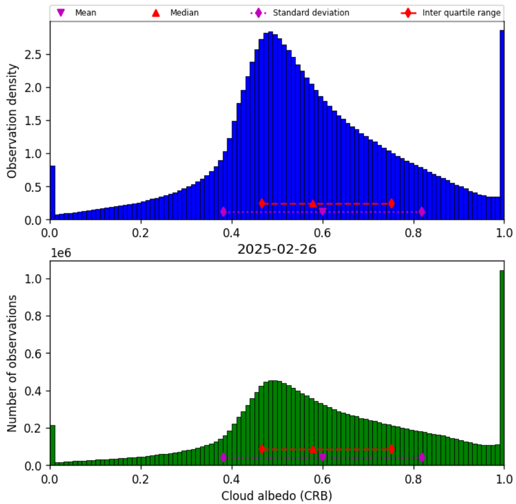
Figure 42: Histogram of “Cloud albedo (CRB)” for 2025-02-26 to 2025-02-27
