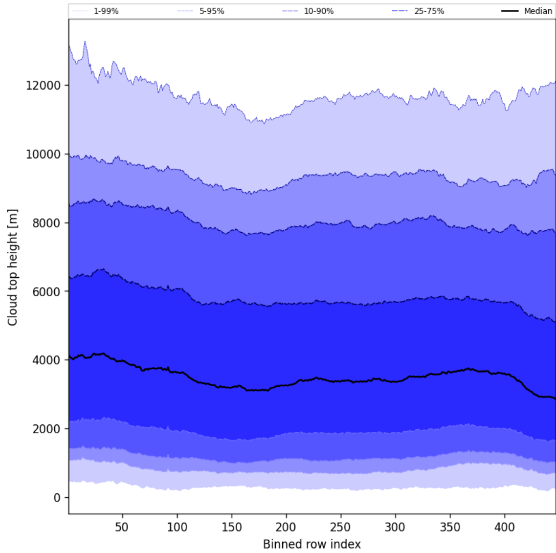
Figure 54: Along track statistics of “Cloud top height” for 2025-02-26 to 2025-02-27
