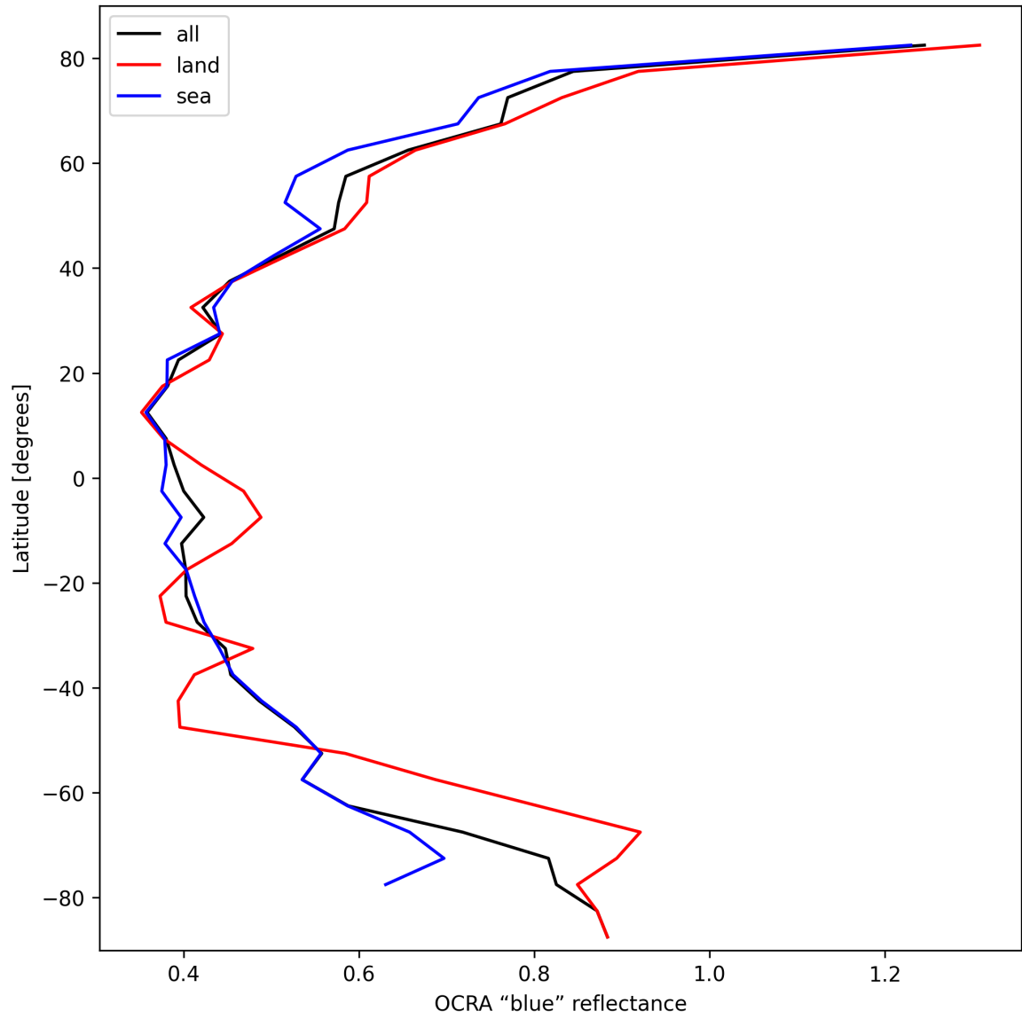
Figure 33: Zonal average of “OCRA “blue” reflectance” for 2025-02-26 to 2025-02-27.
