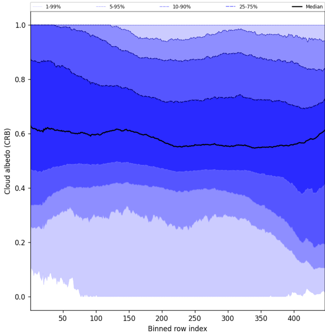
Figure 58: Along track statistics of “Cloud albedo (CRB)” for 2025-02-26 to 2025-02-27
