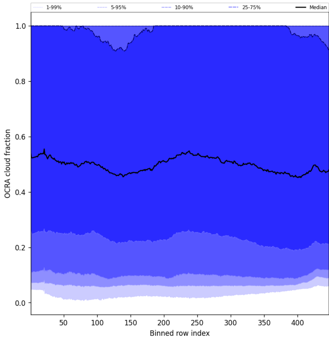
Figure 64: Along track statistics of “OCRA cloud fraction” for 2025-02-26 to 2025-02-27
