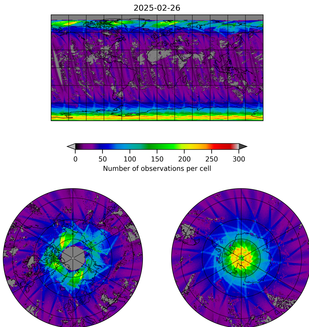
Figure 19: Map of the number of observations for 2025-02-26 to 2025-02-27
