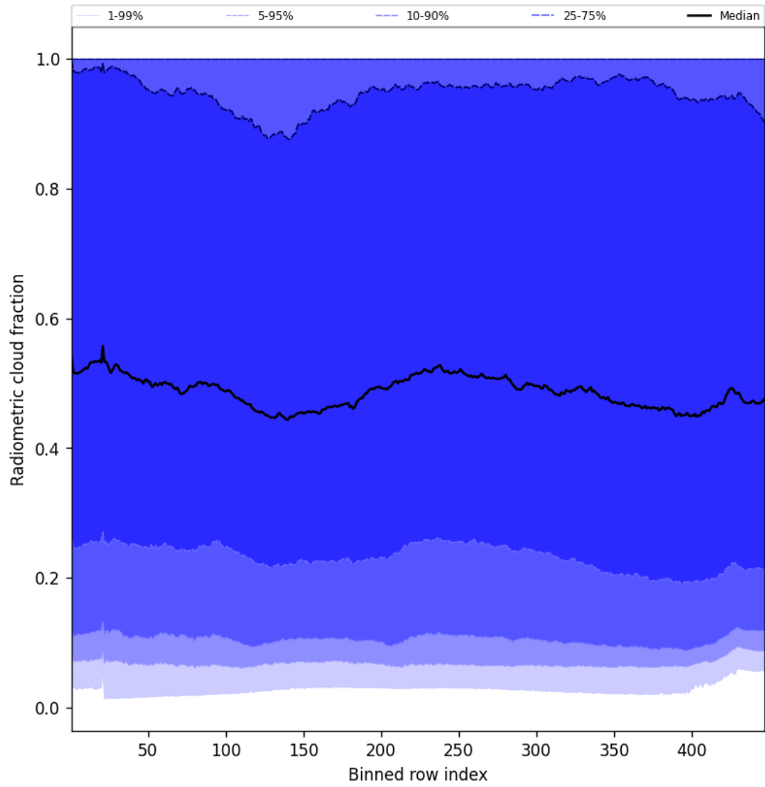
Figure 53: Along track statistics of “Radiometric cloud fraction” for 2025-02-26 to 2025-02-27
