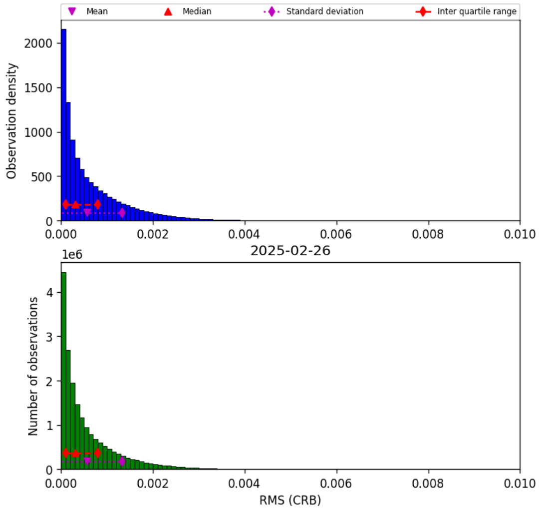
Figure 46: Histogram of “RMS (CRB)” for 2025-02-26 to 2025-02-27
