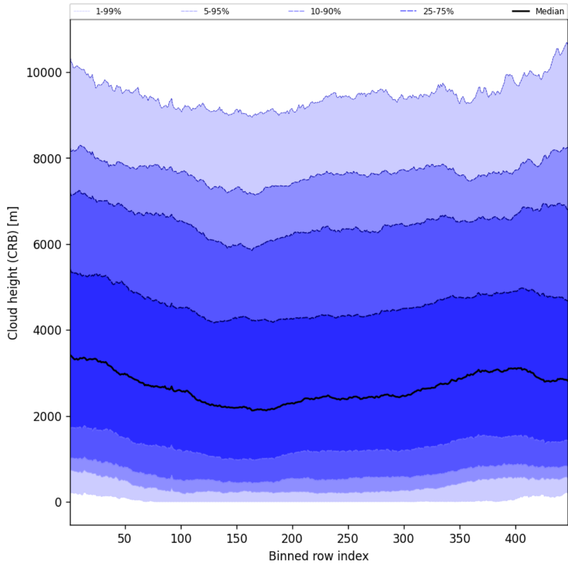
Figure 57: Along track statistics of “Cloud height (CRB)” for 2025-02-26 to 2025-02-27
