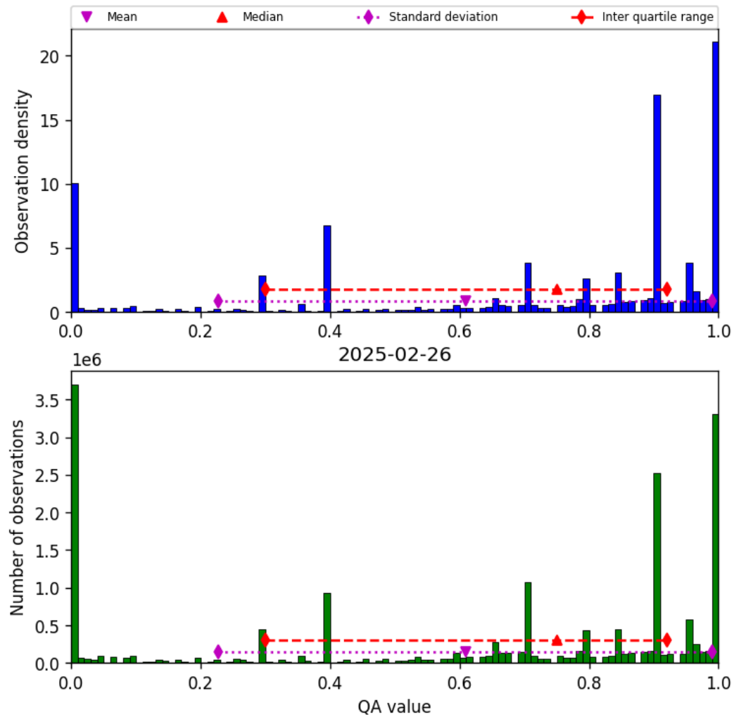
Figure 36: Histogram of “QA value” for 2025-02-26 to 2025-02-27
