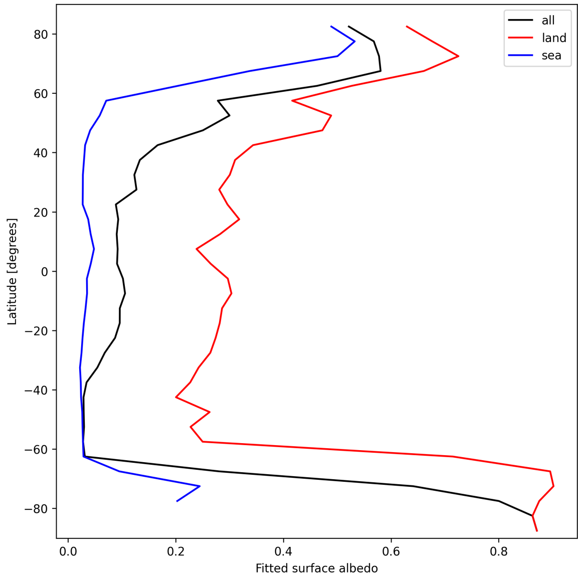
Figure 27: Zonal average of “Fitted surface albedo” for 2025-02-26 to 2025-02-27.
