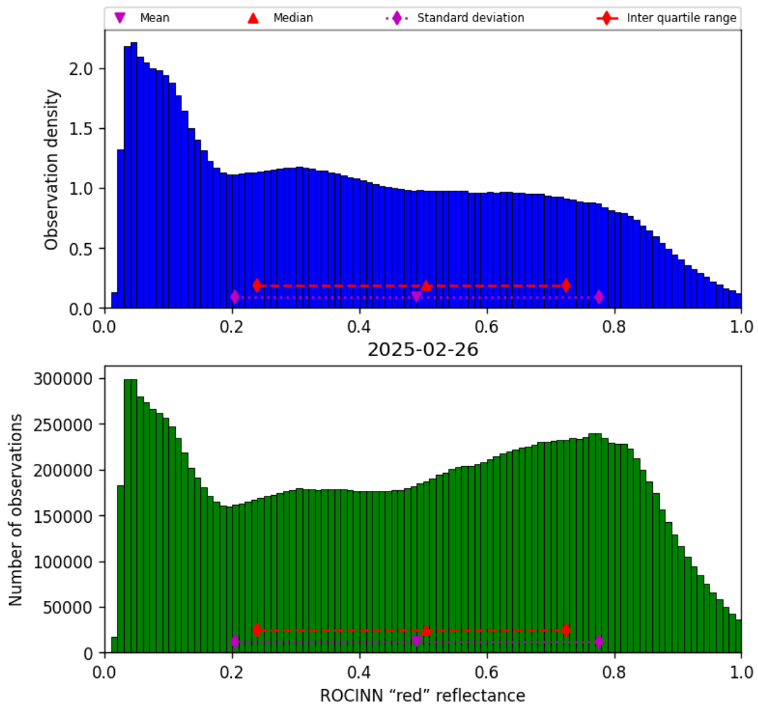
Figure 51: Histogram of “ROCINN “red” reflectance” for 2025-02-26 to 2025-02-27
