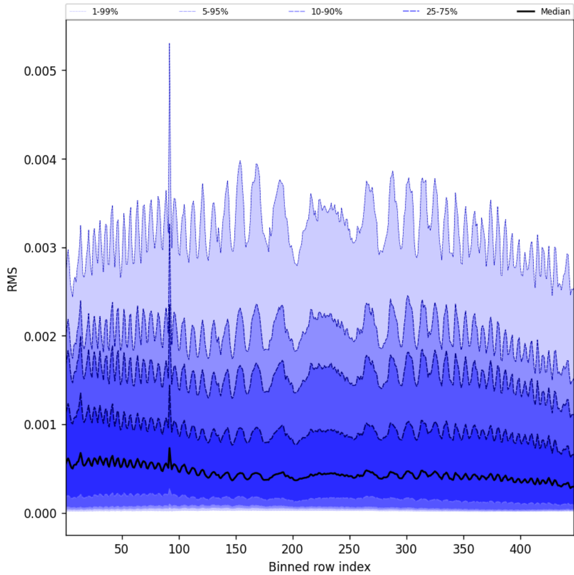
Figure 61: Along track statistics of “RMS” for 2025-02-26 to 2025-02-27
