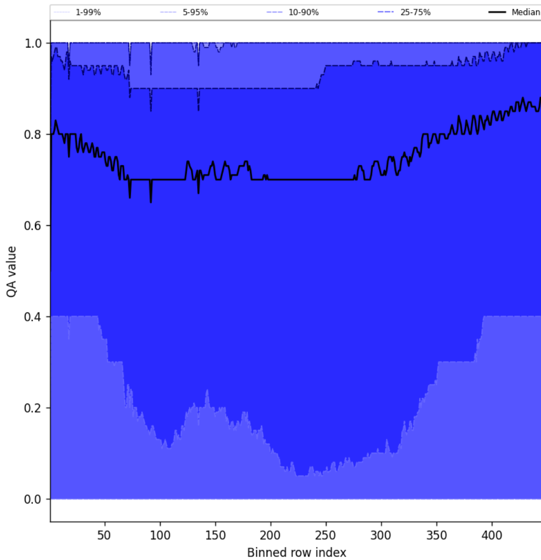
Figure 52: Along track statistics of “QA value” for 2025-02-26 to 2025-02-27
