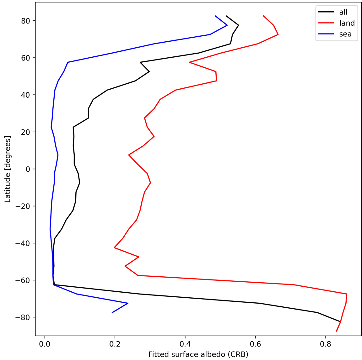
Figure 28: Zonal average of “Fitted surface albedo (CRB)” for 2025-02-26 to 2025-02-27.
