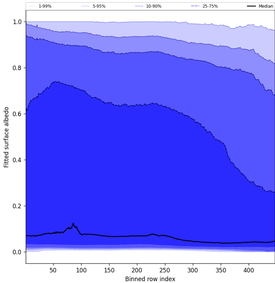
Figure 59: Along track statistics of “Fitted surface albedo” for 2025-02-26 to 2025-02-27
