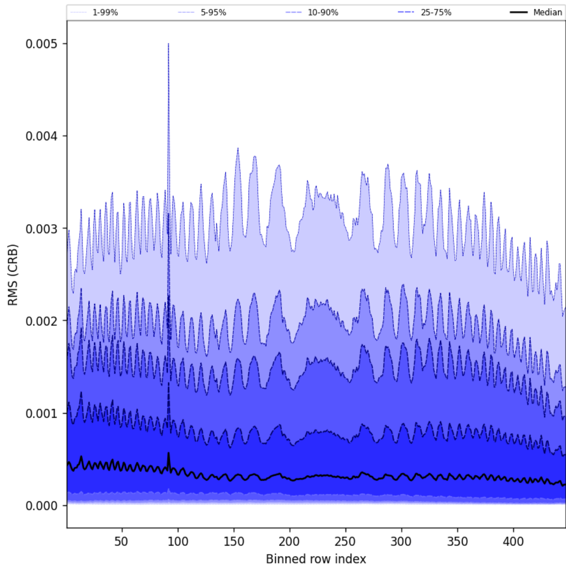
Figure 62: Along track statistics of “RMS (CRB)” for 2025-02-26 to 2025-02-27
