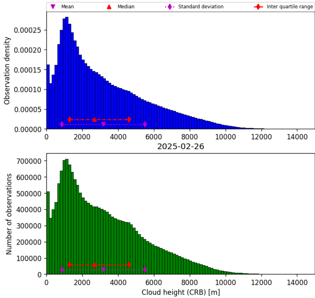
Figure 41: Histogram of “Cloud height (CRB)” for 2025-02-26 to 2025-02-27
