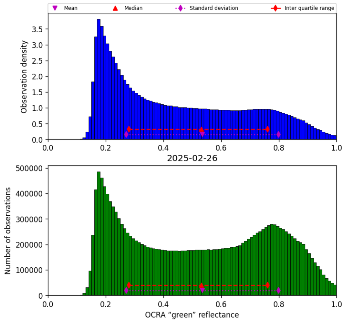
Figure 50: Histogram of “OCRA “green” reflectance” for 2025-02-26 to 2025-02-27
