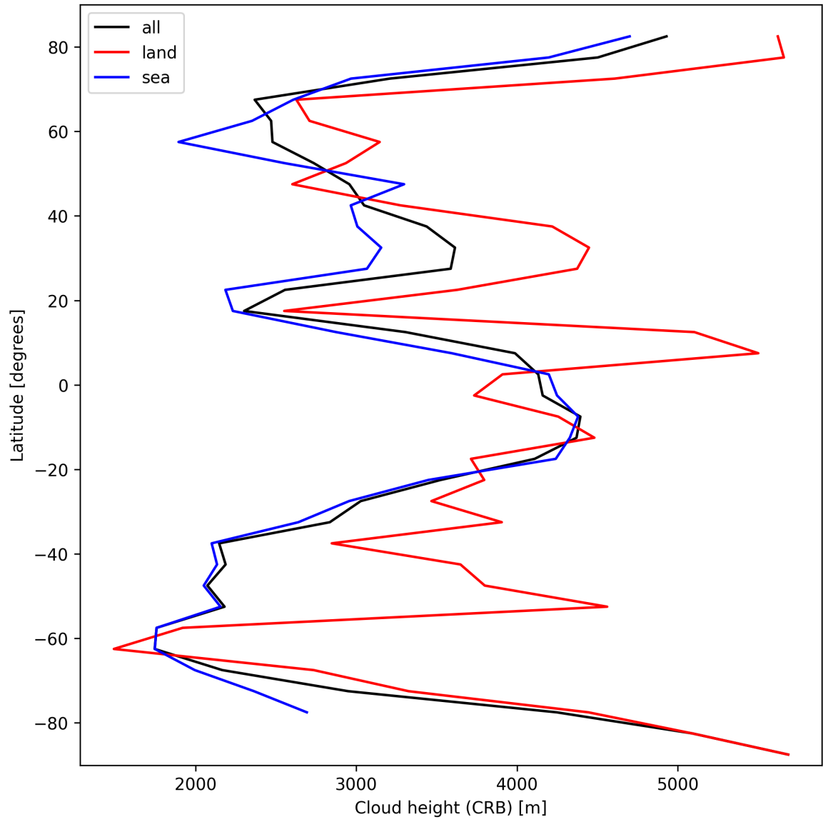
Figure 25: Zonal average of “Cloud height (CRB)” for 2025-02-26 to 2025-02-27.
