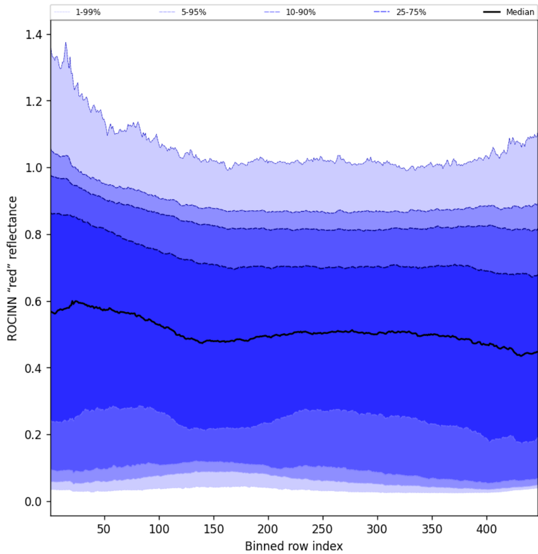
Figure 67: Along track statistics of "ROCINN "red" reflectance" for 2025-02-26 to 2025-02-27
