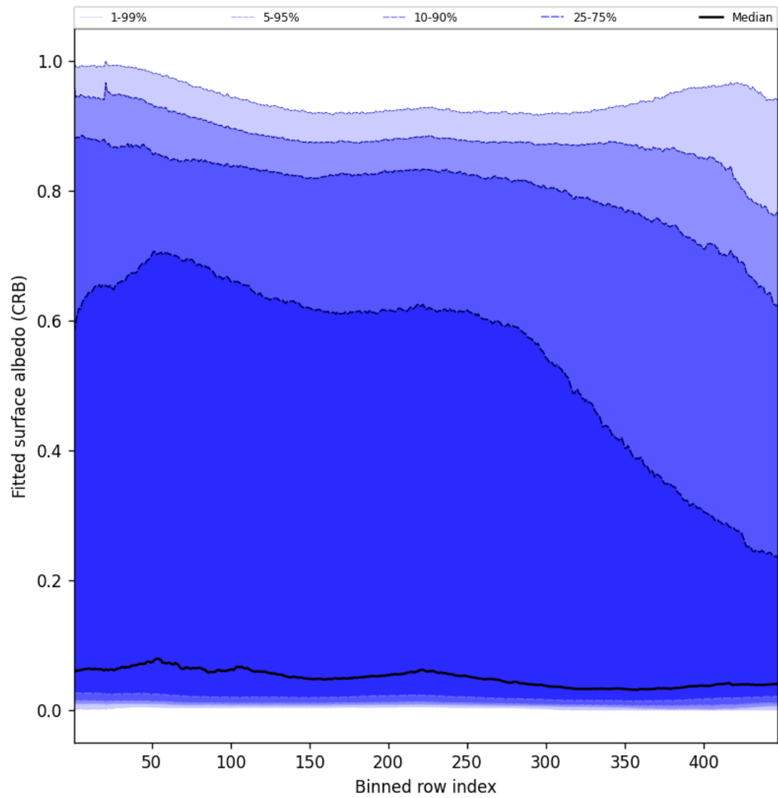
Figure 60: Along track statistics of “Fitted surface albedo (CRB)” for 2025-02-27 to 2025-02-27
