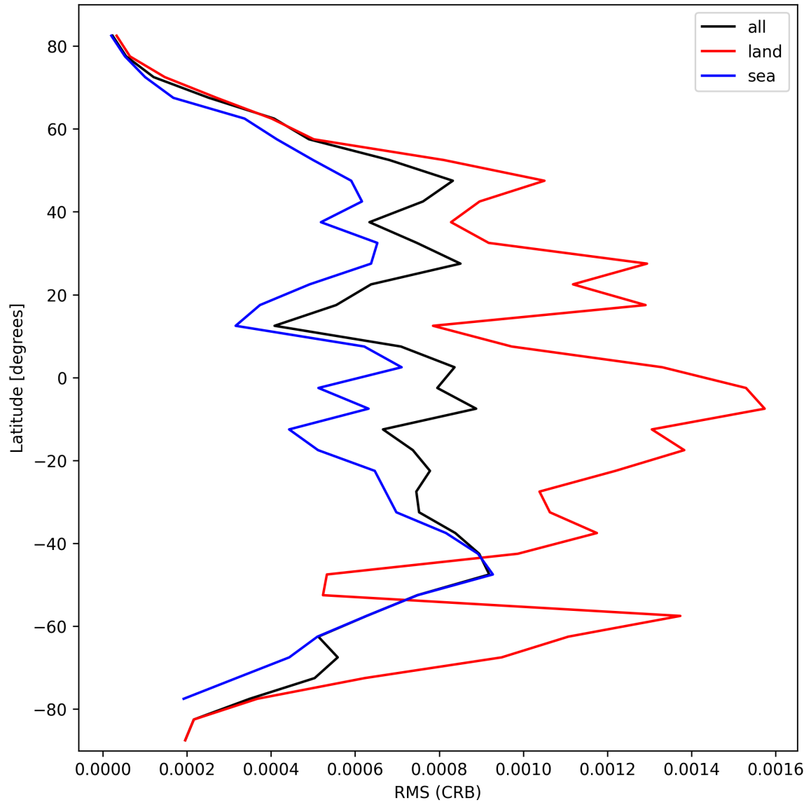
Figure 30: Zonal average of “RMS (CRB)” for 2025-02-27 to 2025-02-27.
