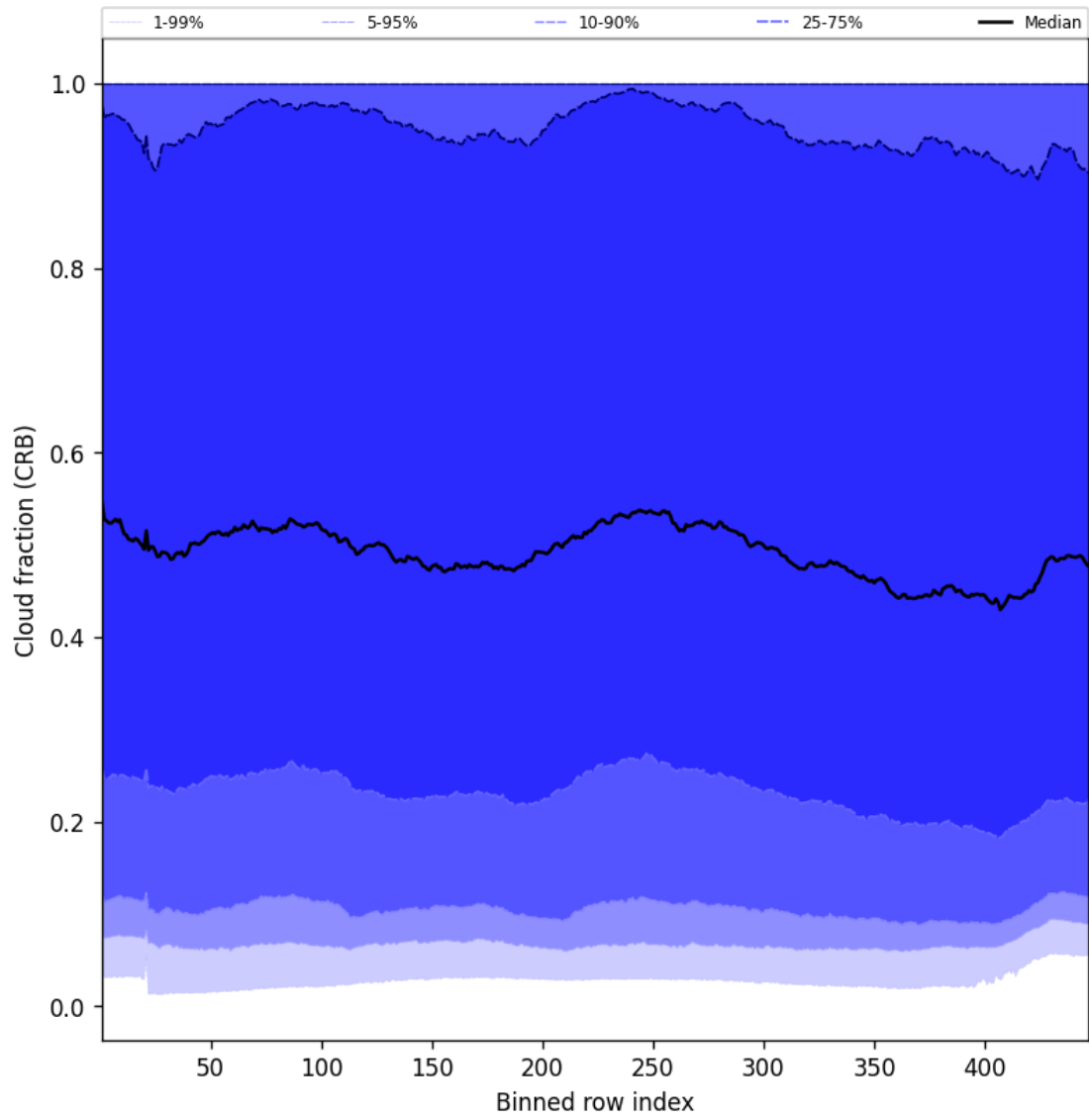
Figure 56: Along track statistics of “Cloud fraction (CRB)” for 2025-02-27 to 2025-02-27
