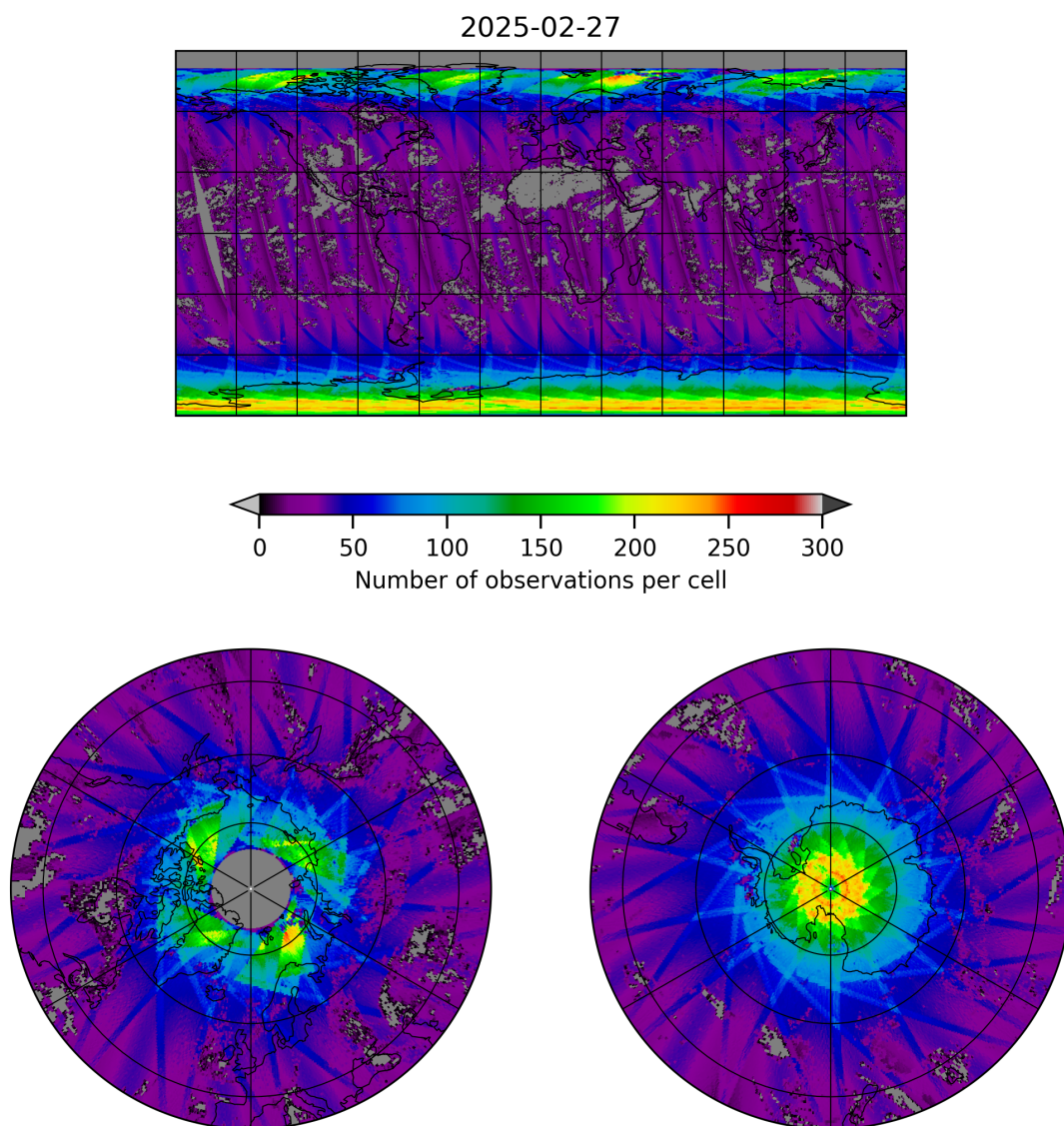
Figure 19: Map of the number of observations for 2025-02-27 to 2025-02-27
