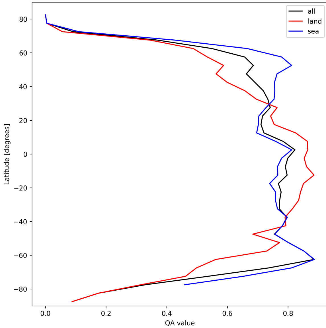
Figure 20: Zonal average of “QA value” for 2025-02-27 to 2025-02-27.
