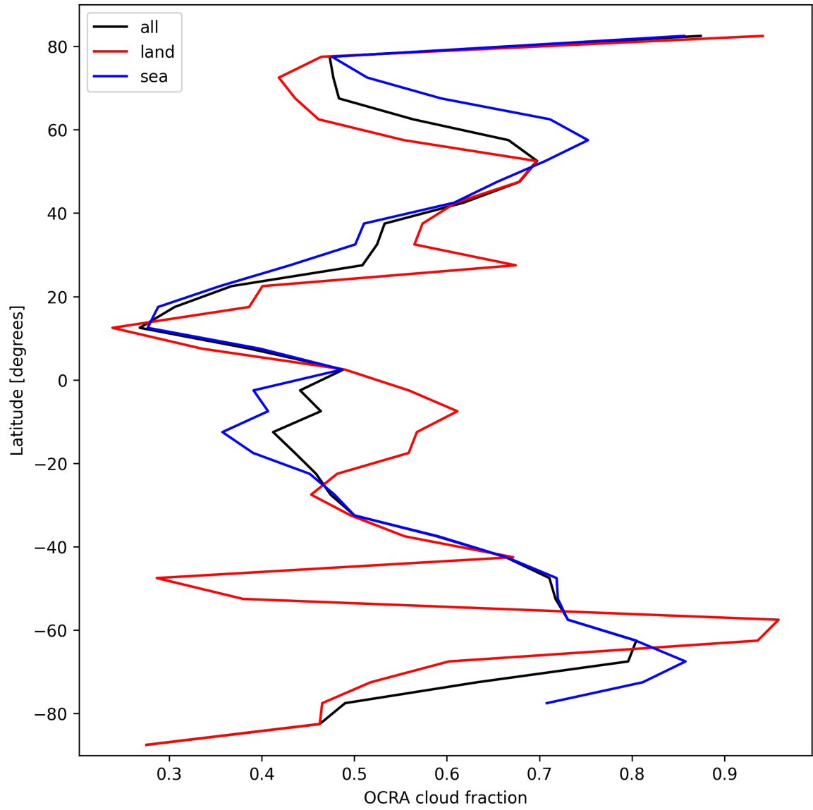
Figure 32: Zonal average of “OCRA cloud fraction” for 2025-02-27 to 2025-02-27.
