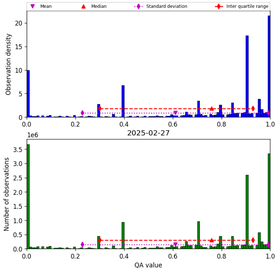
Figure 36: Histogram of “QA value” for 2025-02-27 to 2025-02-27
