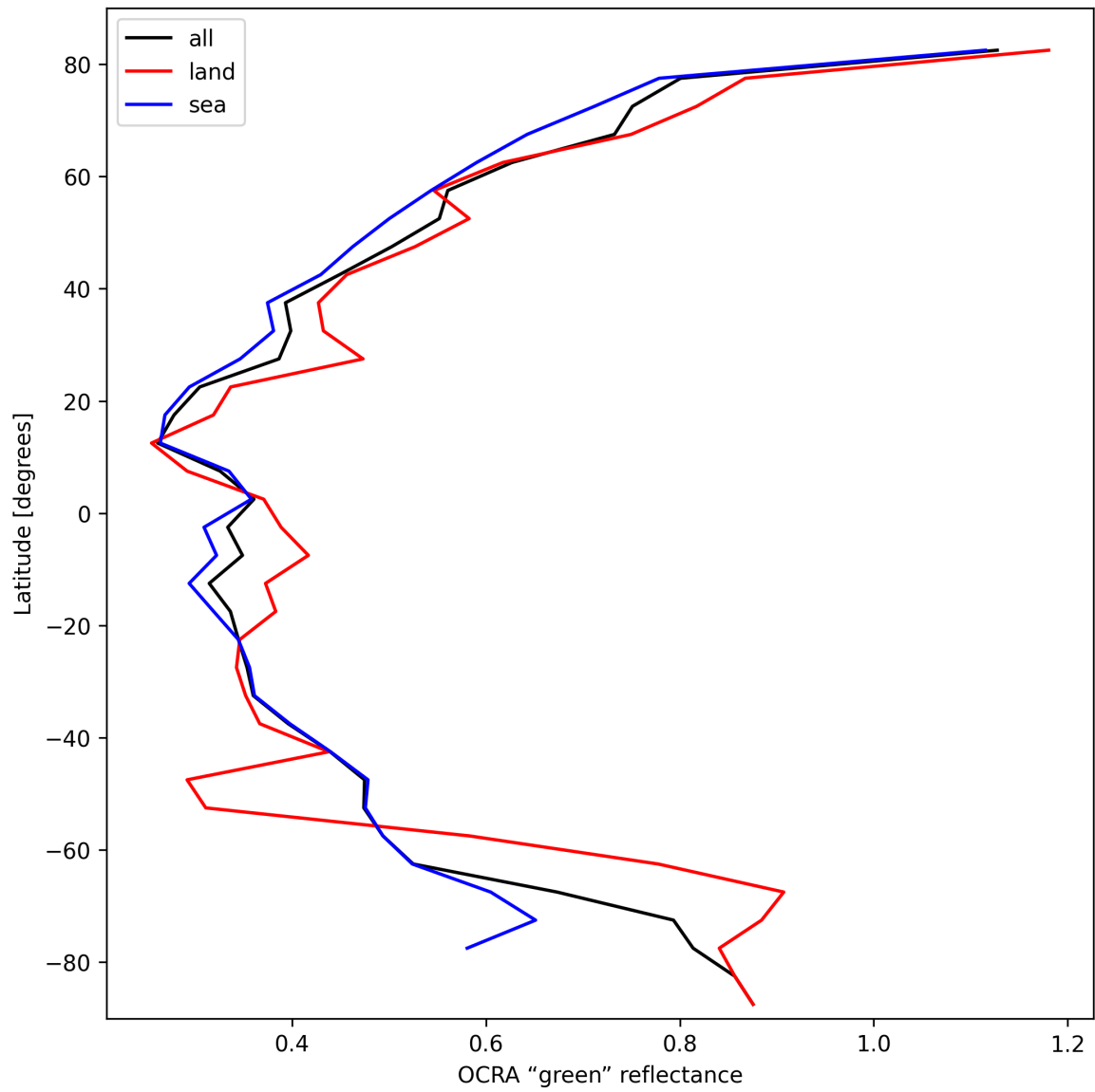
Figure 34: Zonal average of “OCRA “green” reflectance” for 2025-02-27 to 2025-02-27.
