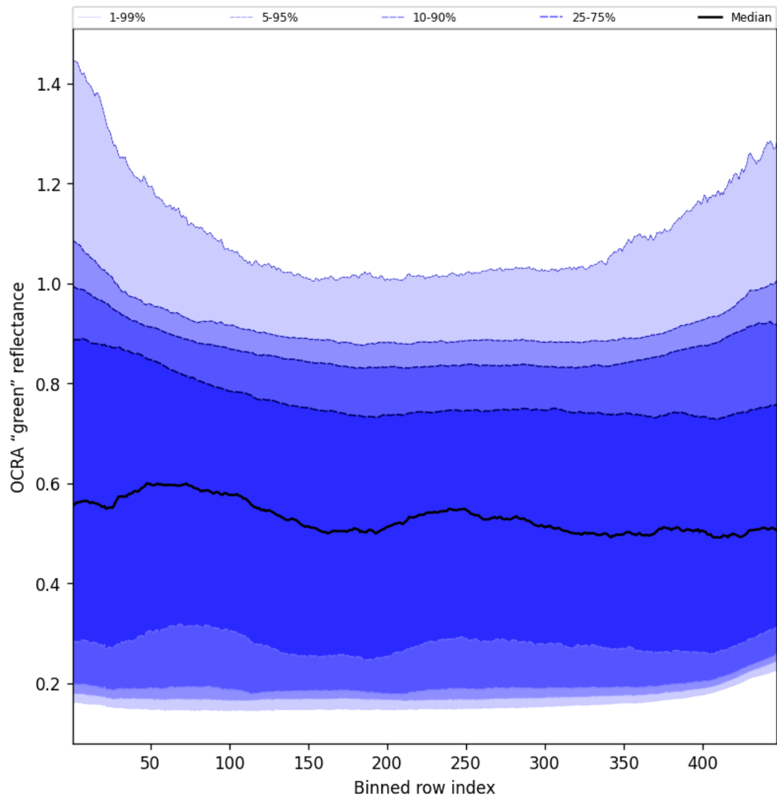
Figure 66: Along track statistics of “OCRA “green” reflectance” for 2025-02-27 to 2025-02-27
