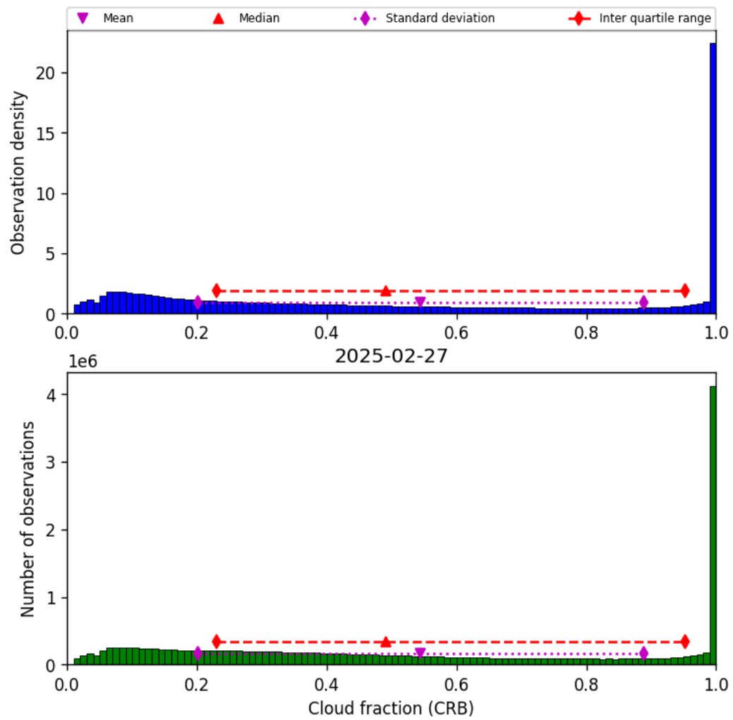
Figure 40: Histogram of “Cloud fraction (CRB)” for 2025-02-27 to 2025-02-27
