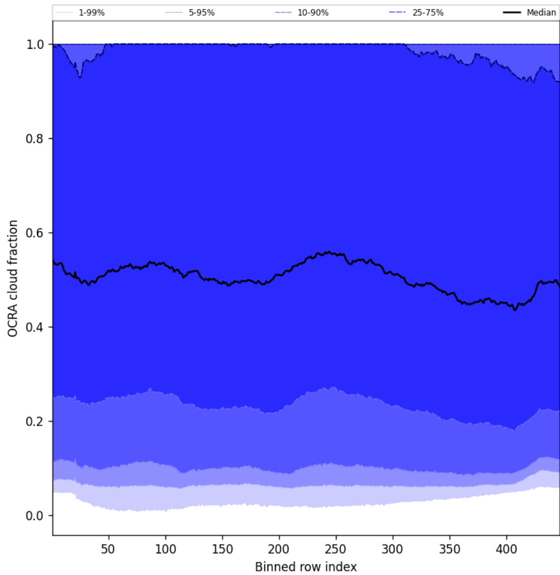
Figure 64: Along track statistics of “OCRA cloud fraction” for 2025-02-27 to 2025-02-27
