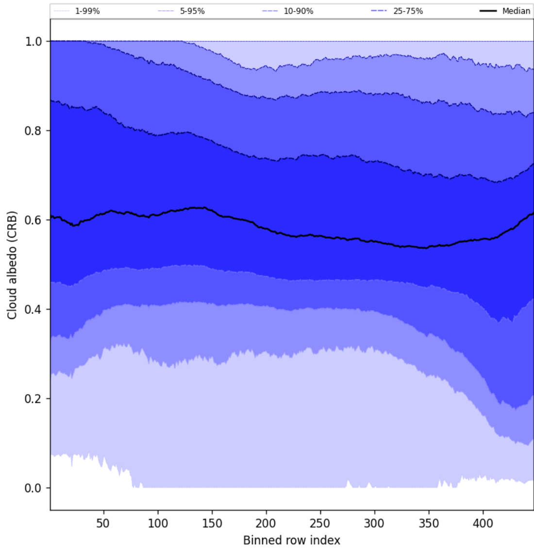
Figure 58: Along track statistics of “Cloud albedo (CRB)” for 2025-02-27 to 2025-02-27
