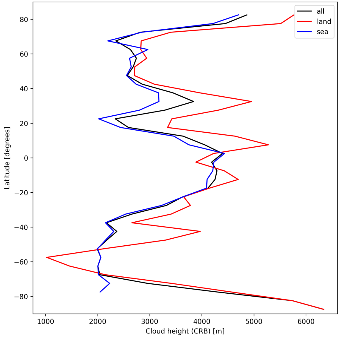
Figure 25: Zonal average of “Cloud height (CRB)” for 2025-02-27 to 2025-02-27.
