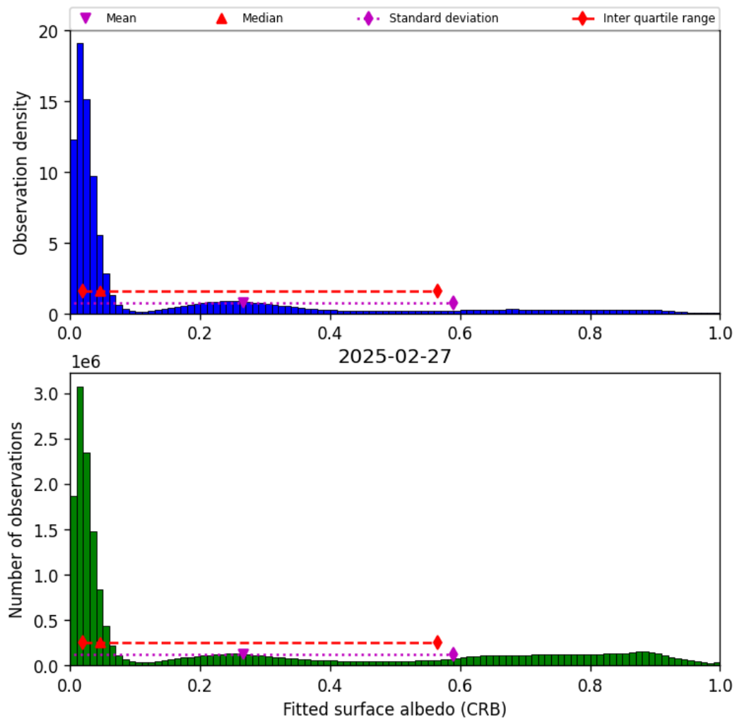
Figure 44: Histogram of “Fitted surface albedo (CRB)” for 2025-02-27 to 2025-02-27
