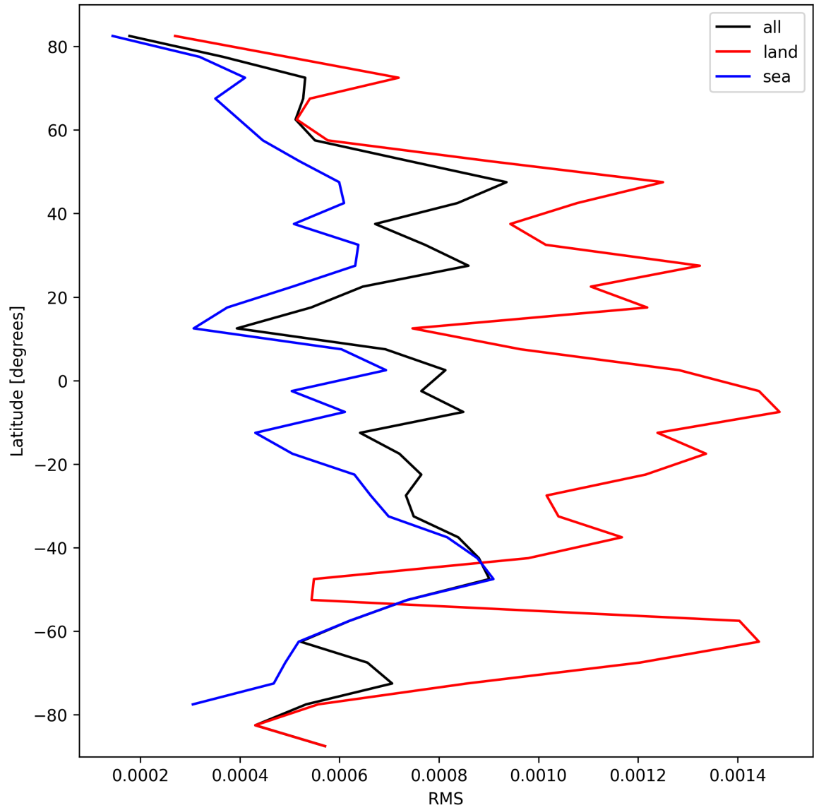
Figure 29: Zonal average of “RMS” for 2025-02-27 to 2025-02-27.
