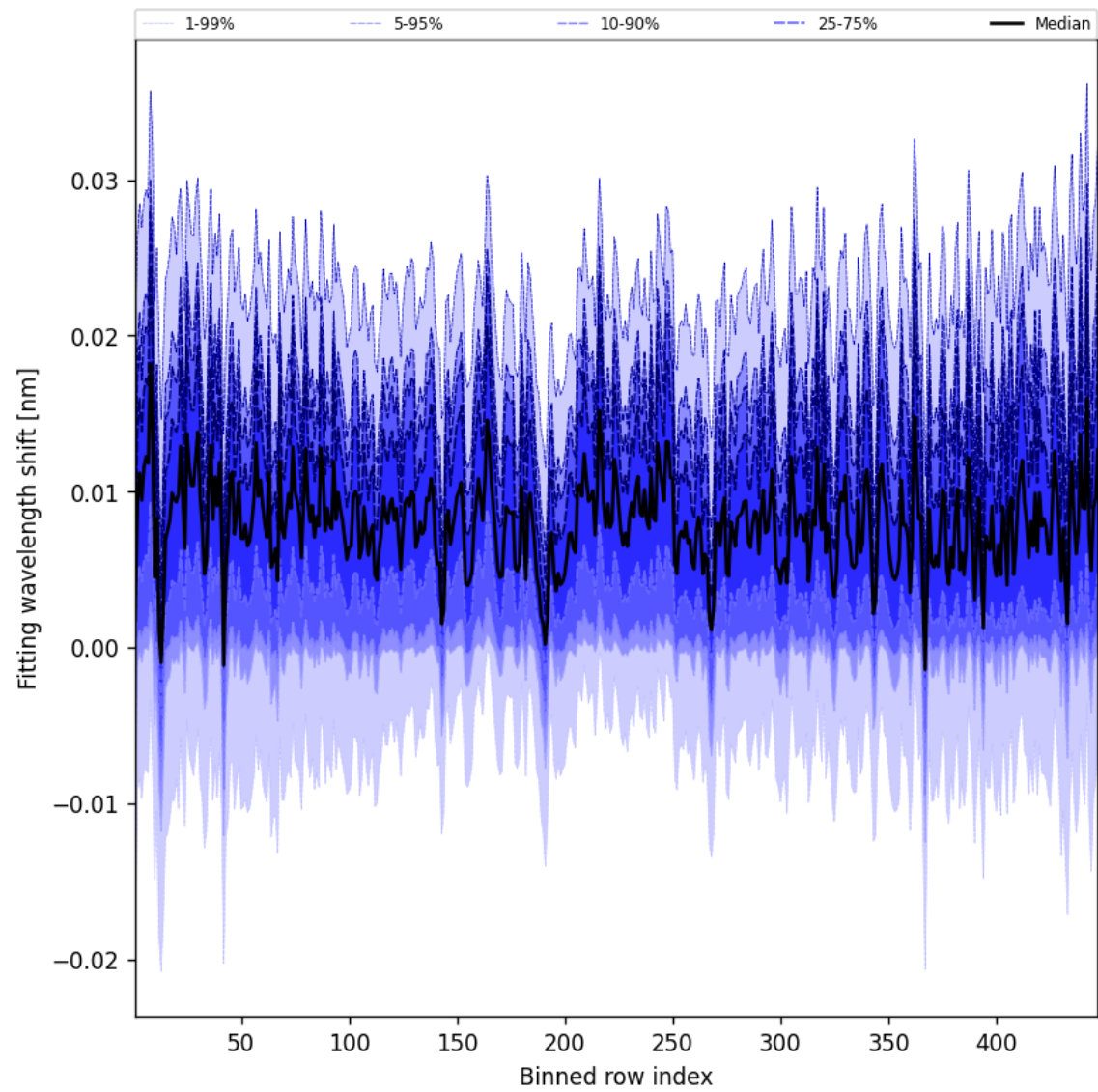
Figure 63: Along track statistics of “Fitting wavelength shift” for 2025-02-27 to 2025-02-27
