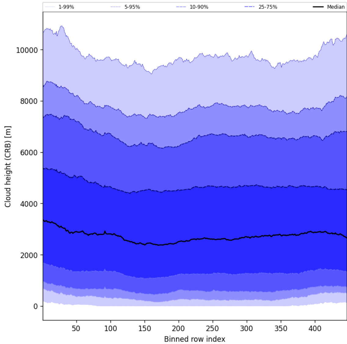
Figure 57: Along track statistics of “Cloud height (CRB)” for 2025-02-27 to 2025-02-27
