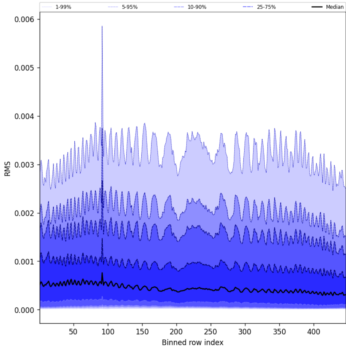
Figure 61: Along track statistics of “RMS” for 2025-02-27 to 2025-02-27
