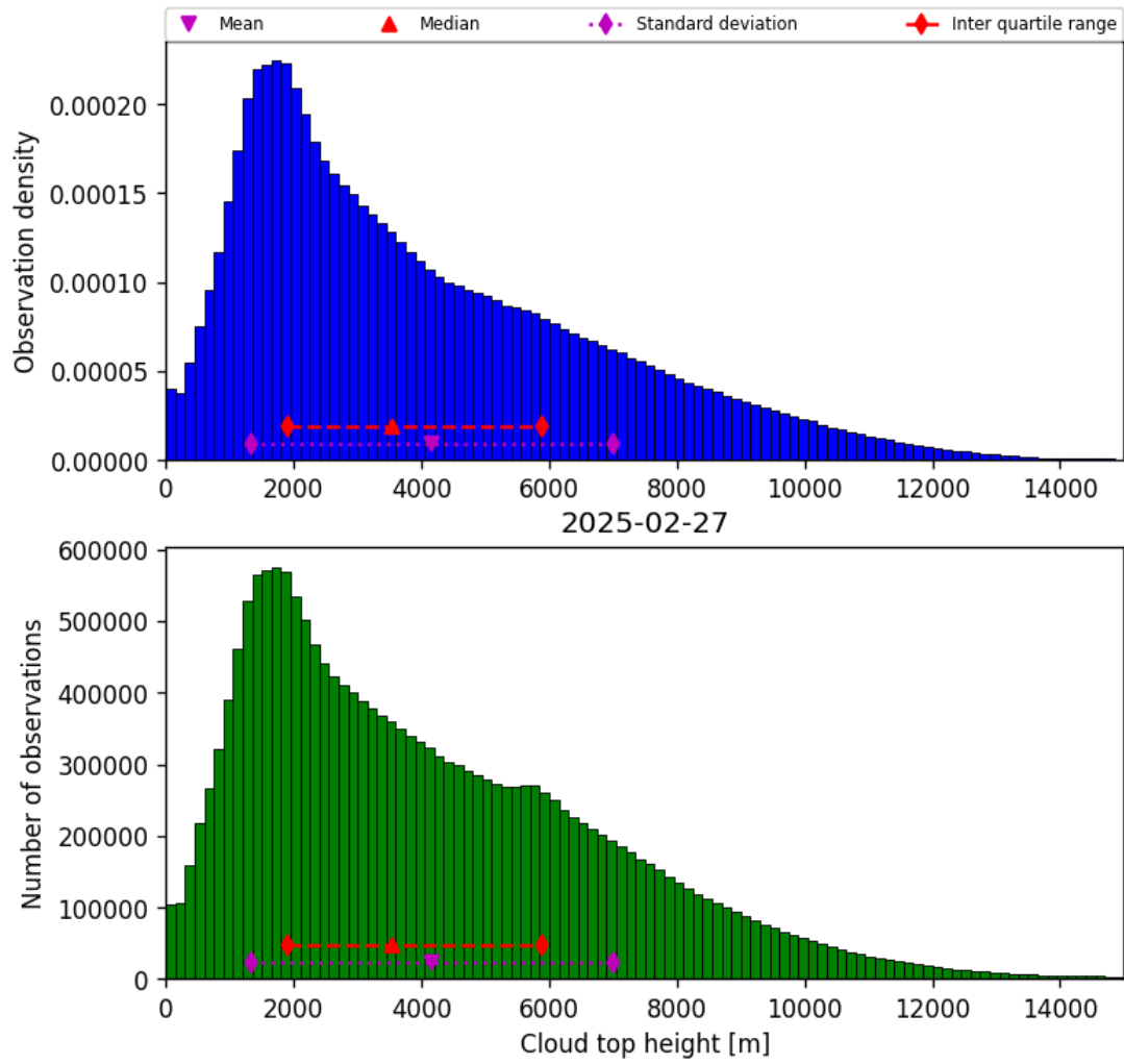
Figure 38: Histogram of “Cloud top height” for 2025-02-27 to 2025-02-27
