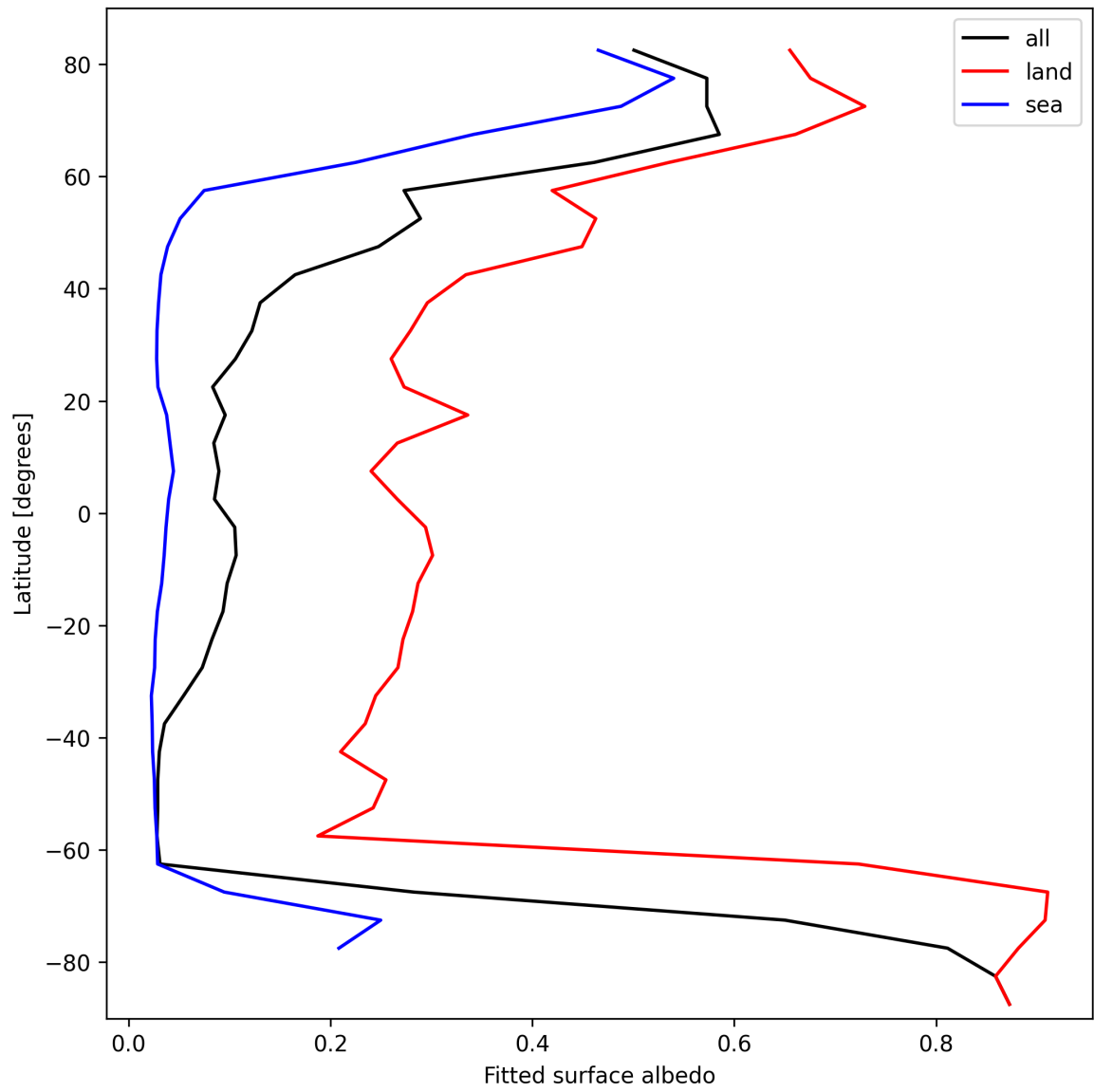
Figure 27: Zonal average of “Fitted surface albedo” for 2025-02-27 to 2025-02-27.
