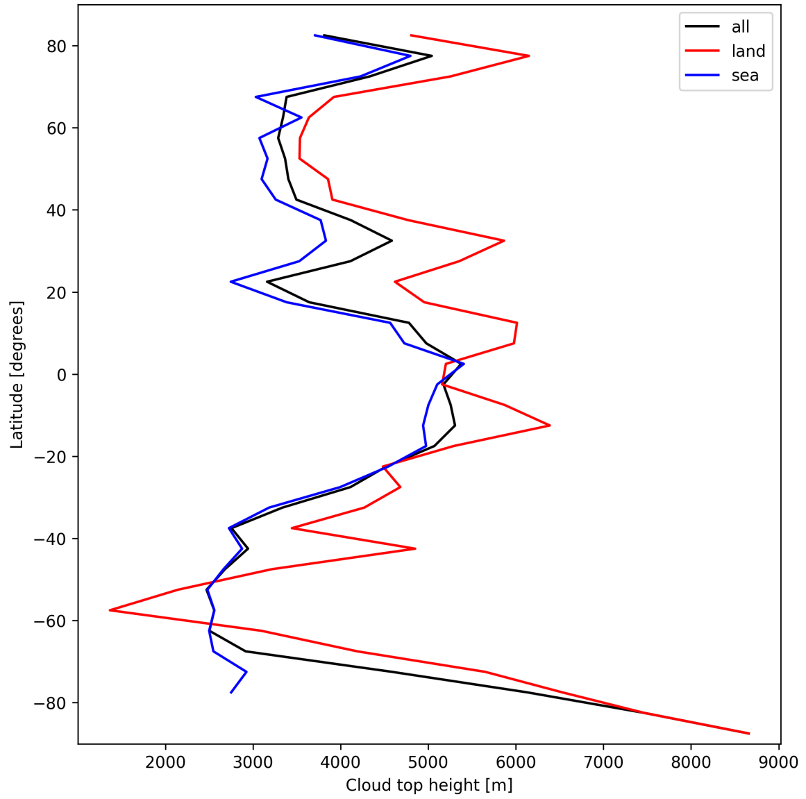
Figure 22: Zonal average of “Cloud top height” for 2025-02-27 to 2025-02-27.
