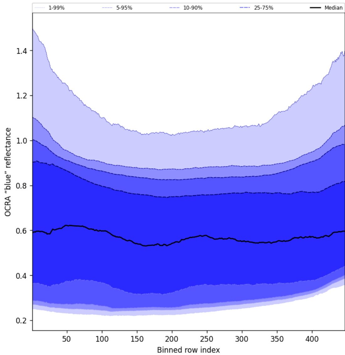
Figure 65: Along track statistics of “OCRA “blue” reflectance” for 2025-02-27 to 2025-02-27
