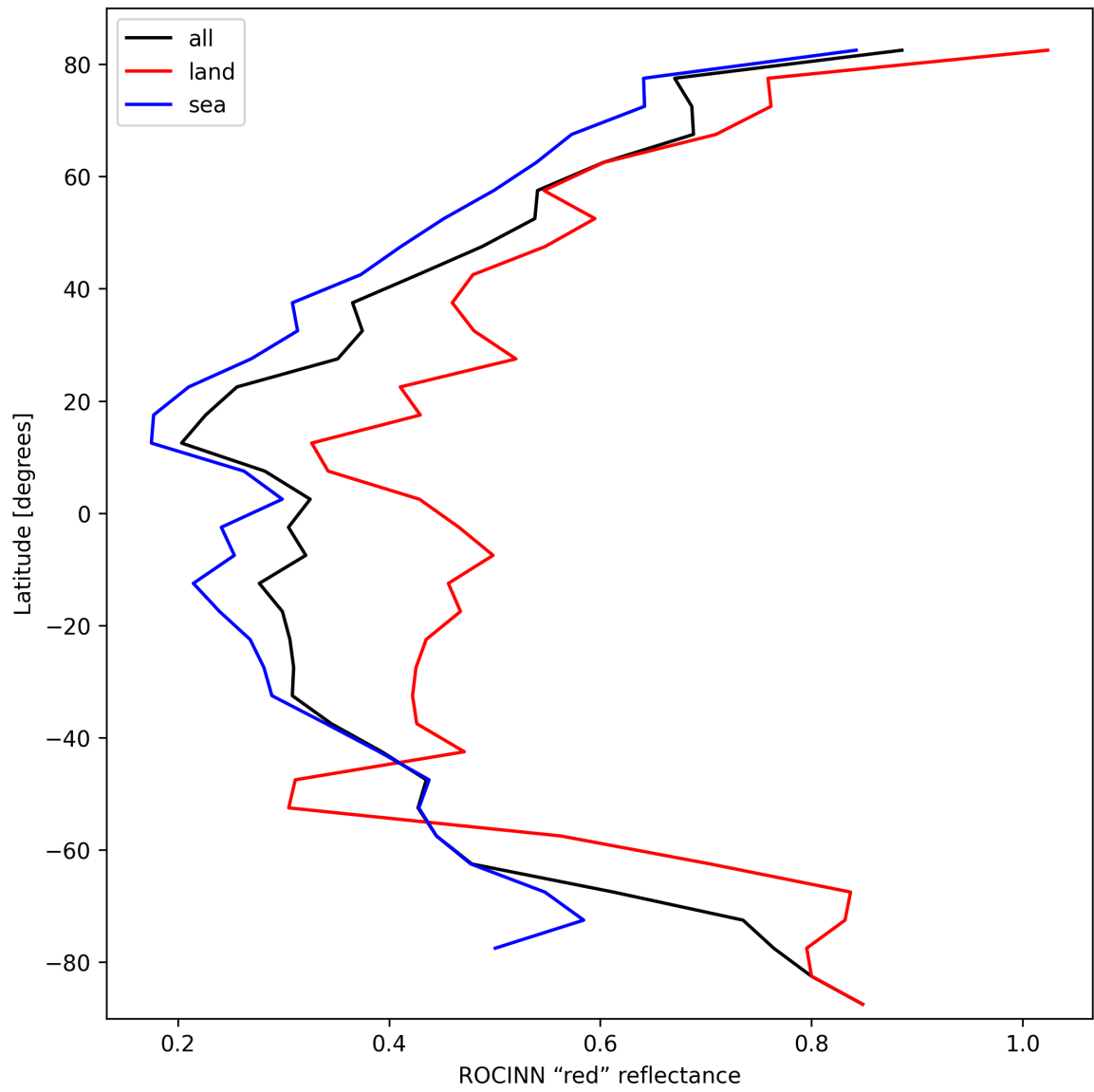
Figure 35: Zonal average of “ROCINN “red” reflectance” for 2025-02-27 to 2025-02-27.
