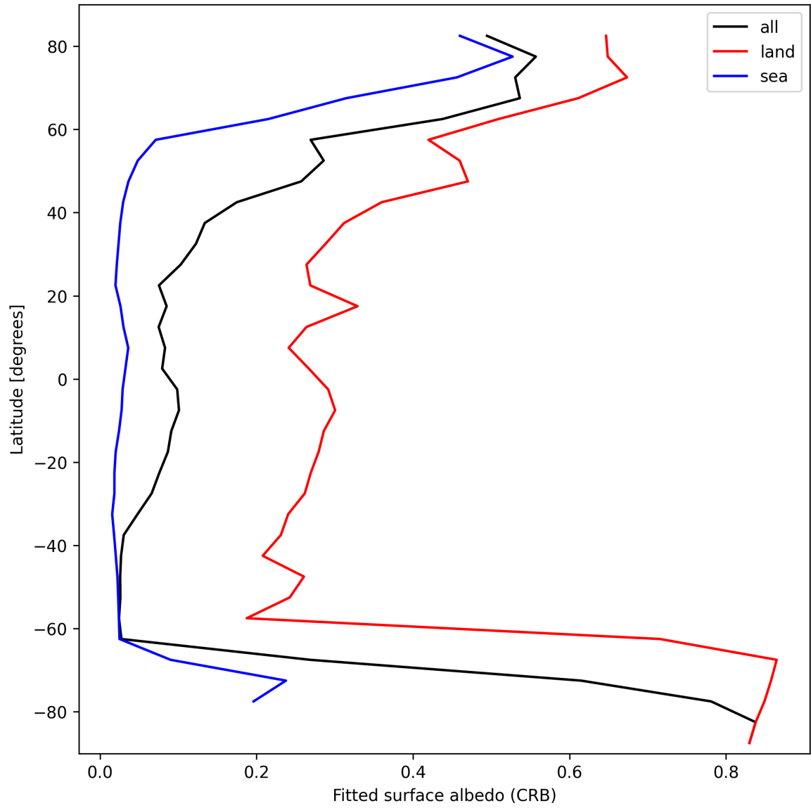
Figure 28: Zonal average of “Fitted surface albedo (CRB)” for 2025-02-27 to 2025-02-27.
