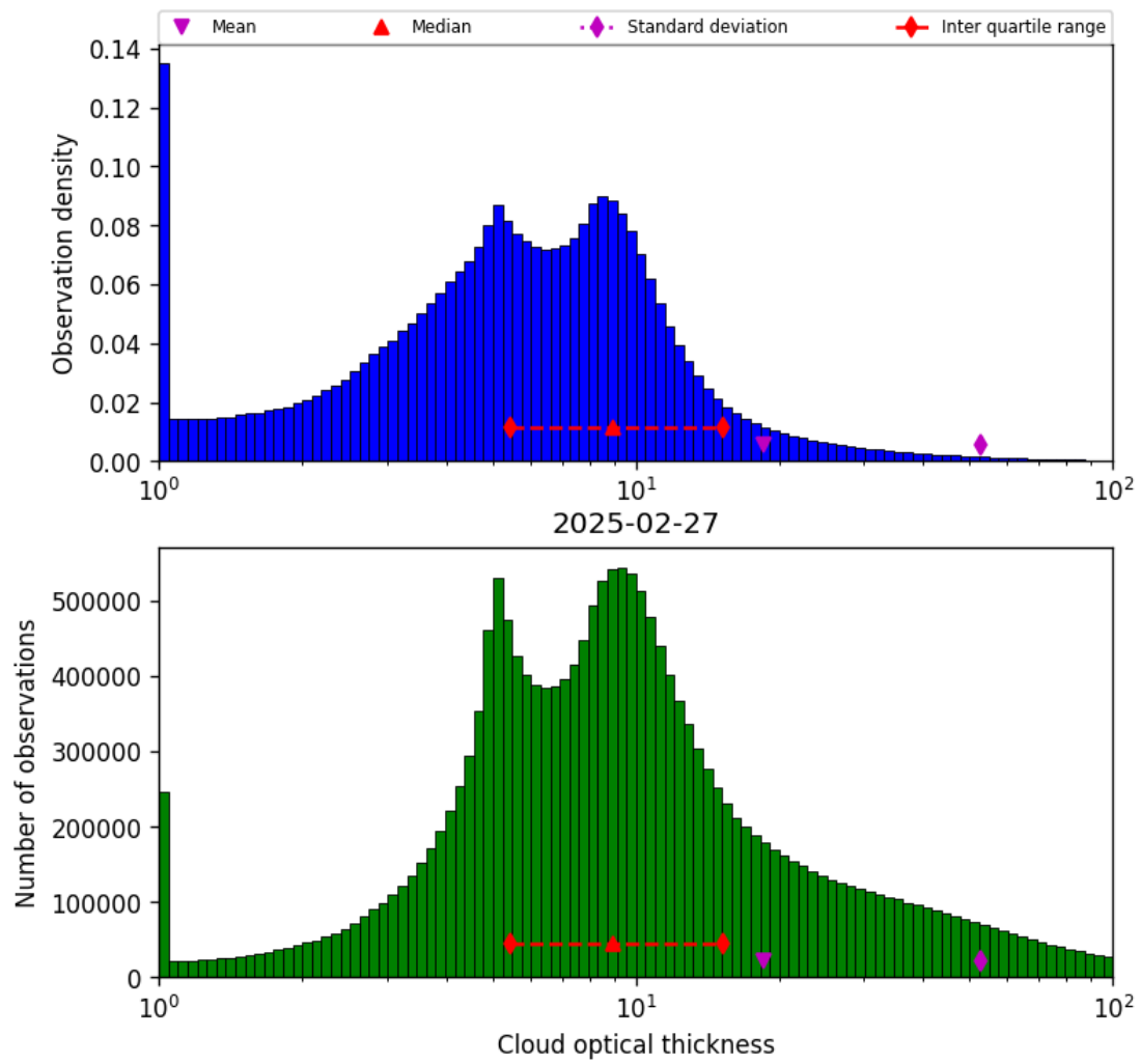
Figure 39: Histogram of “Cloud optical thickness” for 2025-02-27 to 2025-02-27
