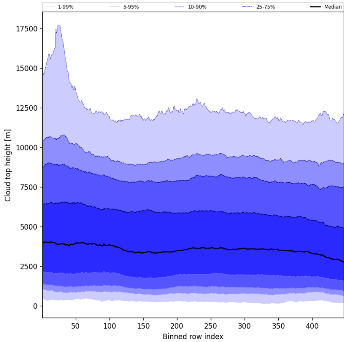
Figure 54: Along track statistics of “Cloud top height” for 2025-02-27 to 2025-02-27
