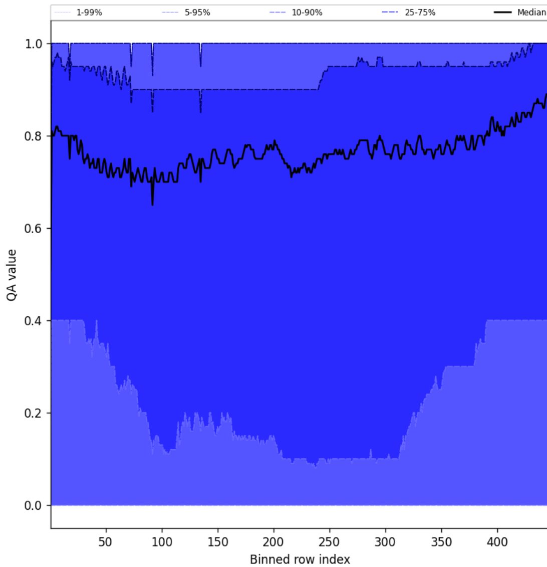
Figure 52: Along track statistics of “QA value” for 2025-02-27 to 2025-02-27
