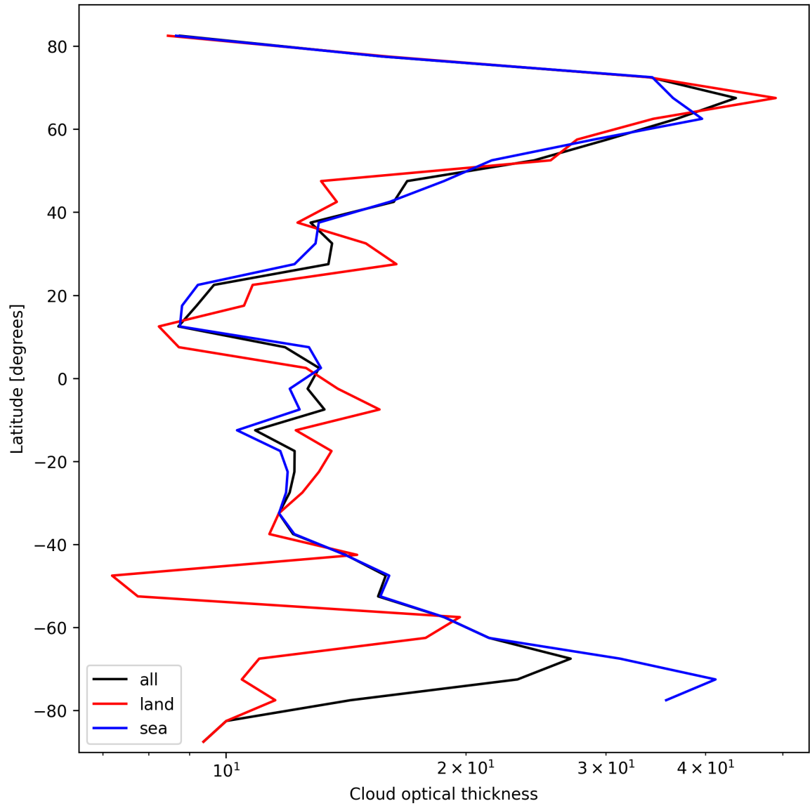
Figure 23: Zonal average of “Cloud optical thickness” for 2025-02-27 to 2025-02-27.
