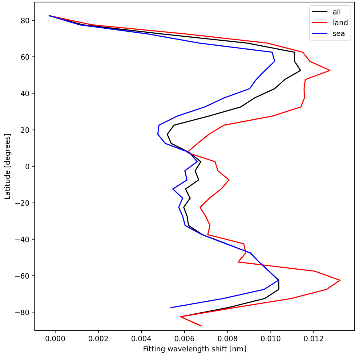
Figure 31: Zonal average of “Fitting wavelength shift” for 2025-02-27 to 2025-02-27.
