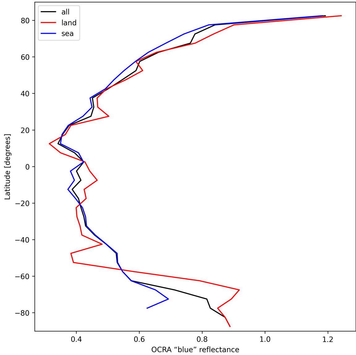
Figure 33: Zonal average of “OCRA “blue” reflectance” for 2025-02-27 to 2025-02-27.
