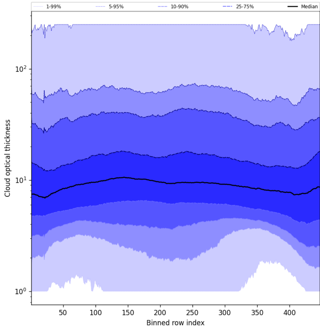
Figure 55: Along track statistics of “Cloud optical thickness” for 2025-02-27 to 2025-02-27
