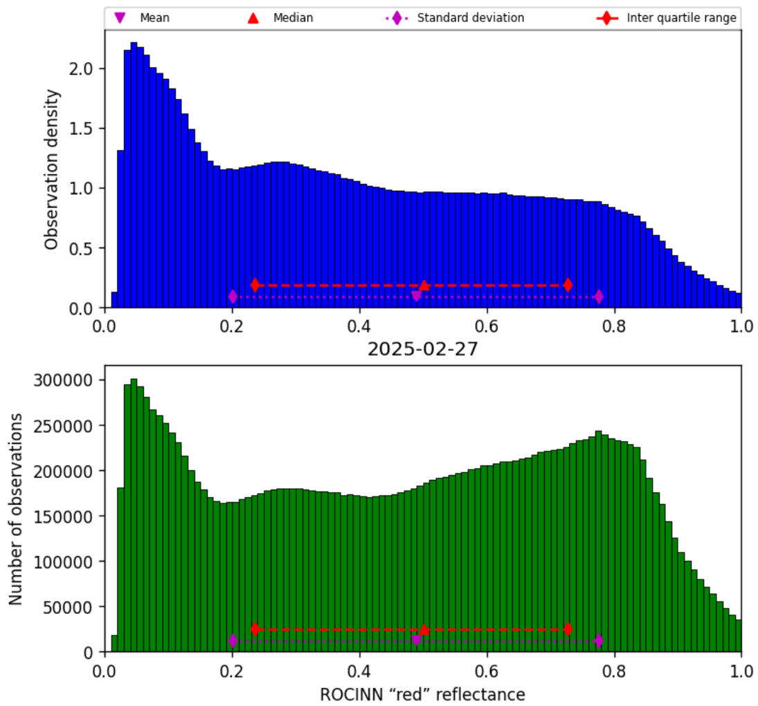
Figure 51: Histogram of “ROCINN “red” reflectance” for 2025-02-27 to 2025-02-27
