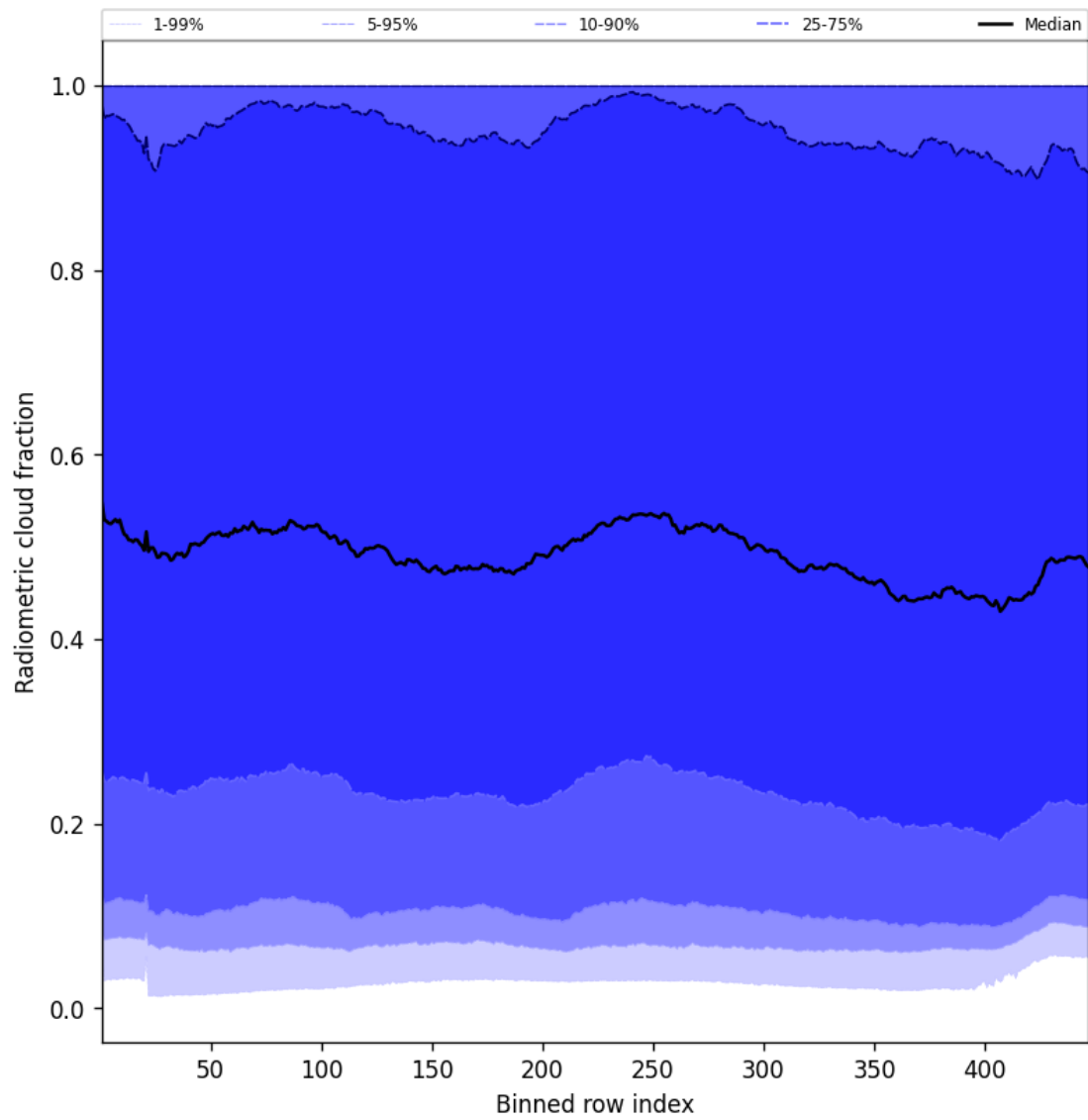
Figure 53: Along track statistics of “Radiometric cloud fraction” for 2025-02-27 to 2025-02-27
