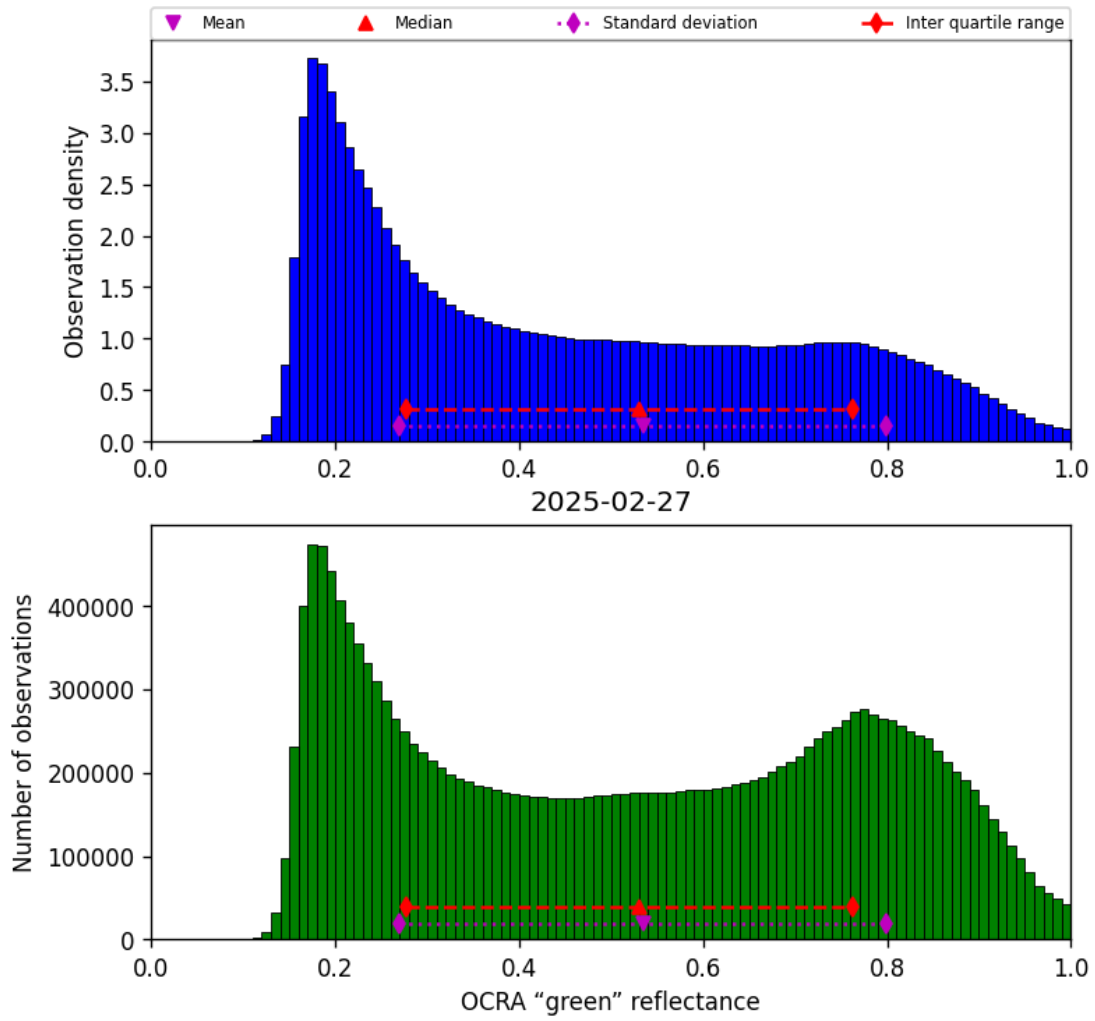
Figure 50: Histogram of “OCRA “green” reflectance” for 2025-02-27 to 2025-02-27
