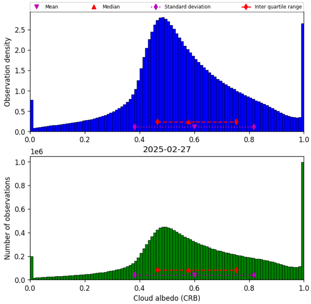
Figure 42: Histogram of “Cloud albedo (CRB)” for 2025-02-27 to 2025-02-27
