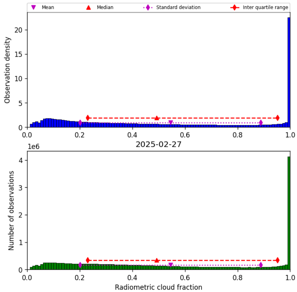
Figure 37: Histogram of “Radiometric cloud fraction” for 2025-02-27 to 2025-02-27
