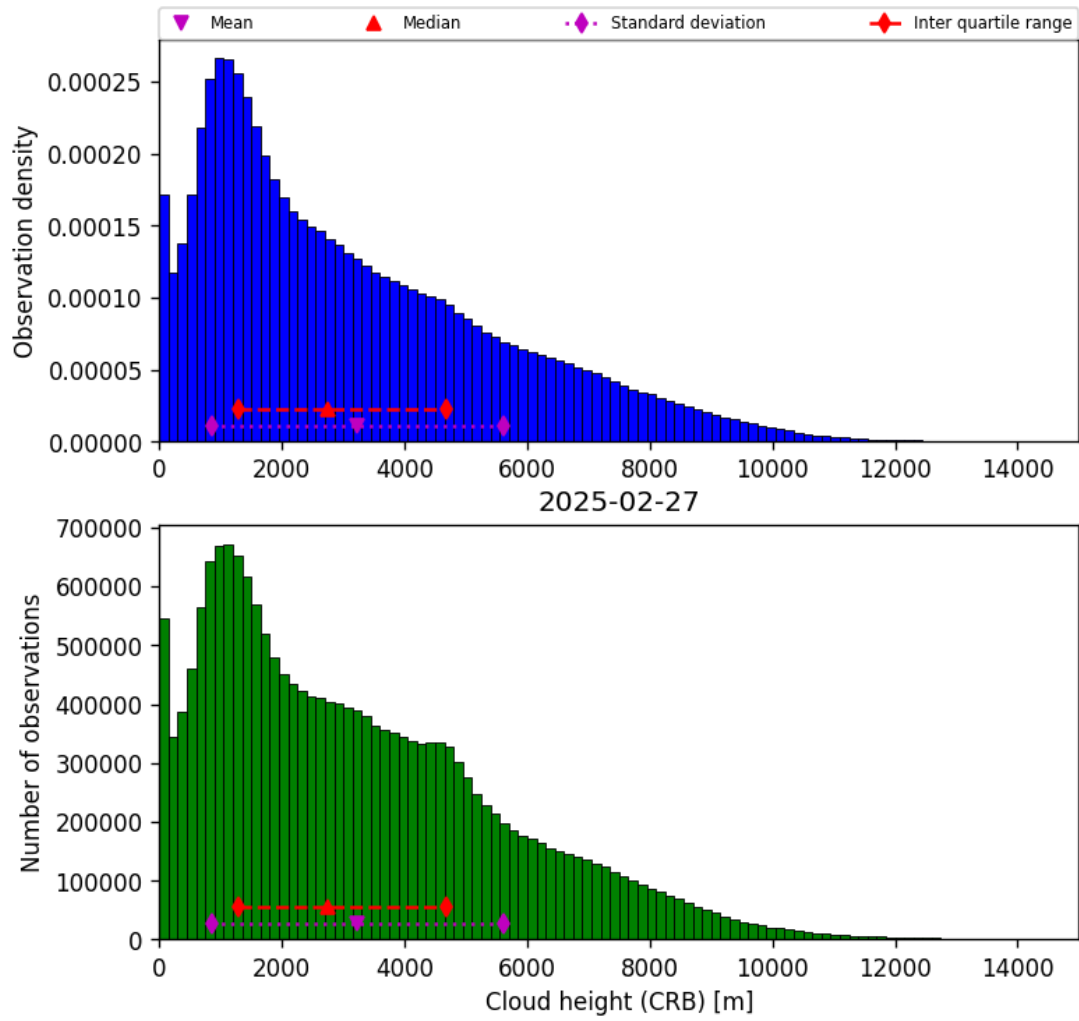
Figure 41: Histogram of “Cloud height (CRB)” for 2025-02-27 to 2025-02-27
