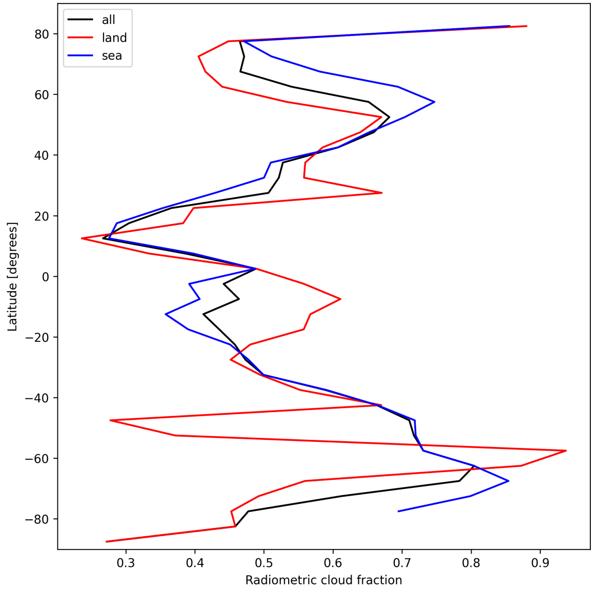
Figure 21: Zonal average of “Radiometric cloud fraction” for 2025-02-27 to 2025-02-27.
