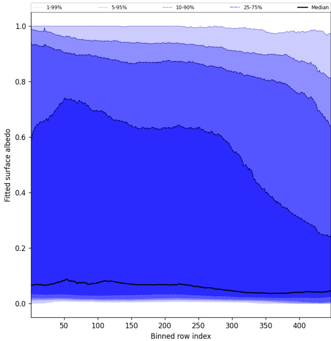
Figure 59: Along track statistics of “Fitted surface albedo” for 2025-02-27 to 2025-02-27
