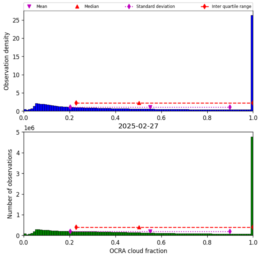
Figure 48: Histogram of “OCRA cloud fraction” for 2025-02-27 to 2025-02-27
