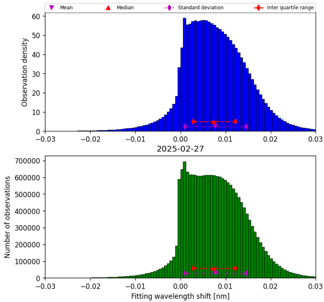
Figure 47: Histogram of “Fitting wavelength shift” for 2025-02-27 to 2025-02-27
