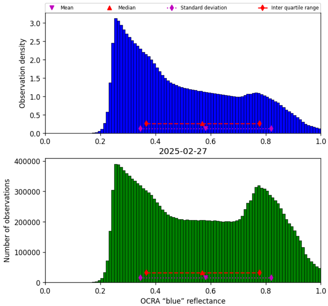
Figure 49: Histogram of “OCRA “blue” reflectance” for 2025-02-27 to 2025-02-27
