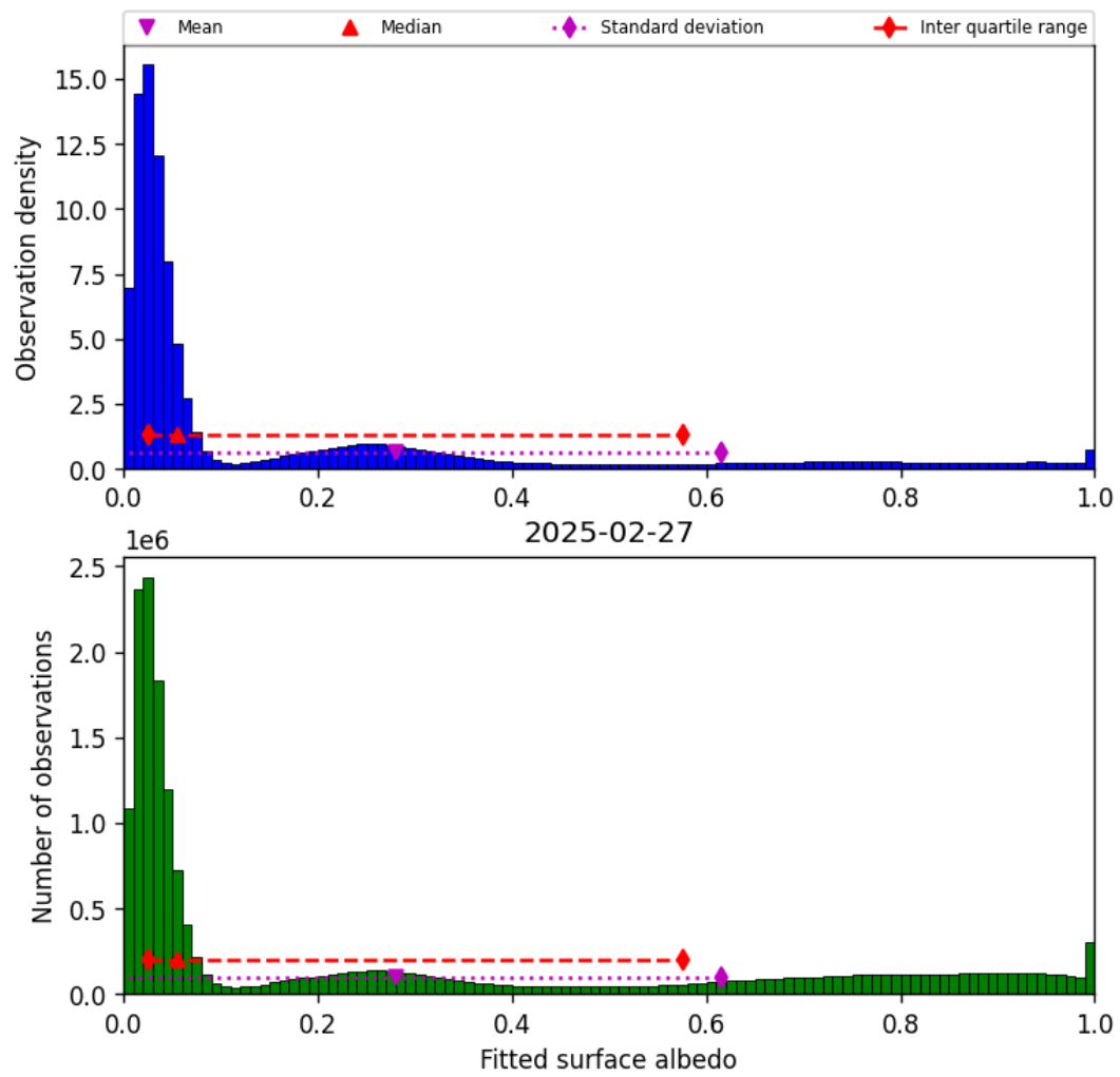
Figure 43: Histogram of “Fitted surface albedo” for 2025-02-27 to 2025-02-27
