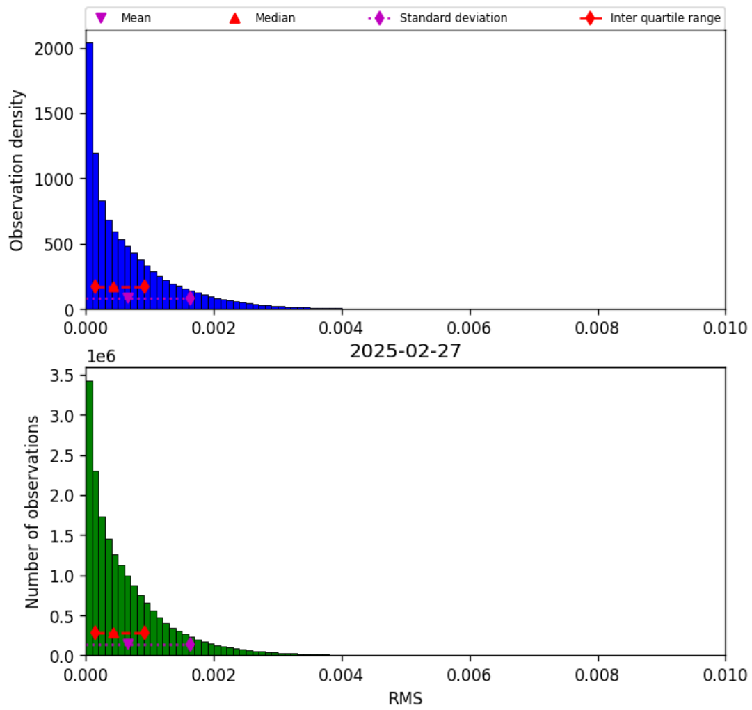
Figure 45: Histogram of “RMS” for 2025-02-27 to 2025-02-27
