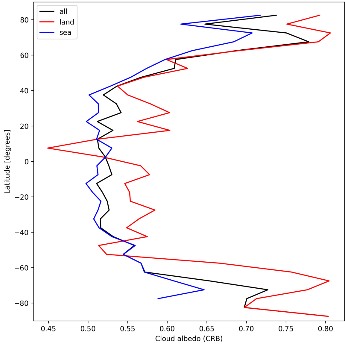
Figure 26: Zonal average of “Cloud albedo (CRB)” for 2025-02-27 to 2025-02-27.
