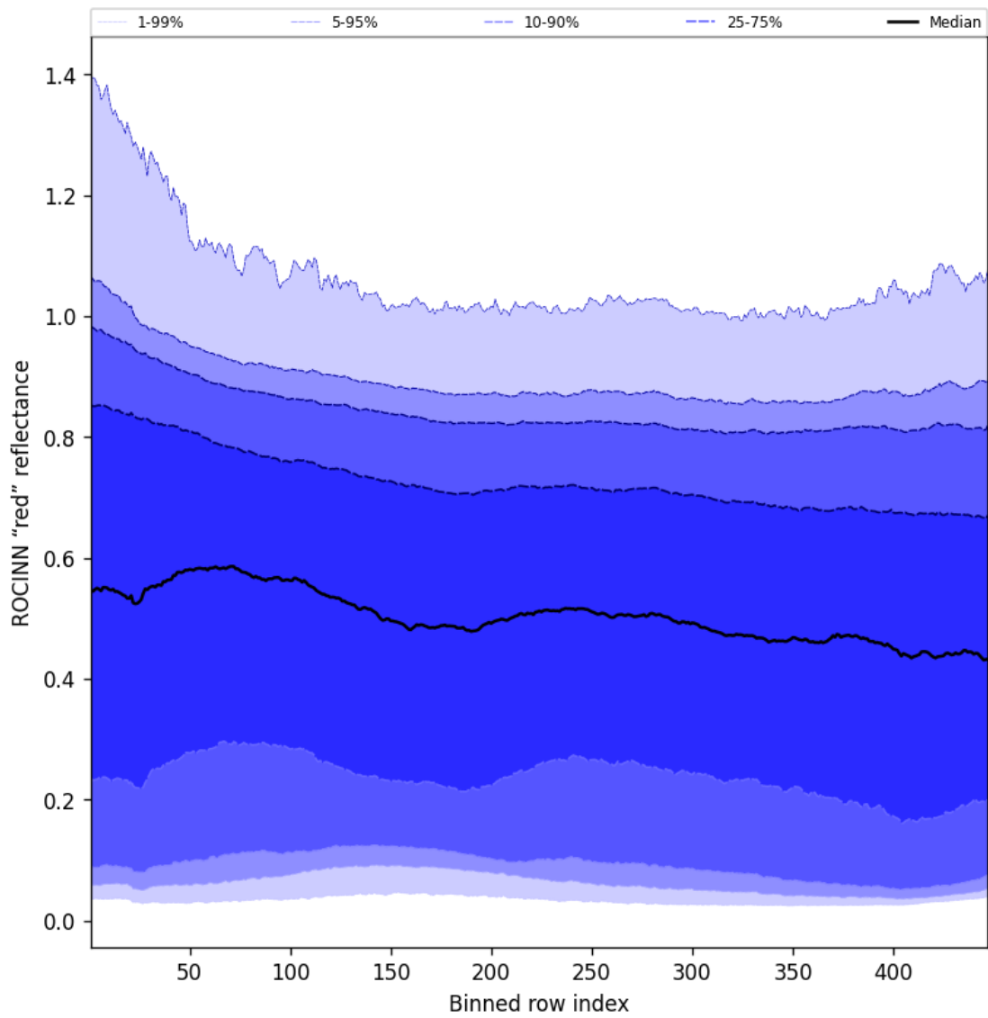
Figure 67: Along track statistics of "ROCINN "red" reflectance" for 2025-02-27 to 2025-02-27
