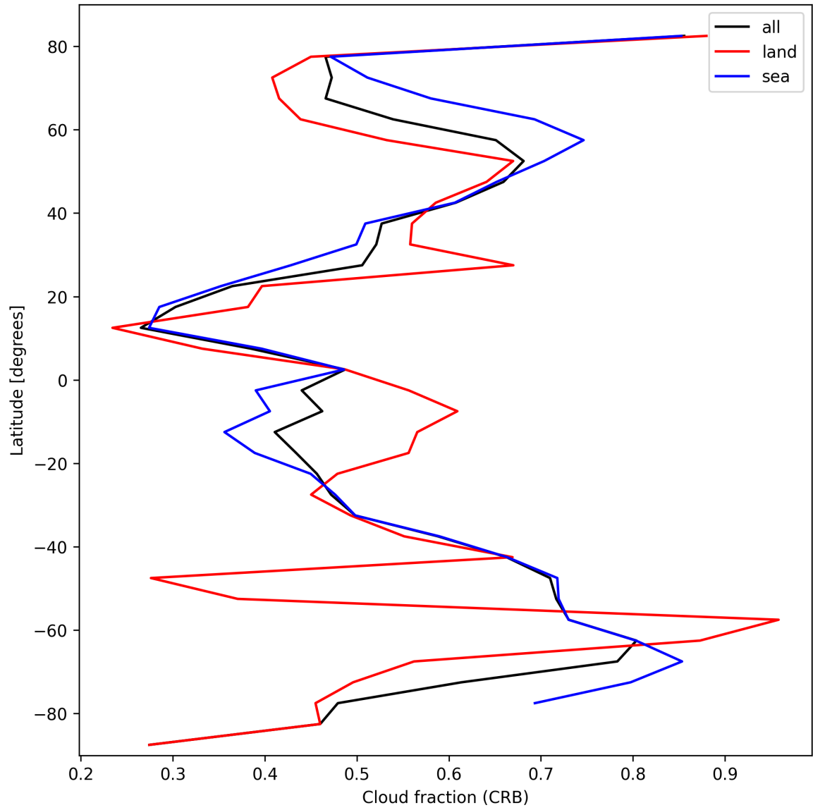
Figure 24: Zonal average of “Cloud fraction (CRB)” for 2025-02-27 to 2025-02-27.
