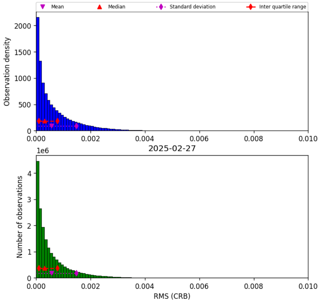
Figure 46: Histogram of “RMS (CRB)” for 2025-02-27 to 2025-02-27
