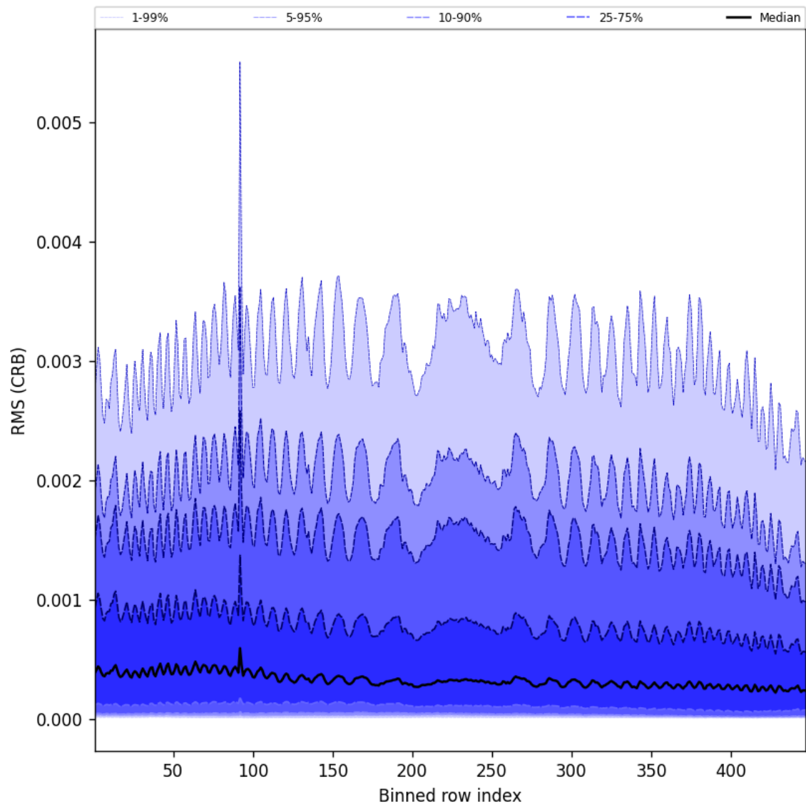
Figure 62: Along track statistics of “RMS (CRB)” for 2025-02-27 to 2025-02-27
