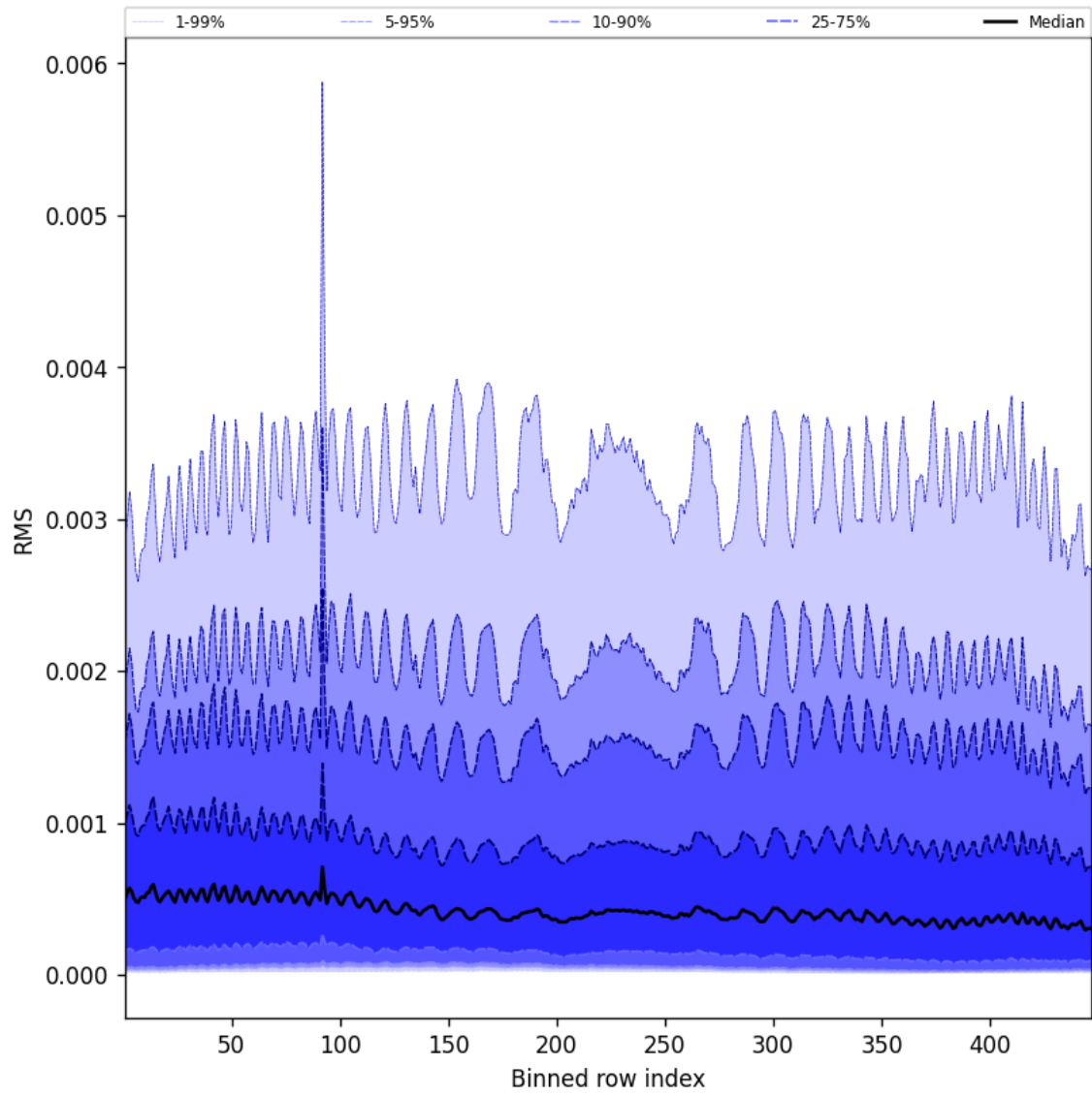
Figure 61: Along track statistics of “RMS” for 2025-03-09 to 2025-03-10
