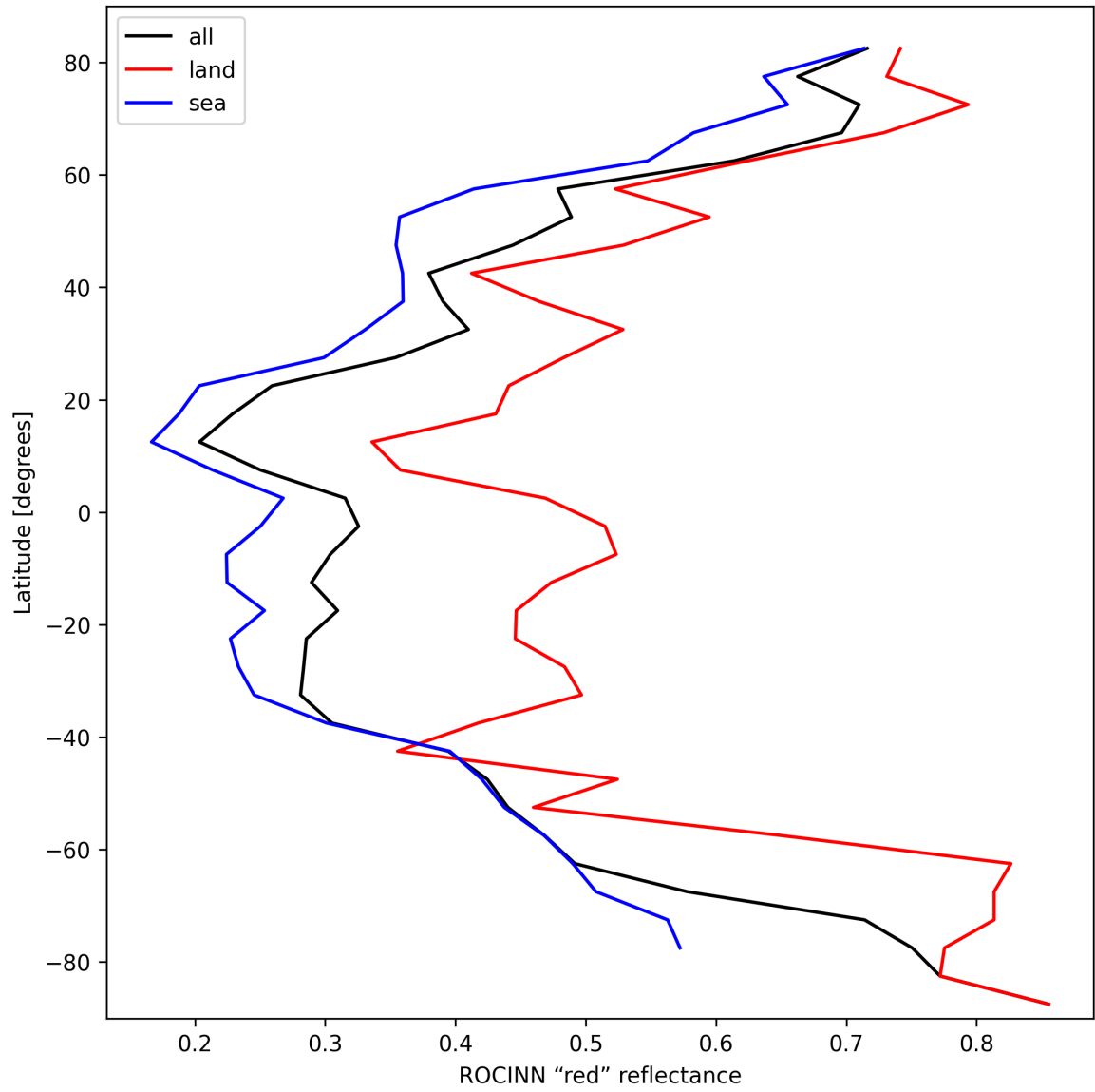
Figure 35: Zonal average of “ROCINN “red” reflectance” for 2025-03-09 to 2025-03-10.
