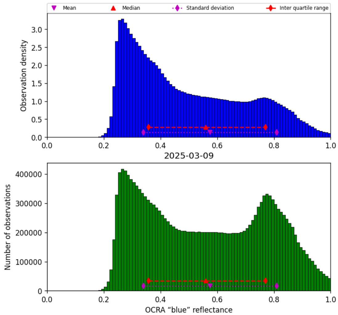
Figure 49: Histogram of “OCRA “blue” reflectance” for 2025-03-09 to 2025-03-10
