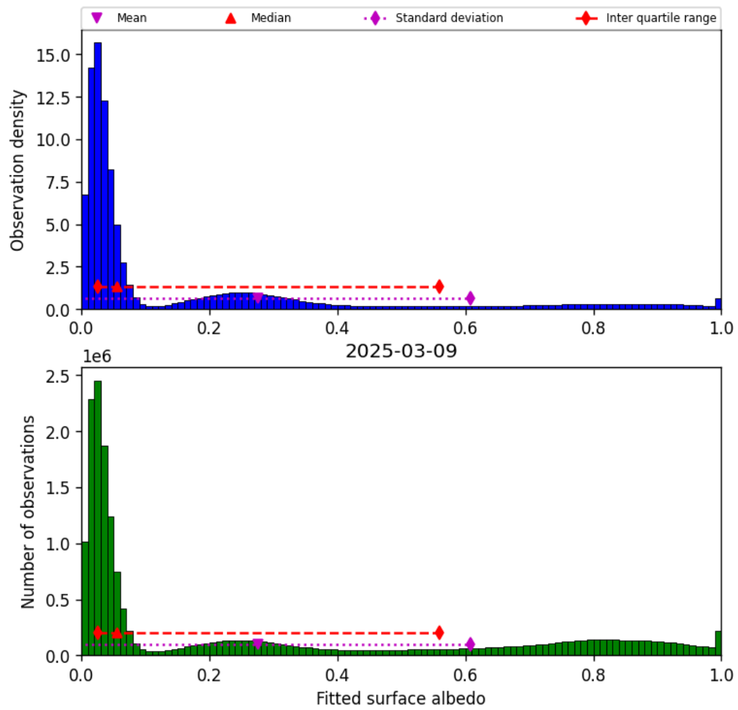
Figure 43: Histogram of “Fitted surface albedo” for 2025-03-09 to 2025-03-10
