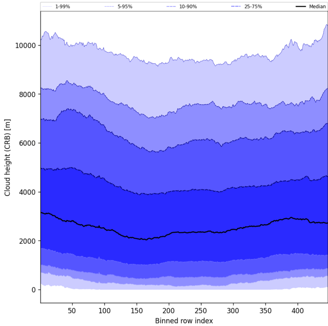
Figure 57: Along track statistics of “Cloud height (CRB)” for 2025-03-09 to 2025-03-10
