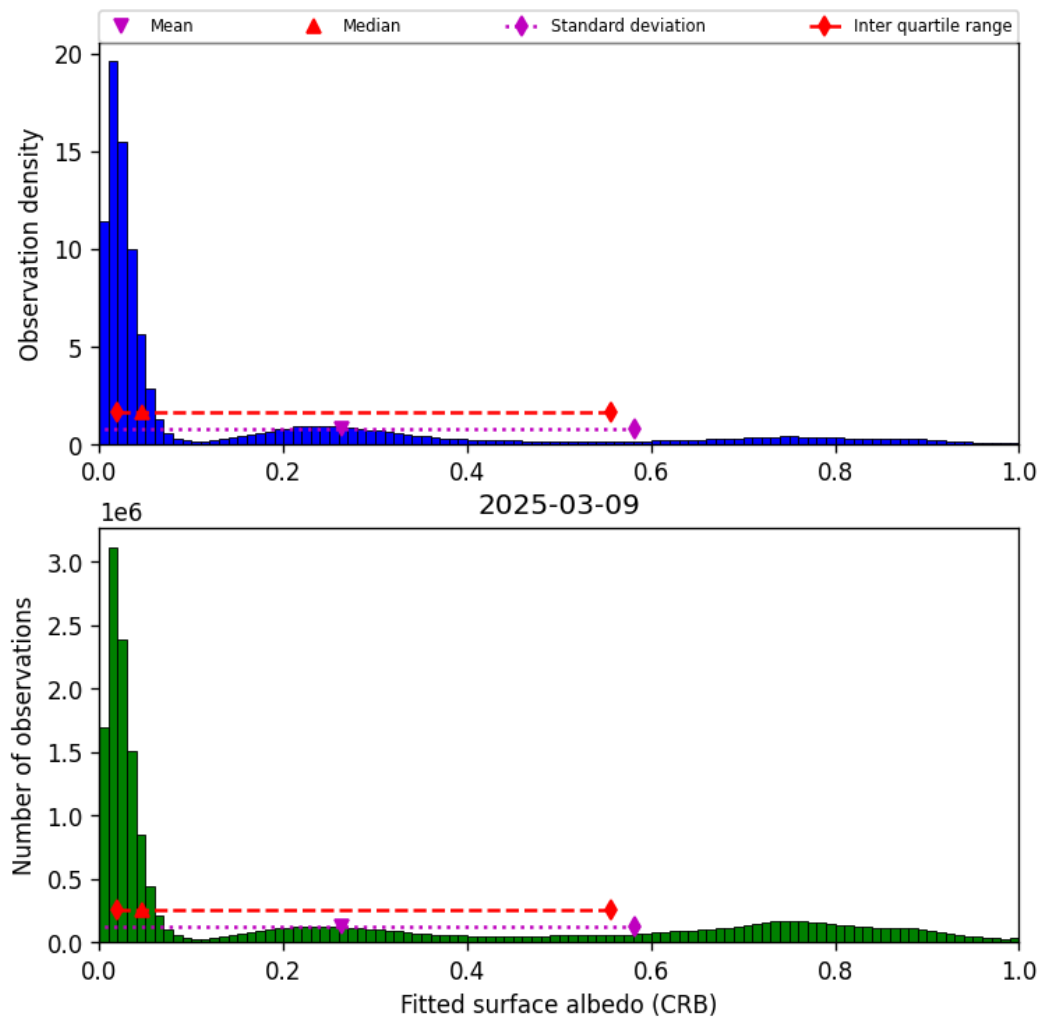
Figure 44: Histogram of “Fitted surface albedo (CRB)” for 2025-03-09 to 2025-03-10
