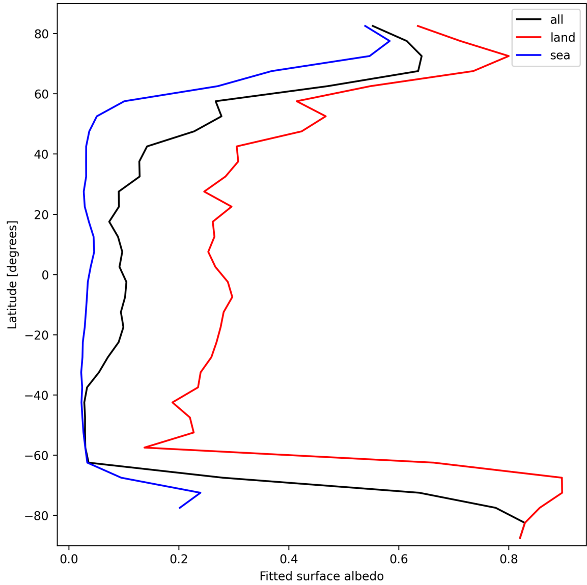
Figure 27: Zonal average of “Fitted surface albedo” for 2025-03-09 to 2025-03-10.
