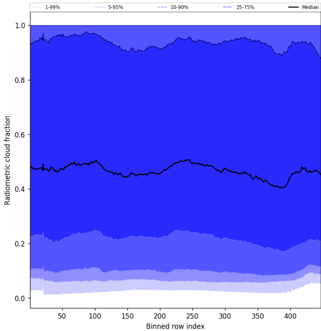
Figure 53: Along track statistics of “Radiometric cloud fraction” for 2025-03-09 to 2025-03-10
