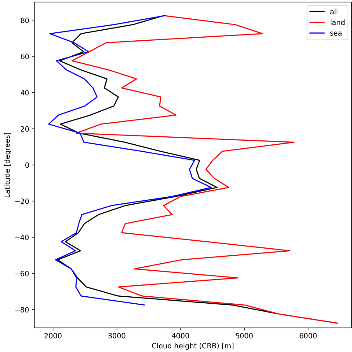
Figure 25: Zonal average of “Cloud height (CRB)” for 2025-03-09 to 2025-03-10.
