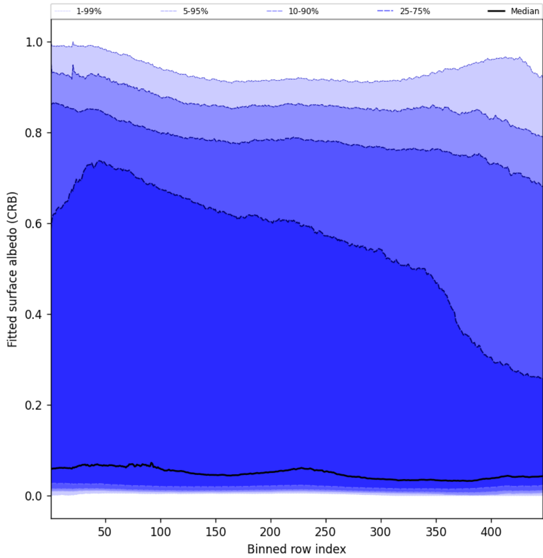
Figure 60: Along track statistics of “Fitted surface albedo (CRB)” for 2025-03-09 to 2025-03-10
