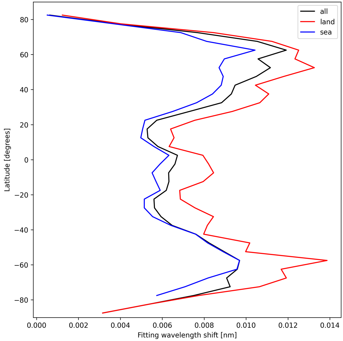
Figure 31: Zonal average of “Fitting wavelength shift” for 2025-03-09 to 2025-03-10.
