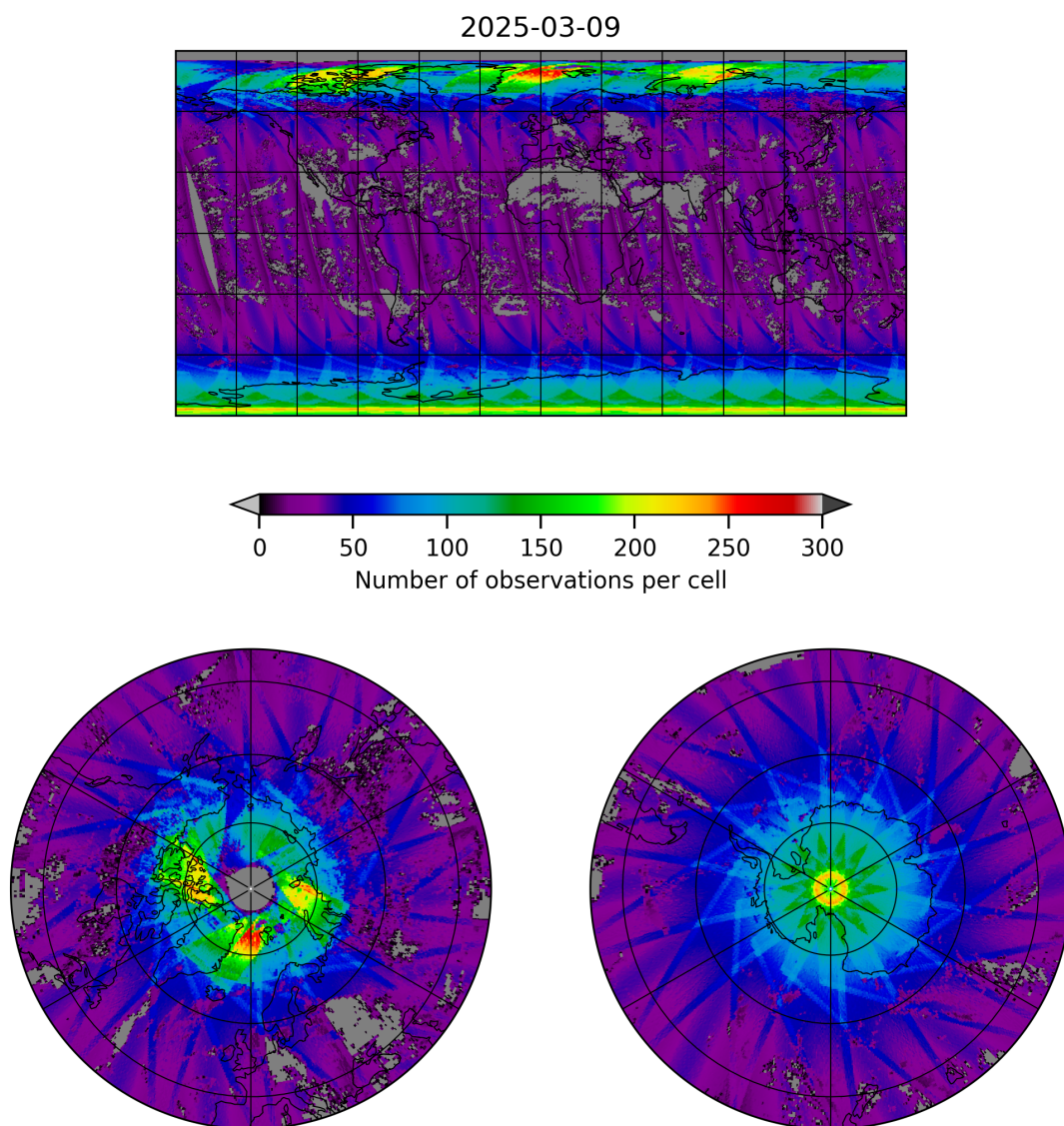
Figure 19: Map of the number of observations for 2025-03-09 to 2025-03-10
