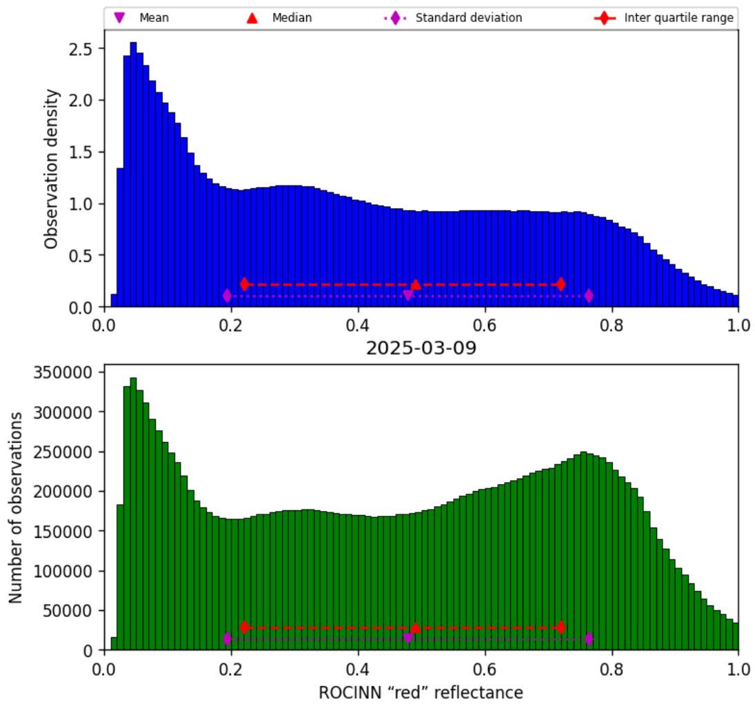
Figure 51: Histogram of “ROCINN “red” reflectance” for 2025-03-09 to 2025-03-10
