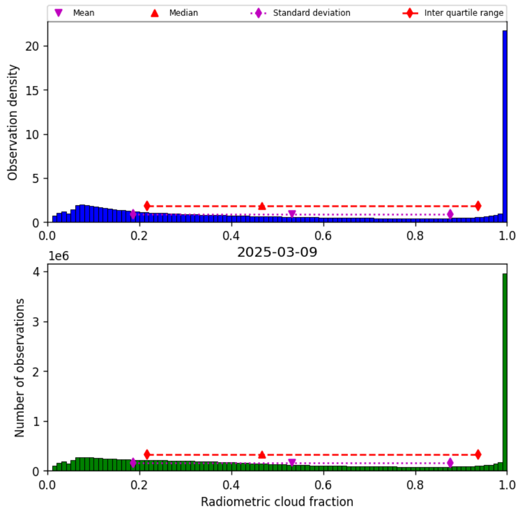
Figure 37: Histogram of "Radiometric cloud fraction" for 2025-03-09 to 2025-03-10
