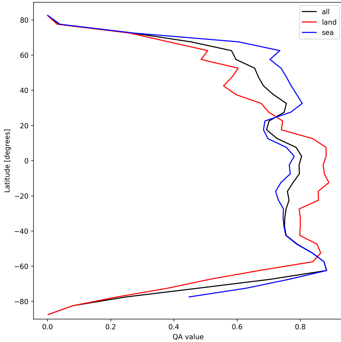
Figure 20: Zonal average of “QA value” for 2025-03-09 to 2025-03-10.
