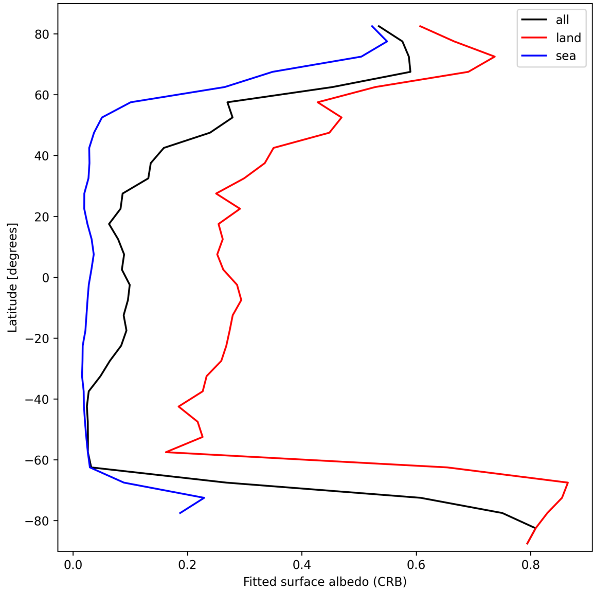
Figure 28: Zonal average of “Fitted surface albedo (CRB)” for 2025-03-09 to 2025-03-10.
