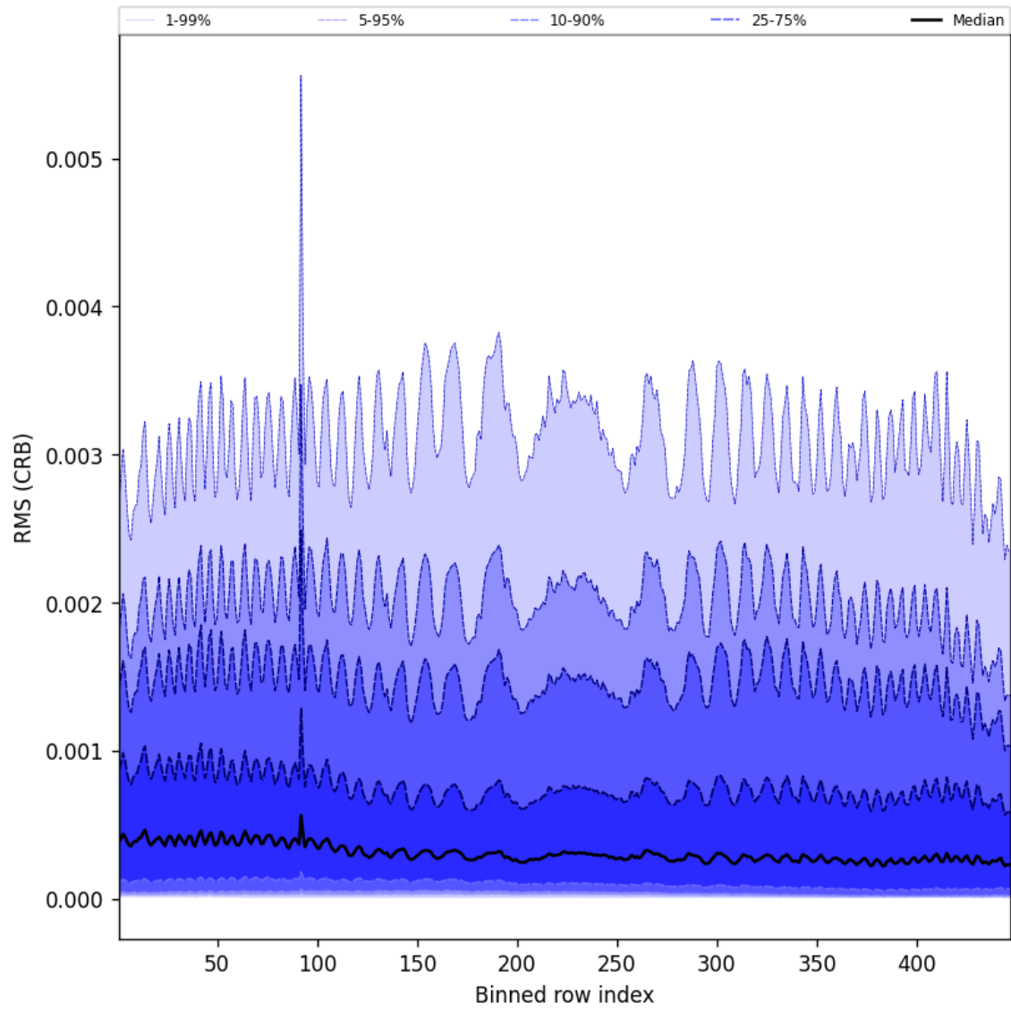
Figure 62: Along track statistics of “RMS (CRB)” for 2025-03-09 to 2025-03-10
