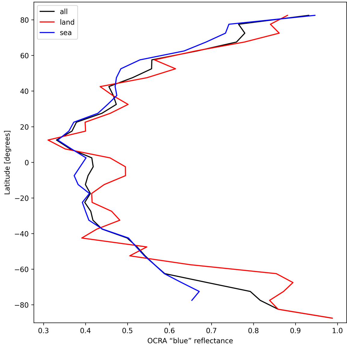
Figure 33: Zonal average of "OCRA "blue" reflectance" for 2025-03-09 to 2025-03-10.
