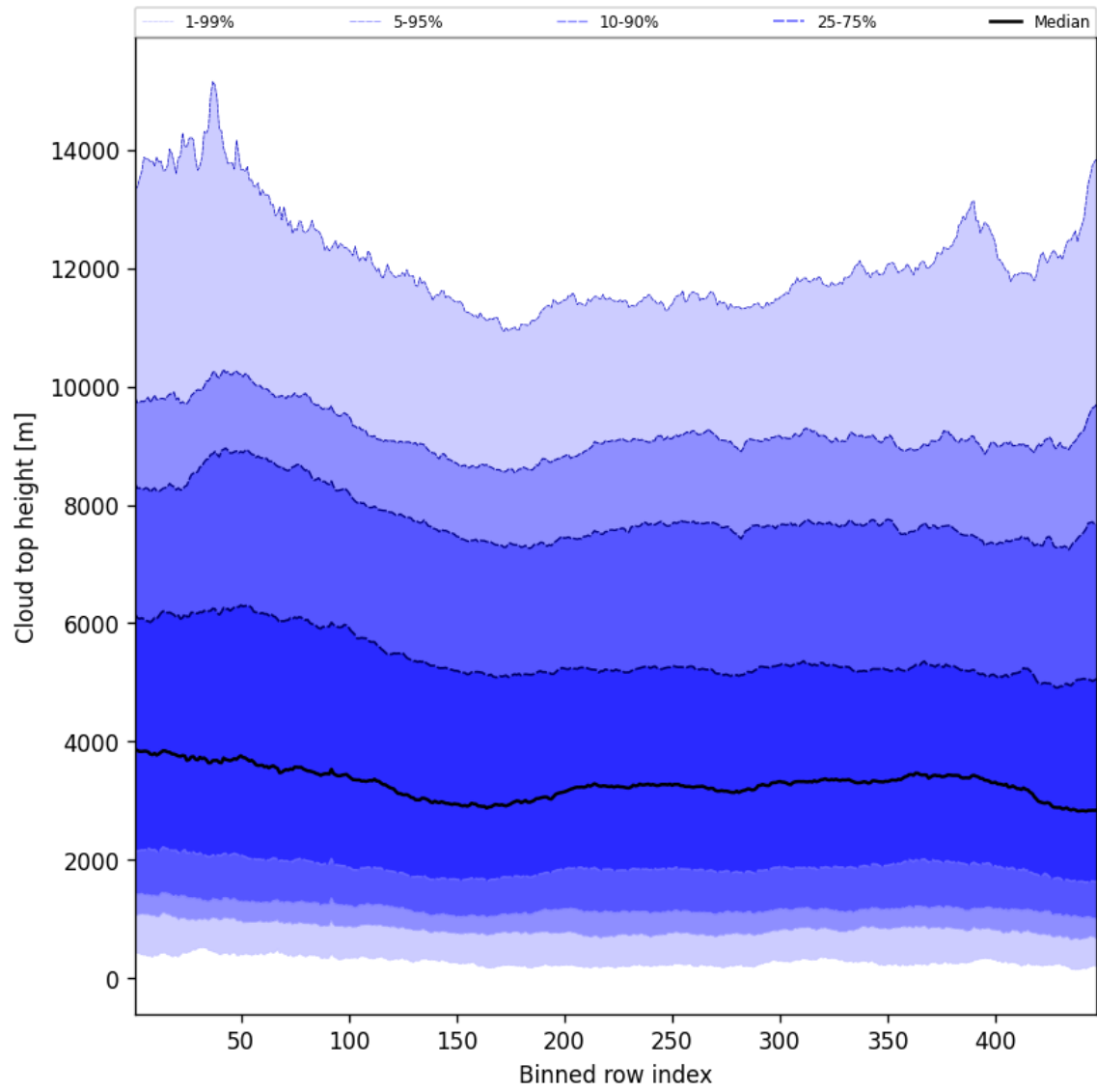
Figure 54: Along track statistics of “Cloud top height” for 2025-03-09 to 2025-03-10
