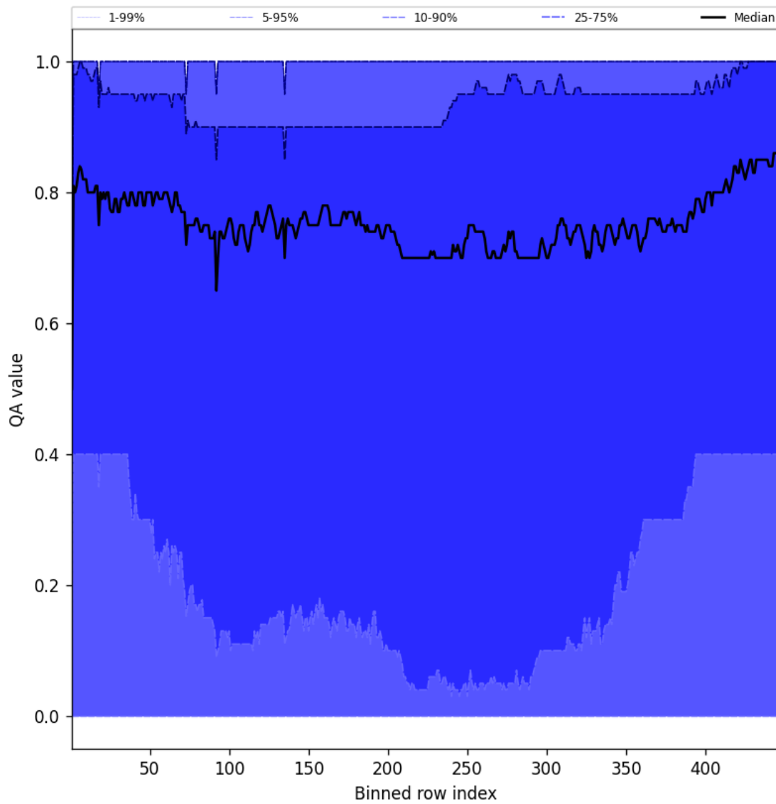
Figure 52: Along track statistics of “QA value” for 2025-03-09 to 2025-03-10
