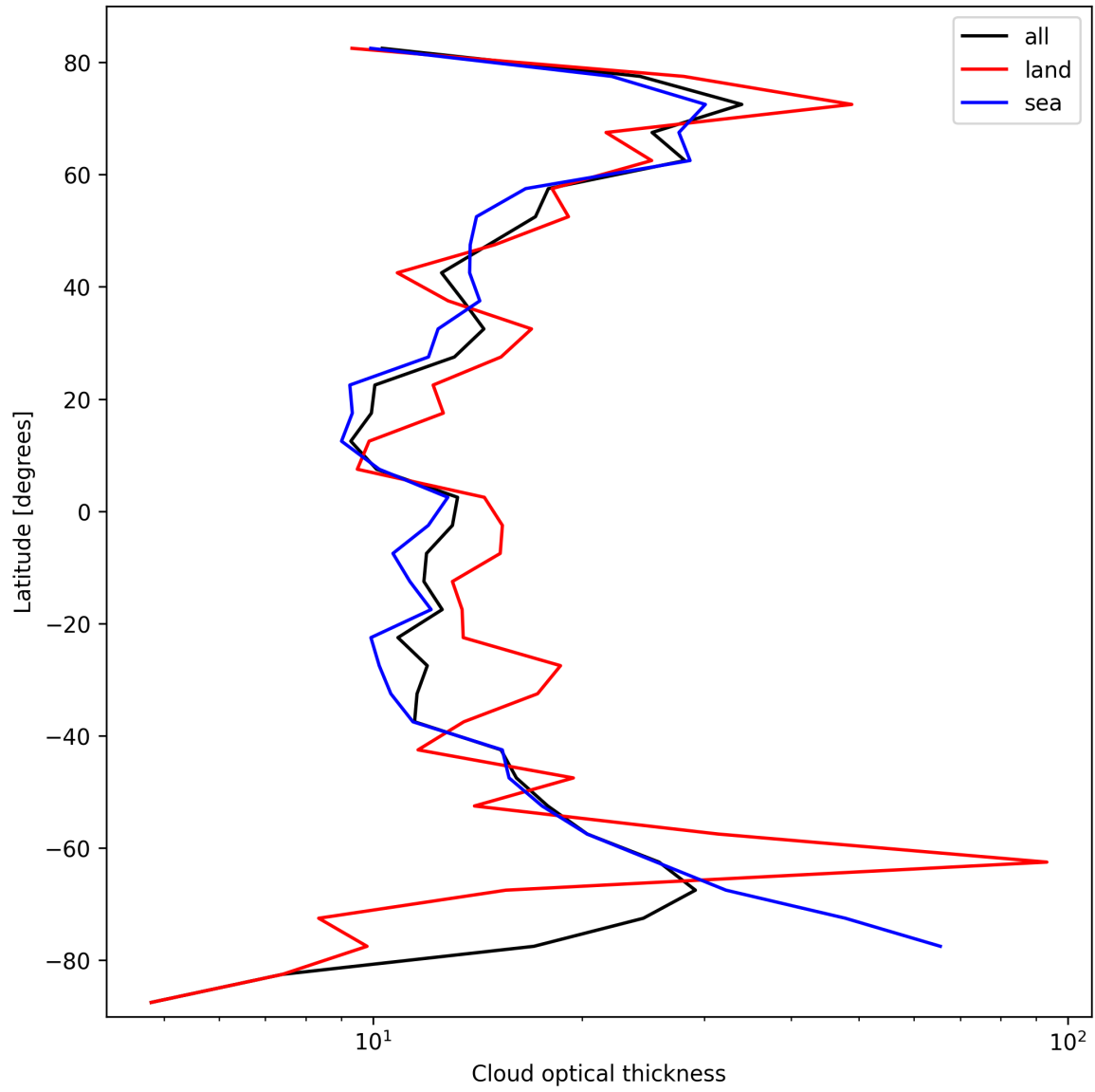
Figure 23: Zonal average of “Cloud optical thickness” for 2025-03-09 to 2025-03-10.
