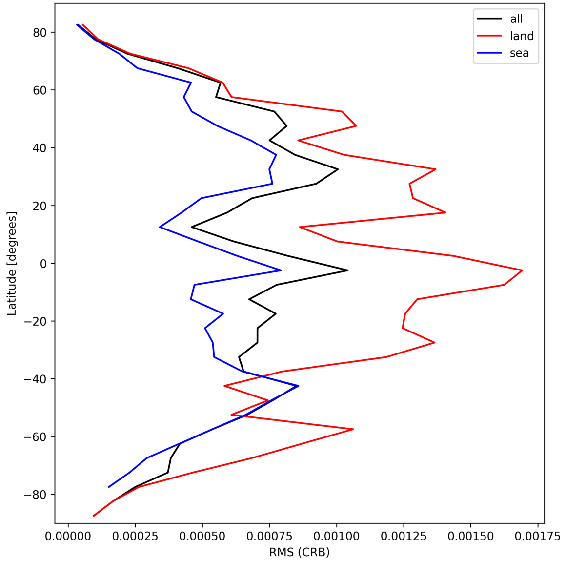
Figure 30: Zonal average of “RMS (CRB)” for 2025-03-09 to 2025-03-10.
