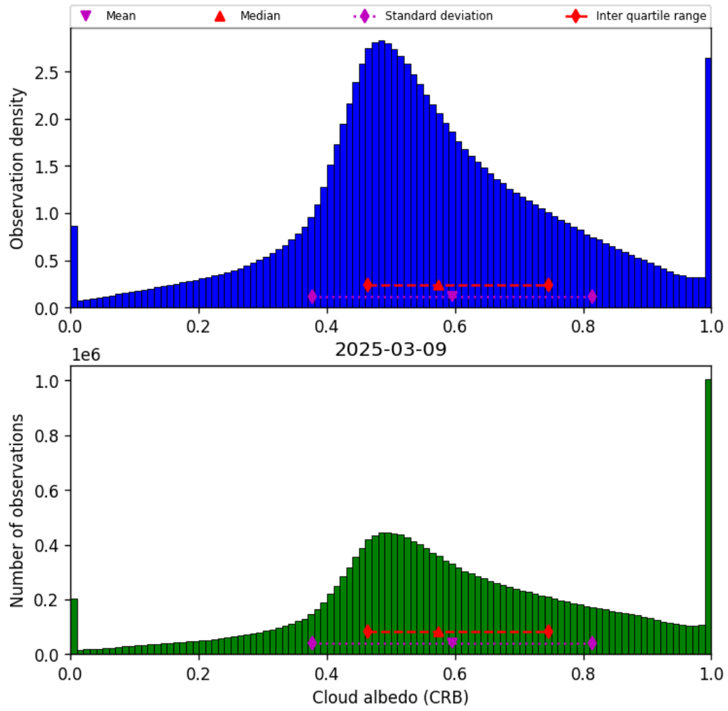
Figure 42: Histogram of “Cloud albedo (CRB)” for 2025-03-09 to 2025-03-10
