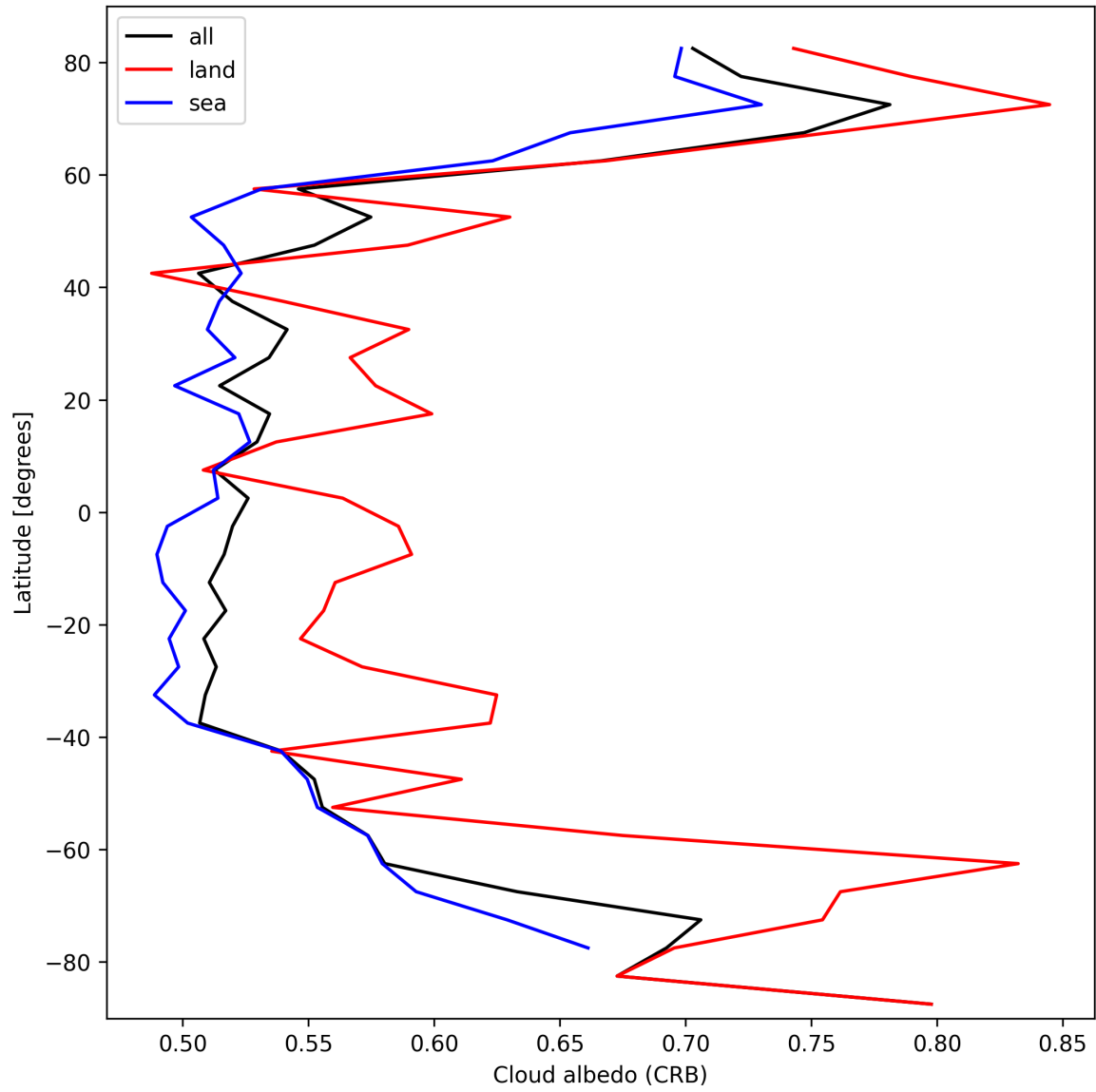
Figure 26: Zonal average of “Cloud albedo (CRB)” for 2025-03-09 to 2025-03-10.
