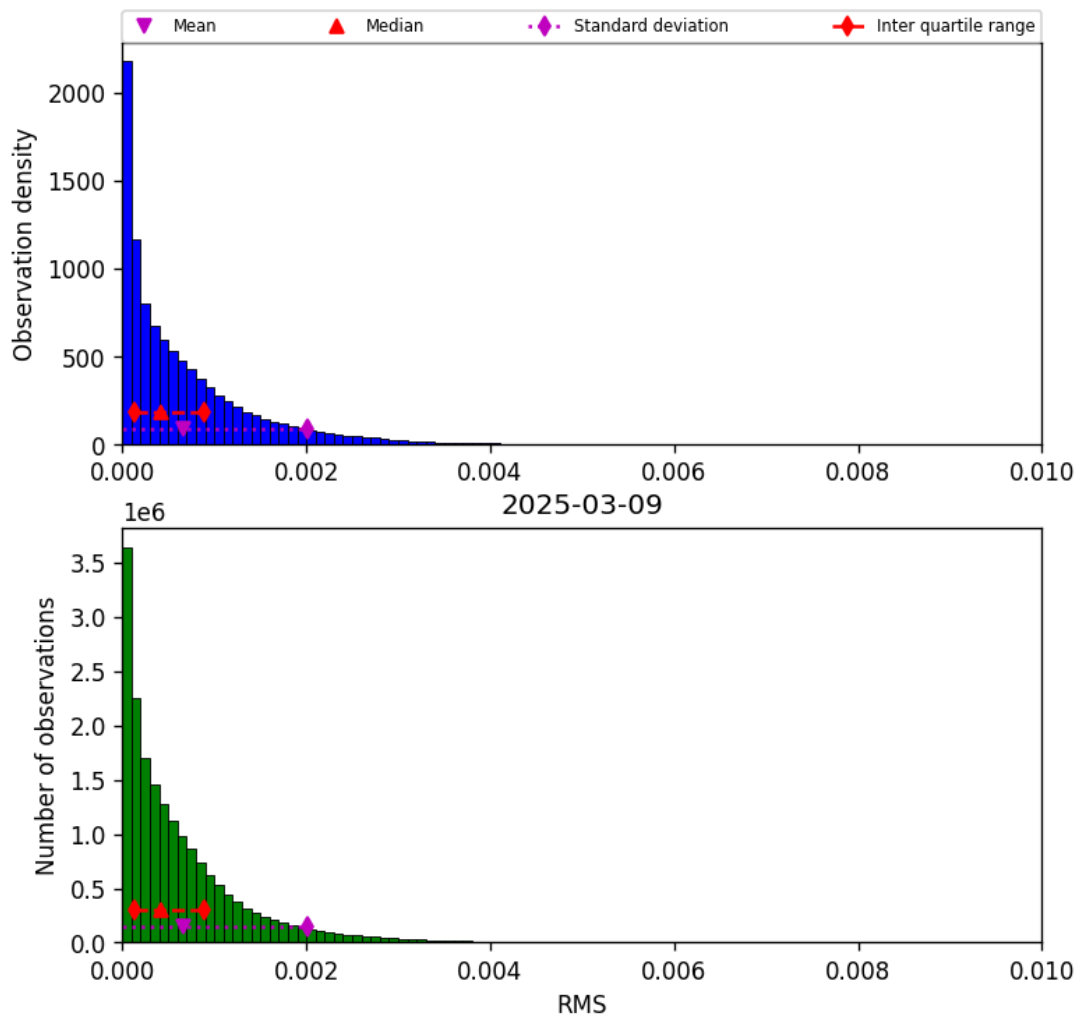
Figure 45: Histogram of “RMS” for 2025-03-09 to 2025-03-10
