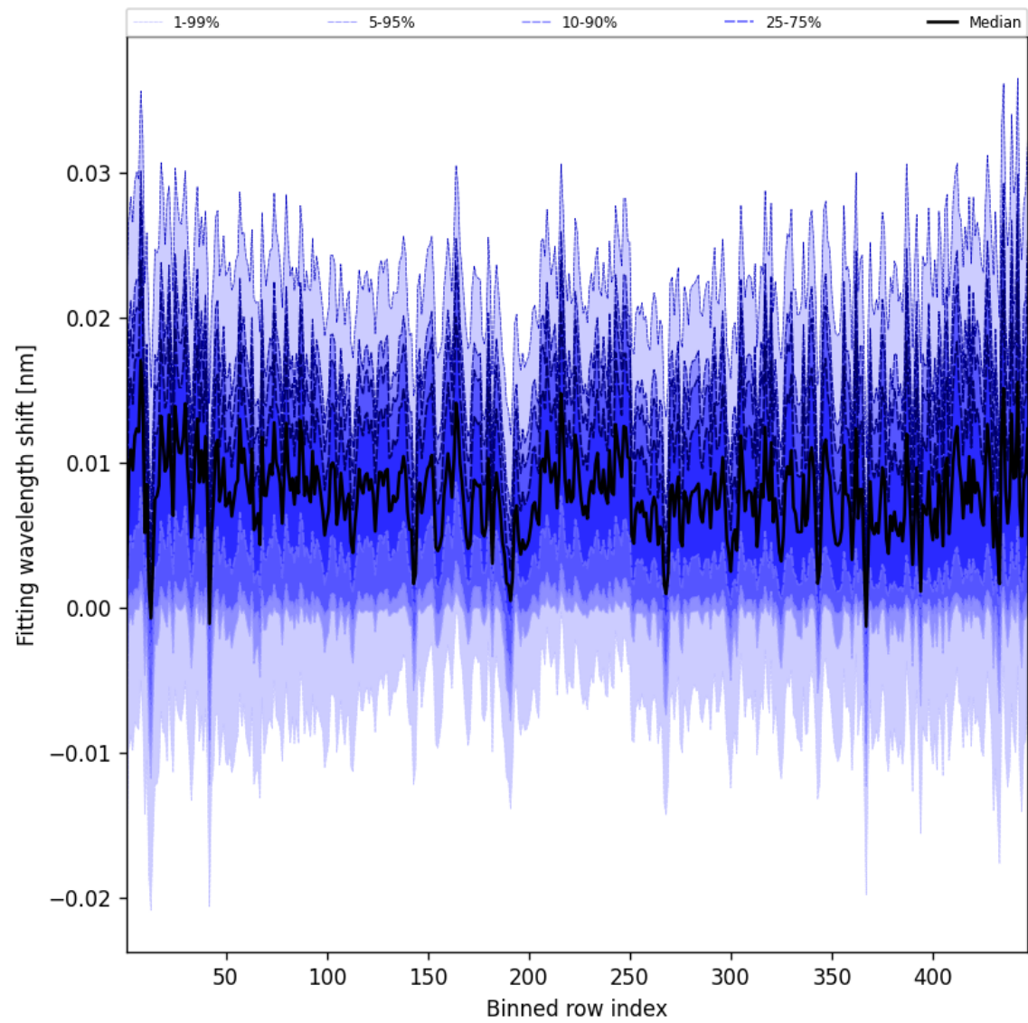
Figure 63: Along track statistics of “Fitting wavelength shift” for 2025-03-09 to 2025-03-10
