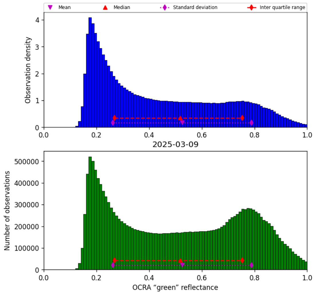
Figure 50: Histogram of “OCRA “green” reflectance” for 2025-03-09 to 2025-03-10
