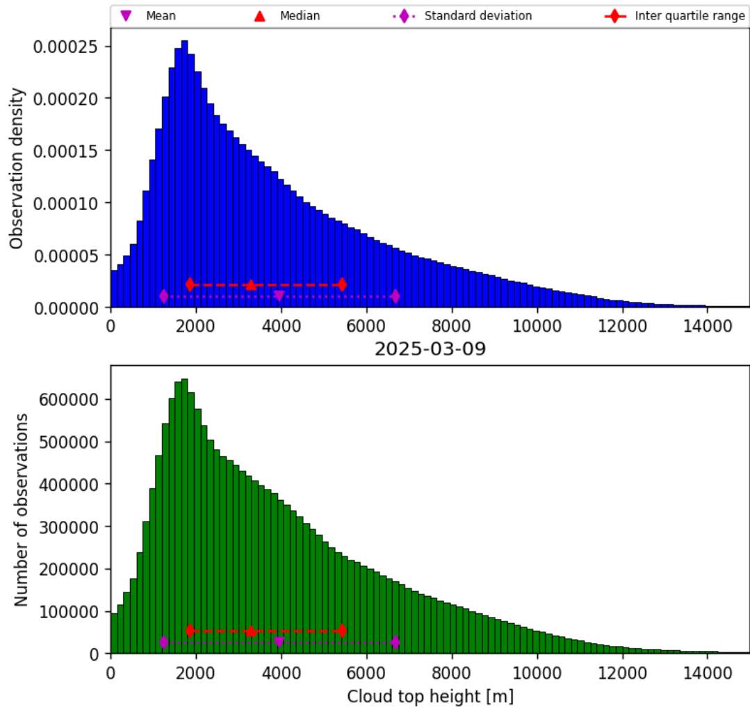
Figure 38: Histogram of “Cloud top height” for 2025-03-09 to 2025-03-10
