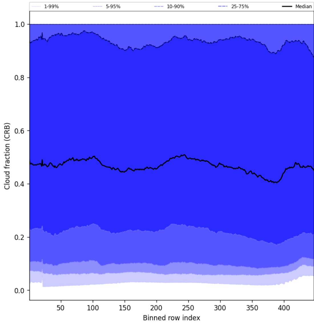
Figure 56: Along track statistics of “Cloud fraction (CRB)” for 2025-03-09 to 2025-03-10
