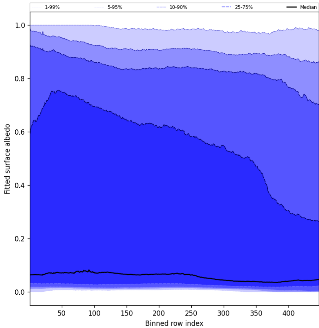
Figure 59: Along track statistics of “Fitted surface albedo” for 2025-03-09 to 2025-03-10
