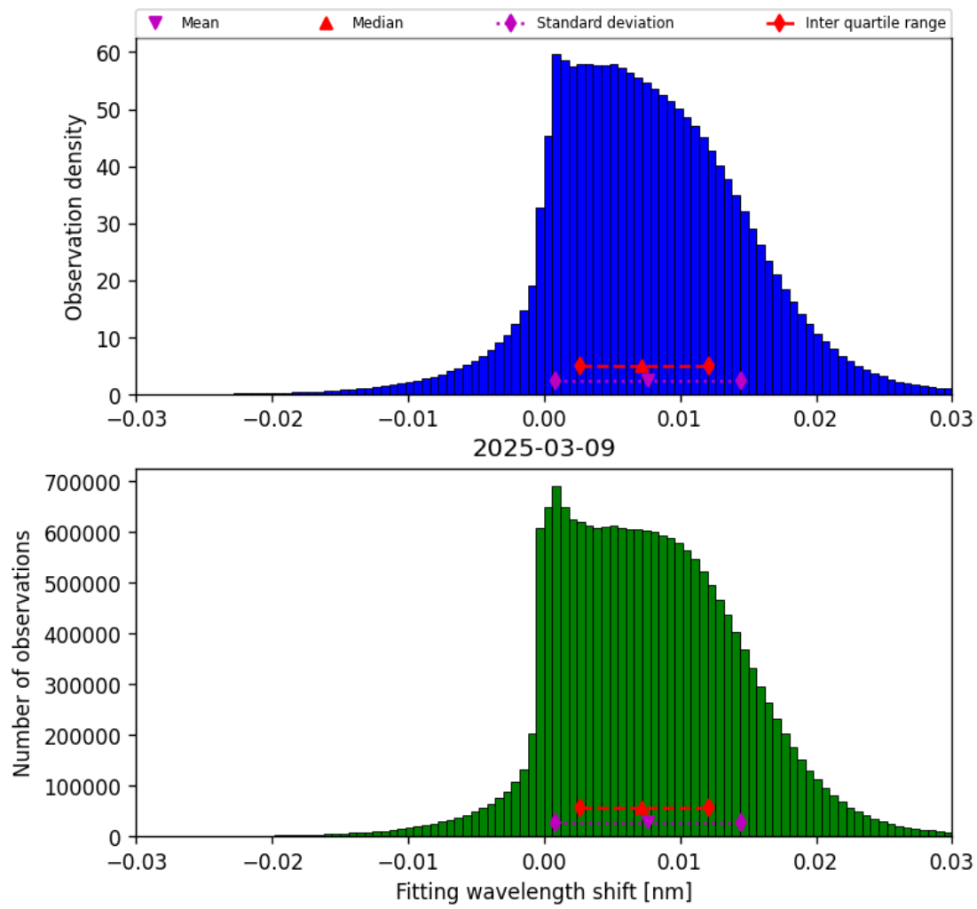
Figure 47: Histogram of “Fitting wavelength shift” for 2025-03-09 to 2025-03-10
