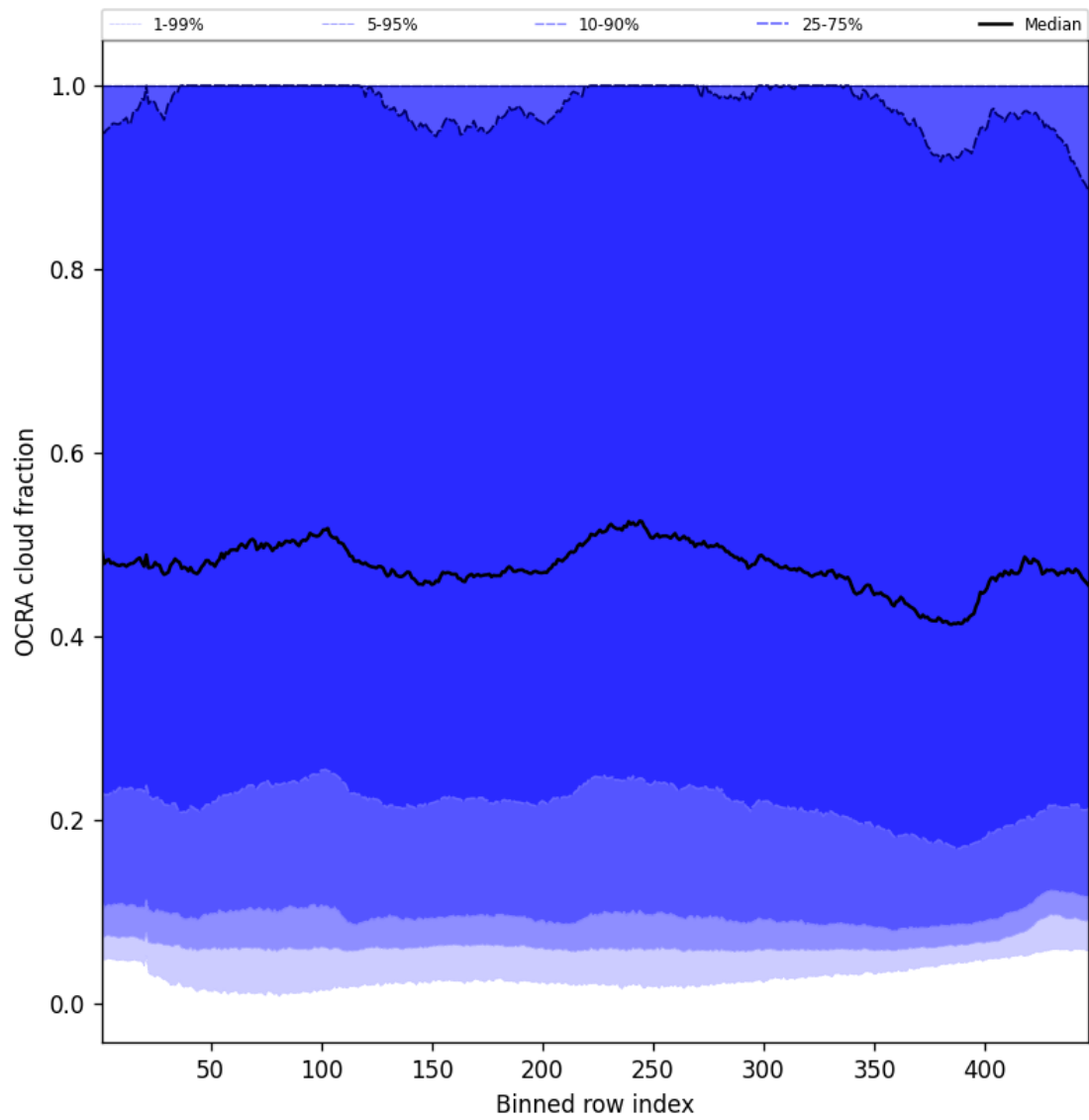
Figure 64: Along track statistics of “OCRA cloud fraction” for 2025-03-09 to 2025-03-10
