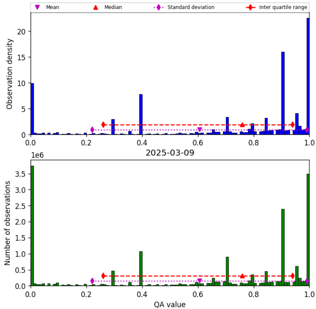
Figure 36: Histogram of “QA value” for 2025-03-09 to 2025-03-10
