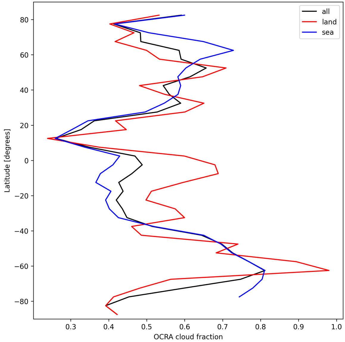
Figure 32: Zonal average of “OCRA cloud fraction” for 2025-03-09 to 2025-03-10.
