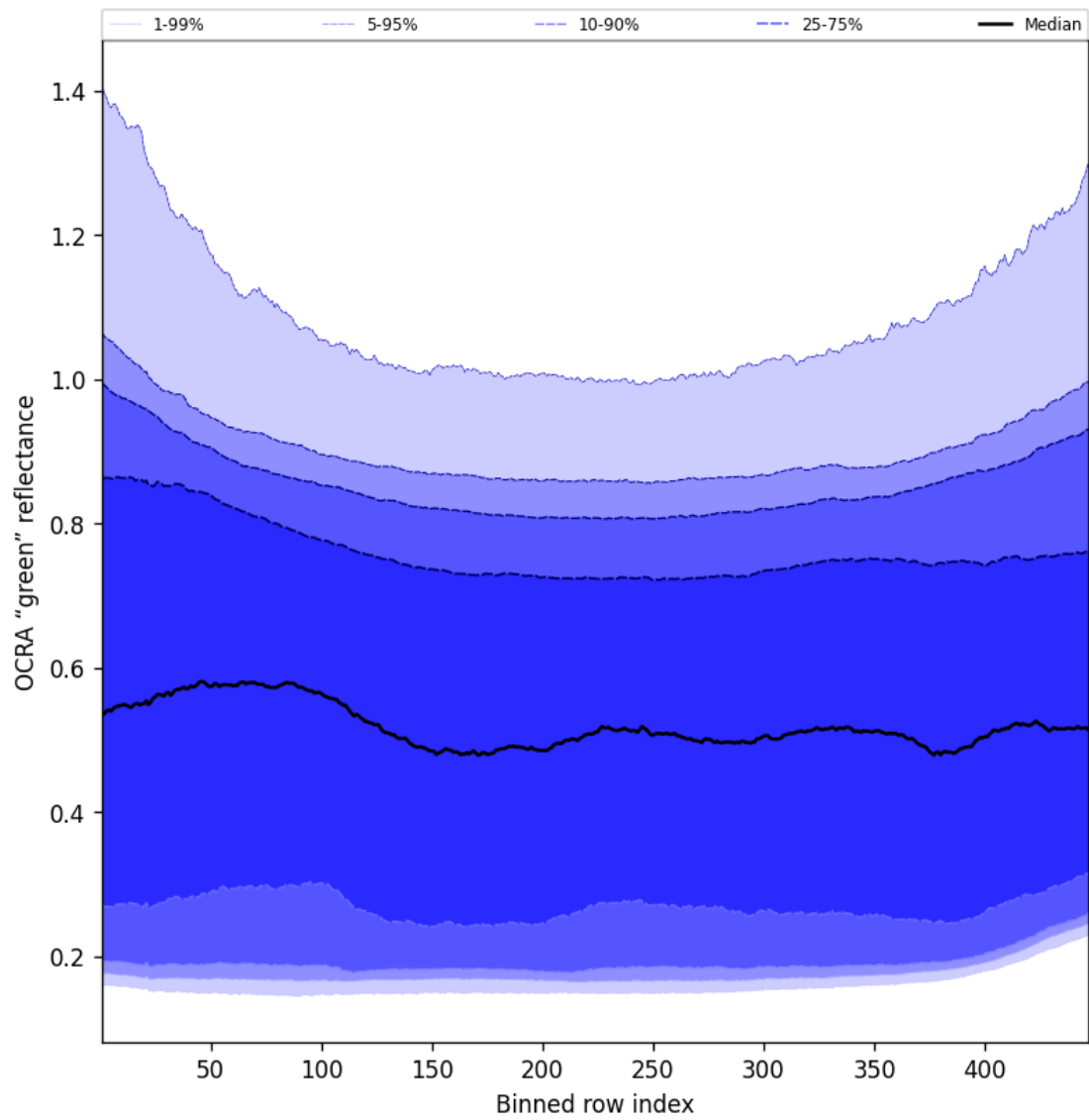
Figure 66: Along track statistics of “OCRA “green” reflectance” for 2025-03-09 to 2025-03-10
