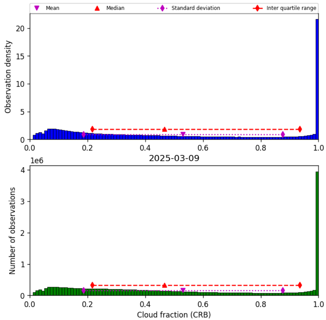
Figure 40: Histogram of “Cloud fraction (CRB)” for 2025-03-09 to 2025-03-10
