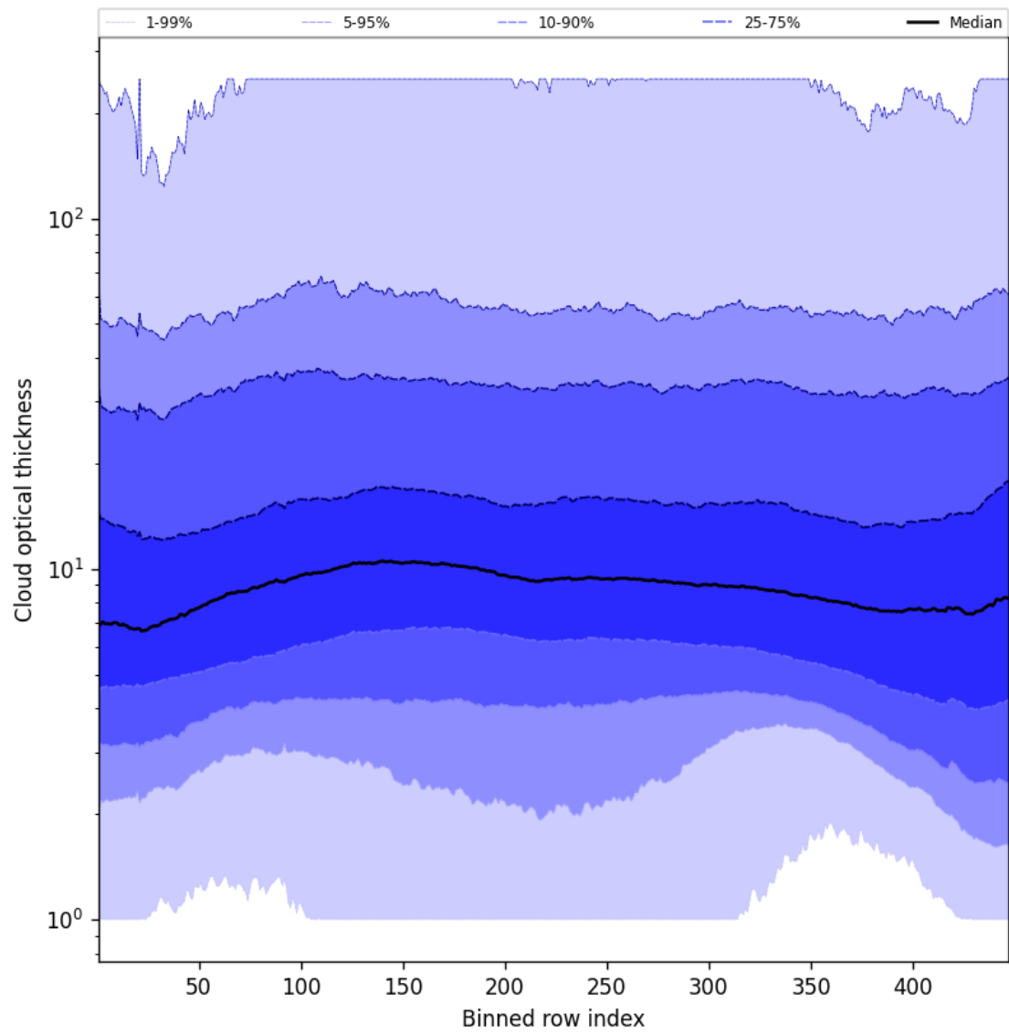
Figure 55: Along track statistics of “Cloud optical thickness” for 2025-03-09 to 2025-03-10
