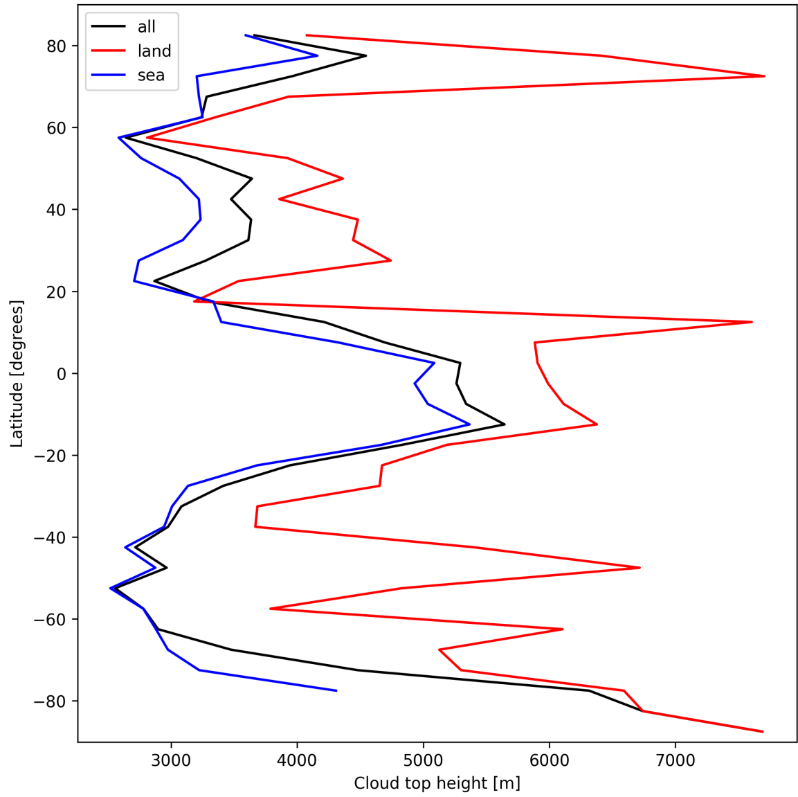
Figure 22: Zonal average of “Cloud top height” for 2025-03-09 to 2025-03-10.
