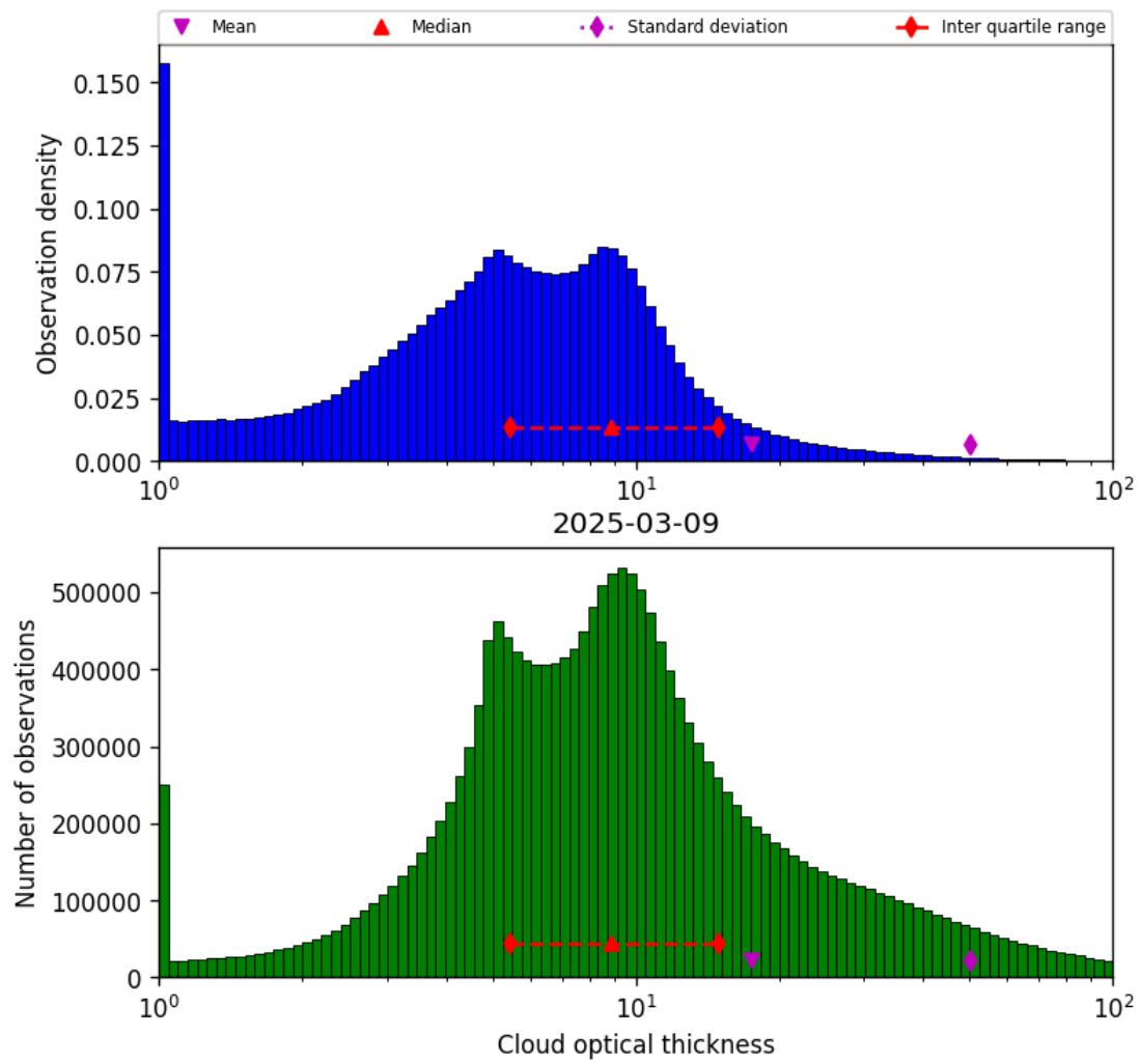
Figure 39: Histogram of “Cloud optical thickness” for 2025-03-09 to 2025-03-10
