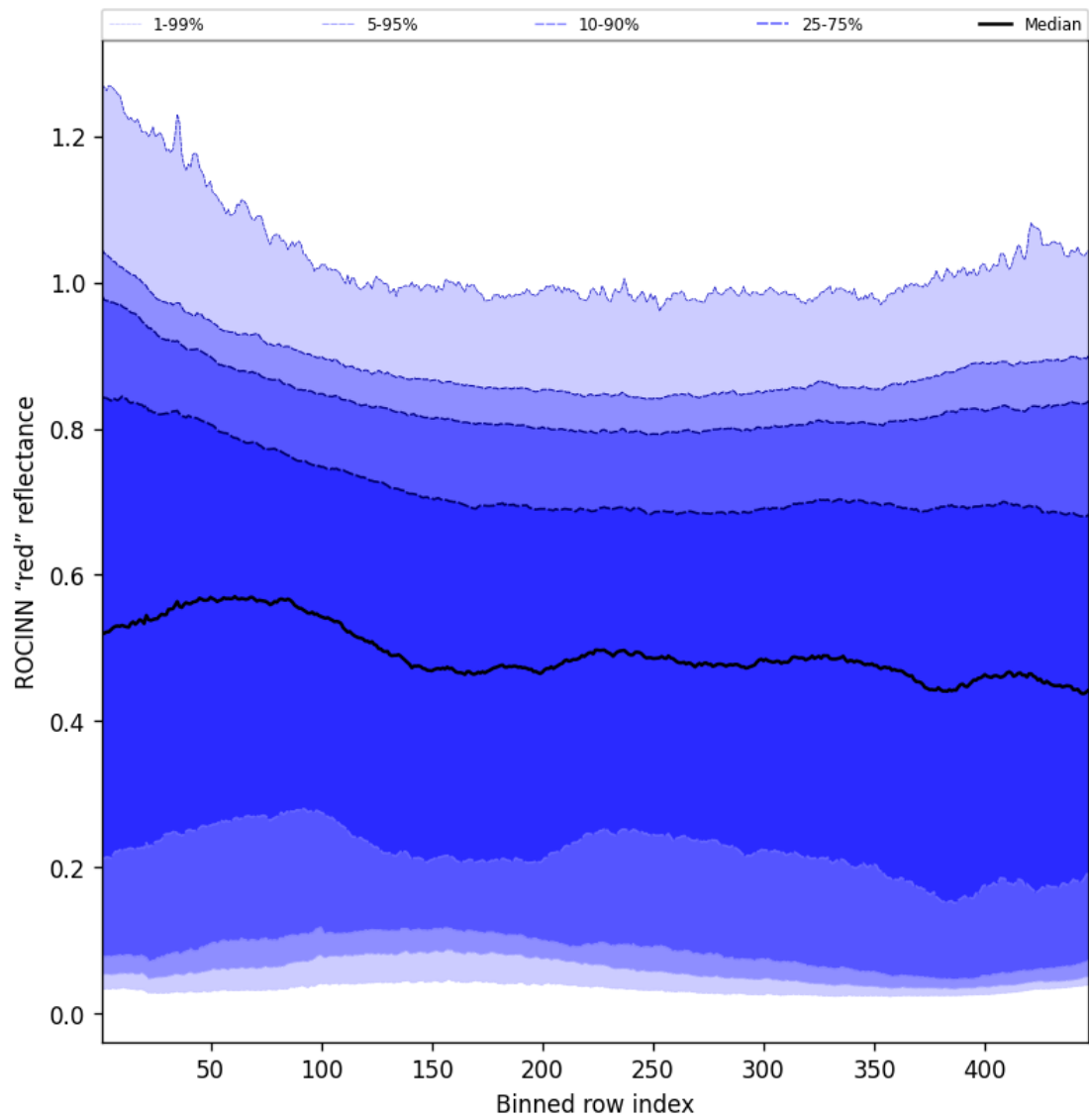
Figure 67: Along track statistics of “ROCINN “red” reflectance” for 2025-03-09 to 2025-03-10
