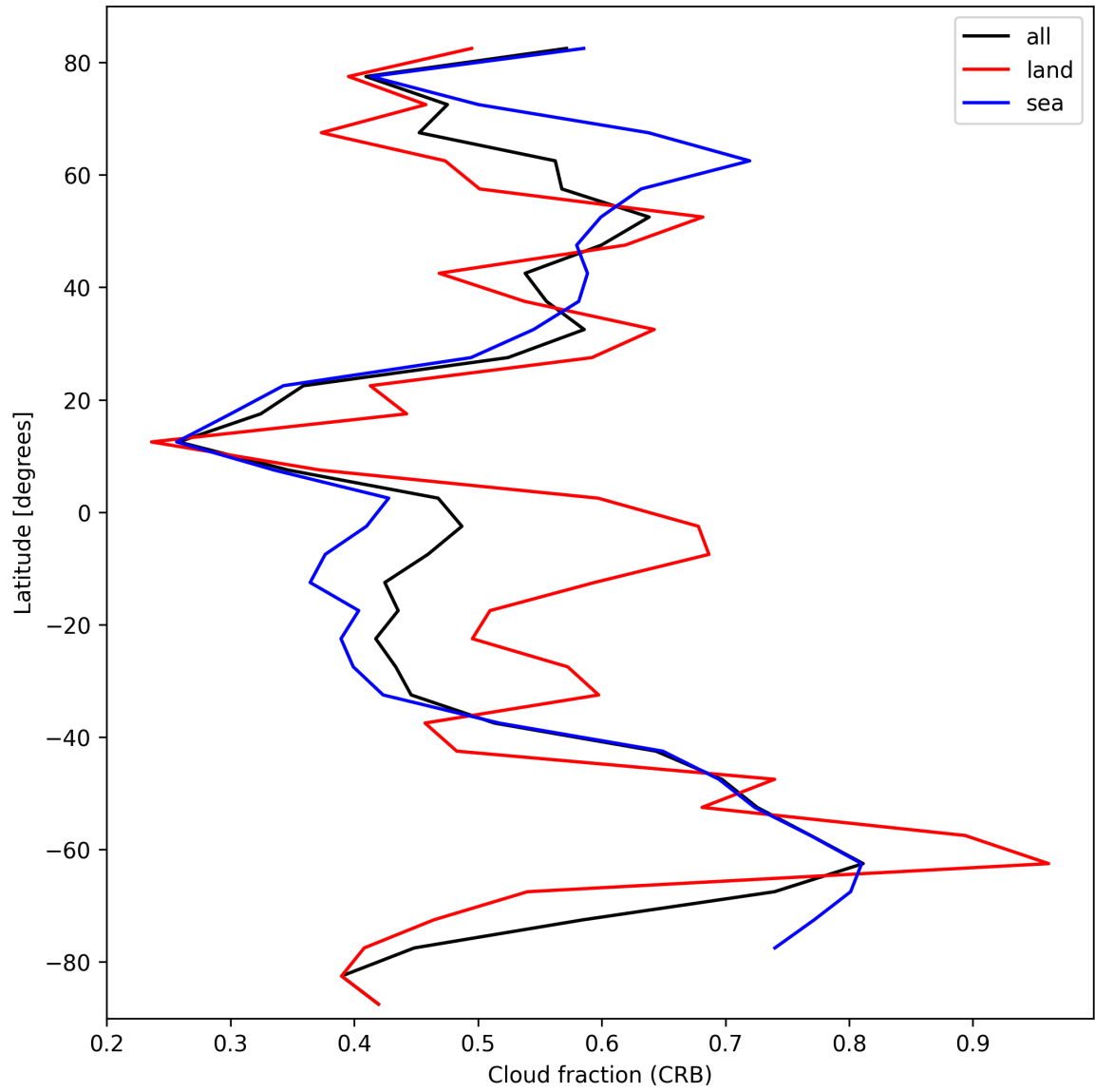
Figure 24: Zonal average of “Cloud fraction (CRB)” for 2025-03-09 to 2025-03-10.
