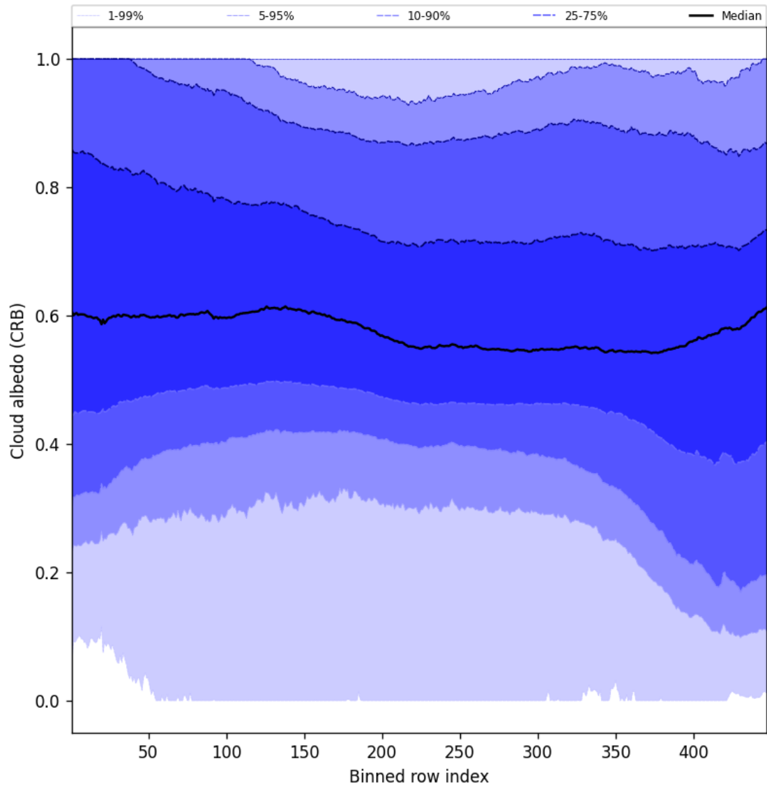
Figure 58: Along track statistics of “Cloud albedo (CRB)” for 2025-03-09 to 2025-03-10
