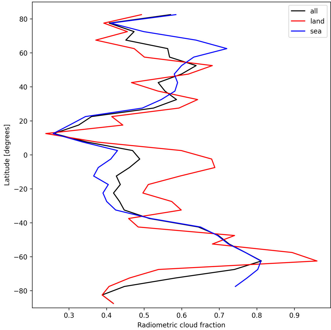
Figure 21: Zonal average of “Radiometric cloud fraction” for 2025-03-09 to 2025-03-10.
