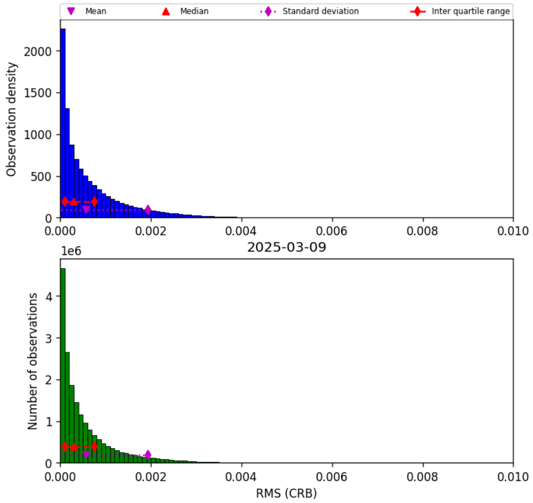
Figure 46: Histogram of “RMS (CRB)” for 2025-03-09 to 2025-03-10
