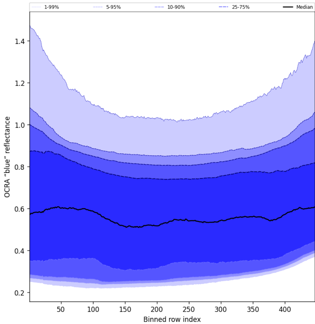
Figure 65: Along track statistics of "OCRA "blue" reflectance" for 2025-03-09 to 2025-03-10
