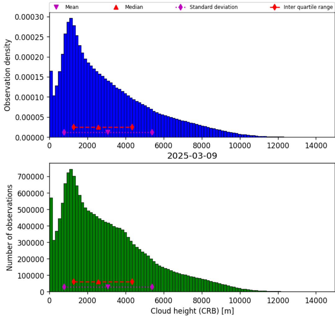
Figure 41: Histogram of “Cloud height (CRB)” for 2025-03-09 to 2025-03-10
