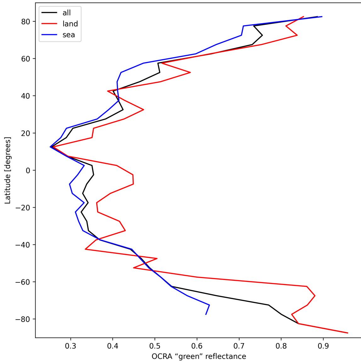
Figure 34: Zonal average of “OCRA “green” reflectance” for 2025-03-09 to 2025-03-10.
