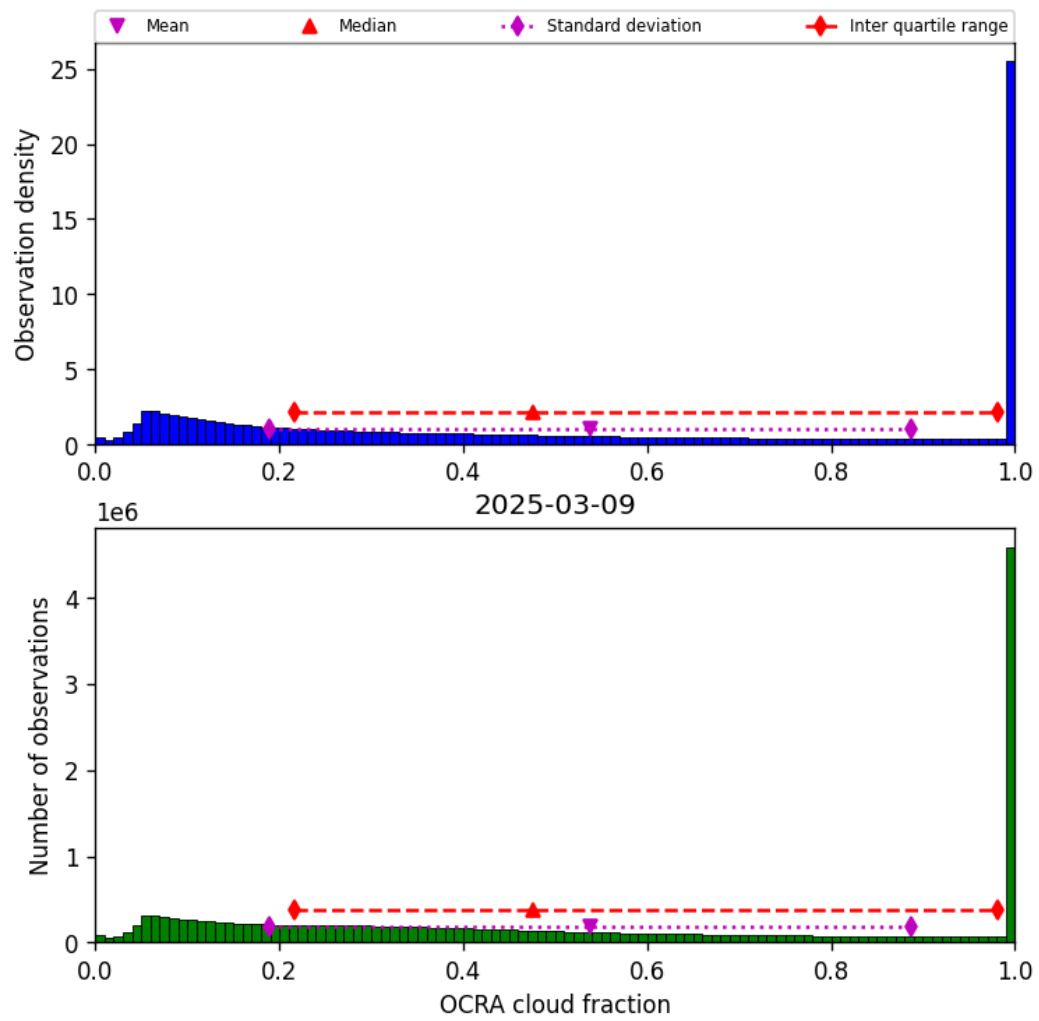
Figure 48: Histogram of “OCRA cloud fraction” for 2025-03-09 to 2025-03-10
