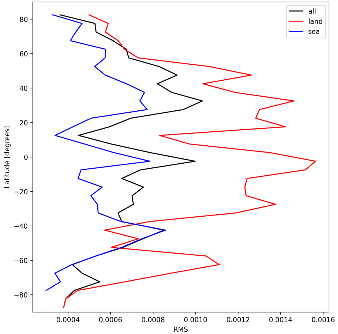
Figure 29: Zonal average of “RMS” for 2025-03-09 to 2025-03-10.
