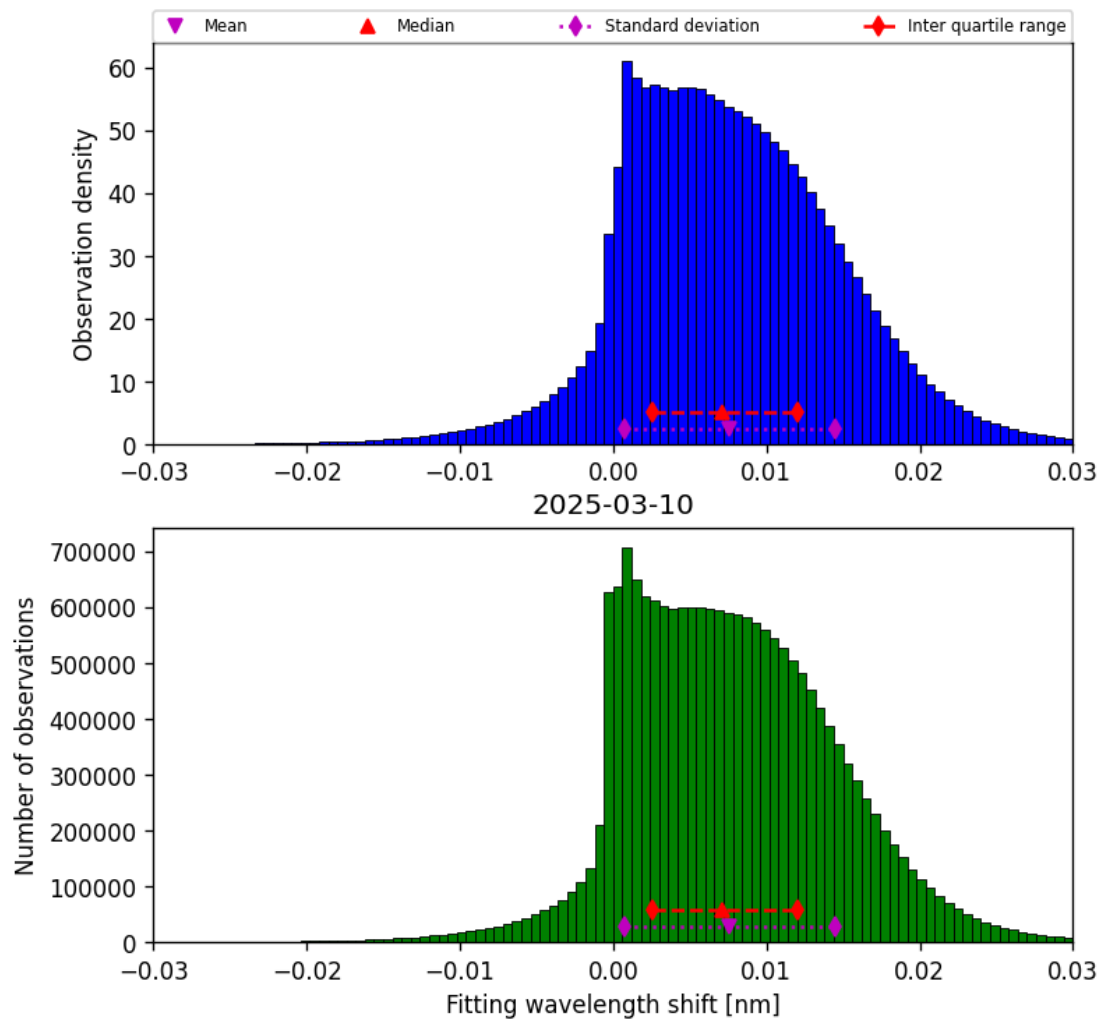
Figure 47: Histogram of “Fitting wavelength shift” for 2025-03-10 to 2025-03-10
