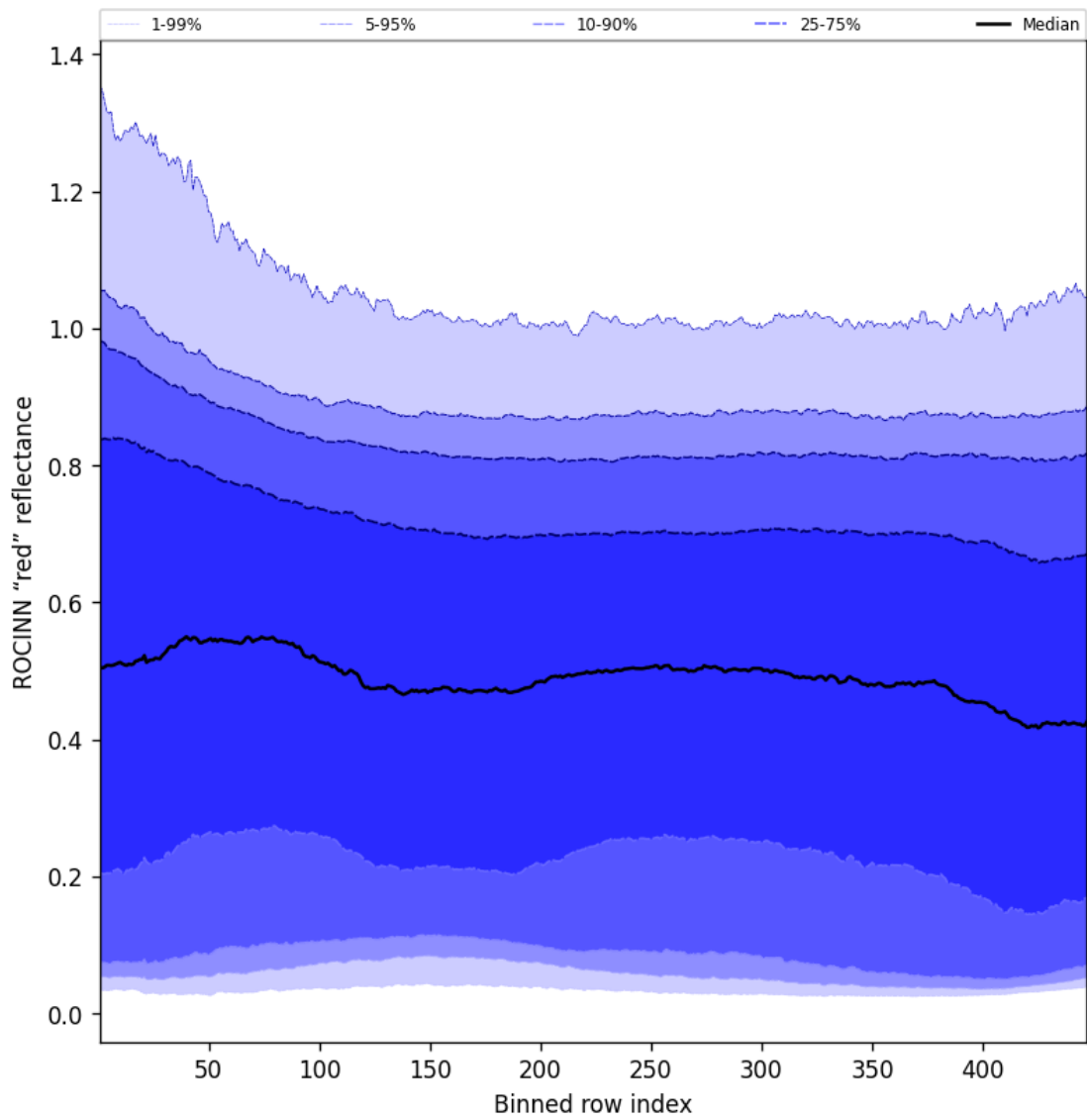
Figure 67: Along track statistics of “ROCINN “red” reflectance” for 2025-03-10 to 2025-03-10
