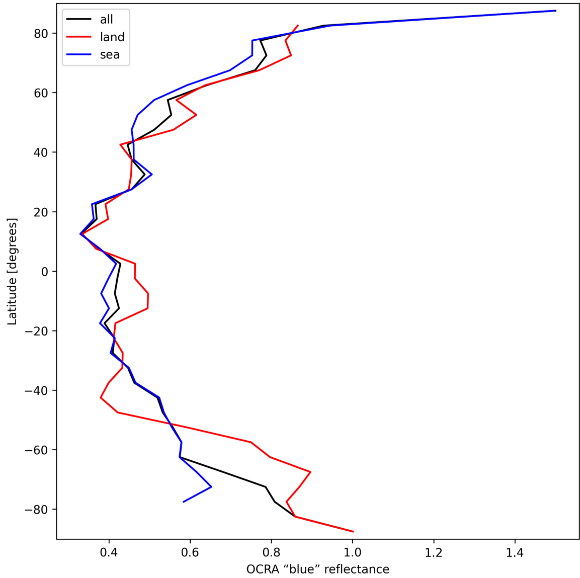
Figure 33: Zonal average of “OCRA “blue” reflectance” for 2025-03-10 to 2025-03-10.
