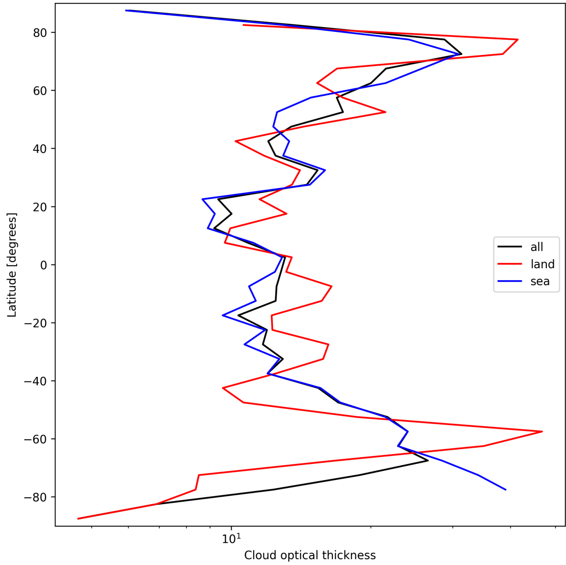
Figure 23: Zonal average of “Cloud optical thickness” for 2025-03-10 to 2025-03-10.
