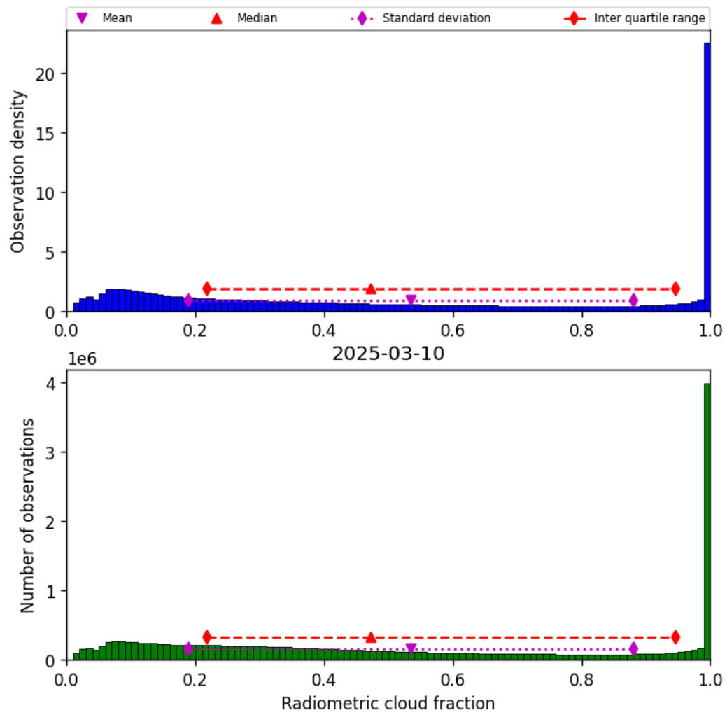
Figure 37: Histogram of “Radiometric cloud fraction” for 2025-03-10 to 2025-03-10
