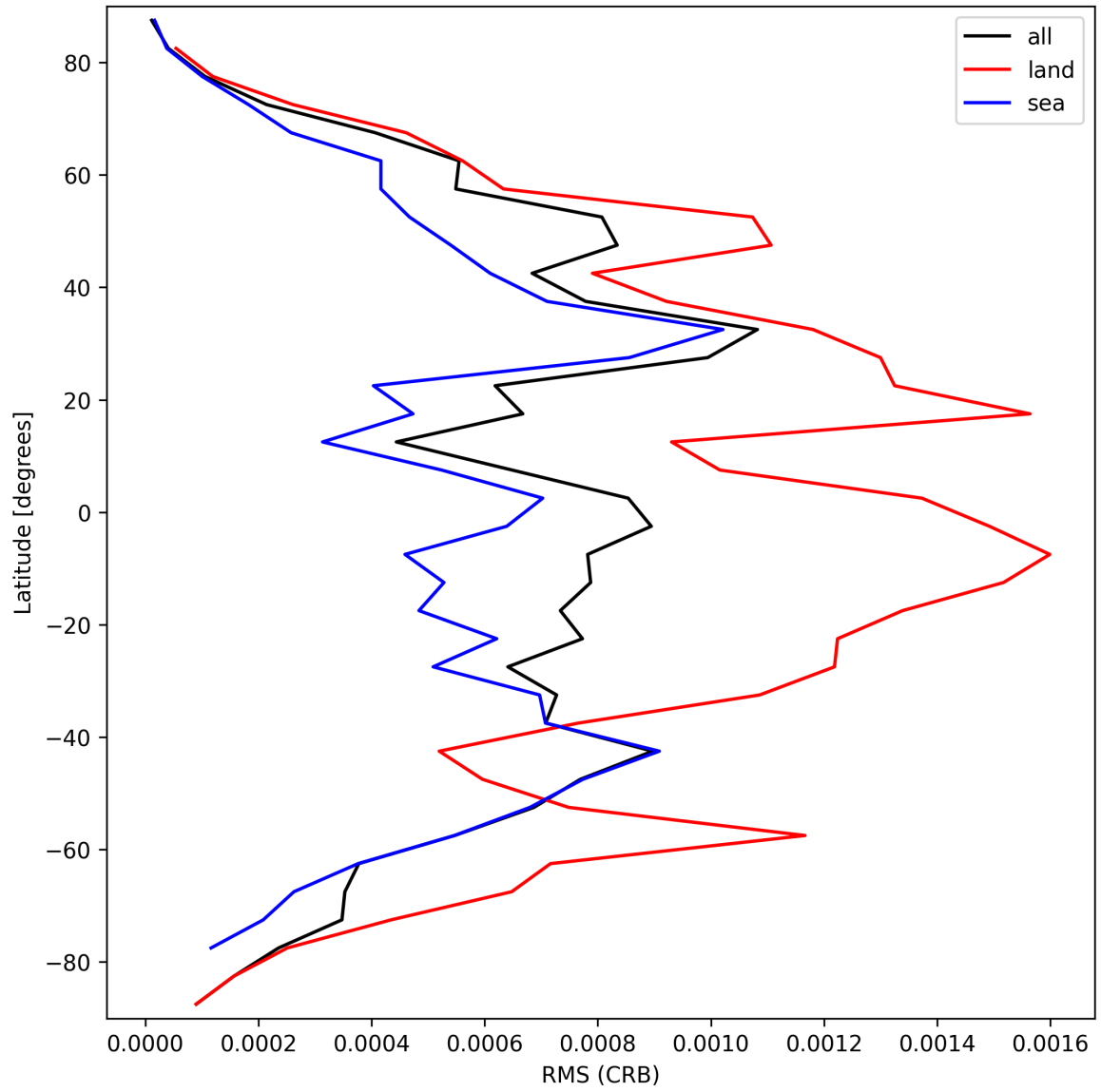
Figure 30: Zonal average of “RMS (CRB)” for 2025-03-10 to 2025-03-10.
