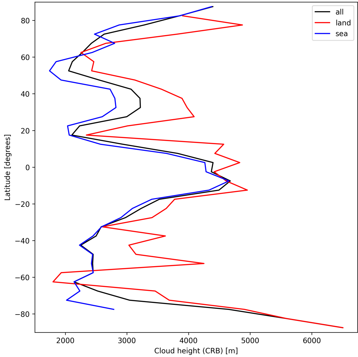
Figure 25: Zonal average of “Cloud height (CRB)” for 2025-03-10 to 2025-03-10.
