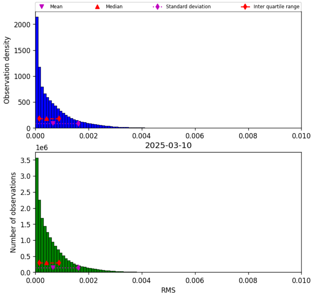
Figure 45: Histogram of “RMS” for 2025-03-10 to 2025-03-10
