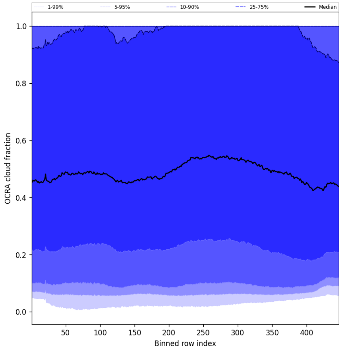
Figure 64: Along track statistics of “OCRA cloud fraction” for 2025-03-10 to 2025-03-10
