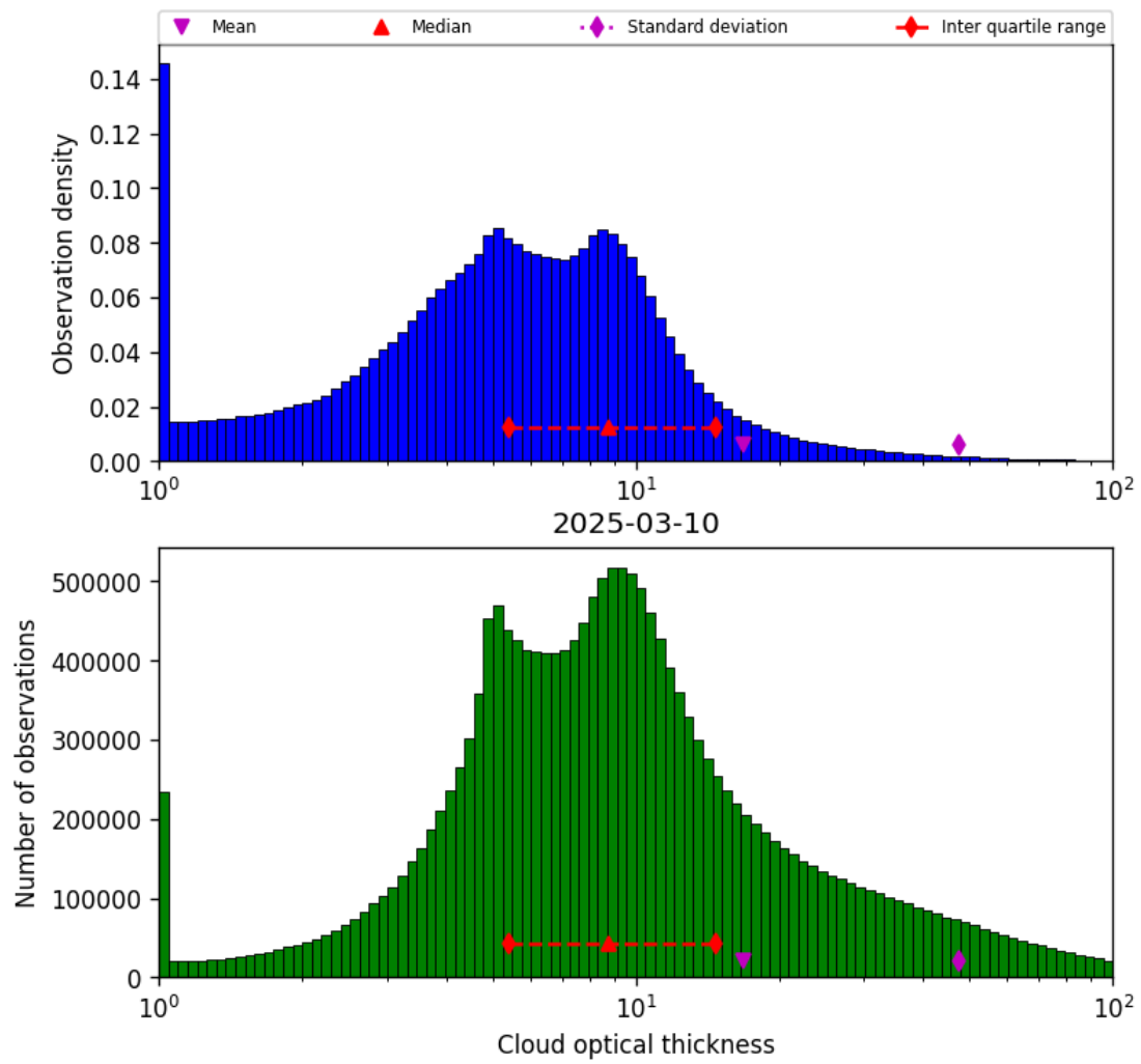
Figure 39: Histogram of “Cloud optical thickness” for 2025-03-10 to 2025-03-10
