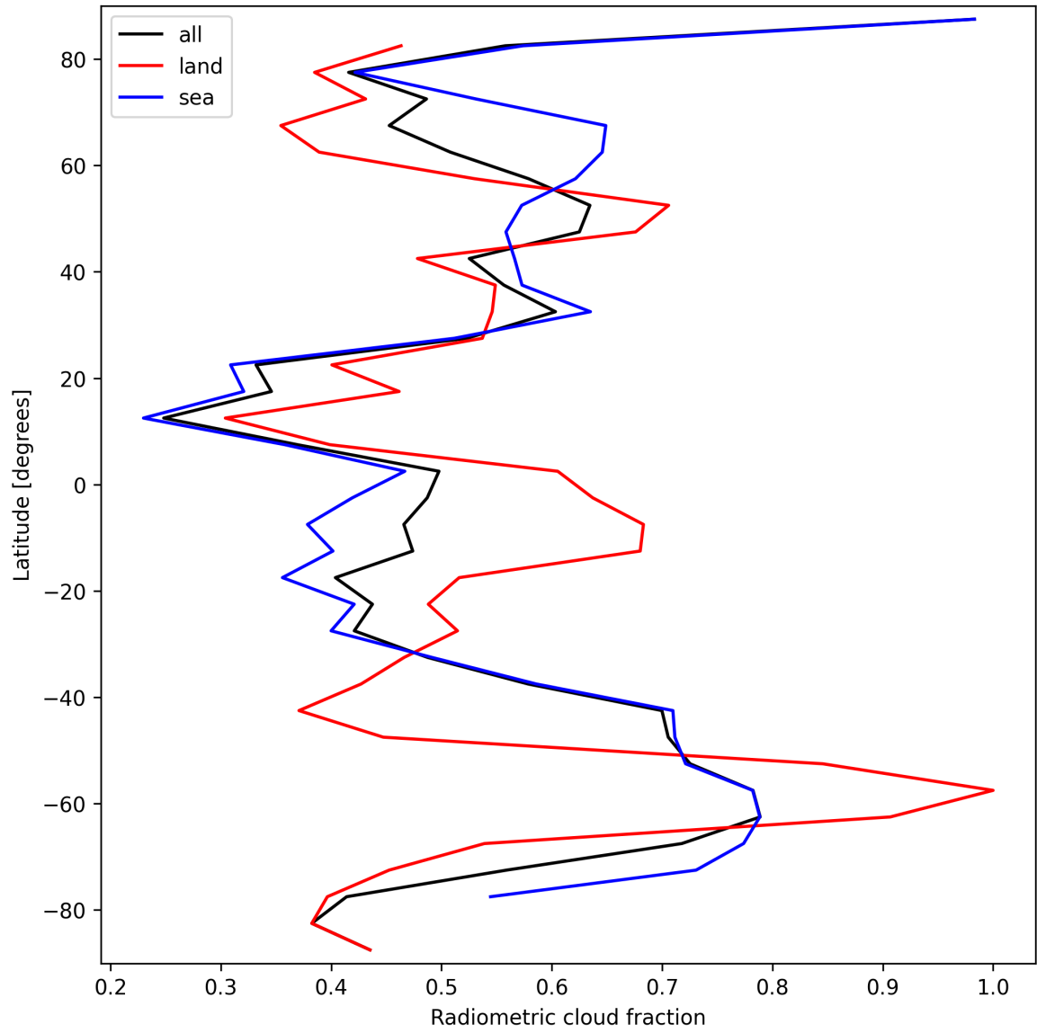
Figure 21: Zonal average of “Radiometric cloud fraction” for 2025-03-10 to 2025-03-10.
