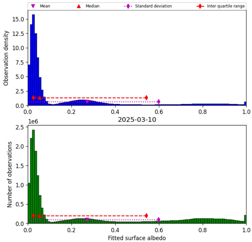
Figure 43: Histogram of “Fitted surface albedo” for 2025-03-10 to 2025-03-10
