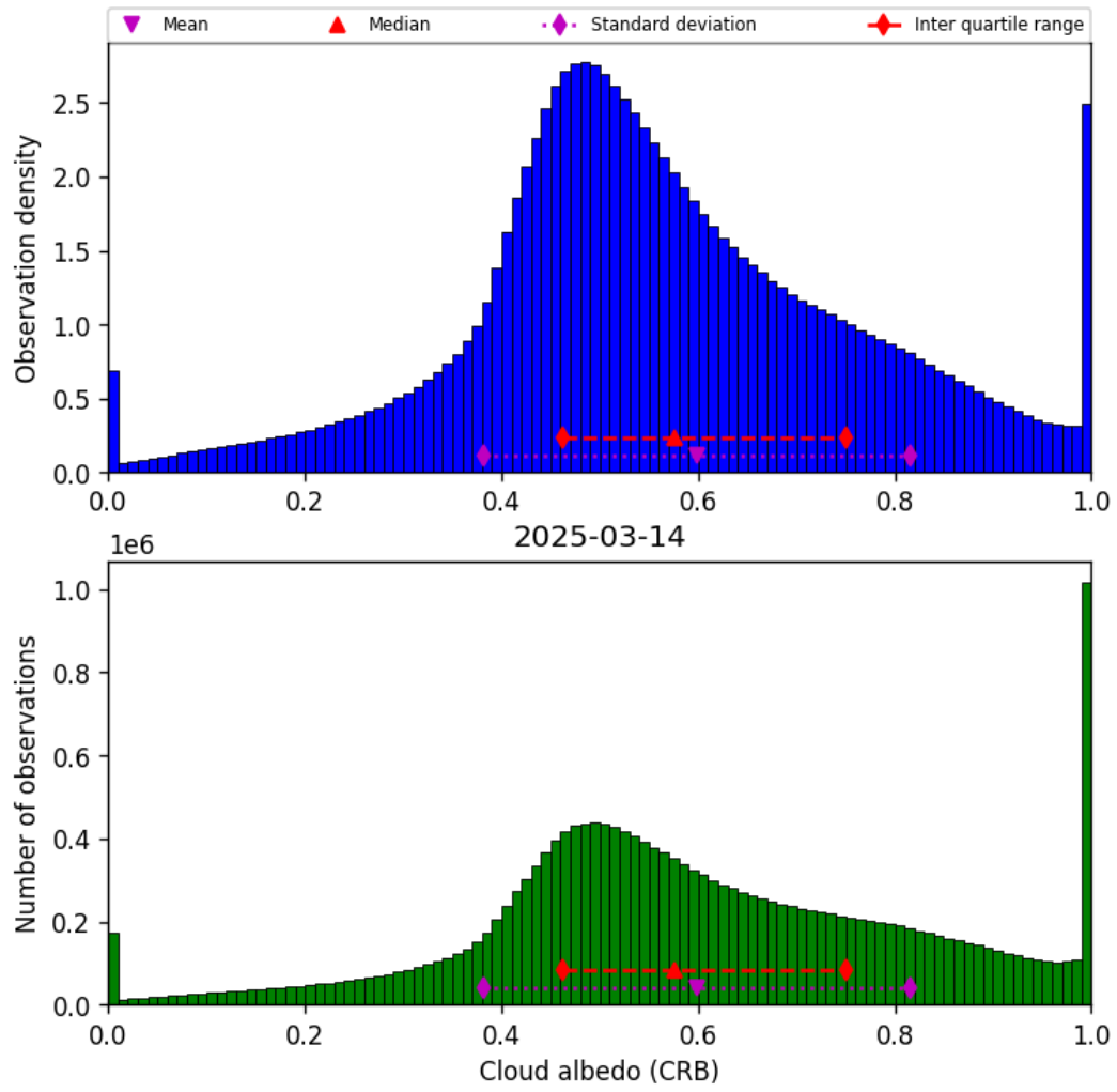
Figure 42: Histogram of “Cloud albedo (CRB)” for 2025-03-14 to 2025-03-15
