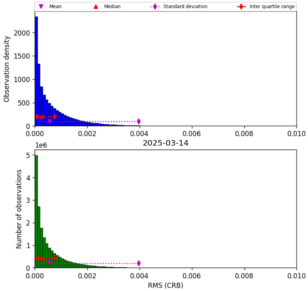
Figure 46: Histogram of “RMS (CRB)” for 2025-03-14 to 2025-03-15
