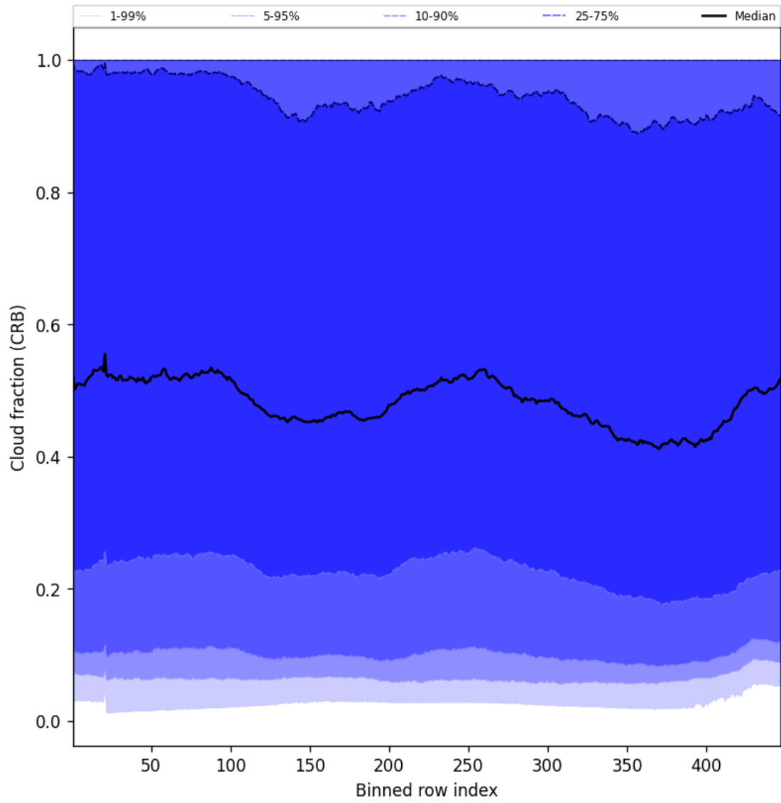
Figure 56: Along track statistics of “Cloud fraction (CRB)” for 2025-03-14 to 2025-03-15
