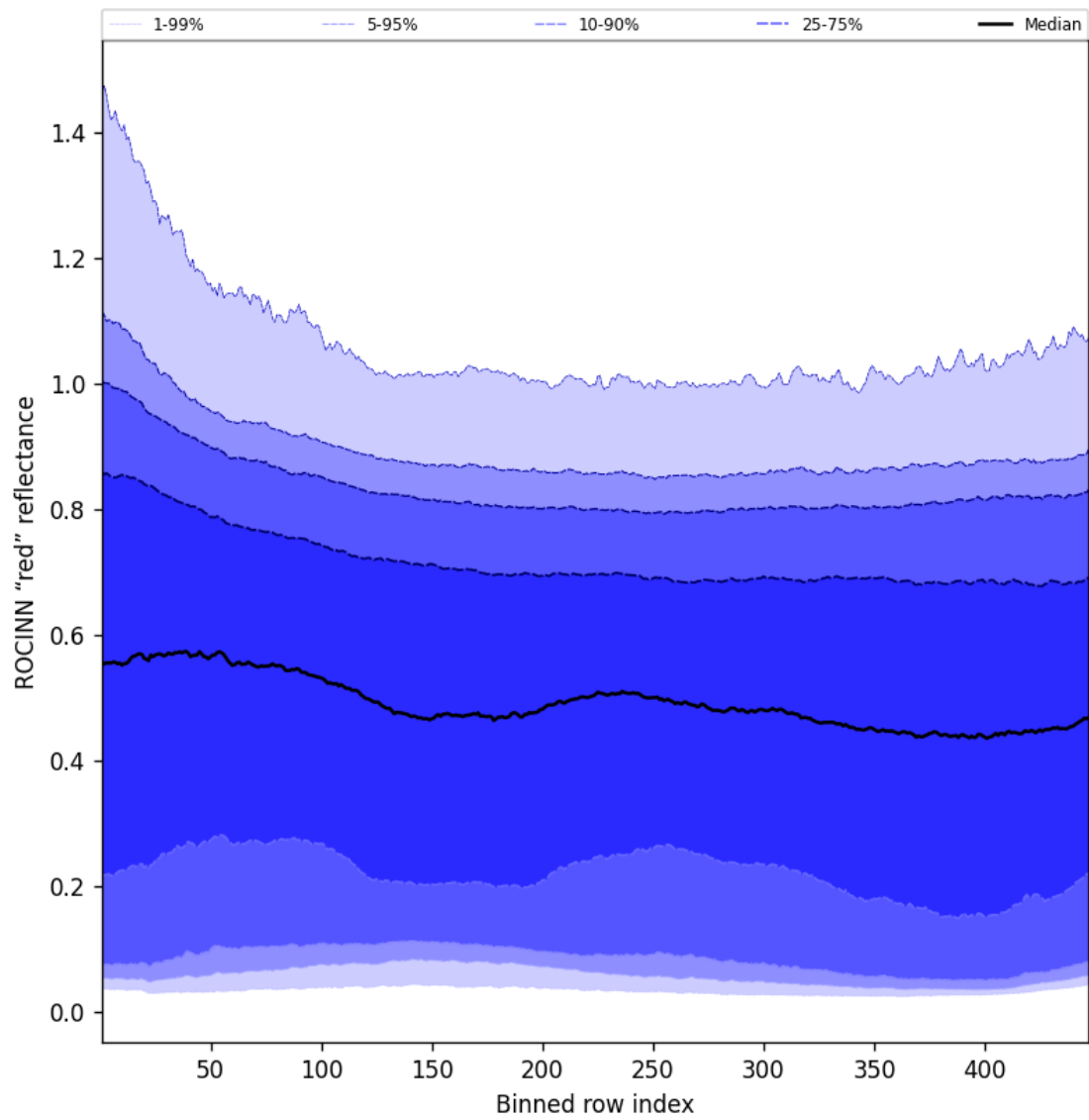
Figure 67: Along track statistics of “ROCINN “red” reflectance” for 2025-03-14 to 2025-03-15
