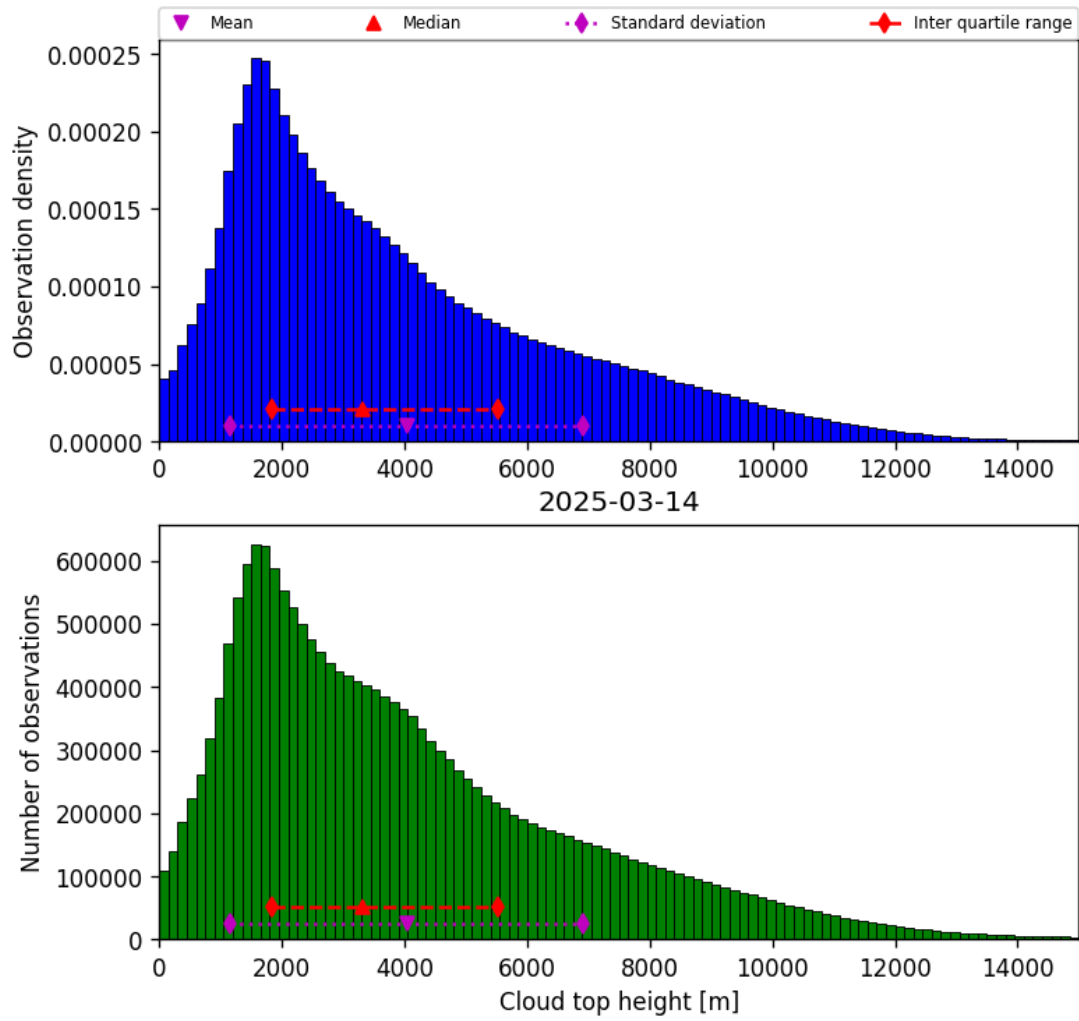
Figure 38: Histogram of “Cloud top height” for 2025-03-14 to 2025-03-15
