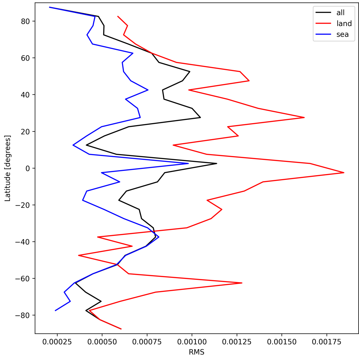
Figure 29: Zonal average of “RMS” for 2025-03-14 to 2025-03-15.
