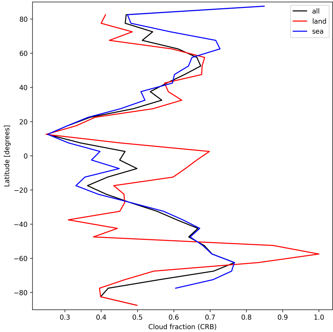
Figure 24: Zonal average of “Cloud fraction (CRB)” for 2025-03-14 to 2025-03-15.
