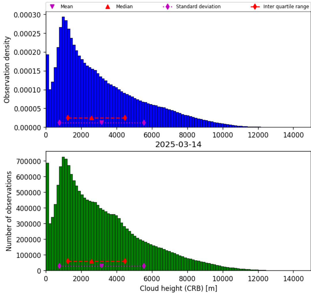
Figure 41: Histogram of “Cloud height (CRB)” for 2025-03-14 to 2025-03-15
