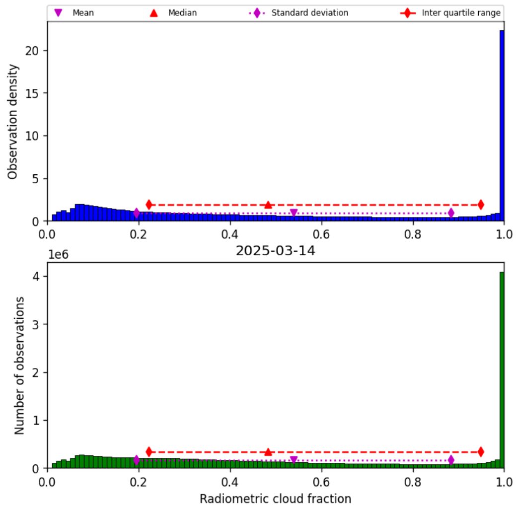
Figure 37: Histogram of “Radiometric cloud fraction” for 2025-03-14 to 2025-03-15
