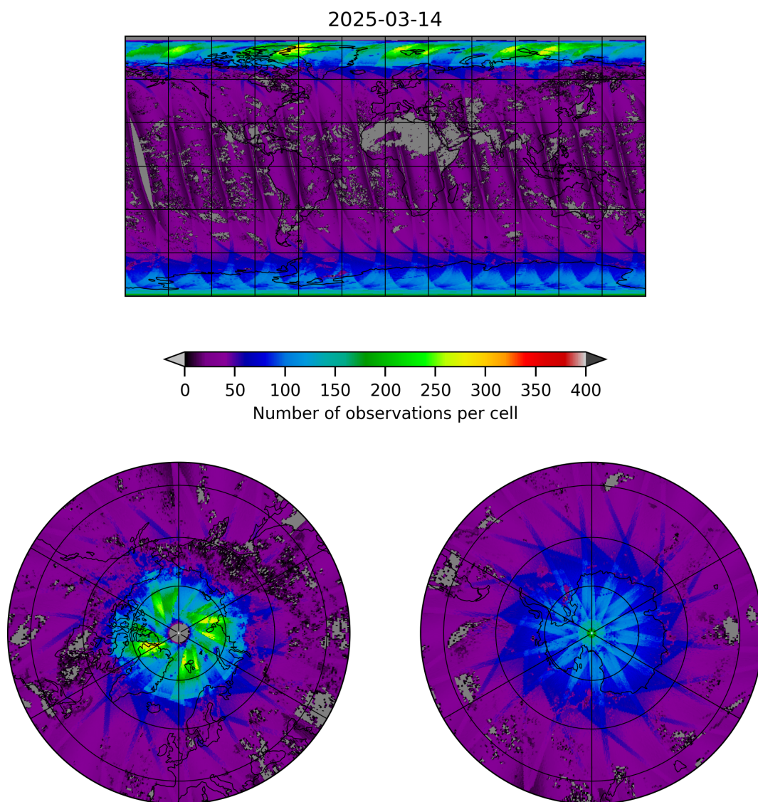
Figure 19: Map of the number of observations for 2025-03-14 to 2025-03-15
