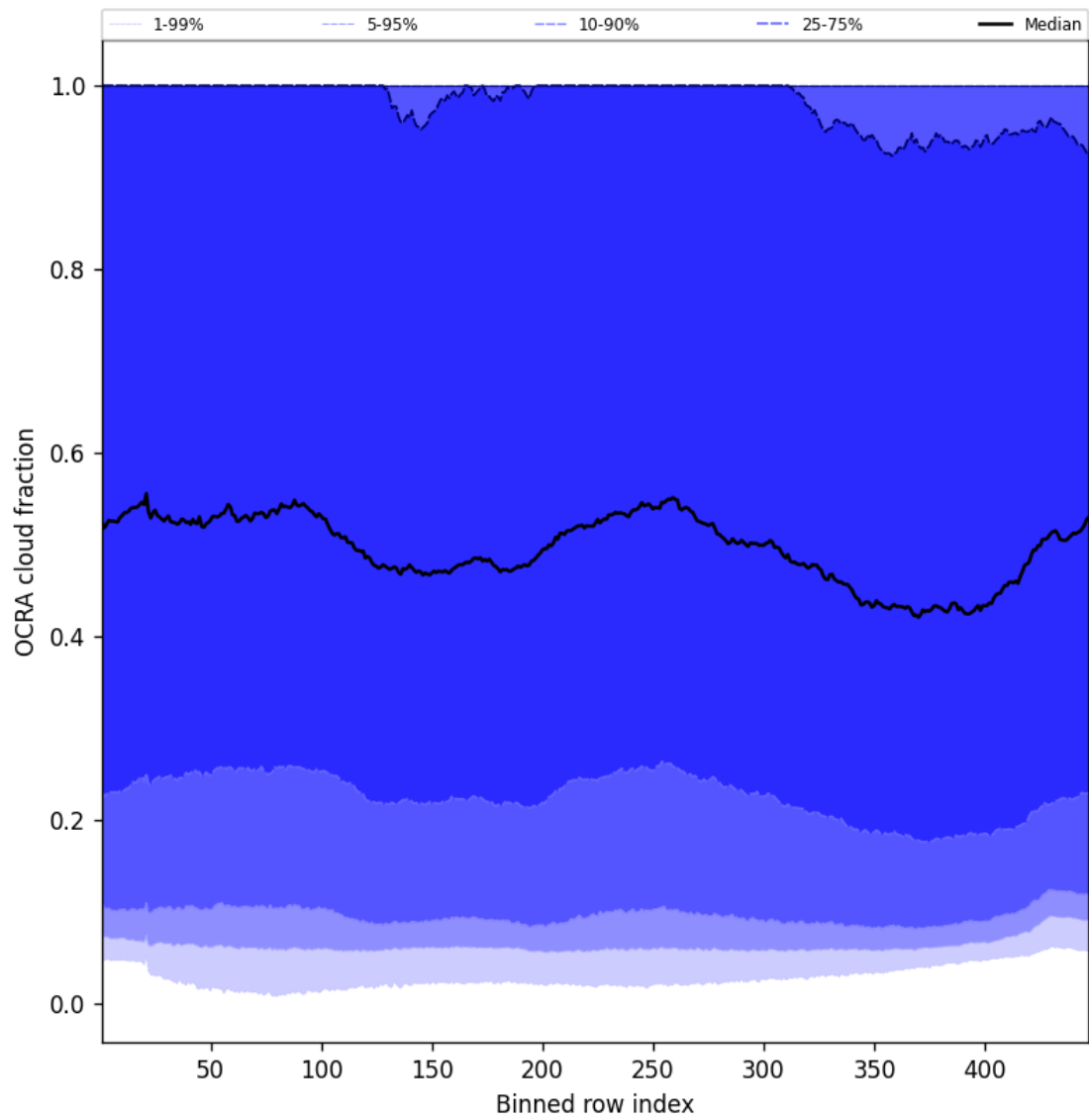
Figure 64: Along track statistics of “OCRA cloud fraction” for 2025-03-14 to 2025-03-15
