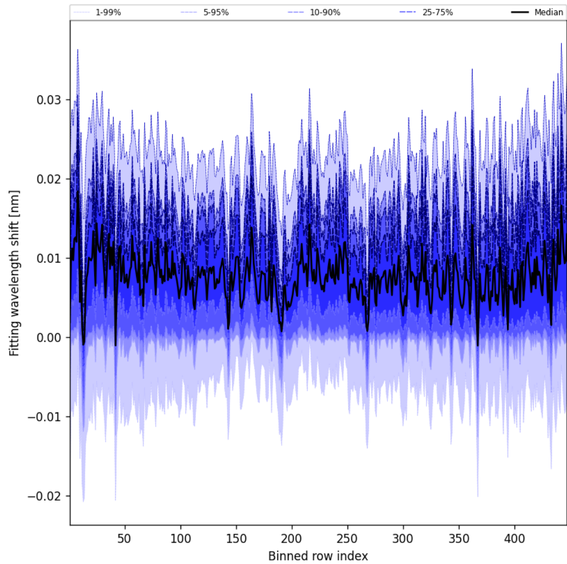
Figure 63: Along track statistics of “Fitting wavelength shift” for 2025-03-14 to 2025-03-15
