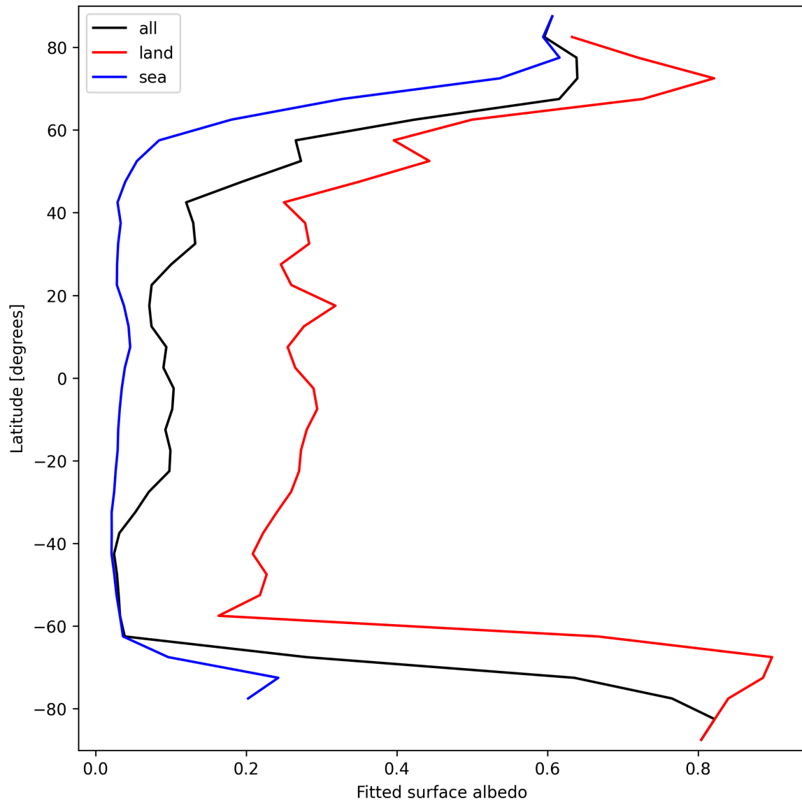
Figure 27: Zonal average of “Fitted surface albedo” for 2025-03-14 to 2025-03-15.
