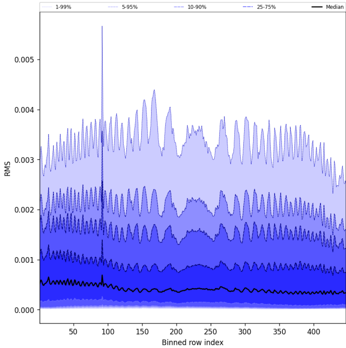
Figure 61: Along track statistics of “RMS” for 2025-03-14 to 2025-03-15
