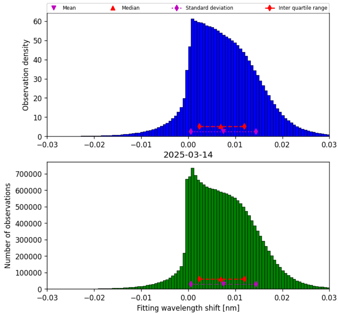
Figure 47: Histogram of “Fitting wavelength shift” for 2025-03-14 to 2025-03-15
