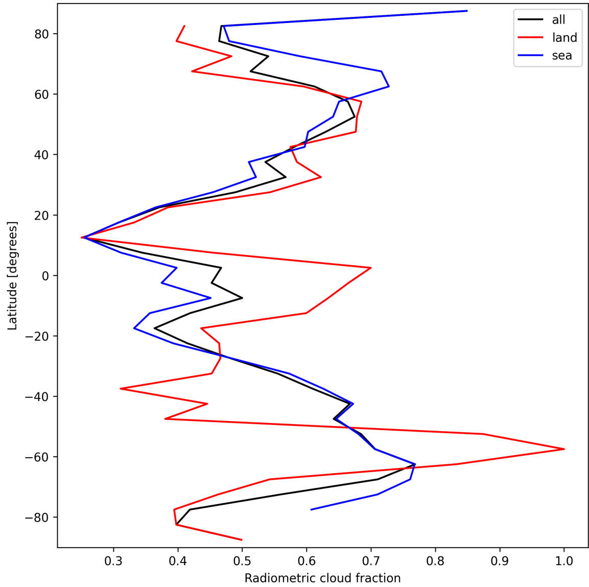
Figure 21: Zonal average of “Radiometric cloud fraction” for 2025-03-14 to 2025-03-15.
