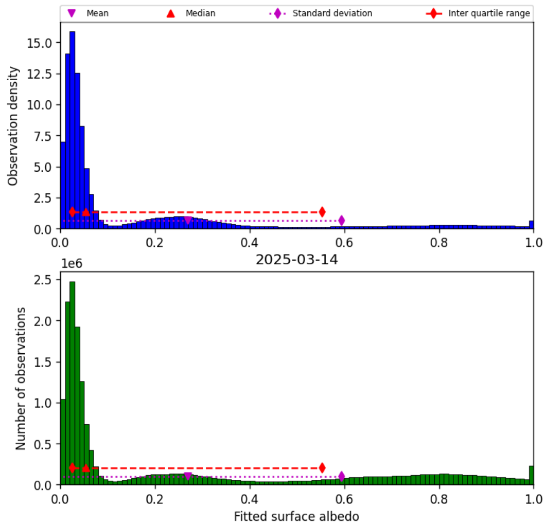
Figure 43: Histogram of “Fitted surface albedo” for 2025-03-14 to 2025-03-15
