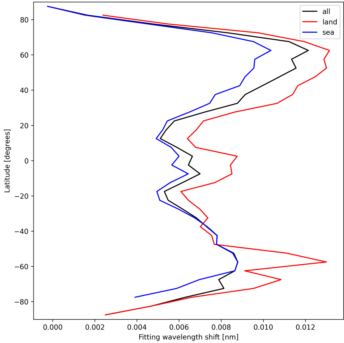
Figure 31: Zonal average of “Fitting wavelength shift” for 2025-03-14 to 2025-03-15.
