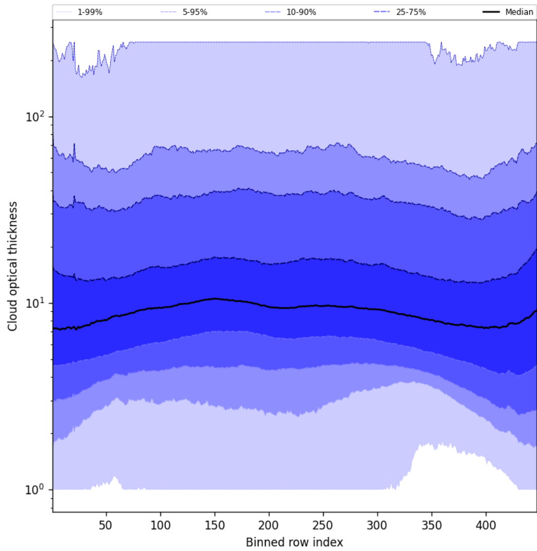
Figure 55: Along track statistics of “Cloud optical thickness” for 2025-03-14 to 2025-03-15
