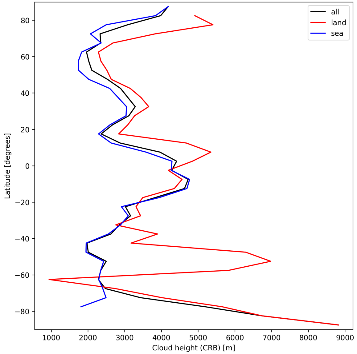
Figure 25: Zonal average of “Cloud height (CRB)” for 2025-03-14 to 2025-03-15.
