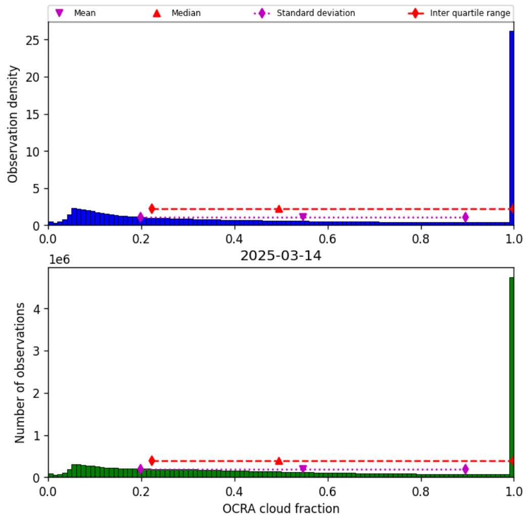
Figure 48: Histogram of “OCRA cloud fraction” for 2025-03-14 to 2025-03-15
