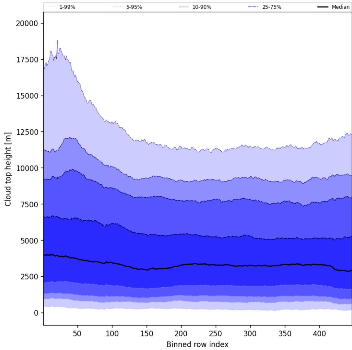
Figure 54: Along track statistics of “Cloud top height” for 2025-03-14 to 2025-03-15
