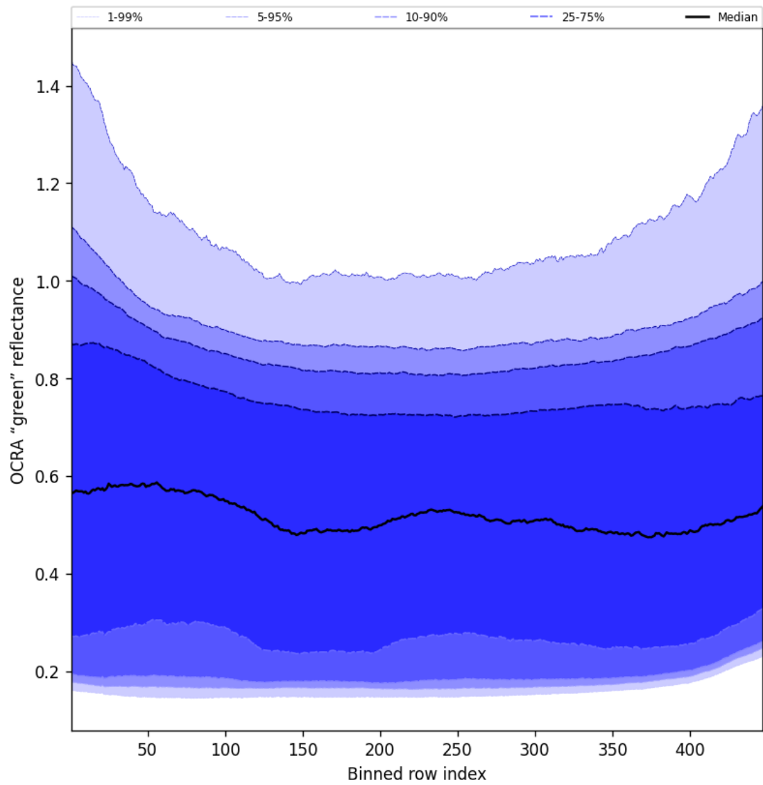
Figure 66: Along track statistics of “OCRA “green” reflectance” for 2025-03-14 to 2025-03-15
