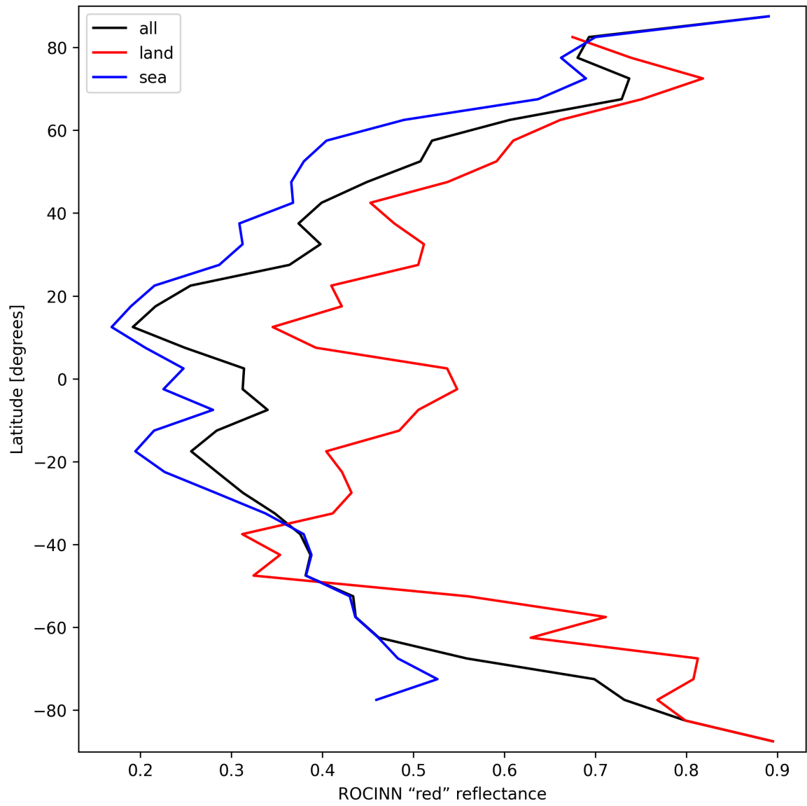
Figure 35: Zonal average of “ROCINN “red” reflectance” for 2025-03-14 to 2025-03-15.
