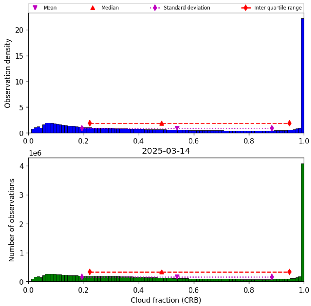
Figure 40: Histogram of “Cloud fraction (CRB)” for 2025-03-14 to 2025-03-15
