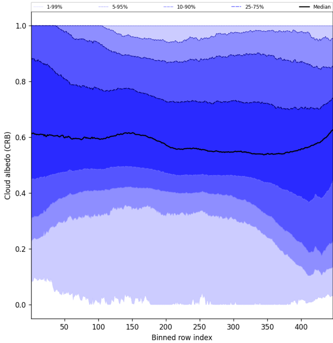
Figure 58: Along track statistics of “Cloud albedo (CRB)” for 2025-03-14 to 2025-03-15
