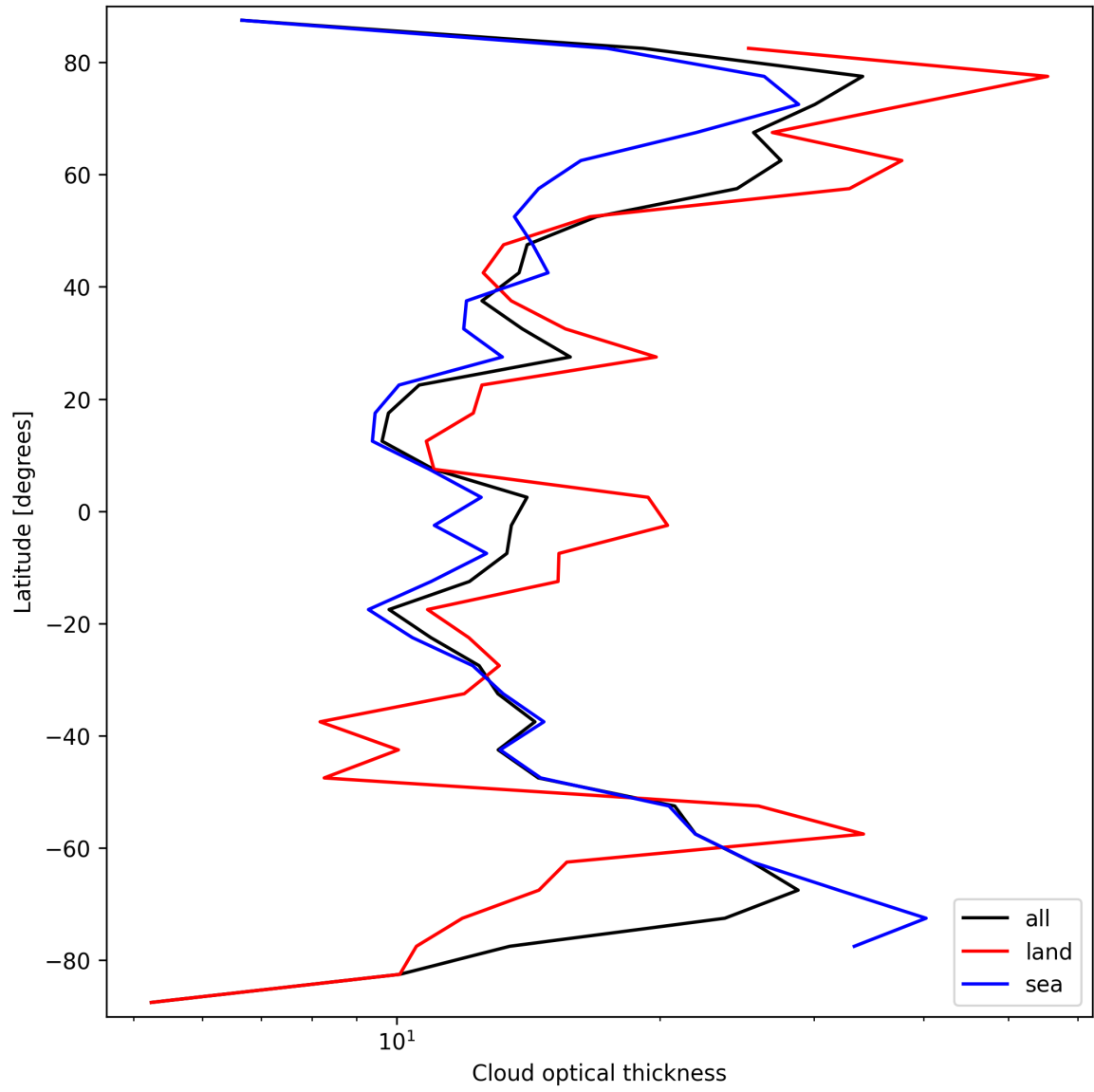
Figure 23: Zonal average of “Cloud optical thickness” for 2025-03-14 to 2025-03-15.
