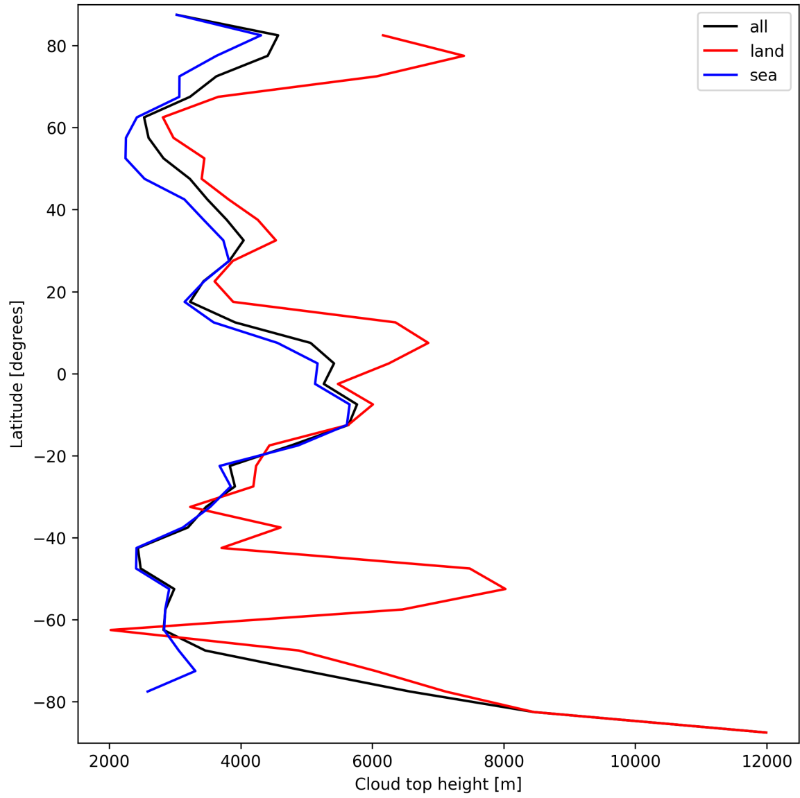
Figure 22: Zonal average of “Cloud top height” for 2025-03-14 to 2025-03-15.
