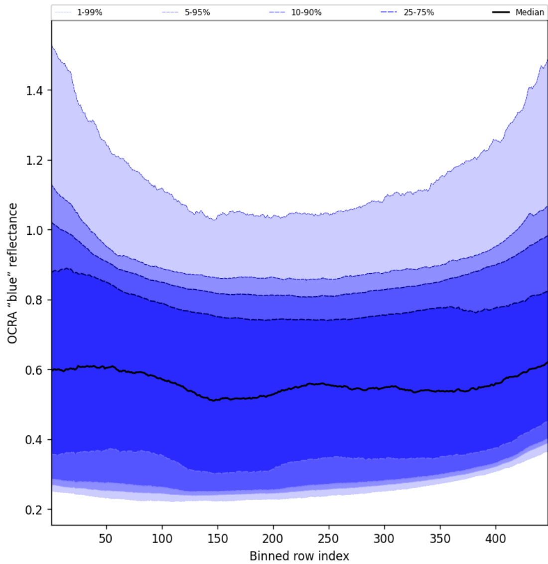
Figure 65: Along track statistics of “OCRA “blue” reflectance” for 2025-03-14 to 2025-03-15
