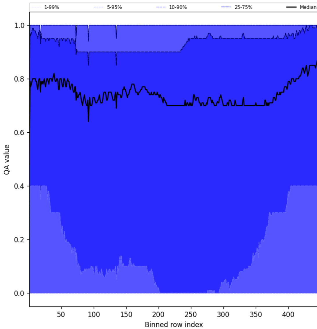
Figure 52: Along track statistics of “QA value” for 2025-03-14 to 2025-03-15
