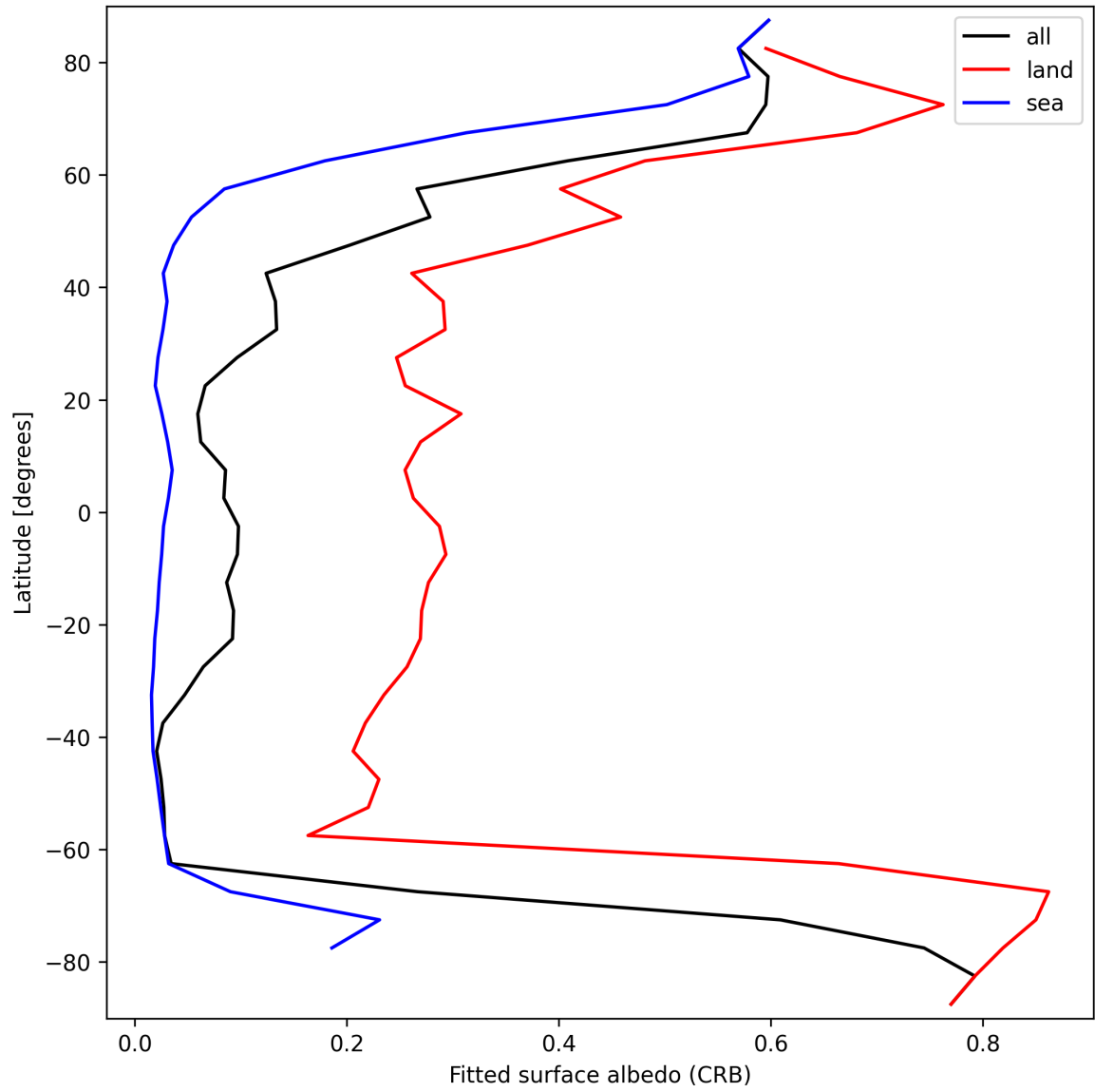
Figure 28: Zonal average of “Fitted surface albedo (CRB)” for 2025-03-14 to 2025-03-15.
