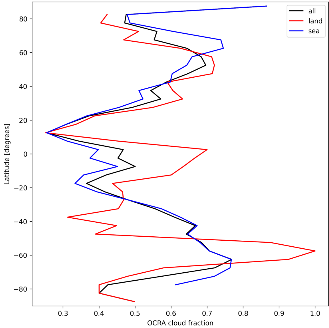
Figure 32: Zonal average of “OCRA cloud fraction” for 2025-03-14 to 2025-03-15.
