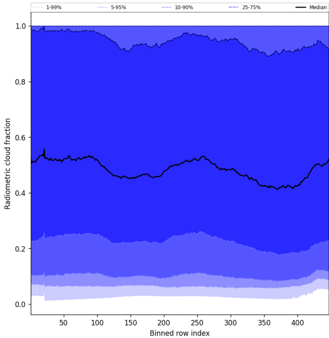
Figure 53: Along track statistics of “Radiometric cloud fraction” for 2025-03-14 to 2025-03-15
