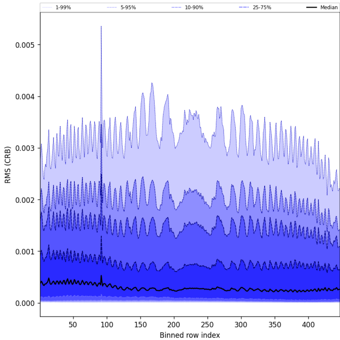
Figure 62: Along track statistics of “RMS (CRB)” for 2025-03-14 to 2025-03-15
