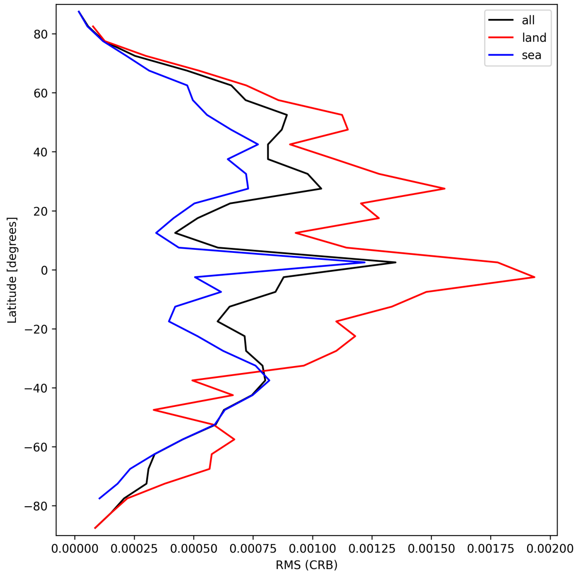
Figure 30: Zonal average of “RMS (CRB)” for 2025-03-14 to 2025-03-15.
