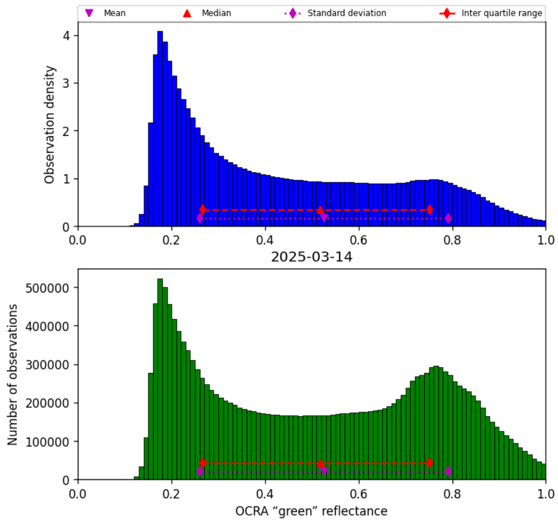
Figure 50: Histogram of “OCRA “green” reflectance” for 2025-03-14 to 2025-03-15
