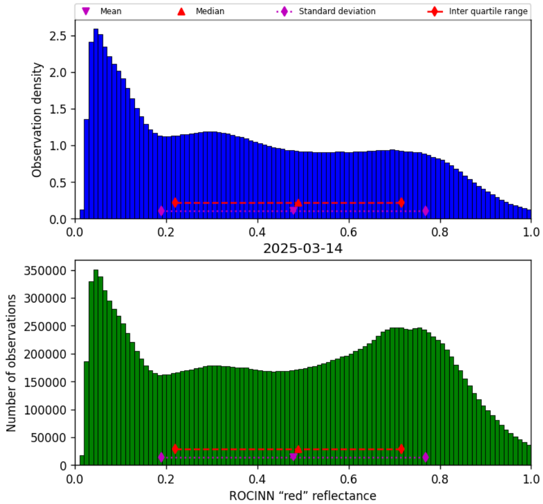
Figure 51: Histogram of “ROCINN “red” reflectance” for 2025-03-14 to 2025-03-15
