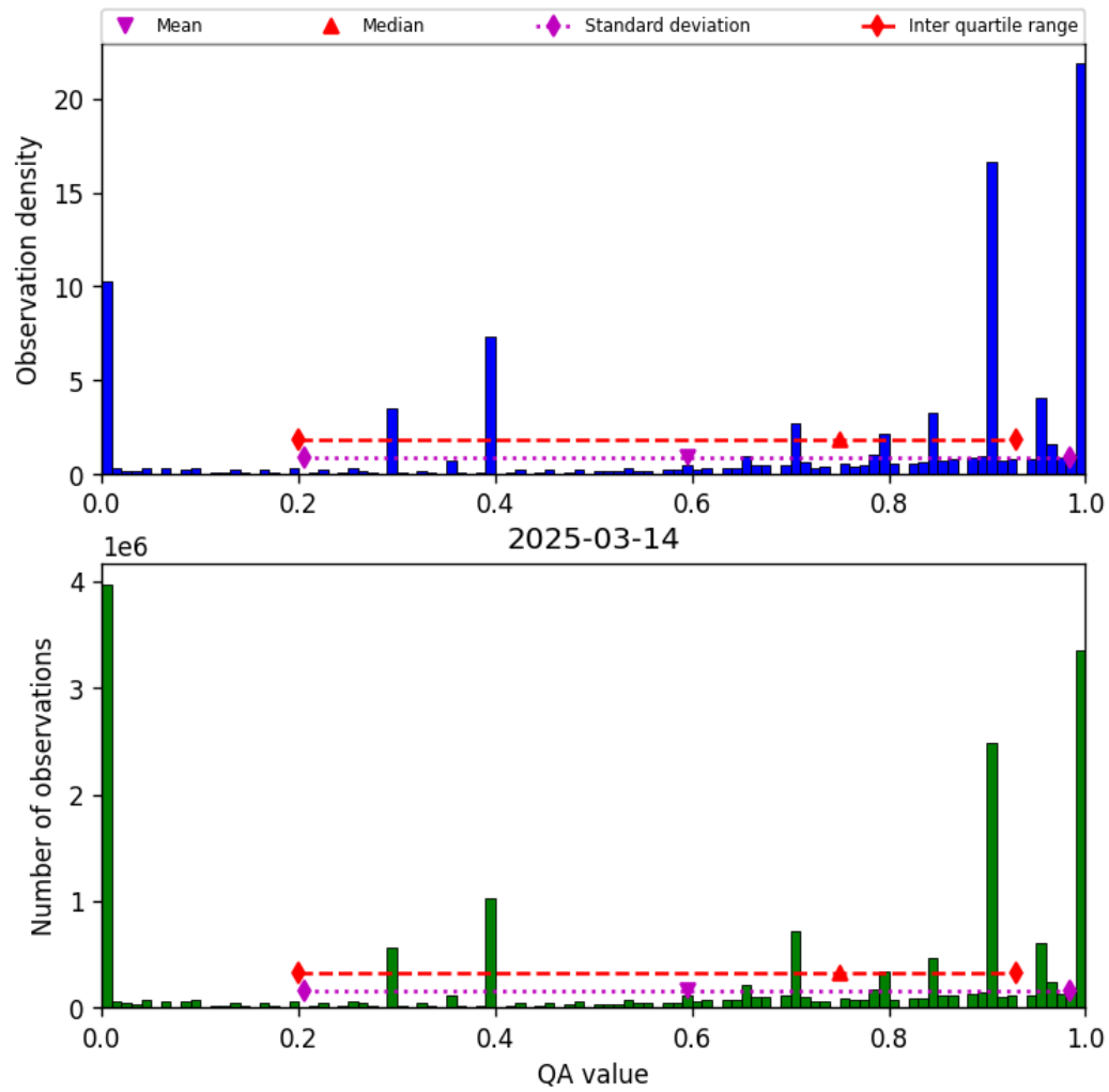
Figure 36: Histogram of “QA value” for 2025-03-14 to 2025-03-15
