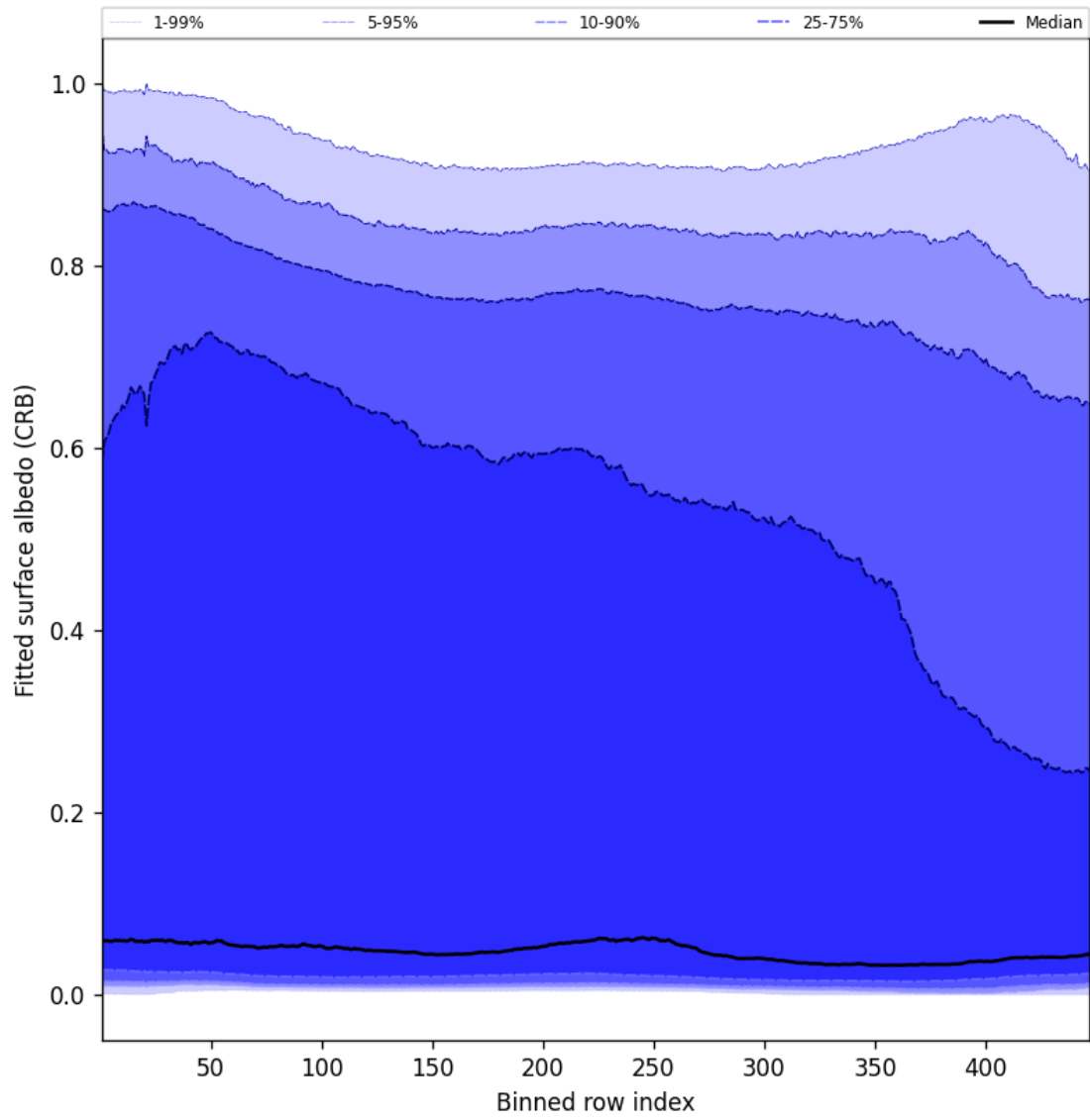
Figure 60: Along track statistics of “Fitted surface albedo (CRB)” for 2025-03-14 to 2025-03-15
