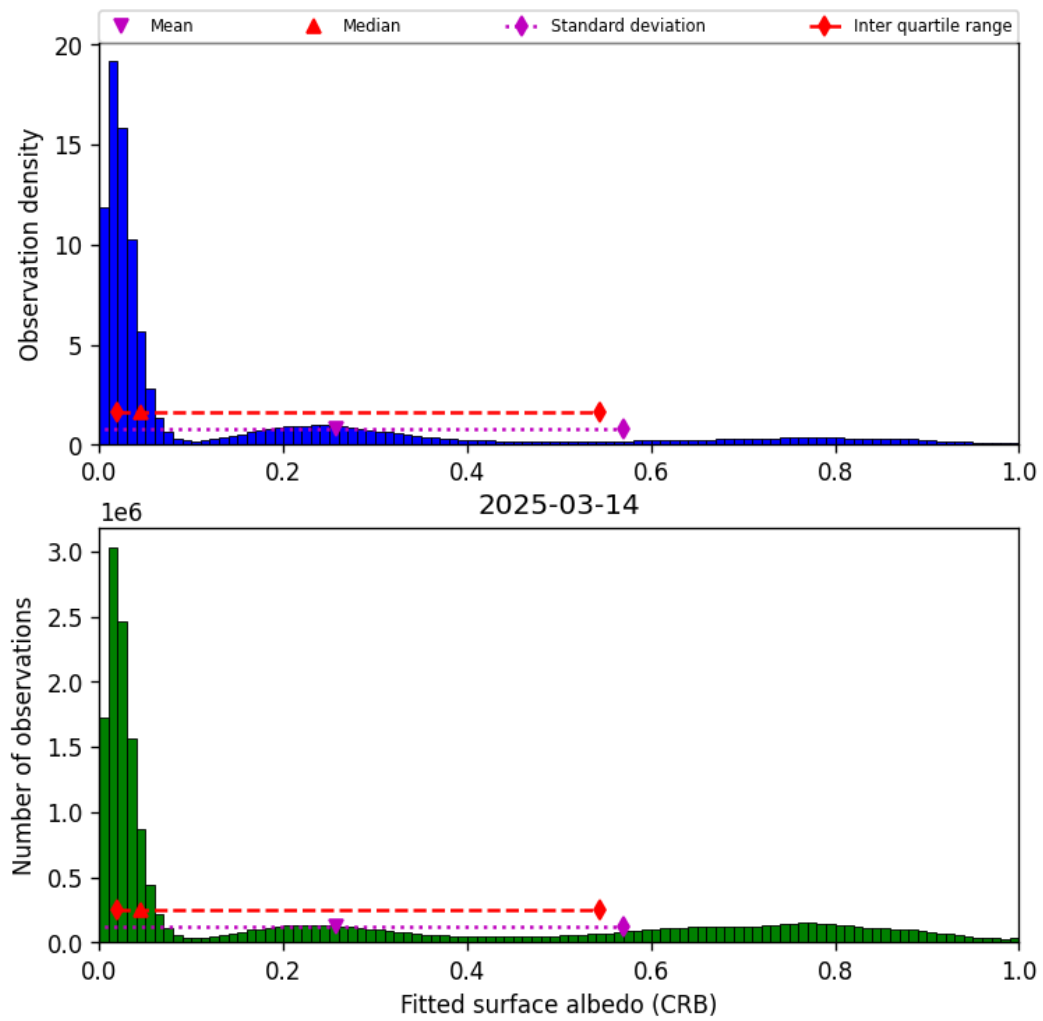
Figure 44: Histogram of “Fitted surface albedo (CRB)” for 2025-03-14 to 2025-03-15
