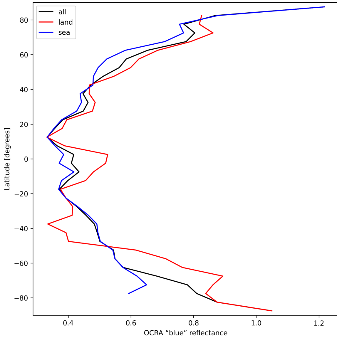
Figure 33: Zonal average of “OCRA “blue” reflectance” for 2025-03-14 to 2025-03-15.
