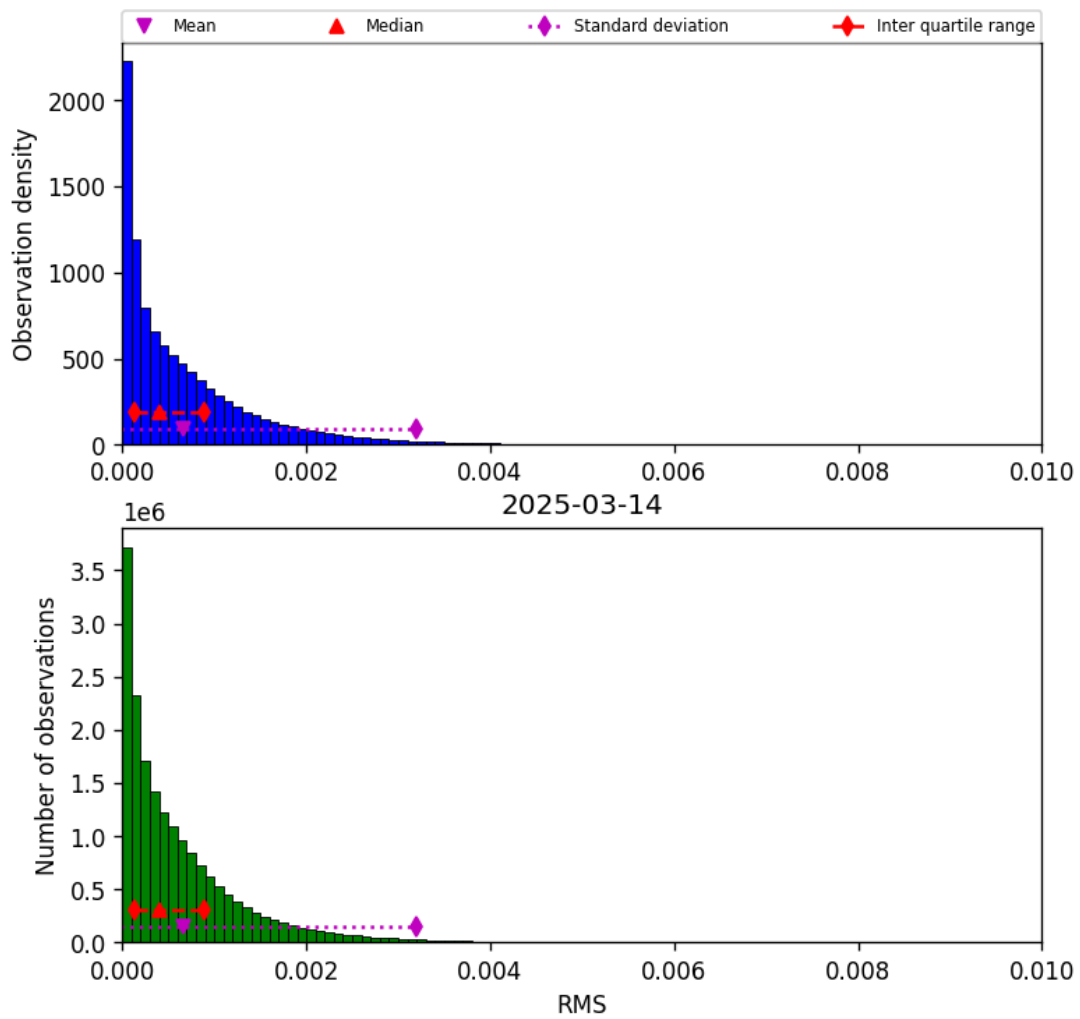
Figure 45: Histogram of “RMS” for 2025-03-14 to 2025-03-15
