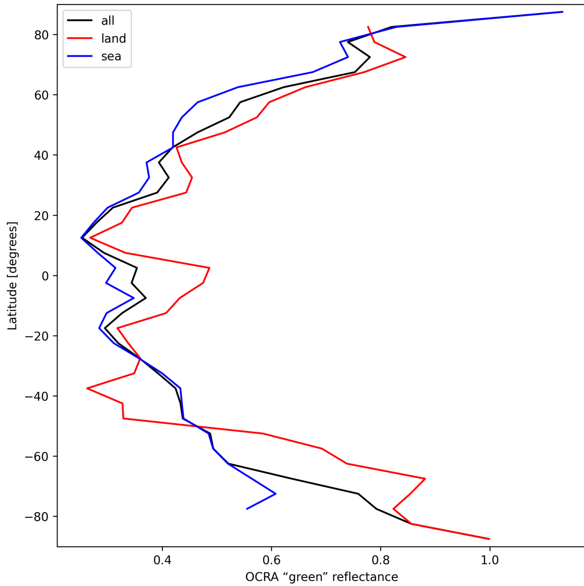
Figure 34: Zonal average of “OCRA “green” reflectance” for 2025-03-14 to 2025-03-15.
