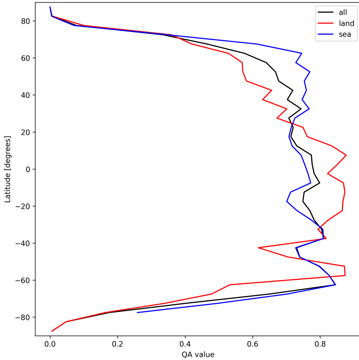
Figure 20: Zonal average of “QA value” for 2025-03-14 to 2025-03-15.
