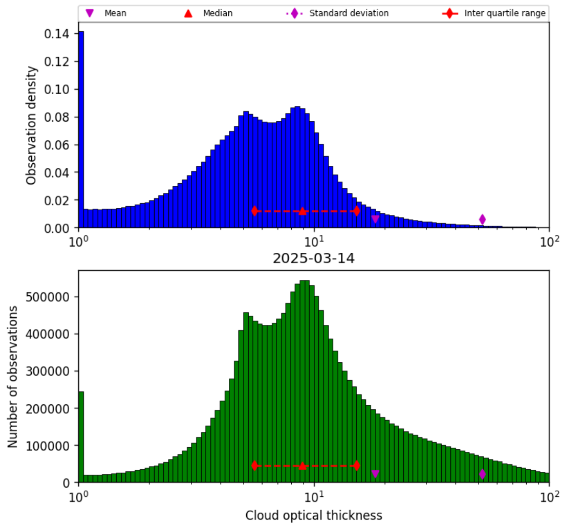
Figure 39: Histogram of “Cloud optical thickness” for 2025-03-14 to 2025-03-15
