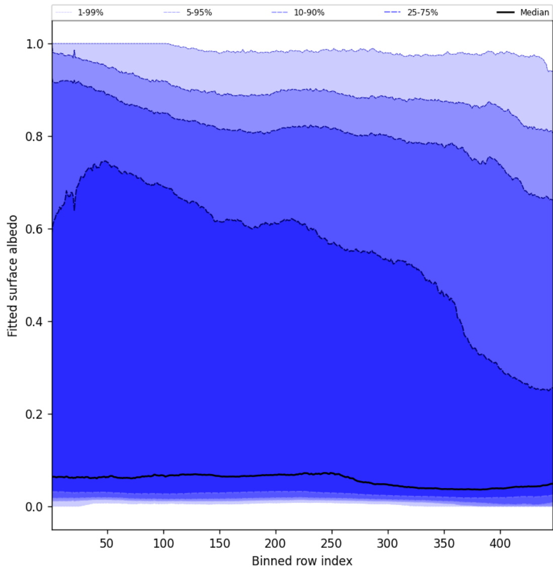
Figure 59: Along track statistics of “Fitted surface albedo” for 2025-03-14 to 2025-03-15
