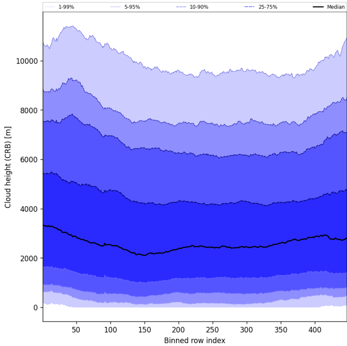
Figure 57: Along track statistics of “Cloud height (CRB)” for 2025-03-14 to 2025-03-15
