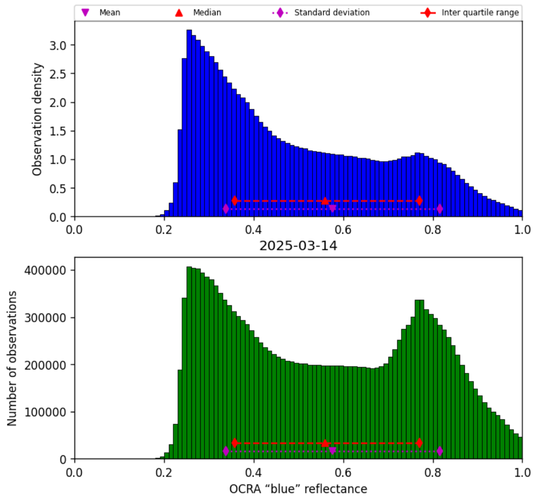
Figure 49: Histogram of “OCRA “blue” reflectance” for 2025-03-14 to 2025-03-15
