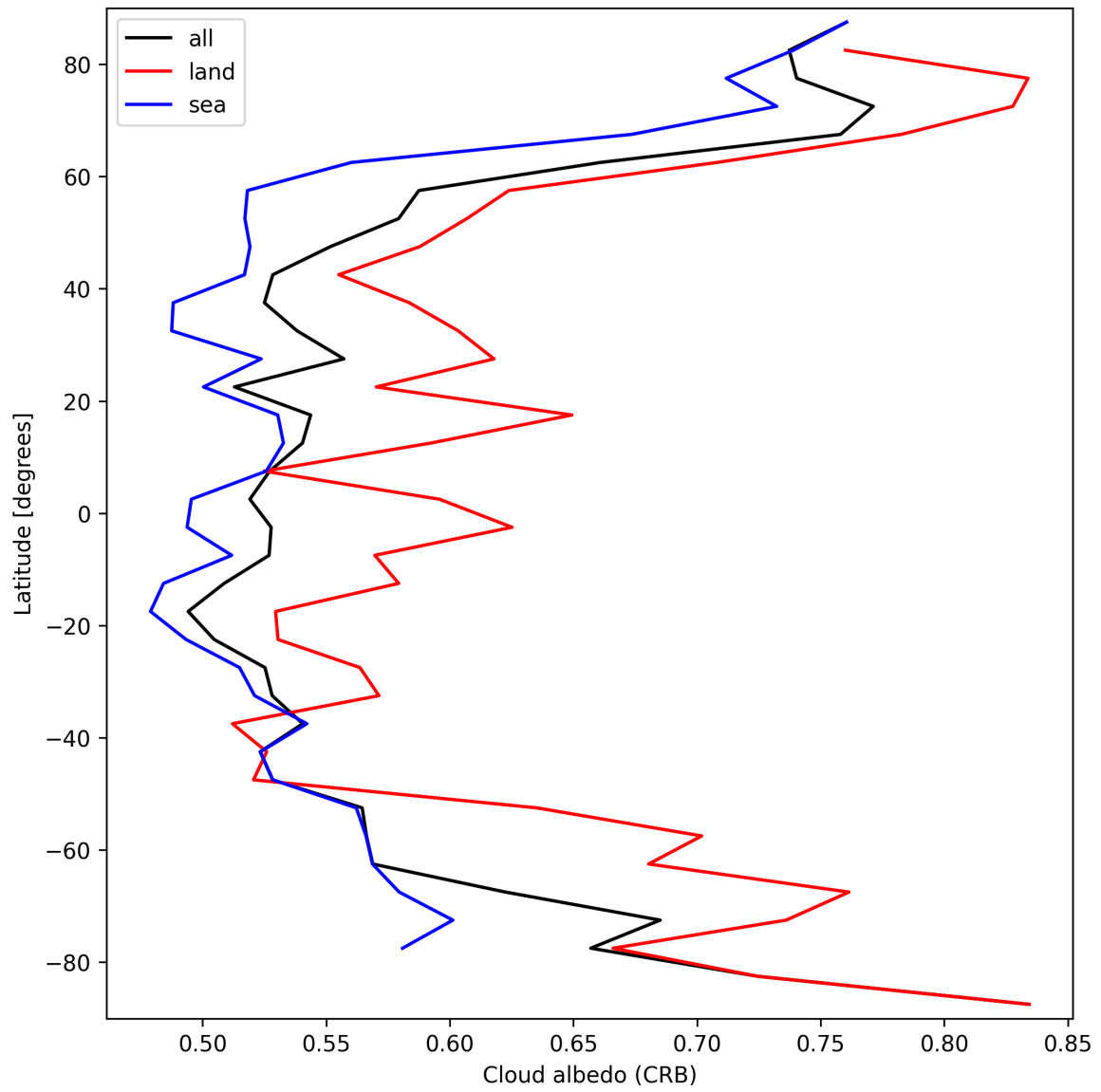
Figure 26: Zonal average of “Cloud albedo (CRB)” for 2025-03-14 to 2025-03-15.
