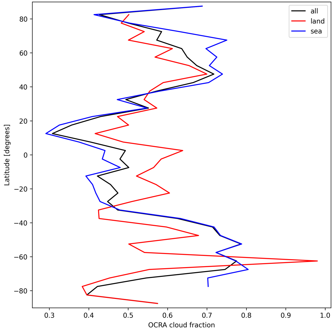
Figure 32: Zonal average of “OCRA cloud fraction” for 2025-03-17 to 2025-03-18.
