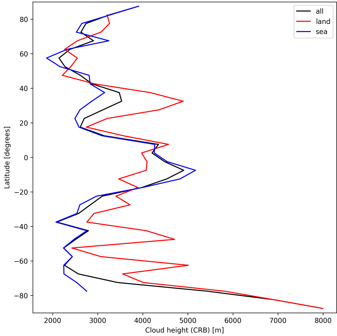
Figure 25: Zonal average of “Cloud height (CRB)” for 2025-03-17 to 2025-03-18.
