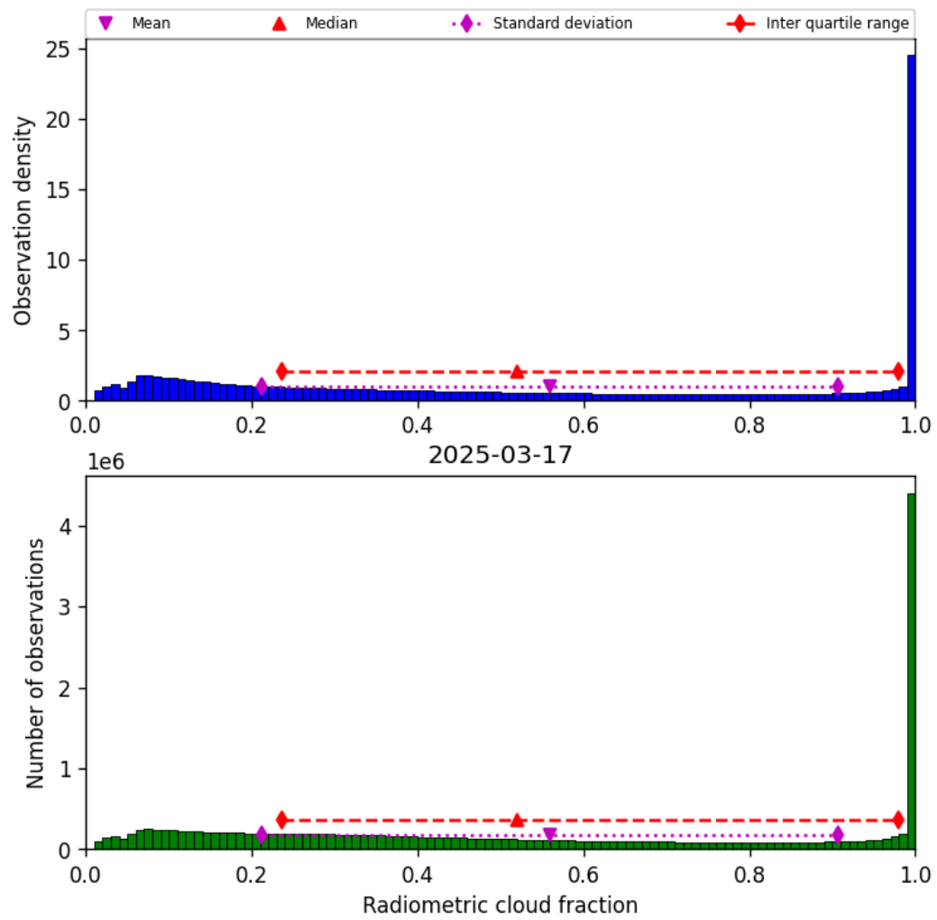
Figure 37: Histogram of “Radiometric cloud fraction” for 2025-03-17 to 2025-03-18
