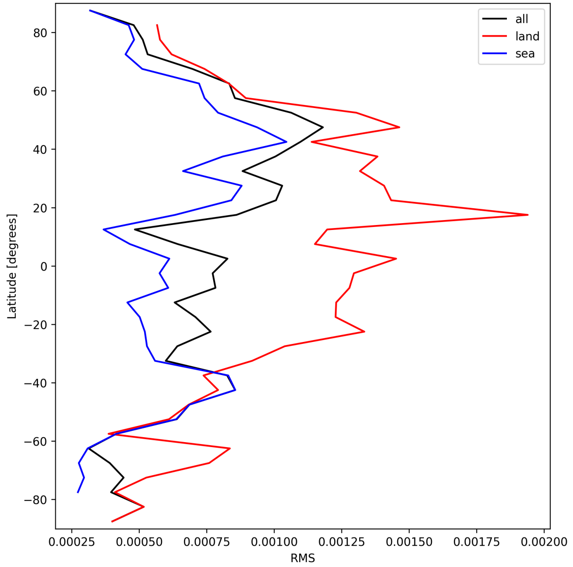
Figure 29: Zonal average of “RMS” for 2025-03-17 to 2025-03-18.
