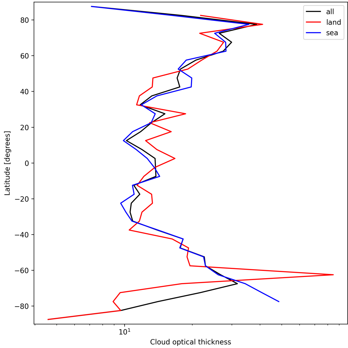
Figure 23: Zonal average of “Cloud optical thickness” for 2025-03-17 to 2025-03-18.
