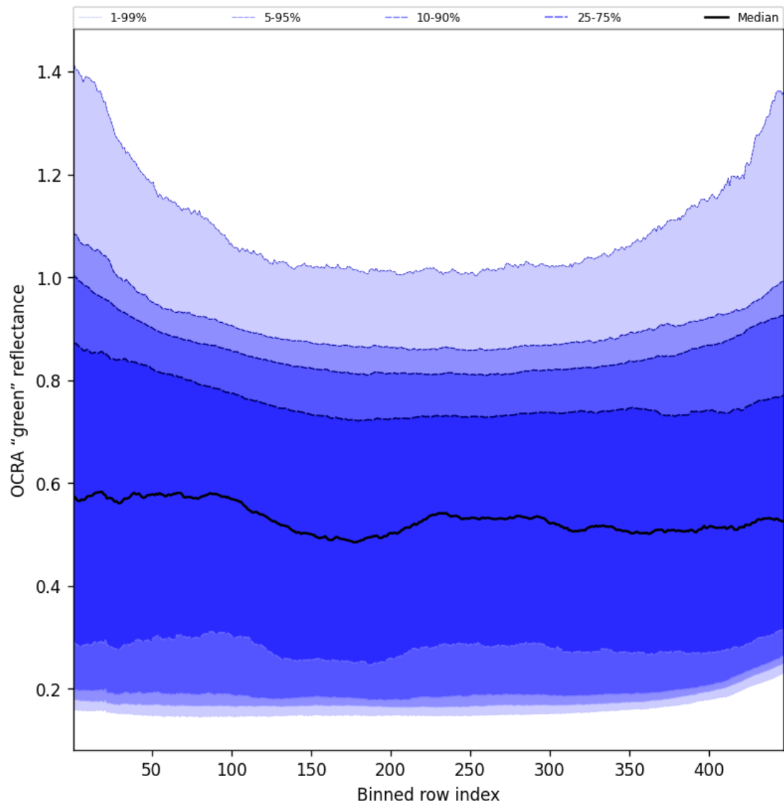
Figure 66: Along track statistics of “OCRA “green” reflectance” for 2025-03-17 to 2025-03-18
