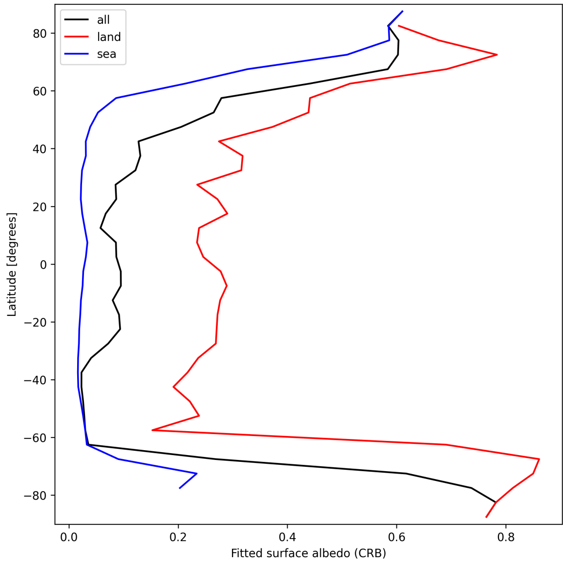
Figure 28: Zonal average of “Fitted surface albedo (CRB)” for 2025-03-17 to 2025-03-18.
