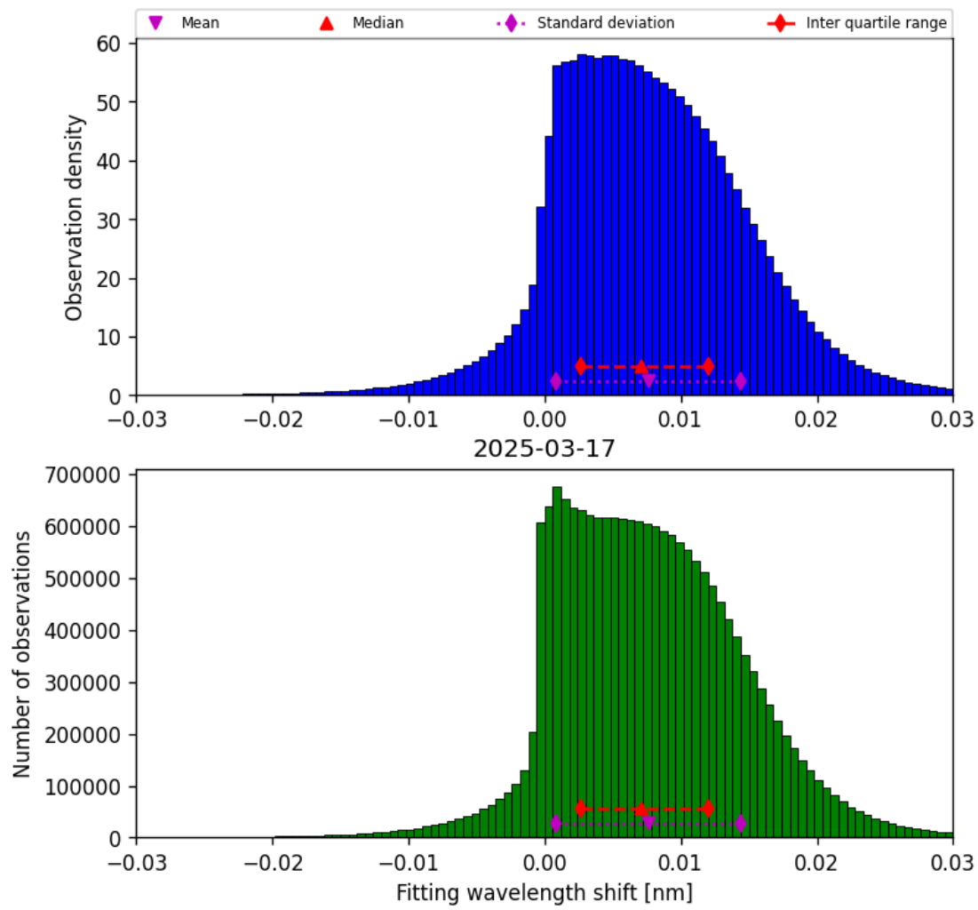
Figure 47: Histogram of “Fitting wavelength shift” for 2025-03-17 to 2025-03-18
