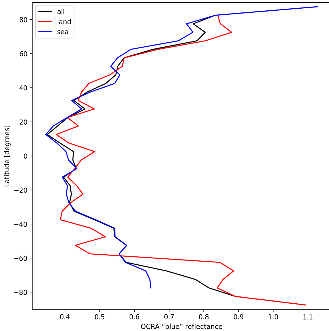
Figure 33: Zonal average of “OCRA “blue” reflectance” for 2025-03-17 to 2025-03-18.
