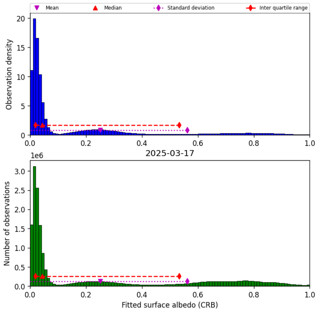
Figure 44: Histogram of “Fitted surface albedo (CRB)” for 2025-03-17 to 2025-03-18
