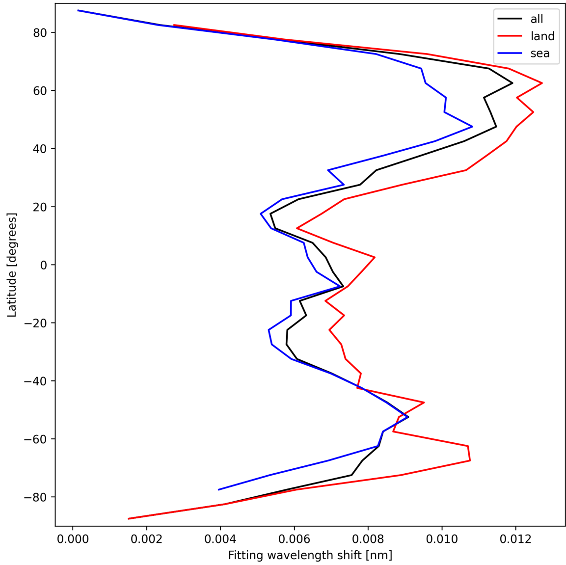
Figure 31: Zonal average of “Fitting wavelength shift” for 2025-03-17 to 2025-03-18.
