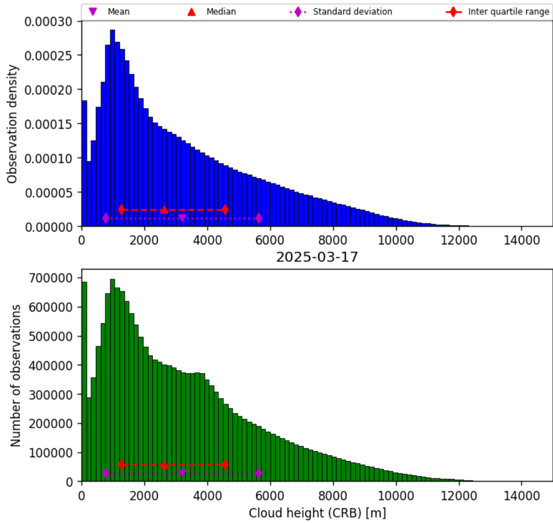
Figure 41: Histogram of “Cloud height (CRB)” for 2025-03-17 to 2025-03-18
