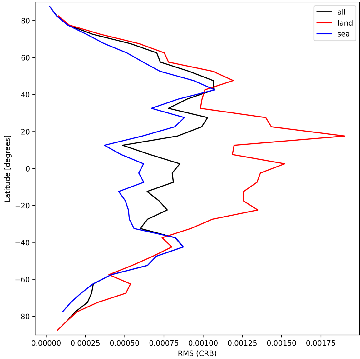
Figure 30: Zonal average of “RMS (CRB)” for 2025-03-17 to 2025-03-18.
