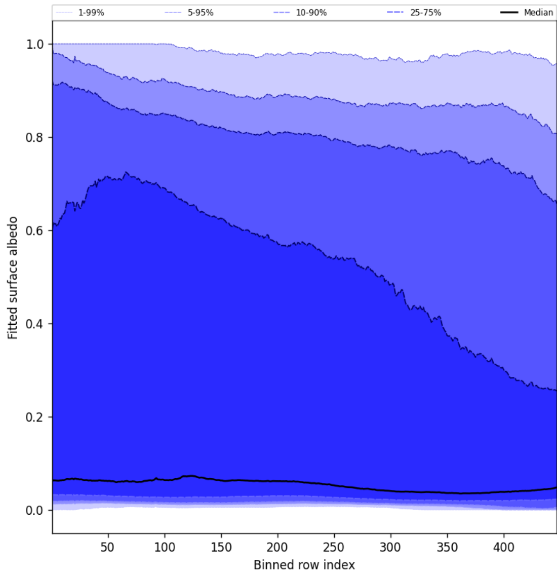
Figure 59: Along track statistics of “Fitted surface albedo” for 2025-03-17 to 2025-03-18
