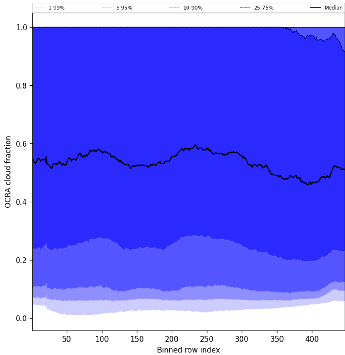
Figure 64: Along track statistics of “OCRA cloud fraction” for 2025-03-17 to 2025-03-18
