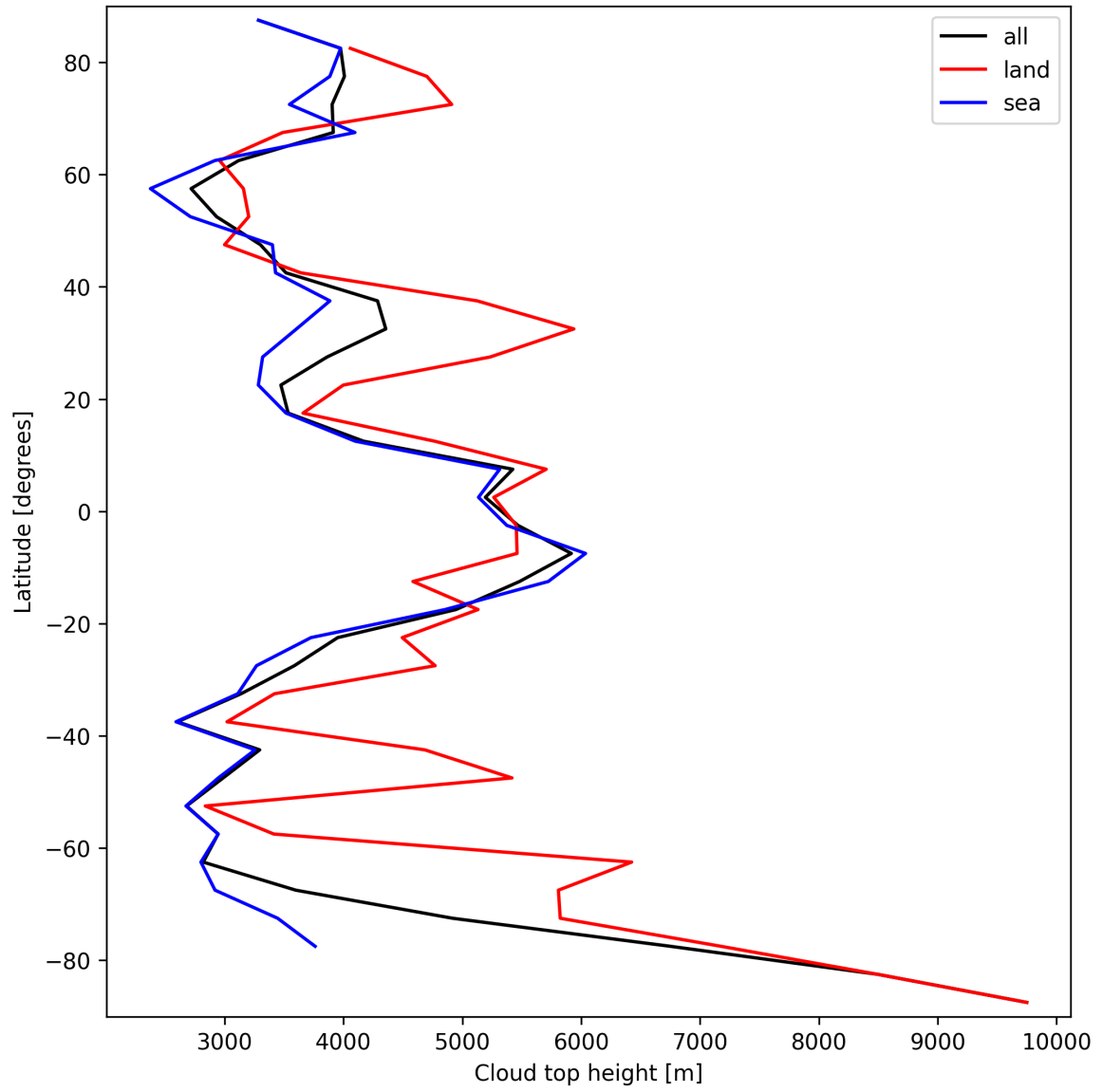
Figure 22: Zonal average of “Cloud top height” for 2025-03-17 to 2025-03-18.
