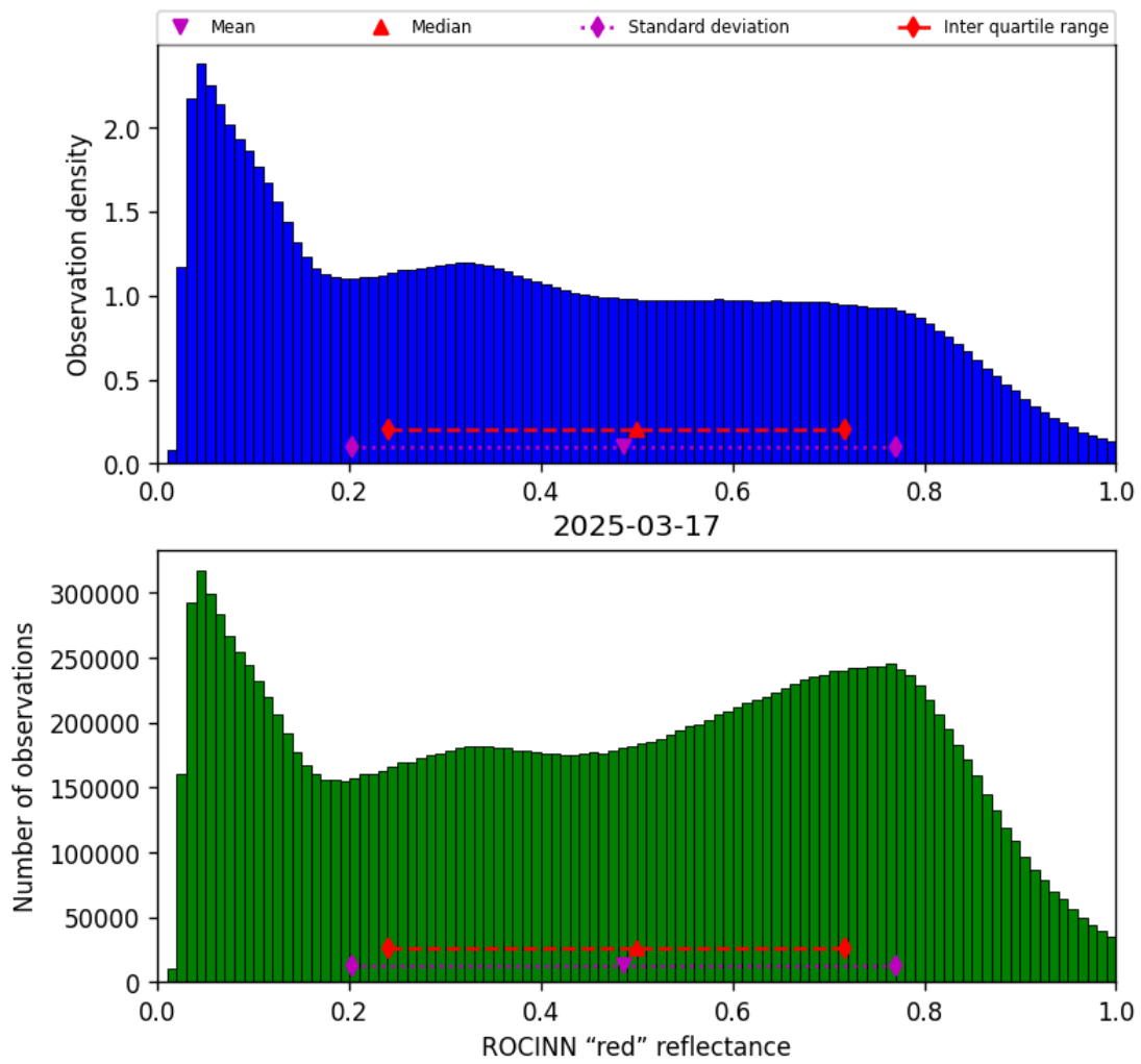
Figure 51: Histogram of "ROCINN "red" reflectance" for 2025-03-17 to 2025-03-18
