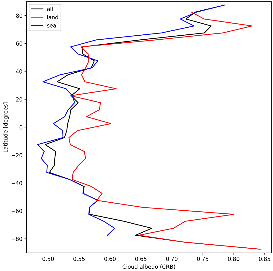
Figure 26: Zonal average of “Cloud albedo (CRB)” for 2025-03-17 to 2025-03-18.
