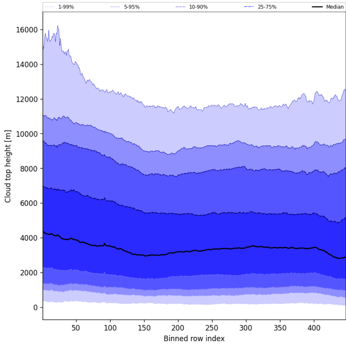
Figure 54: Along track statistics of “Cloud top height” for 2025-03-17 to 2025-03-18
