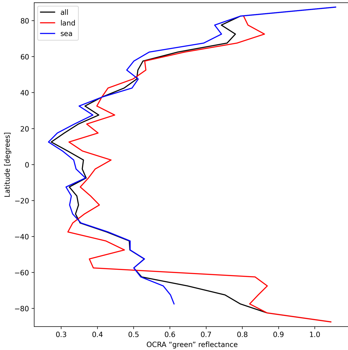
Figure 34: Zonal average of “OCRA “green” reflectance” for 2025-03-17 to 2025-03-18.
