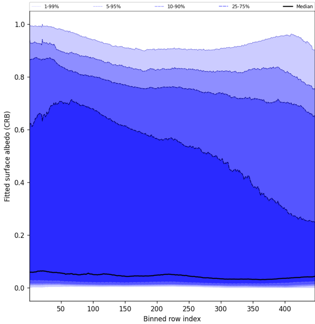
Figure 60: Along track statistics of “Fitted surface albedo (CRB)” for 2025-03-17 to 2025-03-18
