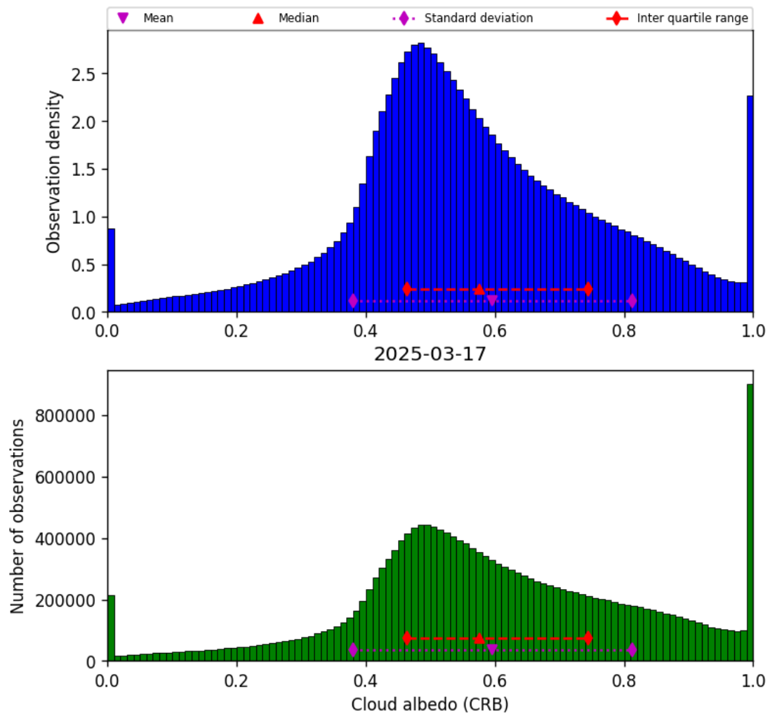
Figure 42: Histogram of “Cloud albedo (CRB)” for 2025-03-17 to 2025-03-18
