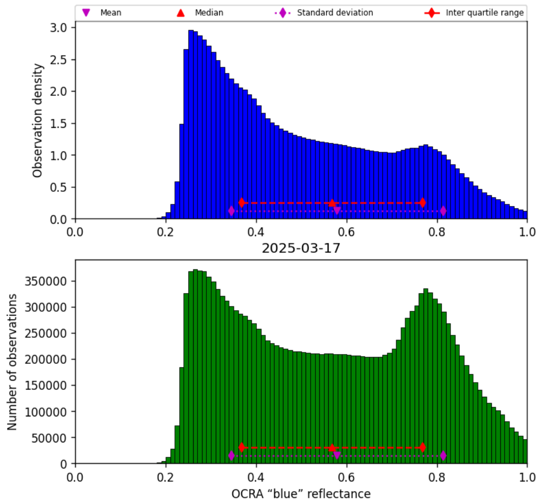
Figure 49: Histogram of “OCRA “blue” reflectance” for 2025-03-17 to 2025-03-18
