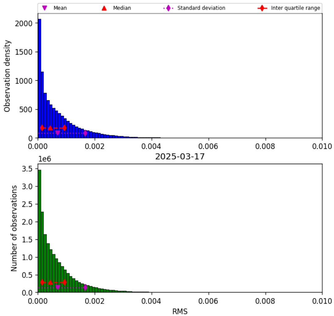
Figure 45: Histogram of “RMS” for 2025-03-17 to 2025-03-18
