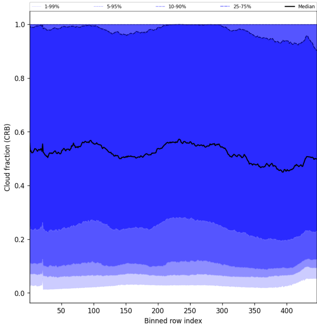
Figure 56: Along track statistics of “Cloud fraction (CRB)” for 2025-03-17 to 2025-03-18
