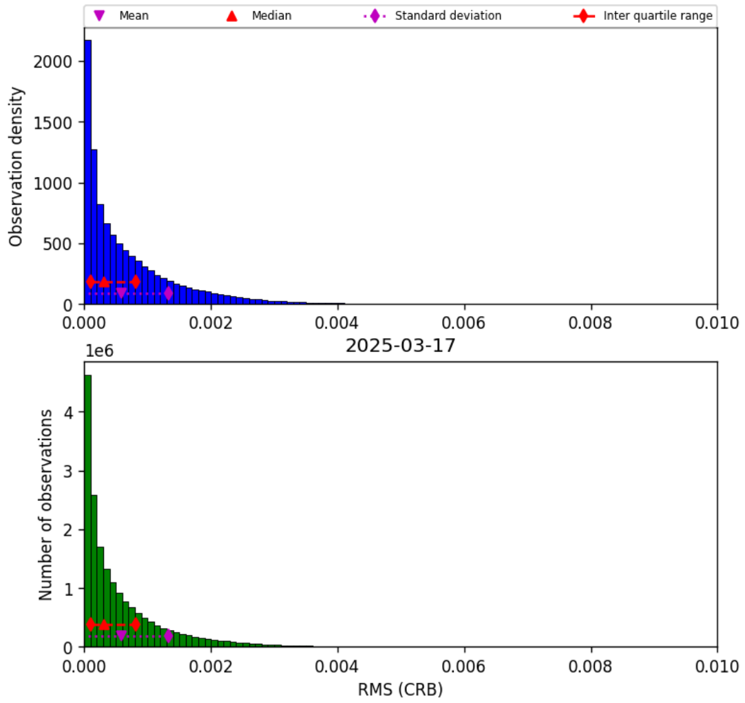
Figure 46: Histogram of "RMS (CRB)" for 2025-03-17 to 2025-03-18
