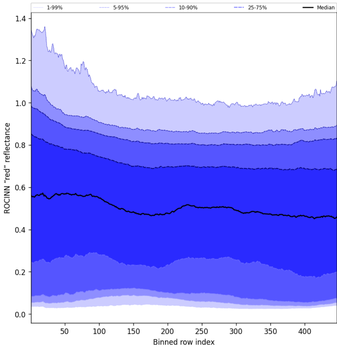
Figure 67: Along track statistics of "ROCINN "red" reflectance" for 2025-03-17 to 2025-03-18
