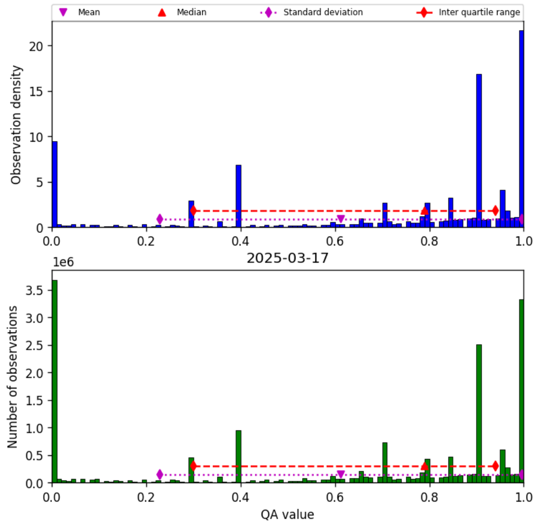
Figure 36: Histogram of “QA value” for 2025-03-17 to 2025-03-18
