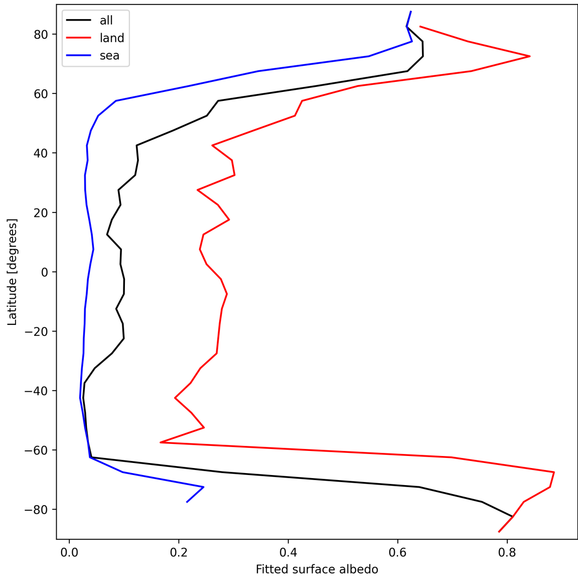
Figure 27: Zonal average of “Fitted surface albedo” for 2025-03-17 to 2025-03-18.
