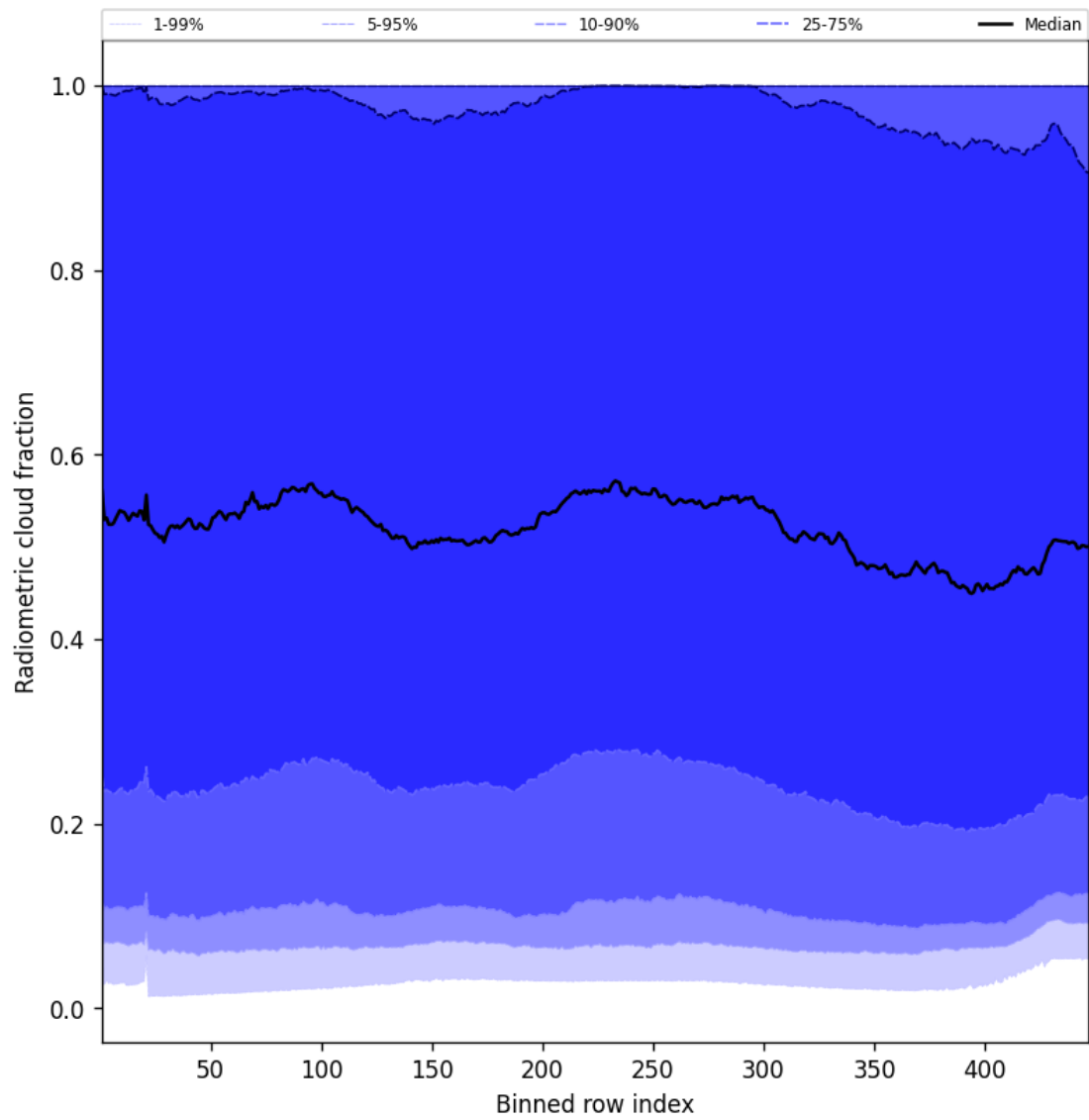
Figure 53: Along track statistics of “Radiometric cloud fraction” for 2025-03-17 to 2025-03-18
