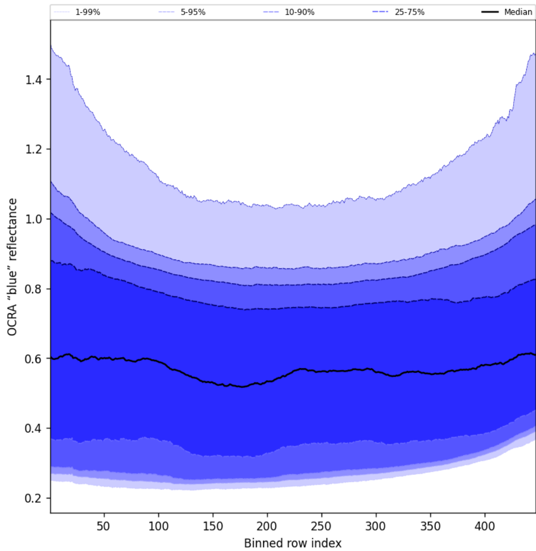
Figure 65: Along track statistics of “OCRA “blue” reflectance” for 2025-03-17 to 2025-03-18
