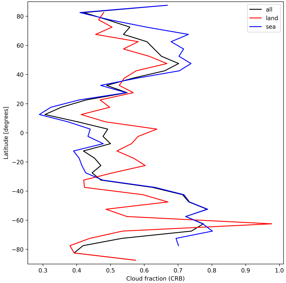
Figure 24: Zonal average of “Cloud fraction (CRB)” for 2025-03-17 to 2025-03-18.
