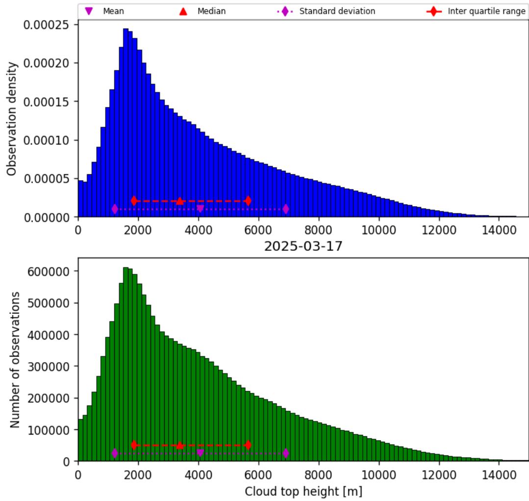
Figure 38: Histogram of “Cloud top height” for 2025-03-17 to 2025-03-18
