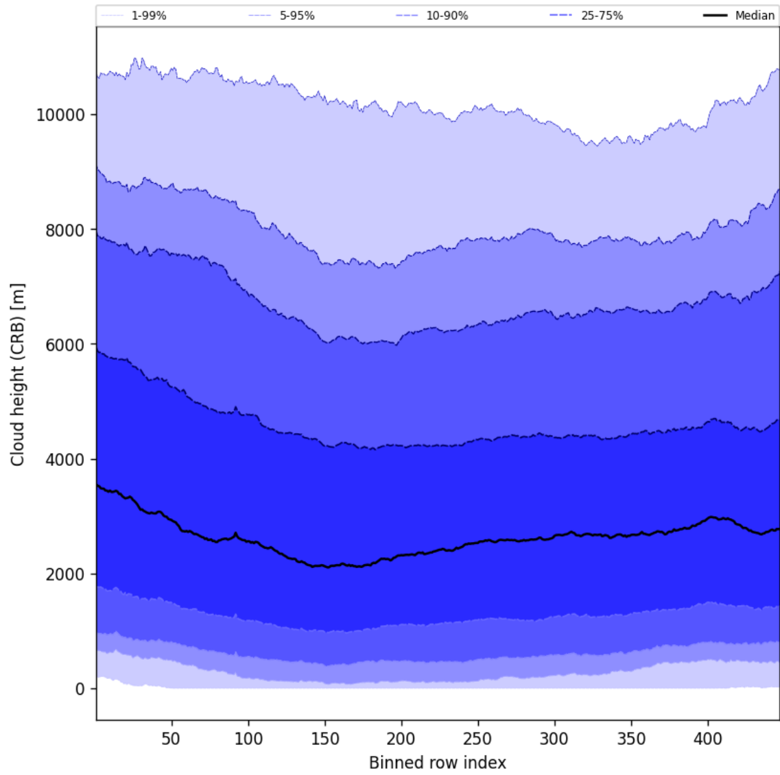
Figure 57: Along track statistics of “Cloud height (CRB)” for 2025-03-17 to 2025-03-18
