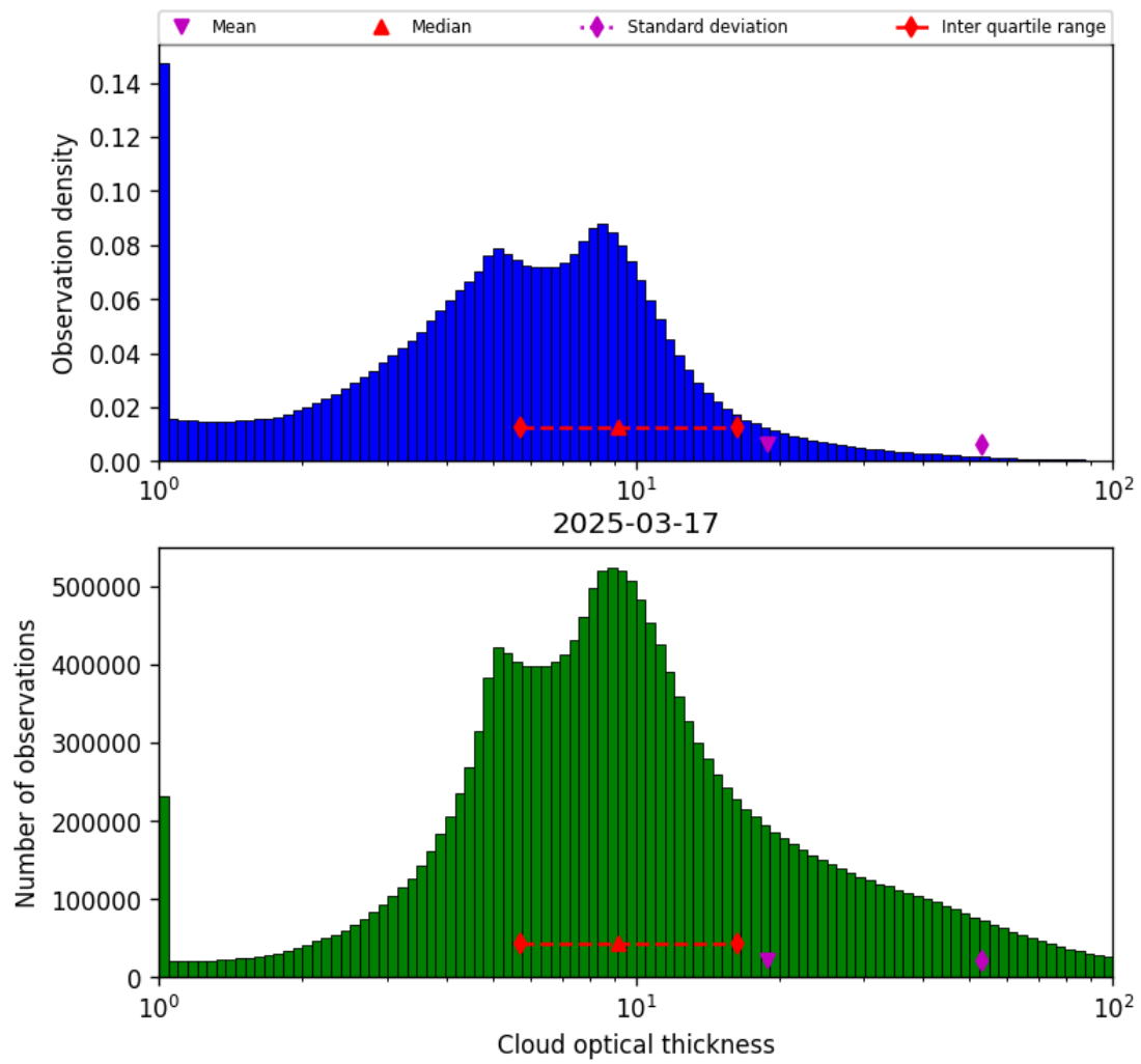
Figure 39: Histogram of “Cloud optical thickness” for 2025-03-17 to 2025-03-18
