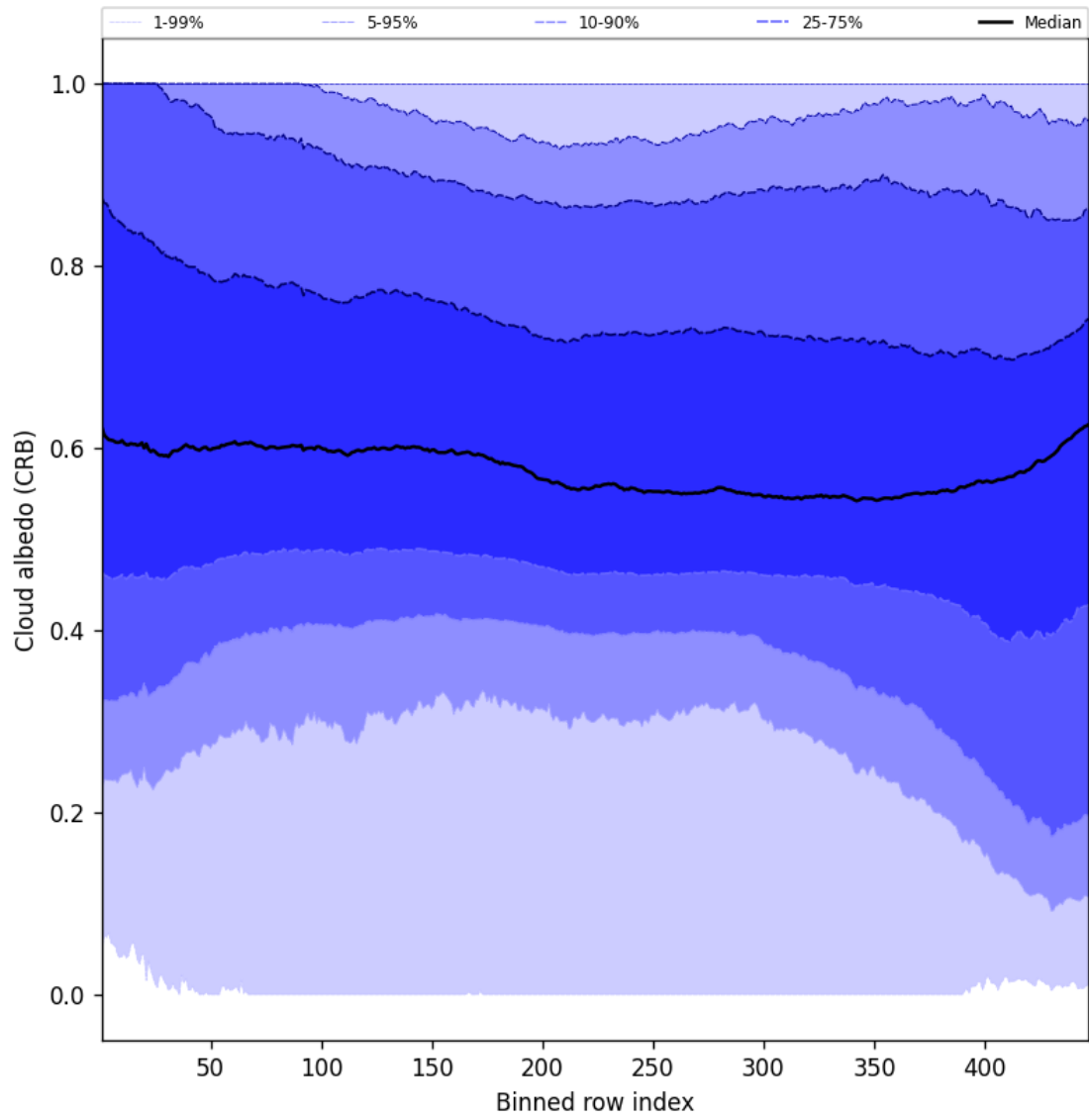
Figure 58: Along track statistics of “Cloud albedo (CRB)” for 2025-03-17 to 2025-03-18
