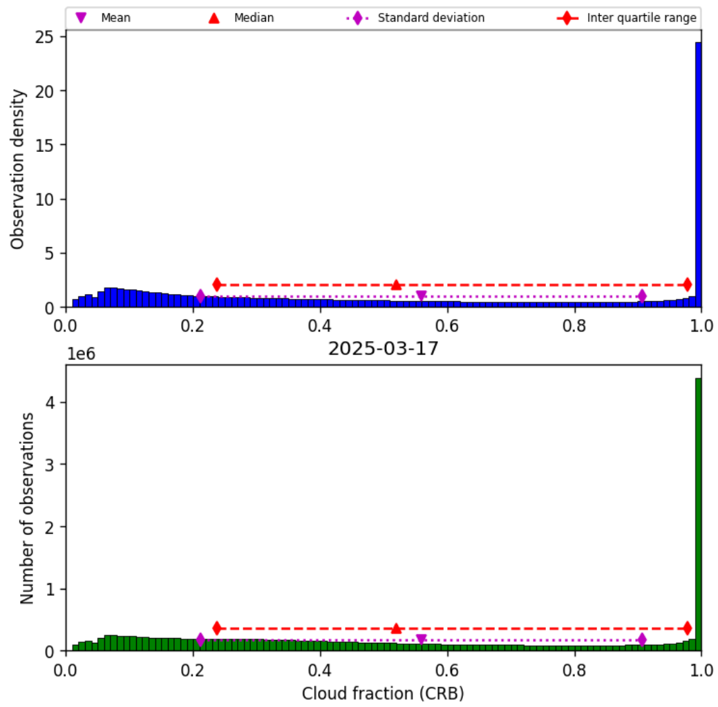
Figure 40: Histogram of “Cloud fraction (CRB)” for 2025-03-17 to 2025-03-18
