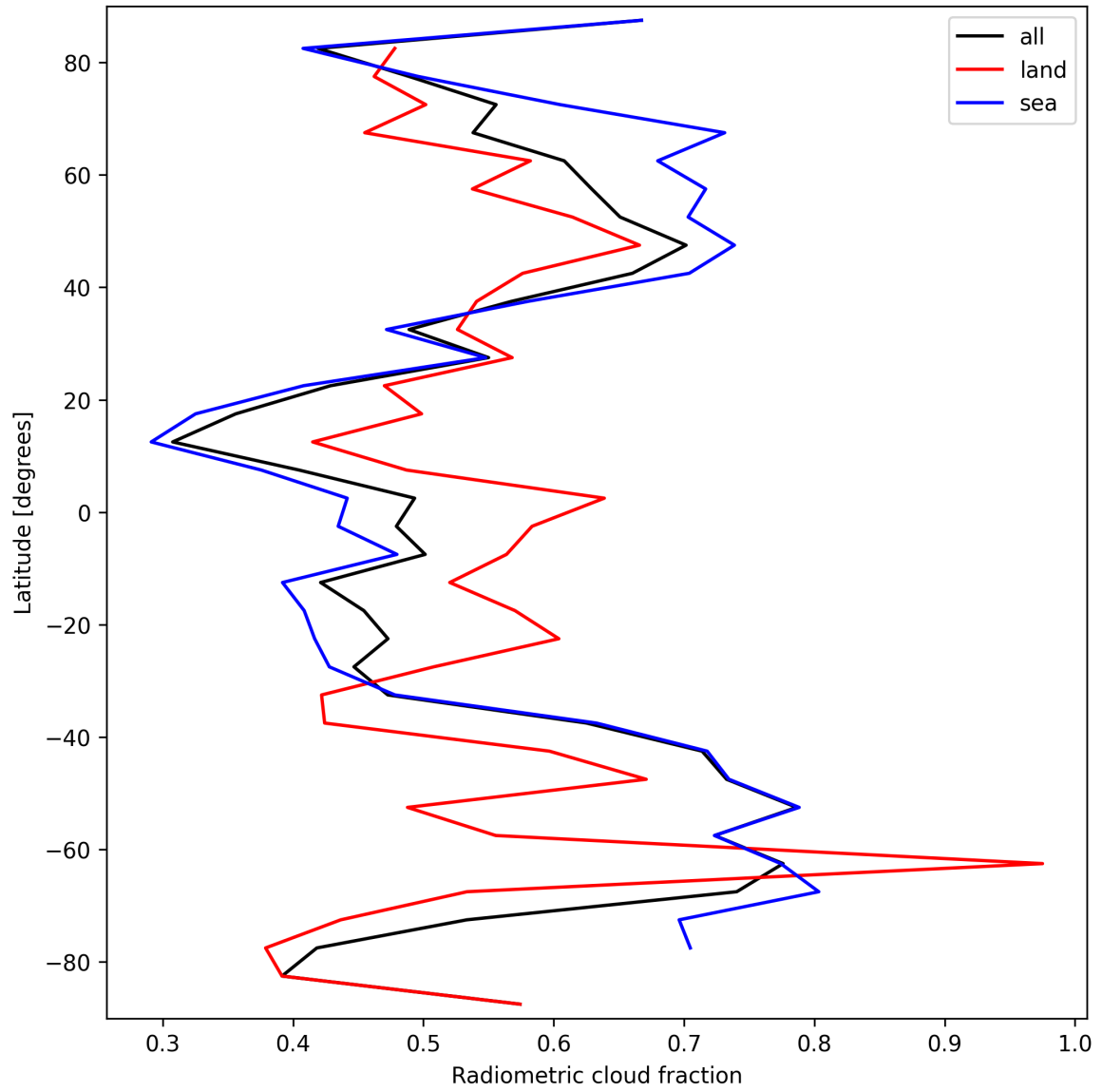
Figure 21: Zonal average of “Radiometric cloud fraction” for 2025-03-17 to 2025-03-18.
