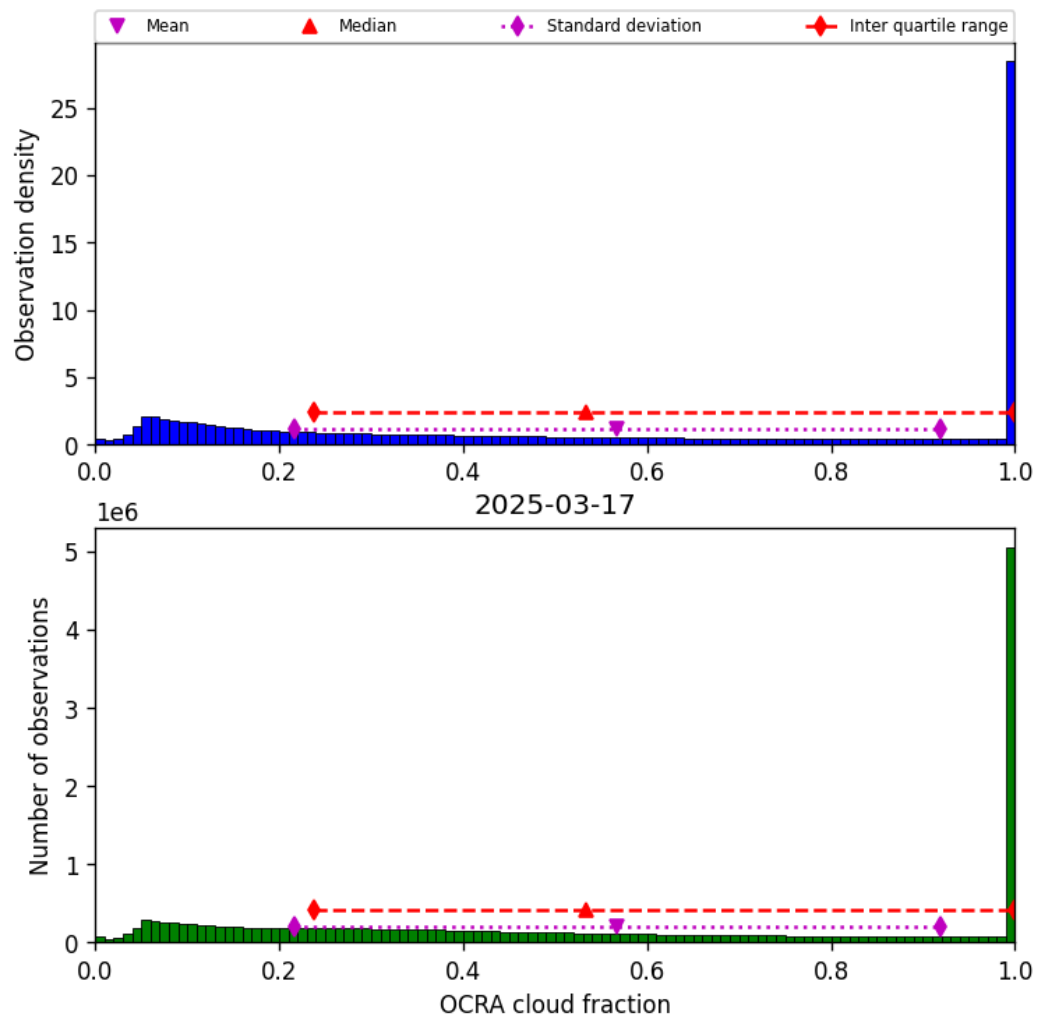
Figure 48: Histogram of “OCRA cloud fraction” for 2025-03-17 to 2025-03-18
