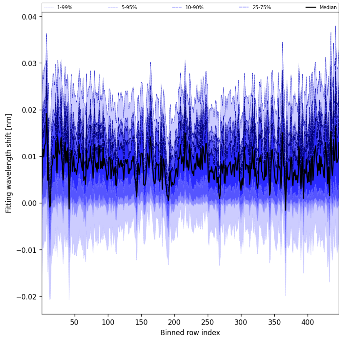
Figure 63: Along track statistics of “Fitting wavelength shift” for 2025-03-17 to 2025-03-18
