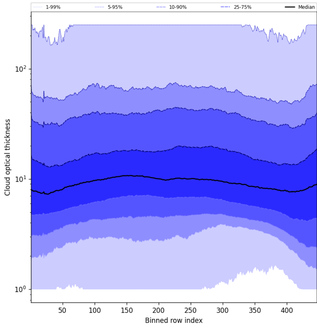
Figure 55: Along track statistics of “Cloud optical thickness” for 2025-03-17 to 2025-03-18
