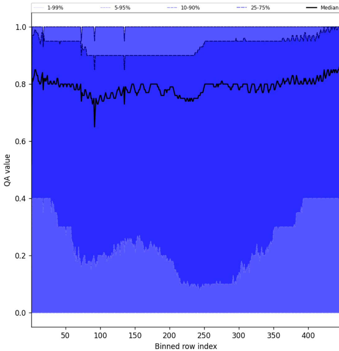
Figure 52: Along track statistics of “QA value” for 2025-03-17 to 2025-03-18
