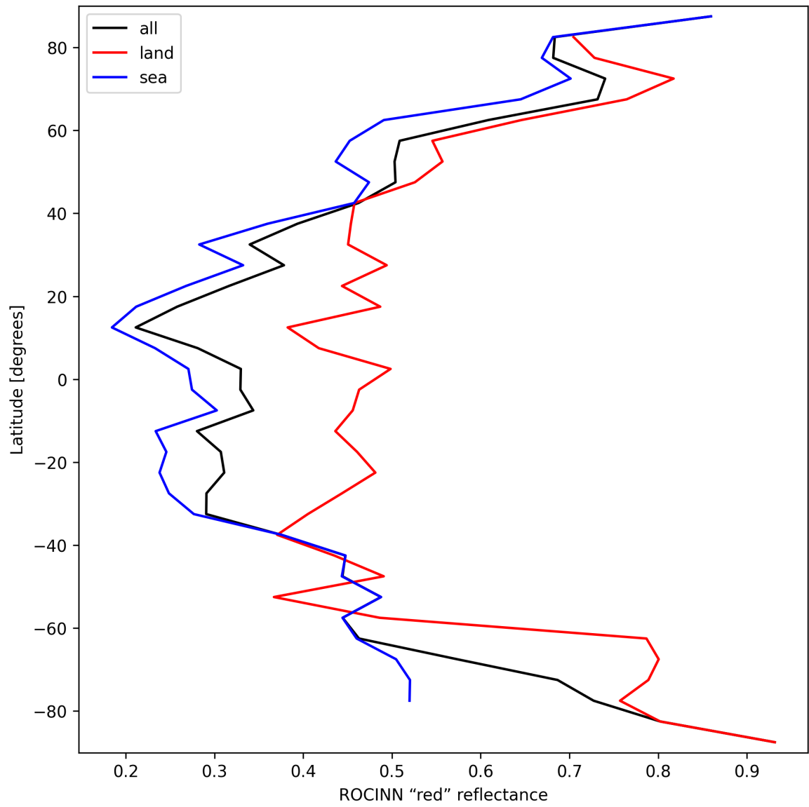
Figure 35: Zonal average of “ROCINN “red” reflectance” for 2025-03-17 to 2025-03-18.
