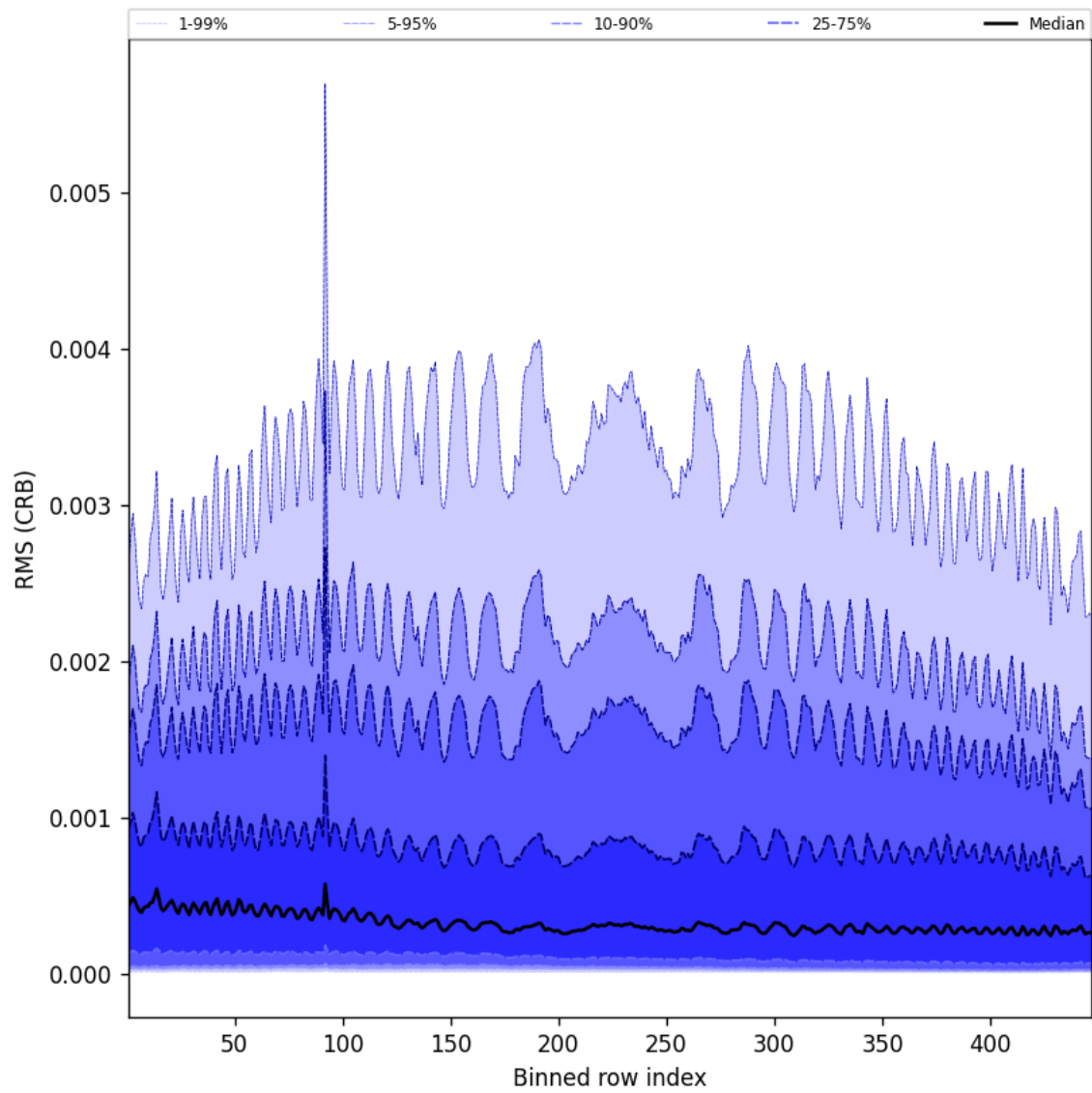
Figure 62: Along track statistics of “RMS (CRB)” for 2025-03-17 to 2025-03-18
