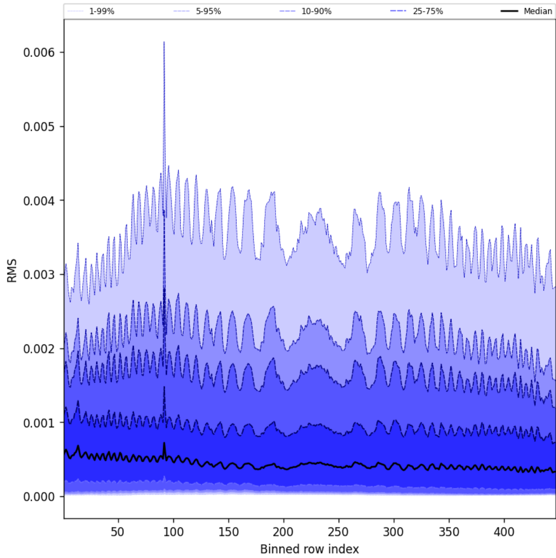
Figure 61: Along track statistics of “RMS” for 2025-03-17 to 2025-03-18
