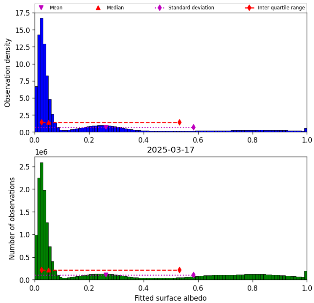
Figure 43: Histogram of “Fitted surface albedo” for 2025-03-17 to 2025-03-18
