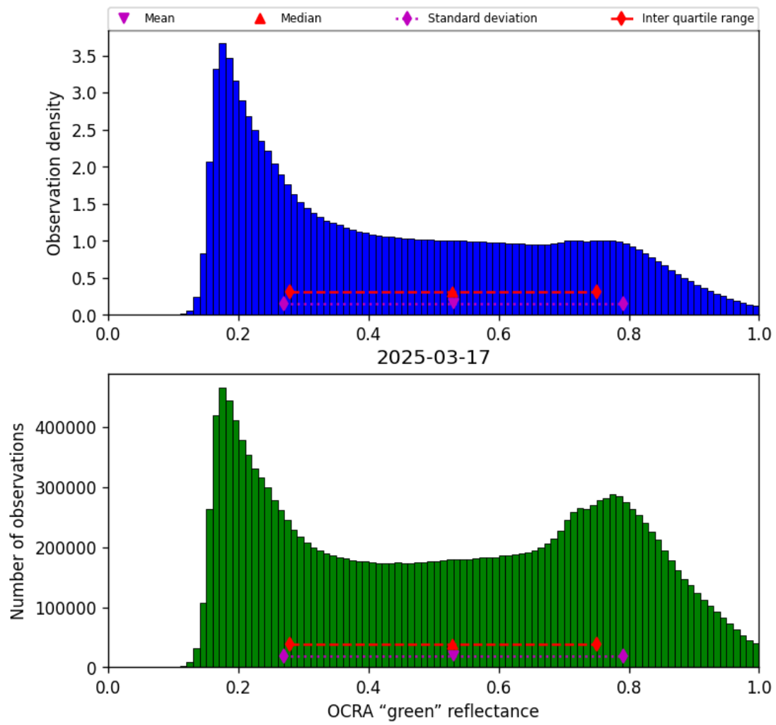
Figure 50: Histogram of “OCRA “green” reflectance” for 2025-03-17 to 2025-03-18
