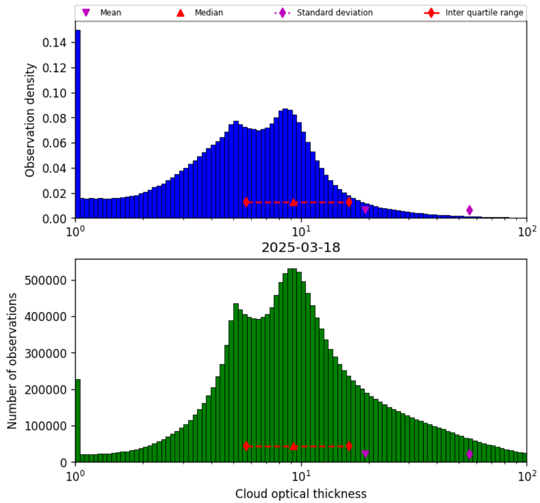
Figure 39: Histogram of “Cloud optical thickness” for 2025-03-18 to 2025-03-19
