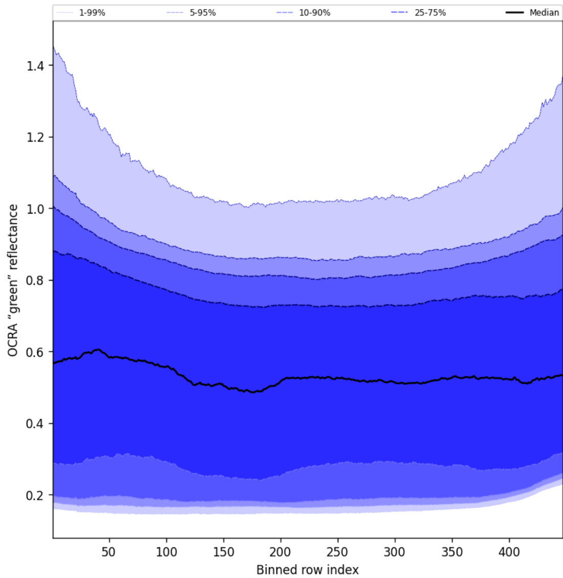
Figure 66: Along track statistics of “OCRA “green” reflectance” for 2025-03-18 to 2025-03-19
