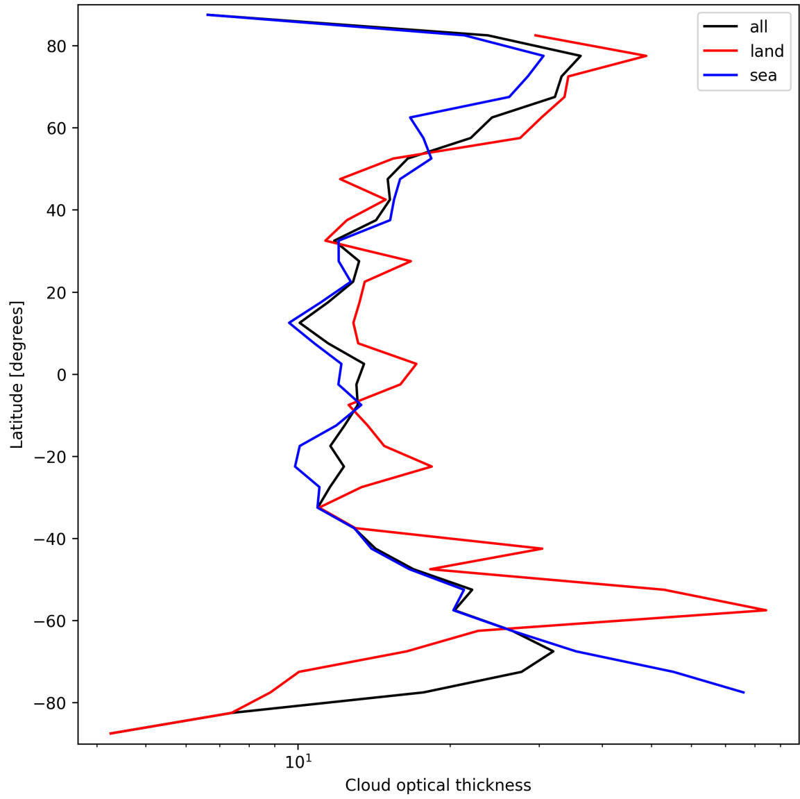
Figure 23: Zonal average of “Cloud optical thickness” for 2025-03-18 to 2025-03-19.
