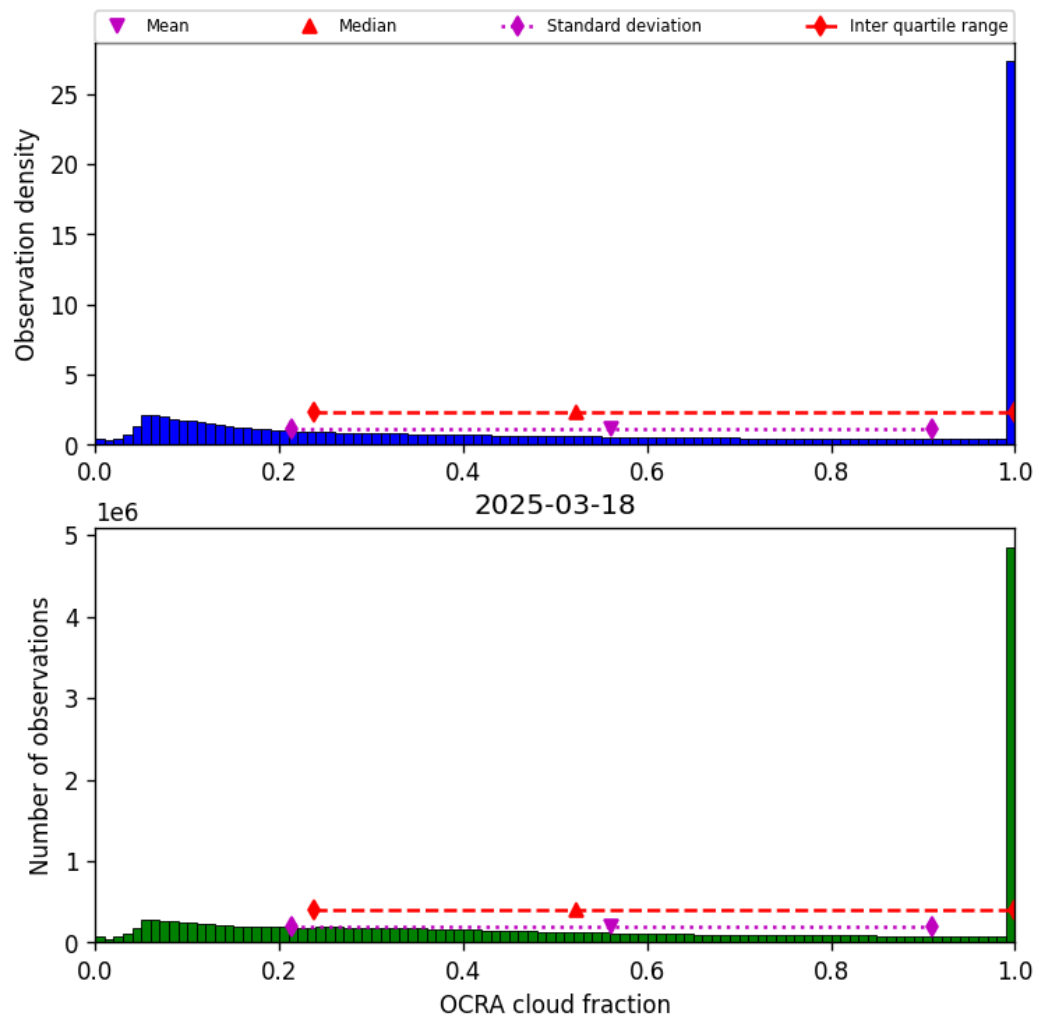
Figure 48: Histogram of “OCRA cloud fraction” for 2025-03-18 to 2025-03-19
