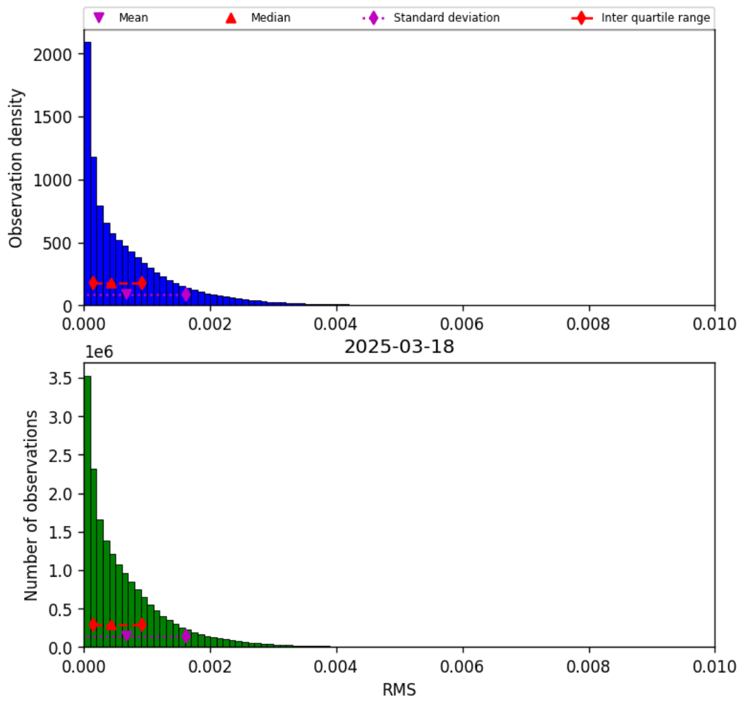
Figure 45: Histogram of “RMS” for 2025-03-18 to 2025-03-19
