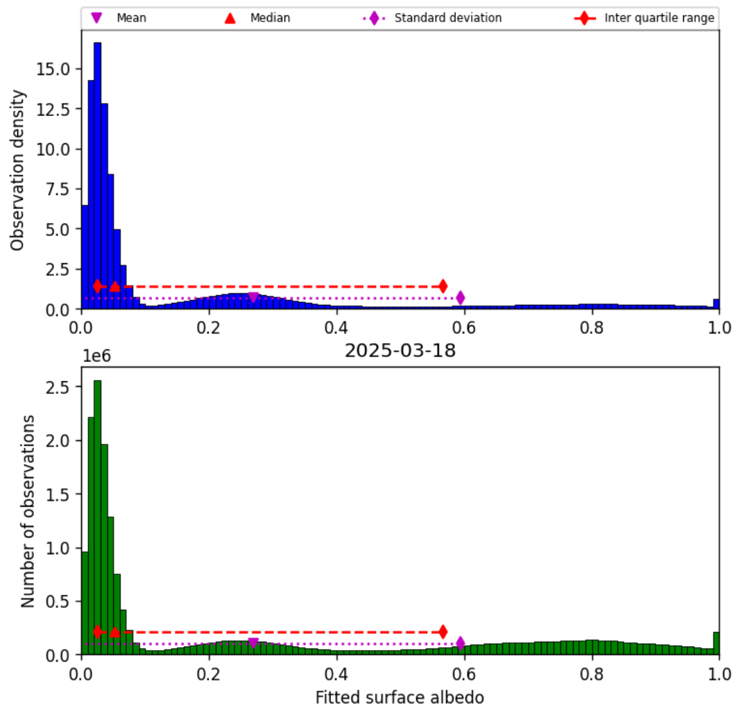
Figure 43: Histogram of “Fitted surface albedo” for 2025-03-18 to 2025-03-19
