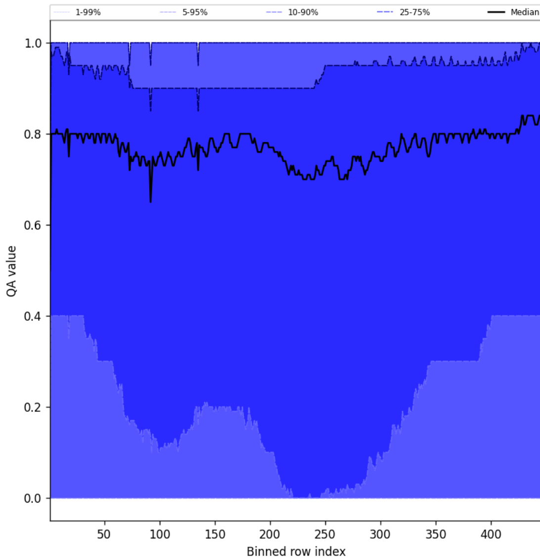
Figure 52: Along track statistics of “QA value” for 2025-03-18 to 2025-03-19
