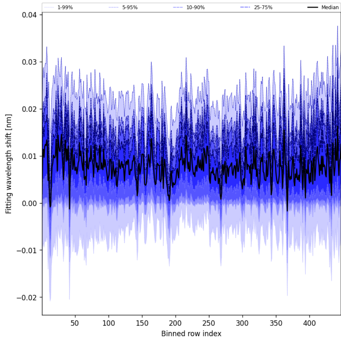
Figure 63: Along track statistics of “Fitting wavelength shift” for 2025-03-18 to 2025-03-19
