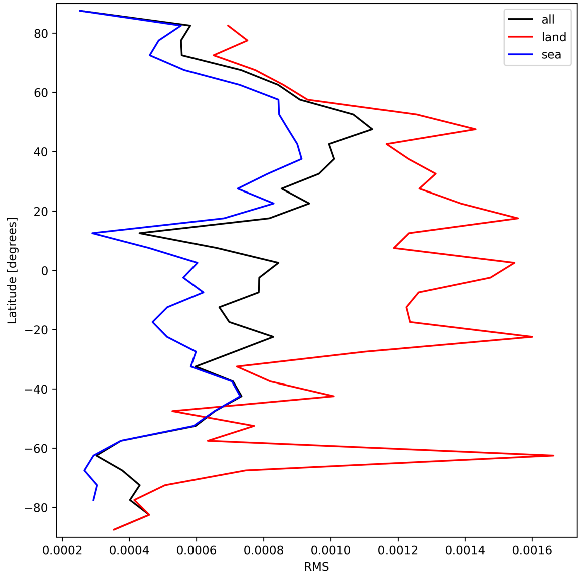
Figure 29: Zonal average of “RMS” for 2025-03-18 to 2025-03-19.
