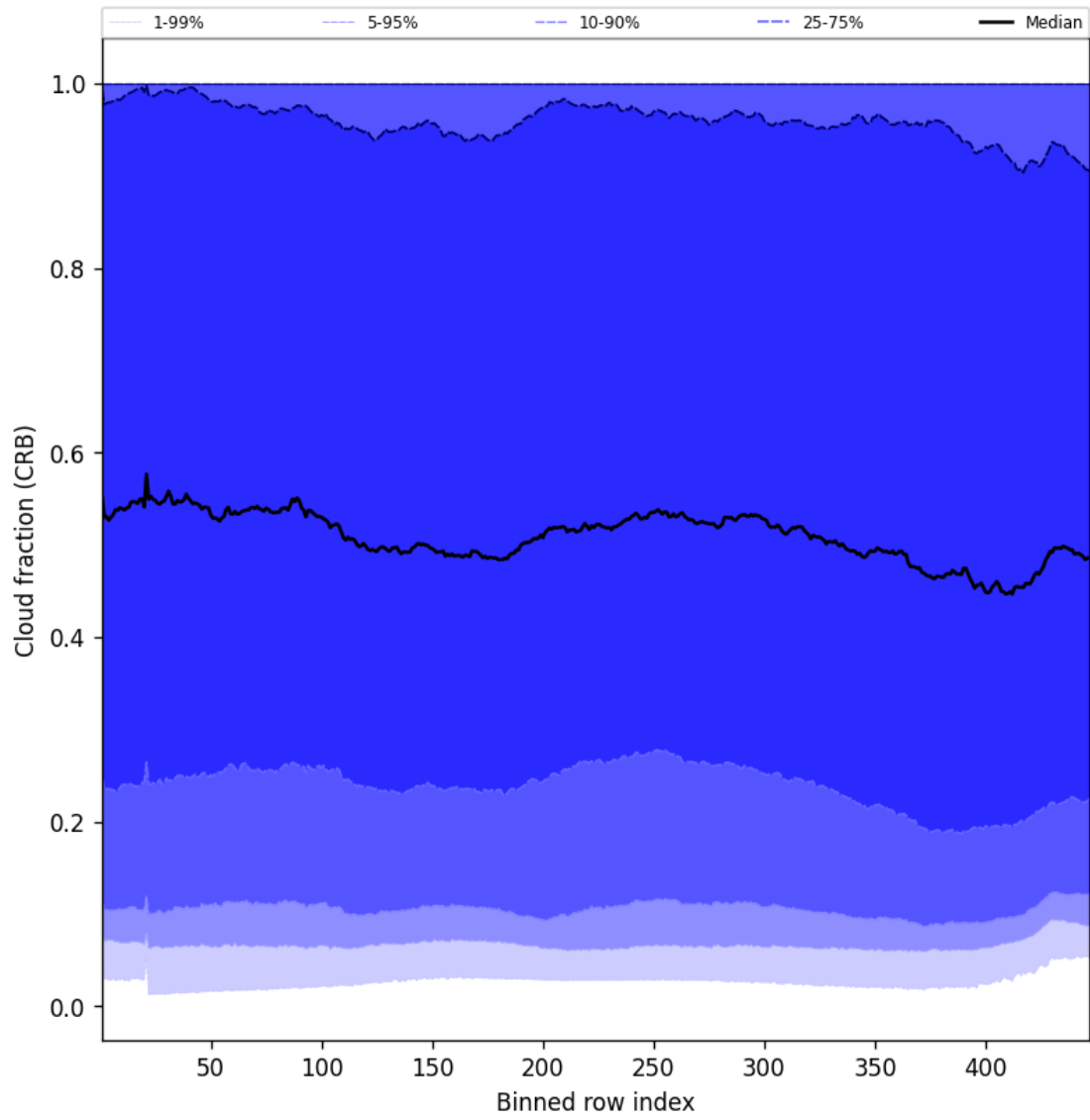
Figure 56: Along track statistics of “Cloud fraction (CRB)” for 2025-03-18 to 2025-03-19
