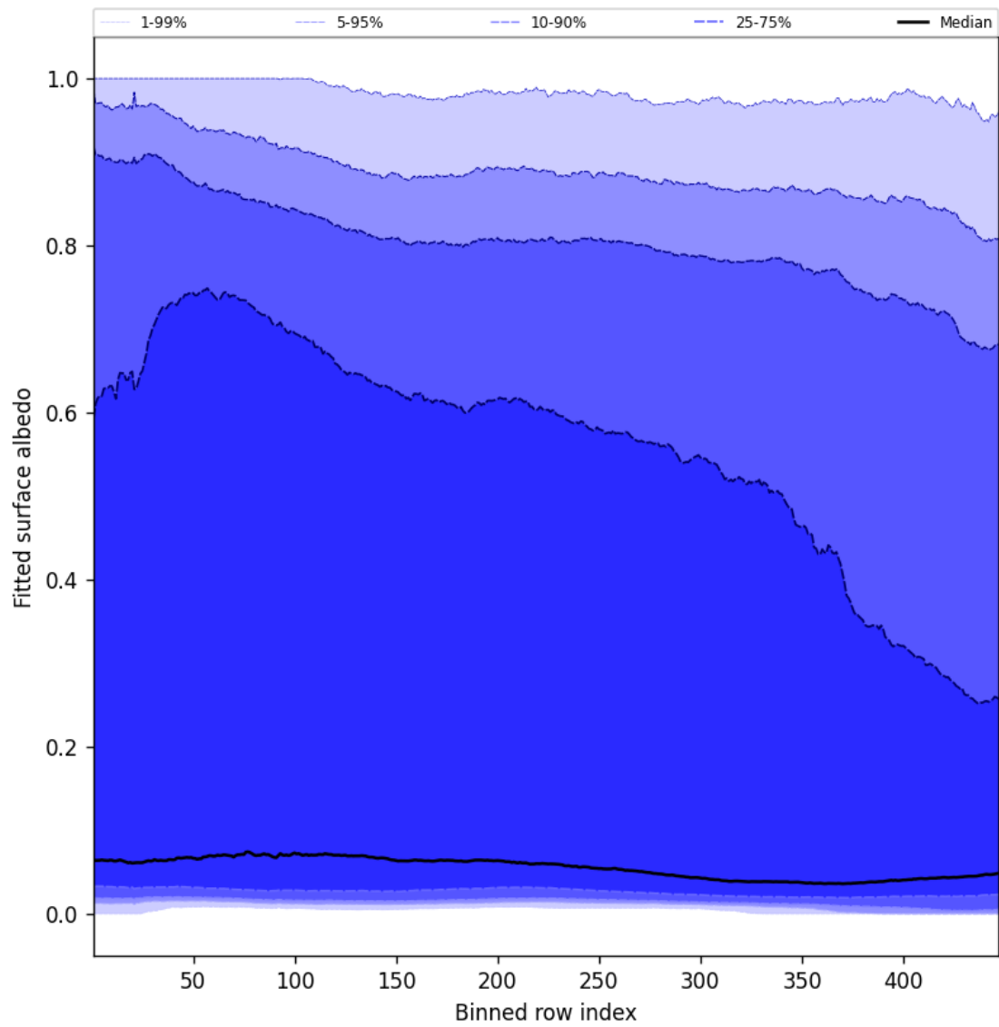
Figure 59: Along track statistics of “Fitted surface albedo” for 2025-03-18 to 2025-03-19
