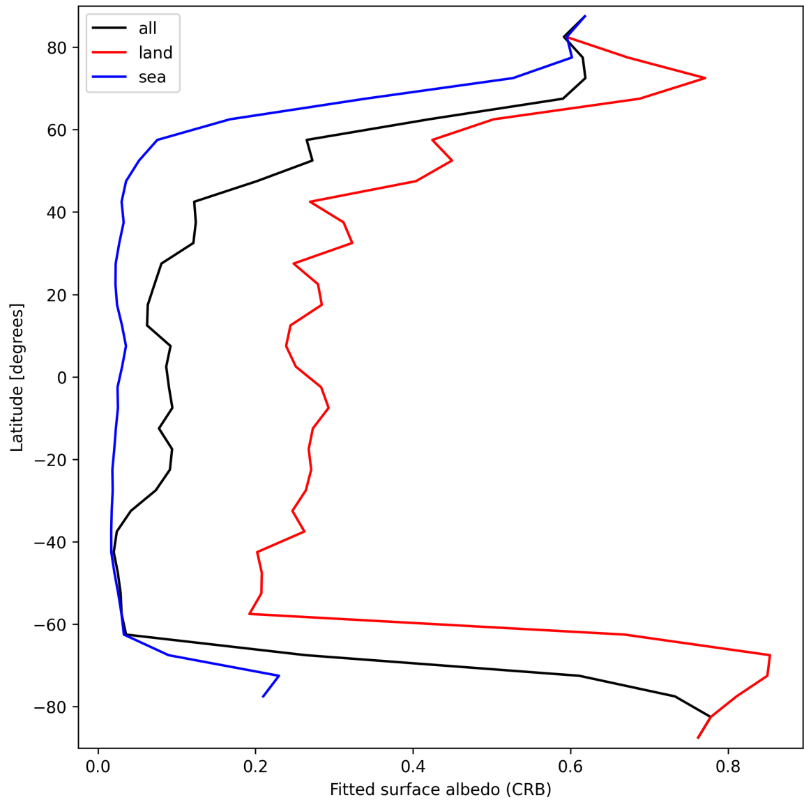
Figure 28: Zonal average of “Fitted surface albedo (CRB)” for 2025-03-18 to 2025-03-19.
