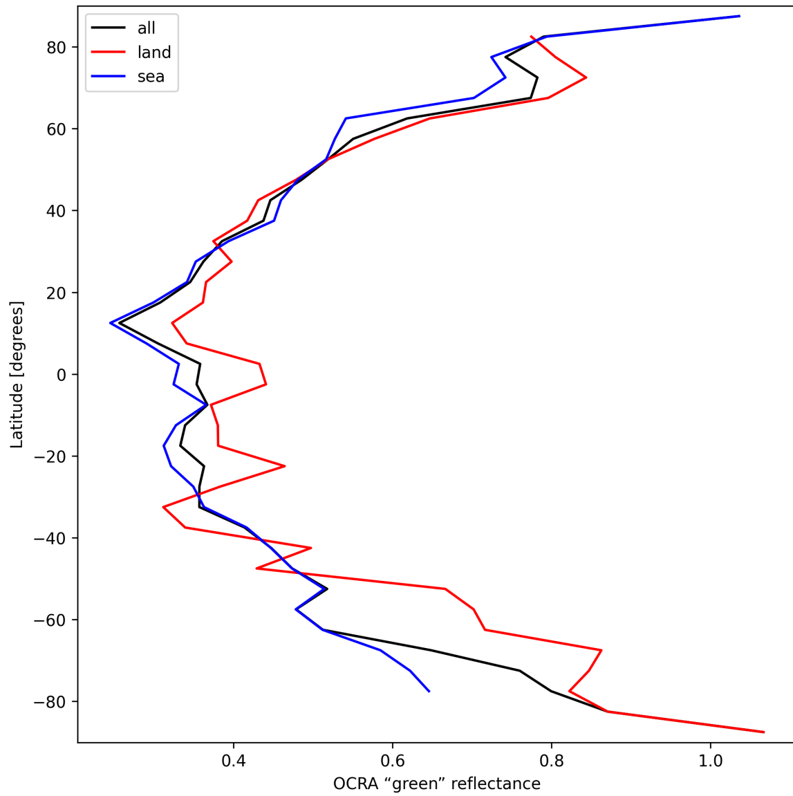
Figure 34: Zonal average of “OCRA “green” reflectance” for 2025-03-18 to 2025-03-19.
