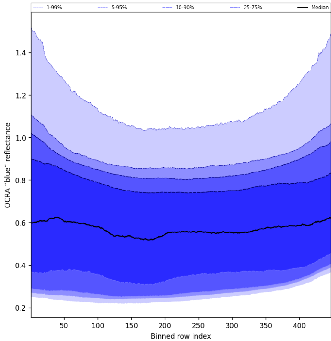
Figure 65: Along track statistics of “OCRA “blue” reflectance” for 2025-03-18 to 2025-03-19
