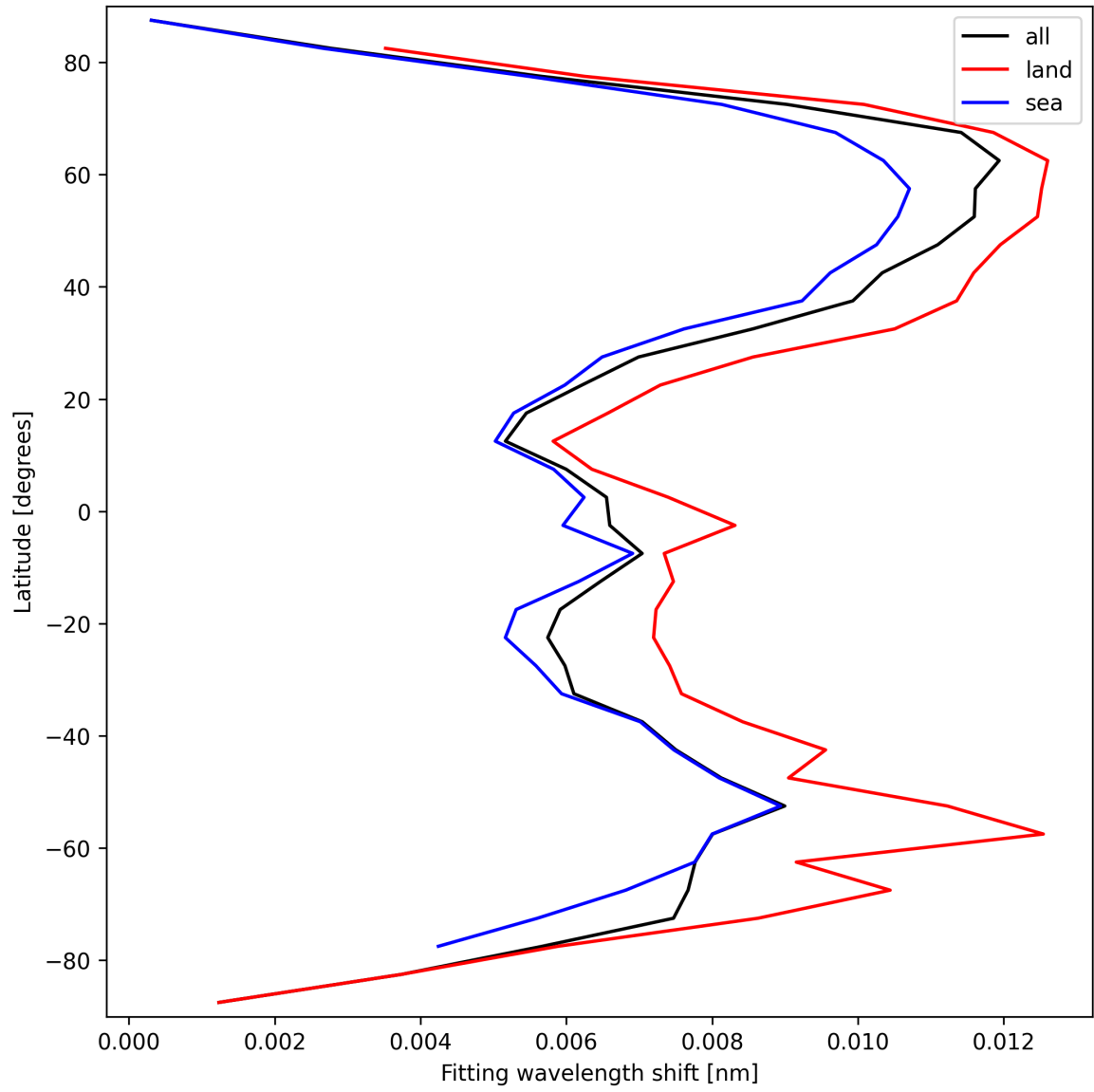
Figure 31: Zonal average of “Fitting wavelength shift” for 2025-03-18 to 2025-03-19.
