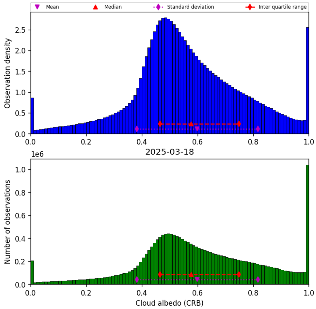
Figure 42: Histogram of “Cloud albedo (CRB)” for 2025-03-18 to 2025-03-19
