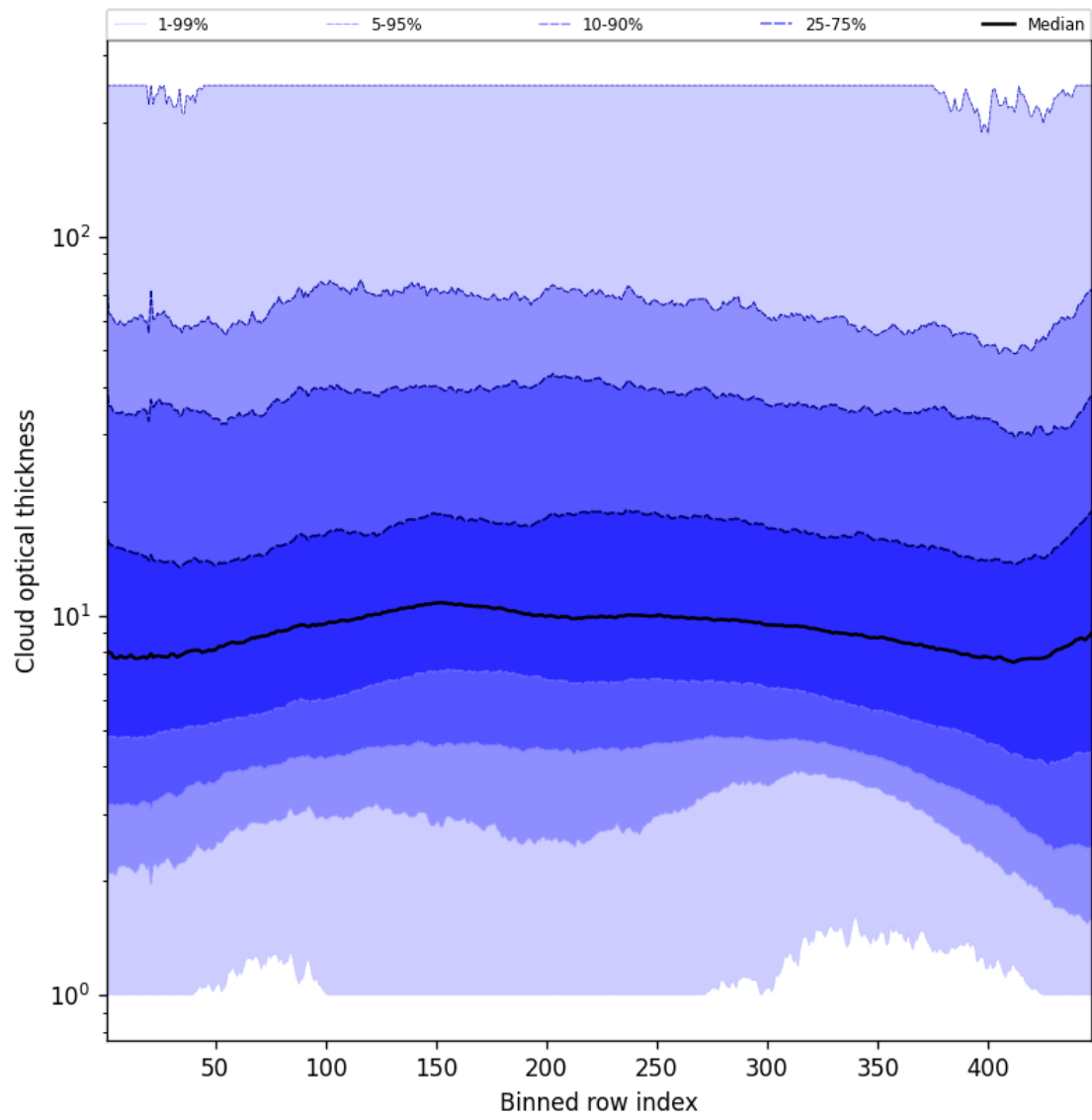
Figure 55: Along track statistics of “Cloud optical thickness” for 2025-03-18 to 2025-03-19
