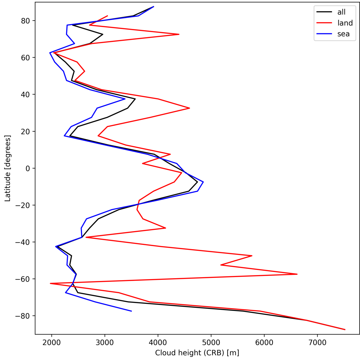
Figure 25: Zonal average of “Cloud height (CRB)” for 2025-03-18 to 2025-03-19.
