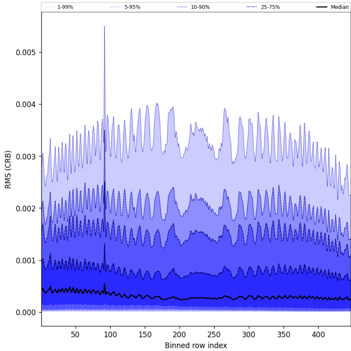
Figure 62: Along track statistics of “RMS (CRB)” for 2025-03-18 to 2025-03-19
