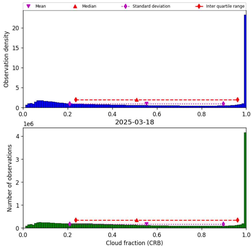
Figure 40: Histogram of “Cloud fraction (CRB)” for 2025-03-18 to 2025-03-19
