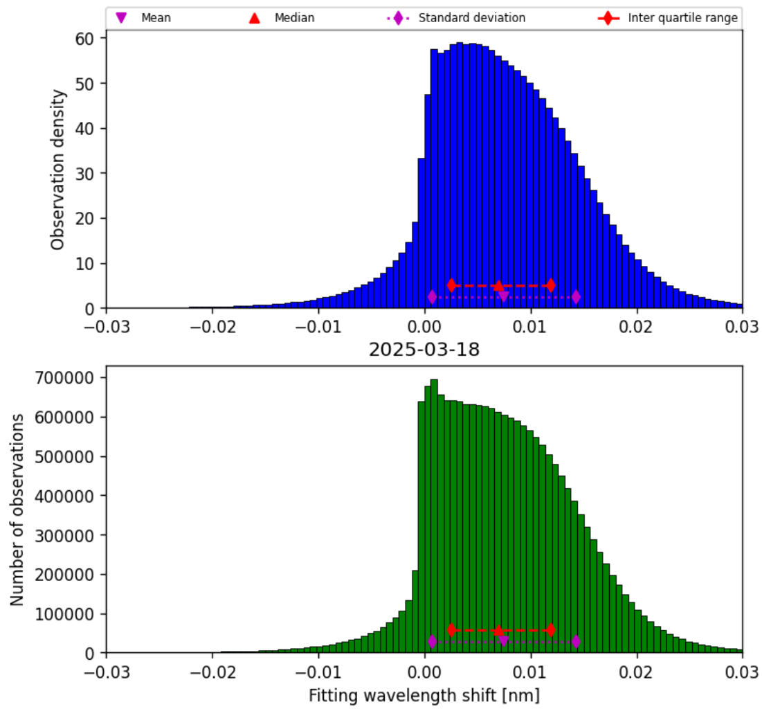
Figure 47: Histogram of “Fitting wavelength shift” for 2025-03-18 to 2025-03-19
