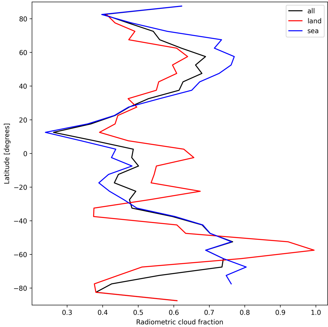
Figure 21: Zonal average of “Radiometric cloud fraction” for 2025-03-18 to 2025-03-19.
