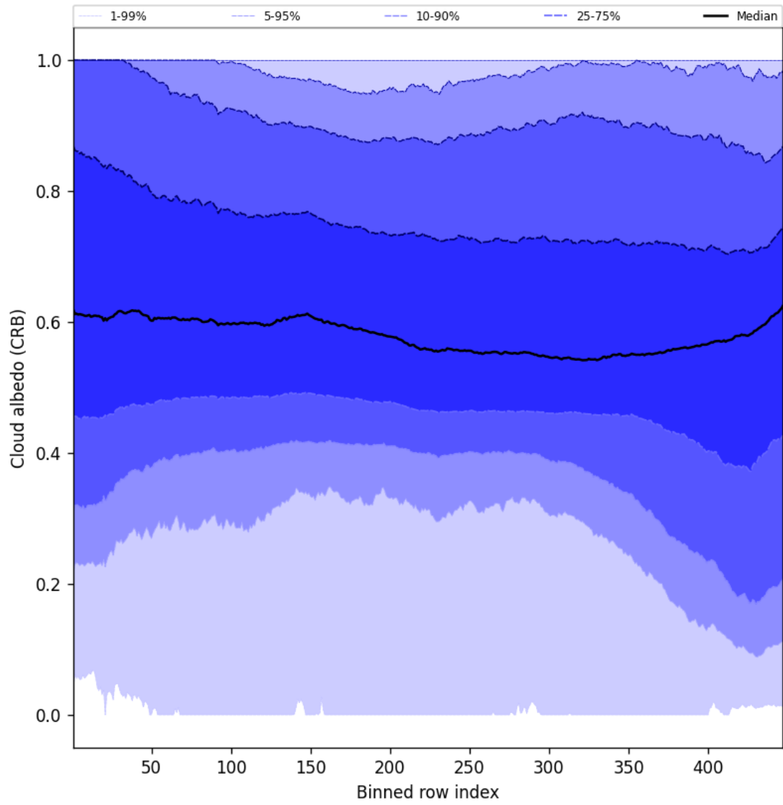
Figure 58: Along track statistics of “Cloud albedo (CRB)” for 2025-03-18 to 2025-03-19
