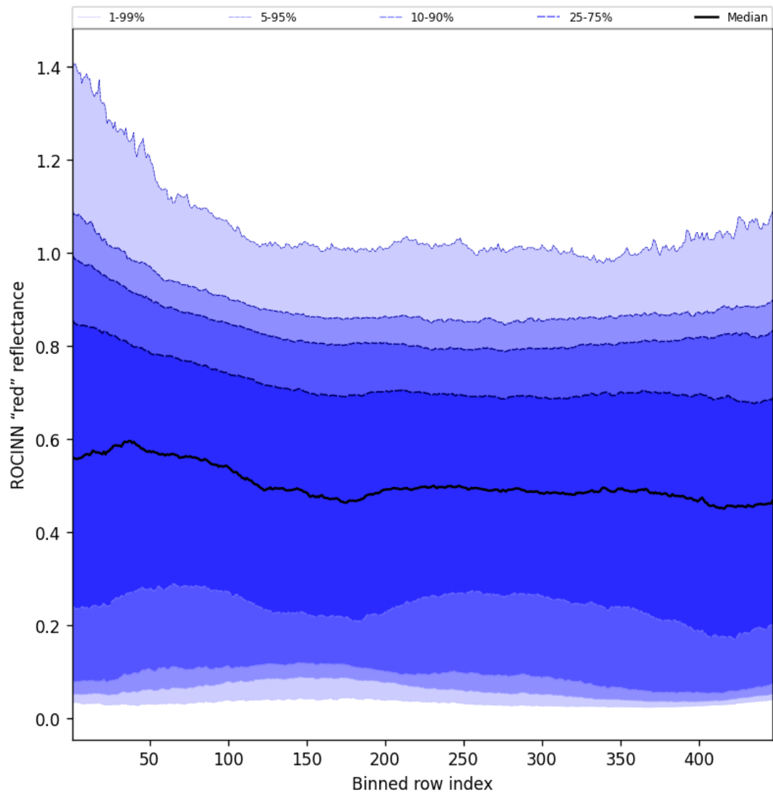
Figure 67: Along track statistics of “ROCINN “red” reflectance” for 2025-03-18 to 2025-03-19
