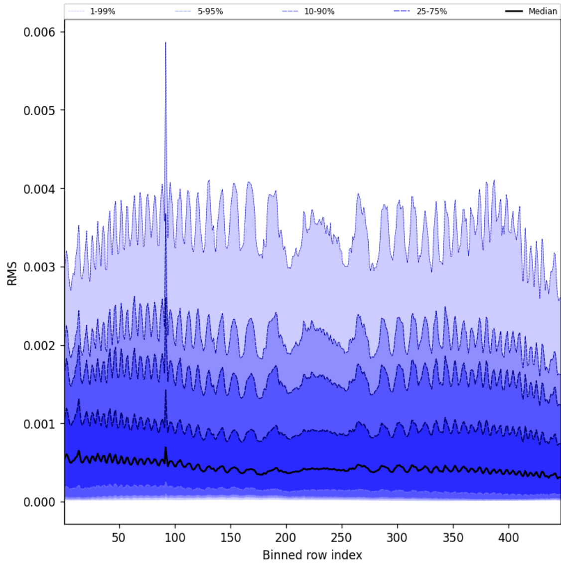
Figure 61: Along track statistics of “RMS” for 2025-03-18 to 2025-03-19
