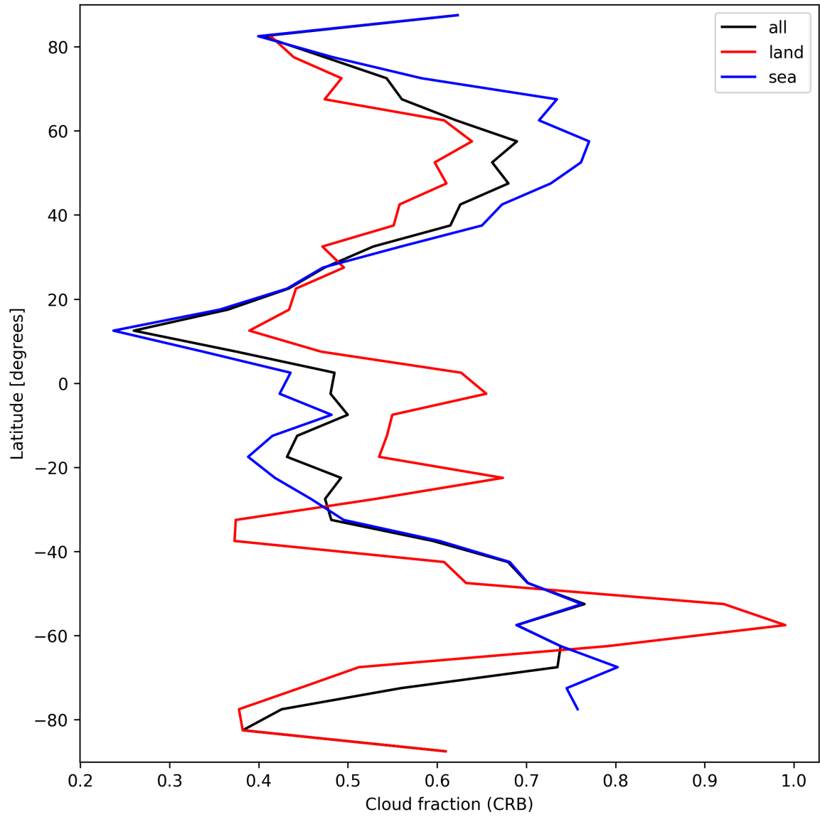
Figure 24: Zonal average of “Cloud fraction (CRB)” for 2025-03-18 to 2025-03-19.
