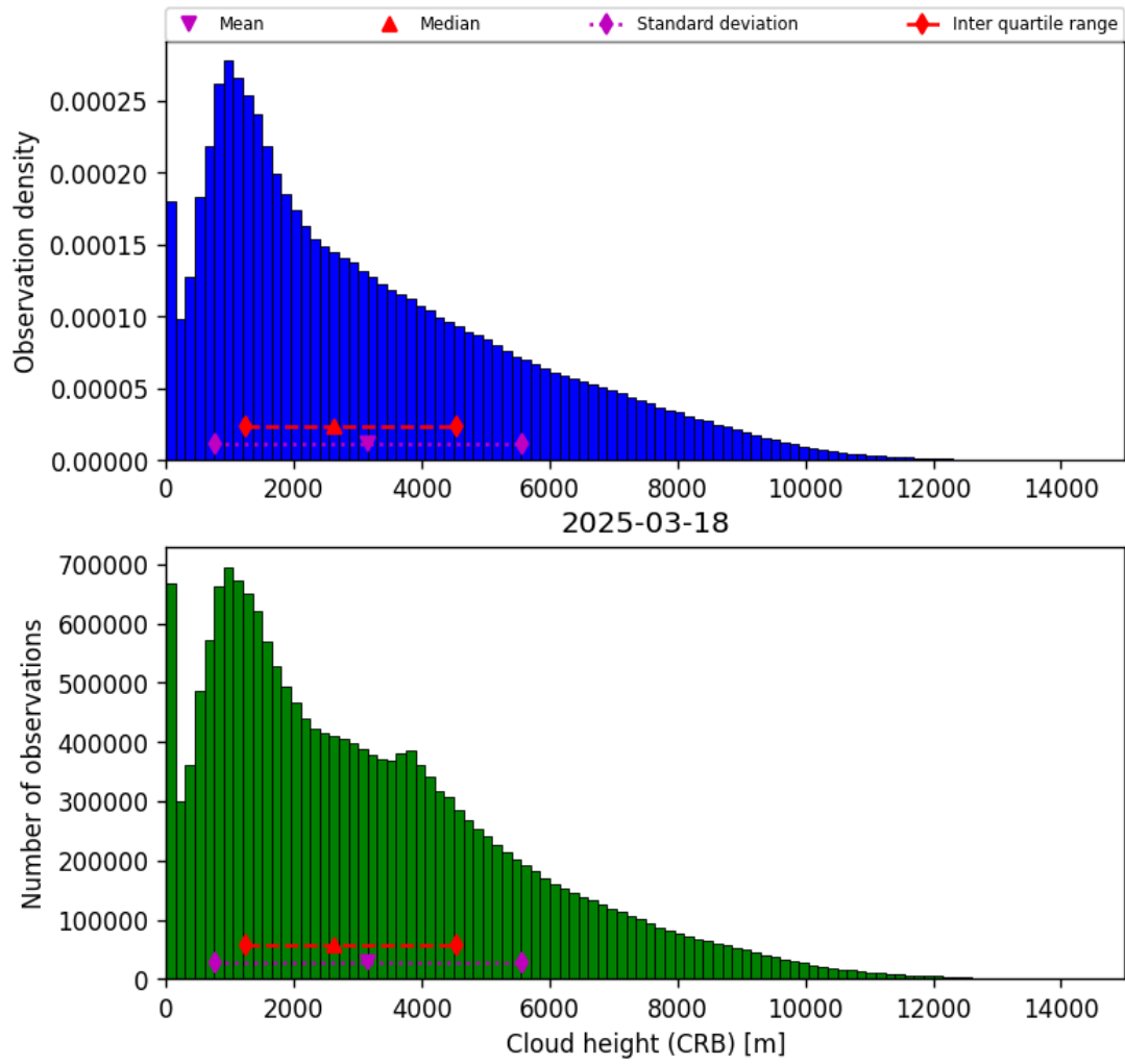
Figure 41: Histogram of “Cloud height (CRB)” for 2025-03-18 to 2025-03-19
