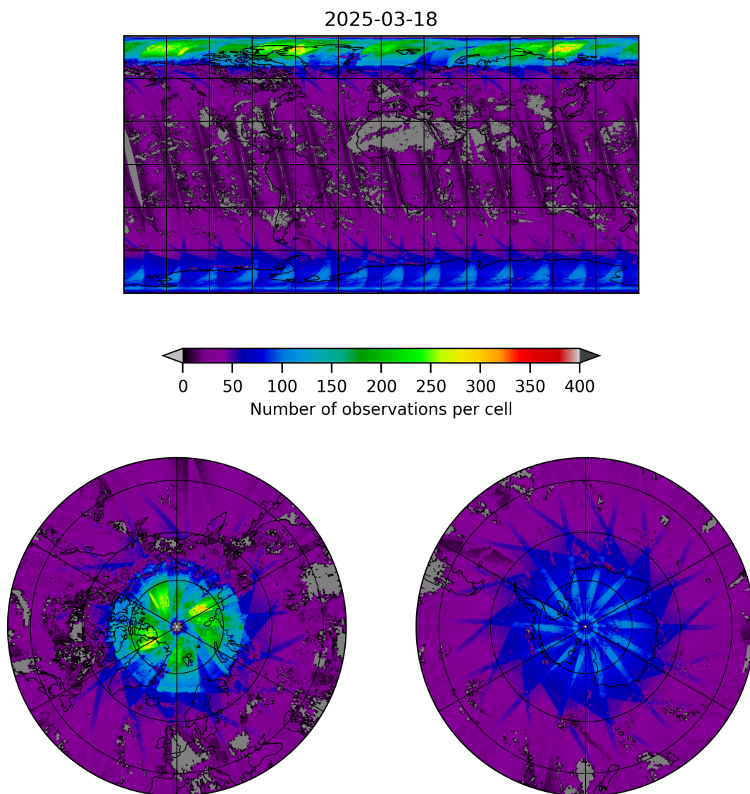
Figure 19: Map of the number of observations for 2025-03-18 to 2025-03-19
