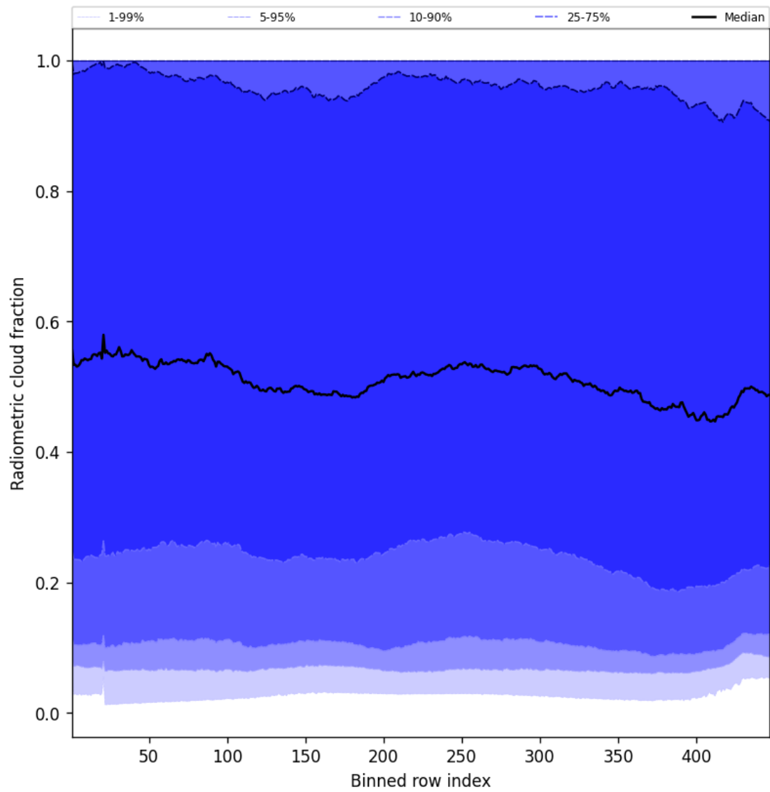
Figure 53: Along track statistics of “Radiometric cloud fraction” for 2025-03-18 to 2025-03-19
