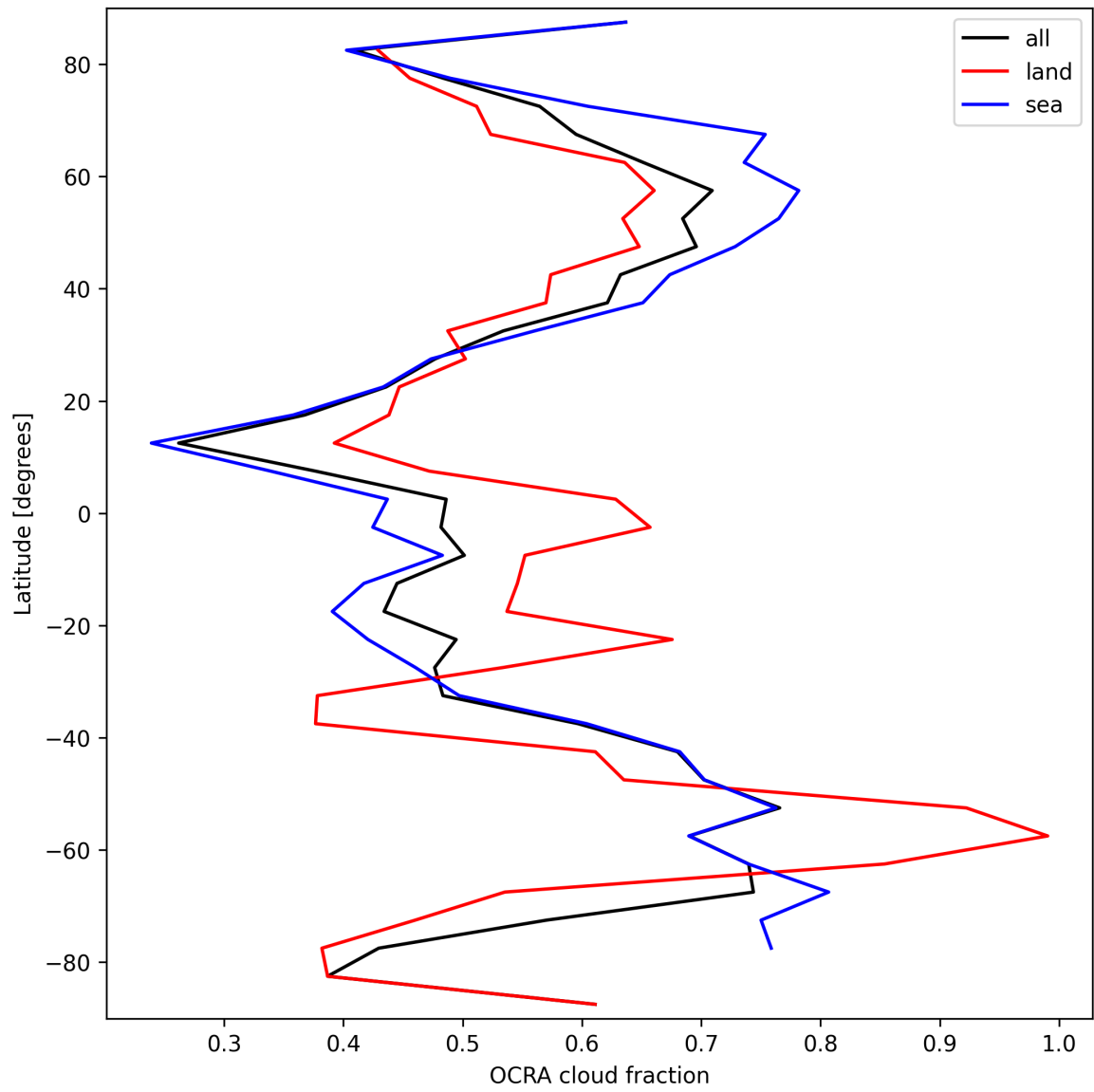
Figure 32: Zonal average of “OCRA cloud fraction” for 2025-03-18 to 2025-03-19.
