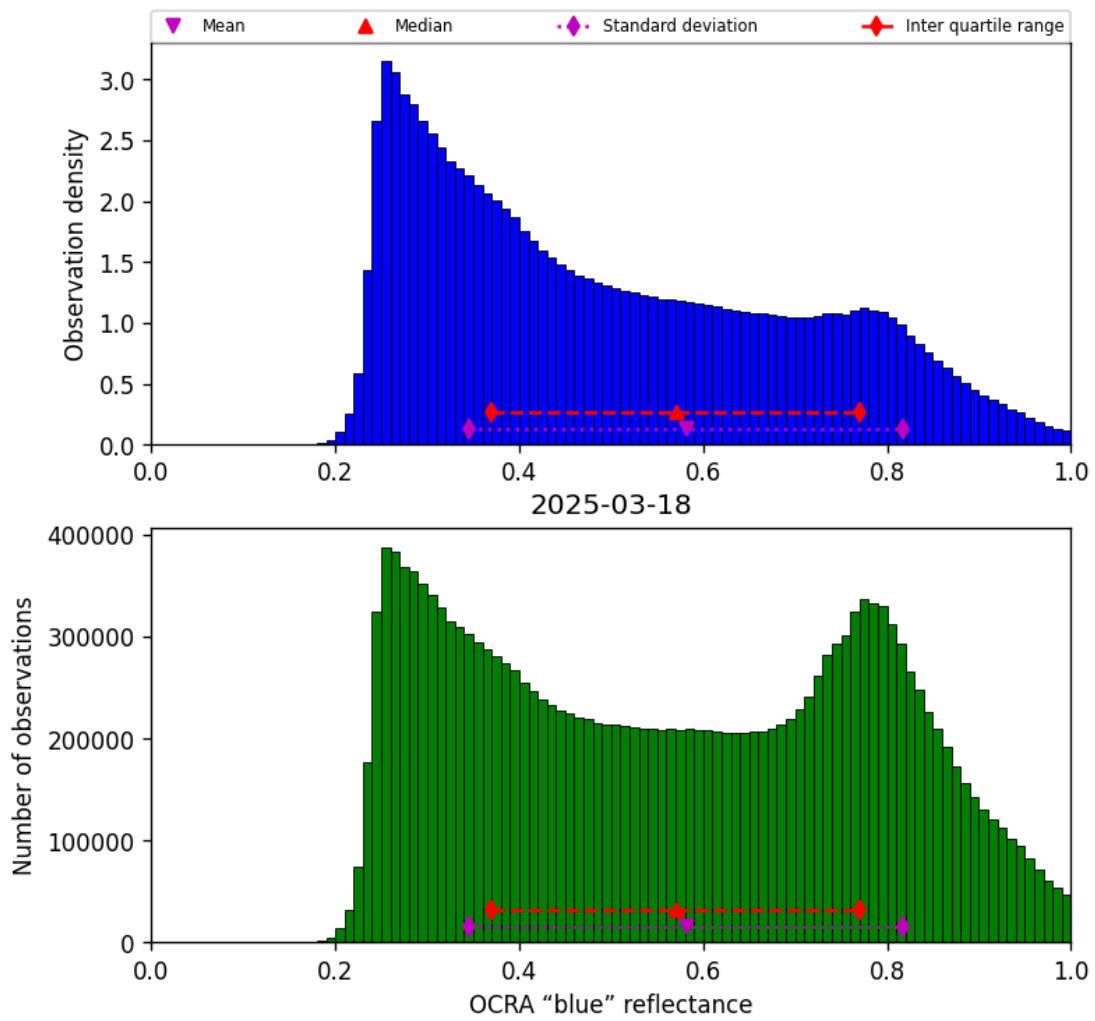
Figure 49: Histogram of “OCRA “blue” reflectance” for 2025-03-18 to 2025-03-19
