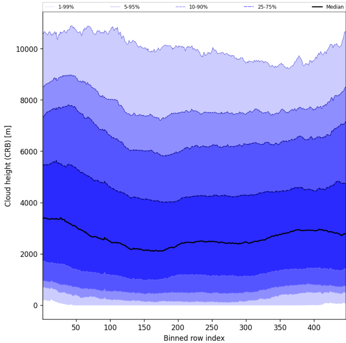
Figure 57: Along track statistics of “Cloud height (CRB)” for 2025-03-18 to 2025-03-19
