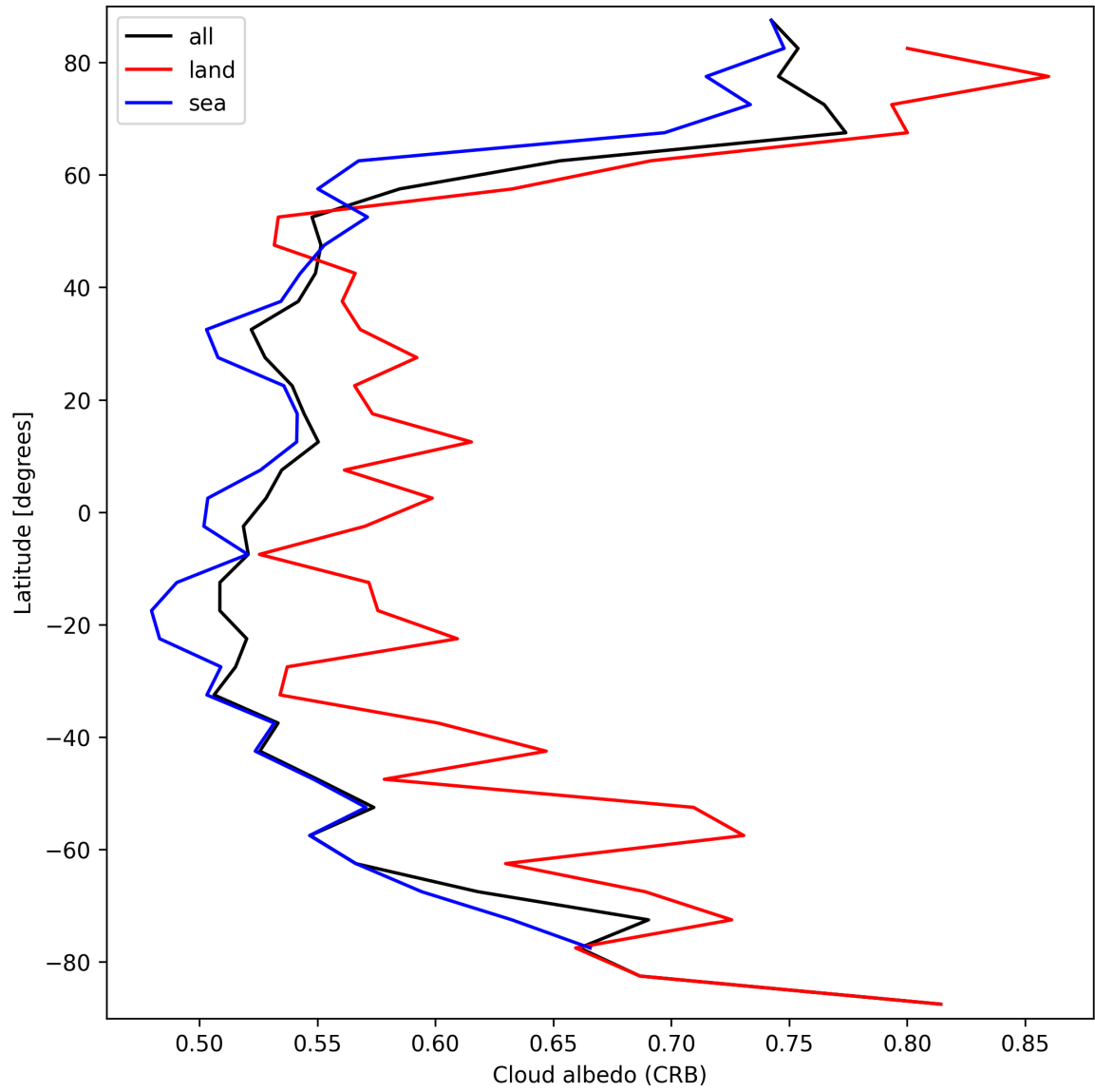
Figure 26: Zonal average of “Cloud albedo (CRB)” for 2025-03-18 to 2025-03-19.
