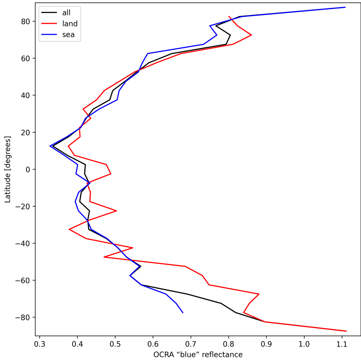
Figure 33: Zonal average of “OCRA “blue” reflectance” for 2025-03-18 to 2025-03-19.
