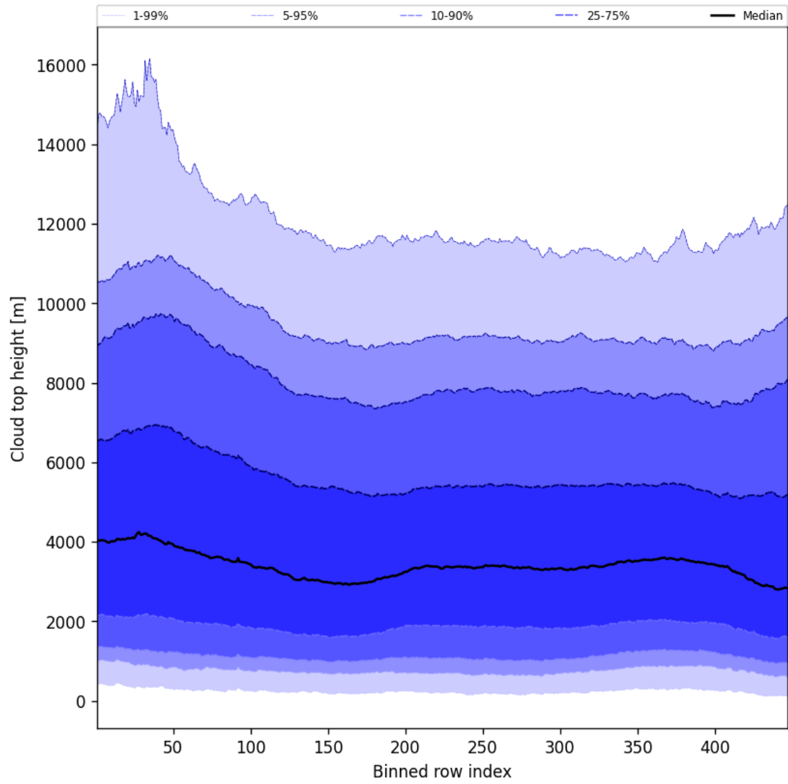
Figure 54: Along track statistics of “Cloud top height” for 2025-03-18 to 2025-03-19
