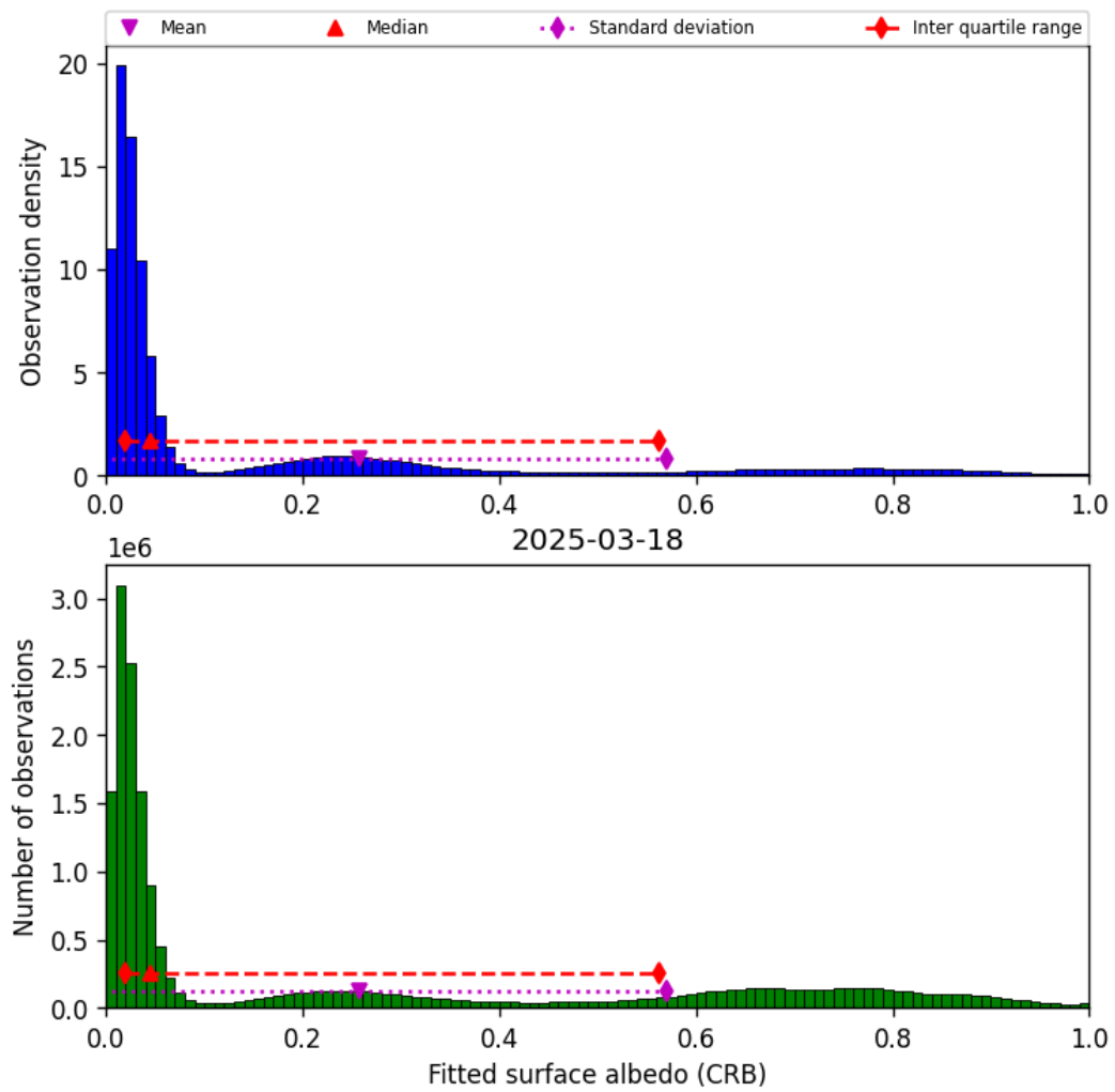
Figure 44: Histogram of “Fitted surface albedo (CRB)” for 2025-03-18 to 2025-03-19
