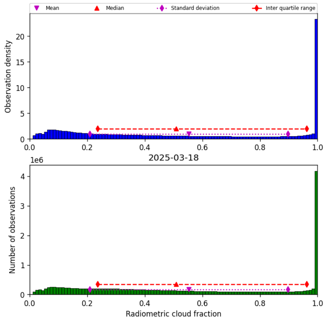
Figure 37: Histogram of “Radiometric cloud fraction” for 2025-03-18 to 2025-03-19
