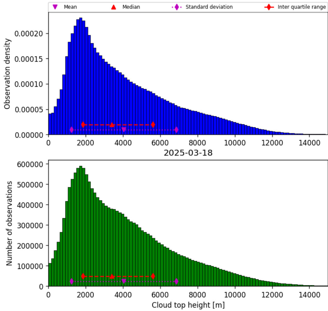
Figure 38: Histogram of “Cloud top height” for 2025-03-18 to 2025-03-19
