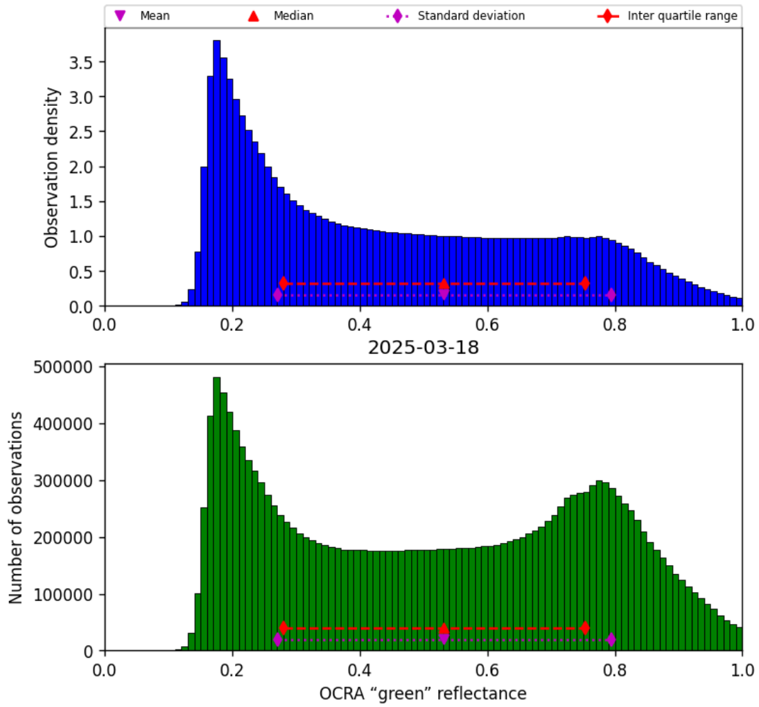
Figure 50: Histogram of “OCRA “green” reflectance” for 2025-03-18 to 2025-03-19
