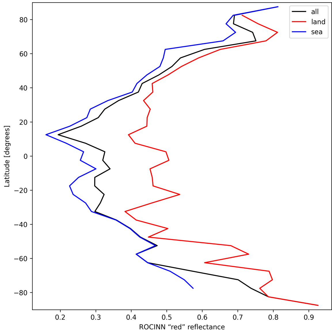
Figure 35: Zonal average of “ROCINN “red” reflectance” for 2025-03-18 to 2025-03-19.
