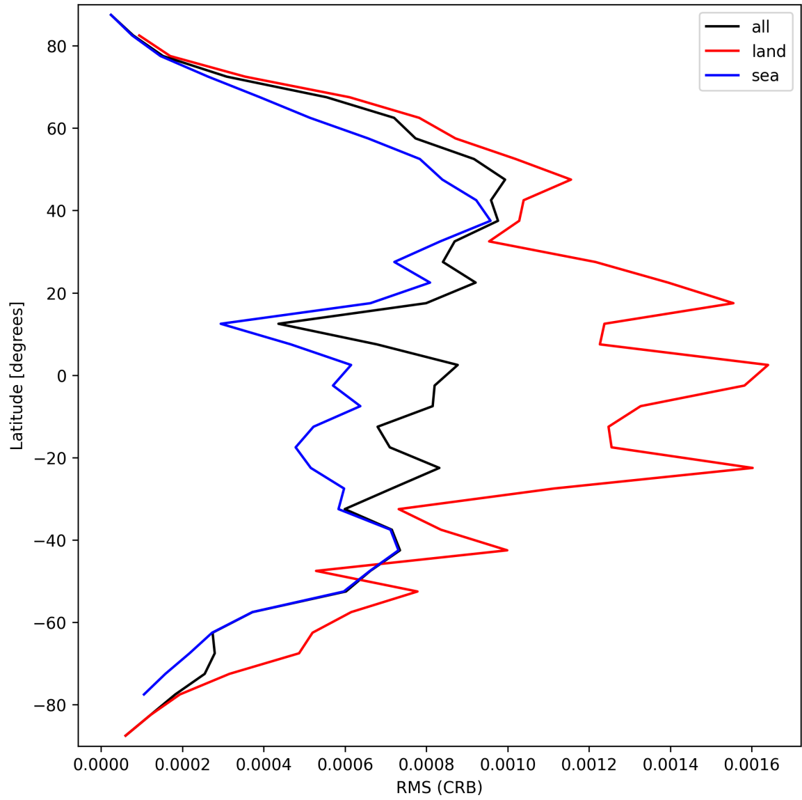
Figure 30: Zonal average of “RMS (CRB)” for 2025-03-18 to 2025-03-19.
