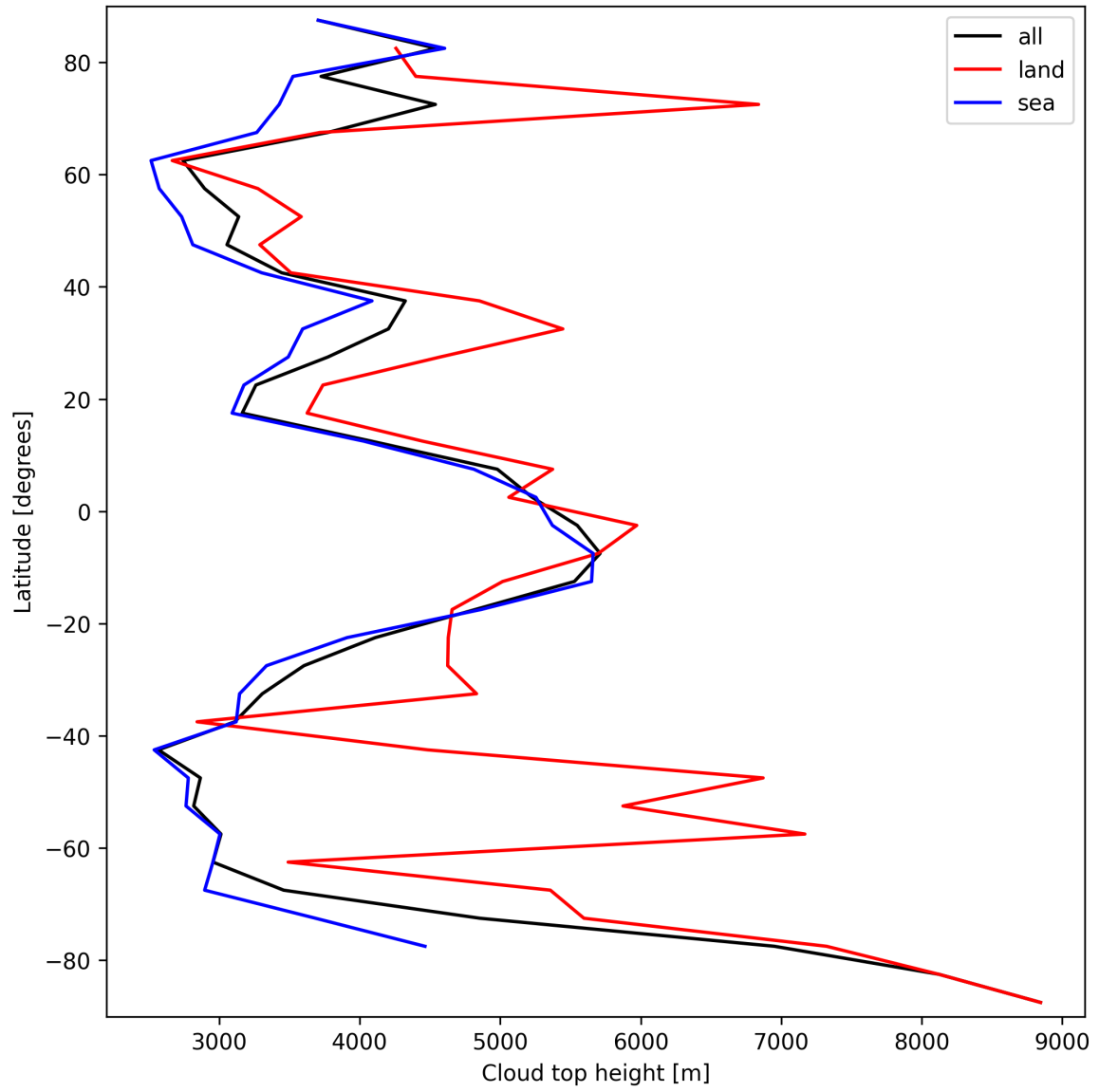
Figure 22: Zonal average of “Cloud top height” for 2025-03-18 to 2025-03-19.
