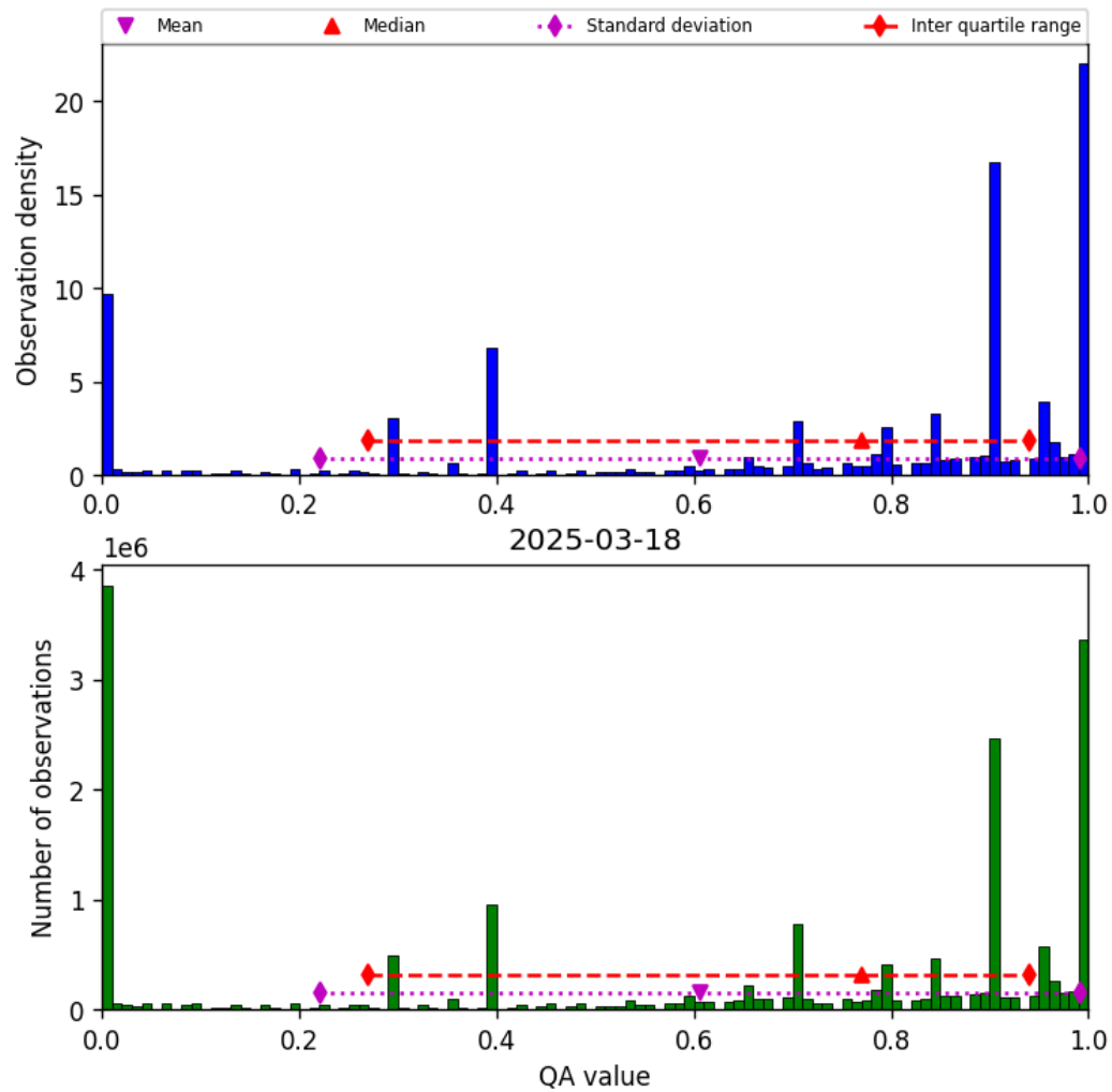
Figure 36: Histogram of “QA value” for 2025-03-18 to 2025-03-19
