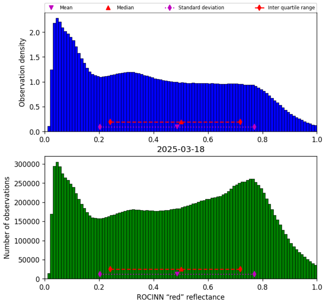
Figure 51: Histogram of “ROCINN “red” reflectance” for 2025-03-18 to 2025-03-19
