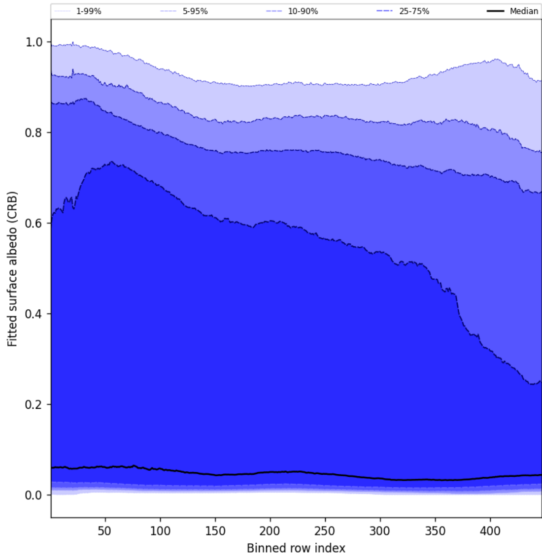
Figure 60: Along track statistics of “Fitted surface albedo (CRB)” for 2025-03-18 to 2025-03-19
