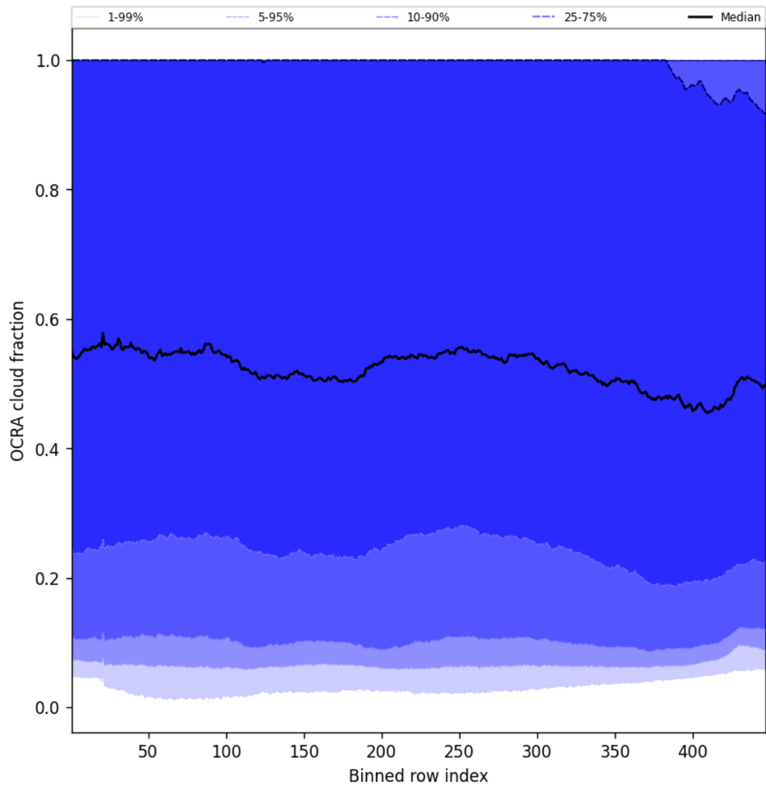
Figure 64: Along track statistics of “OCRA cloud fraction” for 2025-03-18 to 2025-03-19
