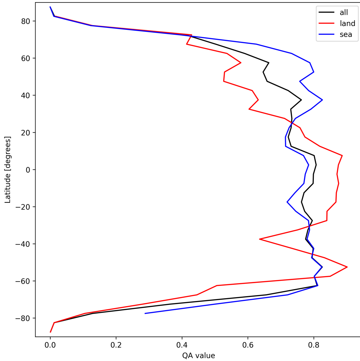
Figure 20: Zonal average of “QA value” for 2025-03-18 to 2025-03-19.
