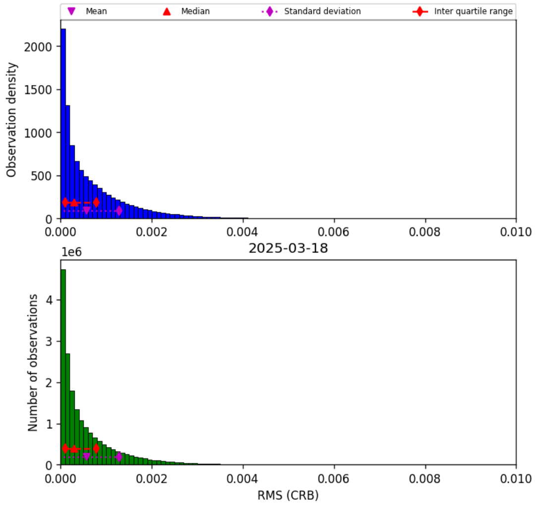
Figure 46: Histogram of “RMS (CRB)” for 2025-03-18 to 2025-03-19
