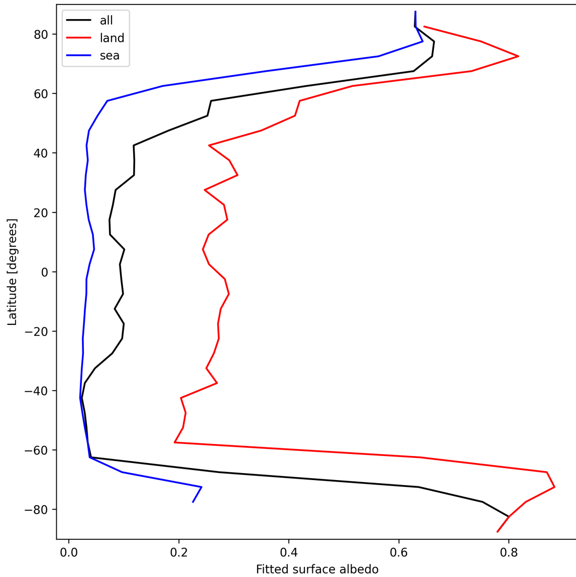
Figure 27: Zonal average of “Fitted surface albedo” for 2025-03-18 to 2025-03-19.
