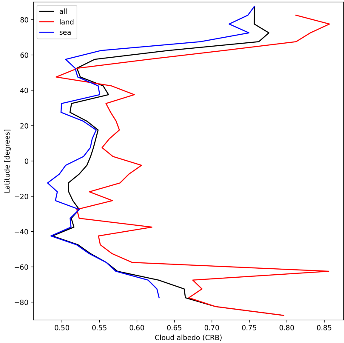
Figure 26: Zonal average of “Cloud albedo (CRB)” for 2025-03-19 to 2025-03-20.
