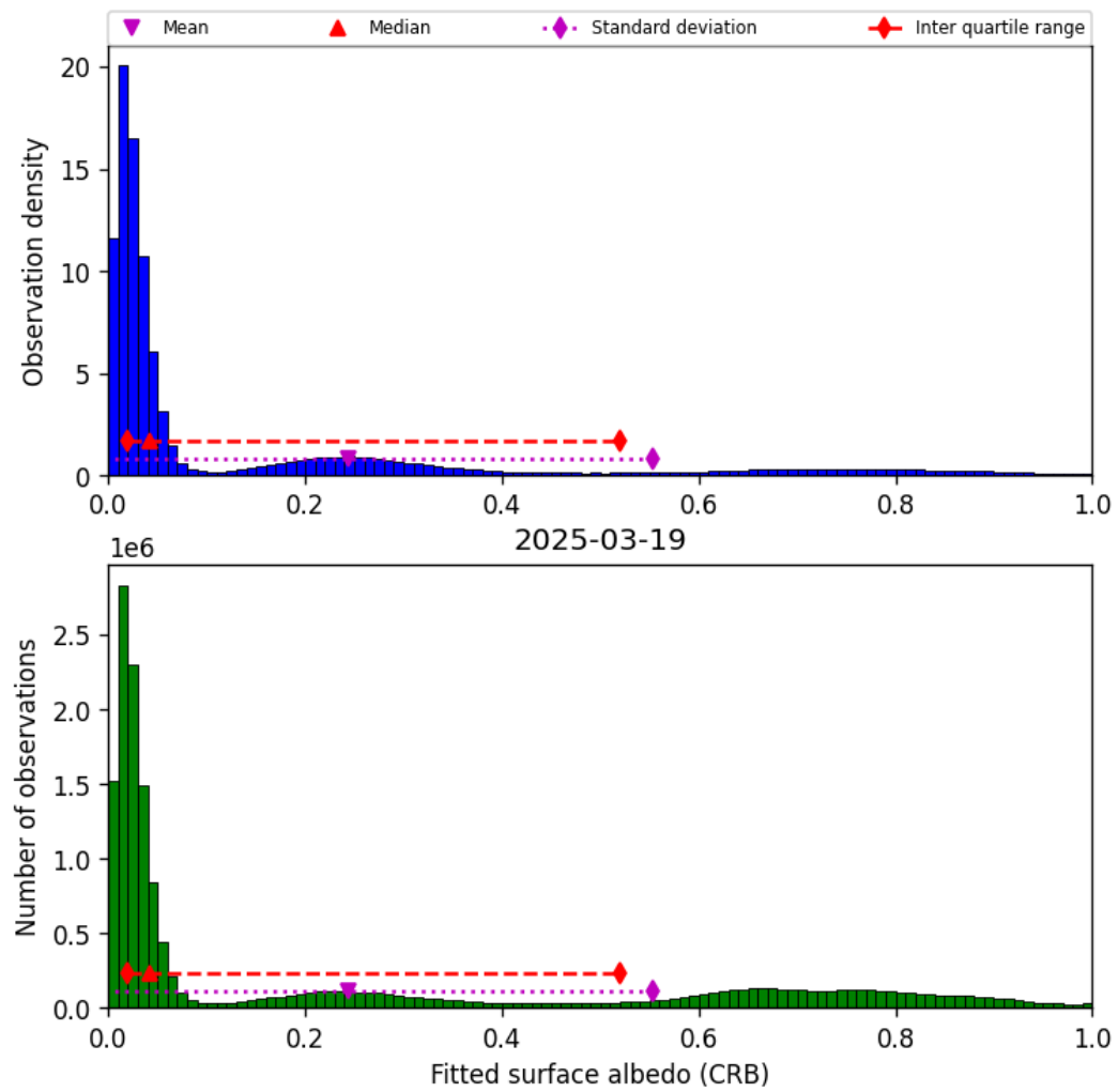
Figure 44: Histogram of “Fitted surface albedo (CRB)” for 2025-03-19 to 2025-03-20
