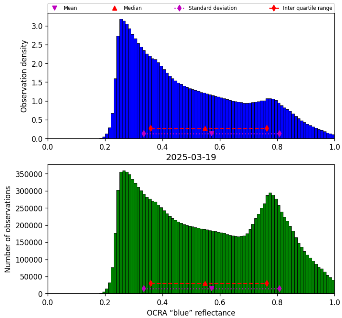
Figure 49: Histogram of “OCRA “blue” reflectance” for 2025-03-19 to 2025-03-20
