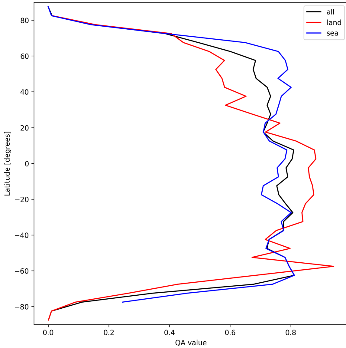
Figure 20: Zonal average of “QA value” for 2025-03-19 to 2025-03-20.
