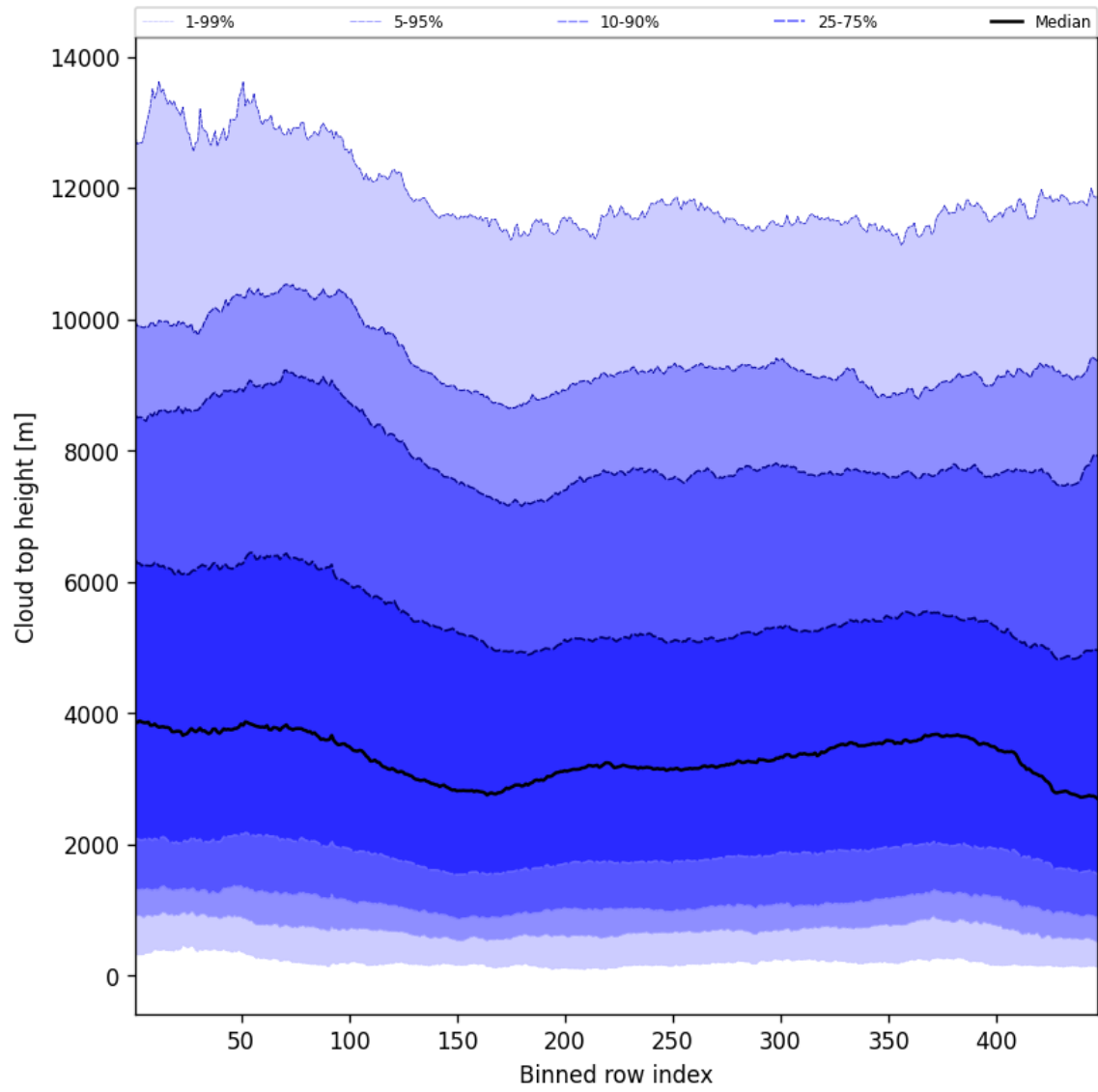
Figure 54: Along track statistics of “Cloud top height” for 2025-03-19 to 2025-03-20
