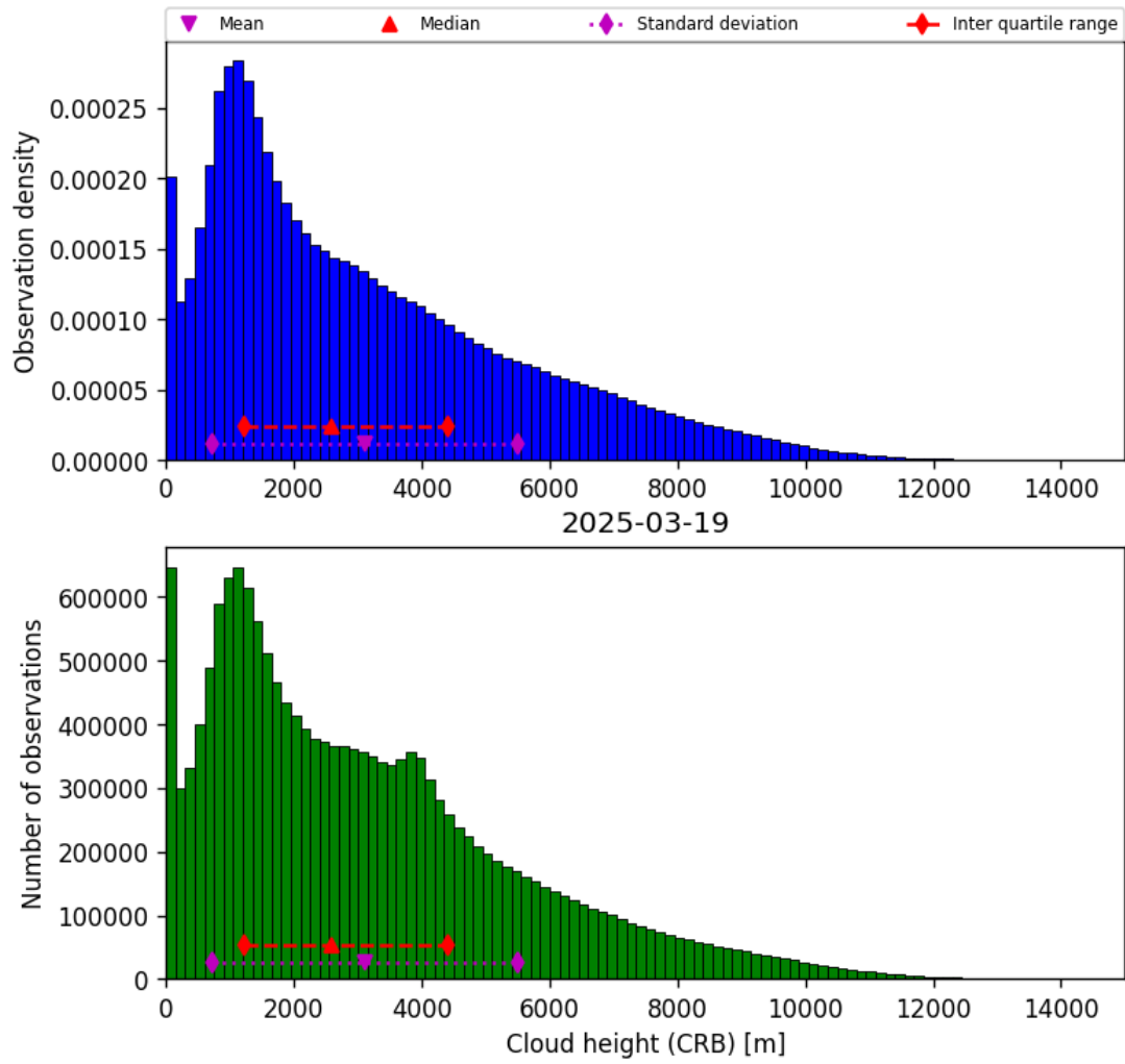
Figure 41: Histogram of “Cloud height (CRB)” for 2025-03-19 to 2025-03-20
