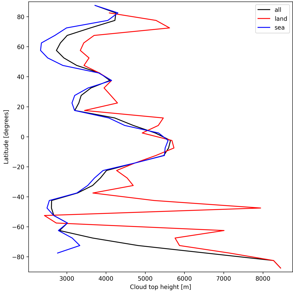
Figure 22: Zonal average of “Cloud top height” for 2025-03-19 to 2025-03-20.
