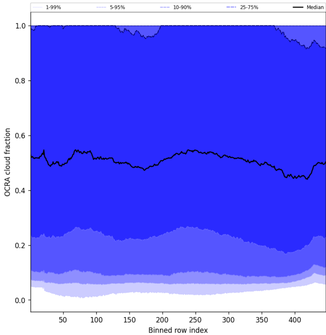
Figure 64: Along track statistics of “OCRA cloud fraction” for 2025-03-19 to 2025-03-20
