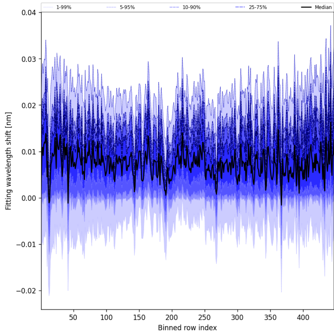
Figure 63: Along track statistics of “Fitting wavelength shift” for 2025-03-19 to 2025-03-20
