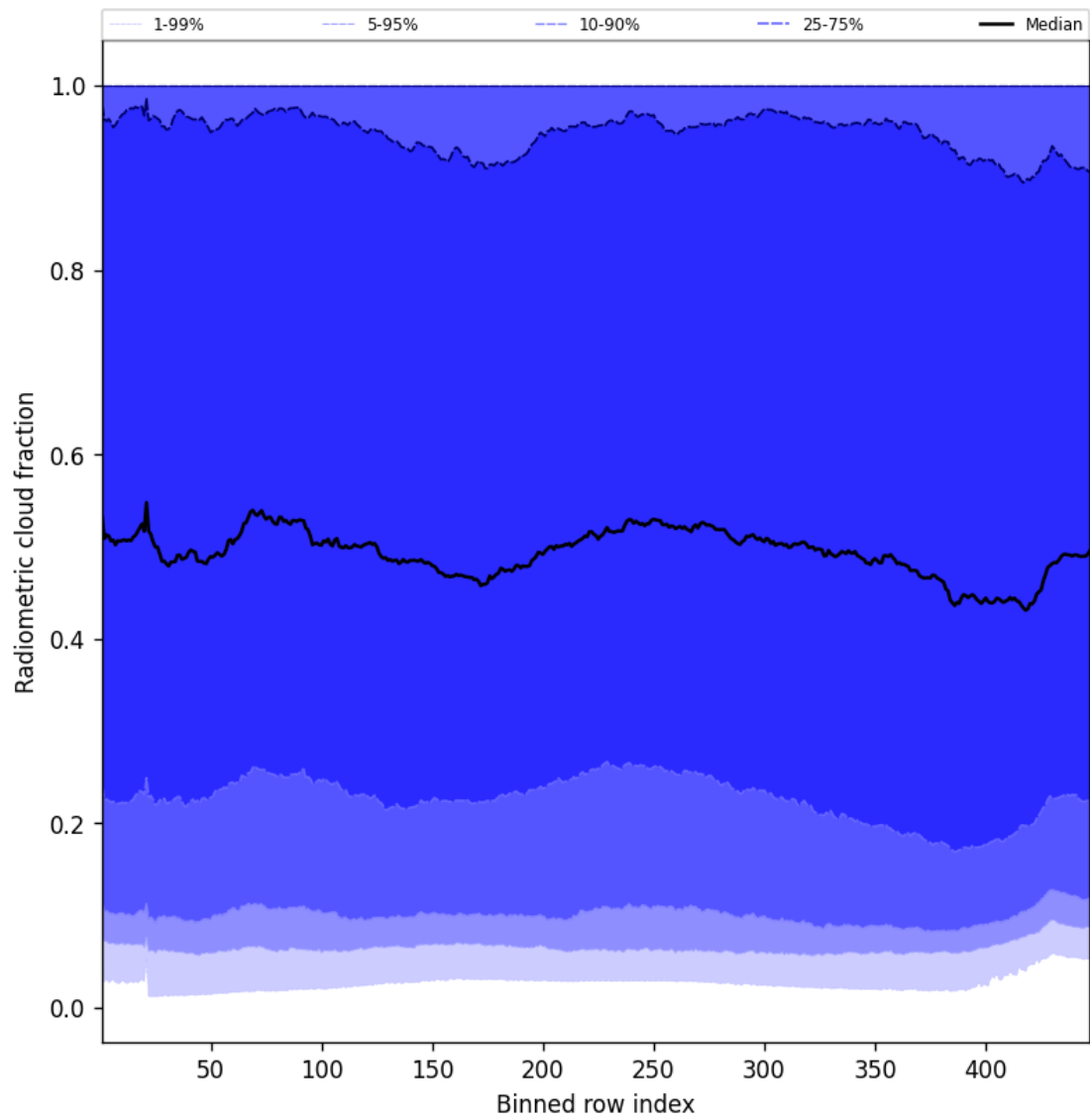
Figure 53: Along track statistics of “Radiometric cloud fraction” for 2025-03-19 to 2025-03-20
