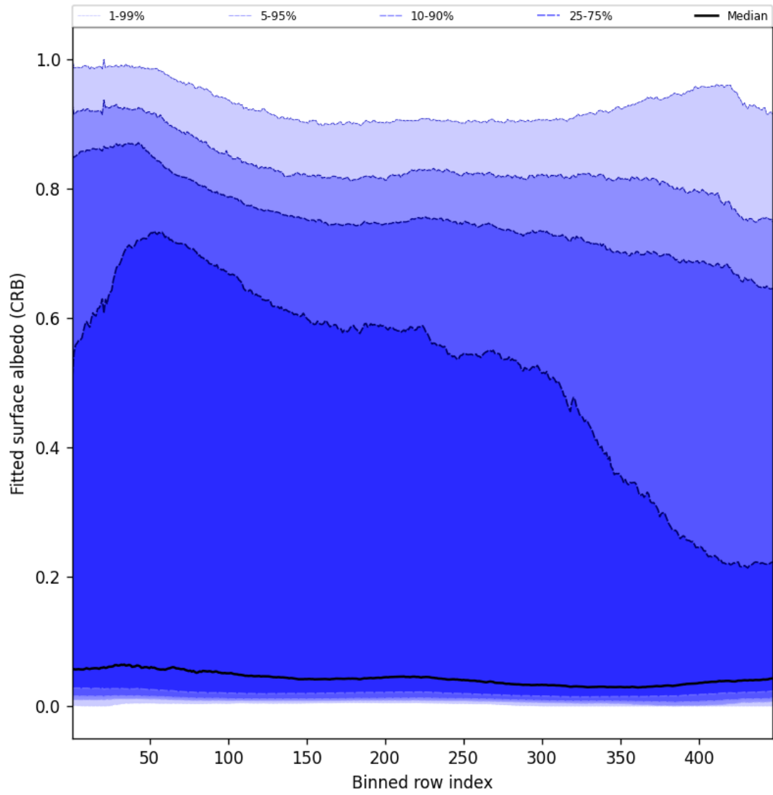
Figure 60: Along track statistics of “Fitted surface albedo (CRB)” for 2025-03-19 to 2025-03-20
