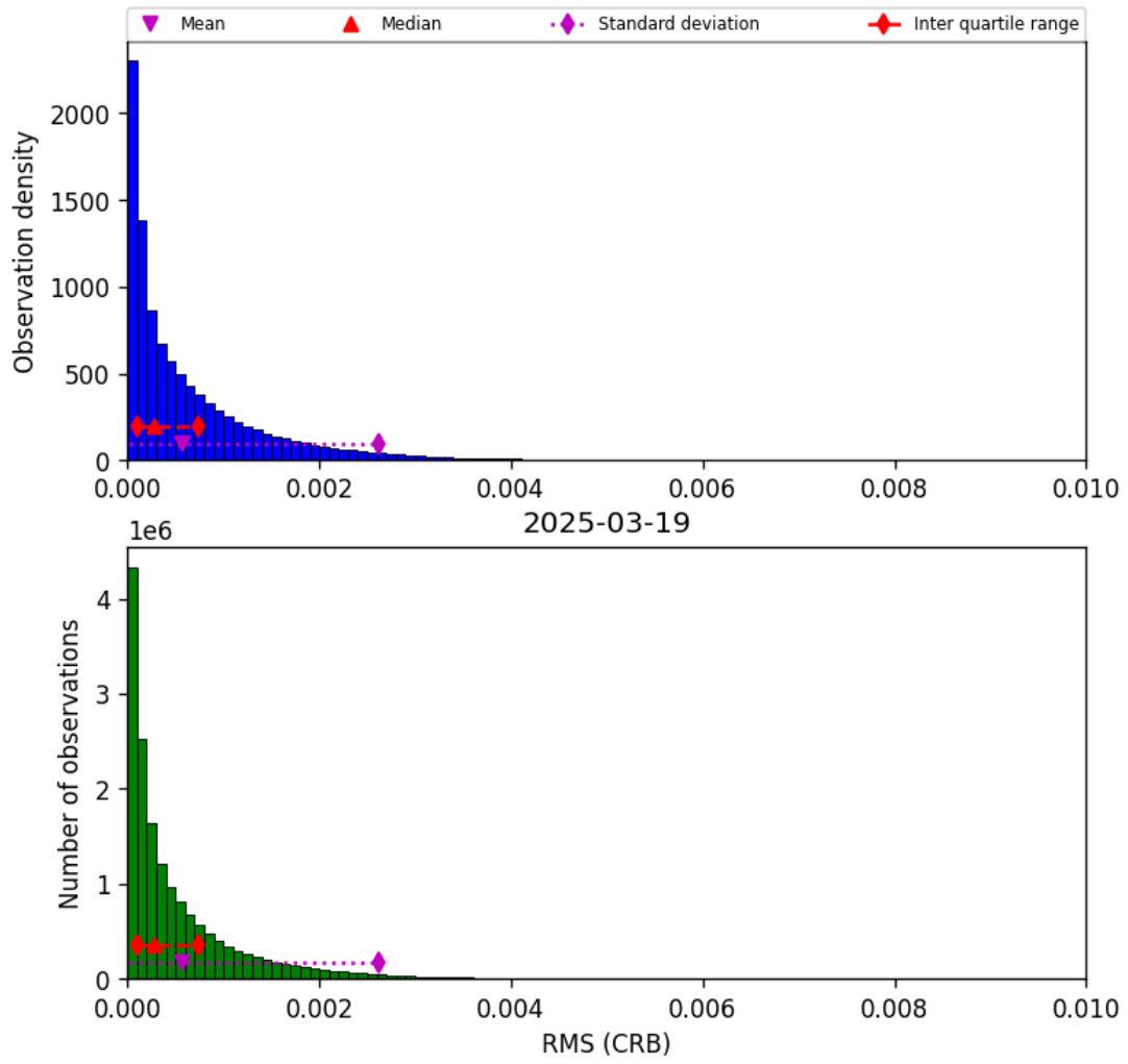
Figure 46: Histogram of "RMS (CRB)" for 2025-03-19 to 2025-03-20
