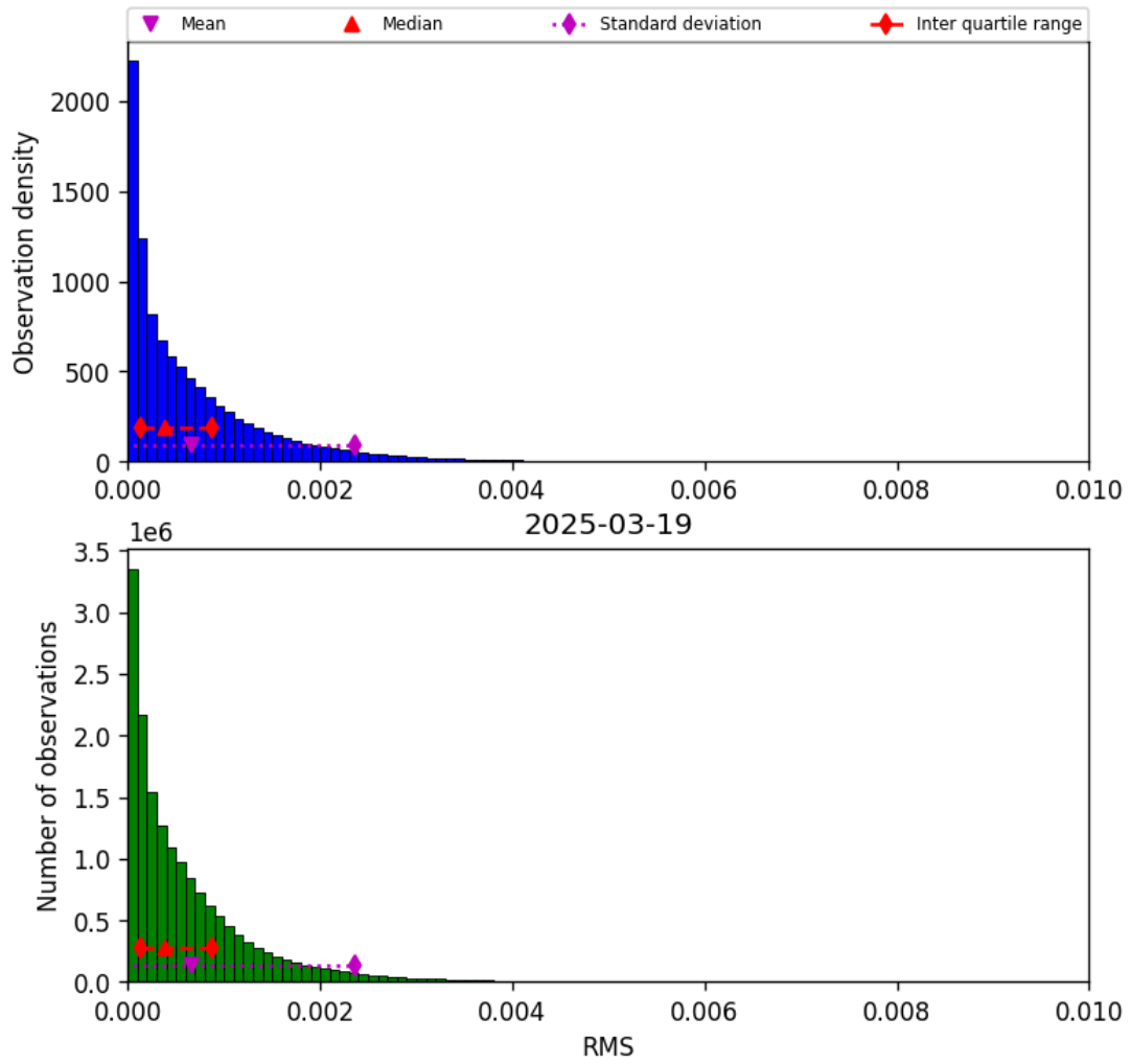
Figure 45: Histogram of “RMS” for 2025-03-19 to 2025-03-20
