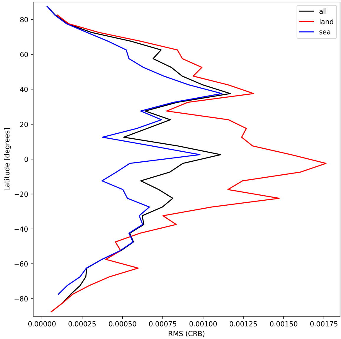
Figure 30: Zonal average of “RMS (CRB)” for 2025-03-19 to 2025-03-20.
