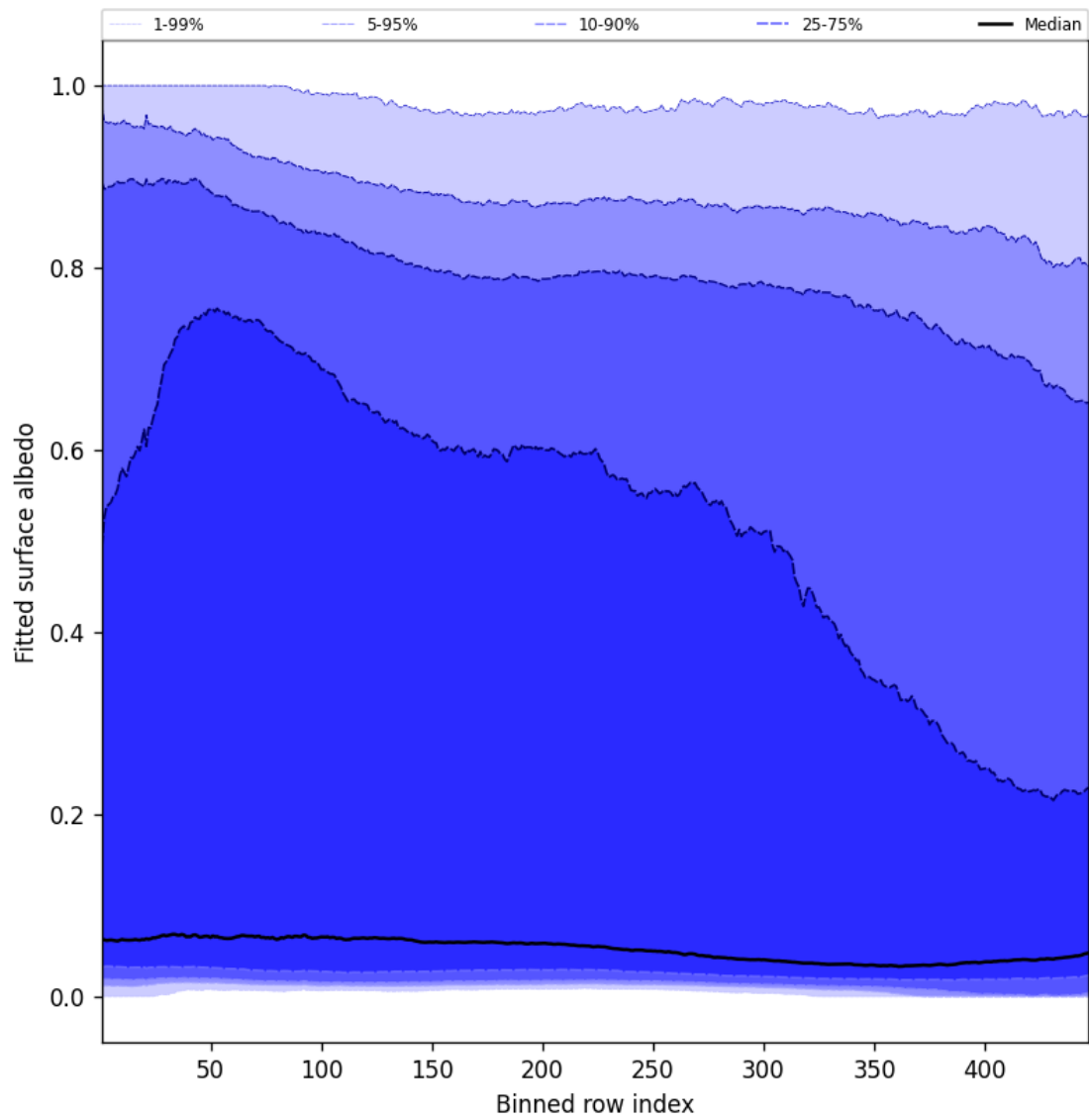
Figure 59: Along track statistics of “Fitted surface albedo” for 2025-03-19 to 2025-03-20
