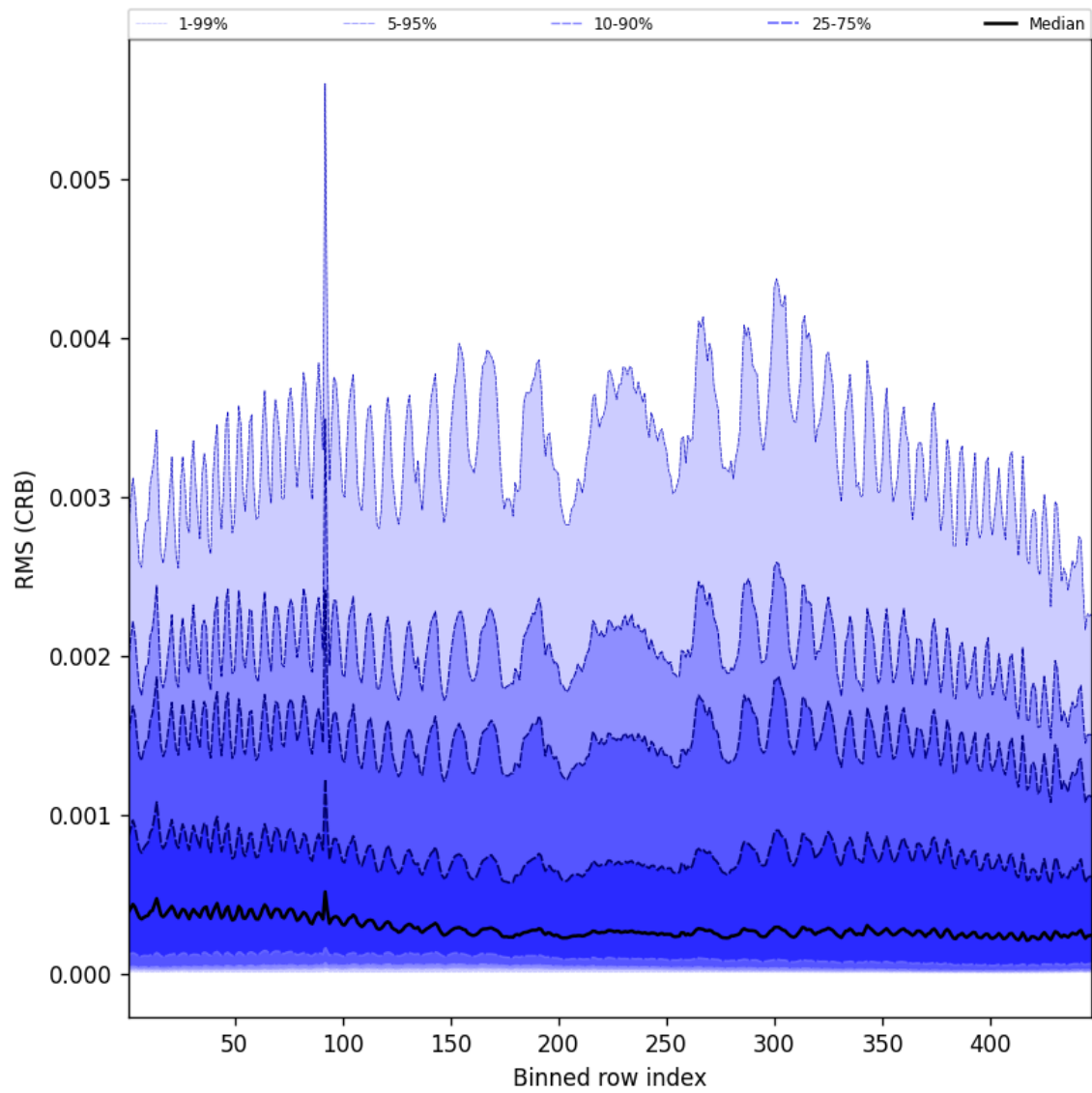
Figure 62: Along track statistics of “RMS (CRB)” for 2025-03-19 to 2025-03-20
