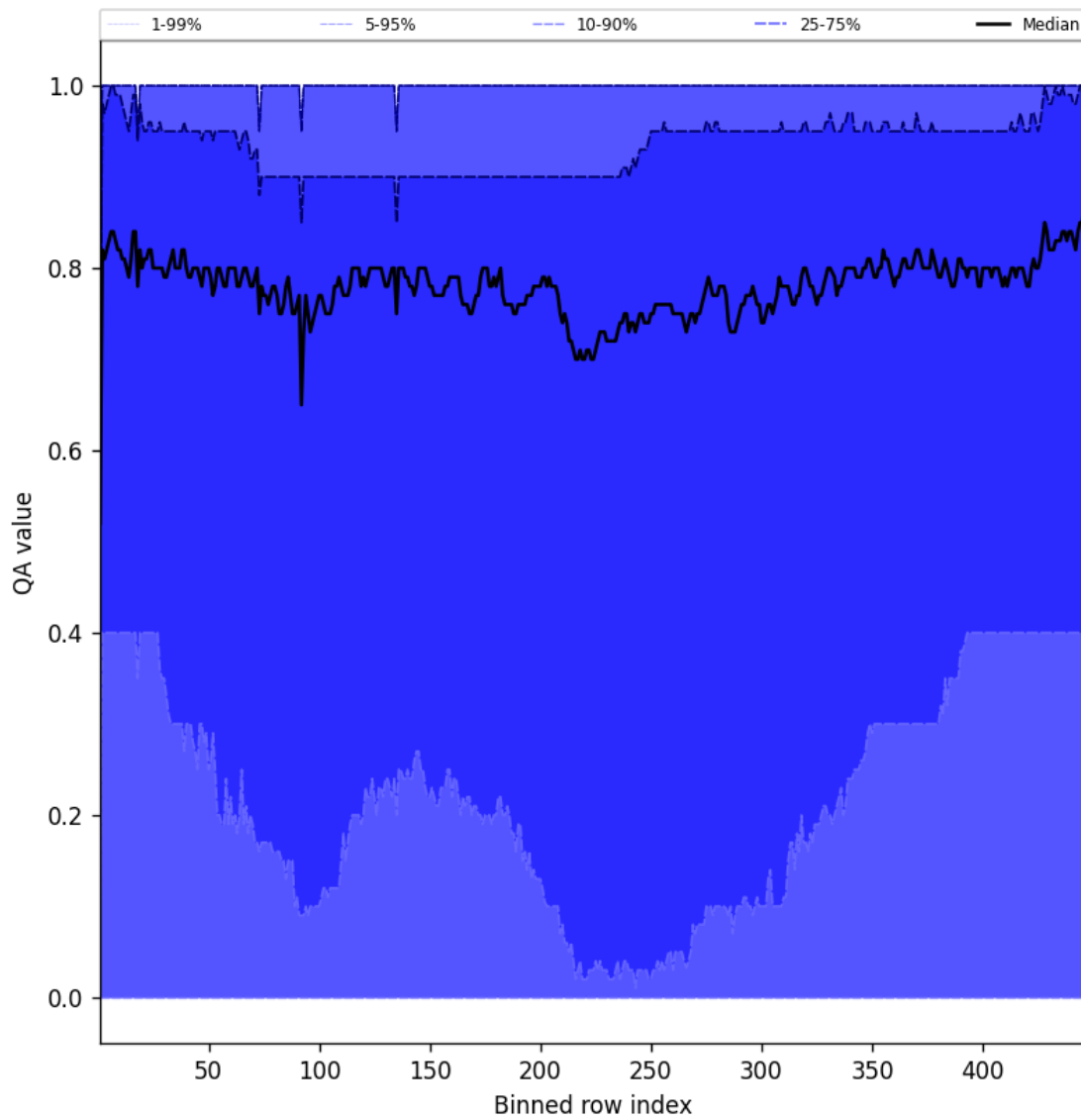
Figure 52: Along track statistics of “QA value” for 2025-03-19 to 2025-03-20
