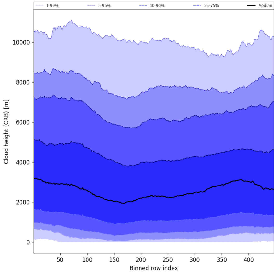
Figure 57: Along track statistics of “Cloud height (CRB)” for 2025-03-19 to 2025-03-20
