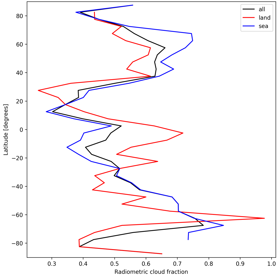
Figure 21: Zonal average of “Radiometric cloud fraction” for 2025-03-19 to 2025-03-20.
