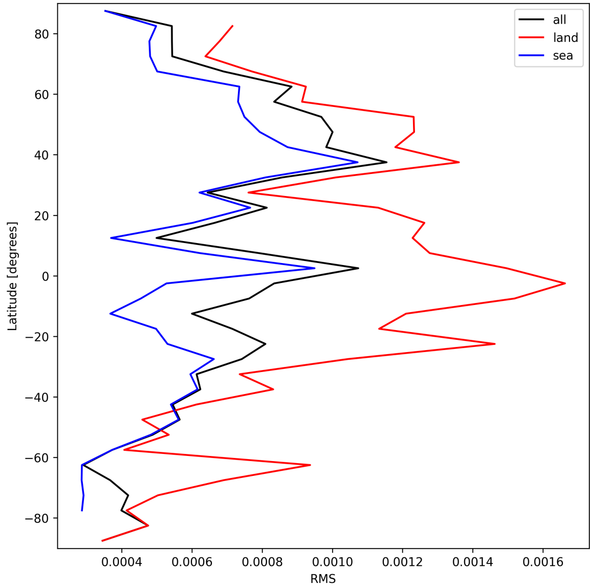
Figure 29: Zonal average of “RMS” for 2025-03-19 to 2025-03-20.
