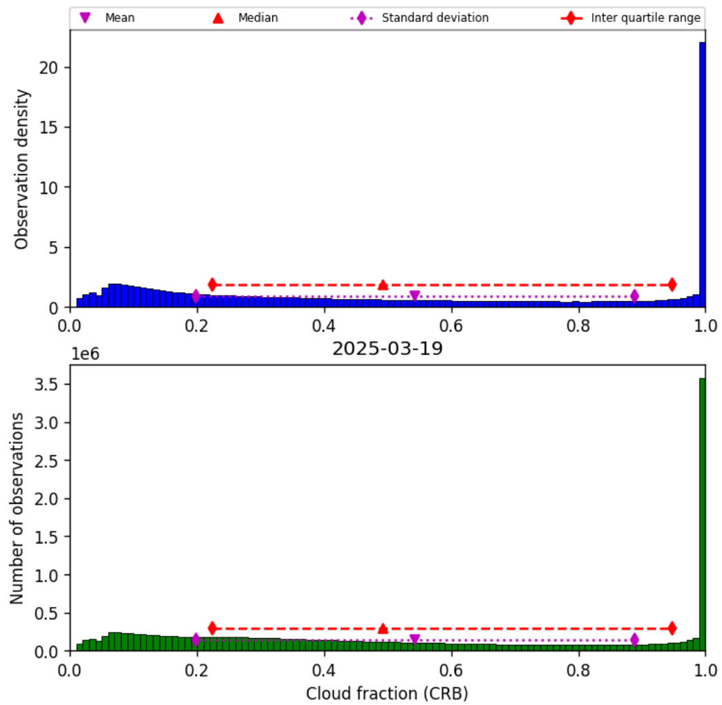
Figure 40: Histogram of “Cloud fraction (CRB)” for 2025-03-19 to 2025-03-20
