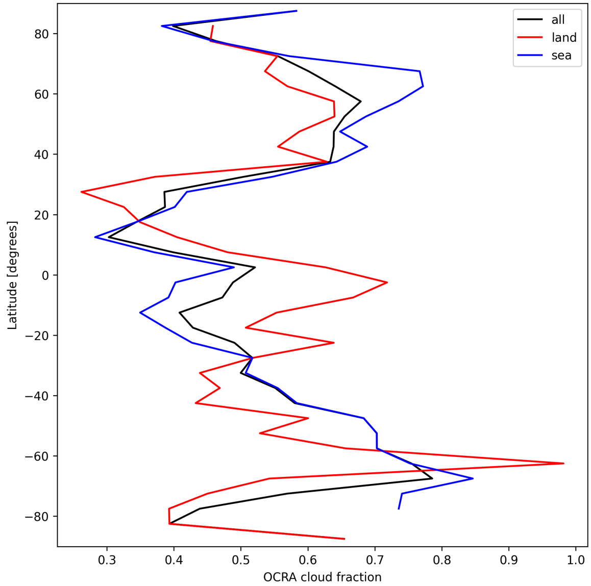
Figure 32: Zonal average of “OCRA cloud fraction” for 2025-03-19 to 2025-03-20.
