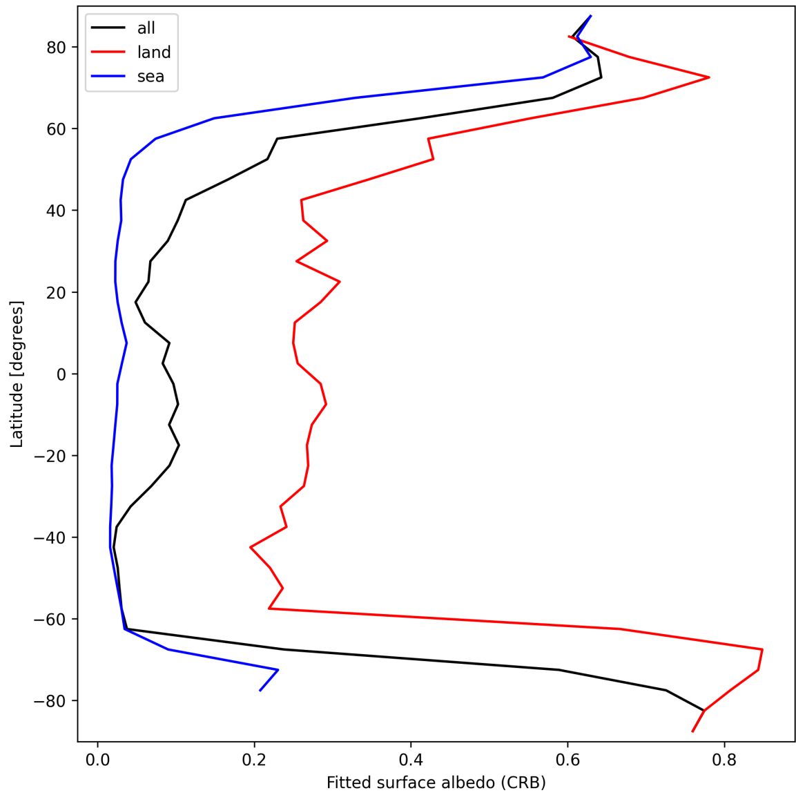
Figure 28: Zonal average of “Fitted surface albedo (CRB)” for 2025-03-19 to 2025-03-20.
