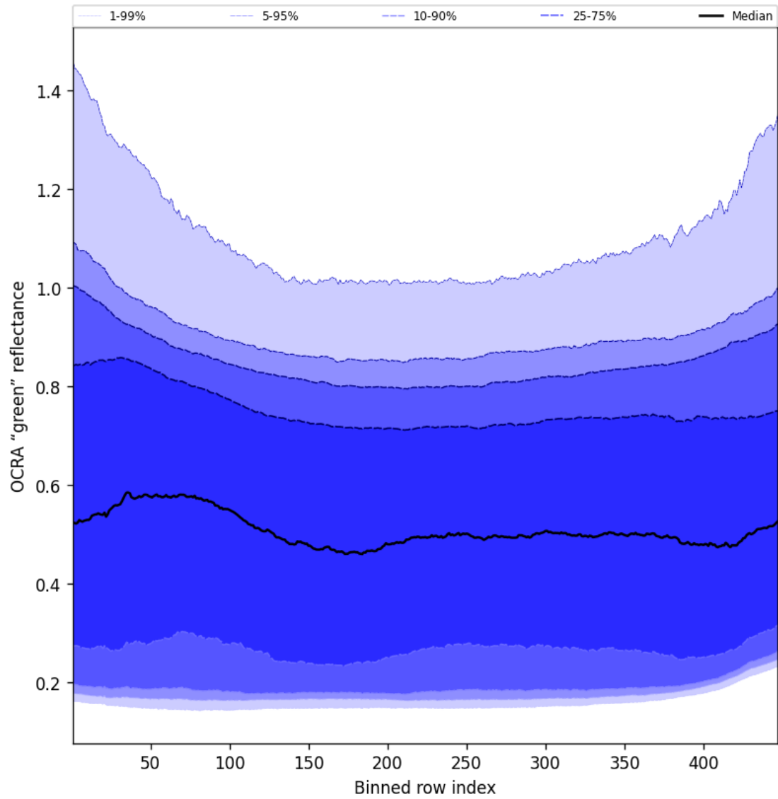
Figure 66: Along track statistics of “OCRA “green” reflectance” for 2025-03-19 to 2025-03-20
