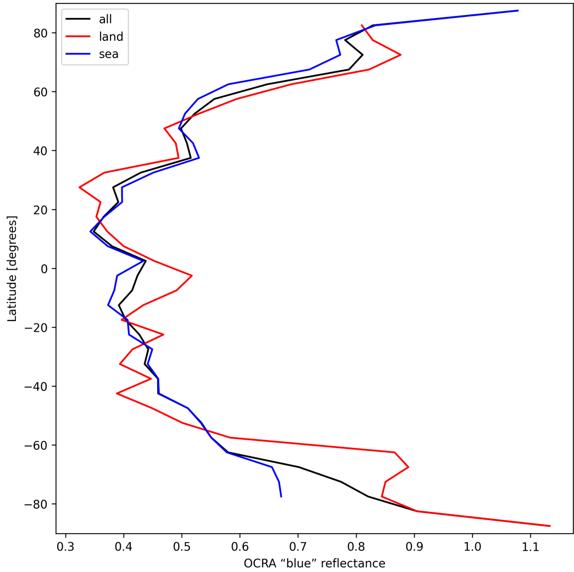
Figure 33: Zonal average of "OCRA "blue" reflectance" for 2025-03-19 to 2025-03-20.
