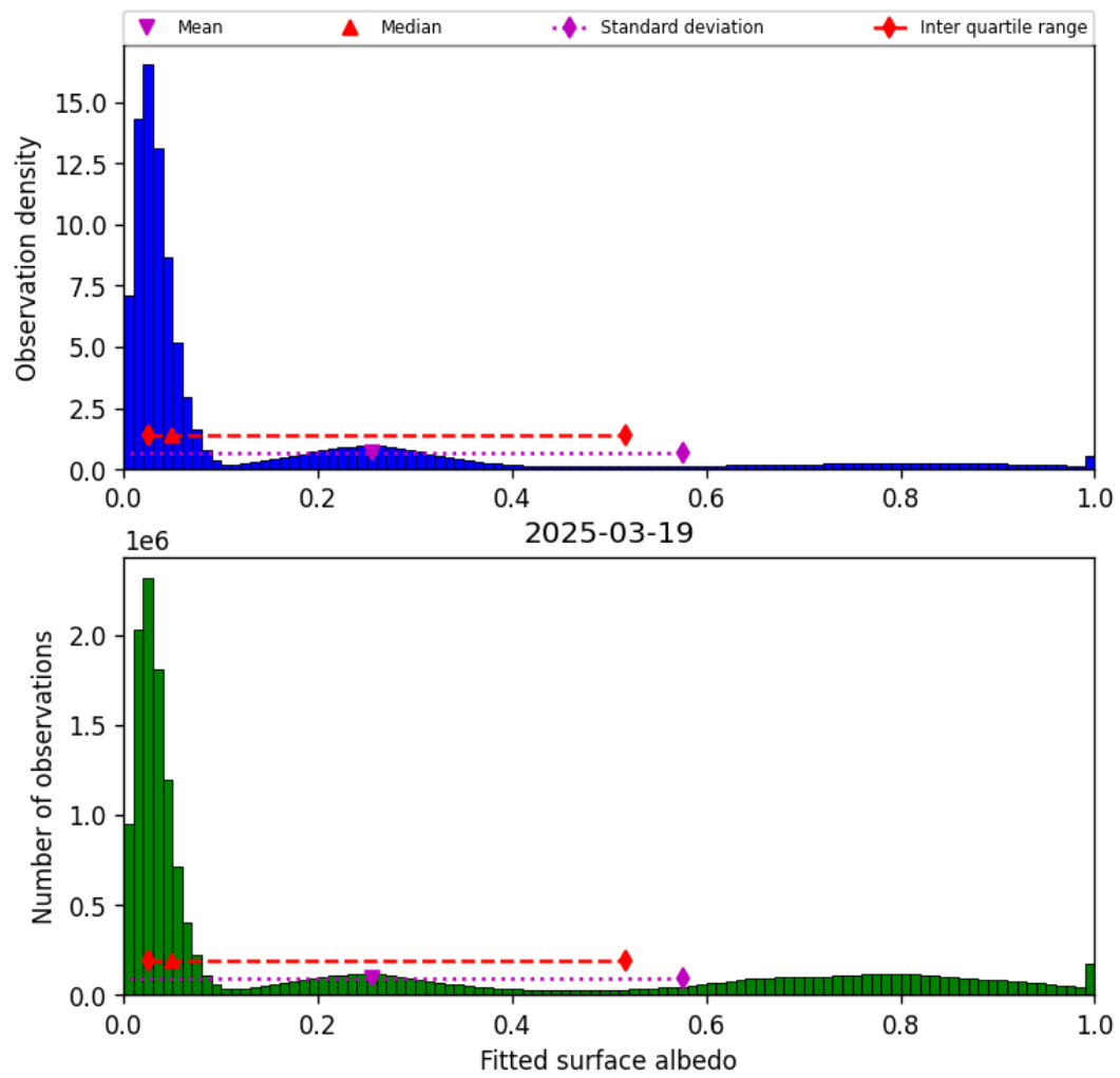
Figure 43: Histogram of “Fitted surface albedo” for 2025-03-19 to 2025-03-20
