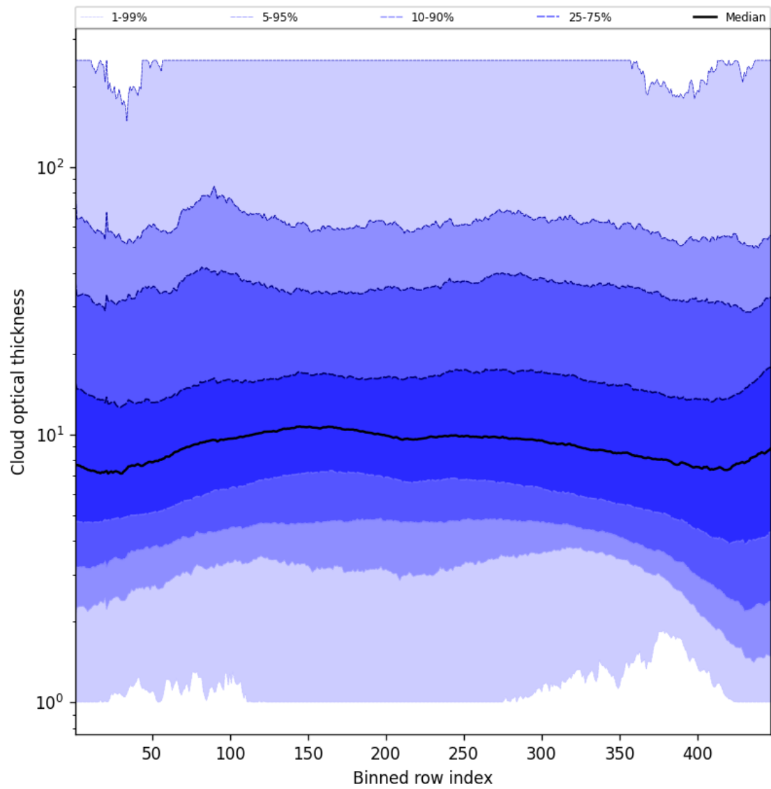
Figure 55: Along track statistics of “Cloud optical thickness” for 2025-03-19 to 2025-03-20
