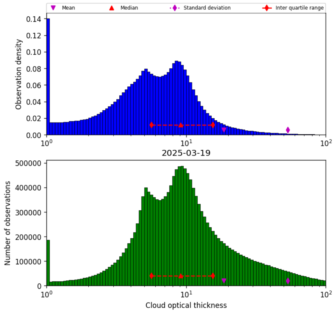
Figure 39: Histogram of “Cloud optical thickness” for 2025-03-19 to 2025-03-20
