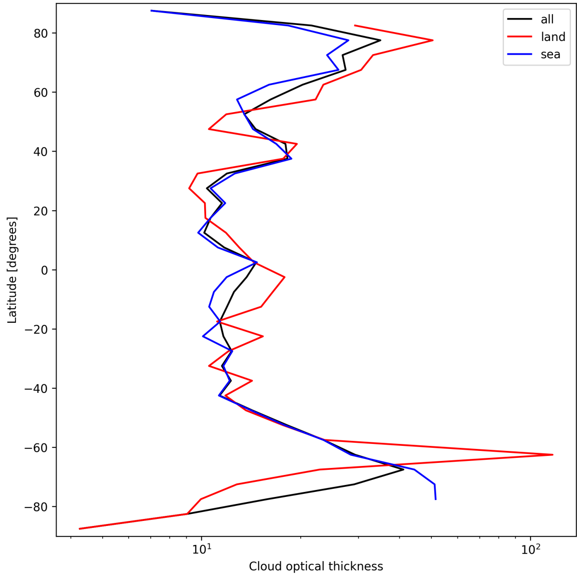
Figure 23: Zonal average of “Cloud optical thickness” for 2025-03-19 to 2025-03-20.
