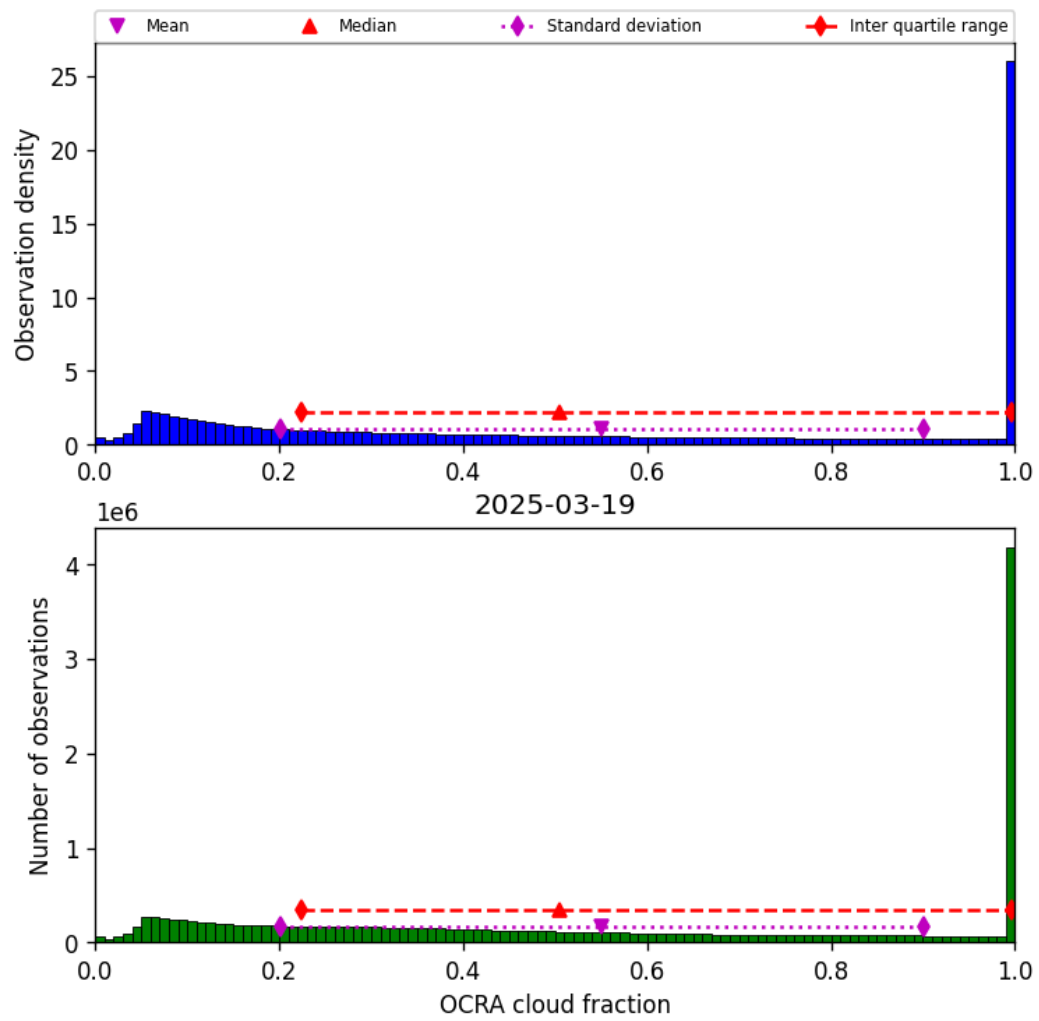
Figure 48: Histogram of “OCRA cloud fraction” for 2025-03-19 to 2025-03-20
