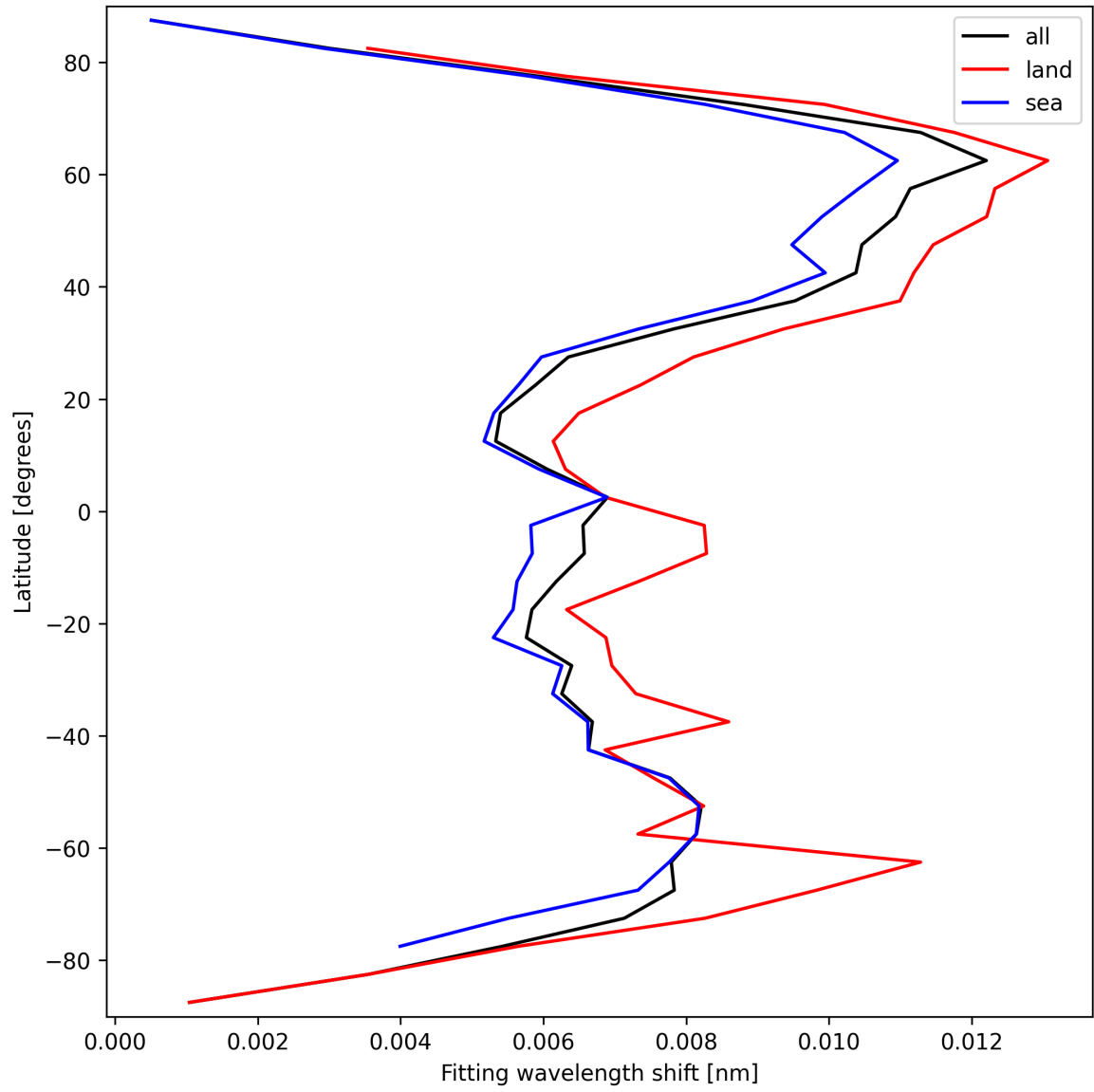
Figure 31: Zonal average of “Fitting wavelength shift” for 2025-03-19 to 2025-03-20.
