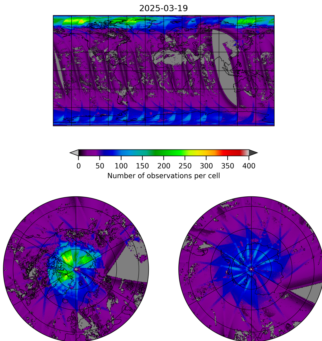
Figure 19: Map of the number of observations for 2025-03-19 to 2025-03-20
