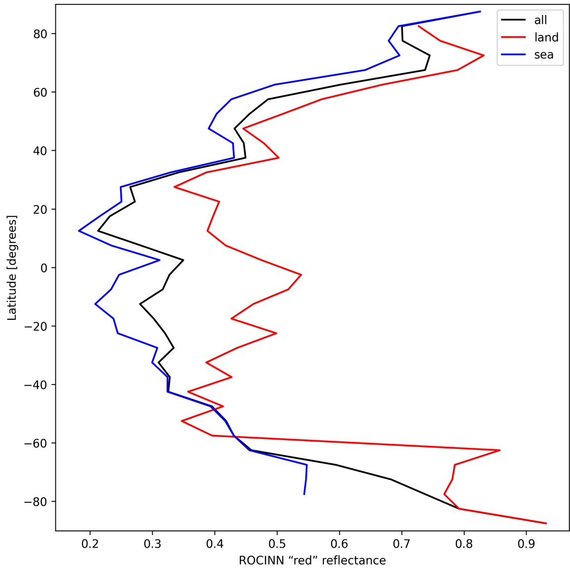
Figure 35: Zonal average of “ROCINN “red” reflectance” for 2025-03-19 to 2025-03-20.
