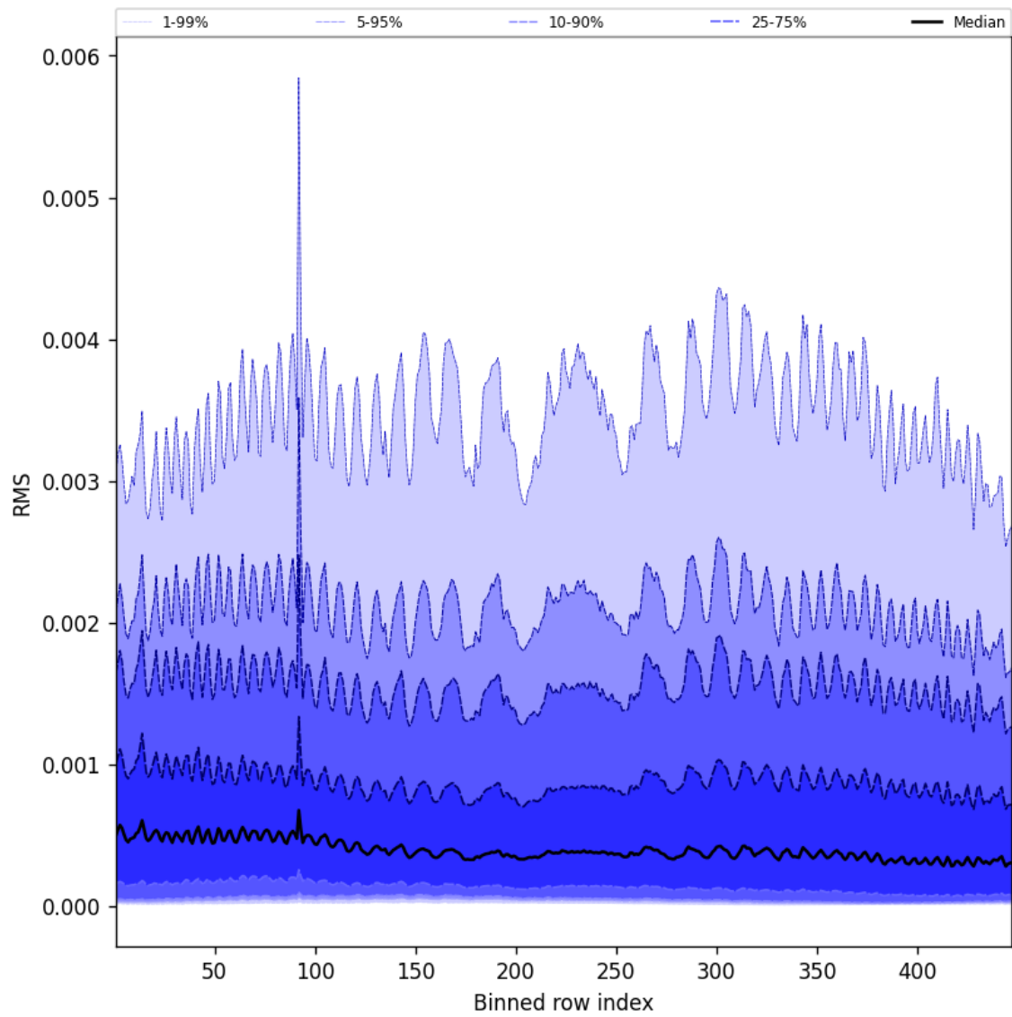
Figure 61: Along track statistics of “RMS” for 2025-03-19 to 2025-03-20
