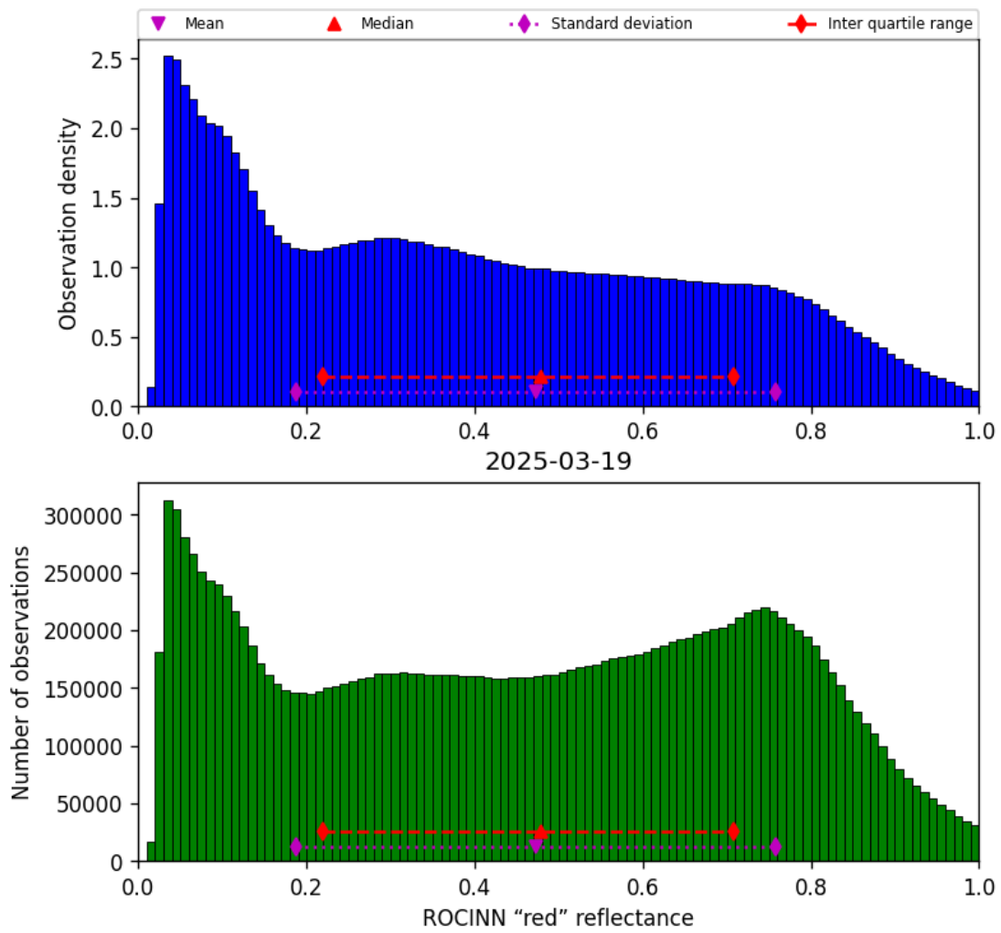
Figure 51: Histogram of “ROCINN “red” reflectance” for 2025-03-19 to 2025-03-20
