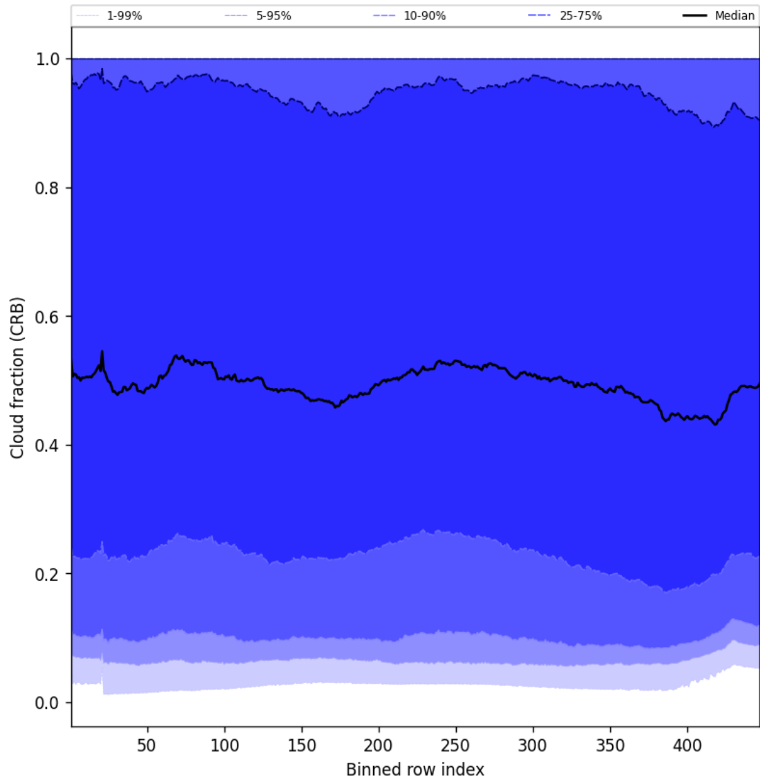
Figure 56: Along track statistics of “Cloud fraction (CRB)” for 2025-03-19 to 2025-03-20
