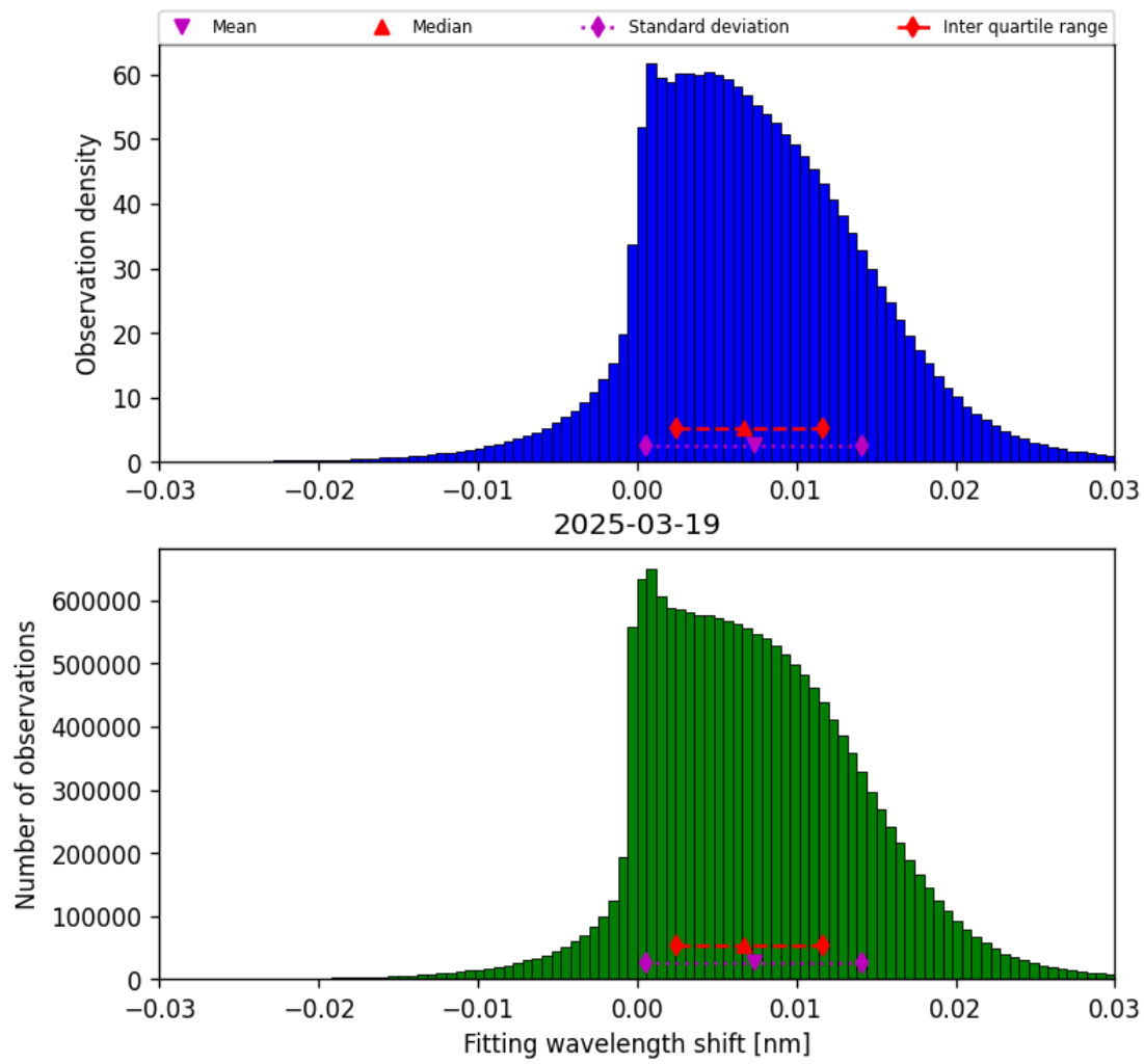
Figure 47: Histogram of “Fitting wavelength shift” for 2025-03-19 to 2025-03-20
