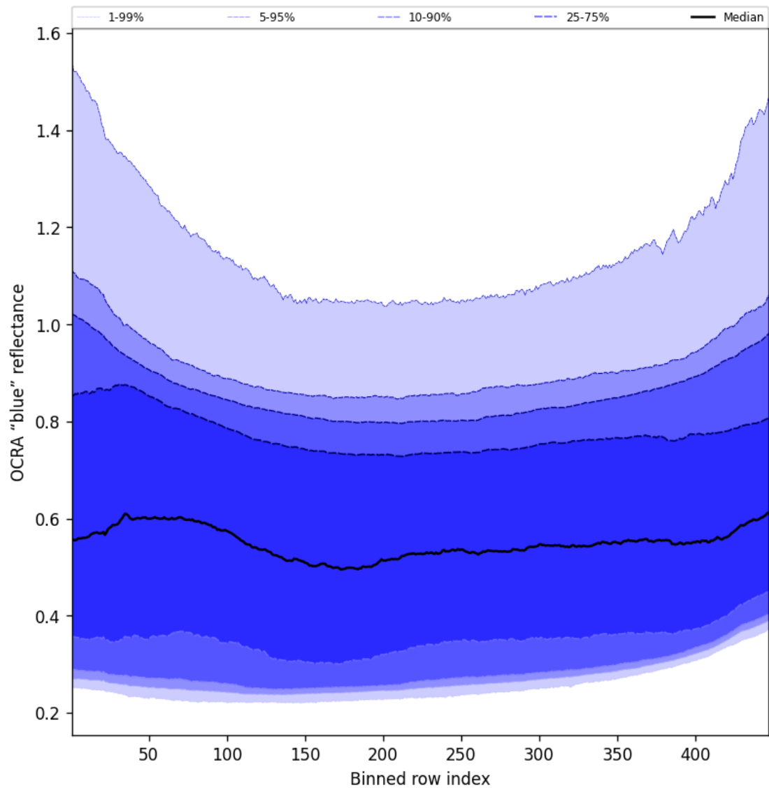
Figure 65: Along track statistics of “OCRA “blue” reflectance” for 2025-03-19 to 2025-03-20
