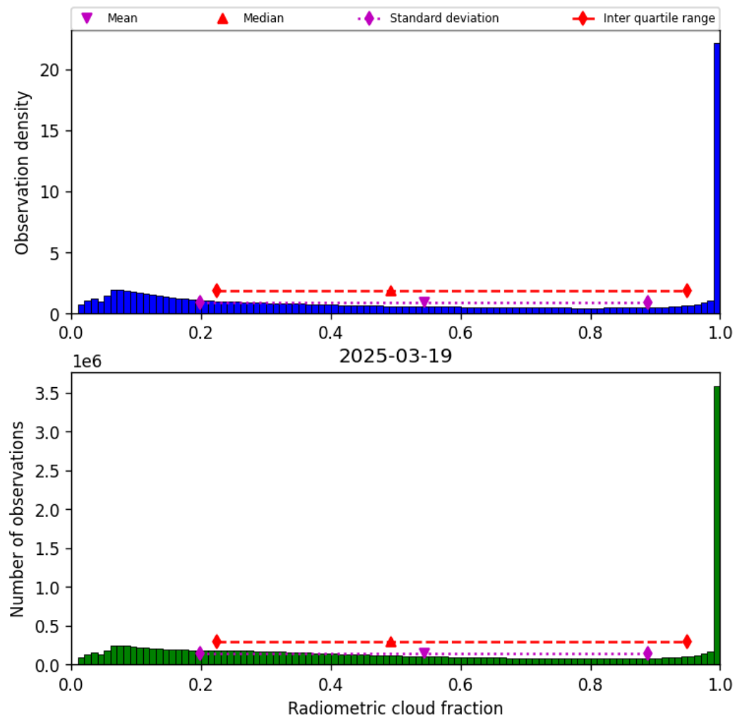
Figure 37: Histogram of “Radiometric cloud fraction” for 2025-03-19 to 2025-03-20
