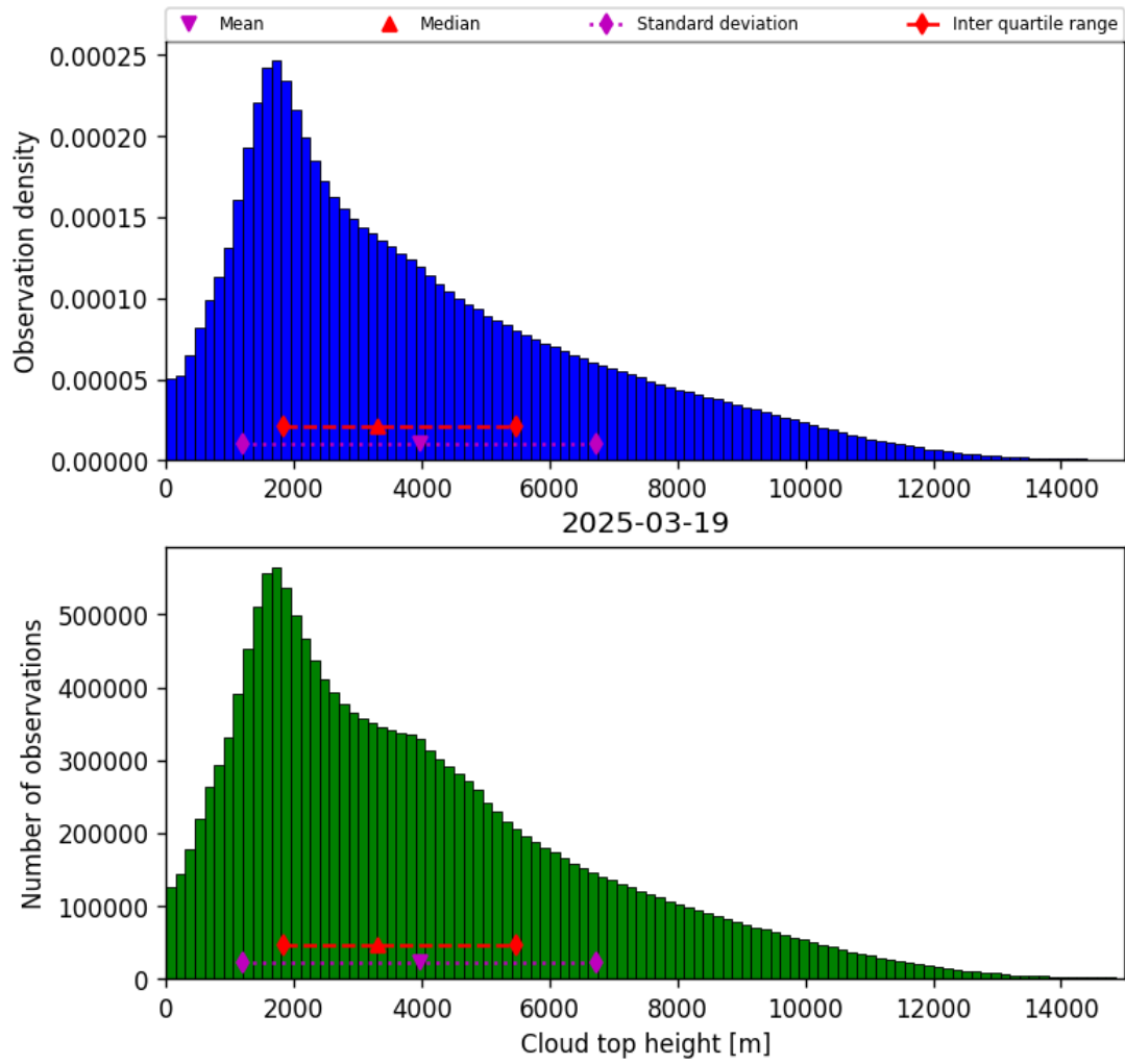
Figure 38: Histogram of “Cloud top height” for 2025-03-19 to 2025-03-20
