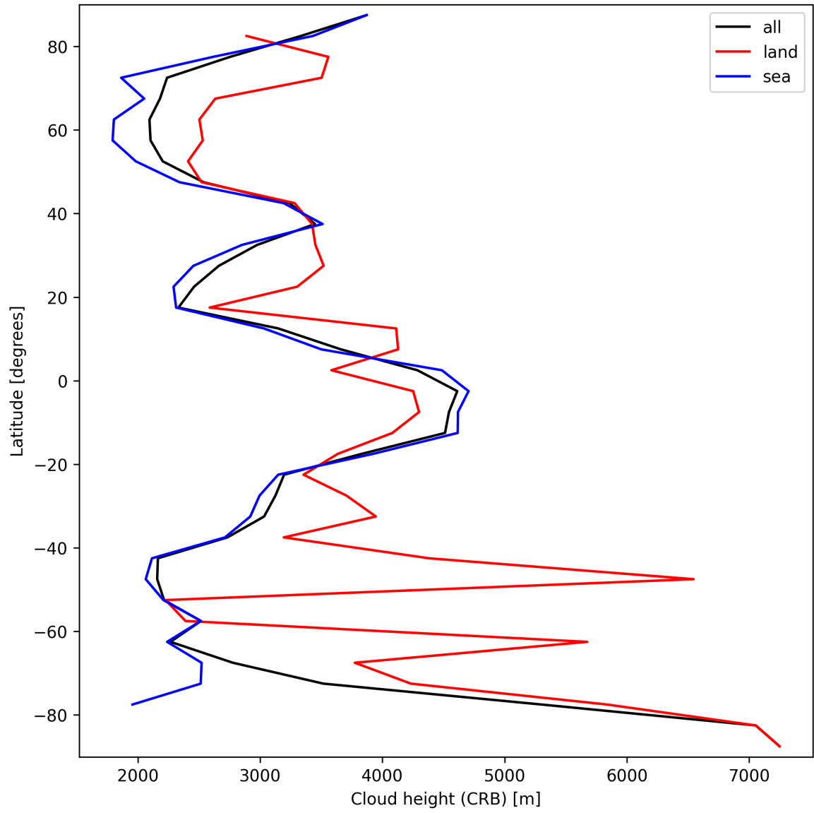
Figure 25: Zonal average of “Cloud height (CRB)” for 2025-03-19 to 2025-03-20.
