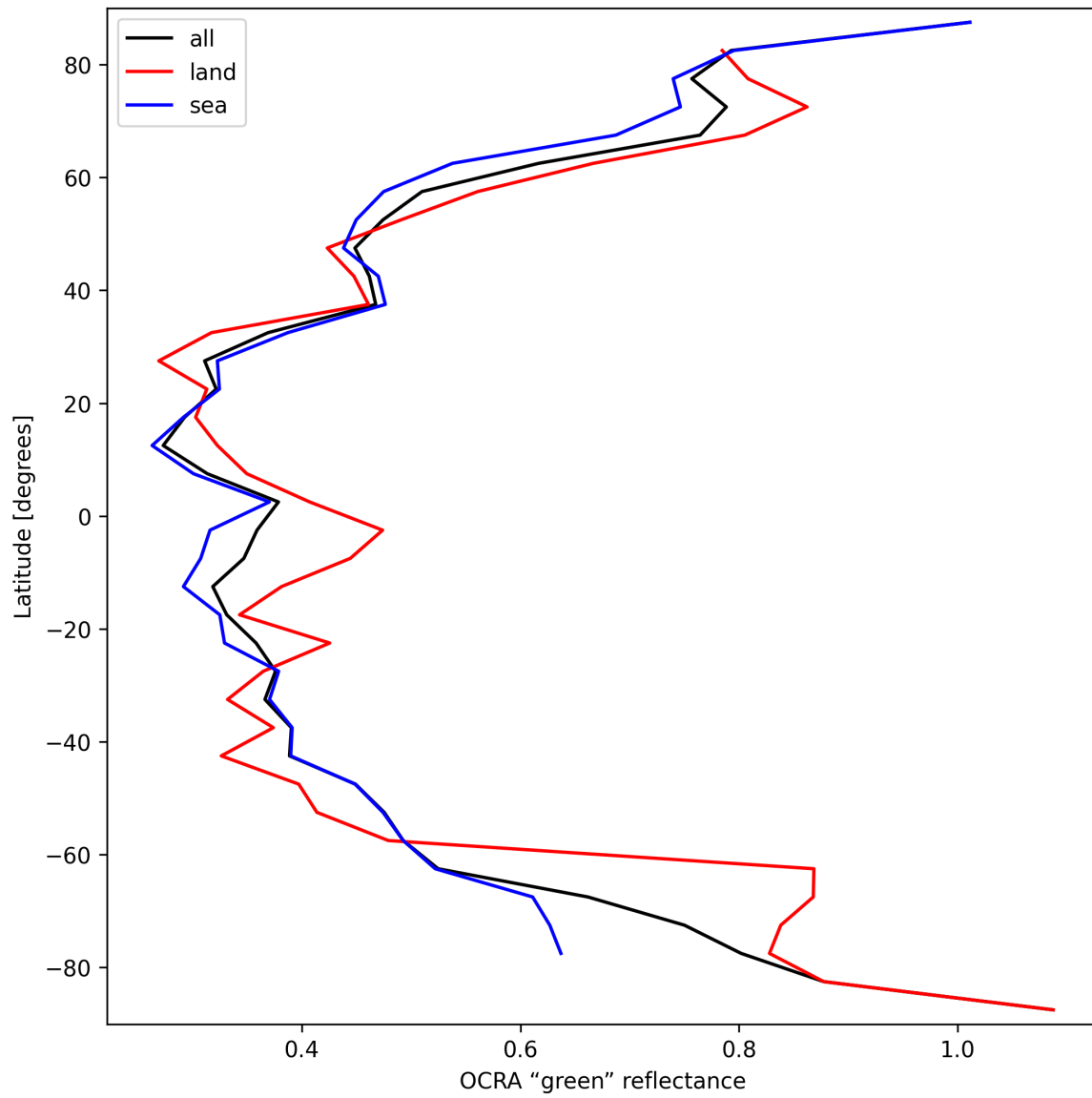
Figure 34: Zonal average of “OCRA “green” reflectance” for 2025-03-19 to 2025-03-20.
