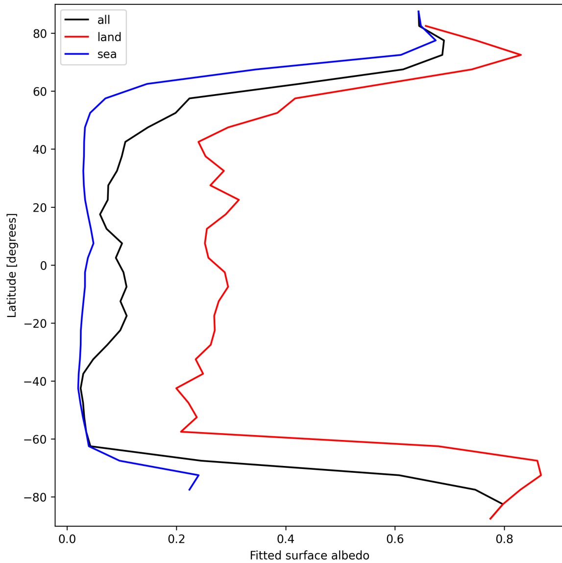
Figure 27: Zonal average of “Fitted surface albedo” for 2025-03-19 to 2025-03-20.
