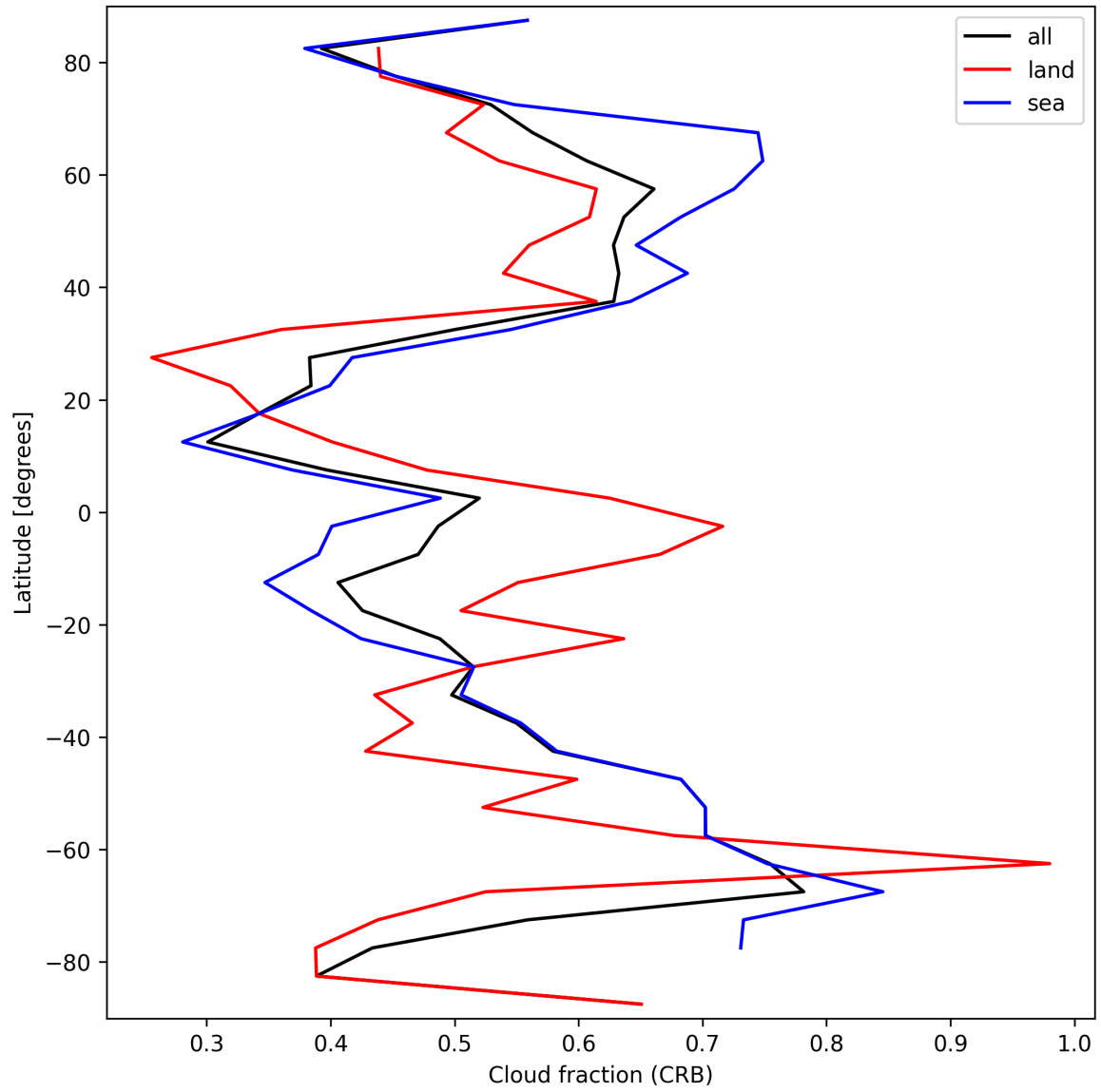
Figure 24: Zonal average of “Cloud fraction (CRB)” for 2025-03-19 to 2025-03-20.
