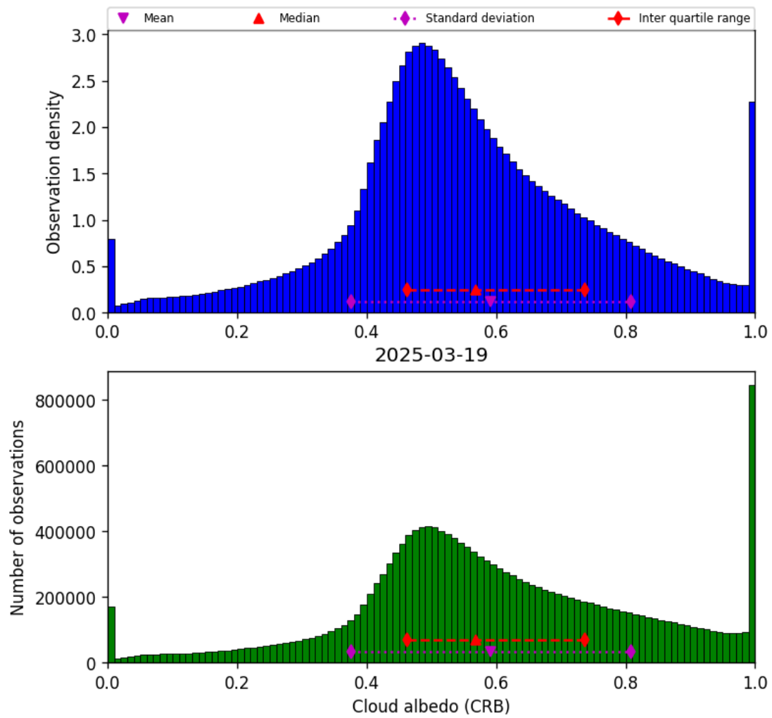
Figure 42: Histogram of “Cloud albedo (CRB)” for 2025-03-19 to 2025-03-20
