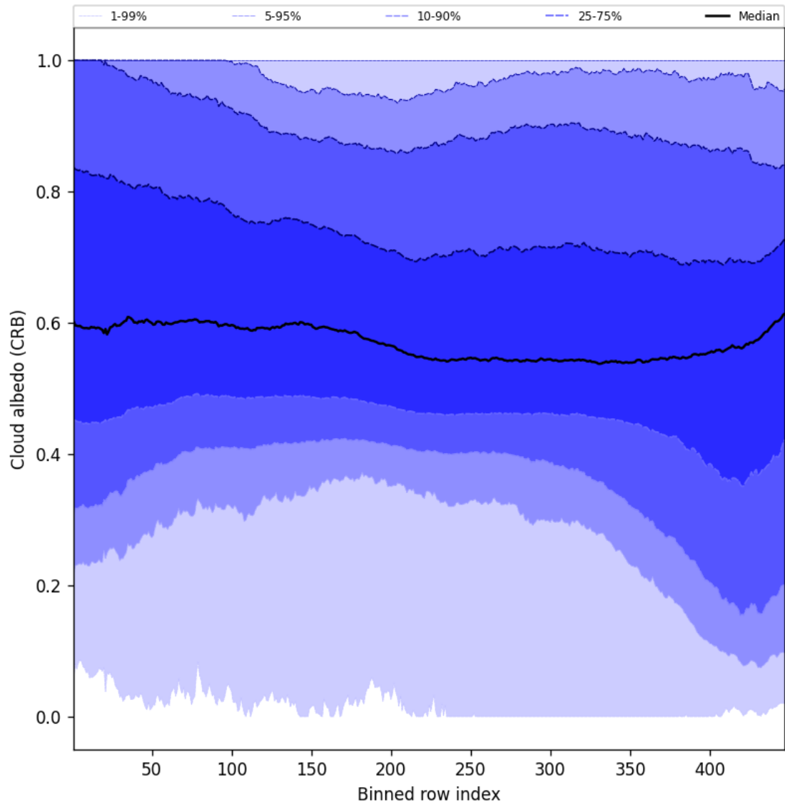
Figure 58: Along track statistics of “Cloud albedo (CRB)” for 2025-03-19 to 2025-03-20
