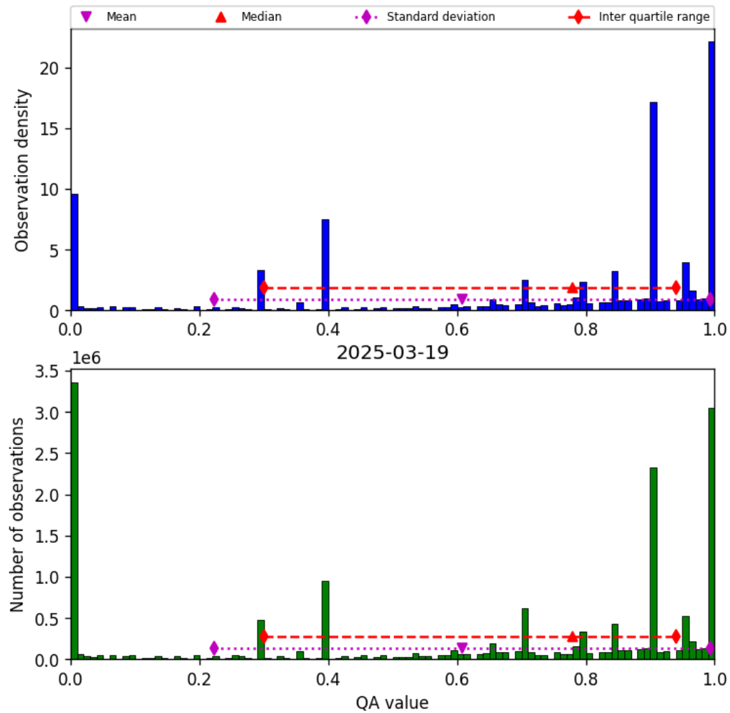
Figure 36: Histogram of “QA value” for 2025-03-19 to 2025-03-20
