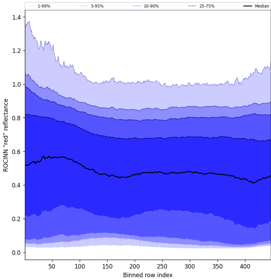
Figure 67: Along track statistics of "ROCINN "red" reflectance" for 2025-03-19 to 2025-03-20
