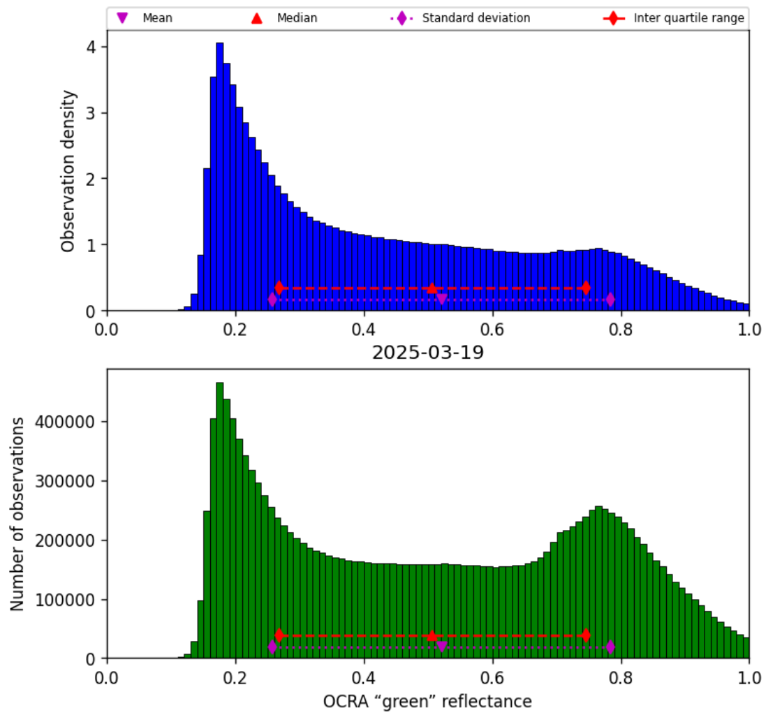
Figure 50: Histogram of “OCRA “green” reflectance” for 2025-03-19 to 2025-03-20
