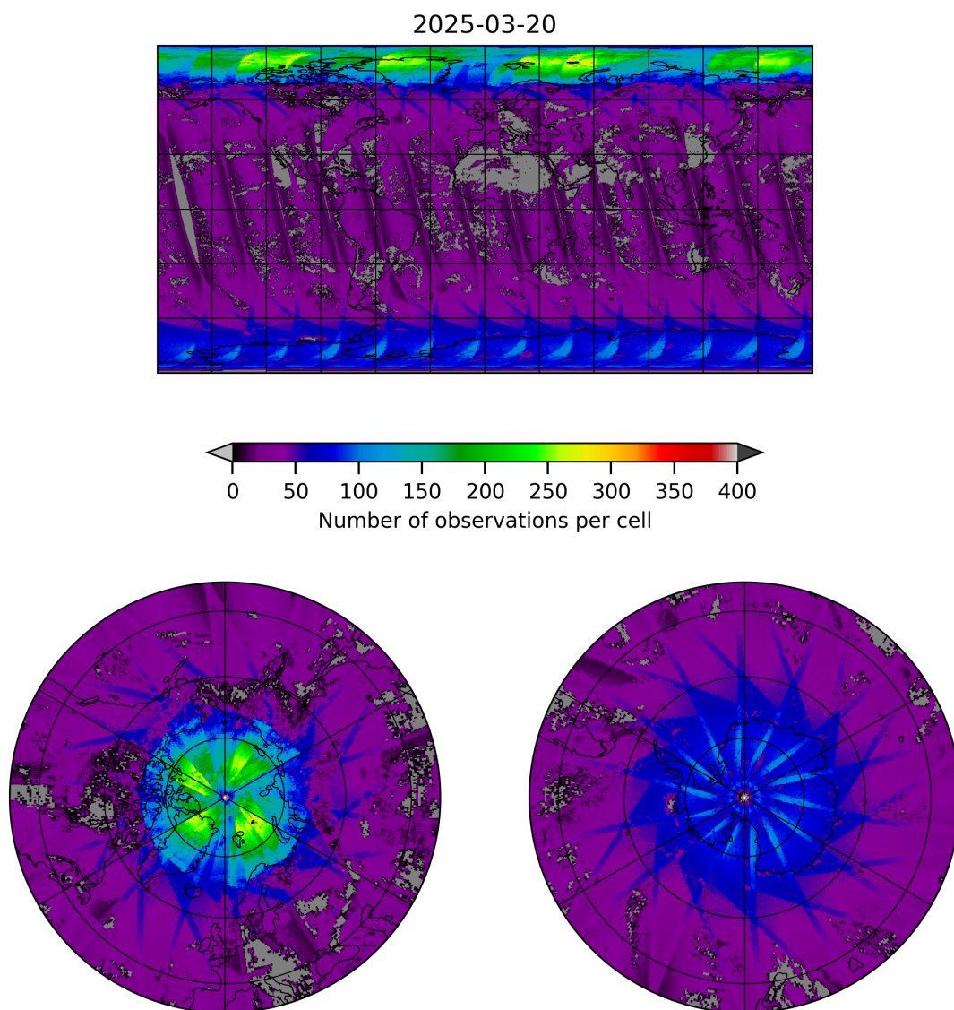
Figure 19: Map of the number of observations for 2025-03-20 to 2025-03-21
