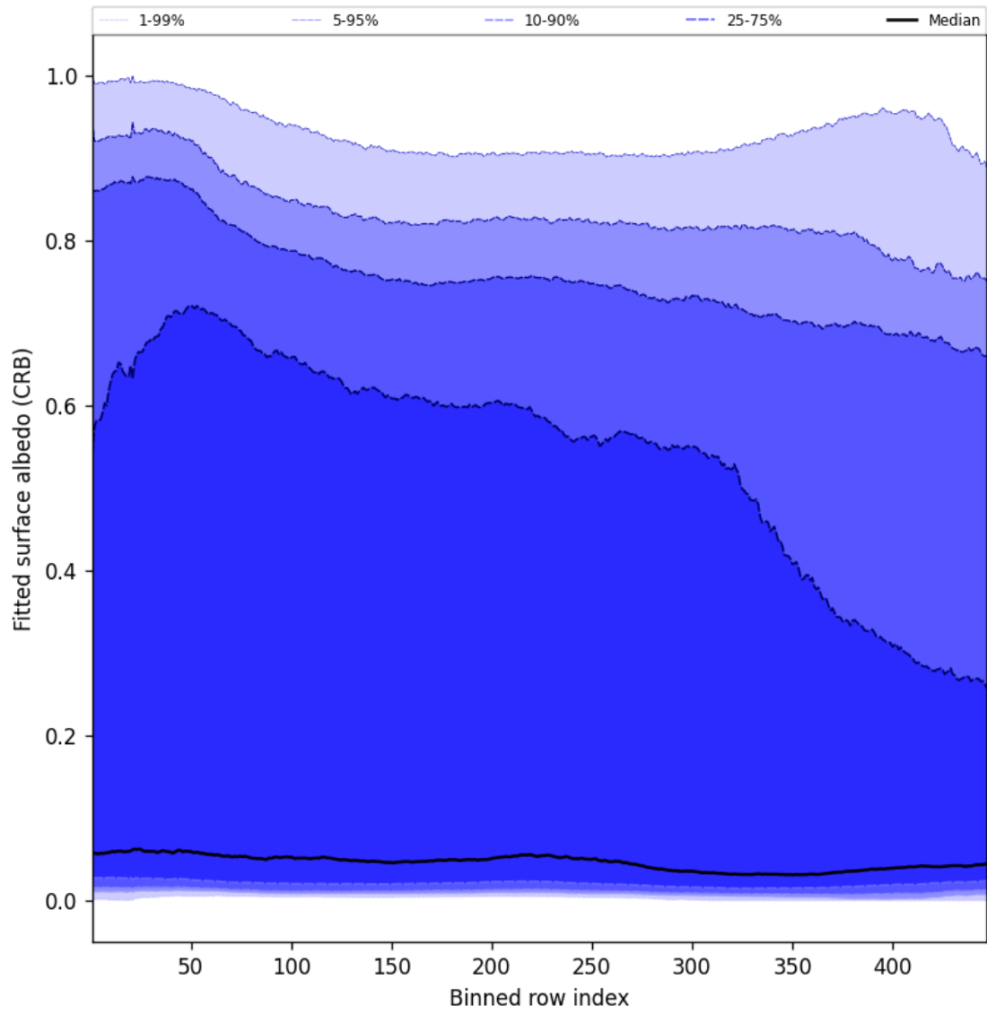
Figure 60: Along track statistics of “Fitted surface albedo (CRB)” for 2025-03-20 to 2025-03-21
