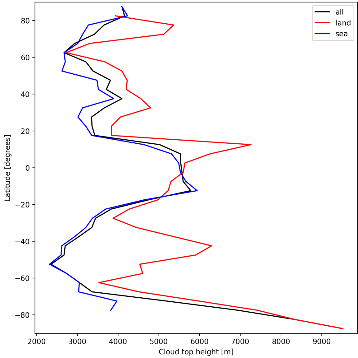
Figure 22: Zonal average of “Cloud top height” for 2025-03-20 to 2025-03-21.
