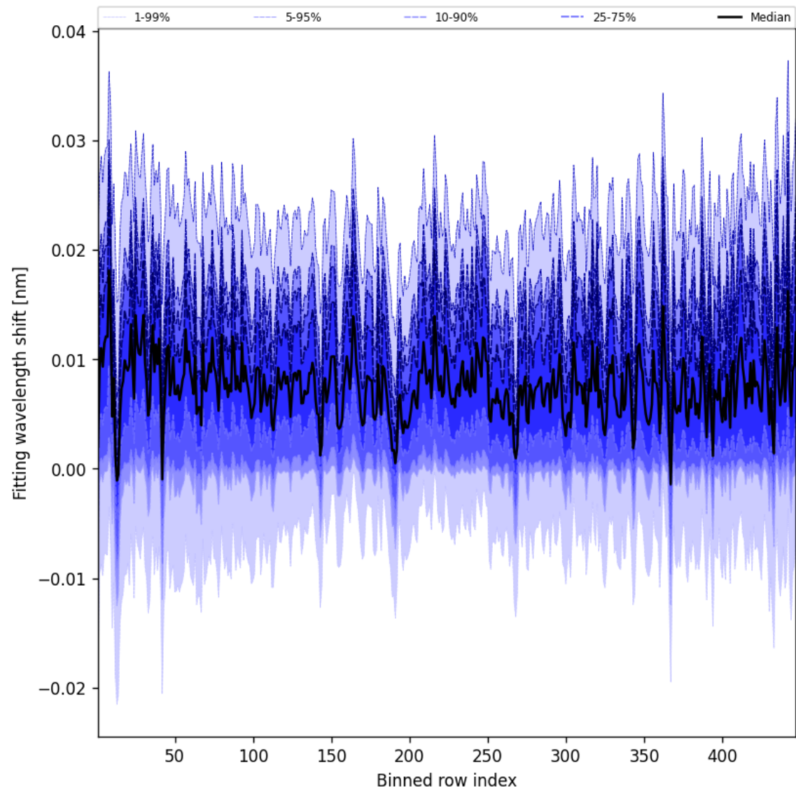
Figure 63: Along track statistics of “Fitting wavelength shift” for 2025-03-20 to 2025-03-21
