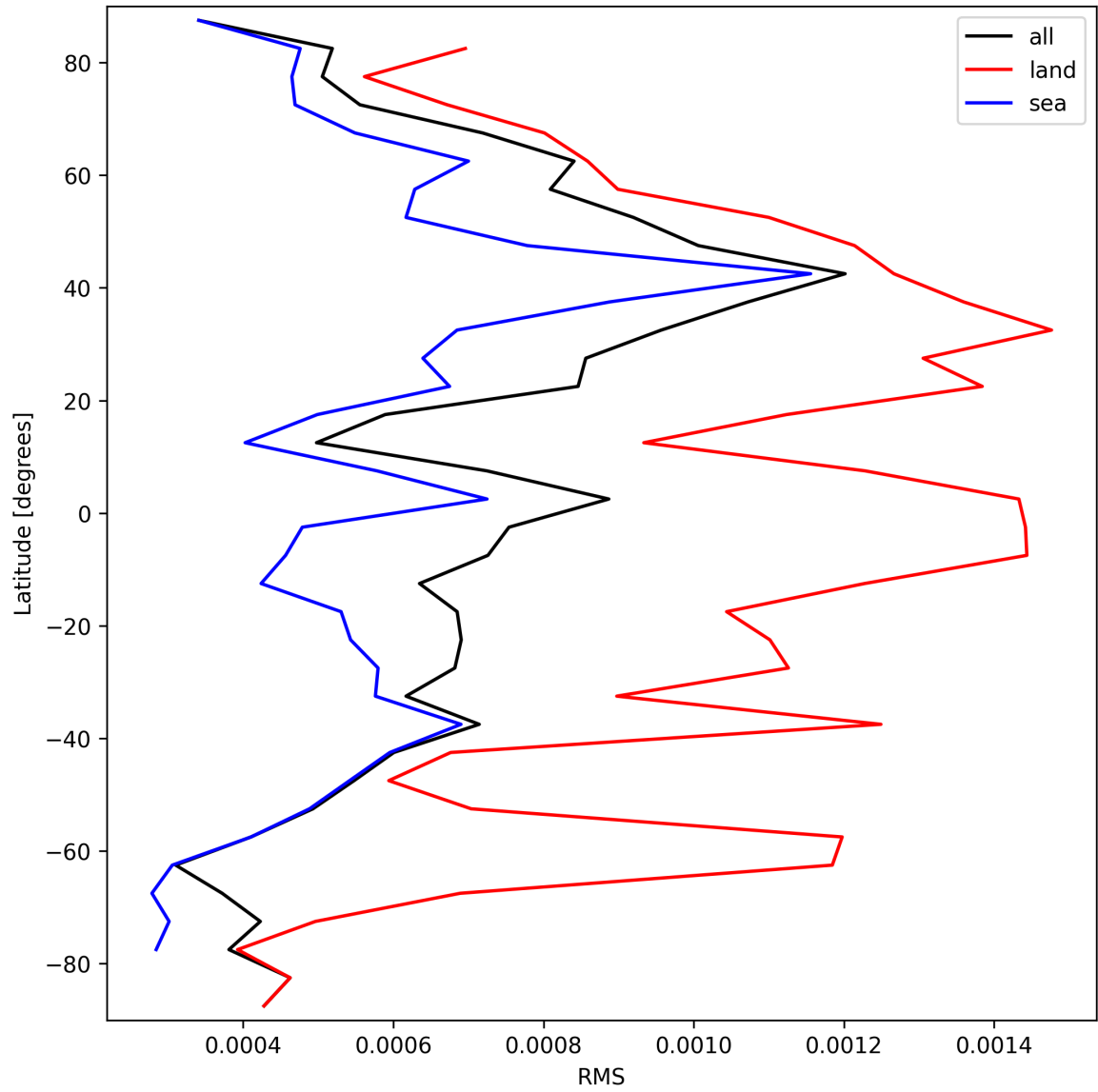
Figure 29: Zonal average of “RMS” for 2025-03-20 to 2025-03-21.
