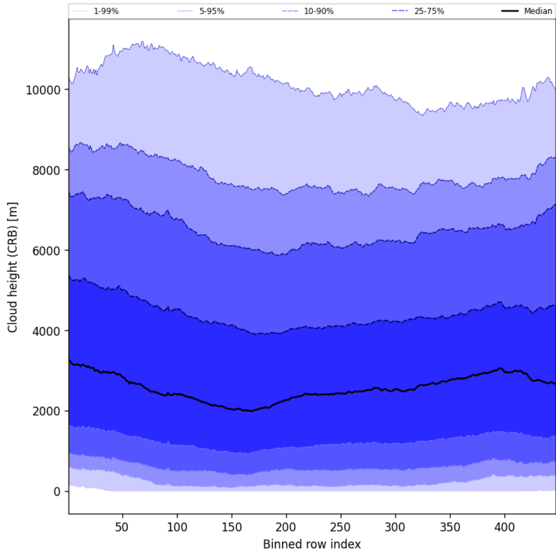
Figure 57: Along track statistics of “Cloud height (CRB)” for 2025-03-20 to 2025-03-21
