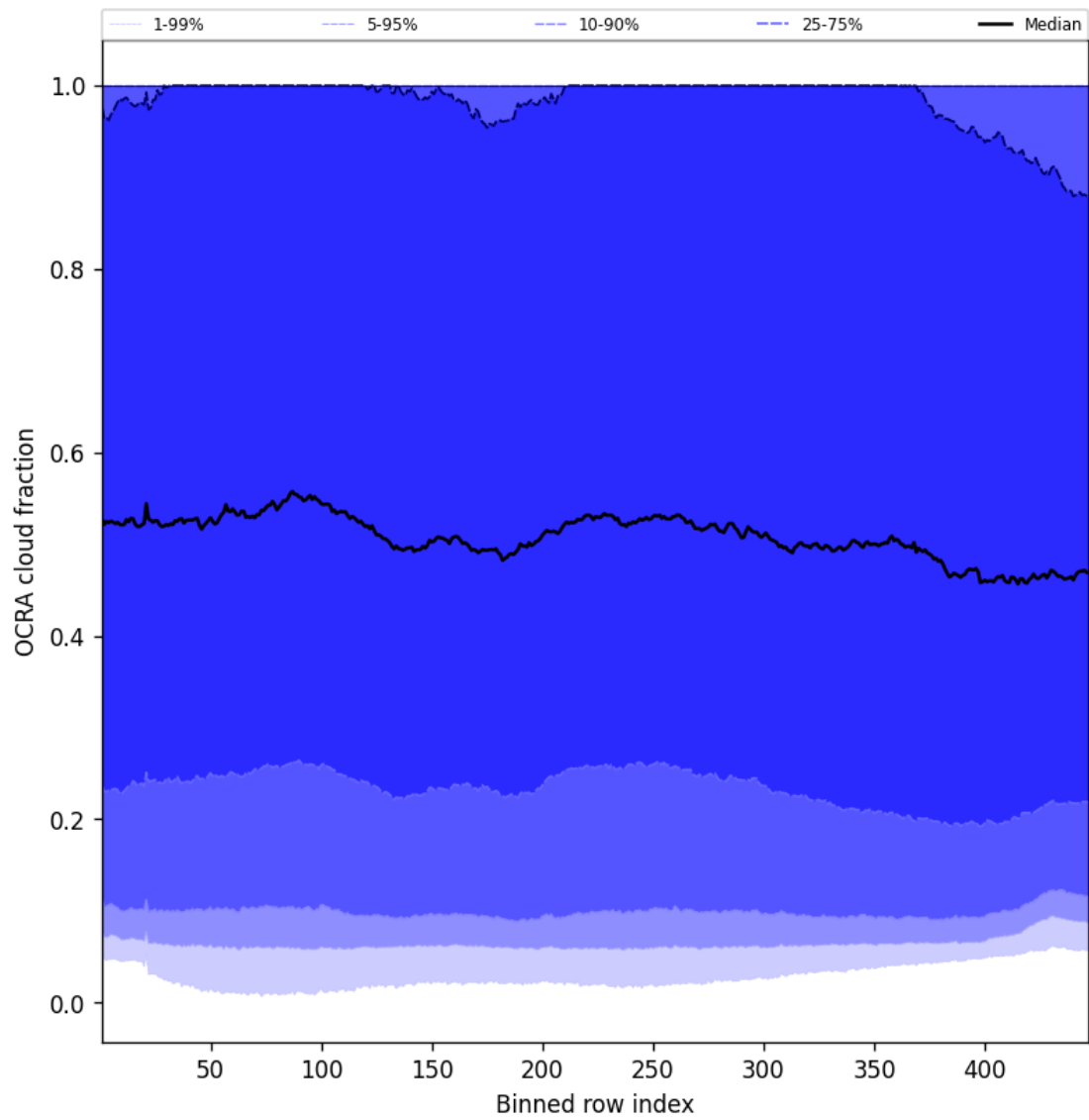
Figure 64: Along track statistics of “OCRA cloud fraction” for 2025-03-20 to 2025-03-21
