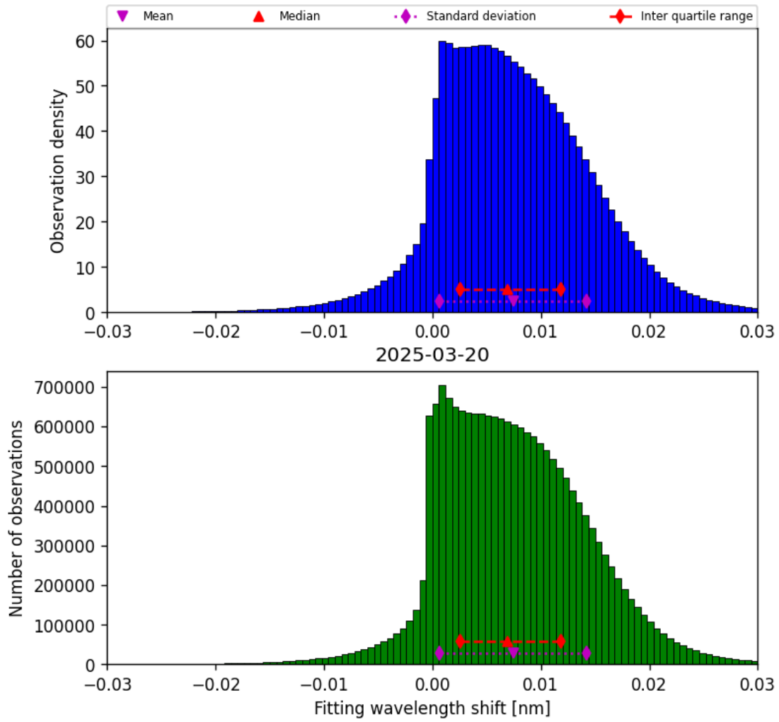
Figure 47: Histogram of “Fitting wavelength shift” for 2025-03-20 to 2025-03-21
