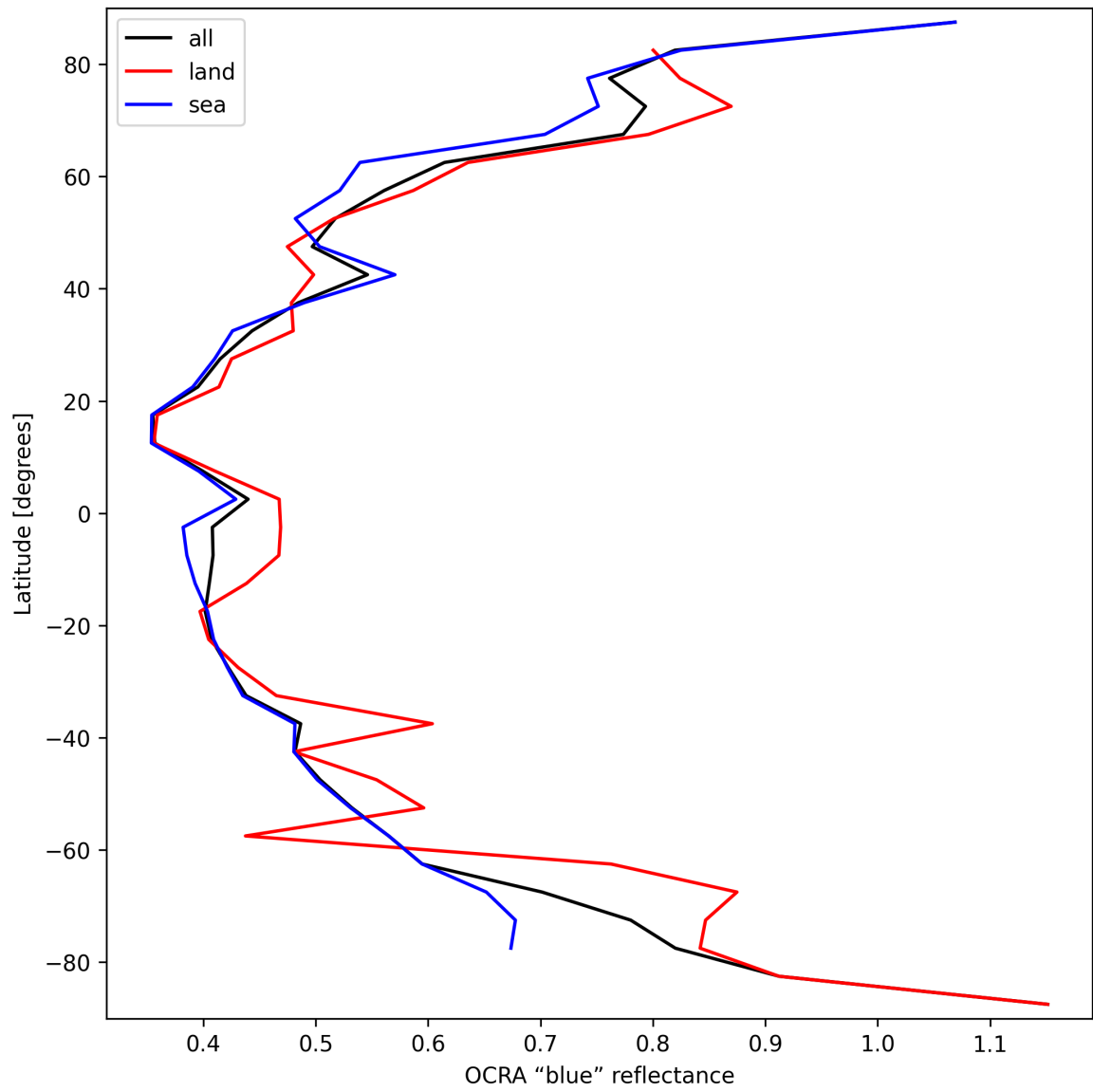
Figure 33: Zonal average of “OCRA “blue” reflectance” for 2025-03-20 to 2025-03-21.
