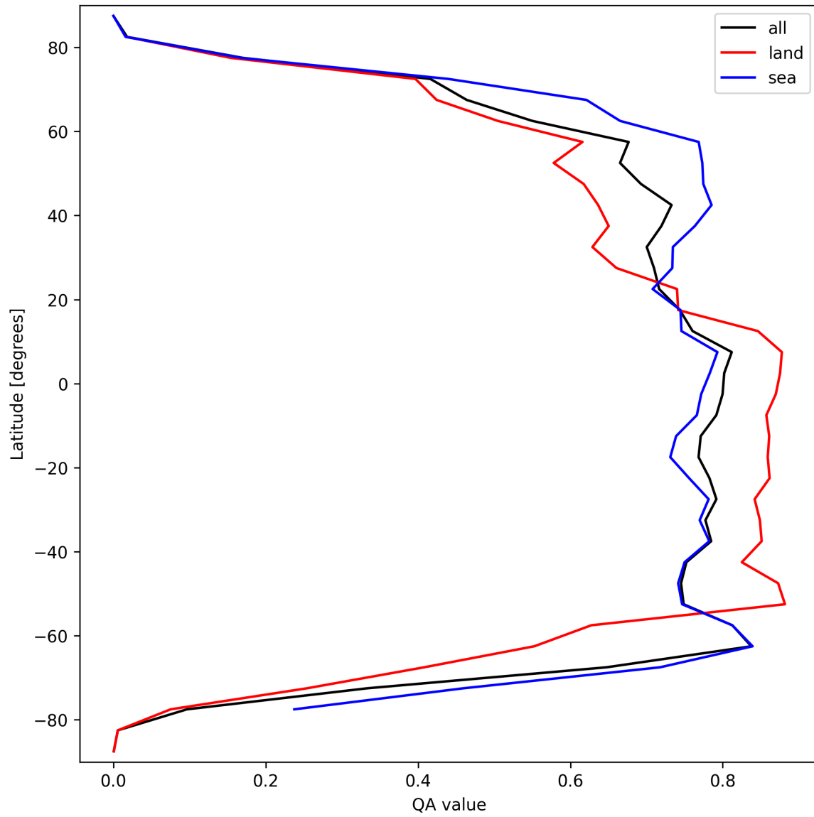
Figure 20: Zonal average of “QA value” for 2025-03-20 to 2025-03-21.
