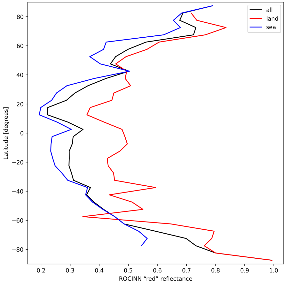
Figure 35: Zonal average of “ROCINN “red” reflectance” for 2025-03-20 to 2025-03-21.
