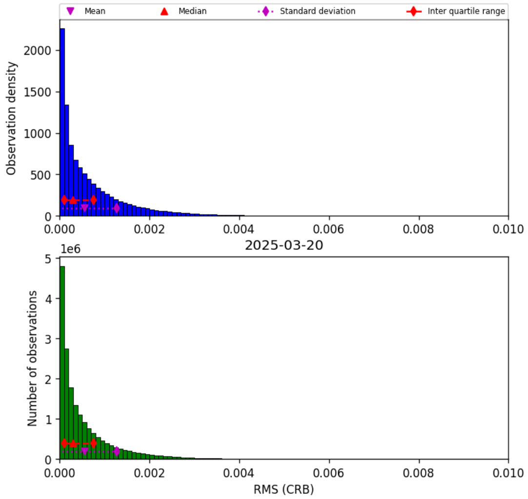
Figure 46: Histogram of "RMS (CRB)" for 2025-03-20 to 2025-03-21
