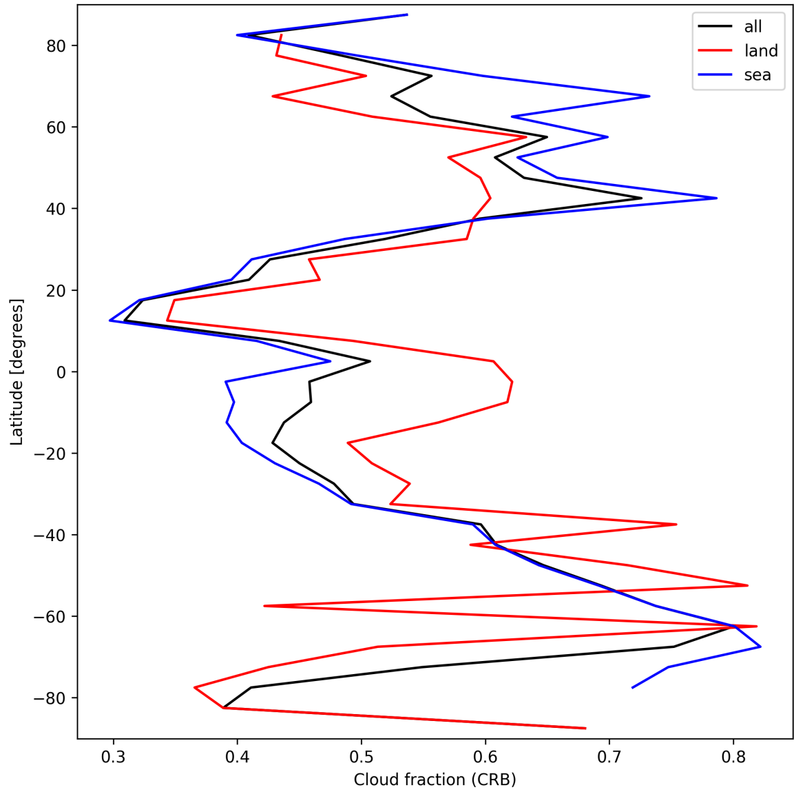
Figure 24: Zonal average of “Cloud fraction (CRB)” for 2025-03-20 to 2025-03-21.
