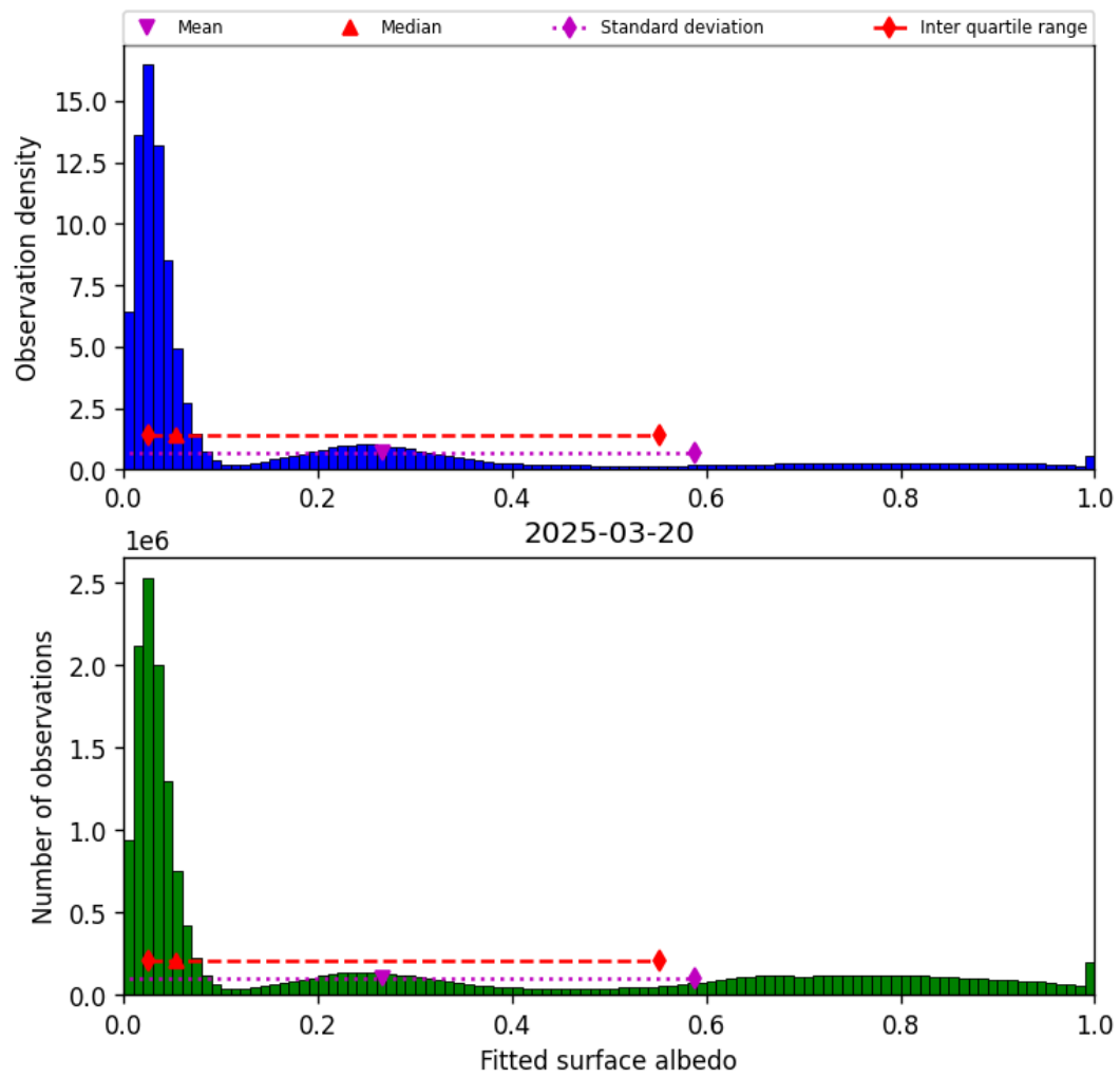
Figure 43: Histogram of “Fitted surface albedo” for 2025-03-20 to 2025-03-21
