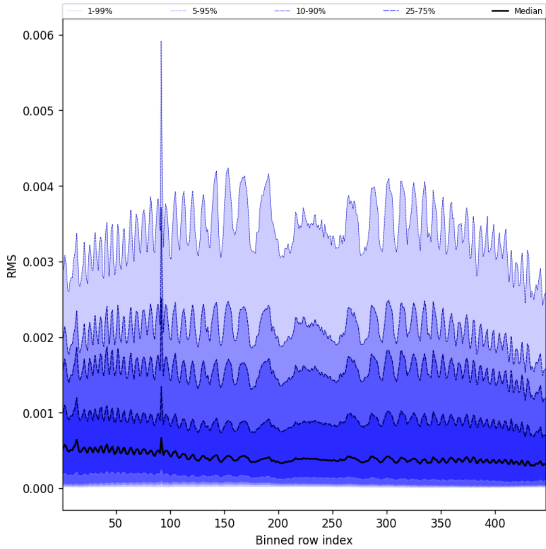
Figure 61: Along track statistics of “RMS” for 2025-03-20 to 2025-03-21
