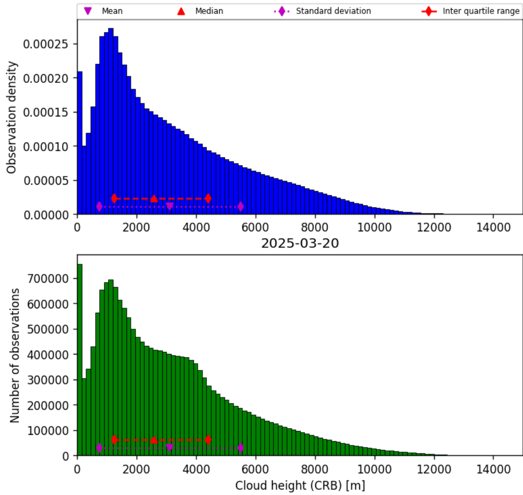
Figure 41: Histogram of “Cloud height (CRB)” for 2025-03-20 to 2025-03-21
