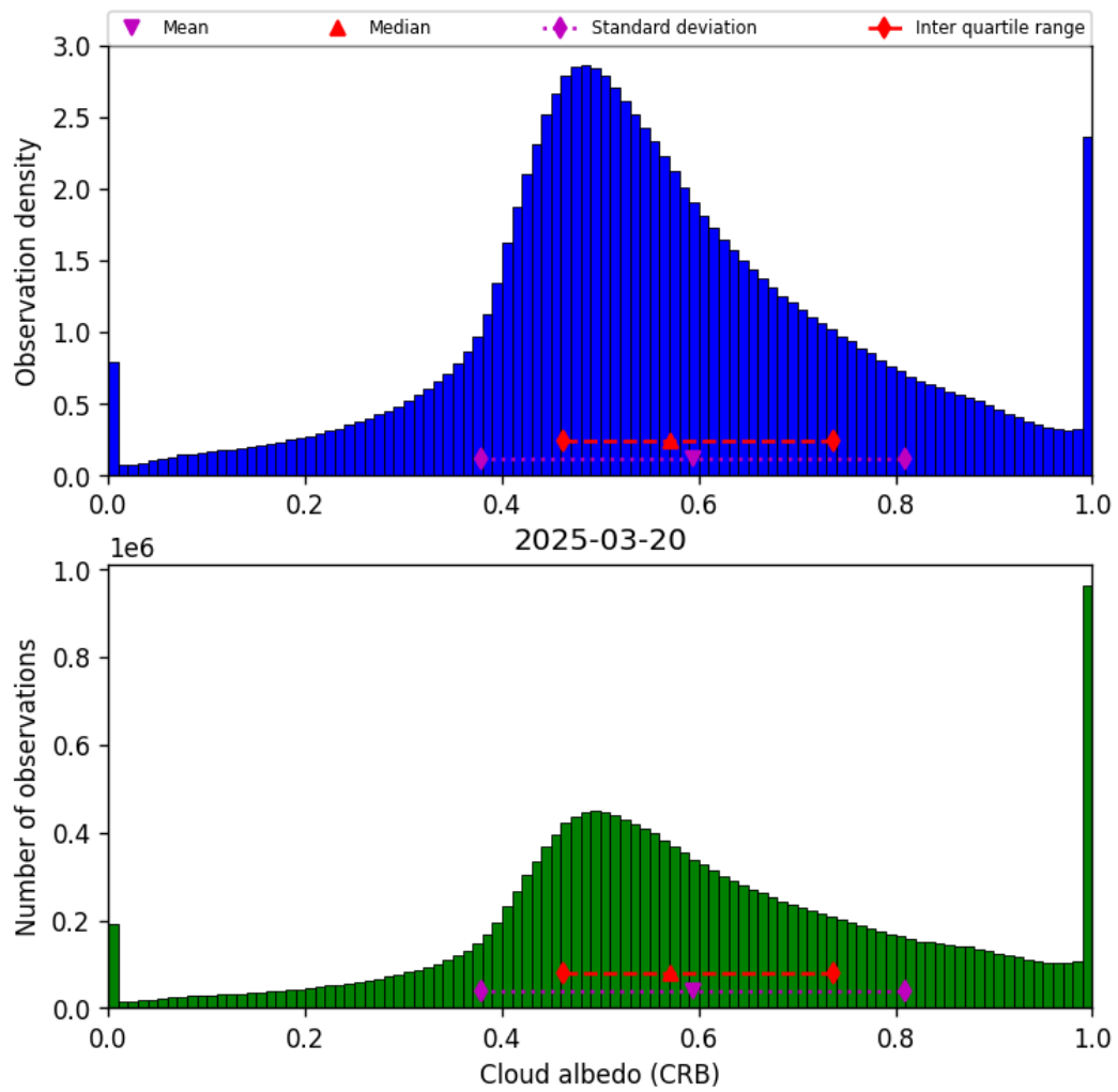
Figure 42: Histogram of “Cloud albedo (CRB)” for 2025-03-20 to 2025-03-21
