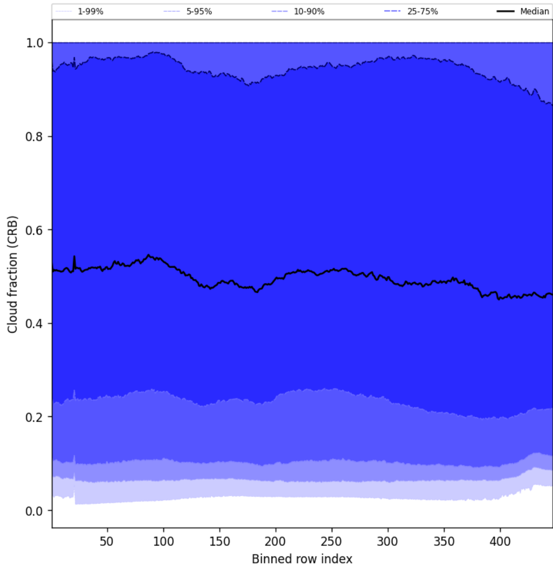
Figure 56: Along track statistics of “Cloud fraction (CRB)” for 2025-03-20 to 2025-03-21
