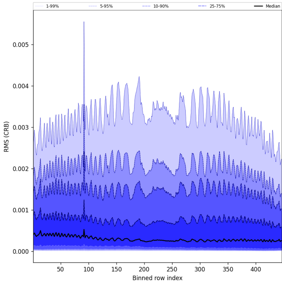
Figure 62: Along track statistics of “RMS (CRB)” for 2025-03-20 to 2025-03-21
