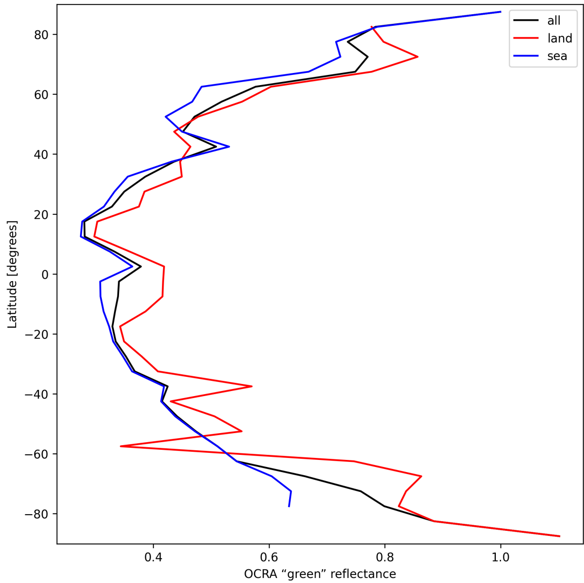
Figure 34: Zonal average of “OCRA “green” reflectance” for 2025-03-20 to 2025-03-21.
