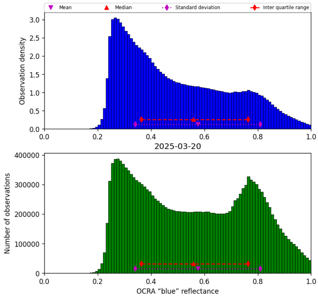
Figure 49: Histogram of “OCRA “blue” reflectance” for 2025-03-20 to 2025-03-21
