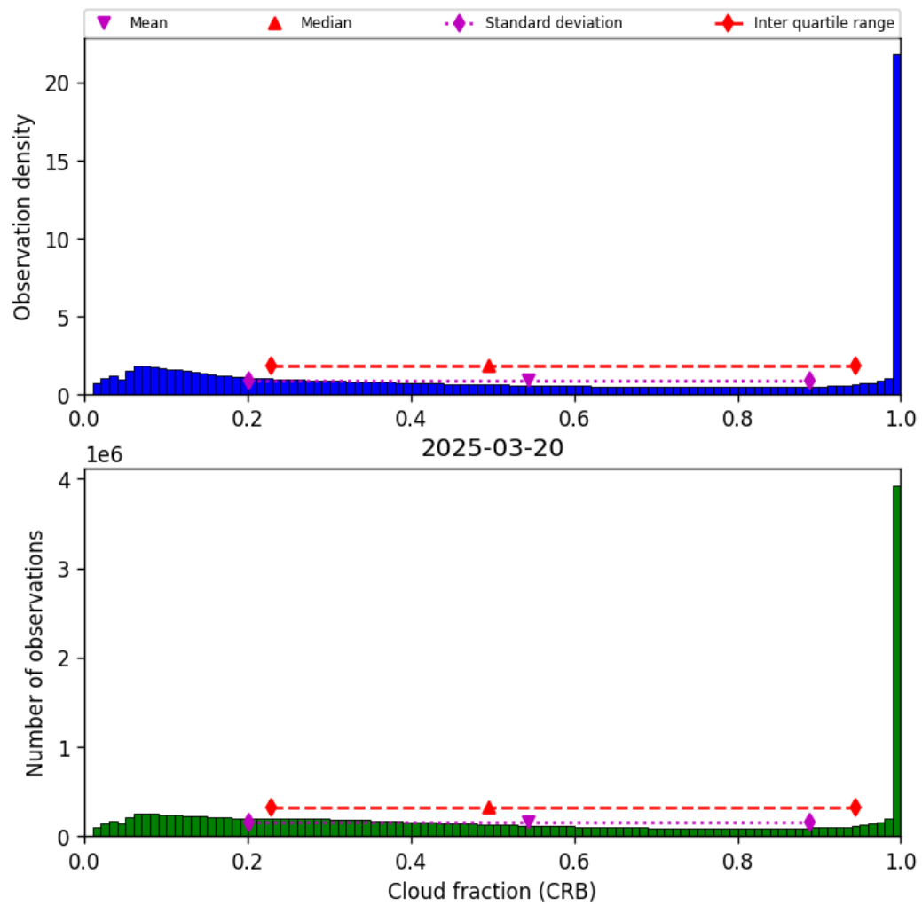
Figure 40: Histogram of “Cloud fraction (CRB)” for 2025-03-20 to 2025-03-21
