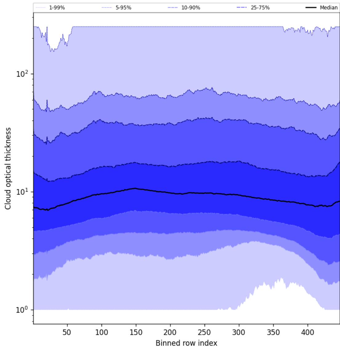
Figure 55: Along track statistics of “Cloud optical thickness” for 2025-03-20 to 2025-03-21
