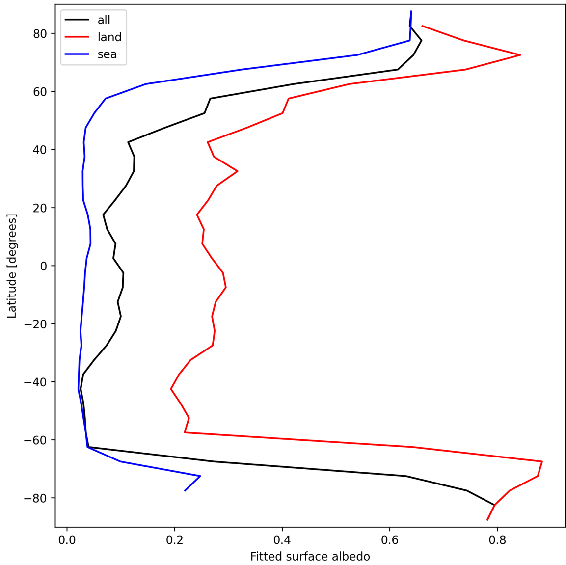
Figure 27: Zonal average of “Fitted surface albedo” for 2025-03-20 to 2025-03-21.
