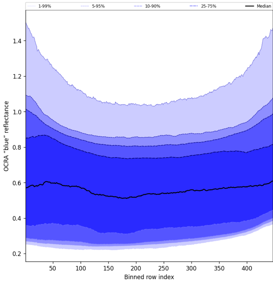
Figure 65: Along track statistics of “OCRA “blue” reflectance” for 2025-03-20 to 2025-03-21
