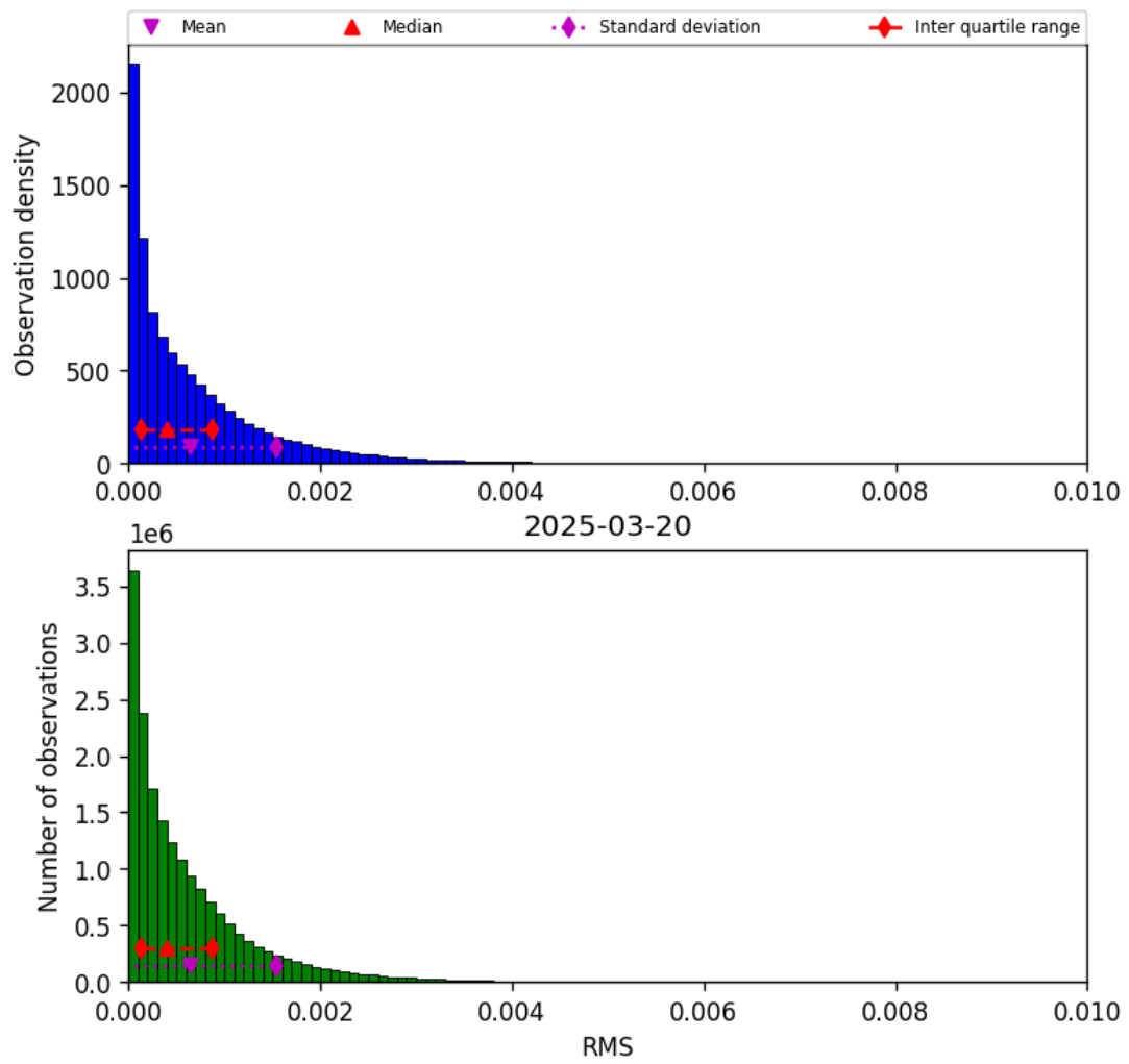
Figure 45: Histogram of “RMS” for 2025-03-20 to 2025-03-21
