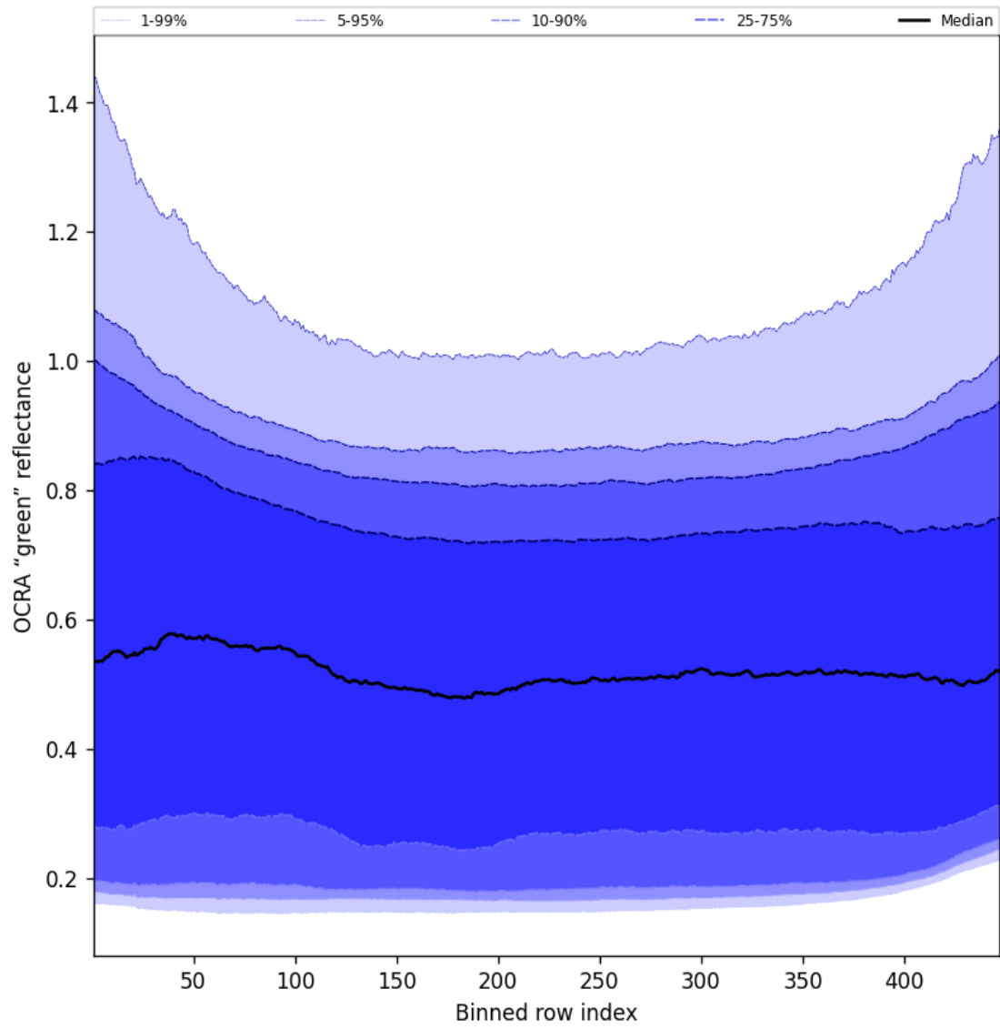
Figure 66: Along track statistics of “OCRA “green” reflectance” for 2025-03-20 to 2025-03-21
