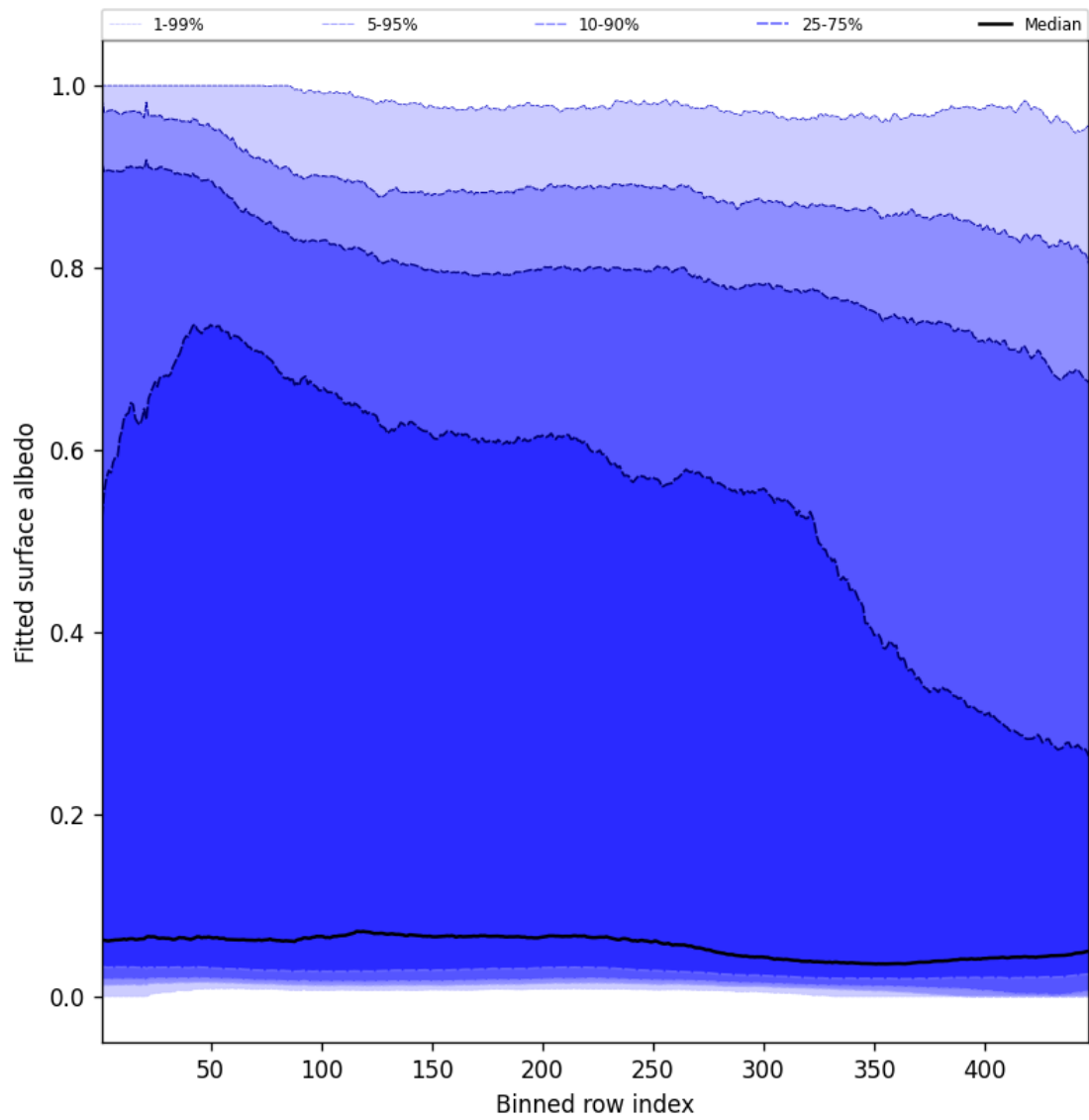
Figure 59: Along track statistics of “Fitted surface albedo” for 2025-03-20 to 2025-03-21
