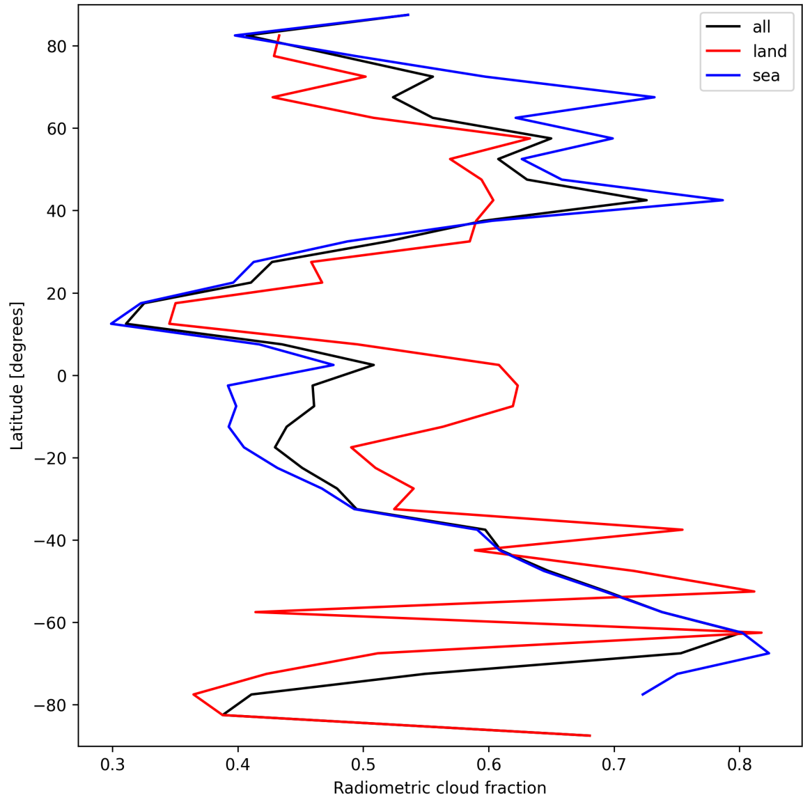
Figure 21: Zonal average of “Radiometric cloud fraction” for 2025-03-20 to 2025-03-21.
