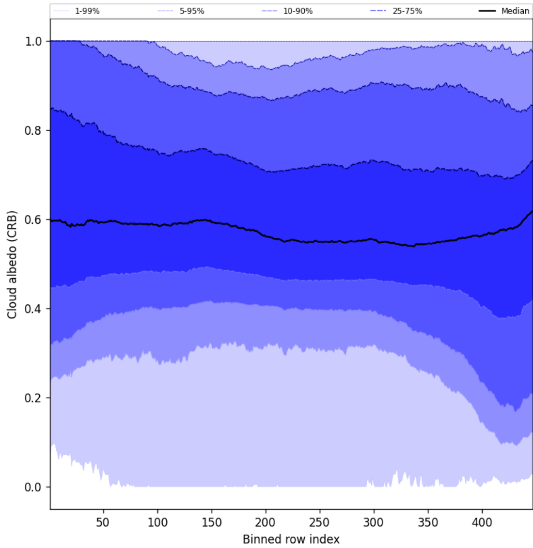
Figure 58: Along track statistics of “Cloud albedo (CRB)” for 2025-03-20 to 2025-03-21
