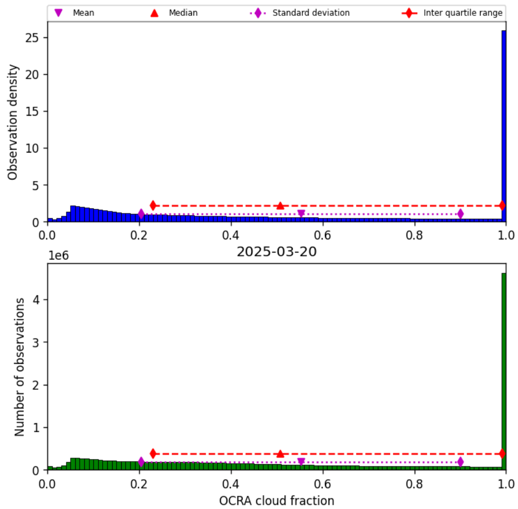
Figure 48: Histogram of “OCRA cloud fraction” for 2025-03-20 to 2025-03-21
