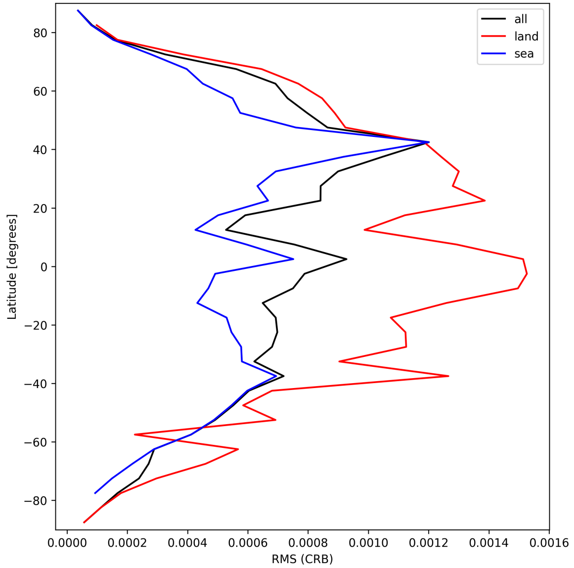
Figure 30: Zonal average of “RMS (CRB)” for 2025-03-20 to 2025-03-21.
