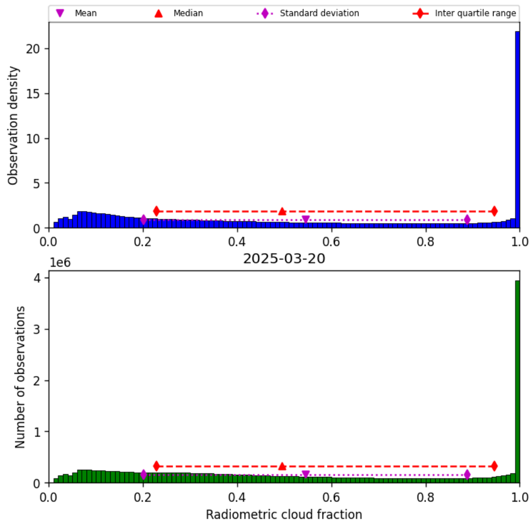
Figure 37: Histogram of “Radiometric cloud fraction” for 2025-03-20 to 2025-03-21
