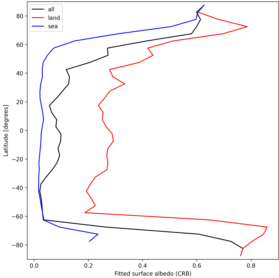
Figure 28: Zonal average of “Fitted surface albedo (CRB)” for 2025-03-20 to 2025-03-21.
