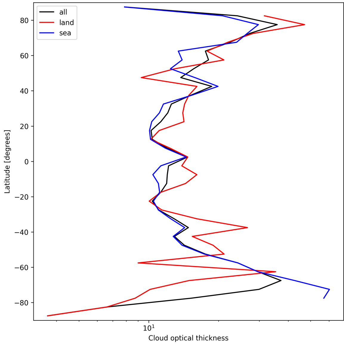
Figure 23: Zonal average of “Cloud optical thickness” for 2025-03-20 to 2025-03-21.
