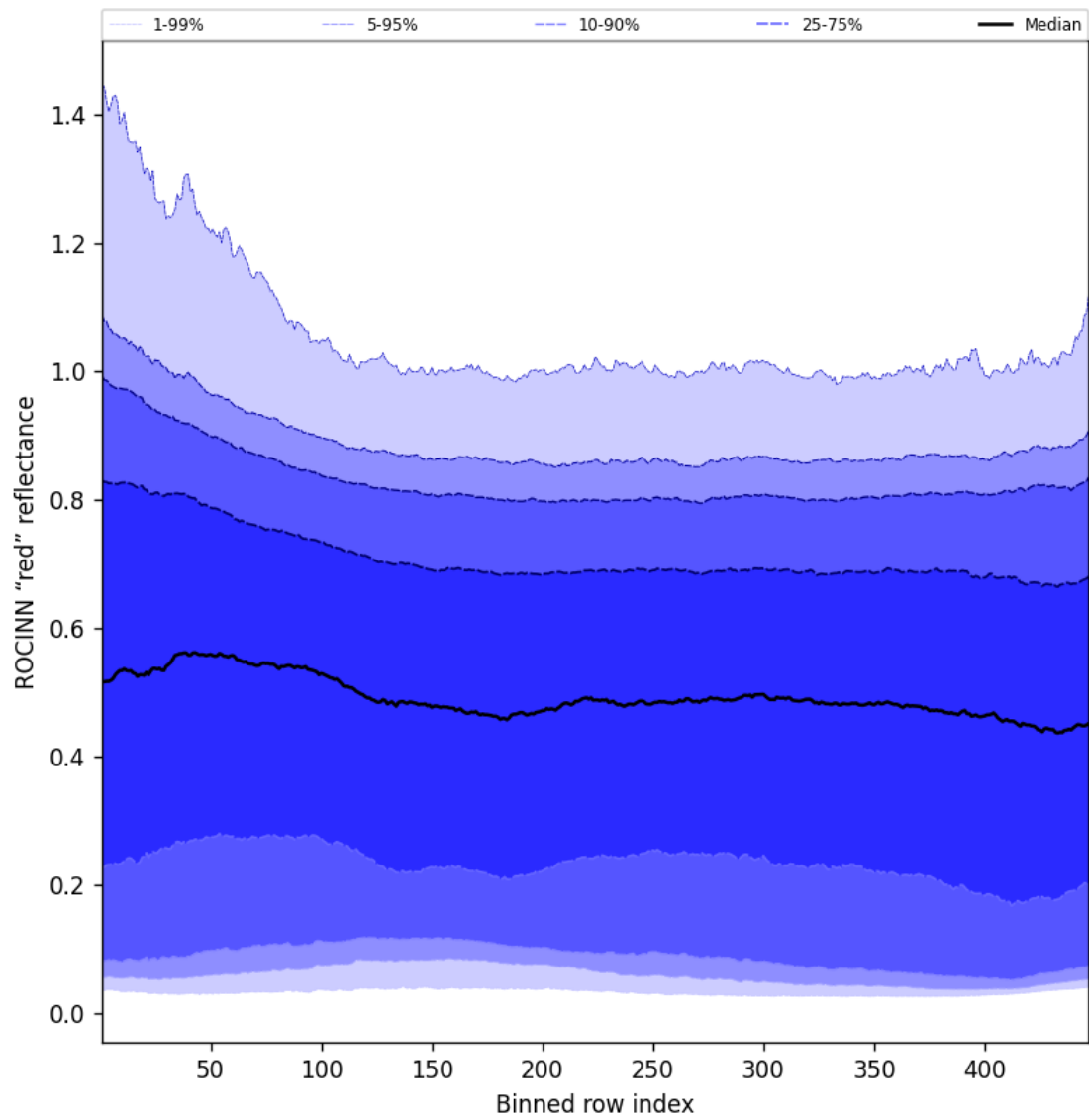
Figure 67: Along track statistics of "ROCINN "red" reflectance" for 2025-03-20 to 2025-03-21
