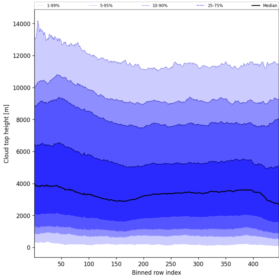
Figure 54: Along track statistics of “Cloud top height” for 2025-03-20 to 2025-03-21
