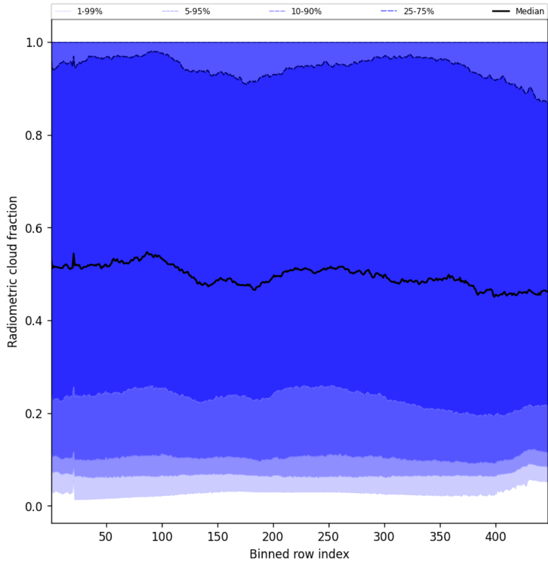
Figure 53: Along track statistics of “Radiometric cloud fraction” for 2025-03-20 to 2025-03-21
