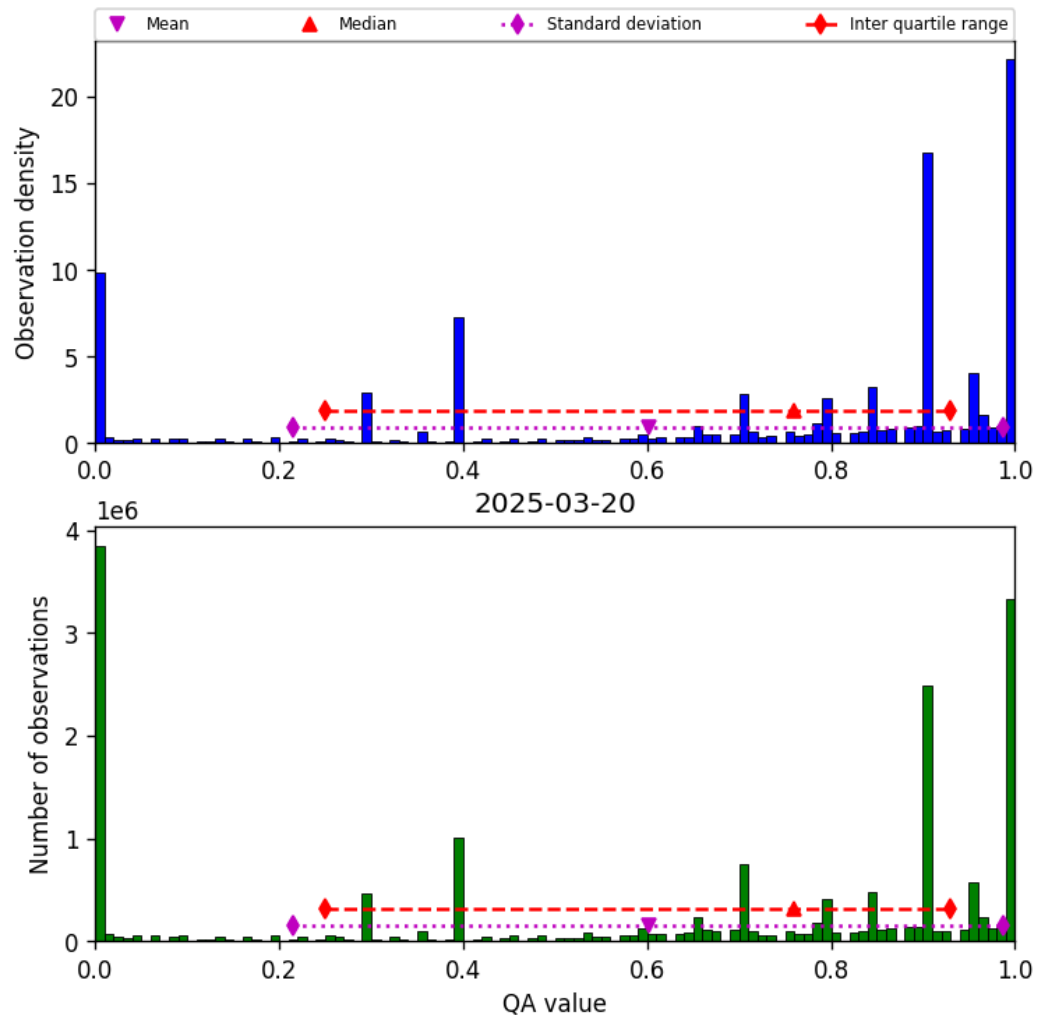
Figure 36: Histogram of “QA value” for 2025-03-20 to 2025-03-21
