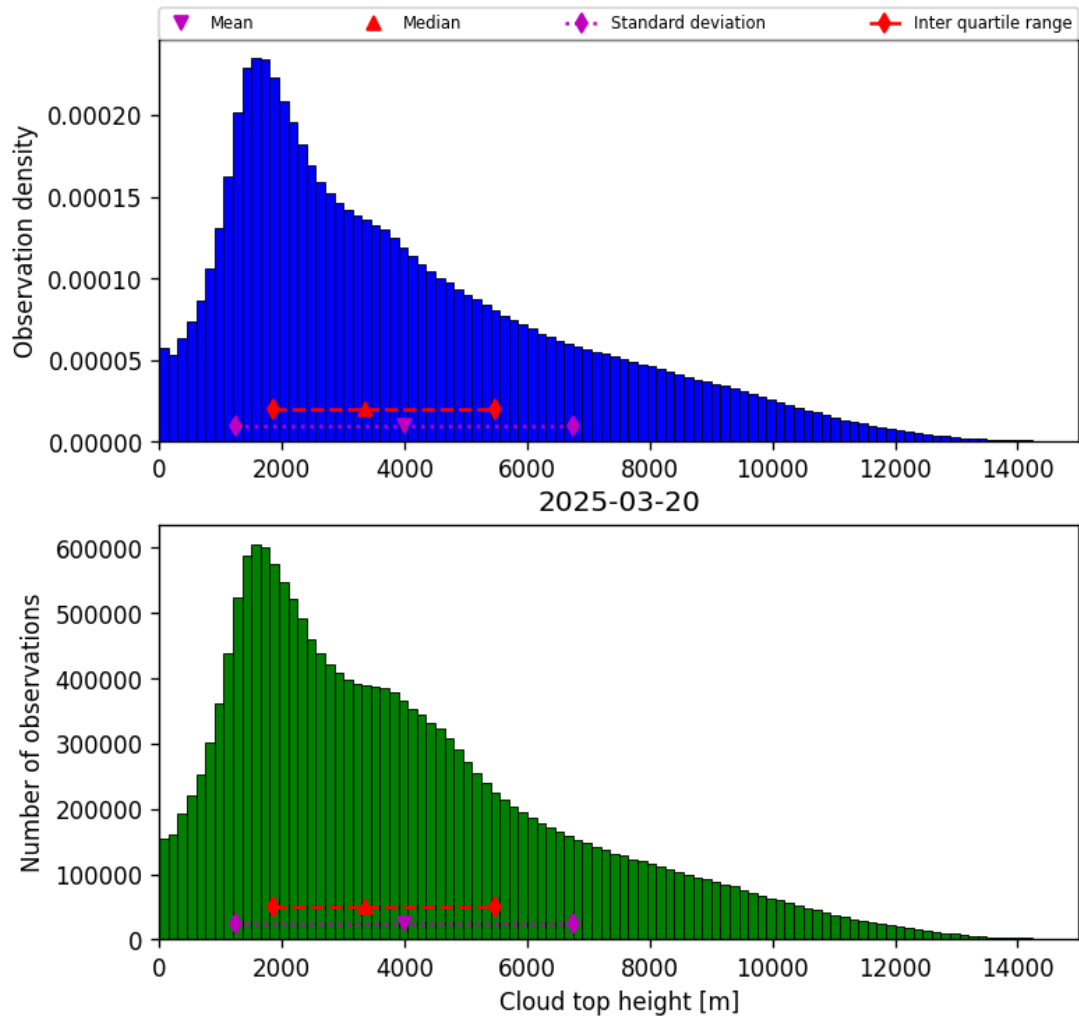
Figure 38: Histogram of “Cloud top height” for 2025-03-20 to 2025-03-21
