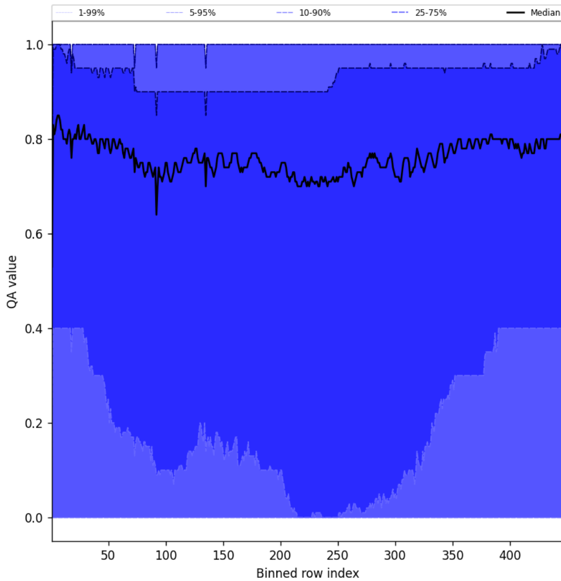
Figure 52: Along track statistics of “QA value” for 2025-03-20 to 2025-03-21
