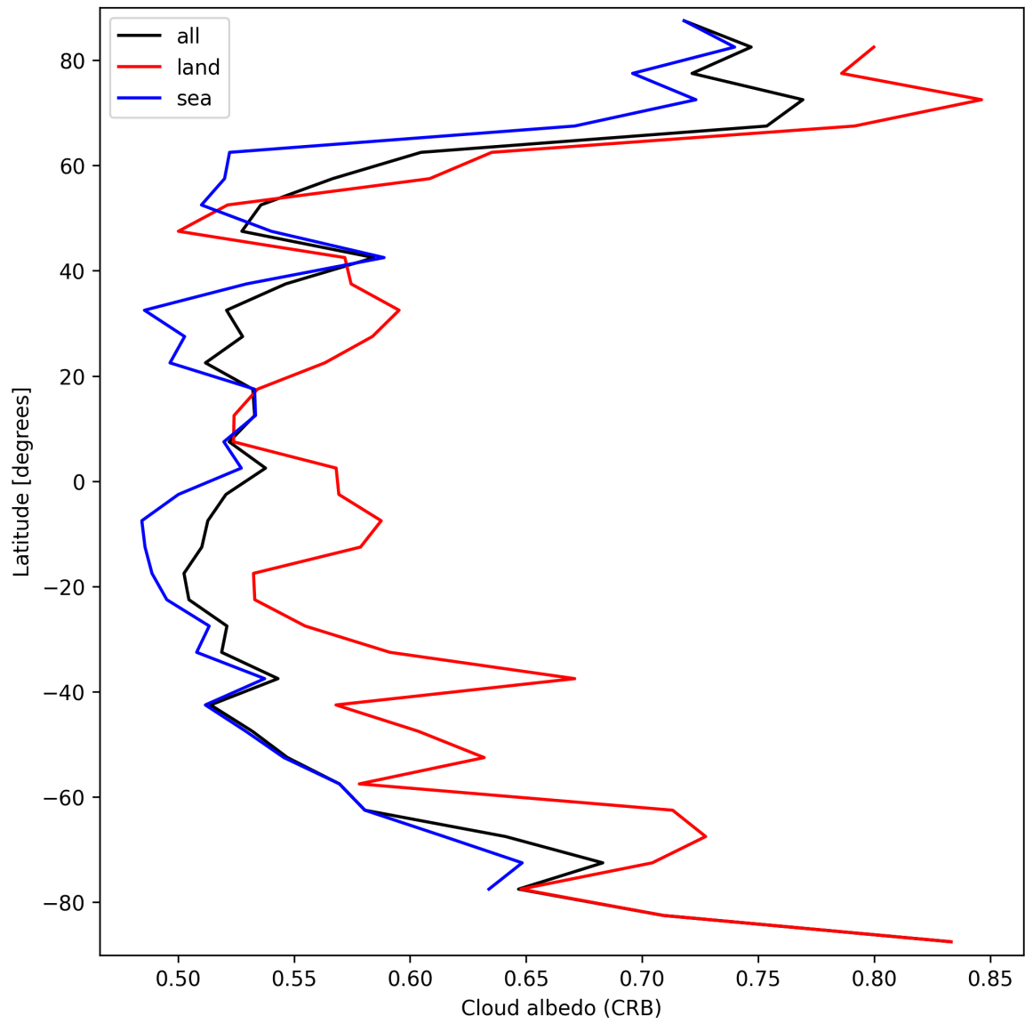
Figure 26: Zonal average of “Cloud albedo (CRB)” for 2025-03-20 to 2025-03-21.
