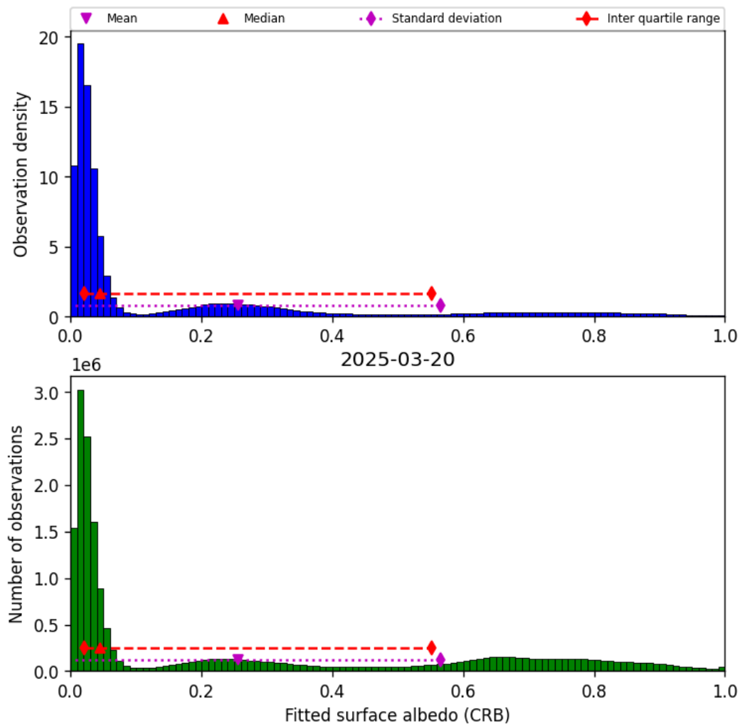
Figure 44: Histogram of “Fitted surface albedo (CRB)” for 2025-03-20 to 2025-03-21
