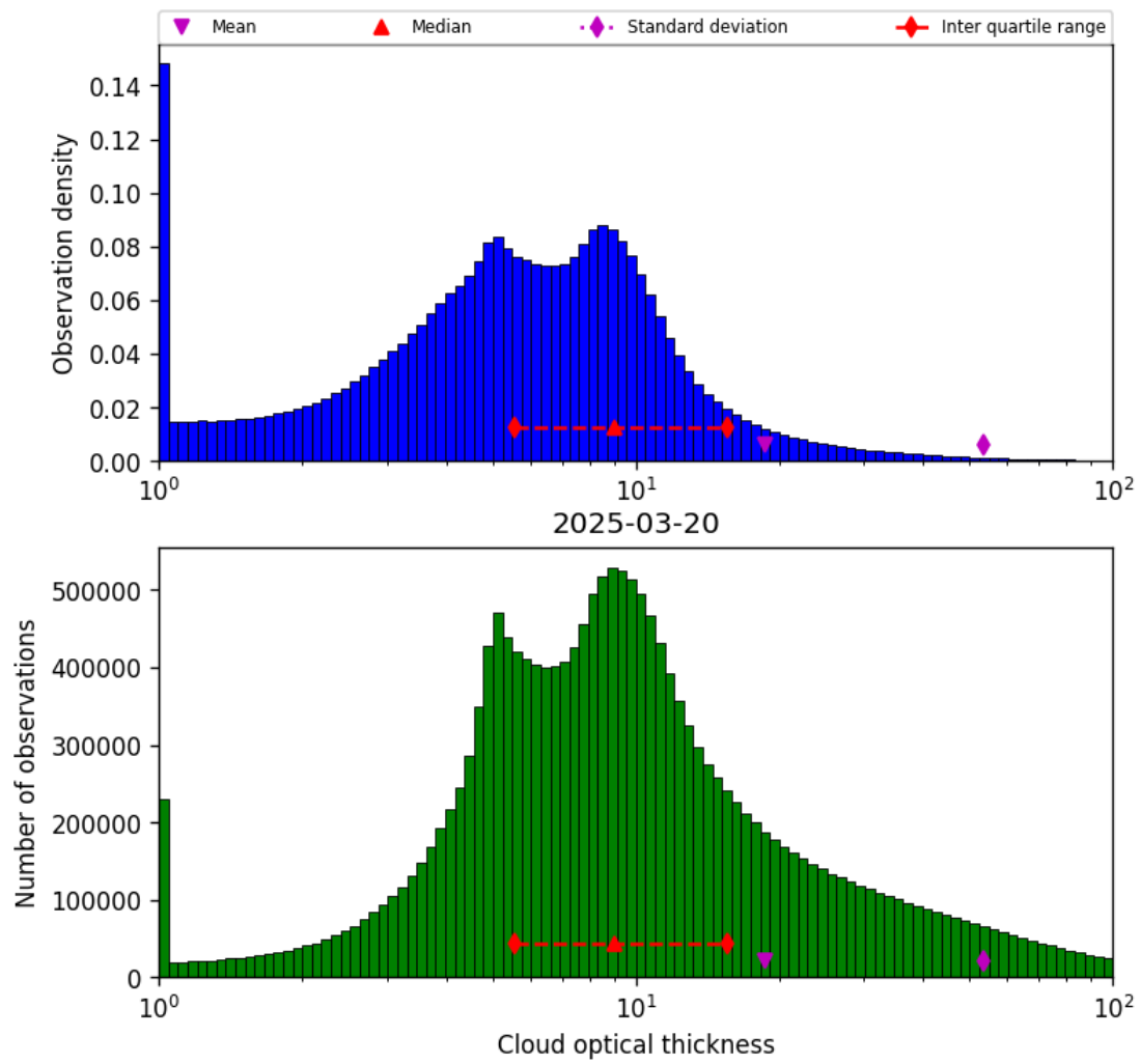
Figure 39: Histogram of “Cloud optical thickness” for 2025-03-20 to 2025-03-21
