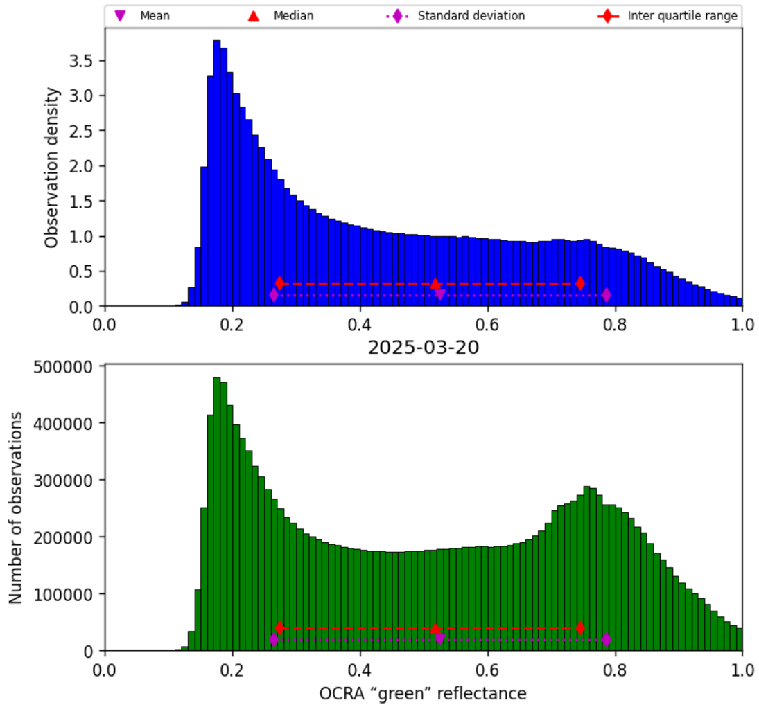
Figure 50: Histogram of “OCRA “green” reflectance” for 2025-03-20 to 2025-03-21
