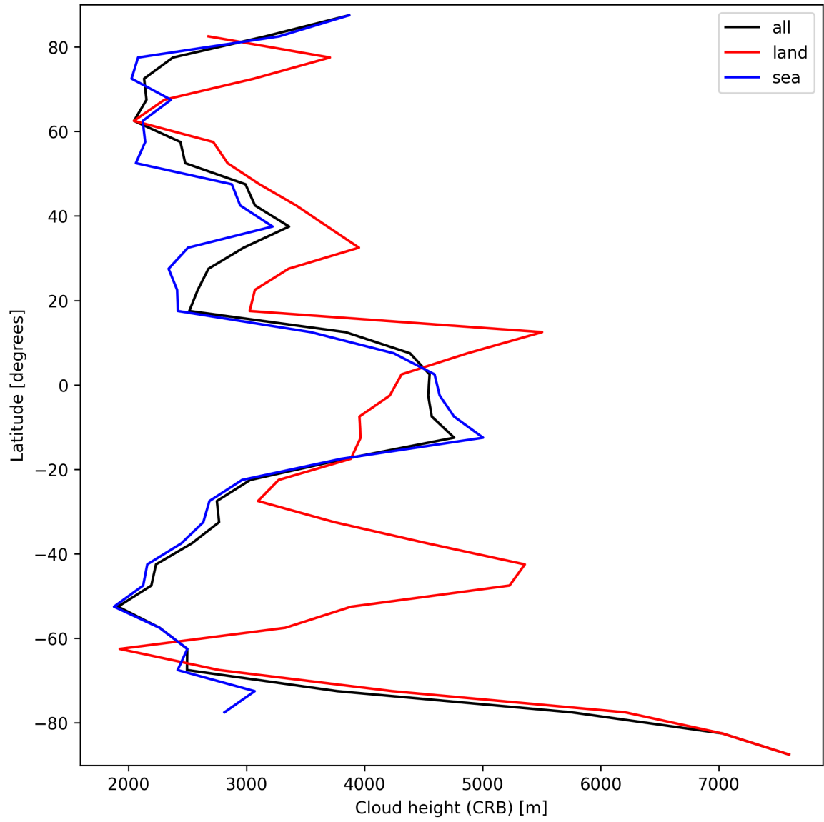
Figure 25: Zonal average of “Cloud height (CRB)” for 2025-03-20 to 2025-03-21.
