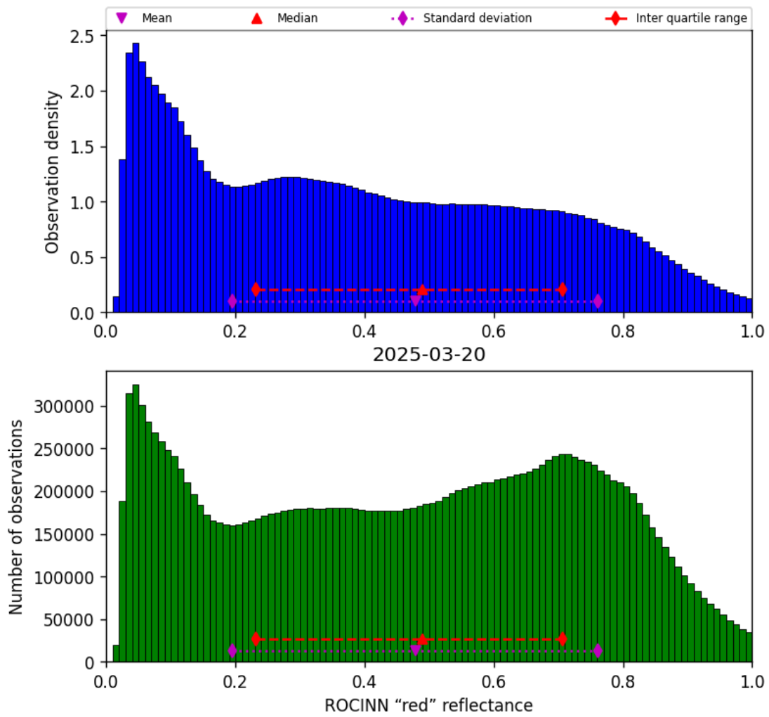
Figure 51: Histogram of “ROCINN “red” reflectance” for 2025-03-20 to 2025-03-21
