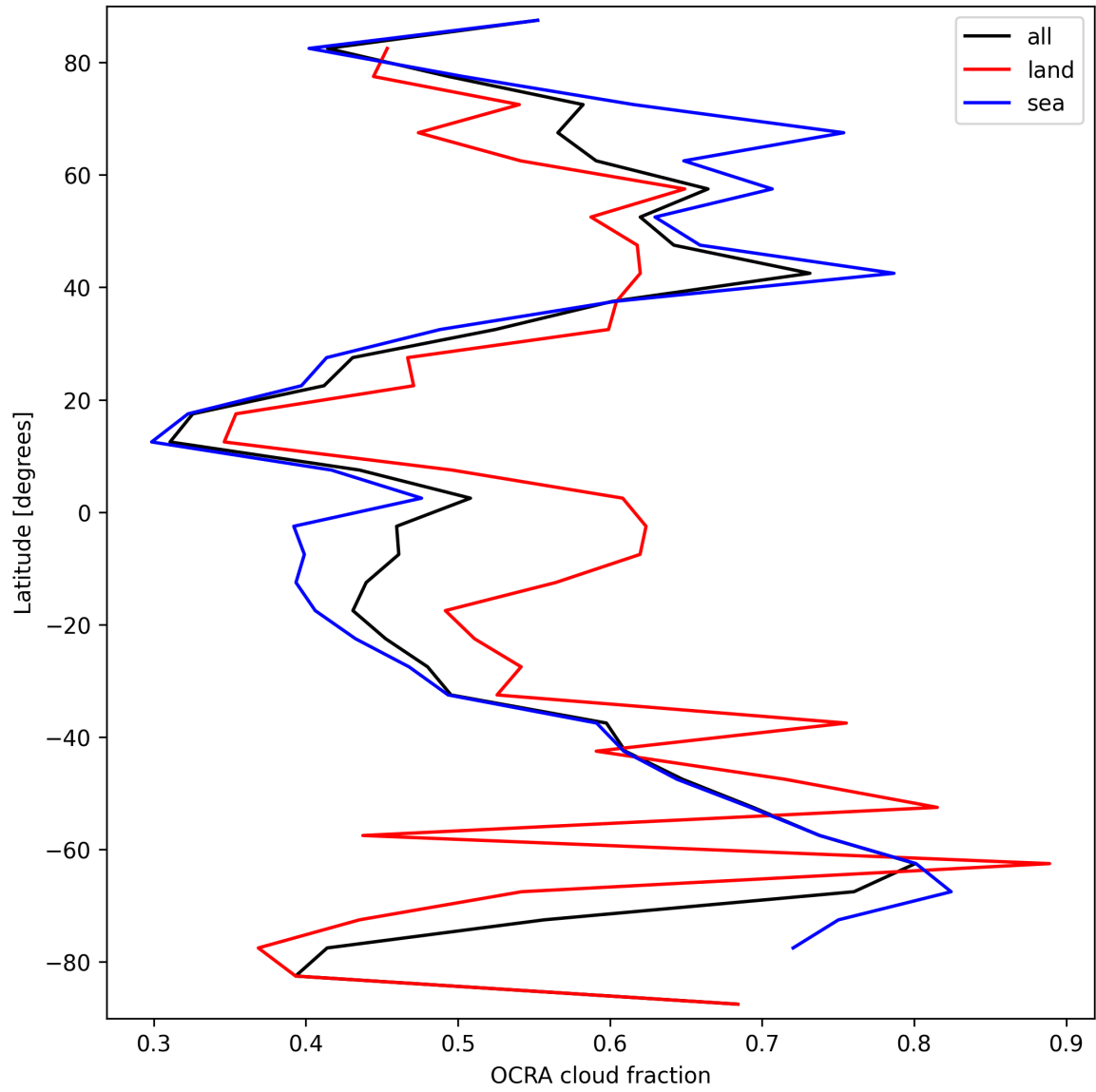
Figure 32: Zonal average of “OCRA cloud fraction” for 2025-03-20 to 2025-03-21.
