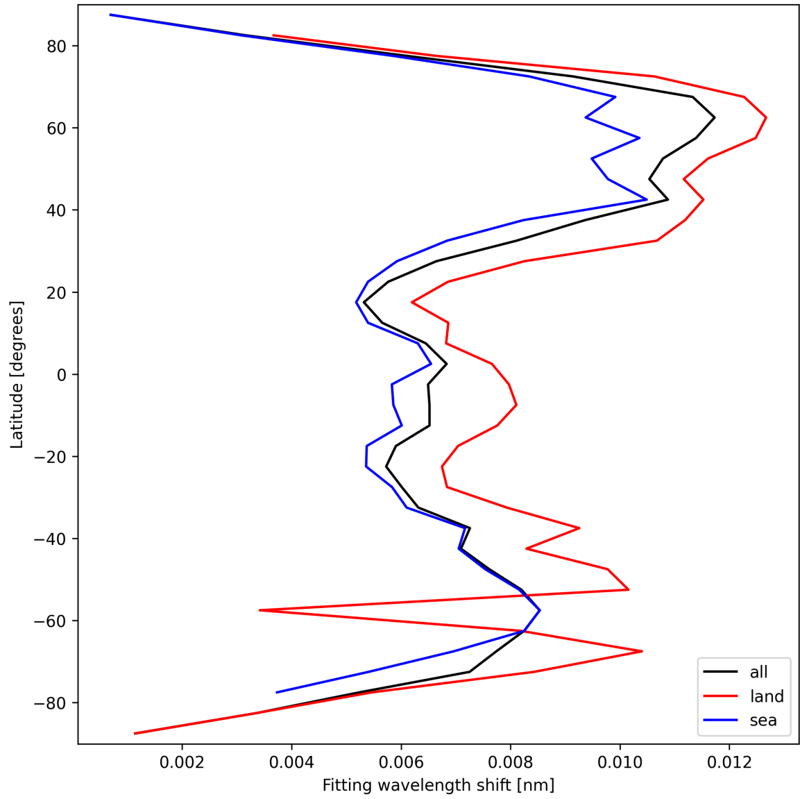
Figure 31: Zonal average of “Fitting wavelength shift” for 2025-03-20 to 2025-03-21.
