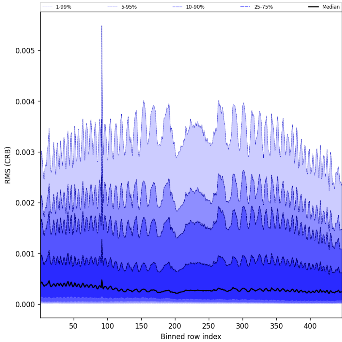
Figure 62: Along track statistics of “RMS (CRB)” for 2025-03-27 to 2025-03-28
