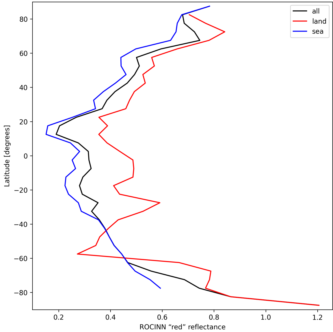
Figure 35: Zonal average of “ROCINN “red” reflectance” for 2025-03-27 to 2025-03-28.
