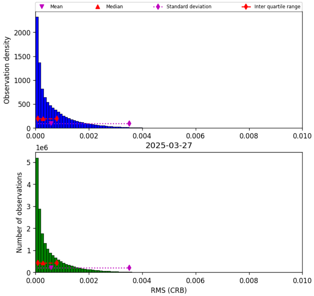
Figure 46: Histogram of "RMS (CRB)" for 2025-03-27 to 2025-03-28
