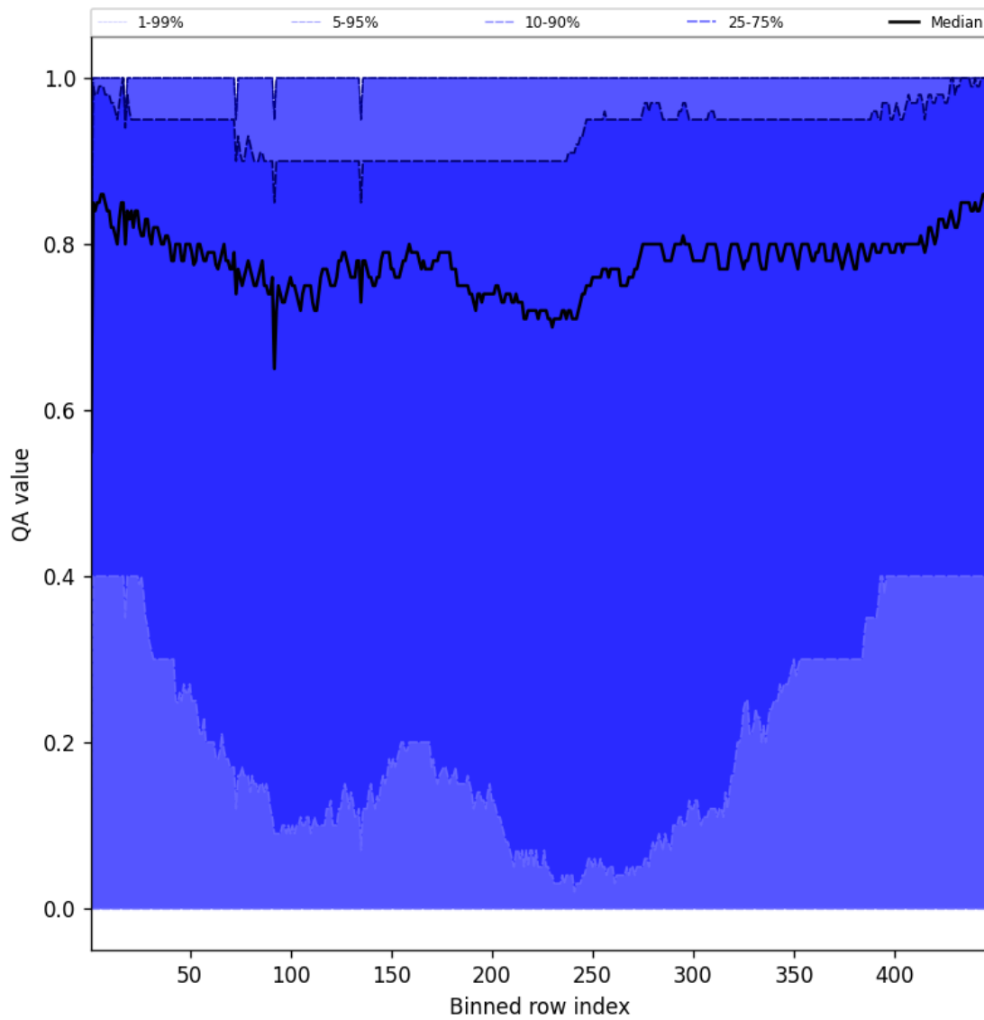
Figure 52: Along track statistics of “QA value” for 2025-03-27 to 2025-03-28
