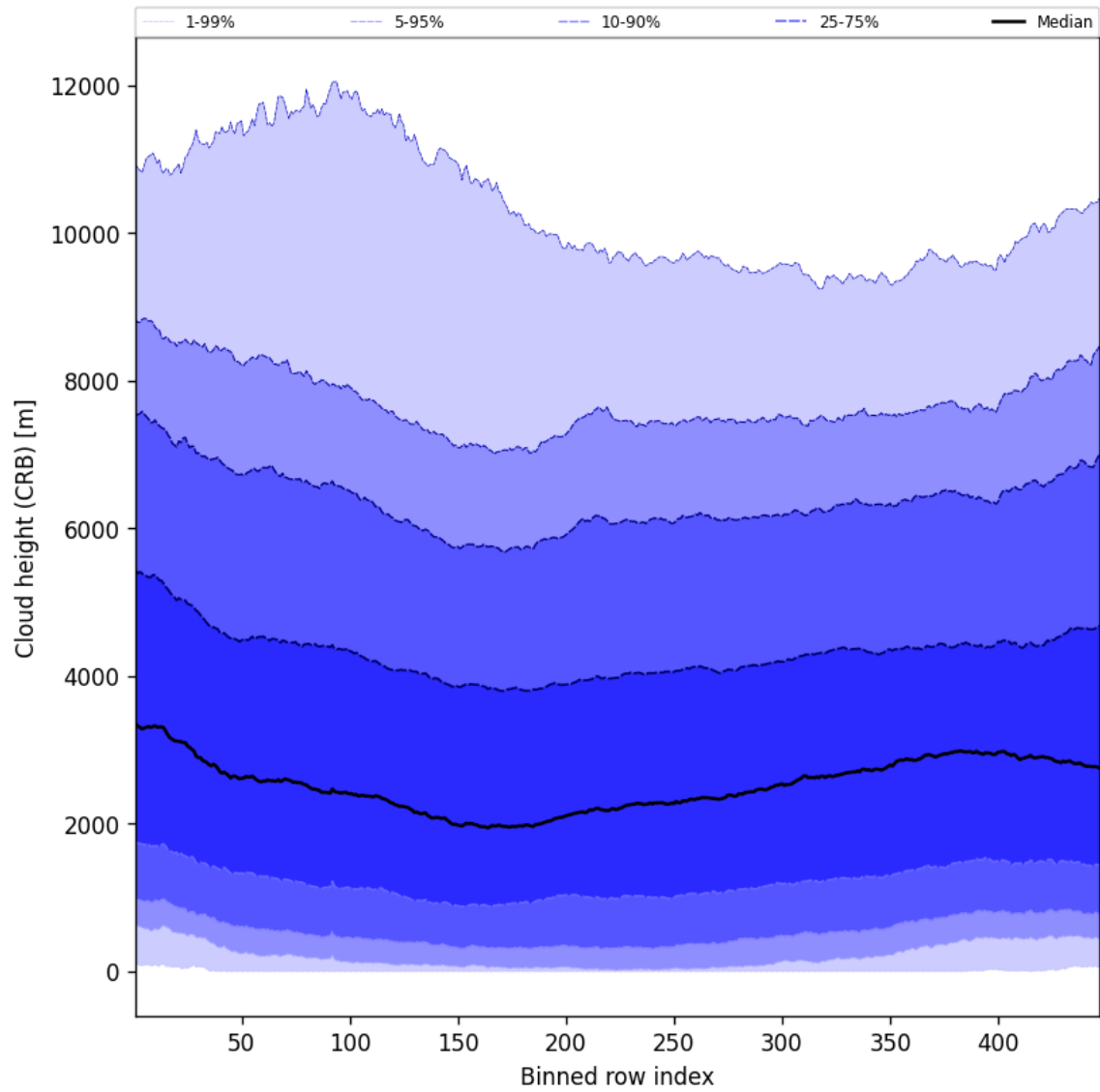
Figure 57: Along track statistics of “Cloud height (CRB)” for 2025-03-27 to 2025-03-28
