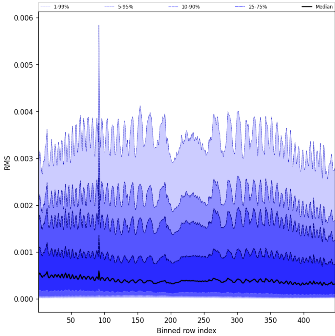
Figure 61: Along track statistics of “RMS” for 2025-03-27 to 2025-03-28
