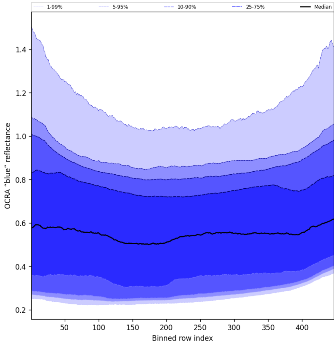
Figure 65: Along track statistics of “OCRA “blue” reflectance” for 2025-03-27 to 2025-03-28
