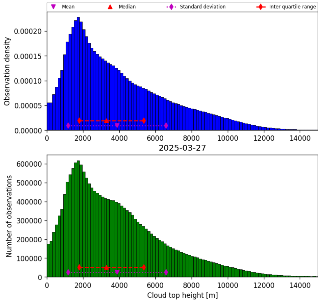
Figure 38: Histogram of “Cloud top height” for 2025-03-27 to 2025-03-28
