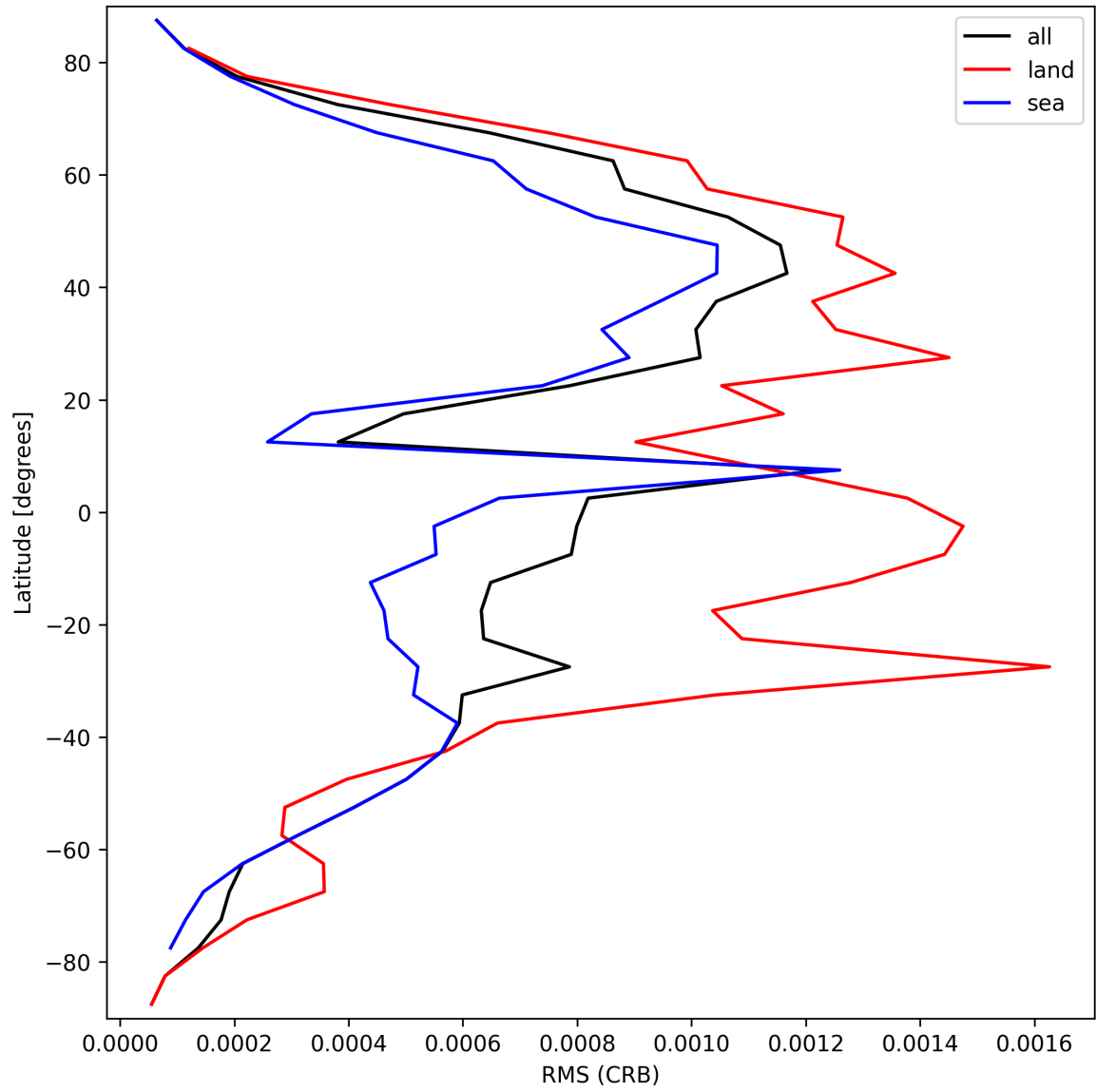
Figure 30: Zonal average of “RMS (CRB)” for 2025-03-27 to 2025-03-28.
