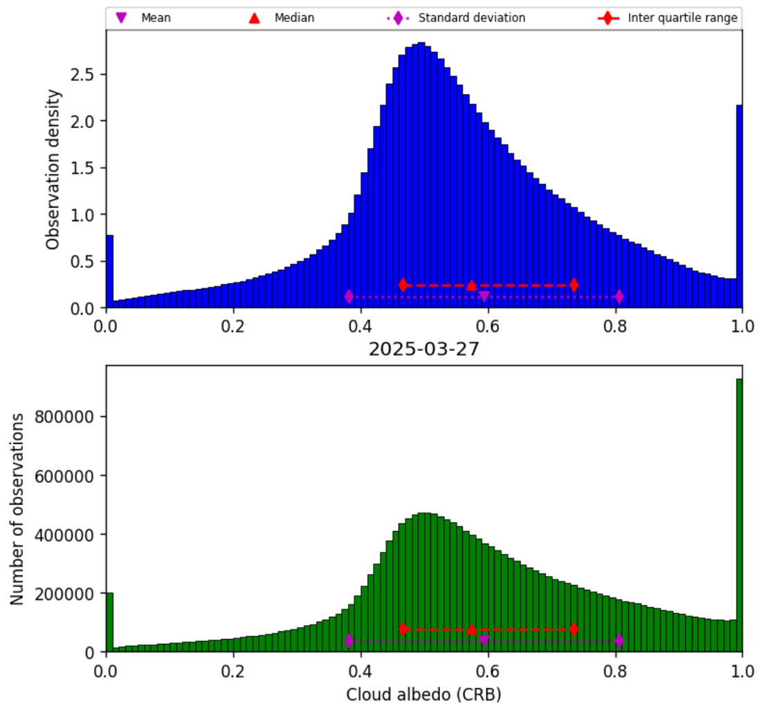
Figure 42: Histogram of “Cloud albedo (CRB)” for 2025-03-27 to 2025-03-28
