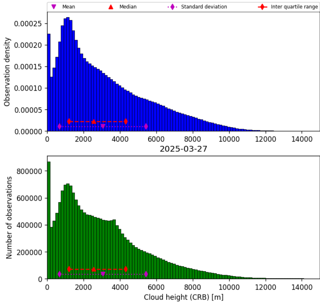
Figure 41: Histogram of “Cloud height (CRB)” for 2025-03-27 to 2025-03-28
