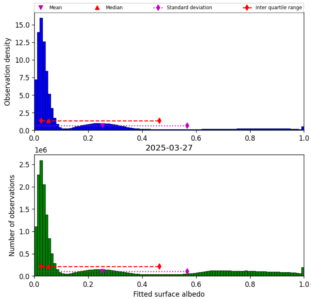
Figure 43: Histogram of “Fitted surface albedo” for 2025-03-27 to 2025-03-28
