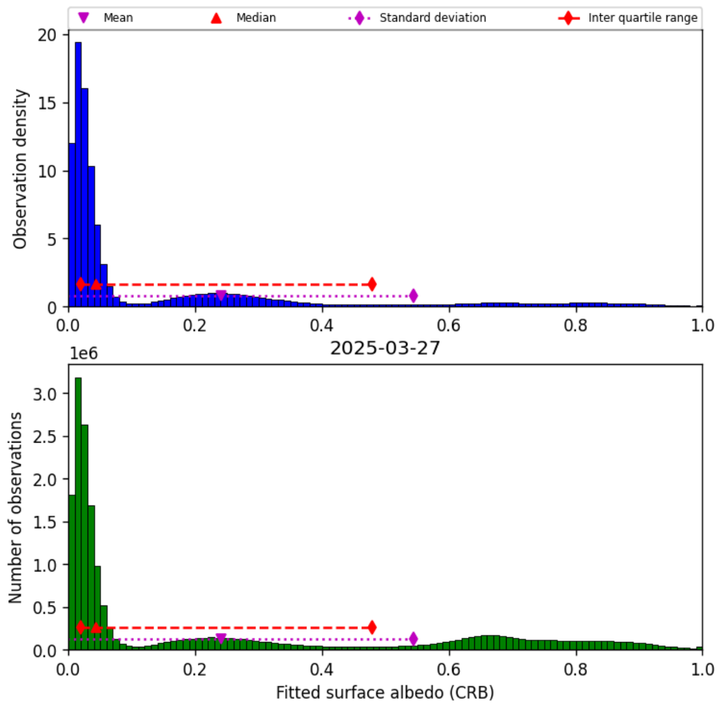
Figure 44: Histogram of “Fitted surface albedo (CRB)” for 2025-03-27 to 2025-03-28
