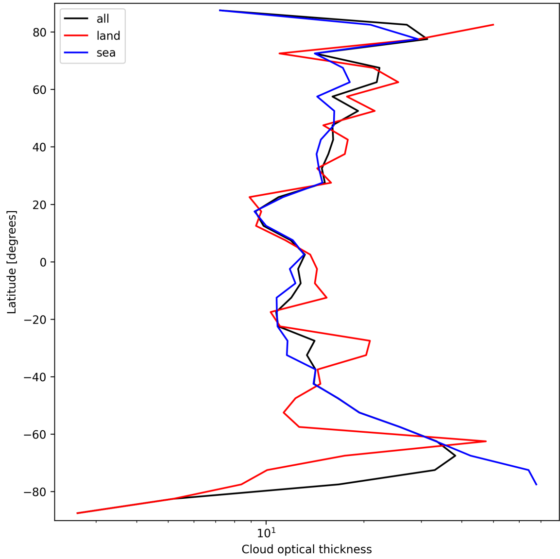
Figure 23: Zonal average of “Cloud optical thickness” for 2025-03-27 to 2025-03-28.
