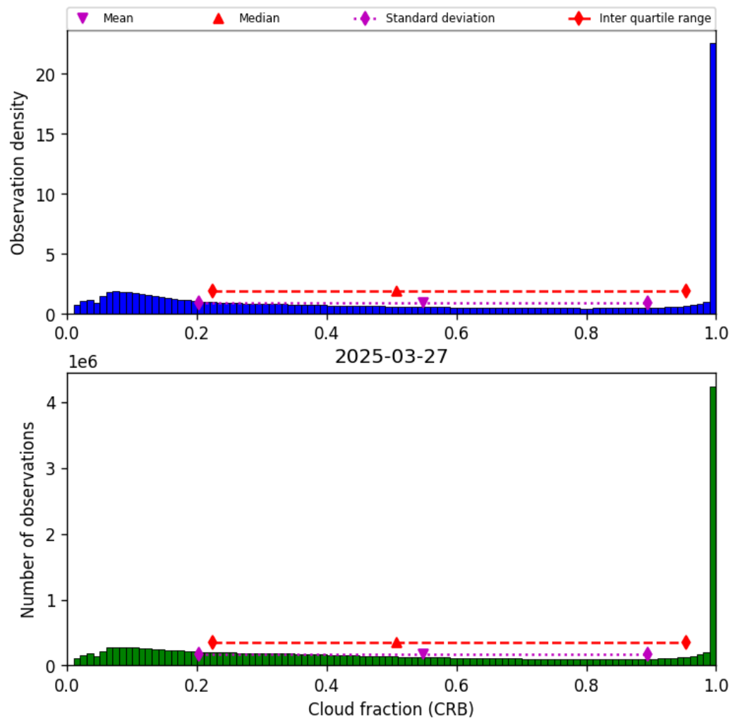
Figure 40: Histogram of “Cloud fraction (CRB)” for 2025-03-27 to 2025-03-28
