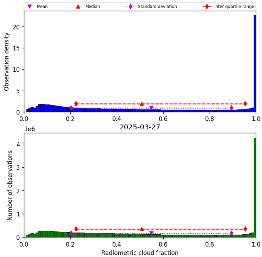
Figure 37: Histogram of “Radiometric cloud fraction” for 2025-03-27 to 2025-03-28
