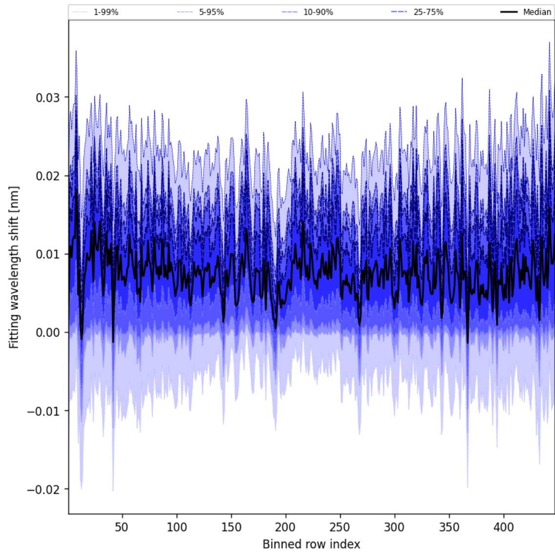
Figure 63: Along track statistics of “Fitting wavelength shift” for 2025-03-27 to 2025-03-28
