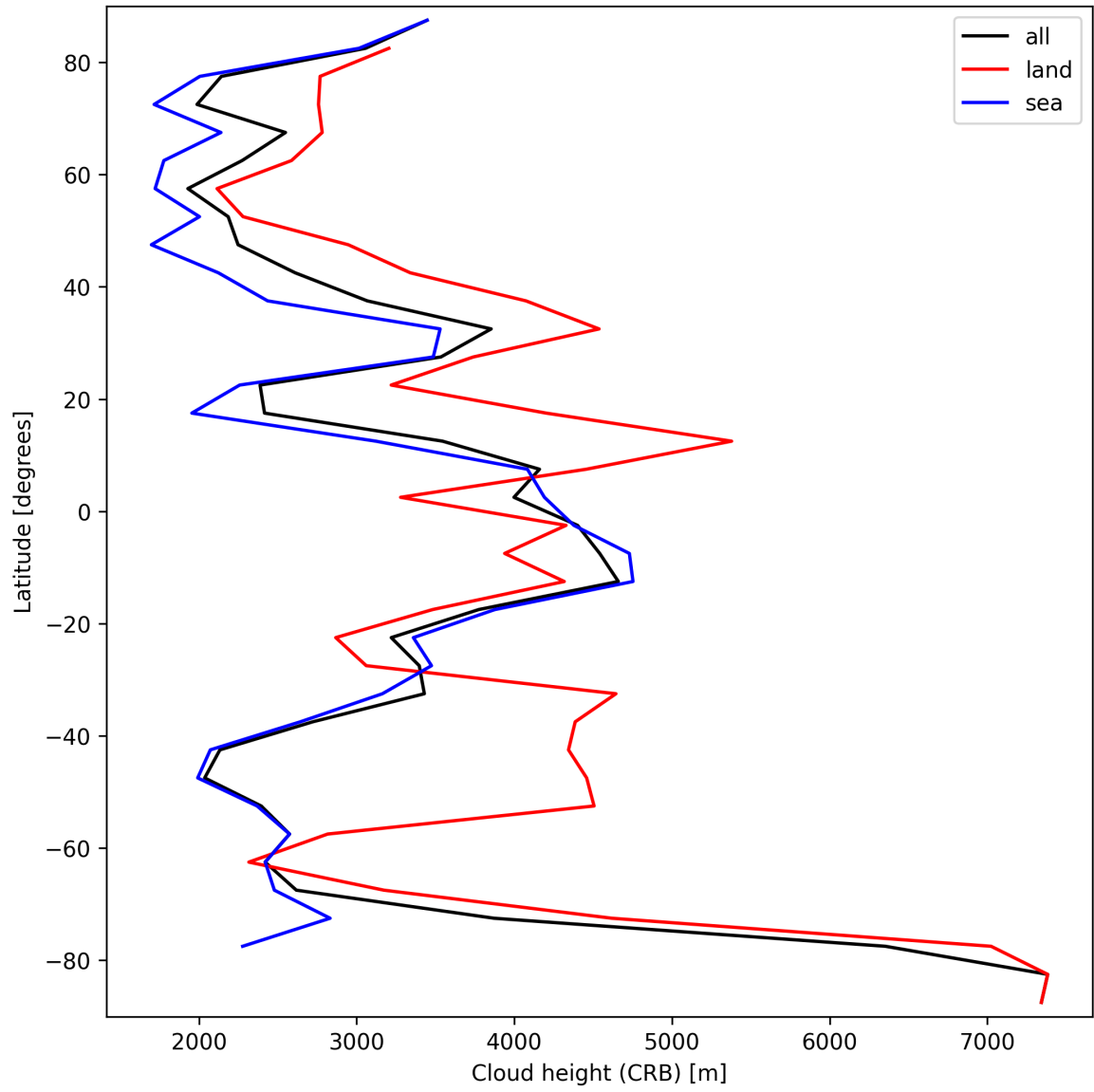
Figure 25: Zonal average of “Cloud height (CRB)” for 2025-03-27 to 2025-03-28.
