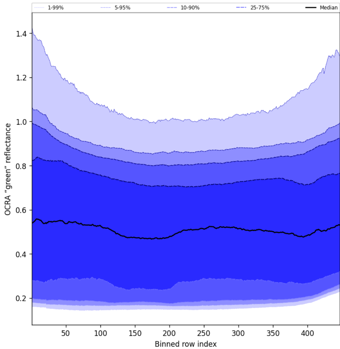
Figure 66: Along track statistics of "OCRA "green" reflectance" for 2025-03-27 to 2025-03-28
