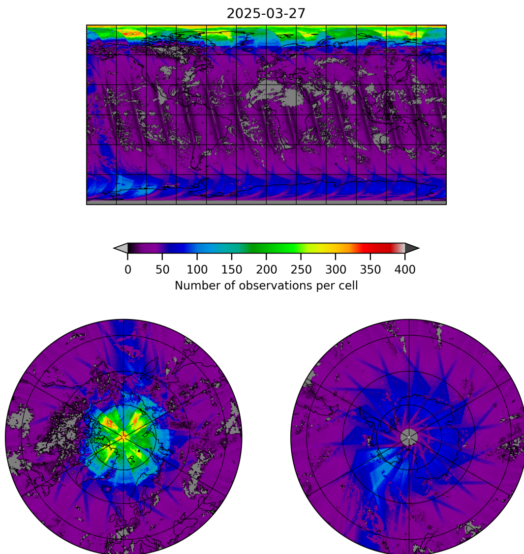
Figure 19: Map of the number of observations for 2025-03-27 to 2025-03-28
