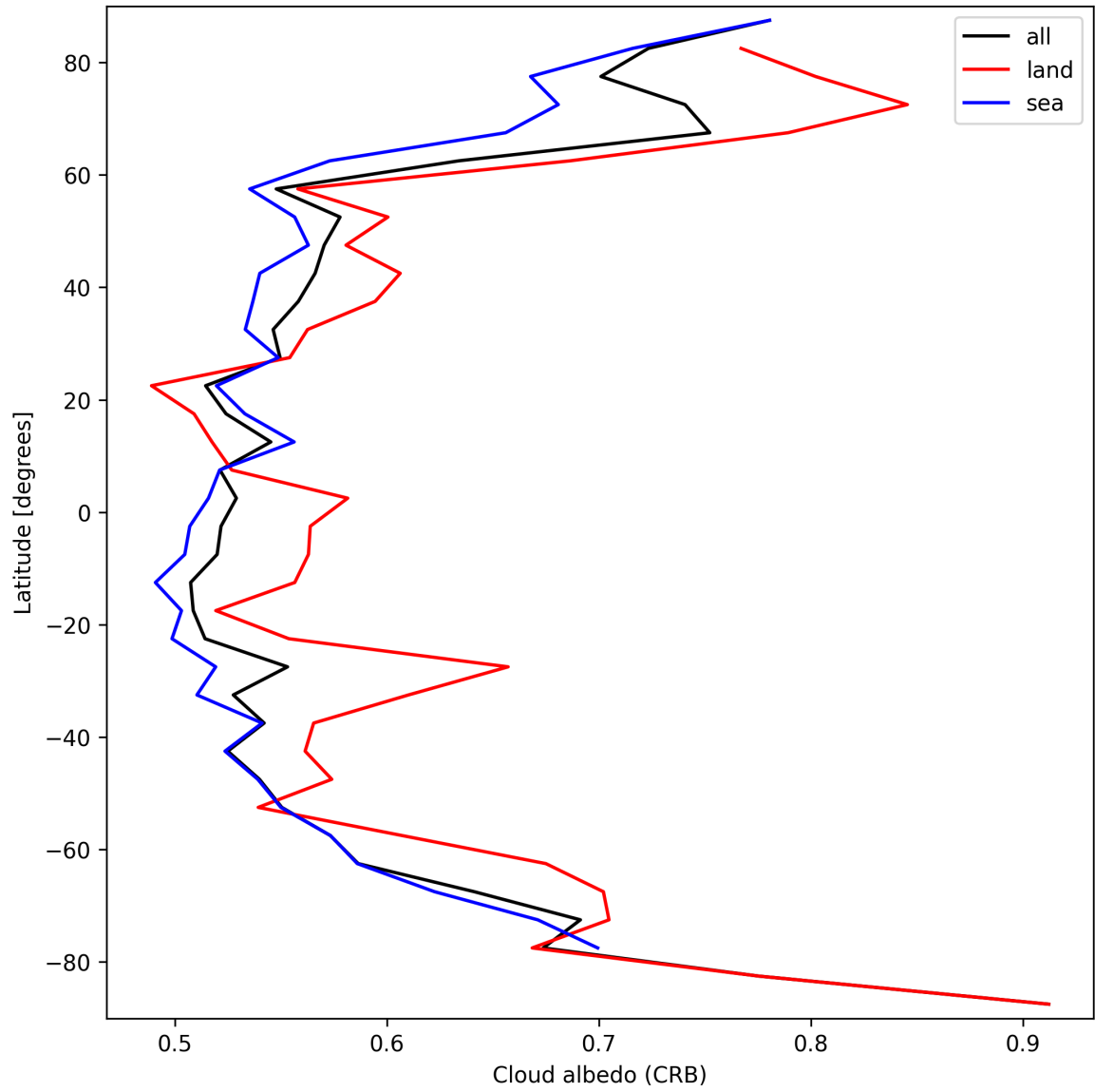
Figure 26: Zonal average of “Cloud albedo (CRB)” for 2025-03-27 to 2025-03-28.
