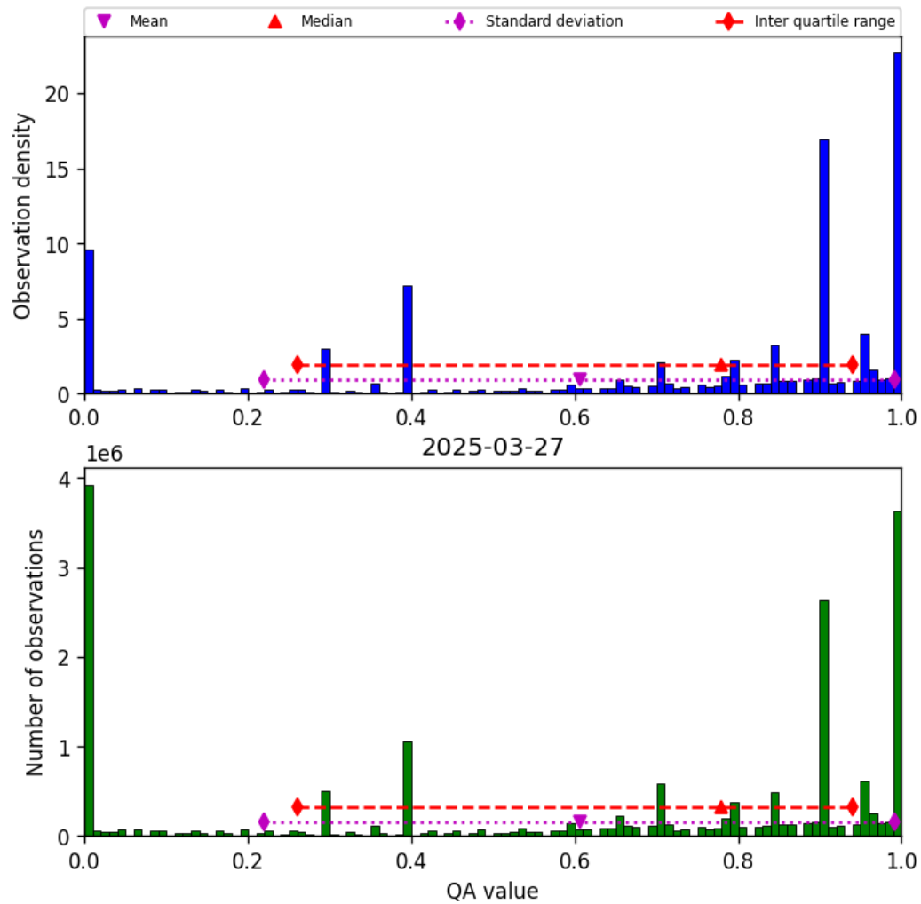
Figure 36: Histogram of “QA value” for 2025-03-27 to 2025-03-28
