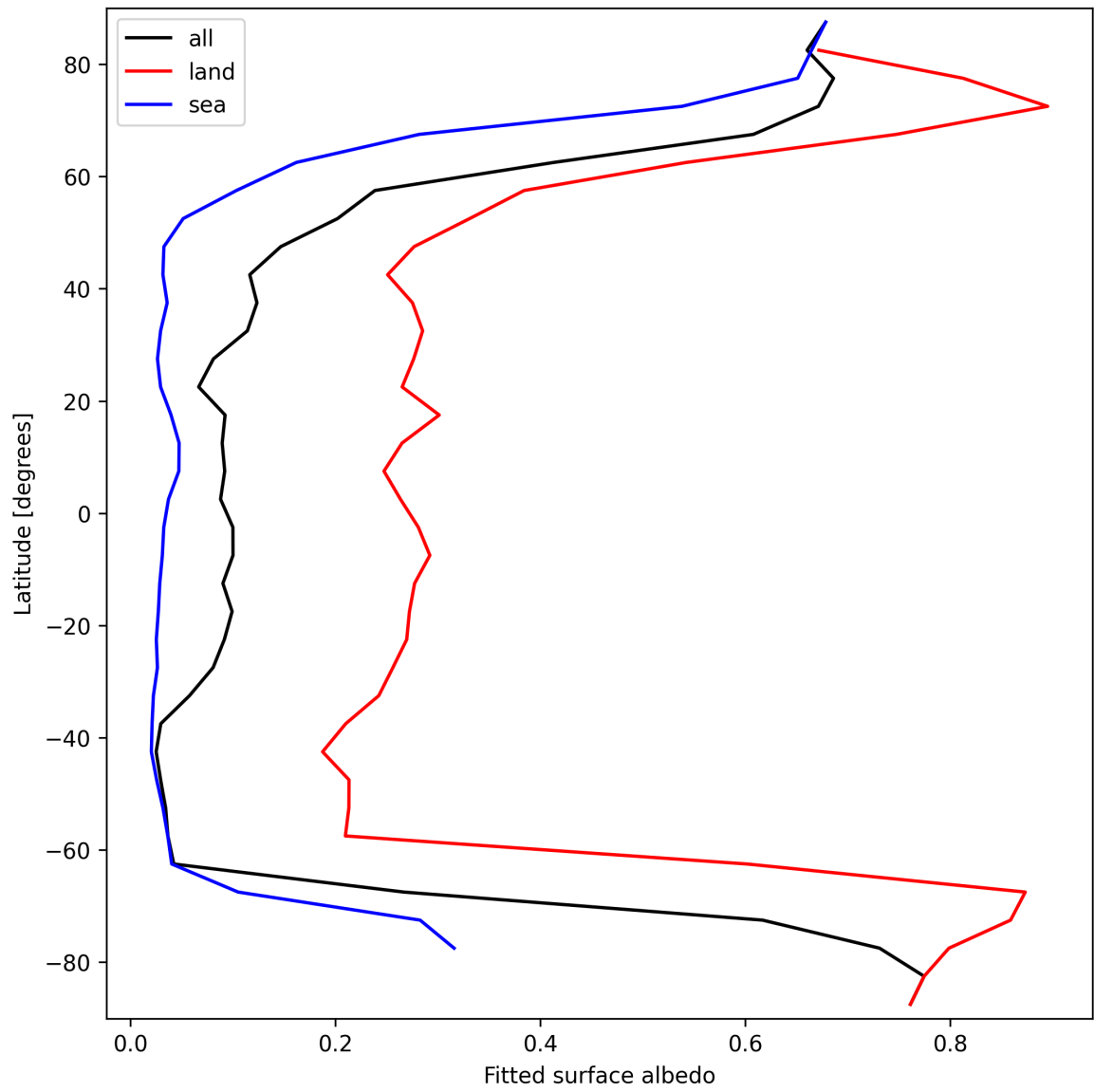
Figure 27: Zonal average of “Fitted surface albedo” for 2025-03-27 to 2025-03-28.
