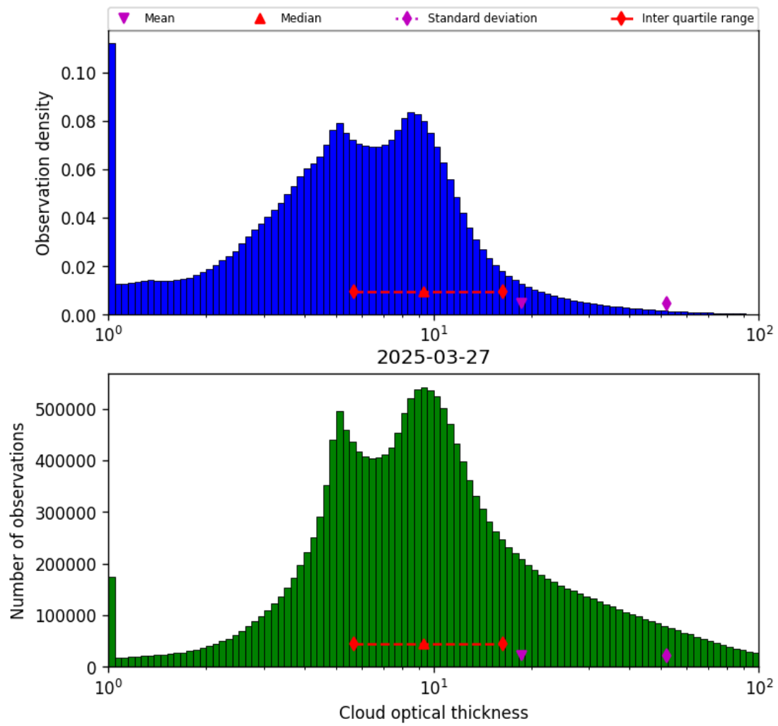
Figure 39: Histogram of “Cloud optical thickness” for 2025-03-27 to 2025-03-28
