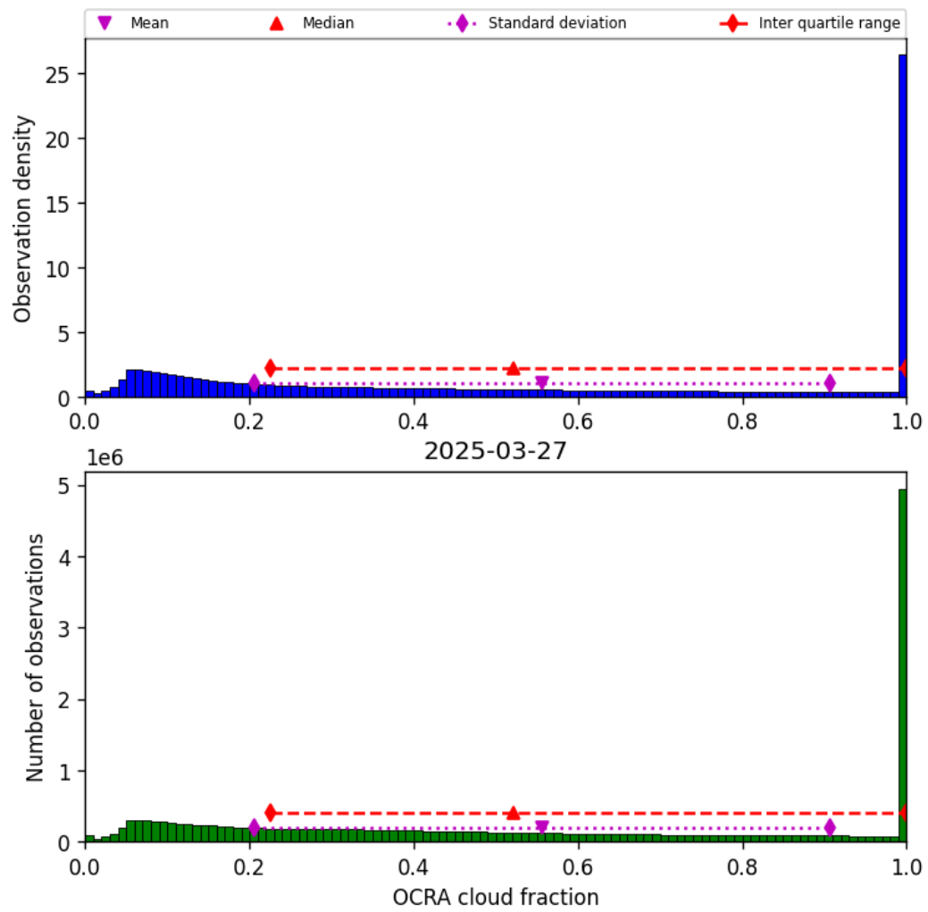
Figure 48: Histogram of “OCRA cloud fraction” for 2025-03-27 to 2025-03-28
