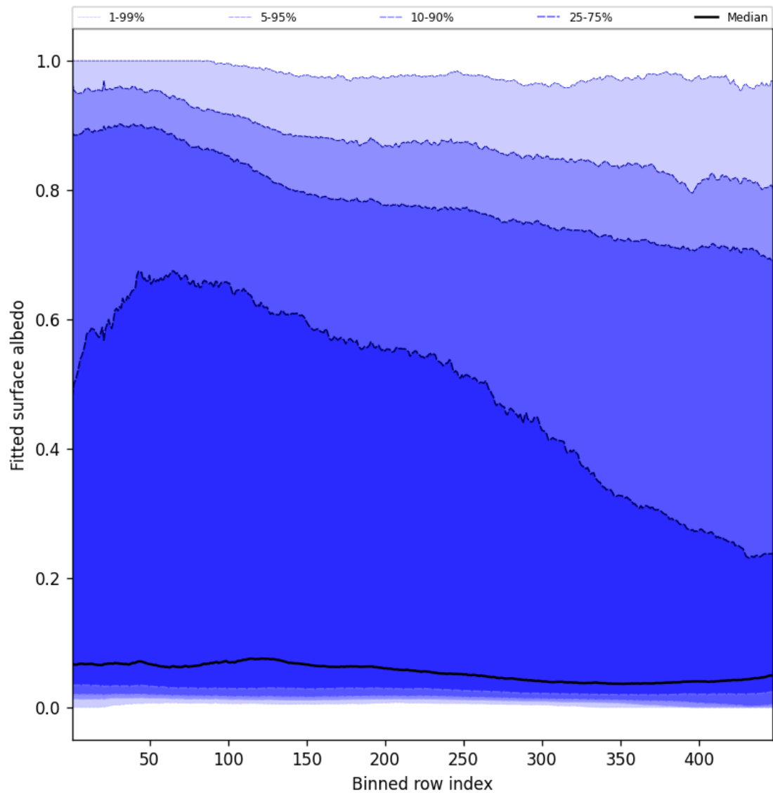
Figure 59: Along track statistics of “Fitted surface albedo” for 2025-03-27 to 2025-03-28
