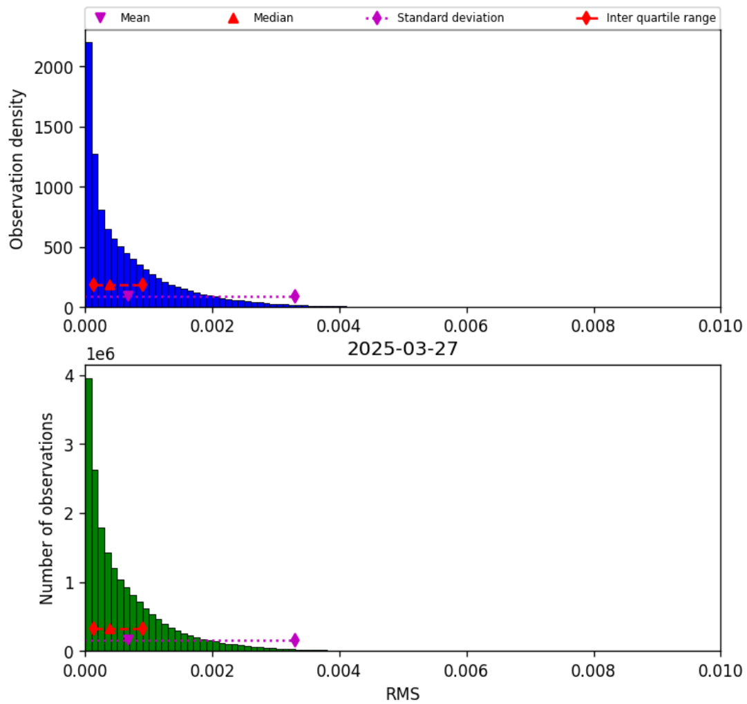
Figure 45: Histogram of “RMS” for 2025-03-27 to 2025-03-28
