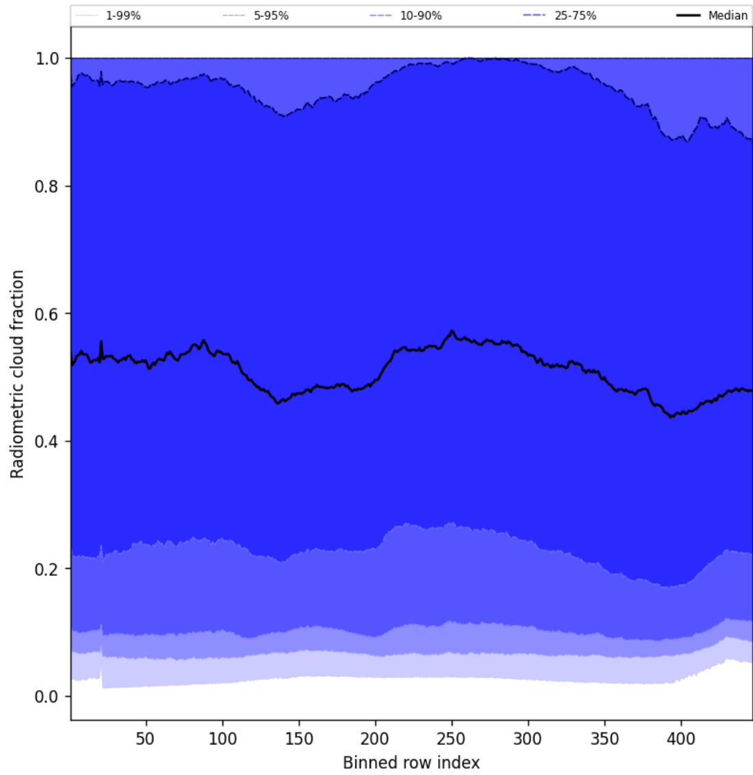
Figure 53: Along track statistics of “Radiometric cloud fraction” for 2025-03-27 to 2025-03-28
