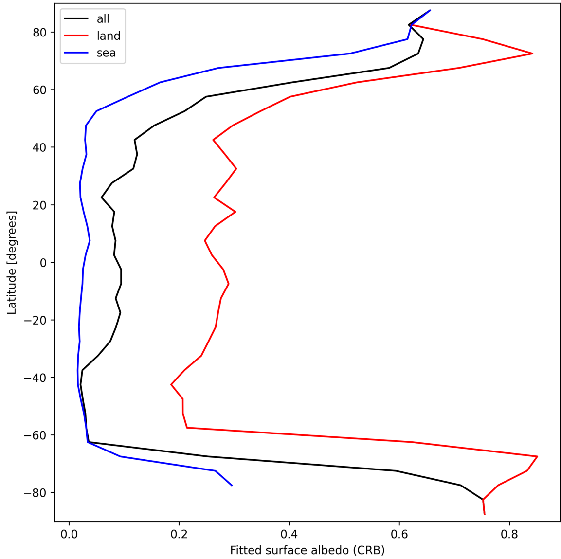
Figure 28: Zonal average of “Fitted surface albedo (CRB)” for 2025-03-27 to 2025-03-28.
