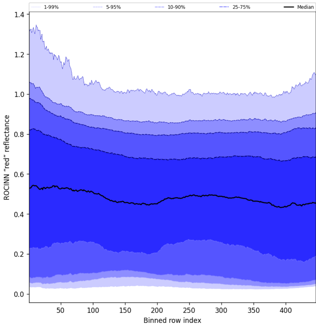
Figure 67: Along track statistics of “ROCINN “red” reflectance” for 2025-03-27 to 2025-03-28
