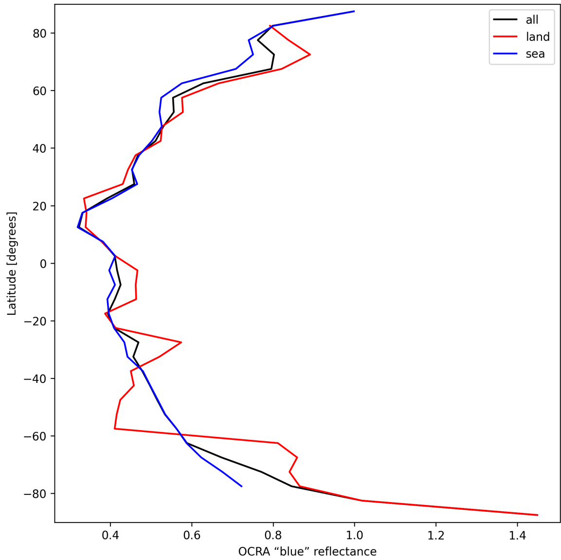
Figure 33: Zonal average of “OCRA “blue” reflectance” for 2025-03-27 to 2025-03-28.
