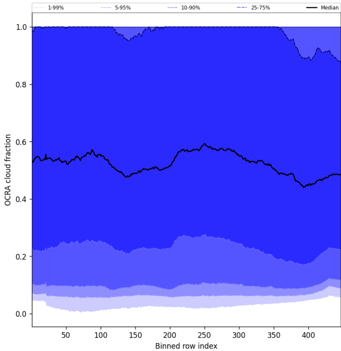
Figure 64: Along track statistics of “OCRA cloud fraction” for 2025-03-27 to 2025-03-28
