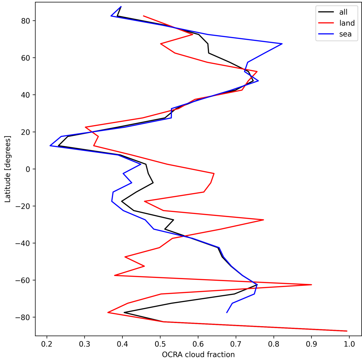
Figure 32: Zonal average of “OCRA cloud fraction” for 2025-03-27 to 2025-03-28.
