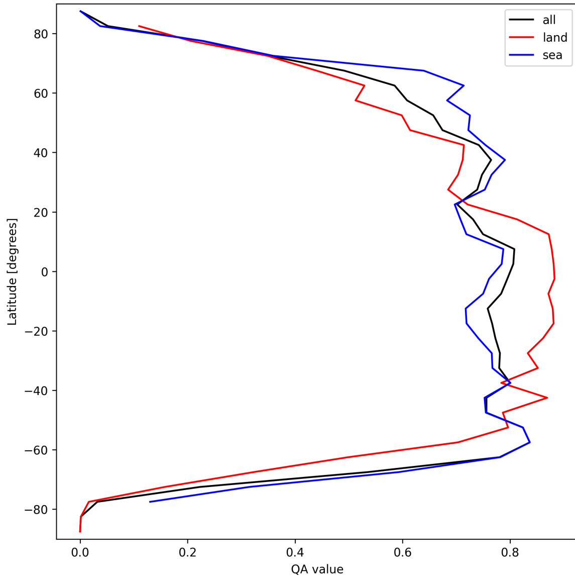
Figure 20: Zonal average of “QA value” for 2025-03-27 to 2025-03-28.
