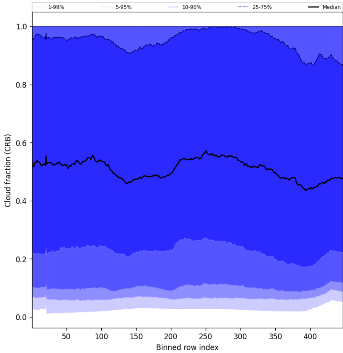
Figure 56: Along track statistics of “Cloud fraction (CRB)” for 2025-03-27 to 2025-03-28
