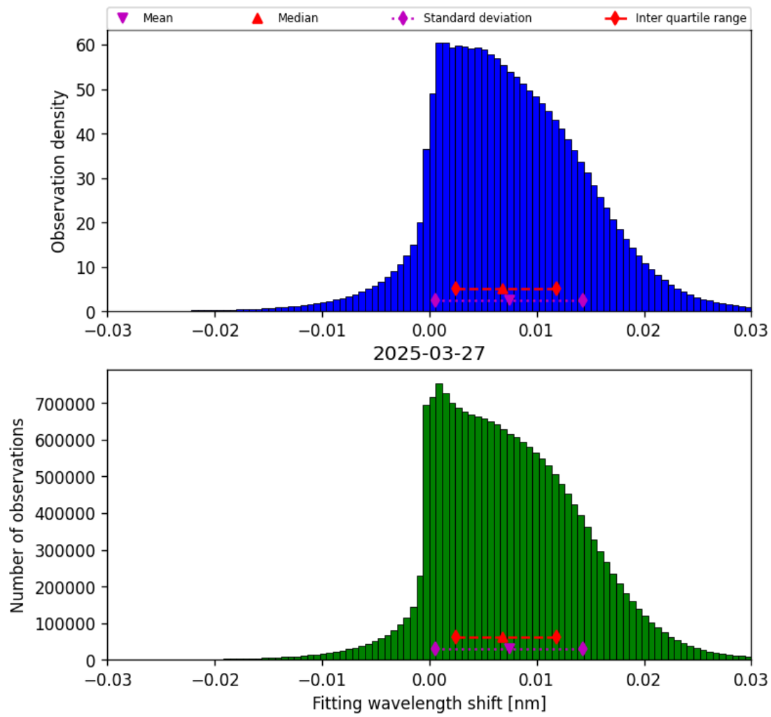
Figure 47: Histogram of “Fitting wavelength shift” for 2025-03-27 to 2025-03-28
