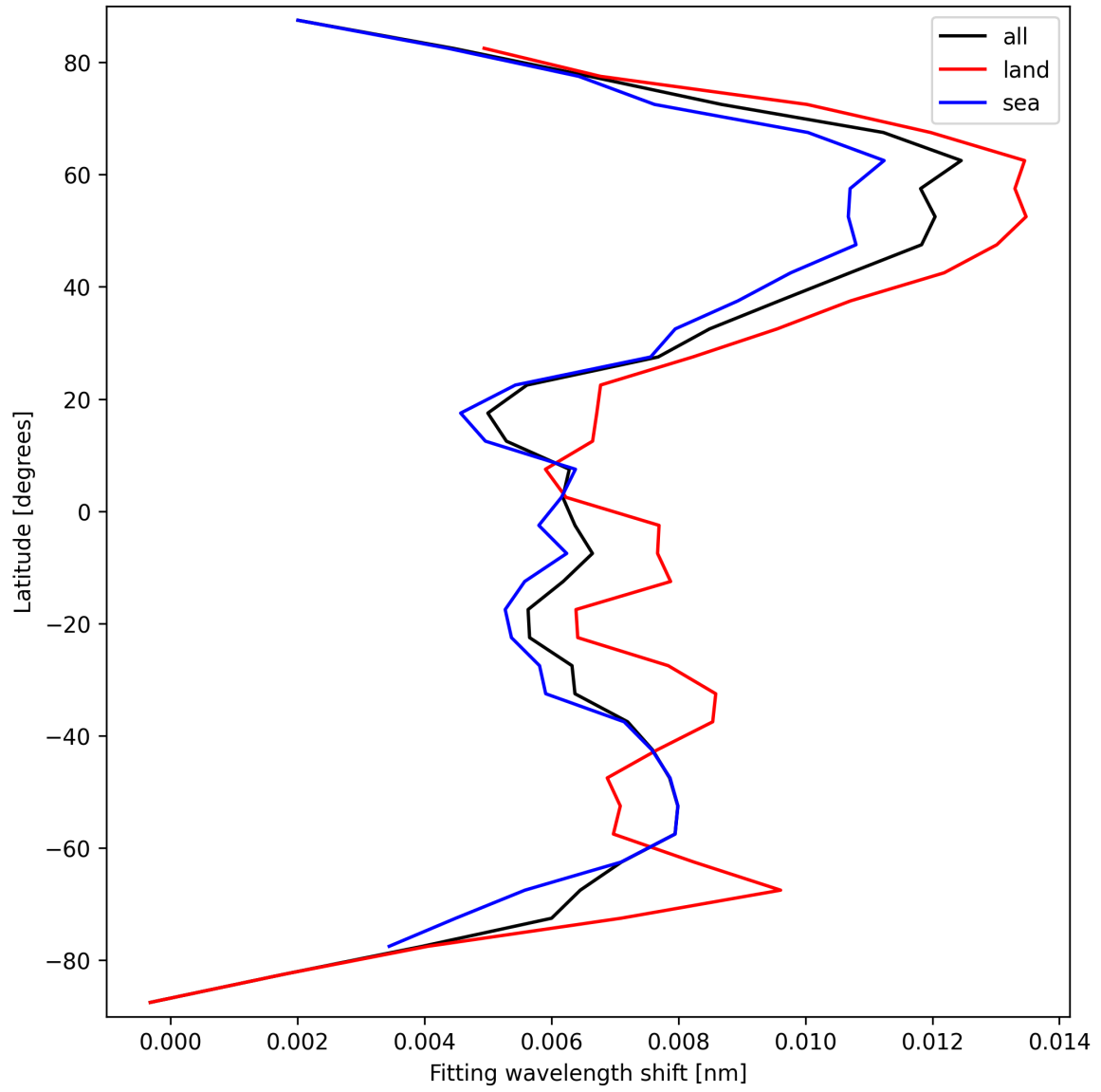
Figure 31: Zonal average of “Fitting wavelength shift” for 2025-03-27 to 2025-03-28.
