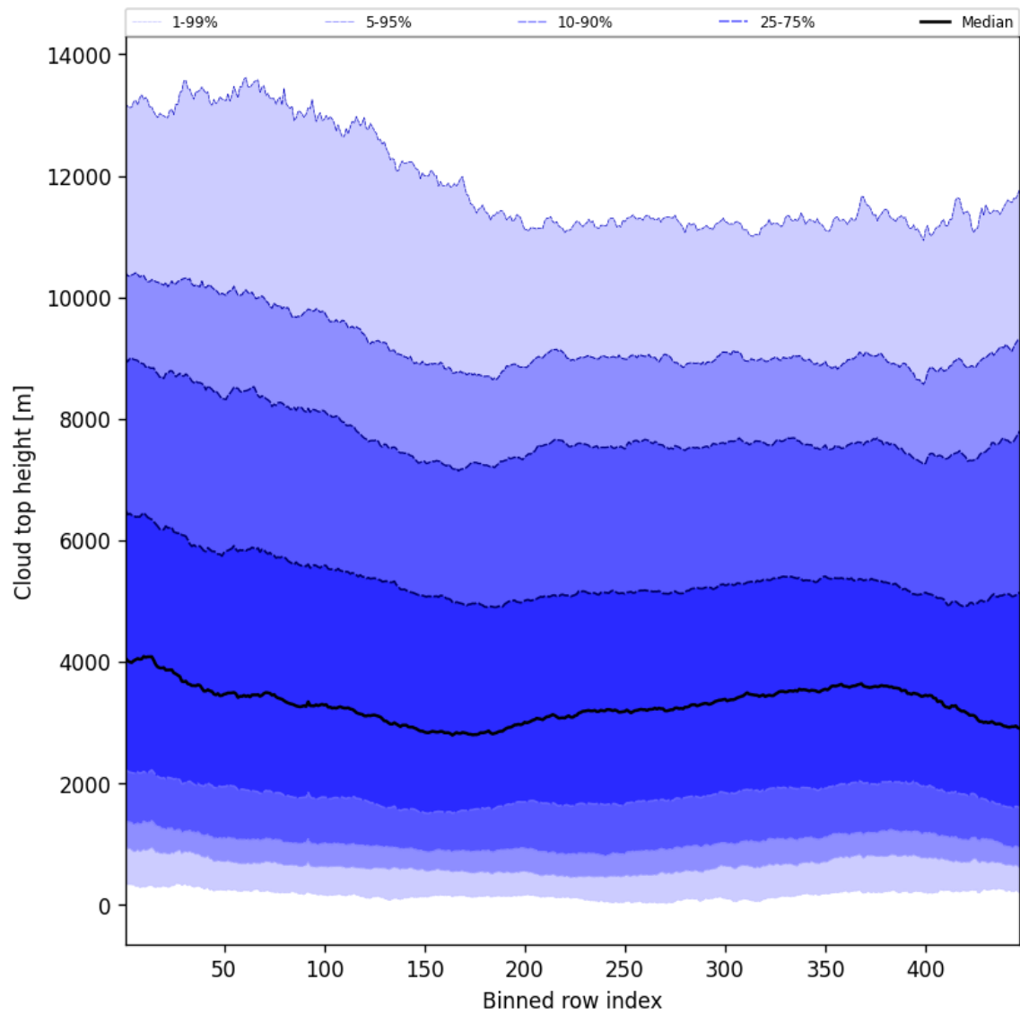
Figure 54: Along track statistics of “Cloud top height” for 2025-03-27 to 2025-03-28
