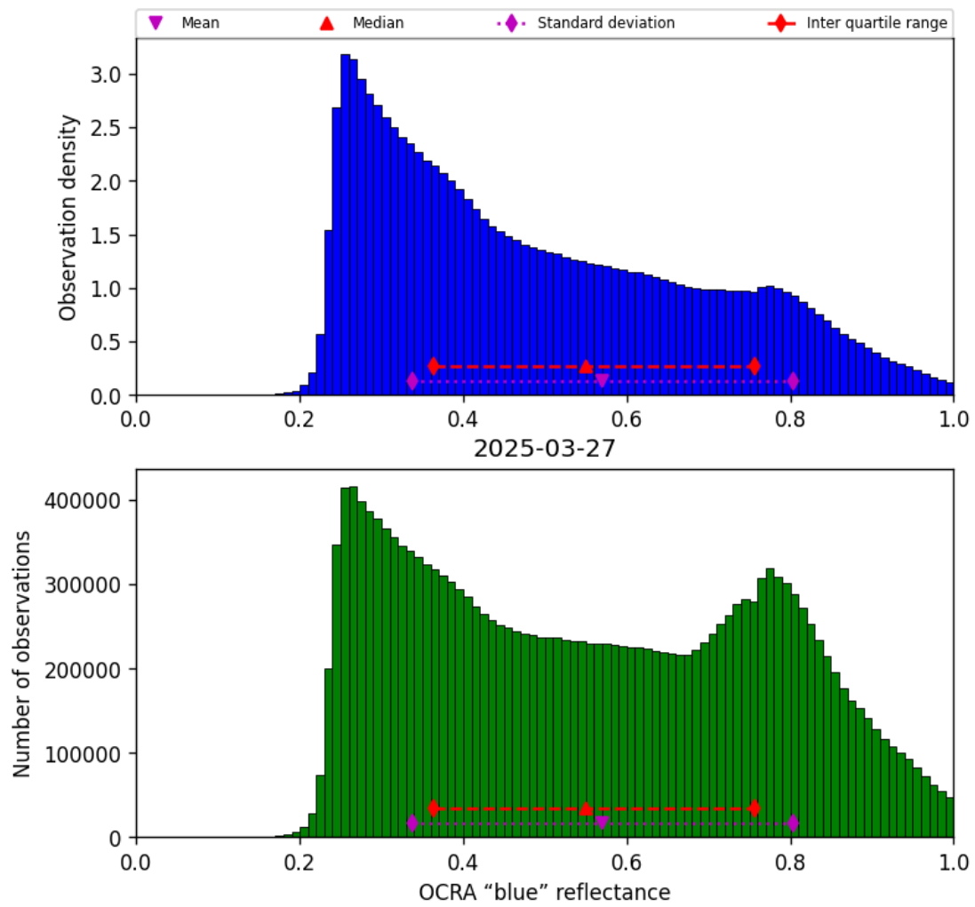
Figure 49: Histogram of “OCRA “blue” reflectance” for 2025-03-27 to 2025-03-28
