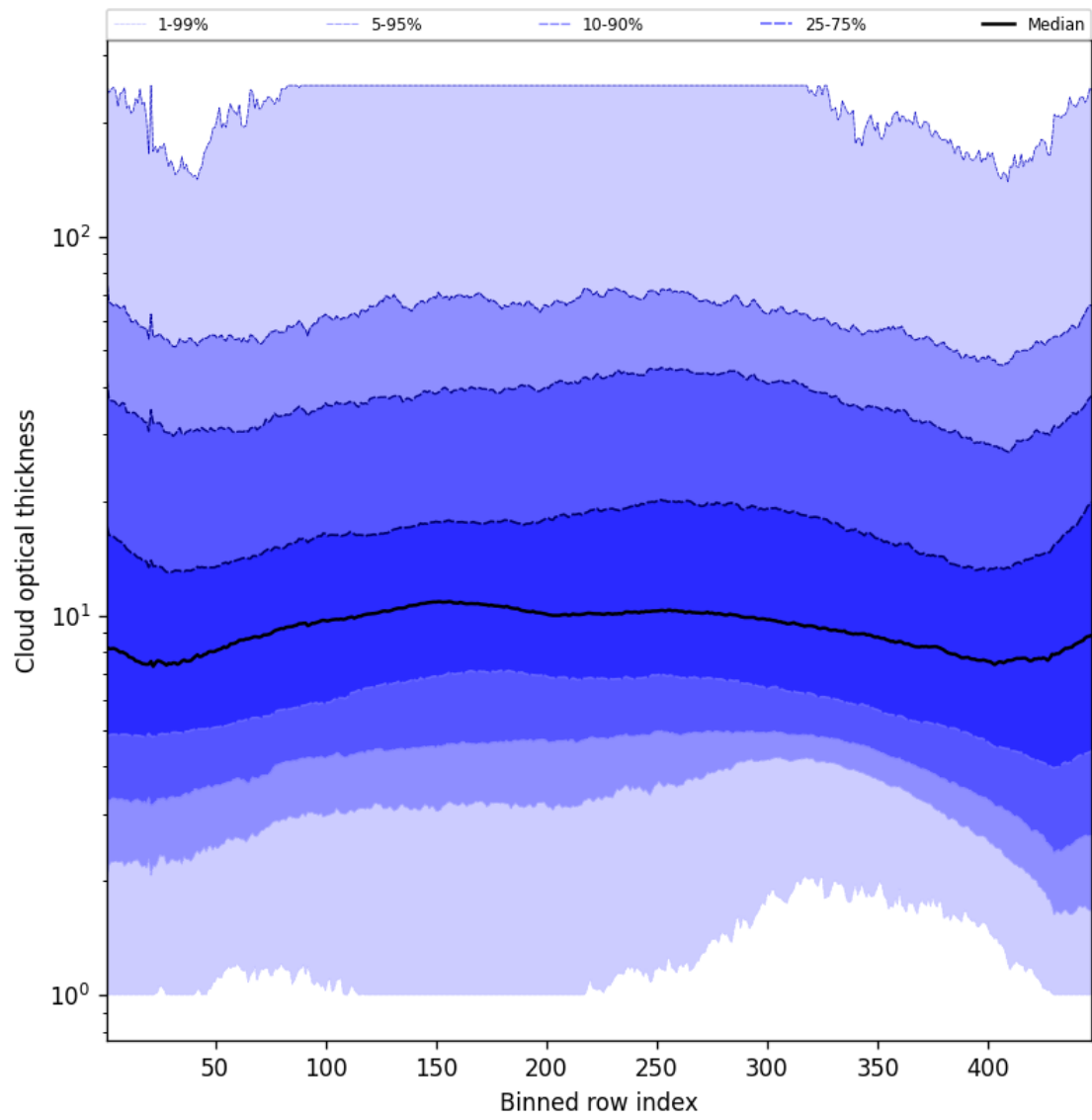
Figure 55: Along track statistics of “Cloud optical thickness” for 2025-03-27 to 2025-03-28
