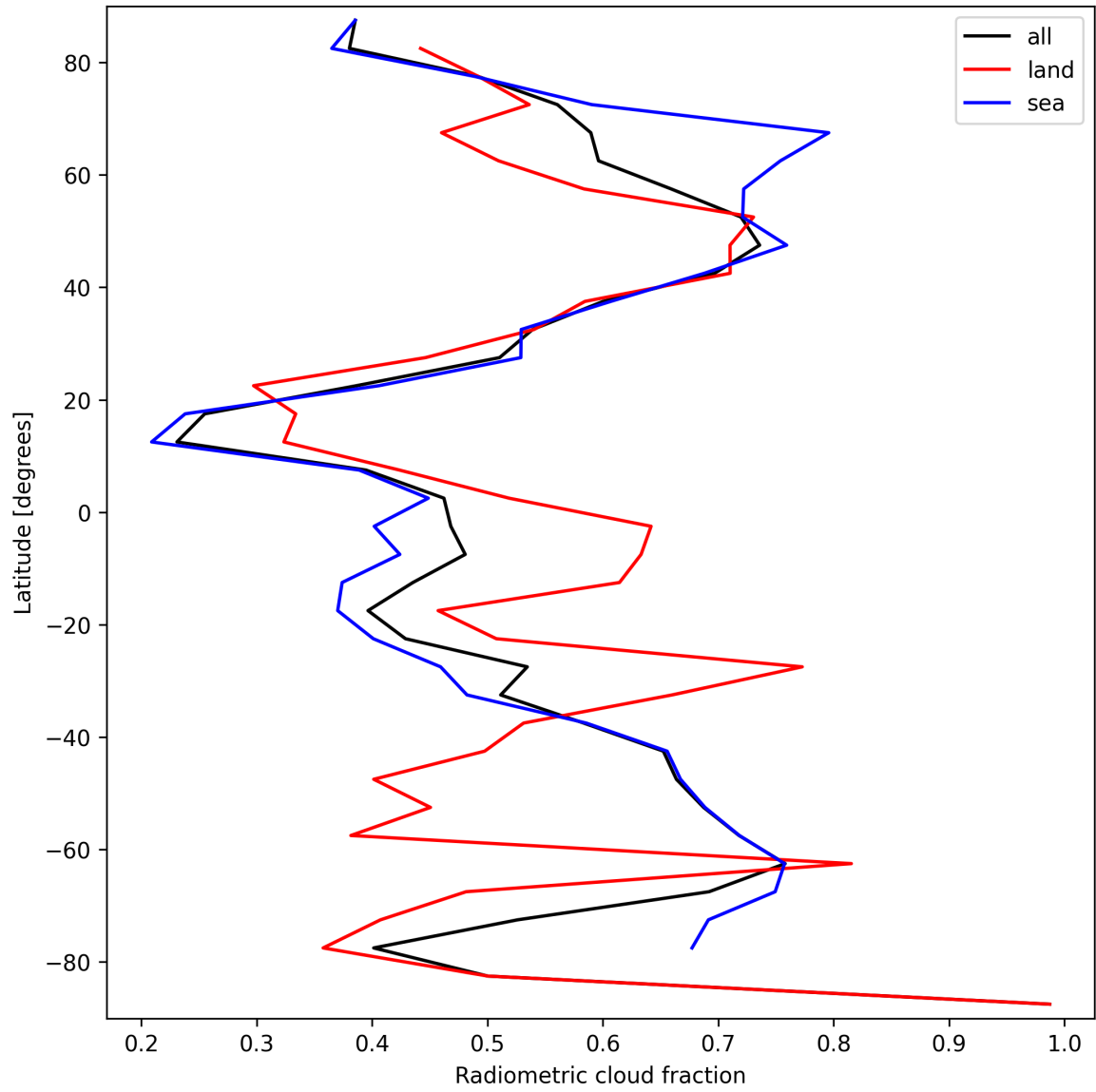
Figure 21: Zonal average of “Radiometric cloud fraction” for 2025-03-27 to 2025-03-28.
