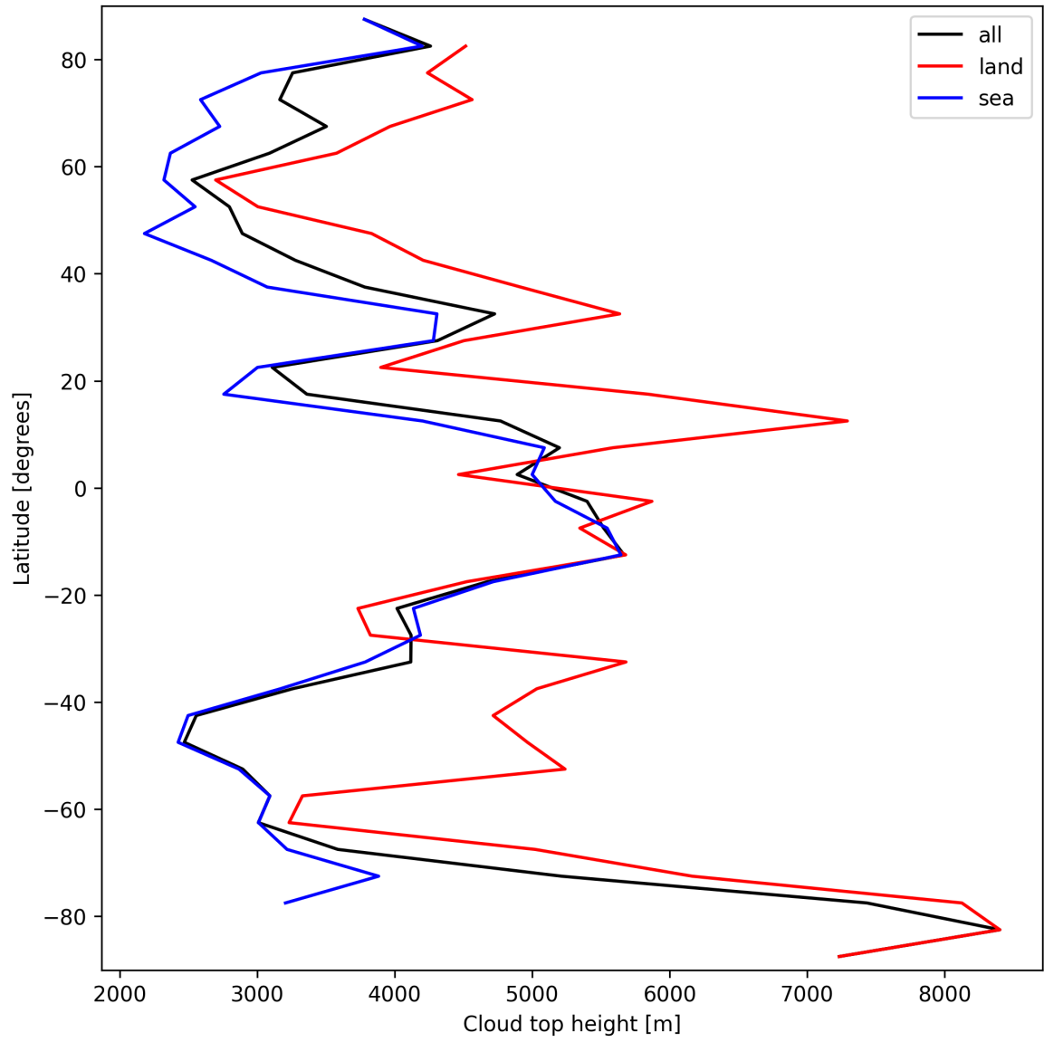
Figure 22: Zonal average of “Cloud top height” for 2025-03-27 to 2025-03-28.
