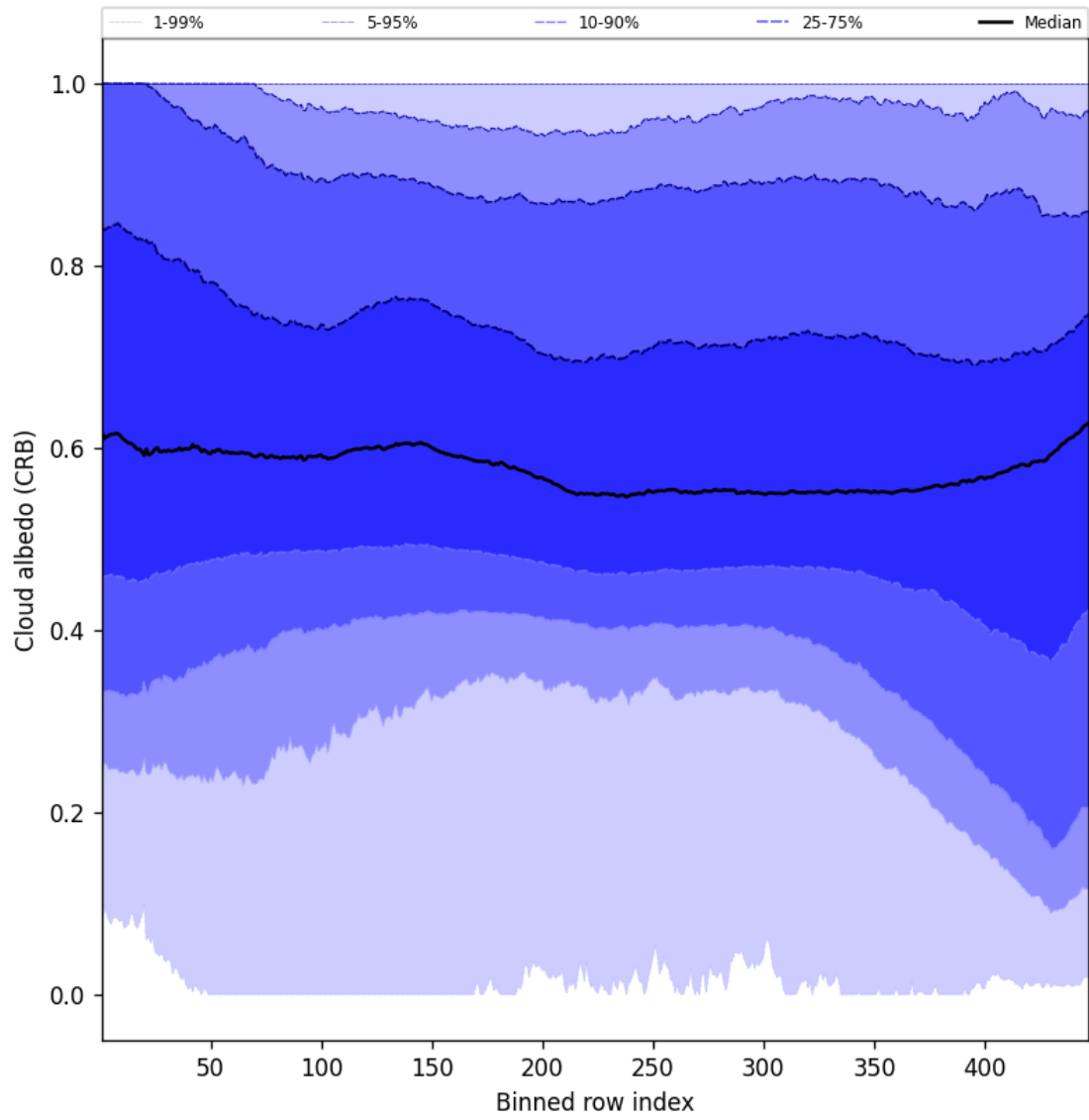
Figure 58: Along track statistics of “Cloud albedo (CRB)” for 2025-03-27 to 2025-03-28
