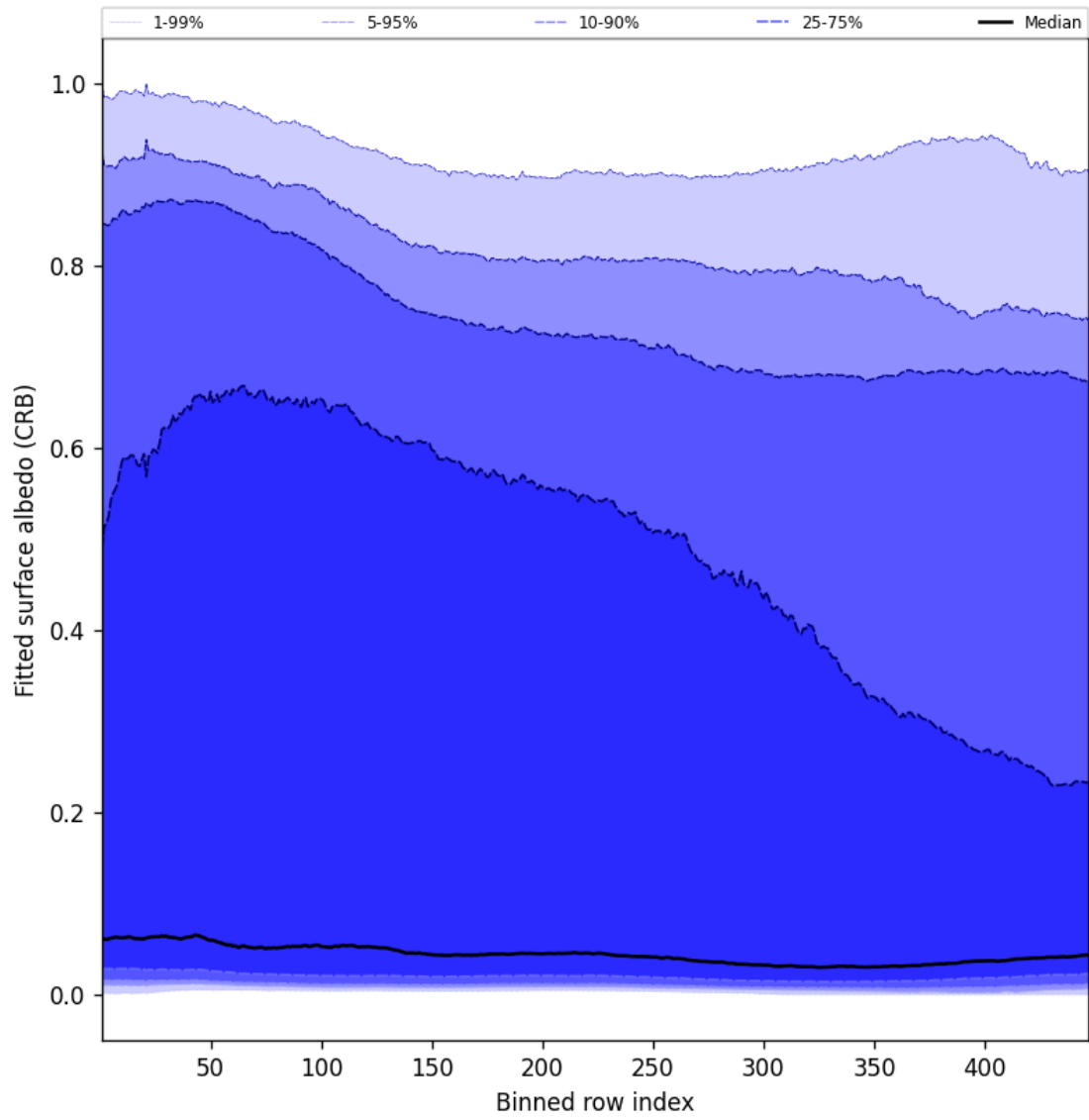
Figure 60: Along track statistics of “Fitted surface albedo (CRB)” for 2025-03-27 to 2025-03-28
