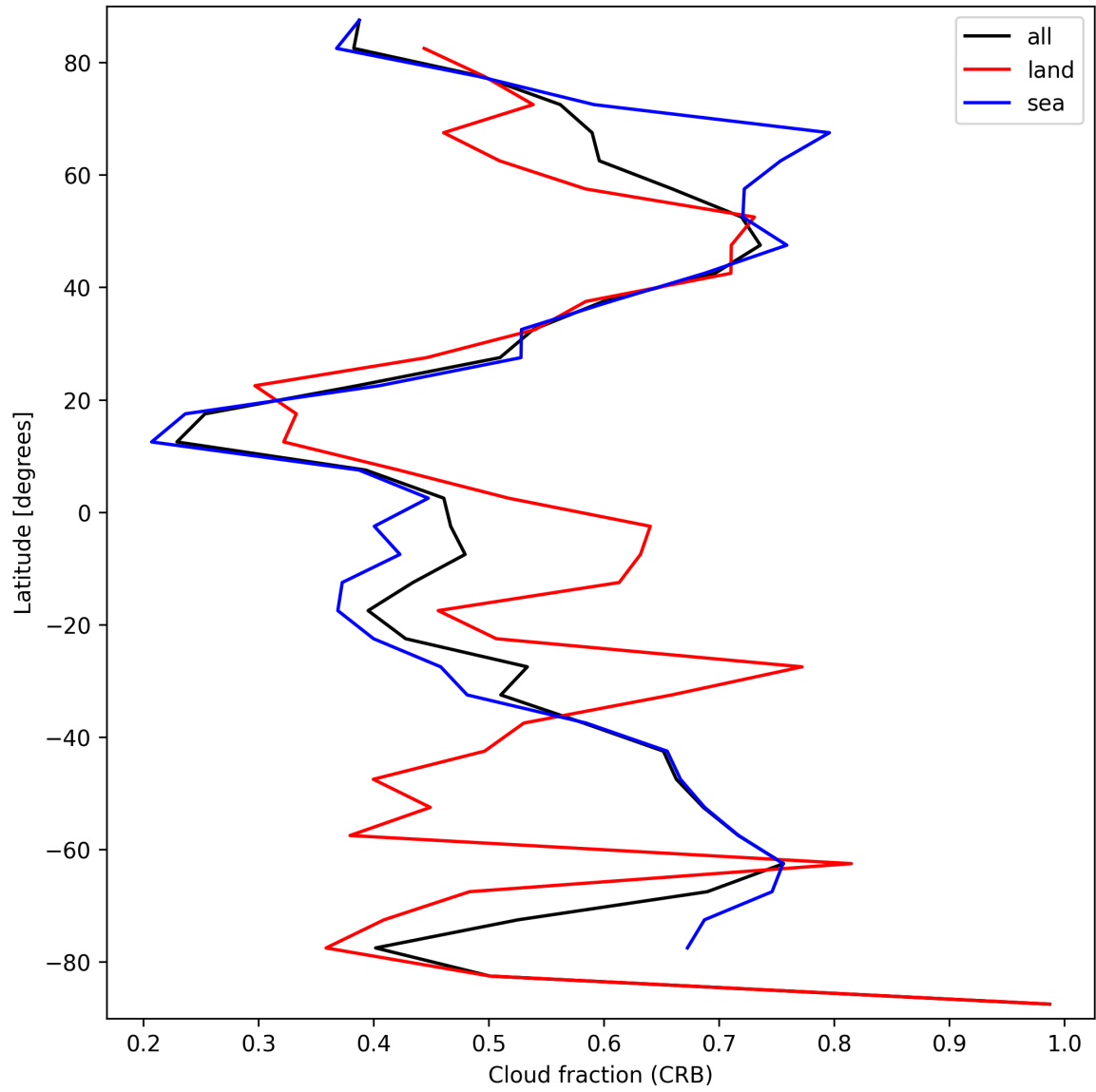
Figure 24: Zonal average of “Cloud fraction (CRB)” for 2025-03-27 to 2025-03-28.
