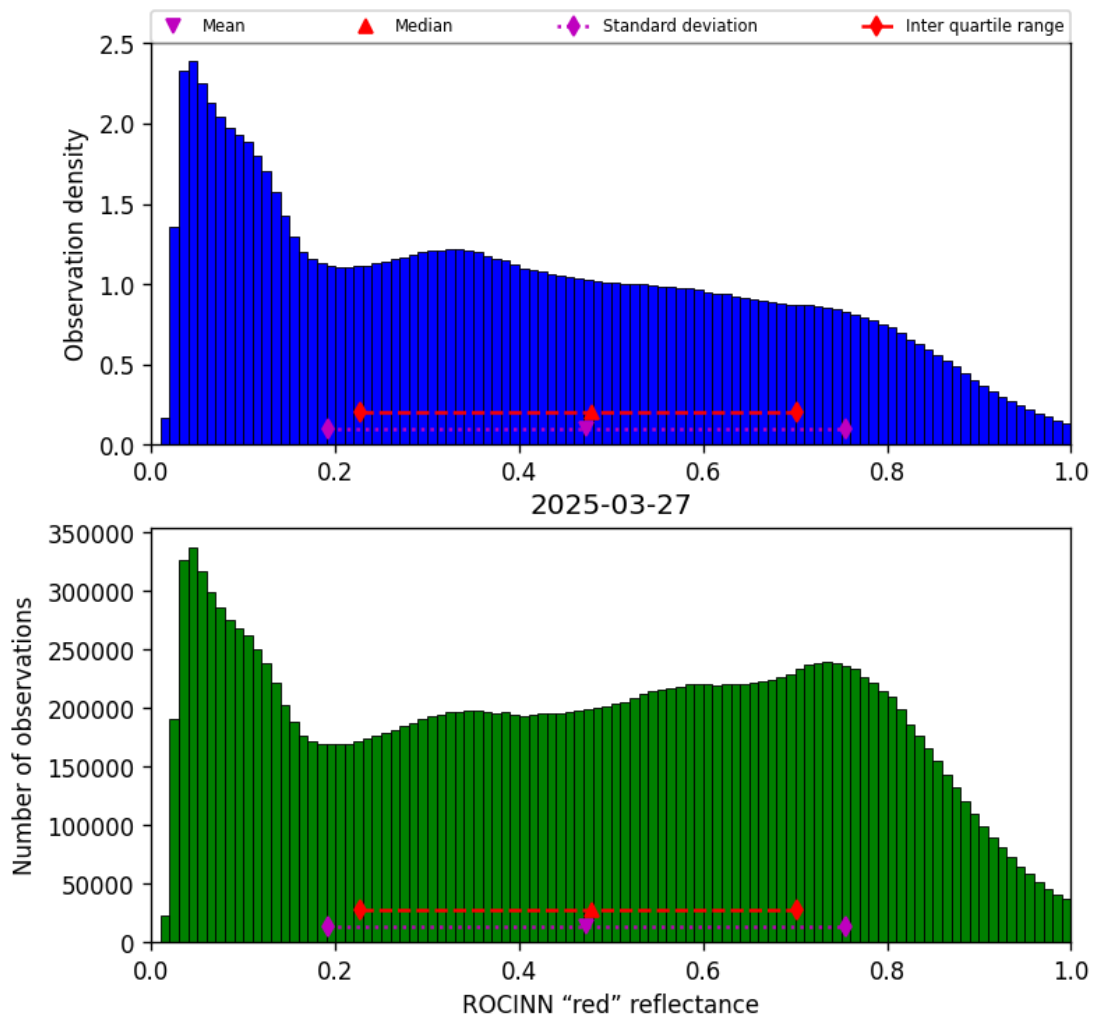
Figure 51: Histogram of “ROCINN “red” reflectance” for 2025-03-27 to 2025-03-28
