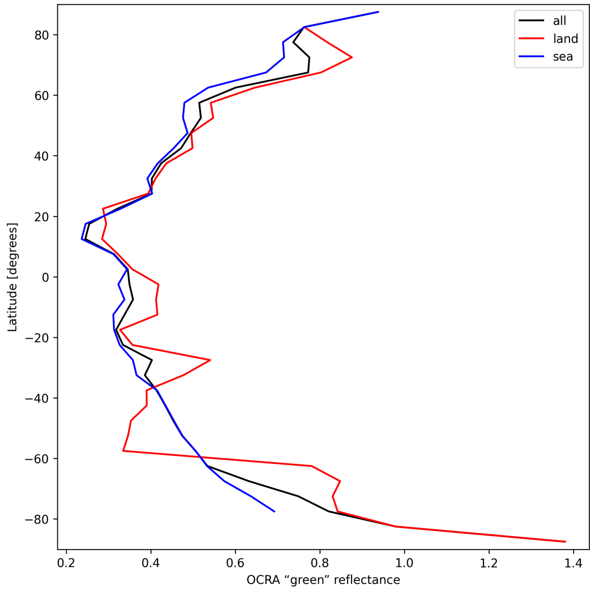
Figure 34: Zonal average of “OCRA “green” reflectance” for 2025-03-27 to 2025-03-28.
