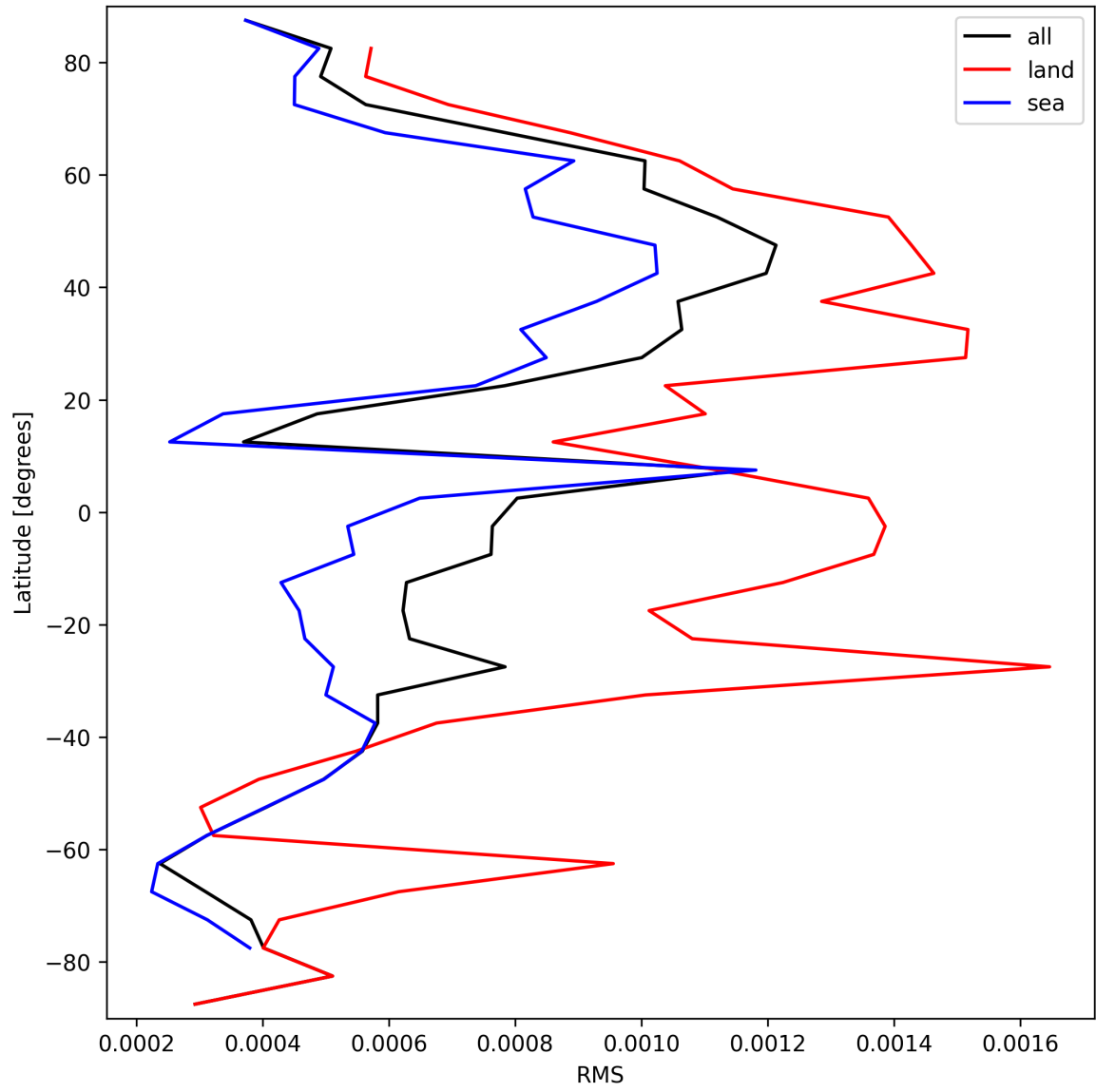
Figure 29: Zonal average of “RMS” for 2025-03-27 to 2025-03-28.
