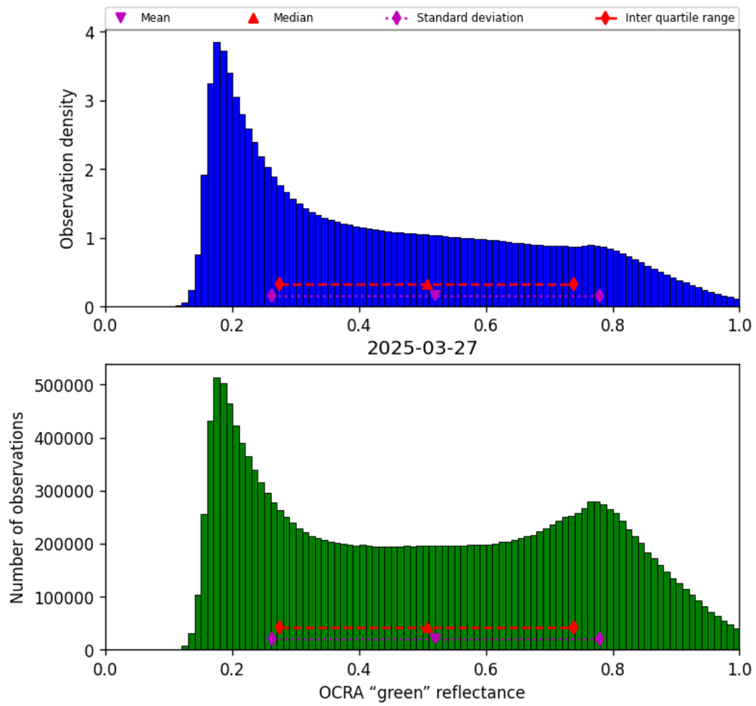
Figure 50: Histogram of “OCRA “green” reflectance” for 2025-03-27 to 2025-03-28
