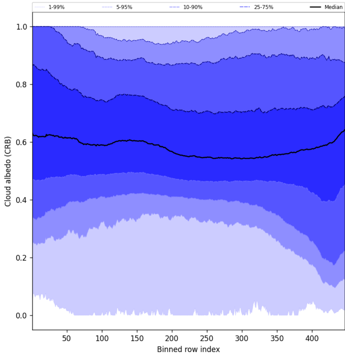
Figure 58: Along track statistics of “Cloud albedo (CRB)” for 2025-03-29 to 2025-03-30
