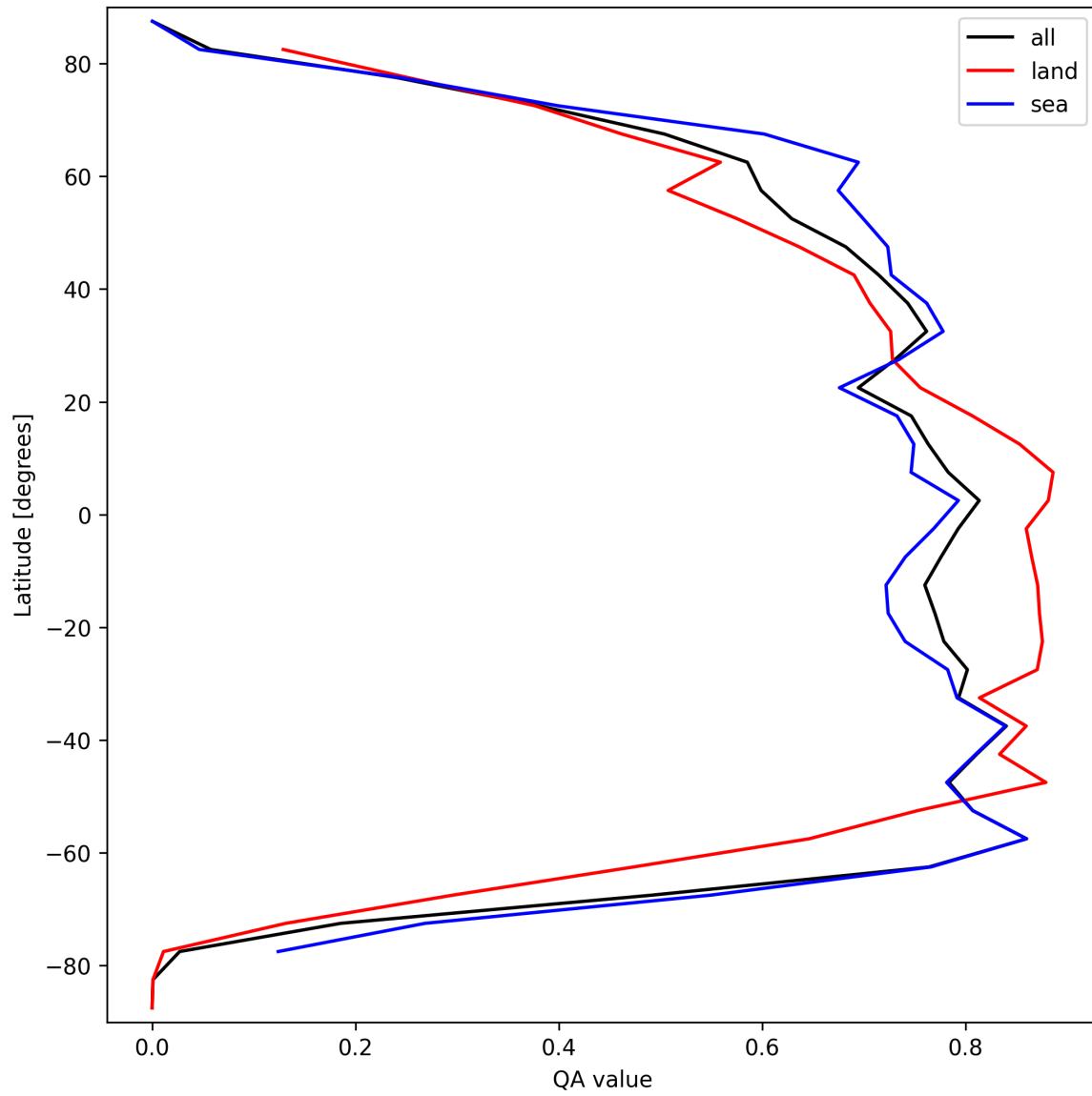
Figure 20: Zonal average of “QA value” for 2025-03-29 to 2025-03-30.
