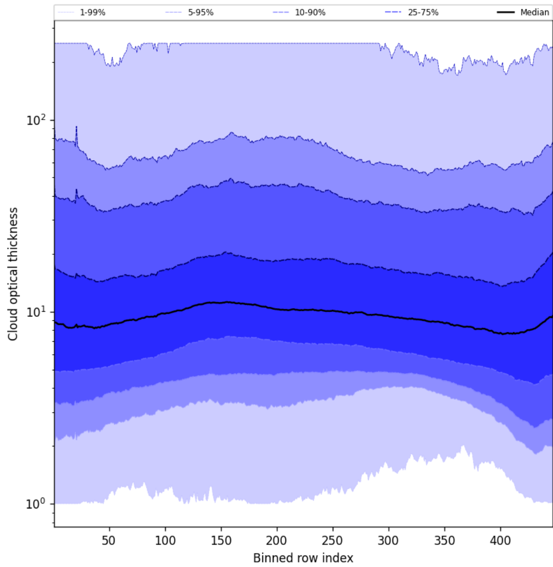
Figure 55: Along track statistics of “Cloud optical thickness” for 2025-03-29 to 2025-03-30
