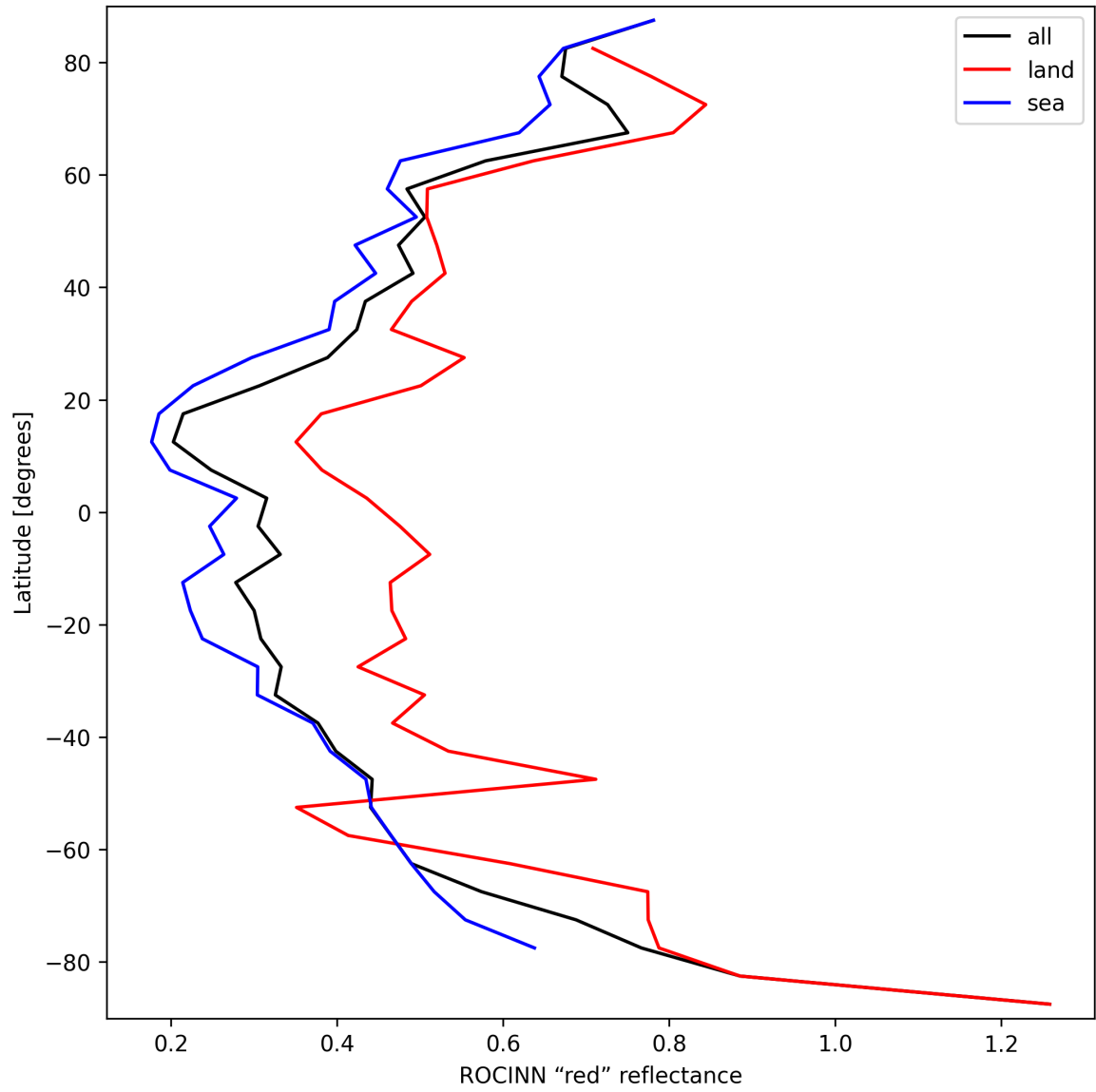
Figure 35: Zonal average of “ROCINN “red” reflectance” for 2025-03-29 to 2025-03-30.
