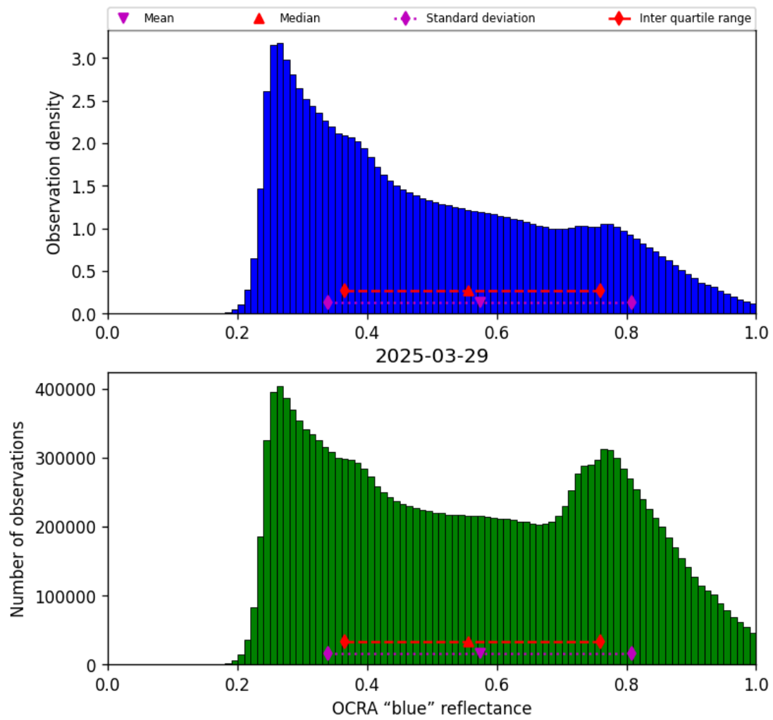
Figure 49: Histogram of "OCRA "blue" reflectance" for 2025-03-29 to 2025-03-30
