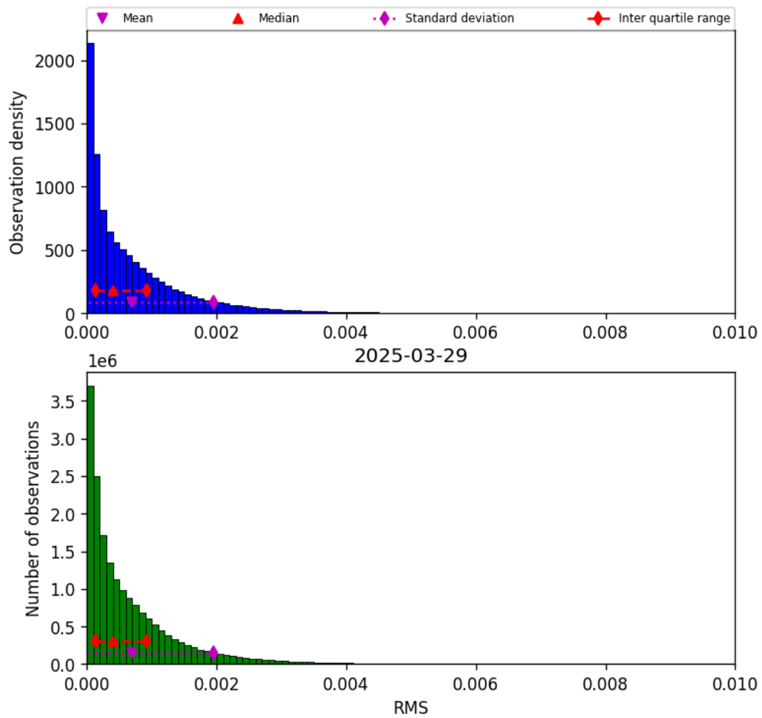
Figure 45: Histogram of “RMS” for 2025-03-29 to 2025-03-30
