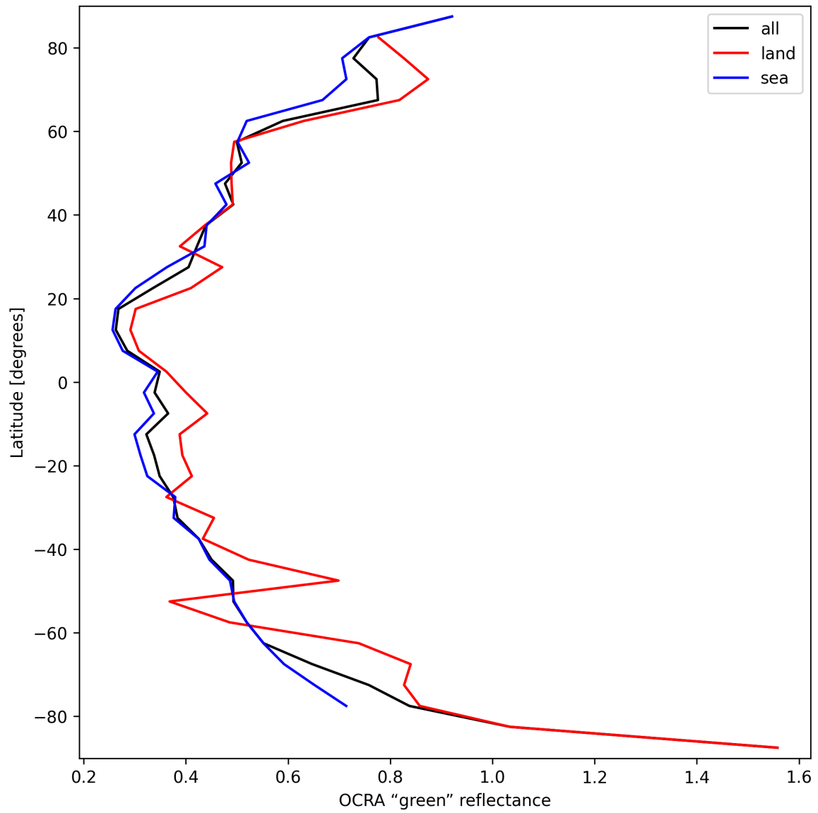
Figure 34: Zonal average of “OCRA “green” reflectance” for 2025-03-29 to 2025-03-30.
