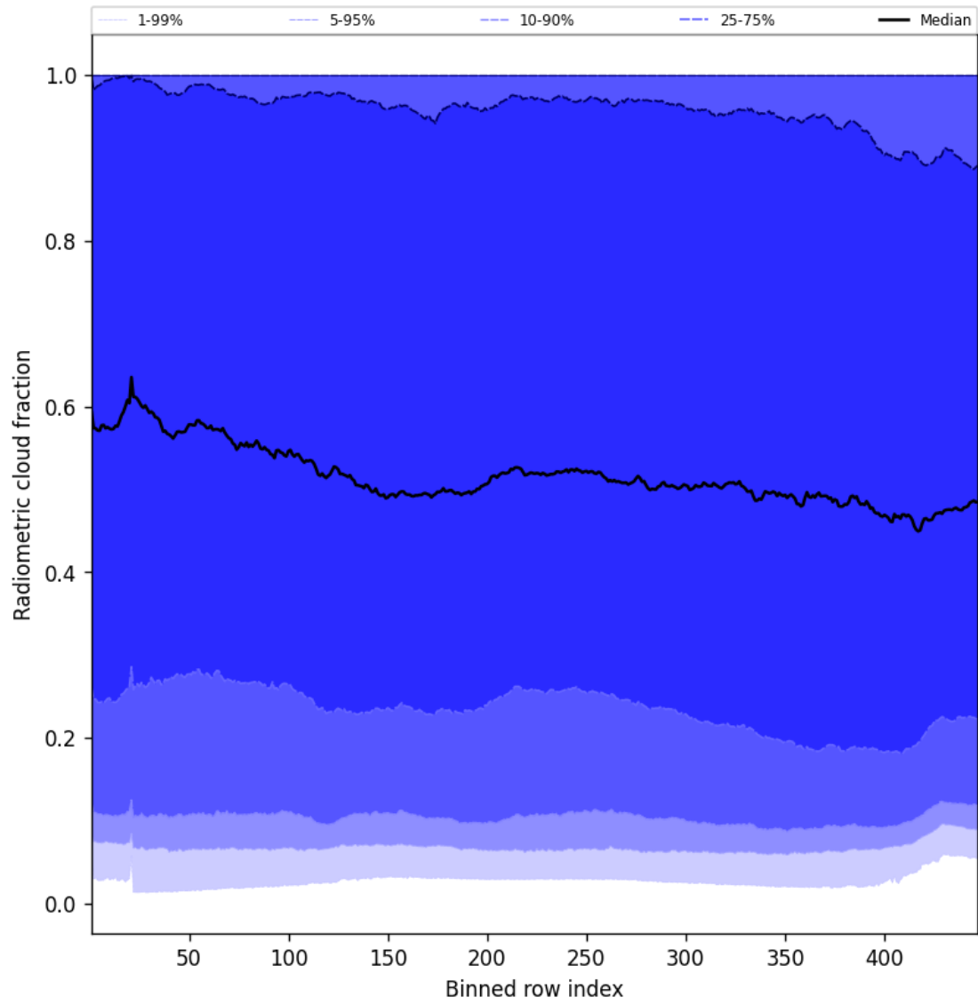
Figure 53: Along track statistics of “Radiometric cloud fraction” for 2025-03-29 to 2025-03-30
