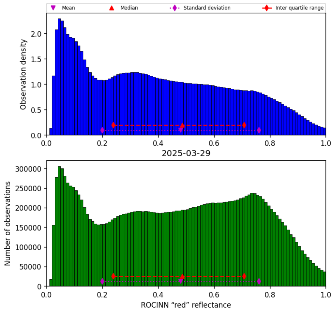
Figure 51: Histogram of “ROCINN “red” reflectance” for 2025-03-29 to 2025-03-30
