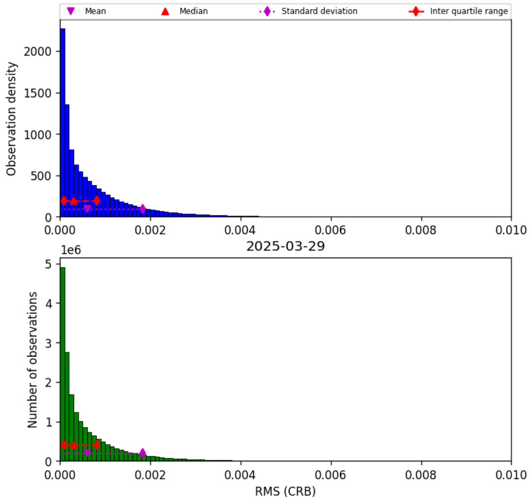
Figure 46: Histogram of “RMS (CRB)” for 2025-03-29 to 2025-03-30
