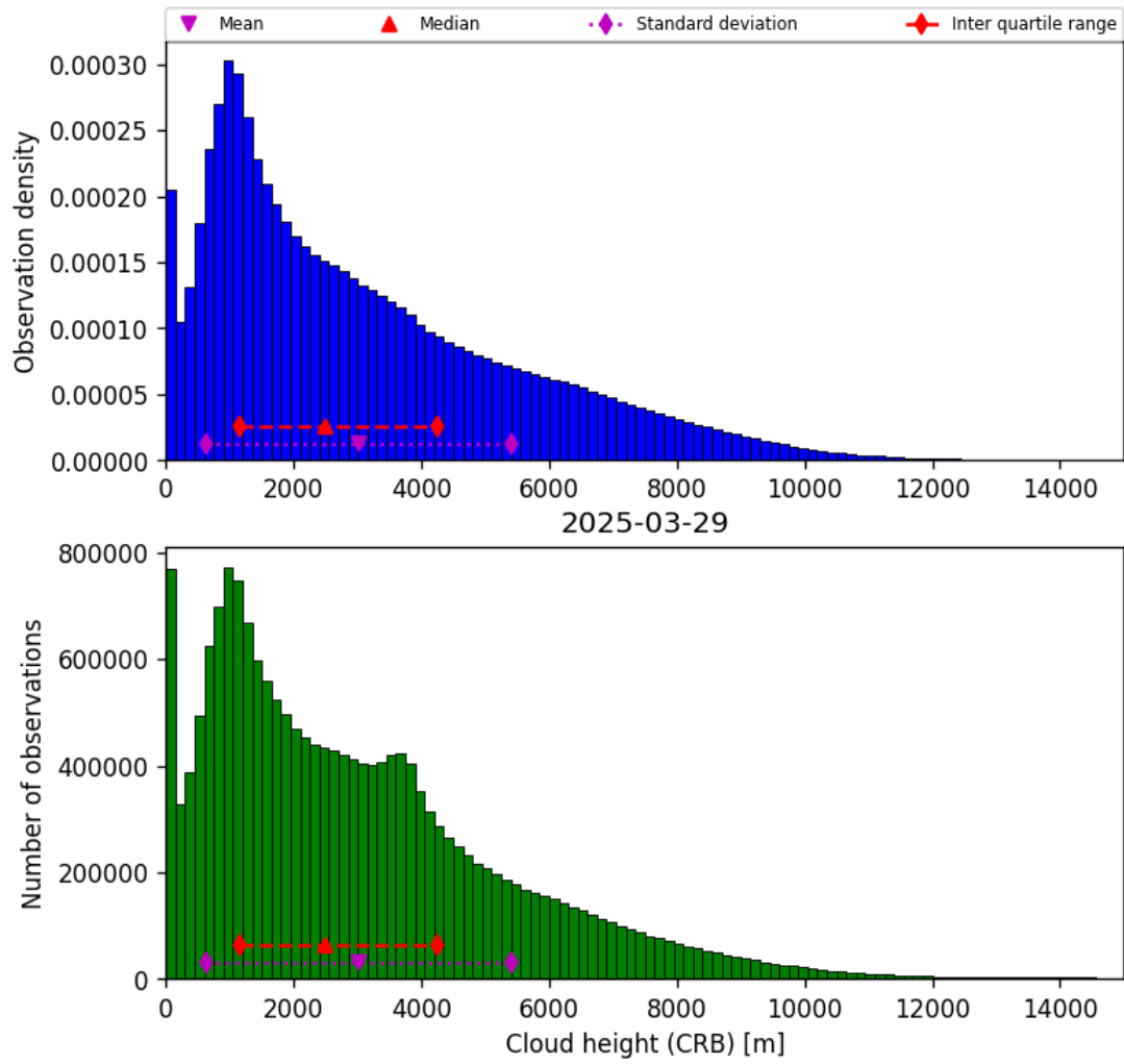
Figure 41: Histogram of “Cloud height (CRB)” for 2025-03-29 to 2025-03-30
