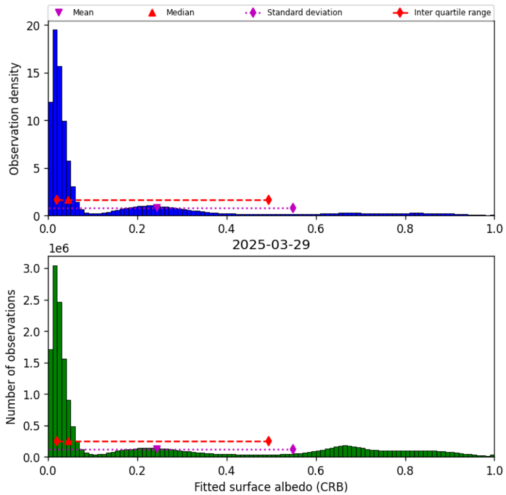
Figure 44: Histogram of “Fitted surface albedo (CRB)” for 2025-03-29 to 2025-03-30
