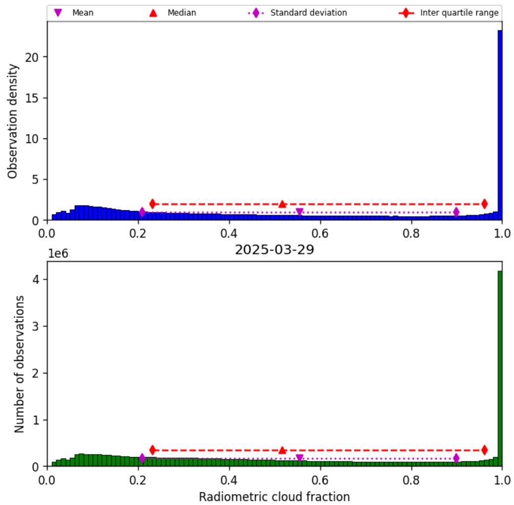
Figure 37: Histogram of “Radiometric cloud fraction” for 2025-03-29 to 2025-03-30
