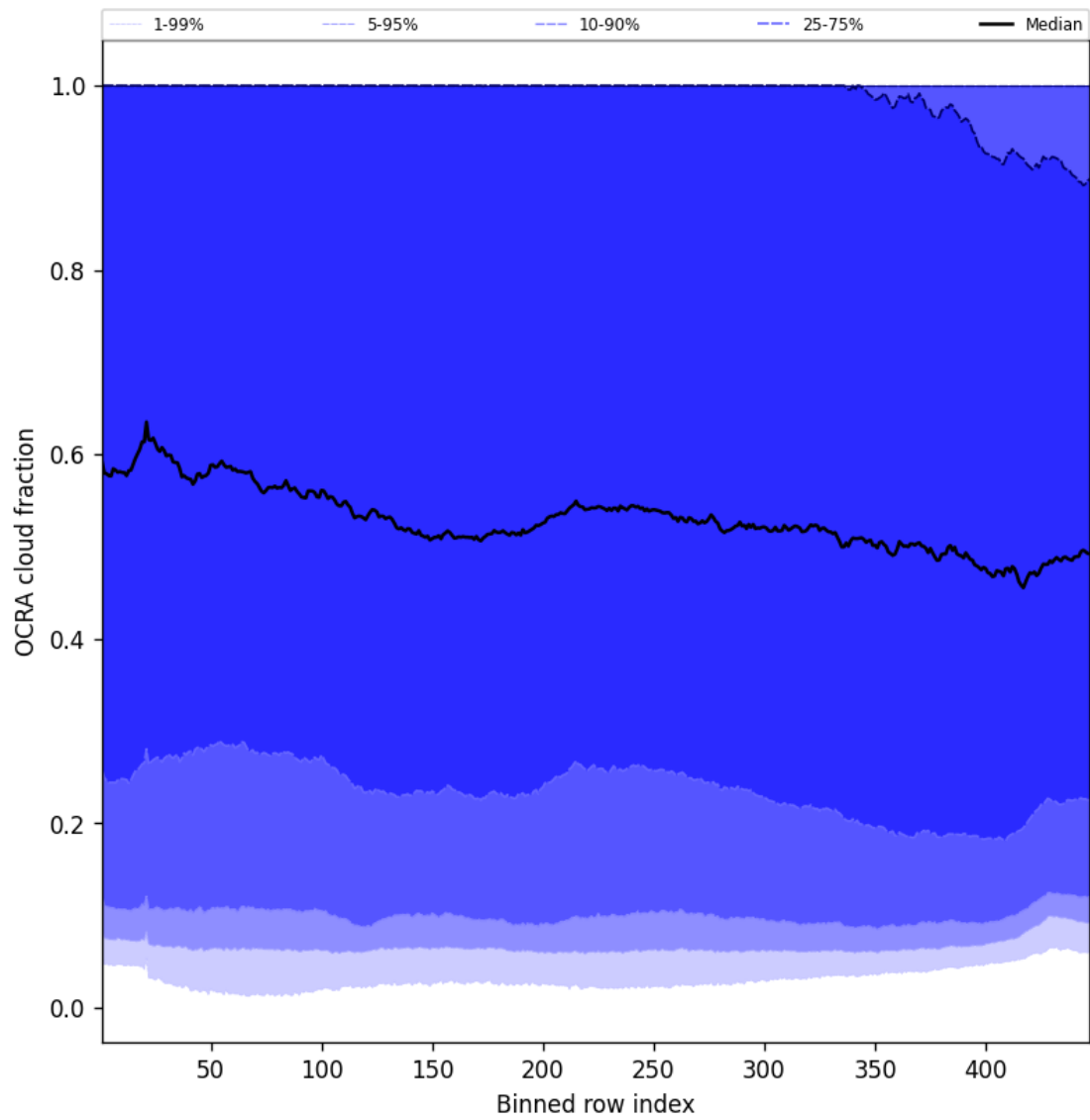
Figure 64: Along track statistics of “OCRA cloud fraction” for 2025-03-29 to 2025-03-30
