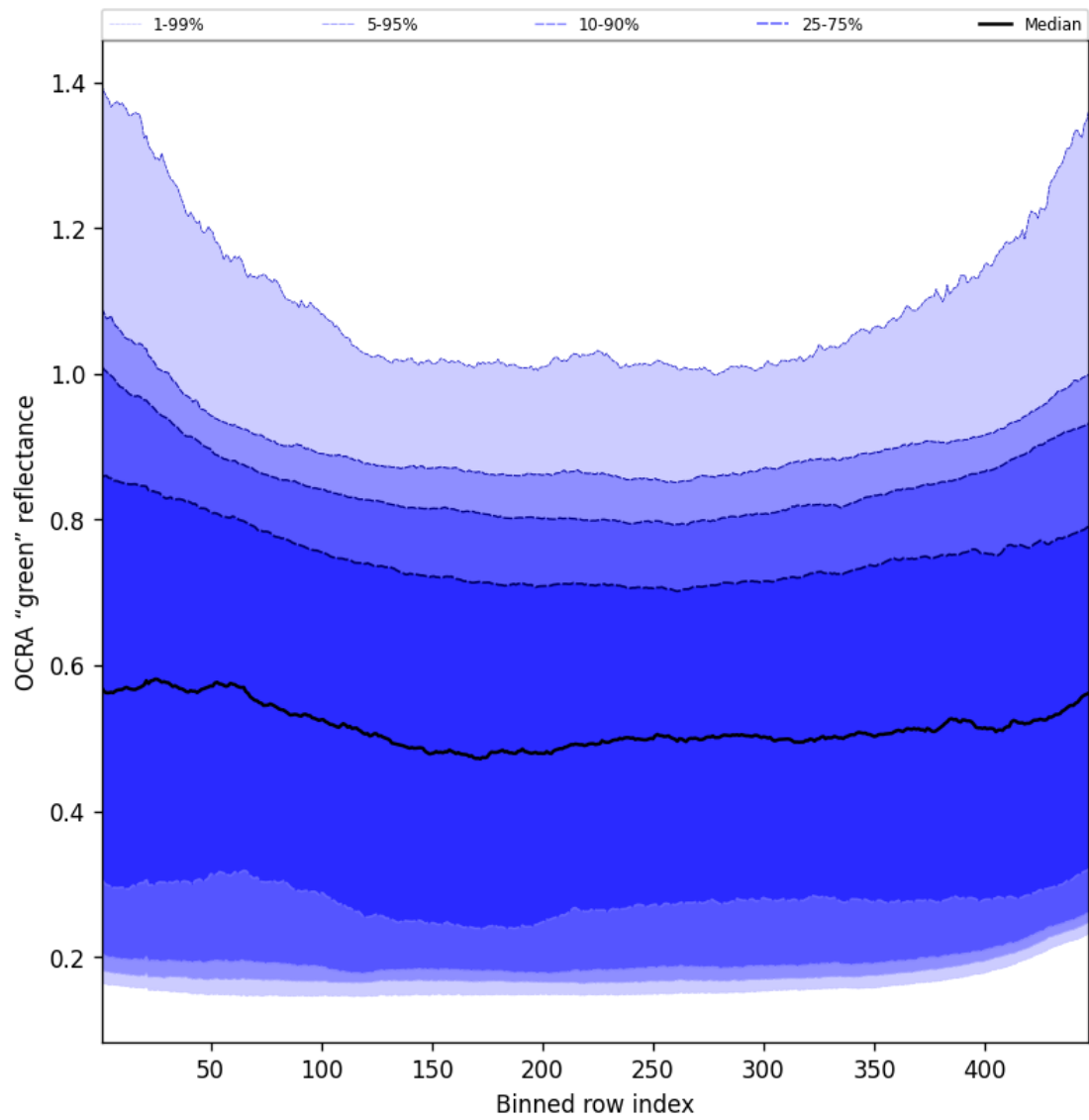
Figure 66: Along track statistics of “OCRA “green” reflectance” for 2025-03-29 to 2025-03-30
