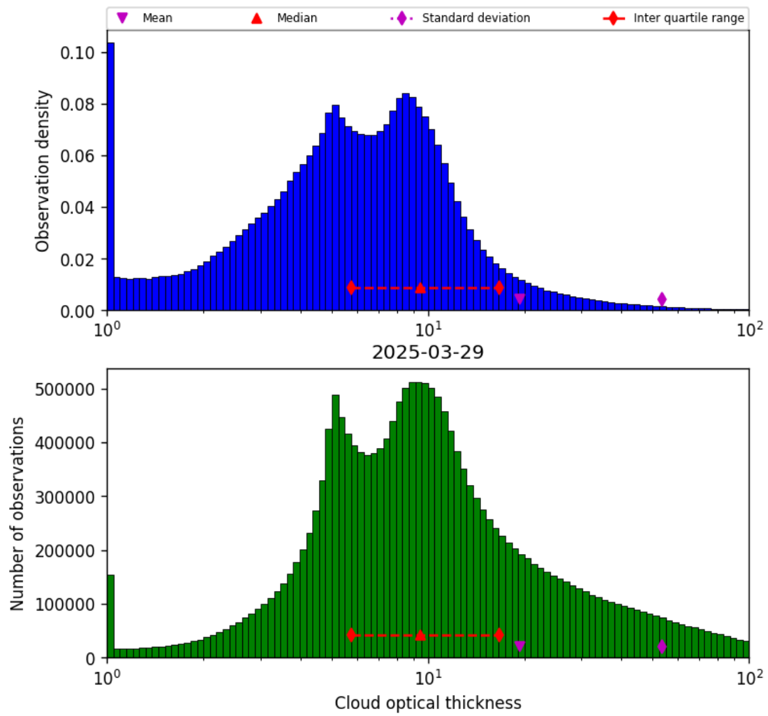
Figure 39: Histogram of “Cloud optical thickness” for 2025-03-29 to 2025-03-30
