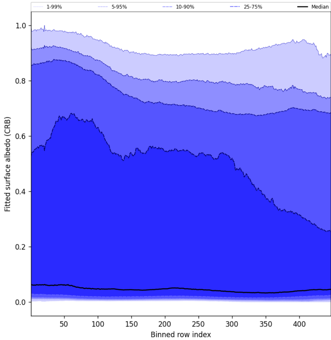
Figure 60: Along track statistics of “Fitted surface albedo (CRB)” for 2025-03-29 to 2025-03-30
