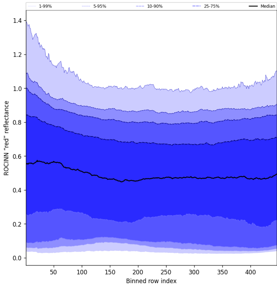
Figure 67: Along track statistics of “ROCINN “red” reflectance” for 2025-03-29 to 2025-03-30
