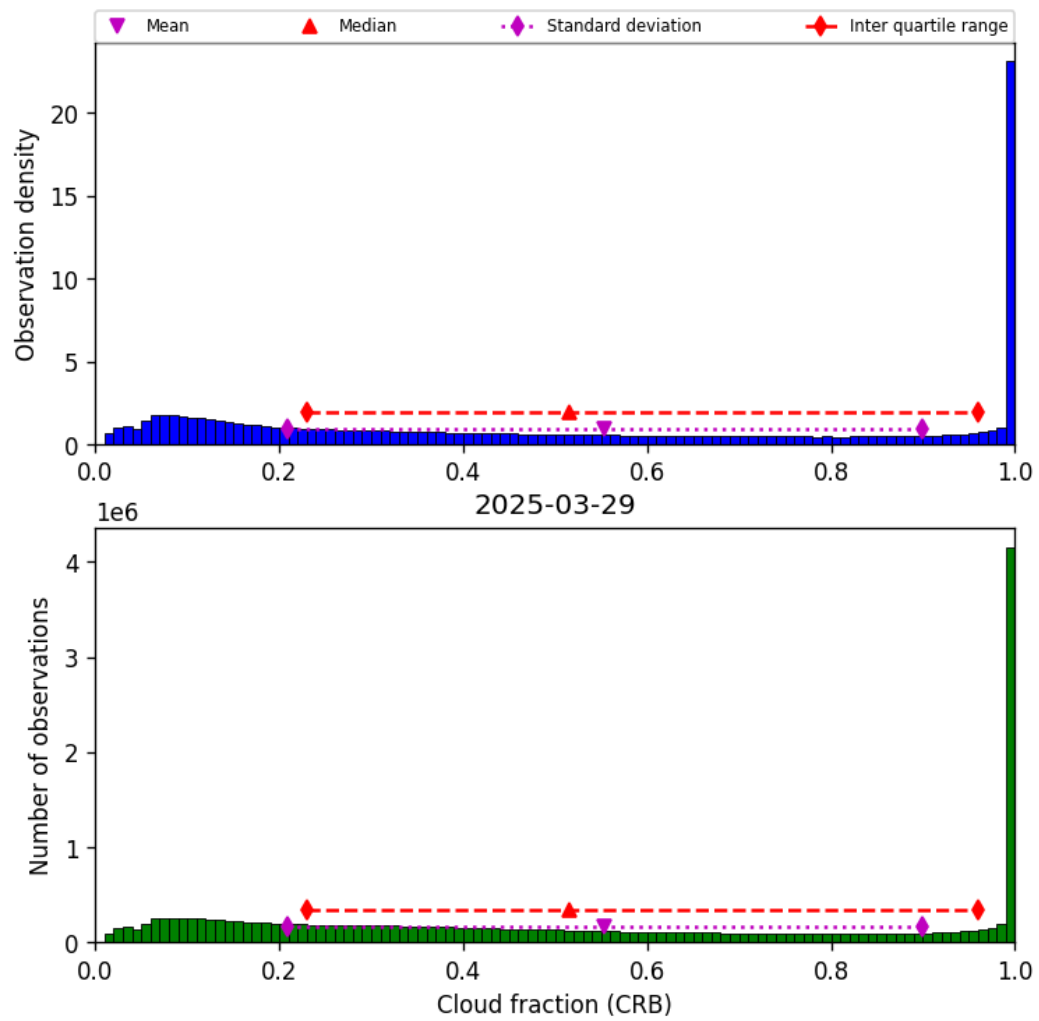
Figure 40: Histogram of “Cloud fraction (CRB)” for 2025-03-29 to 2025-03-30
