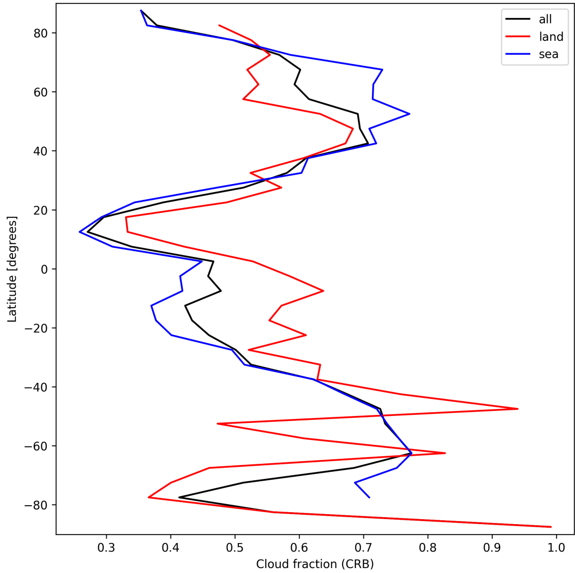
Figure 24: Zonal average of “Cloud fraction (CRB)” for 2025-03-29 to 2025-03-30.
