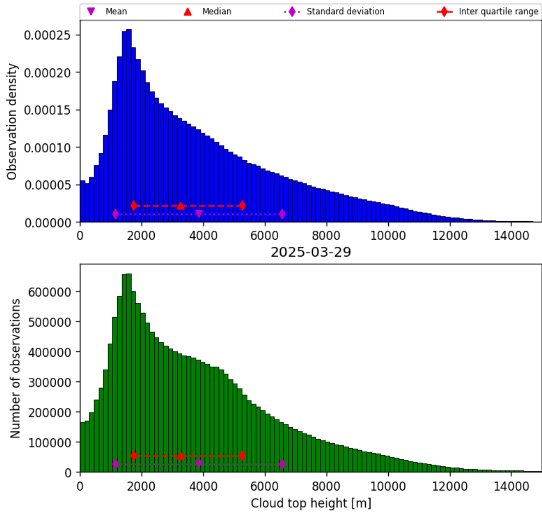
Figure 38: Histogram of “Cloud top height” for 2025-03-29 to 2025-03-30
