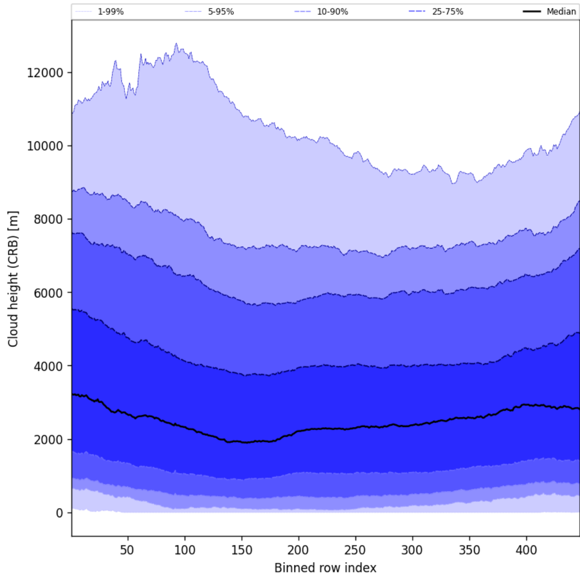
Figure 57: Along track statistics of “Cloud height (CRB)” for 2025-03-29 to 2025-03-30
