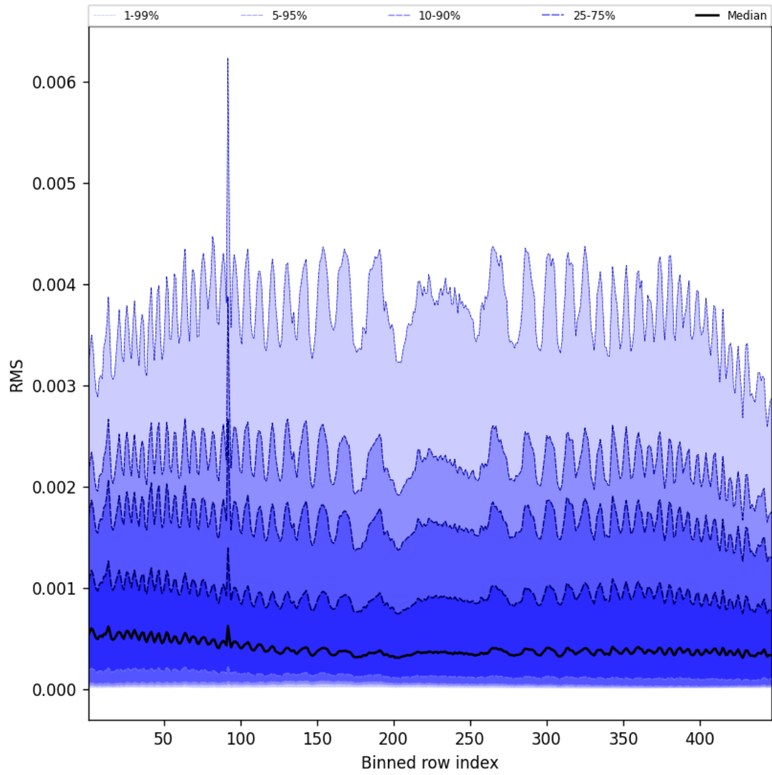
Figure 61: Along track statistics of “RMS” for 2025-03-29 to 2025-03-30
