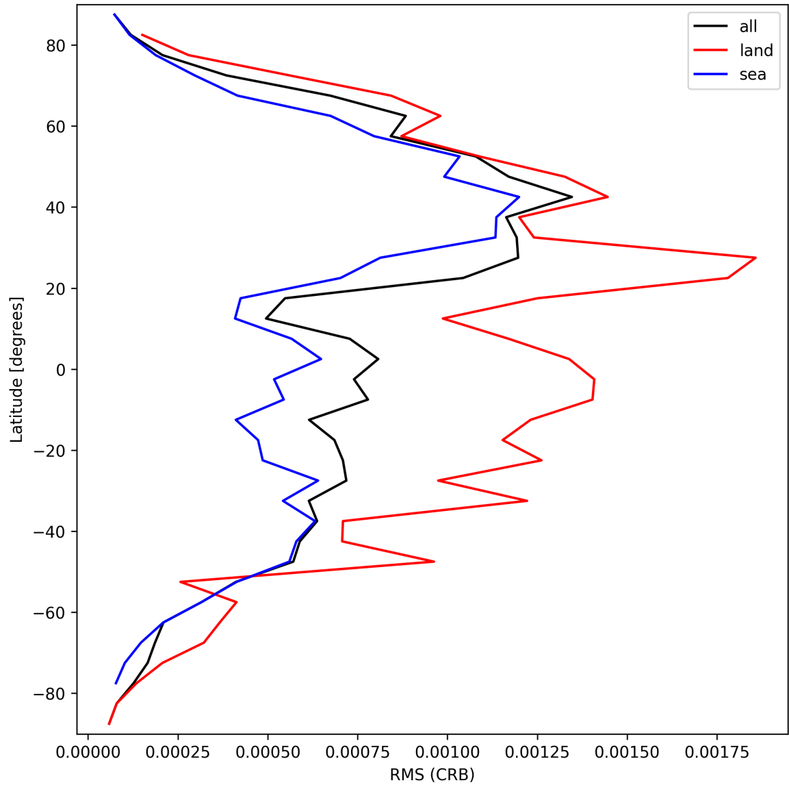
Figure 30: Zonal average of “RMS (CRB)” for 2025-03-29 to 2025-03-30.
