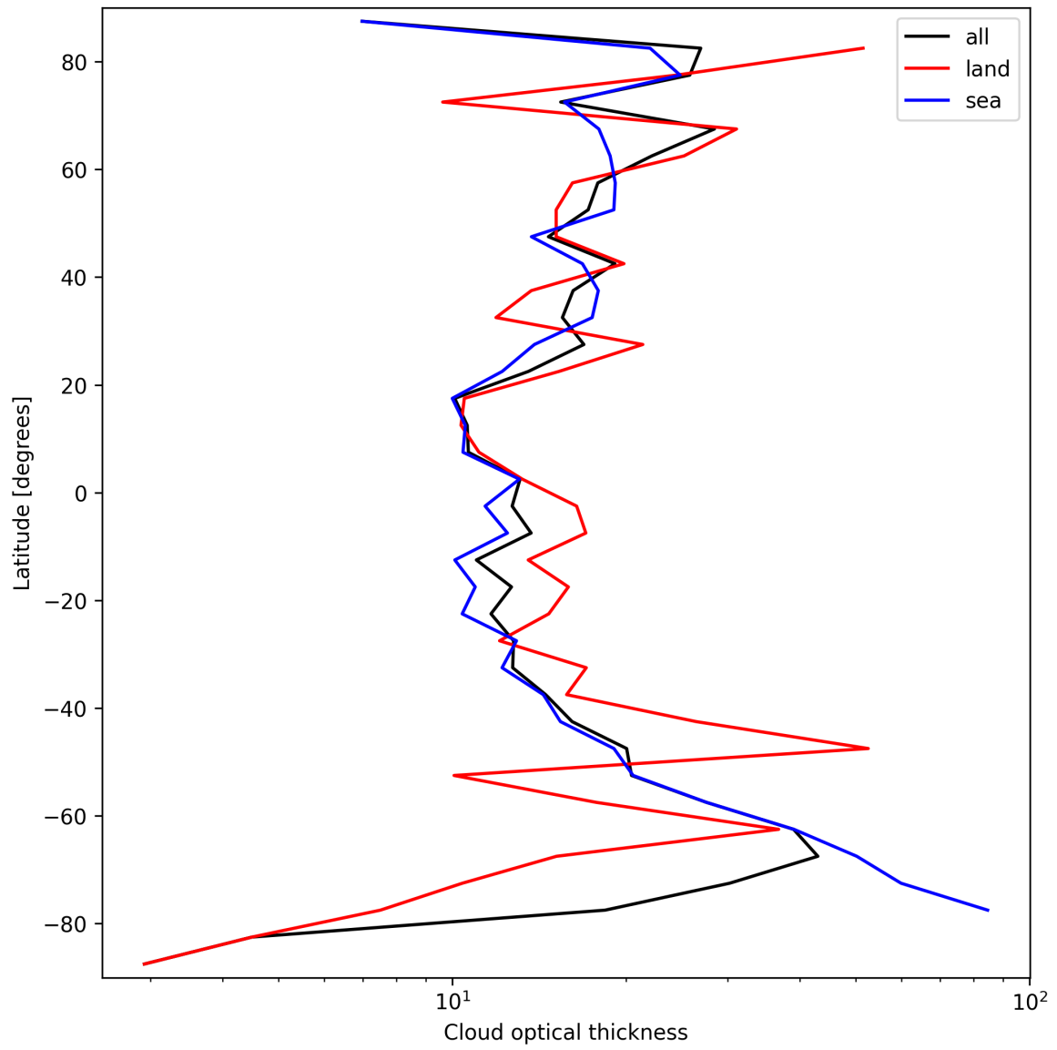
Figure 23: Zonal average of “Cloud optical thickness” for 2025-03-29 to 2025-03-30.
