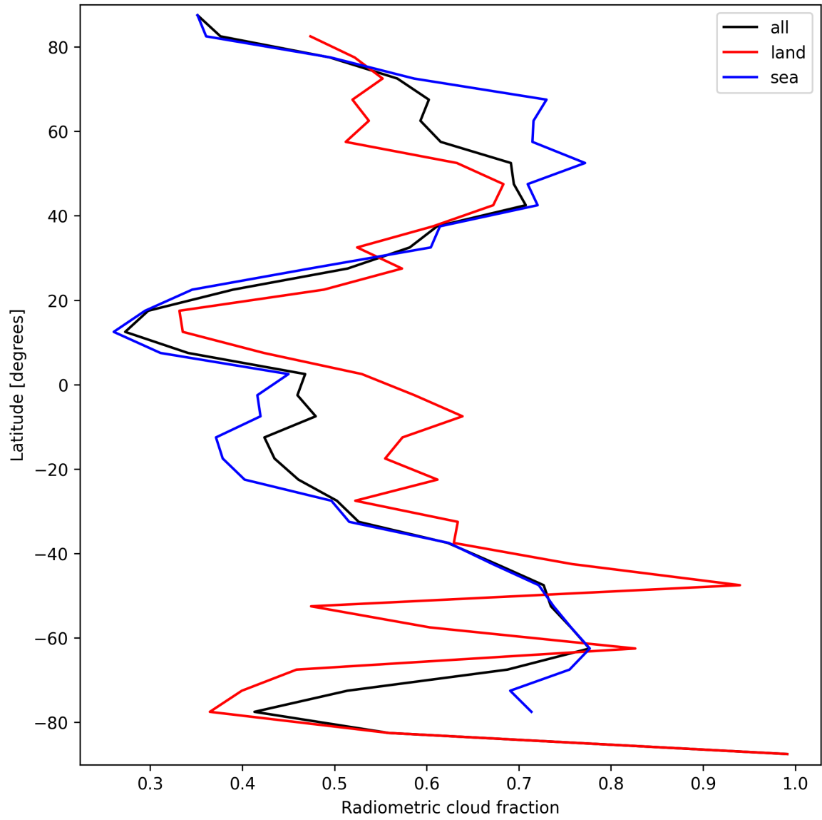
Figure 21: Zonal average of “Radiometric cloud fraction” for 2025-03-29 to 2025-03-30.
