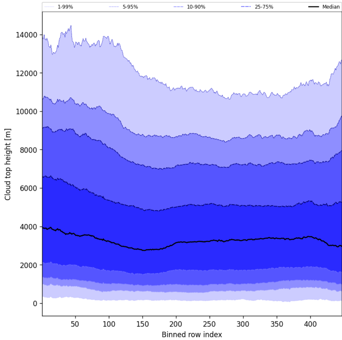
Figure 54: Along track statistics of “Cloud top height” for 2025-03-29 to 2025-03-30
