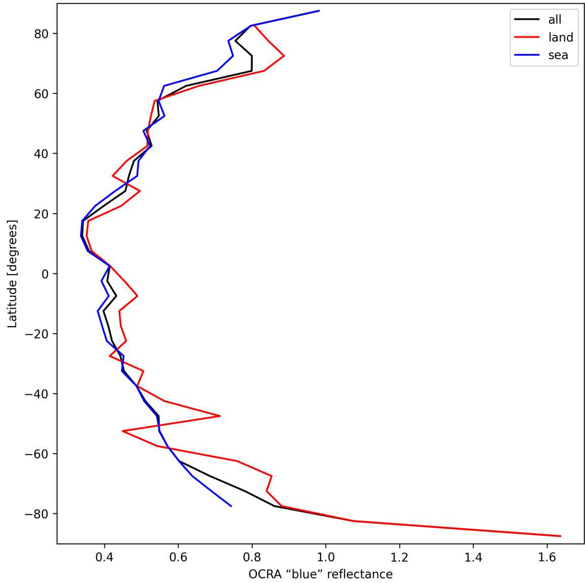
Figure 33: Zonal average of “OCRA “blue” reflectance” for 2025-03-29 to 2025-03-30.
