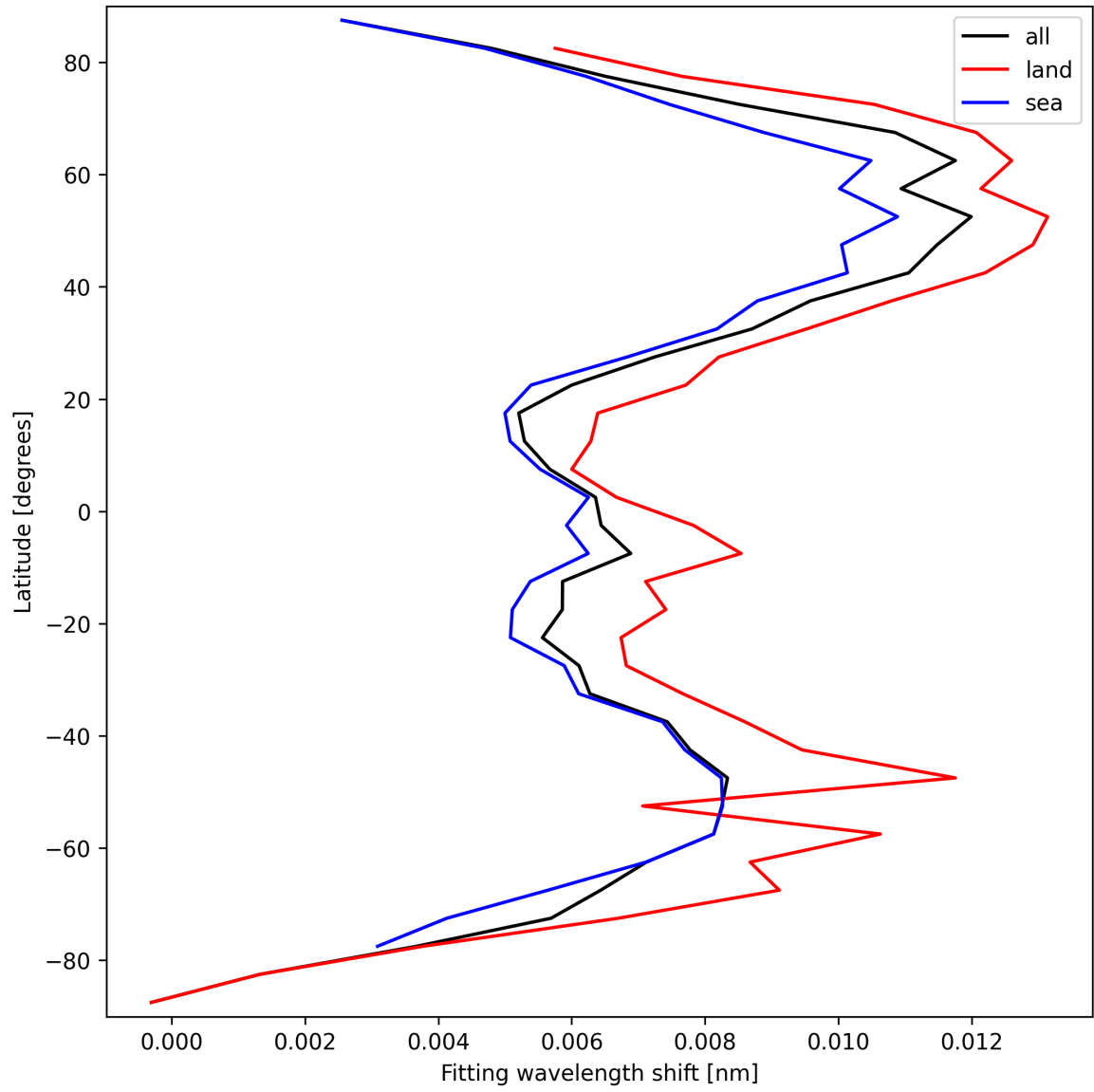
Figure 31: Zonal average of “Fitting wavelength shift” for 2025-03-29 to 2025-03-30.
