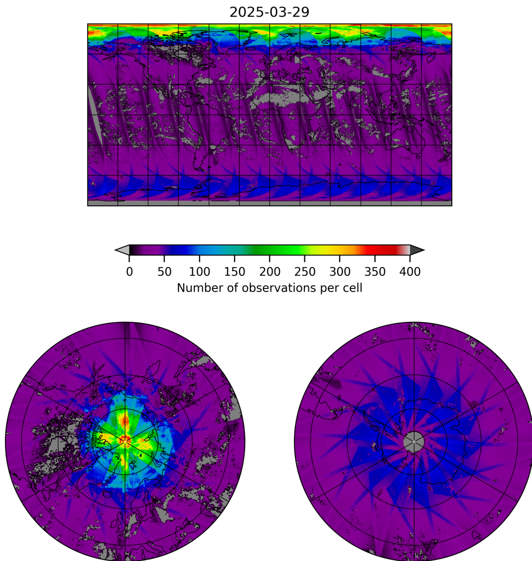
Figure 19: Map of the number of observations for 2025-03-29 to 2025-03-30
