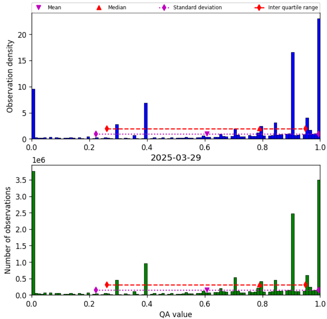
Figure 36: Histogram of “QA value” for 2025-03-29 to 2025-03-30
