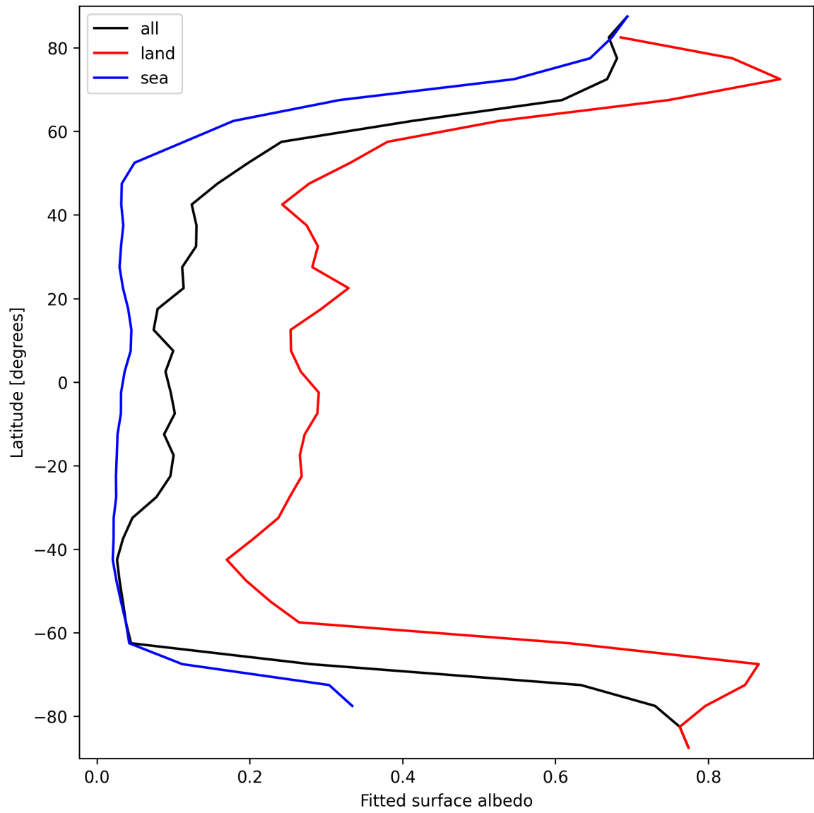
Figure 27: Zonal average of “Fitted surface albedo” for 2025-03-29 to 2025-03-30.
