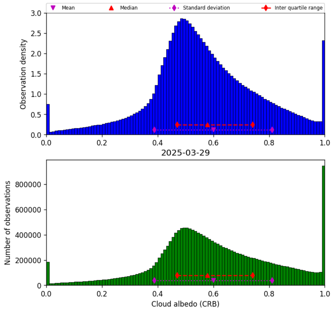
Figure 42: Histogram of “Cloud albedo (CRB)” for 2025-03-29 to 2025-03-30
