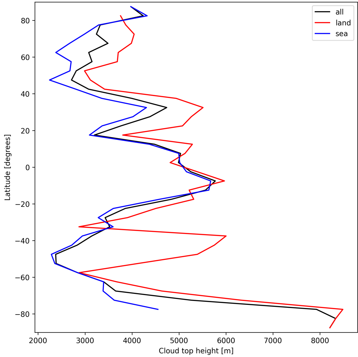
Figure 22: Zonal average of “Cloud top height” for 2025-03-29 to 2025-03-30.
