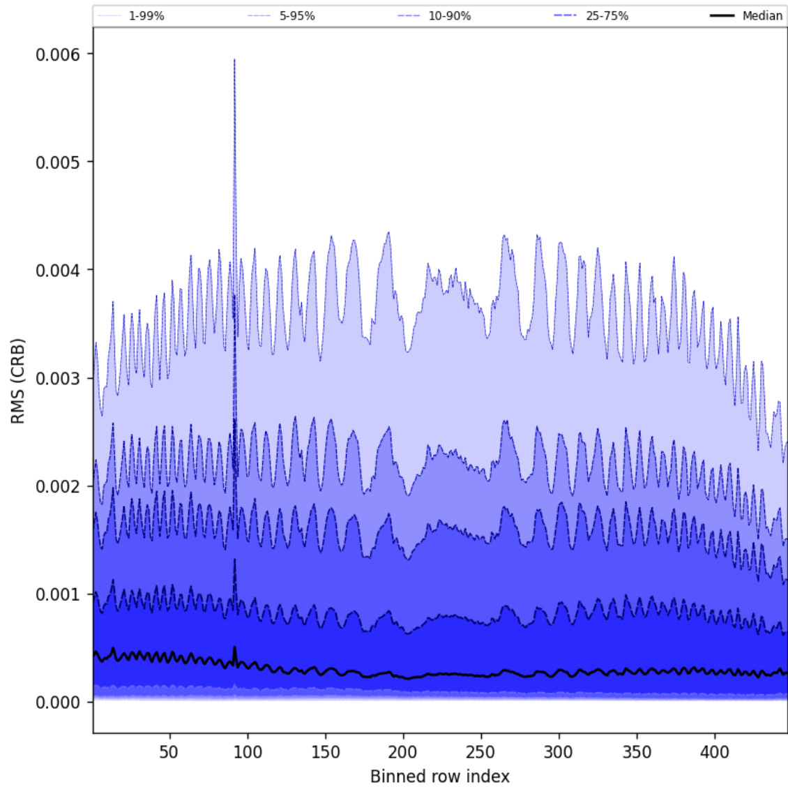
Figure 62: Along track statistics of “RMS (CRB)” for 2025-03-29 to 2025-03-30
