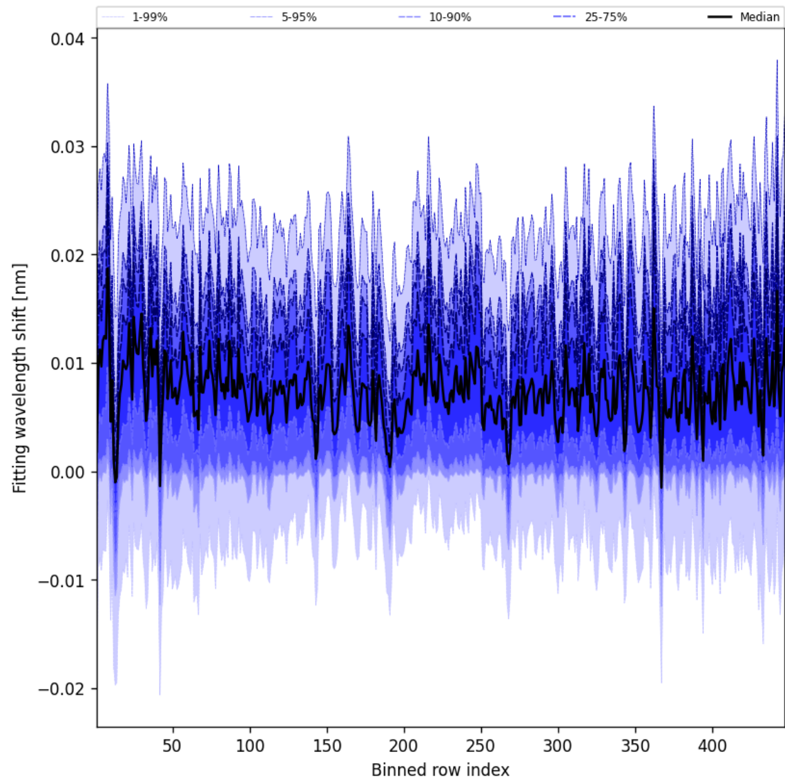
Figure 63: Along track statistics of “Fitting wavelength shift” for 2025-03-29 to 2025-03-30
