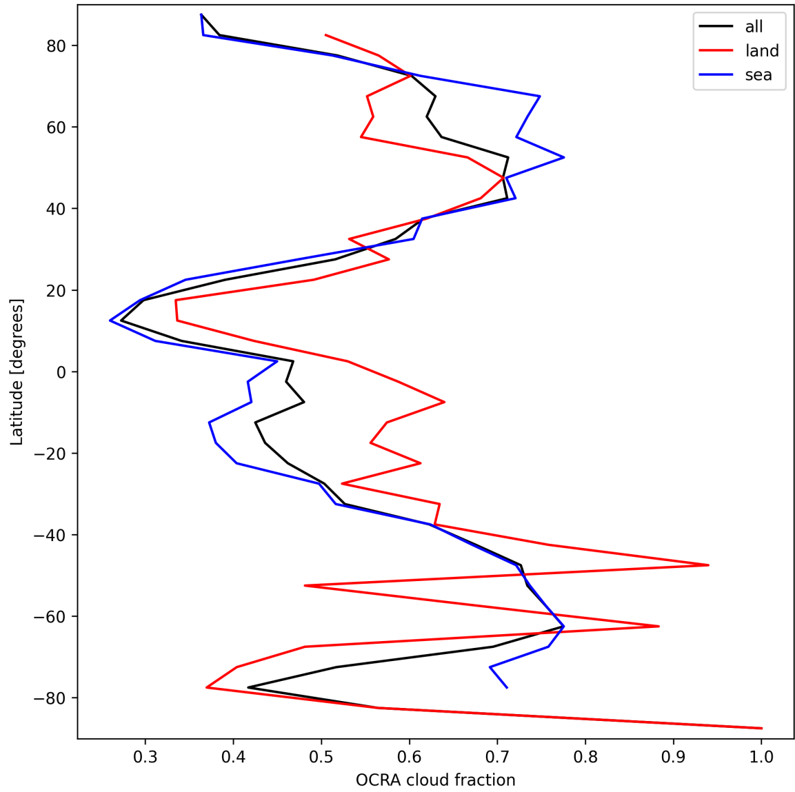
Figure 32: Zonal average of “OCRA cloud fraction” for 2025-03-29 to 2025-03-30.
