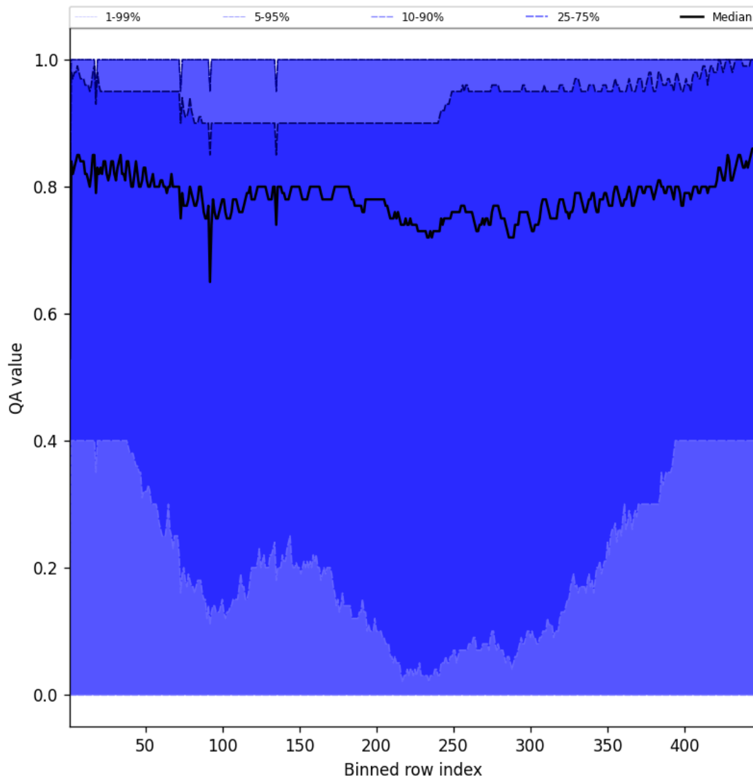
Figure 52: Along track statistics of “QA value” for 2025-03-29 to 2025-03-30
