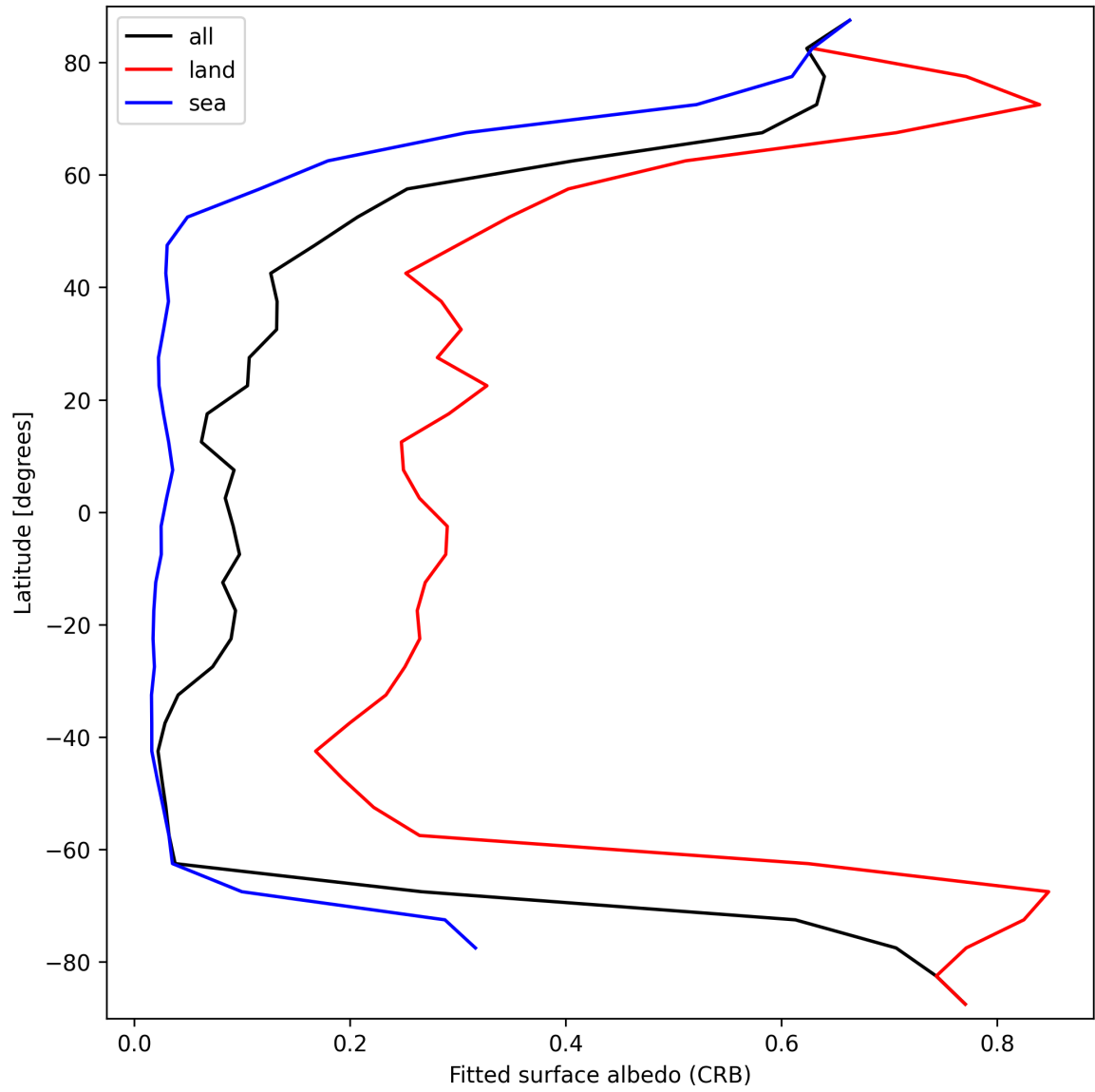
Figure 28: Zonal average of “Fitted surface albedo (CRB)” for 2025-03-29 to 2025-03-30.
