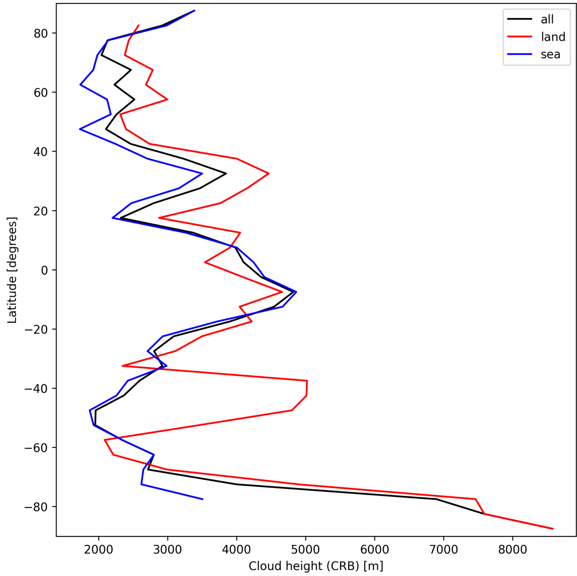
Figure 25: Zonal average of “Cloud height (CRB)” for 2025-03-29 to 2025-03-30.
