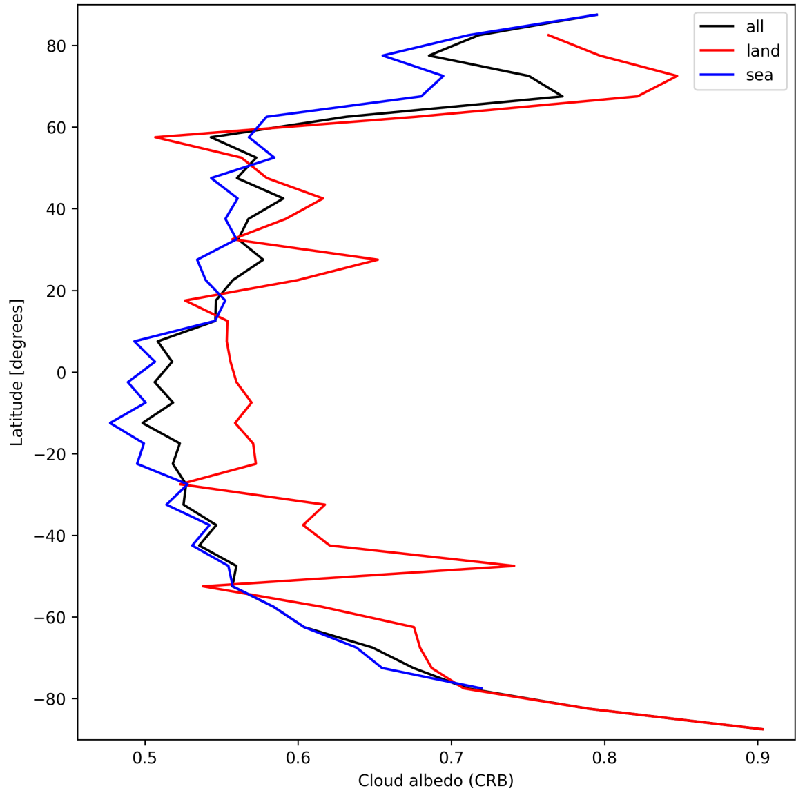
Figure 26: Zonal average of “Cloud albedo (CRB)” for 2025-03-29 to 2025-03-30.
