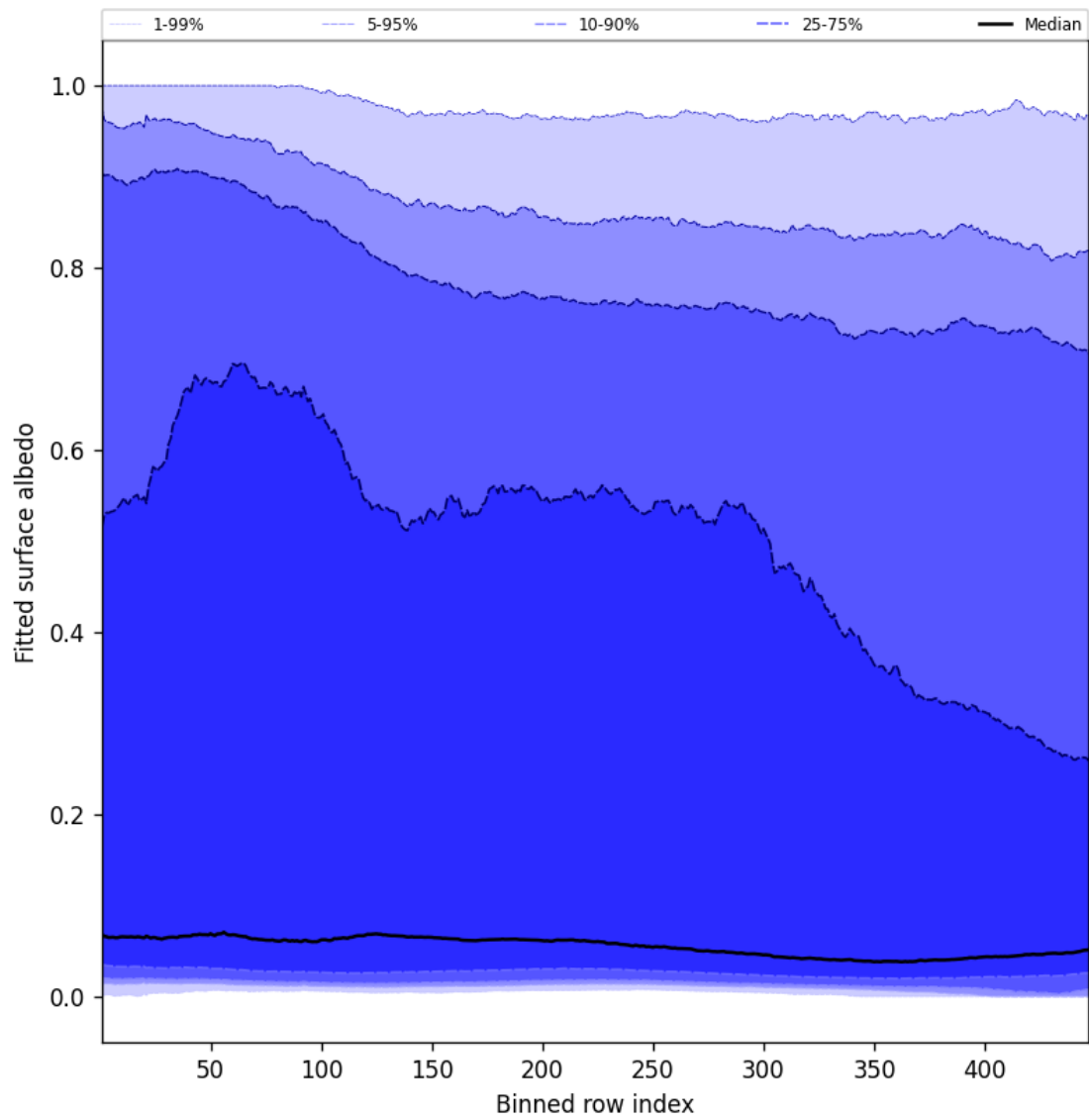
Figure 59: Along track statistics of “Fitted surface albedo” for 2025-03-29 to 2025-03-30
