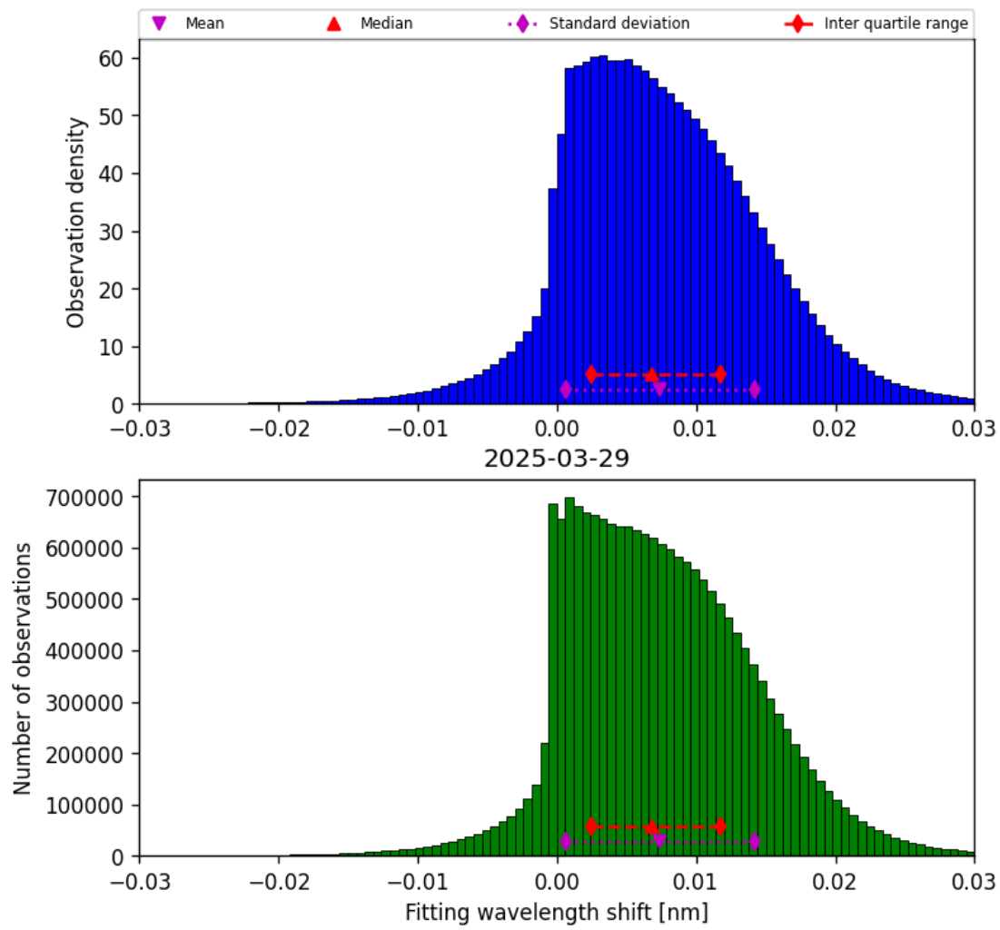
Figure 47: Histogram of “Fitting wavelength shift” for 2025-03-29 to 2025-03-30
