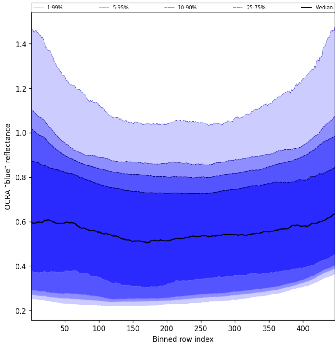
Figure 65: Along track statistics of “OCRA “blue” reflectance” for 2025-03-29 to 2025-03-30
