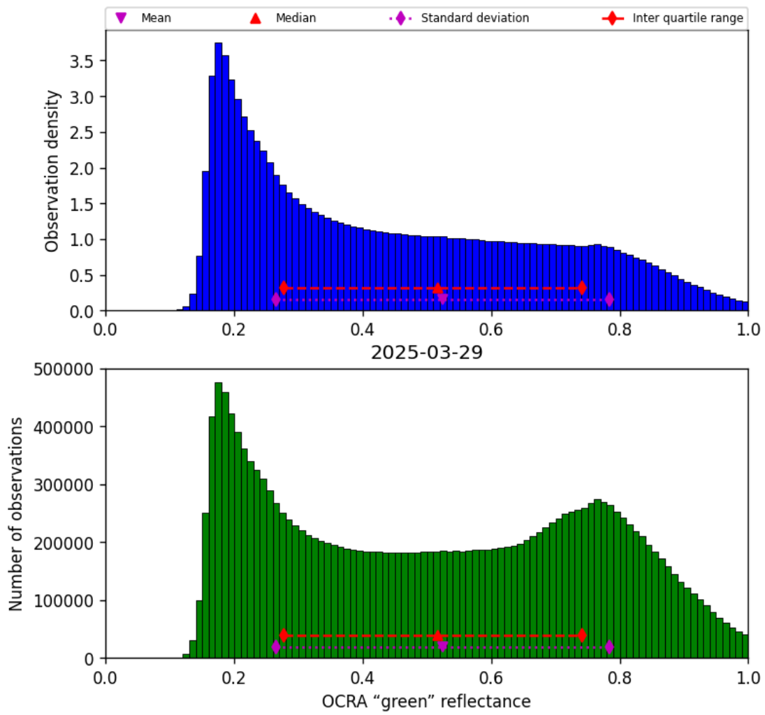
Figure 50: Histogram of “OCRA “green” reflectance” for 2025-03-29 to 2025-03-30
