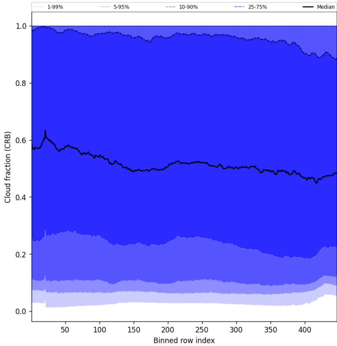
Figure 56: Along track statistics of “Cloud fraction (CRB)” for 2025-03-29 to 2025-03-30
