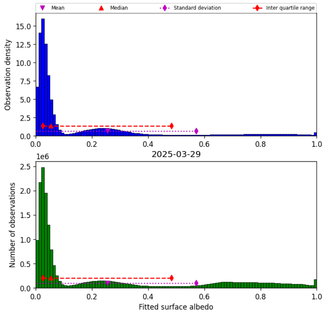
Figure 43: Histogram of “Fitted surface albedo” for 2025-03-29 to 2025-03-30
