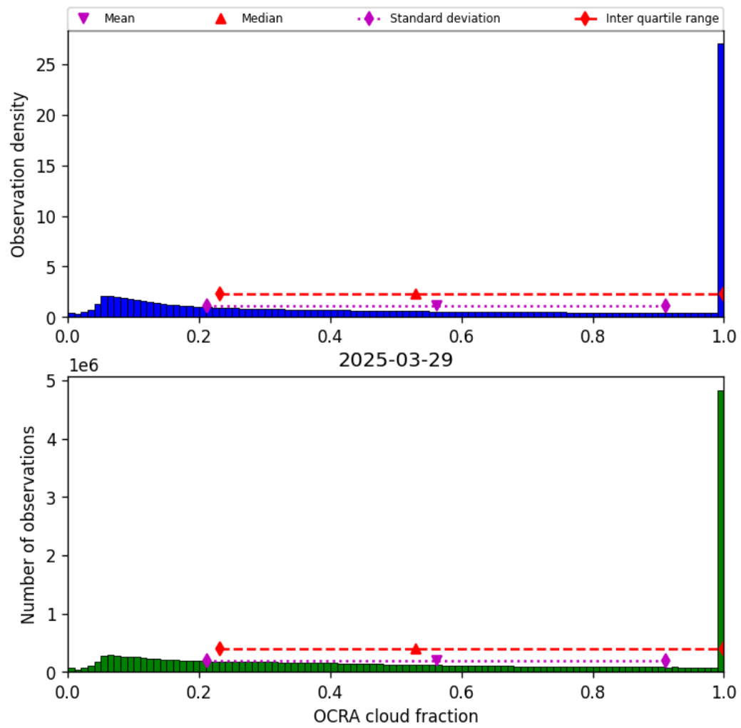
Figure 48: Histogram of “OCRA cloud fraction” for 2025-03-29 to 2025-03-30
