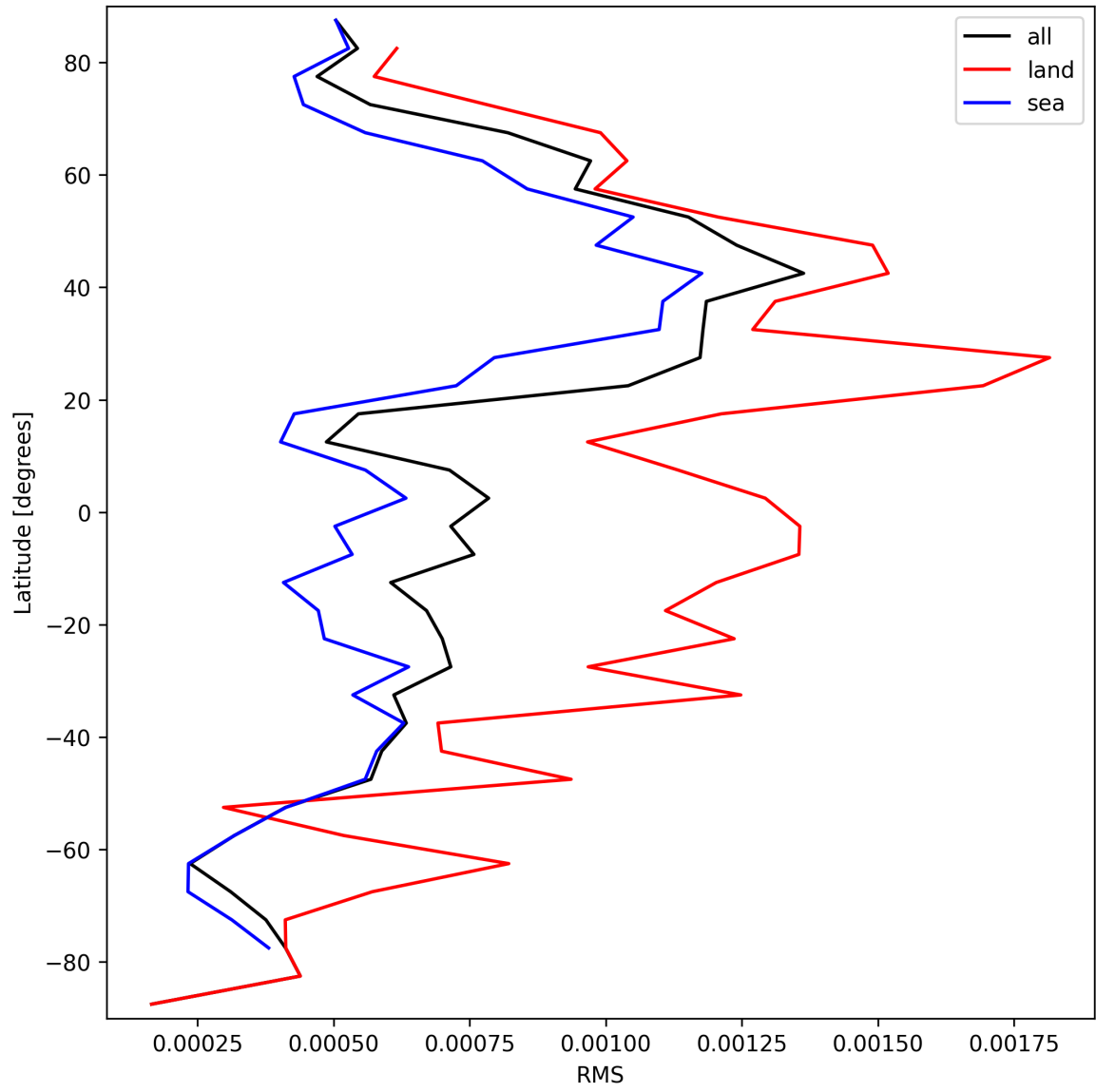
Figure 29: Zonal average of “RMS” for 2025-03-29 to 2025-03-30.
