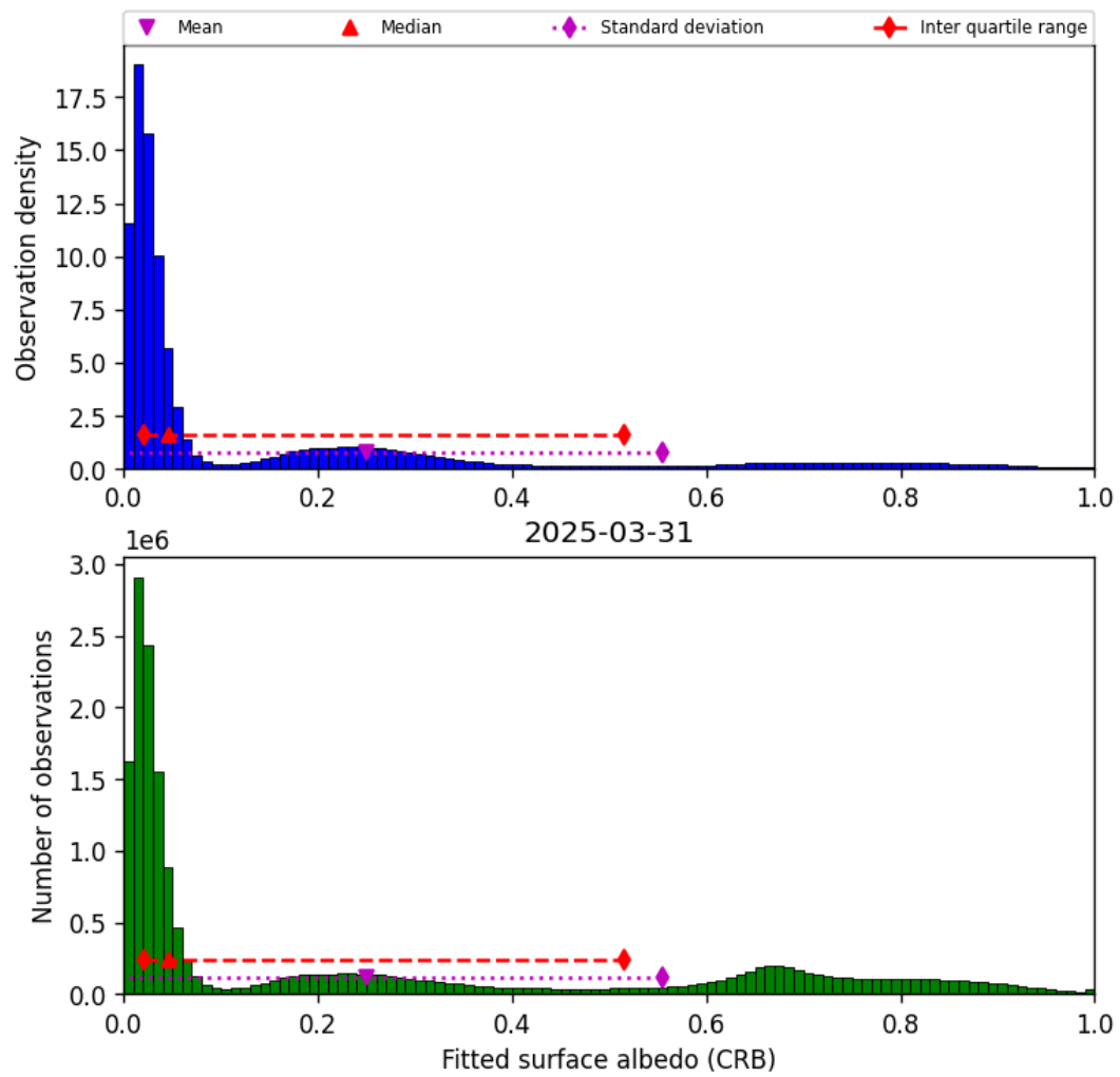
Figure 44: Histogram of “Fitted surface albedo (CRB)” for 2025-03-31 to 2025-03-31
