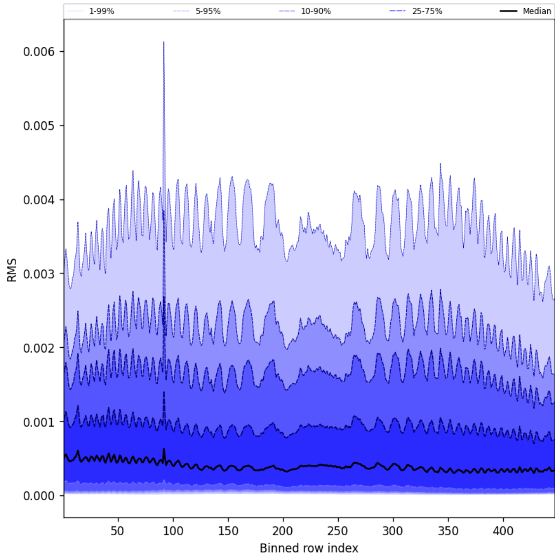
Figure 61: Along track statistics of “RMS” for 2025-03-31 to 2025-03-31
