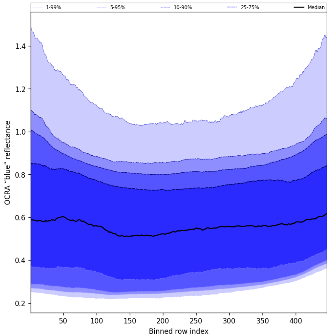
Figure 65: Along track statistics of “OCRA “blue” reflectance” for 2025-03-31 to 2025-03-31
