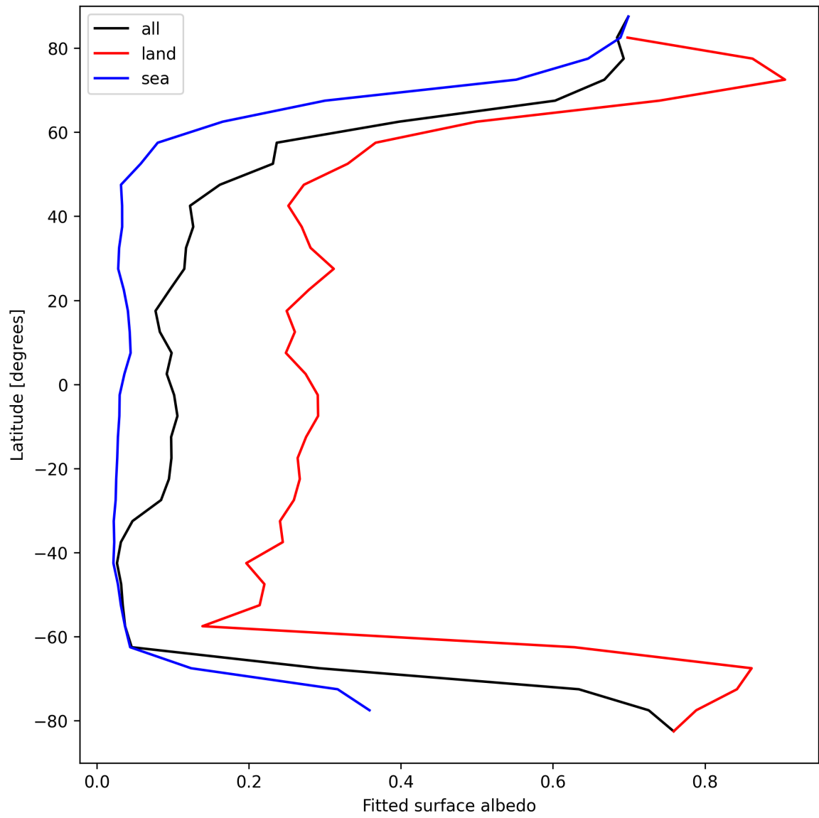
Figure 27: Zonal average of “Fitted surface albedo” for 2025-03-31 to 2025-03-31.
