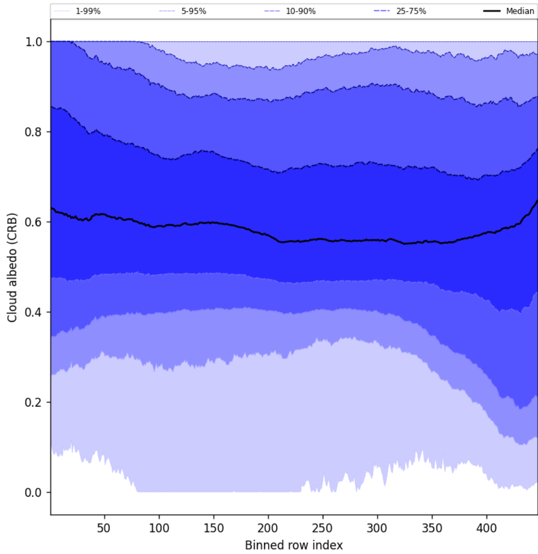
Figure 58: Along track statistics of “Cloud albedo (CRB)” for 2025-03-31 to 2025-03-31
