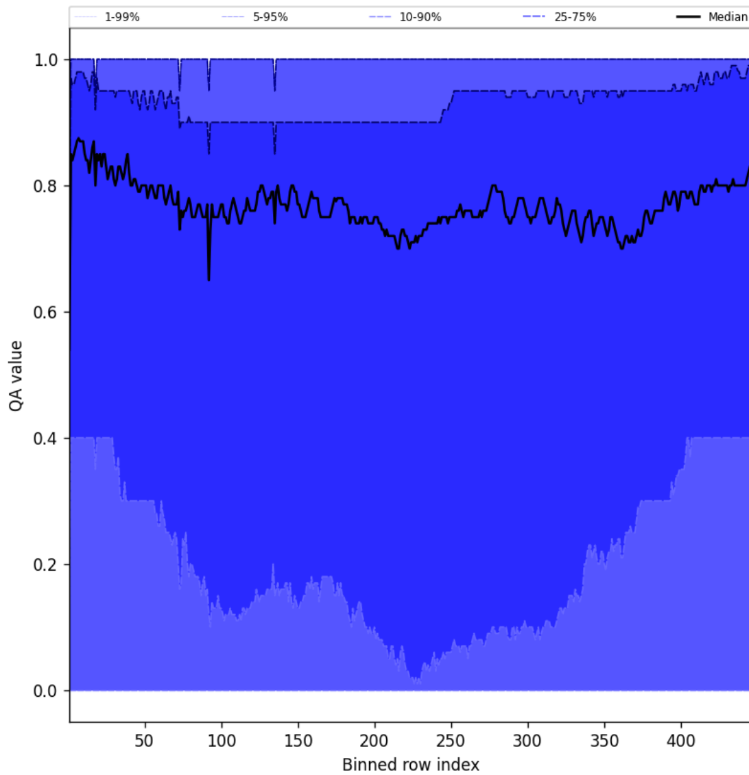
Figure 52: Along track statistics of “QA value” for 2025-03-31 to 2025-03-31
