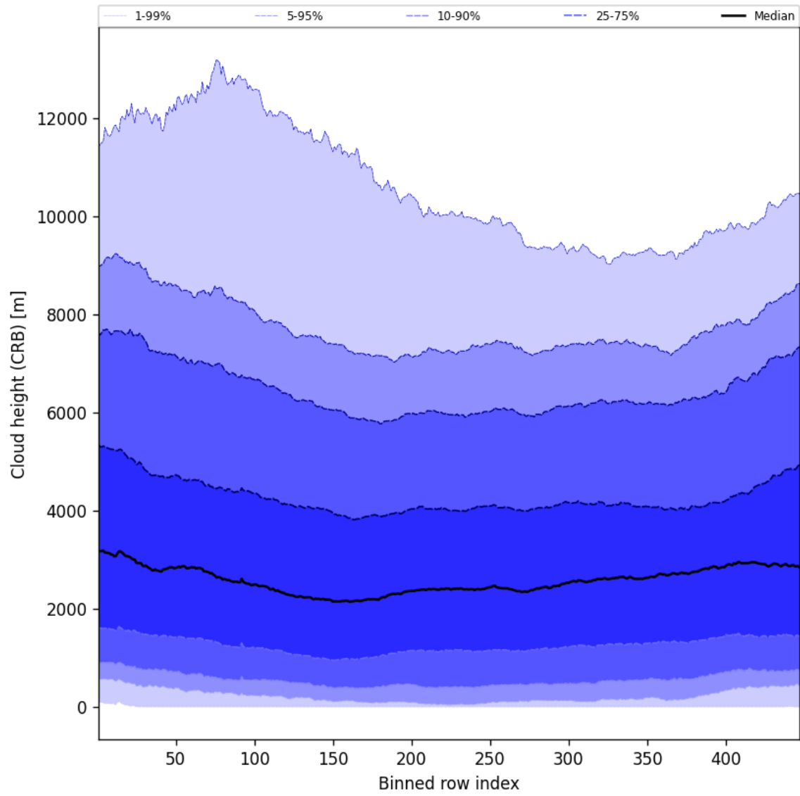
Figure 57: Along track statistics of “Cloud height (CRB)” for 2025-03-31 to 2025-03-31
