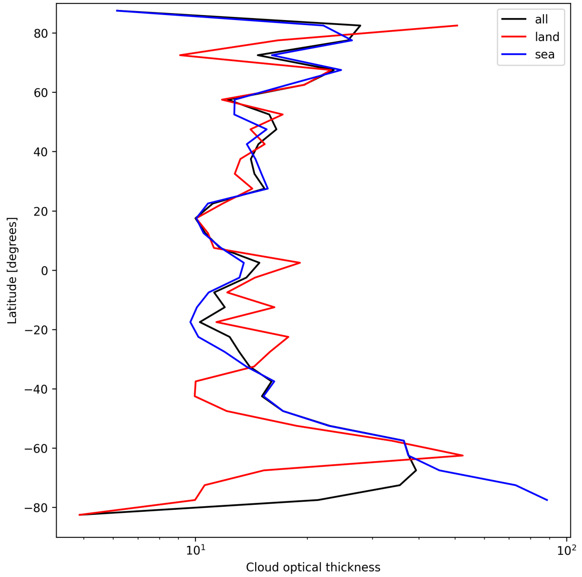
Figure 23: Zonal average of “Cloud optical thickness” for 2025-03-31 to 2025-03-31.
