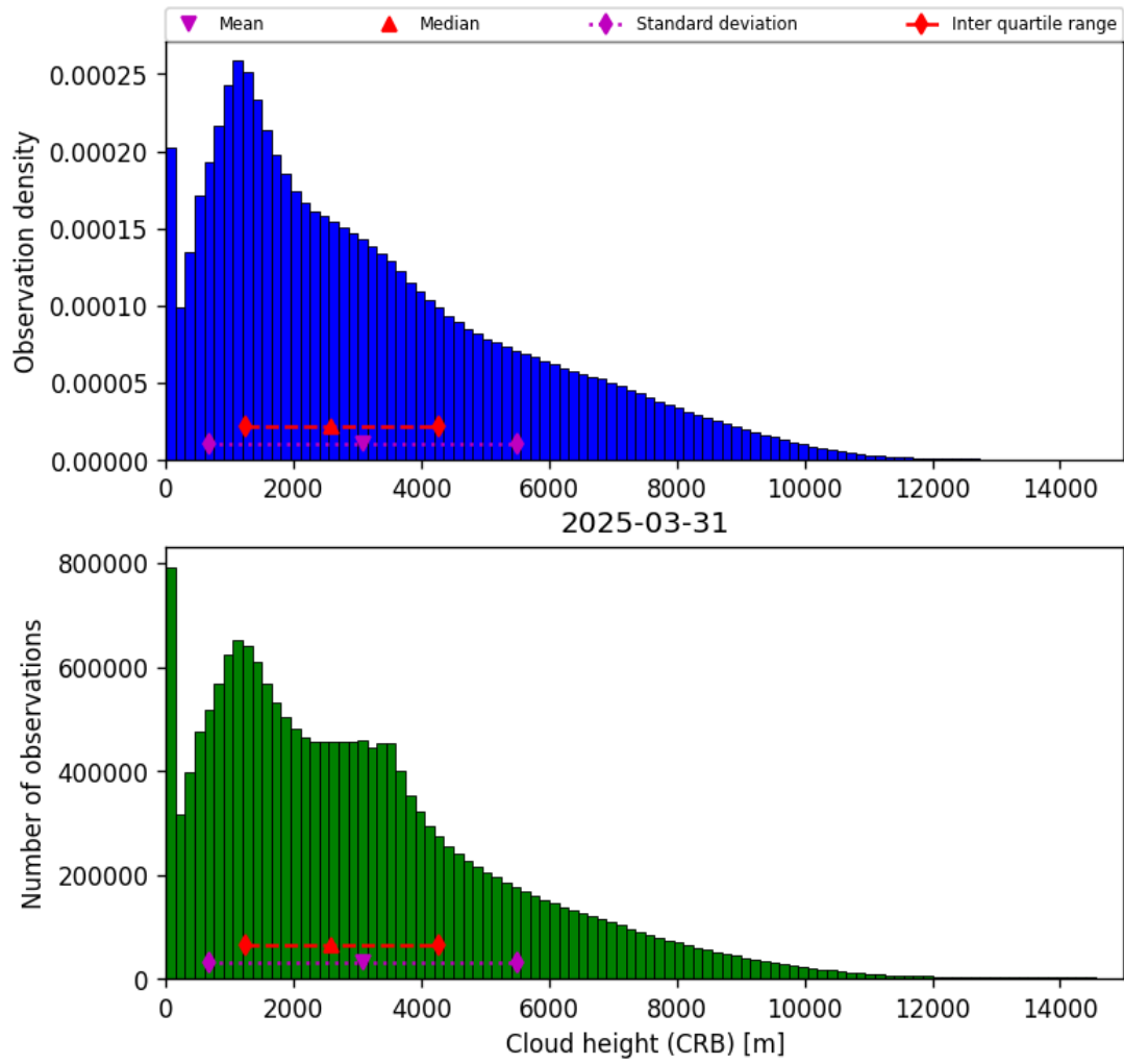
Figure 41: Histogram of “Cloud height (CRB)” for 2025-03-31 to 2025-03-31
