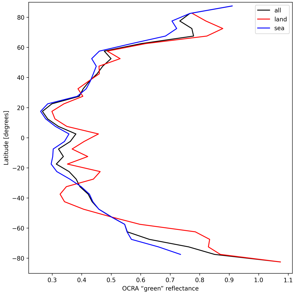
Figure 34: Zonal average of “OCRA “green” reflectance” for 2025-03-31 to 2025-03-31.
