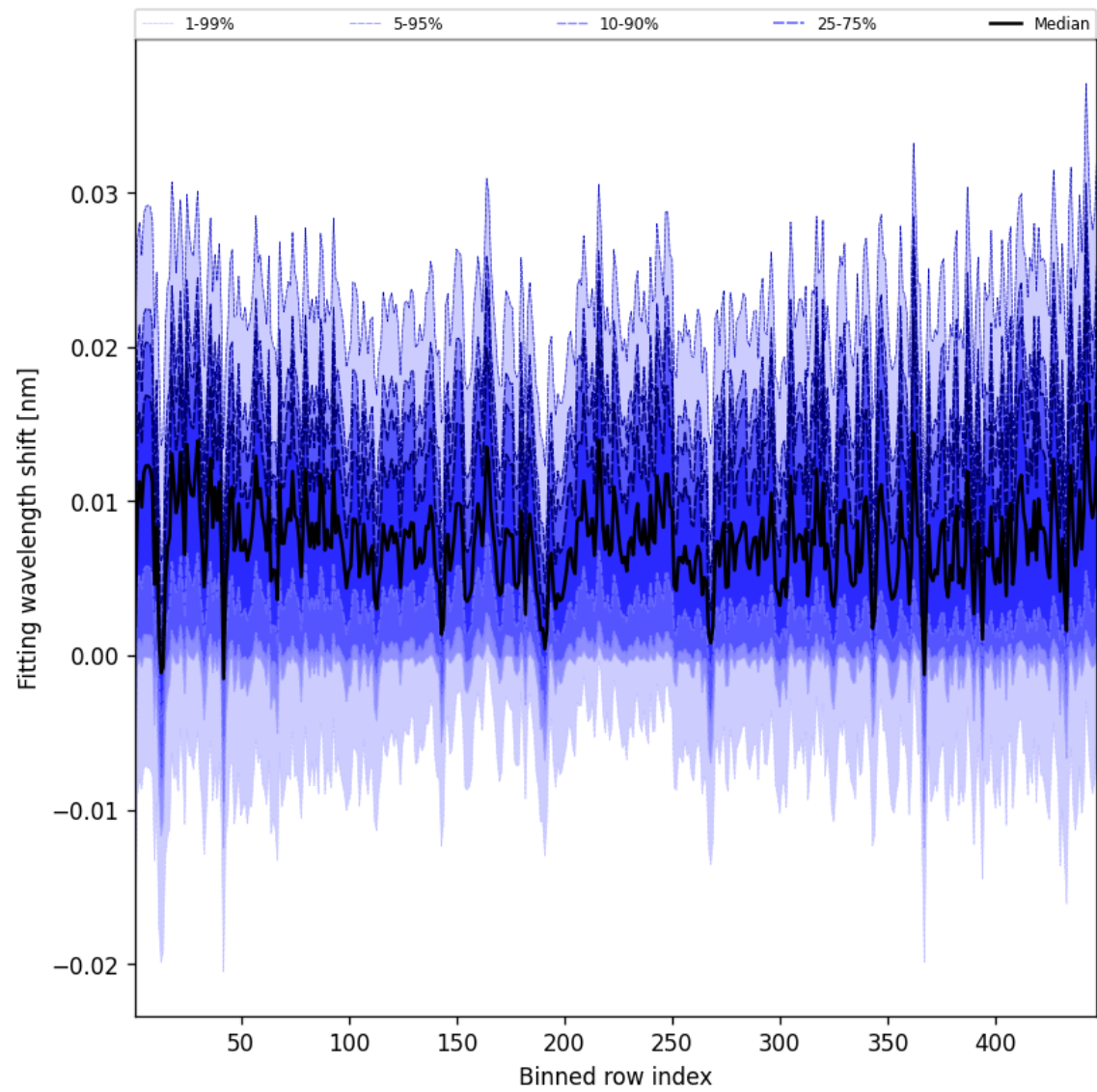
Figure 63: Along track statistics of “Fitting wavelength shift” for 2025-03-31 to 2025-03-31
