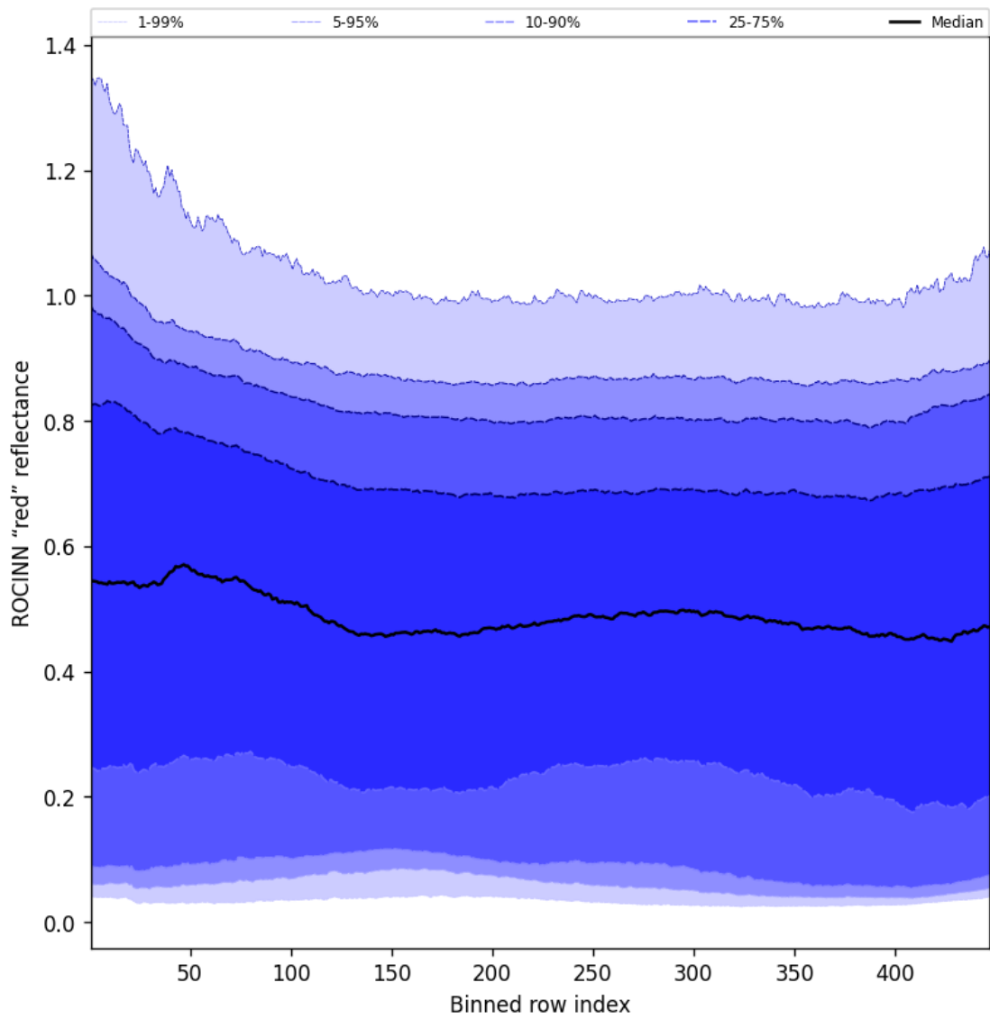
Figure 67: Along track statistics of "ROCINN "red" reflectance" for 2025-03-31 to 2025-03-31
