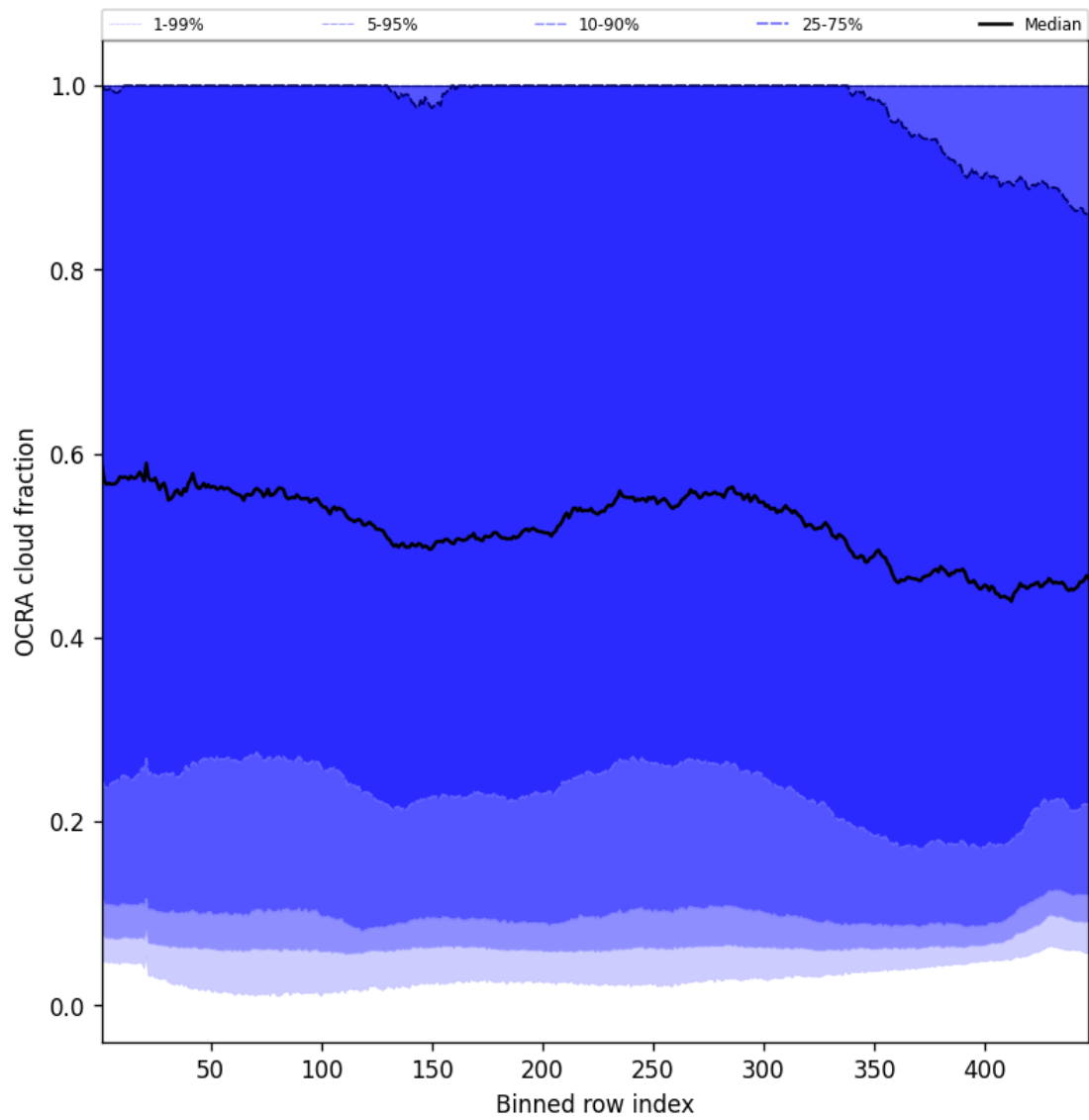
Figure 64: Along track statistics of “OCRA cloud fraction” for 2025-03-31 to 2025-03-31
