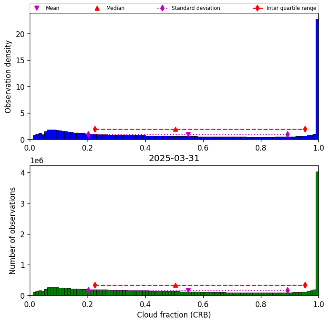
Figure 40: Histogram of “Cloud fraction (CRB)” for 2025-03-31 to 2025-03-31
