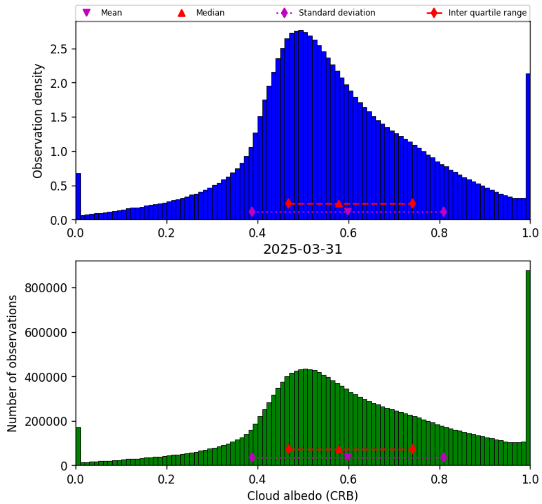
Figure 42: Histogram of “Cloud albedo (CRB)” for 2025-03-31 to 2025-03-31
