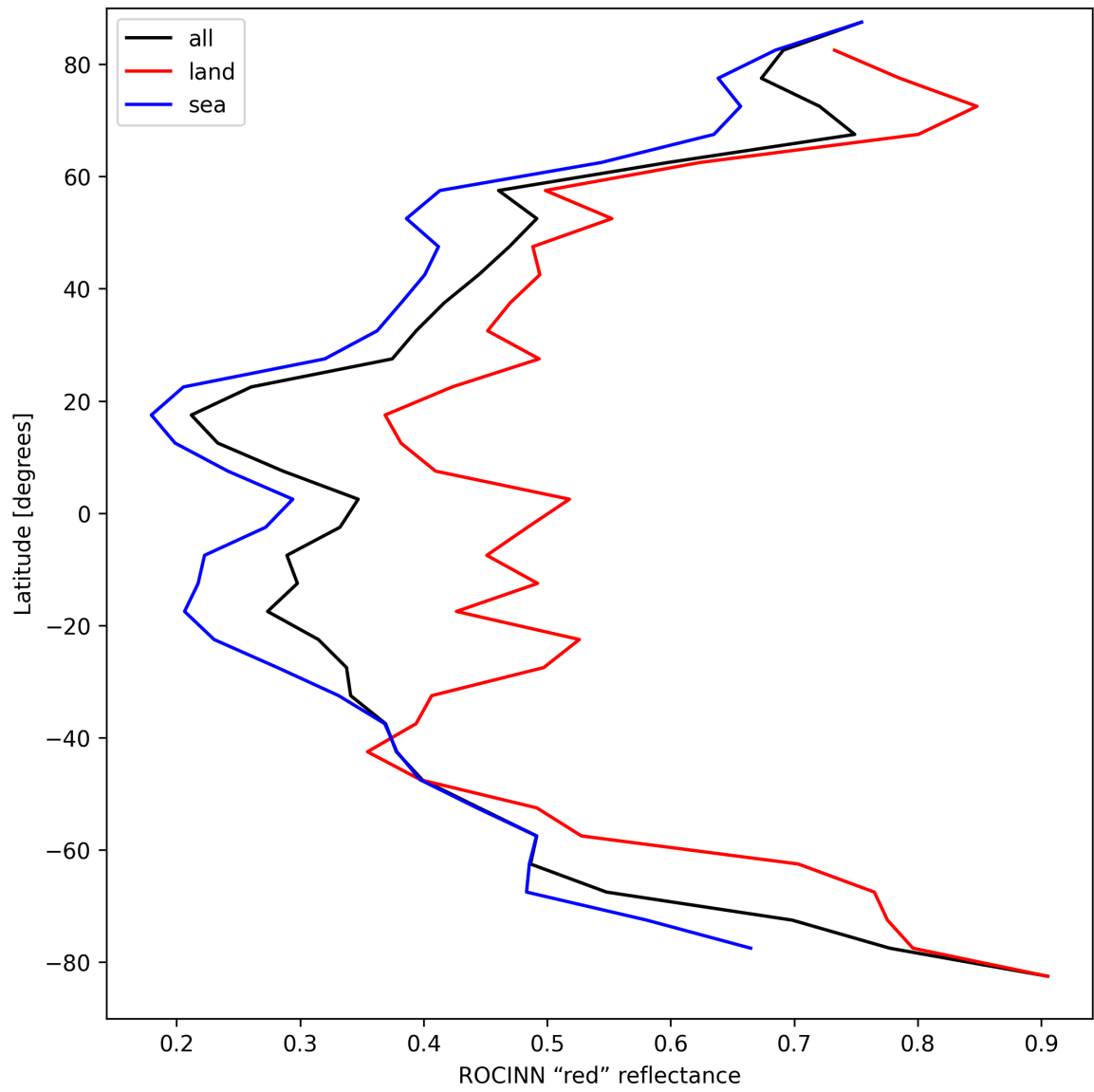
Figure 35: Zonal average of “ROCINN “red” reflectance” for 2025-03-31 to 2025-03-31.
