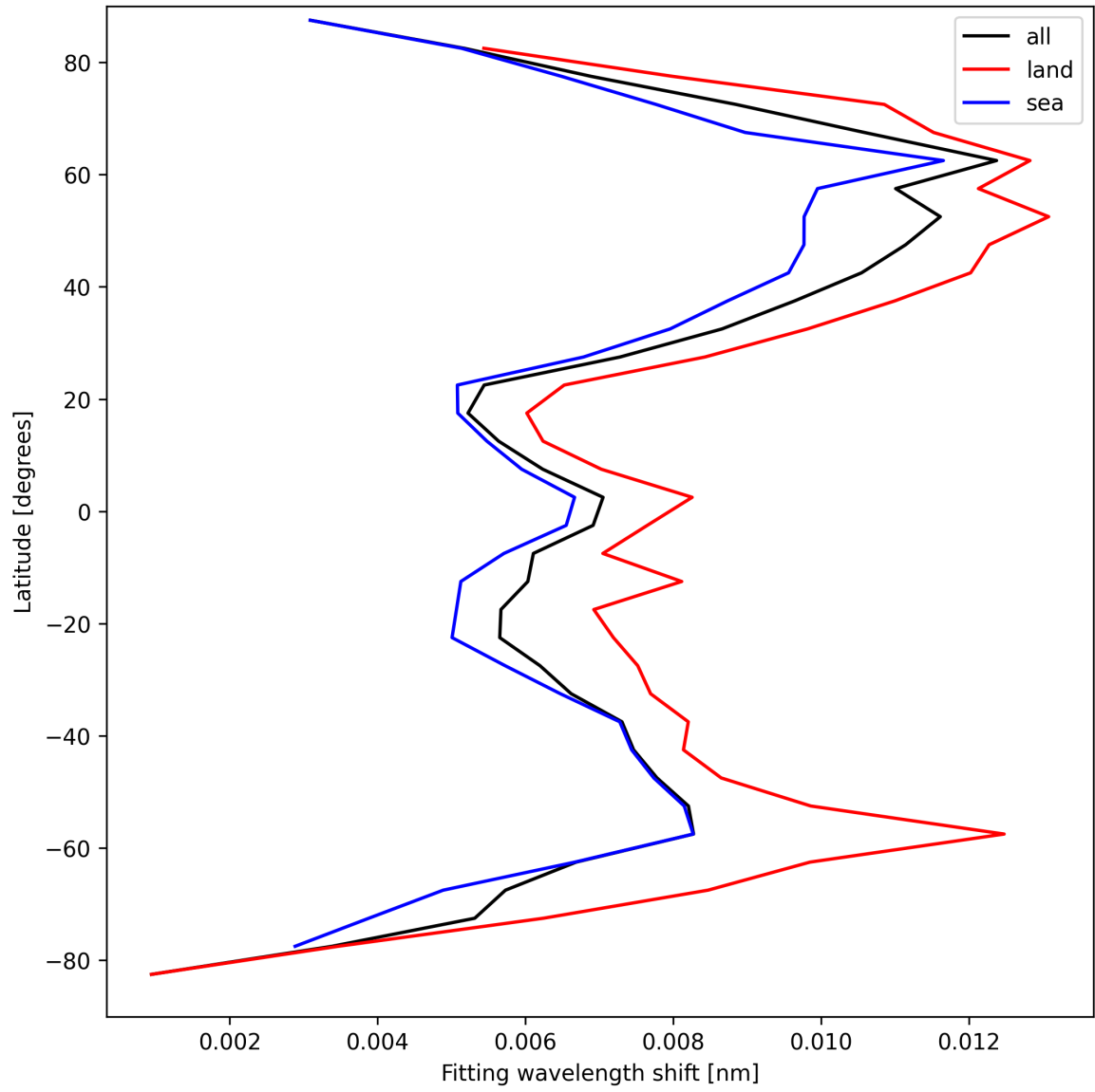
Figure 31: Zonal average of “Fitting wavelength shift” for 2025-03-31 to 2025-03-31.
