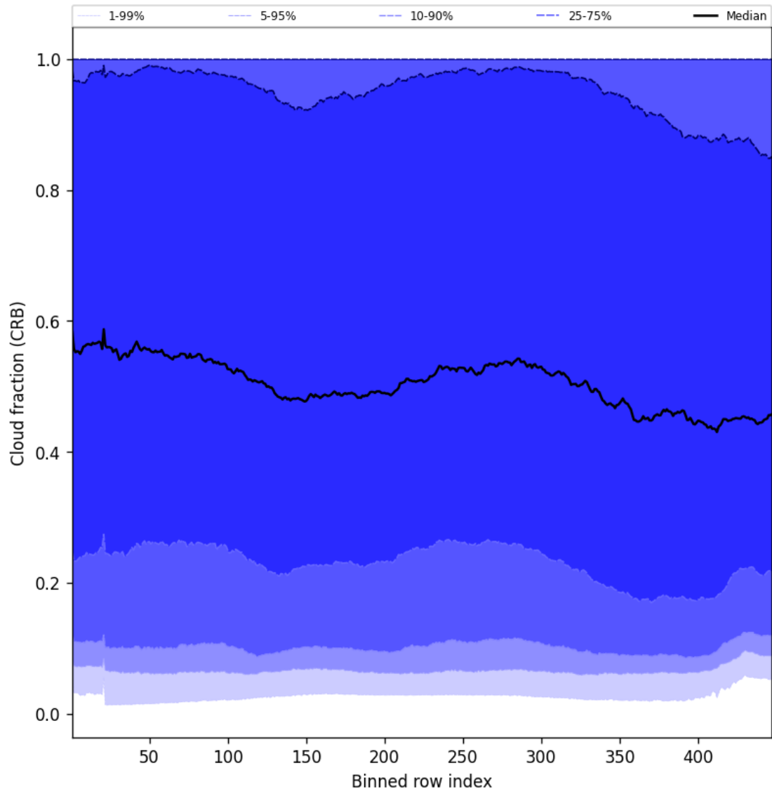
Figure 56: Along track statistics of “Cloud fraction (CRB)” for 2025-03-31 to 2025-03-31
