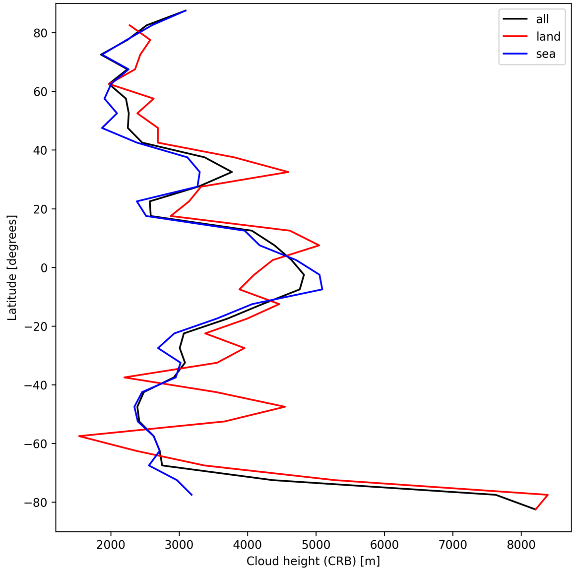
Figure 25: Zonal average of “Cloud height (CRB)” for 2025-03-31 to 2025-03-31.
