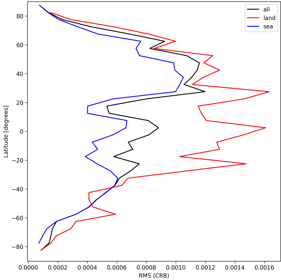
Figure 30: Zonal average of “RMS (CRB)” for 2025-03-31 to 2025-03-31.
