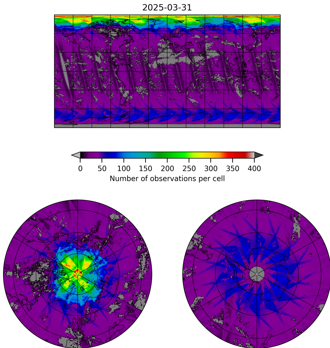
Figure 19: Map of the number of observations for 2025-03-31 to 2025-03-31
