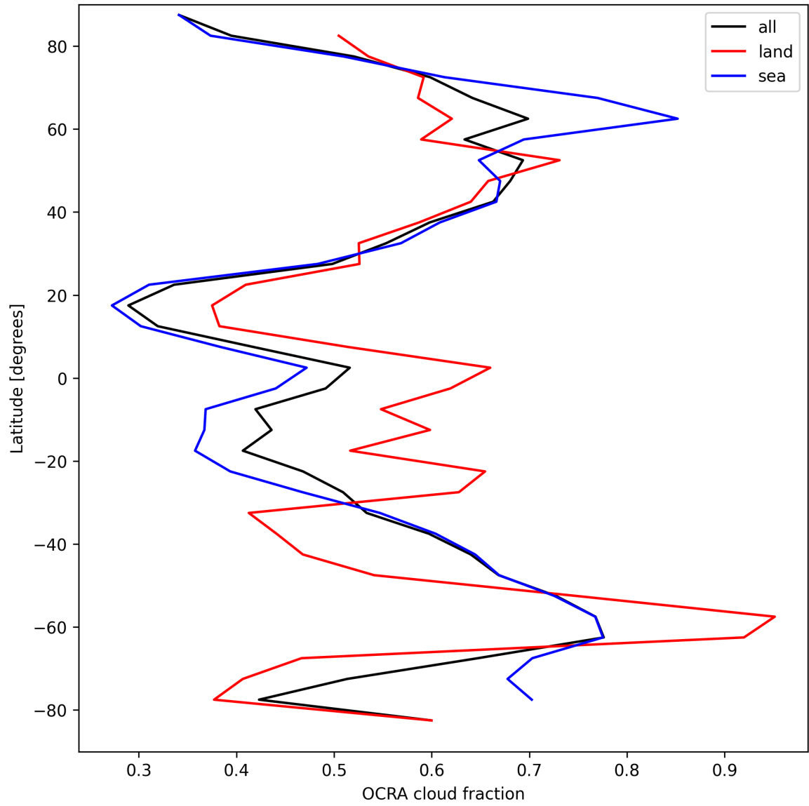
Figure 32: Zonal average of “OCRA cloud fraction” for 2025-03-31 to 2025-03-31.
