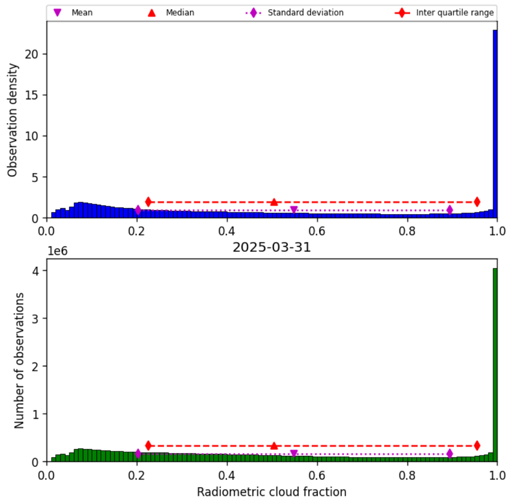
Figure 37: Histogram of “Radiometric cloud fraction” for 2025-03-31 to 2025-03-31
