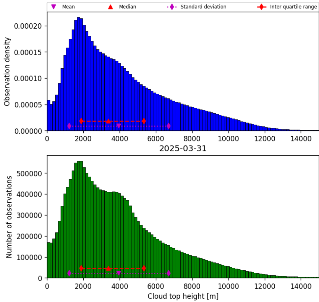
Figure 38: Histogram of “Cloud top height” for 2025-03-31 to 2025-03-31
