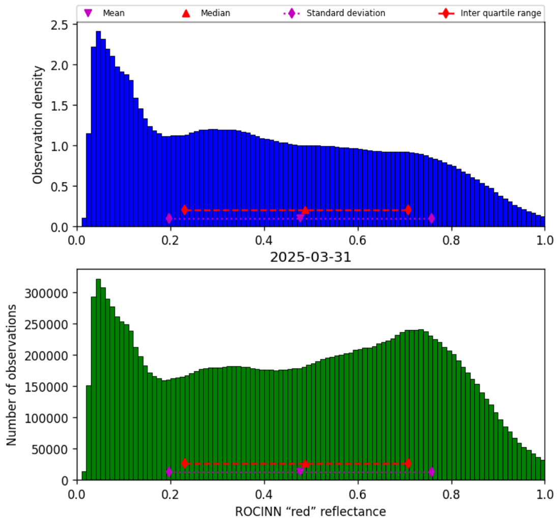
Figure 51: Histogram of “ROCINN “red” reflectance” for 2025-03-31 to 2025-03-31
