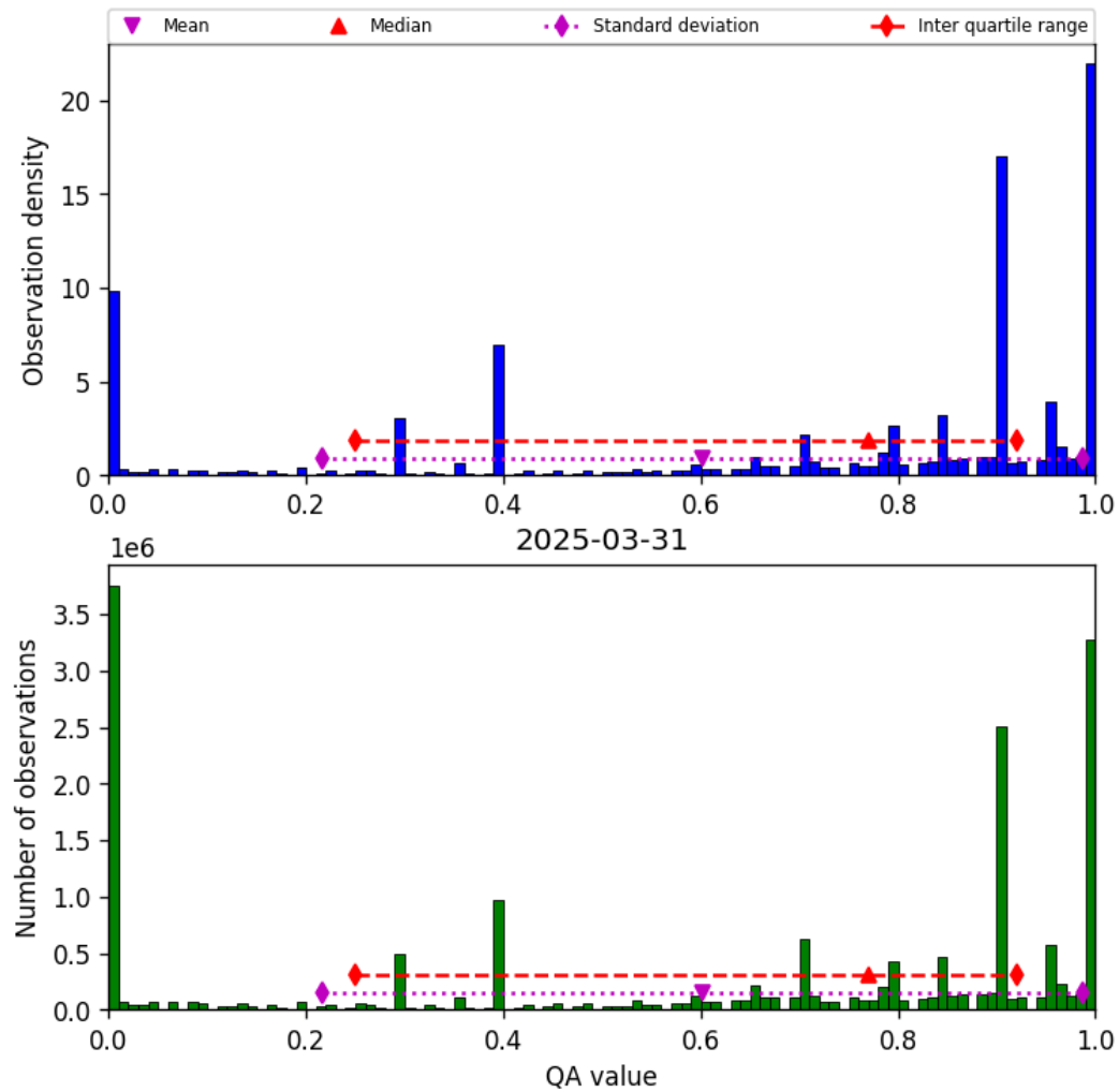
Figure 36: Histogram of “QA value” for 2025-03-31 to 2025-03-31
