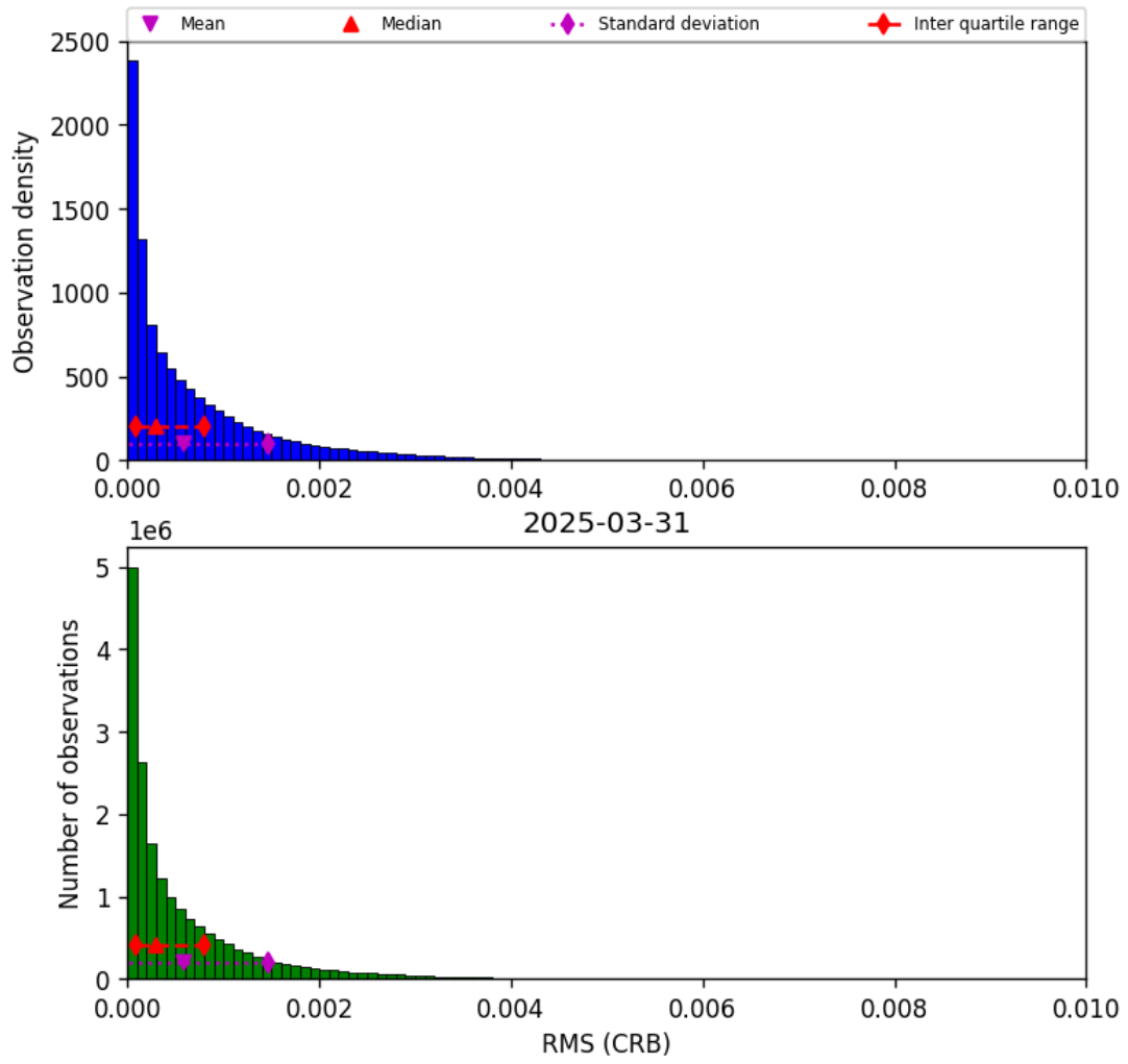
Figure 46: Histogram of “RMS (CRB)” for 2025-03-31 to 2025-03-31
