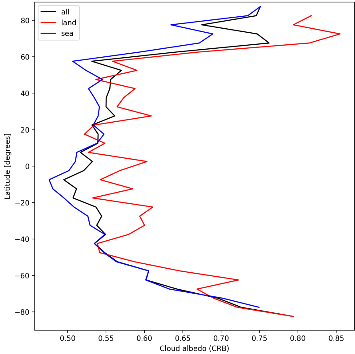
Figure 26: Zonal average of “Cloud albedo (CRB)” for 2025-03-31 to 2025-03-31.
