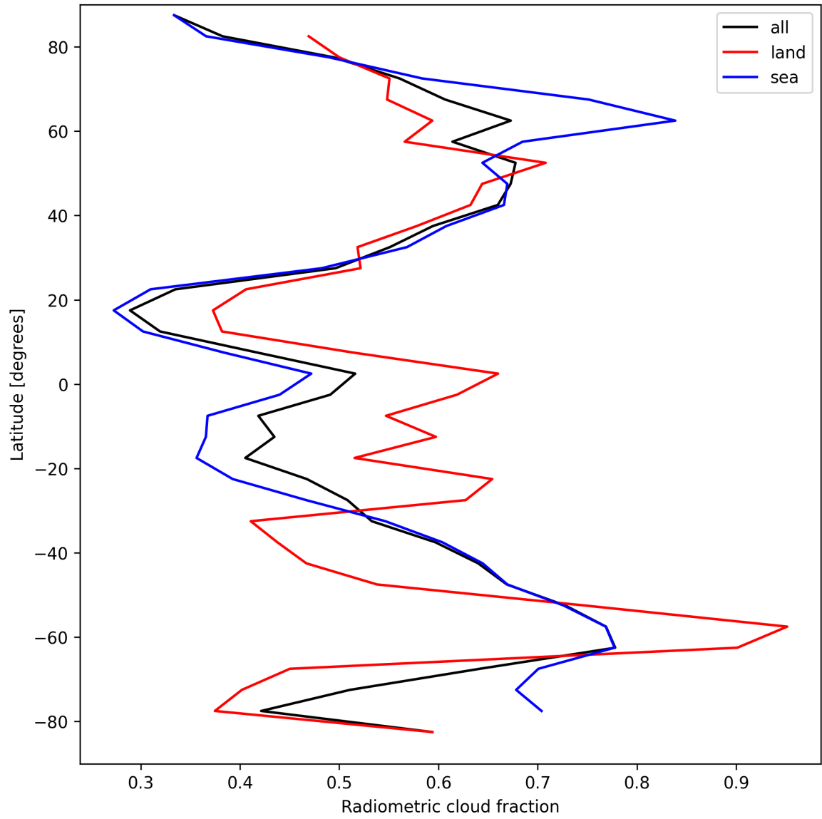
Figure 21: Zonal average of “Radiometric cloud fraction” for 2025-03-31 to 2025-03-31.
