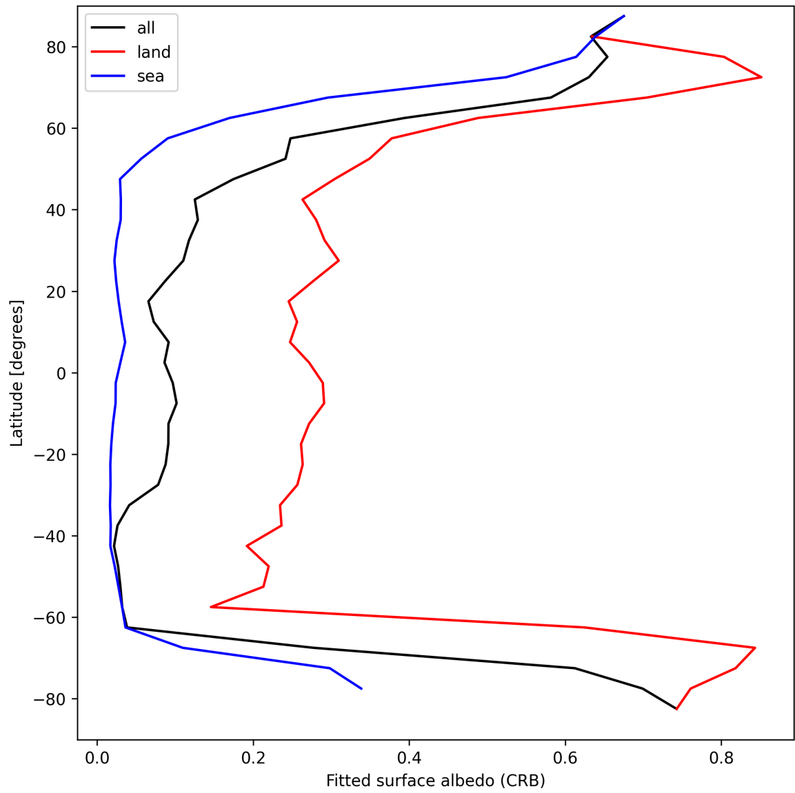
Figure 28: Zonal average of “Fitted surface albedo (CRB)” for 2025-03-31 to 2025-03-31.
