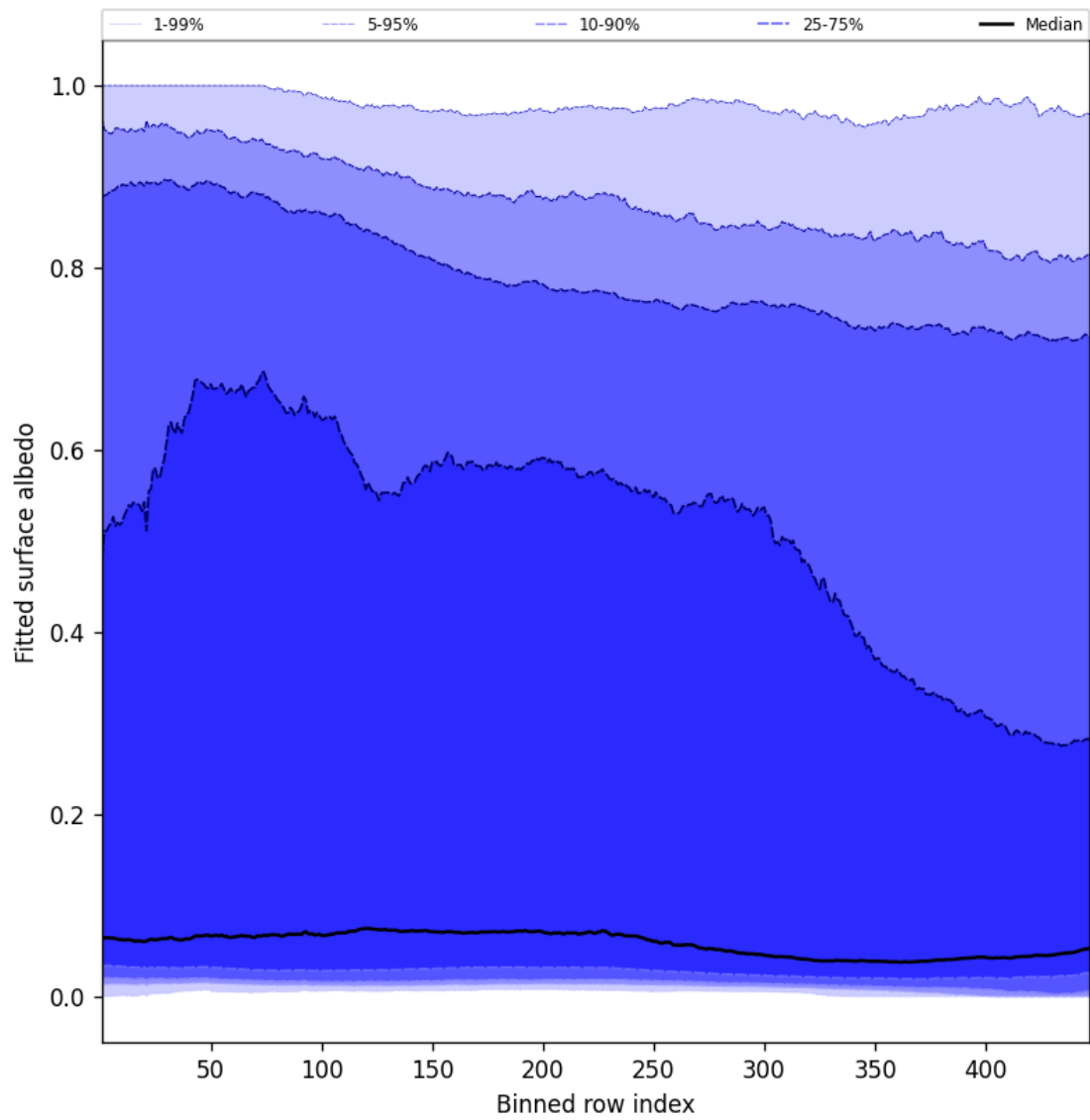
Figure 59: Along track statistics of “Fitted surface albedo” for 2025-03-31 to 2025-03-31
