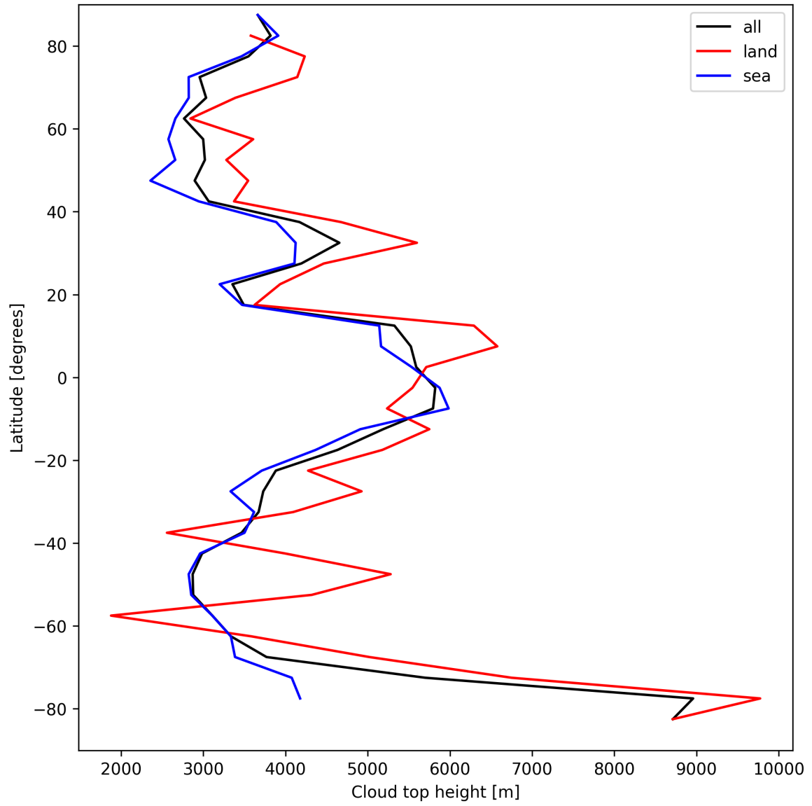
Figure 22: Zonal average of “Cloud top height” for 2025-03-31 to 2025-03-31.
