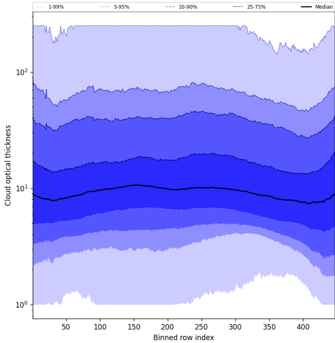
Figure 55: Along track statistics of “Cloud optical thickness” for 2025-03-31 to 2025-03-31
