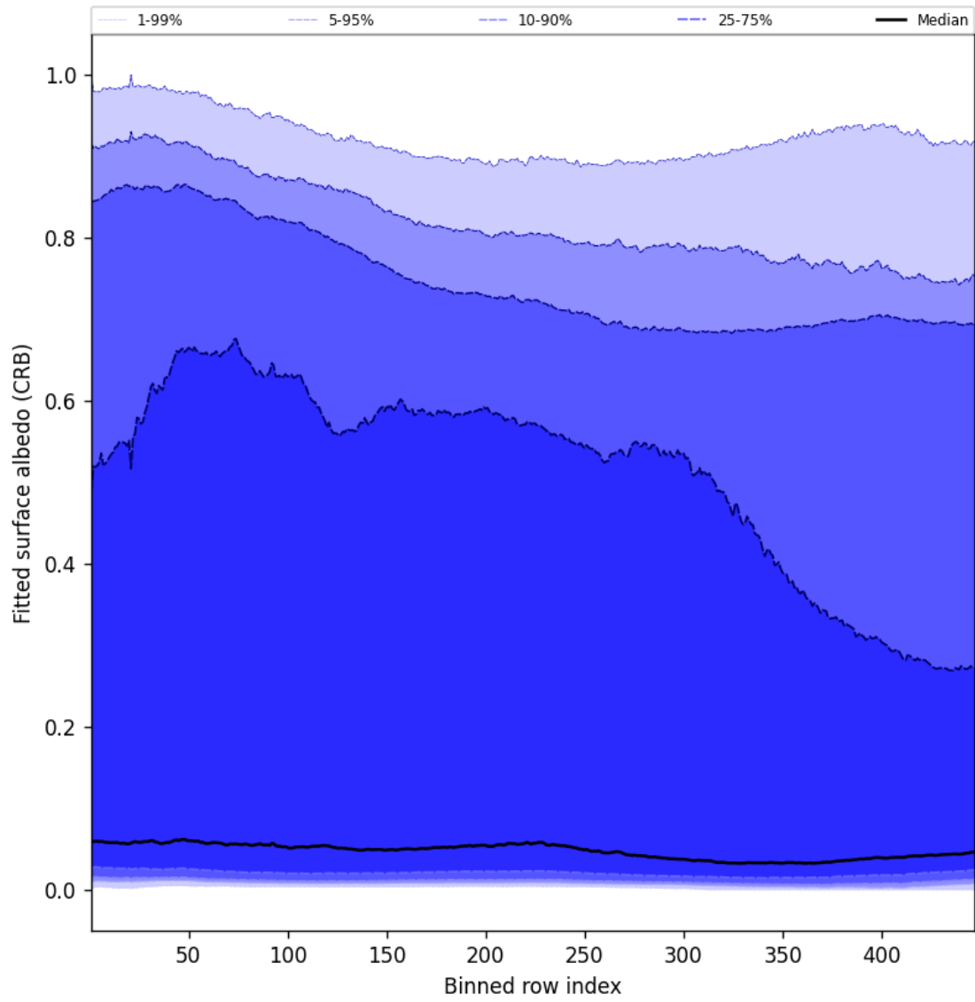
Figure 60: Along track statistics of “Fitted surface albedo (CRB)” for 2025-03-31 to 2025-03-31
