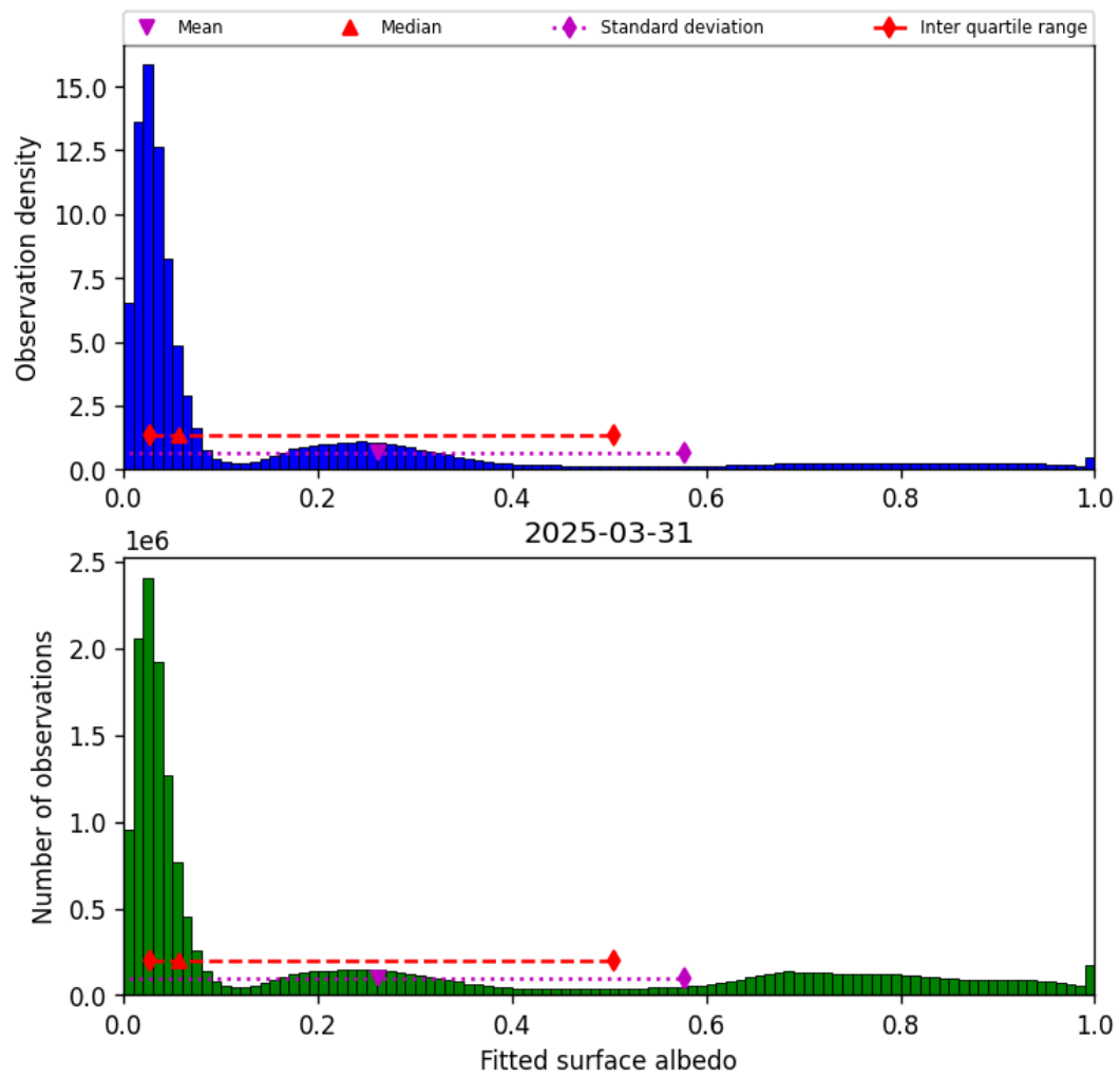
Figure 43: Histogram of “Fitted surface albedo” for 2025-03-31 to 2025-03-31
