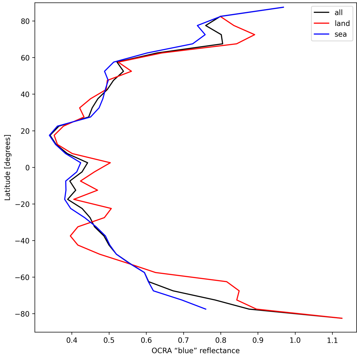
Figure 33: Zonal average of “OCRA “blue” reflectance” for 2025-03-31 to 2025-03-31.
