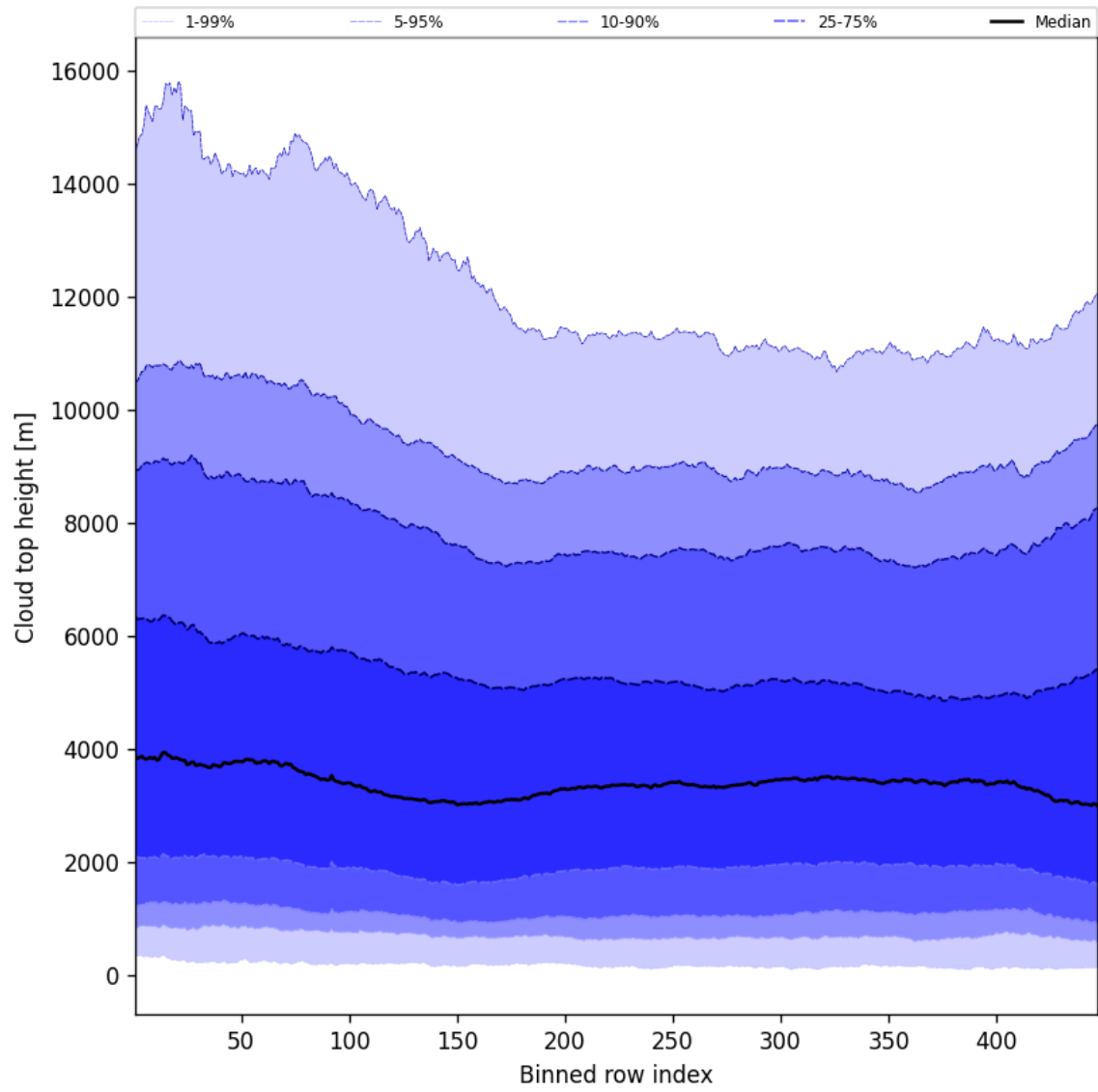
Figure 54: Along track statistics of “Cloud top height” for 2025-03-31 to 2025-03-31
