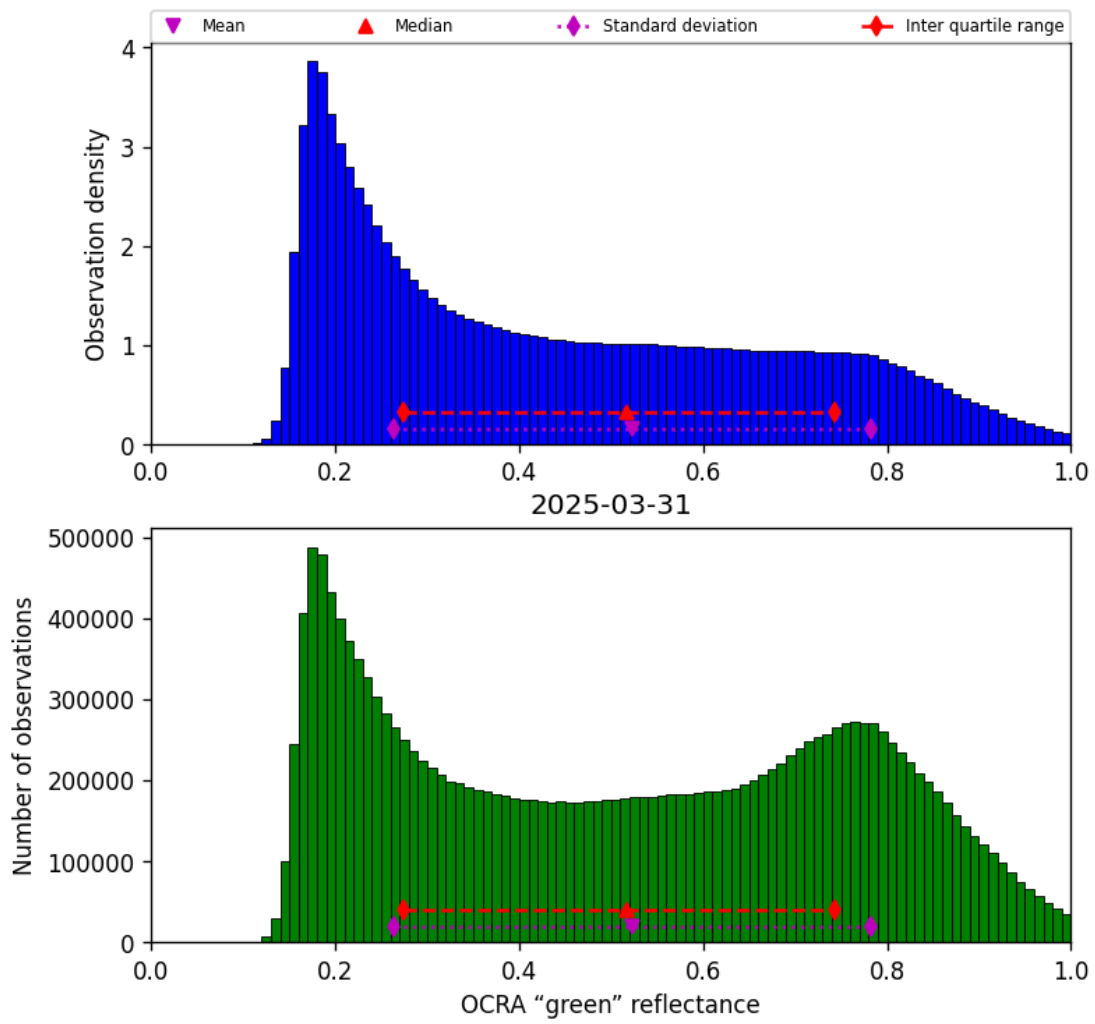
Figure 50: Histogram of “OCRA “green” reflectance” for 2025-03-31 to 2025-03-31
