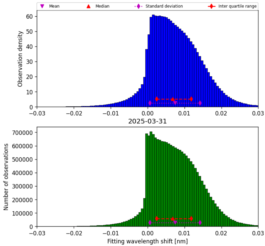
Figure 47: Histogram of “Fitting wavelength shift” for 2025-03-31 to 2025-03-31
