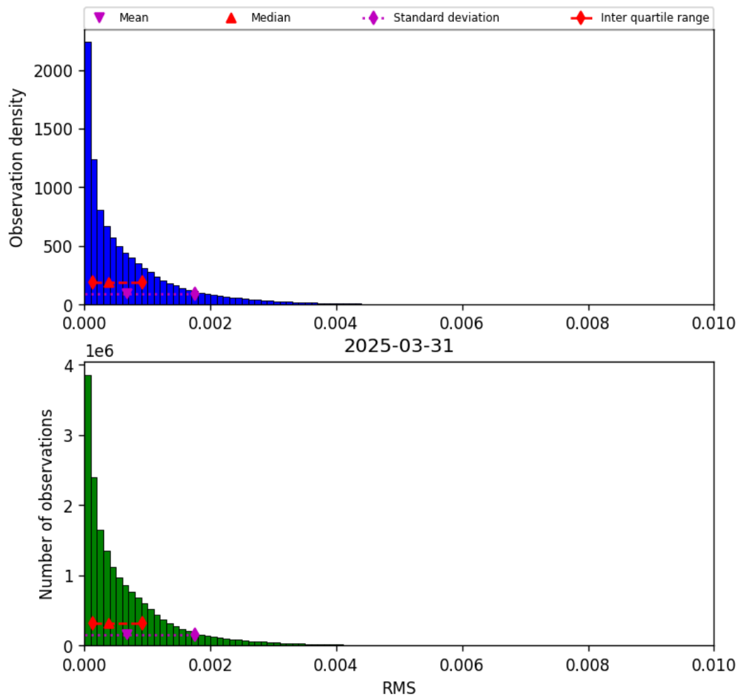
Figure 45: Histogram of “RMS” for 2025-03-31 to 2025-03-31
