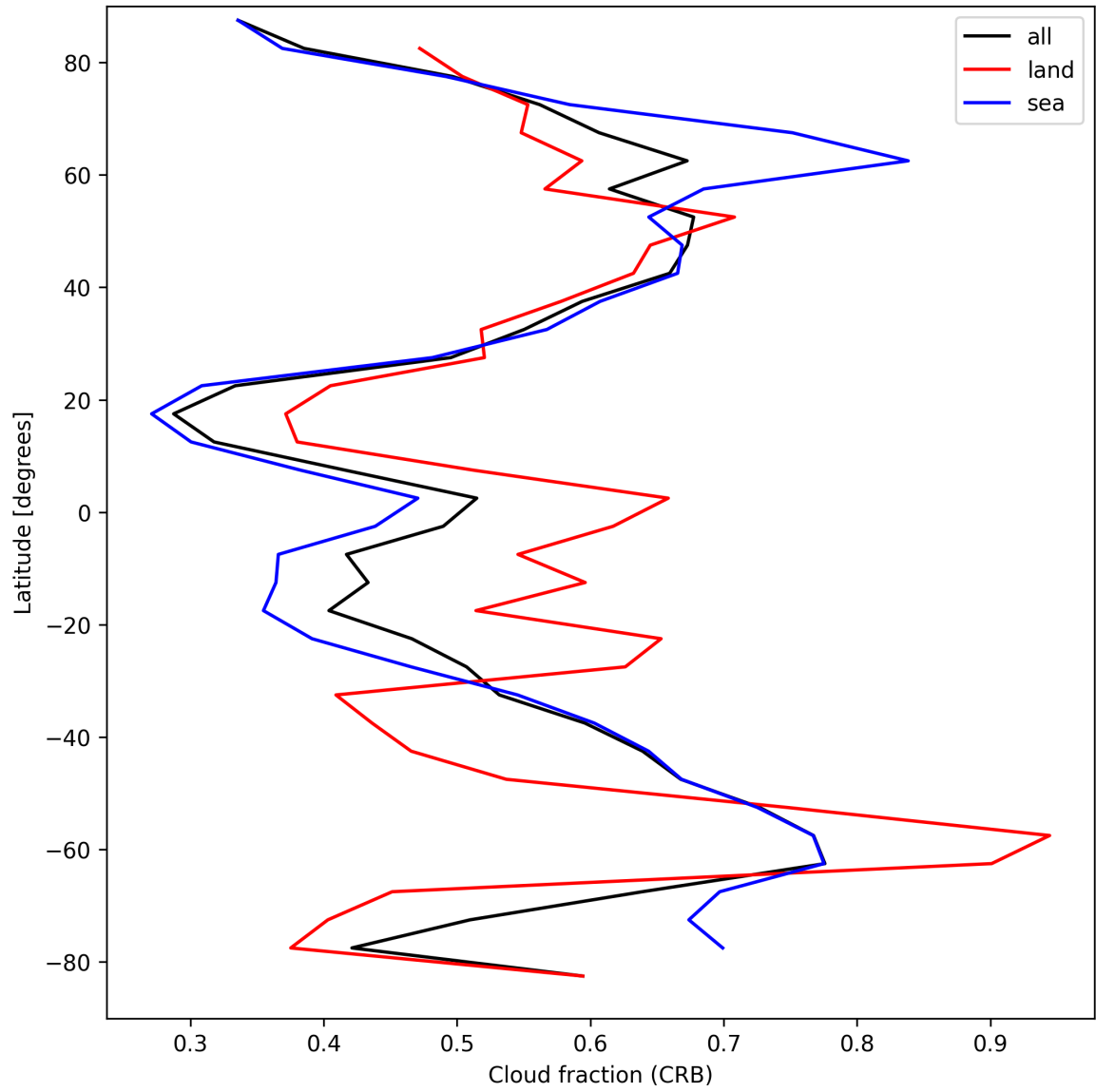
Figure 24: Zonal average of “Cloud fraction (CRB)” for 2025-03-31 to 2025-03-31.
