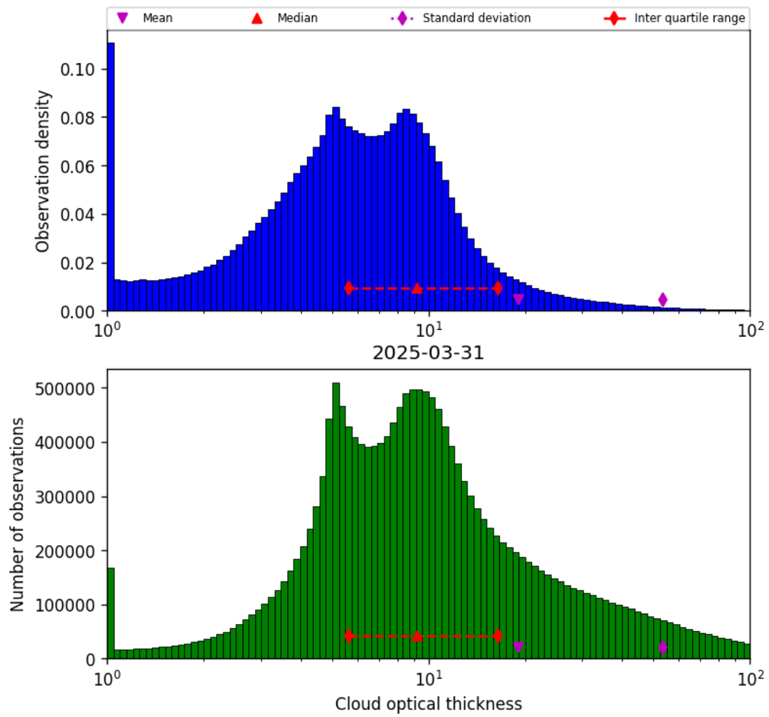
Figure 39: Histogram of “Cloud optical thickness” for 2025-03-31 to 2025-03-31
