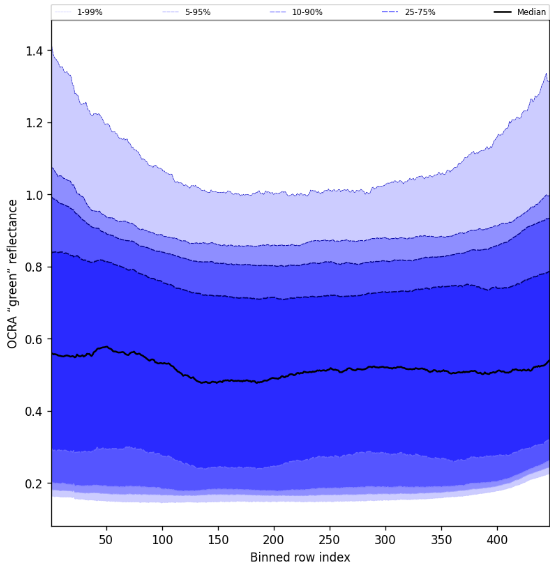
Figure 66: Along track statistics of “OCRA “green” reflectance” for 2025-03-31 to 2025-03-31
