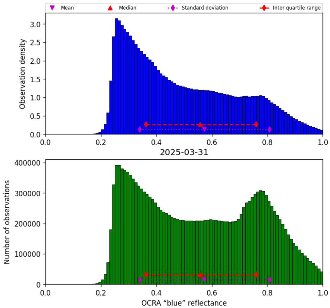
Figure 49: Histogram of “OCRA “blue” reflectance” for 2025-03-31 to 2025-03-31
