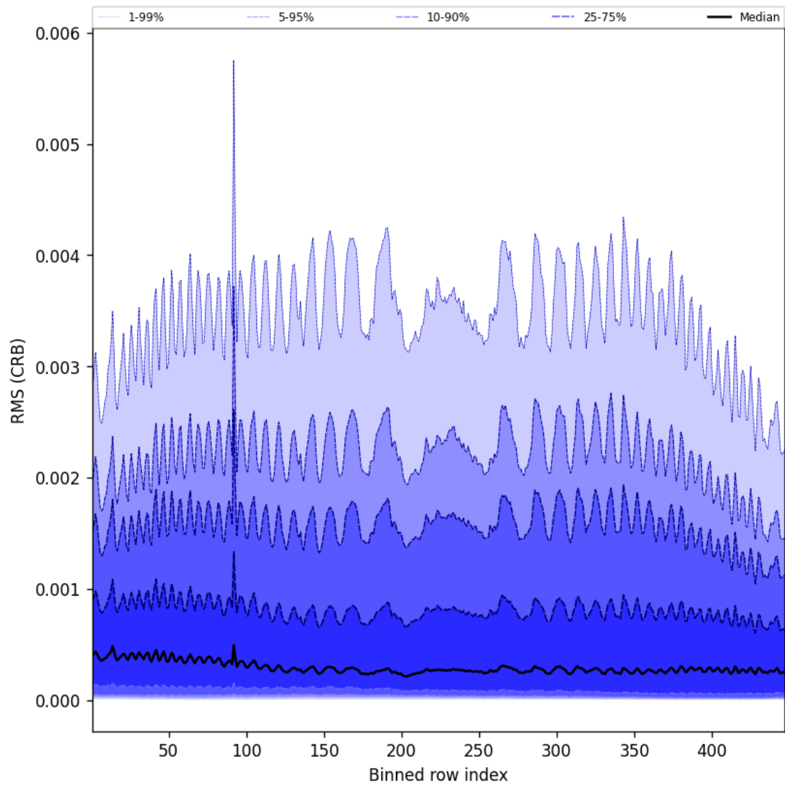
Figure 62: Along track statistics of “RMS (CRB)” for 2025-03-31 to 2025-03-31
