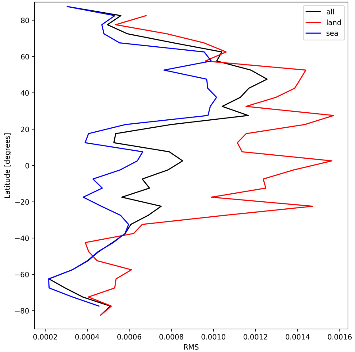
Figure 29: Zonal average of “RMS” for 2025-03-31 to 2025-03-31.
