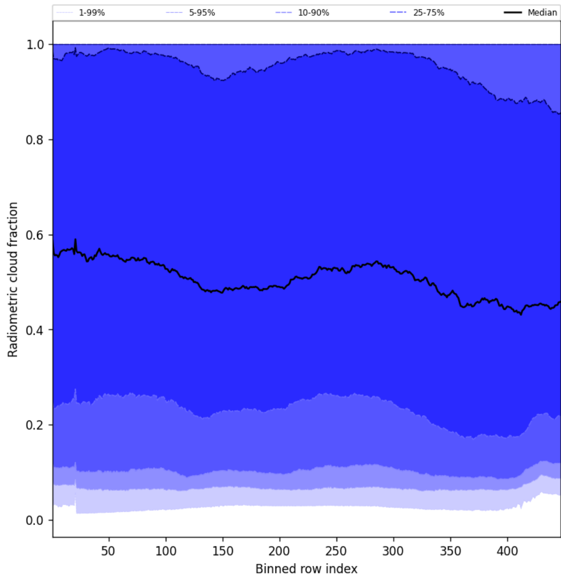
Figure 53: Along track statistics of “Radiometric cloud fraction” for 2025-03-31 to 2025-03-31
