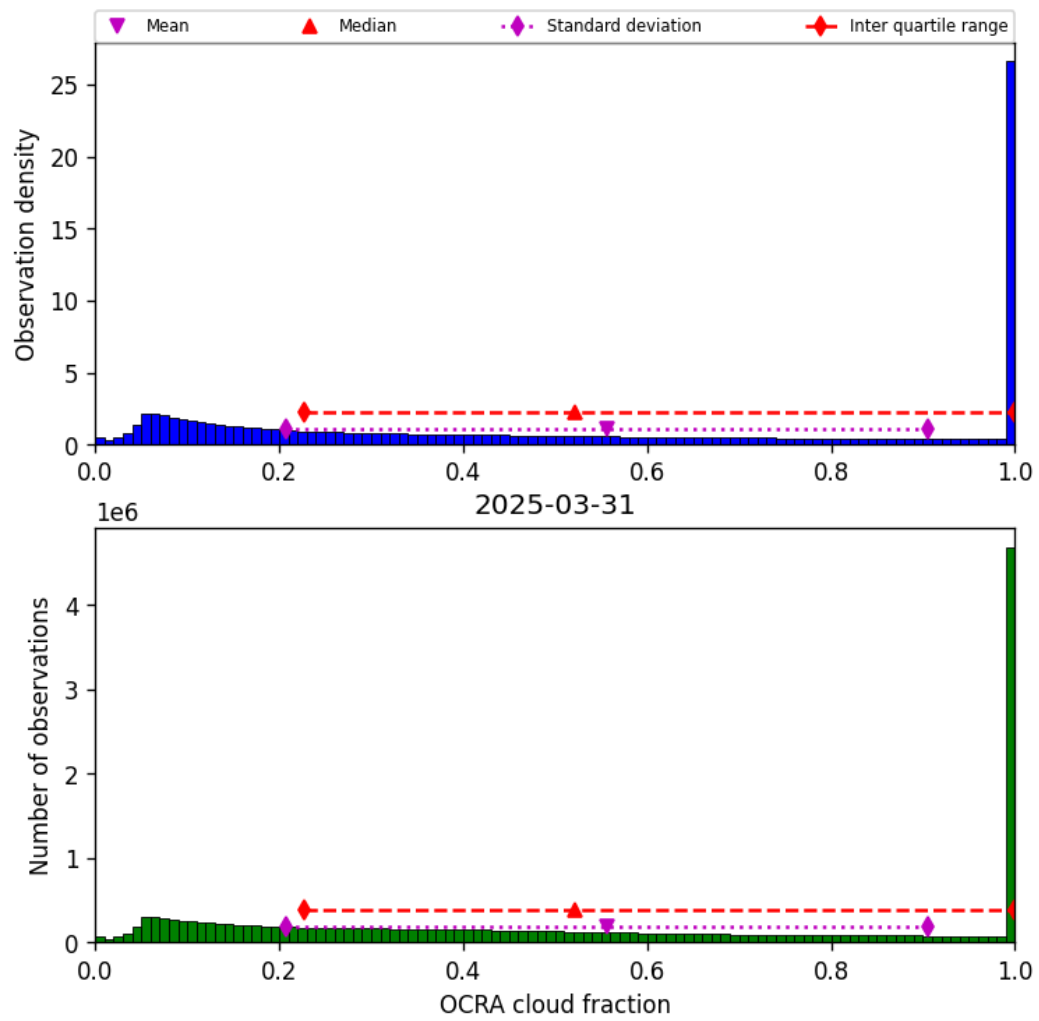
Figure 48: Histogram of “OCRA cloud fraction” for 2025-03-31 to 2025-03-31
