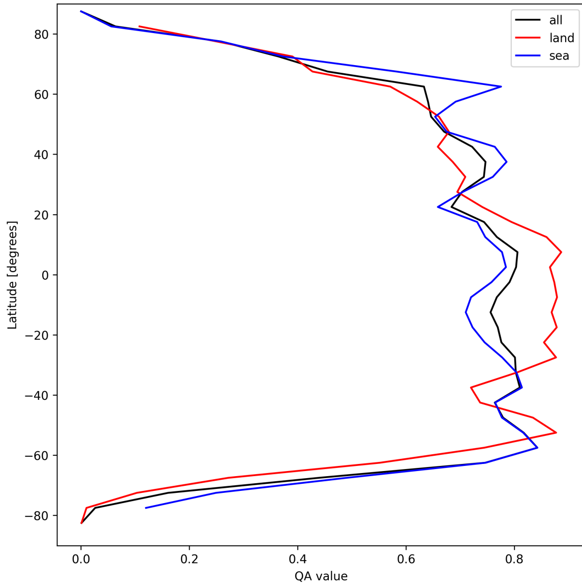
Figure 20: Zonal average of “QA value” for 2025-03-31 to 2025-03-31.
