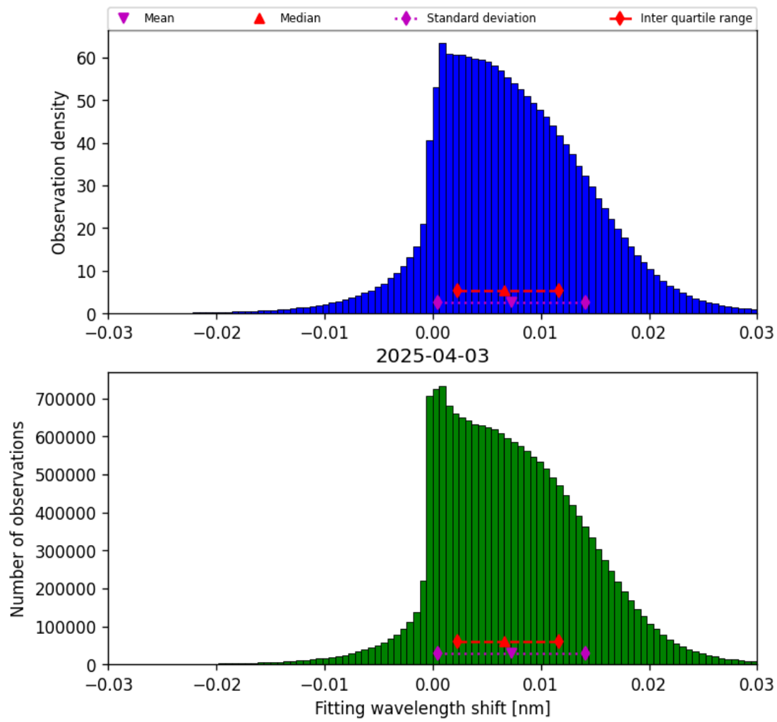
Figure 47: Histogram of “Fitting wavelength shift” for 2025-04-03 to 2025-04-04
