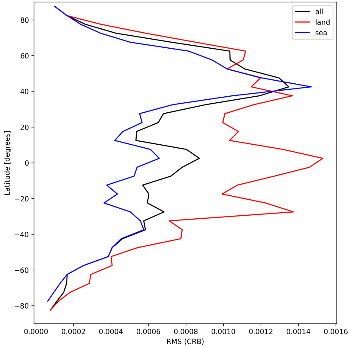
Figure 30: Zonal average of “RMS (CRB)” for 2025-04-03 to 2025-04-04.
