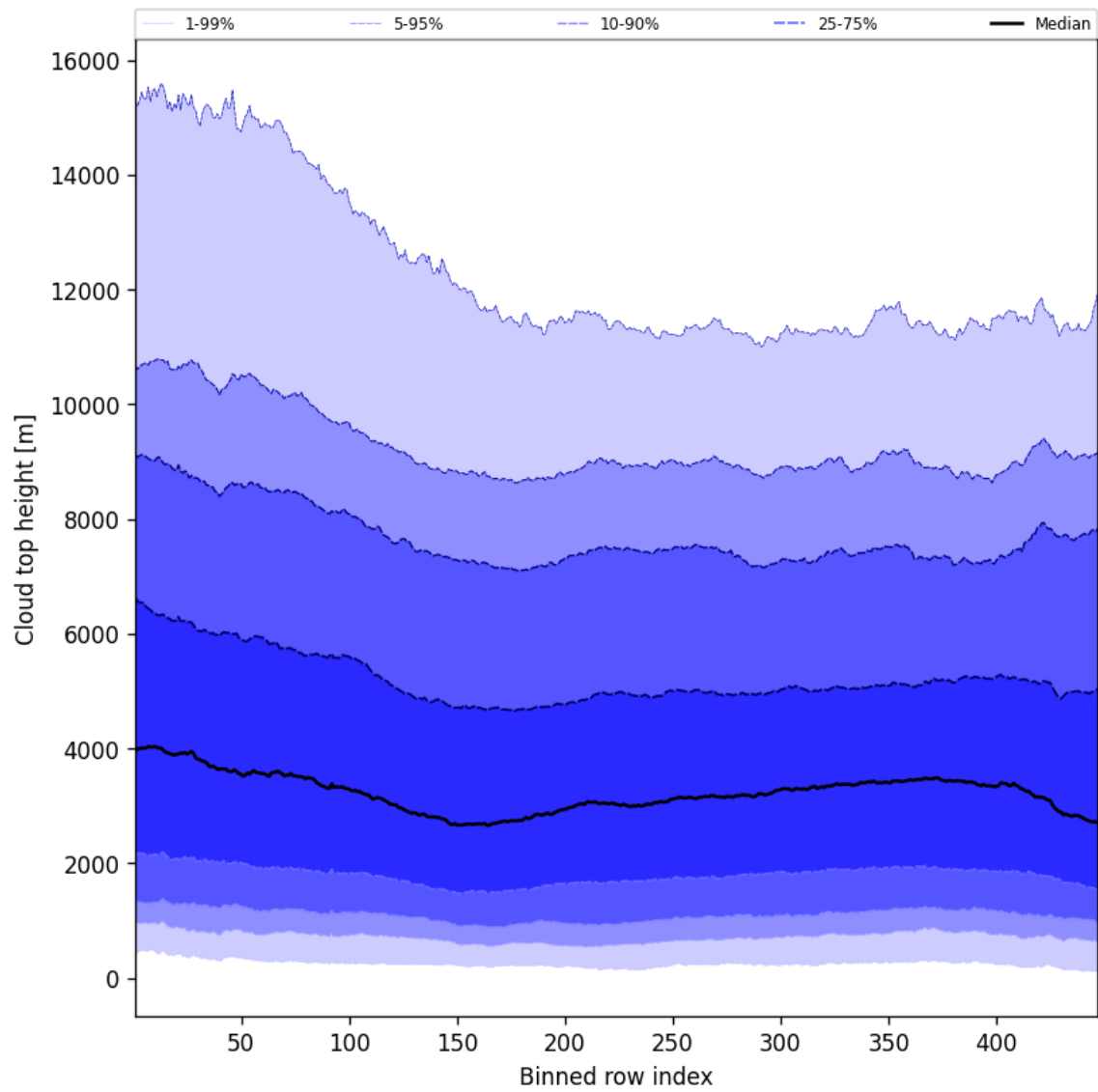
Figure 54: Along track statistics of “Cloud top height” for 2025-04-03 to 2025-04-04
