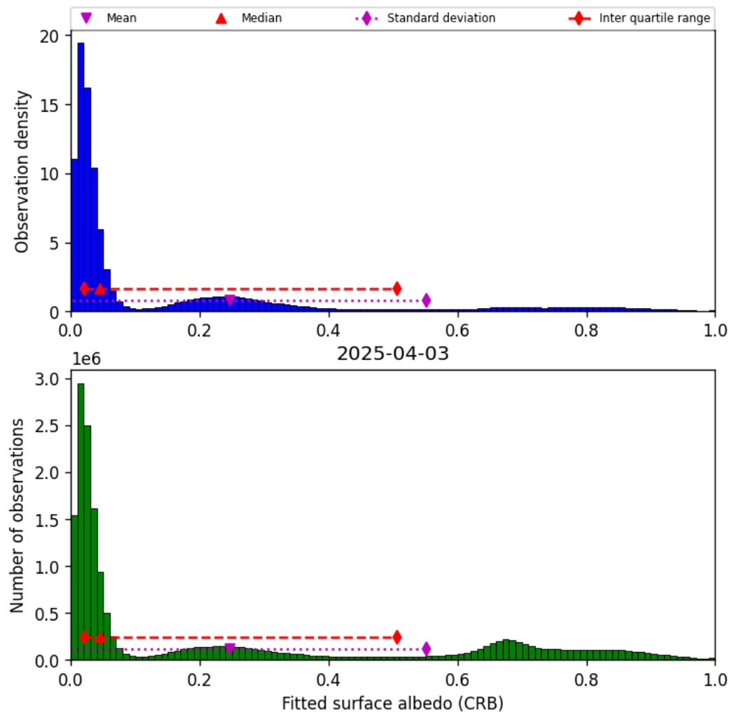
Figure 44: Histogram of “Fitted surface albedo (CRB)” for 2025-04-03 to 2025-04-04
