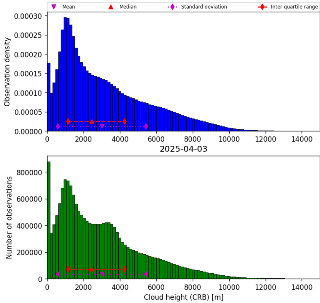
Figure 41: Histogram of “Cloud height (CRB)” for 2025-04-03 to 2025-04-04
