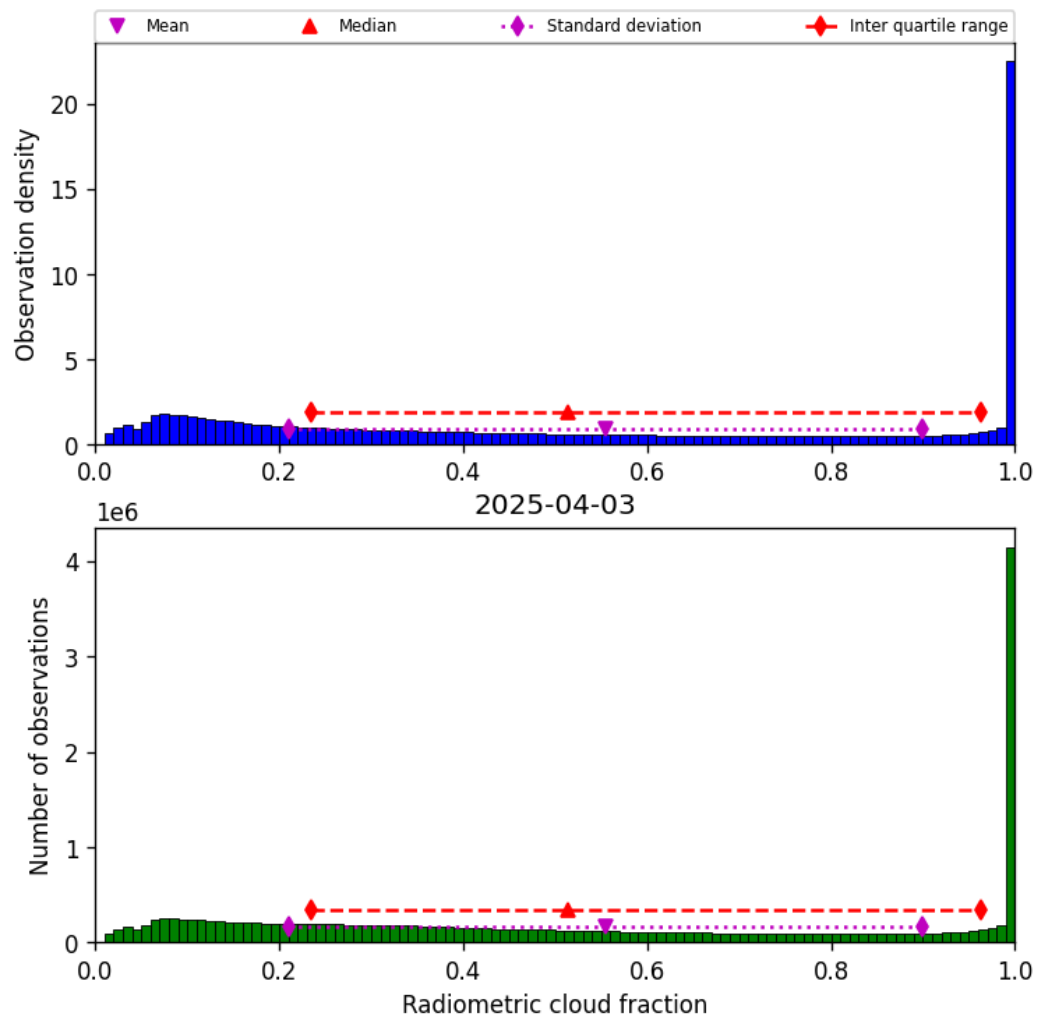
Figure 37: Histogram of “Radiometric cloud fraction” for 2025-04-03 to 2025-04-04
