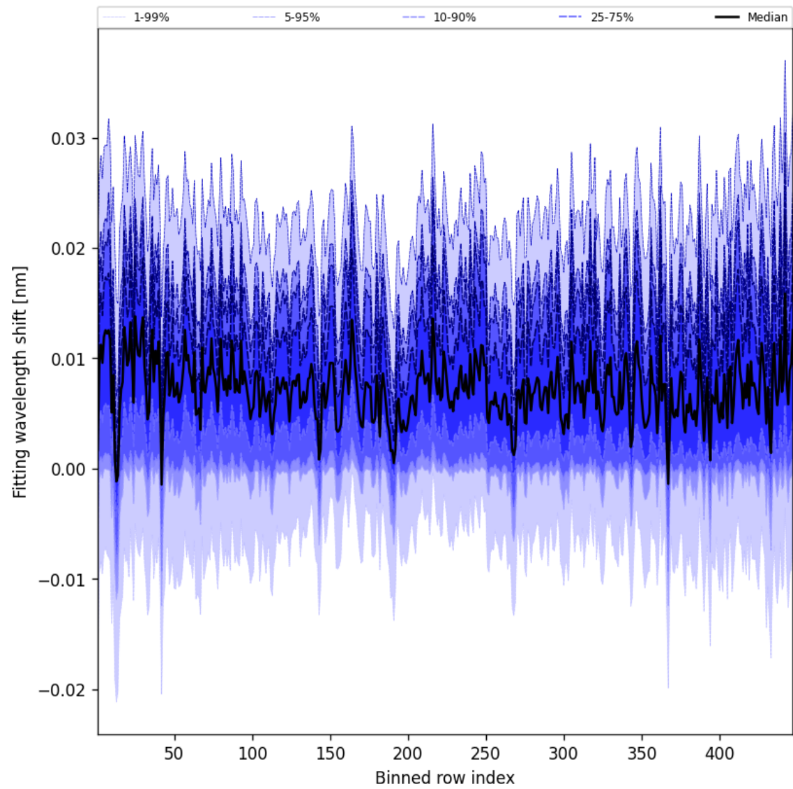
Figure 63: Along track statistics of “Fitting wavelength shift” for 2025-04-03 to 2025-04-04
