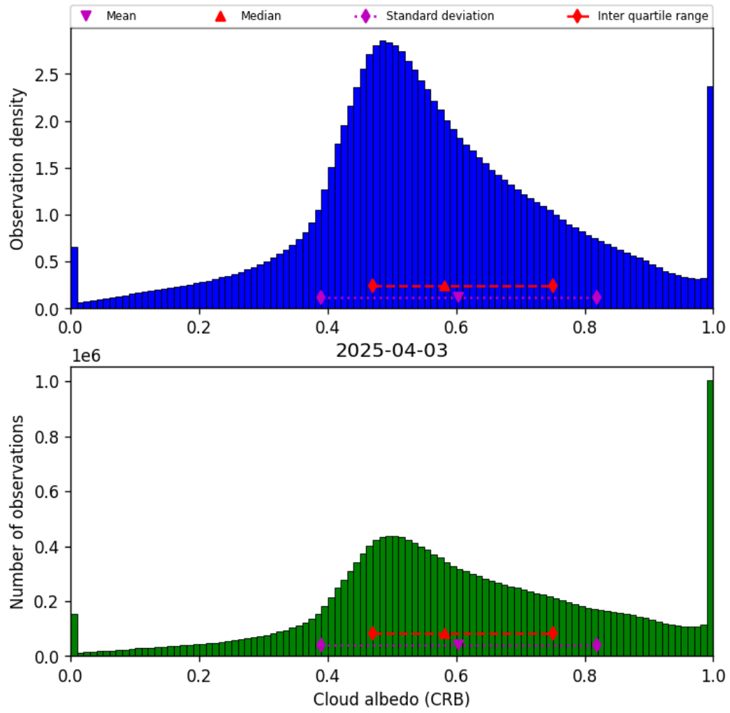
Figure 42: Histogram of “Cloud albedo (CRB)” for 2025-04-03 to 2025-04-04
