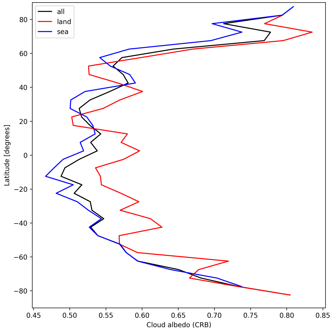
Figure 26: Zonal average of “Cloud albedo (CRB)” for 2025-04-03 to 2025-04-04.
