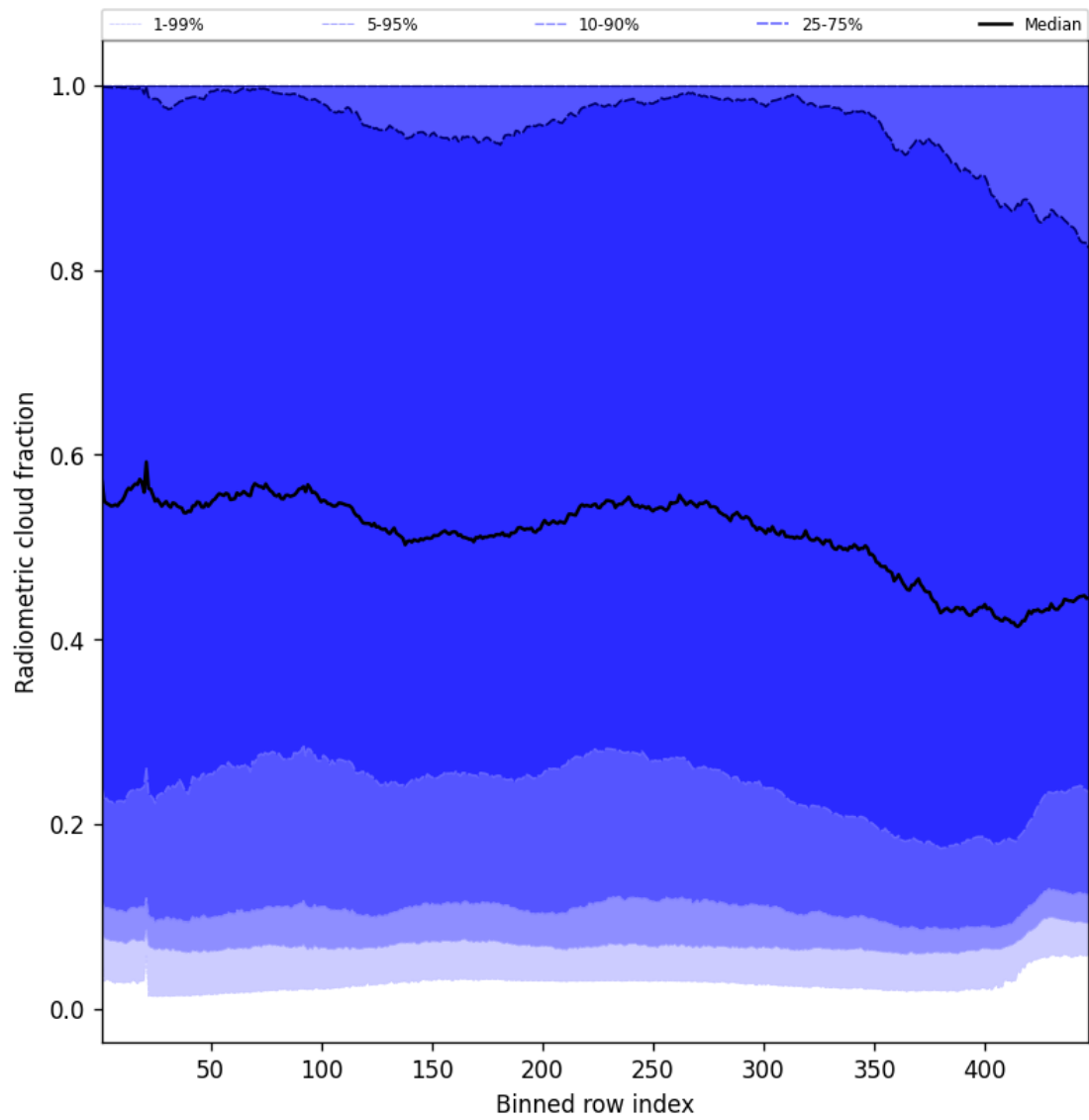
Figure 53: Along track statistics of “Radiometric cloud fraction” for 2025-04-03 to 2025-04-04
