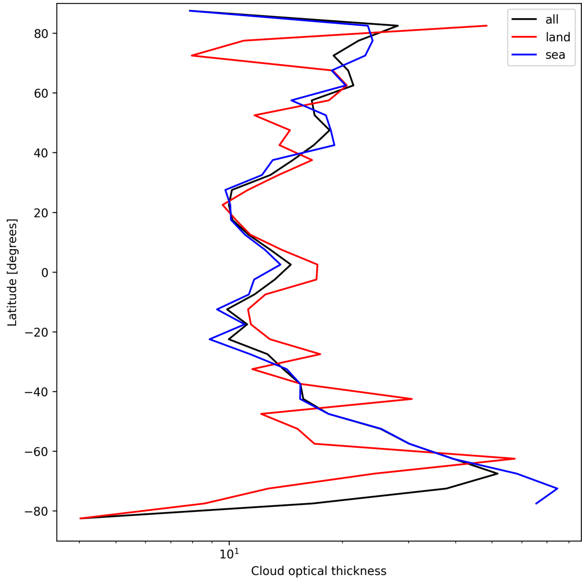
Figure 23: Zonal average of “Cloud optical thickness” for 2025-04-03 to 2025-04-04.
