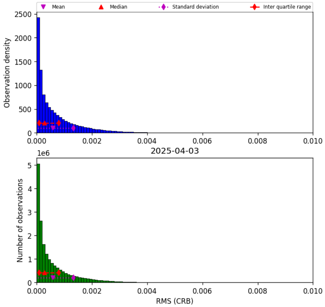
Figure 46: Histogram of “RMS (CRB)” for 2025-04-03 to 2025-04-04
