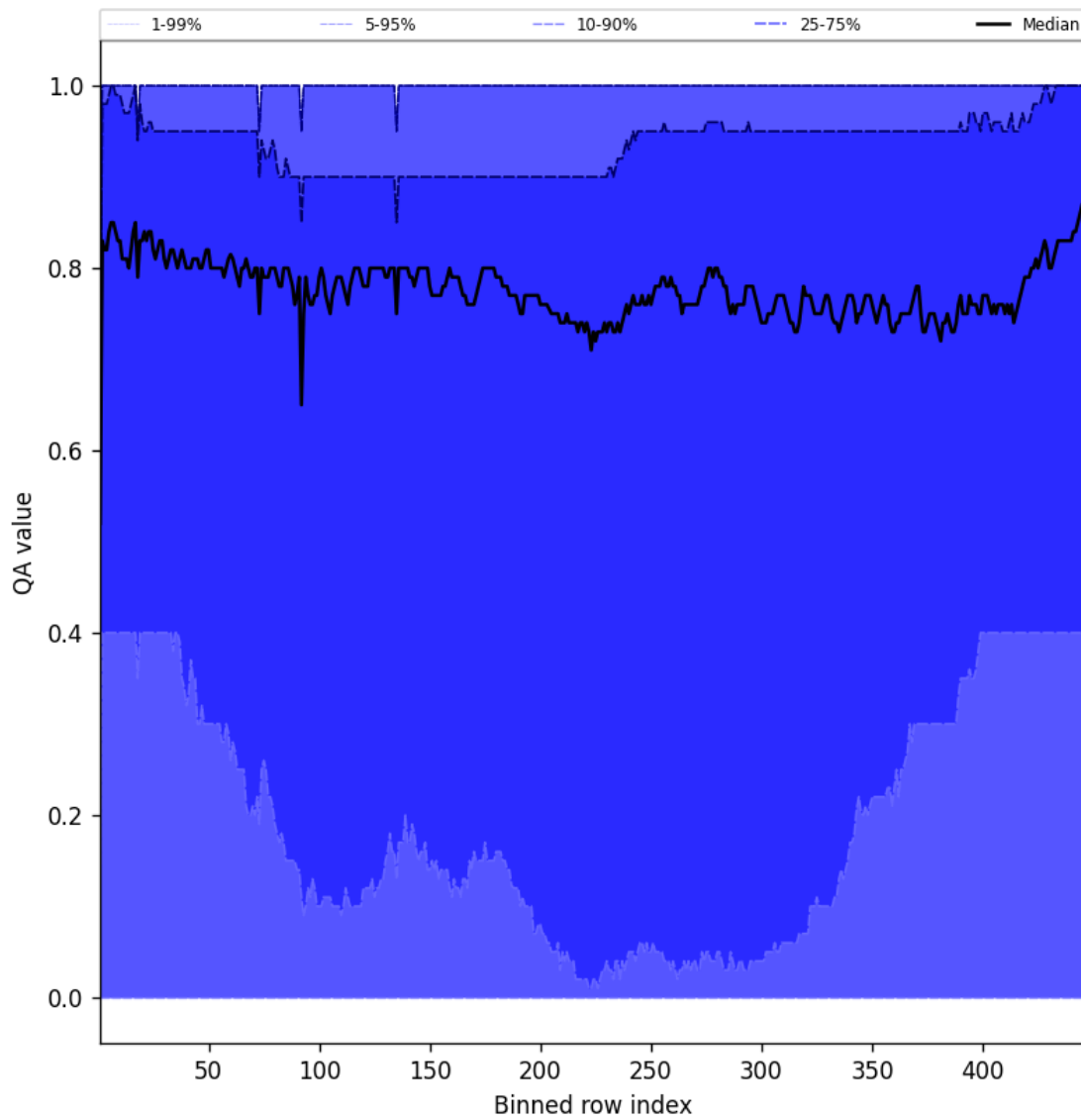
Figure 52: Along track statistics of “QA value” for 2025-04-03 to 2025-04-04
