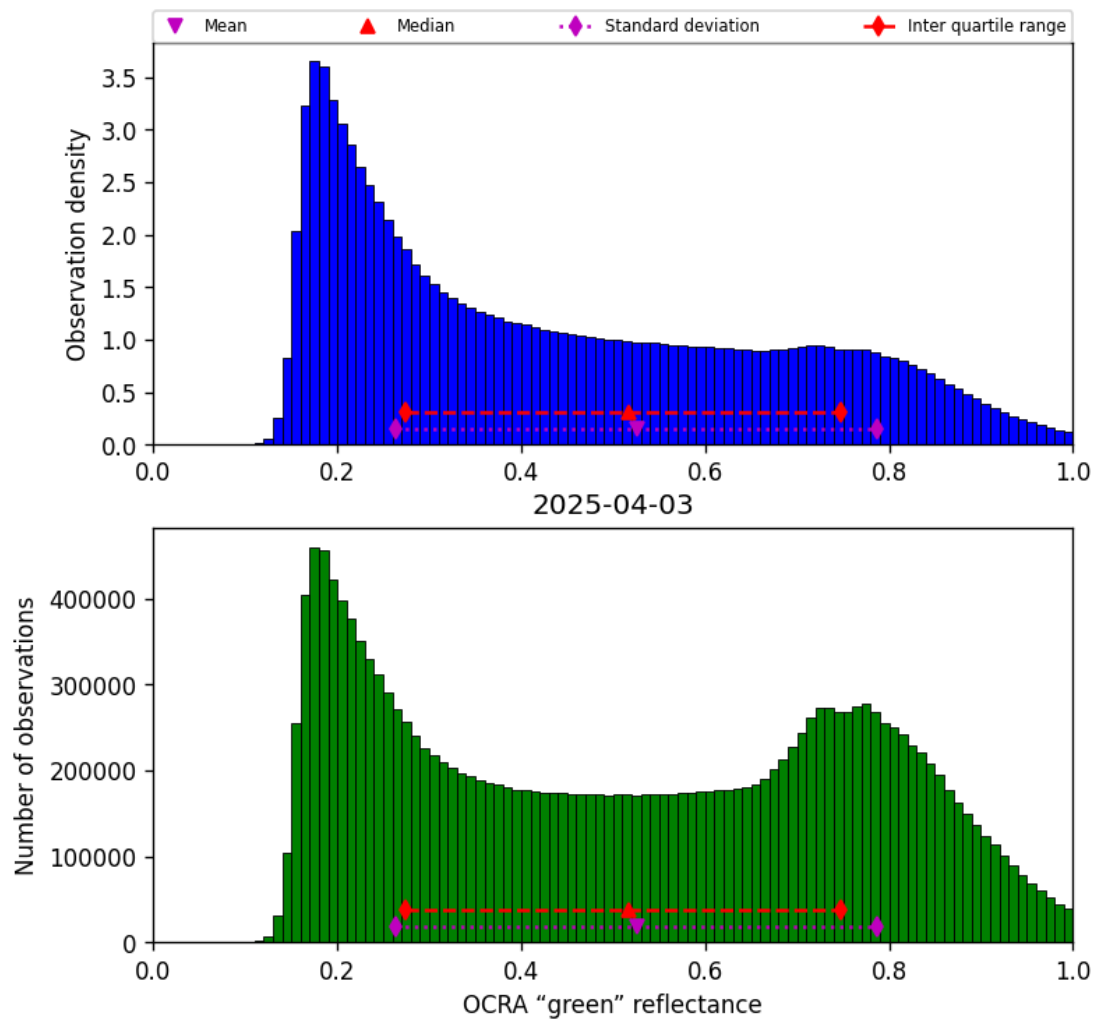
Figure 50: Histogram of “OCRA “green” reflectance” for 2025-04-03 to 2025-04-04
