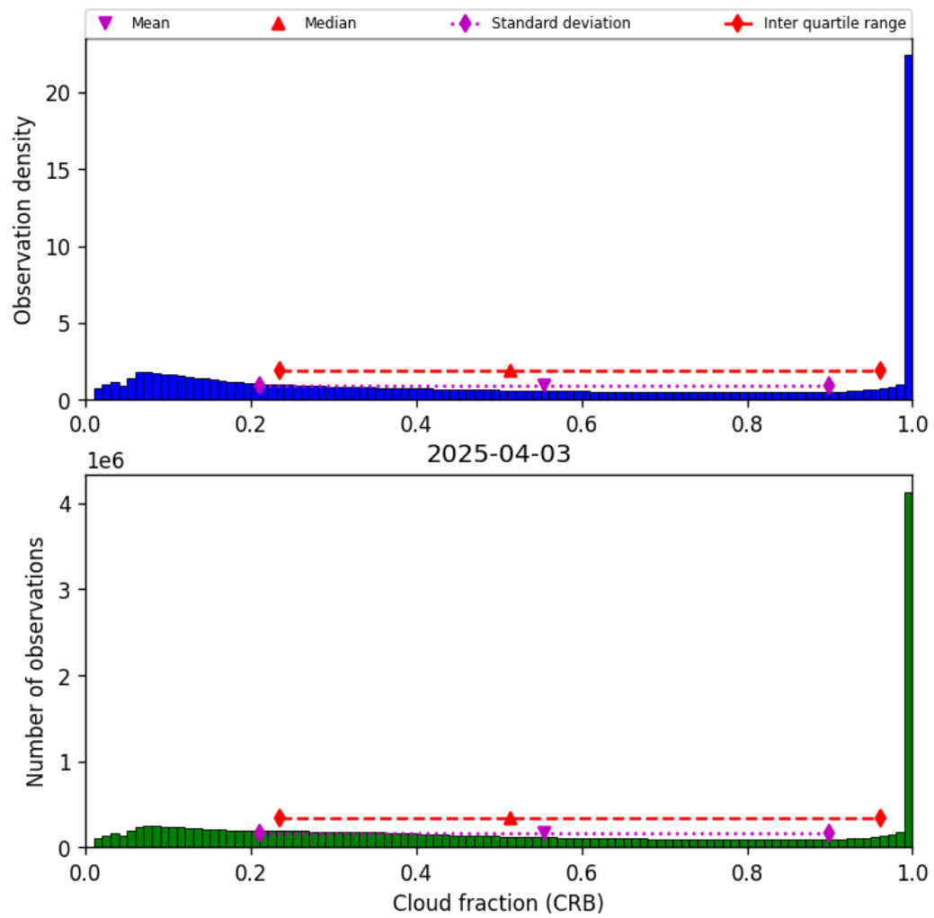
Figure 40: Histogram of “Cloud fraction (CRB)” for 2025-04-03 to 2025-04-04
