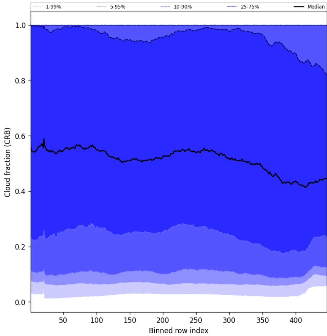
Figure 56: Along track statistics of “Cloud fraction (CRB)” for 2025-04-03 to 2025-04-04
