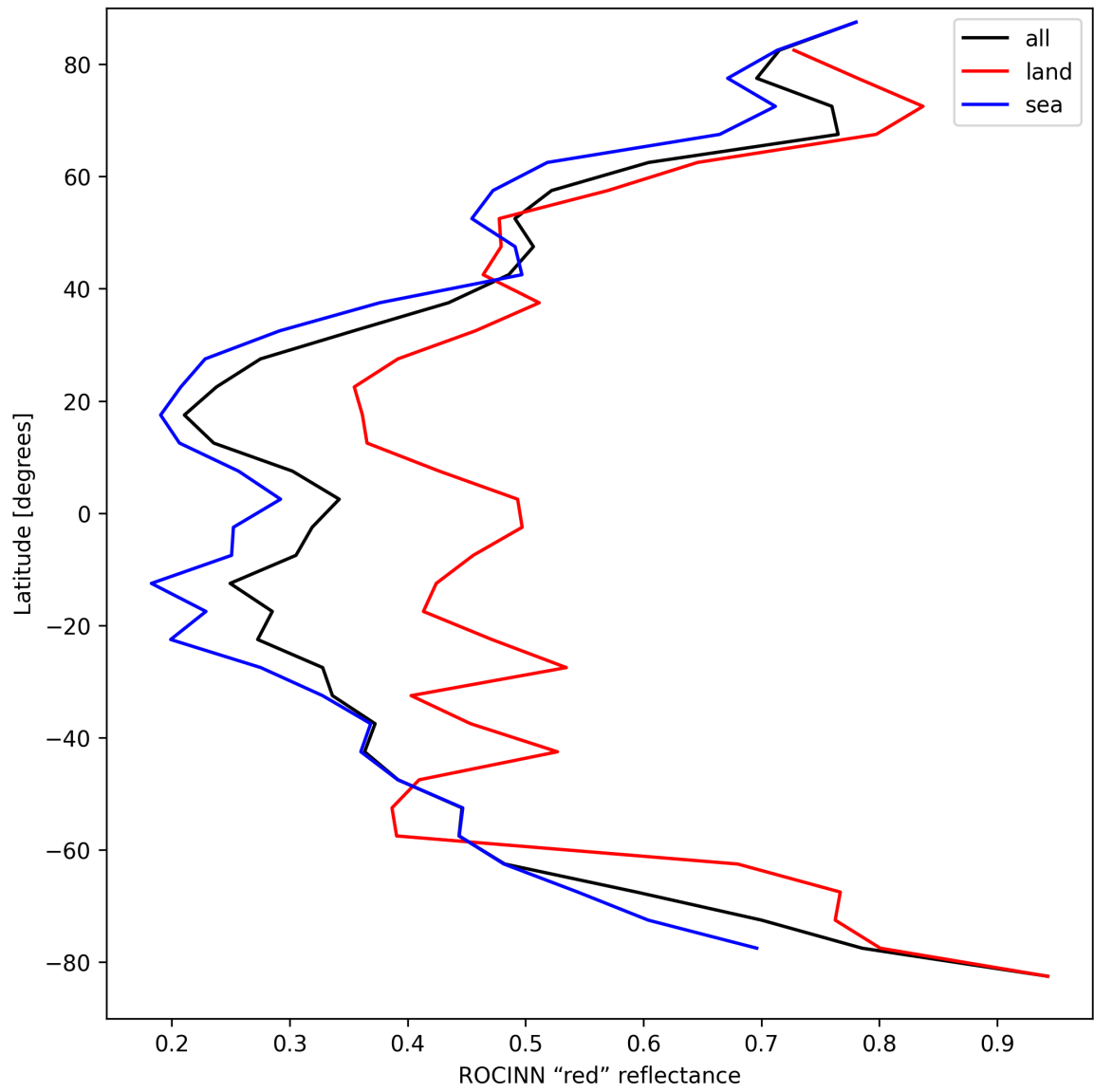
Figure 35: Zonal average of "ROCINN "red" reflectance" for 2025-04-03 to 2025-04-04.
