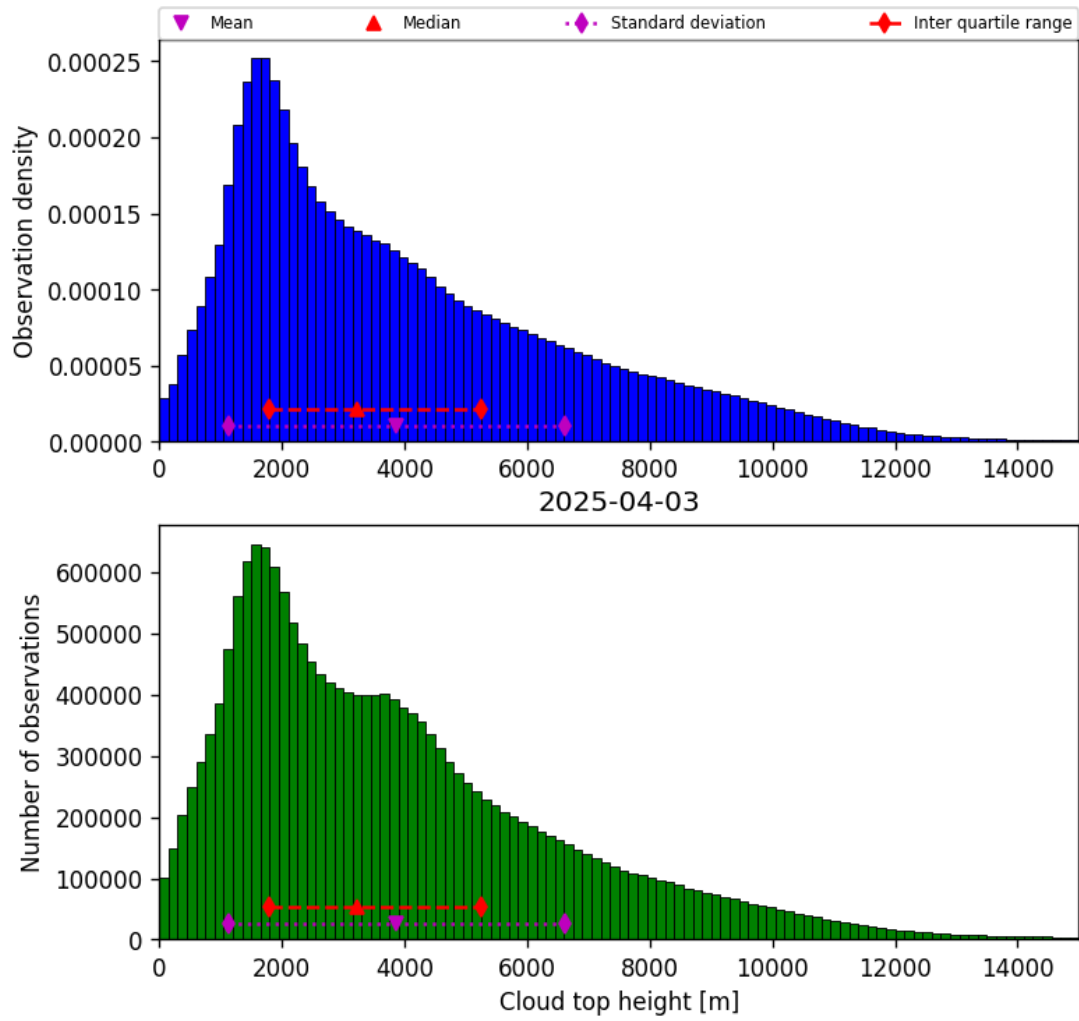
Figure 38: Histogram of “Cloud top height” for 2025-04-03 to 2025-04-04
