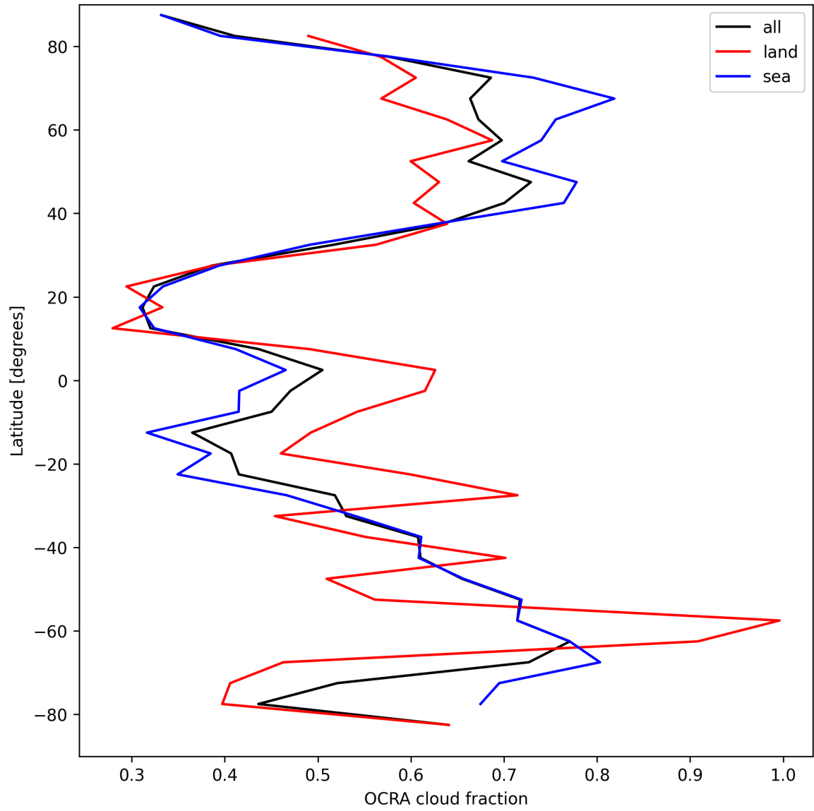
Figure 32: Zonal average of “OCRA cloud fraction” for 2025-04-03 to 2025-04-04.
