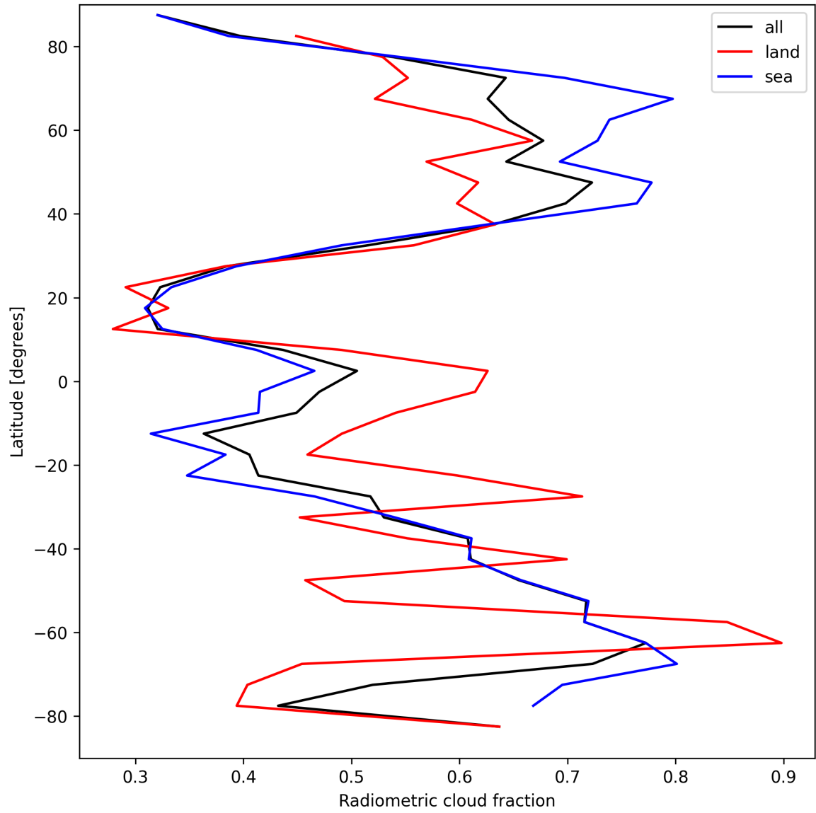
Figure 21: Zonal average of “Radiometric cloud fraction” for 2025-04-03 to 2025-04-04.
