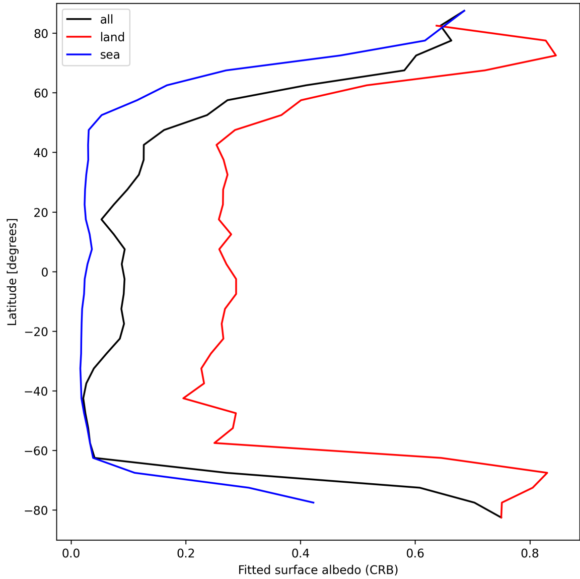
Figure 28: Zonal average of “Fitted surface albedo (CRB)” for 2025-04-03 to 2025-04-04.
