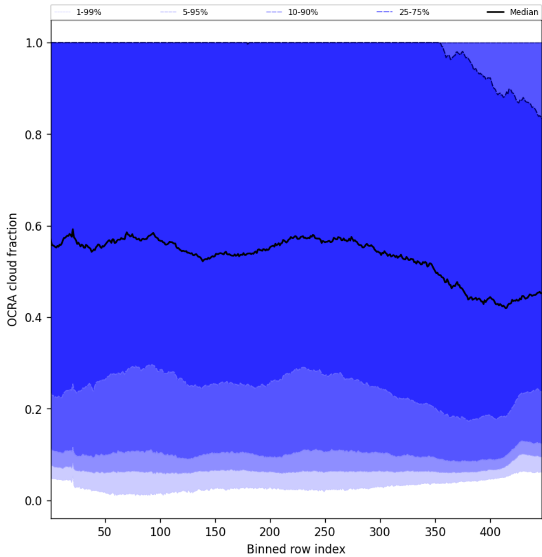
Figure 64: Along track statistics of “OCRA cloud fraction” for 2025-04-03 to 2025-04-04
