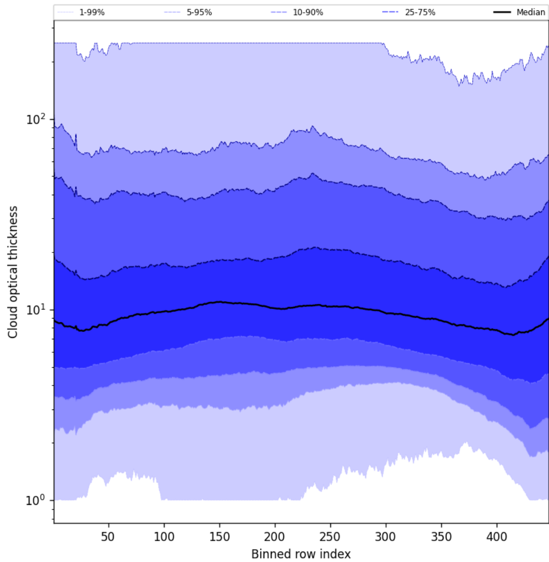
Figure 55: Along track statistics of “Cloud optical thickness” for 2025-04-03 to 2025-04-04
