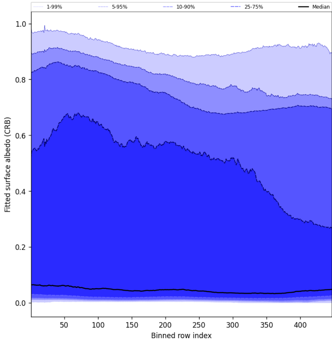
Figure 60: Along track statistics of “Fitted surface albedo (CRB)” for 2025-04-03 to 2025-04-04
