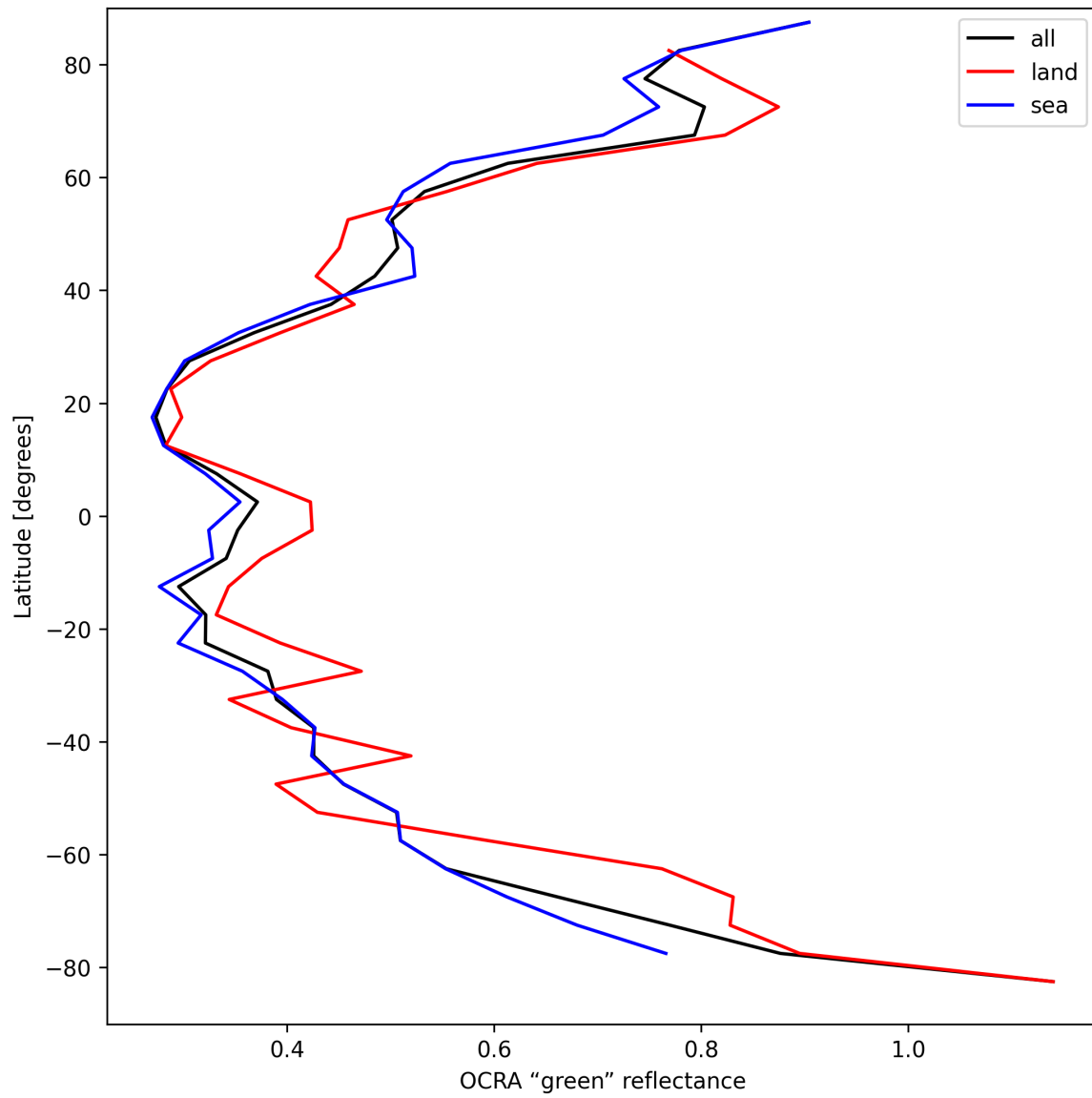
Figure 34: Zonal average of “OCRA “green” reflectance” for 2025-04-03 to 2025-04-04.
