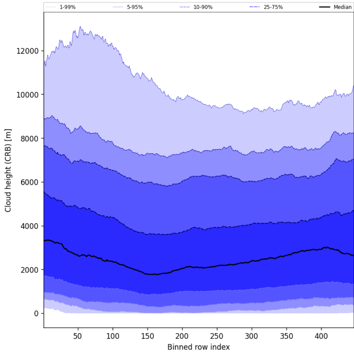
Figure 57: Along track statistics of “Cloud height (CRB)” for 2025-04-03 to 2025-04-04
