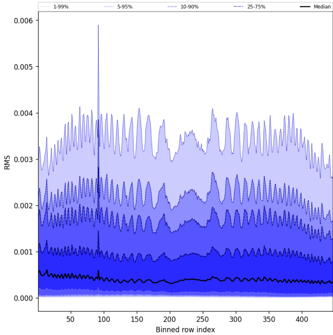
Figure 61: Along track statistics of “RMS” for 2025-04-03 to 2025-04-04
