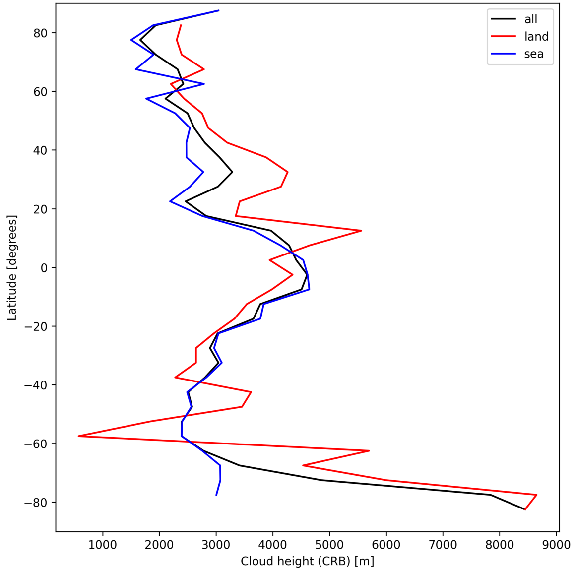
Figure 25: Zonal average of “Cloud height (CRB)” for 2025-04-03 to 2025-04-04.
