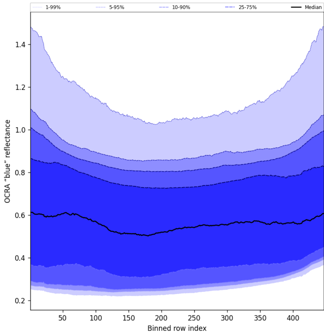
Figure 65: Along track statistics of “OCRA “blue” reflectance” for 2025-04-03 to 2025-04-04
