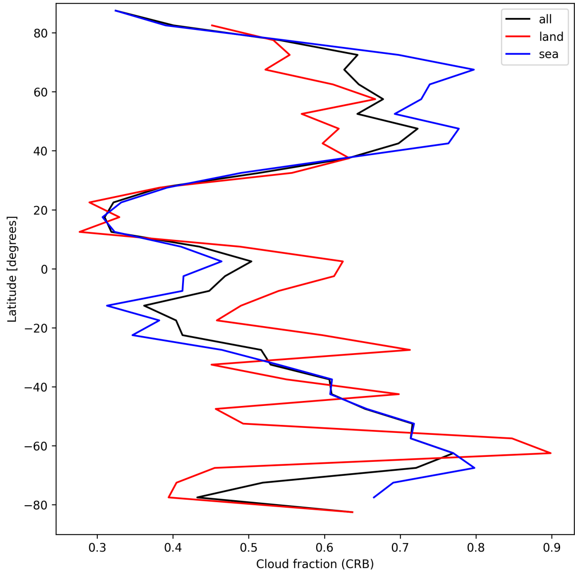
Figure 24: Zonal average of “Cloud fraction (CRB)” for 2025-04-03 to 2025-04-04.
