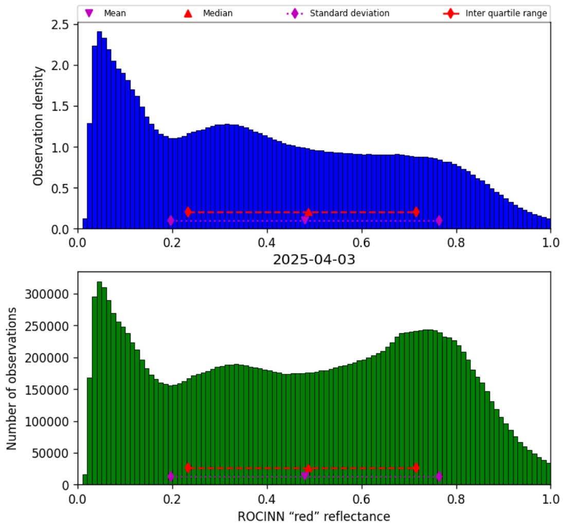
Figure 51: Histogram of “ROCINN “red” reflectance” for 2025-04-03 to 2025-04-04
