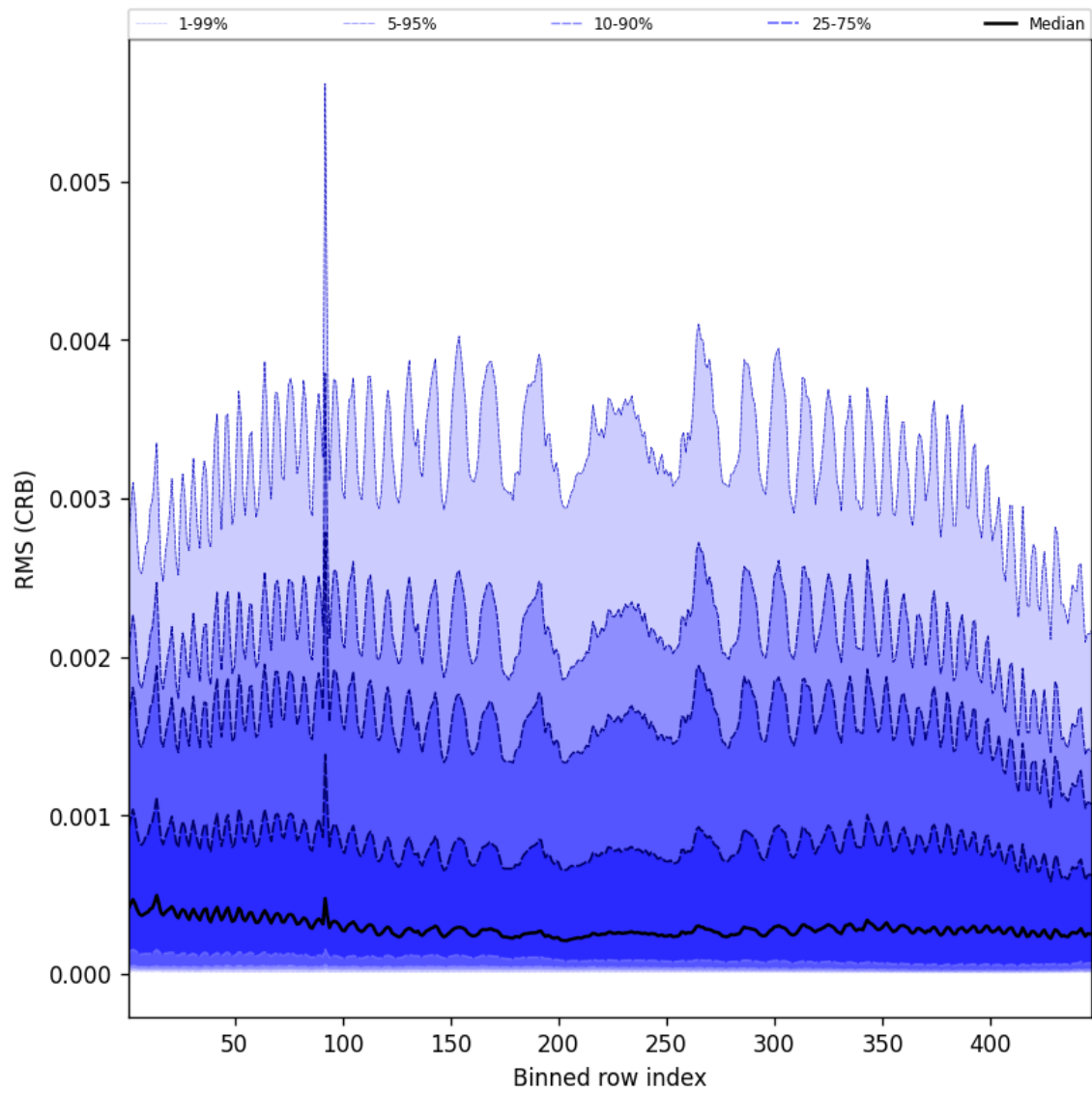
Figure 62: Along track statistics of “RMS (CRB)” for 2025-04-03 to 2025-04-04
