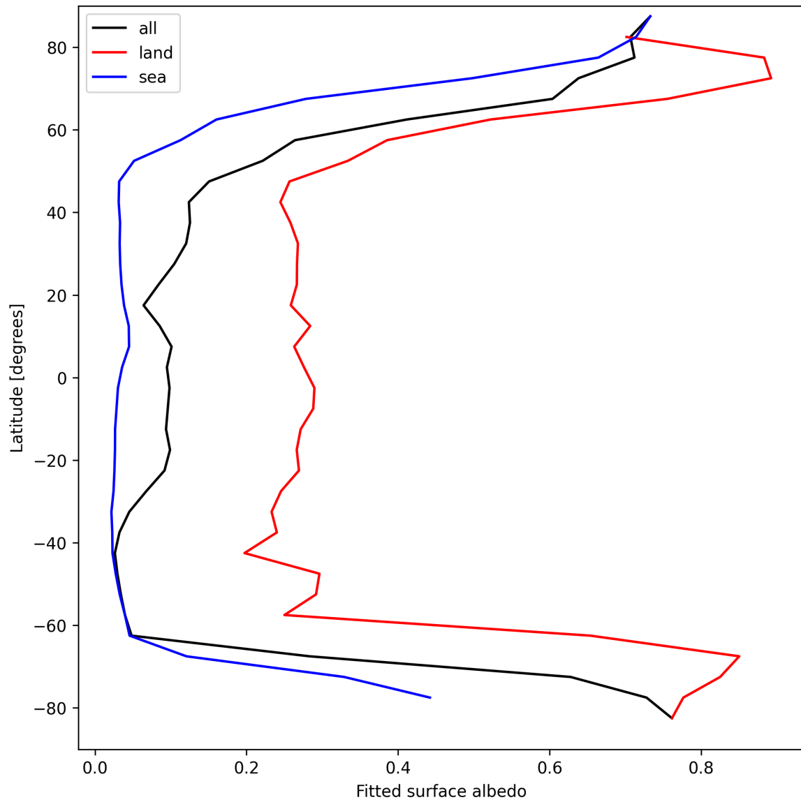
Figure 27: Zonal average of “Fitted surface albedo” for 2025-04-03 to 2025-04-04.
