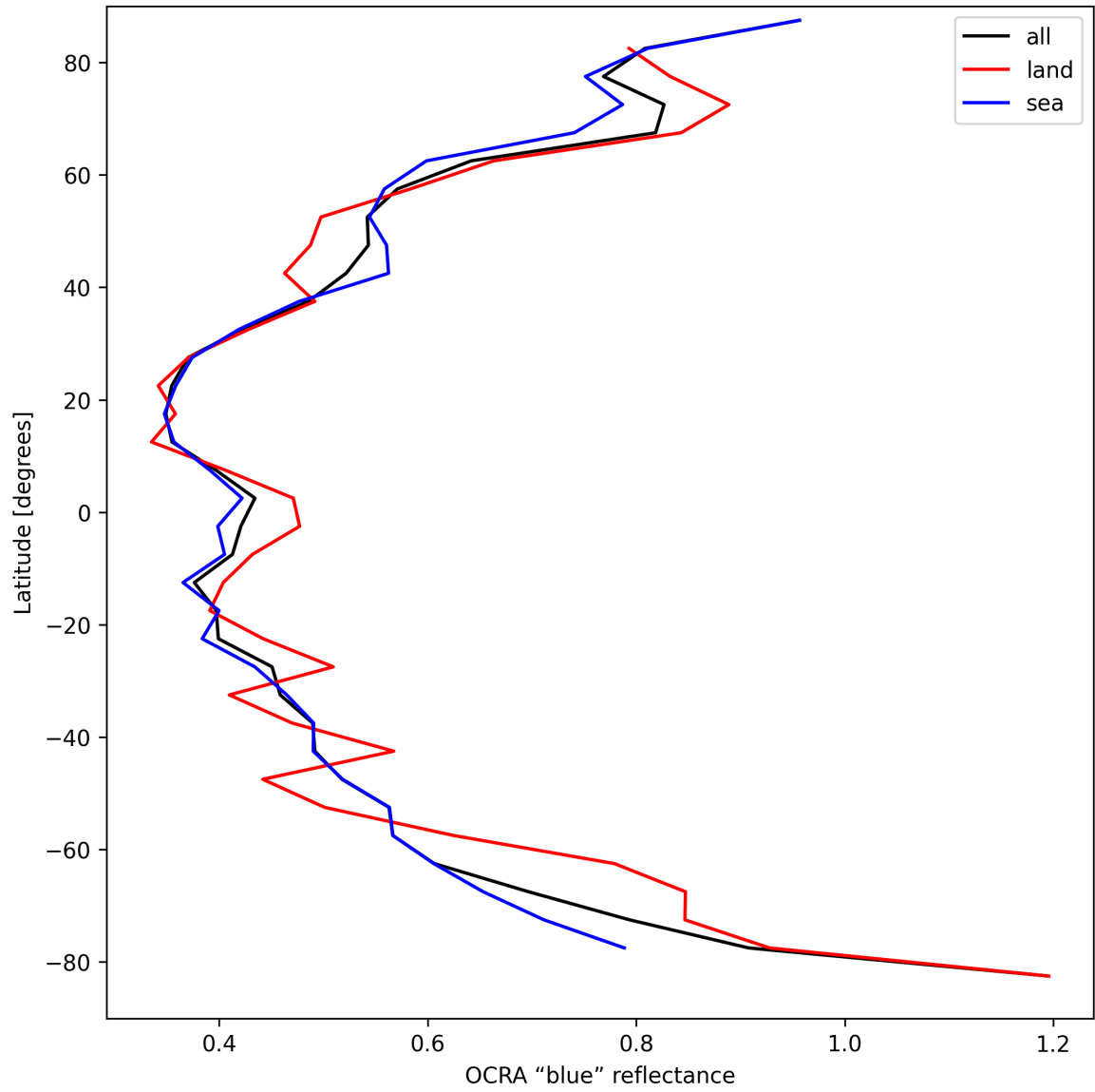
Figure 33: Zonal average of "OCRA "blue" reflectance" for 2025-04-03 to 2025-04-04.
