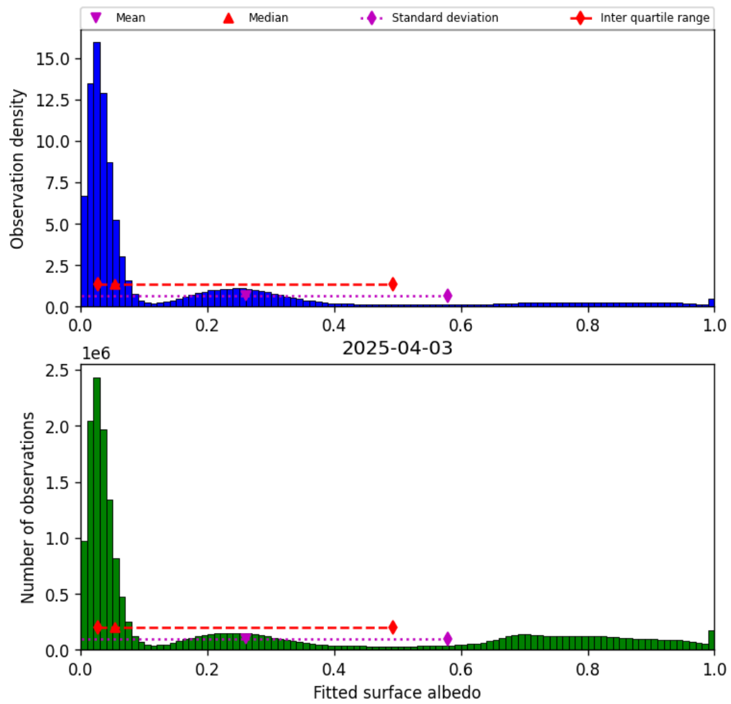
Figure 43: Histogram of “Fitted surface albedo” for 2025-04-03 to 2025-04-04
