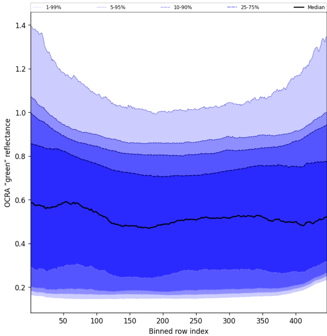
Figure 66: Along track statistics of "OCRA "green" reflectance" for 2025-04-03 to 2025-04-04
