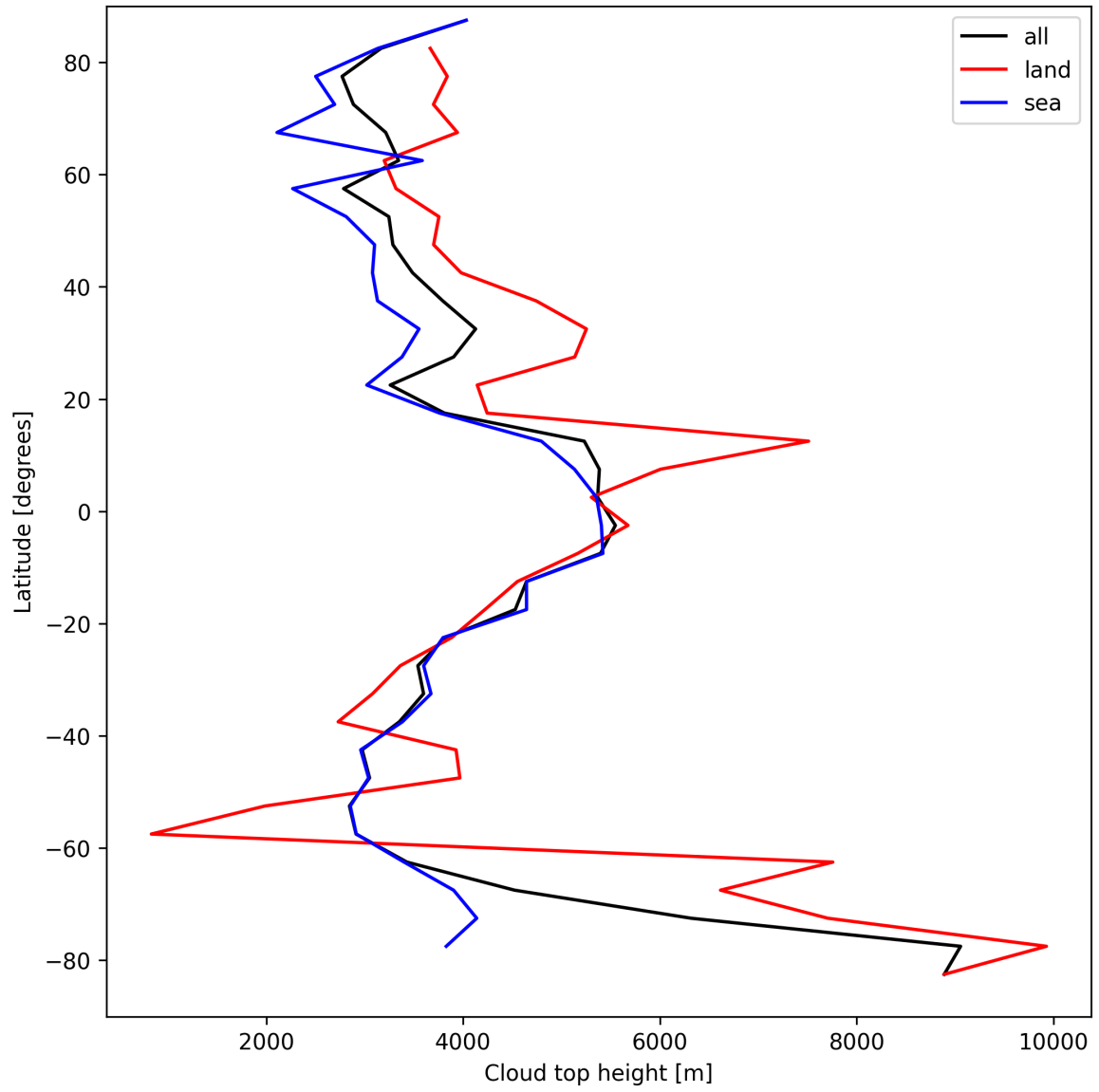
Figure 22: Zonal average of “Cloud top height” for 2025-04-03 to 2025-04-04.
