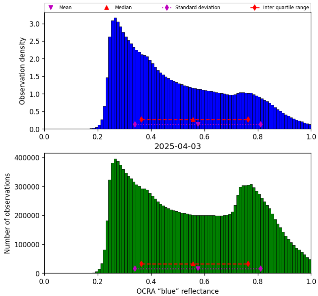
Figure 49: Histogram of “OCRA “blue” reflectance” for 2025-04-03 to 2025-04-04
