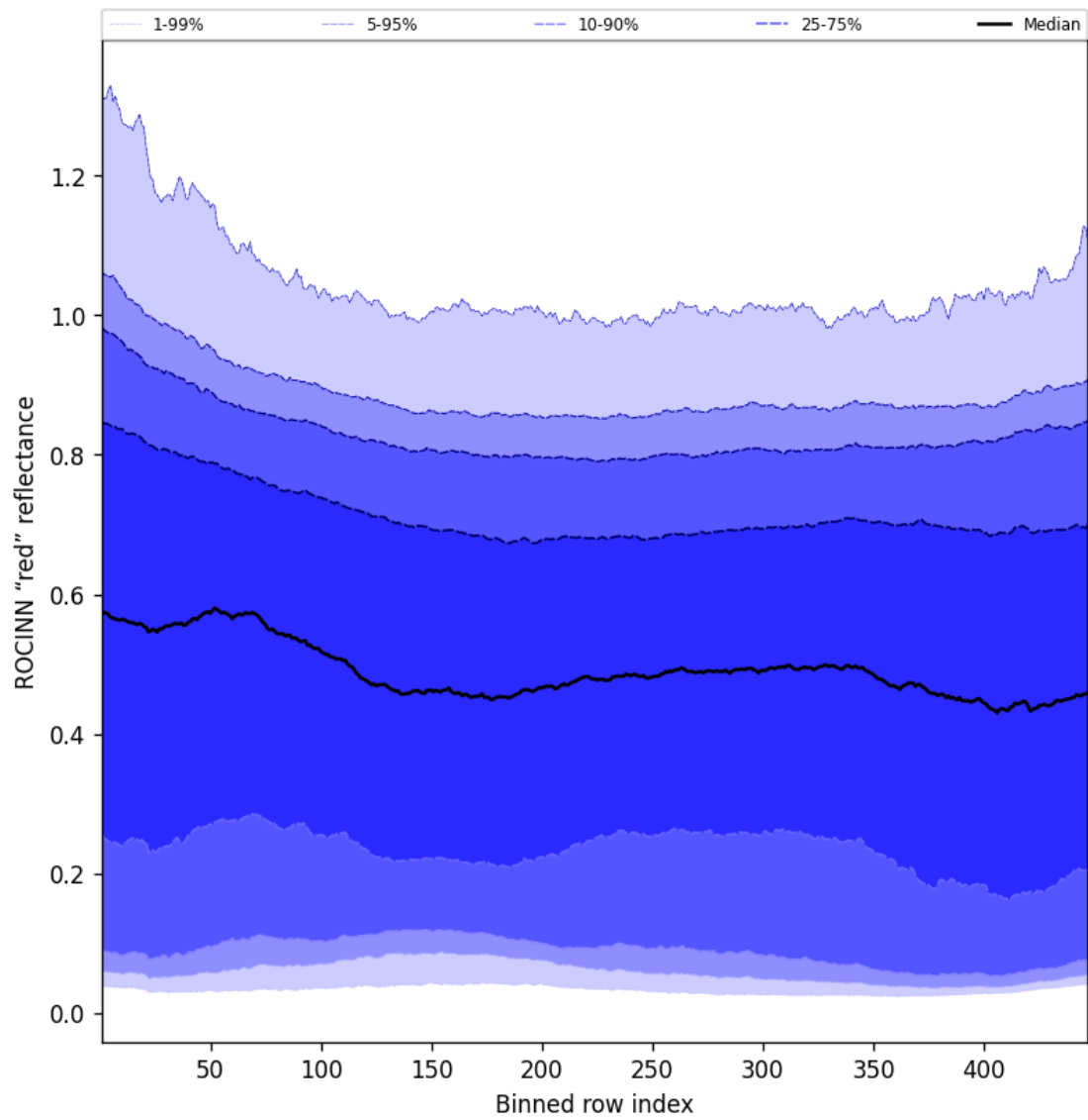
Figure 67: Along track statistics of “ROCINN “red” reflectance” for 2025-04-03 to 2025-04-04
