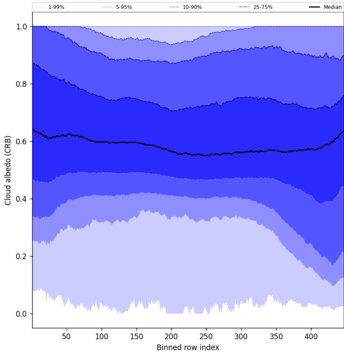
Figure 58: Along track statistics of “Cloud albedo (CRB)” for 2025-04-03 to 2025-04-04
