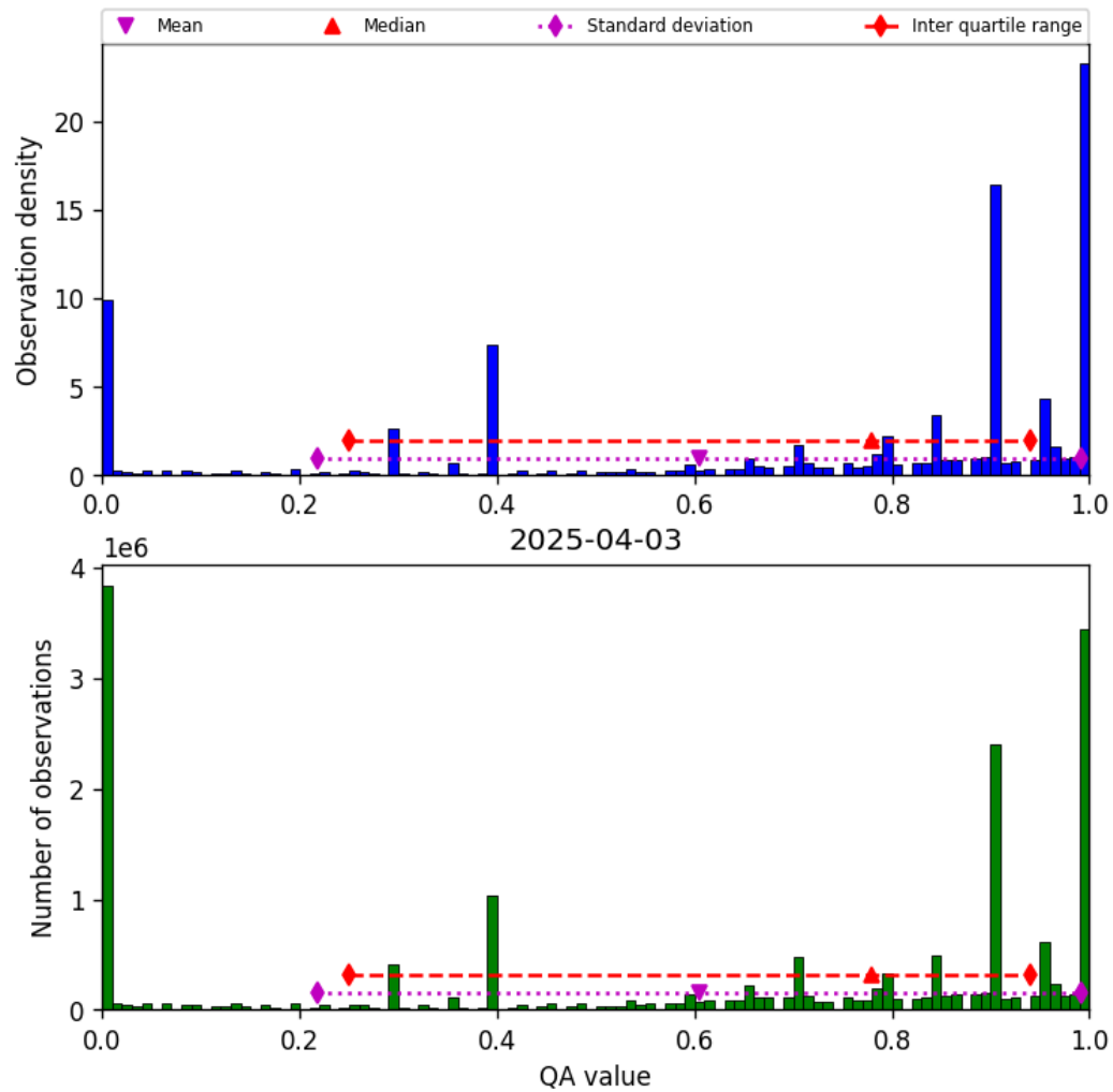
Figure 36: Histogram of “QA value” for 2025-04-03 to 2025-04-04
