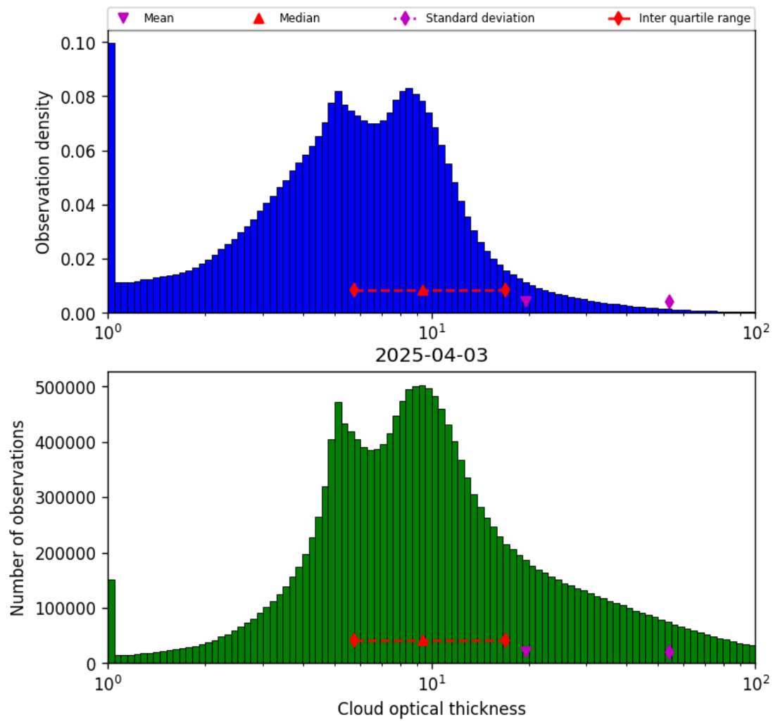
Figure 39: Histogram of “Cloud optical thickness” for 2025-04-03 to 2025-04-04
