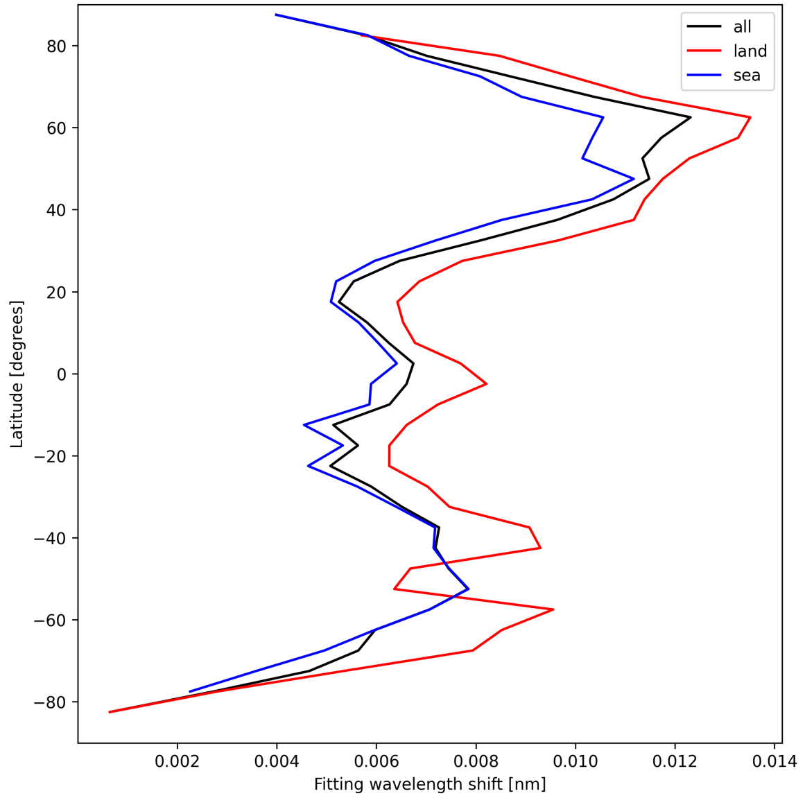
Figure 31: Zonal average of “Fitting wavelength shift” for 2025-04-03 to 2025-04-04.
