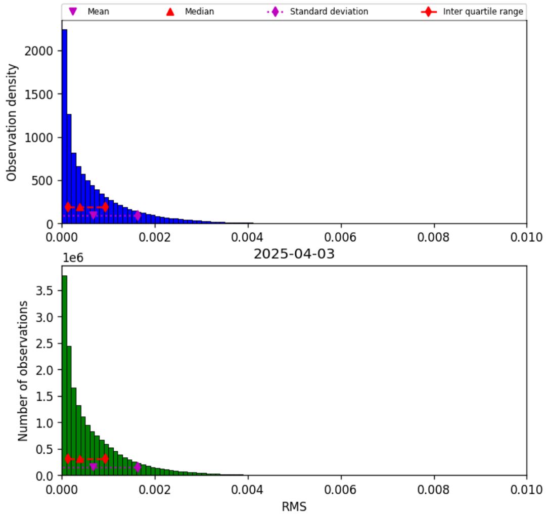
Figure 45: Histogram of “RMS” for 2025-04-03 to 2025-04-04
