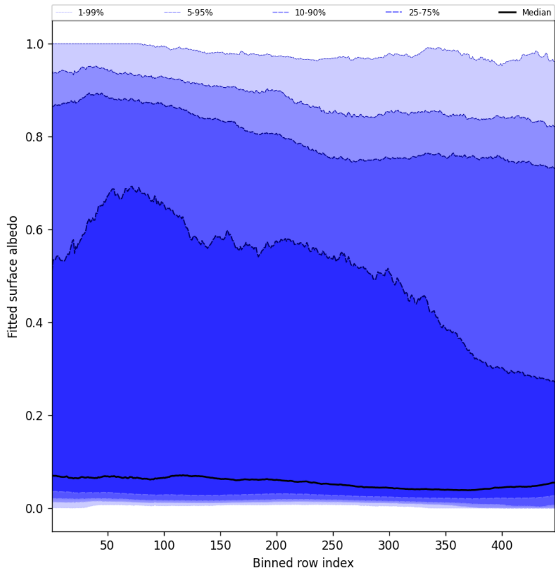
Figure 59: Along track statistics of “Fitted surface albedo” for 2025-04-03 to 2025-04-04
