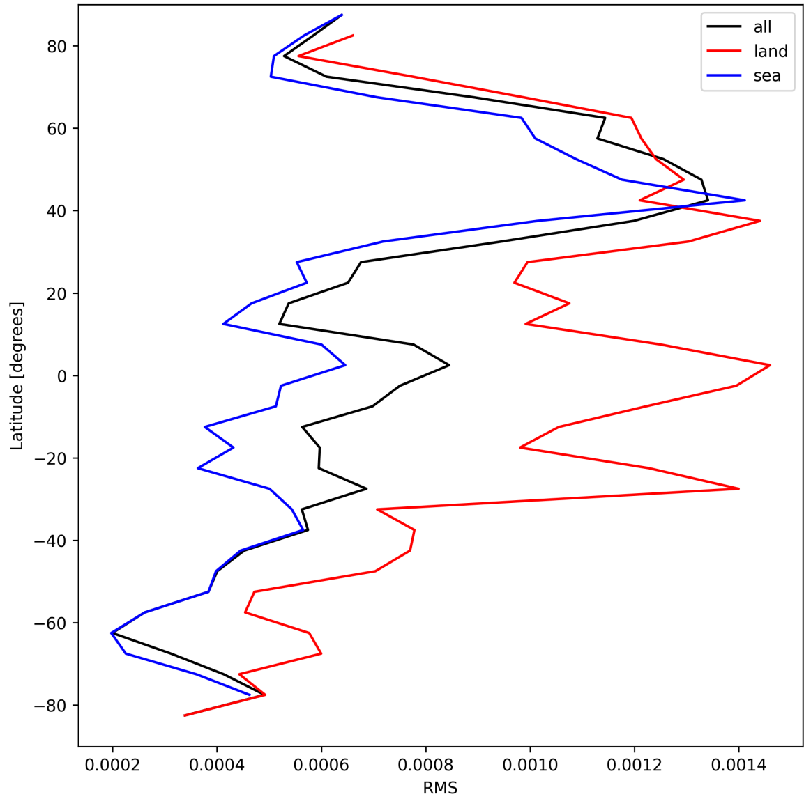
Figure 29: Zonal average of “RMS” for 2025-04-03 to 2025-04-04.
