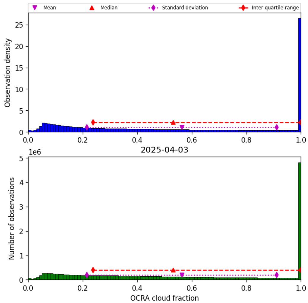
Figure 48: Histogram of “OCRA cloud fraction” for 2025-04-03 to 2025-04-04
