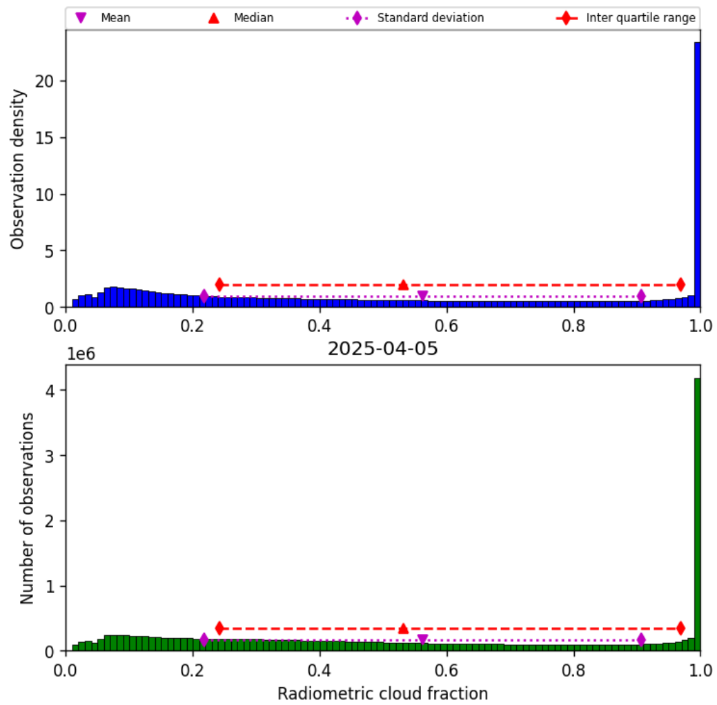
Figure 37: Histogram of “Radiometric cloud fraction” for 2025-04-05 to 2025-04-06
