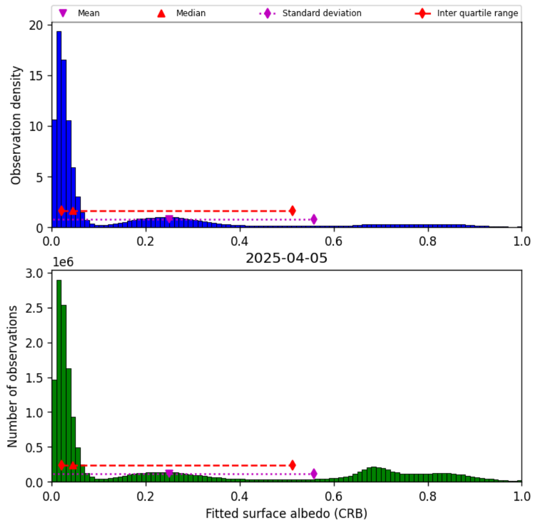
Figure 44: Histogram of “Fitted surface albedo (CRB)” for 2025-04-05 to 2025-04-06
