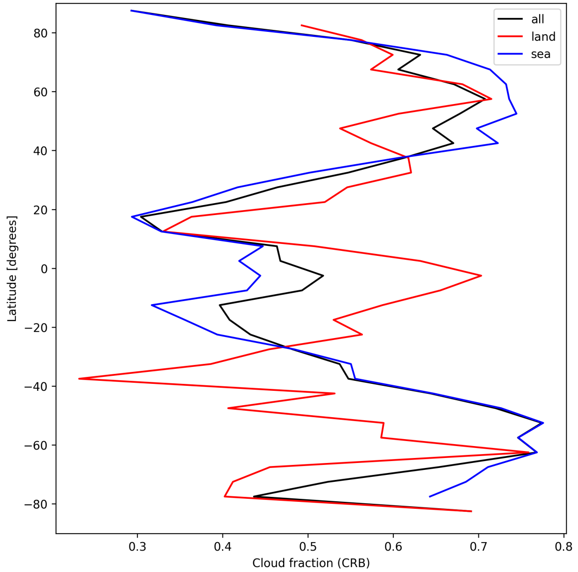
Figure 24: Zonal average of “Cloud fraction (CRB)” for 2025-04-05 to 2025-04-06.
