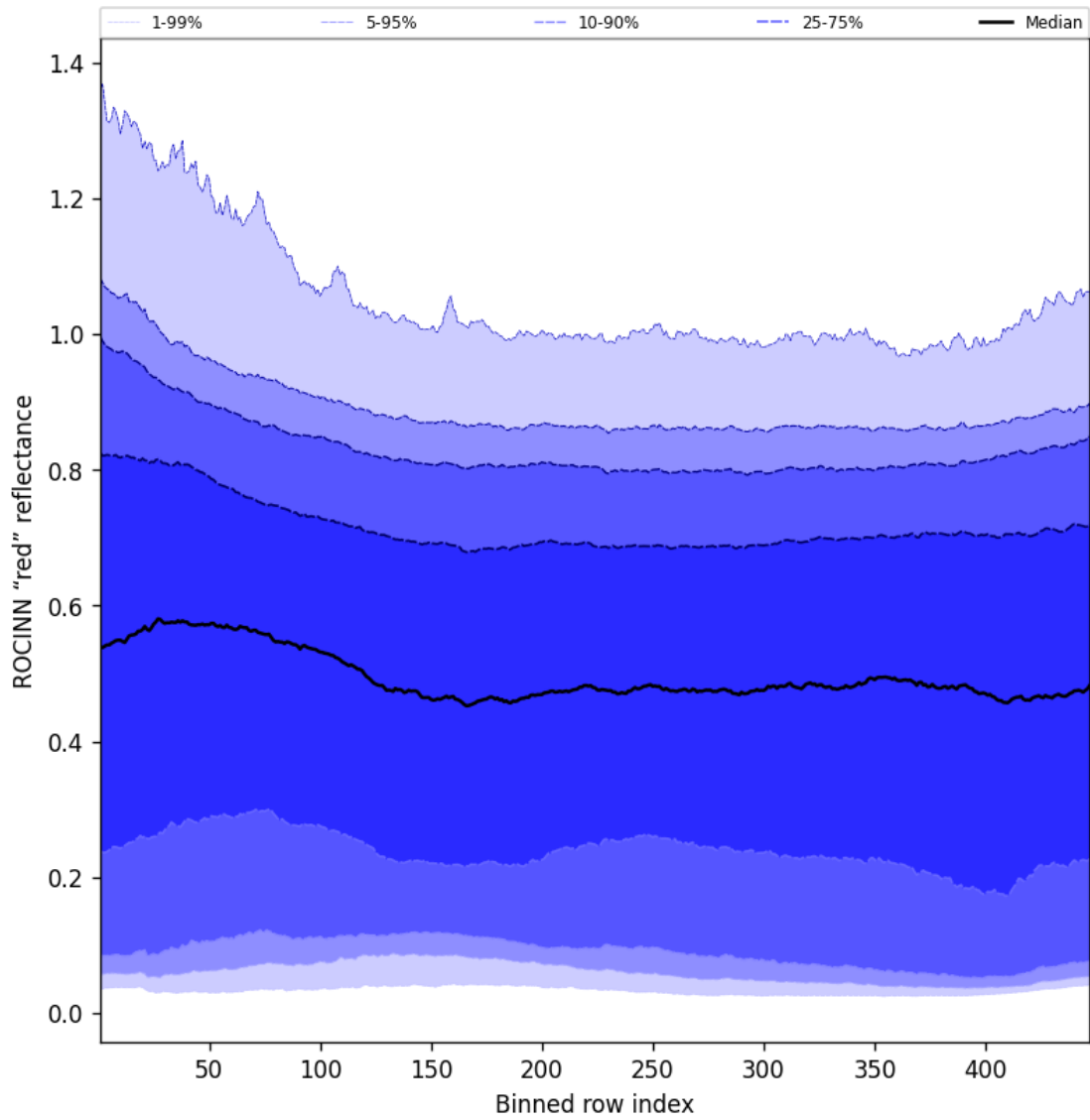
Figure 67: Along track statistics of “ROCINN “red” reflectance” for 2025-04-05 to 2025-04-06
