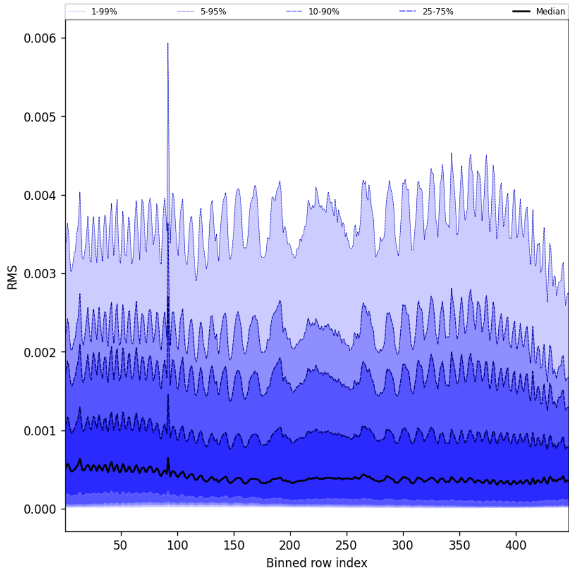
Figure 61: Along track statistics of “RMS” for 2025-04-05 to 2025-04-06
