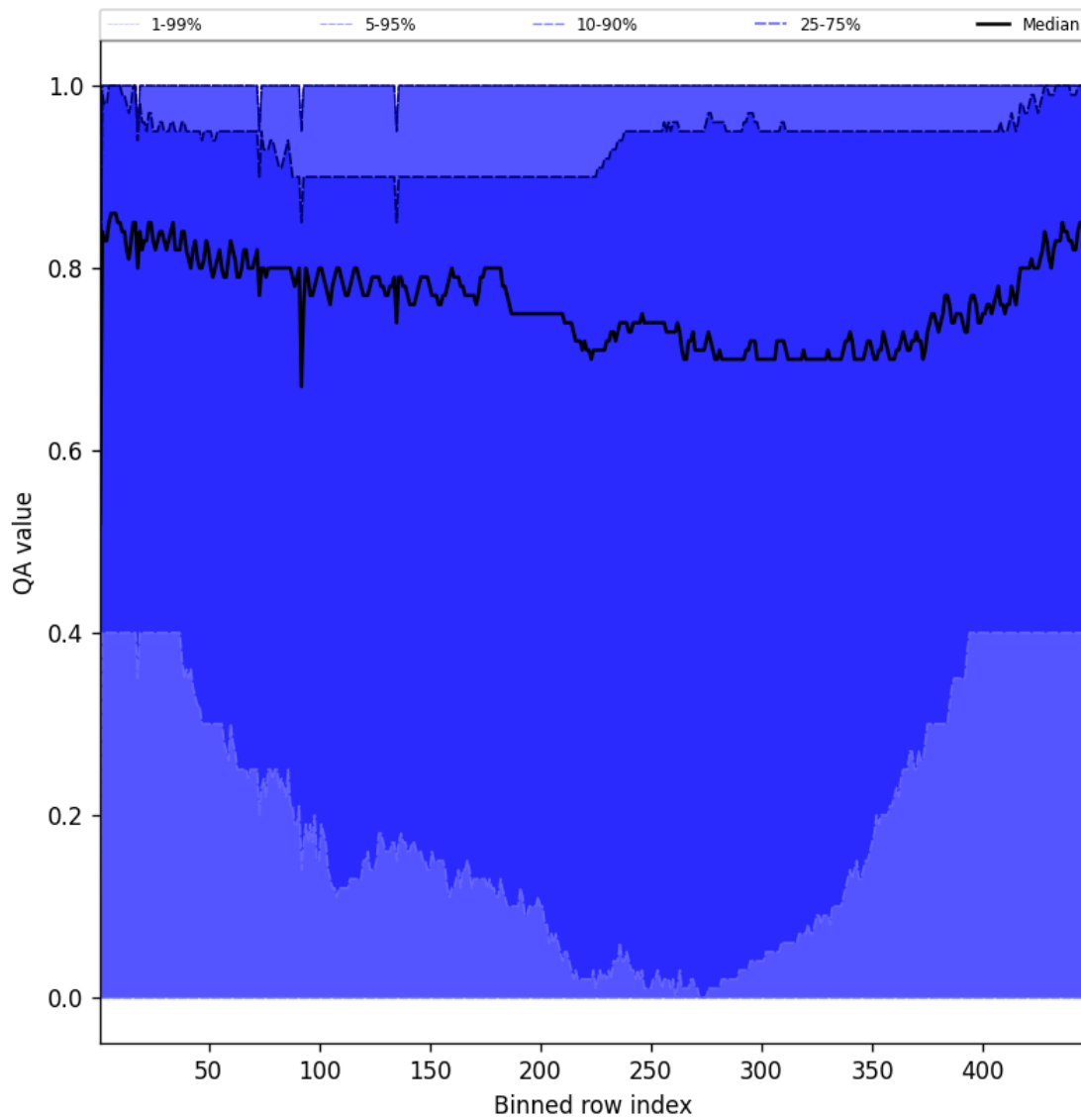
Figure 52: Along track statistics of “QA value” for 2025-04-05 to 2025-04-06
