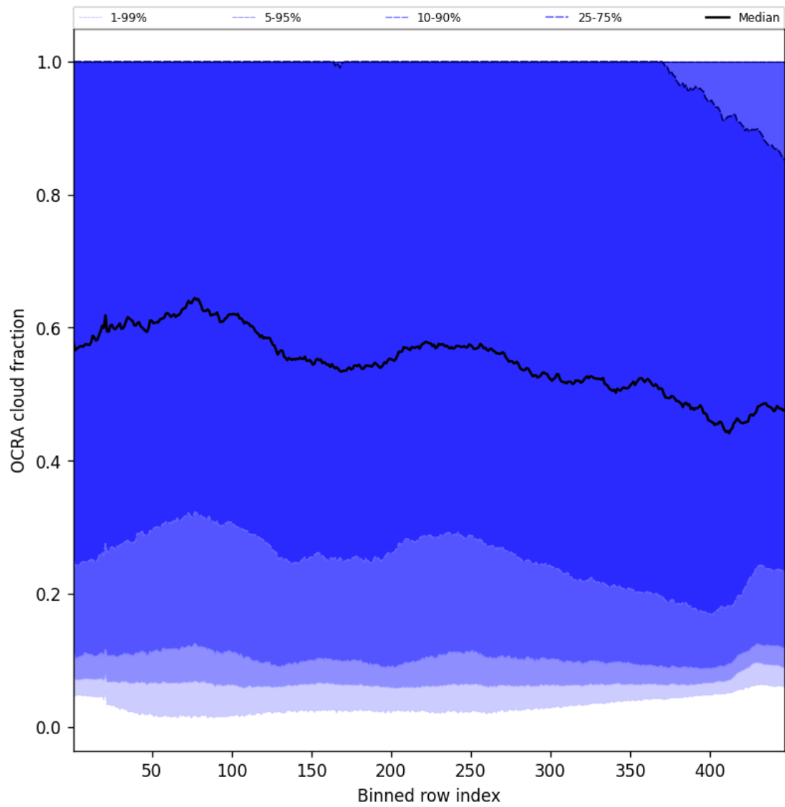
Figure 64: Along track statistics of “OCRA cloud fraction” for 2025-04-05 to 2025-04-06
