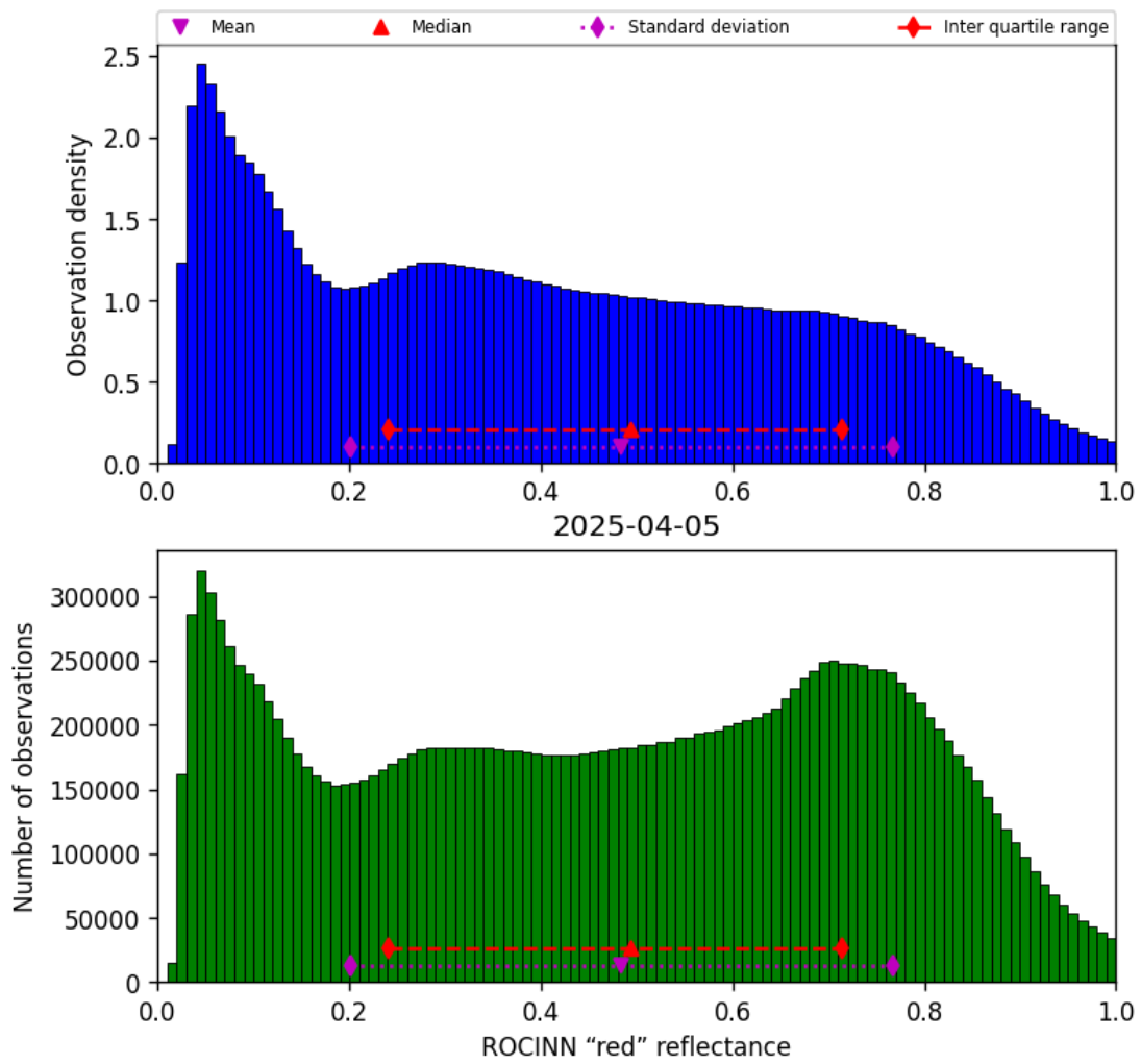
Figure 51: Histogram of “ROCINN “red” reflectance” for 2025-04-05 to 2025-04-06
