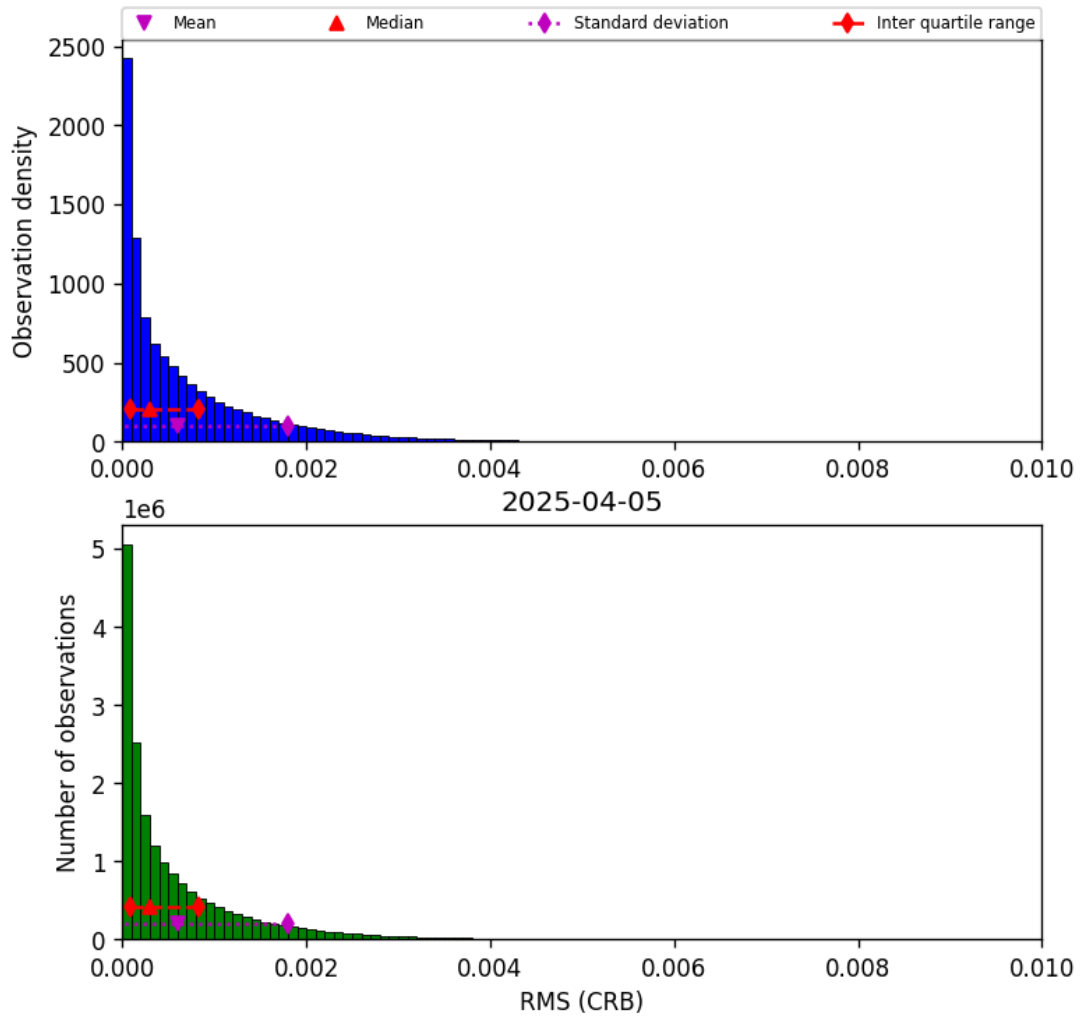
Figure 46: Histogram of “RMS (CRB)” for 2025-04-05 to 2025-04-06
