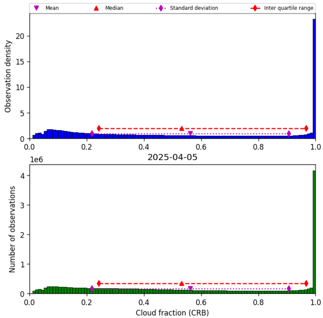
Figure 40: Histogram of “Cloud fraction (CRB)” for 2025-04-05 to 2025-04-06
