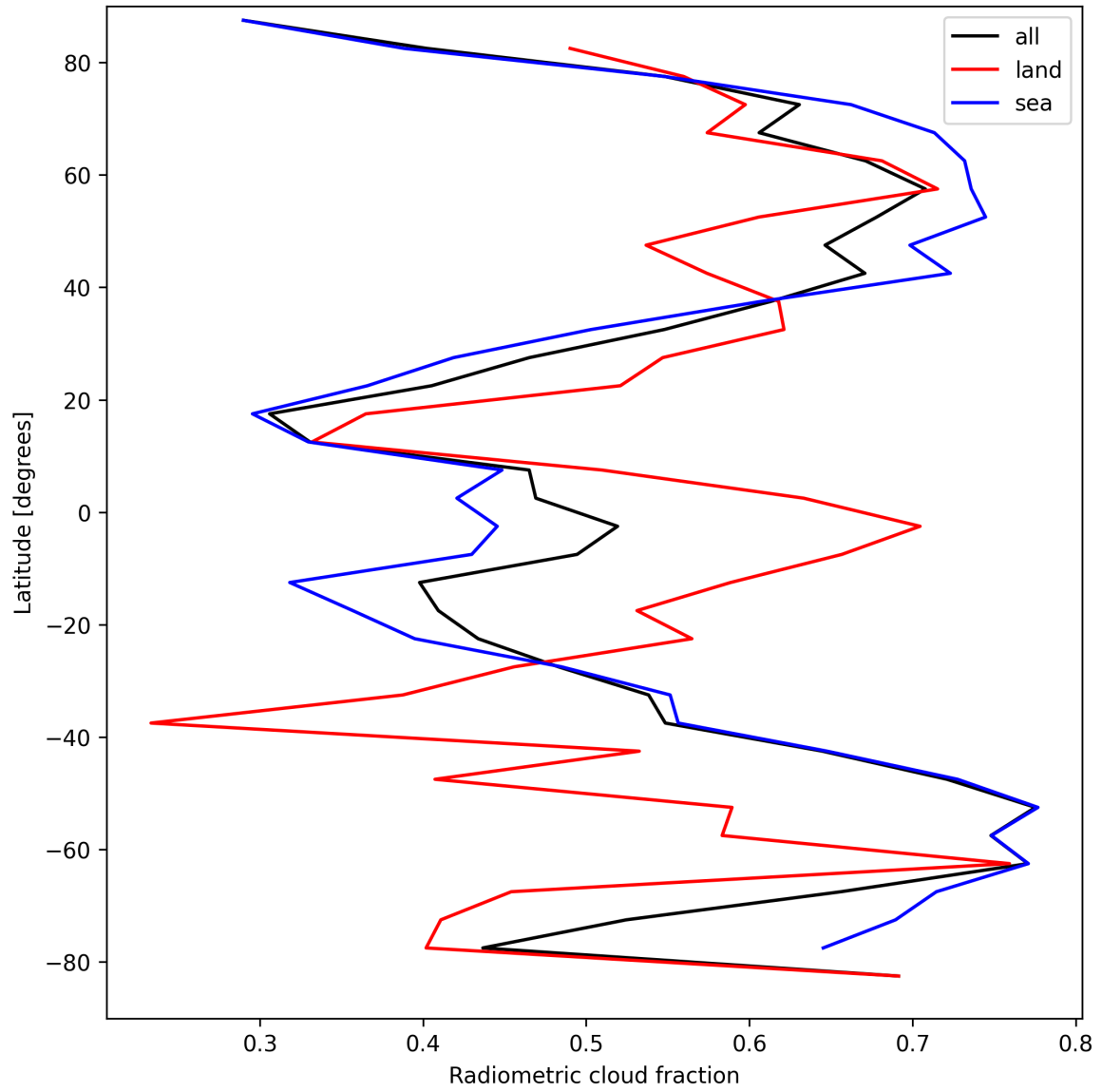
Figure 21: Zonal average of “Radiometric cloud fraction” for 2025-04-05 to 2025-04-06.
