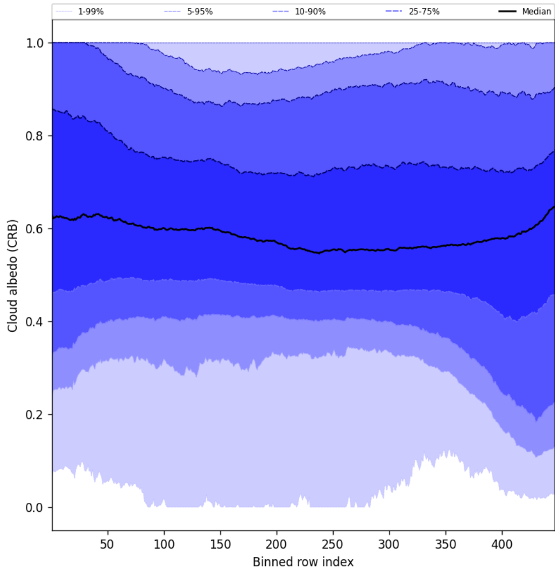
Figure 58: Along track statistics of “Cloud albedo (CRB)” for 2025-04-05 to 2025-04-06
