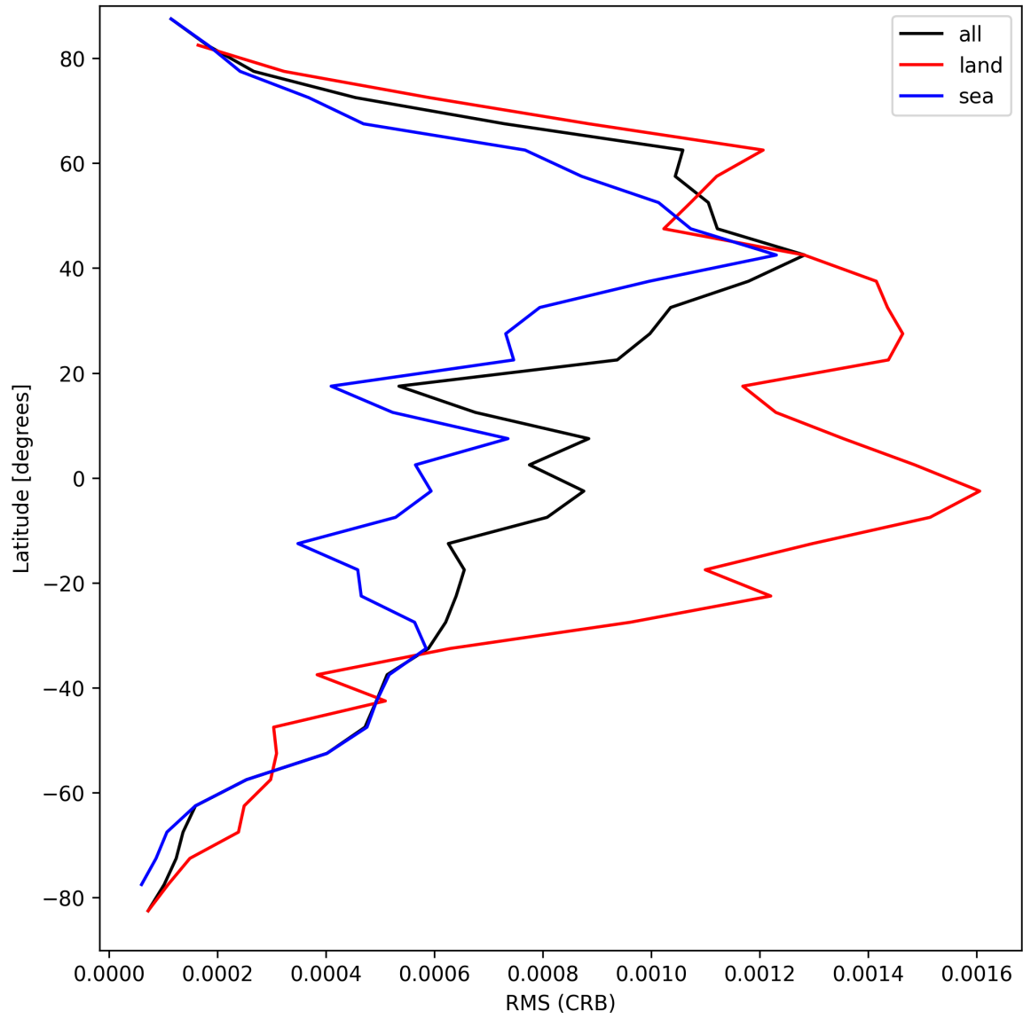
Figure 30: Zonal average of “RMS (CRB)” for 2025-04-05 to 2025-04-06.
