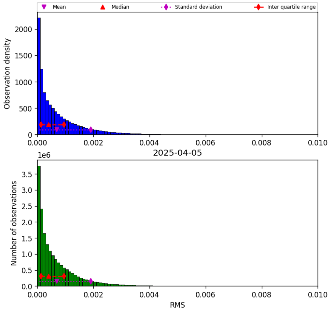
Figure 45: Histogram of “RMS” for 2025-04-05 to 2025-04-06
