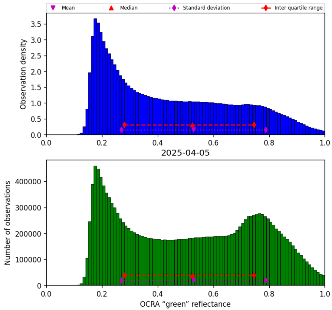
Figure 50: Histogram of “OCRA “green” reflectance” for 2025-04-05 to 2025-04-06
