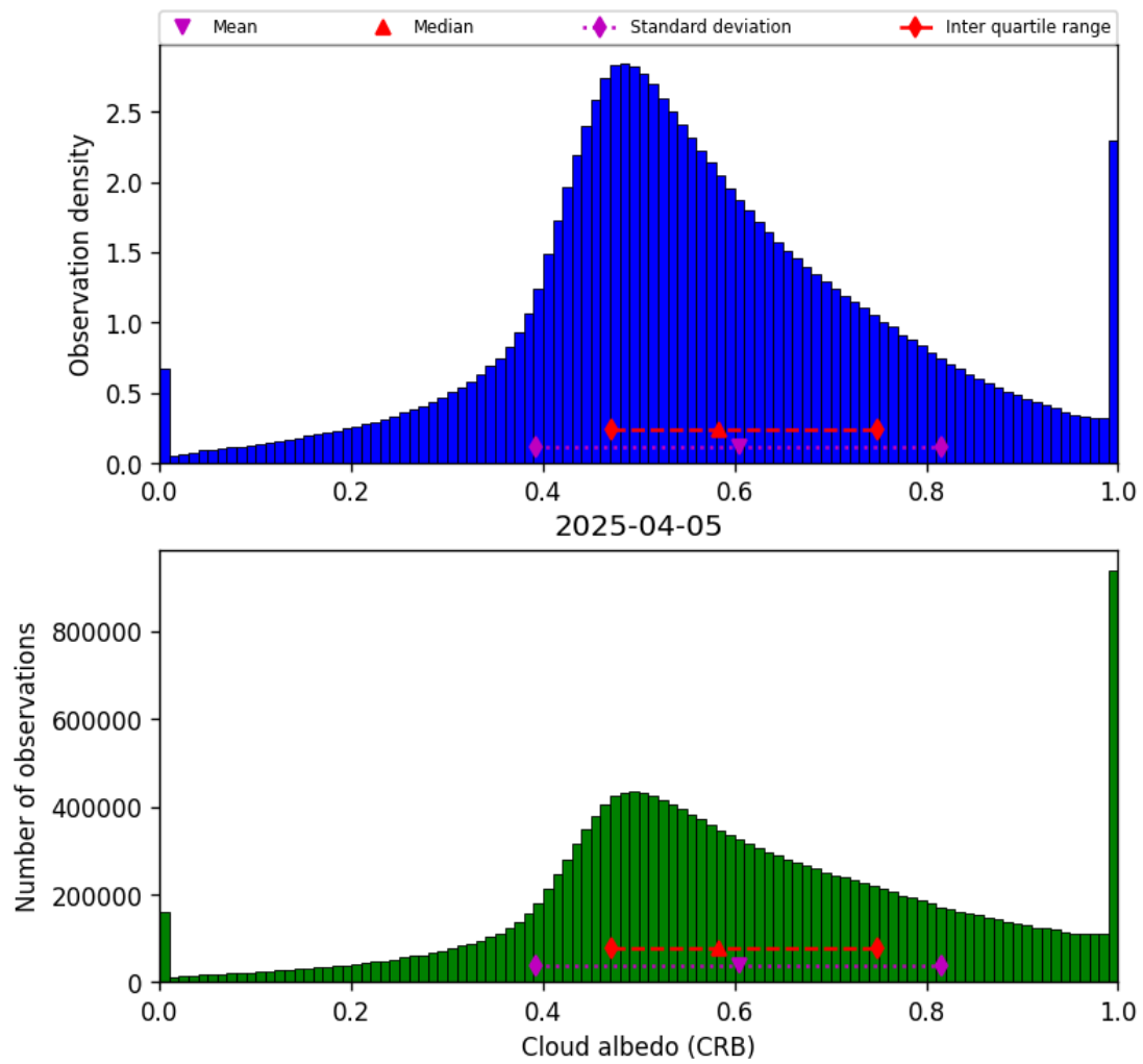
Figure 42: Histogram of “Cloud albedo (CRB)” for 2025-04-05 to 2025-04-06
