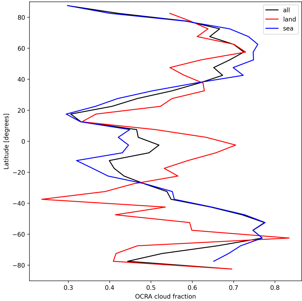
Figure 32: Zonal average of “OCRA cloud fraction” for 2025-04-05 to 2025-04-06.
