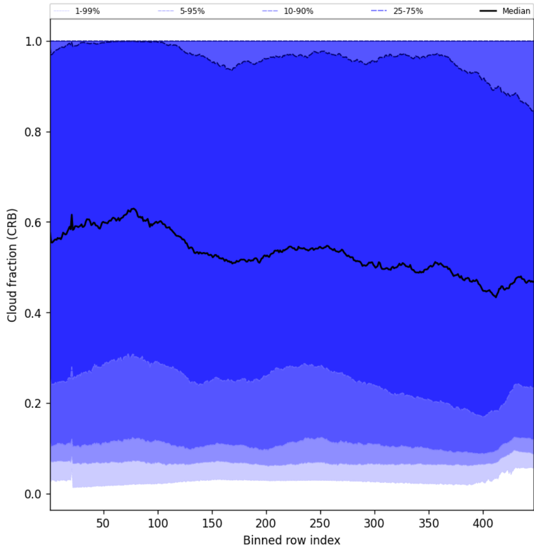
Figure 56: Along track statistics of “Cloud fraction (CRB)” for 2025-04-05 to 2025-04-06
