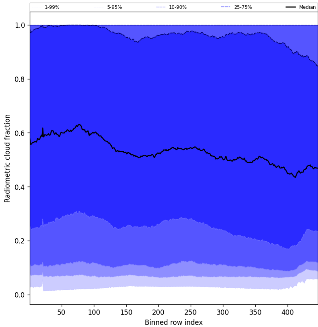
Figure 53: Along track statistics of “Radiometric cloud fraction” for 2025-04-05 to 2025-04-06
