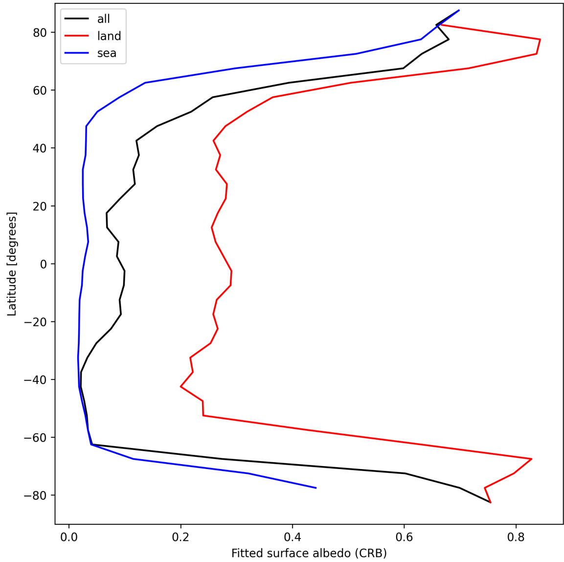
Figure 28: Zonal average of “Fitted surface albedo (CRB)” for 2025-04-05 to 2025-04-06.
