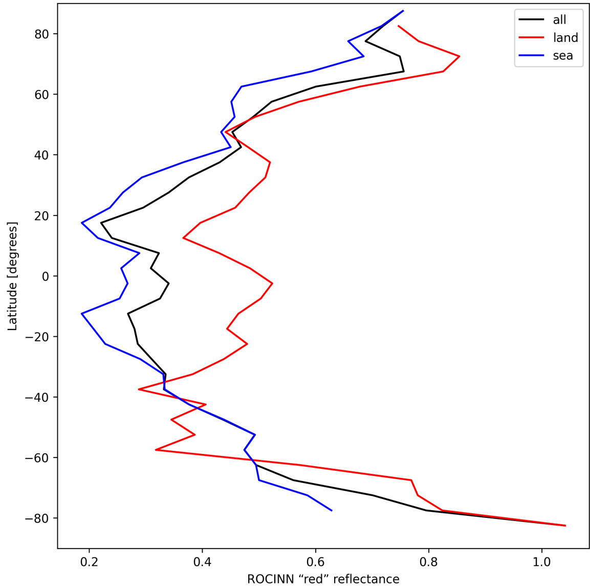
Figure 35: Zonal average of "ROCINN "red" reflectance" for 2025-04-05 to 2025-04-06.
