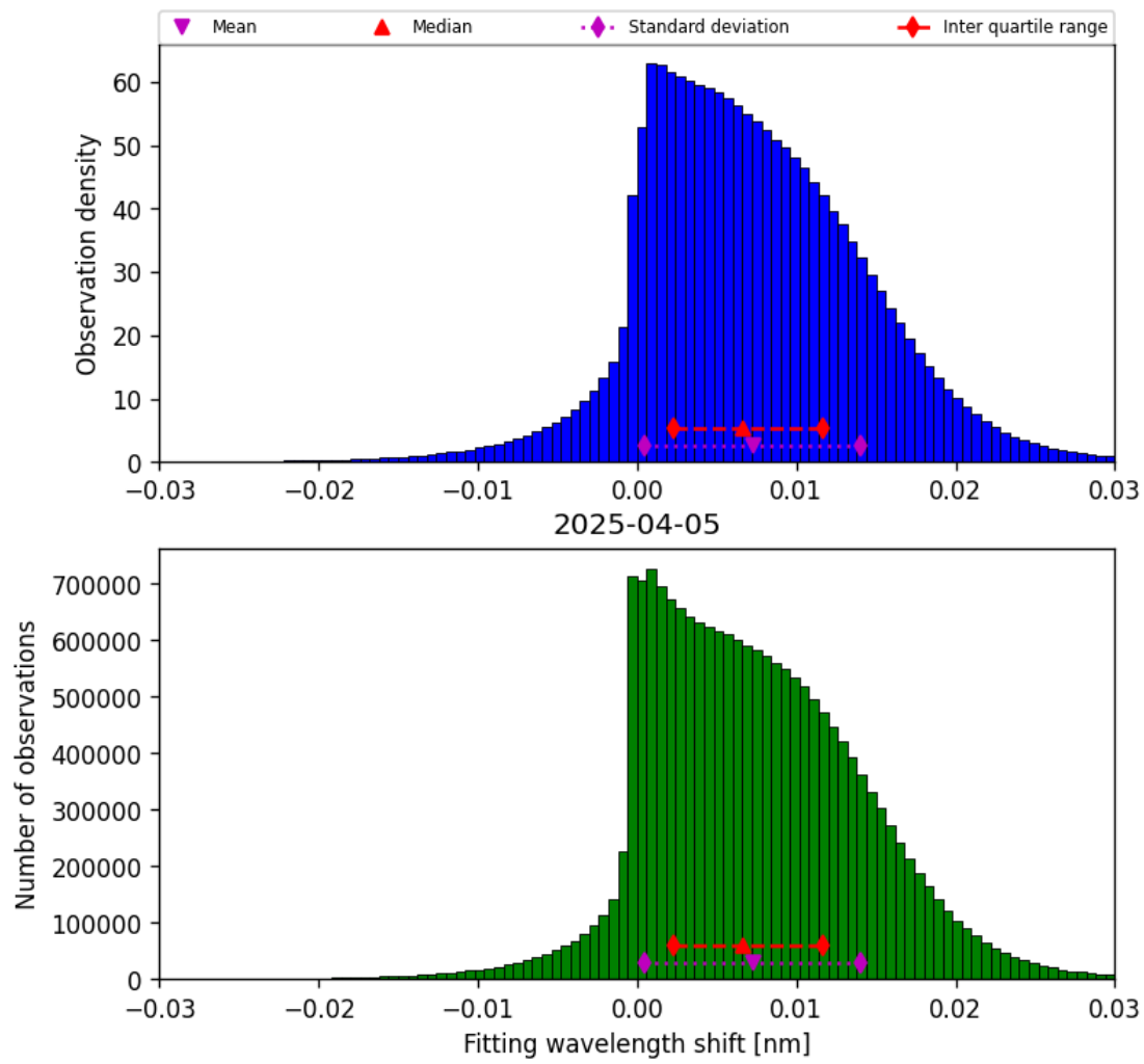
Figure 47: Histogram of “Fitting wavelength shift” for 2025-04-05 to 2025-04-06
