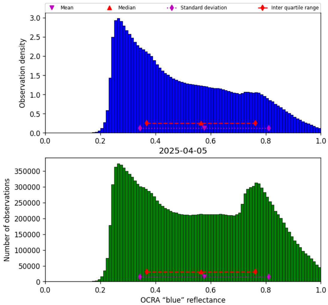
Figure 49: Histogram of “OCRA “blue” reflectance” for 2025-04-05 to 2025-04-06
