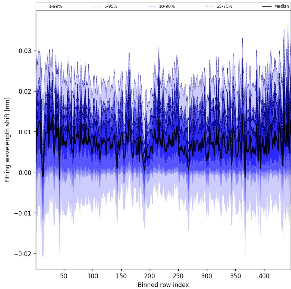
Figure 63: Along track statistics of “Fitting wavelength shift” for 2025-04-05 to 2025-04-06
