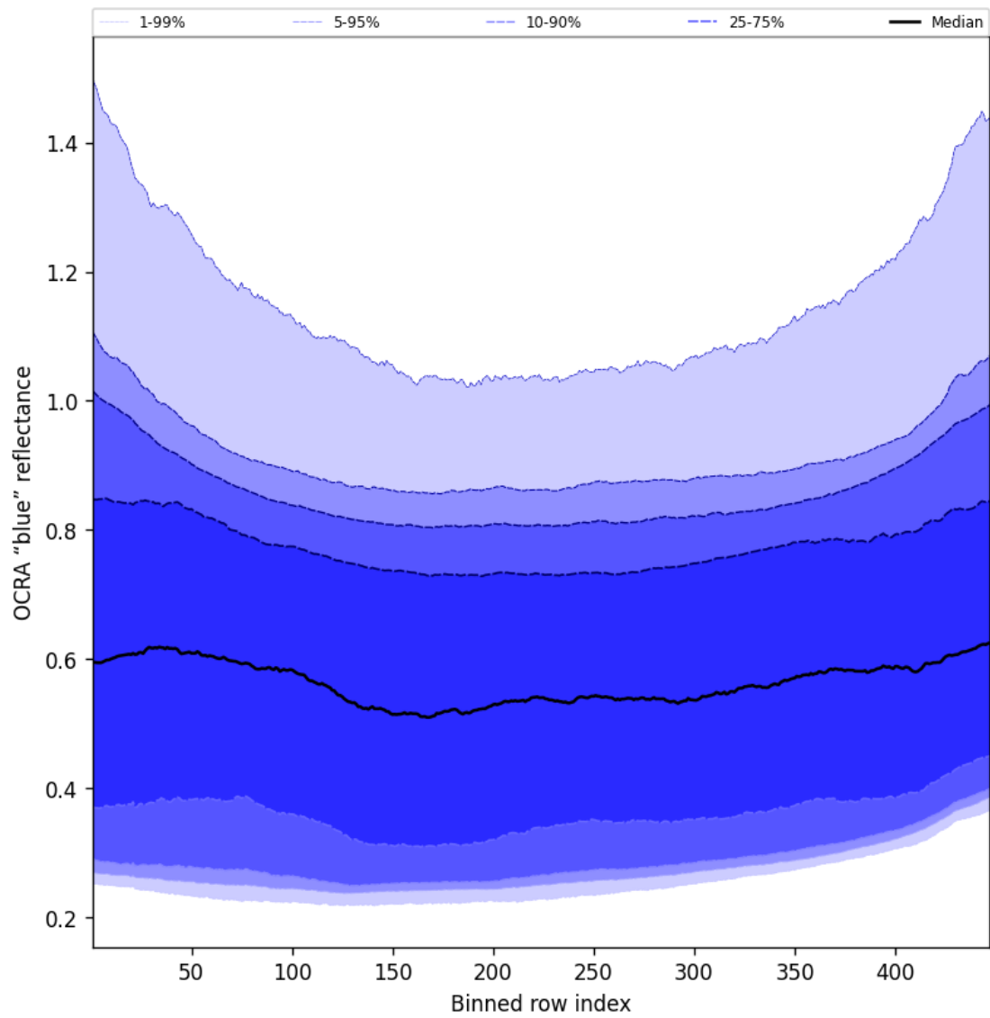
Figure 65: Along track statistics of “OCRA “blue” reflectance” for 2025-04-05 to 2025-04-06
