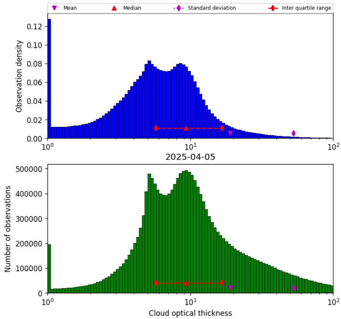
Figure 39: Histogram of “Cloud optical thickness” for 2025-04-05 to 2025-04-06
