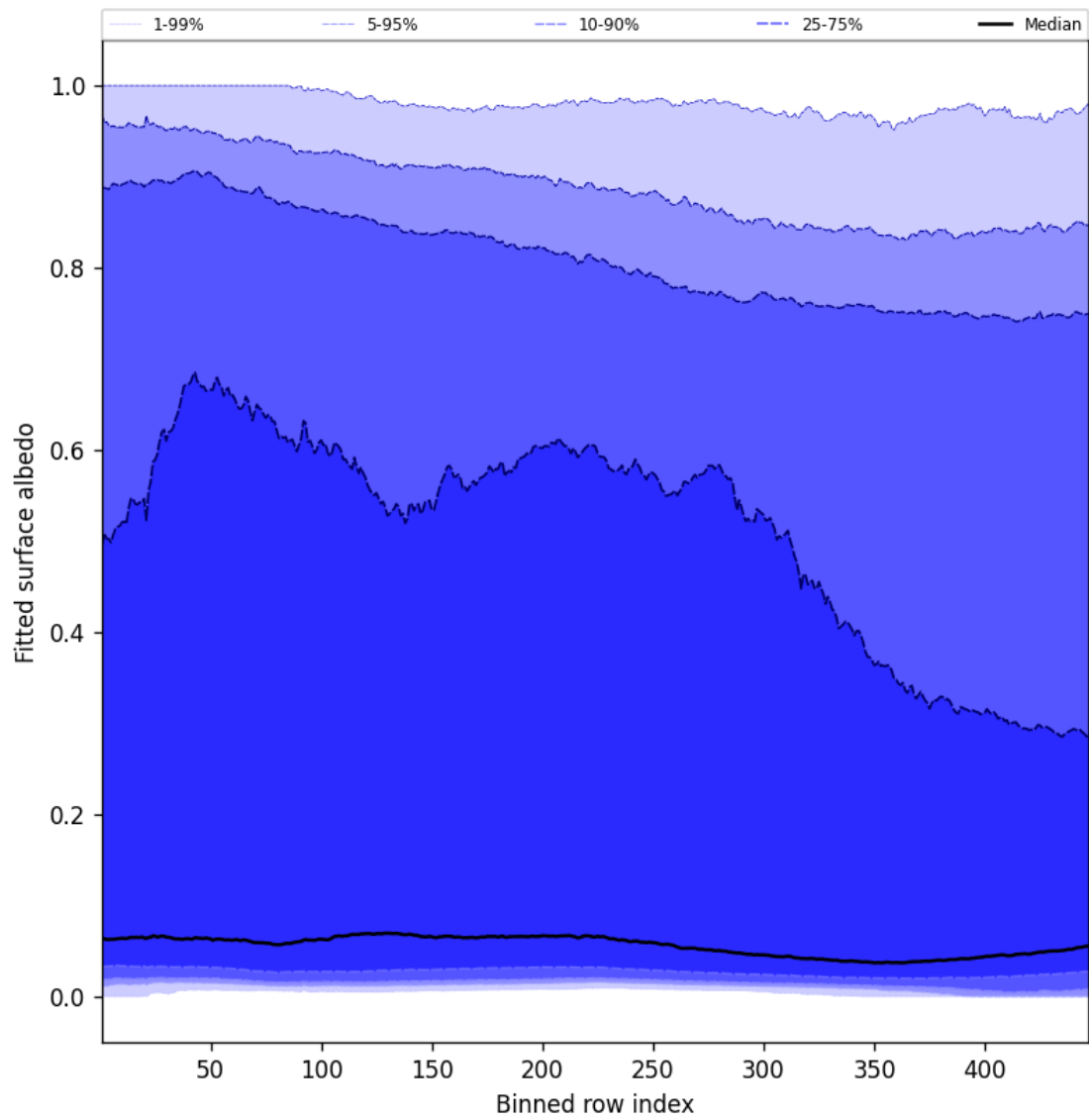
Figure 59: Along track statistics of “Fitted surface albedo” for 2025-04-05 to 2025-04-06
