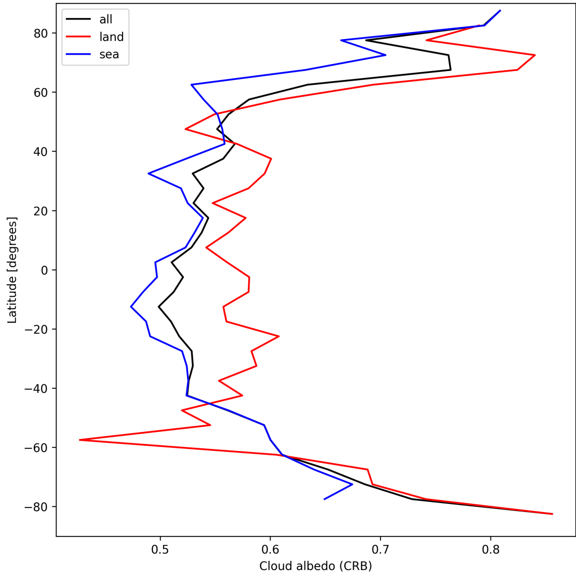
Figure 26: Zonal average of “Cloud albedo (CRB)” for 2025-04-05 to 2025-04-06.
