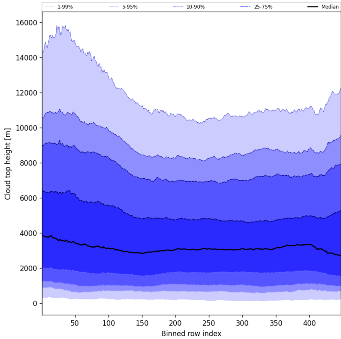
Figure 54: Along track statistics of “Cloud top height” for 2025-04-05 to 2025-04-06
