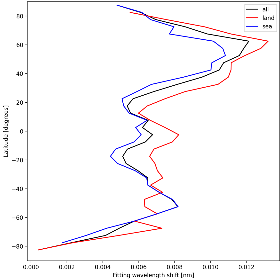
Figure 31: Zonal average of “Fitting wavelength shift” for 2025-04-05 to 2025-04-06.
