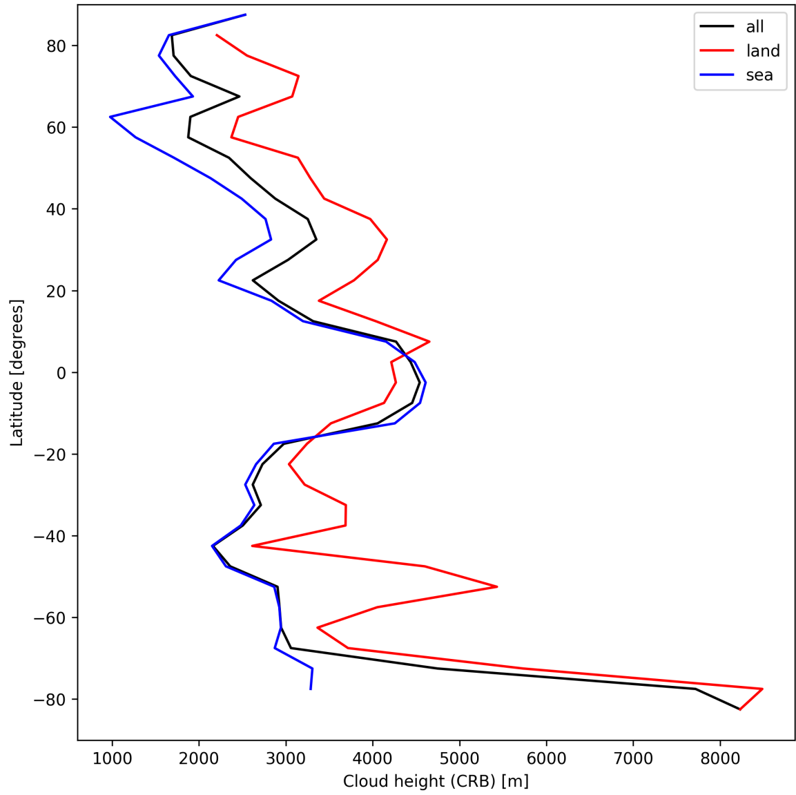
Figure 25: Zonal average of “Cloud height (CRB)” for 2025-04-05 to 2025-04-06.
