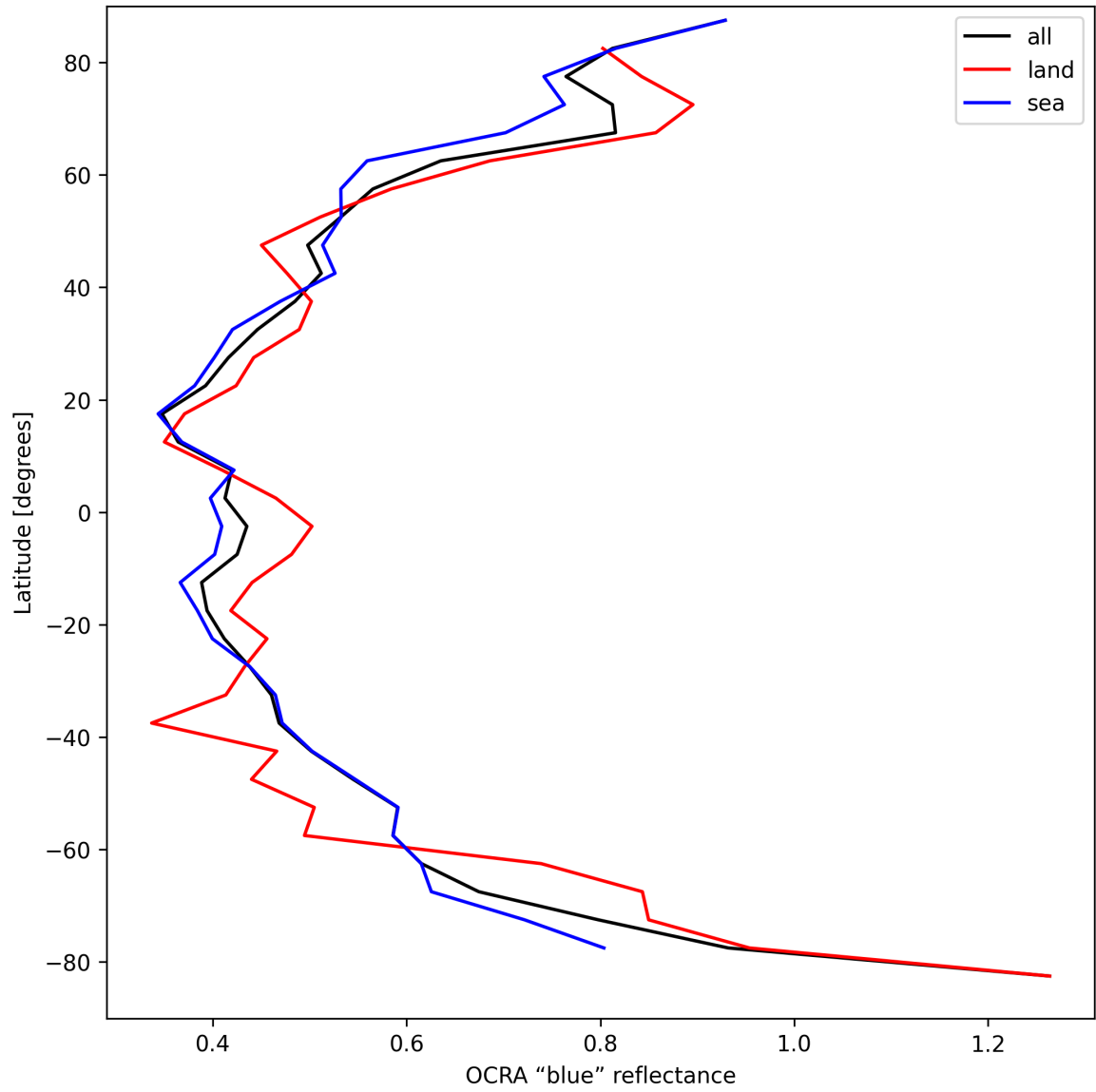
Figure 33: Zonal average of “OCRA “blue” reflectance” for 2025-04-05 to 2025-04-06.
