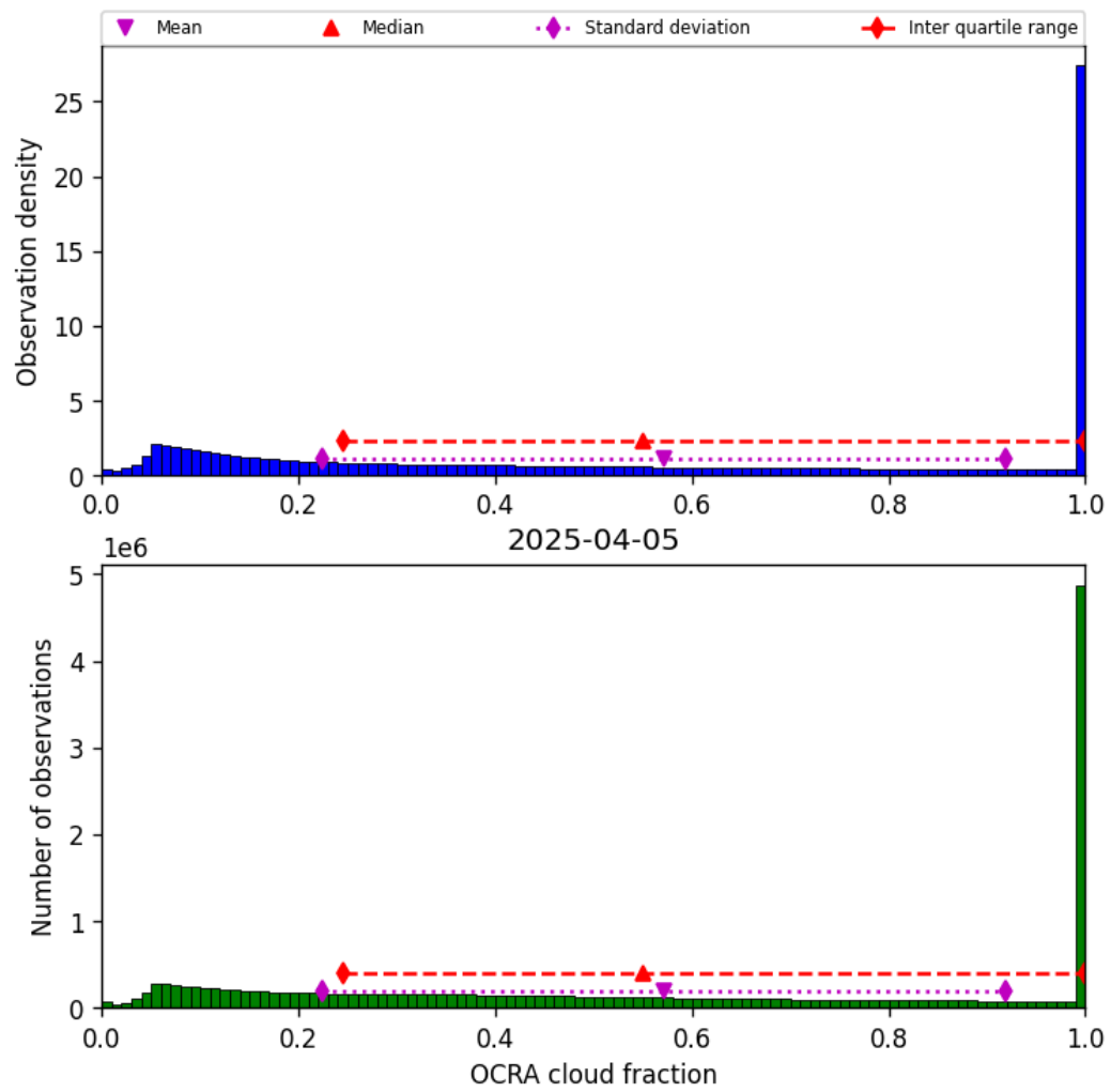
Figure 48: Histogram of “OCRA cloud fraction” for 2025-04-05 to 2025-04-06
