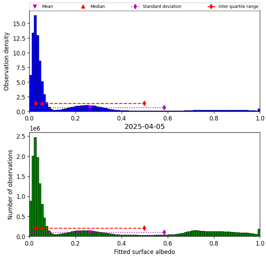
Figure 43: Histogram of “Fitted surface albedo” for 2025-04-05 to 2025-04-06
