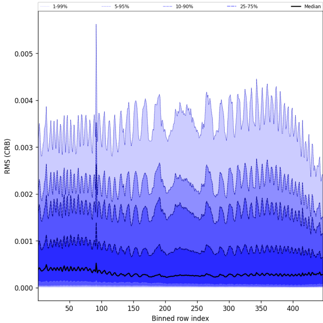
Figure 62: Along track statistics of “RMS (CRB)” for 2025-04-05 to 2025-04-06
