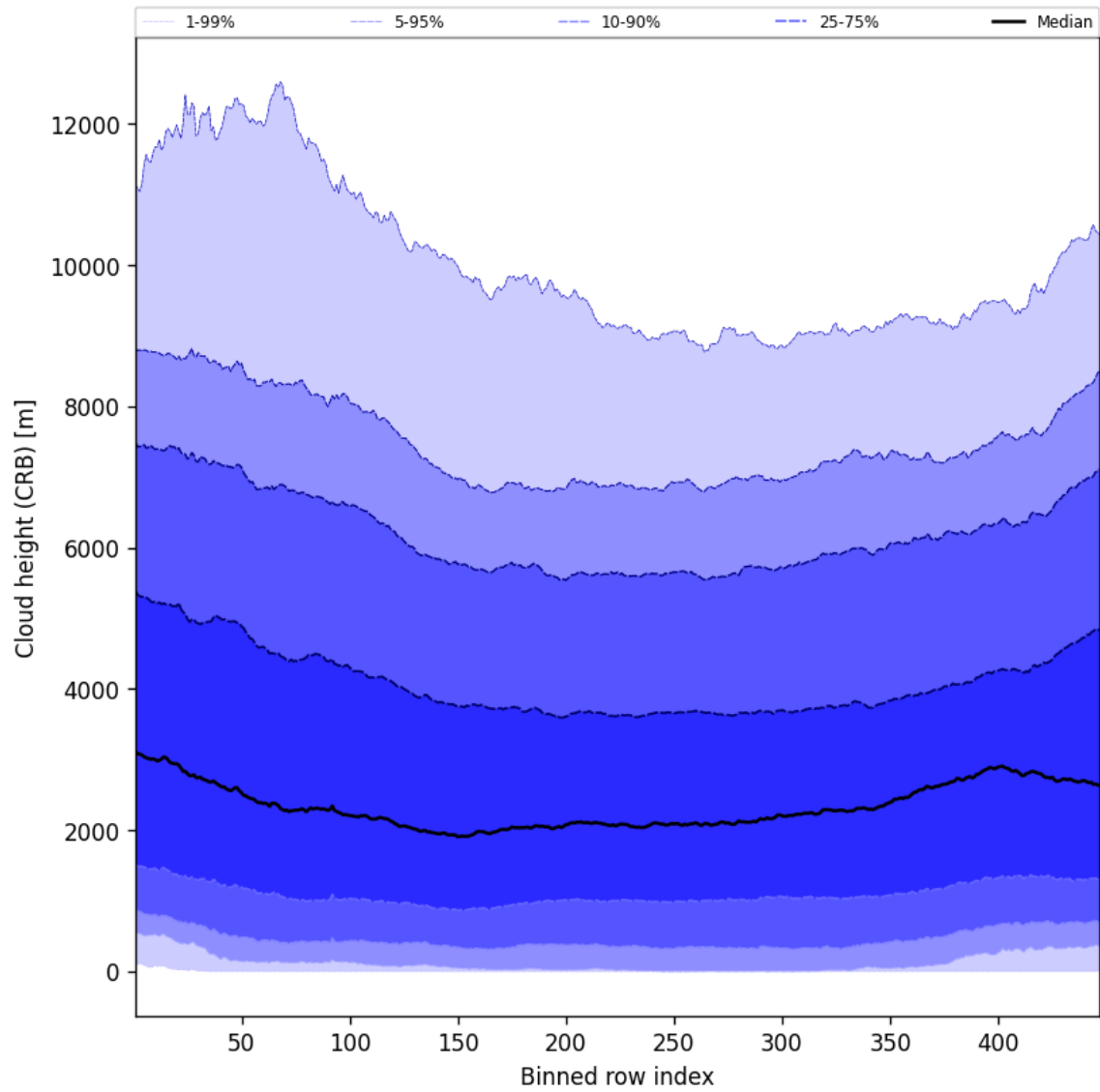
Figure 57: Along track statistics of “Cloud height (CRB)” for 2025-04-05 to 2025-04-06
