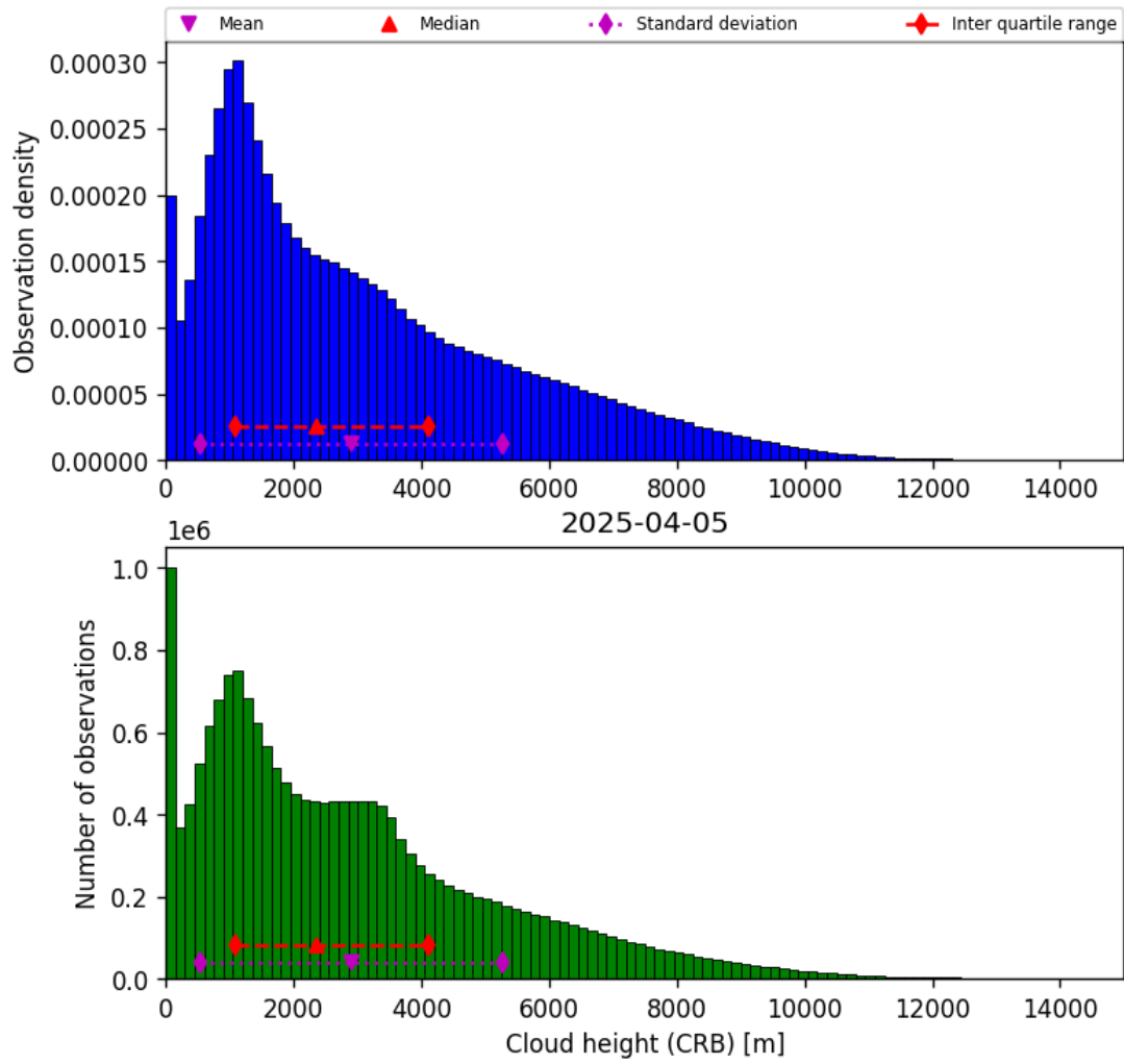
Figure 41: Histogram of “Cloud height (CRB)” for 2025-04-05 to 2025-04-06
