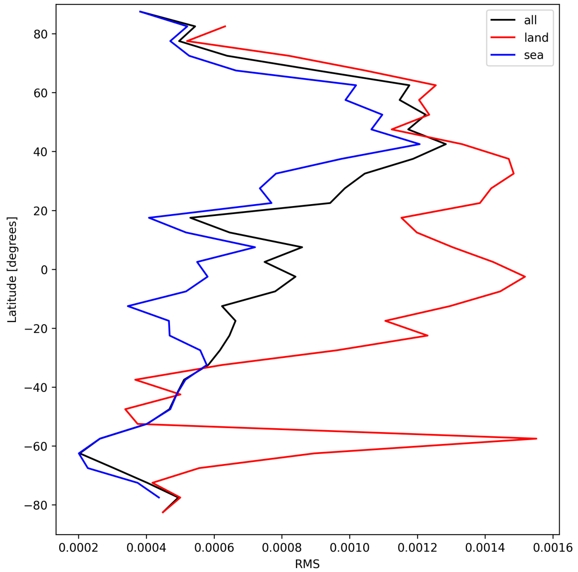
Figure 29: Zonal average of “RMS” for 2025-04-05 to 2025-04-06.
