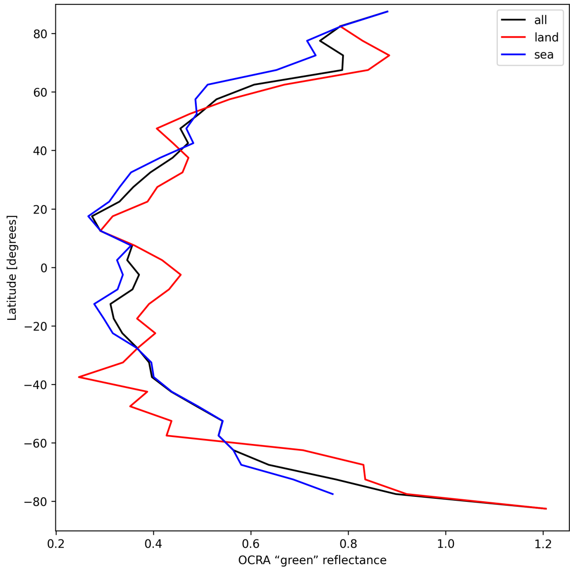
Figure 34: Zonal average of “OCRA “green” reflectance” for 2025-04-05 to 2025-04-06.
