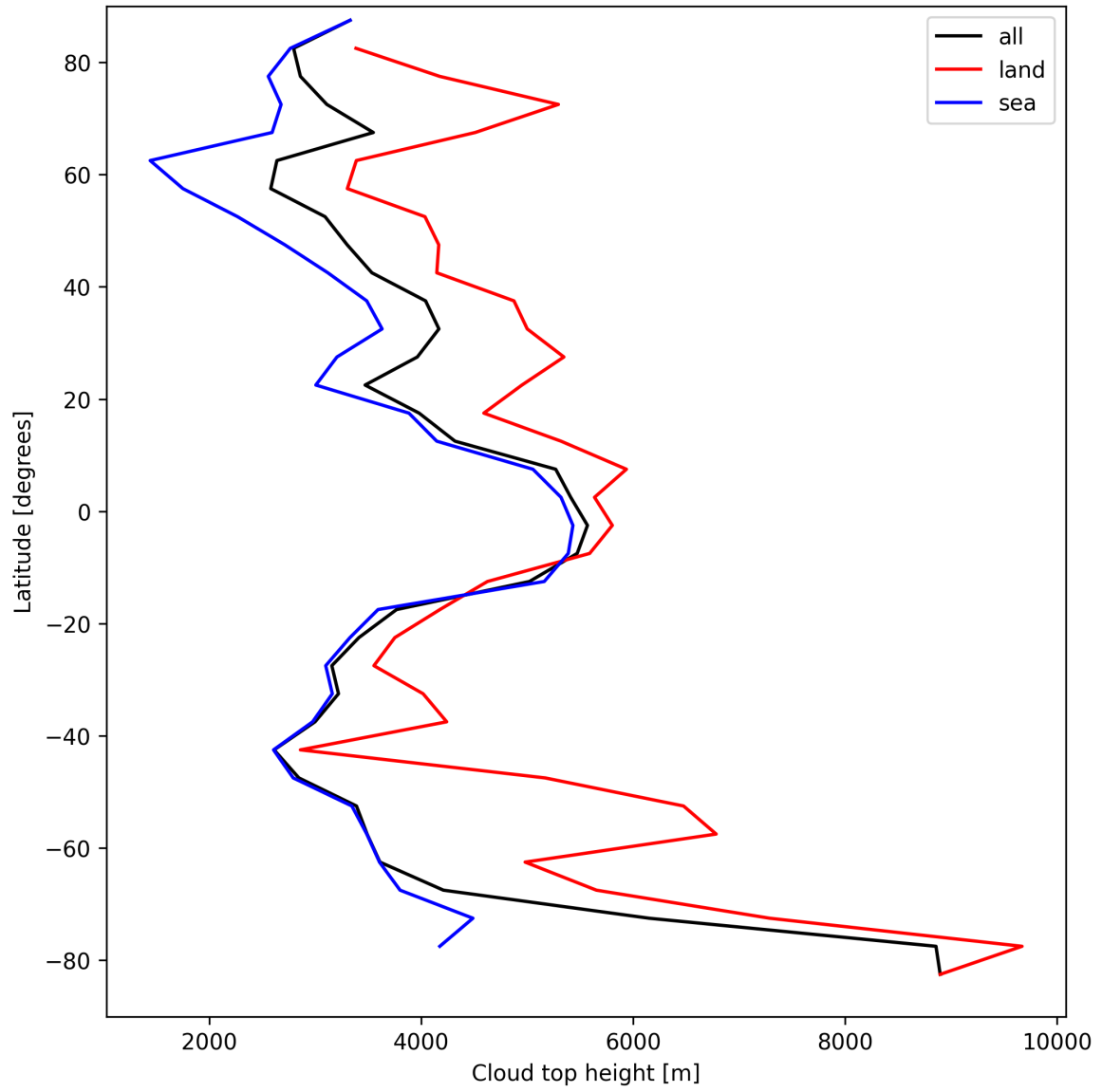
Figure 22: Zonal average of “Cloud top height” for 2025-04-05 to 2025-04-06.
