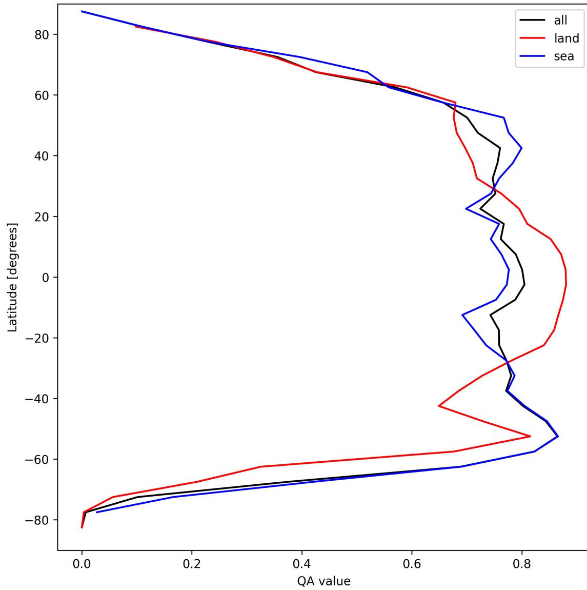
Figure 20: Zonal average of “QA value” for 2025-04-05 to 2025-04-06.
