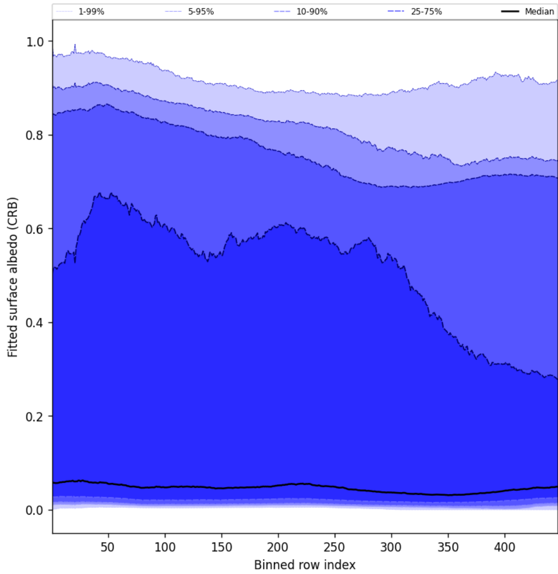
Figure 60: Along track statistics of “Fitted surface albedo (CRB)” for 2025-04-05 to 2025-04-06
