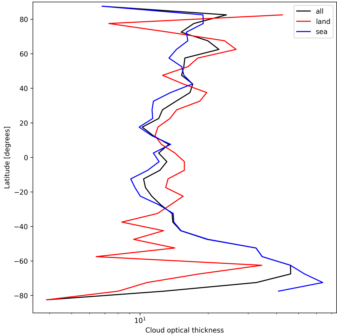
Figure 23: Zonal average of “Cloud optical thickness” for 2025-04-05 to 2025-04-06.
