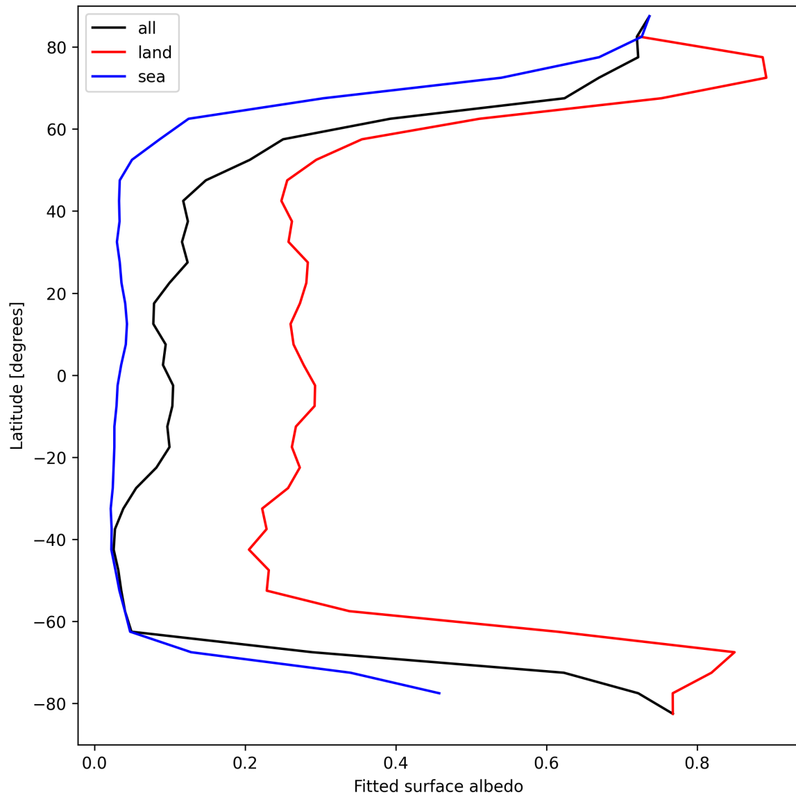
Figure 27: Zonal average of “Fitted surface albedo” for 2025-04-05 to 2025-04-06.
