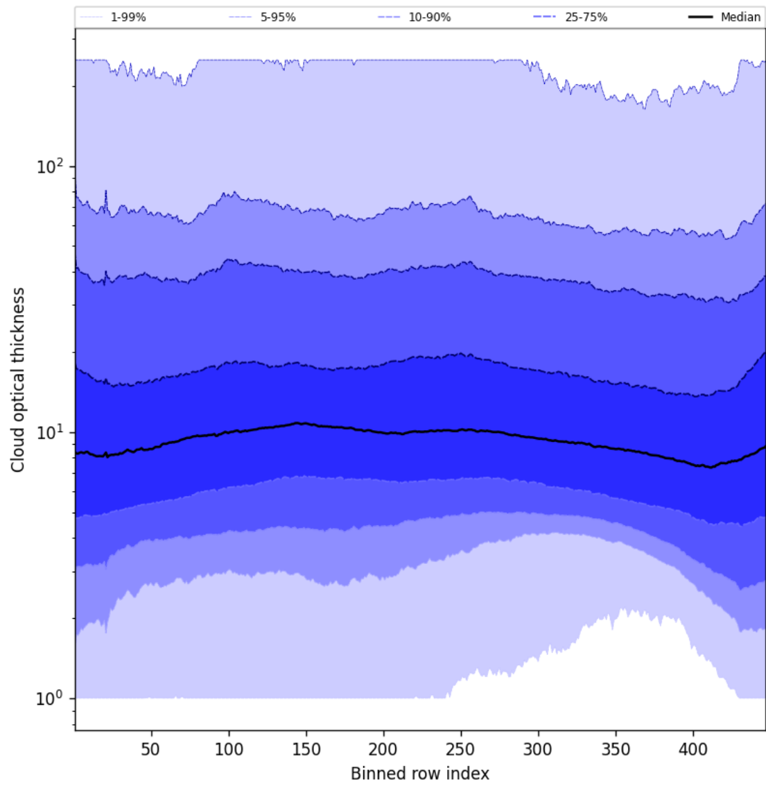
Figure 55: Along track statistics of “Cloud optical thickness” for 2025-04-05 to 2025-04-06
