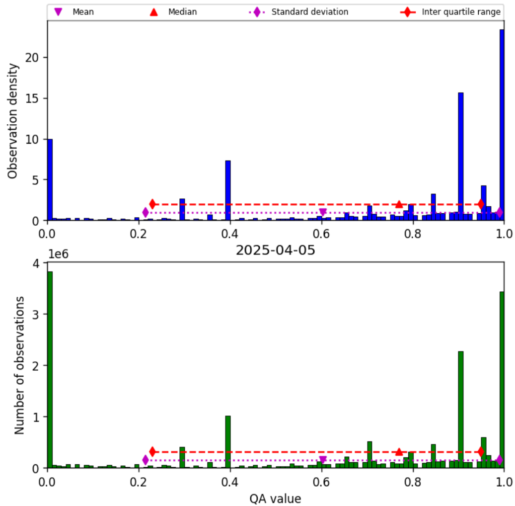
Figure 36: Histogram of “QA value” for 2025-04-05 to 2025-04-06
