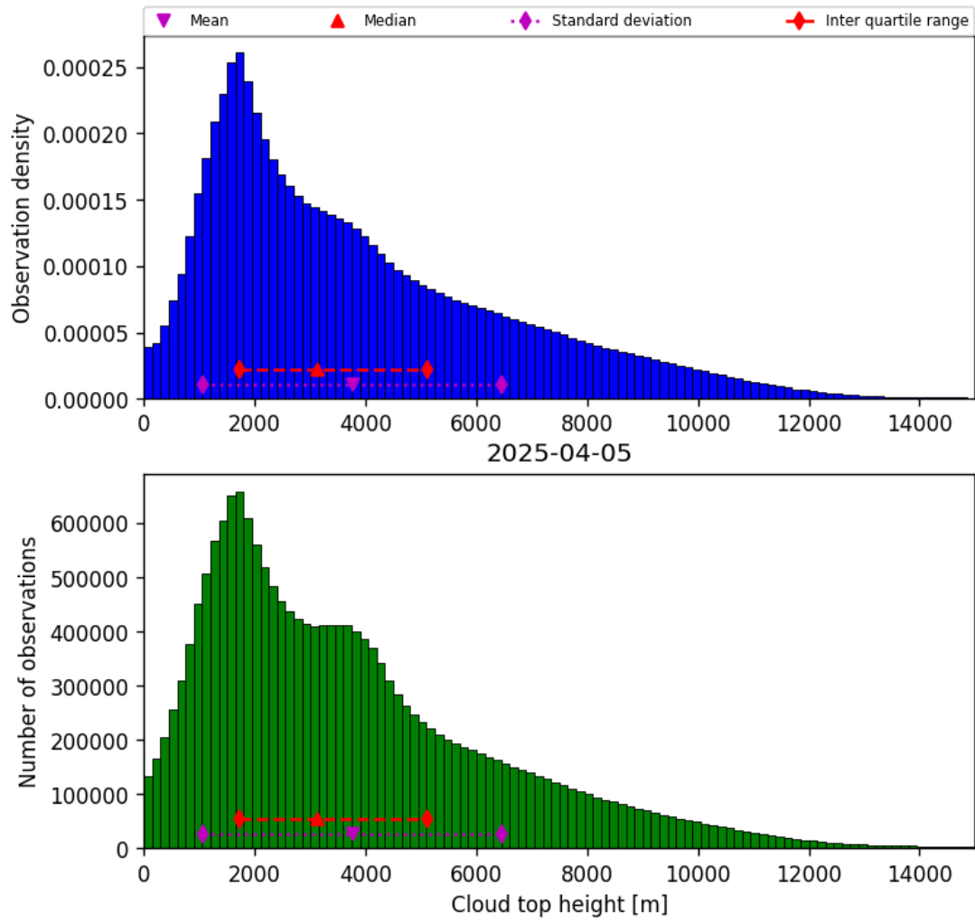
Figure 38: Histogram of “Cloud top height” for 2025-04-05 to 2025-04-06
