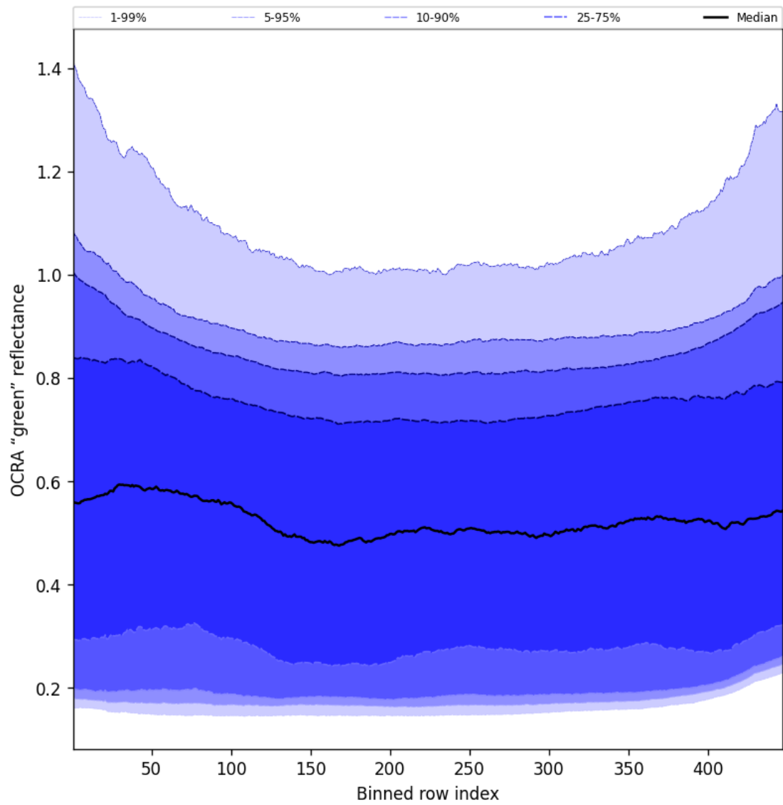
Figure 66: Along track statistics of “OCRA “green” reflectance” for 2025-04-05 to 2025-04-06
