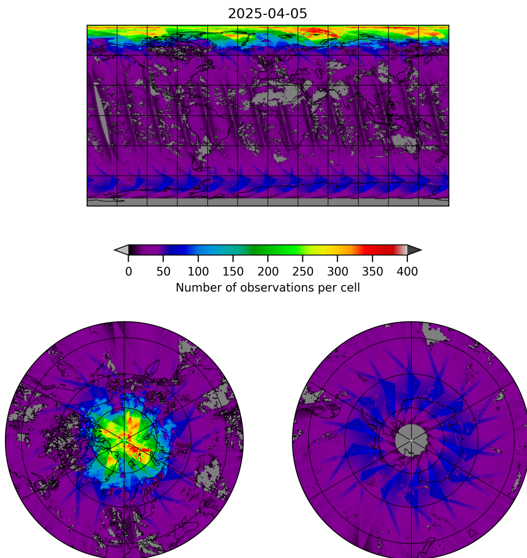
Figure 19: Map of the number of observations for 2025-04-05 to 2025-04-06
