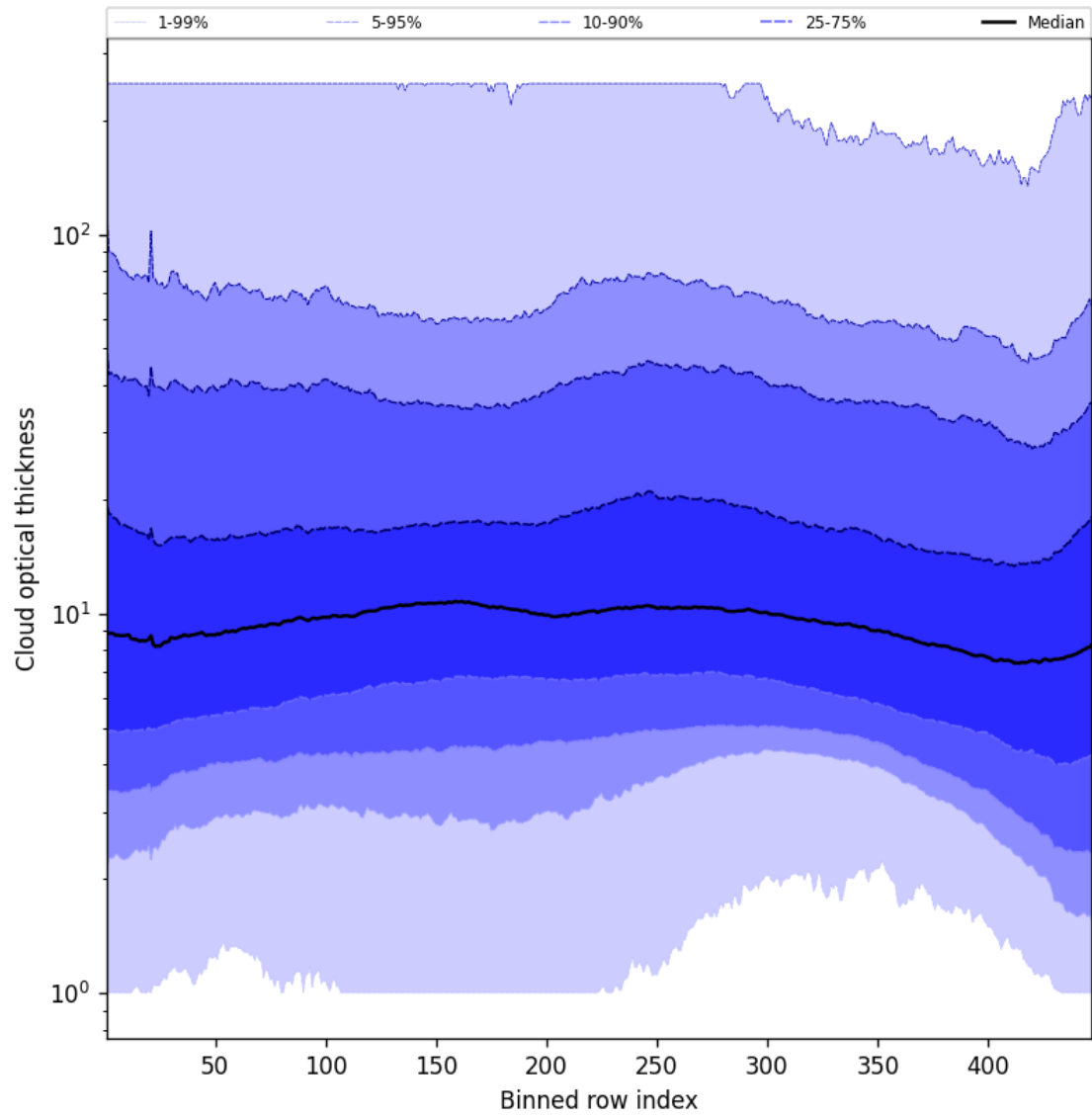
Figure 55: Along track statistics of “Cloud optical thickness” for 2025-04-06 to 2025-04-06
