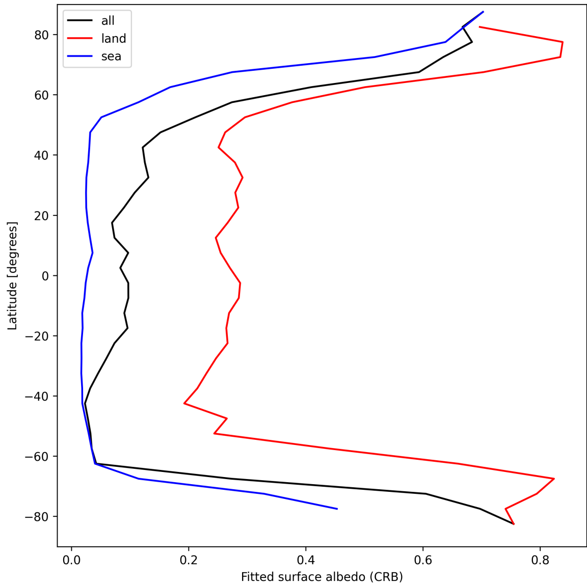
Figure 28: Zonal average of “Fitted surface albedo (CRB)” for 2025-04-06 to 2025-04-06.
