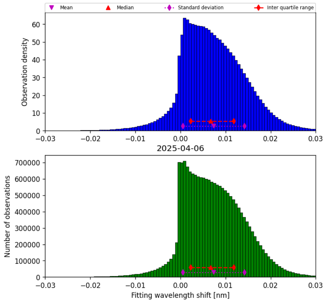
Figure 47: Histogram of “Fitting wavelength shift” for 2025-04-06 to 2025-04-06
