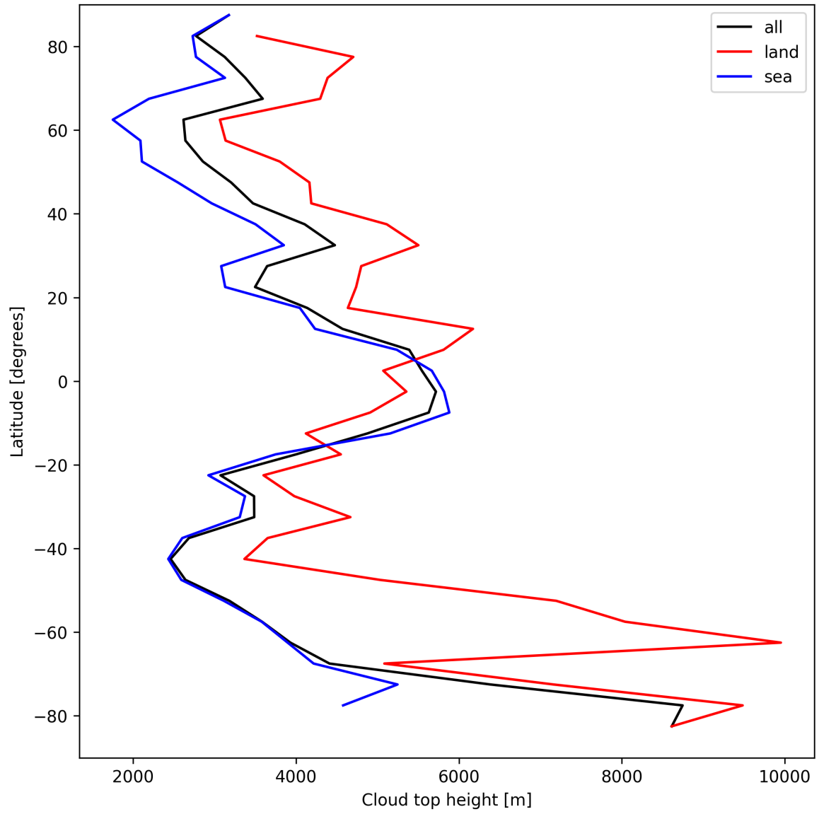
Figure 22: Zonal average of “Cloud top height” for 2025-04-06 to 2025-04-06.
