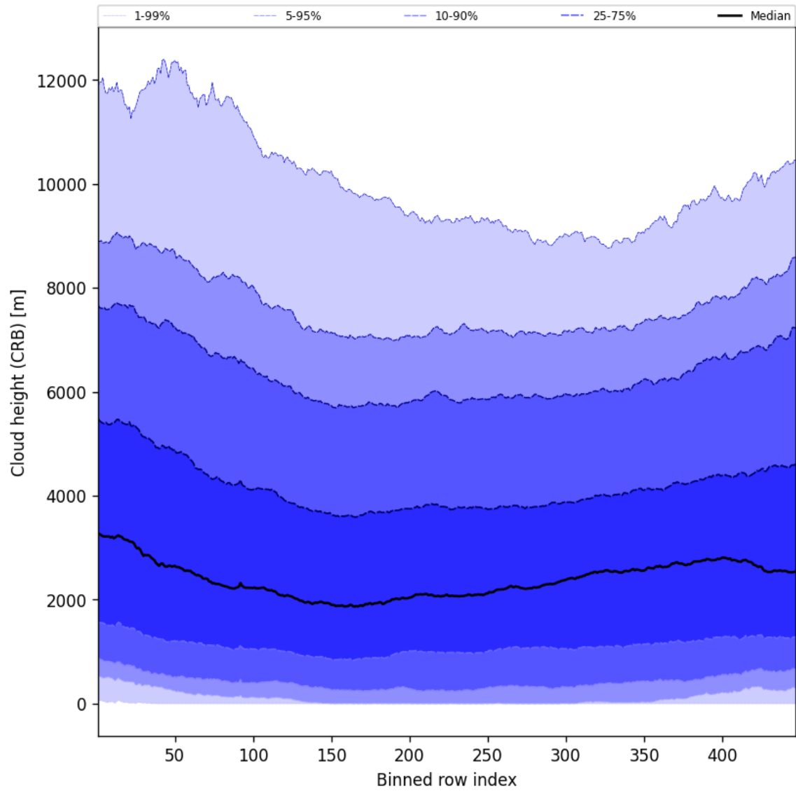
Figure 57: Along track statistics of “Cloud height (CRB)” for 2025-04-06 to 2025-04-06
