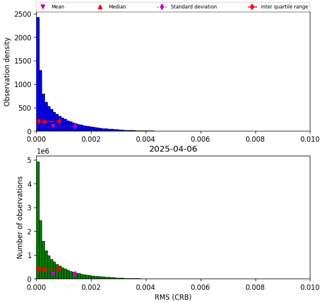
Figure 46: Histogram of “RMS (CRB)” for 2025-04-06 to 2025-04-06
