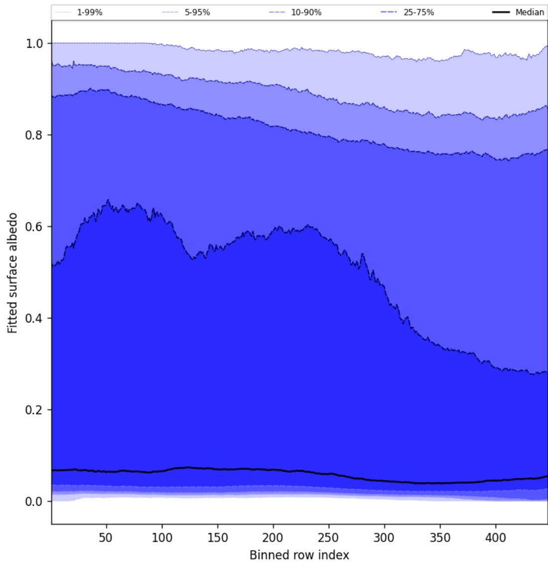
Figure 59: Along track statistics of “Fitted surface albedo” for 2025-04-06 to 2025-04-06
