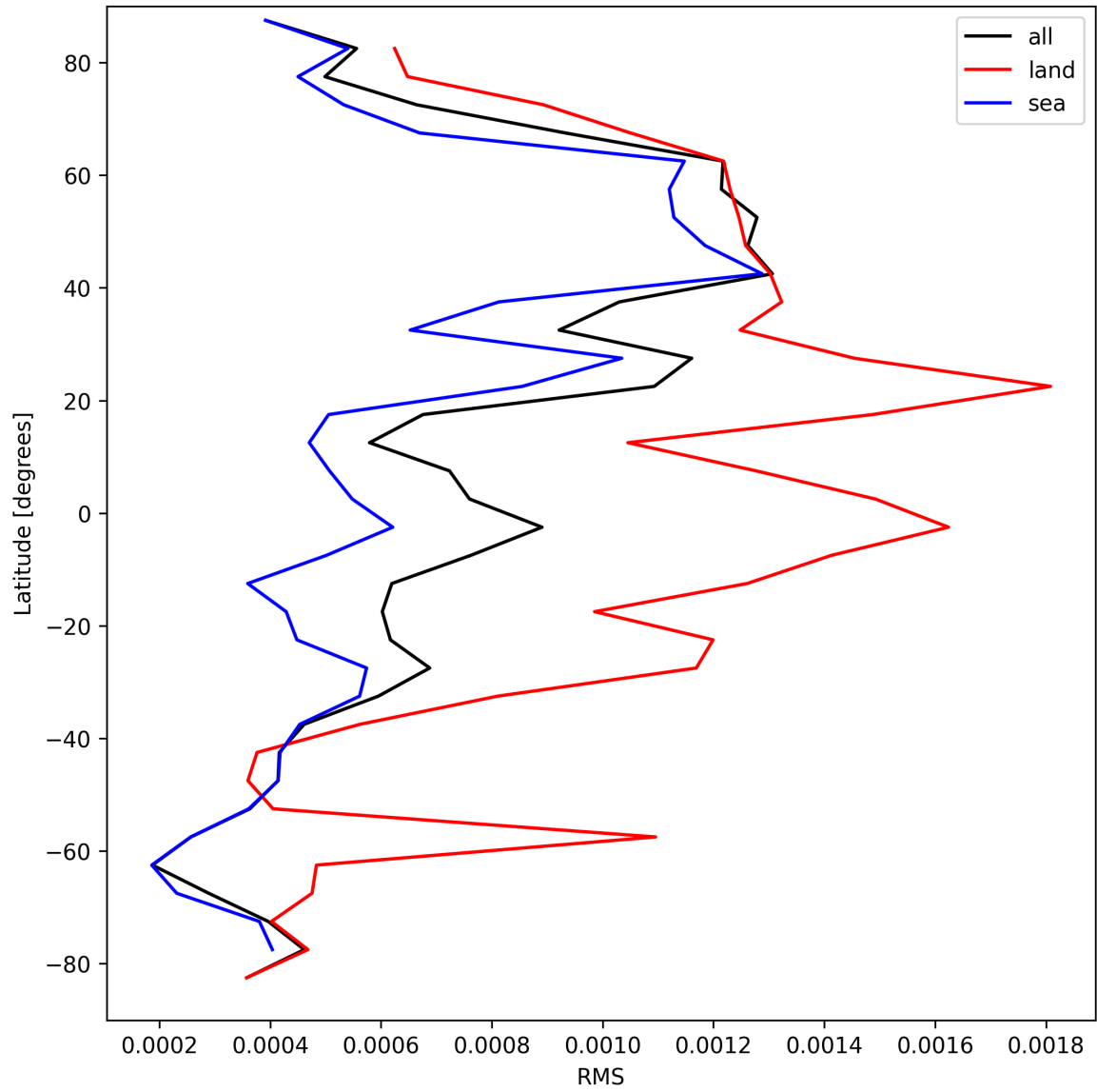
Figure 29: Zonal average of “RMS” for 2025-04-06 to 2025-04-06.
