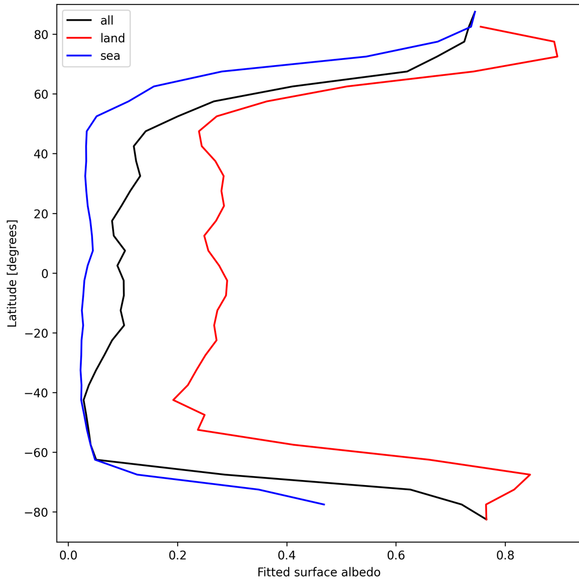
Figure 27: Zonal average of “Fitted surface albedo” for 2025-04-06 to 2025-04-06.
