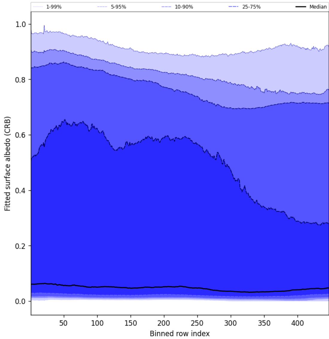
Figure 60: Along track statistics of “Fitted surface albedo (CRB)” for 2025-04-06 to 2025-04-06
