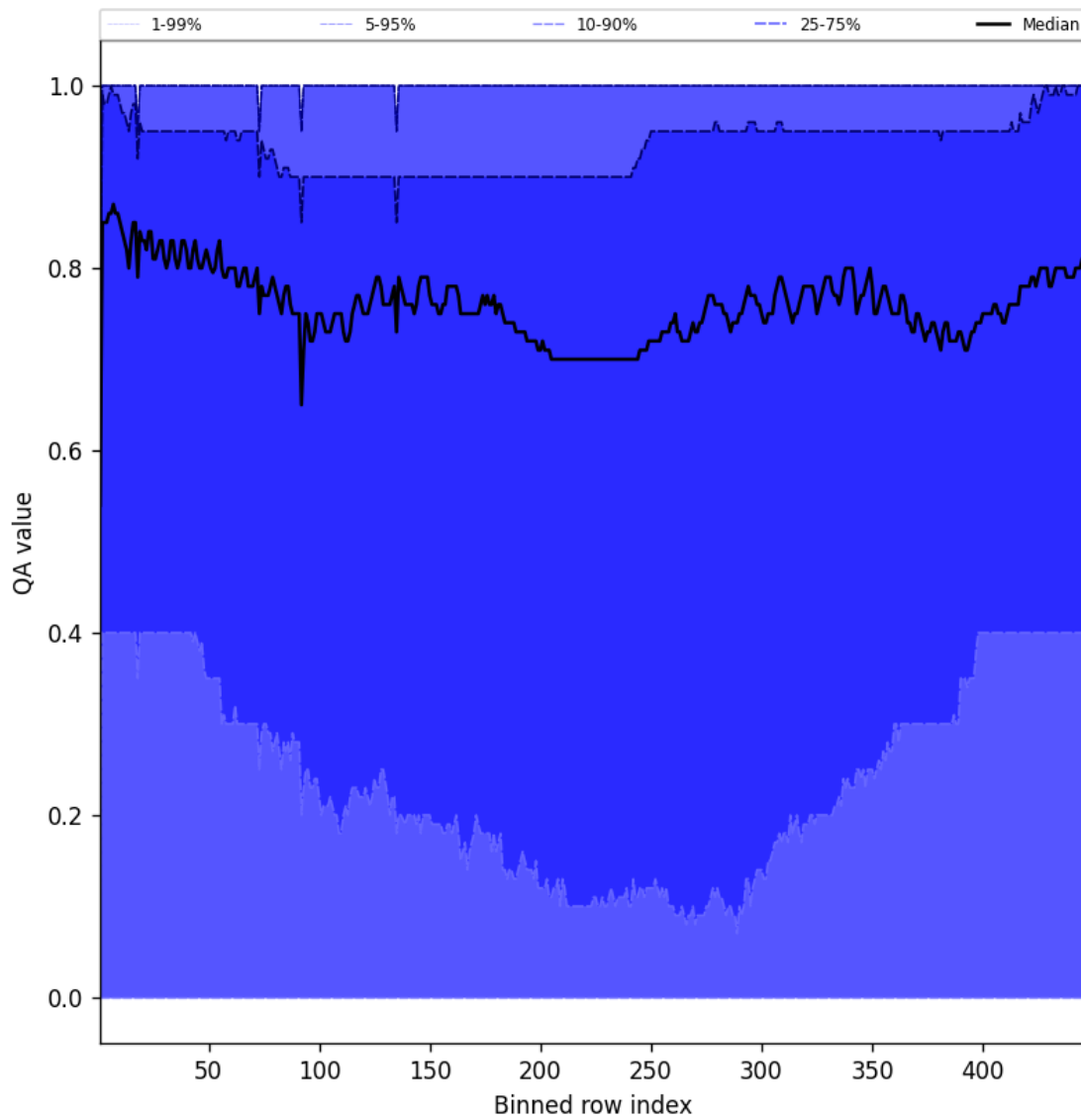
Figure 52: Along track statistics of “QA value” for 2025-04-06 to 2025-04-06
