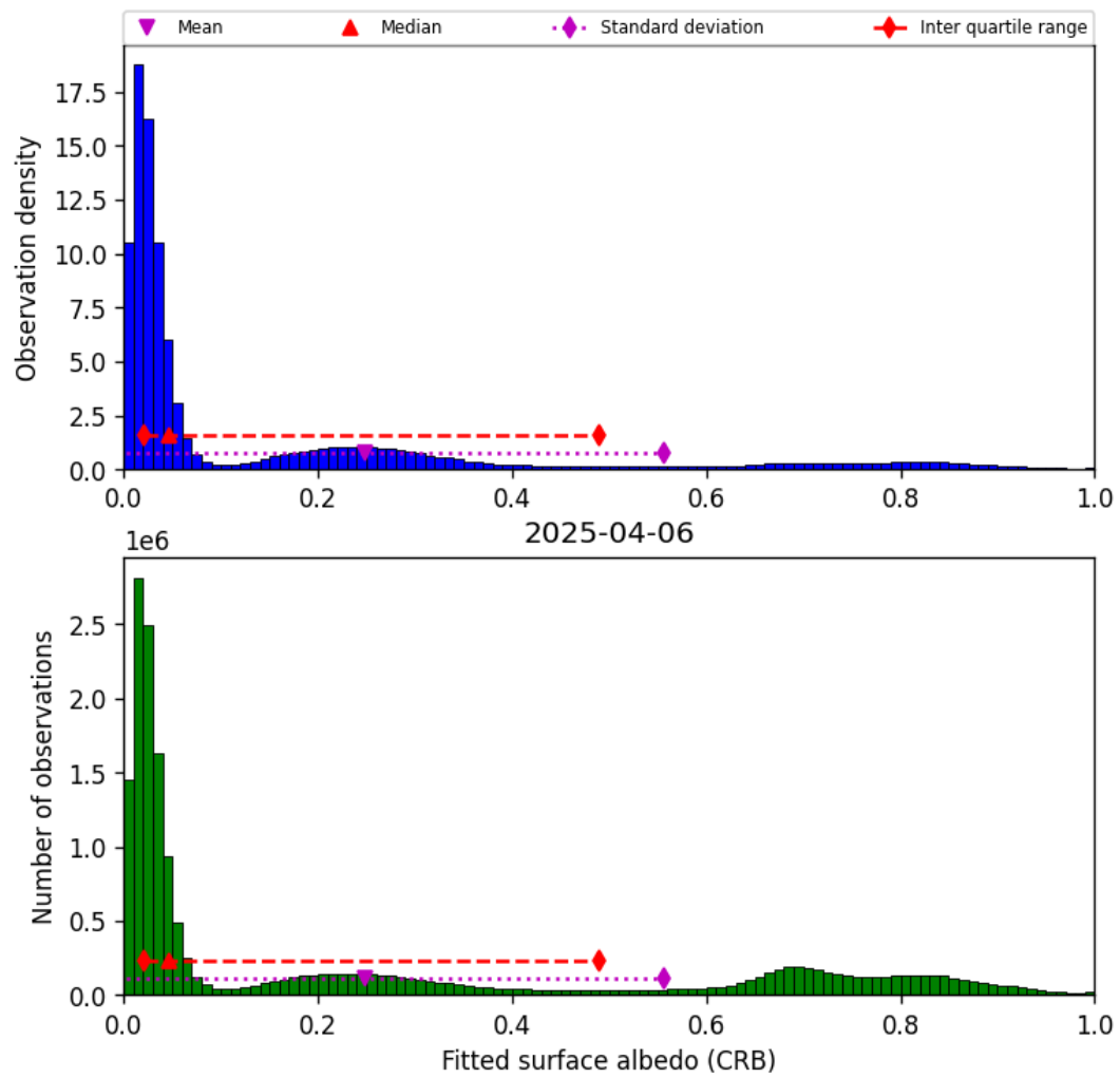
Figure 44: Histogram of “Fitted surface albedo (CRB)” for 2025-04-06 to 2025-04-06
