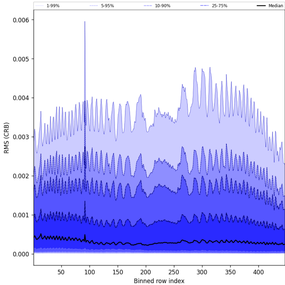
Figure 62: Along track statistics of “RMS (CRB)” for 2025-04-06 to 2025-04-06
