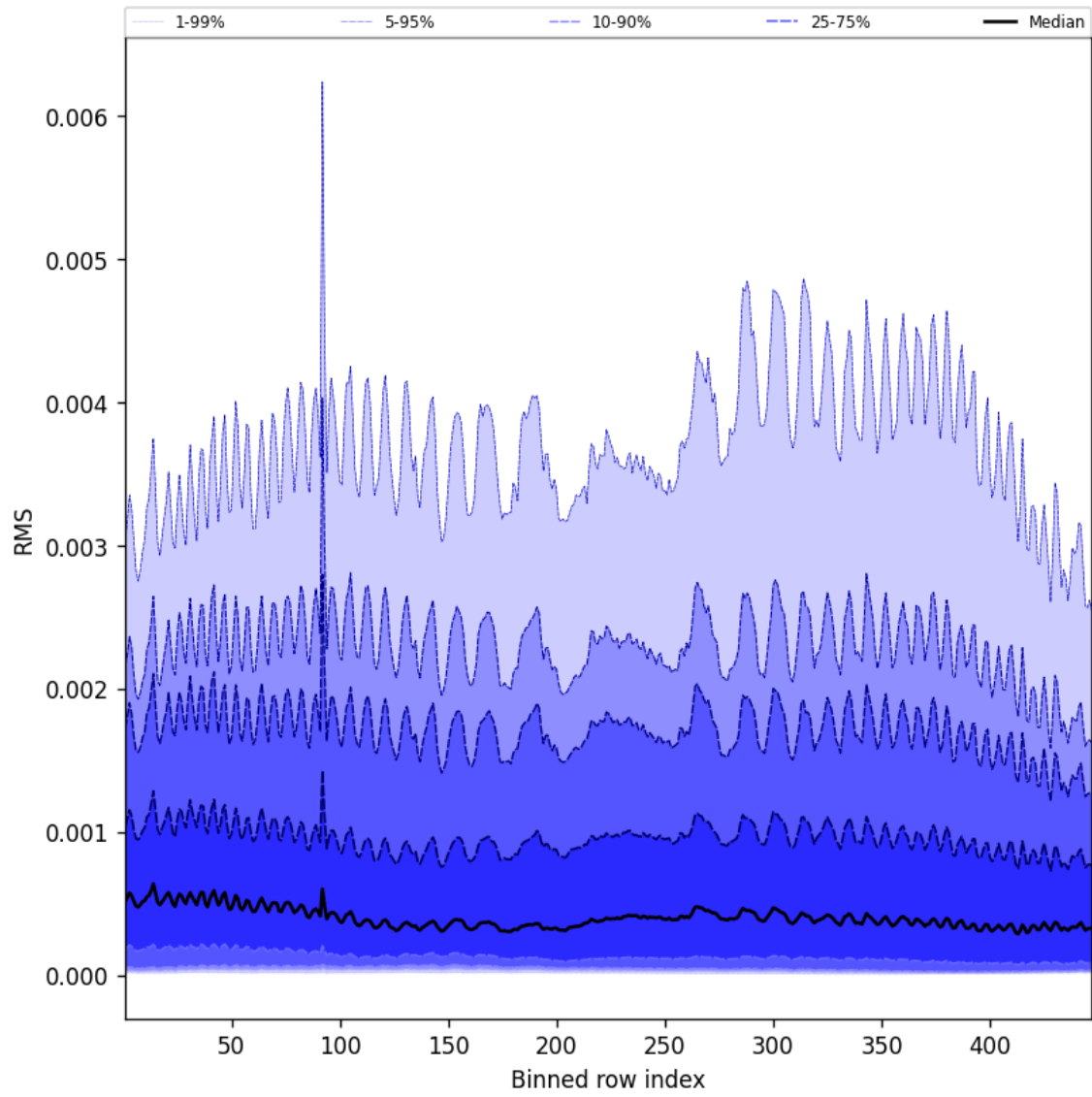
Figure 61: Along track statistics of “RMS” for 2025-04-06 to 2025-04-06
