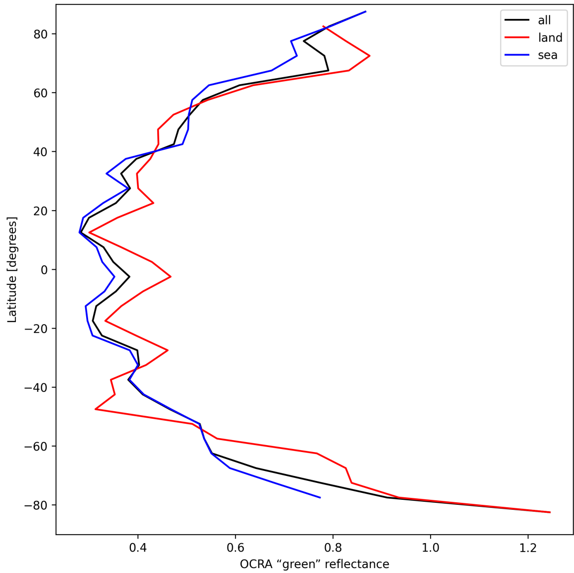
Figure 34: Zonal average of “OCRA “green” reflectance” for 2025-04-06 to 2025-04-06.
