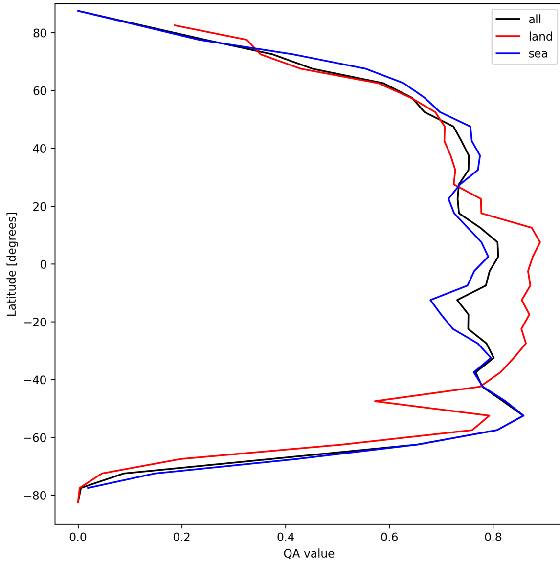
Figure 20: Zonal average of “QA value” for 2025-04-06 to 2025-04-06.
