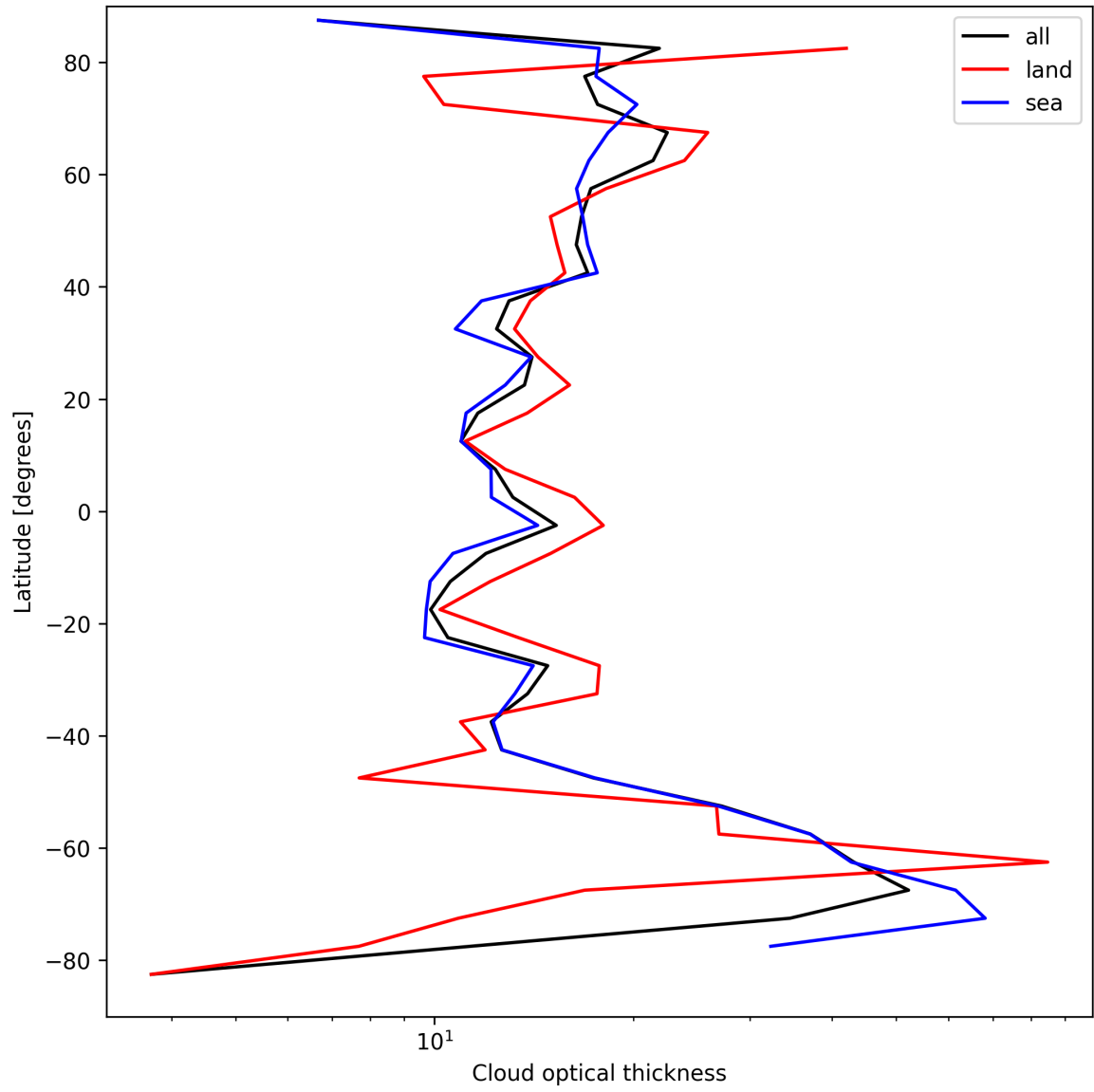
Figure 23: Zonal average of “Cloud optical thickness” for 2025-04-06 to 2025-04-06.
