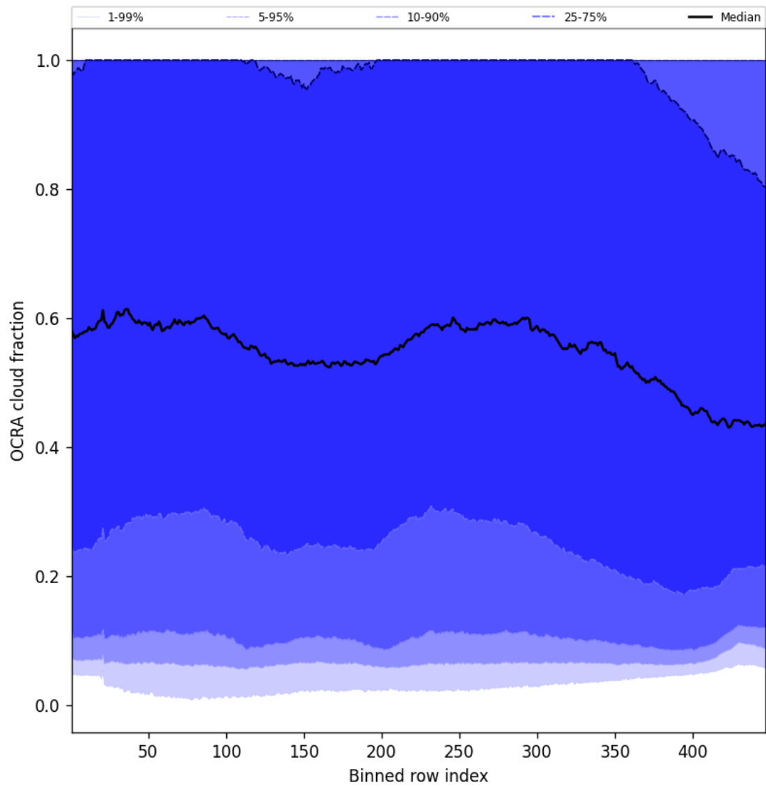
Figure 64: Along track statistics of “OCRA cloud fraction” for 2025-04-06 to 2025-04-06
