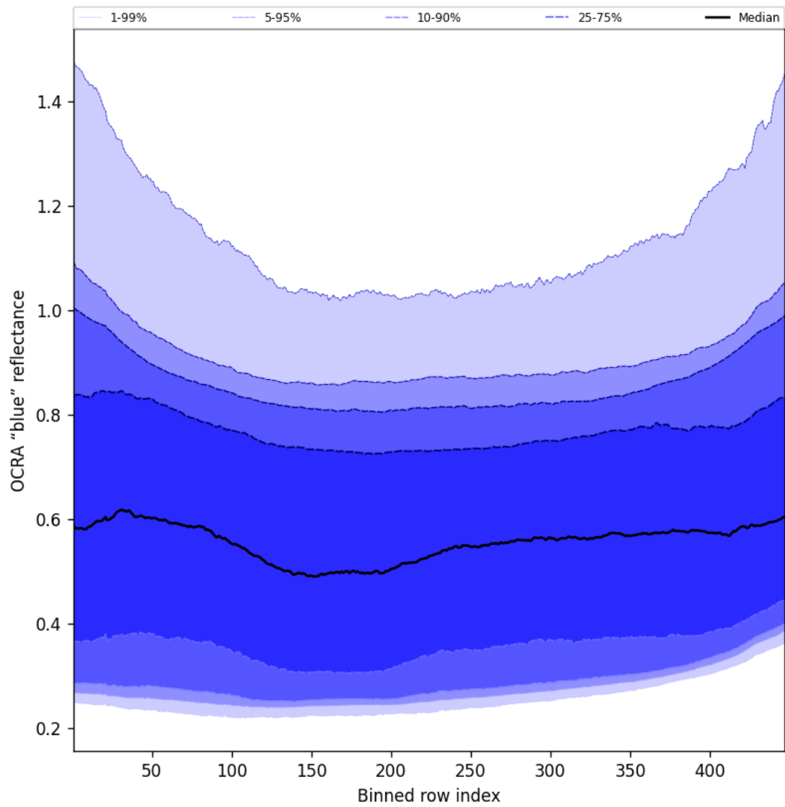
Figure 65: Along track statistics of “OCRA “blue” reflectance” for 2025-04-06 to 2025-04-06
