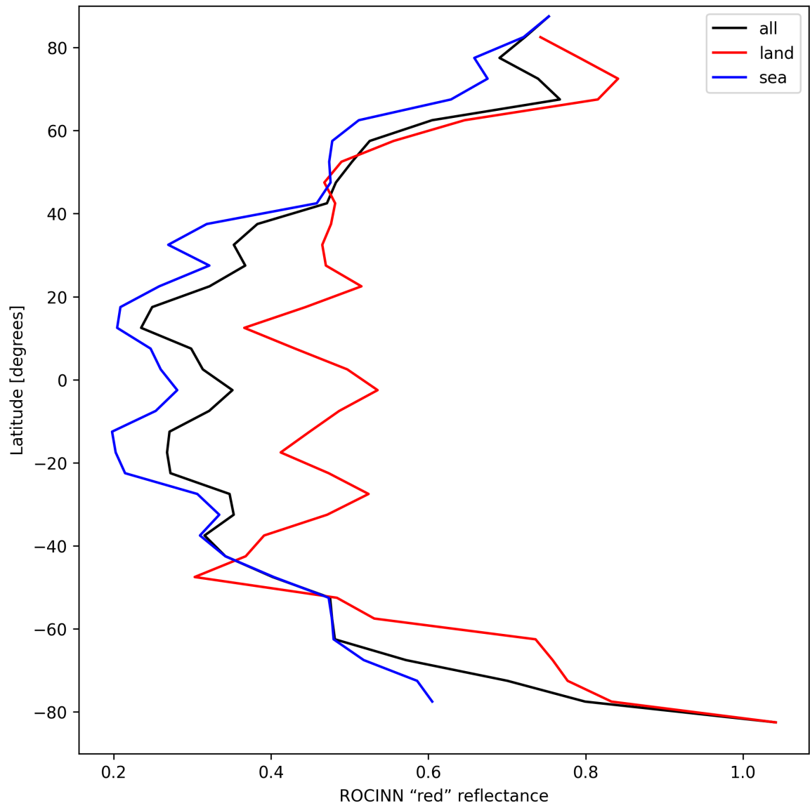
Figure 35: Zonal average of “ROCINN “red” reflectance” for 2025-04-06 to 2025-04-06.
