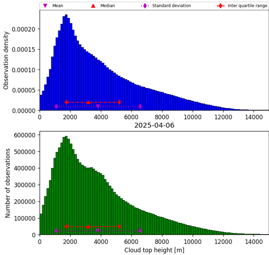
Figure 38: Histogram of "Cloud top height" for 2025-04-06 to 2025-04-06
