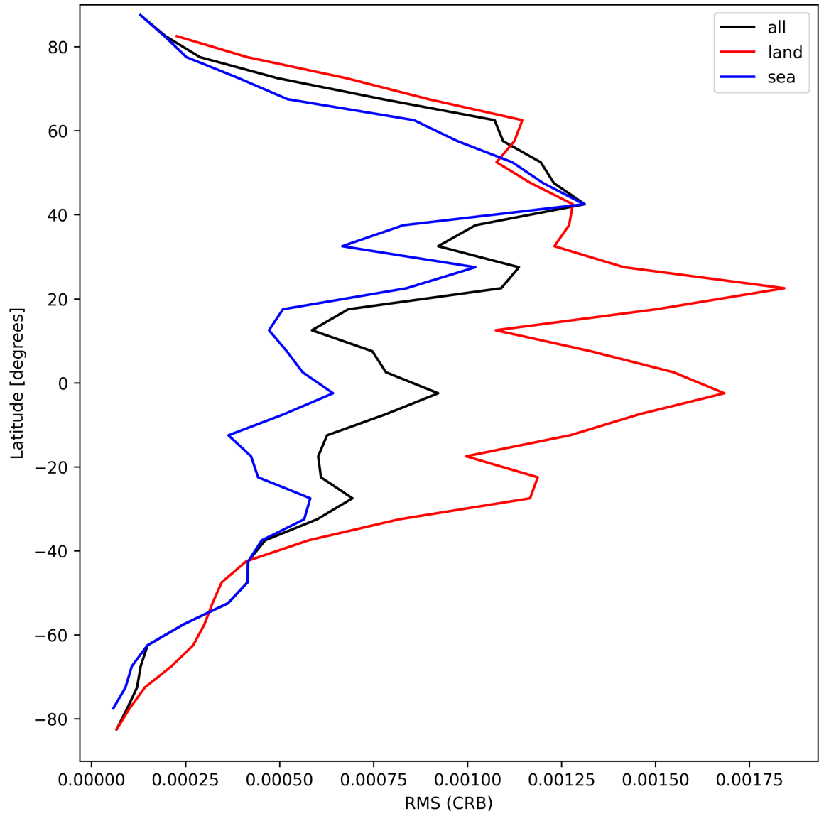
Figure 30: Zonal average of “RMS (CRB)” for 2025-04-06 to 2025-04-06.
