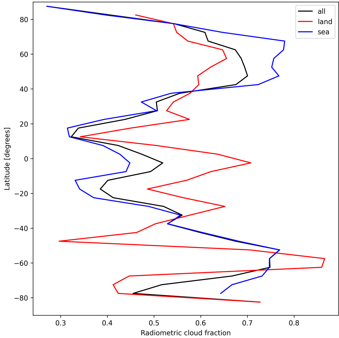
Figure 21: Zonal average of “Radiometric cloud fraction” for 2025-04-06 to 2025-04-06.
