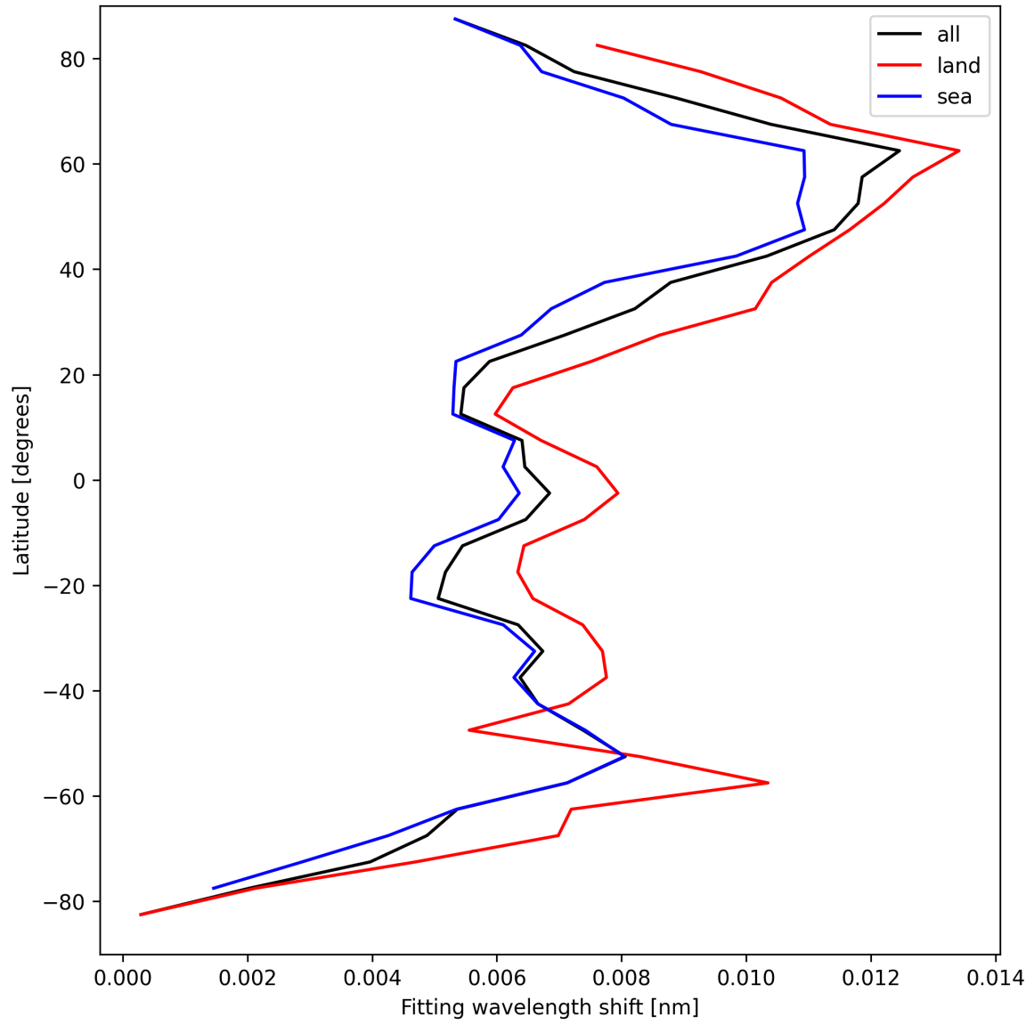
Figure 31: Zonal average of “Fitting wavelength shift” for 2025-04-06 to 2025-04-06.
