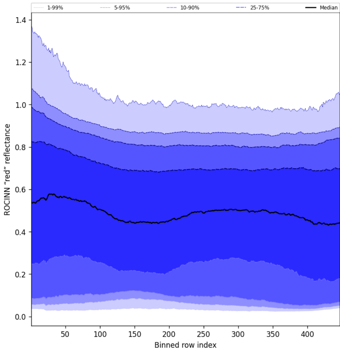
Figure 67: Along track statistics of "ROCINN "red" reflectance" for 2025-04-06 to 2025-04-06
