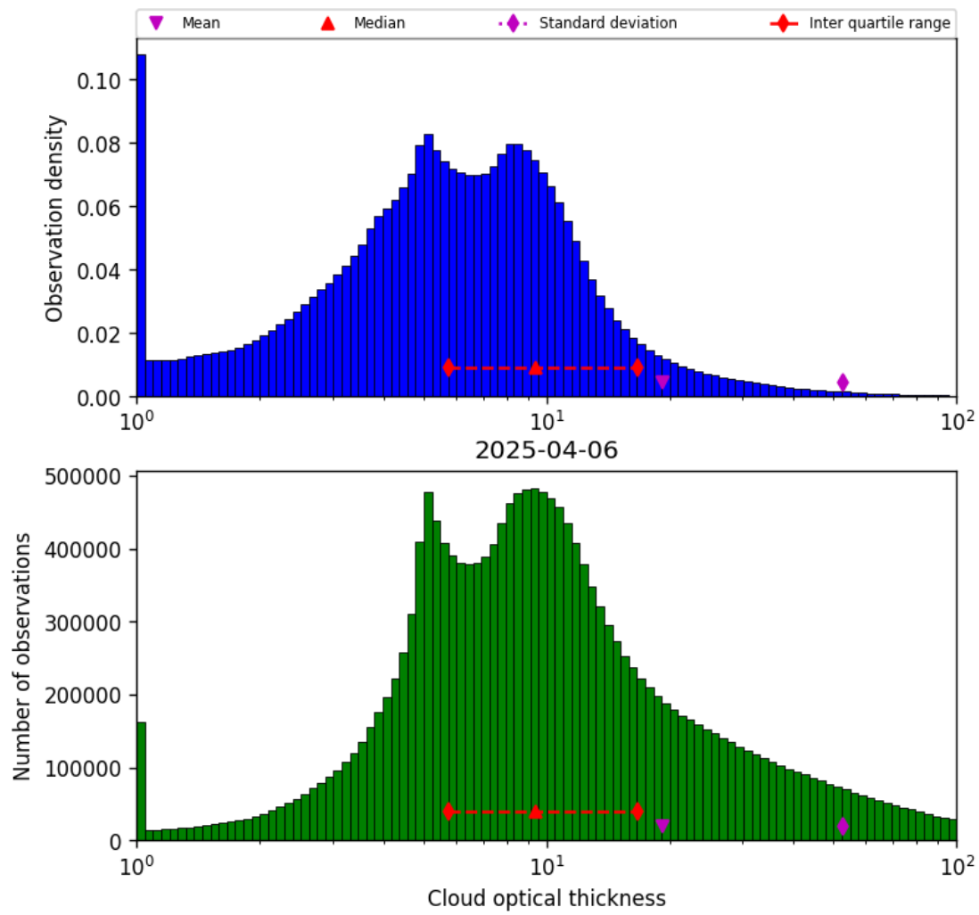
Figure 39: Histogram of “Cloud optical thickness” for 2025-04-06 to 2025-04-06
