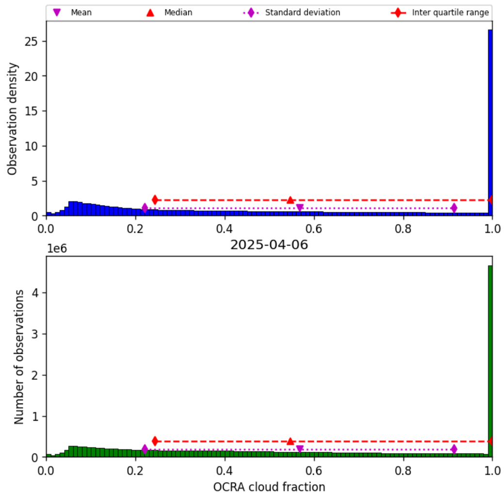
Figure 48: Histogram of “OCRA cloud fraction” for 2025-04-06 to 2025-04-06
