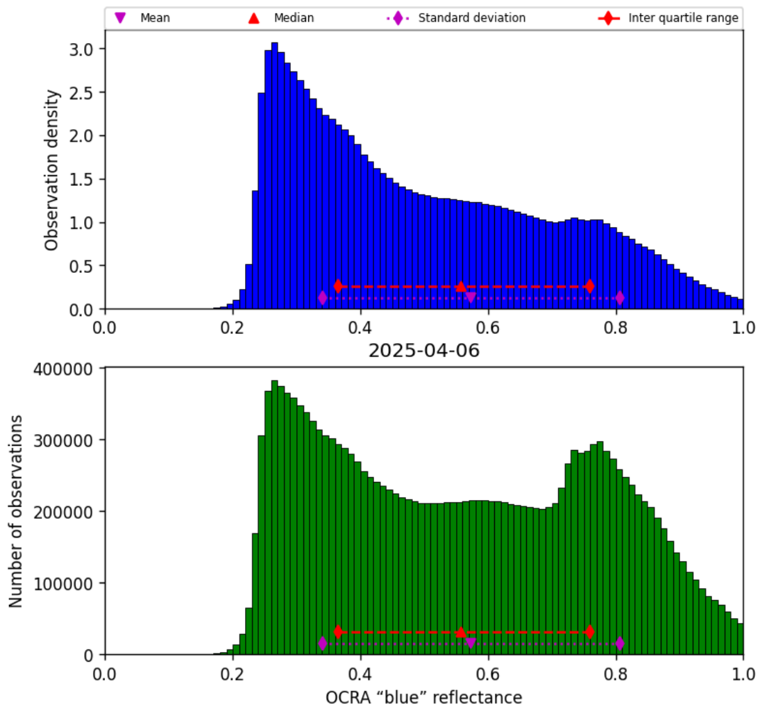
Figure 49: Histogram of “OCRA “blue” reflectance” for 2025-04-06 to 2025-04-06
