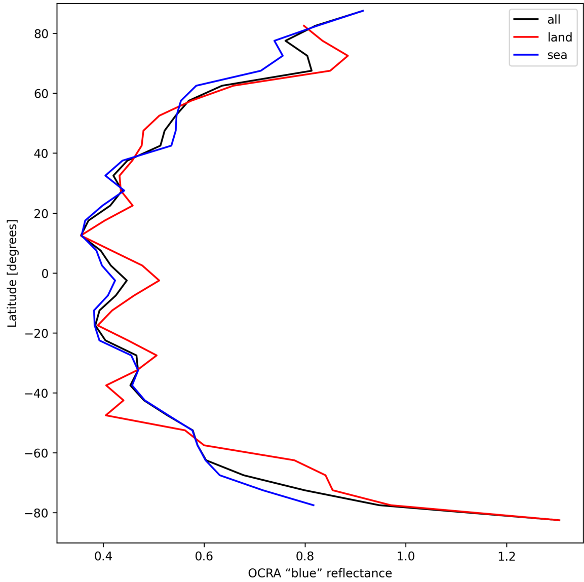
Figure 33: Zonal average of “OCRA “blue” reflectance” for 2025-04-06 to 2025-04-06.
