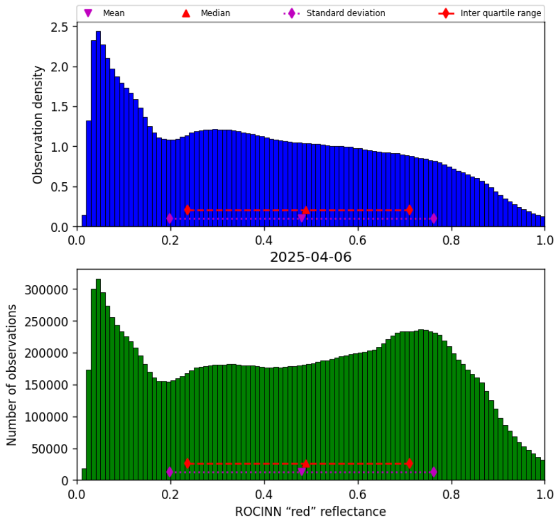
Figure 51: Histogram of “ROCINN “red” reflectance” for 2025-04-06 to 2025-04-06
