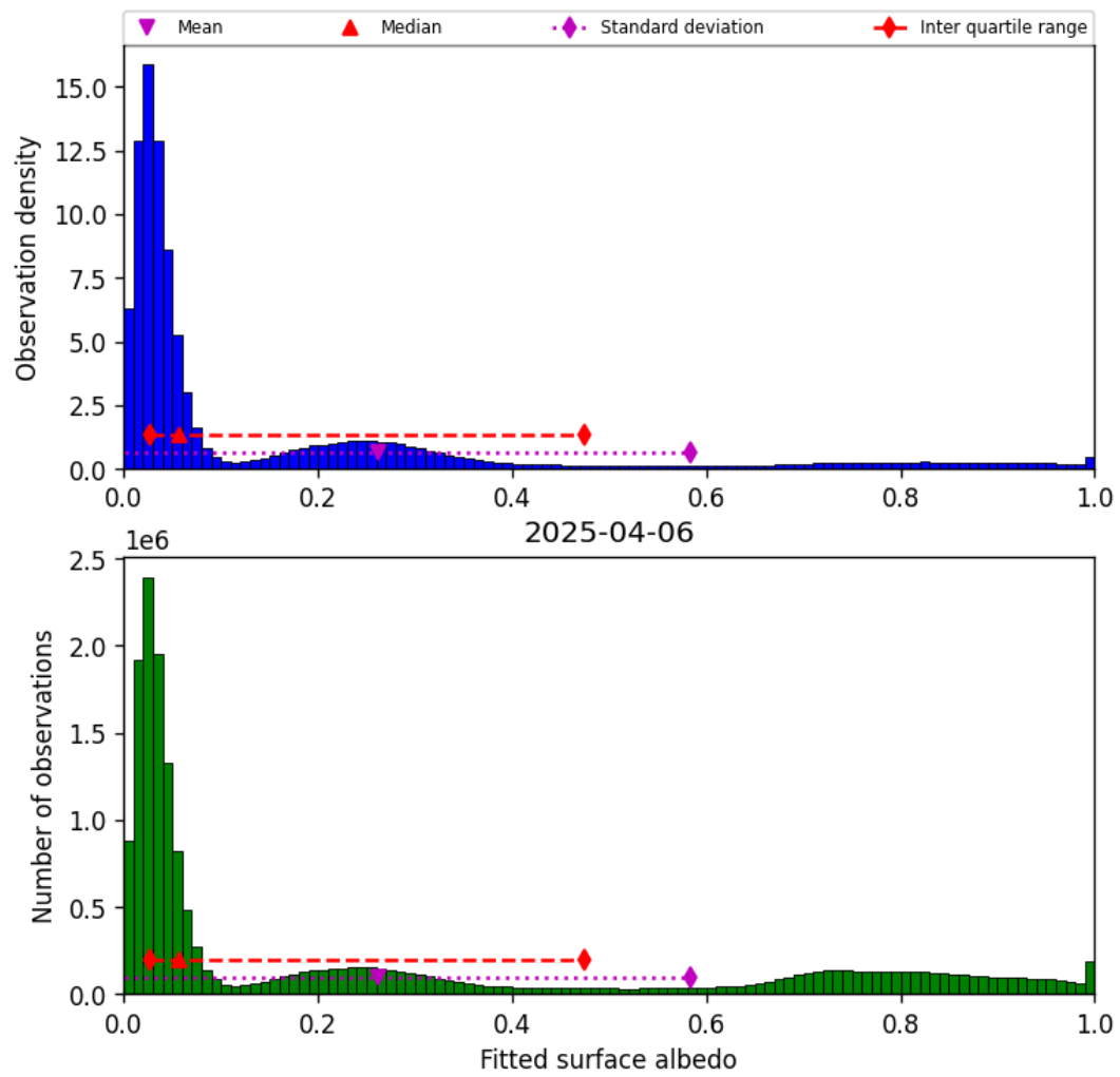
Figure 43: Histogram of “Fitted surface albedo” for 2025-04-06 to 2025-04-06
