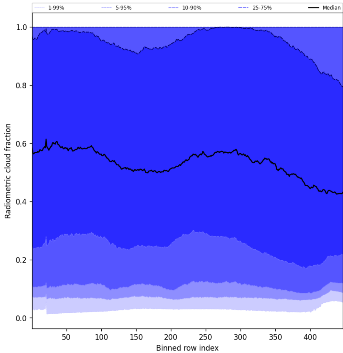
Figure 53: Along track statistics of “Radiometric cloud fraction” for 2025-04-06 to 2025-04-06
