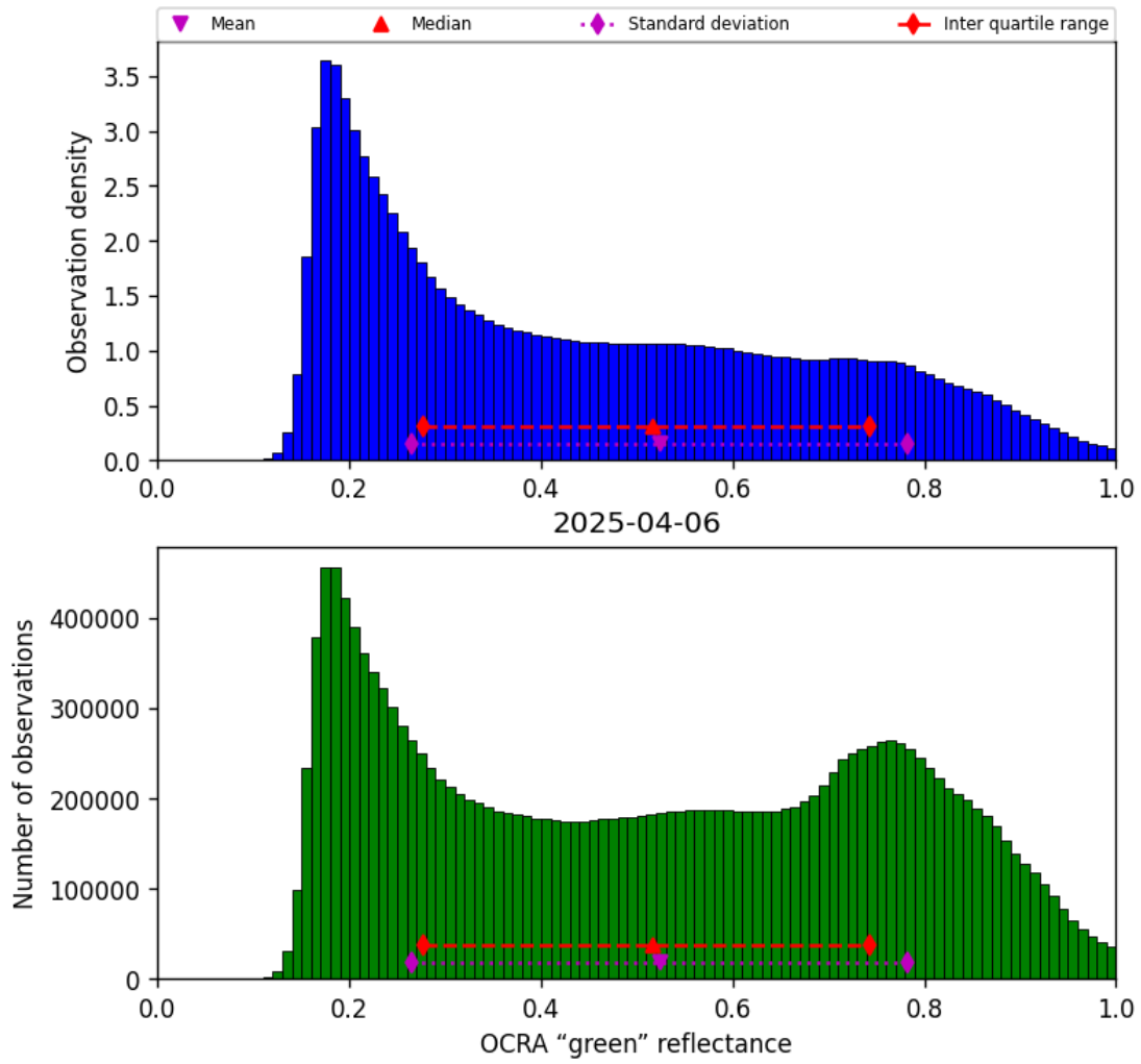
Figure 50: Histogram of “OCRA “green” reflectance” for 2025-04-06 to 2025-04-06
