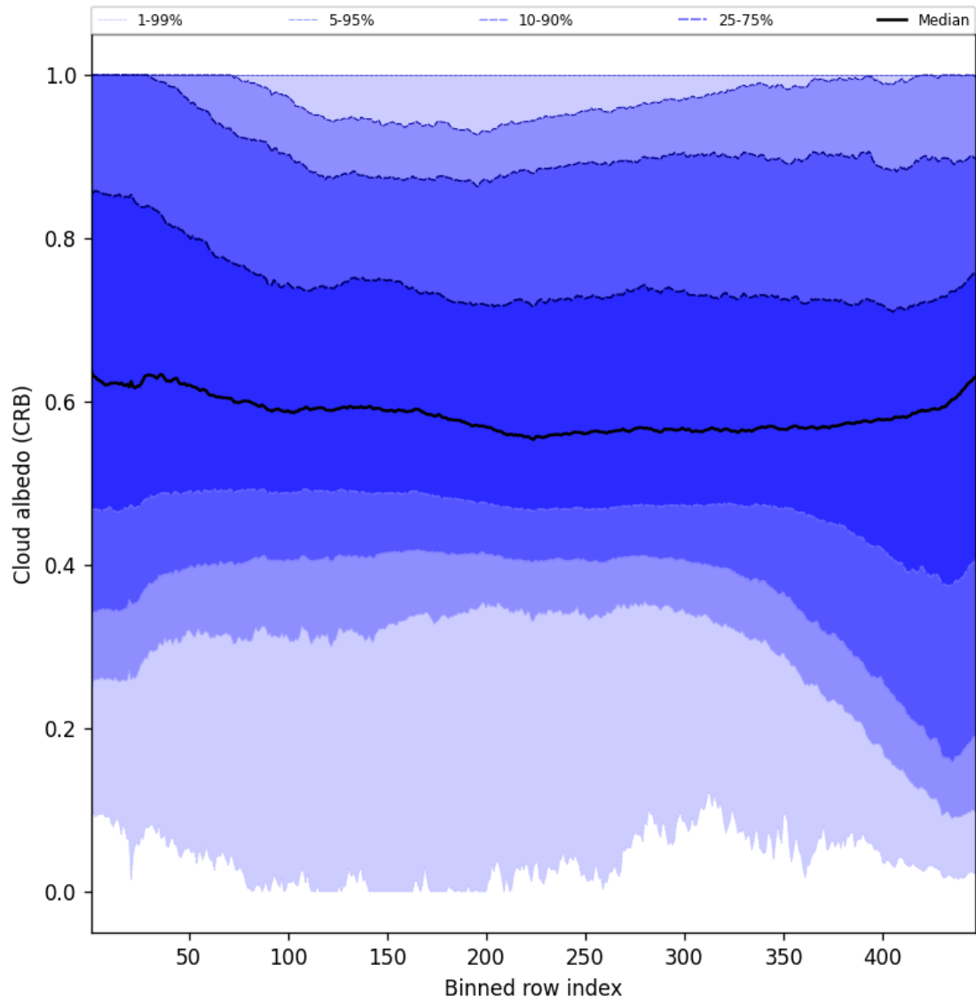
Figure 58: Along track statistics of “Cloud albedo (CRB)” for 2025-04-06 to 2025-04-06
