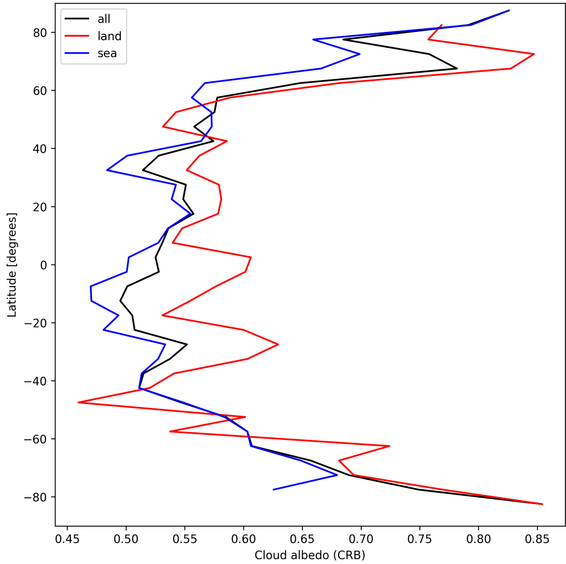
Figure 26: Zonal average of “Cloud albedo (CRB)” for 2025-04-06 to 2025-04-06.
