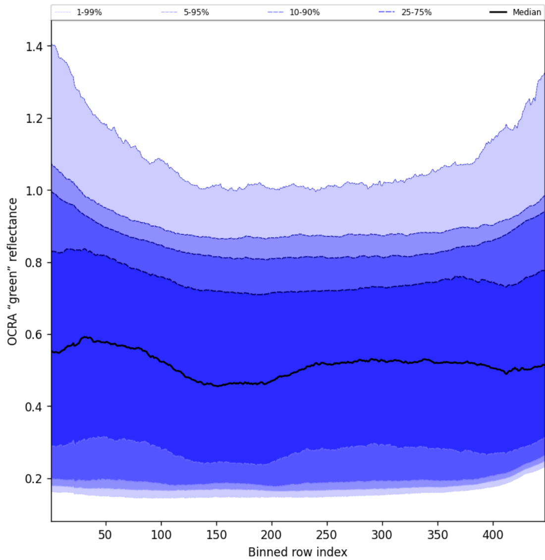
Figure 66: Along track statistics of “OCRA “green” reflectance” for 2025-04-06 to 2025-04-06
