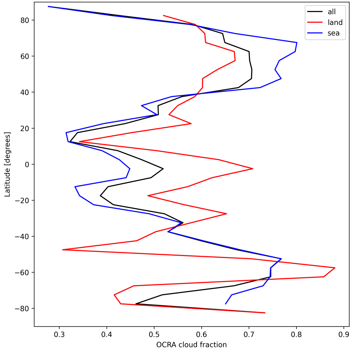
Figure 32: Zonal average of “OCRA cloud fraction” for 2025-04-06 to 2025-04-06.
