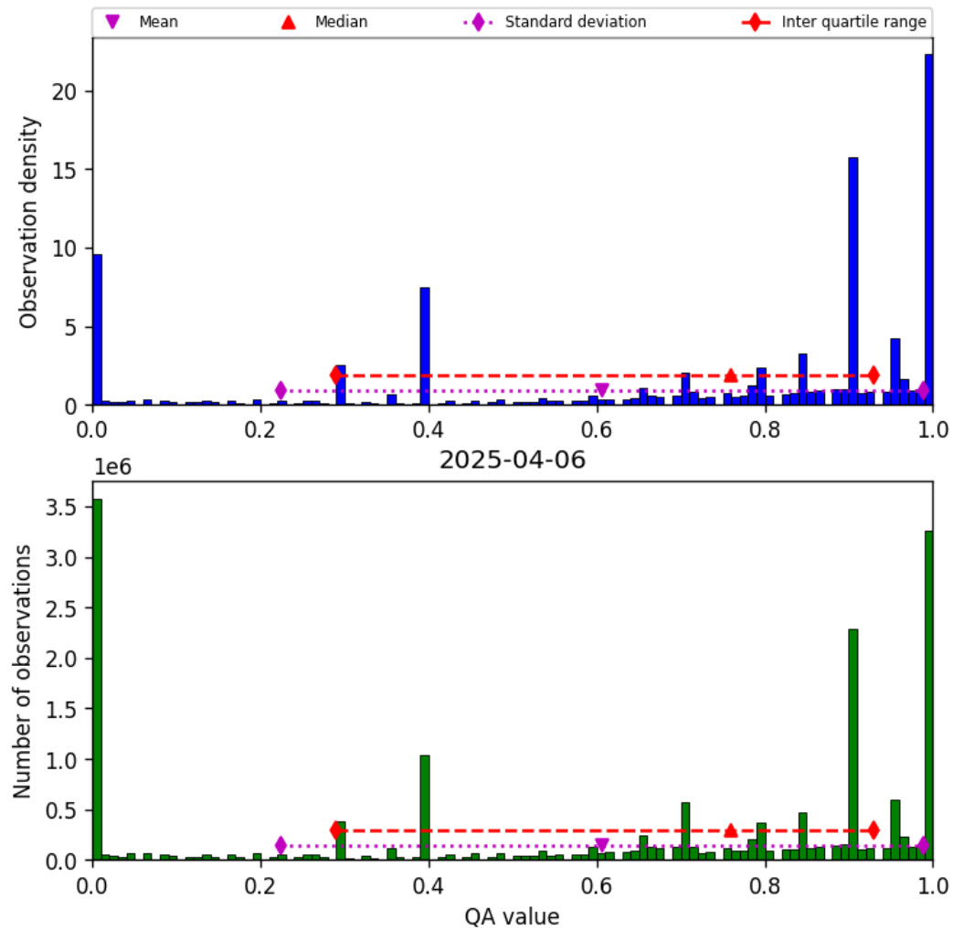
Figure 36: Histogram of “QA value” for 2025-04-06 to 2025-04-06
