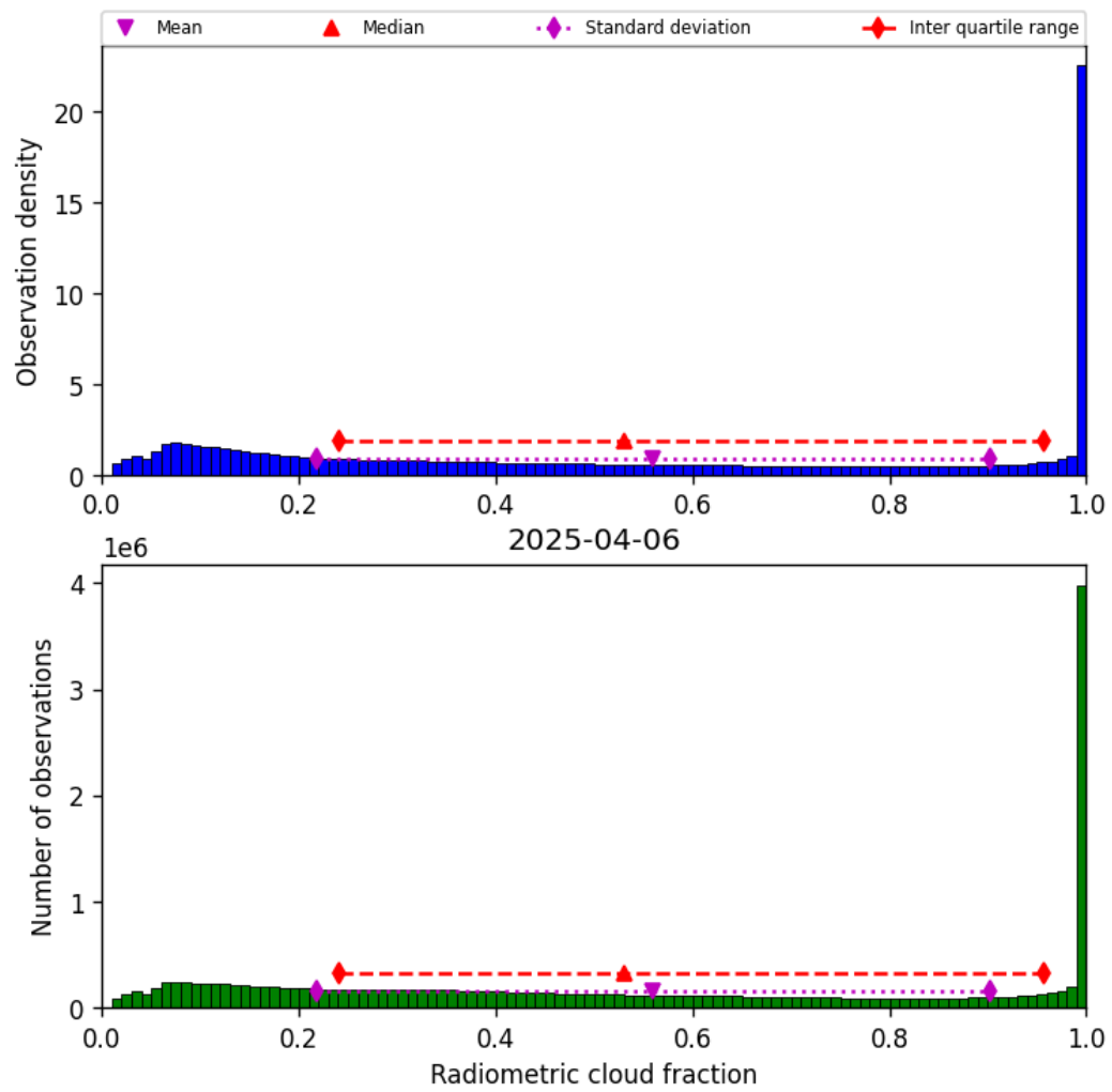
Figure 37: Histogram of “Radiometric cloud fraction” for 2025-04-06 to 2025-04-06
