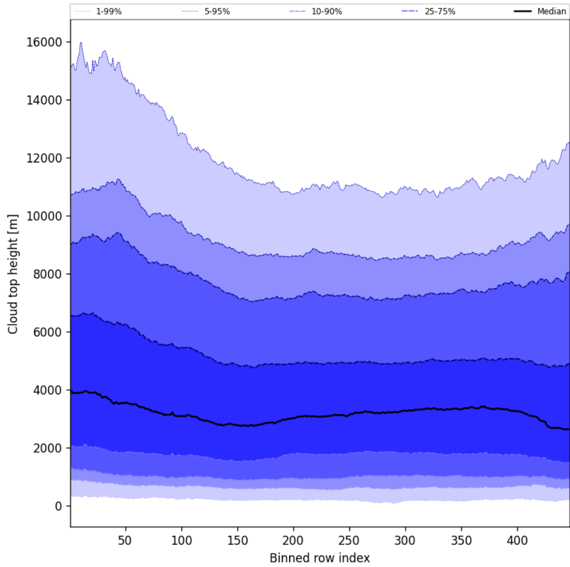
Figure 54: Along track statistics of “Cloud top height” for 2025-04-06 to 2025-04-06
