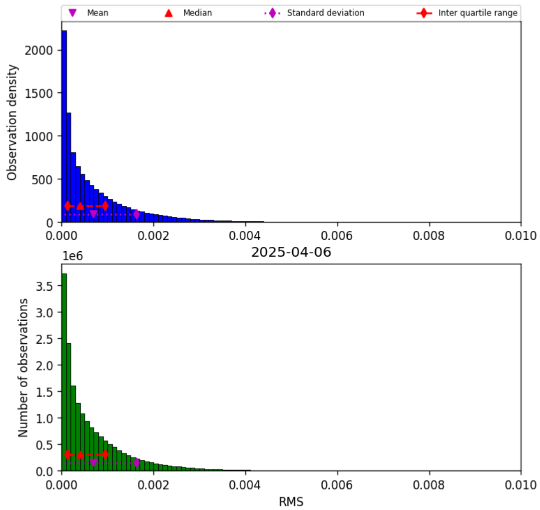
Figure 45: Histogram of “RMS” for 2025-04-06 to 2025-04-06
