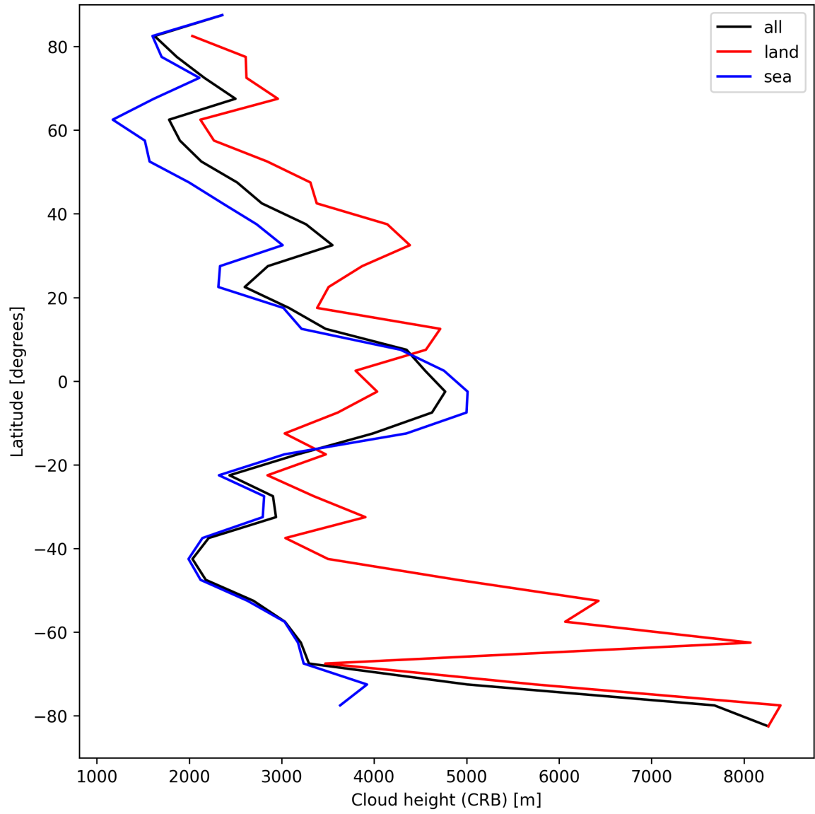
Figure 25: Zonal average of “Cloud height (CRB)” for 2025-04-06 to 2025-04-06.
