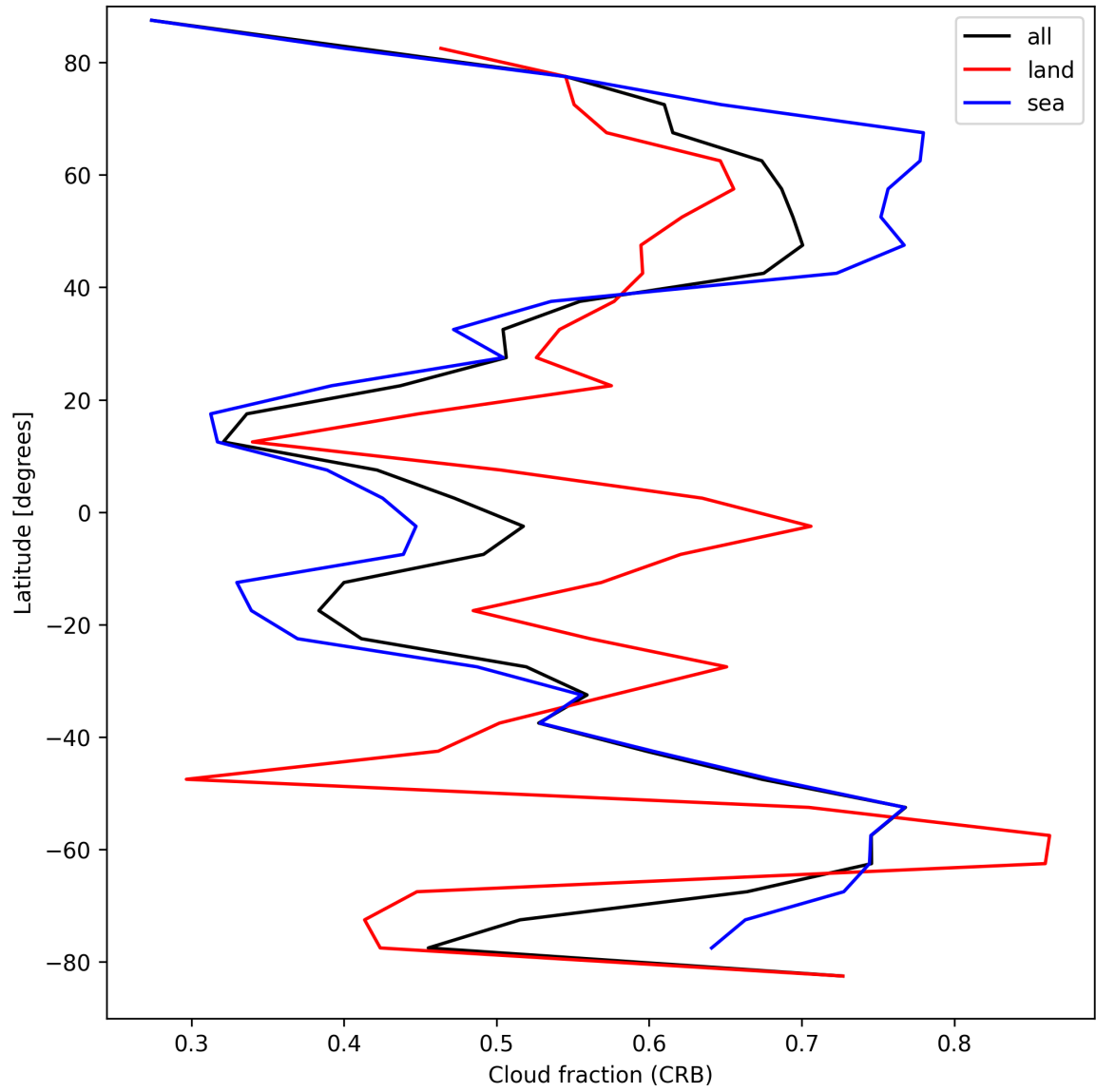
Figure 24: Zonal average of “Cloud fraction (CRB)” for 2025-04-06 to 2025-04-06.
