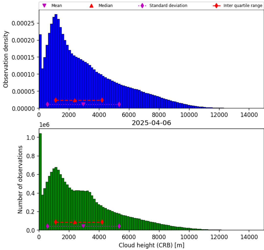
Figure 41: Histogram of “Cloud height (CRB)” for 2025-04-06 to 2025-04-06
