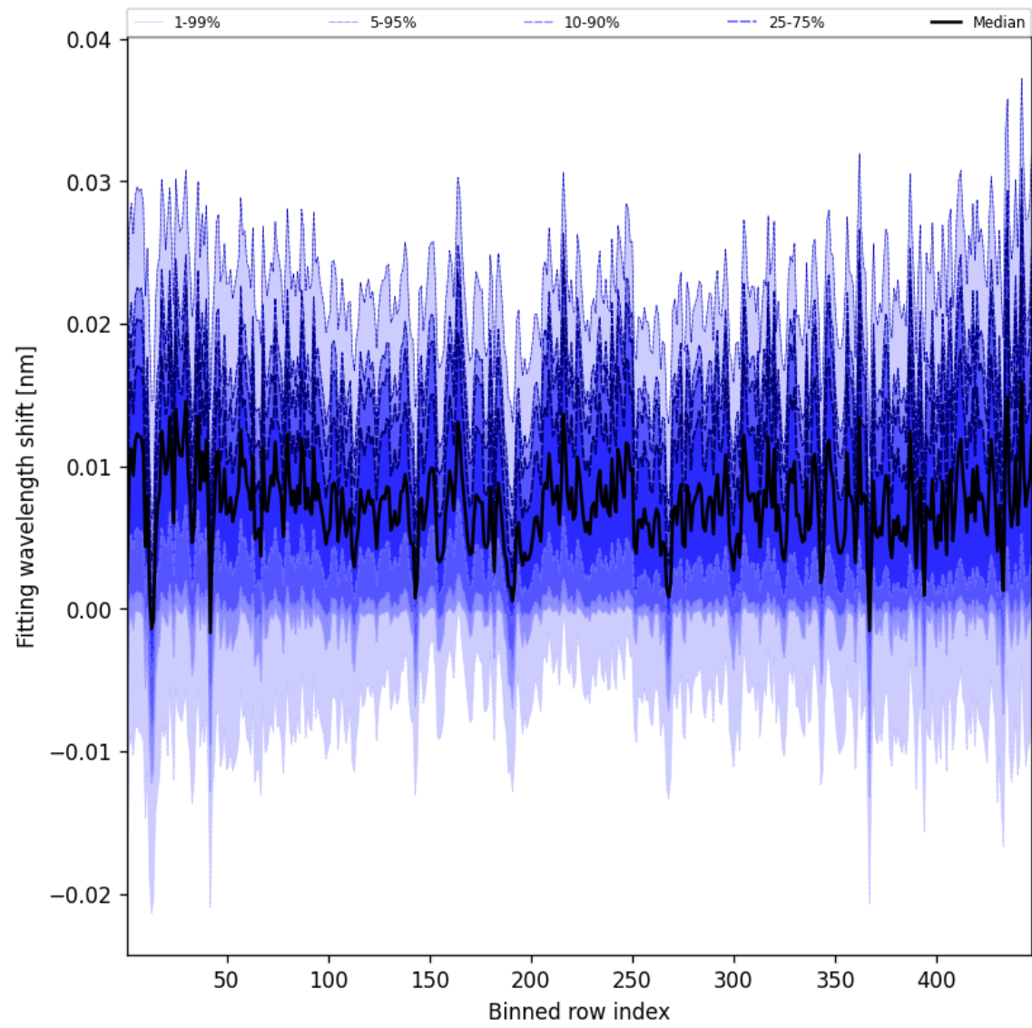
Figure 63: Along track statistics of “Fitting wavelength shift” for 2025-04-06 to 2025-04-06
