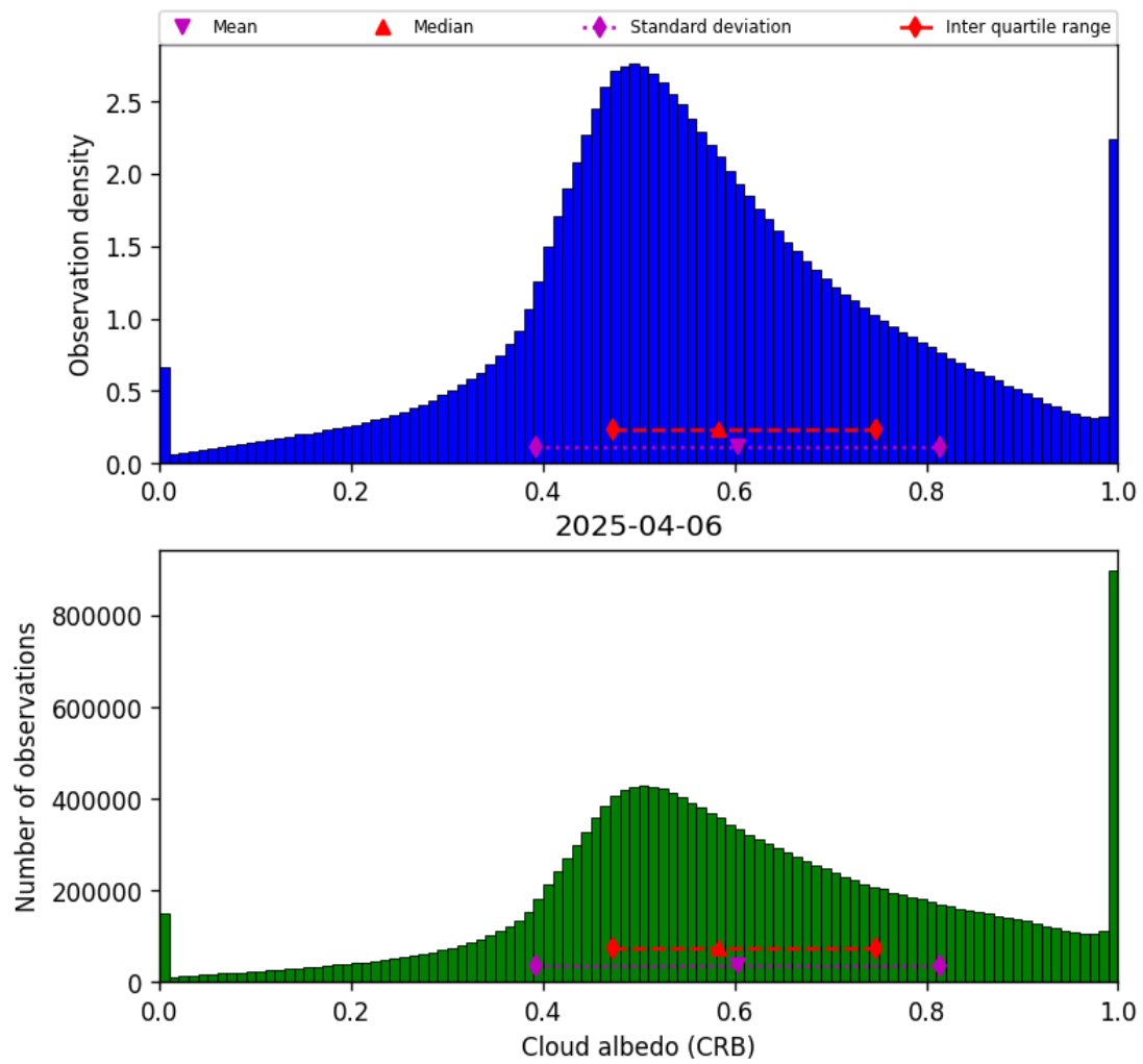
Figure 42: Histogram of “Cloud albedo (CRB)” for 2025-04-06 to 2025-04-06
