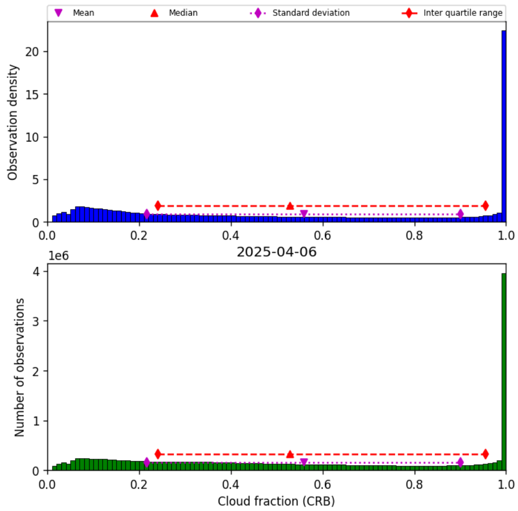
Figure 40: Histogram of “Cloud fraction (CRB)” for 2025-04-06 to 2025-04-06
