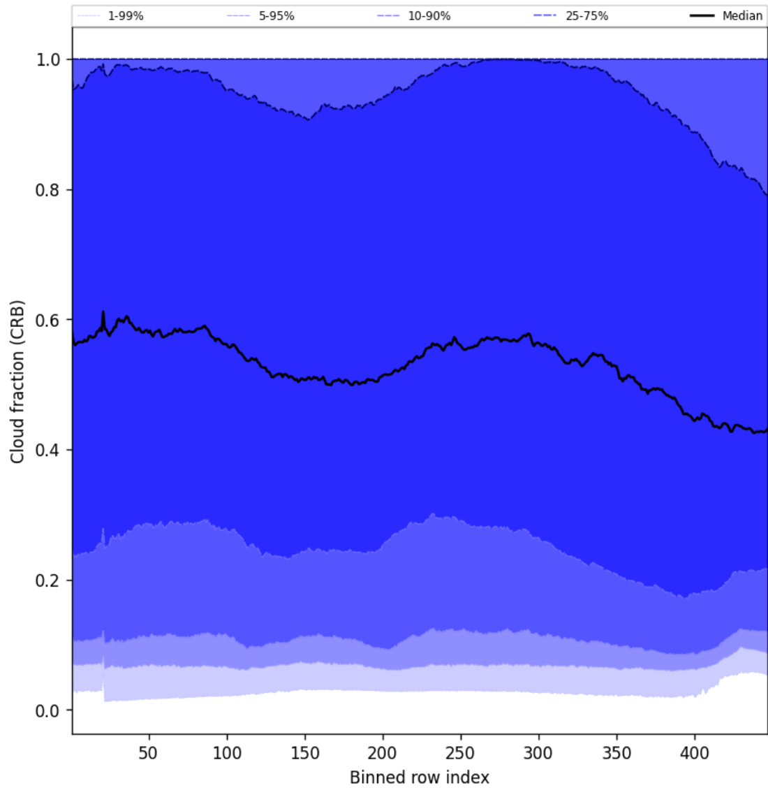
Figure 56: Along track statistics of “Cloud fraction (CRB)” for 2025-04-06 to 2025-04-06
