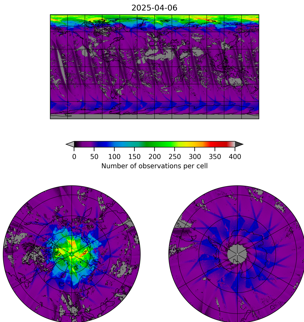
Figure 19: Map of the number of observations for 2025-04-06 to 2025-04-06
