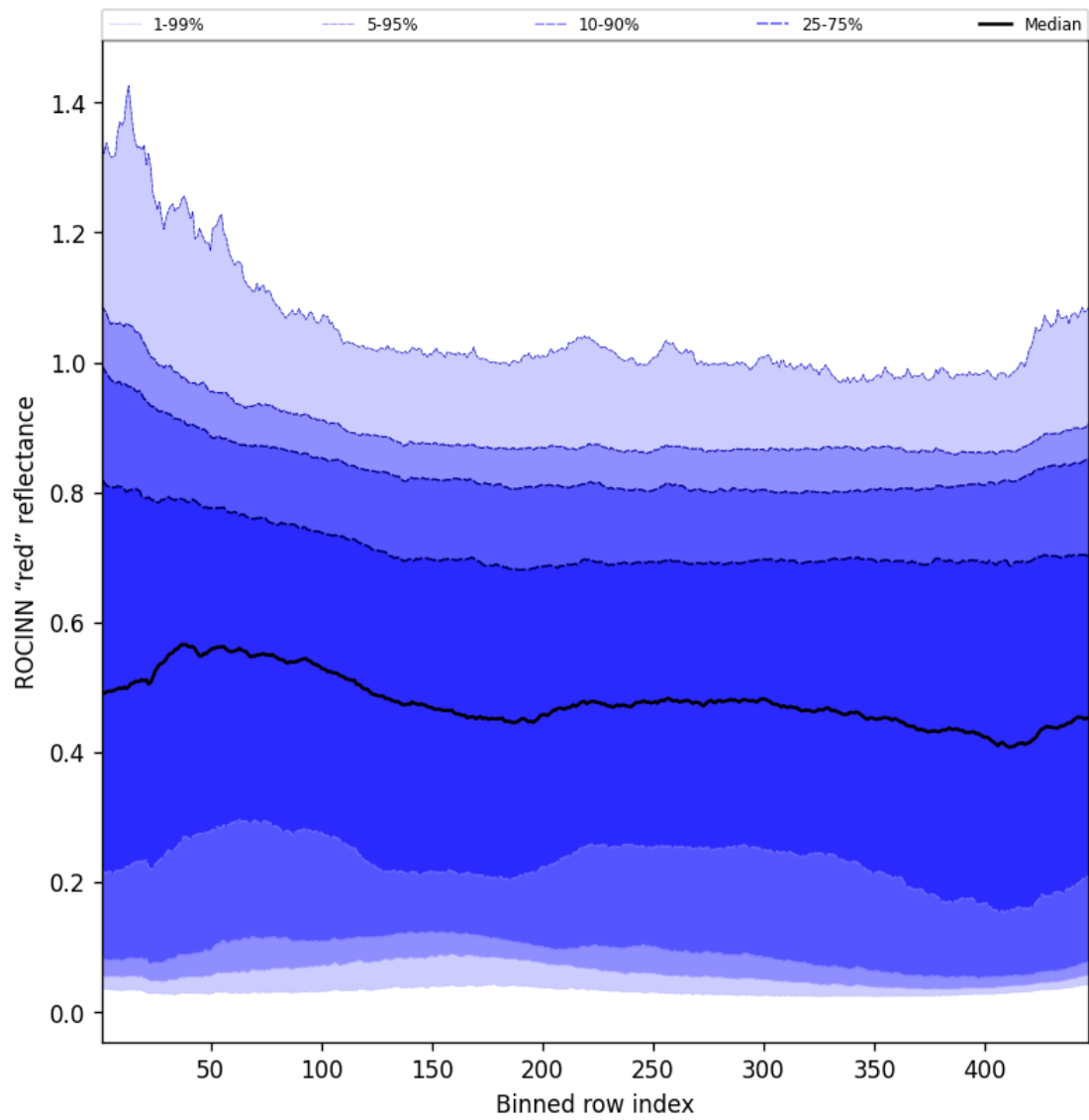
Figure 67: Along track statistics of "ROCINN "red" reflectance" for 2025-04-08 to 2025-04-09
