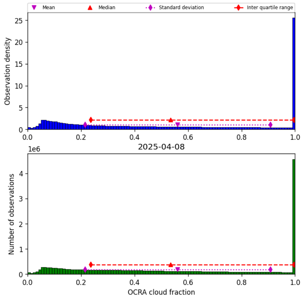
Figure 48: Histogram of “OCRA cloud fraction” for 2025-04-08 to 2025-04-09
