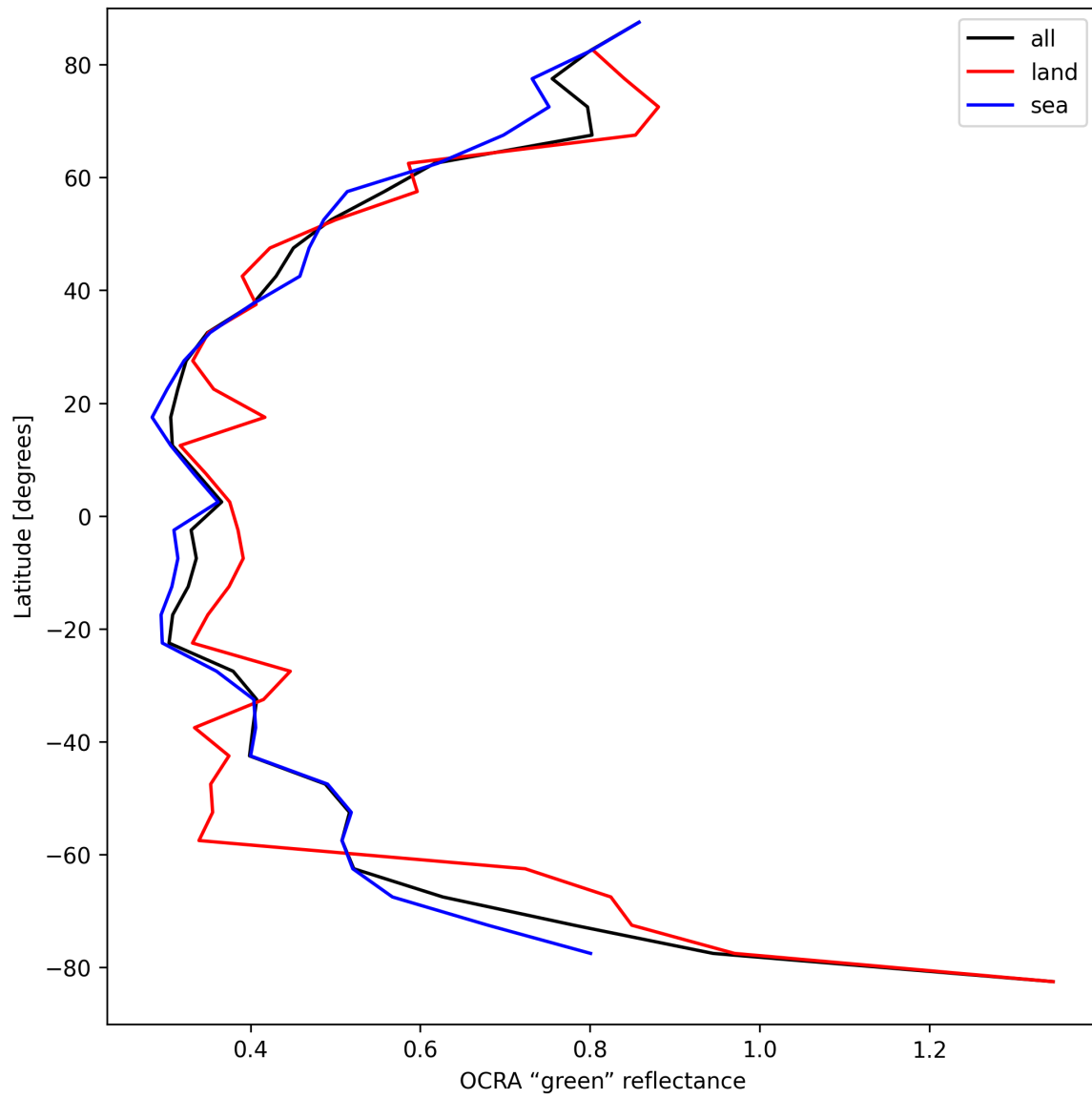
Figure 34: Zonal average of “OCRA “green” reflectance” for 2025-04-08 to 2025-04-09.
