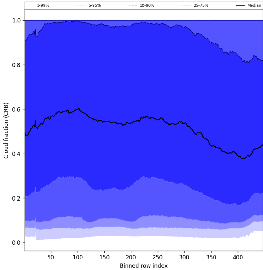
Figure 56: Along track statistics of “Cloud fraction (CRB)” for 2025-04-08 to 2025-04-09
