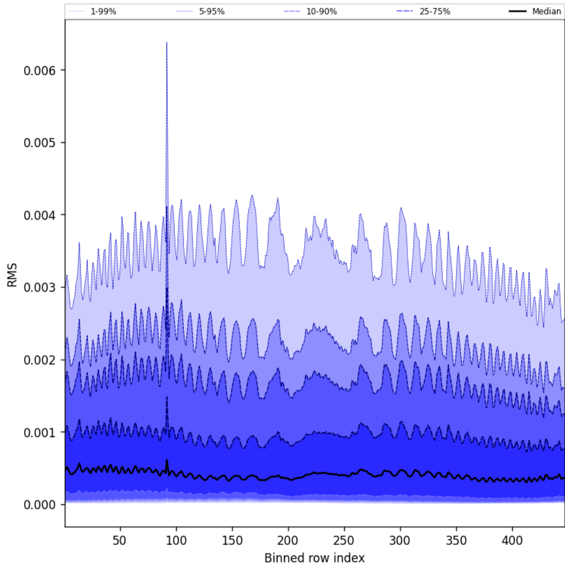
Figure 61: Along track statistics of “RMS” for 2025-04-08 to 2025-04-09
