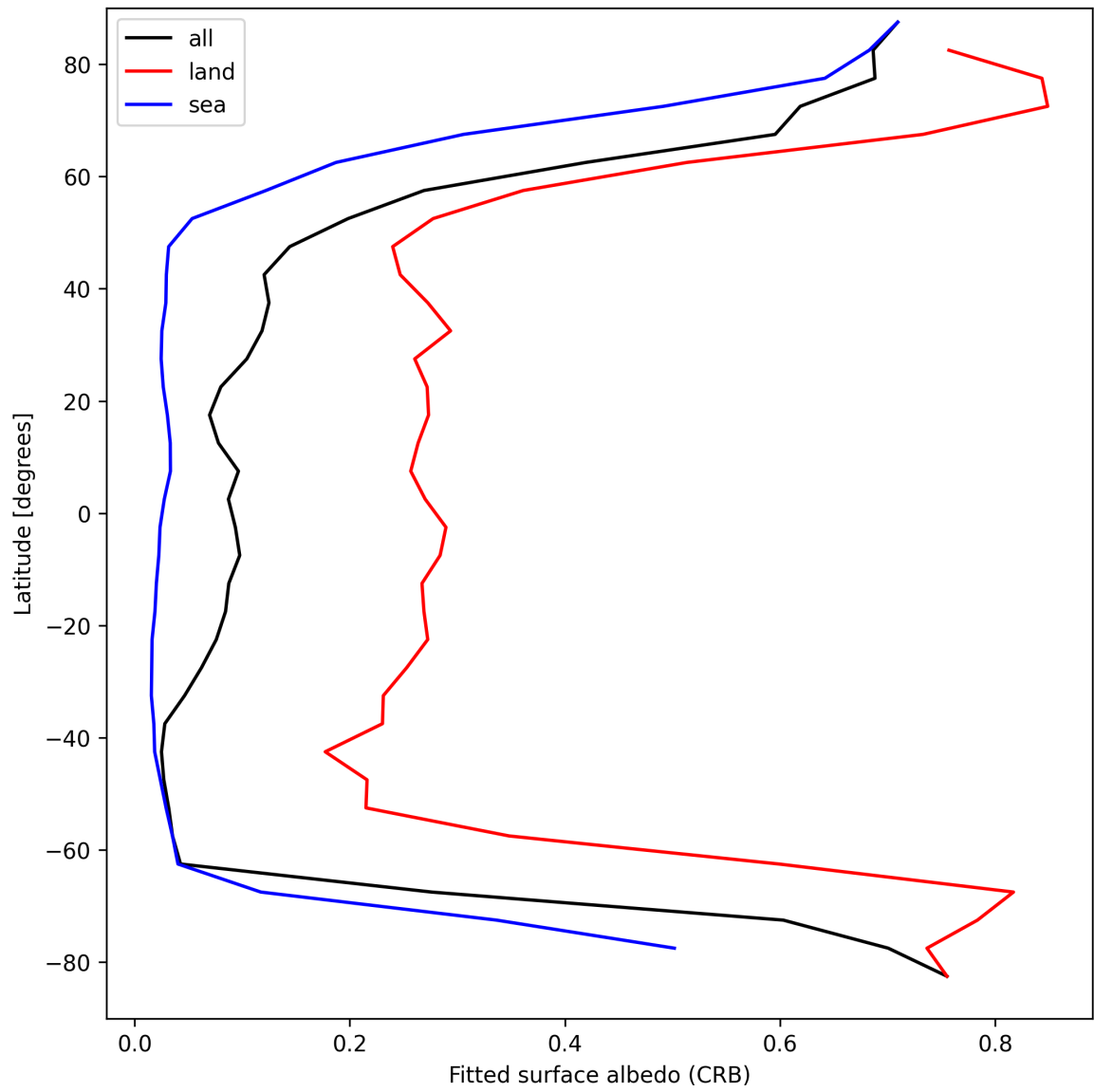
Figure 28: Zonal average of “Fitted surface albedo (CRB)” for 2025-04-08 to 2025-04-09.
