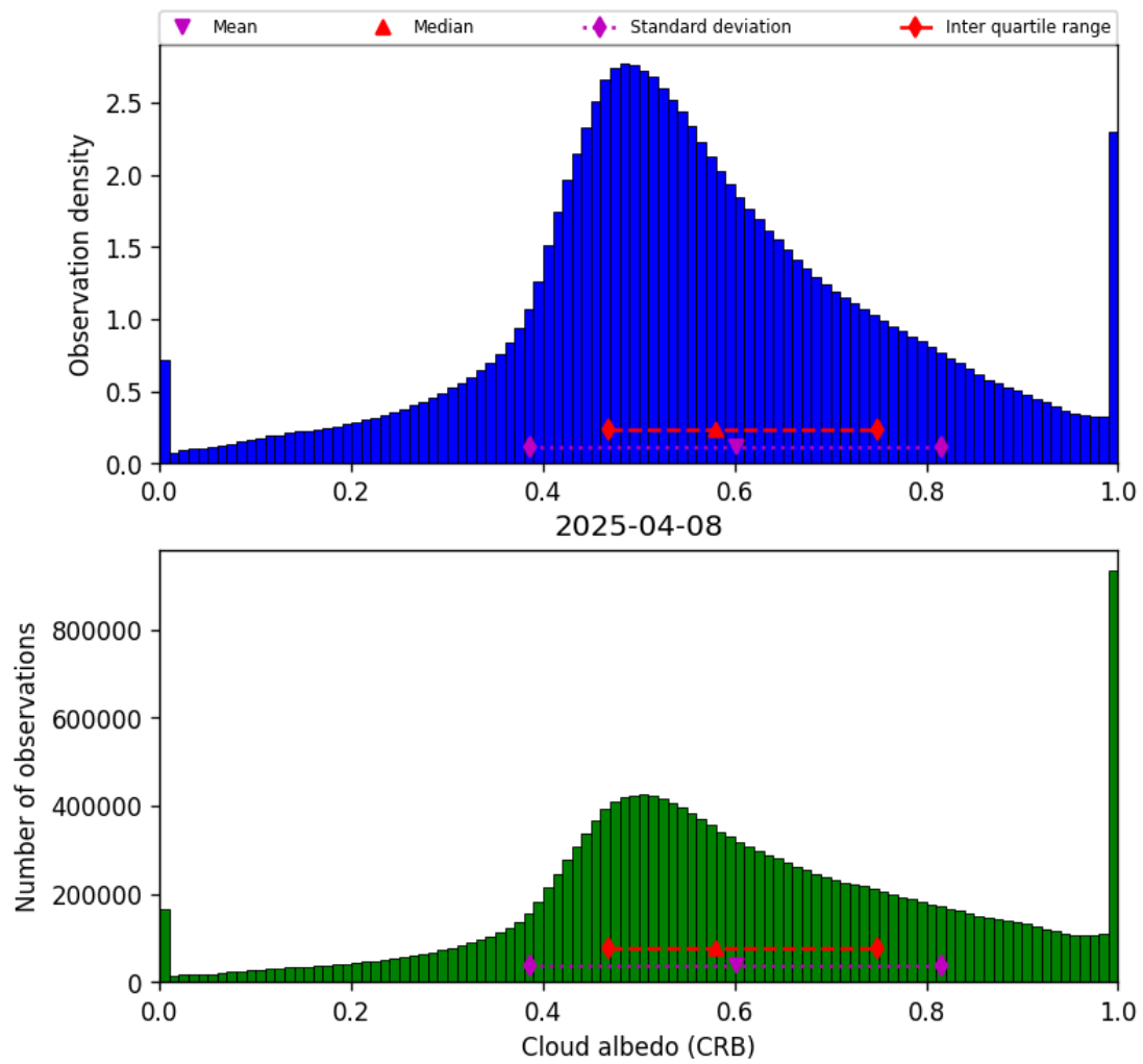
Figure 42: Histogram of “Cloud albedo (CRB)” for 2025-04-08 to 2025-04-09
