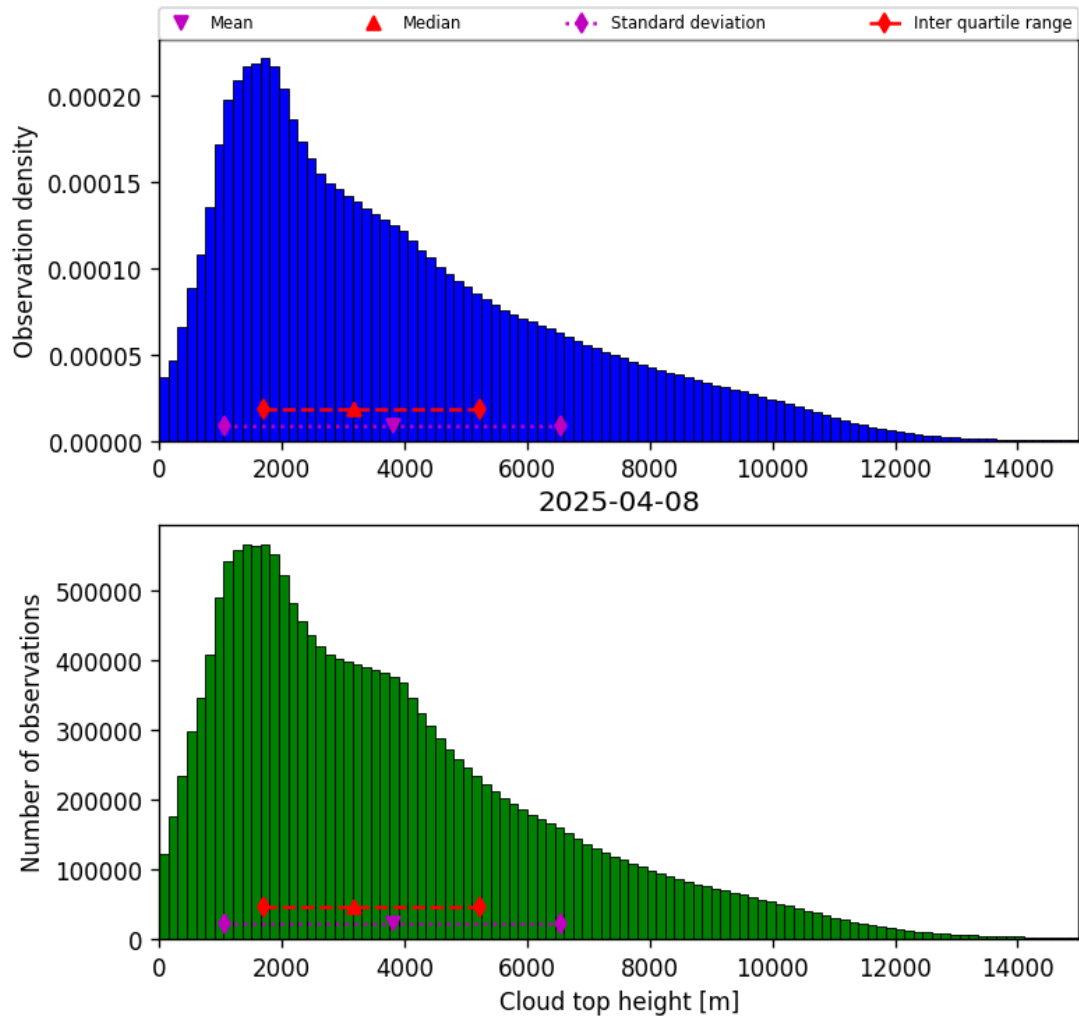
Figure 38: Histogram of “Cloud top height” for 2025-04-08 to 2025-04-09
