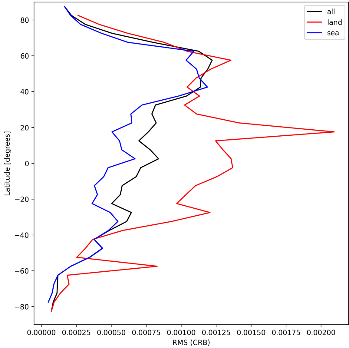
Figure 30: Zonal average of “RMS (CRB)” for 2025-04-08 to 2025-04-09.
