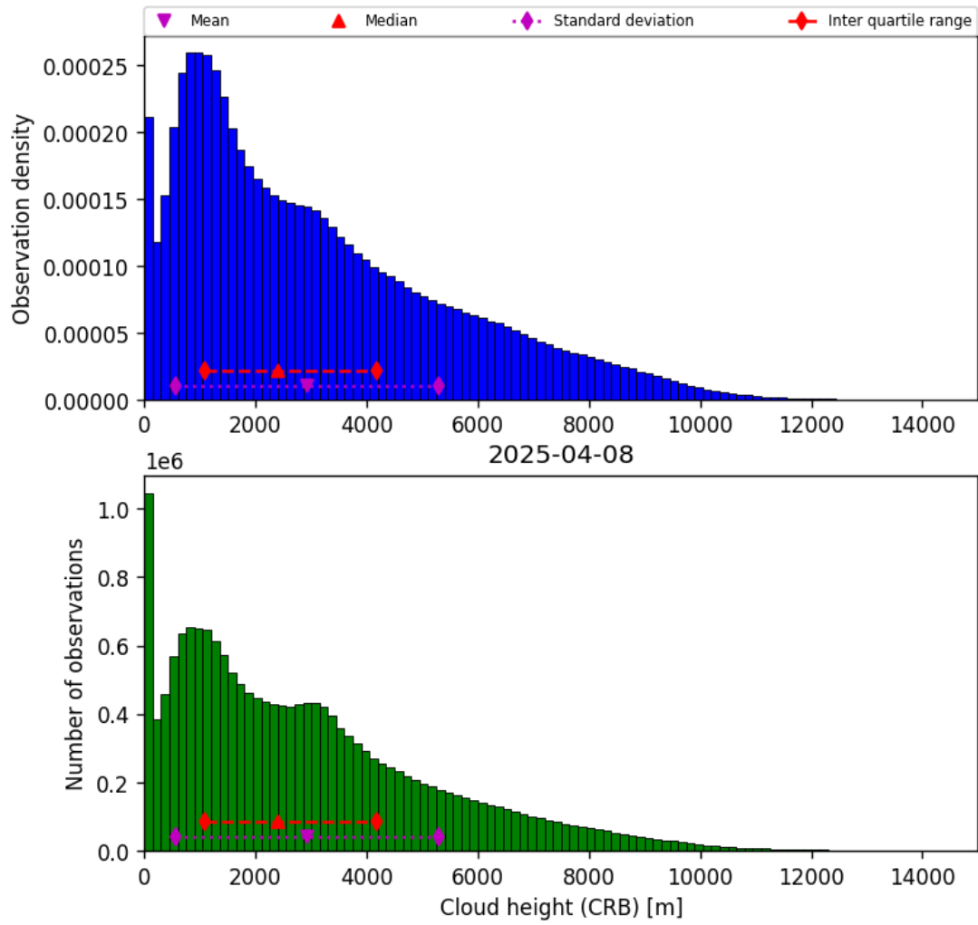
Figure 41: Histogram of “Cloud height (CRB)” for 2025-04-08 to 2025-04-09
