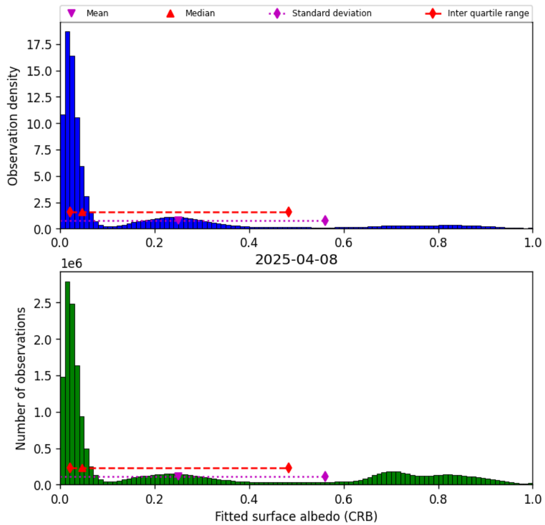
Figure 44: Histogram of “Fitted surface albedo (CRB)” for 2025-04-08 to 2025-04-09
