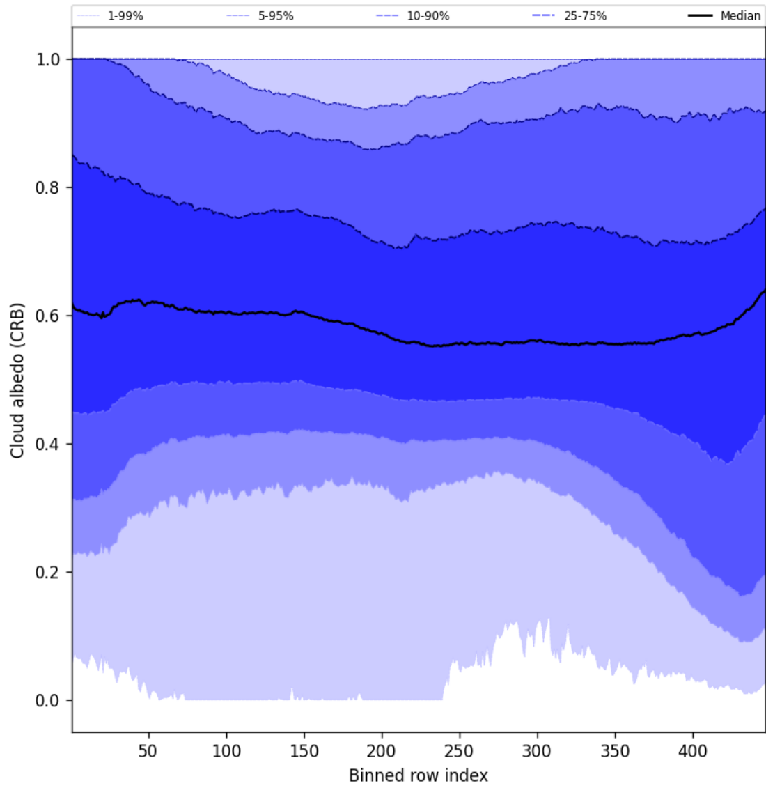
Figure 58: Along track statistics of “Cloud albedo (CRB)” for 2025-04-08 to 2025-04-09
