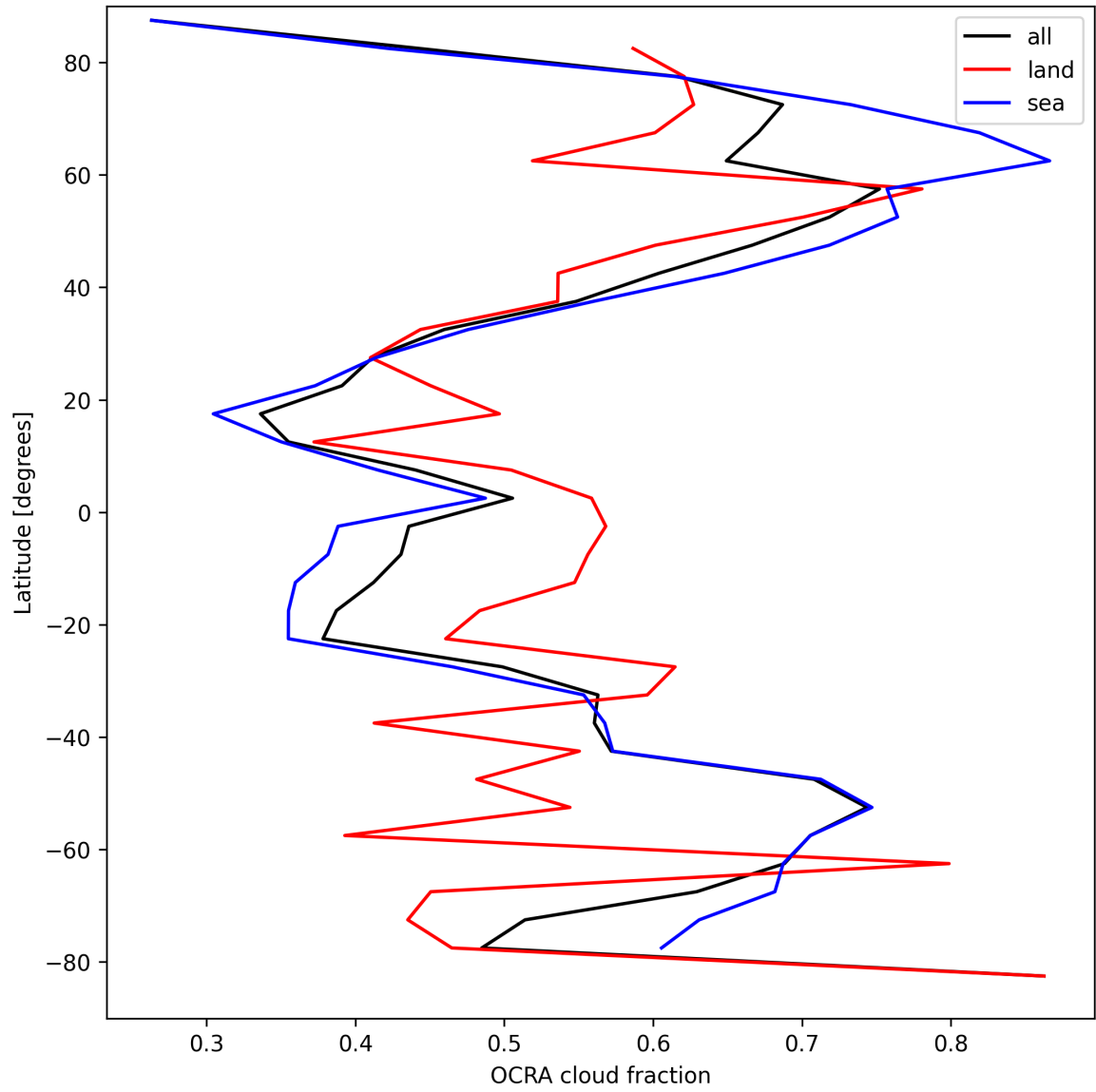
Figure 32: Zonal average of “OCRA cloud fraction” for 2025-04-08 to 2025-04-09.
