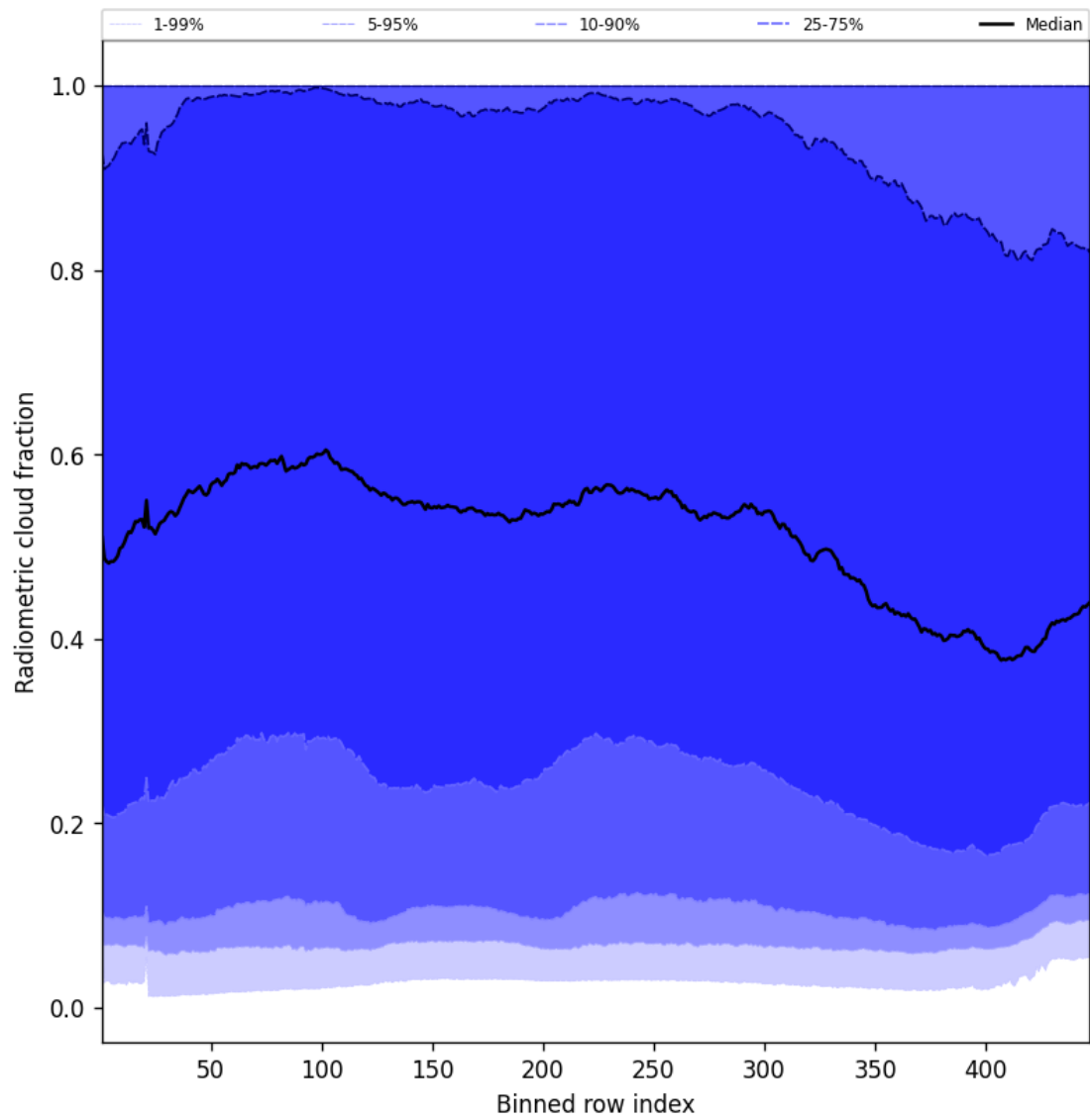
Figure 53: Along track statistics of “Radiometric cloud fraction” for 2025-04-08 to 2025-04-09
