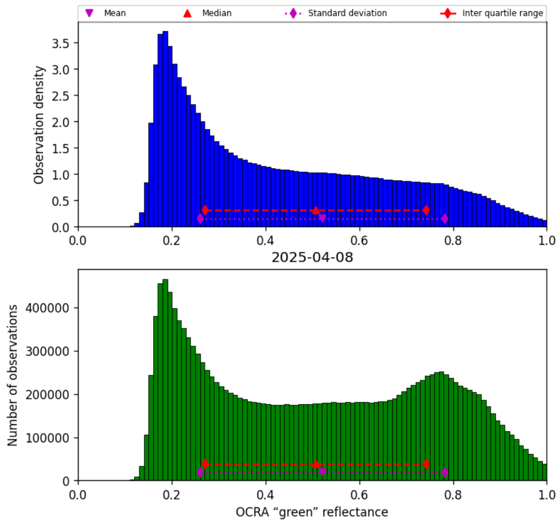
Figure 50: Histogram of “OCRA “green” reflectance” for 2025-04-08 to 2025-04-09
