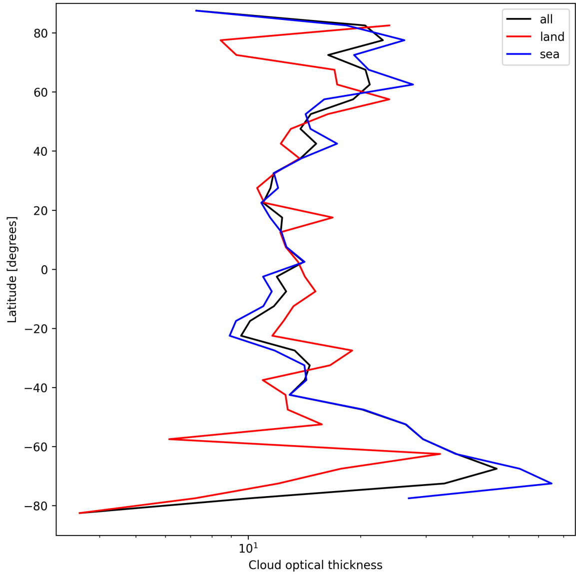
Figure 23: Zonal average of “Cloud optical thickness” for 2025-04-08 to 2025-04-09.
