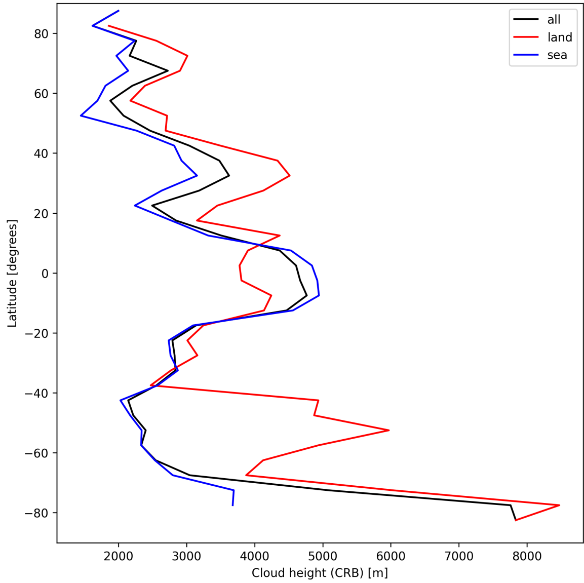
Figure 25: Zonal average of “Cloud height (CRB)” for 2025-04-08 to 2025-04-09.
