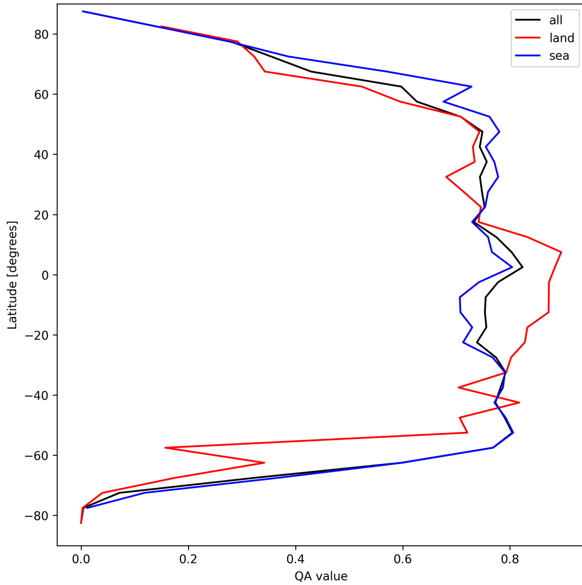
Figure 20: Zonal average of “QA value” for 2025-04-08 to 2025-04-09.
