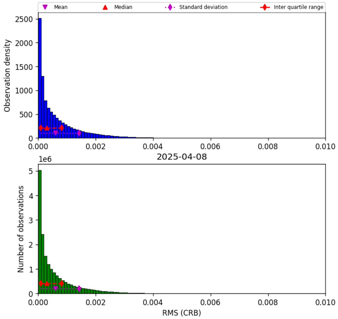
Figure 46: Histogram of “RMS (CRB)” for 2025-04-08 to 2025-04-09
