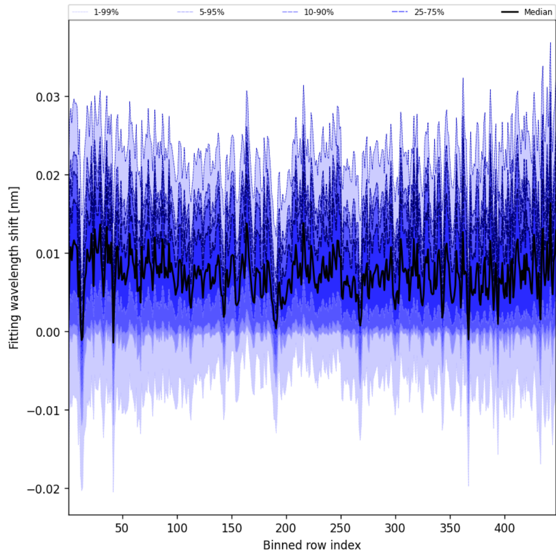
Figure 63: Along track statistics of “Fitting wavelength shift” for 2025-04-08 to 2025-04-09
