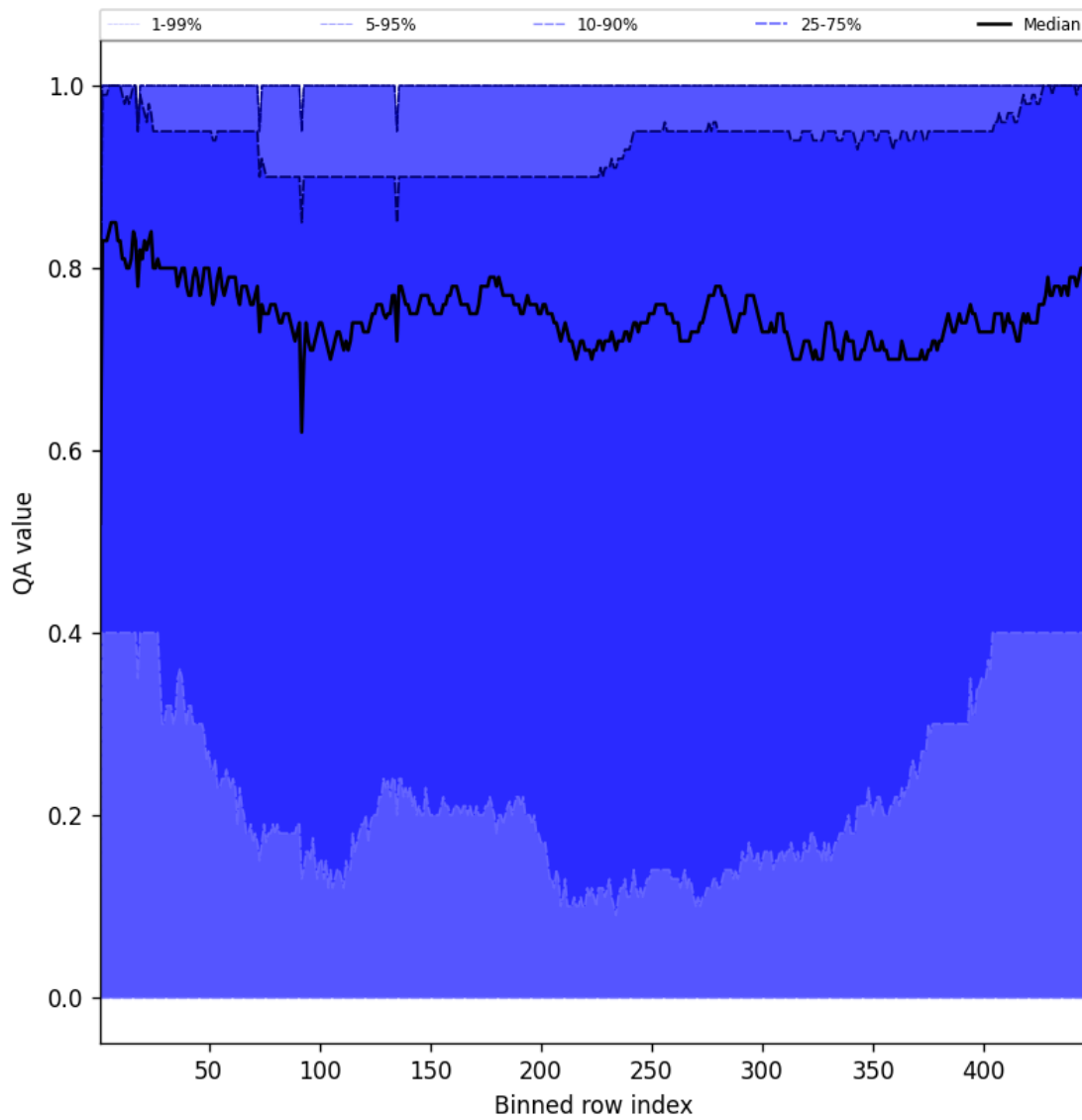
Figure 52: Along track statistics of “QA value” for 2025-04-08 to 2025-04-09
