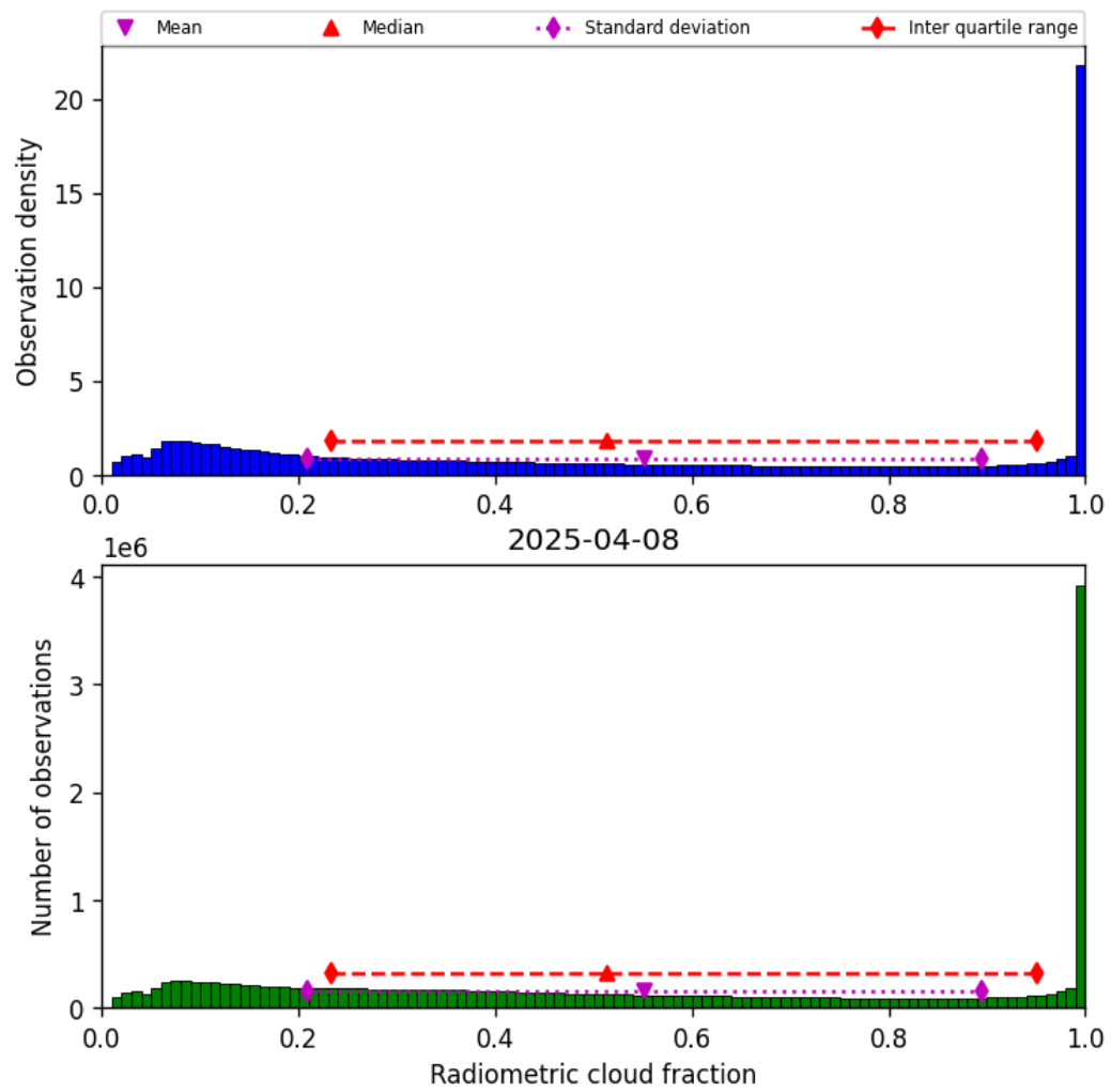
Figure 37: Histogram of “Radiometric cloud fraction” for 2025-04-08 to 2025-04-09
