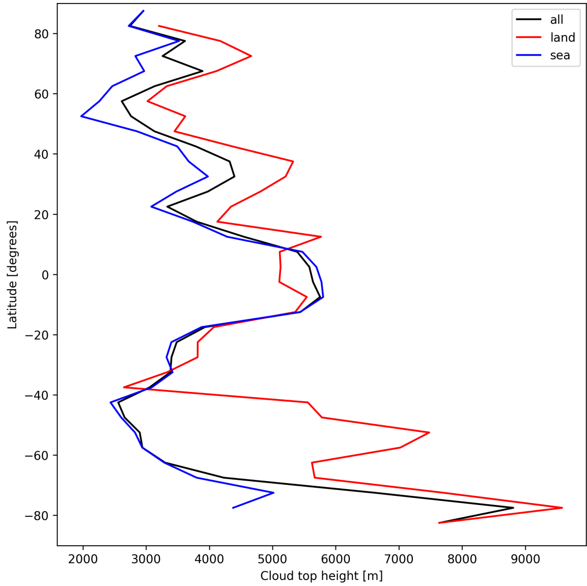
Figure 22: Zonal average of “Cloud top height” for 2025-04-08 to 2025-04-09.
