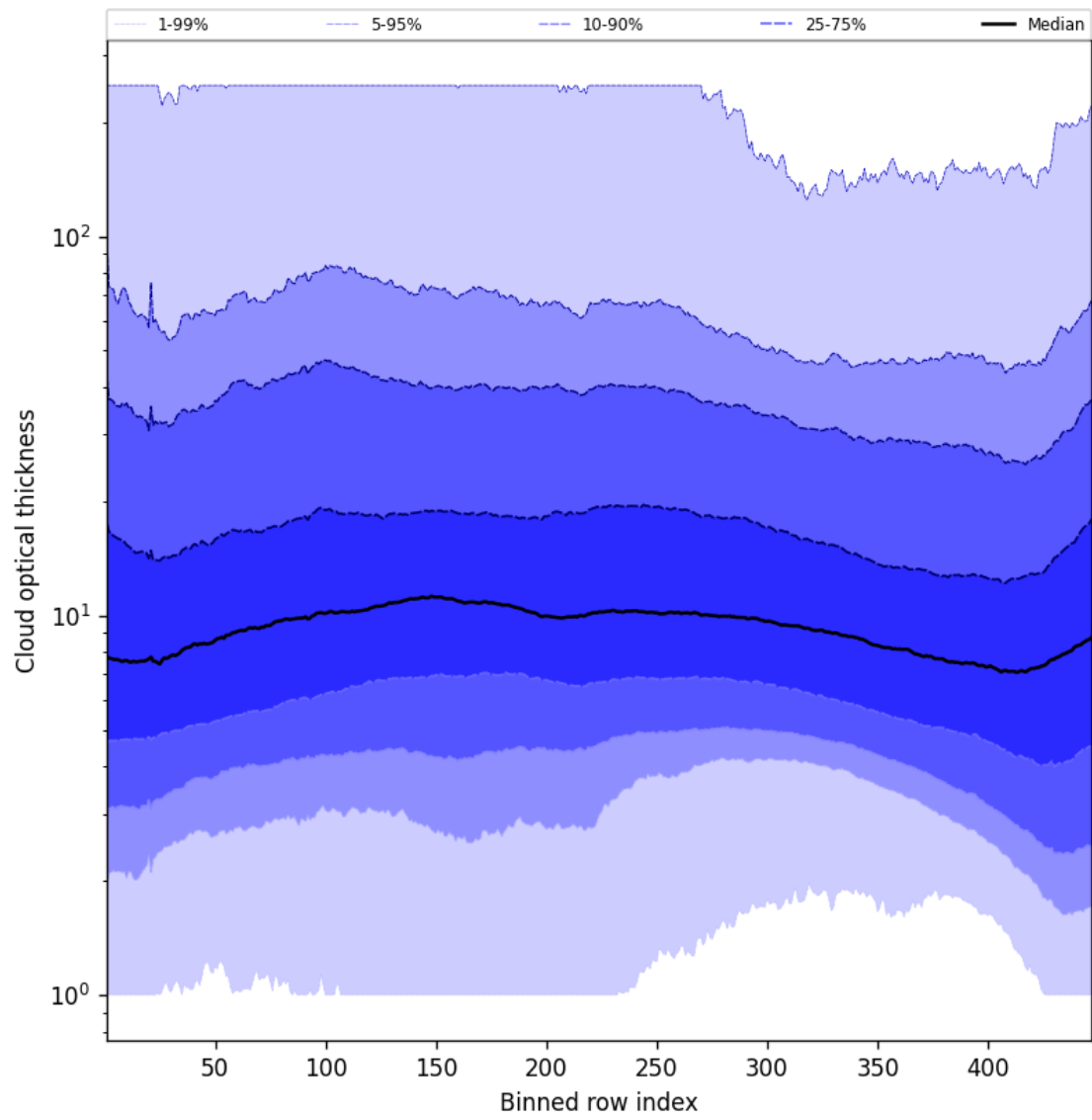
Figure 55: Along track statistics of “Cloud optical thickness” for 2025-04-08 to 2025-04-09
