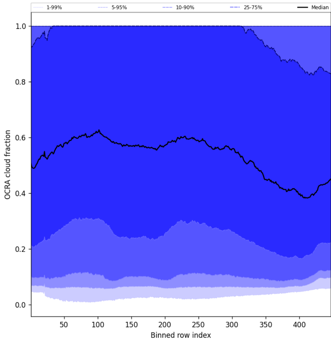
Figure 64: Along track statistics of “OCRA cloud fraction” for 2025-04-08 to 2025-04-09
