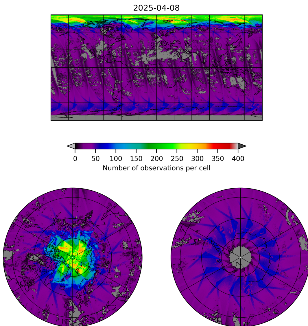
Figure 19: Map of the number of observations for 2025-04-08 to 2025-04-09
