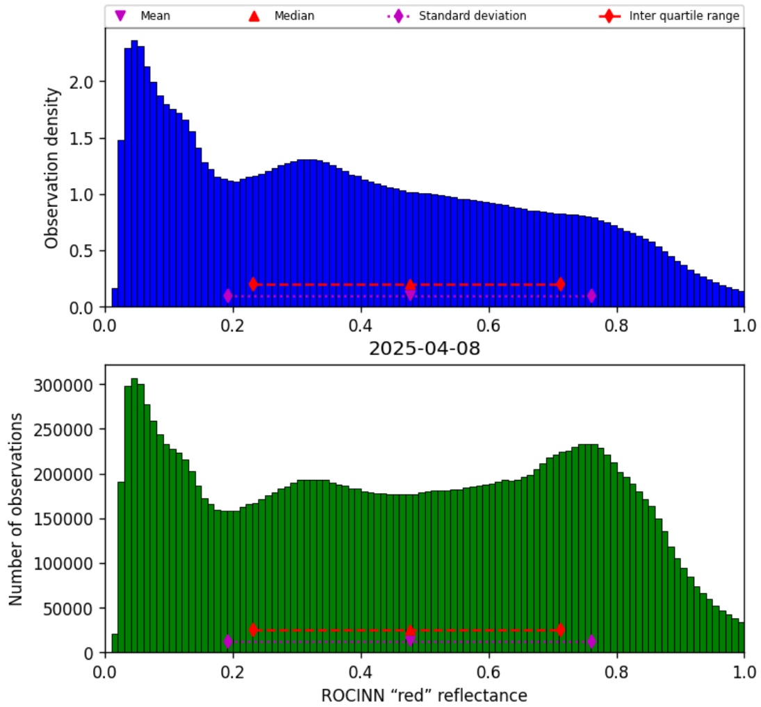
Figure 51: Histogram of “ROCINN “red” reflectance” for 2025-04-08 to 2025-04-09
