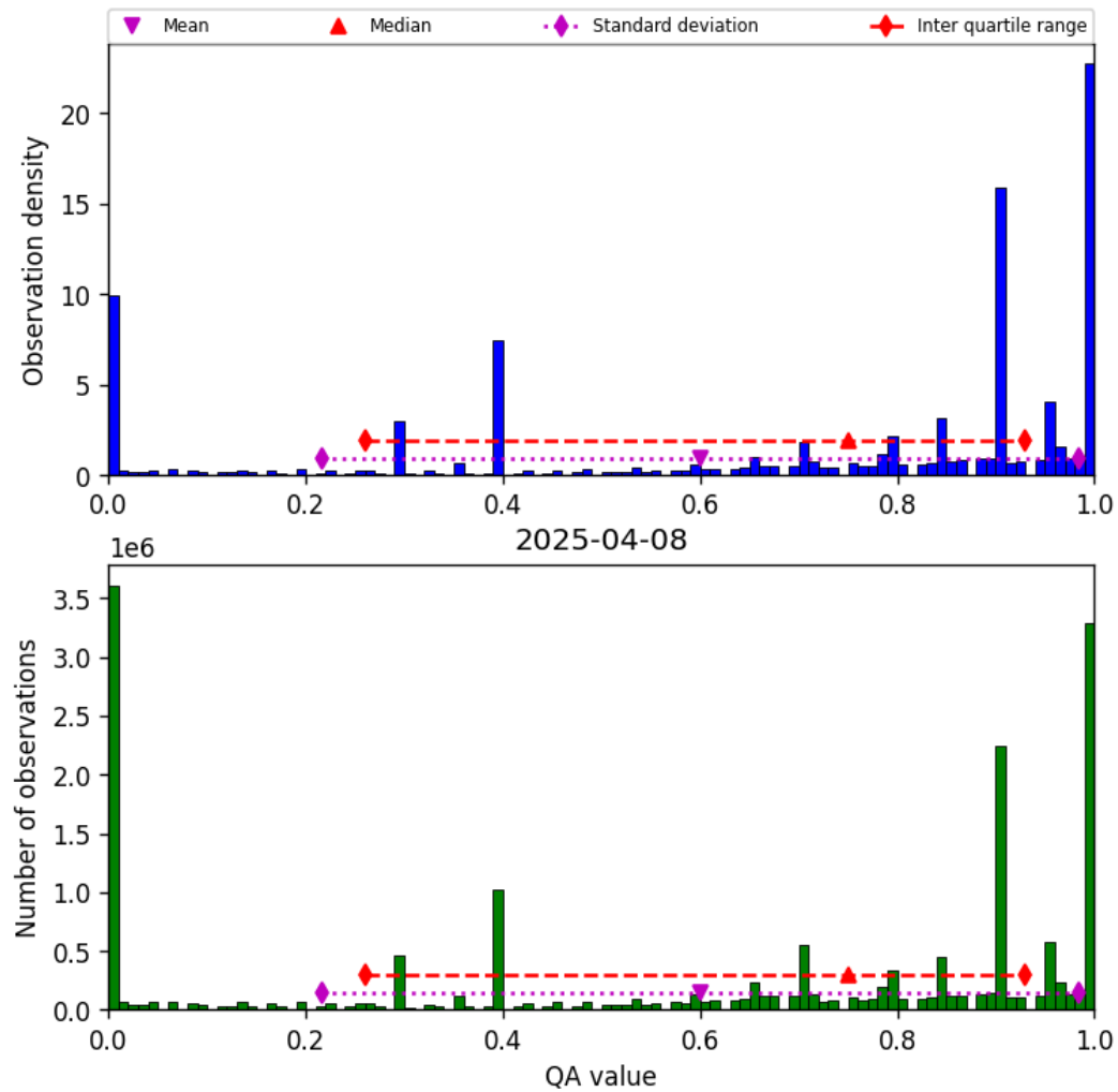
Figure 36: Histogram of “QA value” for 2025-04-08 to 2025-04-09
