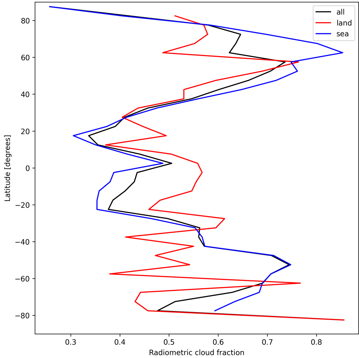
Figure 21: Zonal average of “Radiometric cloud fraction” for 2025-04-08 to 2025-04-09.
