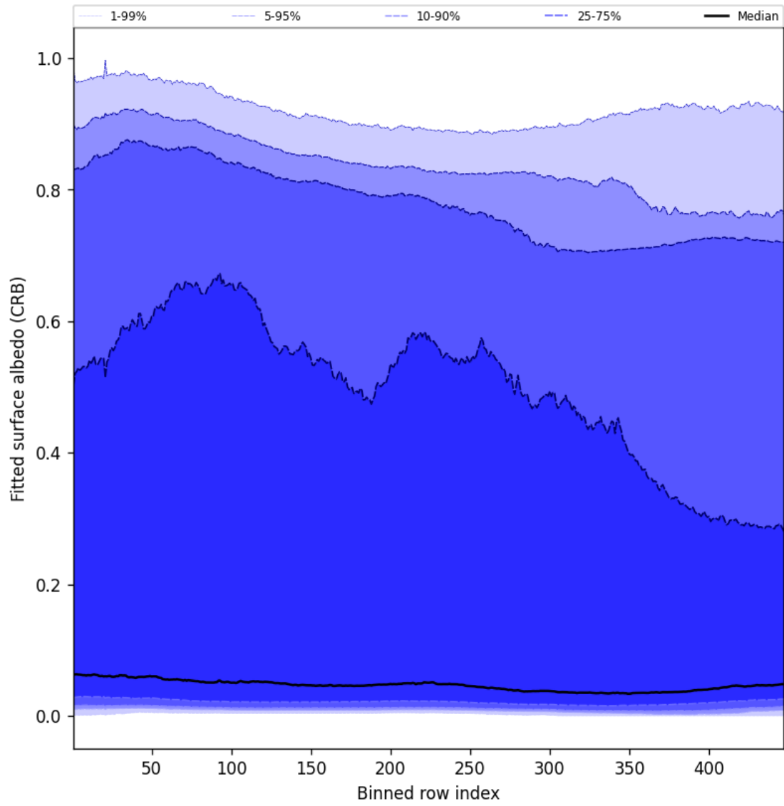
Figure 60: Along track statistics of “Fitted surface albedo (CRB)” for 2025-04-08 to 2025-04-09
