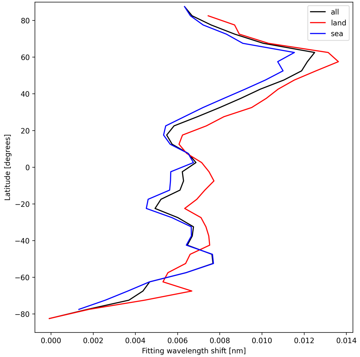
Figure 31: Zonal average of “Fitting wavelength shift” for 2025-04-08 to 2025-04-09.
