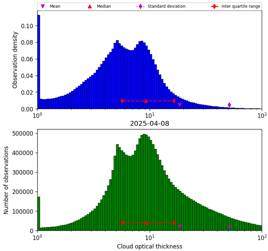
Figure 39: Histogram of “Cloud optical thickness” for 2025-04-08 to 2025-04-09
