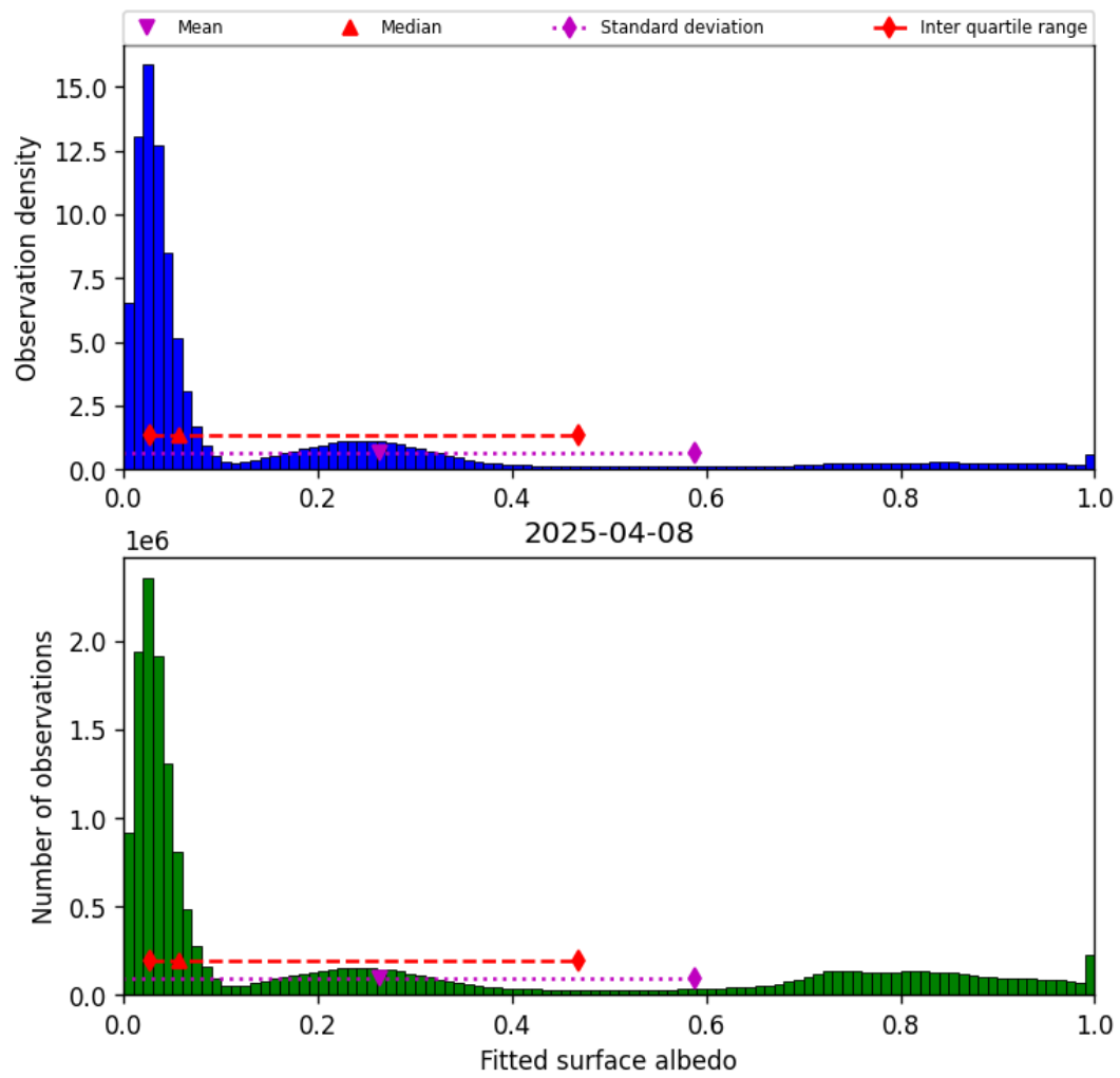
Figure 43: Histogram of “Fitted surface albedo” for 2025-04-08 to 2025-04-09
