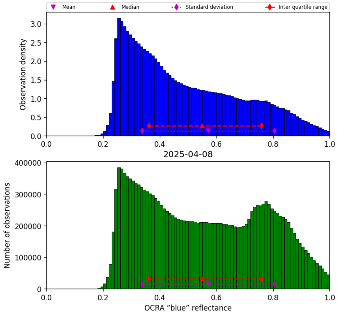
Figure 49: Histogram of “OCRA “blue” reflectance” for 2025-04-08 to 2025-04-09
