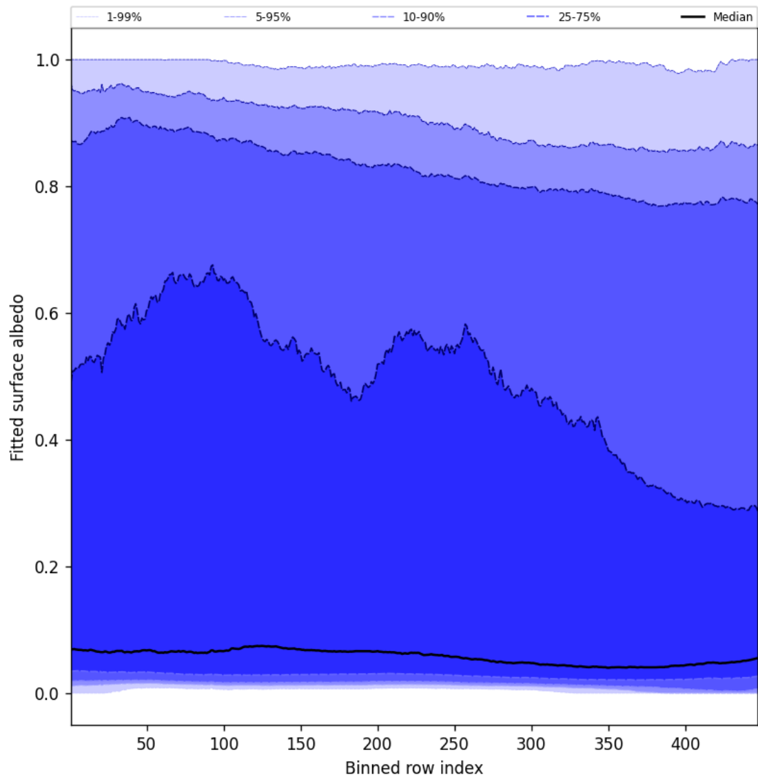
Figure 59: Along track statistics of “Fitted surface albedo” for 2025-04-08 to 2025-04-09
