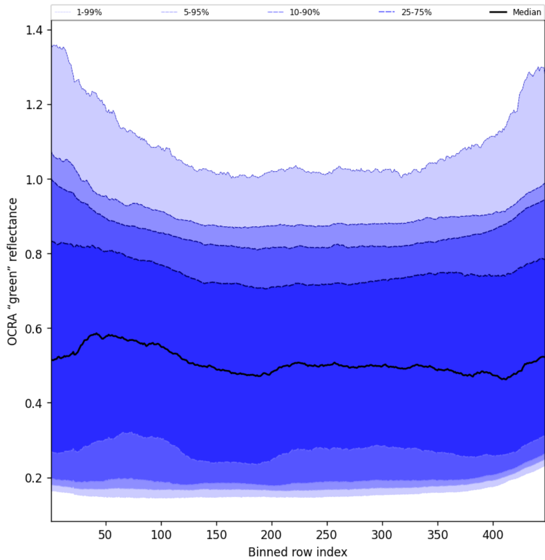
Figure 66: Along track statistics of “OCRA “green” reflectance” for 2025-04-08 to 2025-04-09
