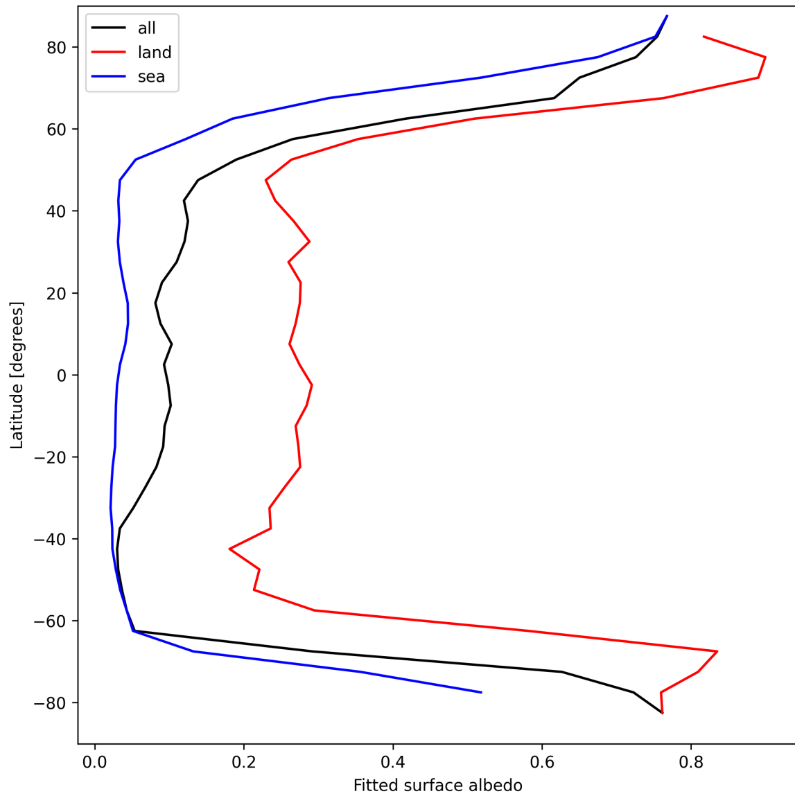
Figure 27: Zonal average of “Fitted surface albedo” for 2025-04-08 to 2025-04-09.
