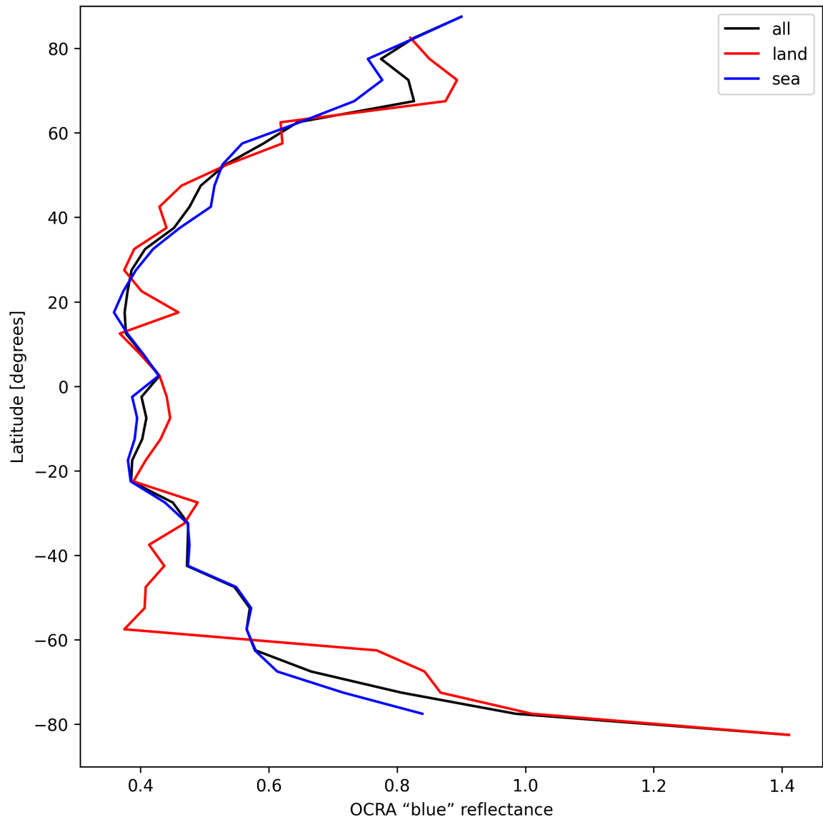
Figure 33: Zonal average of “OCRA “blue” reflectance” for 2025-04-08 to 2025-04-09.
