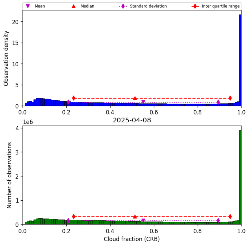
Figure 40: Histogram of “Cloud fraction (CRB)” for 2025-04-08 to 2025-04-09
