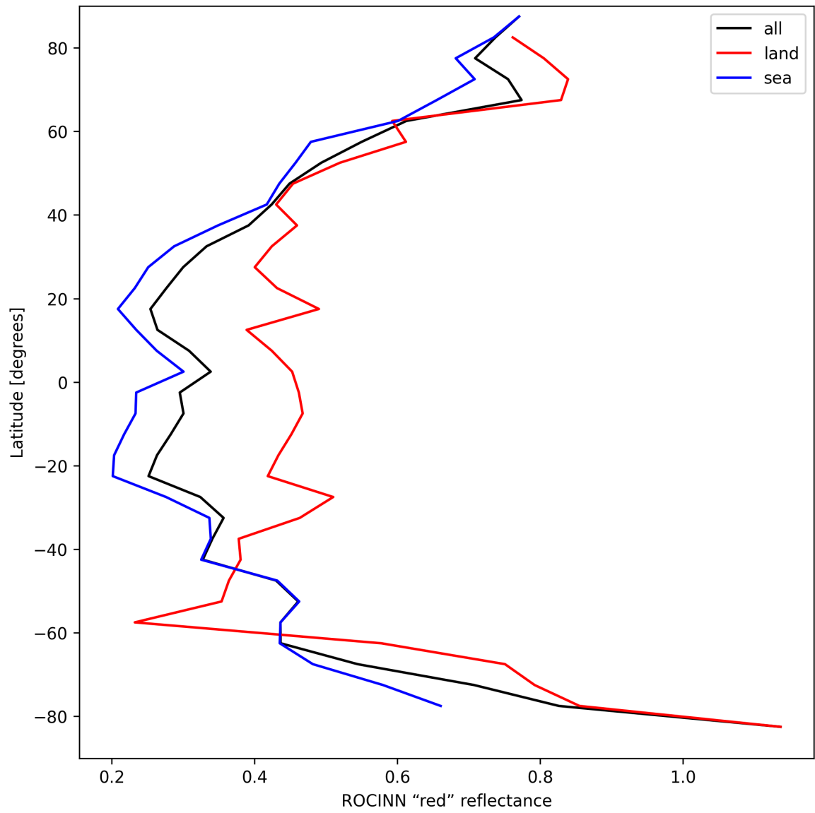
Figure 35: Zonal average of “ROCINN “red” reflectance” for 2025-04-08 to 2025-04-09.
