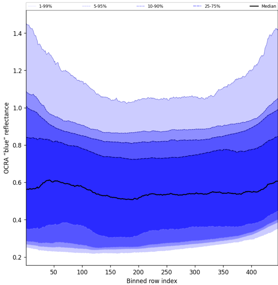
Figure 65: Along track statistics of “OCRA “blue” reflectance” for 2025-04-08 to 2025-04-09
