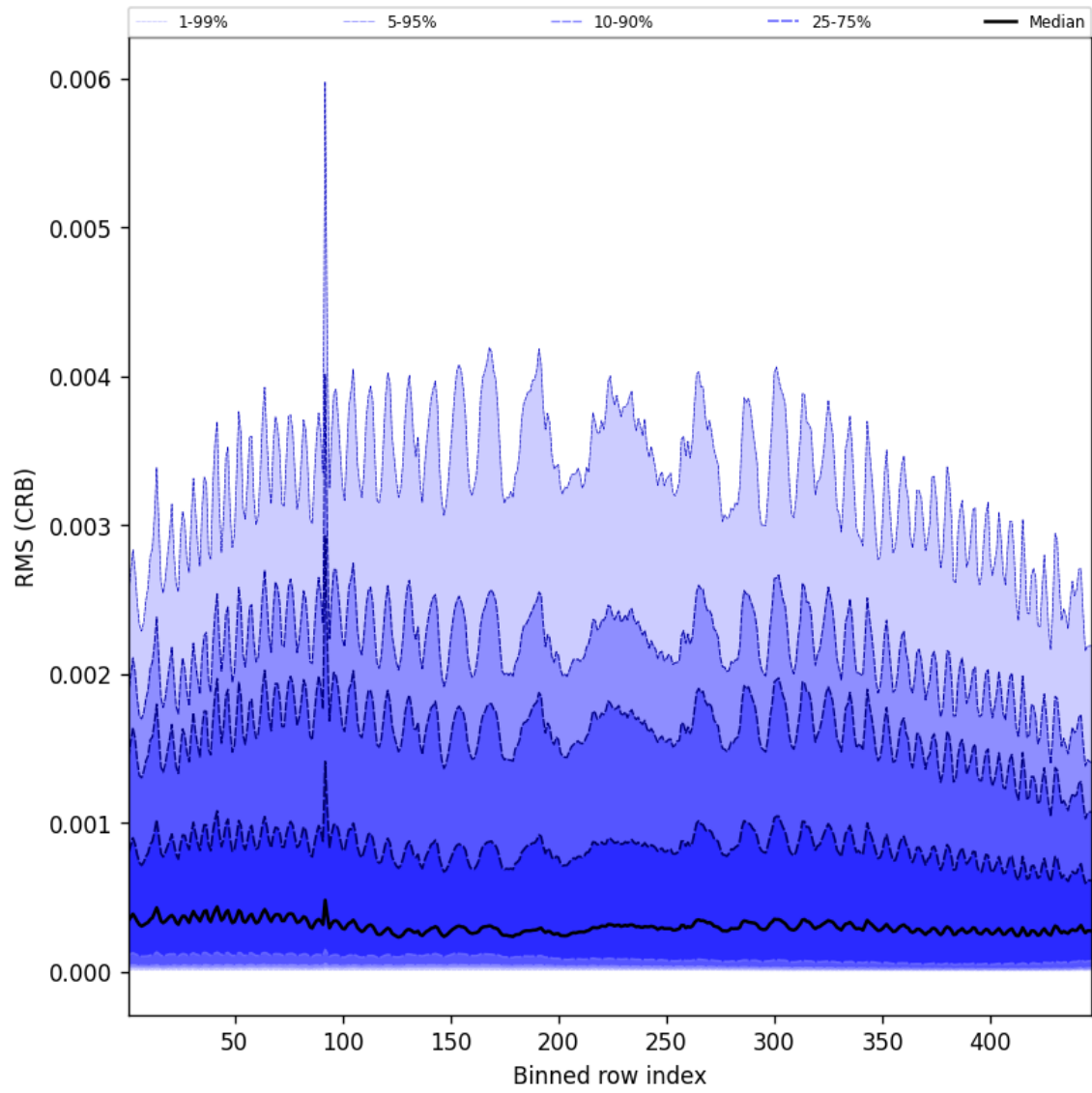
Figure 62: Along track statistics of “RMS (CRB)” for 2025-04-08 to 2025-04-09
