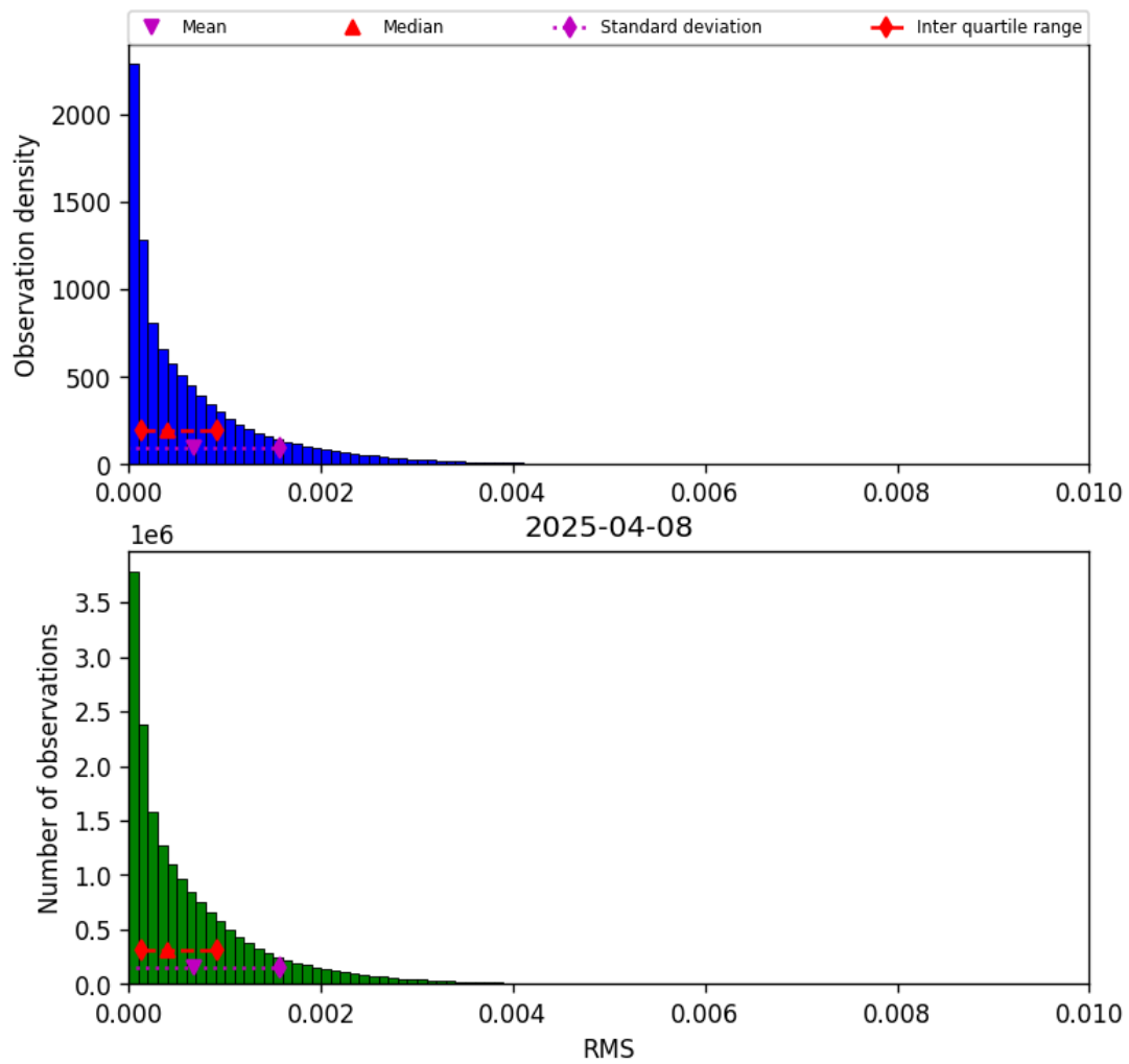
Figure 45: Histogram of “RMS” for 2025-04-08 to 2025-04-09
