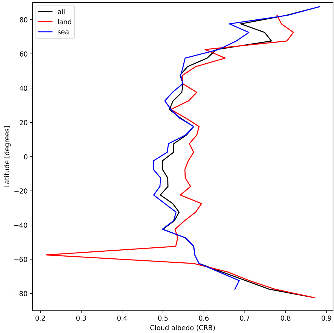
Figure 26: Zonal average of “Cloud albedo (CRB)” for 2025-04-08 to 2025-04-09.
