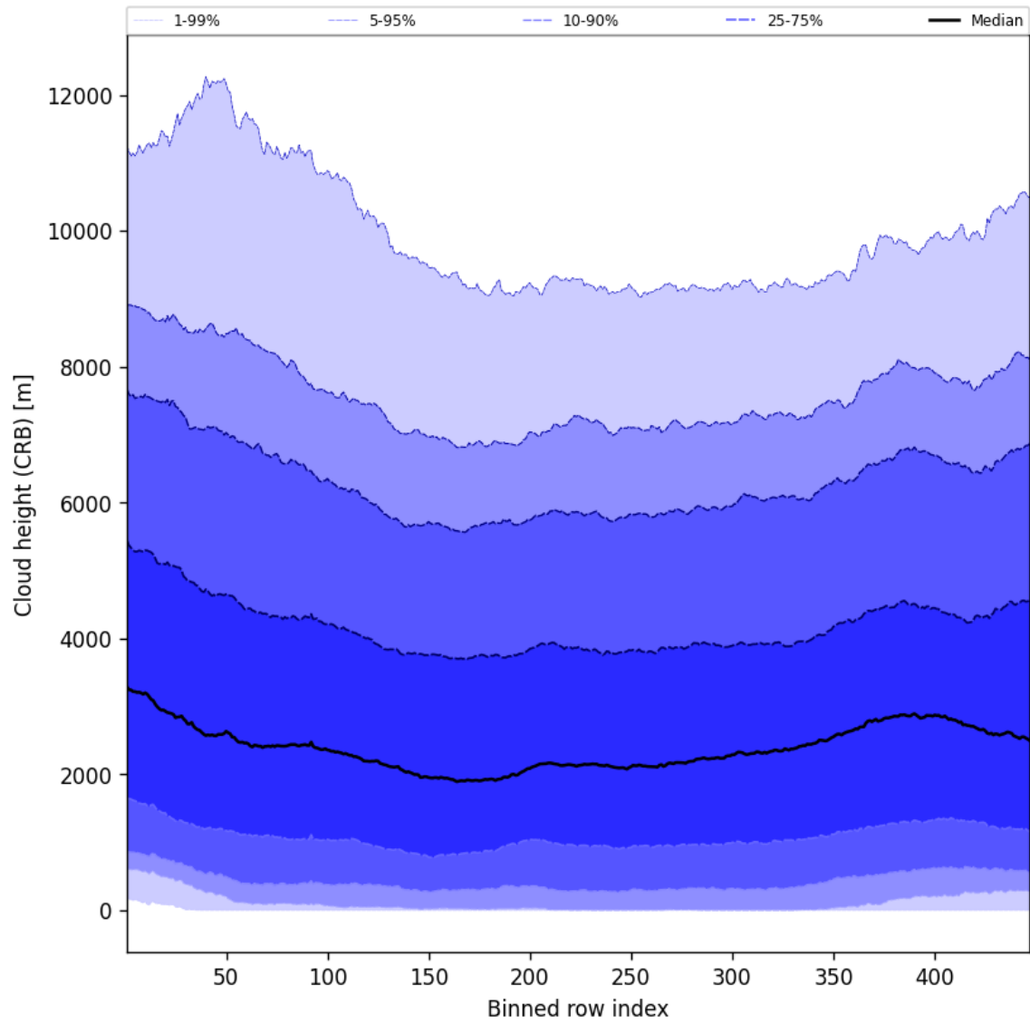
Figure 57: Along track statistics of “Cloud height (CRB)” for 2025-04-08 to 2025-04-09
