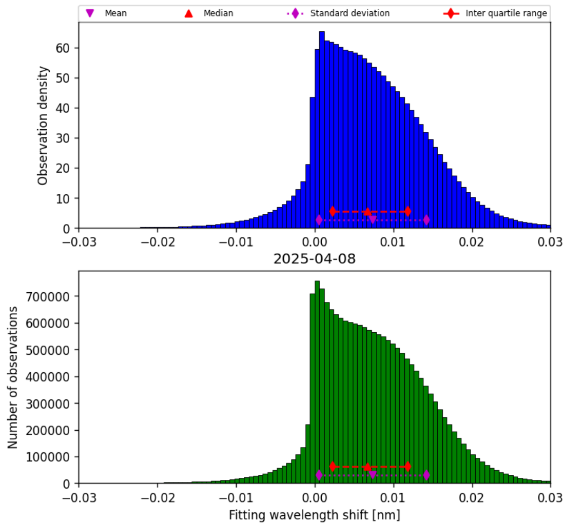
Figure 47: Histogram of “Fitting wavelength shift” for 2025-04-08 to 2025-04-09
