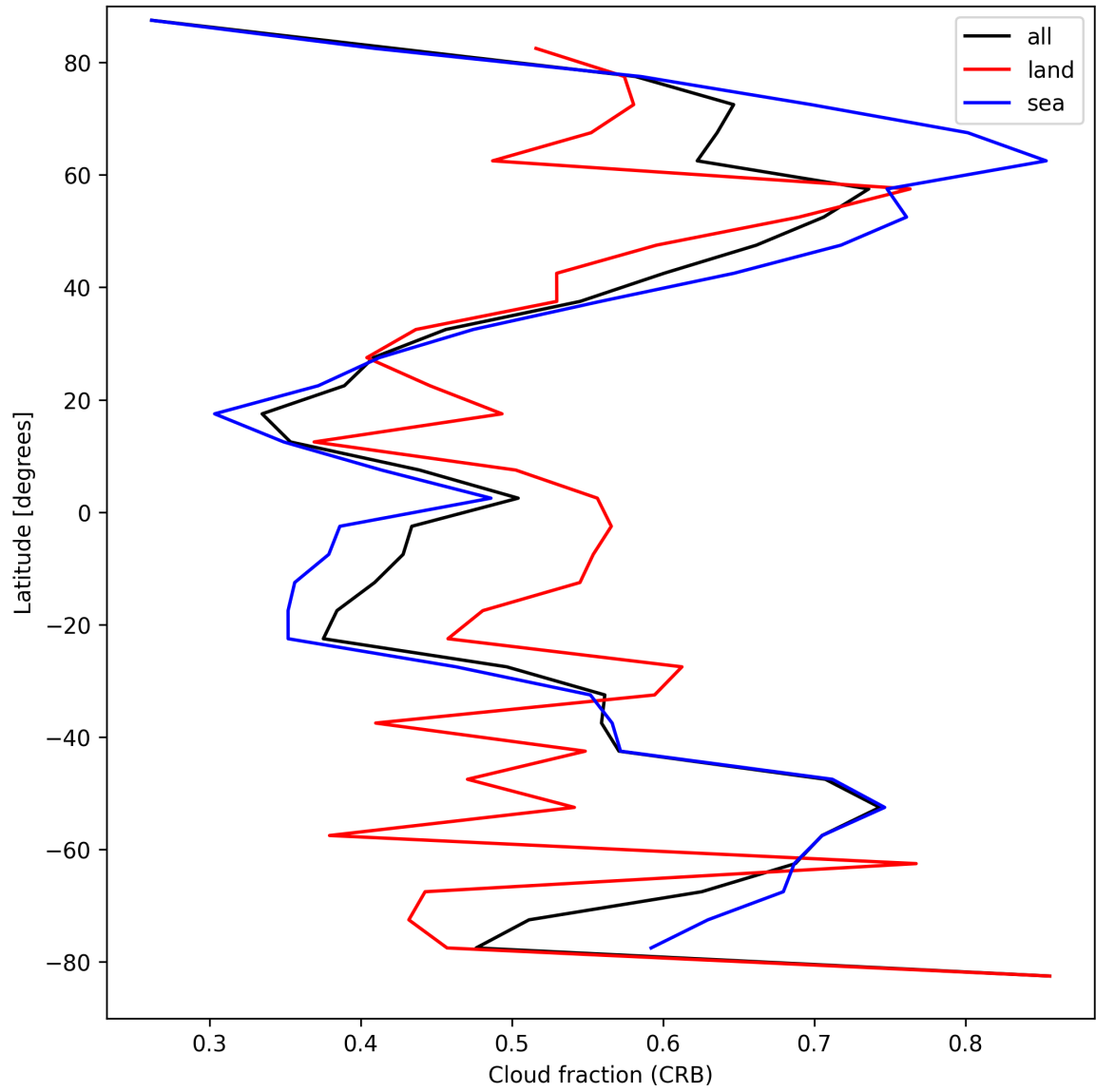
Figure 24: Zonal average of “Cloud fraction (CRB)” for 2025-04-08 to 2025-04-09.
