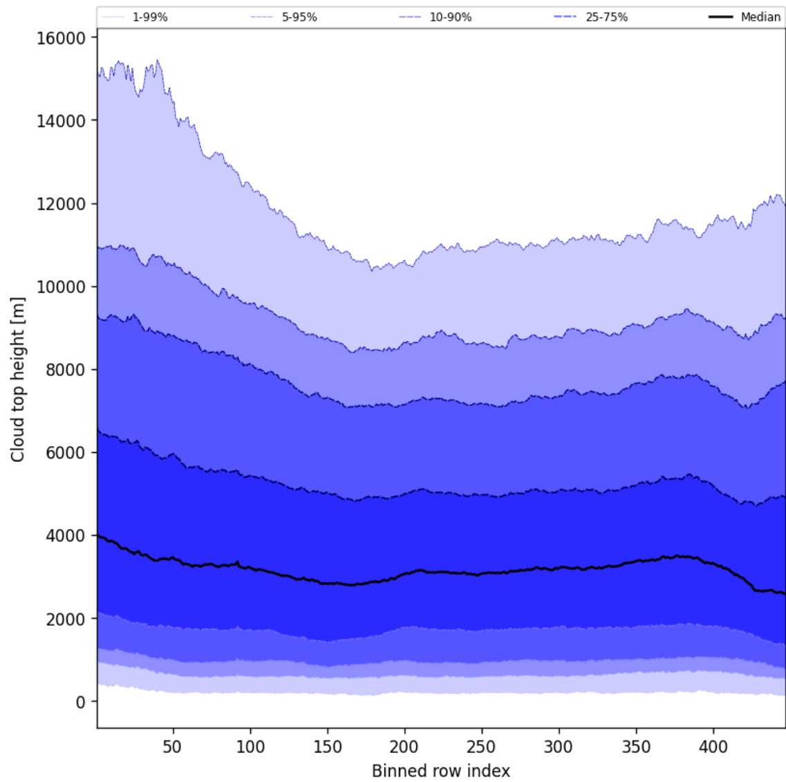
Figure 54: Along track statistics of “Cloud top height” for 2025-04-08 to 2025-04-09
