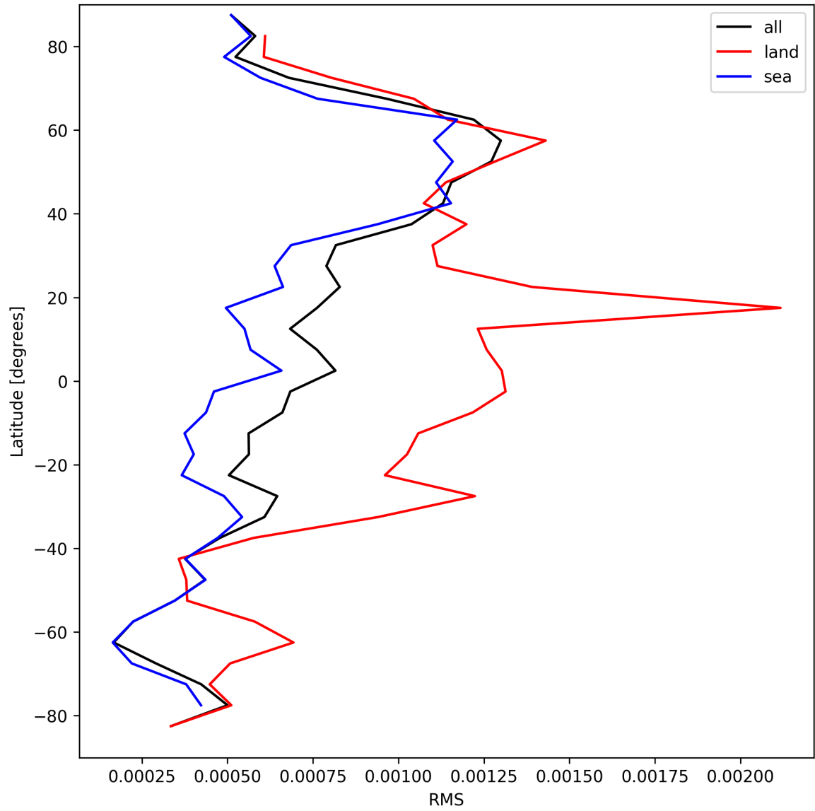
Figure 29: Zonal average of “RMS” for 2025-04-08 to 2025-04-09.
