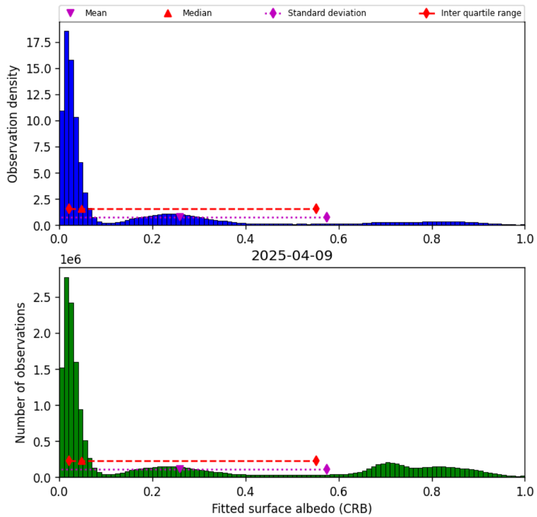
Figure 44: Histogram of “Fitted surface albedo (CRB)” for 2025-04-09 to 2025-04-10
