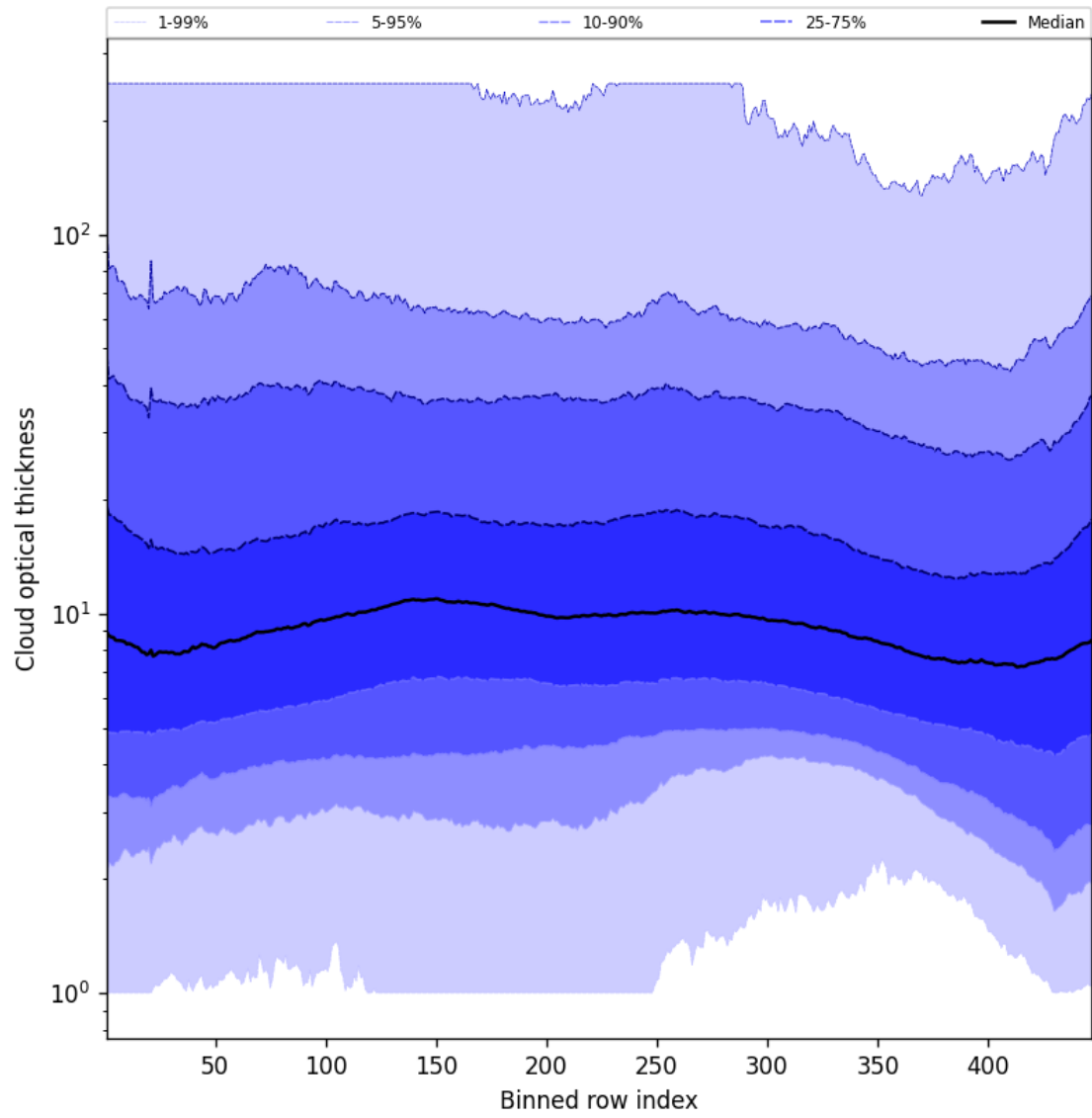
Figure 55: Along track statistics of “Cloud optical thickness” for 2025-04-09 to 2025-04-10
