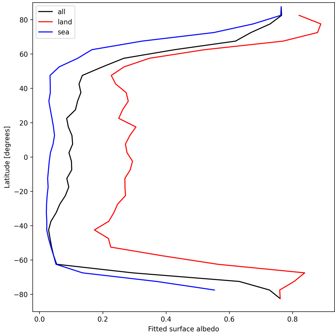
Figure 27: Zonal average of “Fitted surface albedo” for 2025-04-09 to 2025-04-10.
