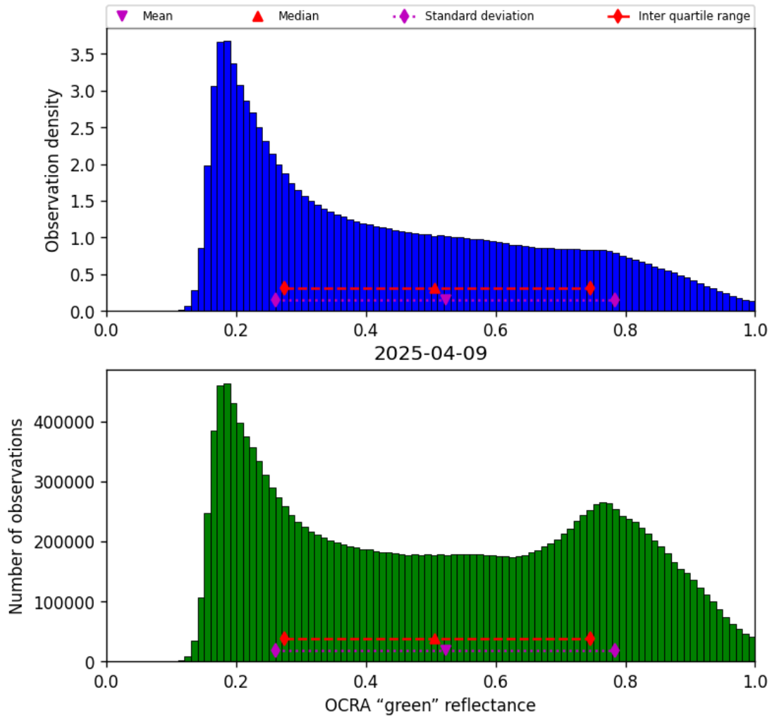
Figure 50: Histogram of “OCRA “green” reflectance” for 2025-04-09 to 2025-04-10
