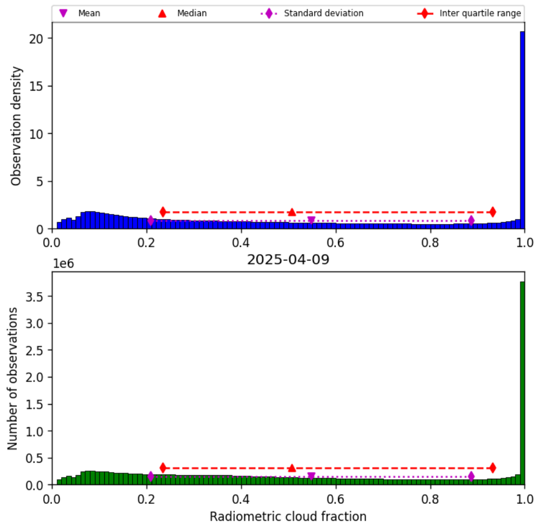
Figure 37: Histogram of “Radiometric cloud fraction” for 2025-04-09 to 2025-04-10
