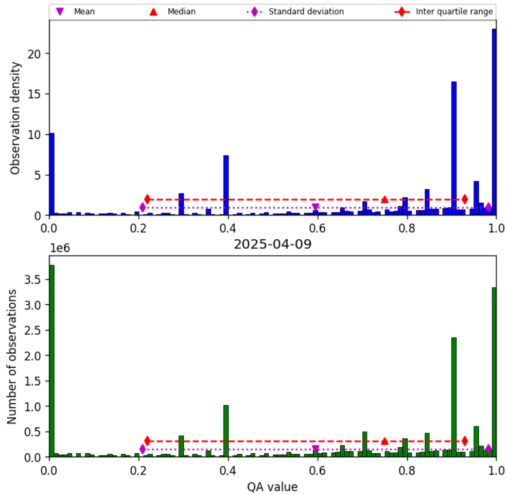
Figure 36: Histogram of “QA value” for 2025-04-09 to 2025-04-10
