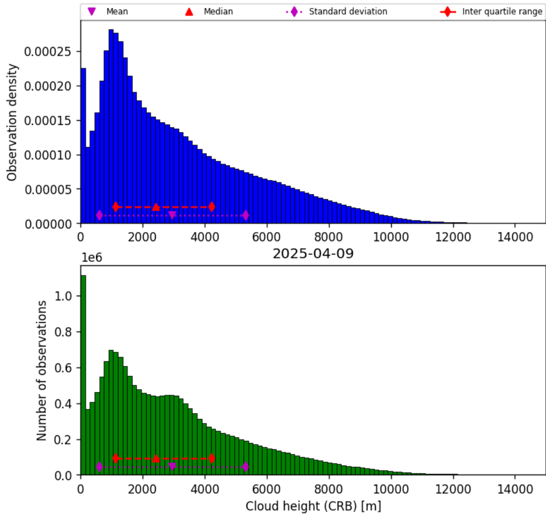
Figure 41: Histogram of “Cloud height (CRB)” for 2025-04-09 to 2025-04-10
