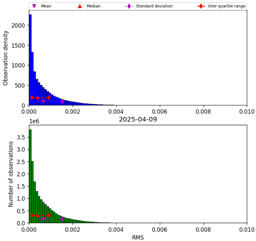
Figure 45: Histogram of “RMS” for 2025-04-09 to 2025-04-10
