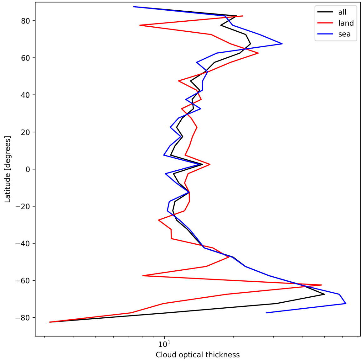
Figure 23: Zonal average of “Cloud optical thickness” for 2025-04-09 to 2025-04-10.
