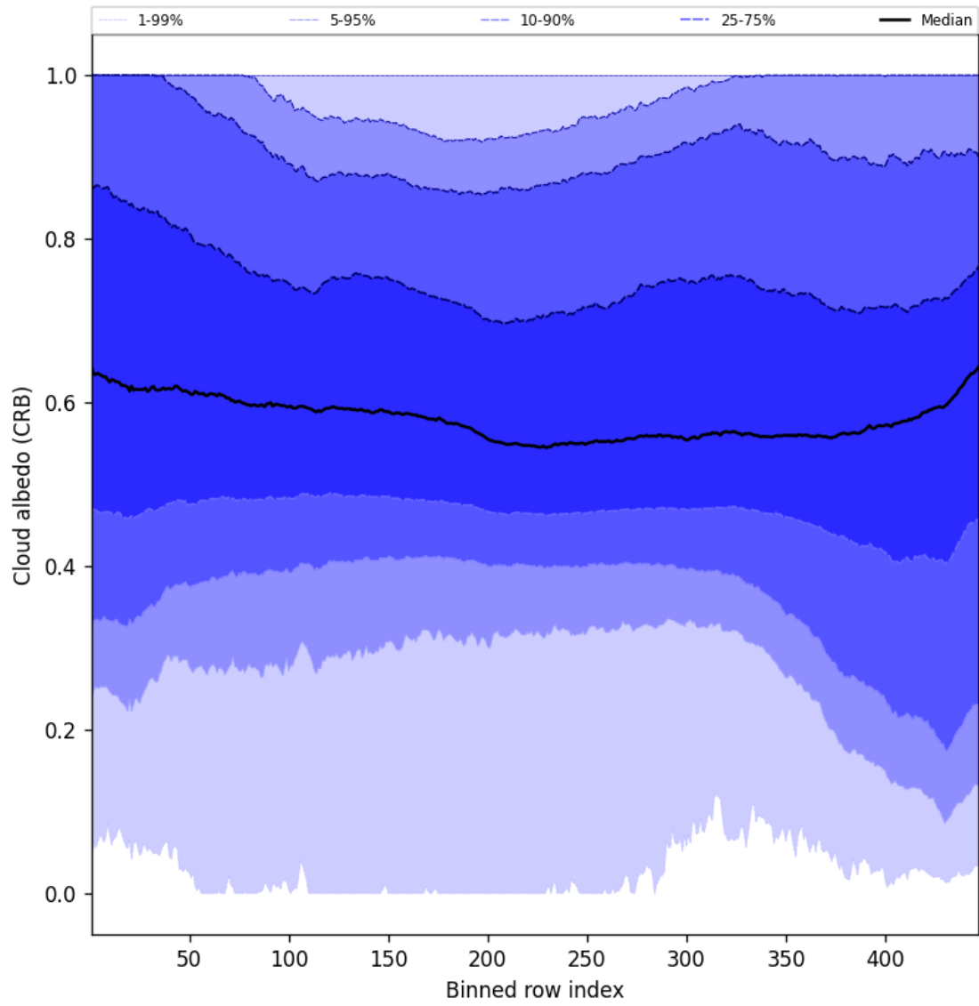
Figure 58: Along track statistics of “Cloud albedo (CRB)” for 2025-04-09 to 2025-04-10
