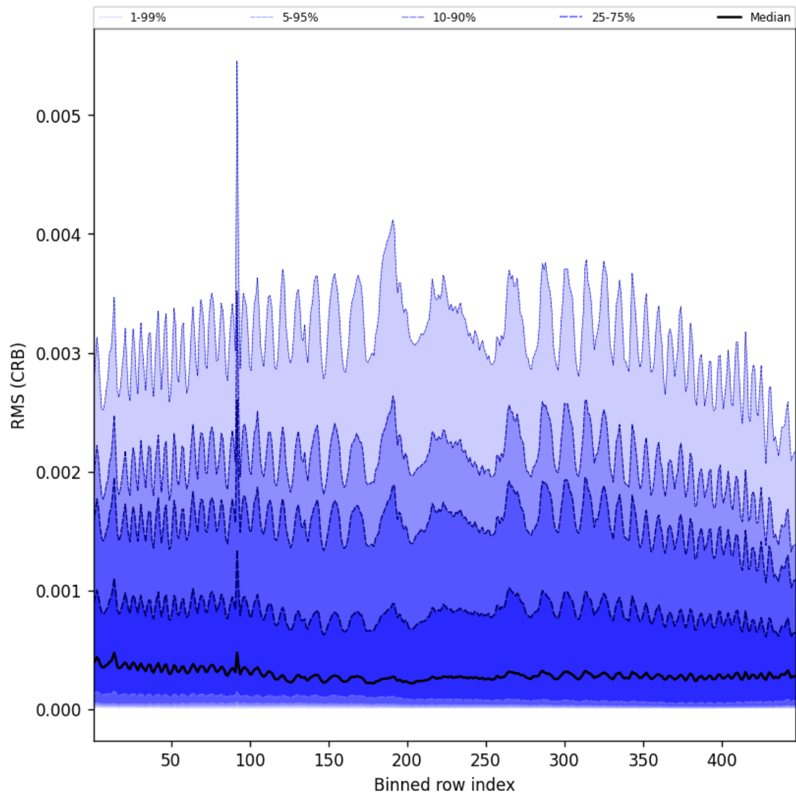
Figure 62: Along track statistics of “RMS (CRB)” for 2025-04-09 to 2025-04-10
