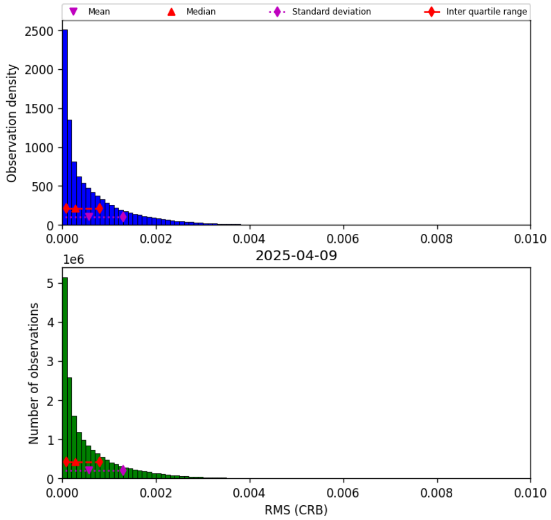
Figure 46: Histogram of “RMS (CRB)” for 2025-04-09 to 2025-04-10
