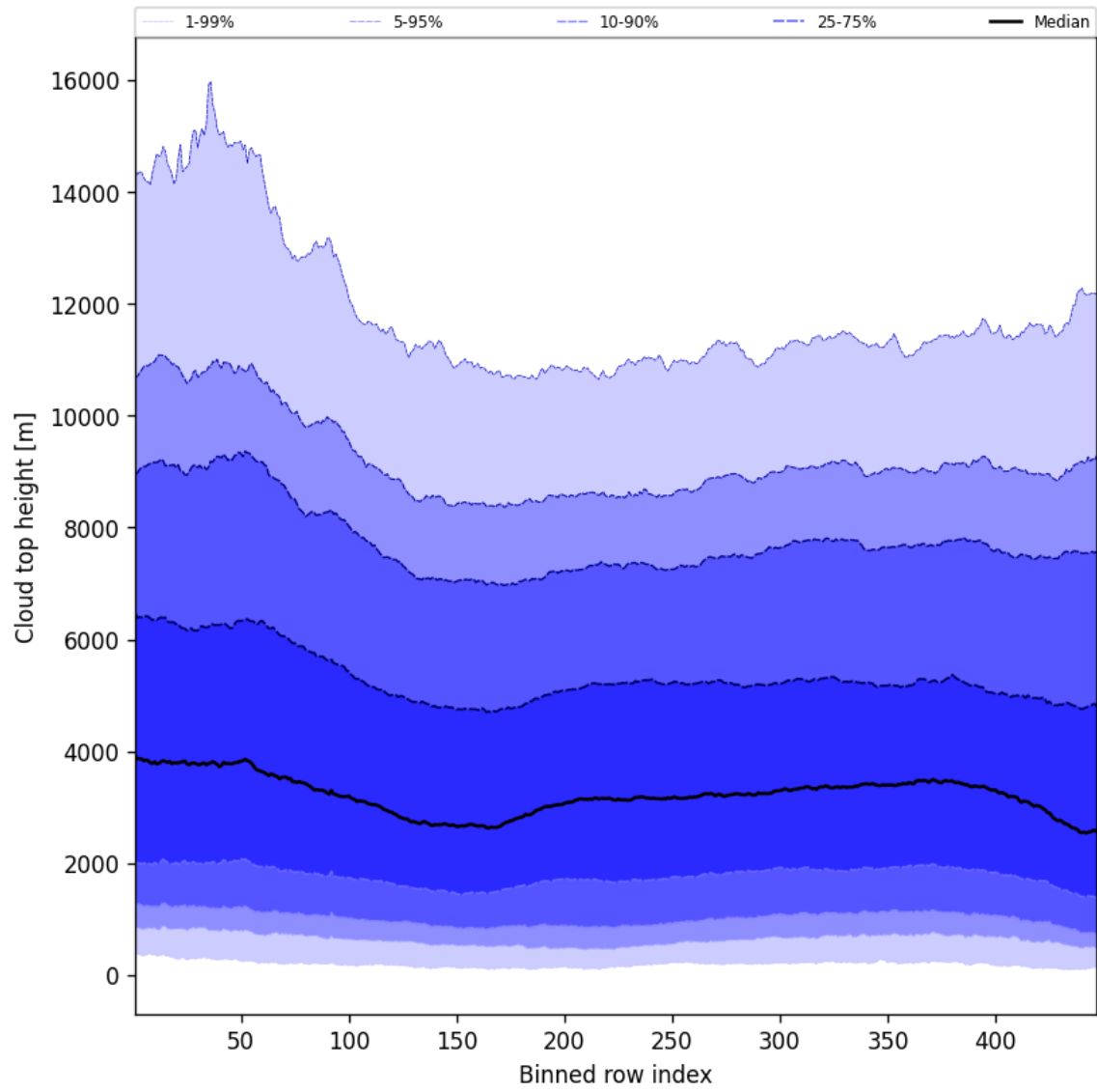
Figure 54: Along track statistics of “Cloud top height” for 2025-04-09 to 2025-04-10
