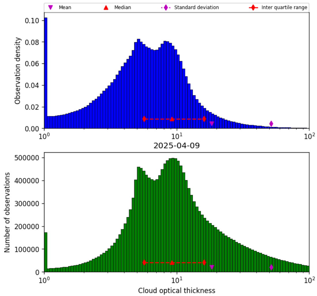
Figure 39: Histogram of “Cloud optical thickness” for 2025-04-09 to 2025-04-10
