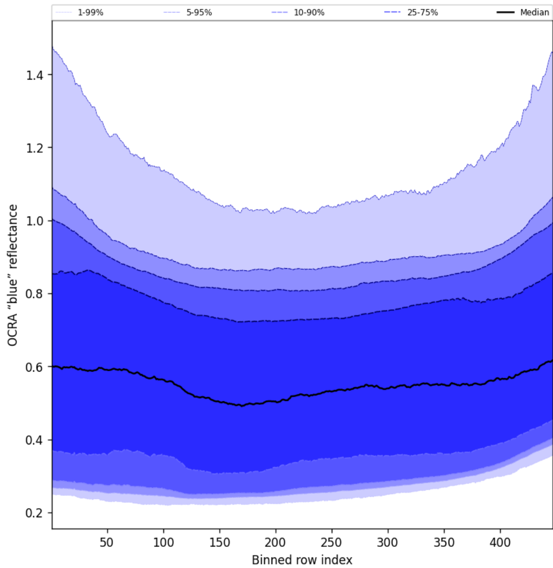
Figure 65: Along track statistics of “OCRA “blue” reflectance” for 2025-04-09 to 2025-04-10
