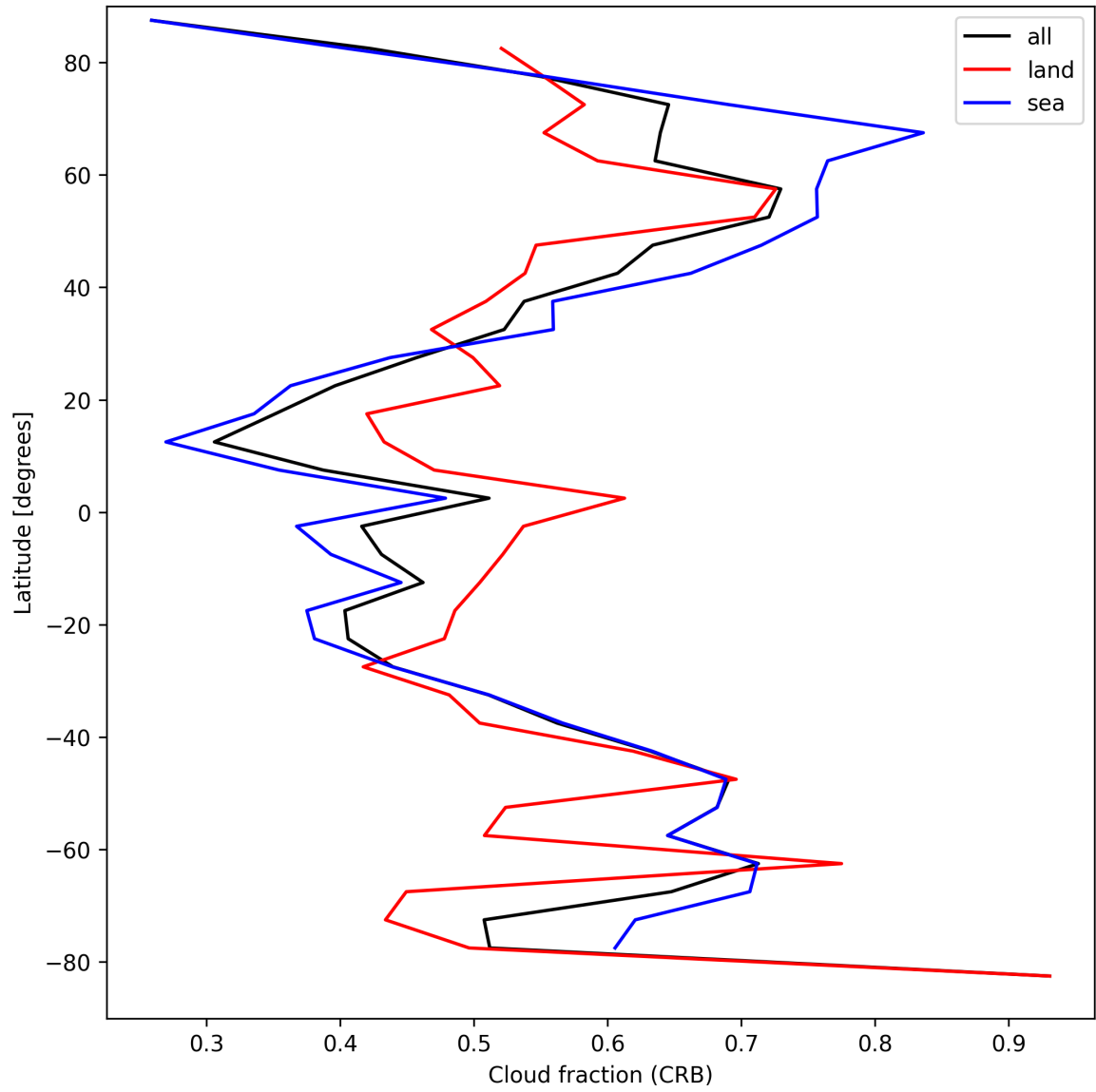
Figure 24: Zonal average of “Cloud fraction (CRB)” for 2025-04-09 to 2025-04-10.
