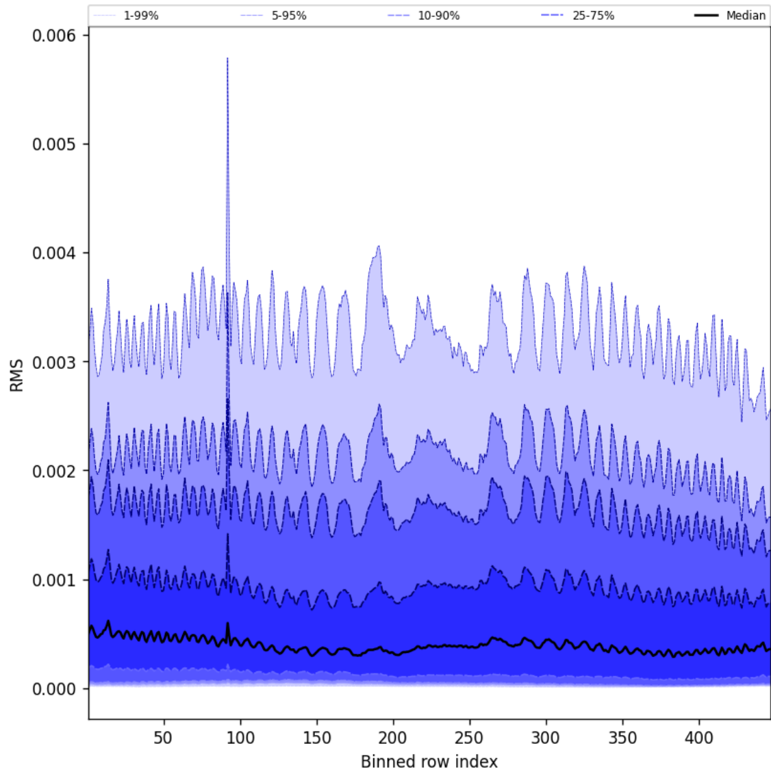
Figure 61: Along track statistics of “RMS” for 2025-04-09 to 2025-04-10
