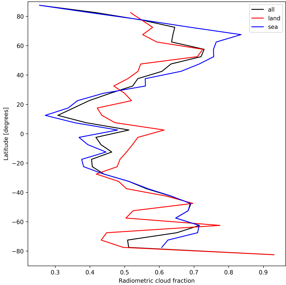
Figure 21: Zonal average of “Radiometric cloud fraction” for 2025-04-09 to 2025-04-10.
