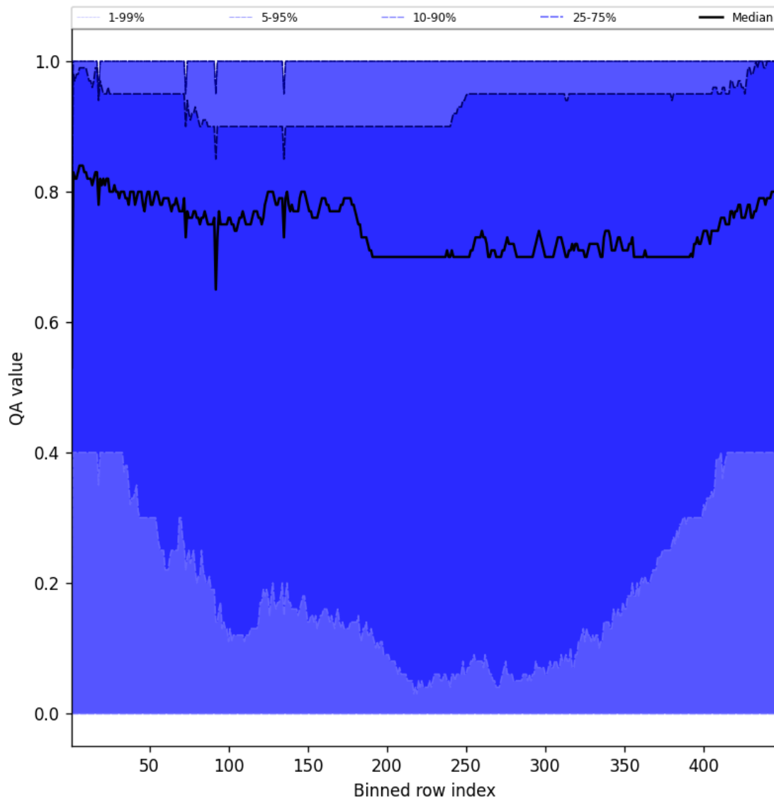
Figure 52: Along track statistics of “QA value” for 2025-04-09 to 2025-04-10
