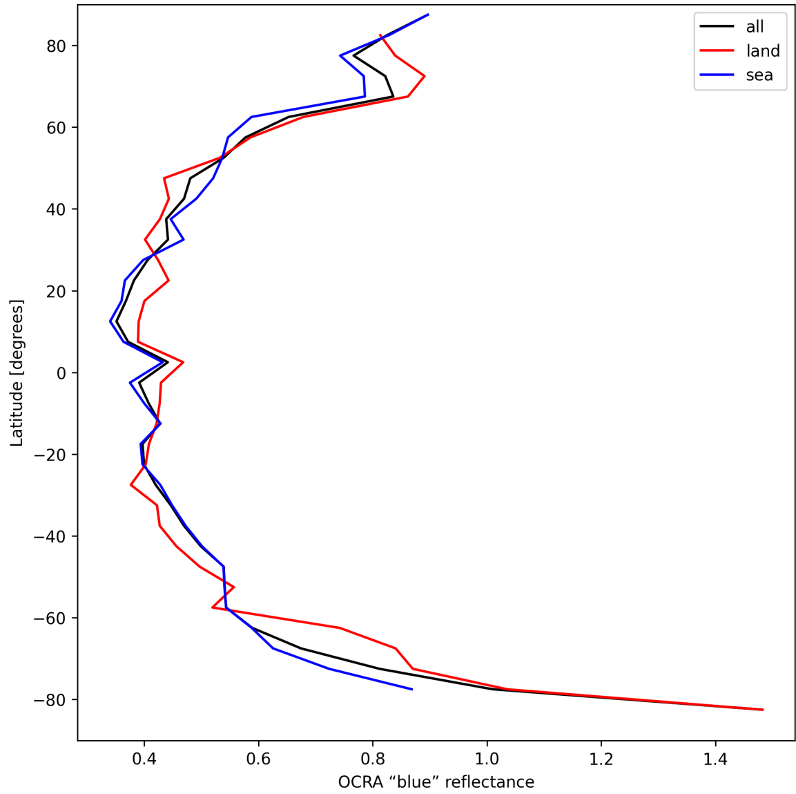
Figure 33: Zonal average of “OCRA “blue” reflectance” for 2025-04-09 to 2025-04-10.
