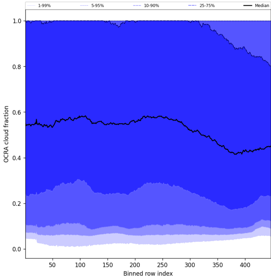
Figure 64: Along track statistics of “OCRA cloud fraction” for 2025-04-09 to 2025-04-10
