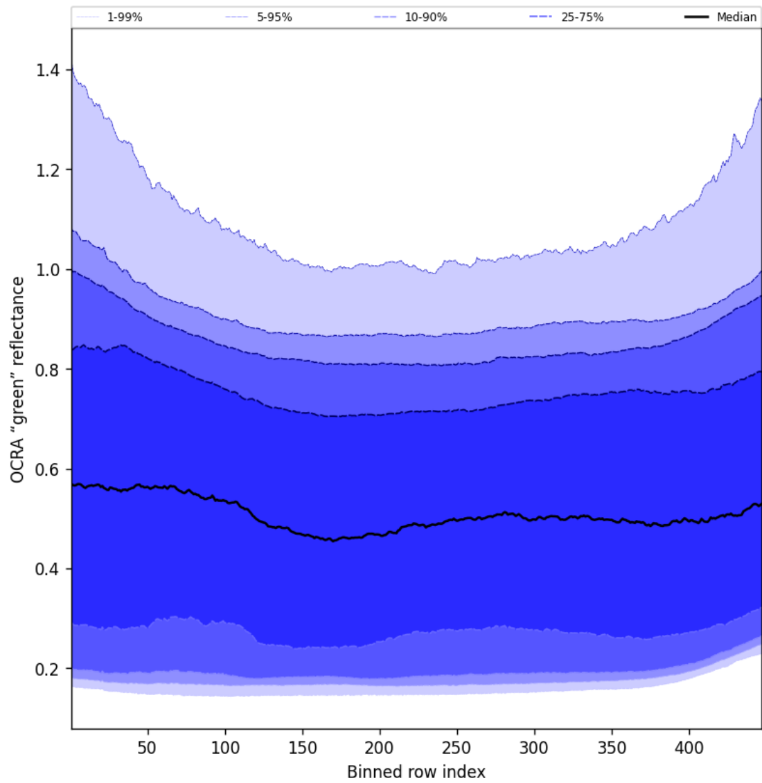
Figure 66: Along track statistics of “OCRA “green” reflectance” for 2025-04-09 to 2025-04-10
