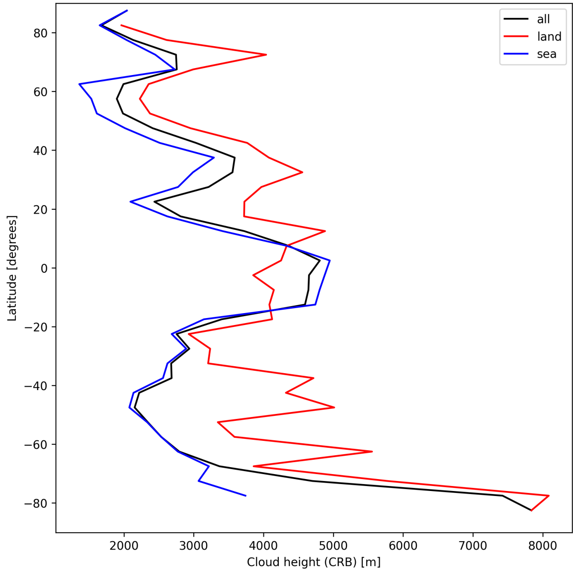
Figure 25: Zonal average of “Cloud height (CRB)” for 2025-04-09 to 2025-04-10.
