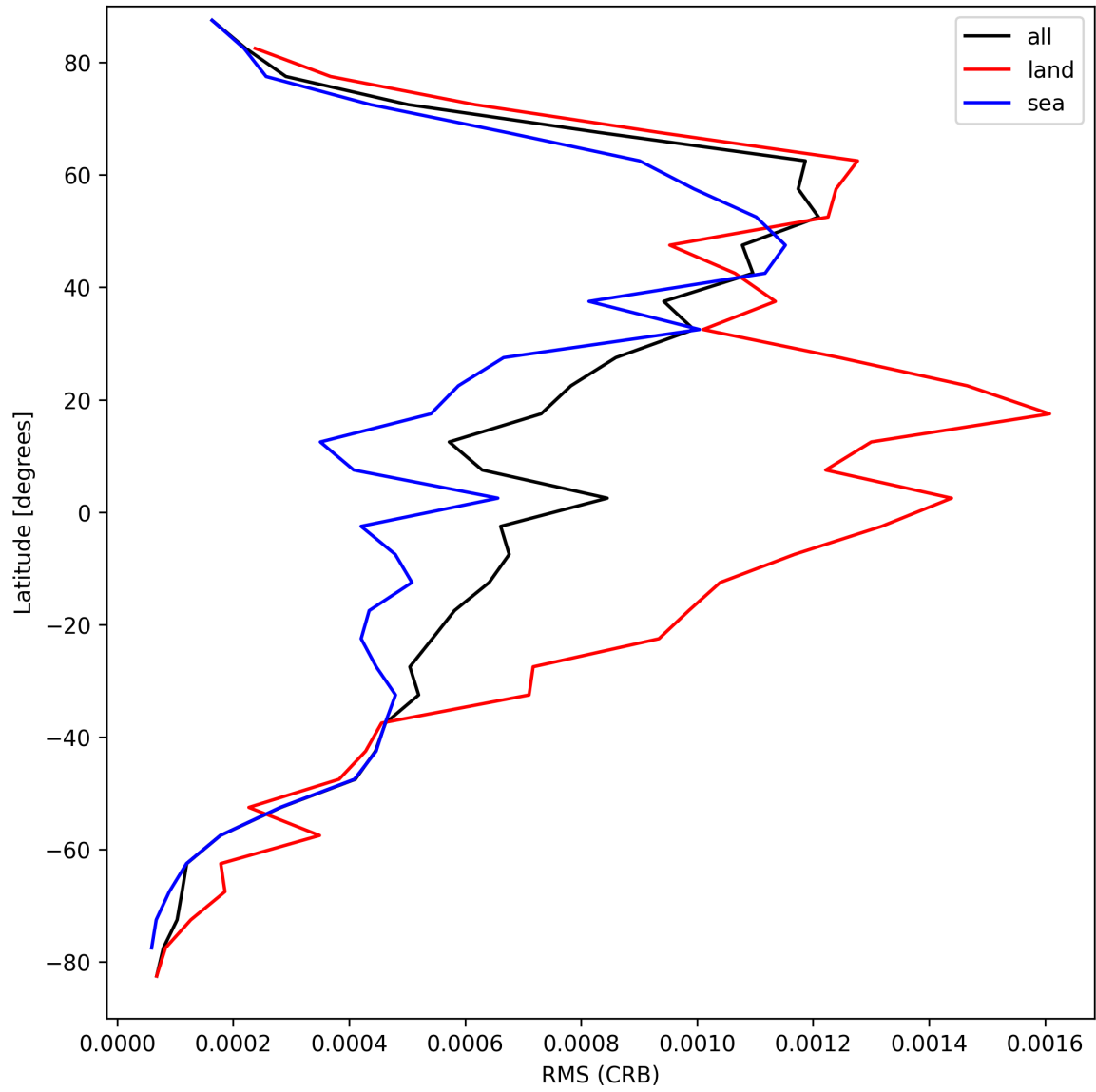
Figure 30: Zonal average of “RMS (CRB)” for 2025-04-09 to 2025-04-10.
