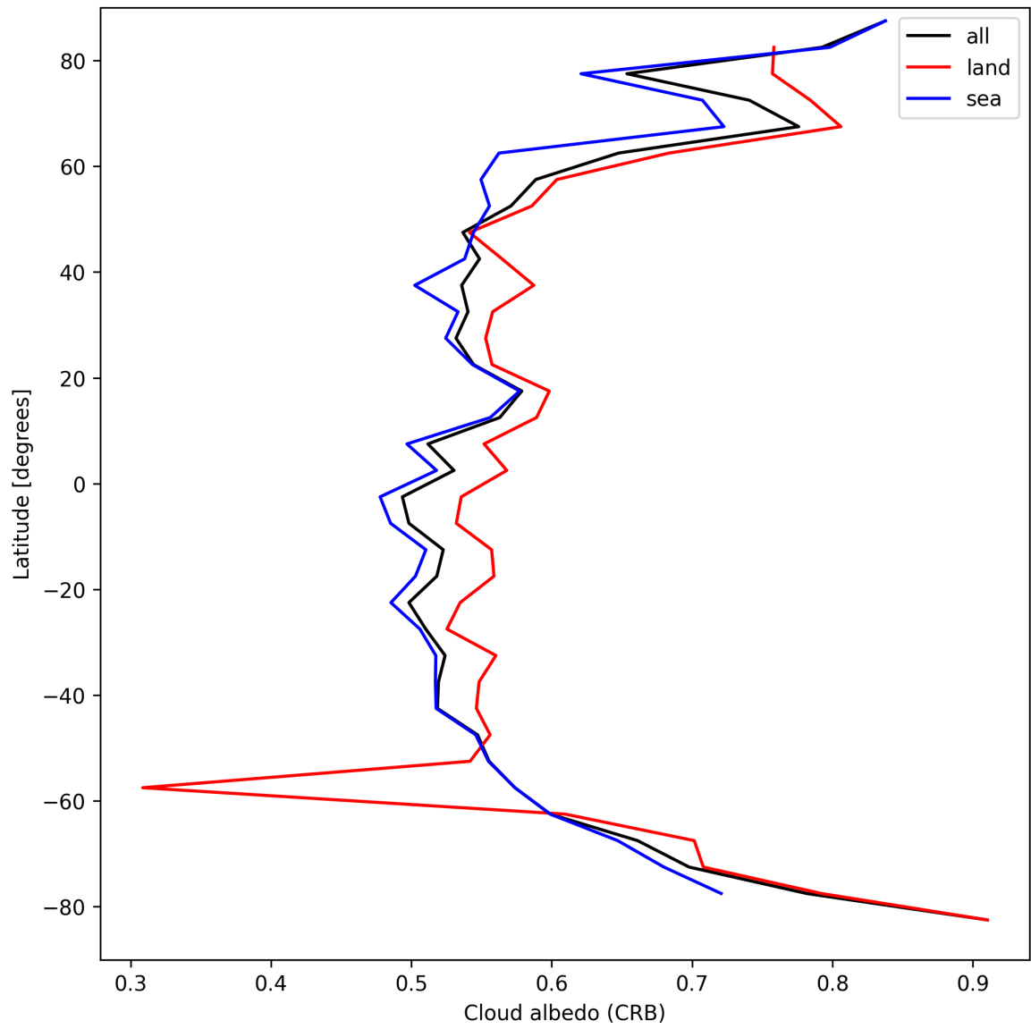
Figure 26: Zonal average of “Cloud albedo (CRB)” for 2025-04-09 to 2025-04-10.
