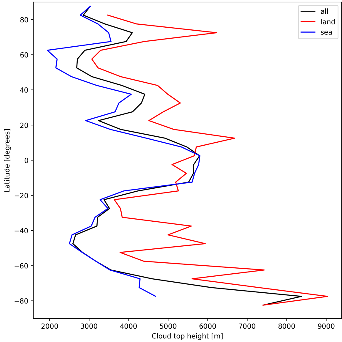
Figure 22: Zonal average of “Cloud top height” for 2025-04-09 to 2025-04-10.
