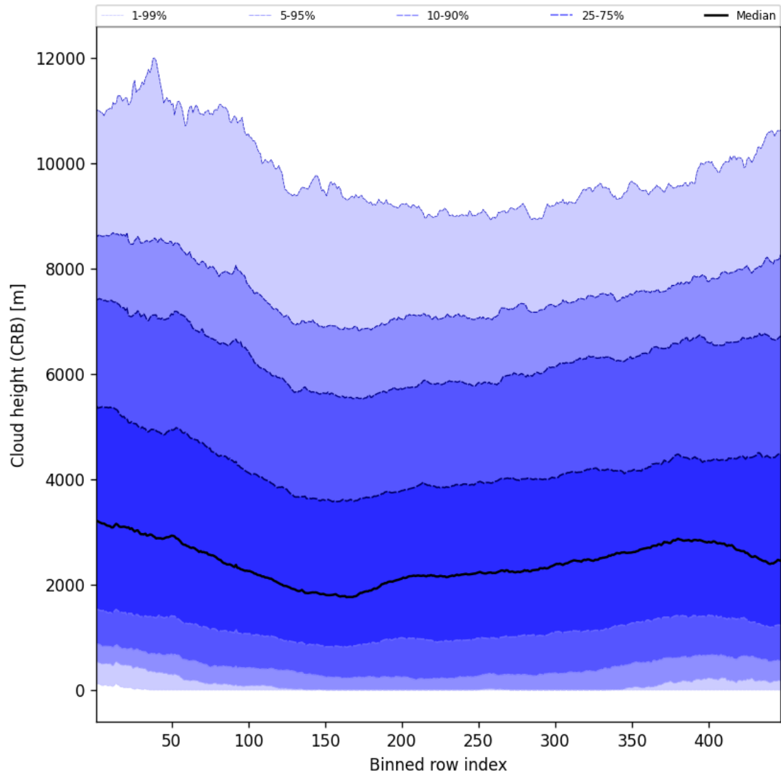
Figure 57: Along track statistics of “Cloud height (CRB)” for 2025-04-09 to 2025-04-10
