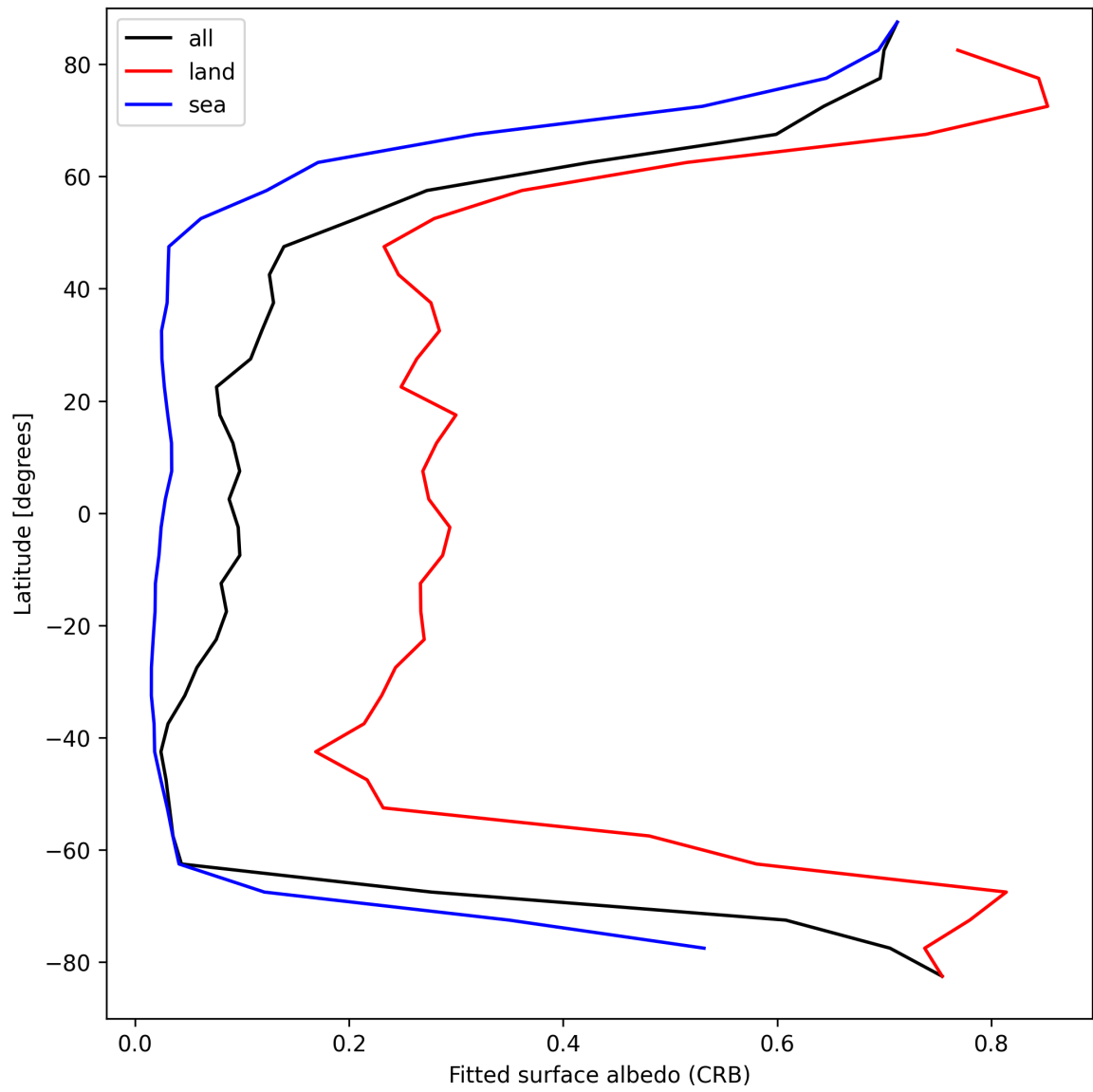
Figure 28: Zonal average of “Fitted surface albedo (CRB)” for 2025-04-09 to 2025-04-10.
