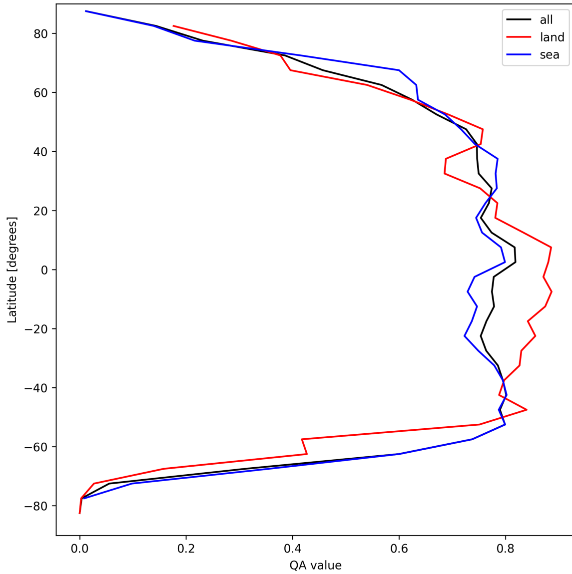
Figure 20: Zonal average of “QA value” for 2025-04-09 to 2025-04-10.
