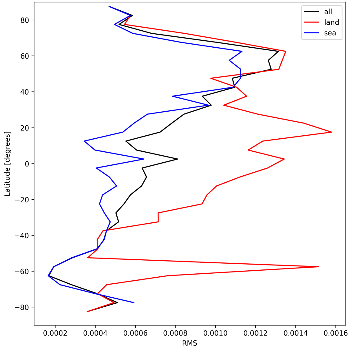
Figure 29: Zonal average of “RMS” for 2025-04-09 to 2025-04-10.
