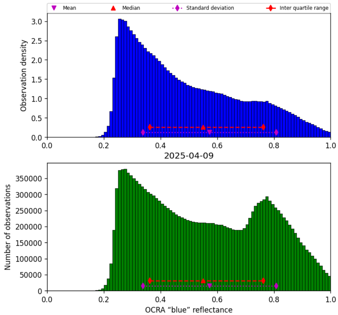
Figure 49: Histogram of “OCRA “blue” reflectance” for 2025-04-09 to 2025-04-10
