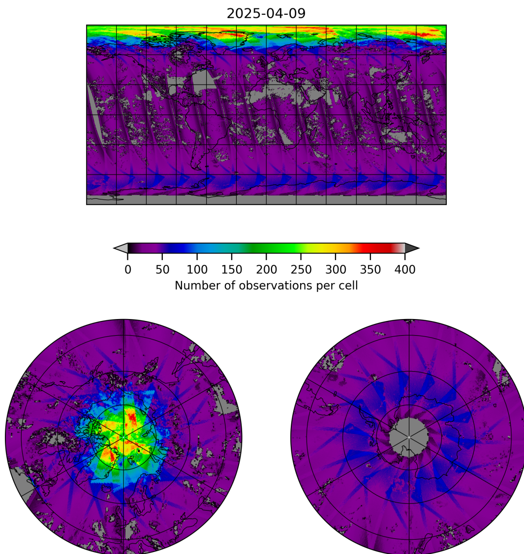
Figure 19: Map of the number of observations for 2025-04-09 to 2025-04-10
