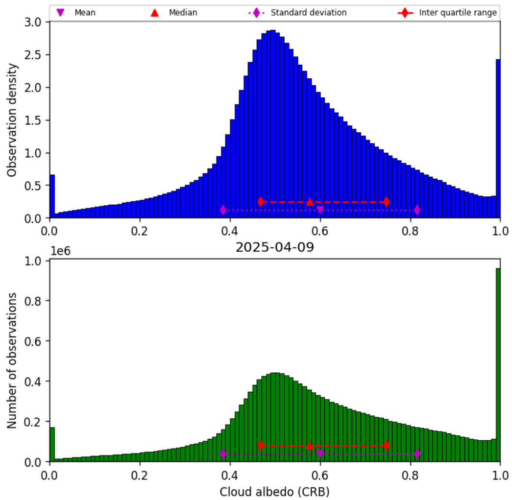
Figure 42: Histogram of “Cloud albedo (CRB)” for 2025-04-09 to 2025-04-10
