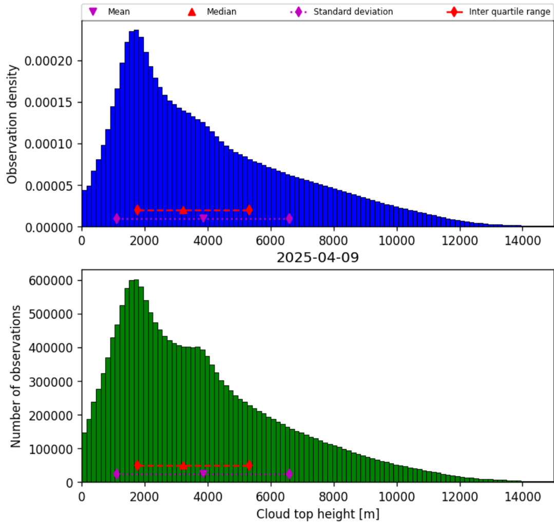
Figure 38: Histogram of “Cloud top height” for 2025-04-09 to 2025-04-10
