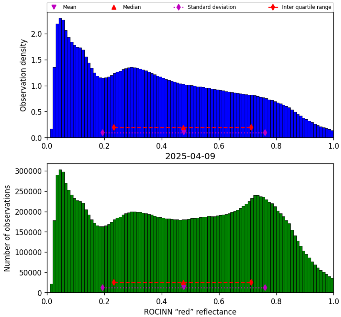
Figure 51: Histogram of “ROCINN “red” reflectance” for 2025-04-09 to 2025-04-10
