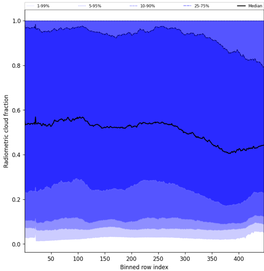
Figure 53: Along track statistics of “Radiometric cloud fraction” for 2025-04-09 to 2025-04-10
