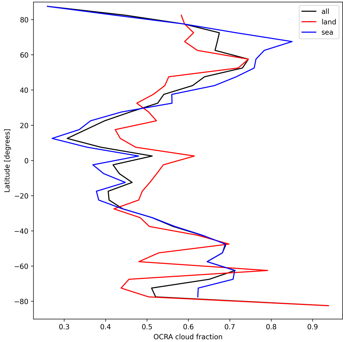
Figure 32: Zonal average of “OCRA cloud fraction” for 2025-04-09 to 2025-04-10.
