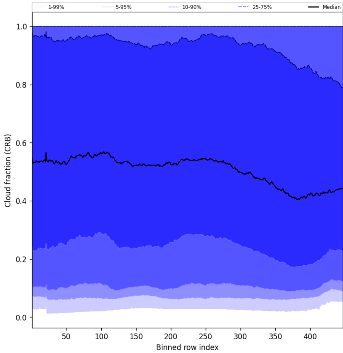
Figure 56: Along track statistics of “Cloud fraction (CRB)” for 2025-04-09 to 2025-04-10
