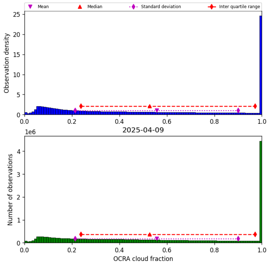
Figure 48: Histogram of “OCRA cloud fraction” for 2025-04-09 to 2025-04-10
