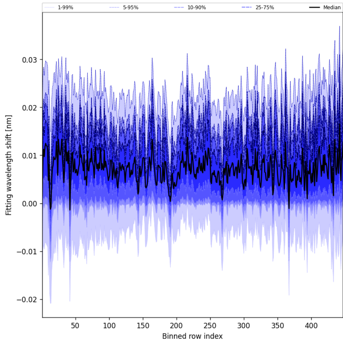
Figure 63: Along track statistics of “Fitting wavelength shift” for 2025-04-09 to 2025-04-10
