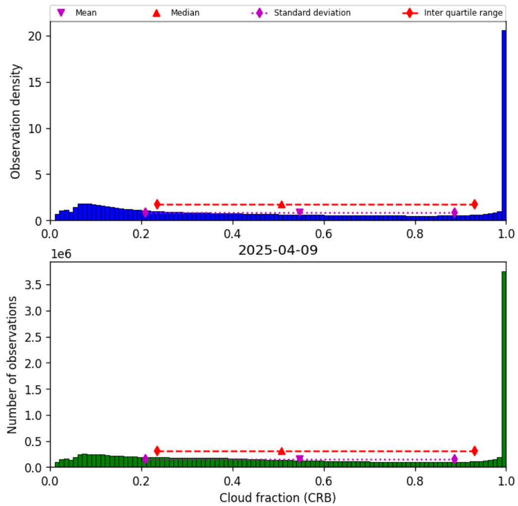
Figure 40: Histogram of "Cloud fraction (CRB)" for 2025-04-09 to 2025-04-10
