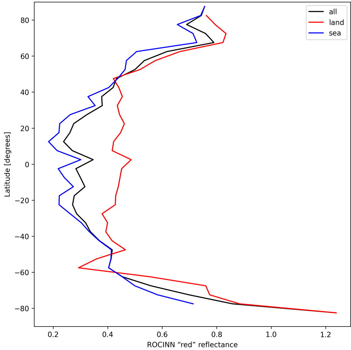
Figure 35: Zonal average of “ROCINN “red” reflectance” for 2025-04-09 to 2025-04-10.
