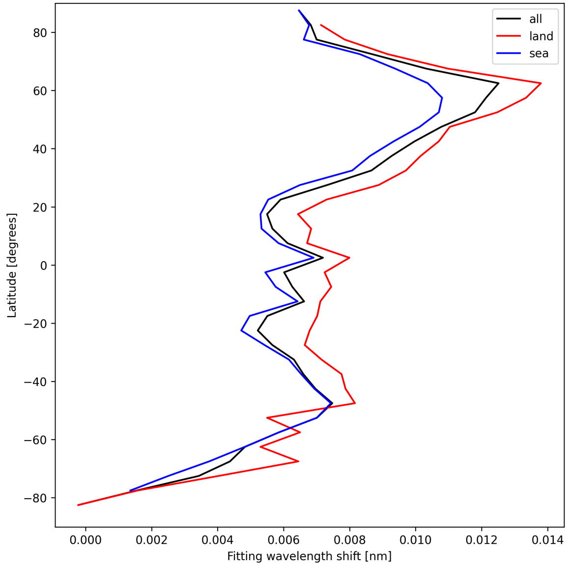
Figure 31: Zonal average of “Fitting wavelength shift” for 2025-04-09 to 2025-04-10.
