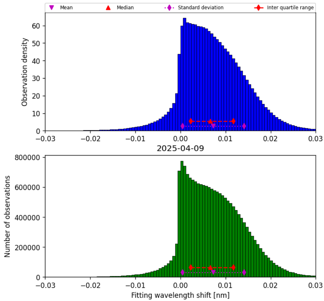
Figure 47: Histogram of “Fitting wavelength shift” for 2025-04-09 to 2025-04-10
