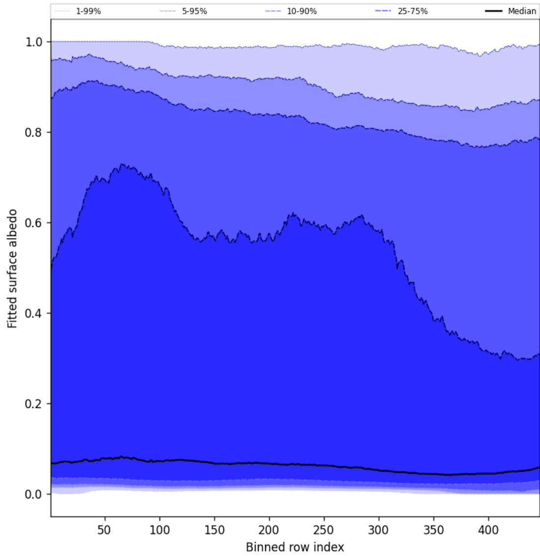
Figure 59: Along track statistics of “Fitted surface albedo” for 2025-04-09 to 2025-04-10
