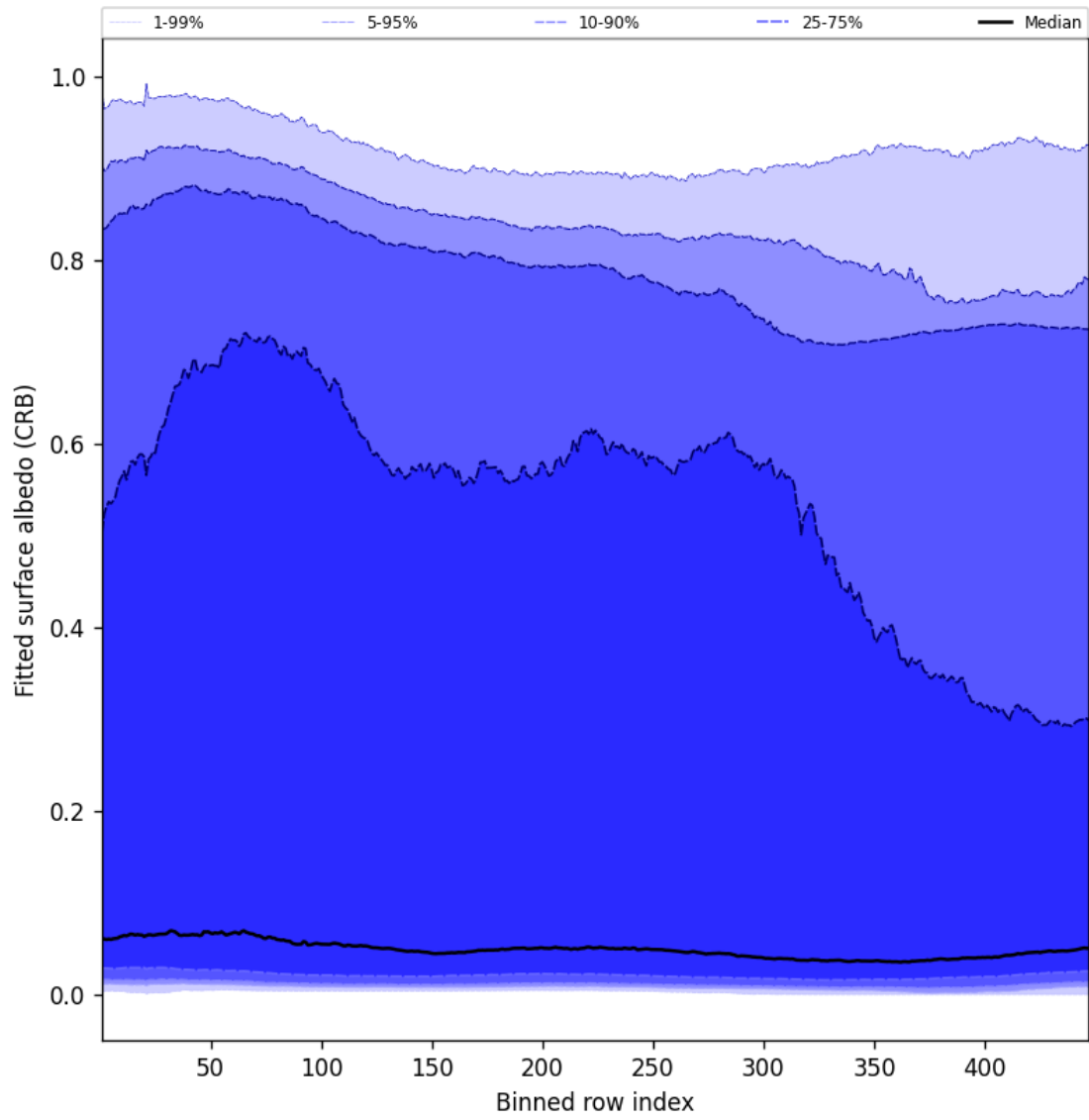
Figure 60: Along track statistics of “Fitted surface albedo (CRB)” for 2025-04-09 to 2025-04-10
