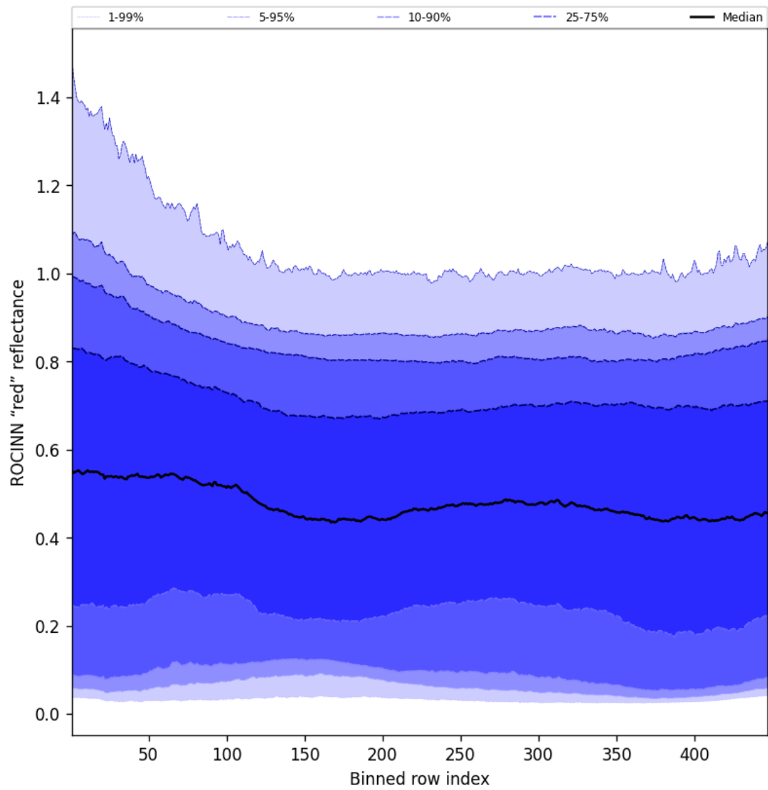
Figure 67: Along track statistics of “ROCINN “red” reflectance” for 2025-04-09 to 2025-04-10
