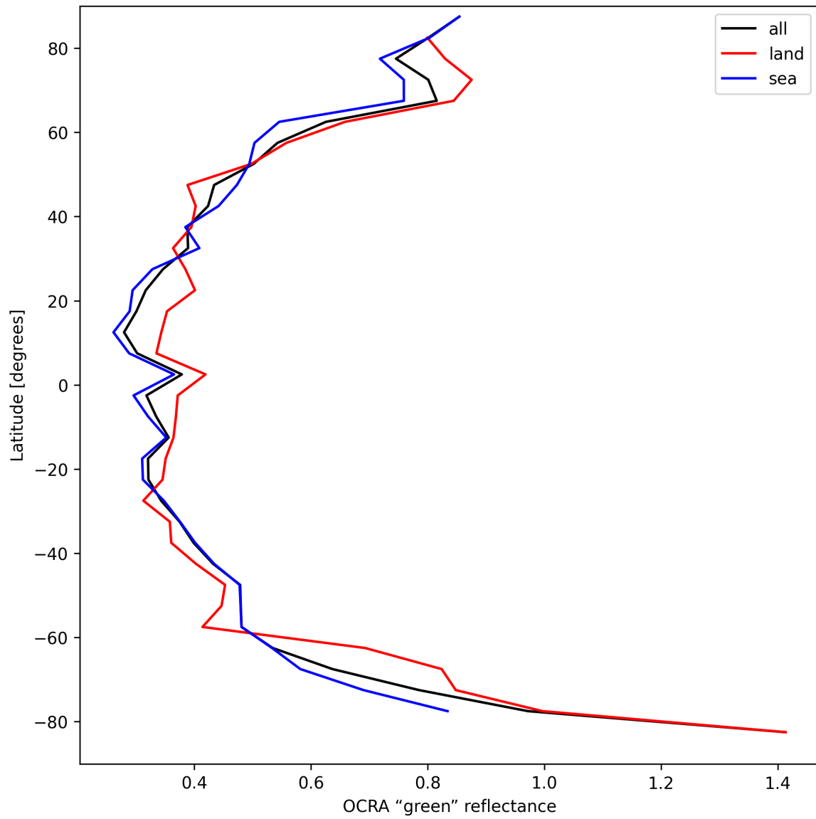
Figure 34: Zonal average of “OCRA “green” reflectance” for 2025-04-09 to 2025-04-10.
