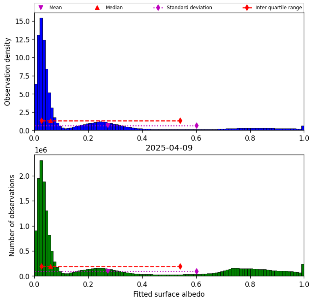
Figure 43: Histogram of “Fitted surface albedo” for 2025-04-09 to 2025-04-10
