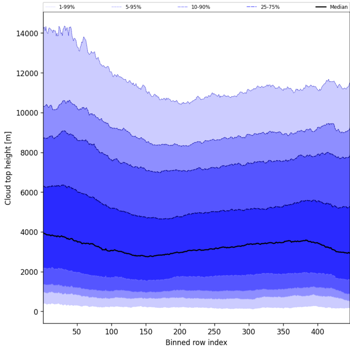
Figure 54: Along track statistics of “Cloud top height” for 2025-04-11 to 2025-04-11
