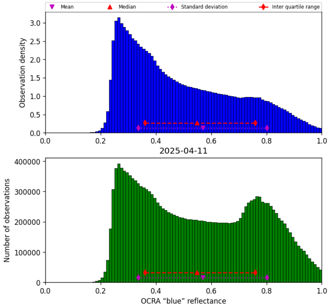
Figure 49: Histogram of “OCRA “blue” reflectance” for 2025-04-11 to 2025-04-11
