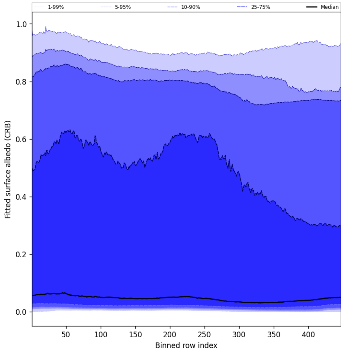
Figure 60: Along track statistics of “Fitted surface albedo (CRB)” for 2025-04-11 to 2025-04-11
