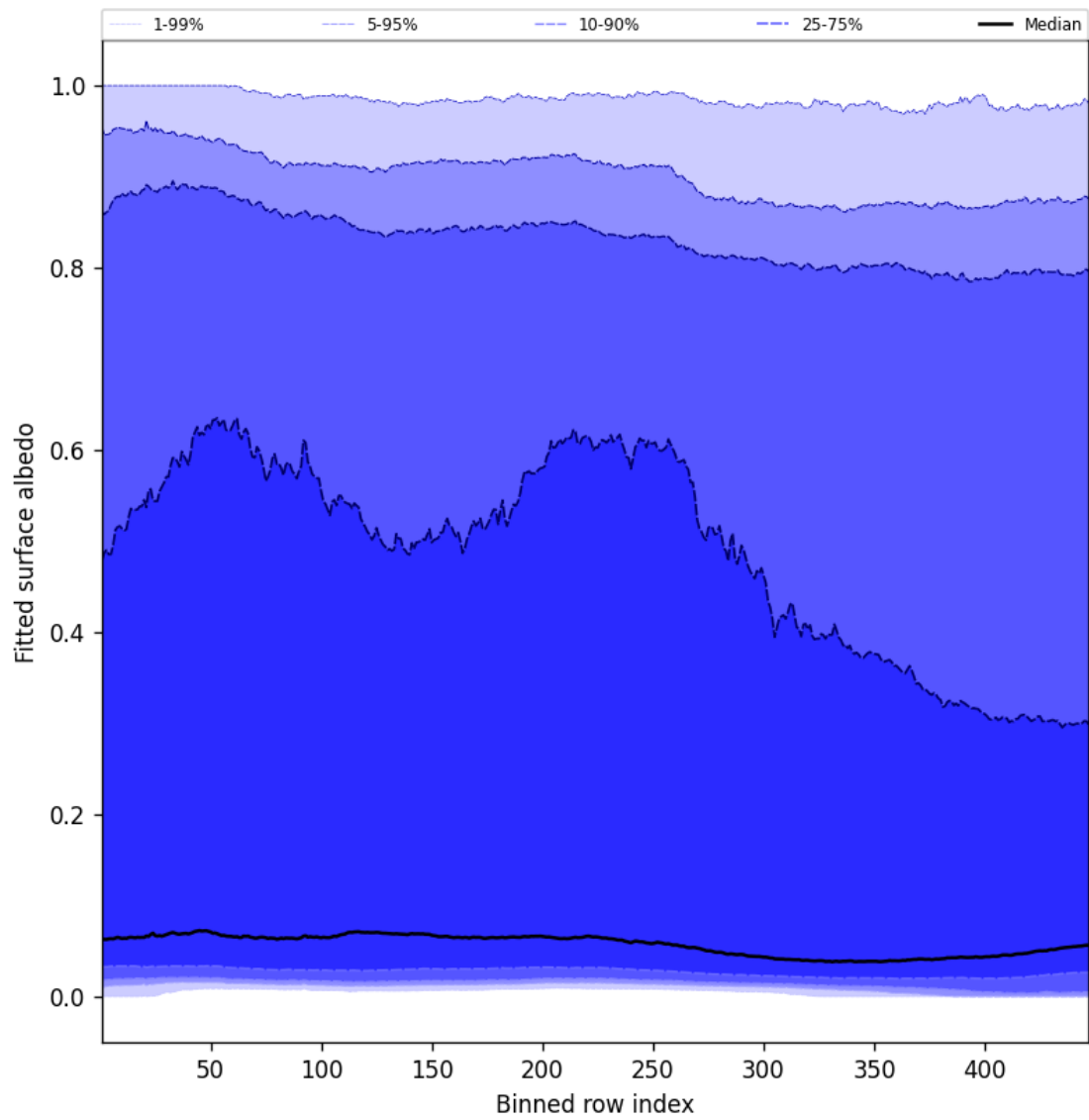
Figure 59: Along track statistics of “Fitted surface albedo” for 2025-04-11 to 2025-04-11
