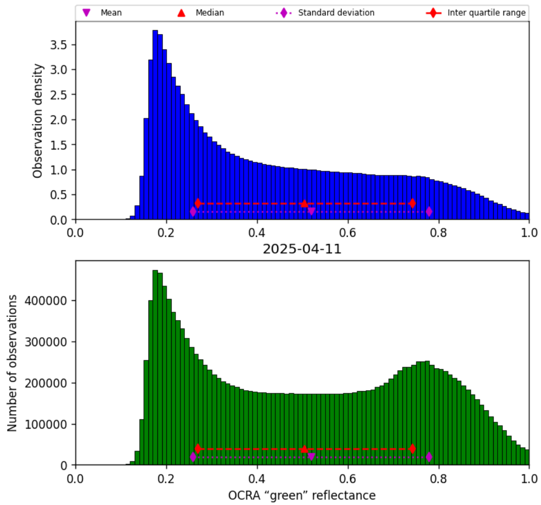
Figure 50: Histogram of “OCRA “green” reflectance” for 2025-04-11 to 2025-04-11
