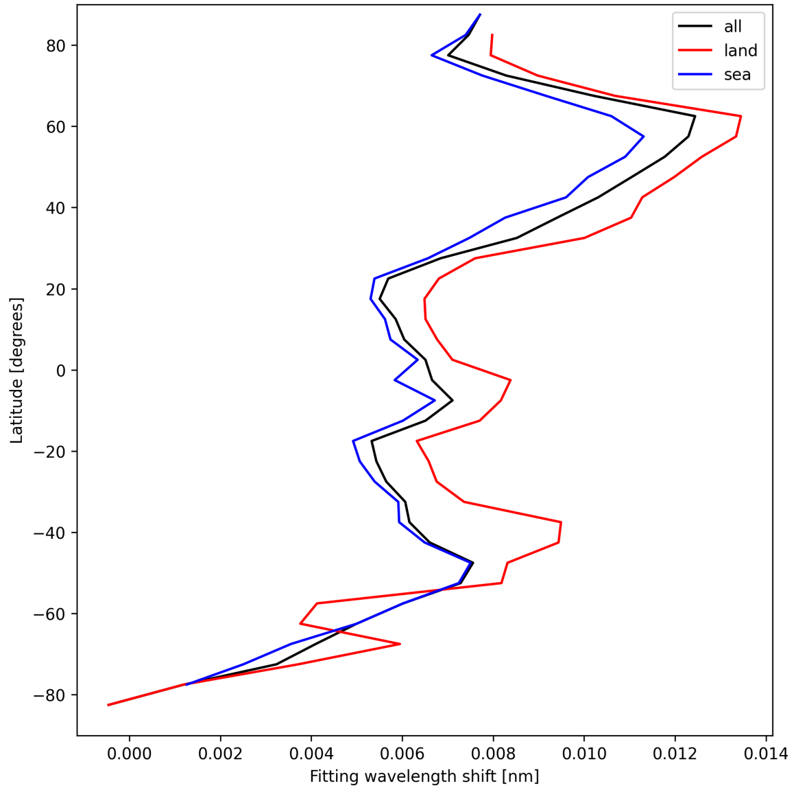
Figure 31: Zonal average of “Fitting wavelength shift” for 2025-04-11 to 2025-04-11.
