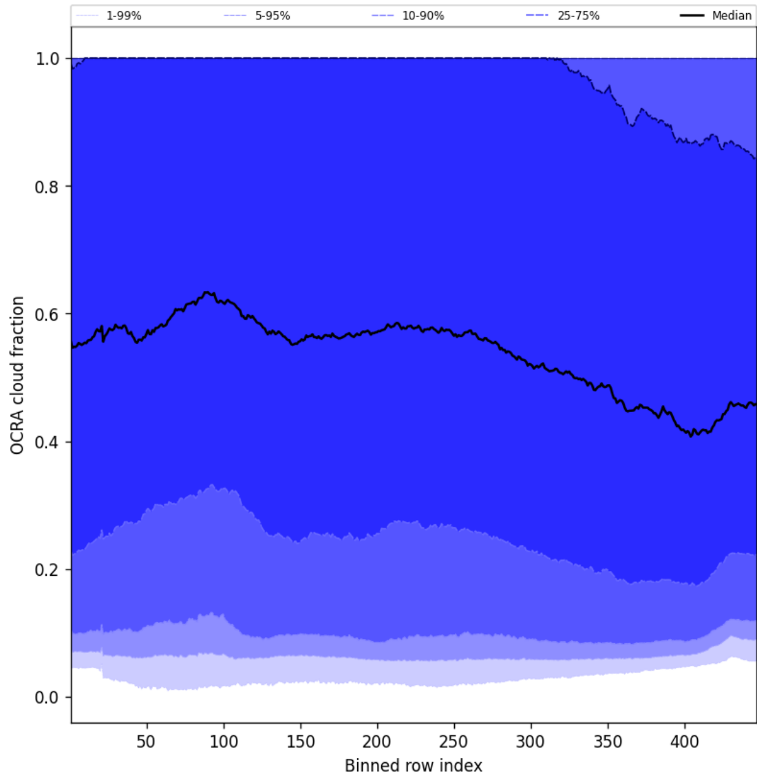
Figure 64: Along track statistics of “OCRA cloud fraction” for 2025-04-11 to 2025-04-11
