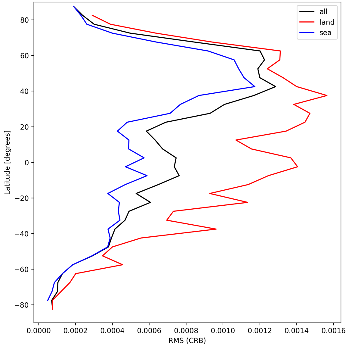
Figure 30: Zonal average of “RMS (CRB)” for 2025-04-11 to 2025-04-11.
