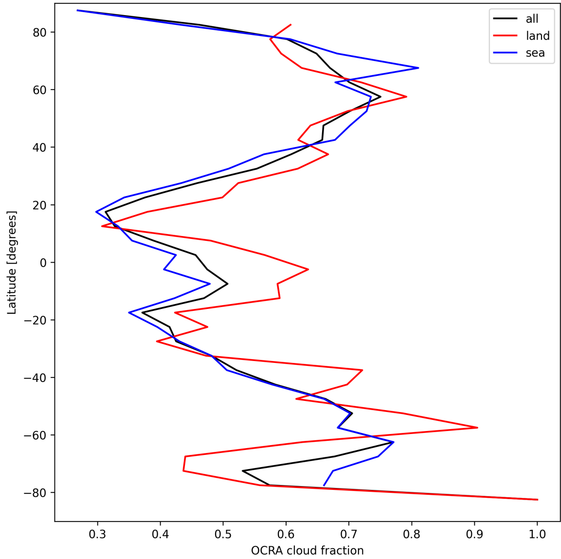
Figure 32: Zonal average of “OCRA cloud fraction” for 2025-04-11 to 2025-04-11.
