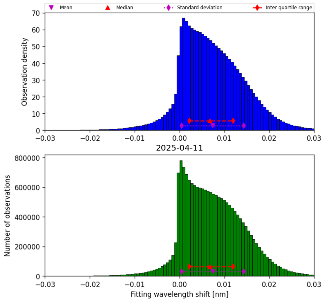
Figure 47: Histogram of “Fitting wavelength shift” for 2025-04-11 to 2025-04-11
