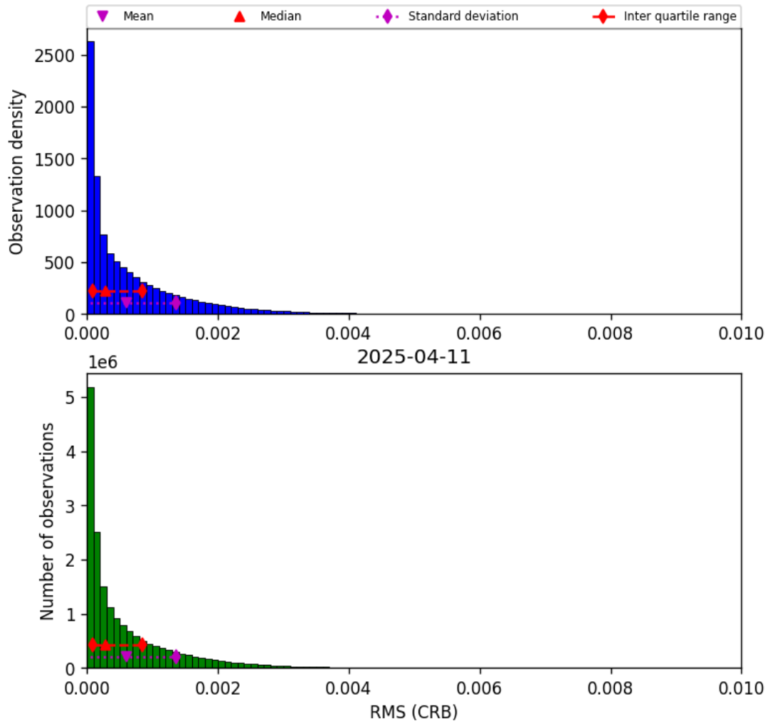
Figure 46: Histogram of “RMS (CRB)” for 2025-04-11 to 2025-04-11
