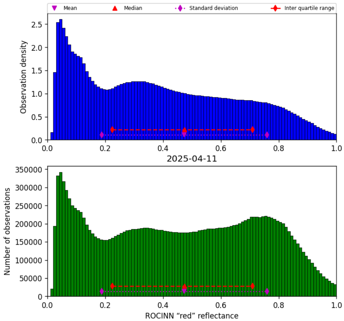
Figure 51: Histogram of "ROCINN "red" reflectance" for 2025-04-11 to 2025-04-11
