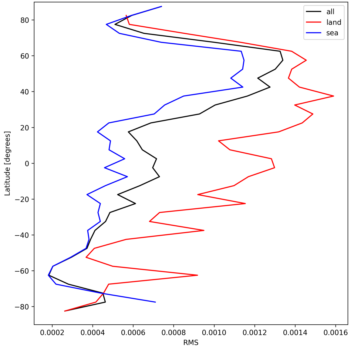
Figure 29: Zonal average of “RMS” for 2025-04-11 to 2025-04-11.
