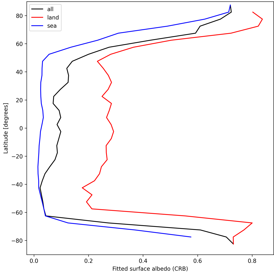
Figure 28: Zonal average of “Fitted surface albedo (CRB)” for 2025-04-11 to 2025-04-11.
