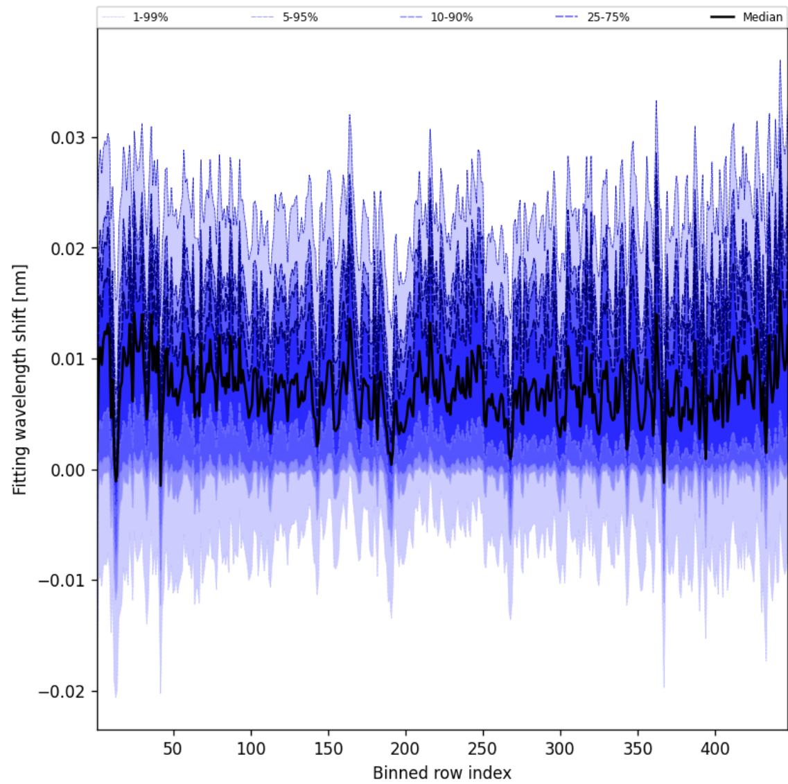
Figure 63: Along track statistics of “Fitting wavelength shift” for 2025-04-11 to 2025-04-11
