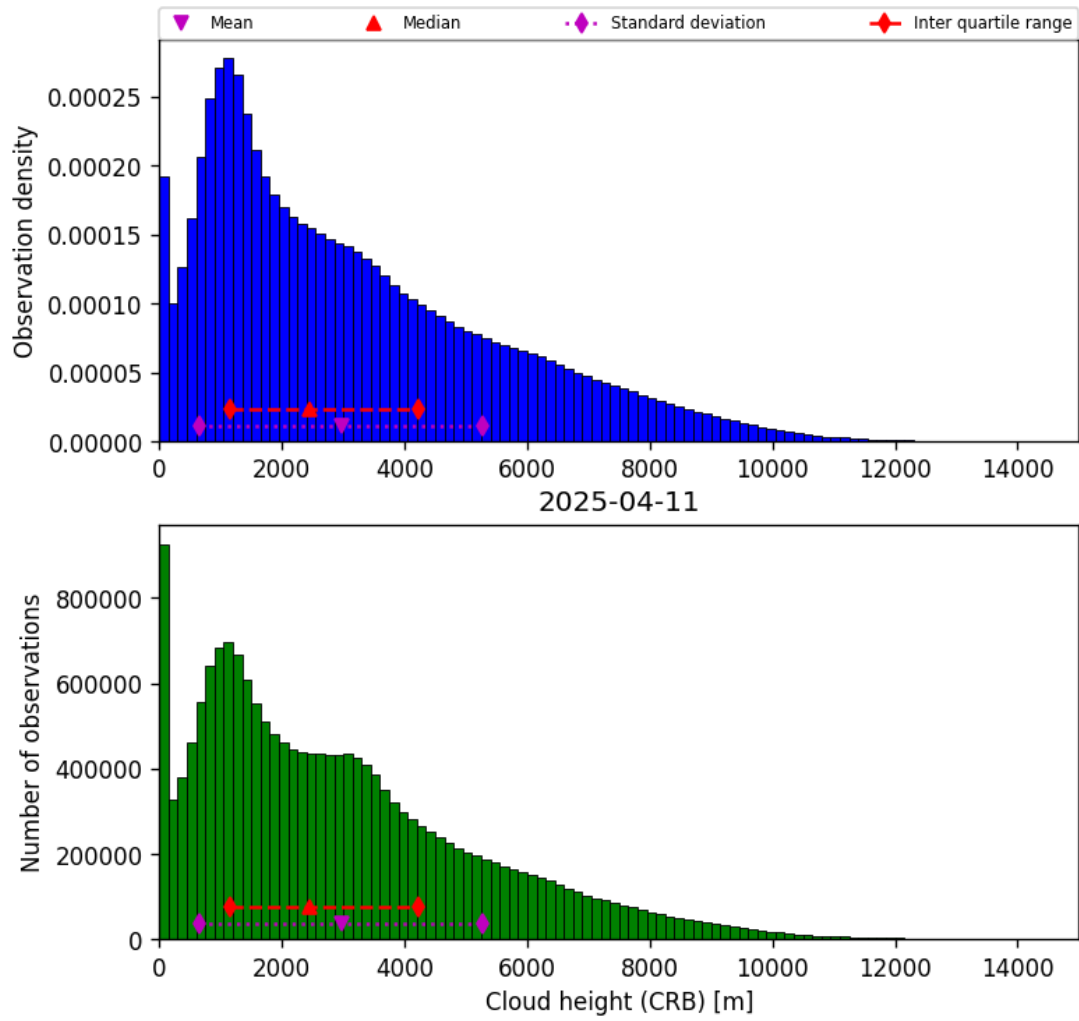
Figure 41: Histogram of “Cloud height (CRB)” for 2025-04-11 to 2025-04-11
