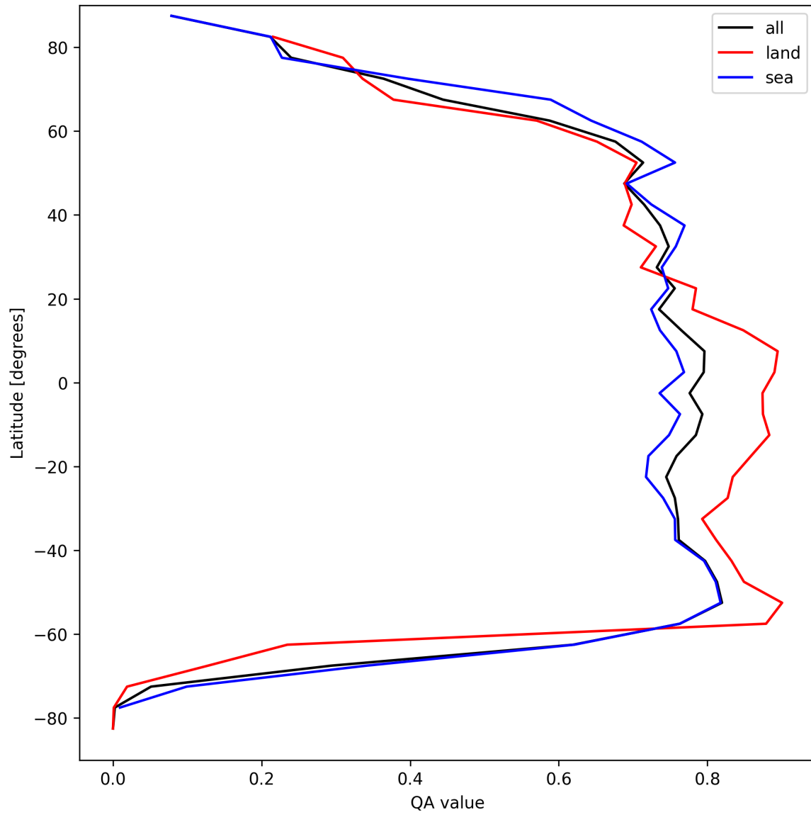
Figure 20: Zonal average of “QA value” for 2025-04-11 to 2025-04-11.
