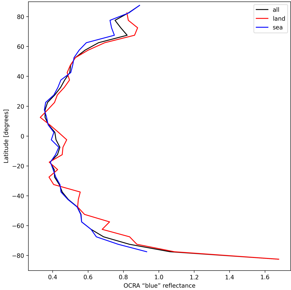
Figure 33: Zonal average of “OCRA “blue” reflectance” for 2025-04-11 to 2025-04-11.
