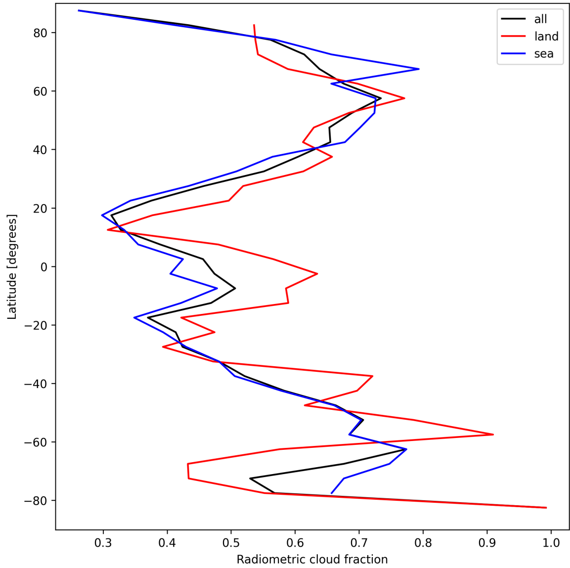
Figure 21: Zonal average of “Radiometric cloud fraction” for 2025-04-11 to 2025-04-11.
