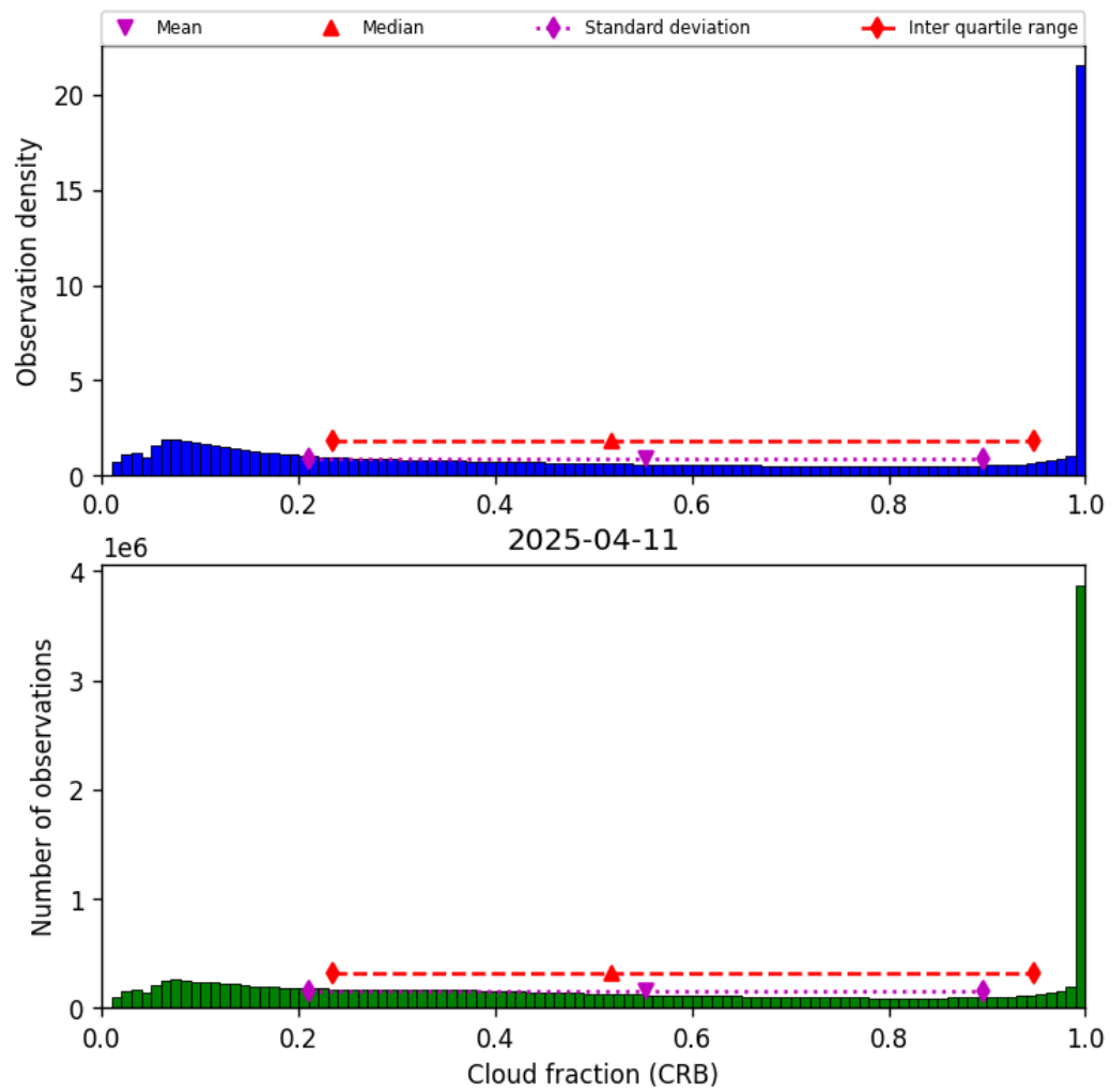
Figure 40: Histogram of “Cloud fraction (CRB)” for 2025-04-11 to 2025-04-11
