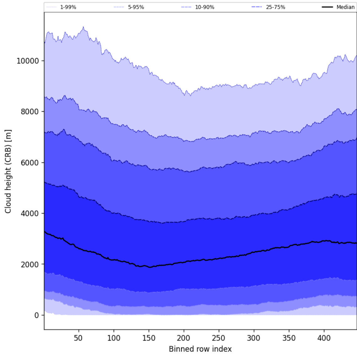
Figure 57: Along track statistics of “Cloud height (CRB)” for 2025-04-11 to 2025-04-11
