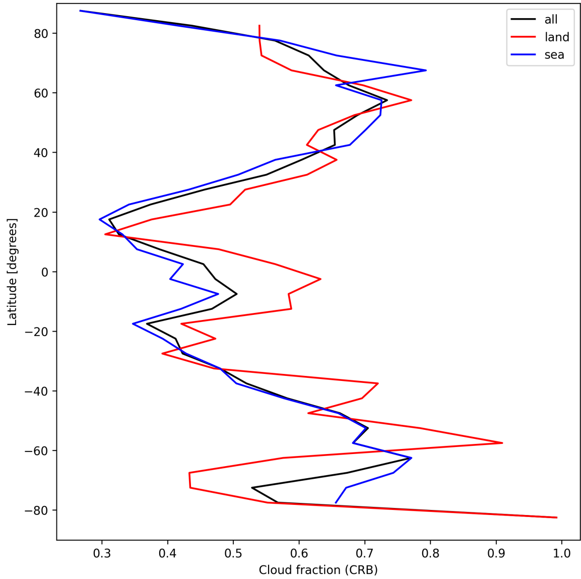
Figure 24: Zonal average of “Cloud fraction (CRB)” for 2025-04-11 to 2025-04-11.
