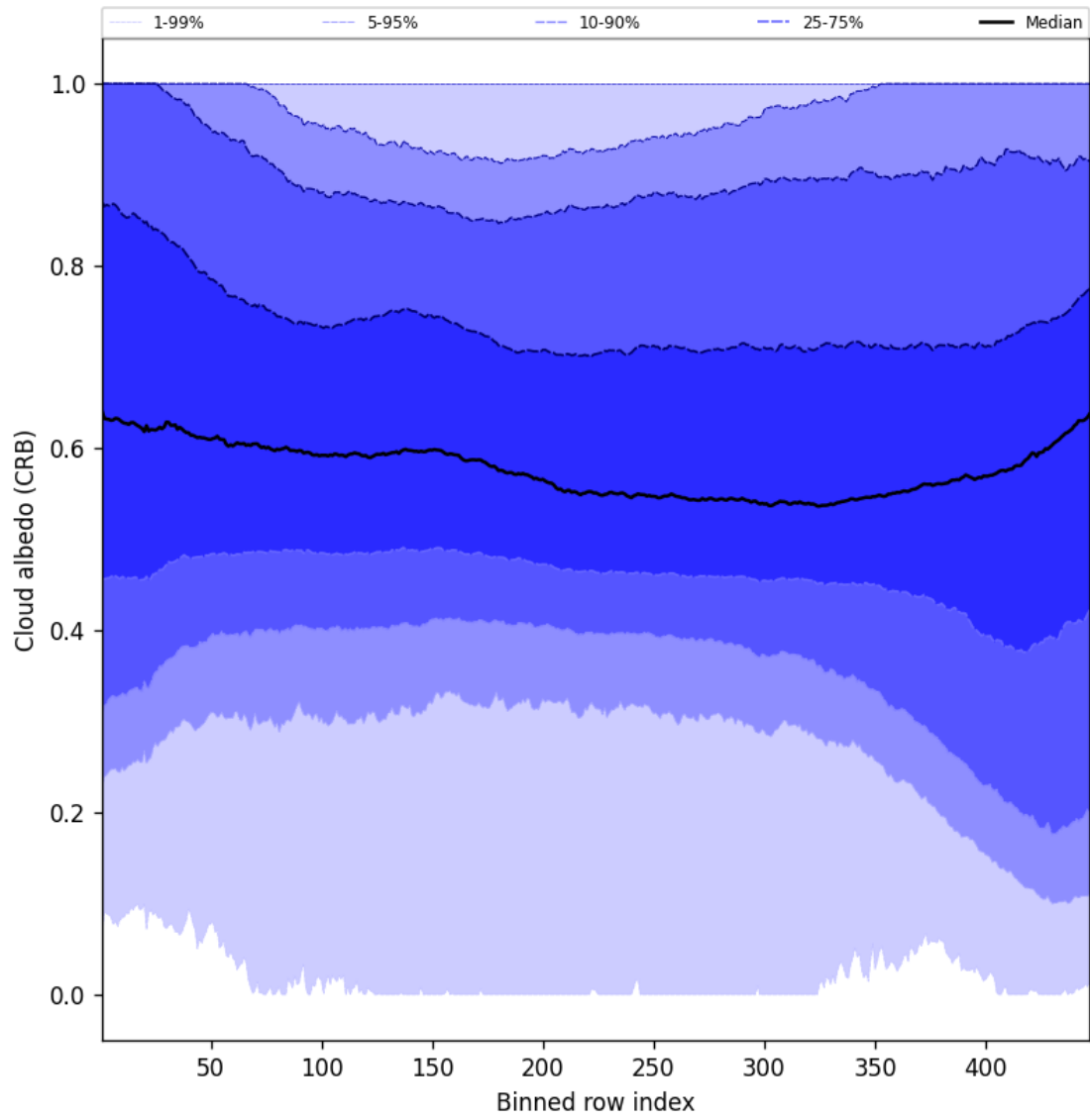
Figure 58: Along track statistics of “Cloud albedo (CRB)” for 2025-04-11 to 2025-04-11
