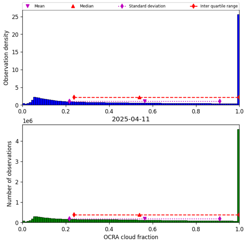
Figure 48: Histogram of “OCRA cloud fraction” for 2025-04-11 to 2025-04-11
