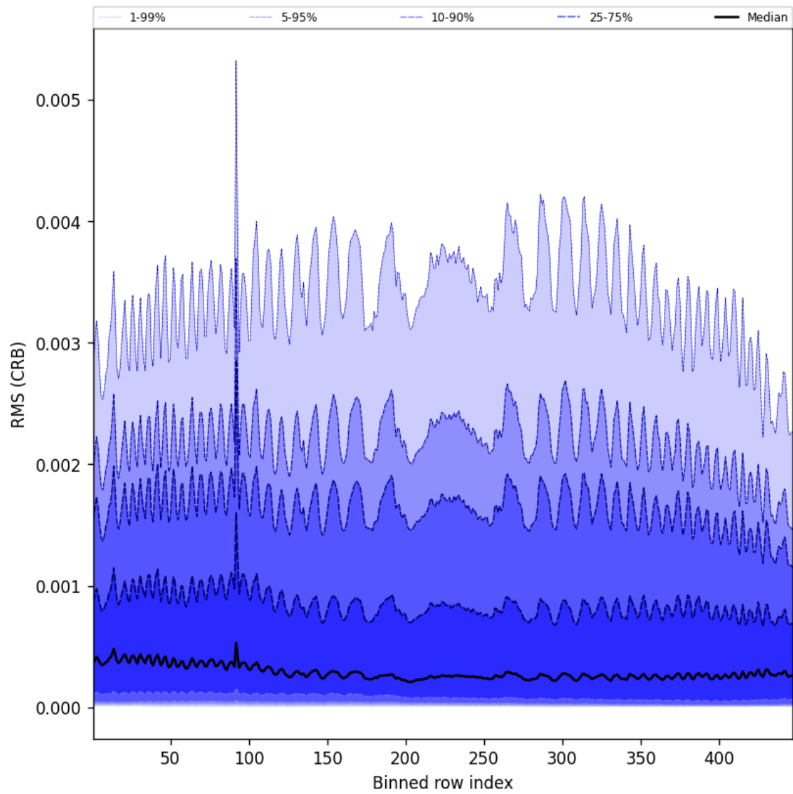
Figure 62: Along track statistics of “RMS (CRB)” for 2025-04-11 to 2025-04-11
