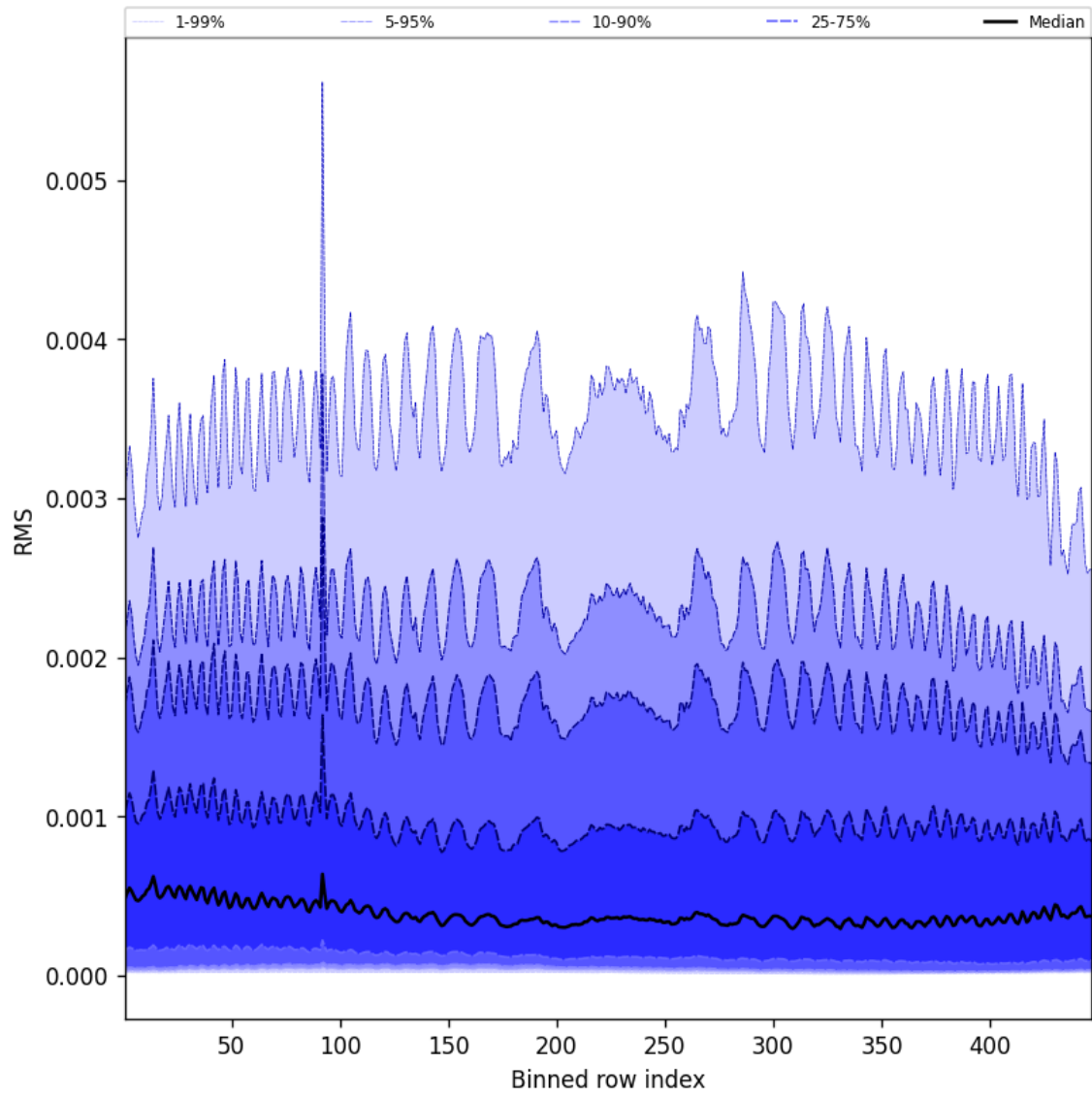
Figure 61: Along track statistics of “RMS” for 2025-04-11 to 2025-04-11
