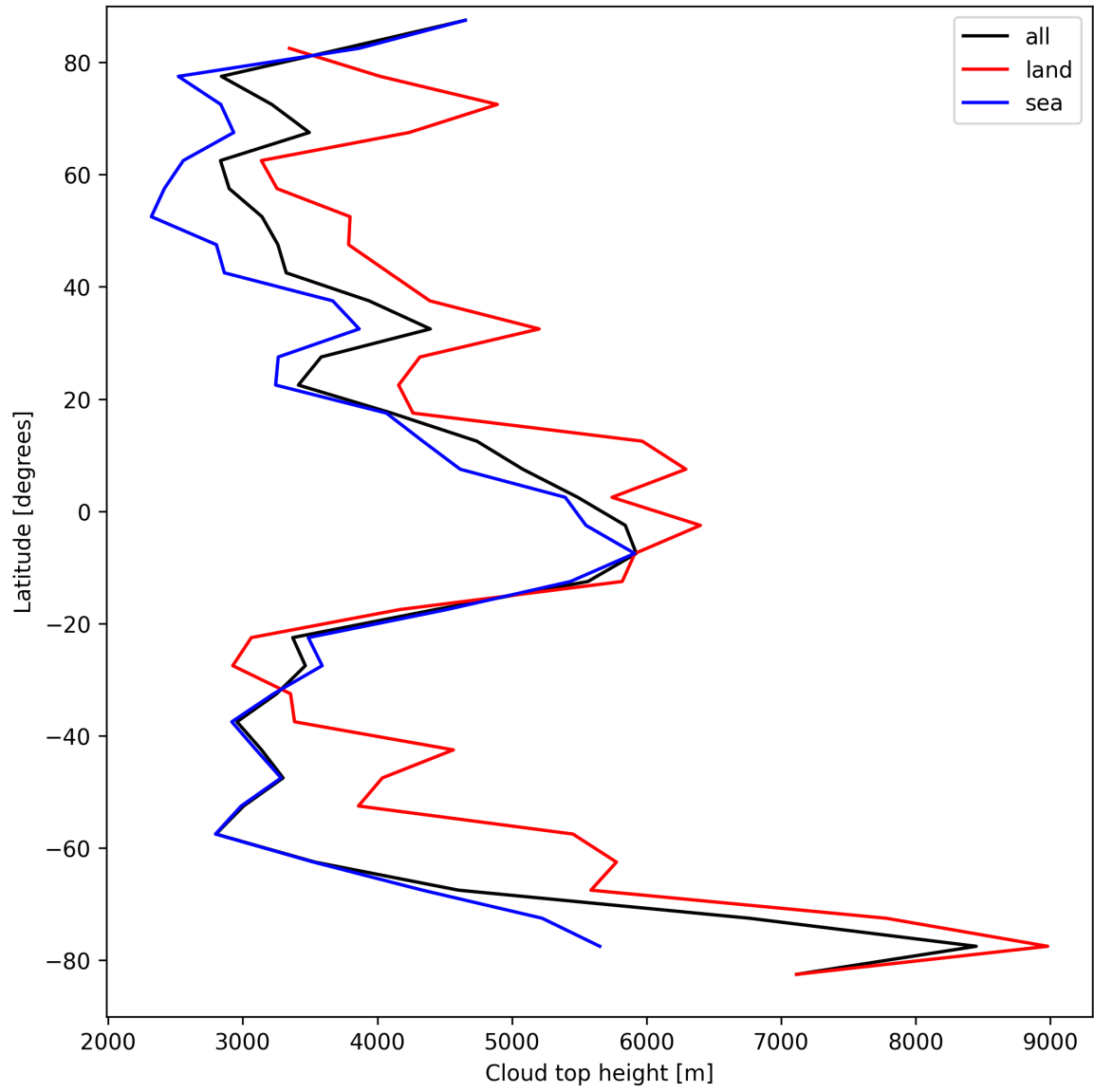
Figure 22: Zonal average of “Cloud top height” for 2025-04-11 to 2025-04-11.
