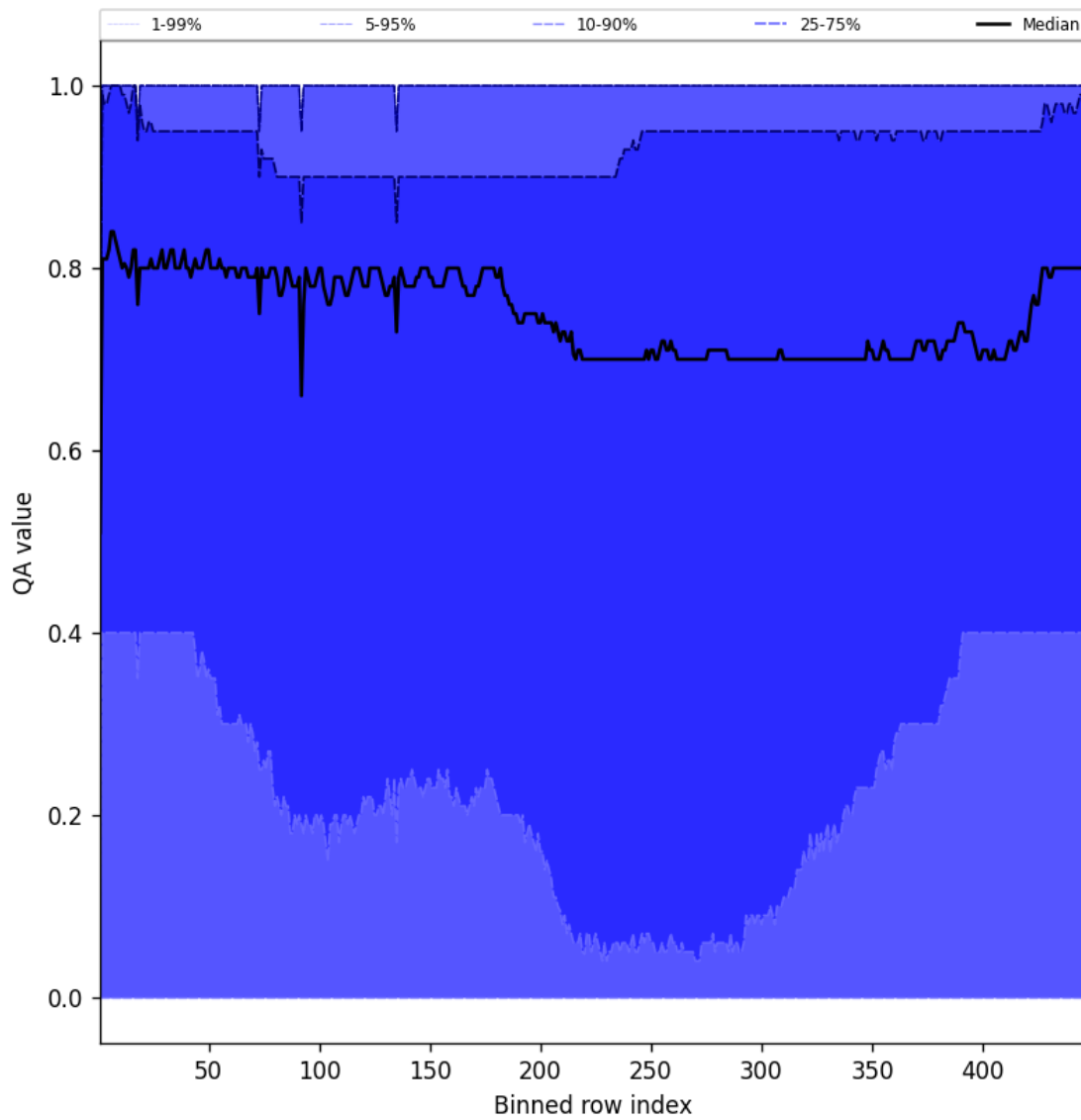
Figure 52: Along track statistics of “QA value” for 2025-04-11 to 2025-04-11
