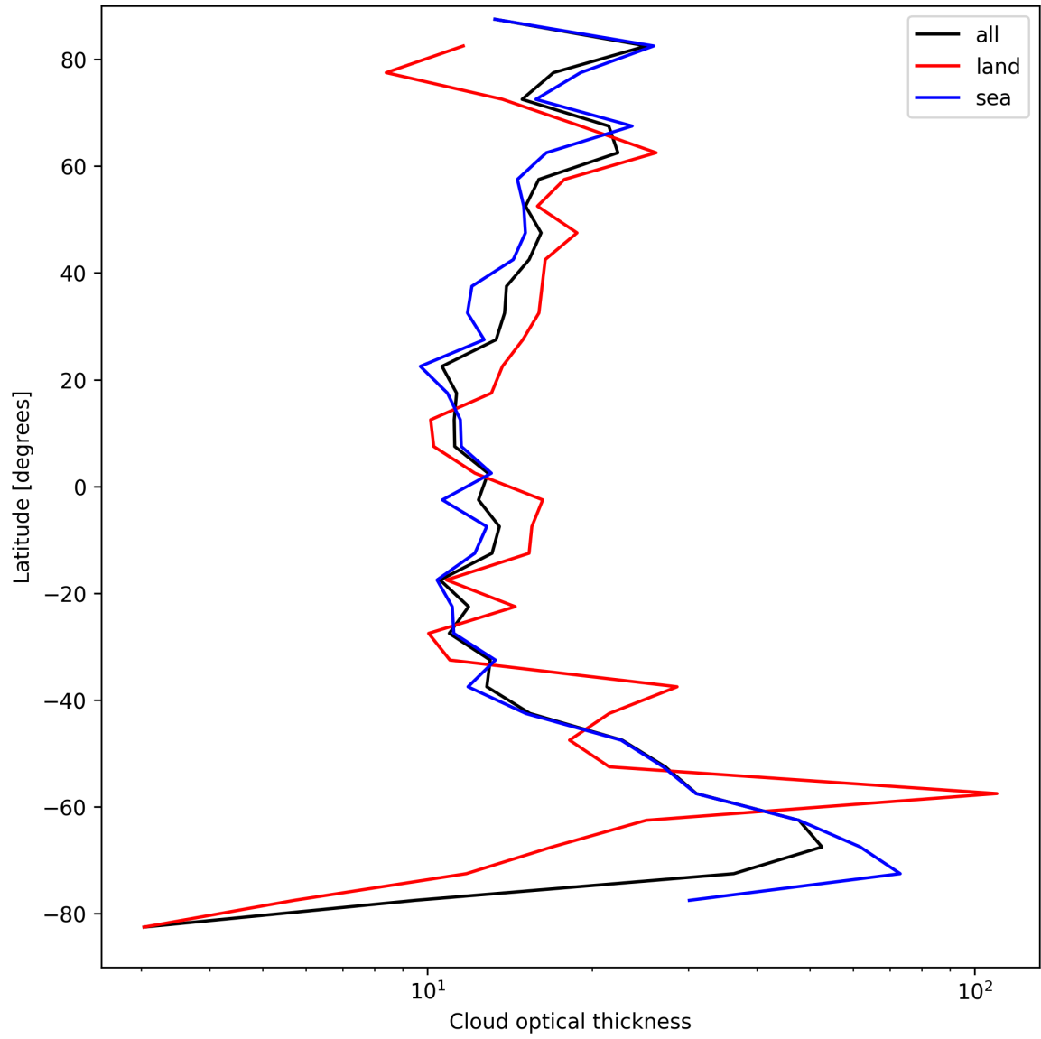
Figure 23: Zonal average of “Cloud optical thickness” for 2025-04-11 to 2025-04-11.
