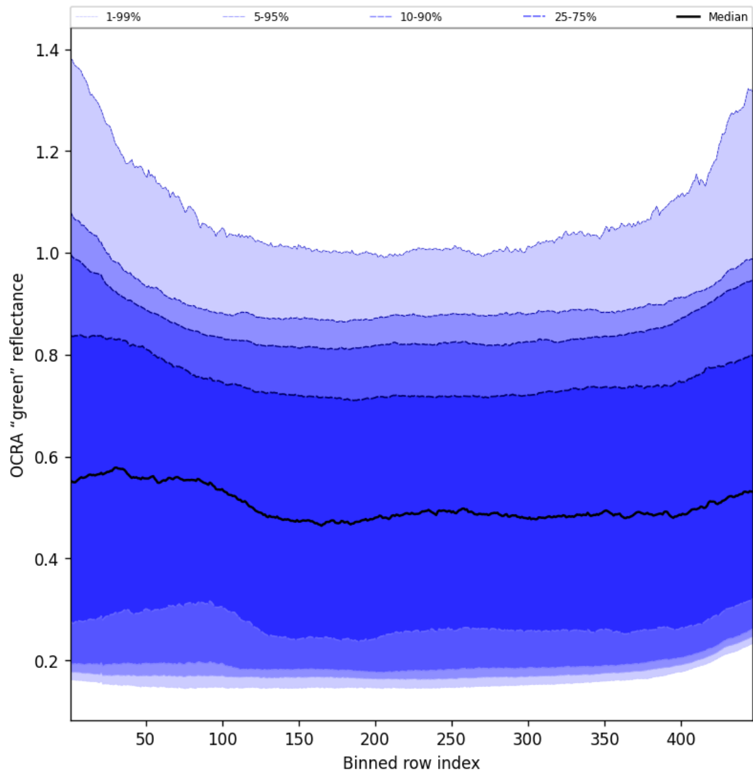
Figure 66: Along track statistics of “OCRA “green” reflectance” for 2025-04-11 to 2025-04-11
