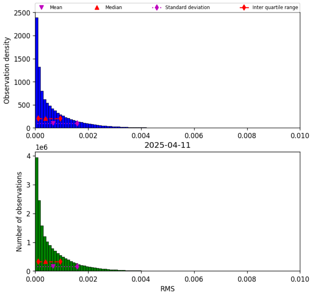
Figure 45: Histogram of “RMS” for 2025-04-11 to 2025-04-11
