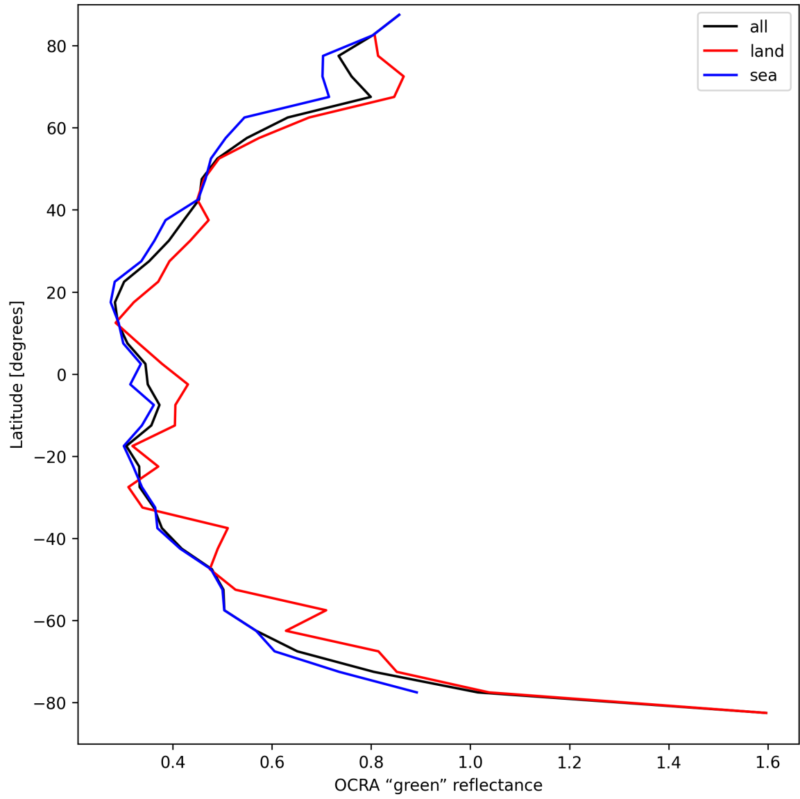
Figure 34: Zonal average of “OCRA “green” reflectance” for 2025-04-11 to 2025-04-11.
