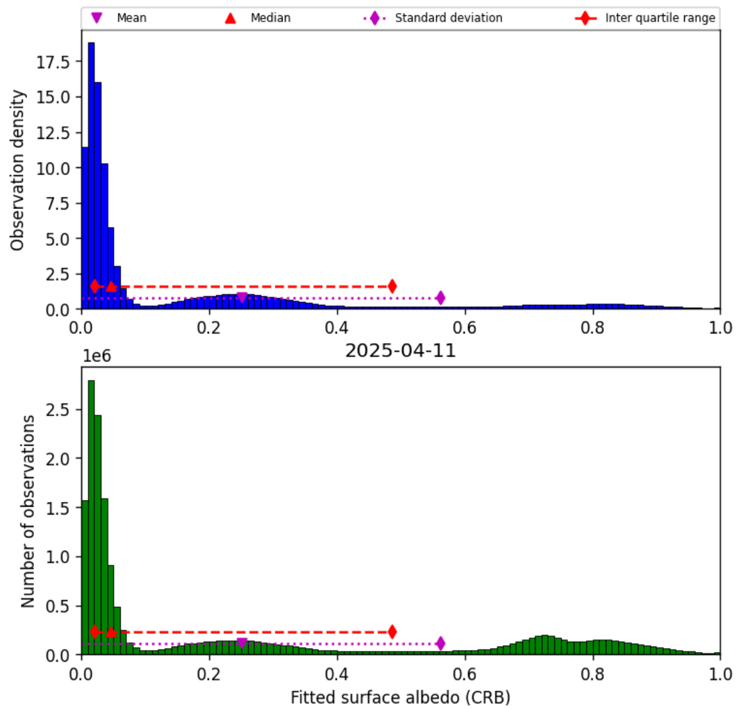
Figure 44: Histogram of “Fitted surface albedo (CRB)” for 2025-04-11 to 2025-04-11
