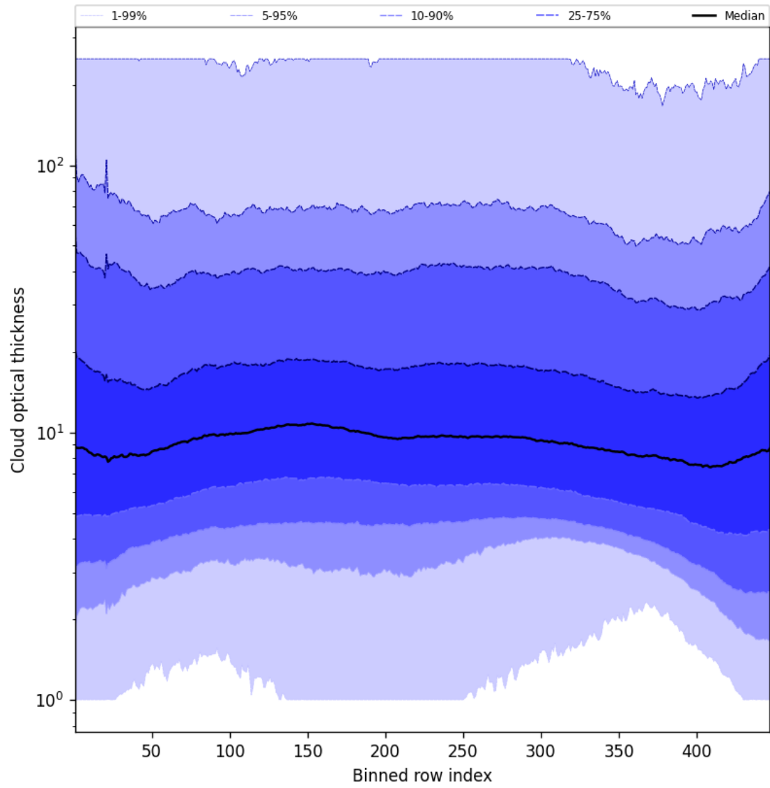
Figure 55: Along track statistics of “Cloud optical thickness” for 2025-04-11 to 2025-04-11
