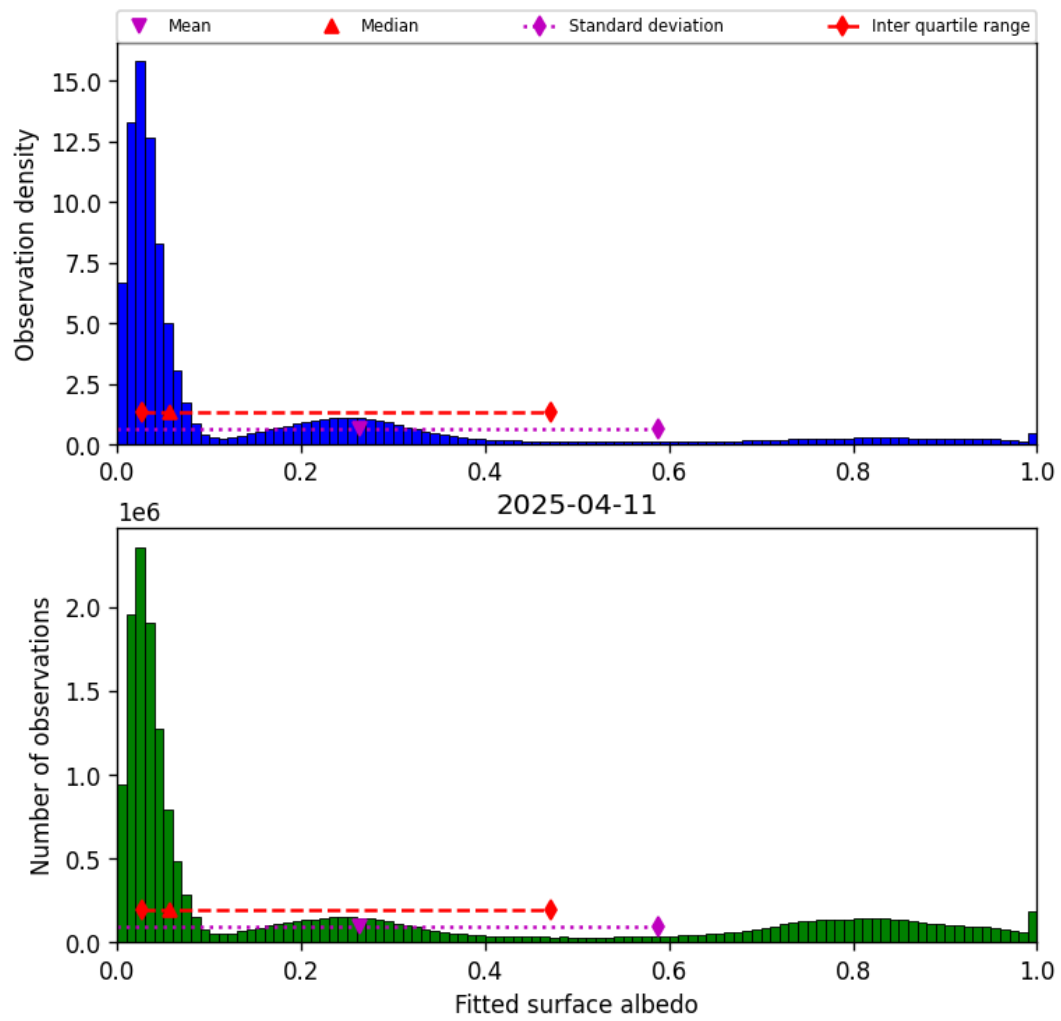
Figure 43: Histogram of “Fitted surface albedo” for 2025-04-11 to 2025-04-11
