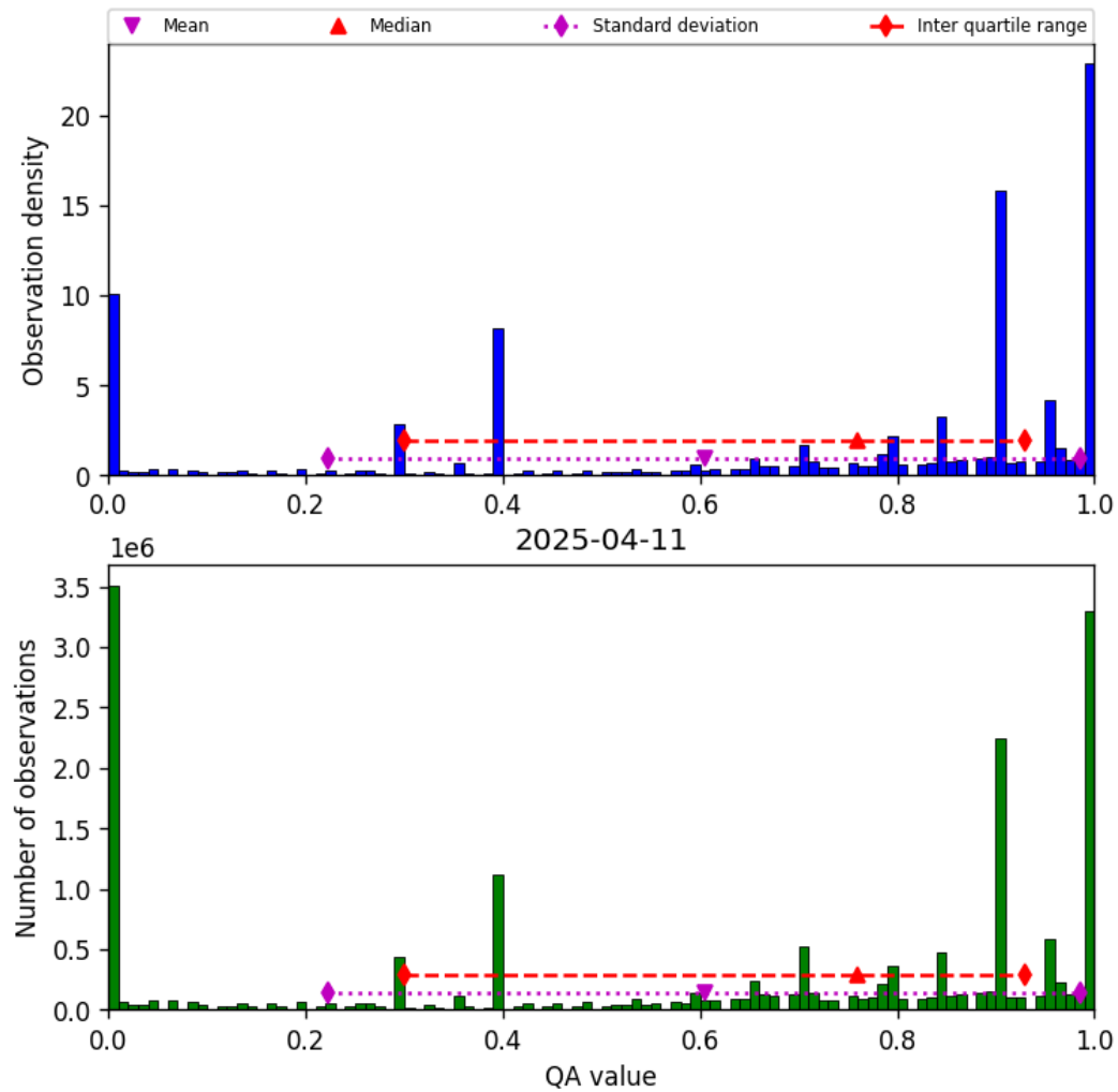
Figure 36: Histogram of “QA value” for 2025-04-11 to 2025-04-11
