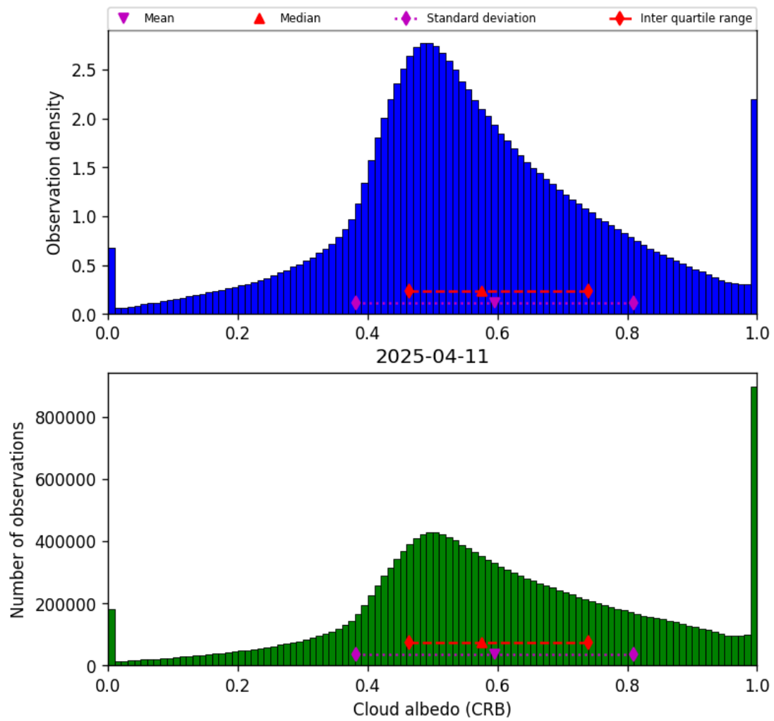
Figure 42: Histogram of “Cloud albedo (CRB)” for 2025-04-11 to 2025-04-11
