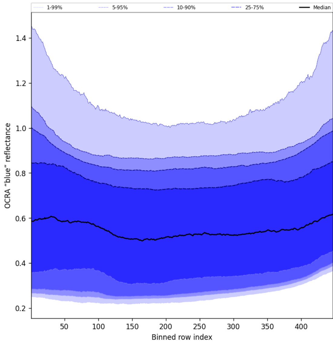
Figure 65: Along track statistics of “OCRA “blue” reflectance” for 2025-04-11 to 2025-04-11
