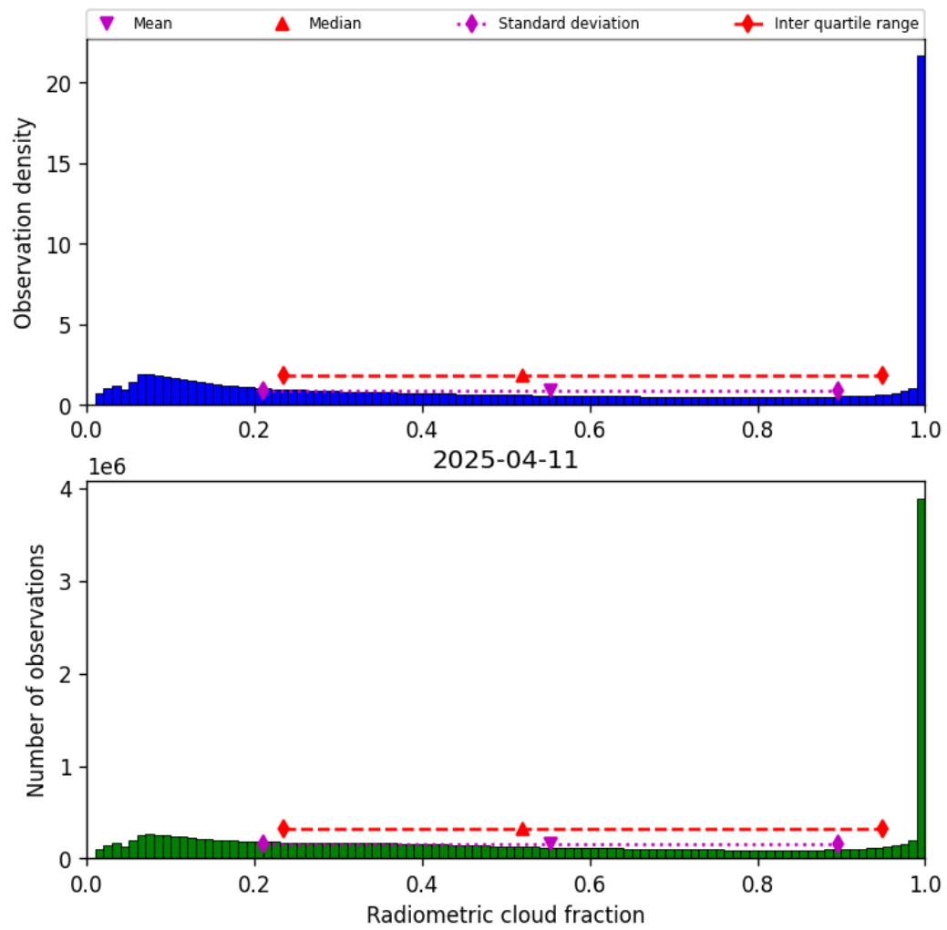
Figure 37: Histogram of “Radiometric cloud fraction” for 2025-04-11 to 2025-04-11
