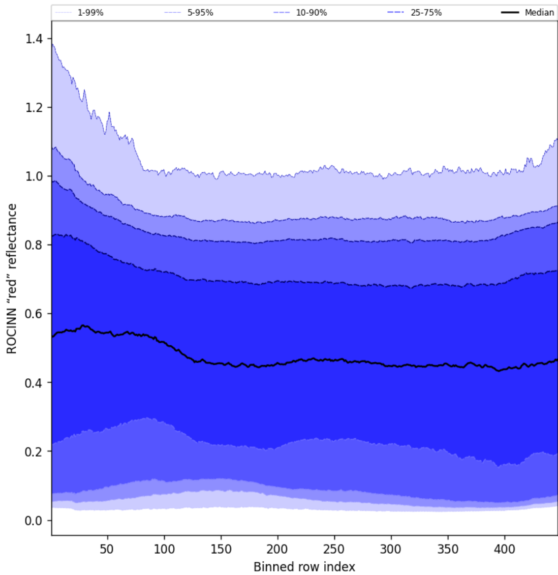
Figure 67: Along track statistics of "ROCINN "red" reflectance" for 2025-04-11 to 2025-04-11
