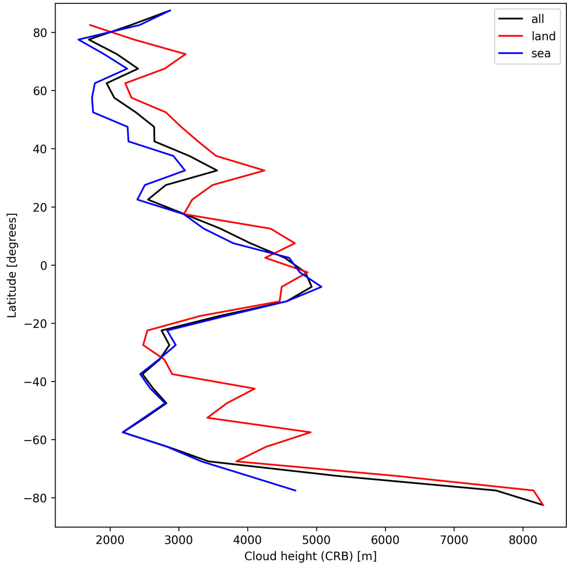
Figure 25: Zonal average of “Cloud height (CRB)” for 2025-04-11 to 2025-04-11.
