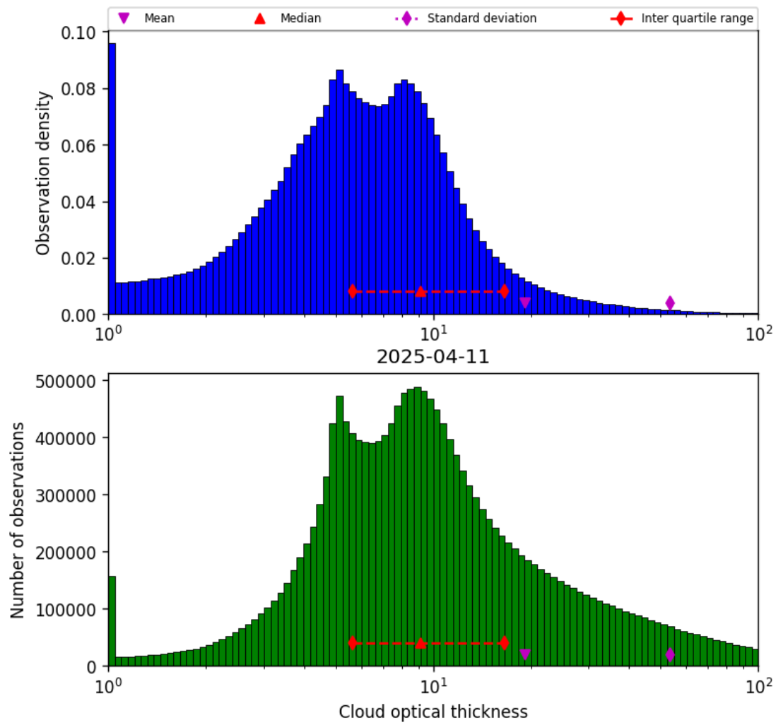
Figure 39: Histogram of “Cloud optical thickness” for 2025-04-11 to 2025-04-11
