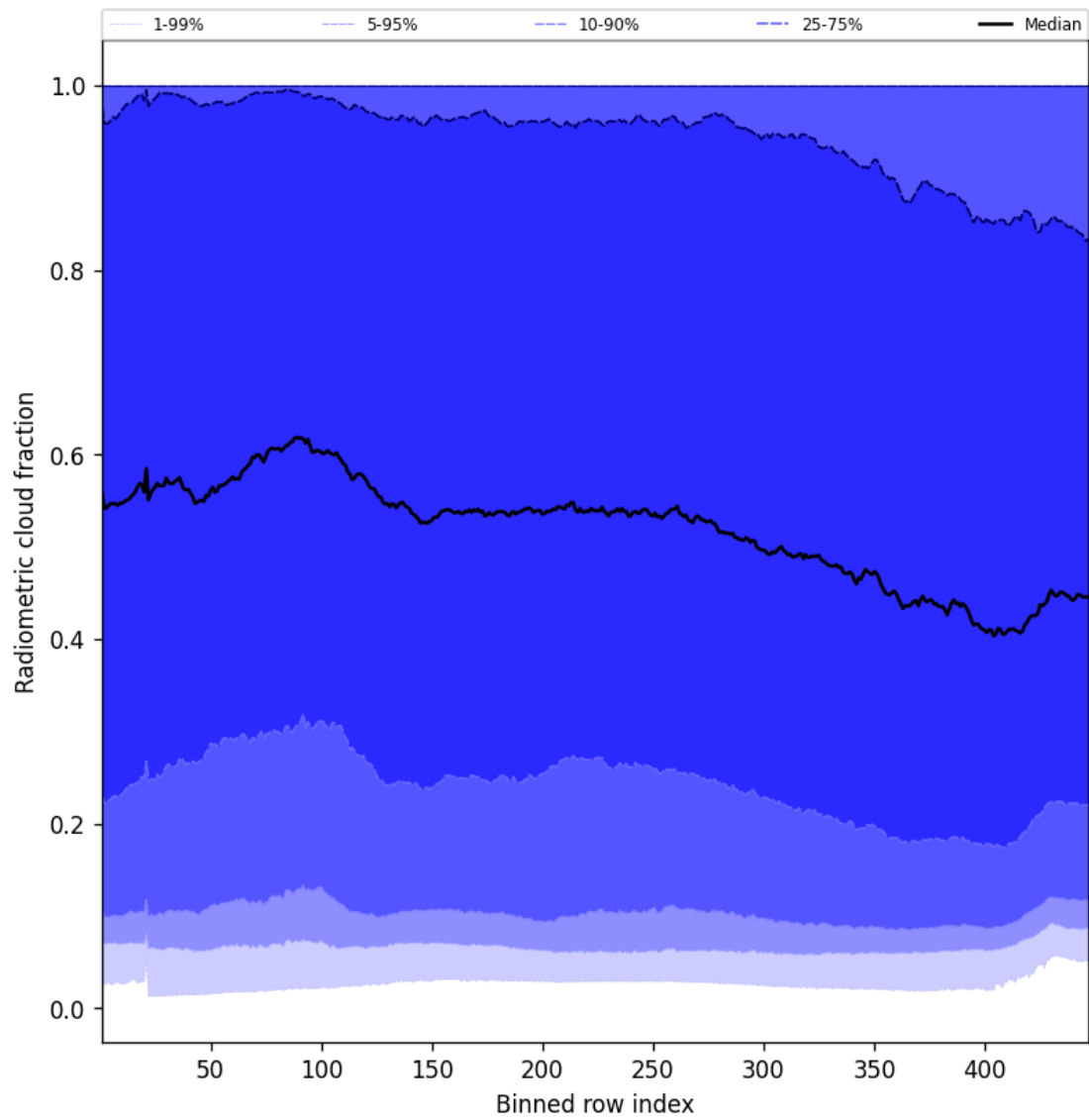
Figure 53: Along track statistics of “Radiometric cloud fraction” for 2025-04-11 to 2025-04-11
