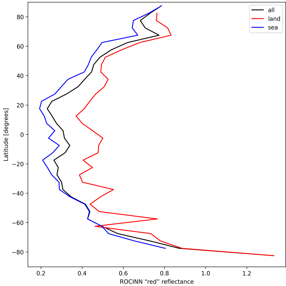
Figure 35: Zonal average of “ROCINN “red” reflectance” for 2025-04-11 to 2025-04-11.
