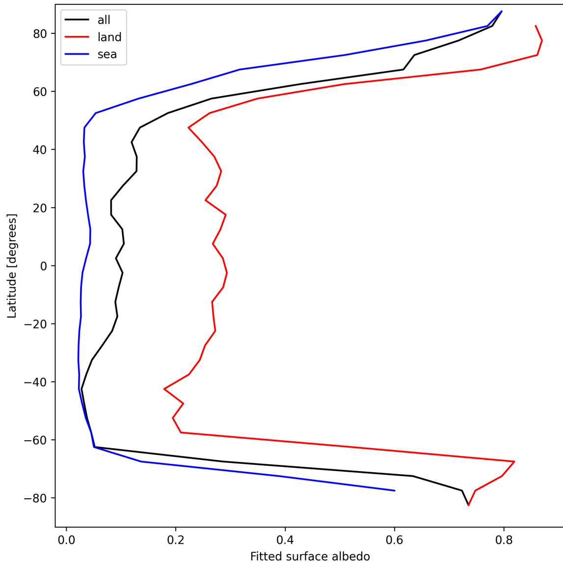
Figure 27: Zonal average of “Fitted surface albedo” for 2025-04-11 to 2025-04-11.
