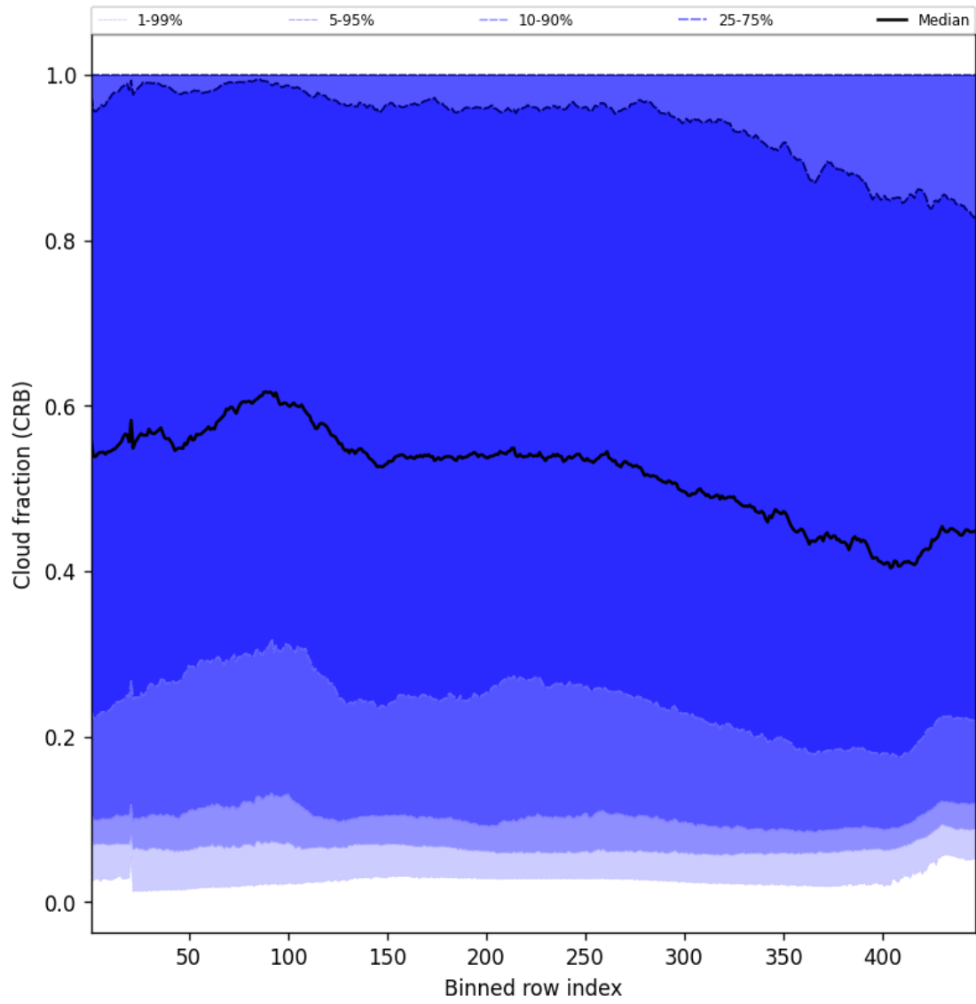
Figure 56: Along track statistics of “Cloud fraction (CRB)” for 2025-04-11 to 2025-04-11
