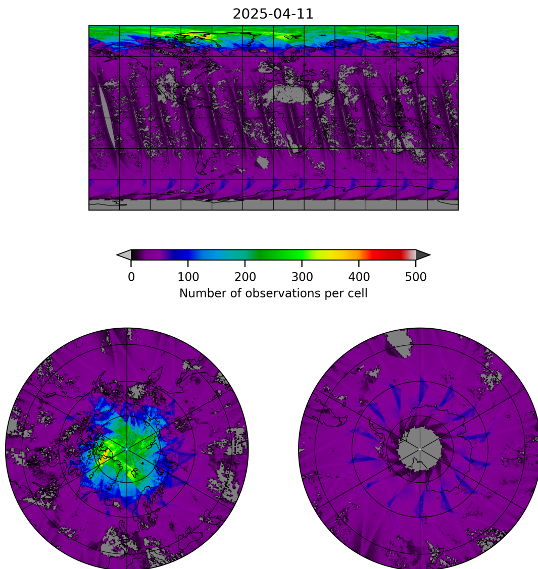
Figure 19: Map of the number of observations for 2025-04-11 to 2025-04-11
