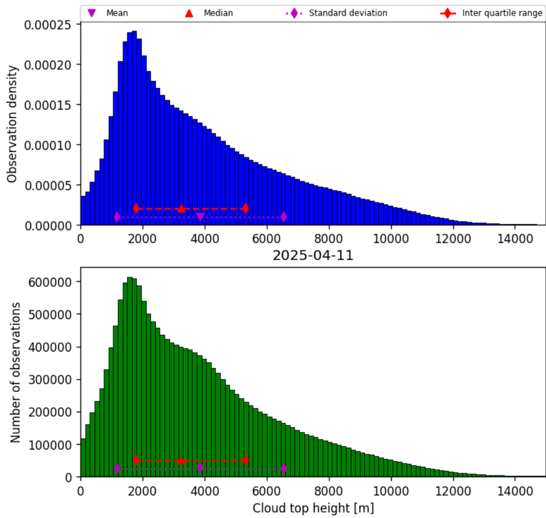
Figure 38: Histogram of “Cloud top height” for 2025-04-11 to 2025-04-11
