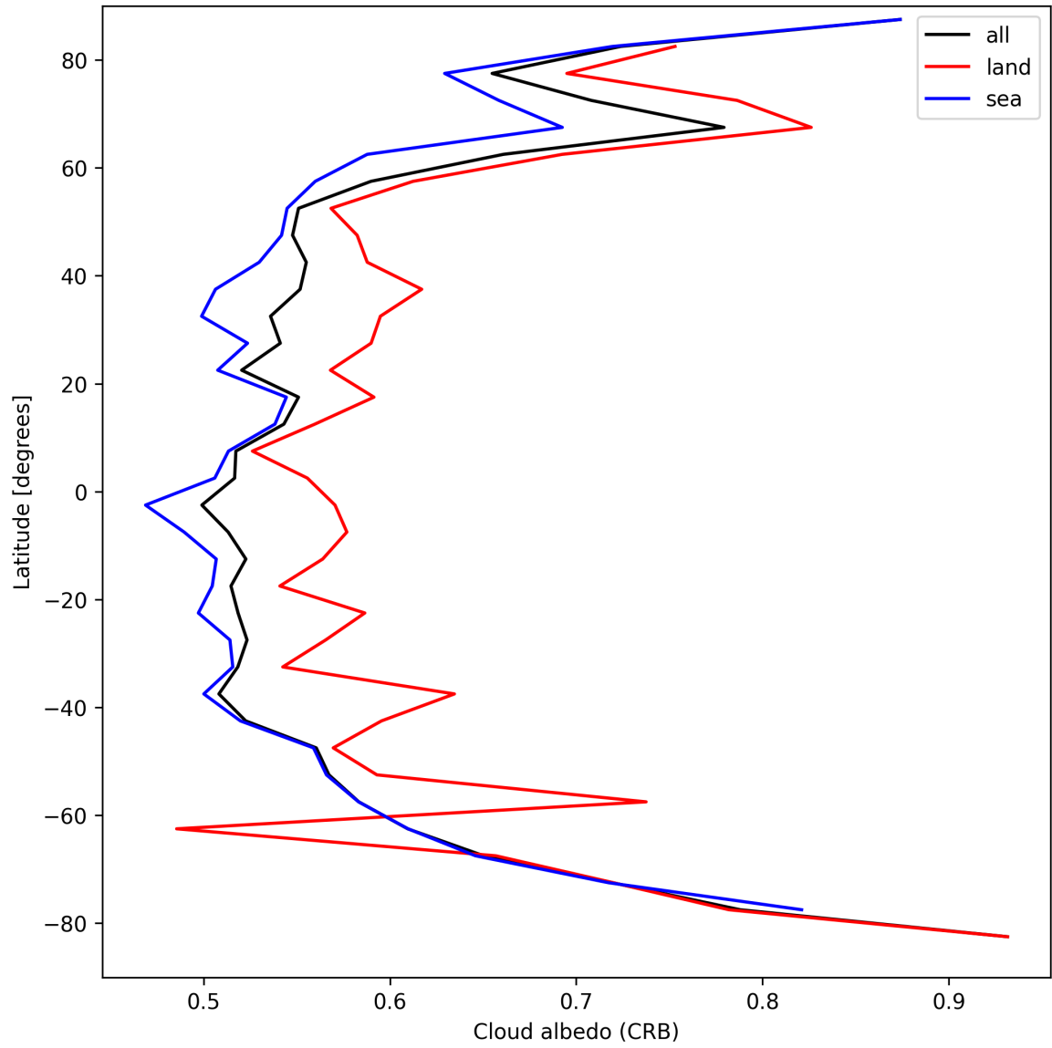
Figure 26: Zonal average of “Cloud albedo (CRB)” for 2025-04-11 to 2025-04-11.
