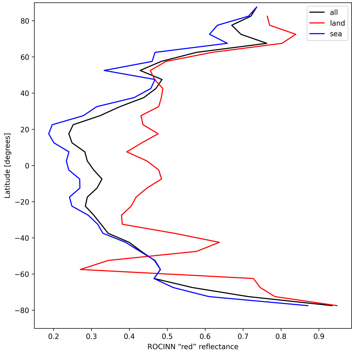
Figure 35: Zonal average of "ROCINN "red" reflectance" for 2025-04-14 to 2025-04-15.
