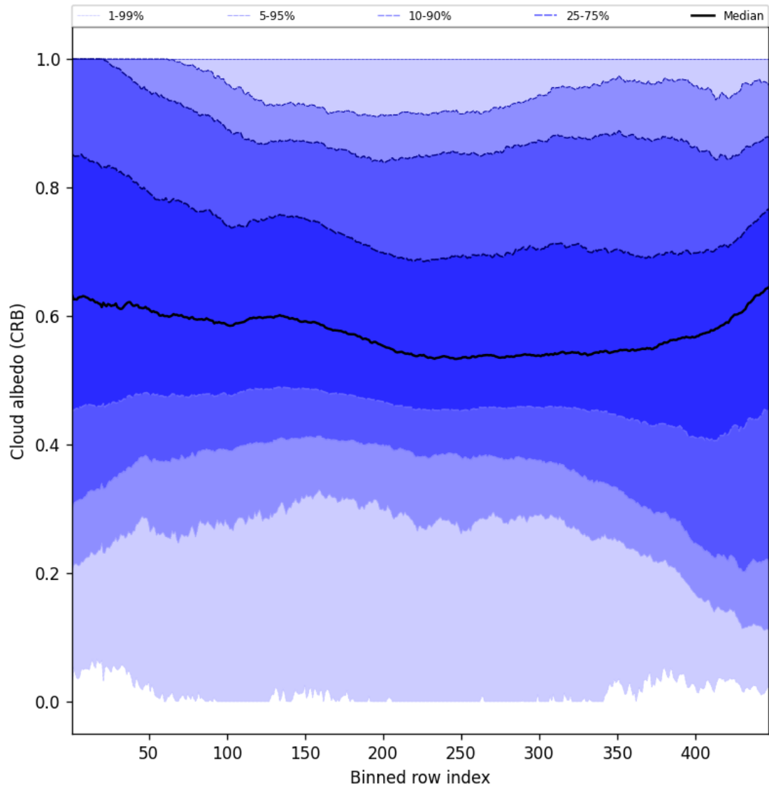
Figure 58: Along track statistics of “Cloud albedo (CRB)” for 2025-04-14 to 2025-04-15
