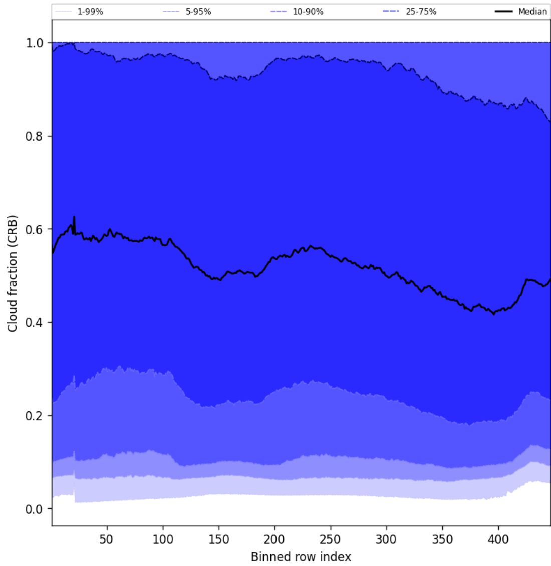
Figure 56: Along track statistics of “Cloud fraction (CRB)” for 2025-04-14 to 2025-04-15
