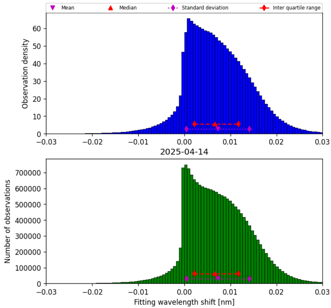
Figure 47: Histogram of “Fitting wavelength shift” for 2025-04-14 to 2025-04-15
