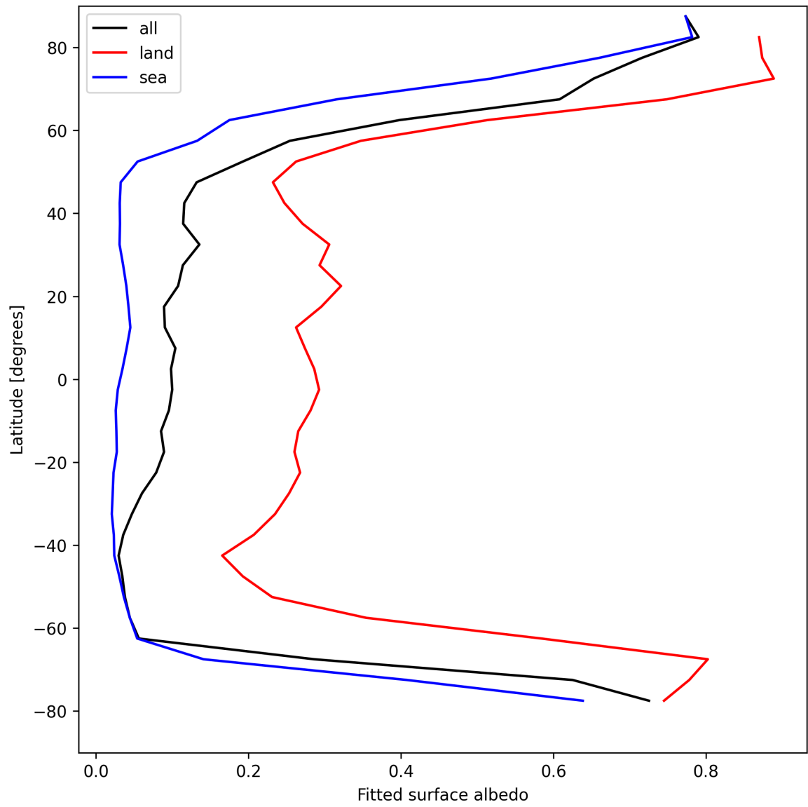
Figure 27: Zonal average of “Fitted surface albedo” for 2025-04-14 to 2025-04-15.
