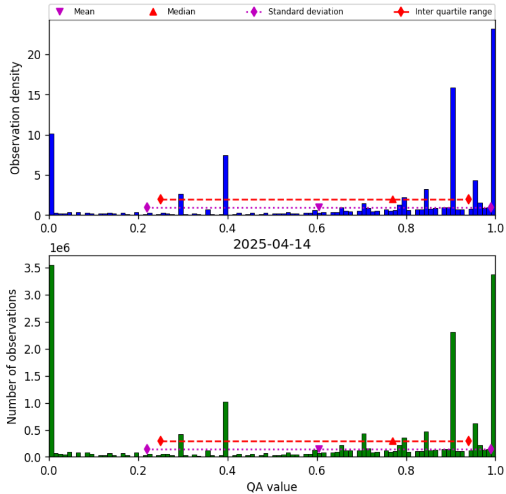
Figure 36: Histogram of “QA value” for 2025-04-14 to 2025-04-15
