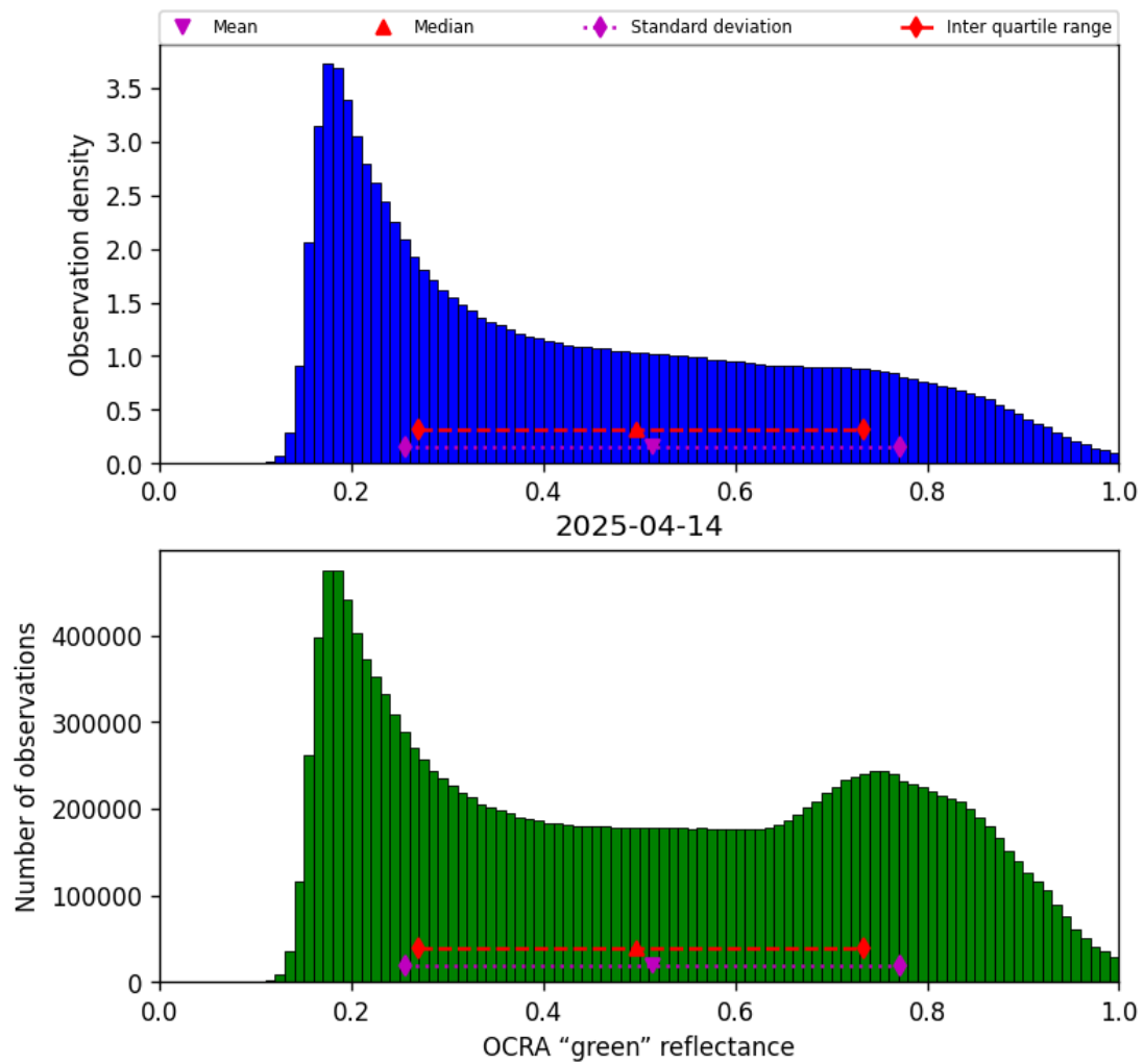
Figure 50: Histogram of “OCRA “green” reflectance” for 2025-04-14 to 2025-04-15
