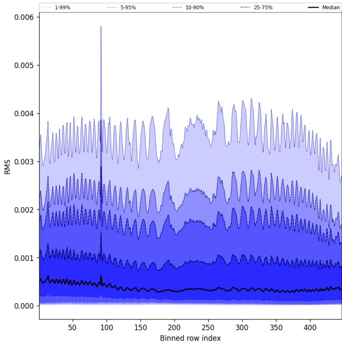
Figure 61: Along track statistics of “RMS” for 2025-04-14 to 2025-04-15
