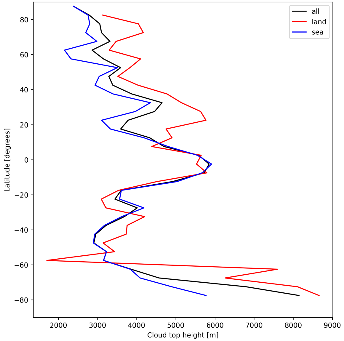
Figure 22: Zonal average of “Cloud top height” for 2025-04-14 to 2025-04-15.
