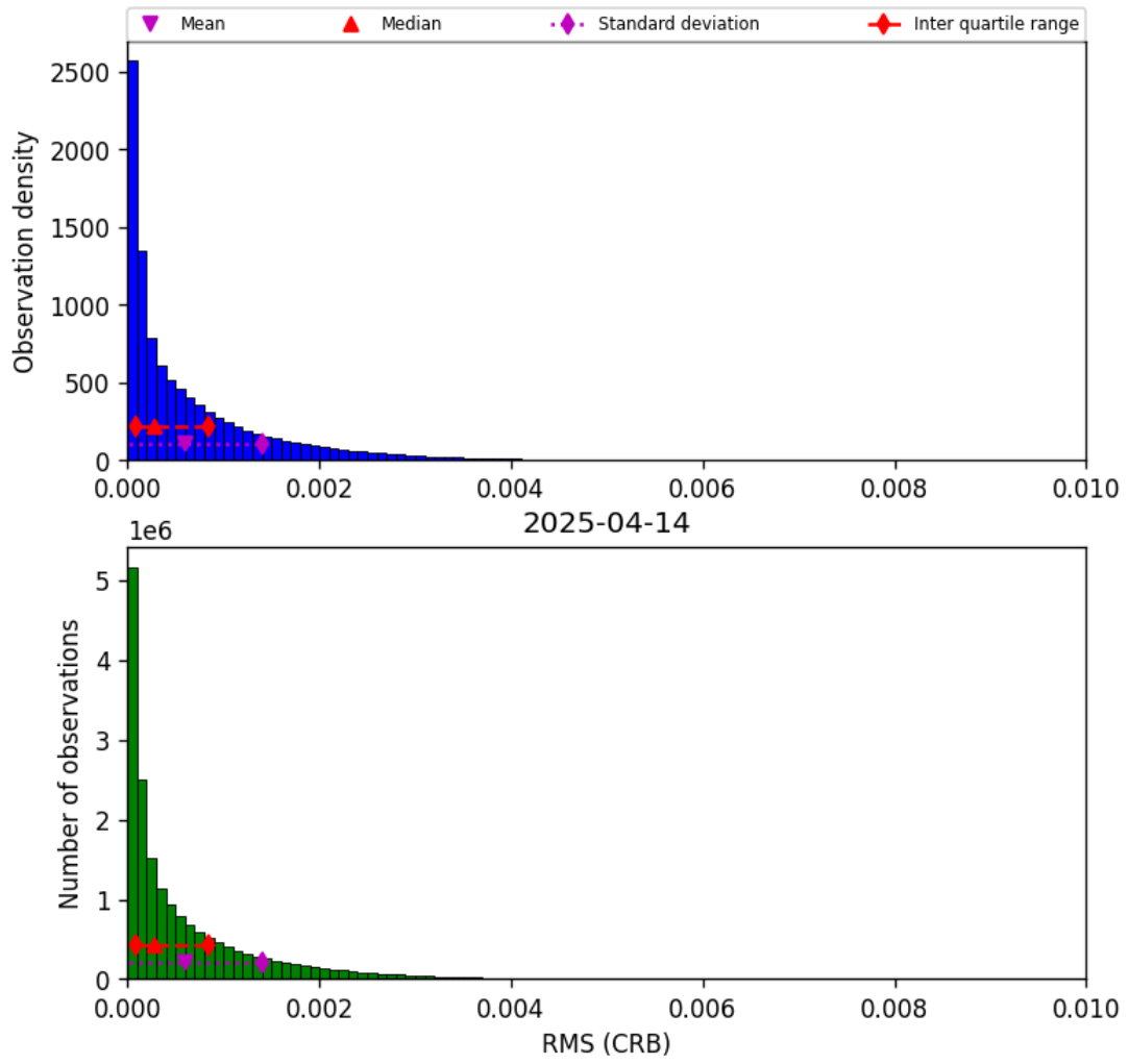
Figure 46: Histogram of “RMS (CRB)” for 2025-04-14 to 2025-04-15
