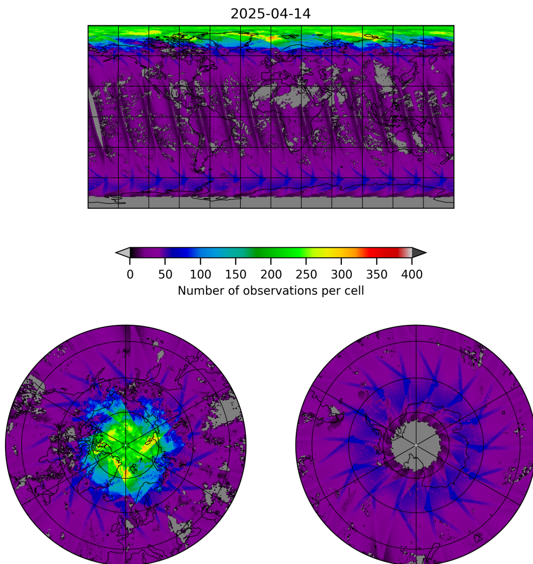
Figure 19: Map of the number of observations for 2025-04-14 to 2025-04-15
