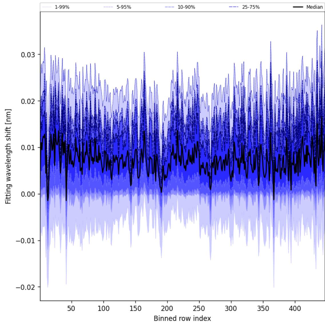
Figure 63: Along track statistics of “Fitting wavelength shift” for 2025-04-14 to 2025-04-15
