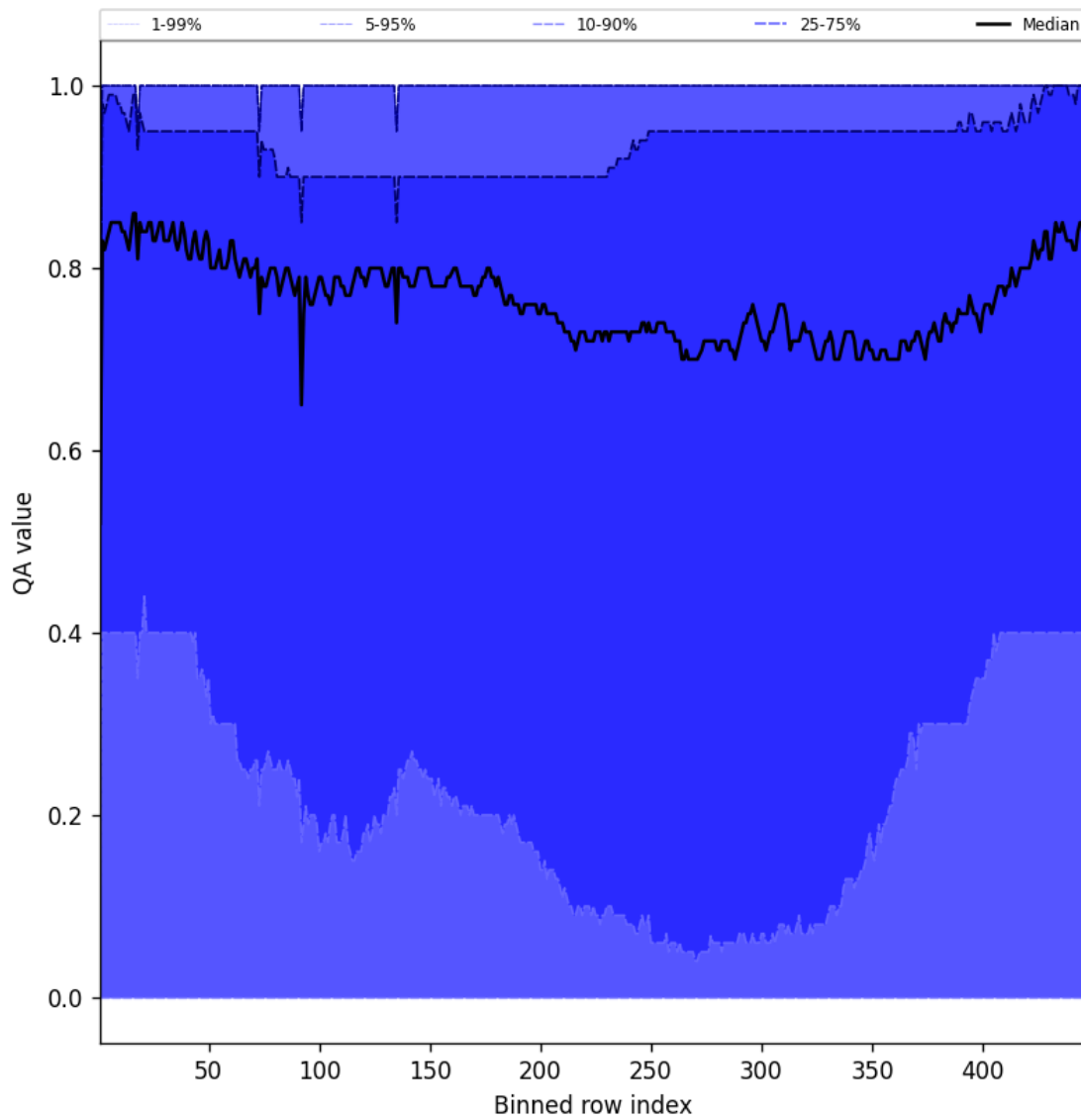
Figure 52: Along track statistics of “QA value” for 2025-04-14 to 2025-04-15
