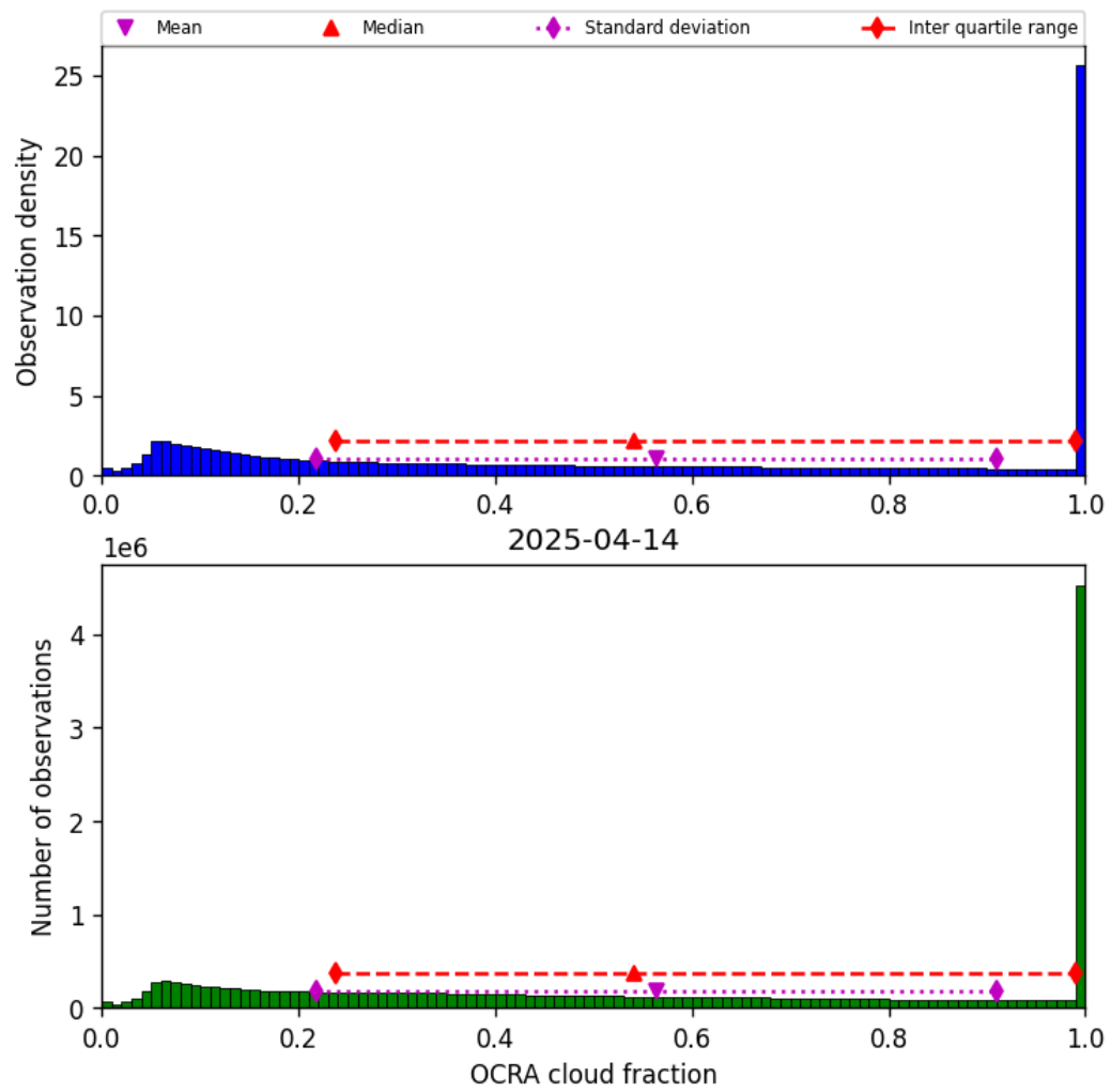
Figure 48: Histogram of “OCRA cloud fraction” for 2025-04-14 to 2025-04-15
