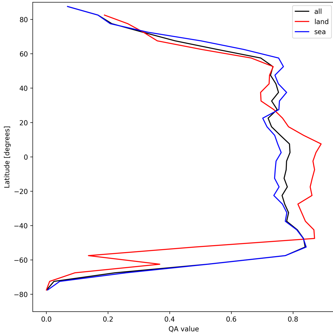
Figure 20: Zonal average of “QA value” for 2025-04-14 to 2025-04-15.
