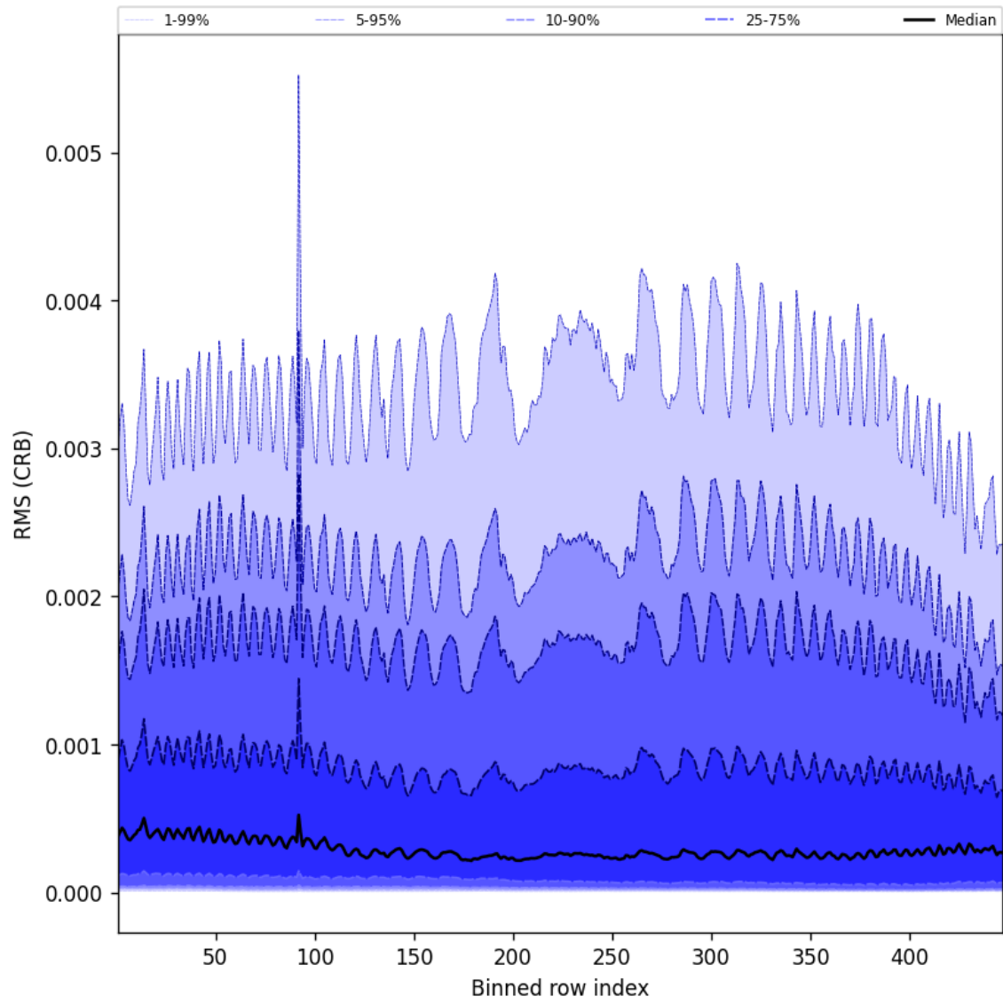
Figure 62: Along track statistics of “RMS (CRB)” for 2025-04-14 to 2025-04-15
