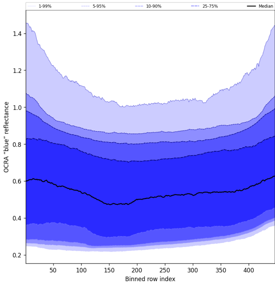
Figure 65: Along track statistics of “OCRA “blue” reflectance” for 2025-04-14 to 2025-04-15
