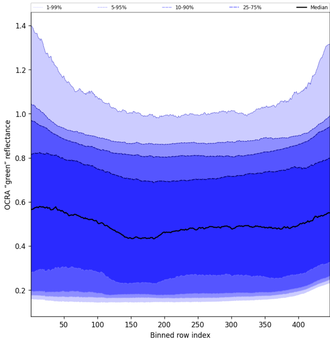
Figure 66: Along track statistics of “OCRA “green” reflectance” for 2025-04-14 to 2025-04-15
