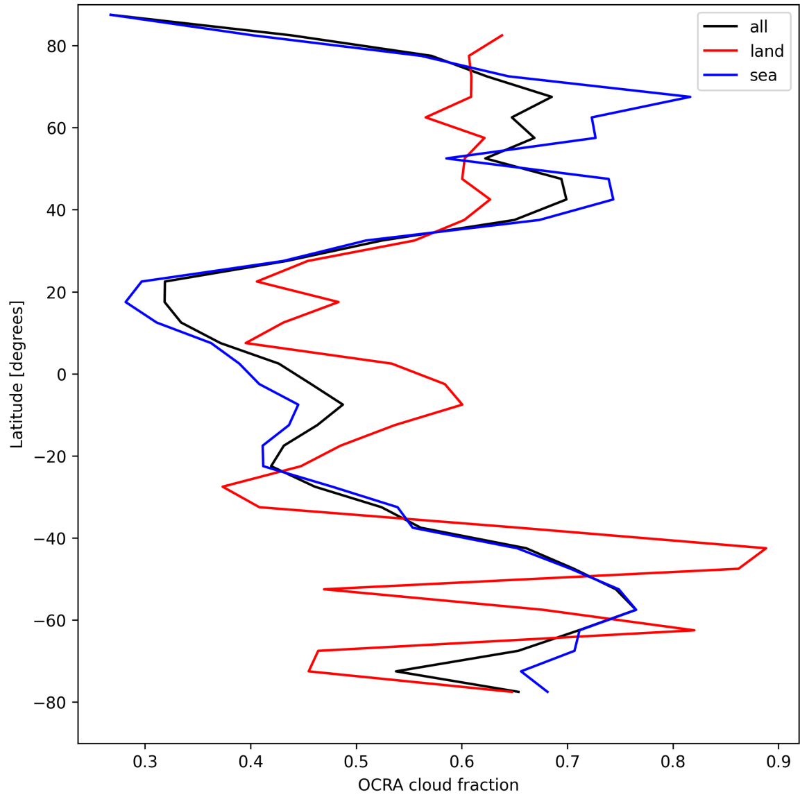
Figure 32: Zonal average of “OCRA cloud fraction” for 2025-04-14 to 2025-04-15.
