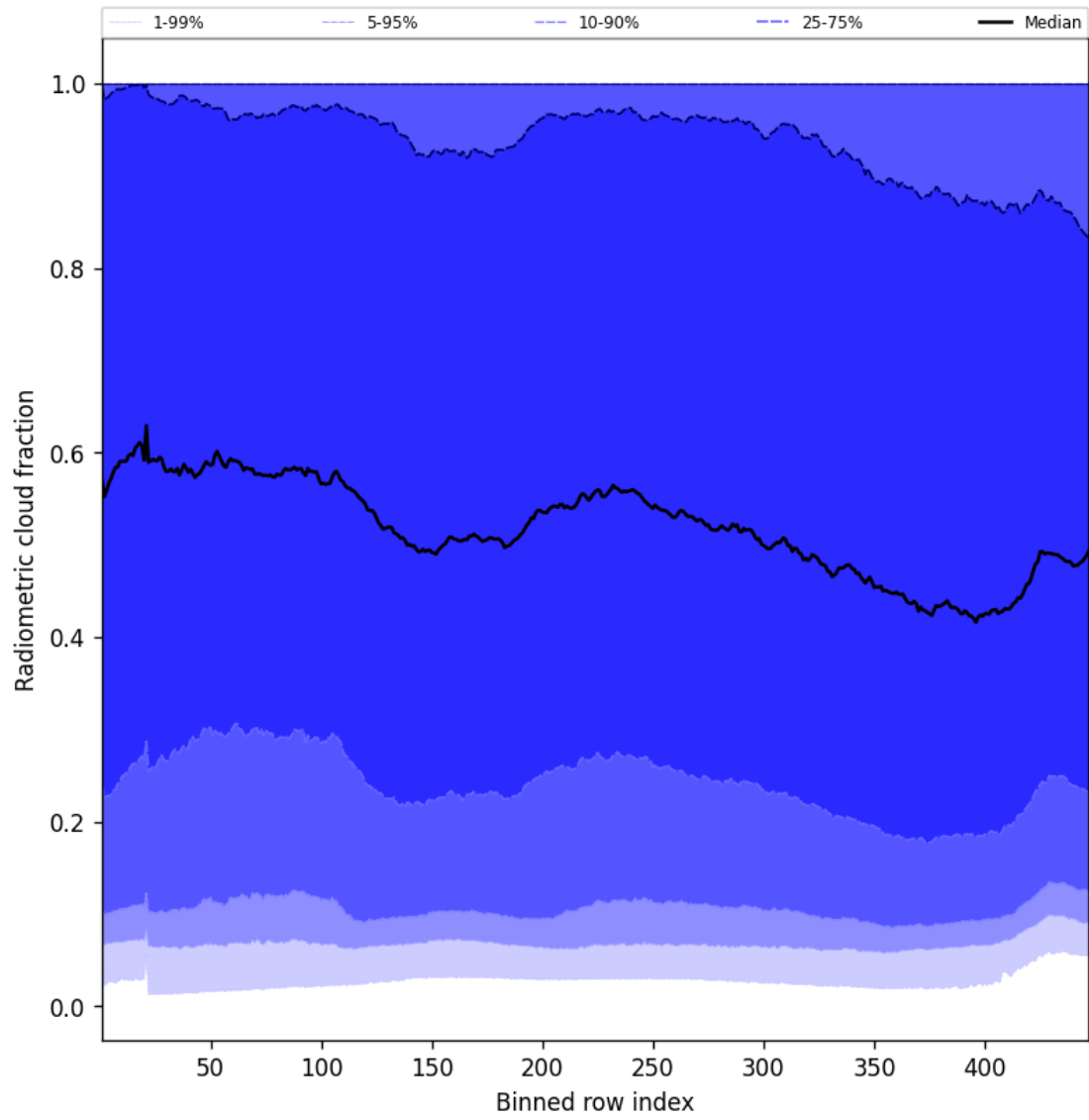
Figure 53: Along track statistics of “Radiometric cloud fraction” for 2025-04-14 to 2025-04-15
