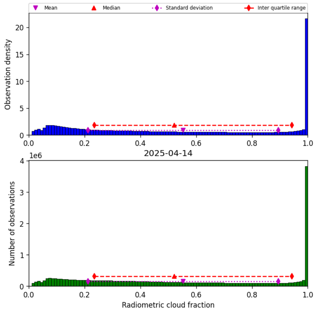
Figure 37: Histogram of “Radiometric cloud fraction” for 2025-04-14 to 2025-04-15
