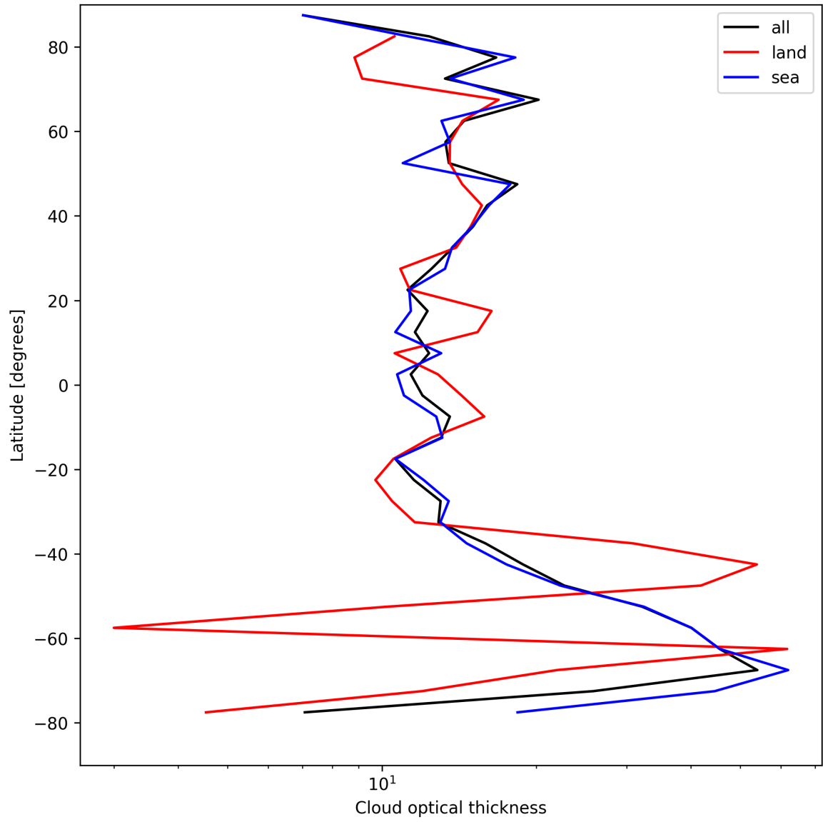
Figure 23: Zonal average of “Cloud optical thickness” for 2025-04-14 to 2025-04-15.
