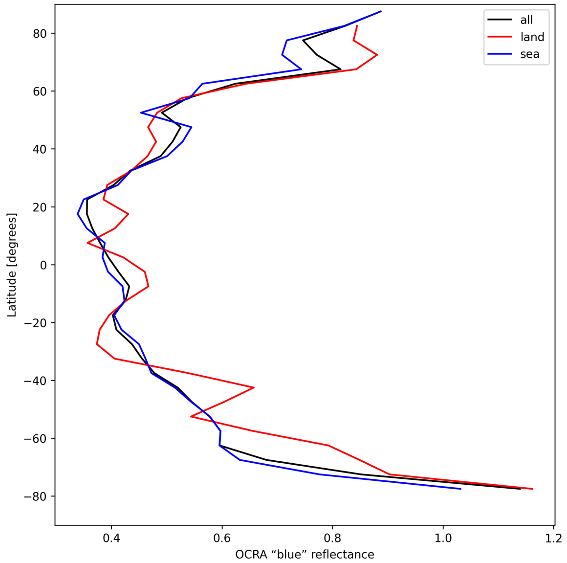
Figure 33: Zonal average of “OCRA “blue” reflectance” for 2025-04-14 to 2025-04-15.
