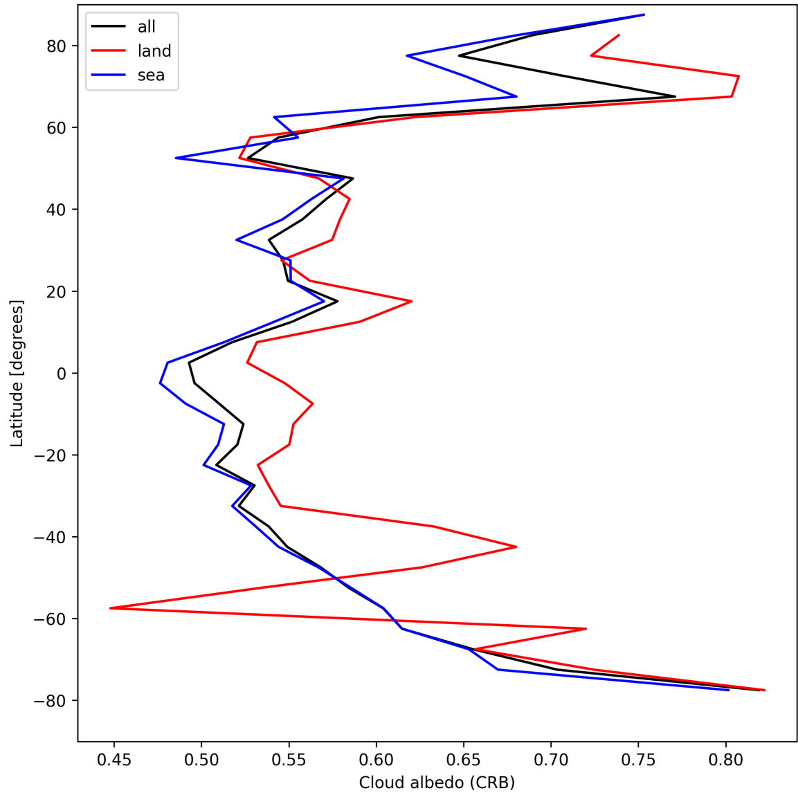
Figure 26: Zonal average of “Cloud albedo (CRB)” for 2025-04-14 to 2025-04-15.
