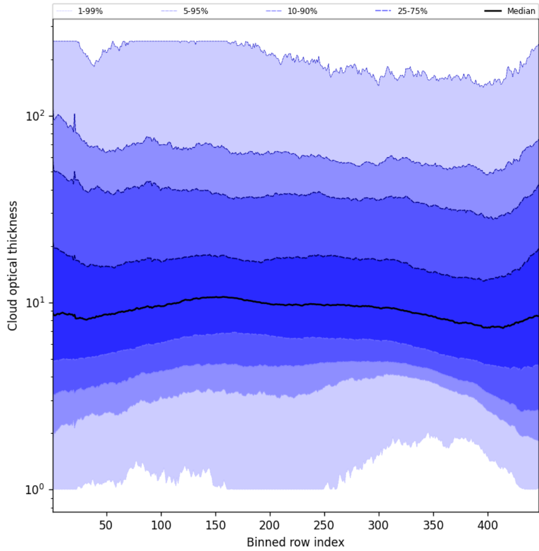
Figure 55: Along track statistics of “Cloud optical thickness” for 2025-04-14 to 2025-04-15
