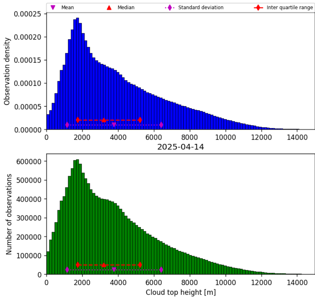
Figure 38: Histogram of “Cloud top height” for 2025-04-14 to 2025-04-15
