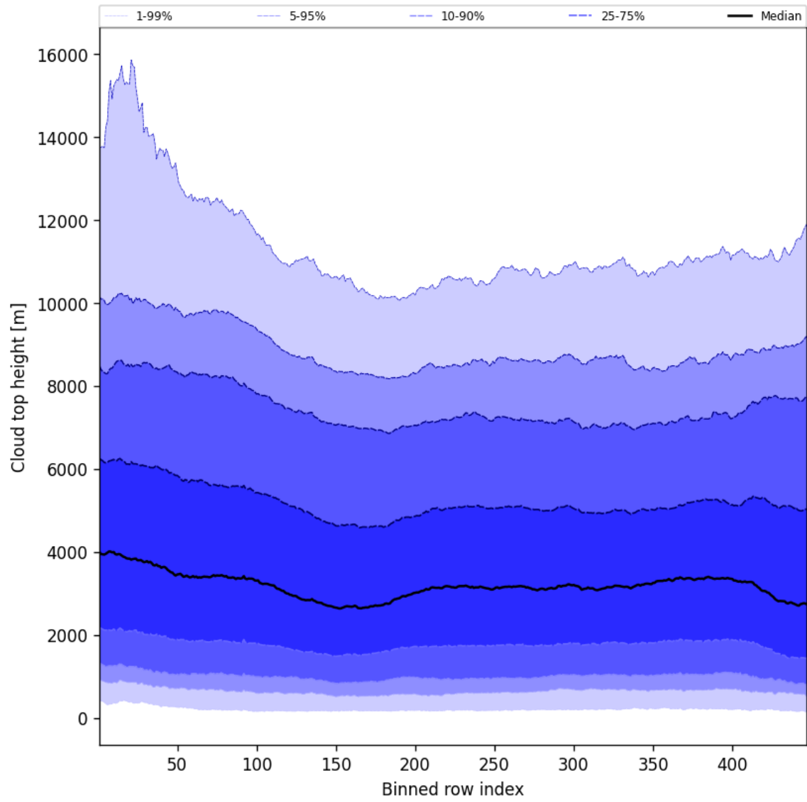
Figure 54: Along track statistics of “Cloud top height” for 2025-04-14 to 2025-04-15
