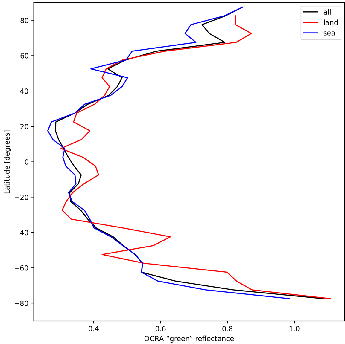
Figure 34: Zonal average of “OCRA “green” reflectance” for 2025-04-14 to 2025-04-15.
