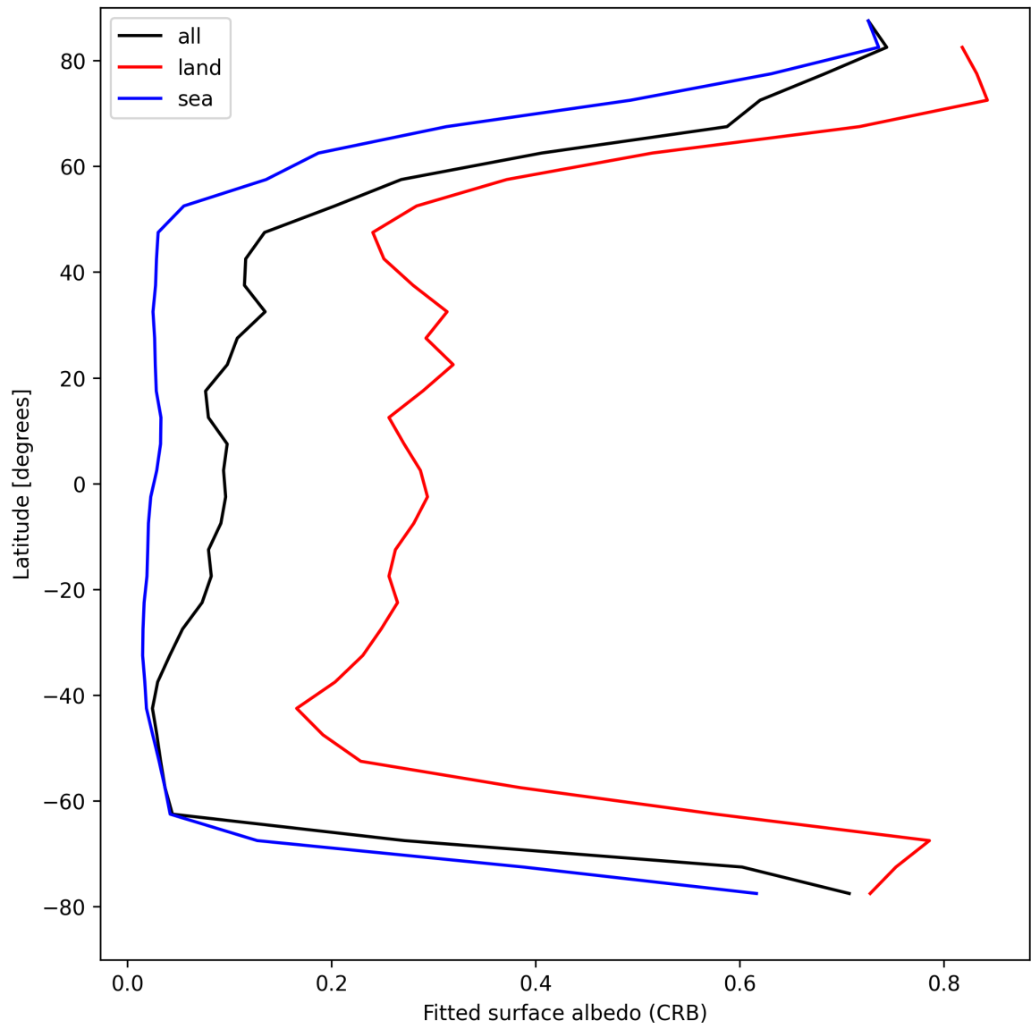
Figure 28: Zonal average of “Fitted surface albedo (CRB)” for 2025-04-14 to 2025-04-15.
