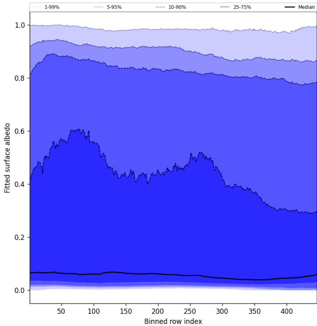
Figure 59: Along track statistics of “Fitted surface albedo” for 2025-04-14 to 2025-04-15
