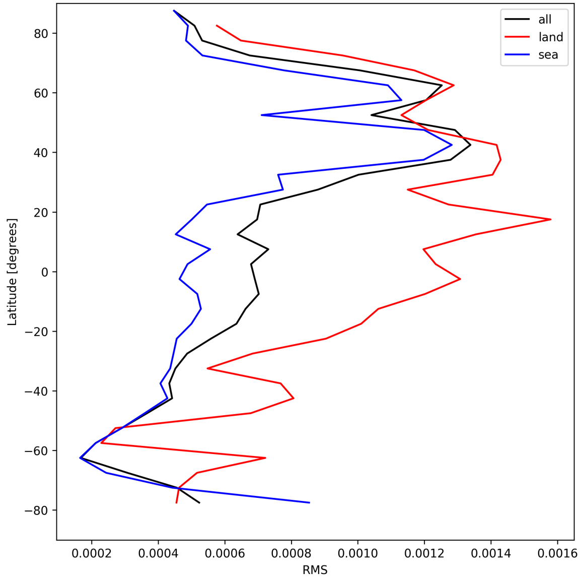
Figure 29: Zonal average of “RMS” for 2025-04-14 to 2025-04-15.
