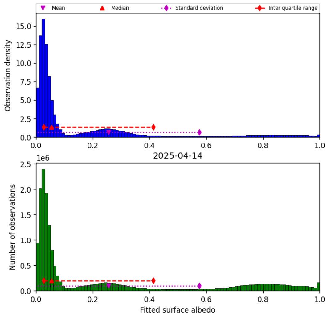
Figure 43: Histogram of “Fitted surface albedo” for 2025-04-14 to 2025-04-15
