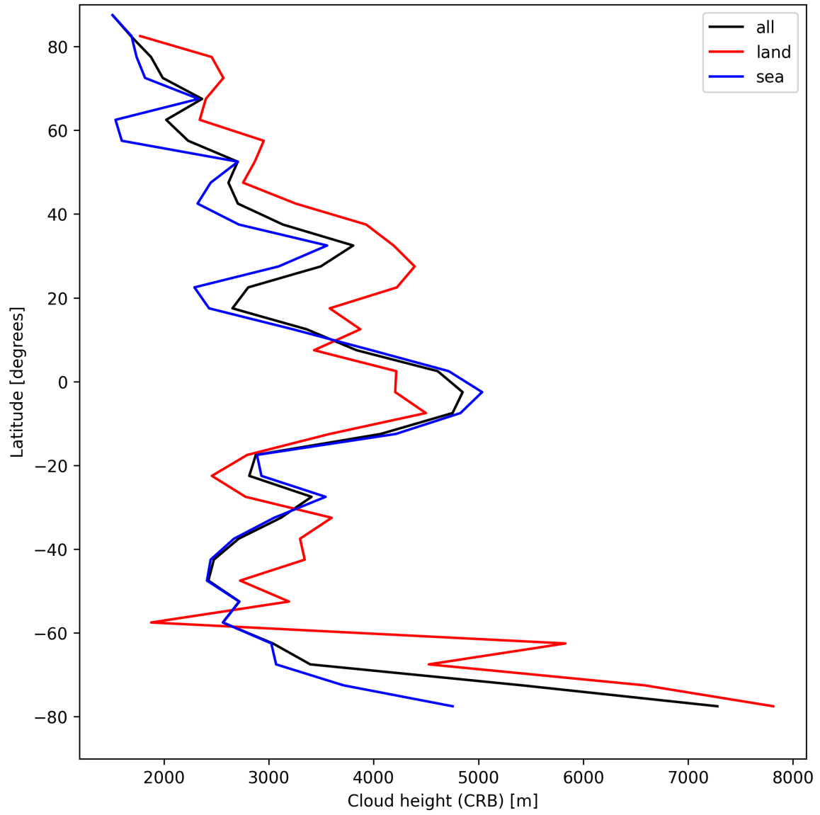
Figure 25: Zonal average of “Cloud height (CRB)” for 2025-04-14 to 2025-04-15.
