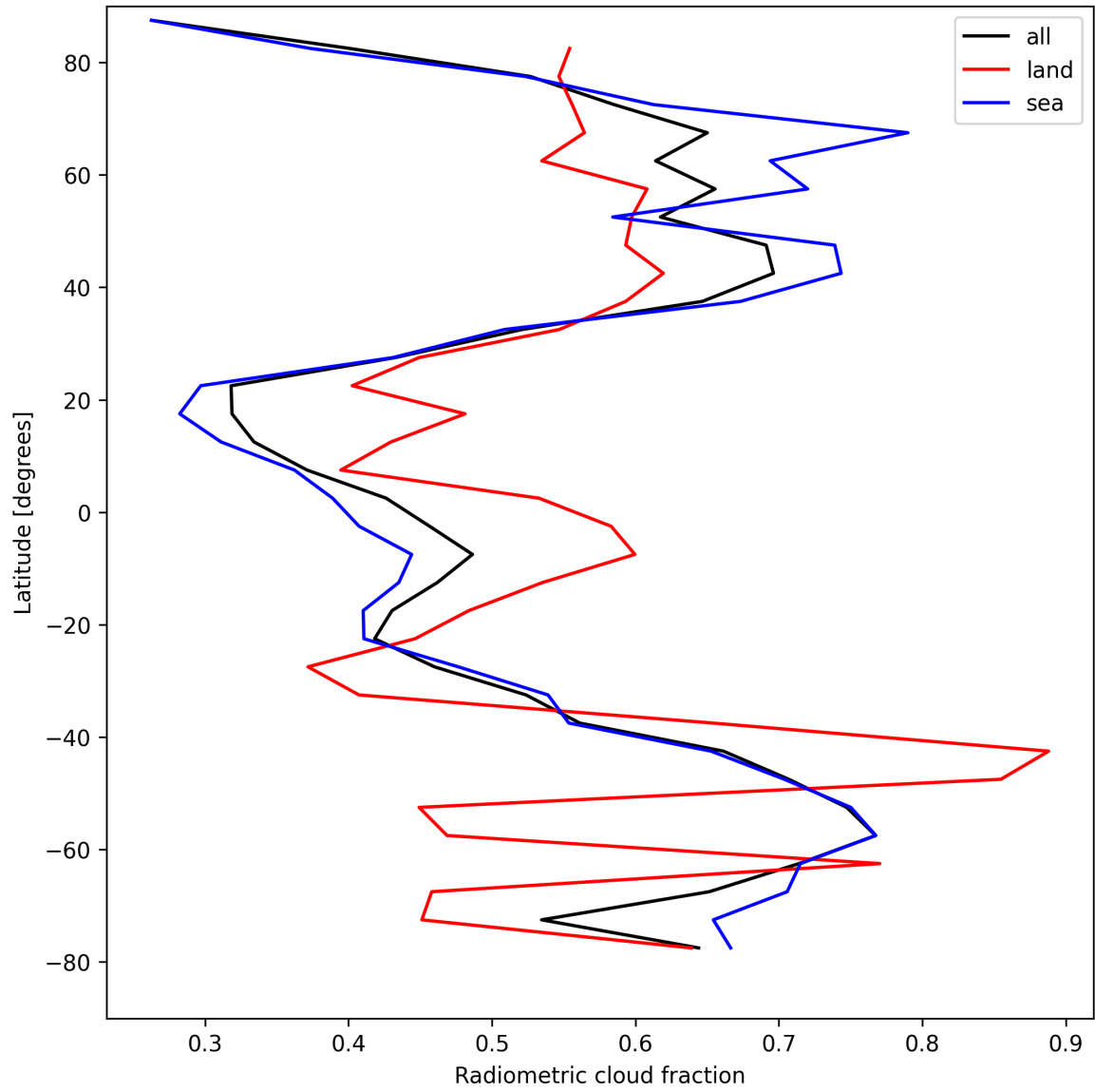
Figure 21: Zonal average of “Radiometric cloud fraction” for 2025-04-14 to 2025-04-15.
