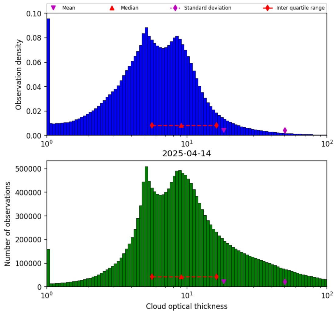
Figure 39: Histogram of “Cloud optical thickness” for 2025-04-14 to 2025-04-15
