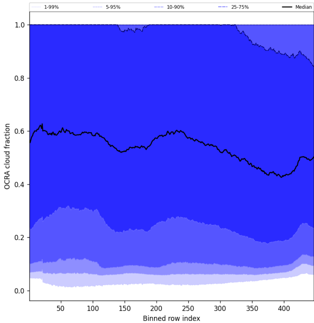
Figure 64: Along track statistics of “OCRA cloud fraction” for 2025-04-14 to 2025-04-15
