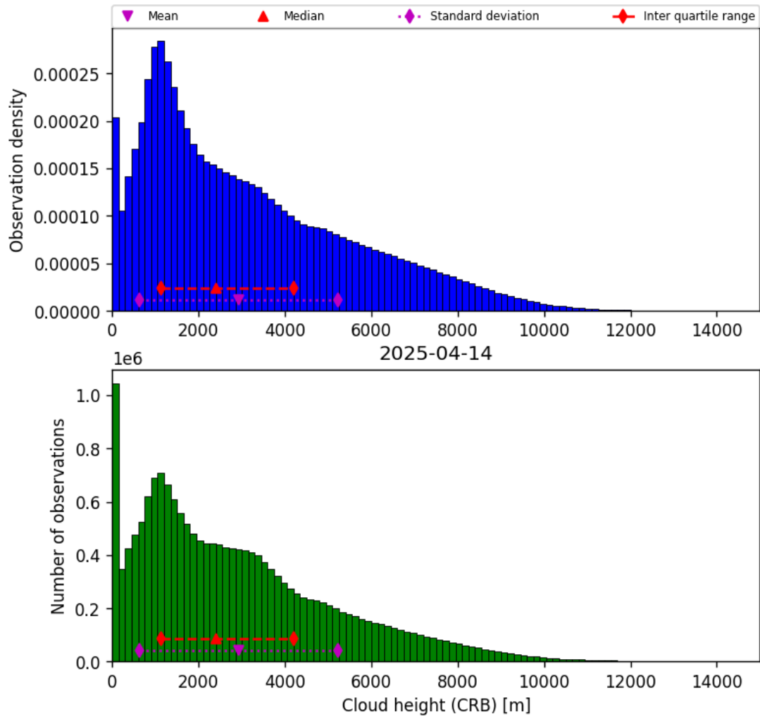
Figure 41: Histogram of “Cloud height (CRB)” for 2025-04-14 to 2025-04-15
