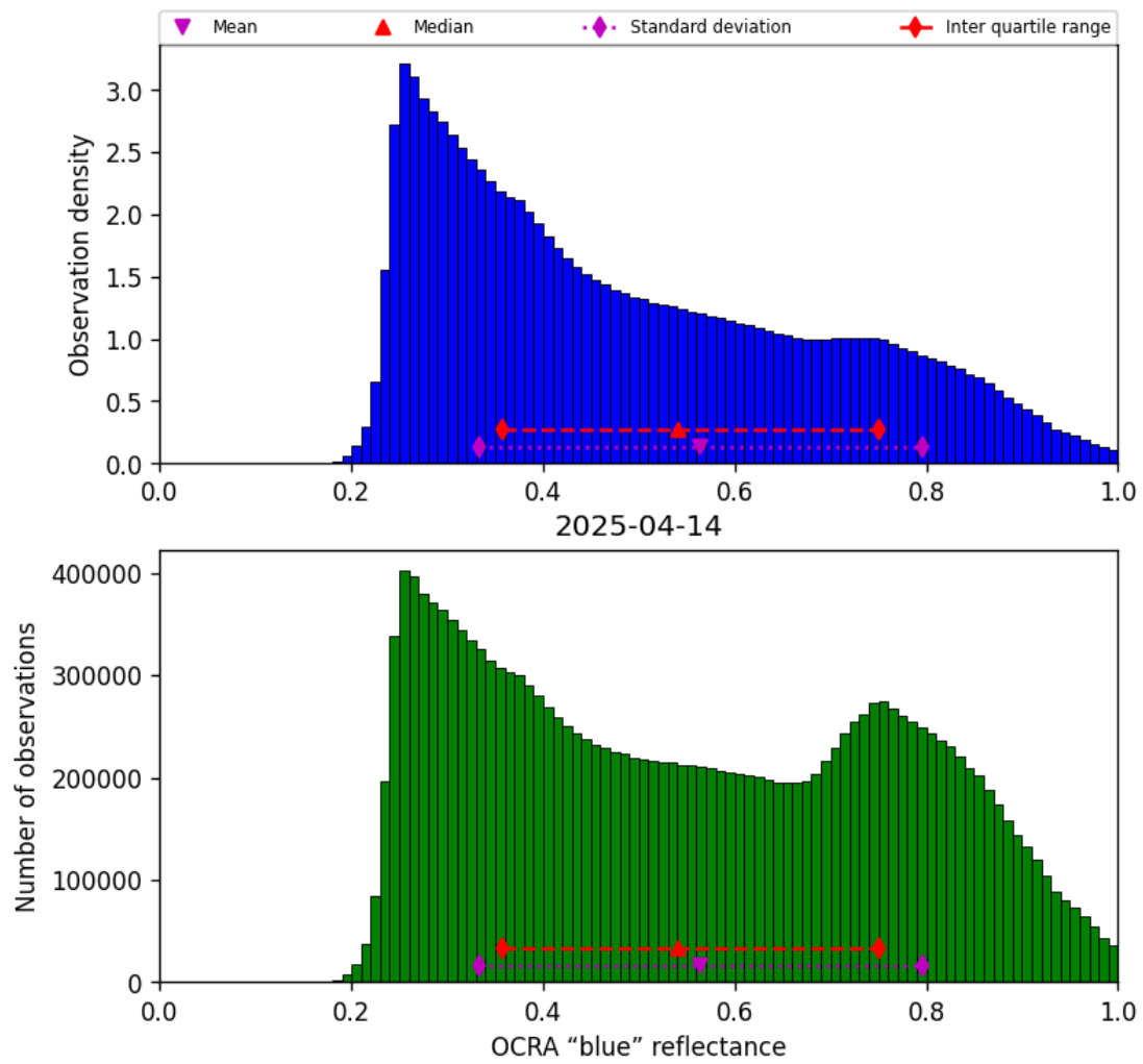
Figure 49: Histogram of “OCRA “blue” reflectance” for 2025-04-14 to 2025-04-15
