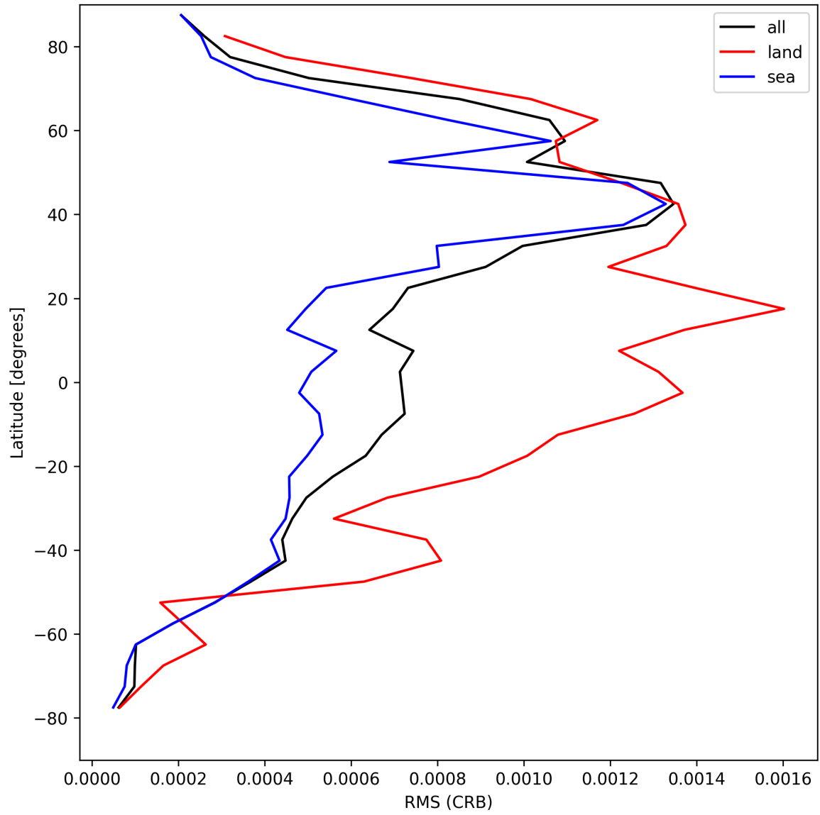
Figure 30: Zonal average of “RMS (CRB)” for 2025-04-14 to 2025-04-15.
