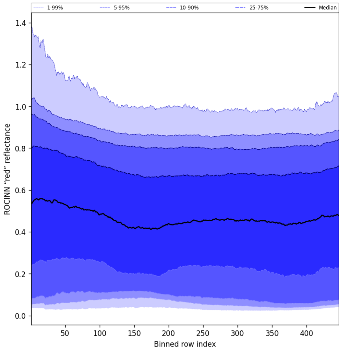
Figure 67: Along track statistics of "ROCINN "red" reflectance" for 2025-04-14 to 2025-04-15
