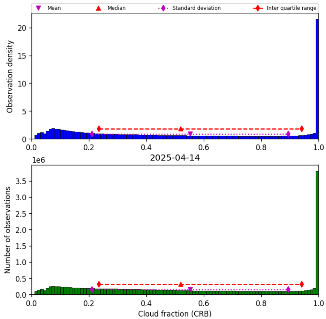
Figure 40: Histogram of “Cloud fraction (CRB)” for 2025-04-14 to 2025-04-15
