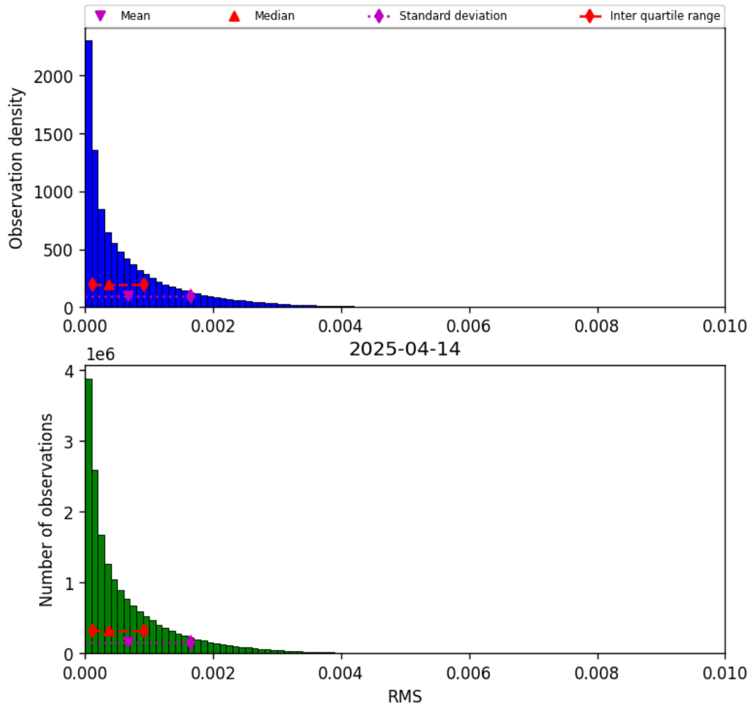
Figure 45: Histogram of “RMS” for 2025-04-14 to 2025-04-15
