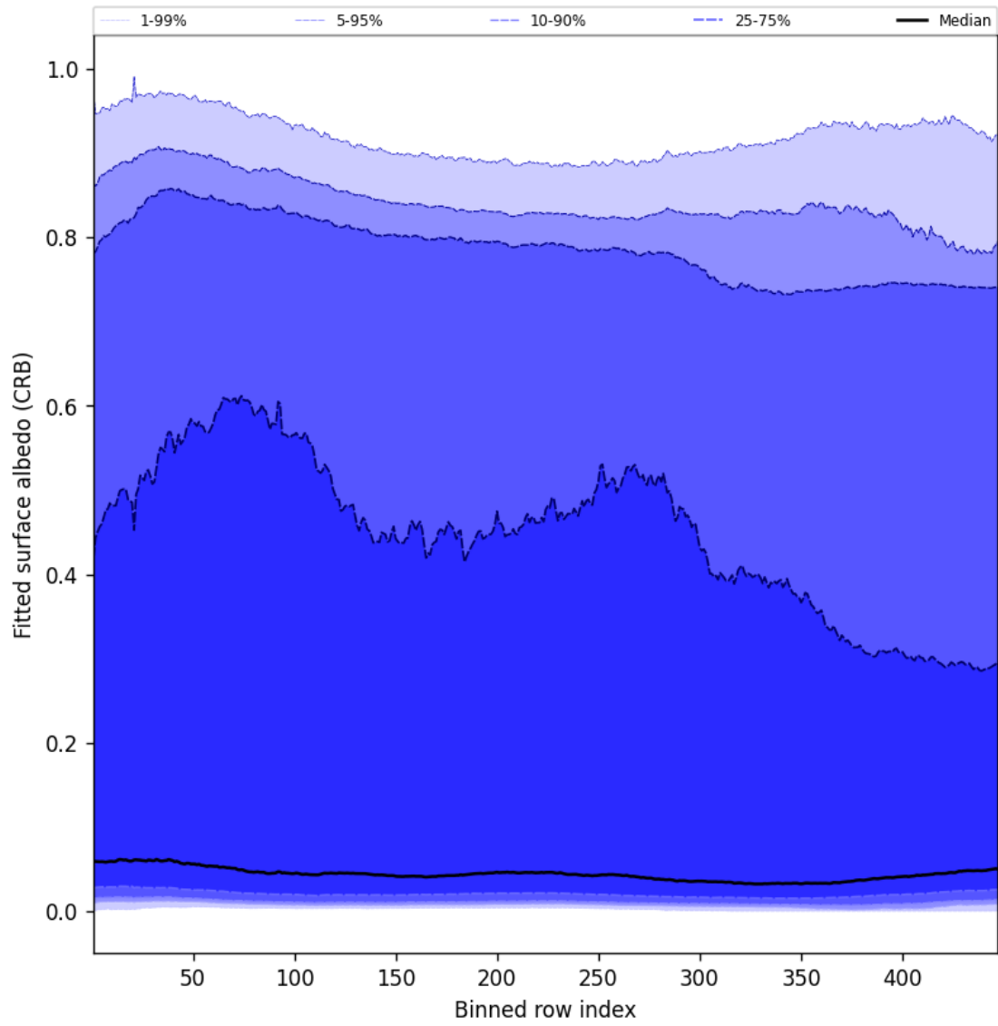
Figure 60: Along track statistics of “Fitted surface albedo (CRB)” for 2025-04-14 to 2025-04-15
