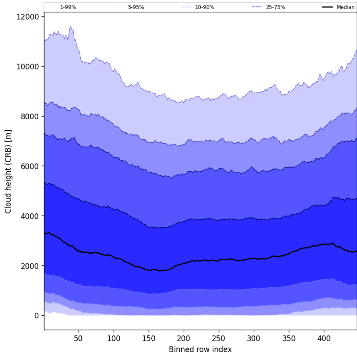
Figure 57: Along track statistics of “Cloud height (CRB)” for 2025-04-14 to 2025-04-15
