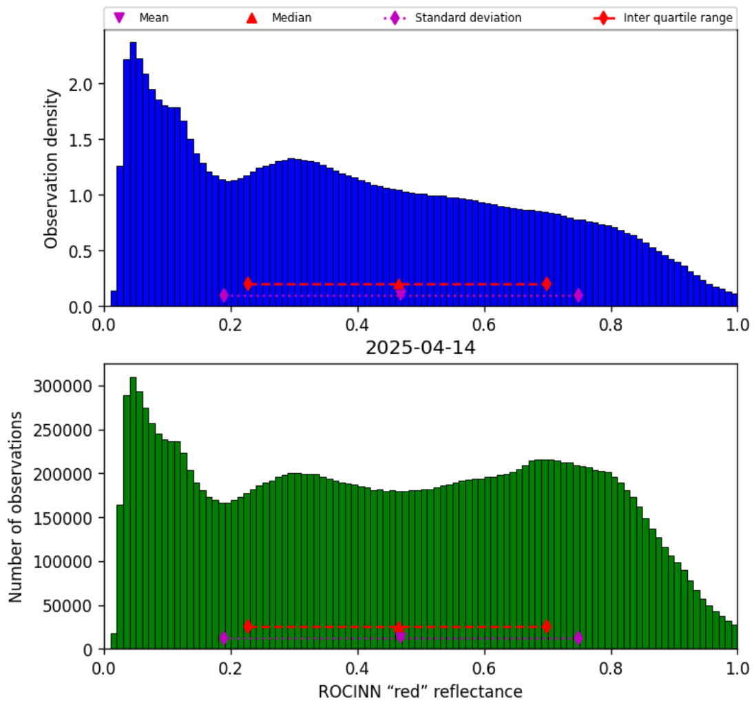
Figure 51: Histogram of “ROCINN “red” reflectance” for 2025-04-14 to 2025-04-15
