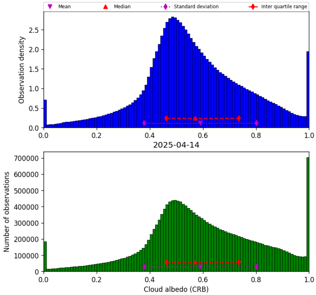
Figure 42: Histogram of “Cloud albedo (CRB)” for 2025-04-14 to 2025-04-15
