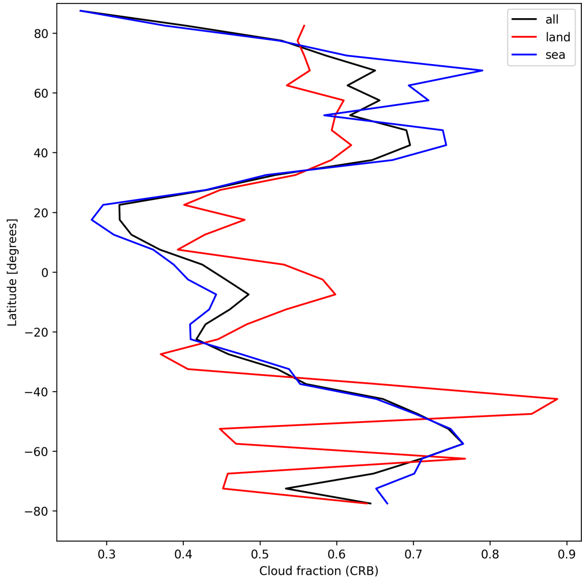
Figure 24: Zonal average of “Cloud fraction (CRB)” for 2025-04-14 to 2025-04-15.
