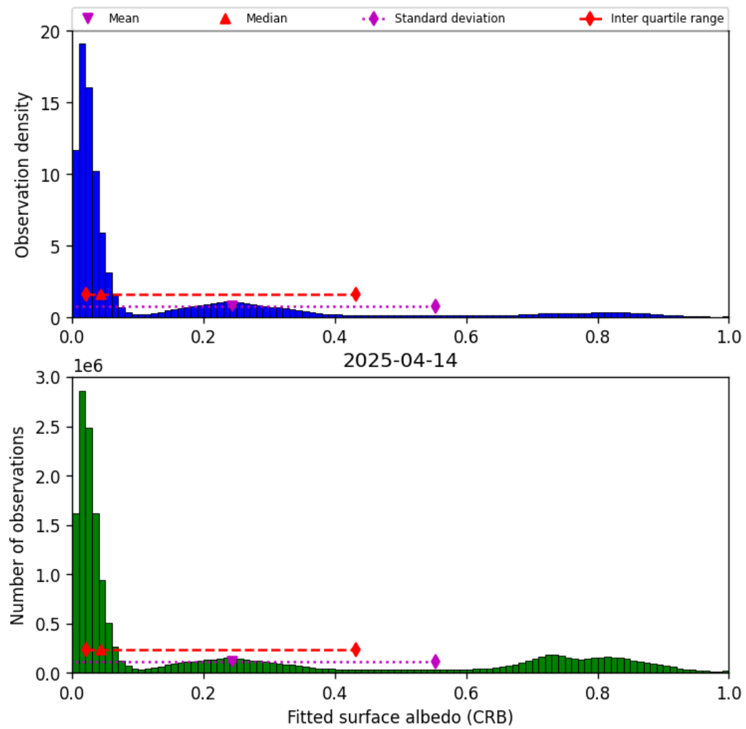
Figure 44: Histogram of “Fitted surface albedo (CRB)” for 2025-04-14 to 2025-04-15
