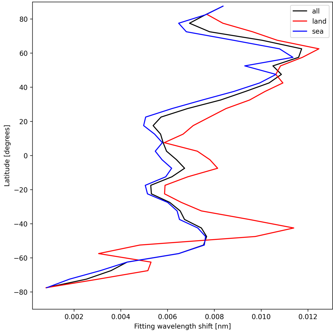
Figure 31: Zonal average of “Fitting wavelength shift” for 2025-04-14 to 2025-04-15.
