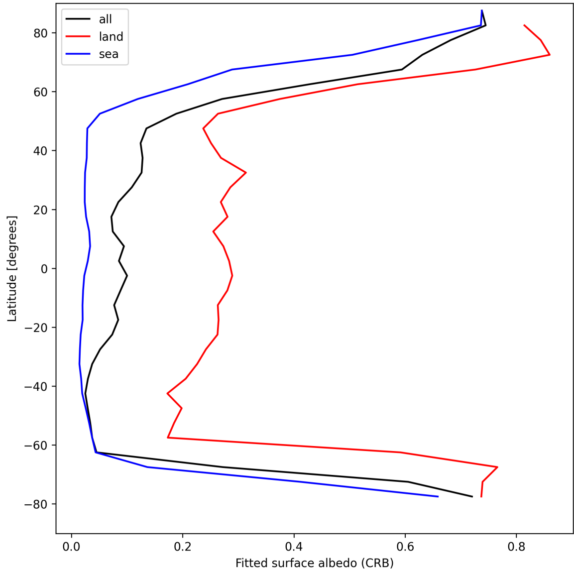
Figure 28: Zonal average of “Fitted surface albedo (CRB)” for 2025-04-16 to 2025-04-16.
