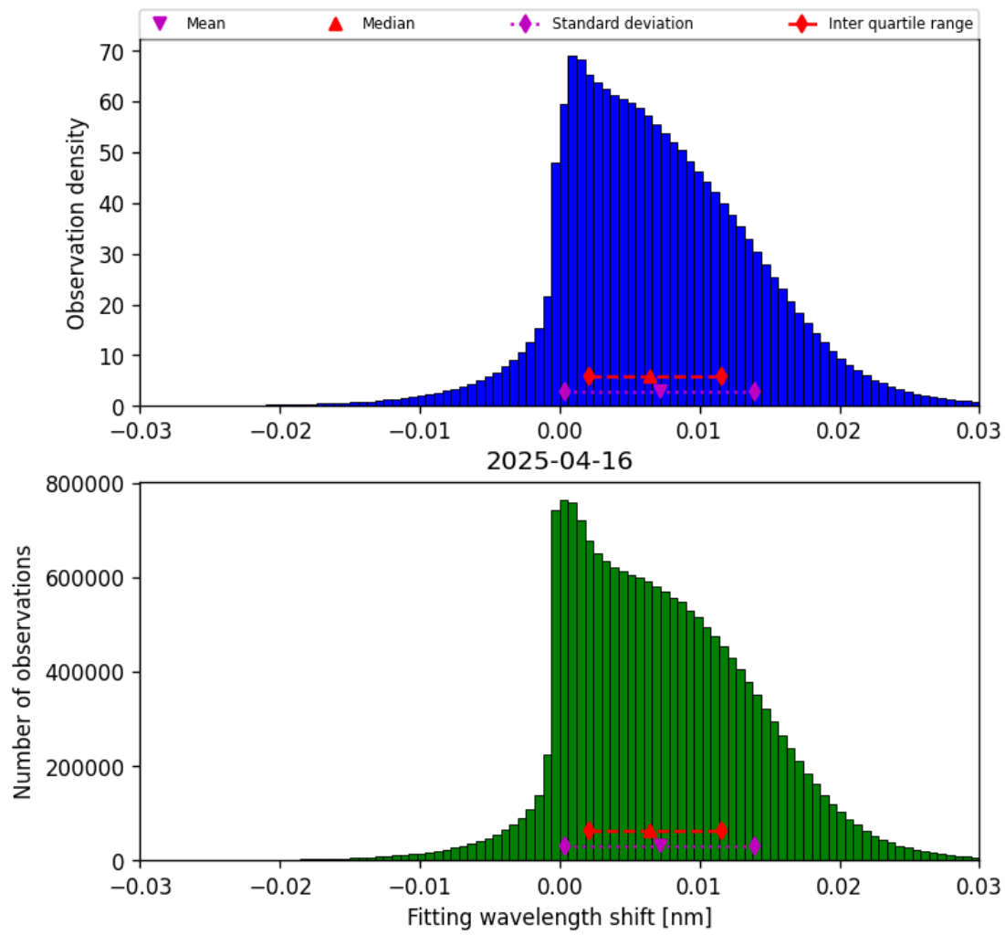
Figure 47: Histogram of “Fitting wavelength shift” for 2025-04-16 to 2025-04-16
