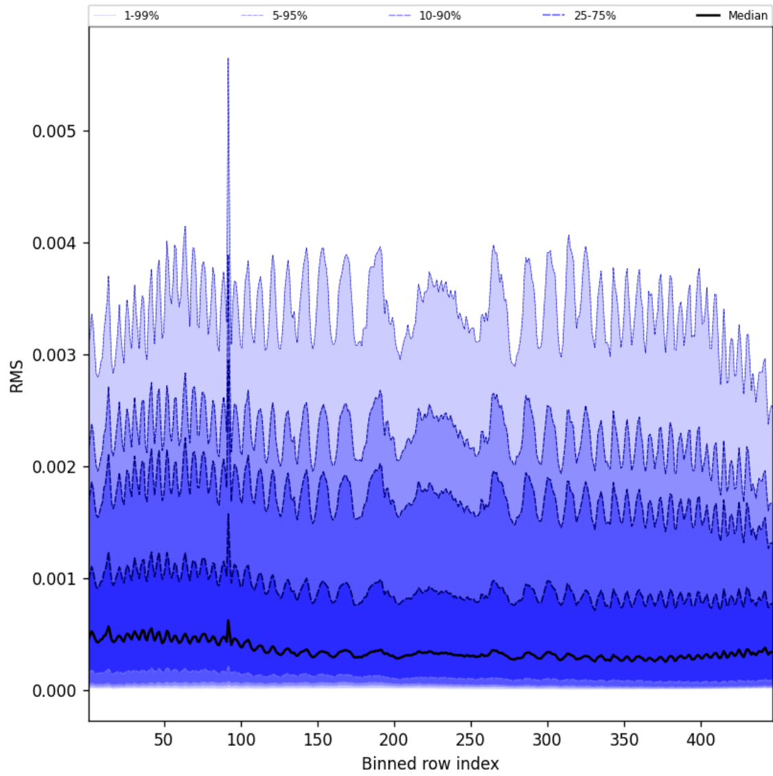
Figure 61: Along track statistics of “RMS” for 2025-04-16 to 2025-04-16
