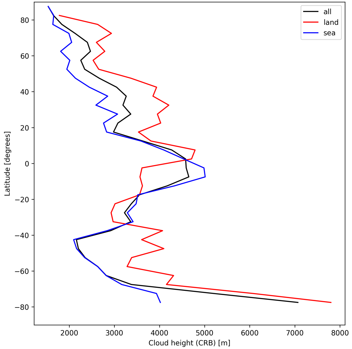
Figure 25: Zonal average of “Cloud height (CRB)” for 2025-04-16 to 2025-04-16.
