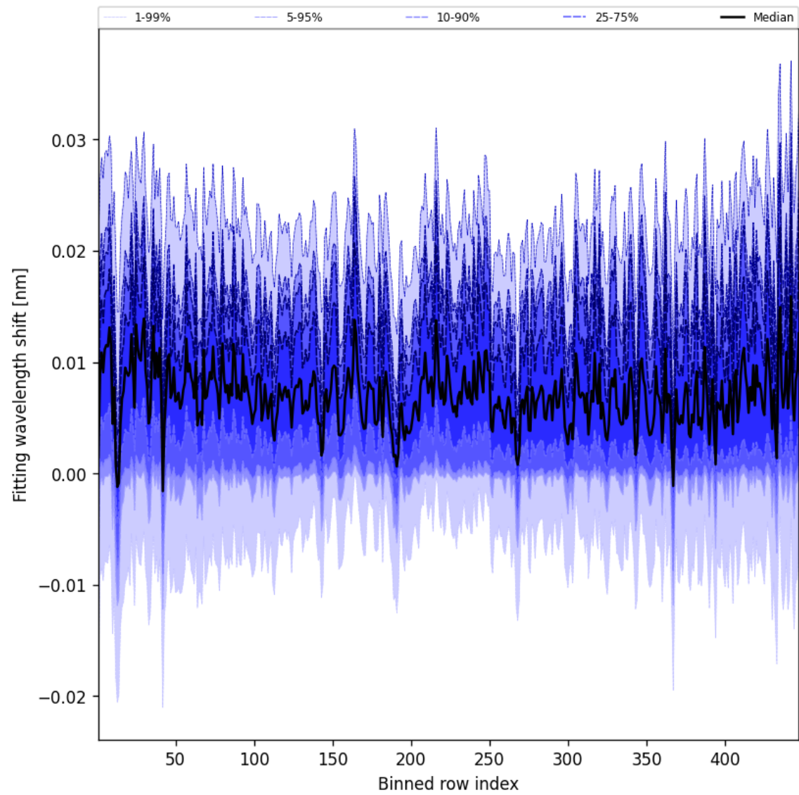
Figure 63: Along track statistics of “Fitting wavelength shift” for 2025-04-16 to 2025-04-16
