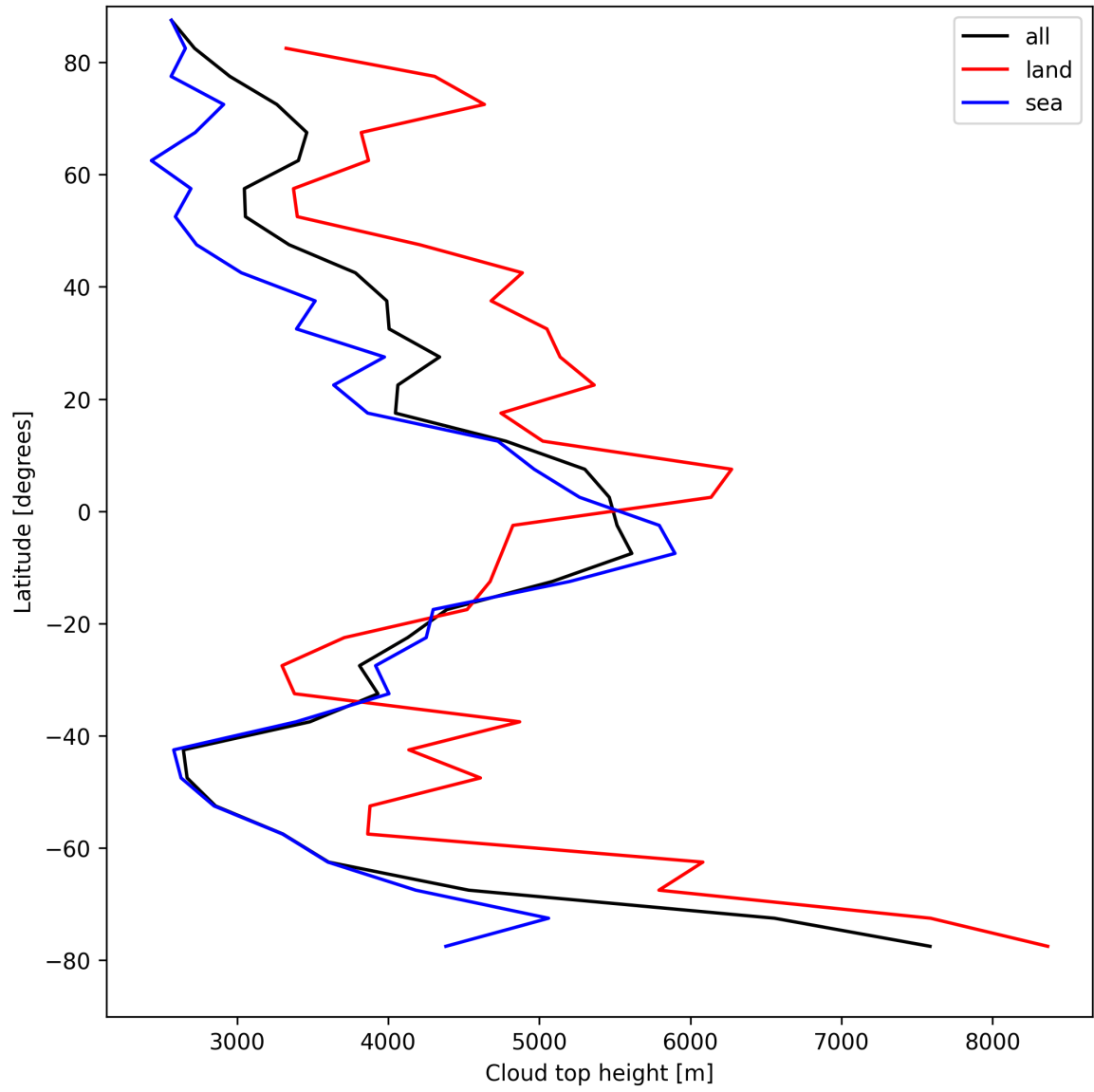
Figure 22: Zonal average of “Cloud top height” for 2025-04-16 to 2025-04-16.
