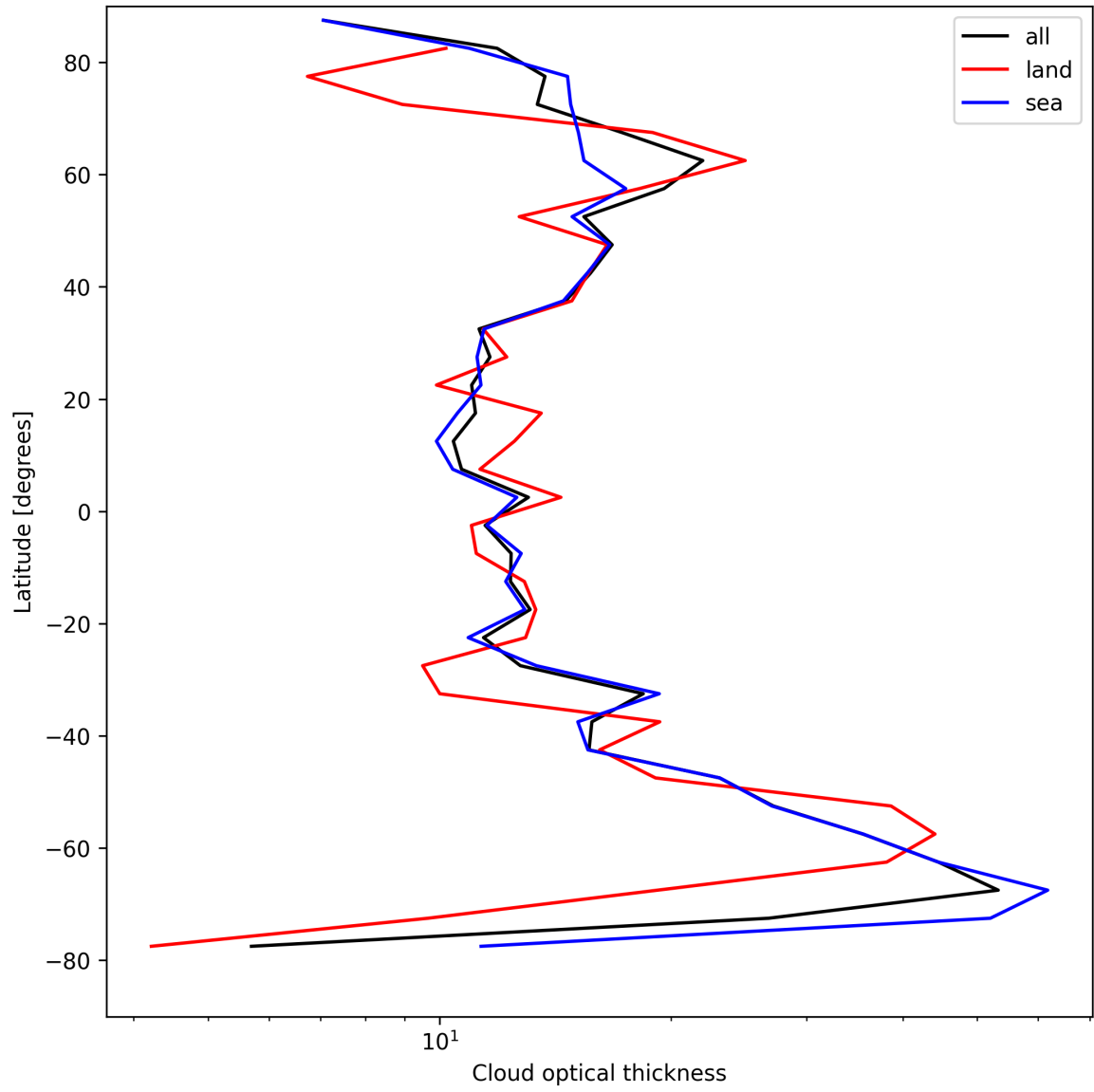
Figure 23: Zonal average of “Cloud optical thickness” for 2025-04-16 to 2025-04-16.
