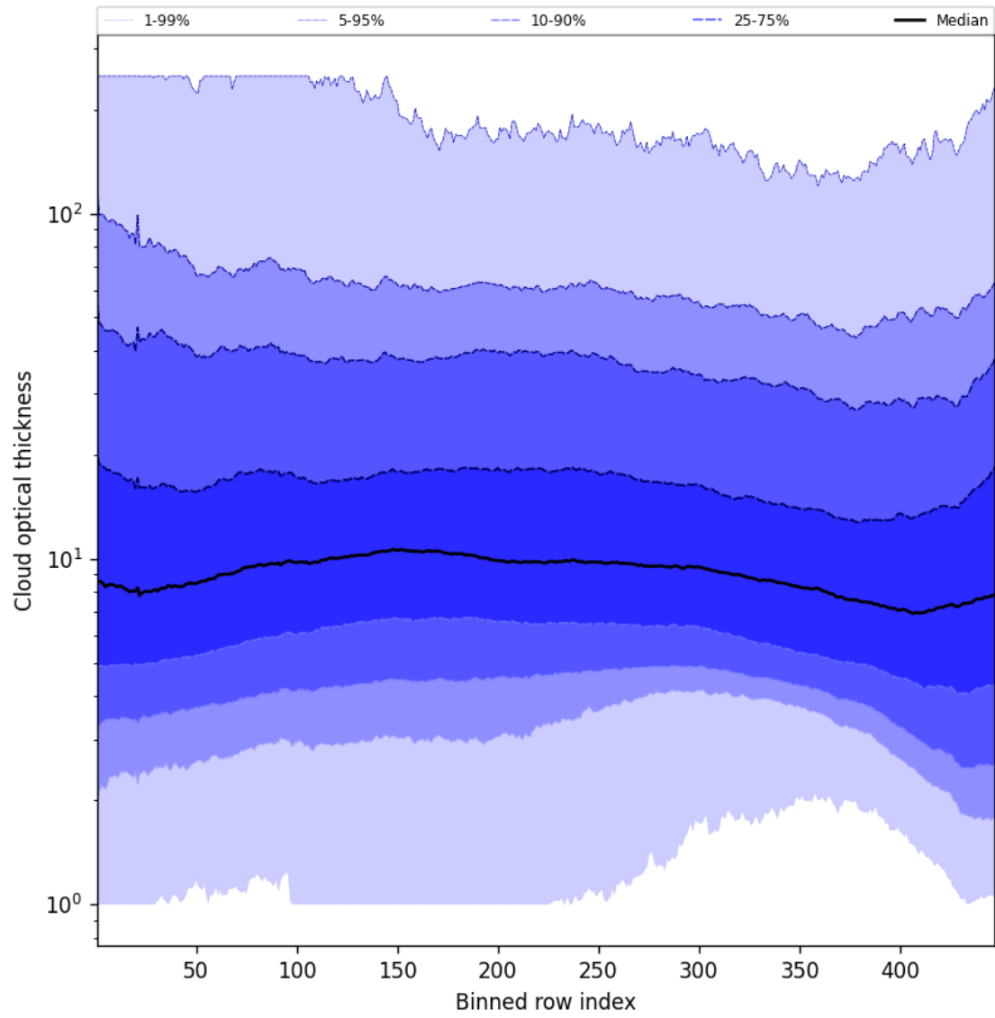
Figure 55: Along track statistics of “Cloud optical thickness” for 2025-04-16 to 2025-04-16
