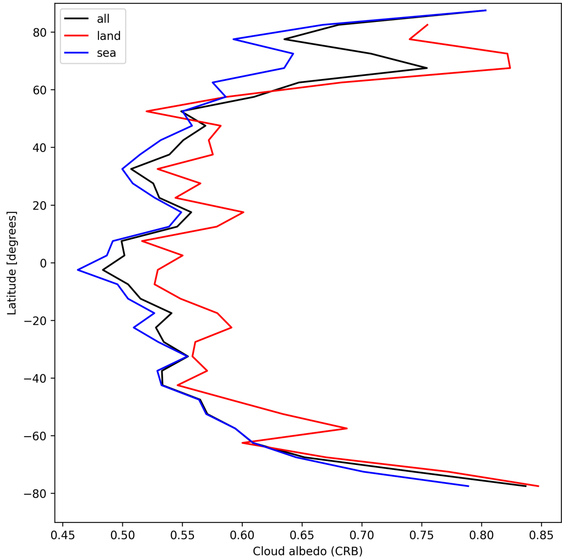
Figure 26: Zonal average of “Cloud albedo (CRB)” for 2025-04-16 to 2025-04-16.
