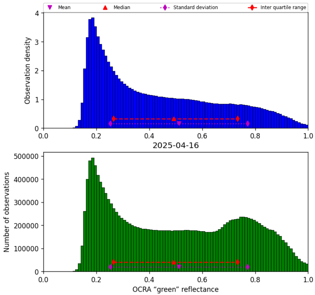
Figure 50: Histogram of “OCRA “green” reflectance” for 2025-04-16 to 2025-04-16
