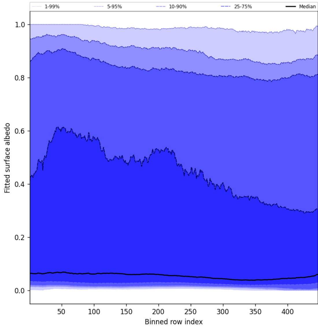
Figure 59: Along track statistics of “Fitted surface albedo” for 2025-04-16 to 2025-04-16
