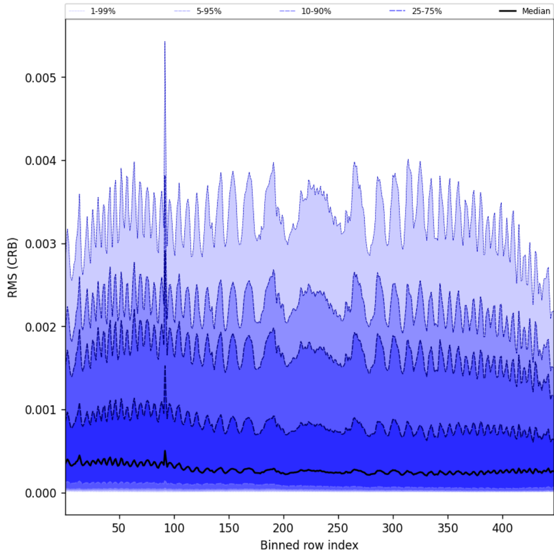
Figure 62: Along track statistics of “RMS (CRB)” for 2025-04-16 to 2025-04-16
