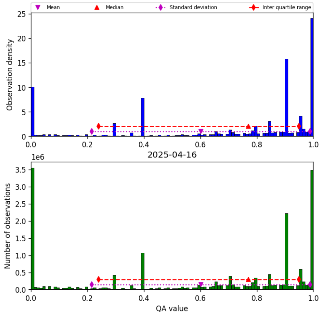
Figure 36: Histogram of “QA value” for 2025-04-16 to 2025-04-16
