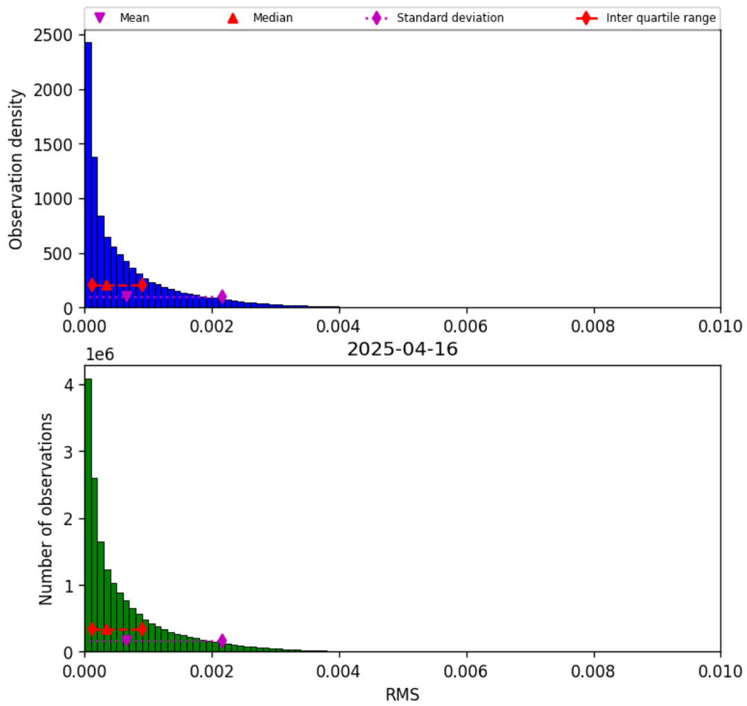
Figure 45: Histogram of “RMS” for 2025-04-16 to 2025-04-16
