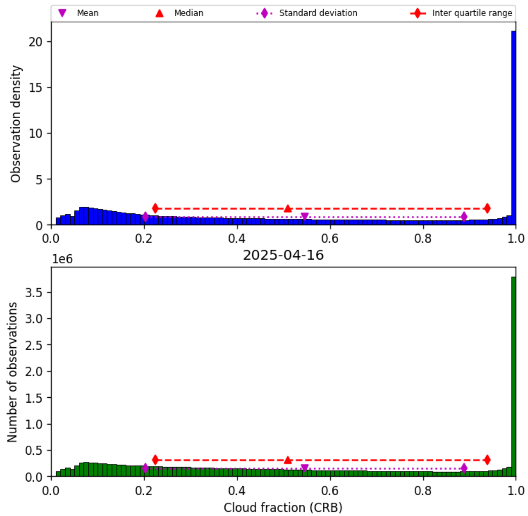
Figure 40: Histogram of “Cloud fraction (CRB)” for 2025-04-16 to 2025-04-16
