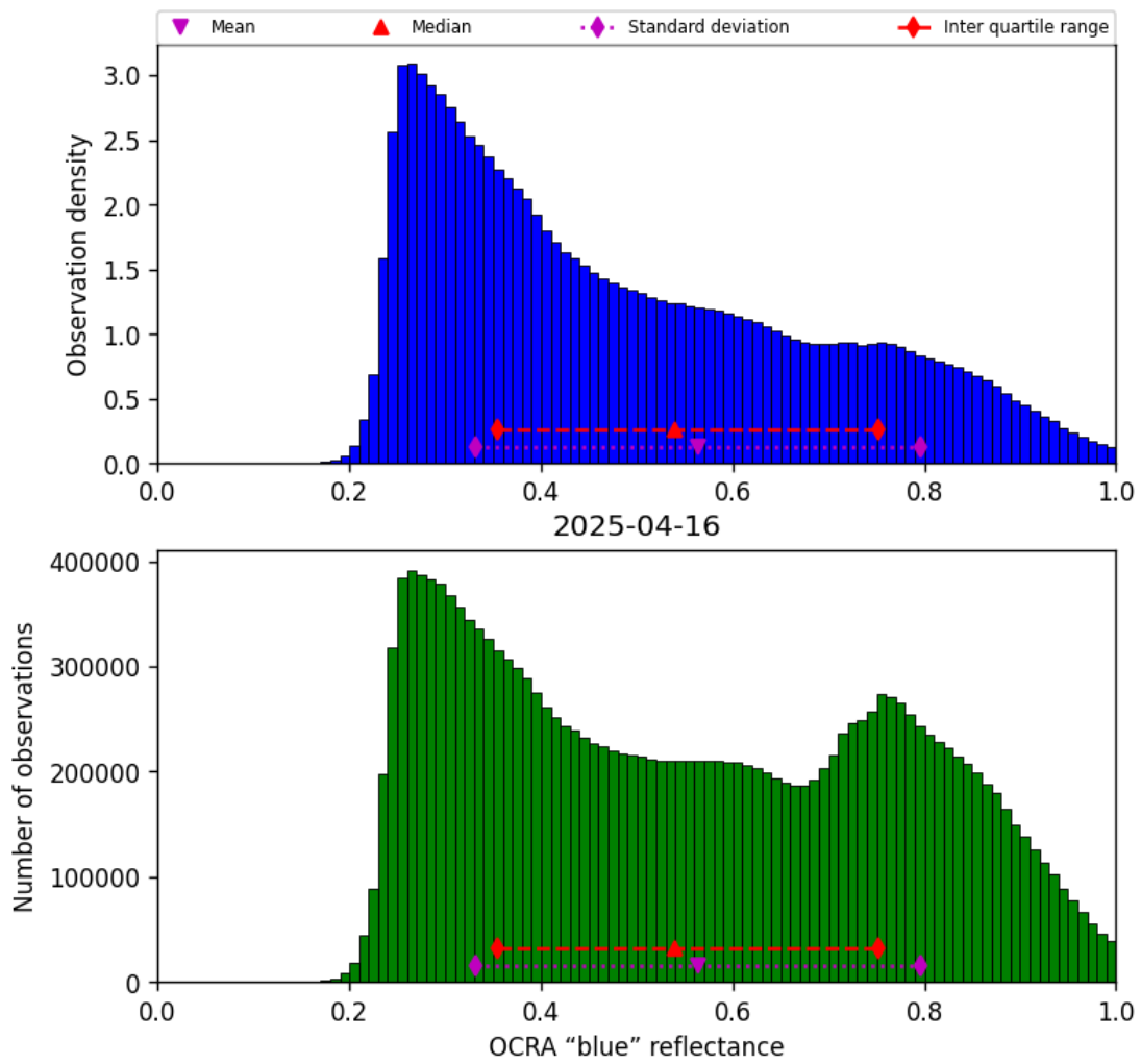
Figure 49: Histogram of “OCRA “blue” reflectance” for 2025-04-16 to 2025-04-16
