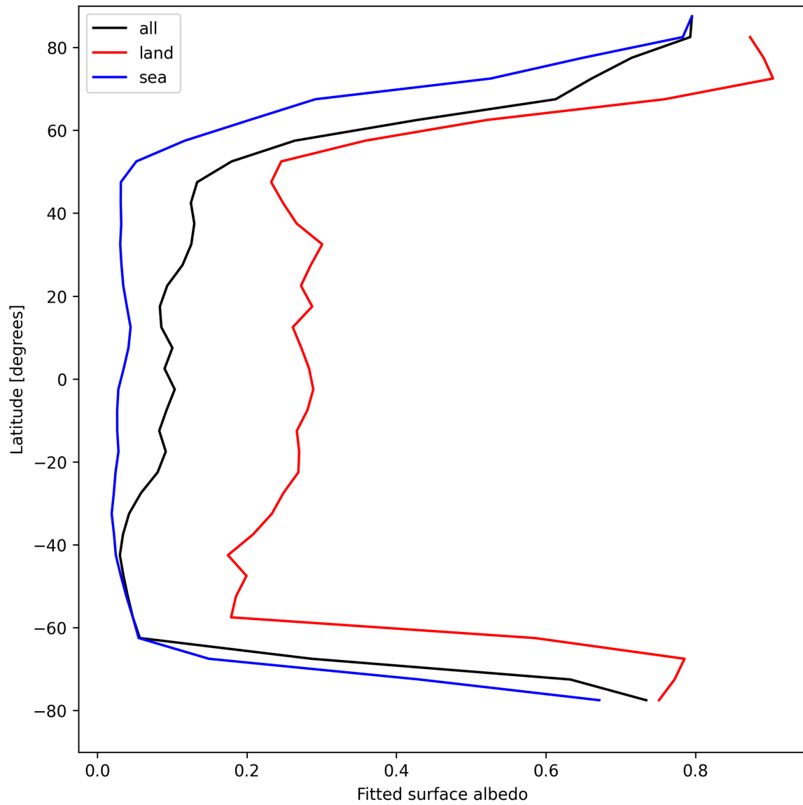
Figure 27: Zonal average of “Fitted surface albedo” for 2025-04-16 to 2025-04-16.
