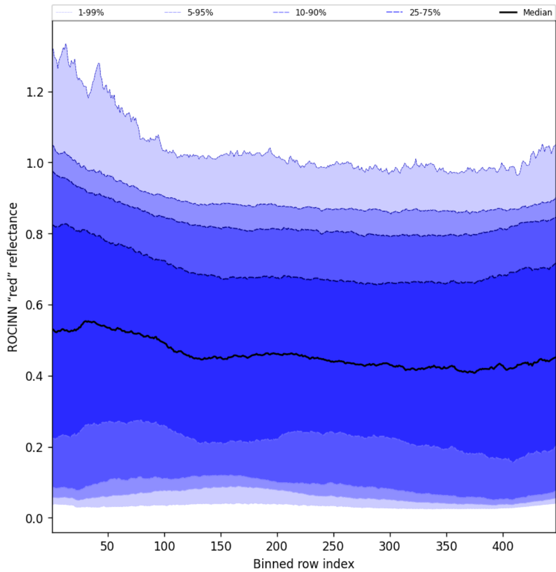
Figure 67: Along track statistics of "ROCINN "red" reflectance" for 2025-04-16 to 2025-04-16
