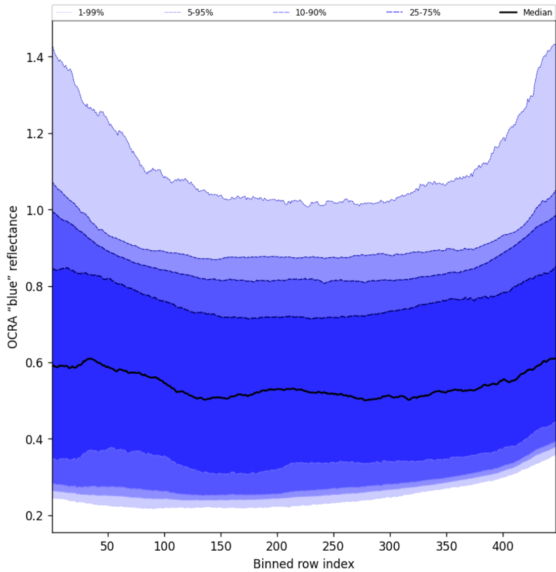
Figure 65: Along track statistics of “OCRA “blue” reflectance” for 2025-04-16 to 2025-04-16
