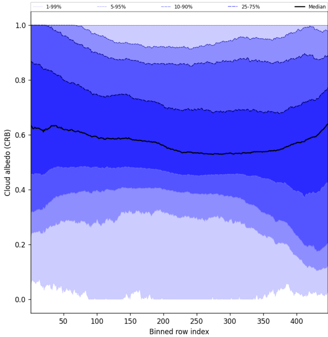
Figure 58: Along track statistics of “Cloud albedo (CRB)” for 2025-04-16 to 2025-04-16
