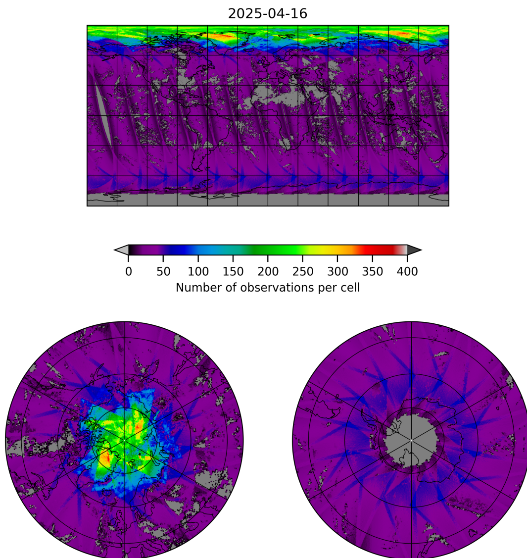
Figure 19: Map of the number of observations for 2025-04-16 to 2025-04-16
