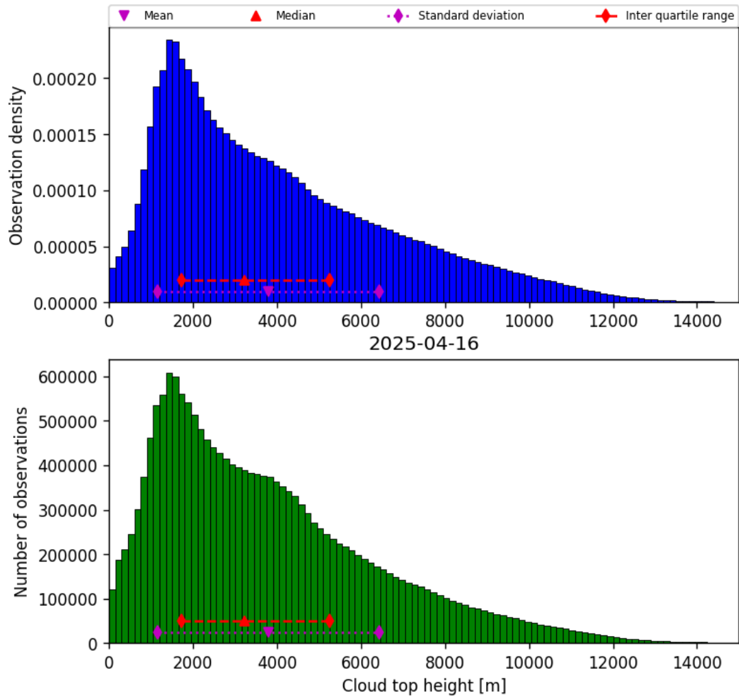
Figure 38: Histogram of “Cloud top height” for 2025-04-16 to 2025-04-16
