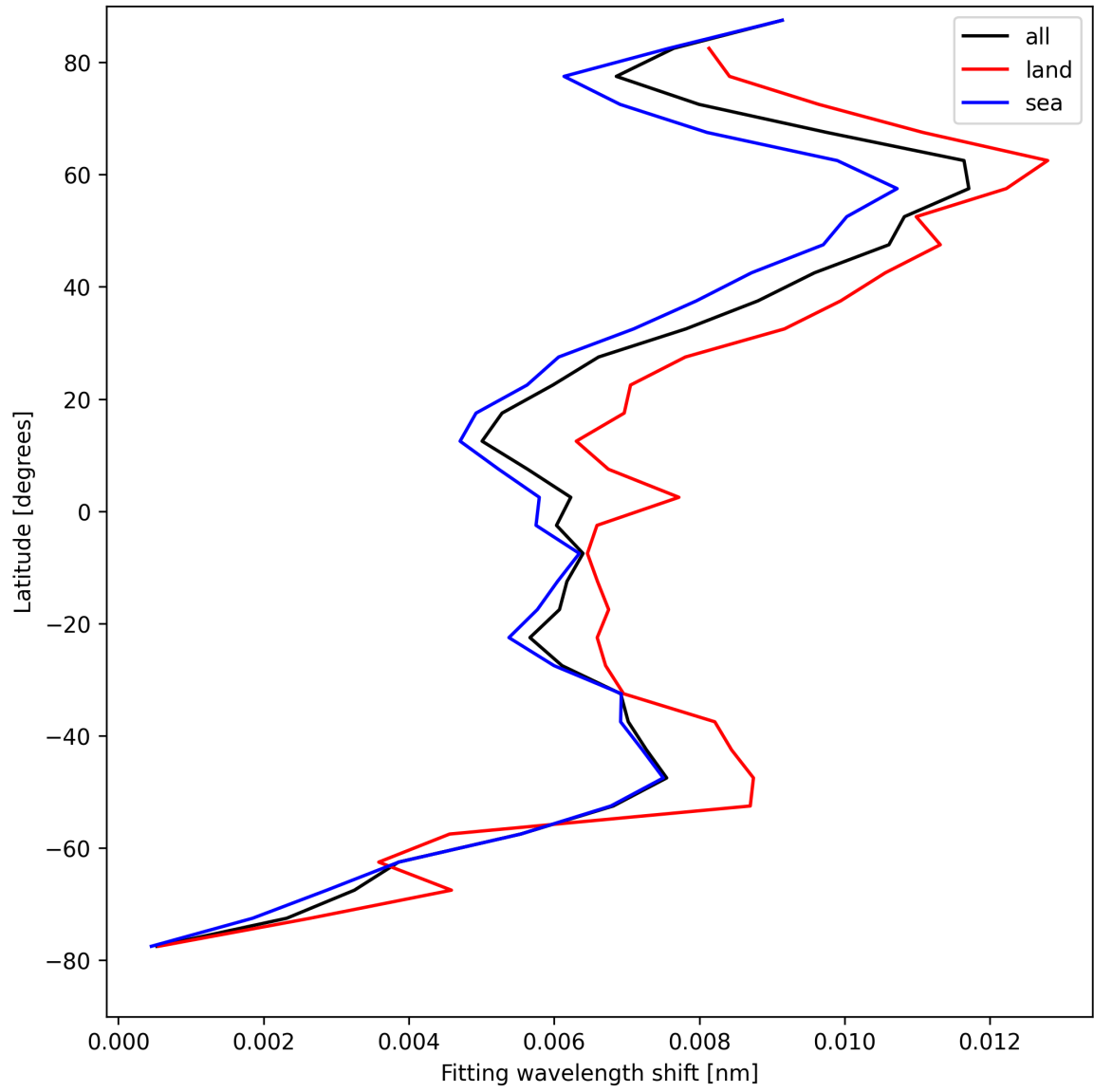
Figure 31: Zonal average of “Fitting wavelength shift” for 2025-04-16 to 2025-04-16.
