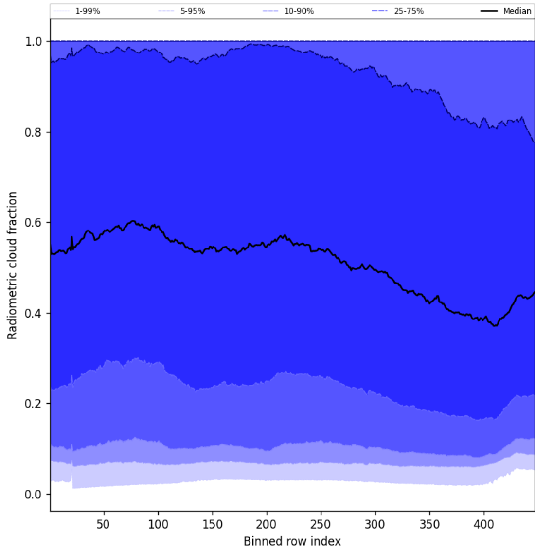
Figure 53: Along track statistics of “Radiometric cloud fraction” for 2025-04-16 to 2025-04-16
