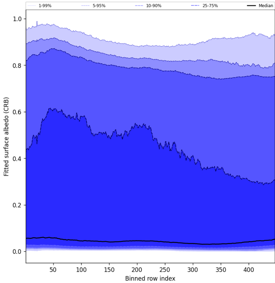
Figure 60: Along track statistics of “Fitted surface albedo (CRB)” for 2025-04-16 to 2025-04-16
