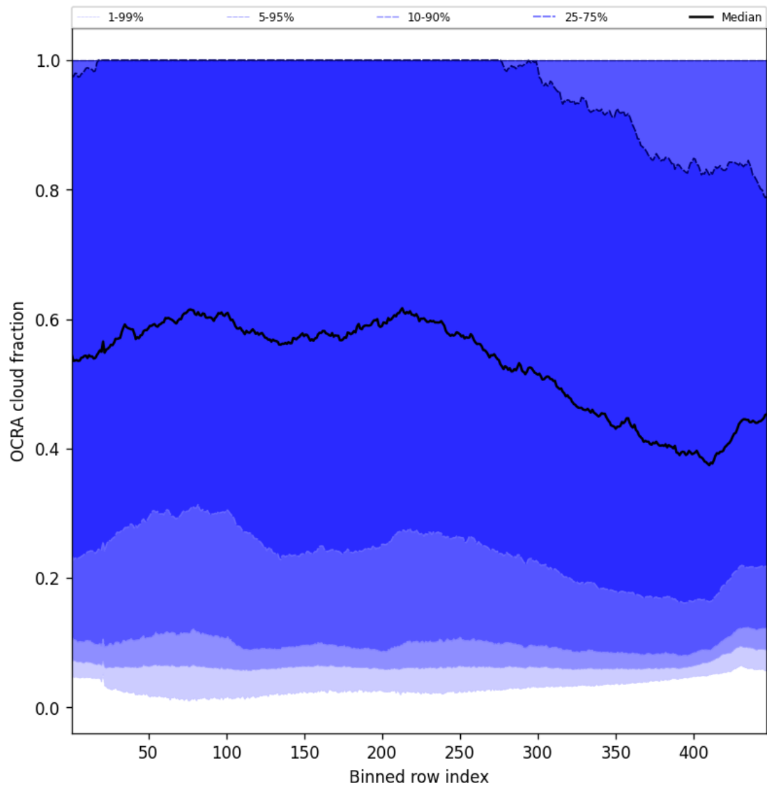
Figure 64: Along track statistics of “OCRA cloud fraction” for 2025-04-16 to 2025-04-16
