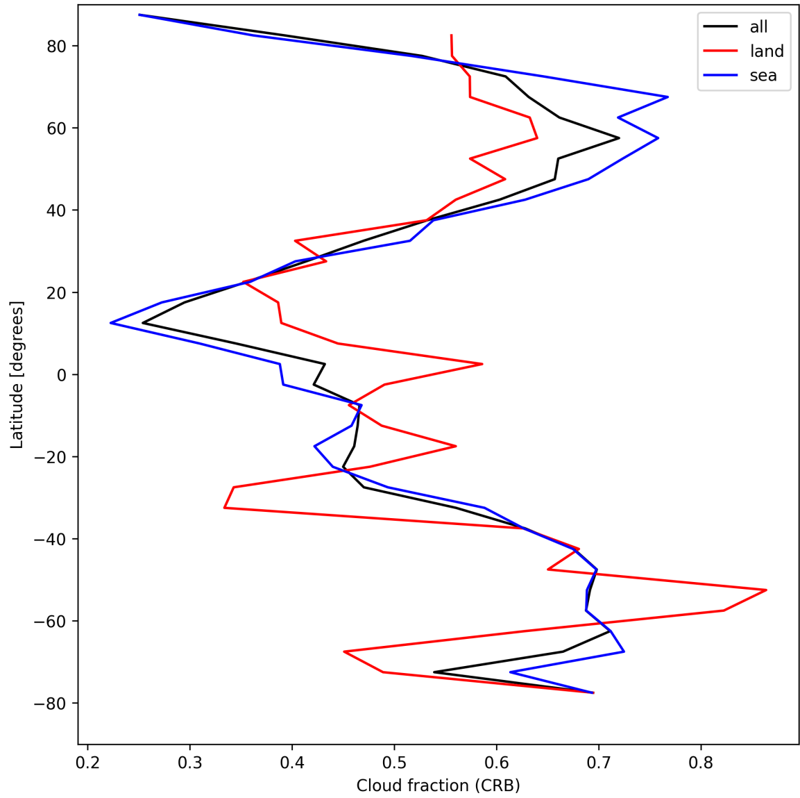
Figure 24: Zonal average of “Cloud fraction (CRB)” for 2025-04-16 to 2025-04-16.
