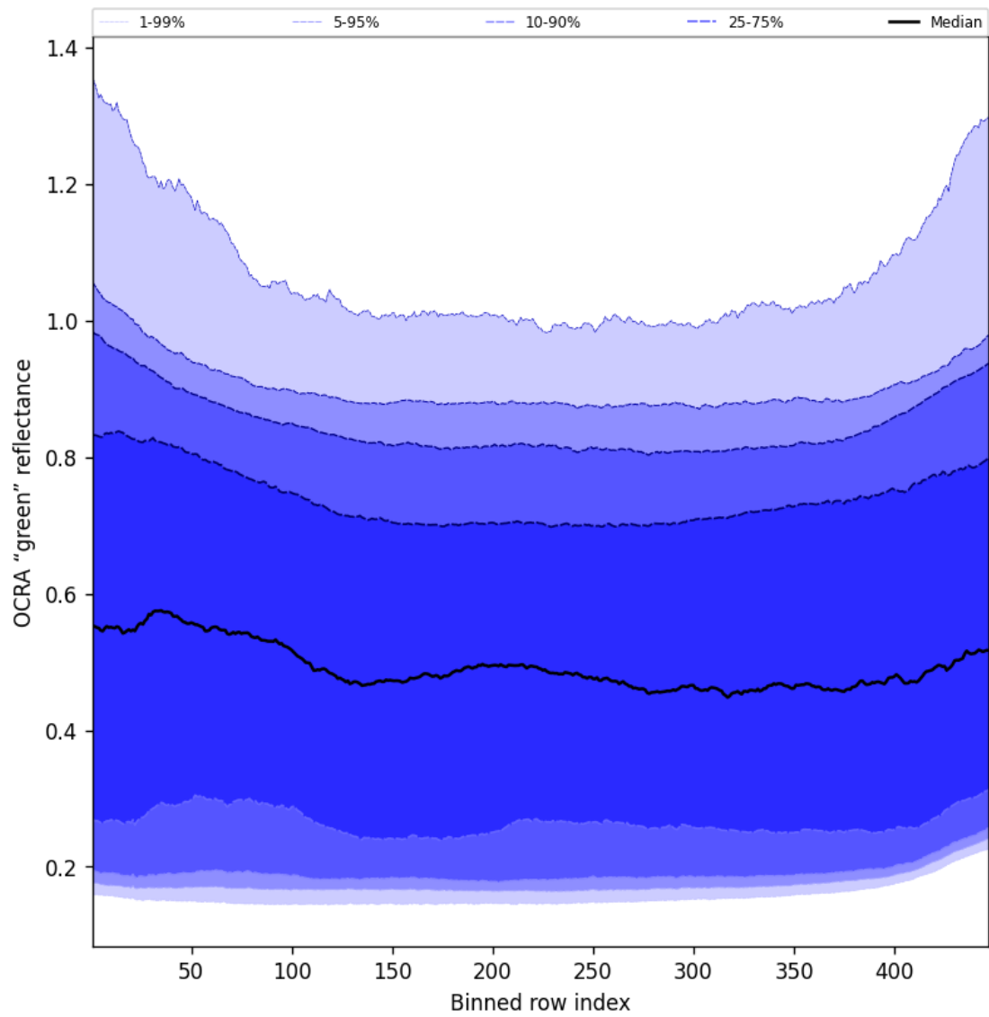
Figure 66: Along track statistics of "OCRA "green" reflectance" for 2025-04-16 to 2025-04-16
