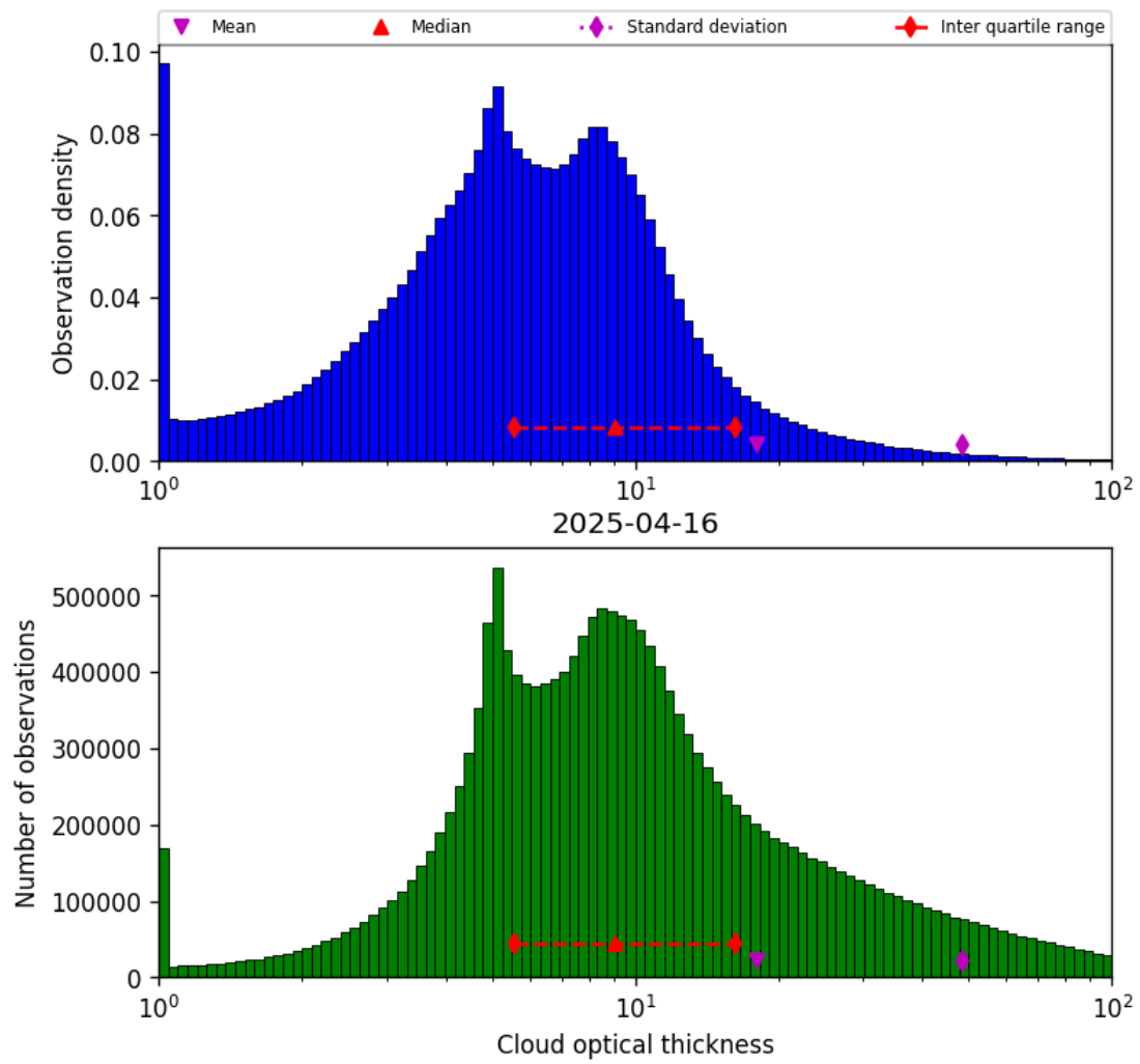
Figure 39: Histogram of “Cloud optical thickness” for 2025-04-16 to 2025-04-16
