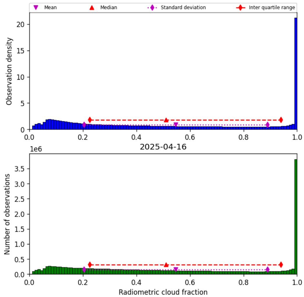
Figure 37: Histogram of “Radiometric cloud fraction” for 2025-04-16 to 2025-04-16
