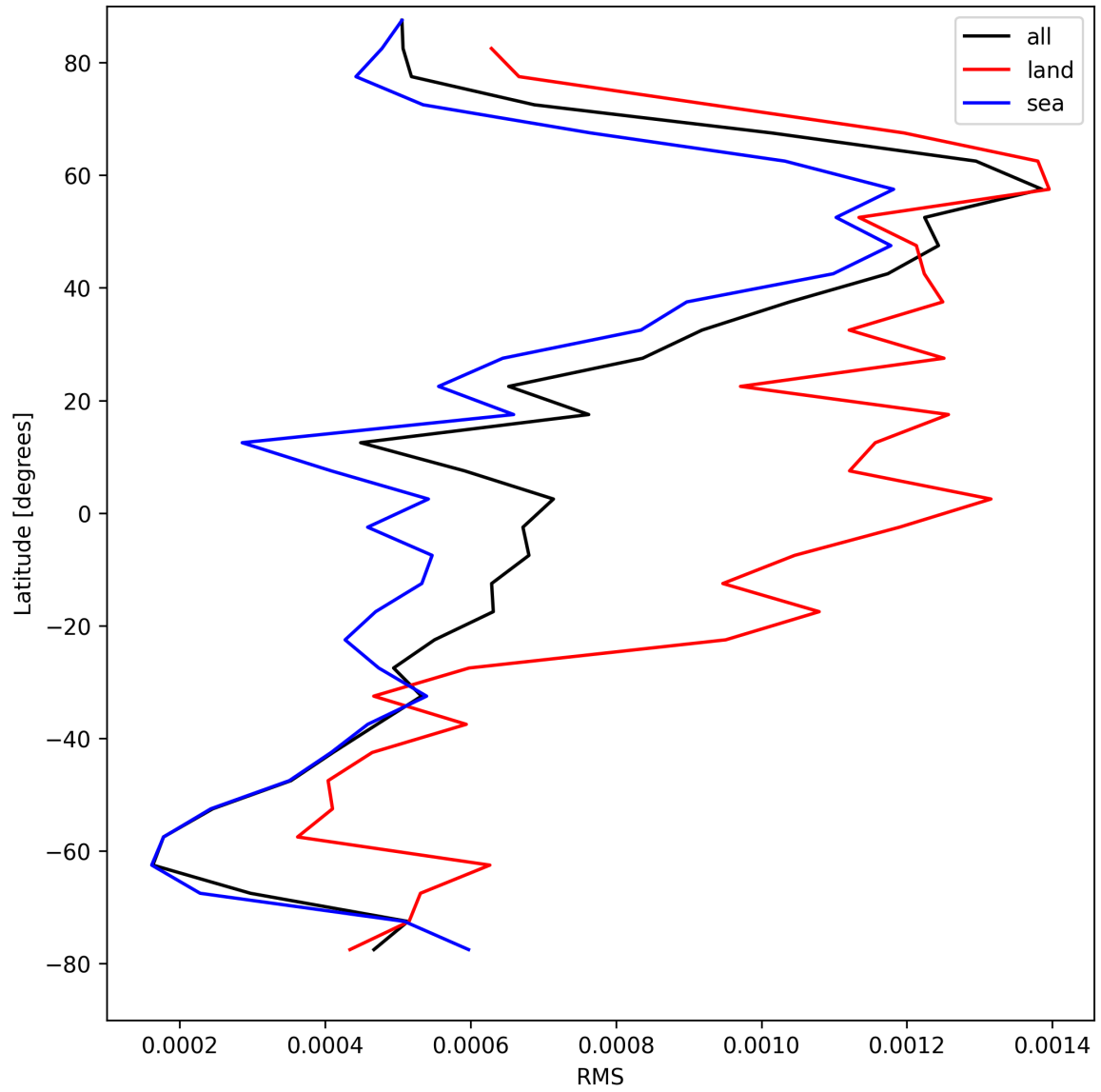
Figure 29: Zonal average of “RMS” for 2025-04-16 to 2025-04-16.
