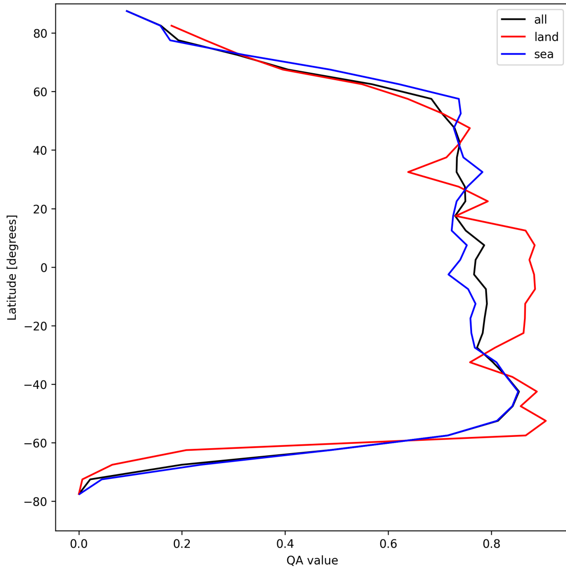
Figure 20: Zonal average of “QA value” for 2025-04-16 to 2025-04-16.
