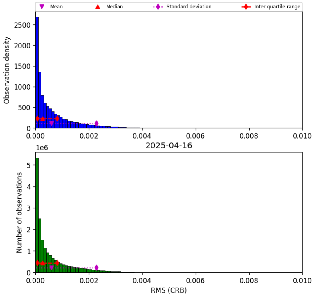
Figure 46: Histogram of “RMS (CRB)” for 2025-04-16 to 2025-04-16
