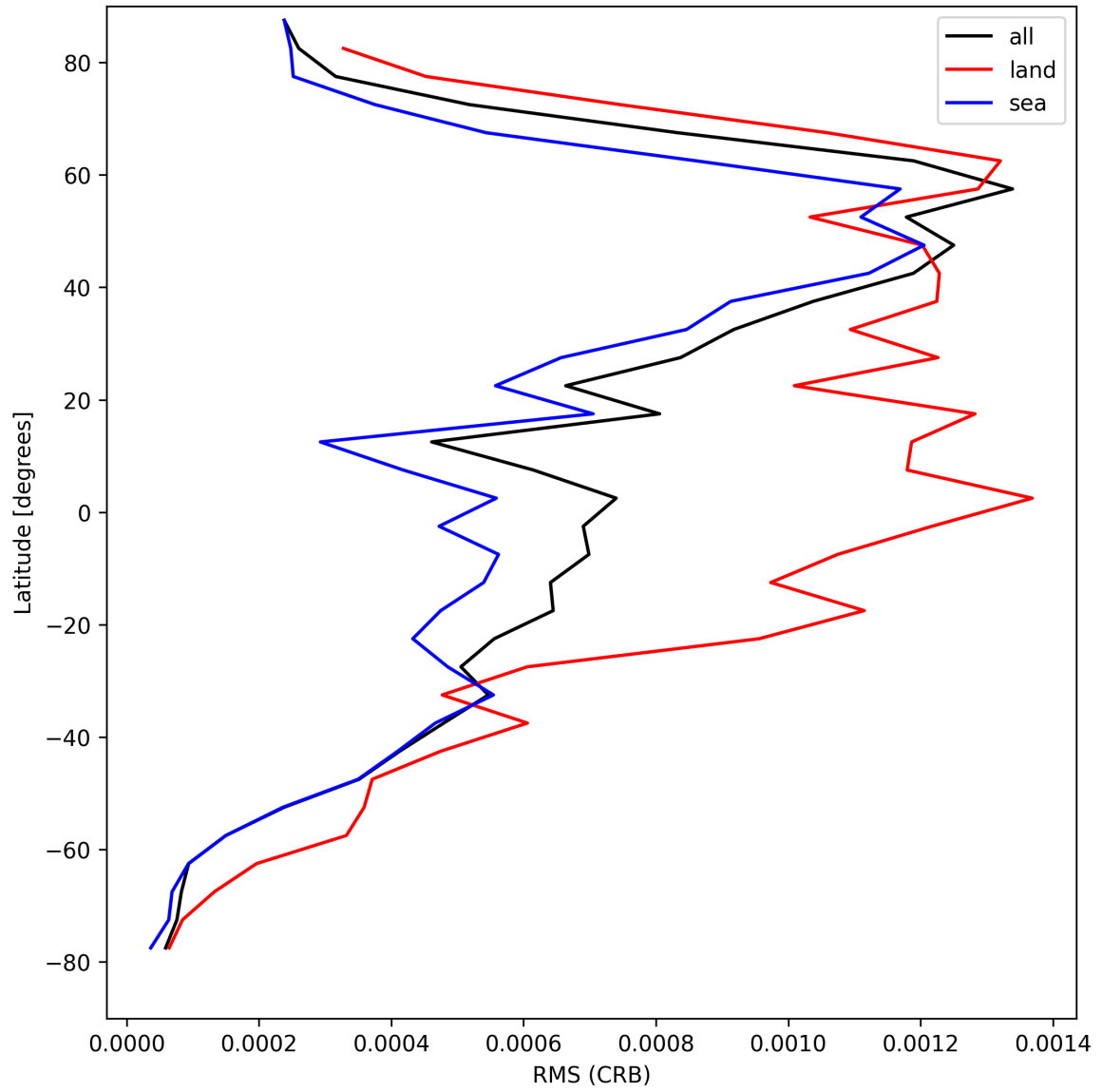
Figure 30: Zonal average of “RMS (CRB)” for 2025-04-16 to 2025-04-16.
