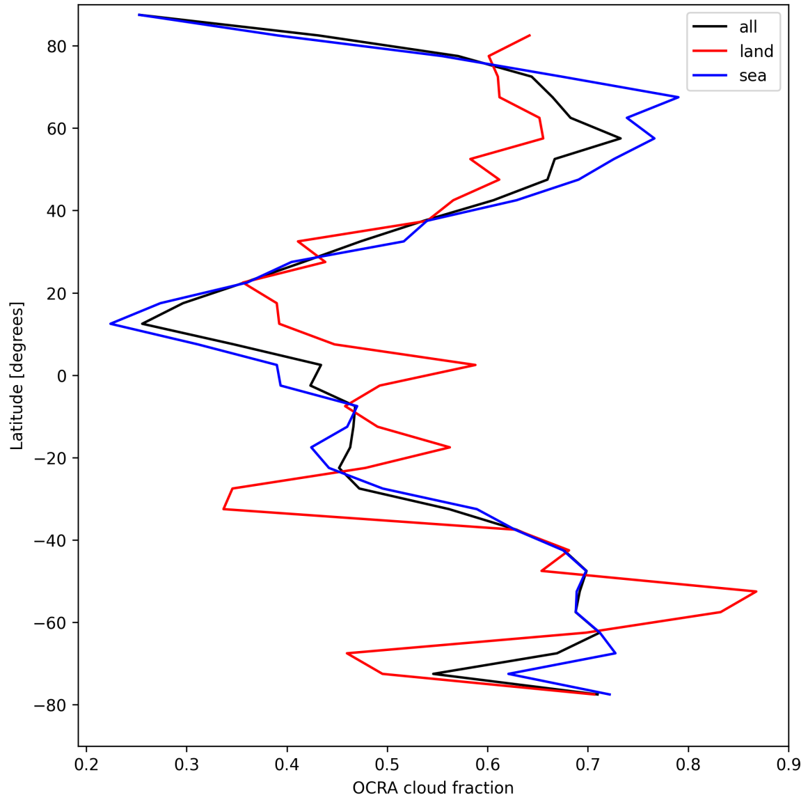
Figure 32: Zonal average of “OCRA cloud fraction” for 2025-04-16 to 2025-04-16.
