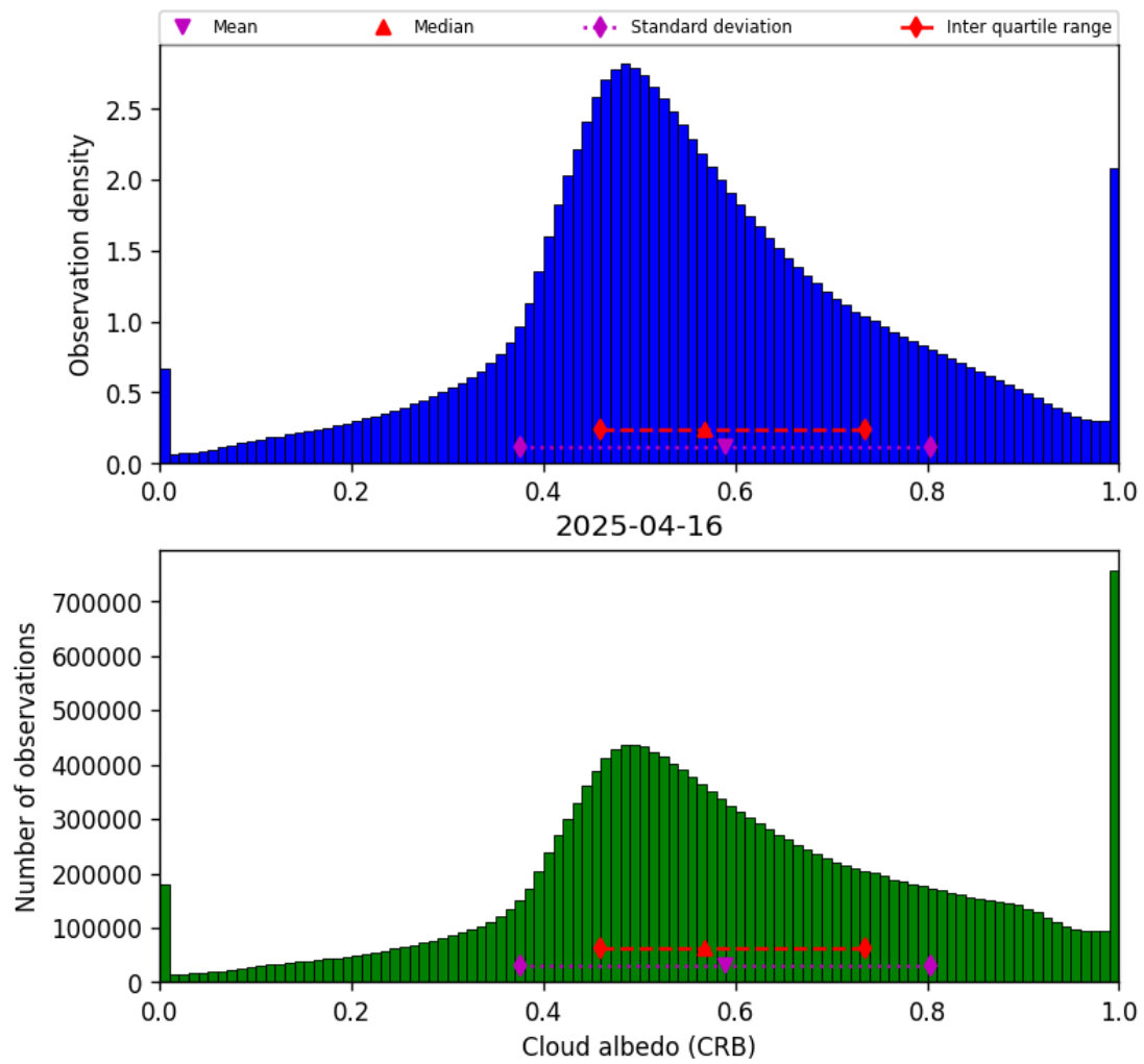
Figure 42: Histogram of “Cloud albedo (CRB)” for 2025-04-16 to 2025-04-16
