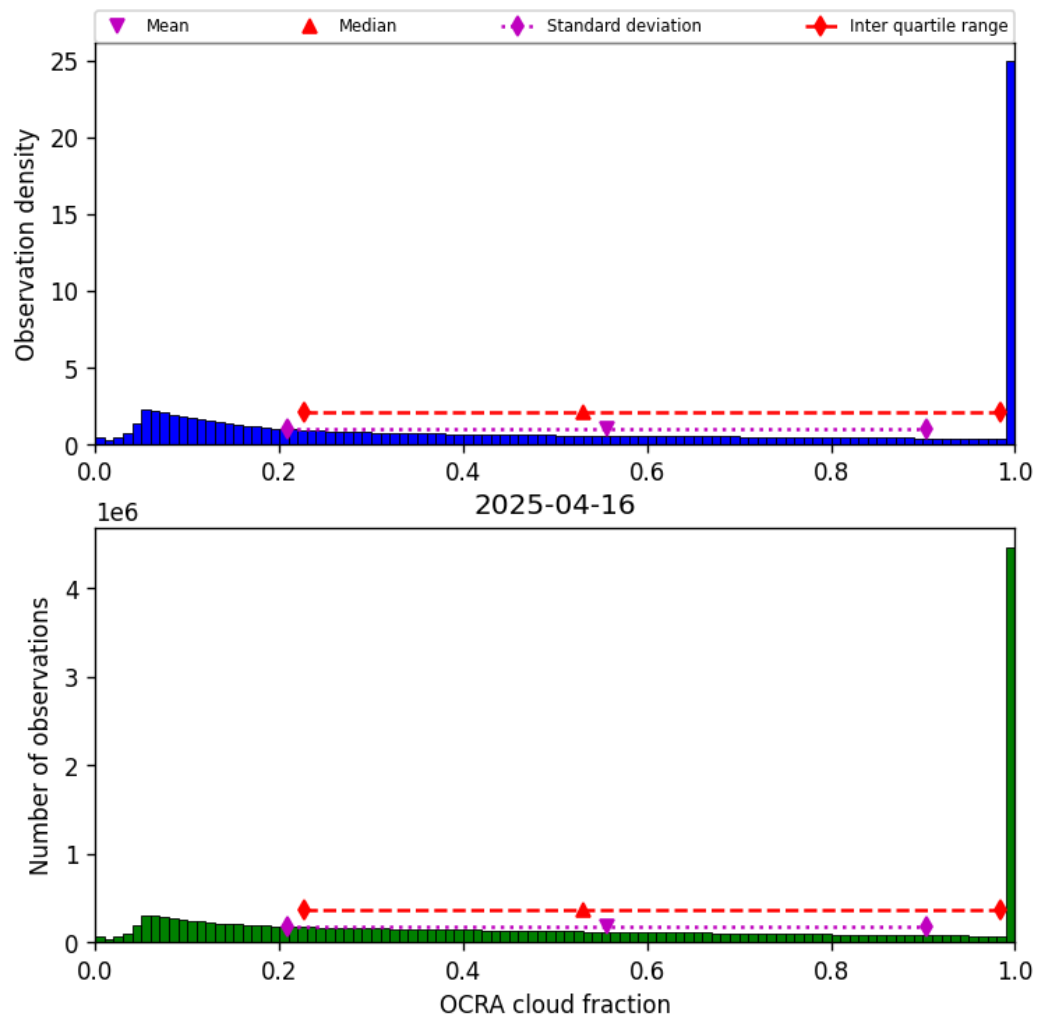
Figure 48: Histogram of “OCRA cloud fraction” for 2025-04-16 to 2025-04-16
