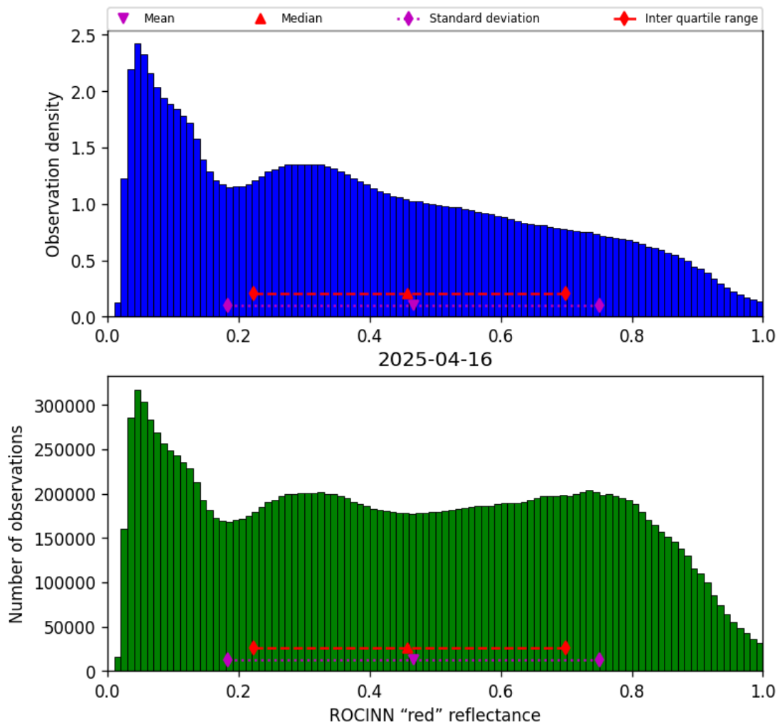
Figure 51: Histogram of “ROCINN “red” reflectance” for 2025-04-16 to 2025-04-16
