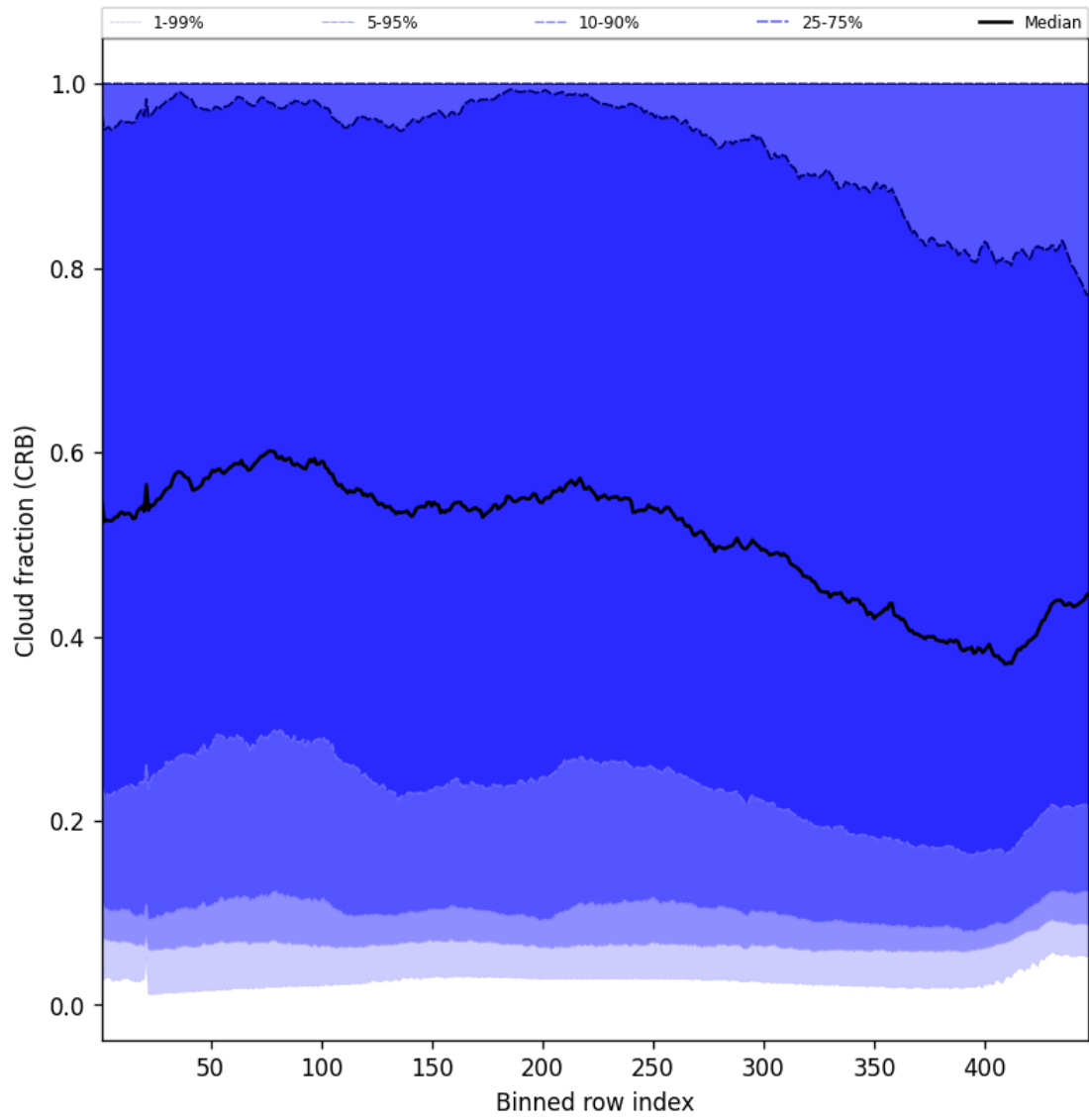
Figure 56: Along track statistics of “Cloud fraction (CRB)” for 2025-04-16 to 2025-04-16
