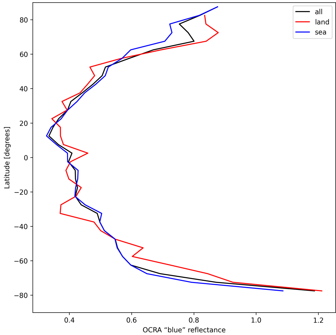
Figure 33: Zonal average of “OCRA “blue” reflectance” for 2025-04-16 to 2025-04-16.
