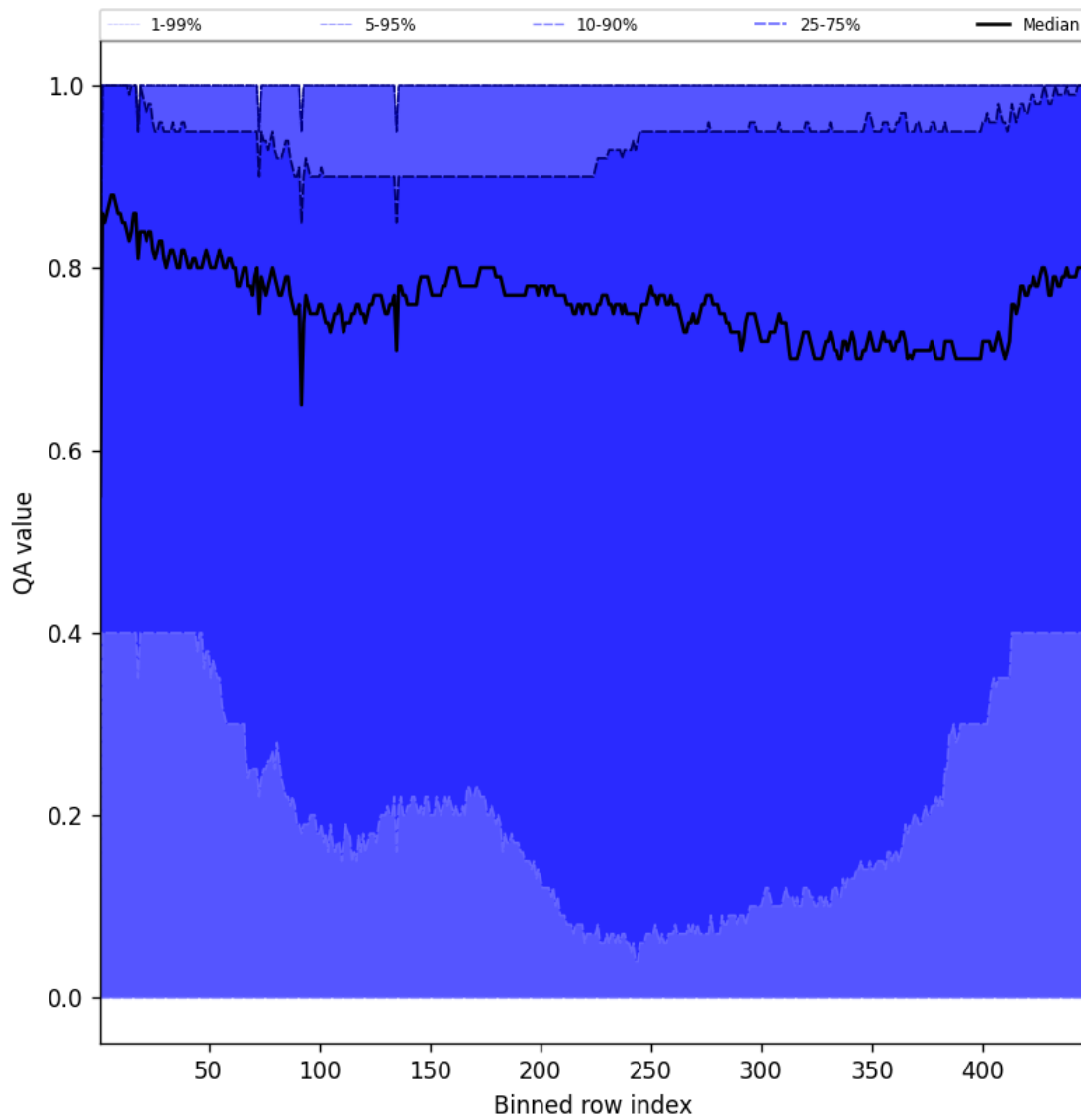
Figure 52: Along track statistics of “QA value” for 2025-04-16 to 2025-04-16
