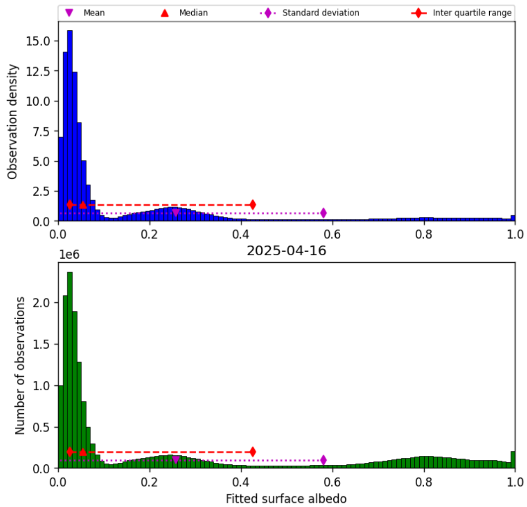
Figure 43: Histogram of “Fitted surface albedo” for 2025-04-16 to 2025-04-16
