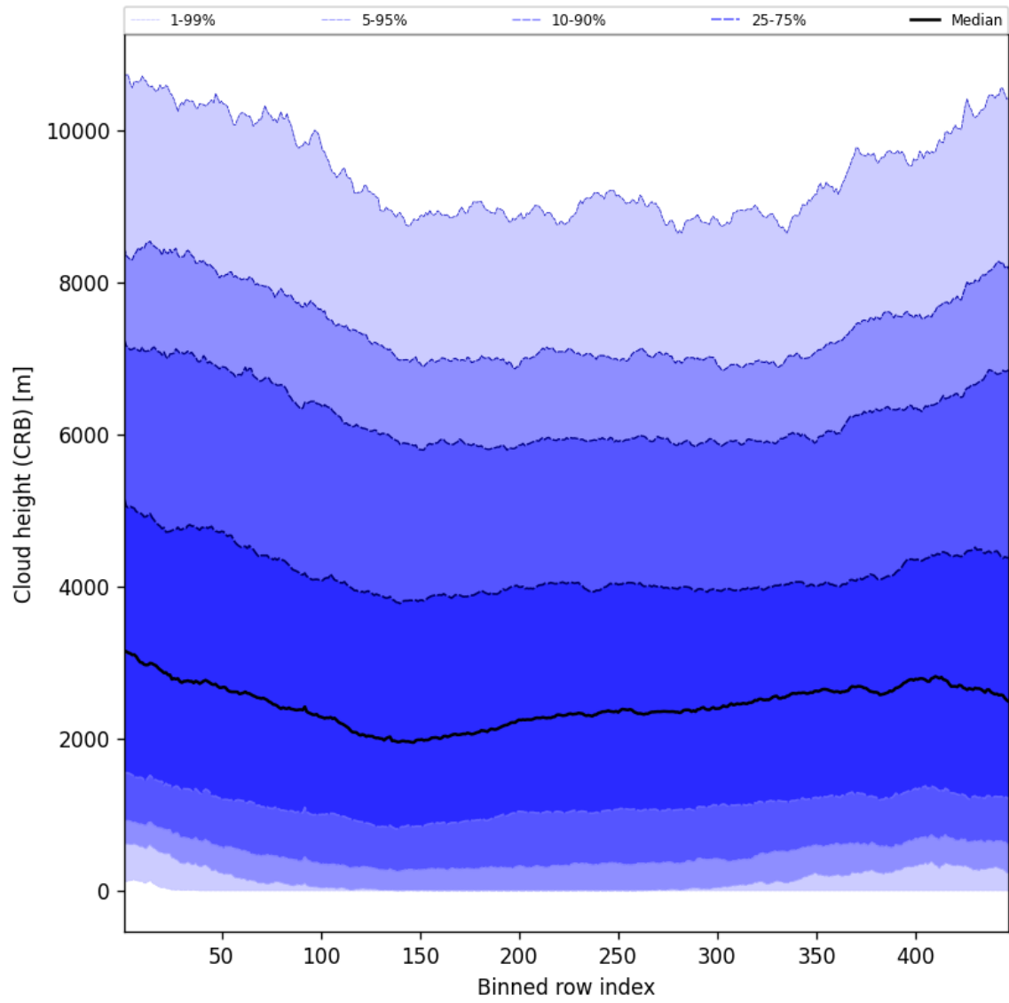
Figure 57: Along track statistics of “Cloud height (CRB)” for 2025-04-16 to 2025-04-16
