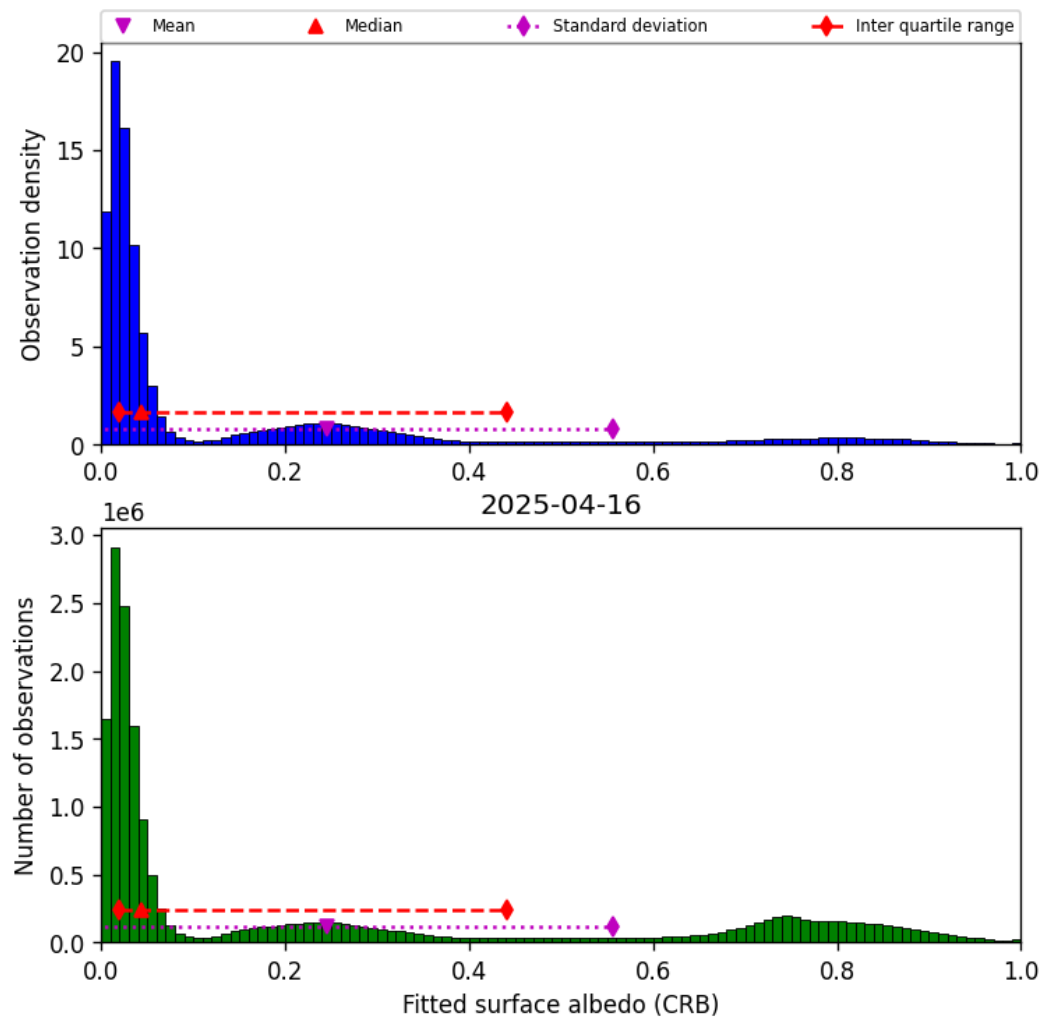
Figure 44: Histogram of “Fitted surface albedo (CRB)” for 2025-04-16 to 2025-04-16
