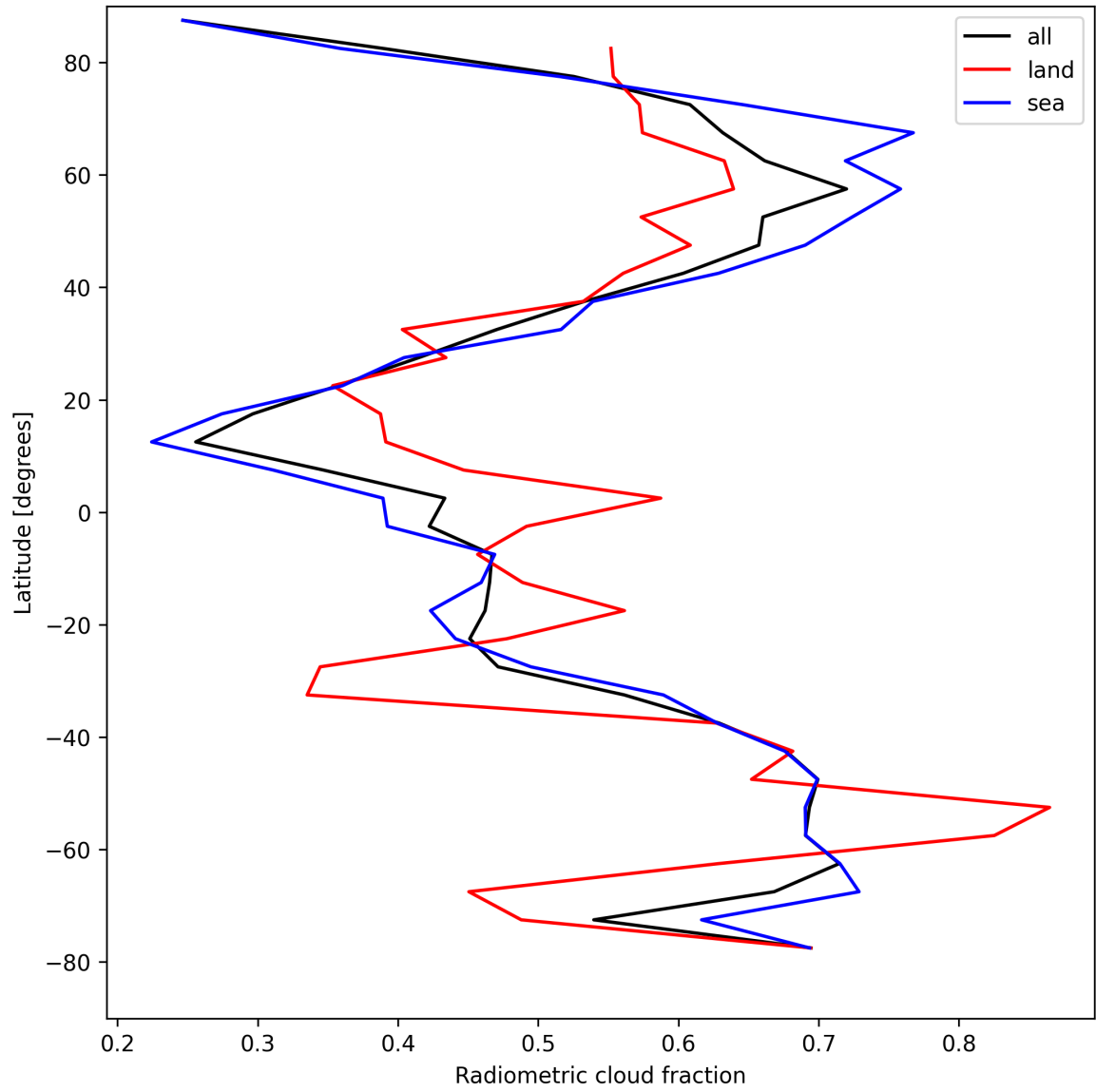
Figure 21: Zonal average of “Radiometric cloud fraction” for 2025-04-16 to 2025-04-16.
