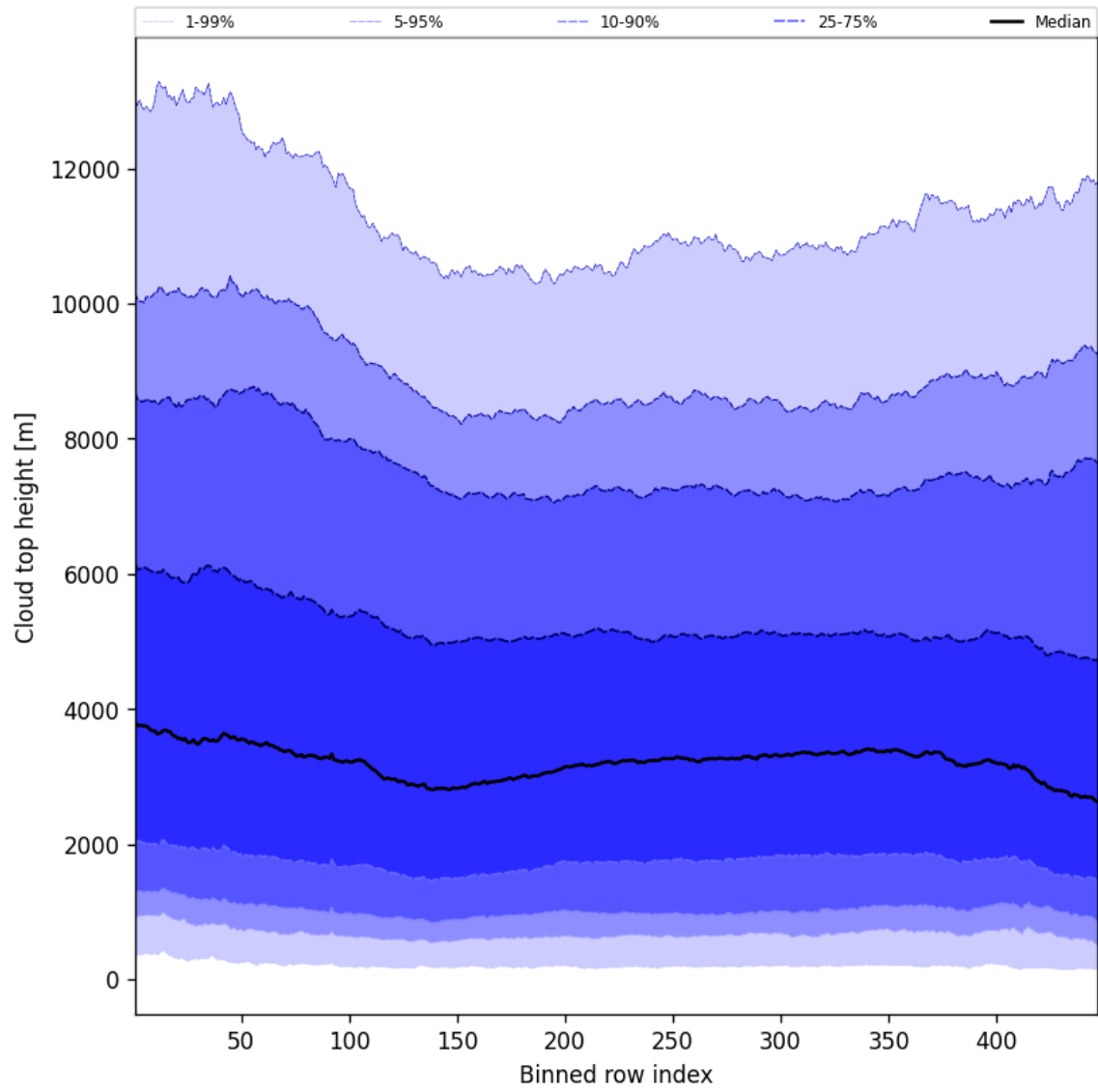
Figure 54: Along track statistics of “Cloud top height” for 2025-04-16 to 2025-04-16
