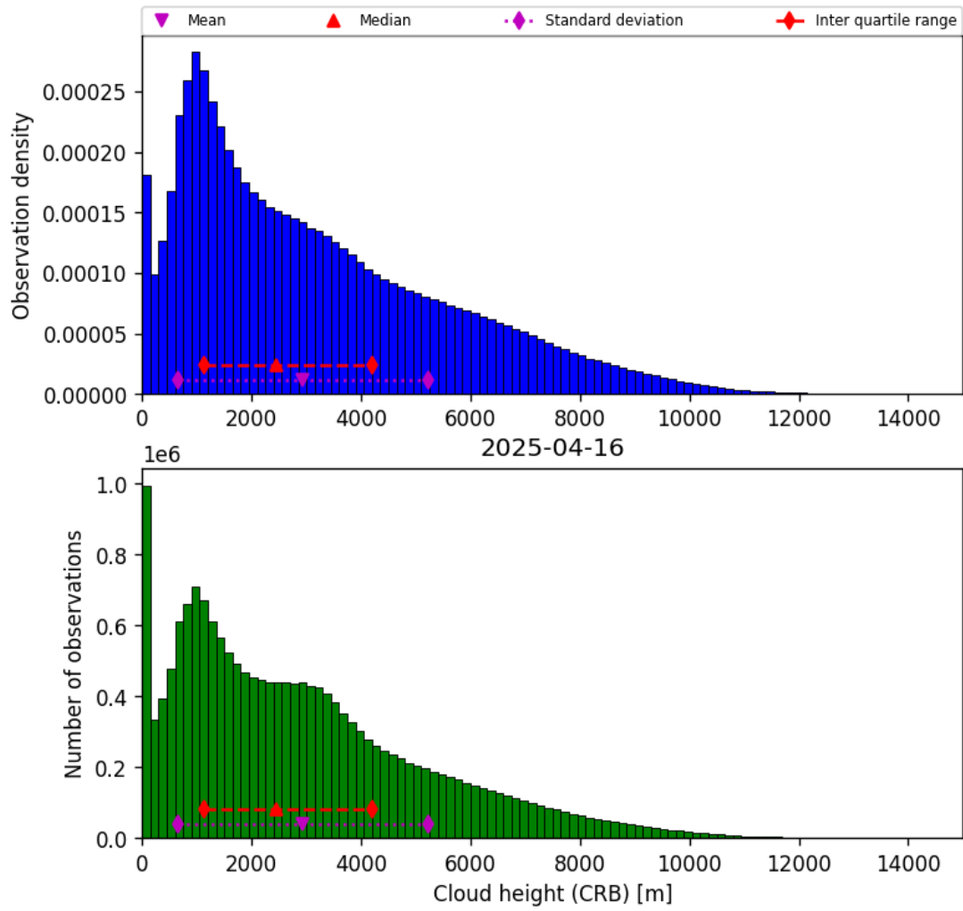
Figure 41: Histogram of “Cloud height (CRB)” for 2025-04-16 to 2025-04-16
