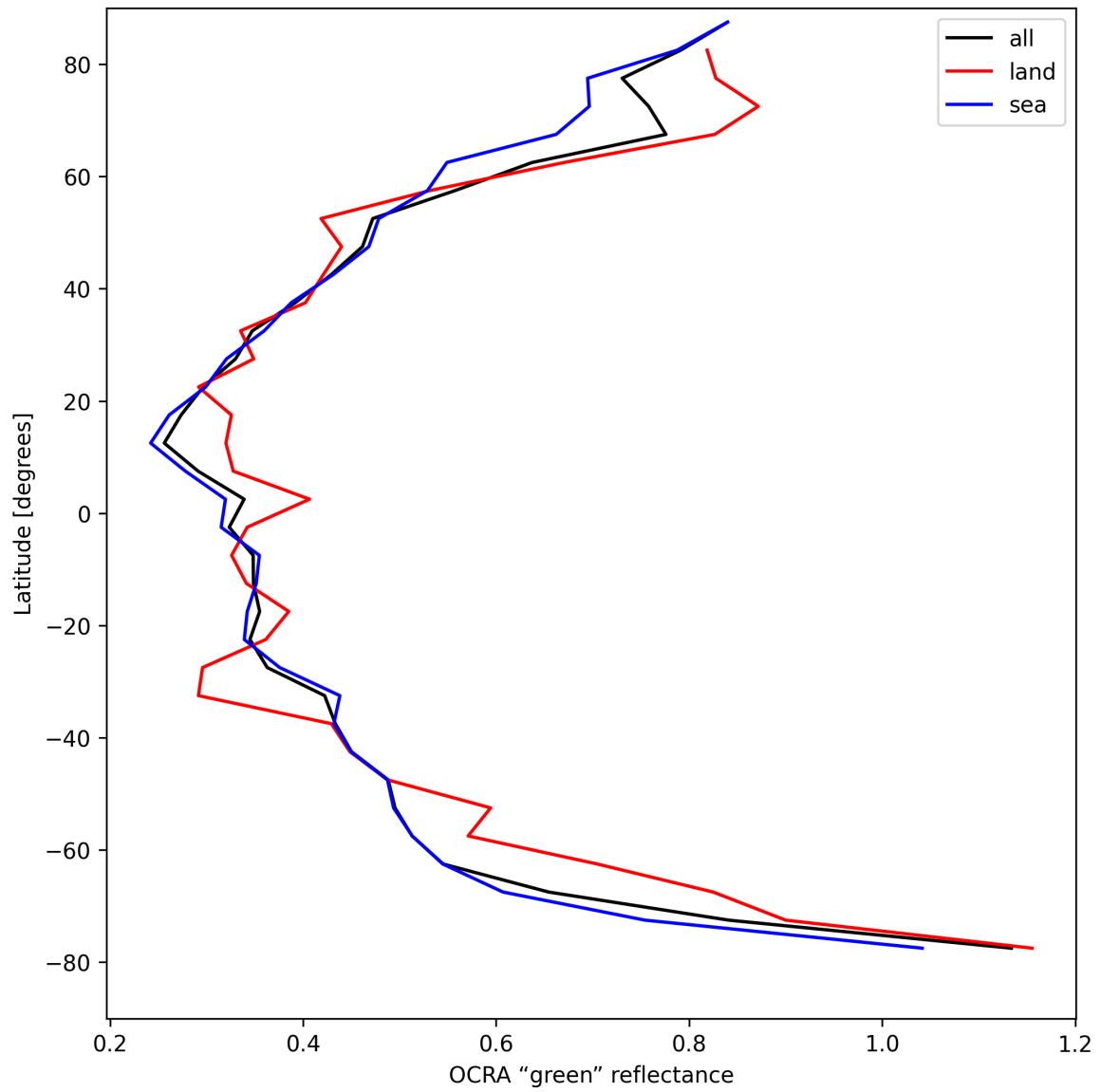
Figure 34: Zonal average of “OCRA “green” reflectance” for 2025-04-16 to 2025-04-16.
