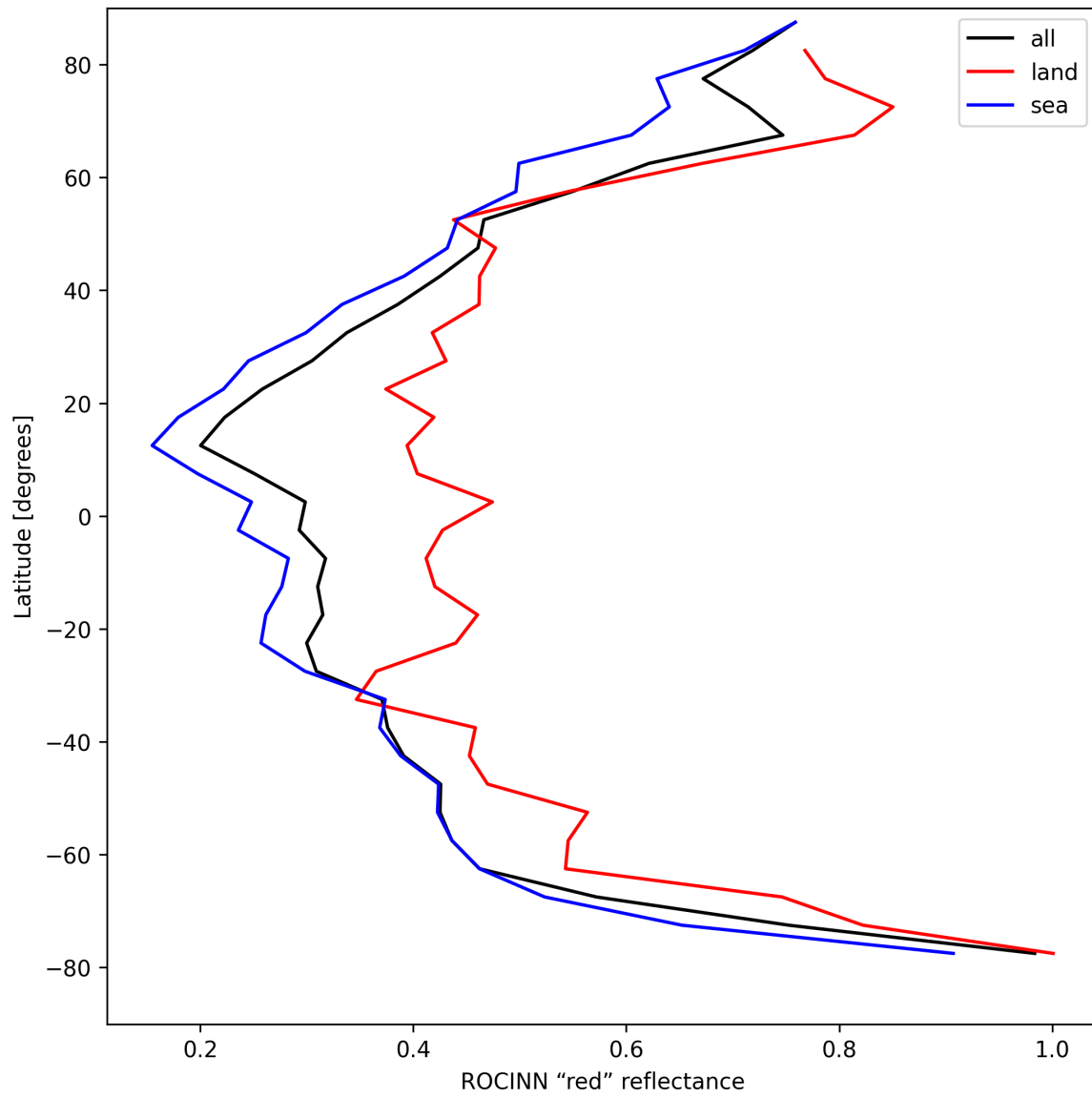
Figure 35: Zonal average of “ROCINN “red” reflectance” for 2025-04-16 to 2025-04-16.
