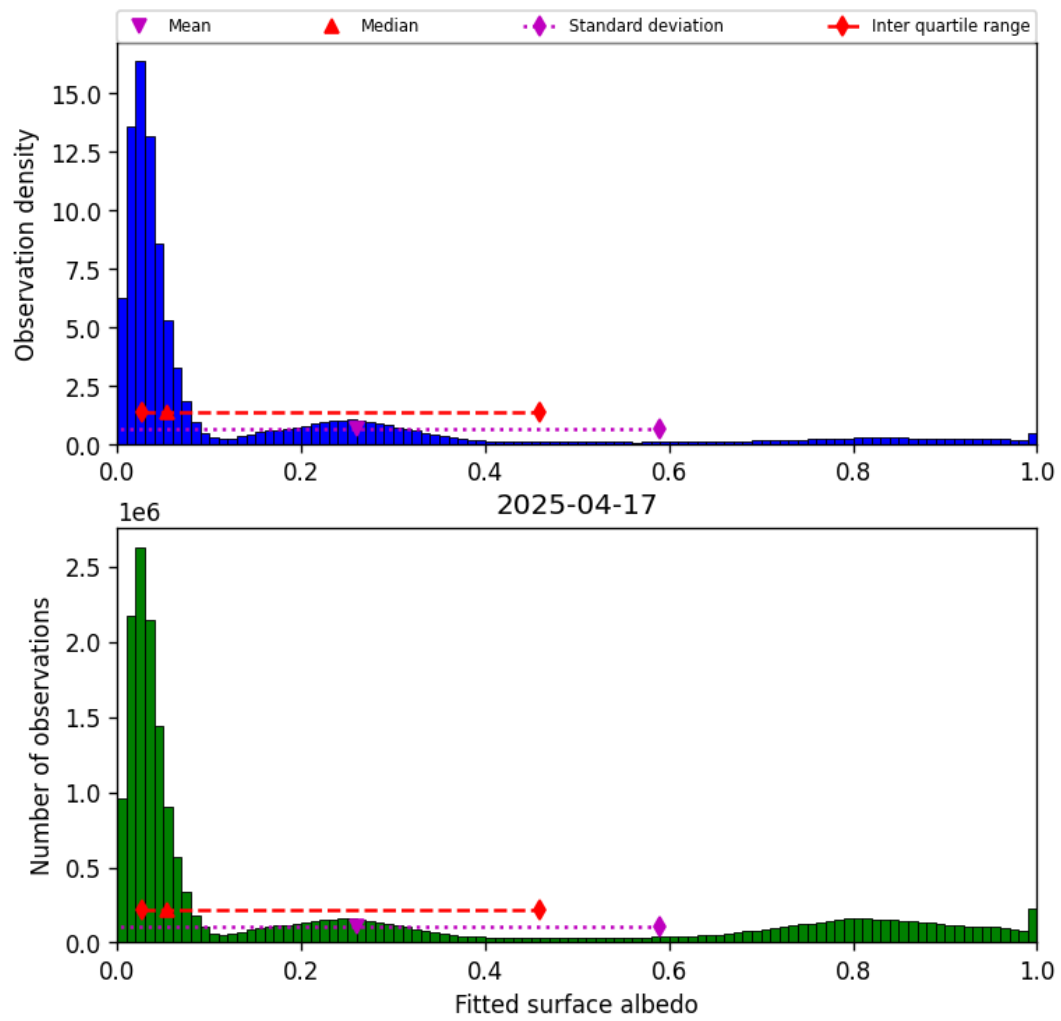
Figure 43: Histogram of “Fitted surface albedo” for 2025-04-17 to 2025-04-18
