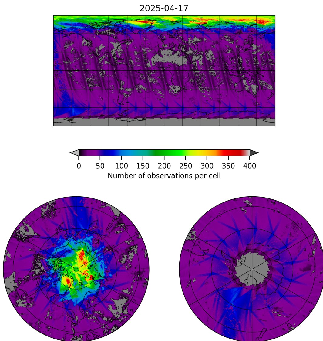
Figure 19: Map of the number of observations for 2025-04-17 to 2025-04-18
