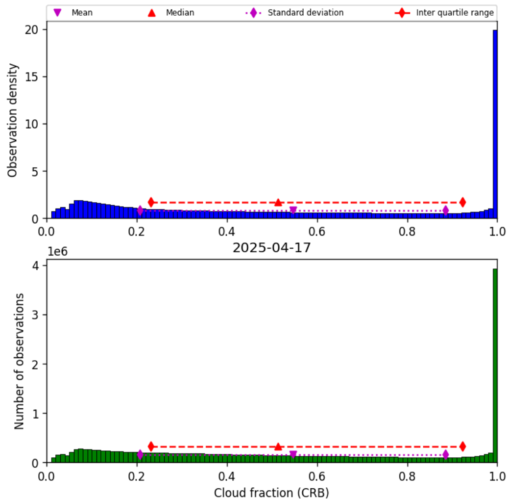
Figure 40: Histogram of “Cloud fraction (CRB)” for 2025-04-17 to 2025-04-18
