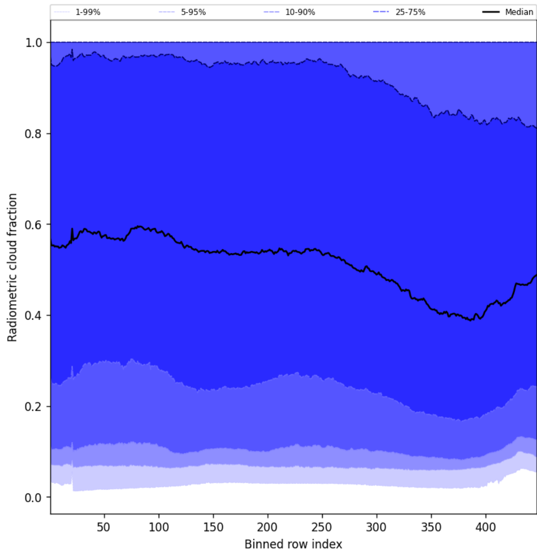
Figure 53: Along track statistics of “Radiometric cloud fraction” for 2025-04-17 to 2025-04-18
