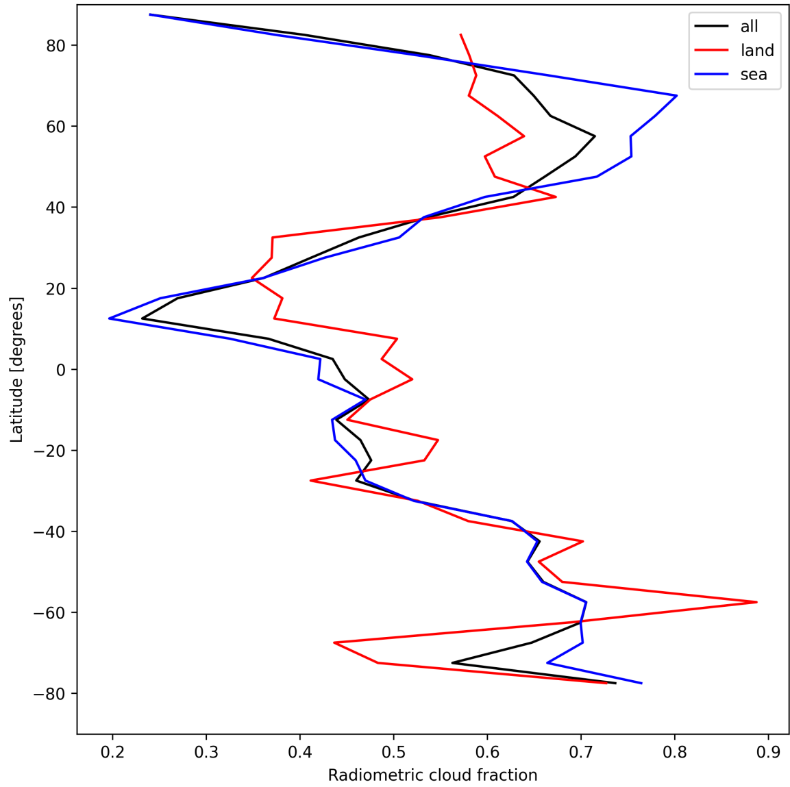
Figure 21: Zonal average of “Radiometric cloud fraction” for 2025-04-17 to 2025-04-18.
