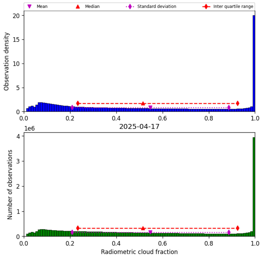
Figure 37: Histogram of “Radiometric cloud fraction” for 2025-04-17 to 2025-04-18
