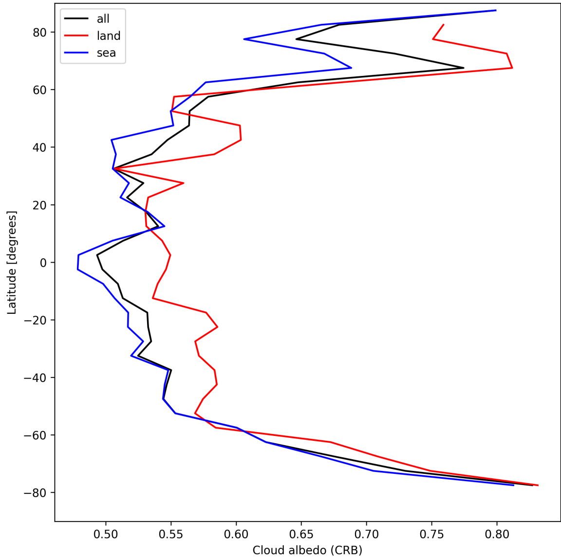
Figure 26: Zonal average of “Cloud albedo (CRB)” for 2025-04-17 to 2025-04-18.
