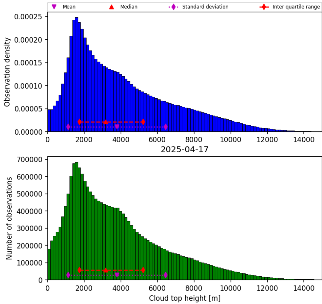
Figure 38: Histogram of “Cloud top height” for 2025-04-17 to 2025-04-18
