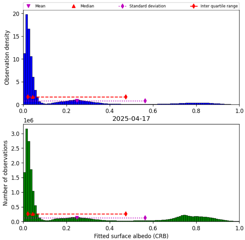
Figure 44: Histogram of “Fitted surface albedo (CRB)” for 2025-04-17 to 2025-04-18
