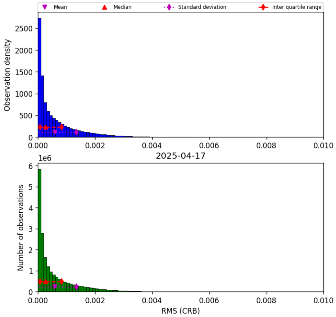
Figure 46: Histogram of “RMS (CRB)” for 2025-04-17 to 2025-04-18
