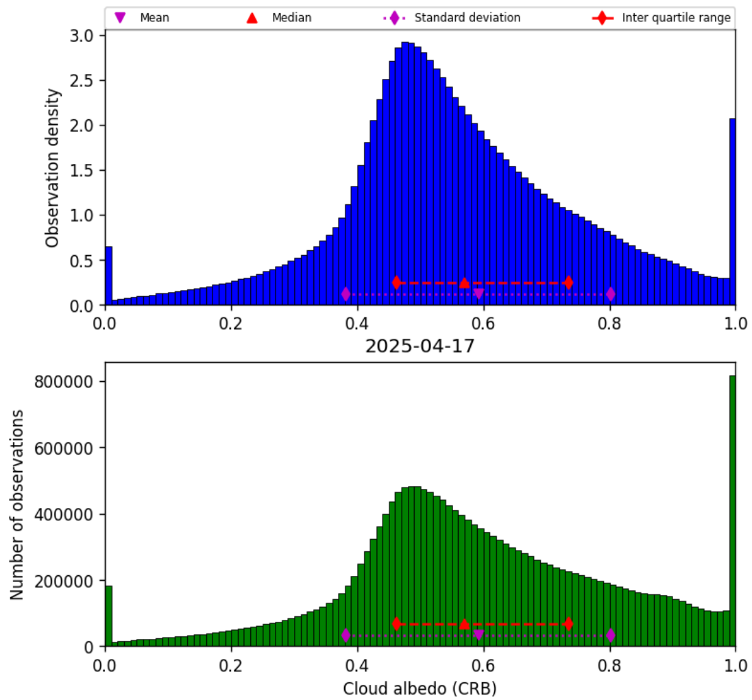
Figure 42: Histogram of “Cloud albedo (CRB)” for 2025-04-17 to 2025-04-18
