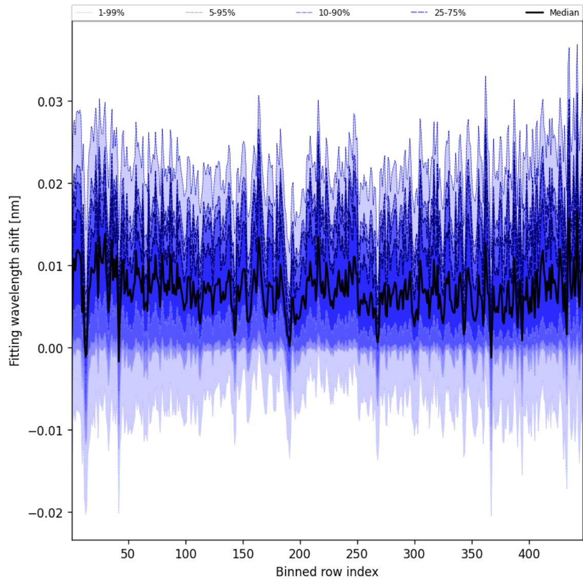
Figure 63: Along track statistics of “Fitting wavelength shift” for 2025-04-17 to 2025-04-18
