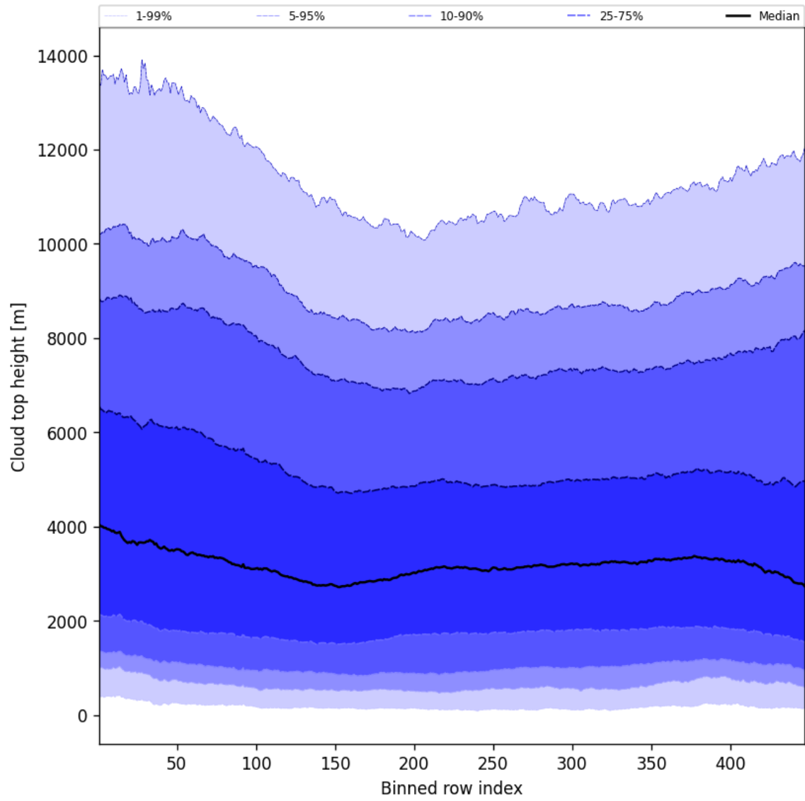
Figure 54: Along track statistics of “Cloud top height” for 2025-04-17 to 2025-04-18
