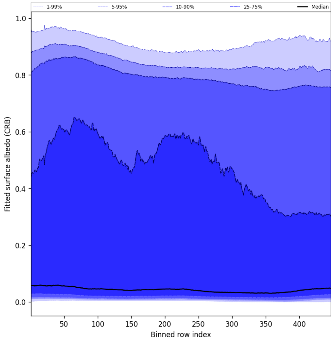
Figure 60: Along track statistics of “Fitted surface albedo (CRB)” for 2025-04-17 to 2025-04-18
