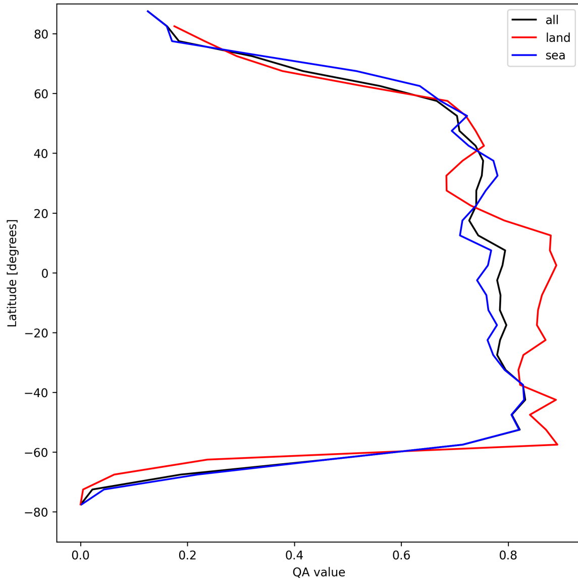
Figure 20: Zonal average of “QA value” for 2025-04-17 to 2025-04-18.
