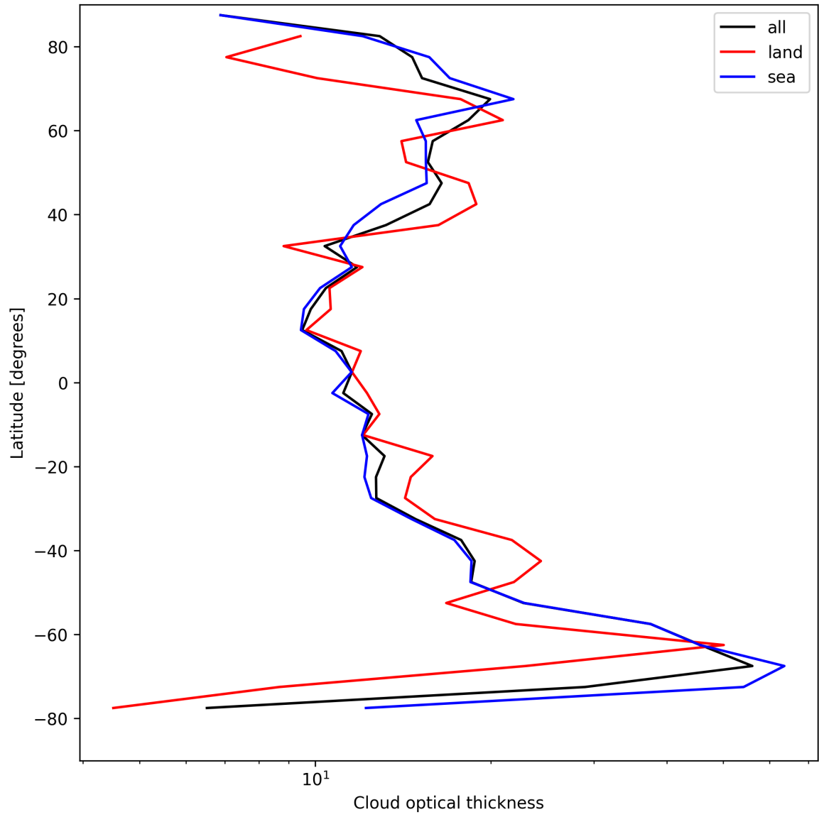
Figure 23: Zonal average of “Cloud optical thickness” for 2025-04-17 to 2025-04-18.
