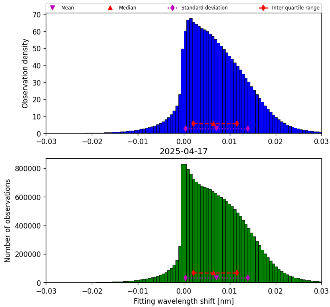
Figure 47: Histogram of “Fitting wavelength shift” for 2025-04-17 to 2025-04-18
