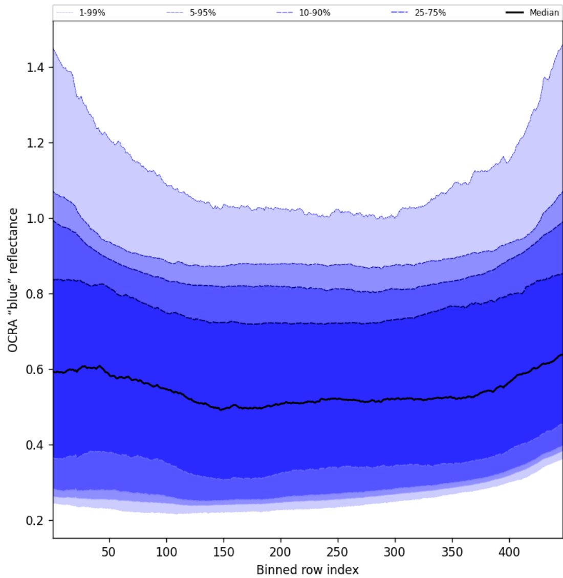
Figure 65: Along track statistics of “OCRA “blue” reflectance” for 2025-04-17 to 2025-04-18
