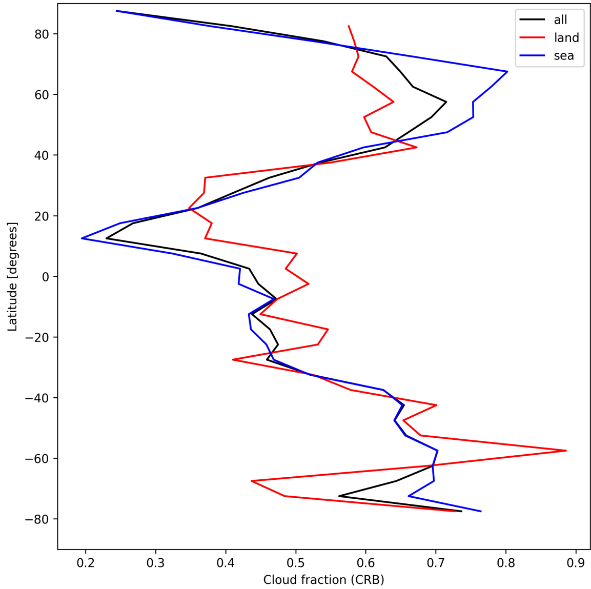
Figure 24: Zonal average of “Cloud fraction (CRB)” for 2025-04-17 to 2025-04-18.
