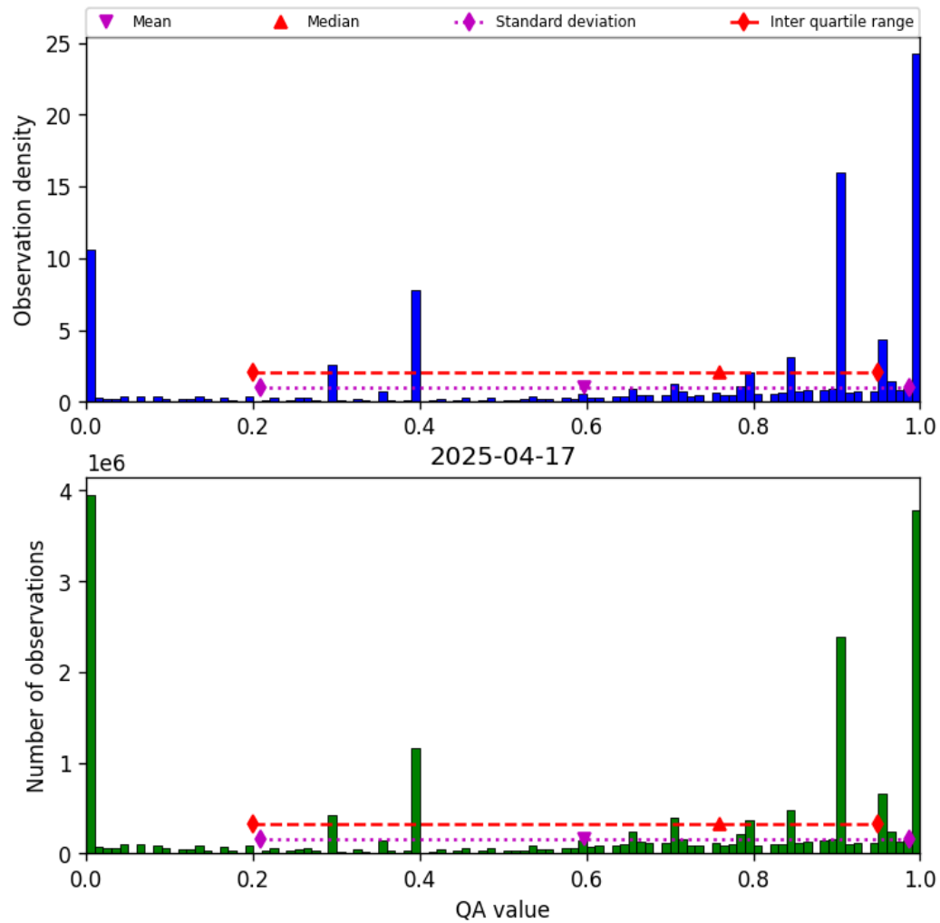
Figure 36: Histogram of “QA value” for 2025-04-17 to 2025-04-18
