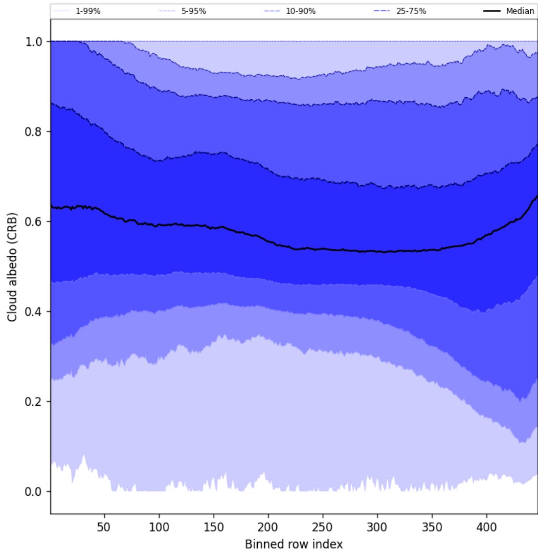
Figure 58: Along track statistics of “Cloud albedo (CRB)” for 2025-04-17 to 2025-04-18
