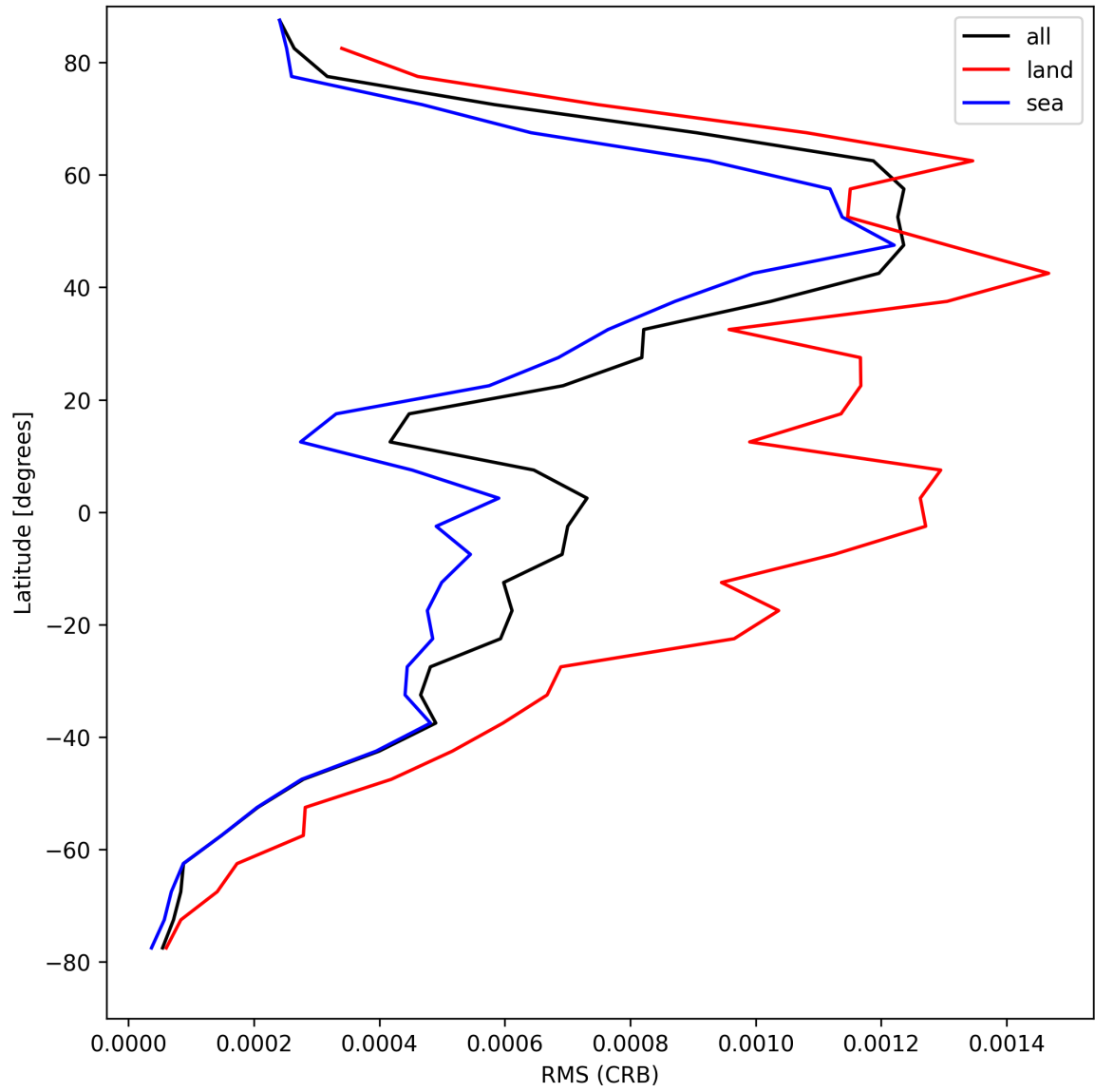
Figure 30: Zonal average of “RMS (CRB)” for 2025-04-17 to 2025-04-18.
