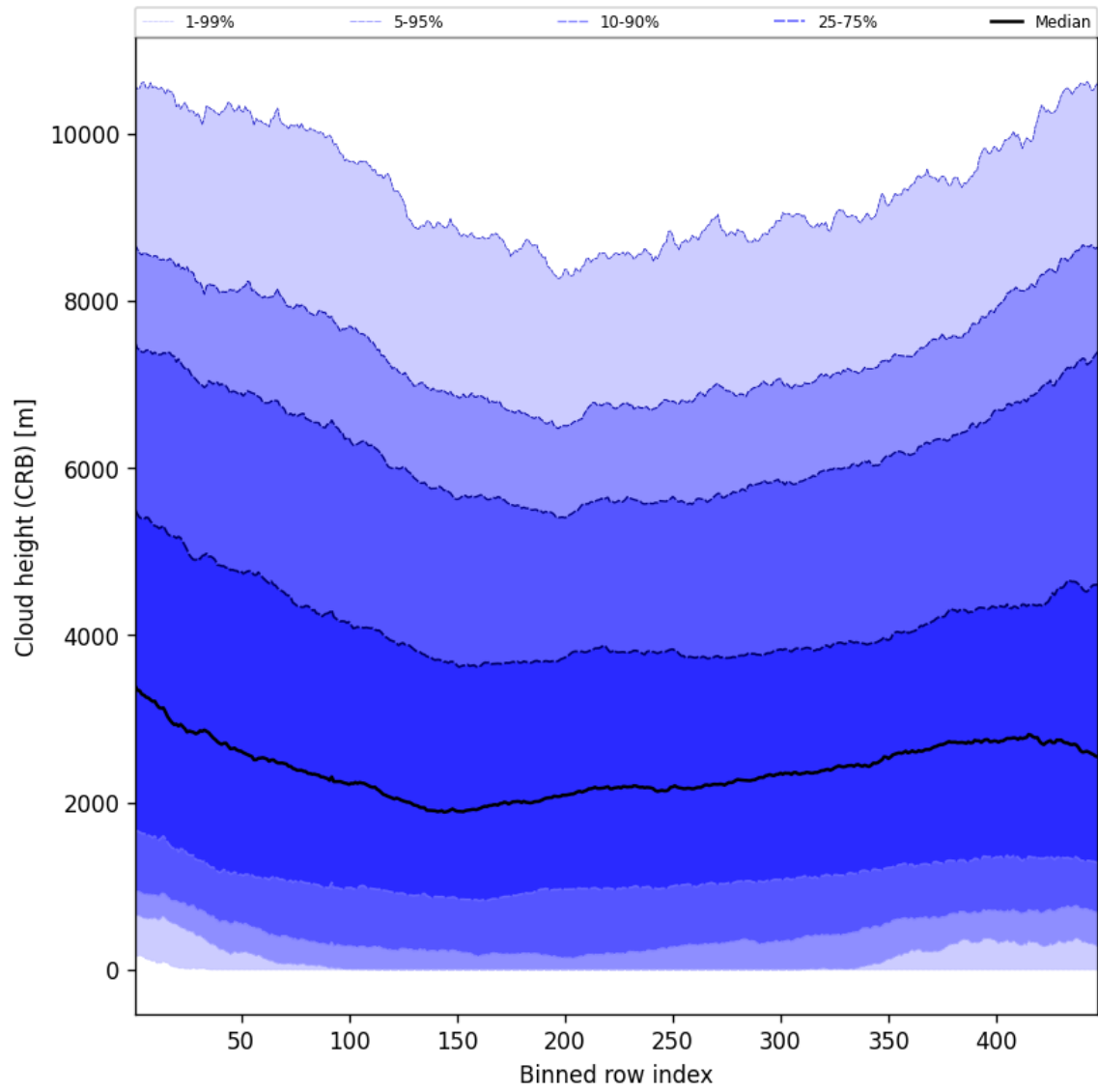
Figure 57: Along track statistics of “Cloud height (CRB)” for 2025-04-17 to 2025-04-18
