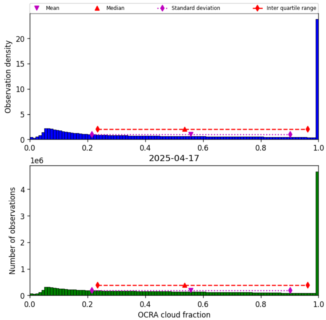
Figure 48: Histogram of “OCRA cloud fraction” for 2025-04-17 to 2025-04-18
