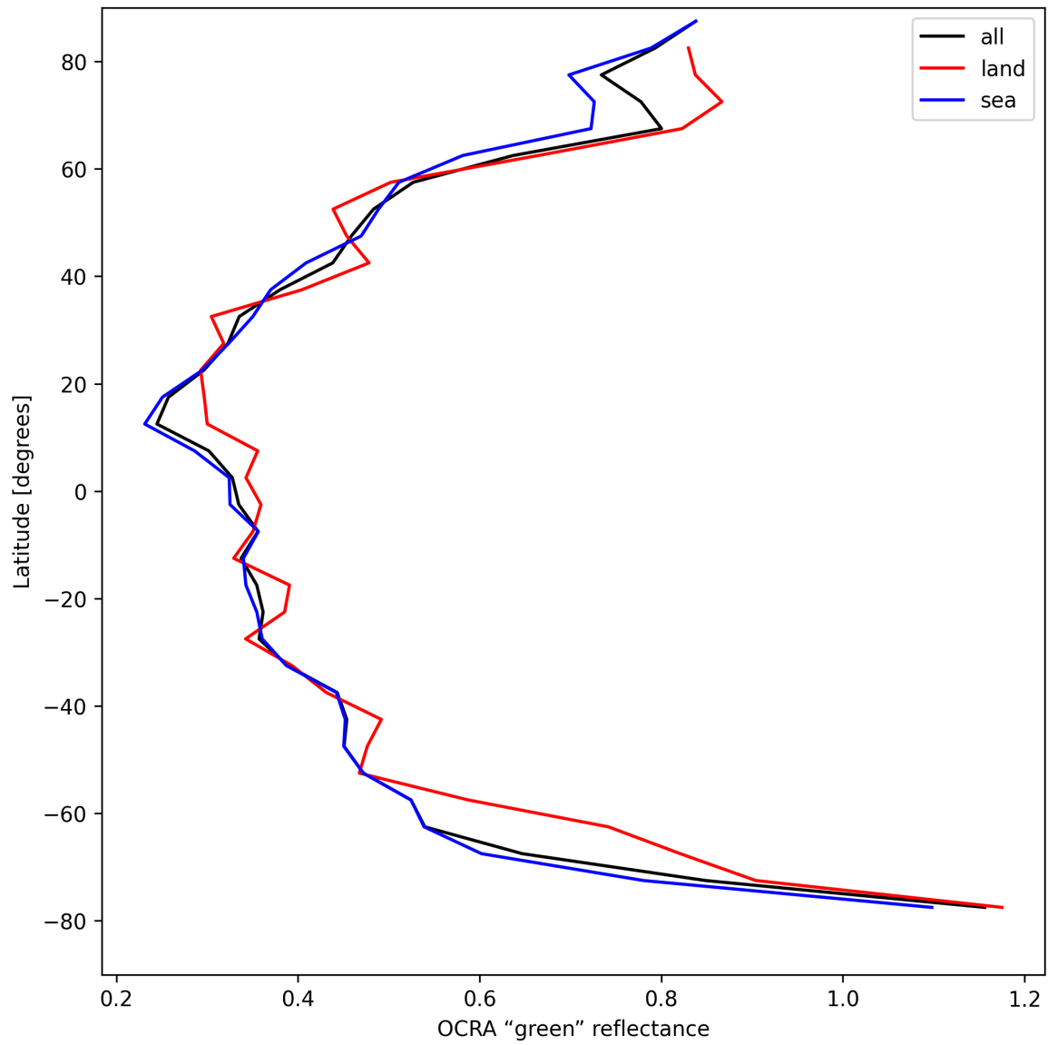
Figure 34: Zonal average of "OCRA "green" reflectance" for 2025-04-17 to 2025-04-18.
