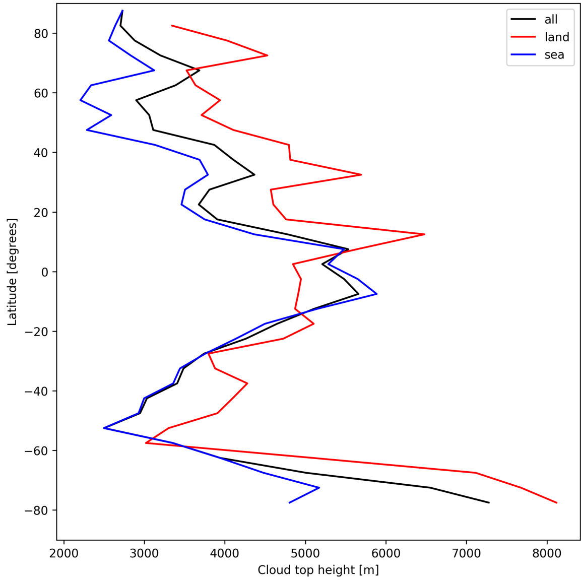
Figure 22: Zonal average of “Cloud top height” for 2025-04-17 to 2025-04-18.
