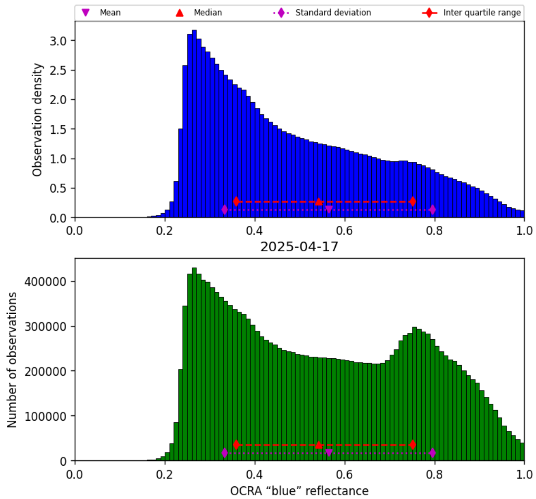
Figure 49: Histogram of “OCRA “blue” reflectance” for 2025-04-17 to 2025-04-18
