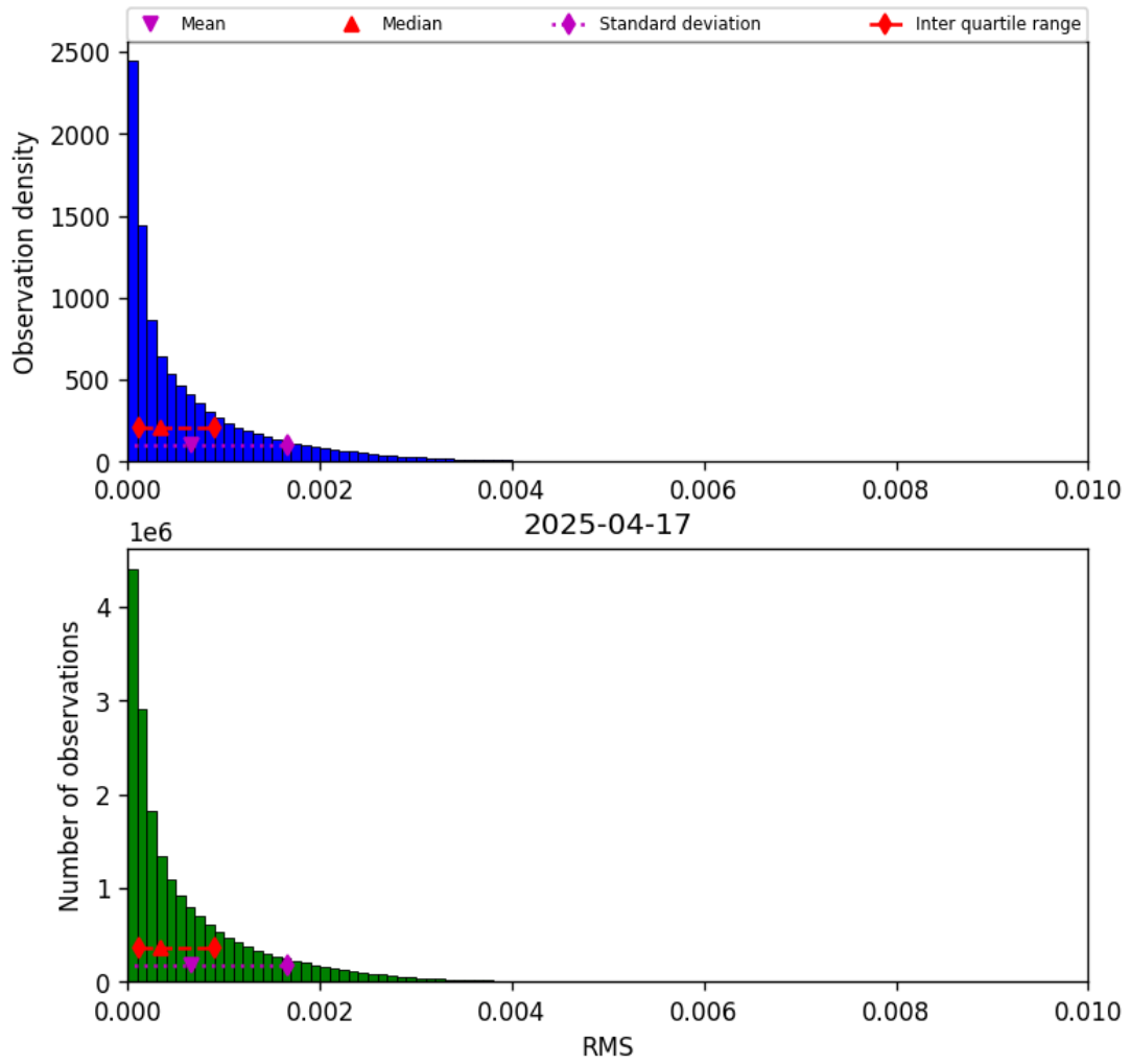
Figure 45: Histogram of “RMS” for 2025-04-17 to 2025-04-18
