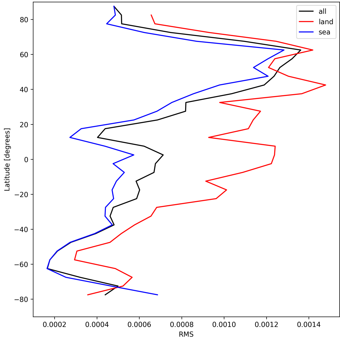
Figure 29: Zonal average of “RMS” for 2025-04-17 to 2025-04-18.
