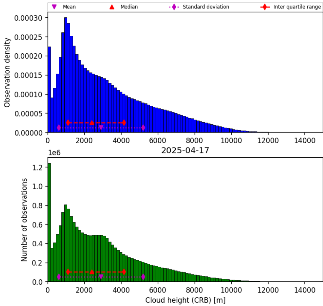
Figure 41: Histogram of “Cloud height (CRB)” for 2025-04-17 to 2025-04-18
