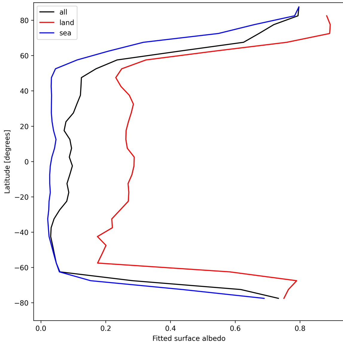
Figure 27: Zonal average of “Fitted surface albedo” for 2025-04-17 to 2025-04-18.
