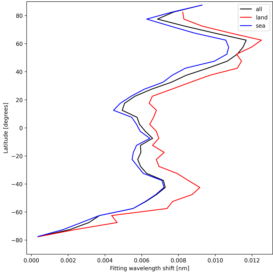
Figure 31: Zonal average of “Fitting wavelength shift” for 2025-04-17 to 2025-04-18.
