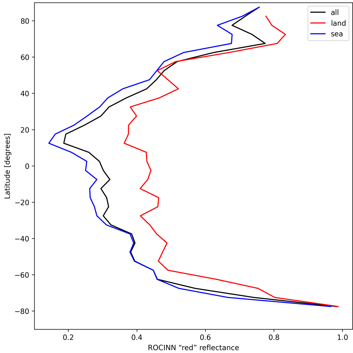
Figure 35: Zonal average of “ROCINN “red” reflectance” for 2025-04-17 to 2025-04-18.
