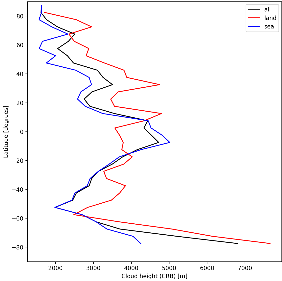
Figure 25: Zonal average of “Cloud height (CRB)” for 2025-04-17 to 2025-04-18.
