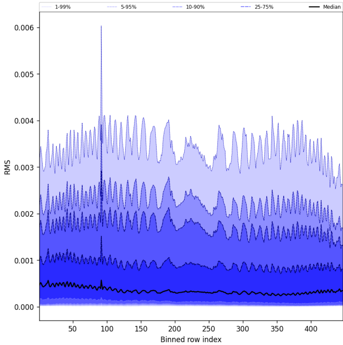
Figure 61: Along track statistics of “RMS” for 2025-04-17 to 2025-04-18
