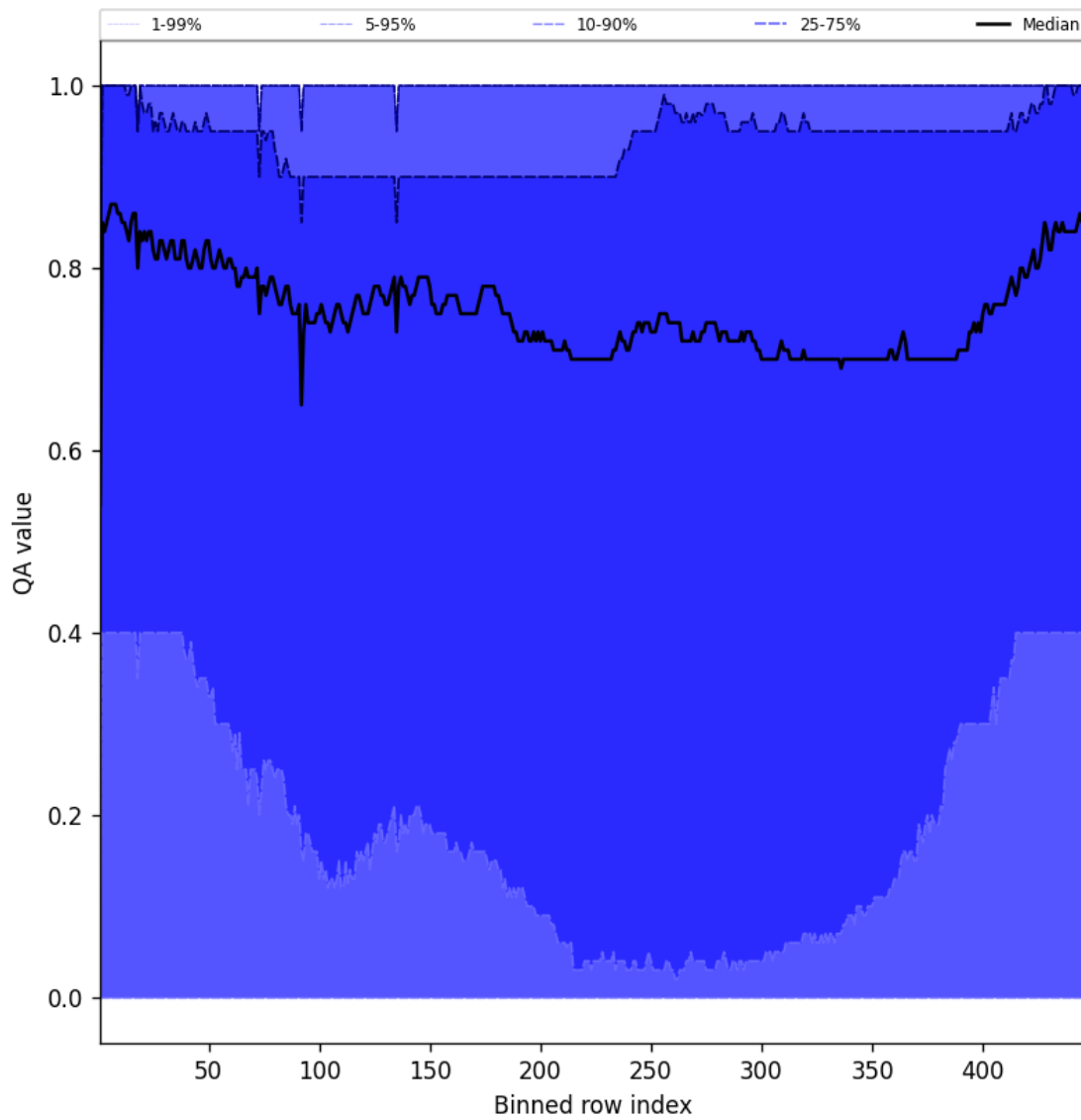
Figure 52: Along track statistics of “QA value” for 2025-04-17 to 2025-04-18
