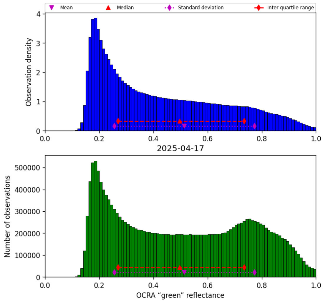
Figure 50: Histogram of “OCRA “green” reflectance” for 2025-04-17 to 2025-04-18
