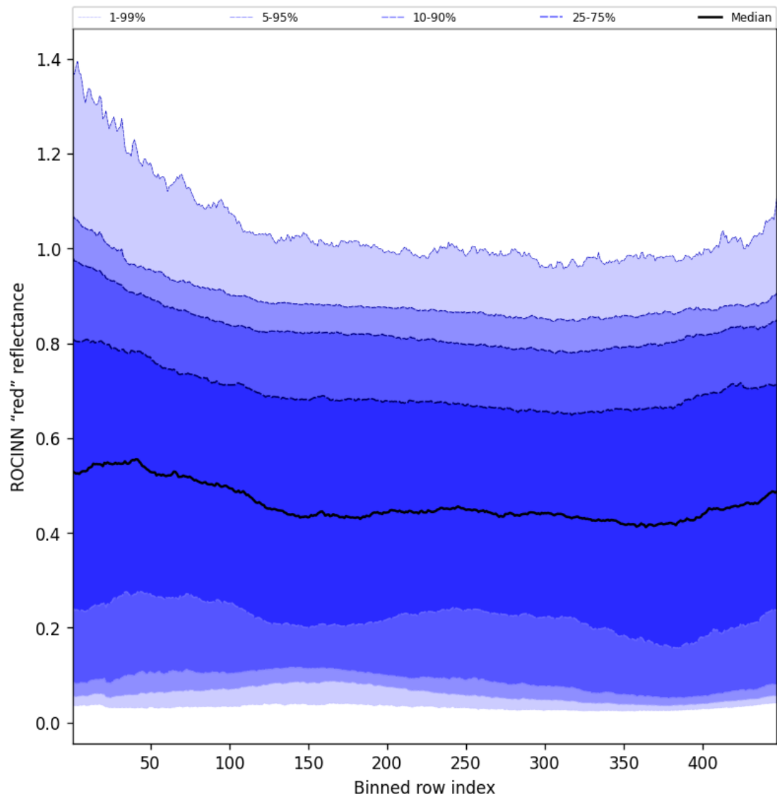
Figure 67: Along track statistics of "ROCINN "red" reflectance" for 2025-04-17 to 2025-04-18
