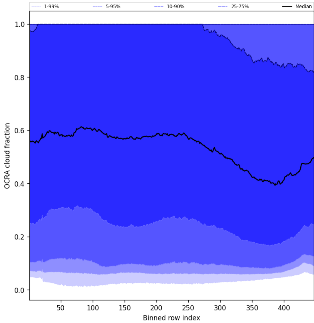
Figure 64: Along track statistics of “OCRA cloud fraction” for 2025-04-17 to 2025-04-18
