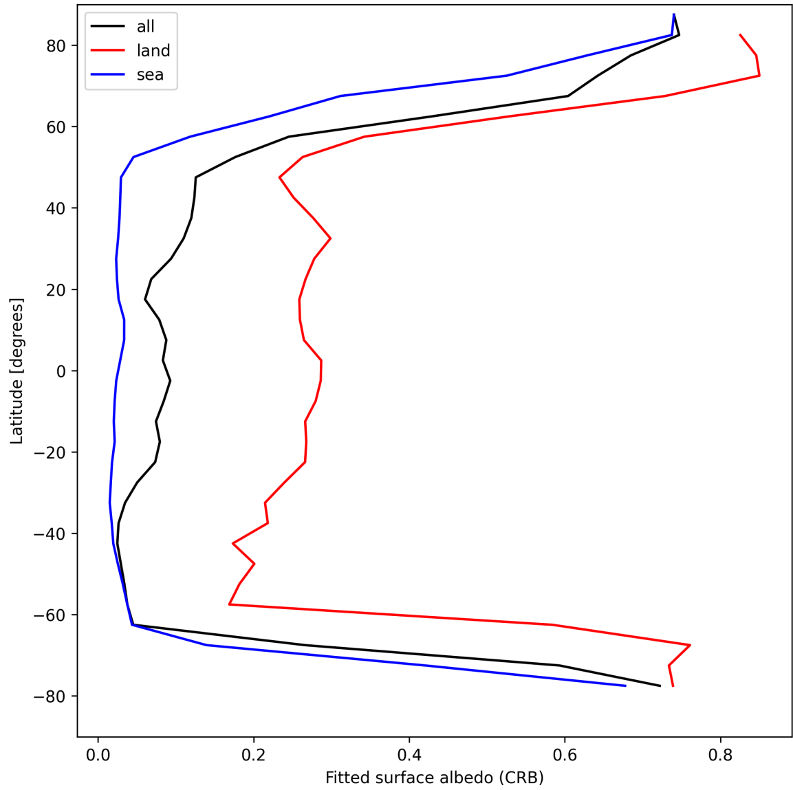
Figure 28: Zonal average of “Fitted surface albedo (CRB)” for 2025-04-17 to 2025-04-18.
