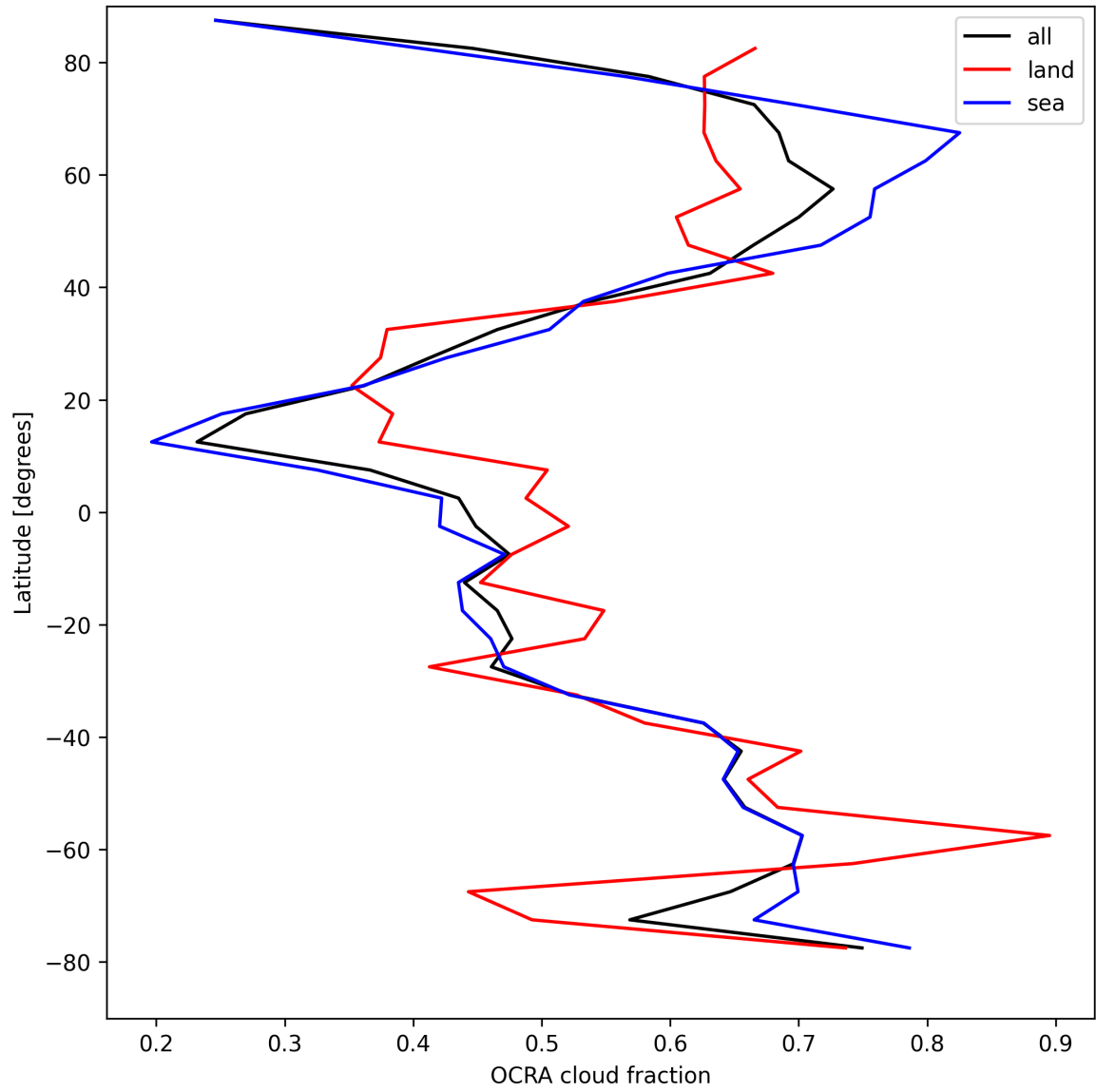
Figure 32: Zonal average of “OCRA cloud fraction” for 2025-04-17 to 2025-04-18.
