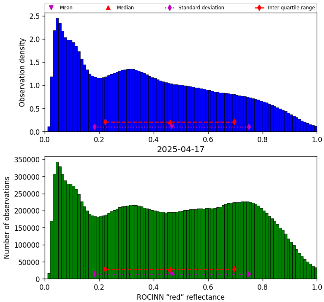
Figure 51: Histogram of “ROCINN “red” reflectance” for 2025-04-17 to 2025-04-18
