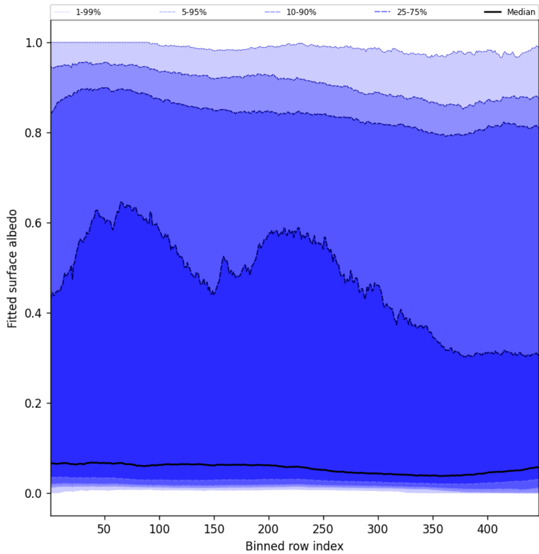
Figure 59: Along track statistics of “Fitted surface albedo” for 2025-04-17 to 2025-04-18
