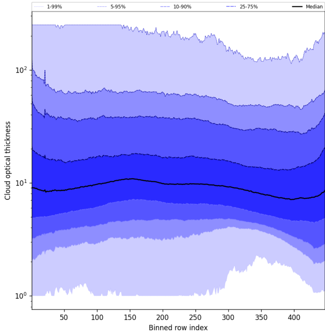
Figure 55: Along track statistics of “Cloud optical thickness” for 2025-04-17 to 2025-04-18
