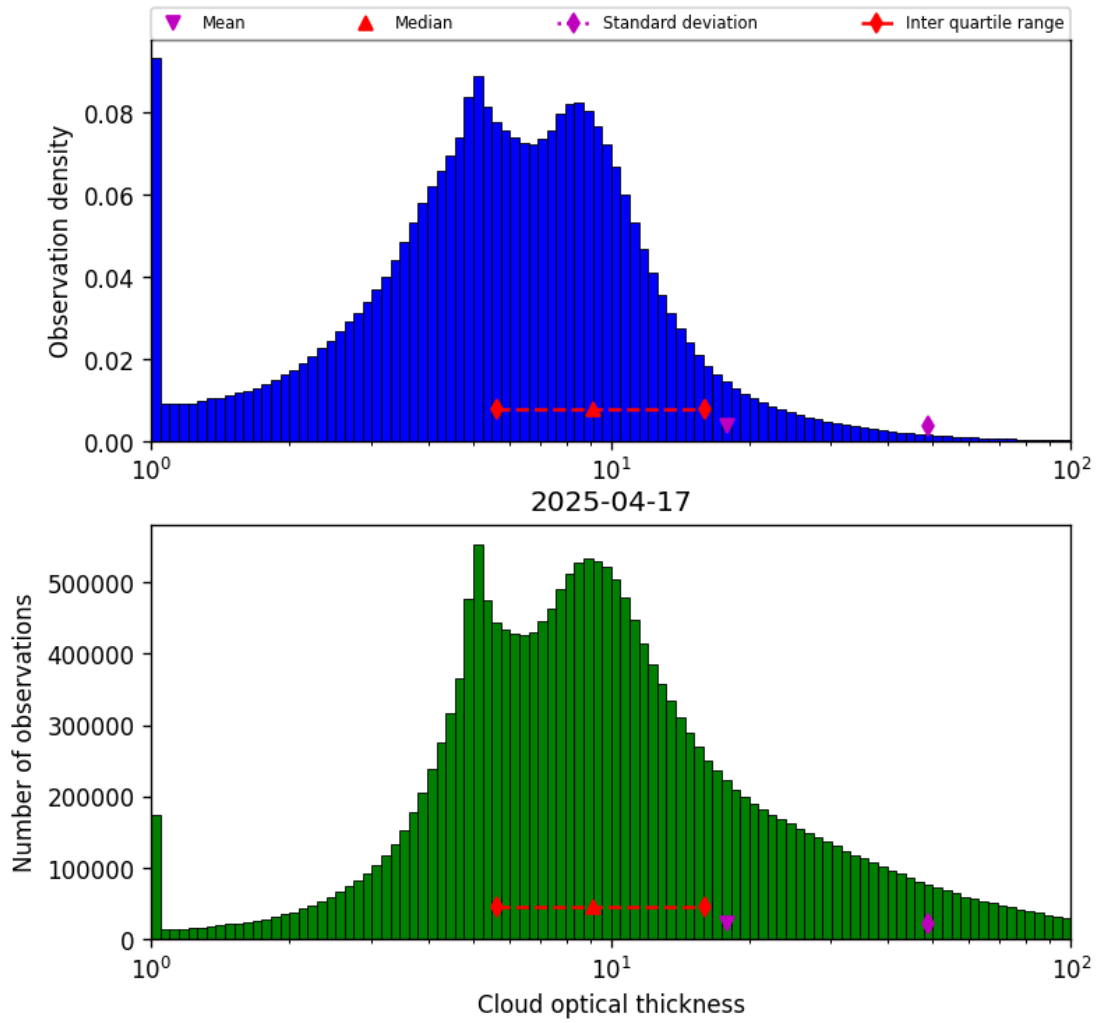
Figure 39: Histogram of “Cloud optical thickness” for 2025-04-17 to 2025-04-18
