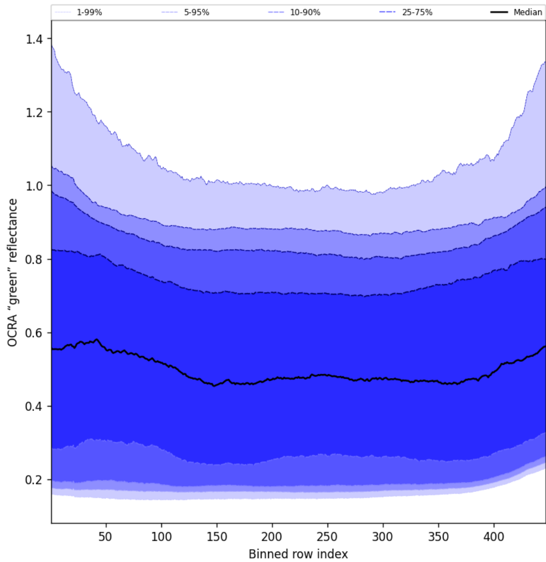
Figure 66: Along track statistics of “OCRA “green” reflectance” for 2025-04-17 to 2025-04-18
