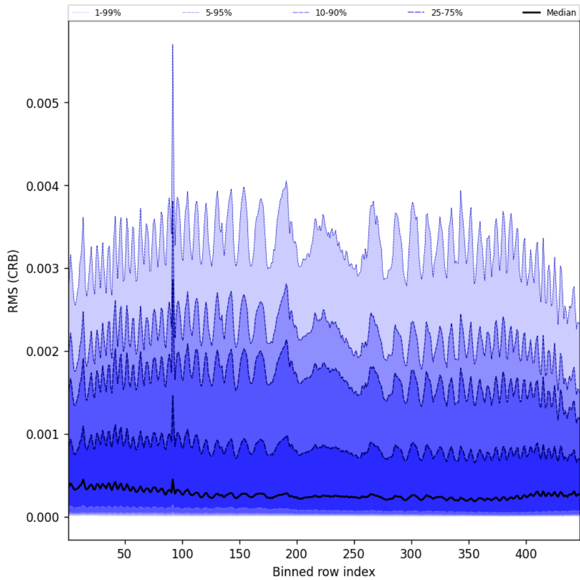
Figure 62: Along track statistics of “RMS (CRB)” for 2025-04-17 to 2025-04-18
