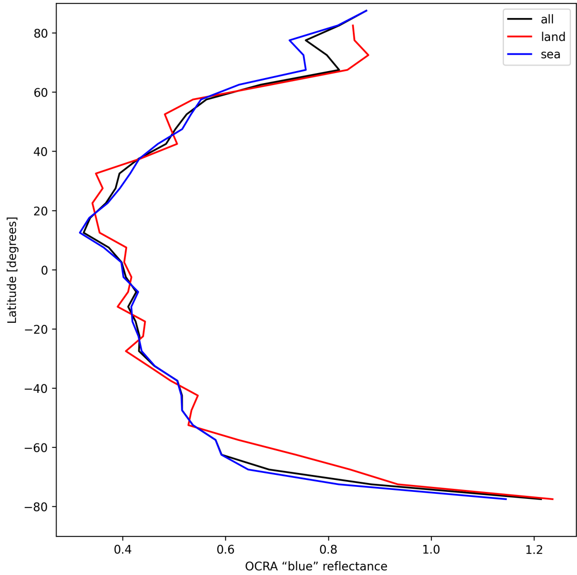
Figure 33: Zonal average of “OCRA “blue” reflectance” for 2025-04-17 to 2025-04-18.
