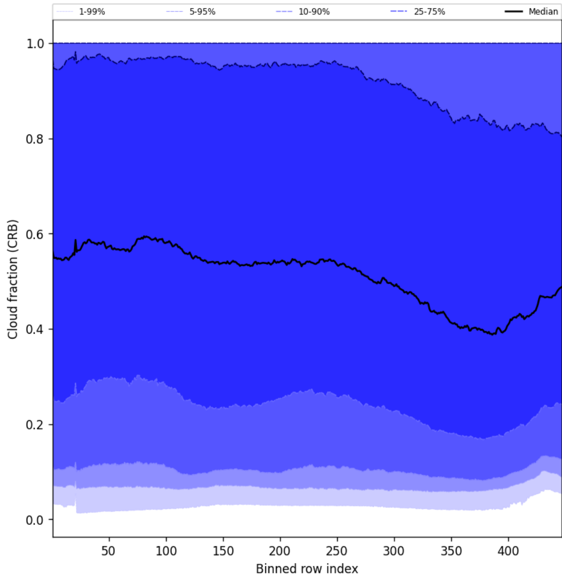
Figure 56: Along track statistics of “Cloud fraction (CRB)” for 2025-04-17 to 2025-04-18
