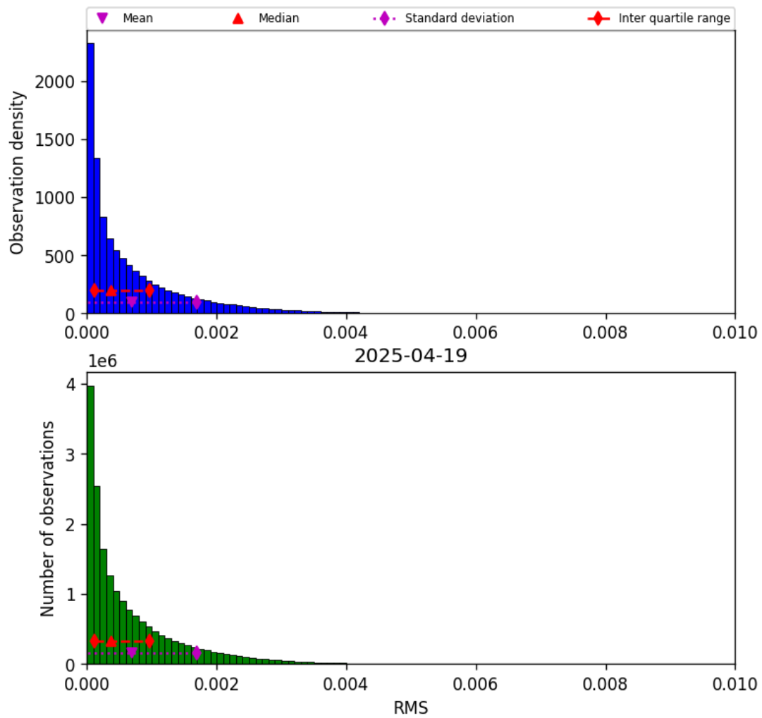
Figure 45: Histogram of “RMS” for 2025-04-19 to 2025-04-20
