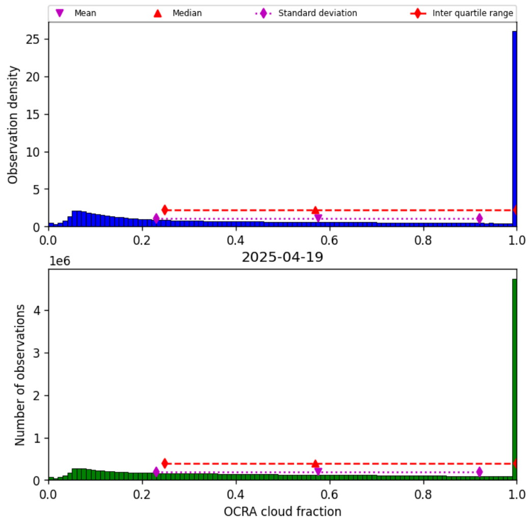
Figure 48: Histogram of “OCRA cloud fraction” for 2025-04-19 to 2025-04-20
