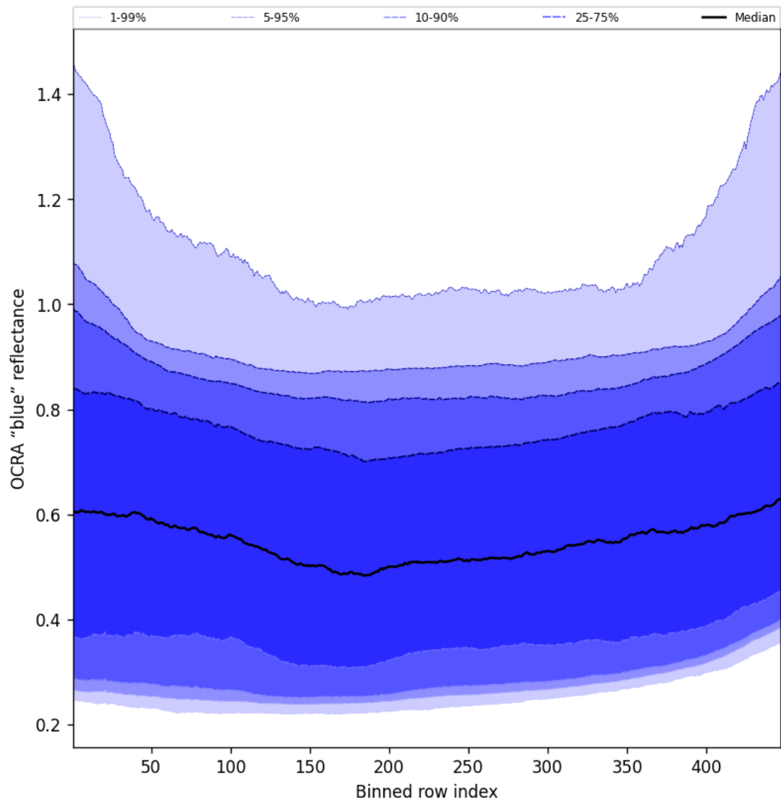
Figure 65: Along track statistics of “OCRA “blue” reflectance” for 2025-04-19 to 2025-04-20
