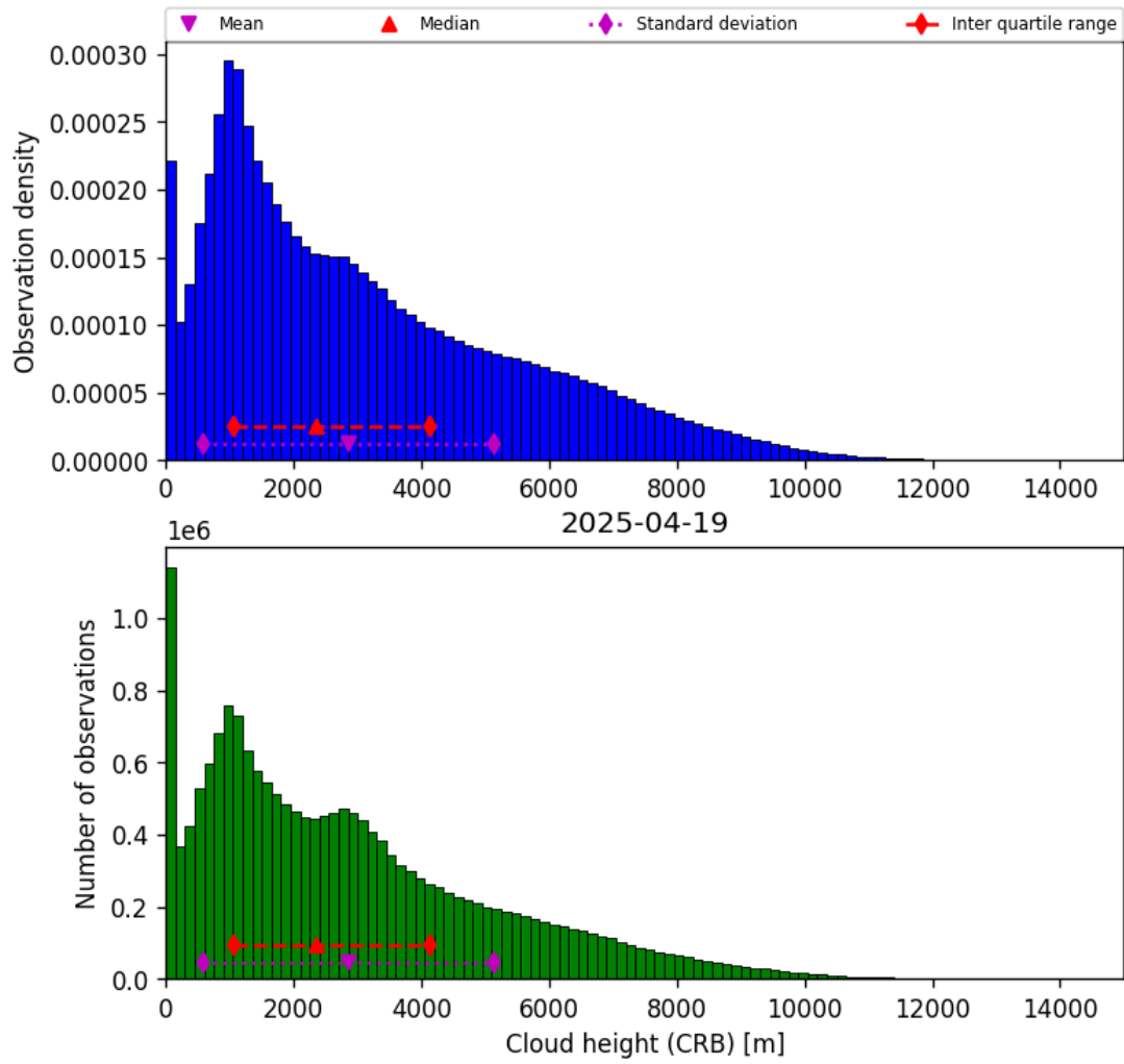
Figure 41: Histogram of “Cloud height (CRB)” for 2025-04-19 to 2025-04-20
