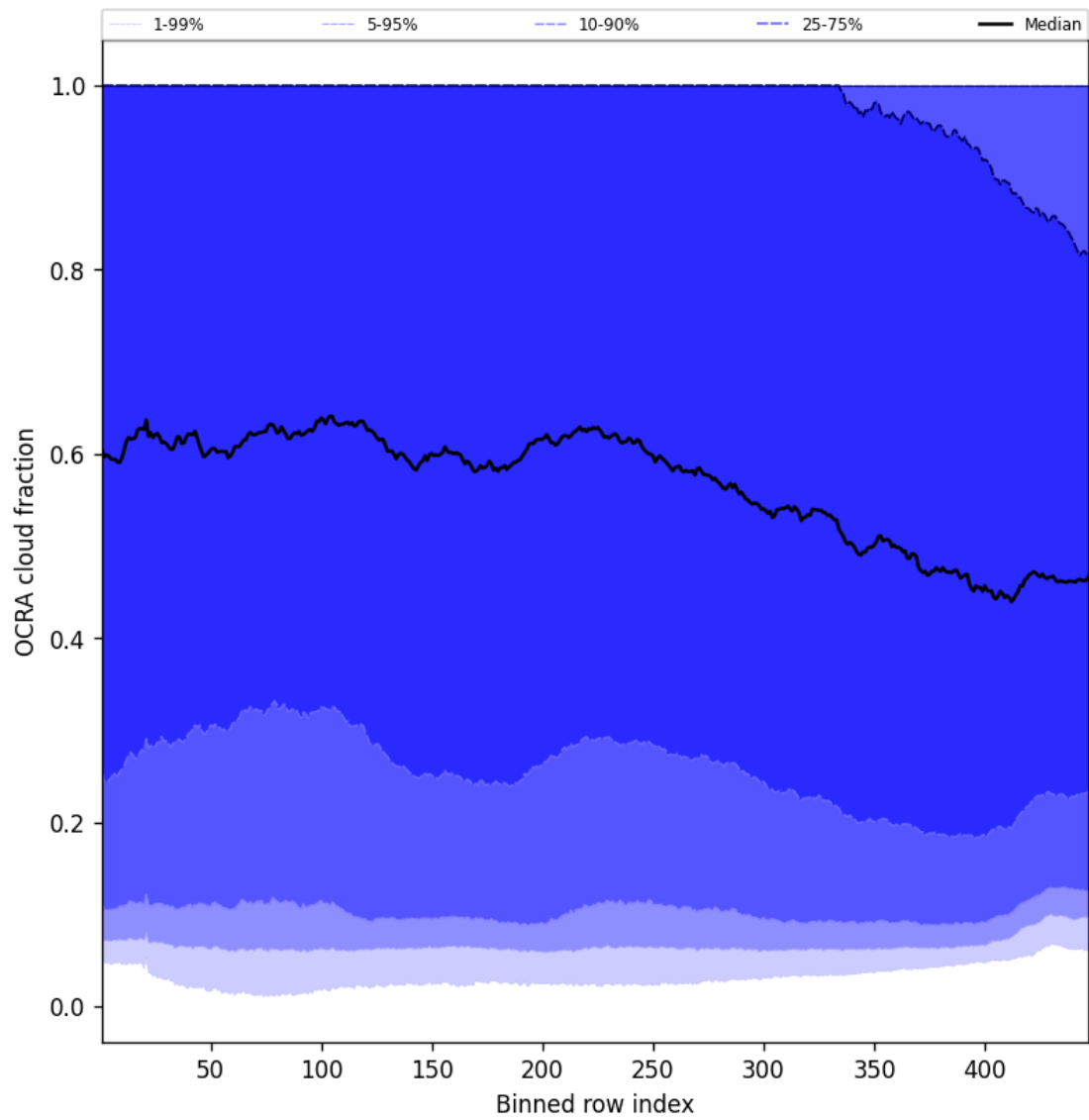
Figure 64: Along track statistics of “OCRA cloud fraction” for 2025-04-19 to 2025-04-20
