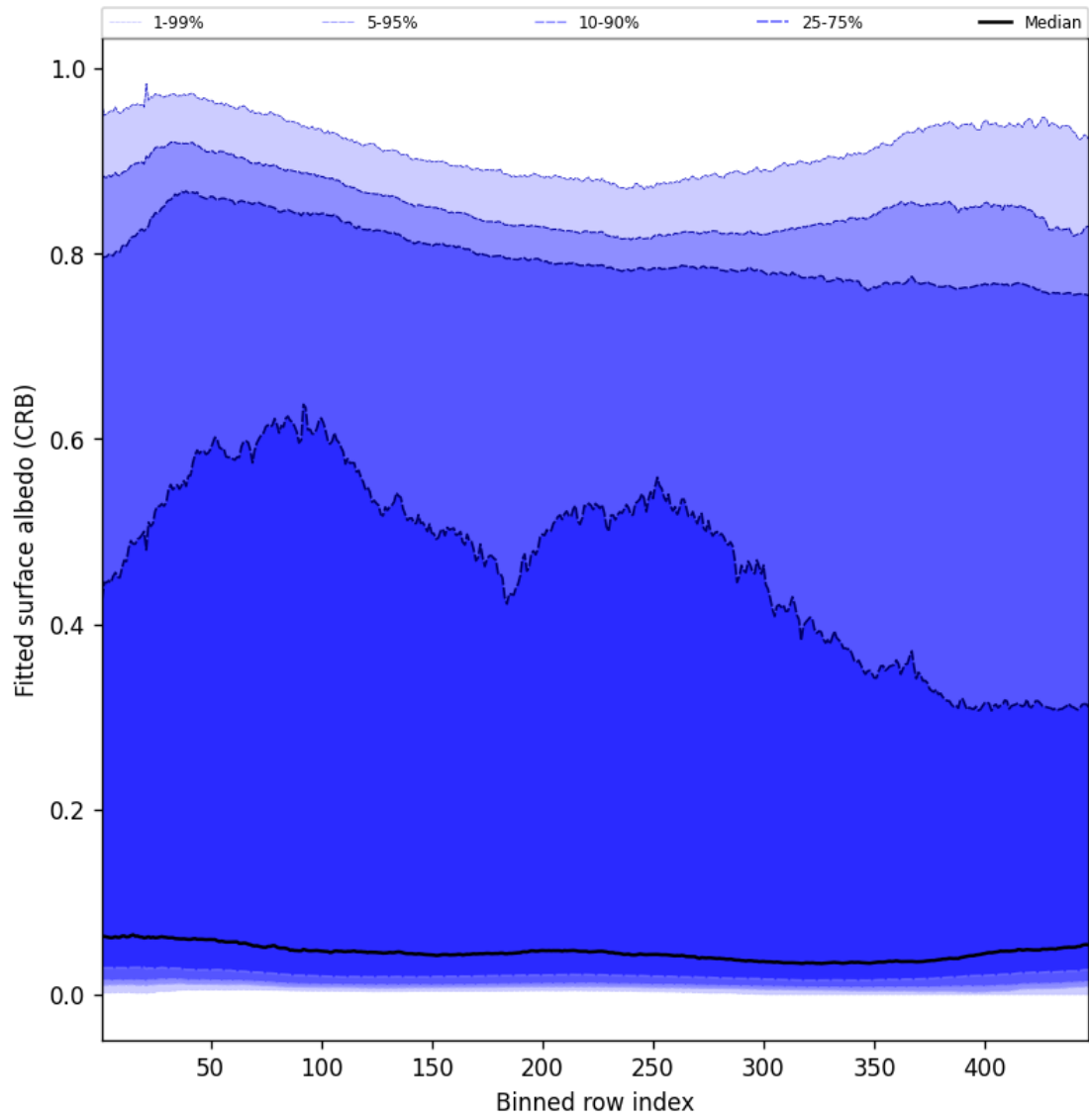
Figure 60: Along track statistics of “Fitted surface albedo (CRB)” for 2025-04-19 to 2025-04-20
