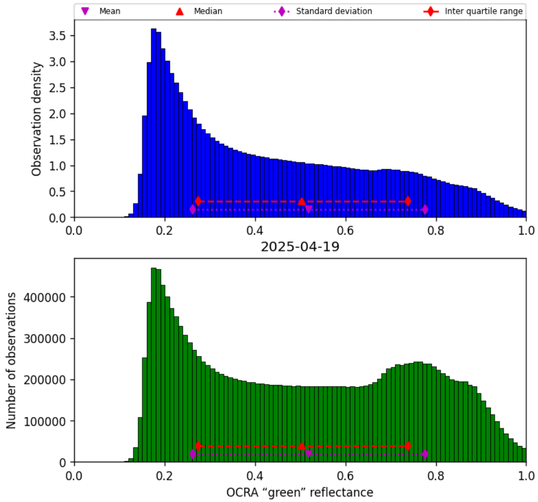
Figure 50: Histogram of “OCRA “green” reflectance” for 2025-04-19 to 2025-04-20
