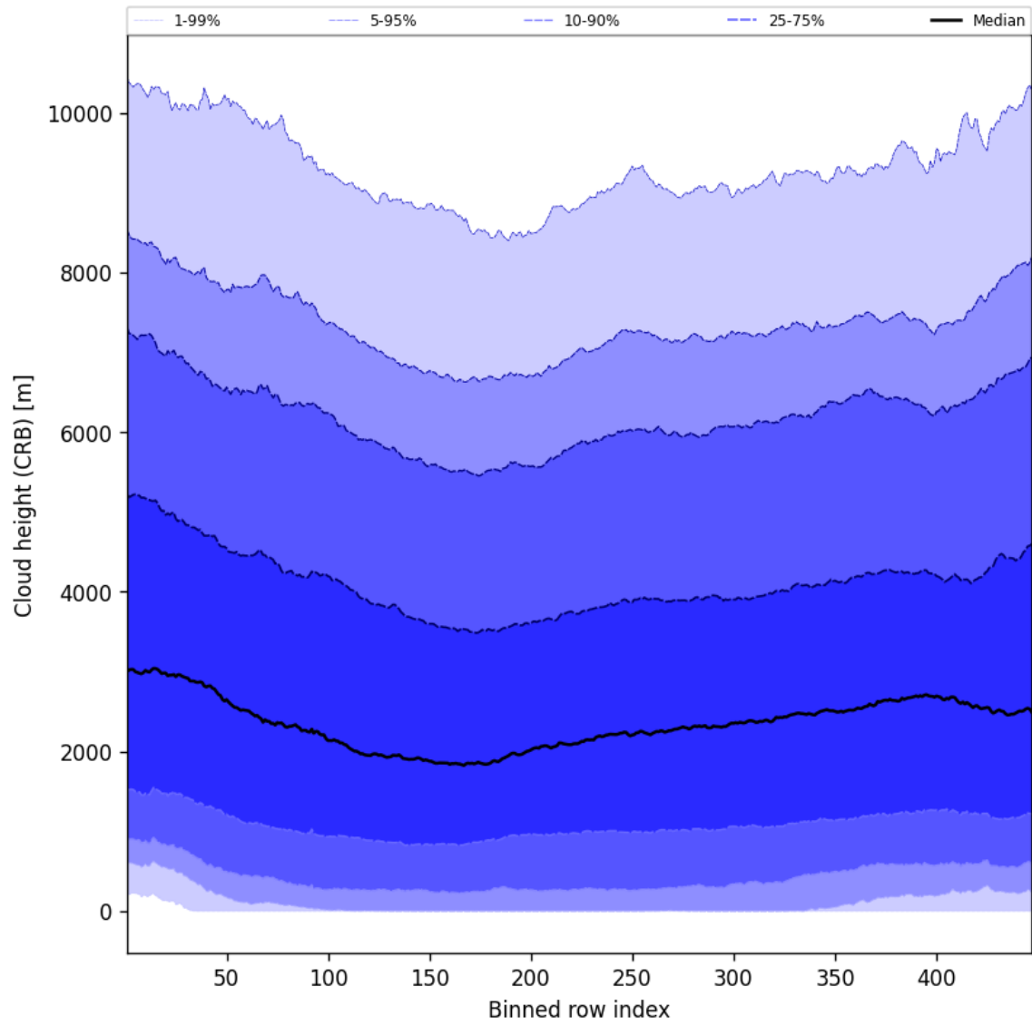
Figure 57: Along track statistics of “Cloud height (CRB)” for 2025-04-19 to 2025-04-20
