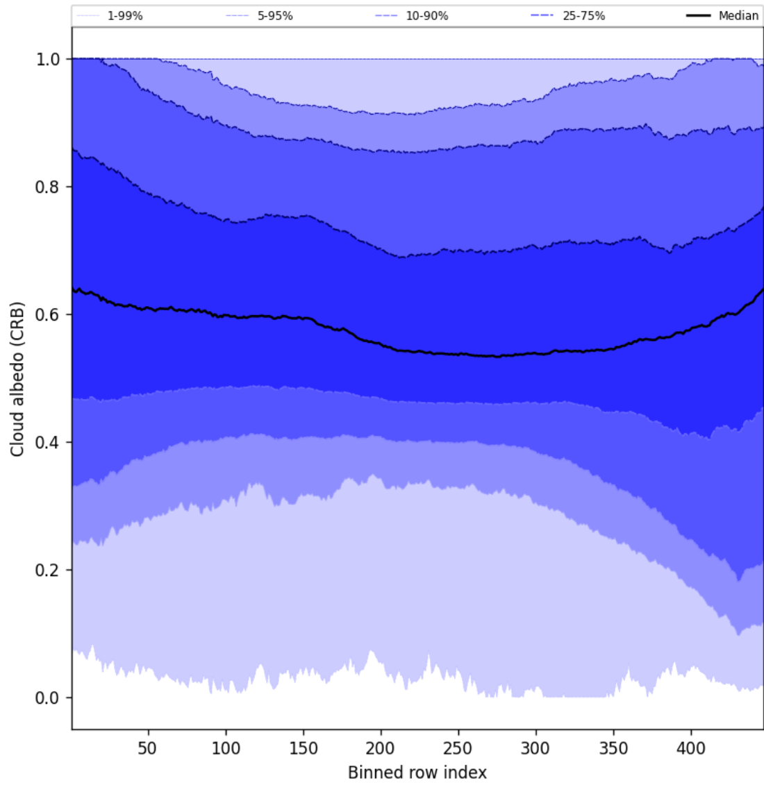
Figure 58: Along track statistics of “Cloud albedo (CRB)” for 2025-04-19 to 2025-04-20
