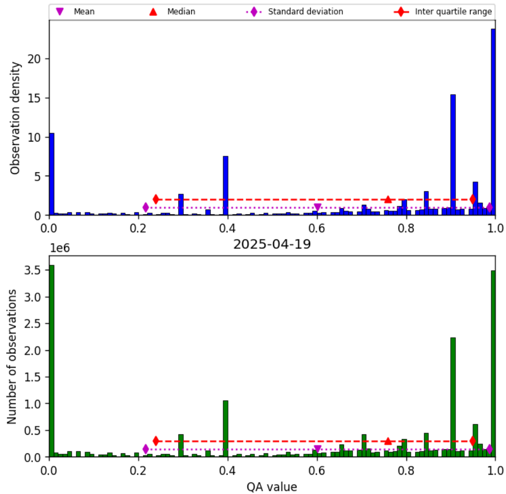
Figure 36: Histogram of “QA value” for 2025-04-19 to 2025-04-20
