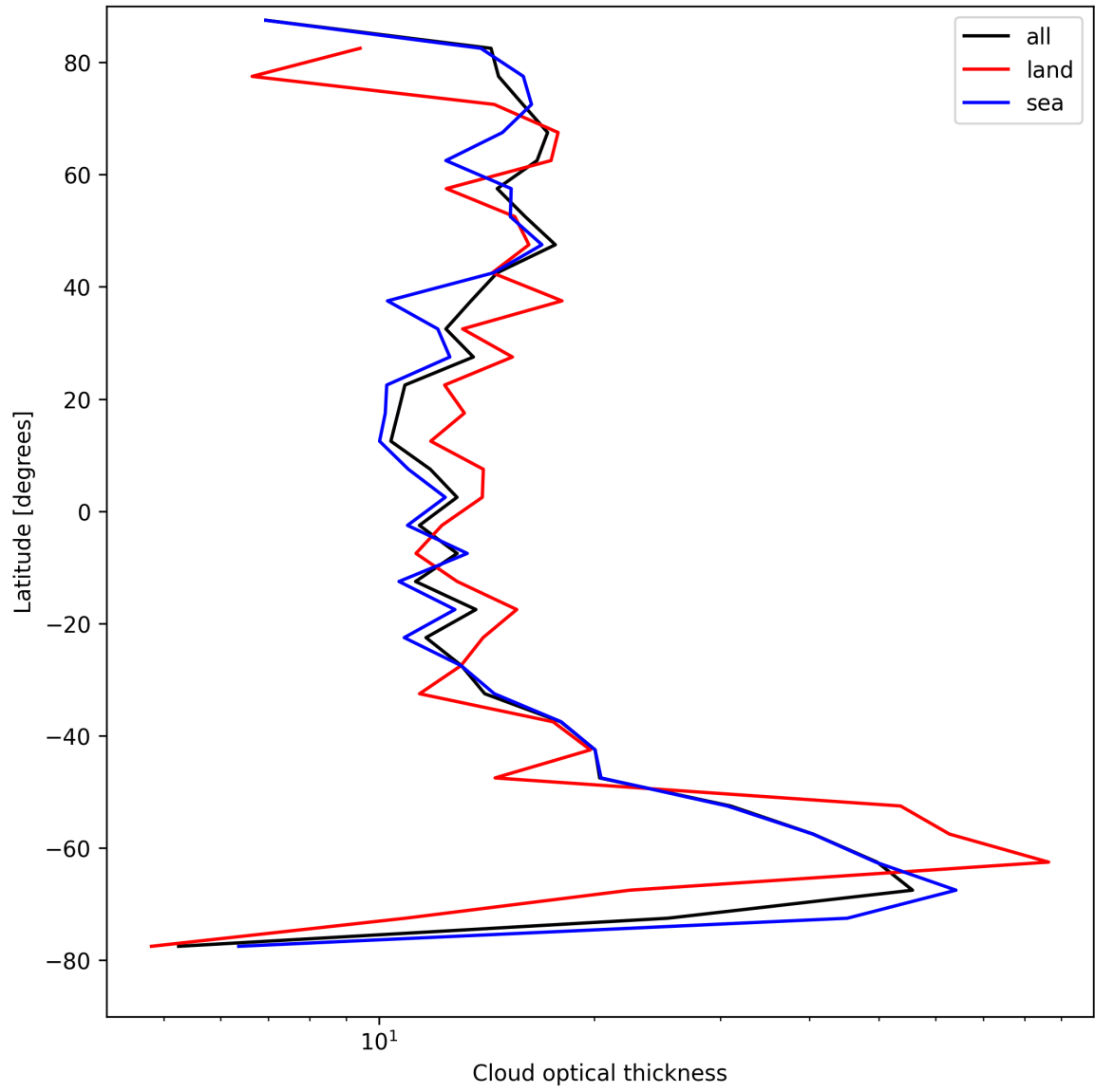
Figure 23: Zonal average of “Cloud optical thickness” for 2025-04-19 to 2025-04-20.
