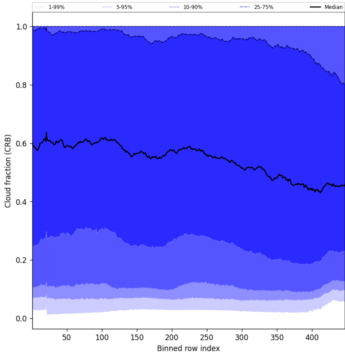
Figure 56: Along track statistics of “Cloud fraction (CRB)” for 2025-04-19 to 2025-04-20
