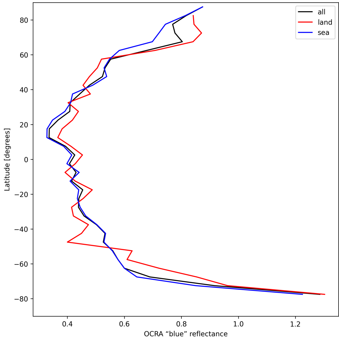
Figure 33: Zonal average of “OCRA “blue” reflectance” for 2025-04-19 to 2025-04-20.
