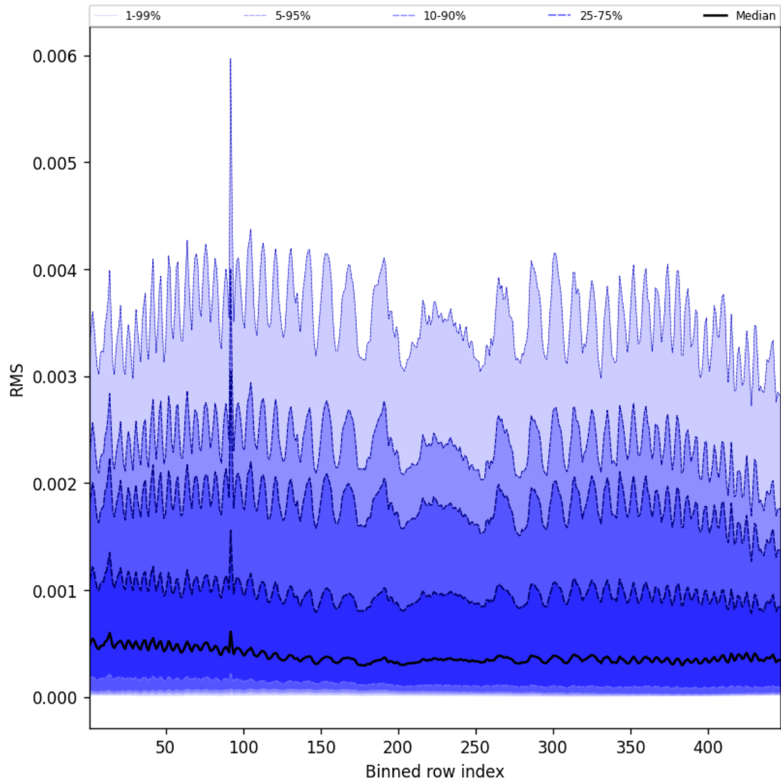
Figure 61: Along track statistics of “RMS” for 2025-04-19 to 2025-04-20
