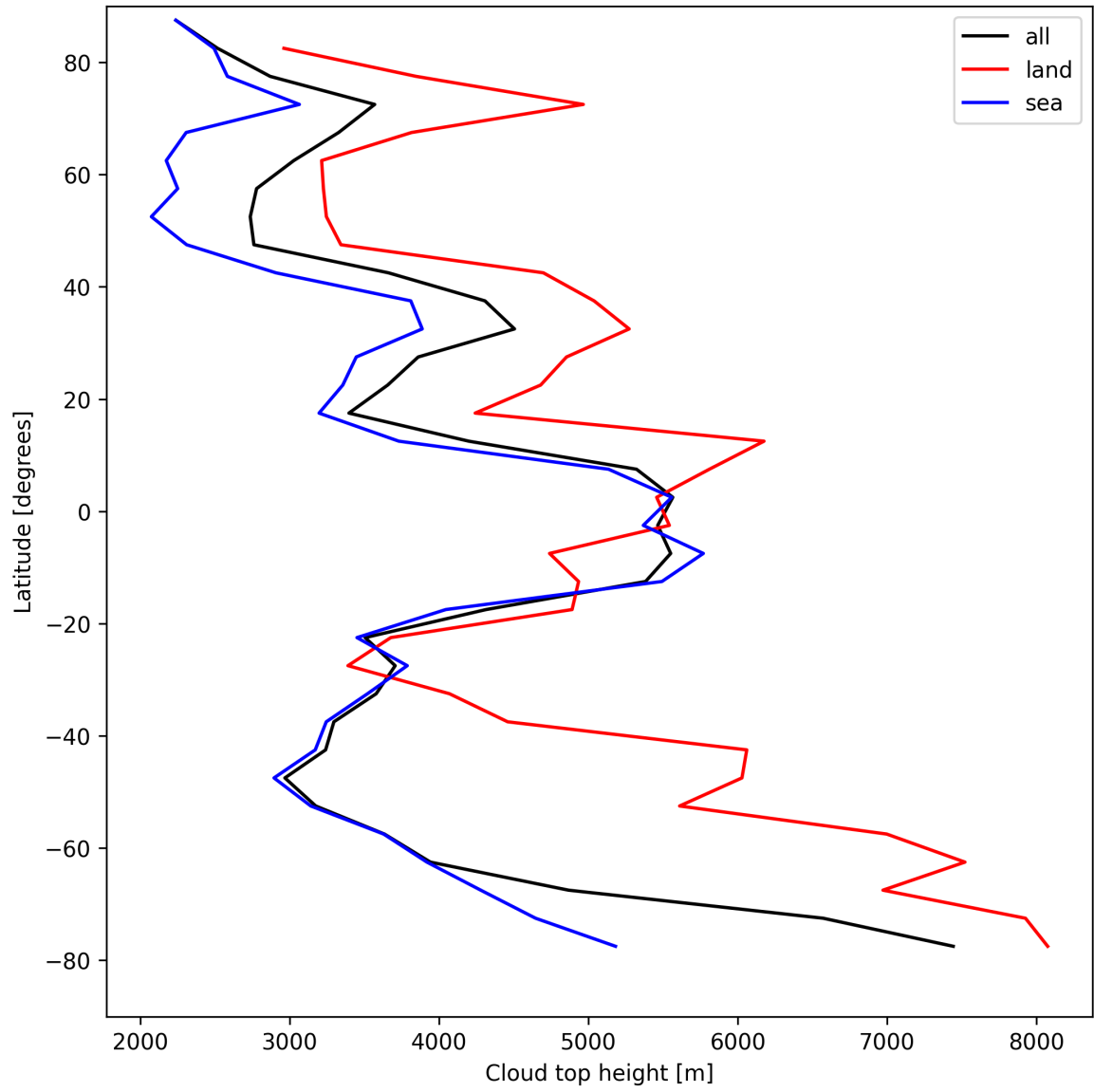
Figure 22: Zonal average of “Cloud top height” for 2025-04-19 to 2025-04-20.
