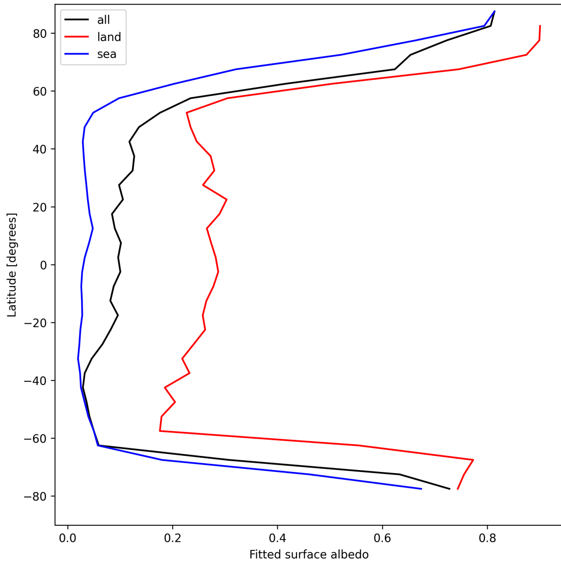
Figure 27: Zonal average of “Fitted surface albedo” for 2025-04-19 to 2025-04-20.
