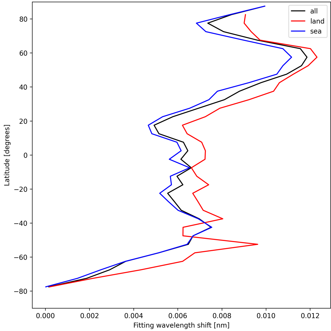
Figure 31: Zonal average of “Fitting wavelength shift” for 2025-04-19 to 2025-04-20.
