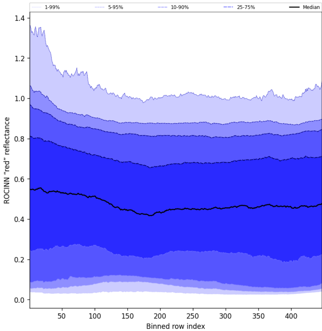
Figure 67: Along track statistics of "ROCINN "red" reflectance" for 2025-04-19 to 2025-04-20
