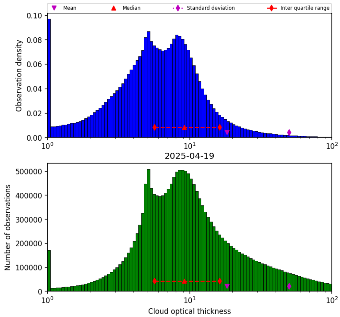
Figure 39: Histogram of “Cloud optical thickness” for 2025-04-19 to 2025-04-20
