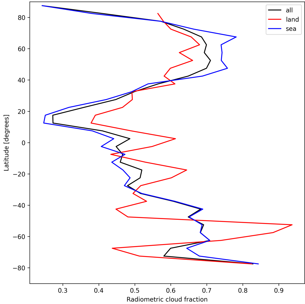
Figure 21: Zonal average of “Radiometric cloud fraction” for 2025-04-19 to 2025-04-20.
