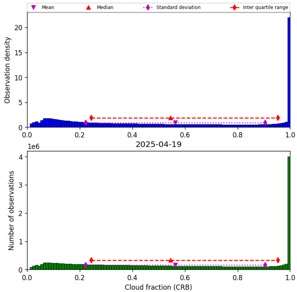
Figure 40: Histogram of “Cloud fraction (CRB)” for 2025-04-19 to 2025-04-20
