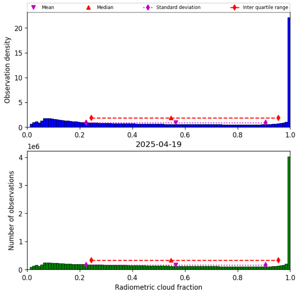
Figure 37: Histogram of “Radiometric cloud fraction” for 2025-04-19 to 2025-04-20
