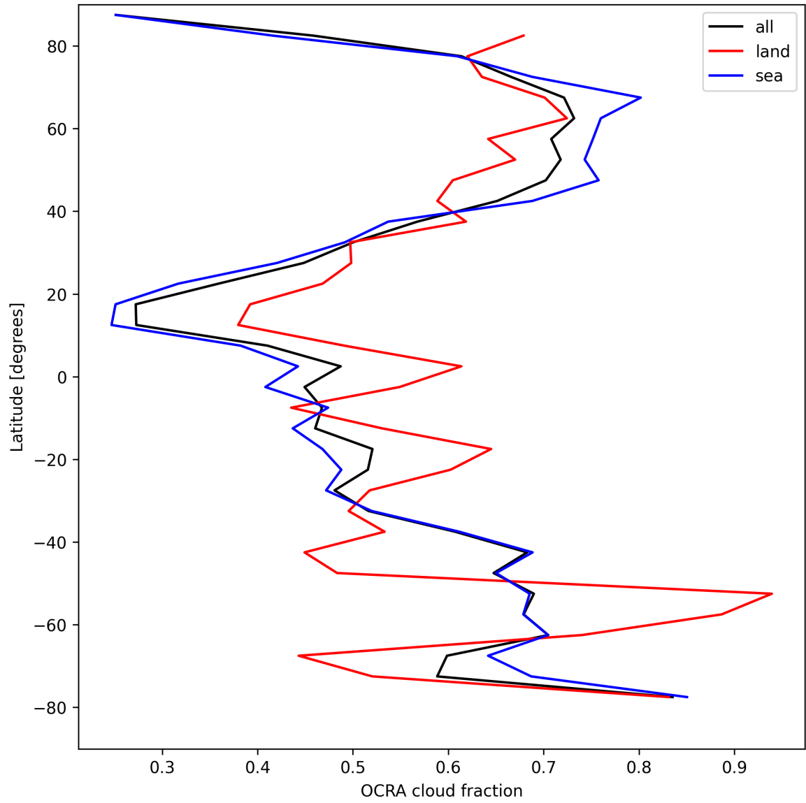
Figure 32: Zonal average of “OCRA cloud fraction” for 2025-04-19 to 2025-04-20.
