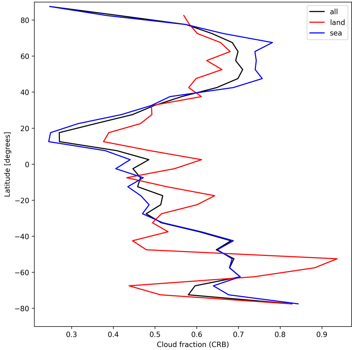
Figure 24: Zonal average of “Cloud fraction (CRB)” for 2025-04-19 to 2025-04-20.
