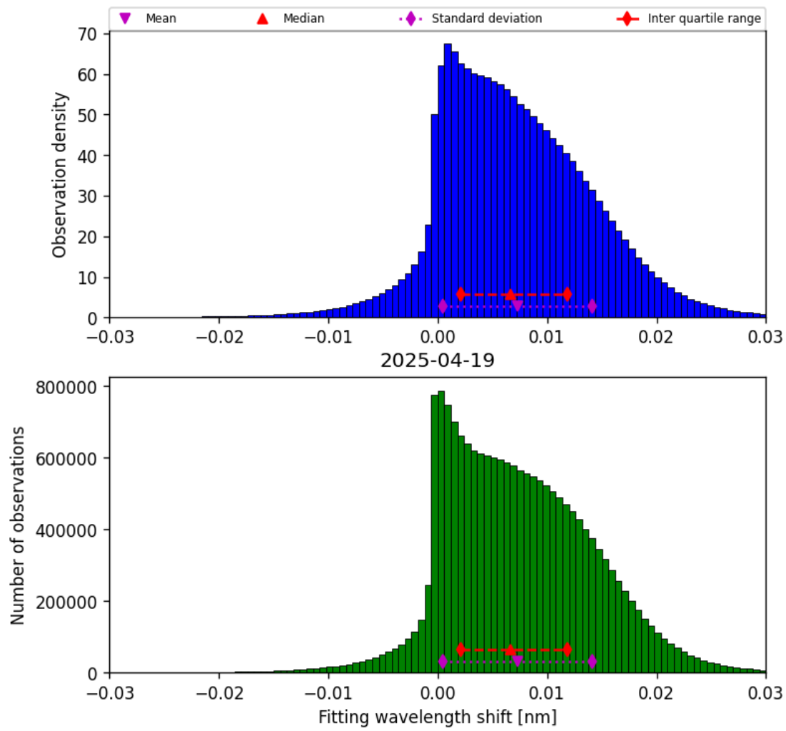
Figure 47: Histogram of “Fitting wavelength shift” for 2025-04-19 to 2025-04-20
