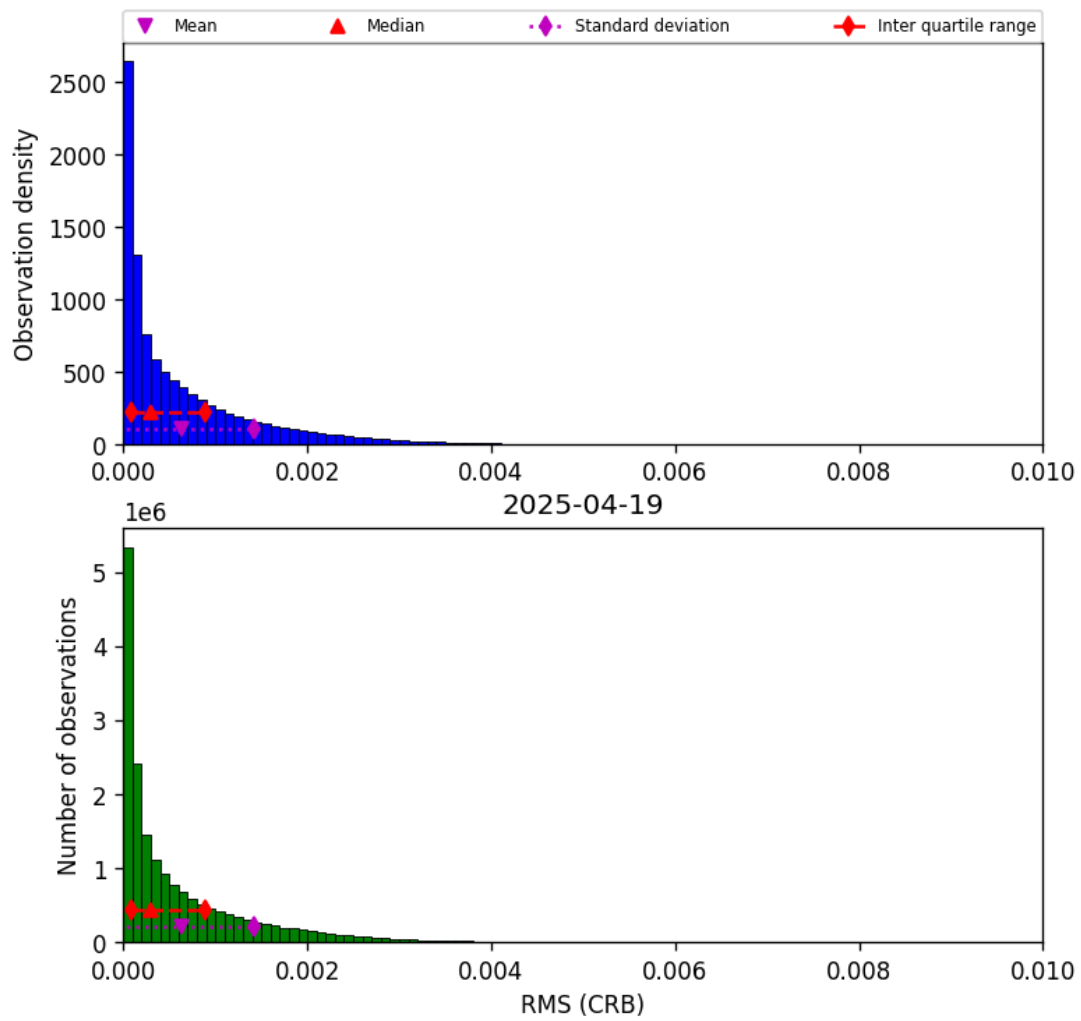
Figure 46: Histogram of "RMS (CRB)" for 2025-04-19 to 2025-04-20
