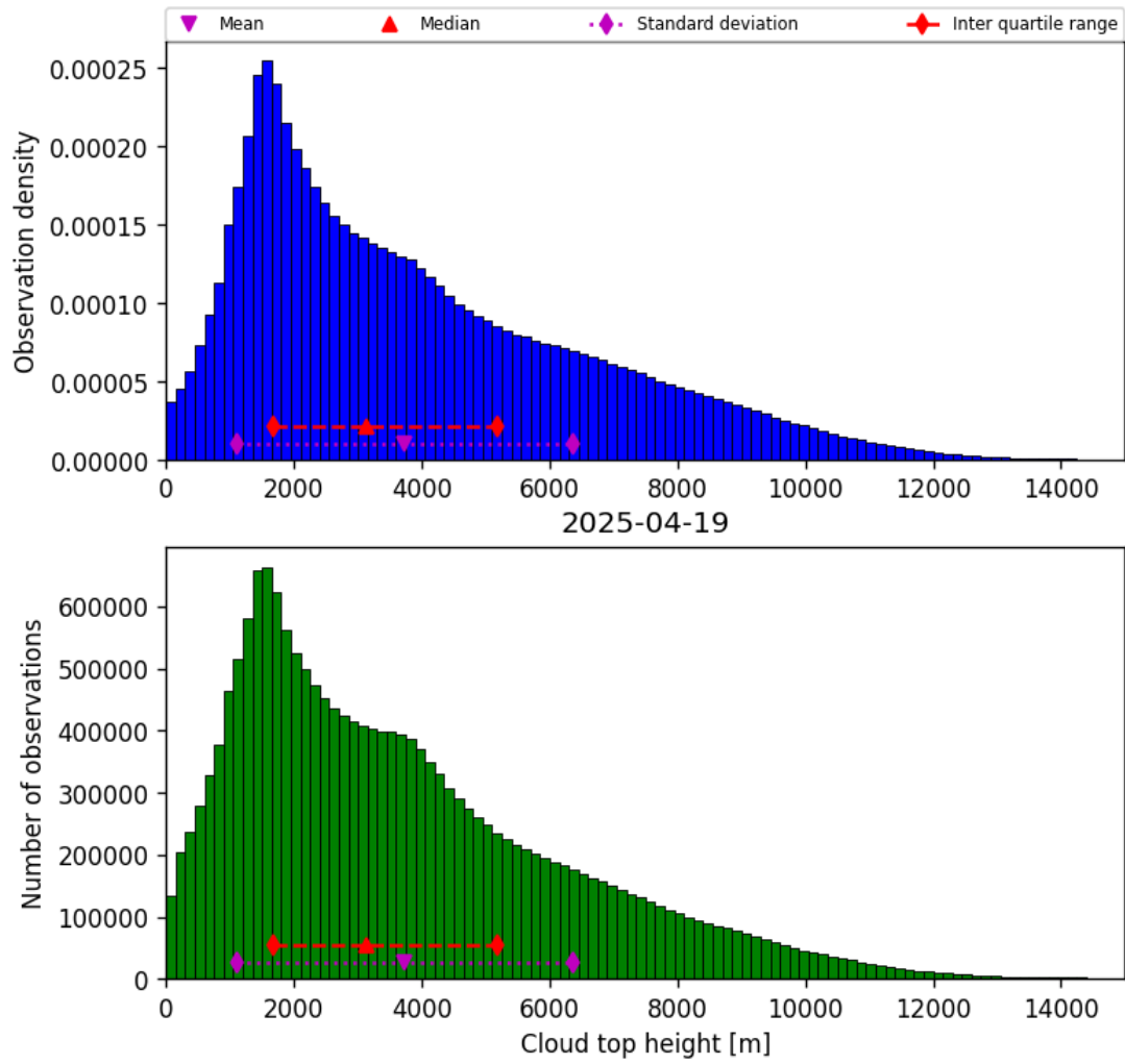
Figure 38: Histogram of “Cloud top height” for 2025-04-19 to 2025-04-20
