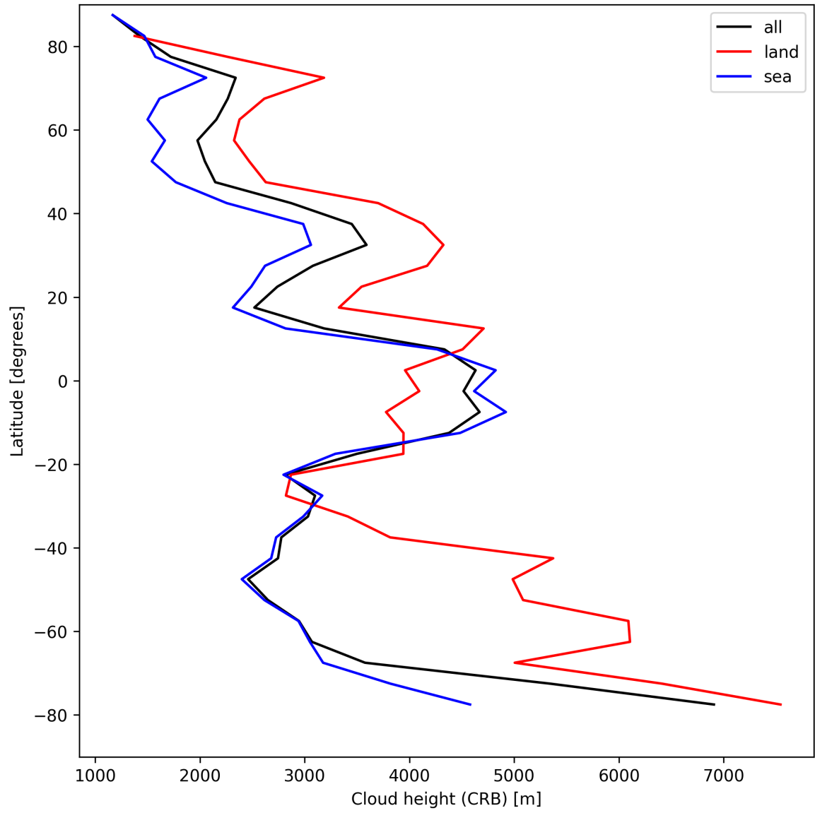
Figure 25: Zonal average of “Cloud height (CRB)” for 2025-04-19 to 2025-04-20.
