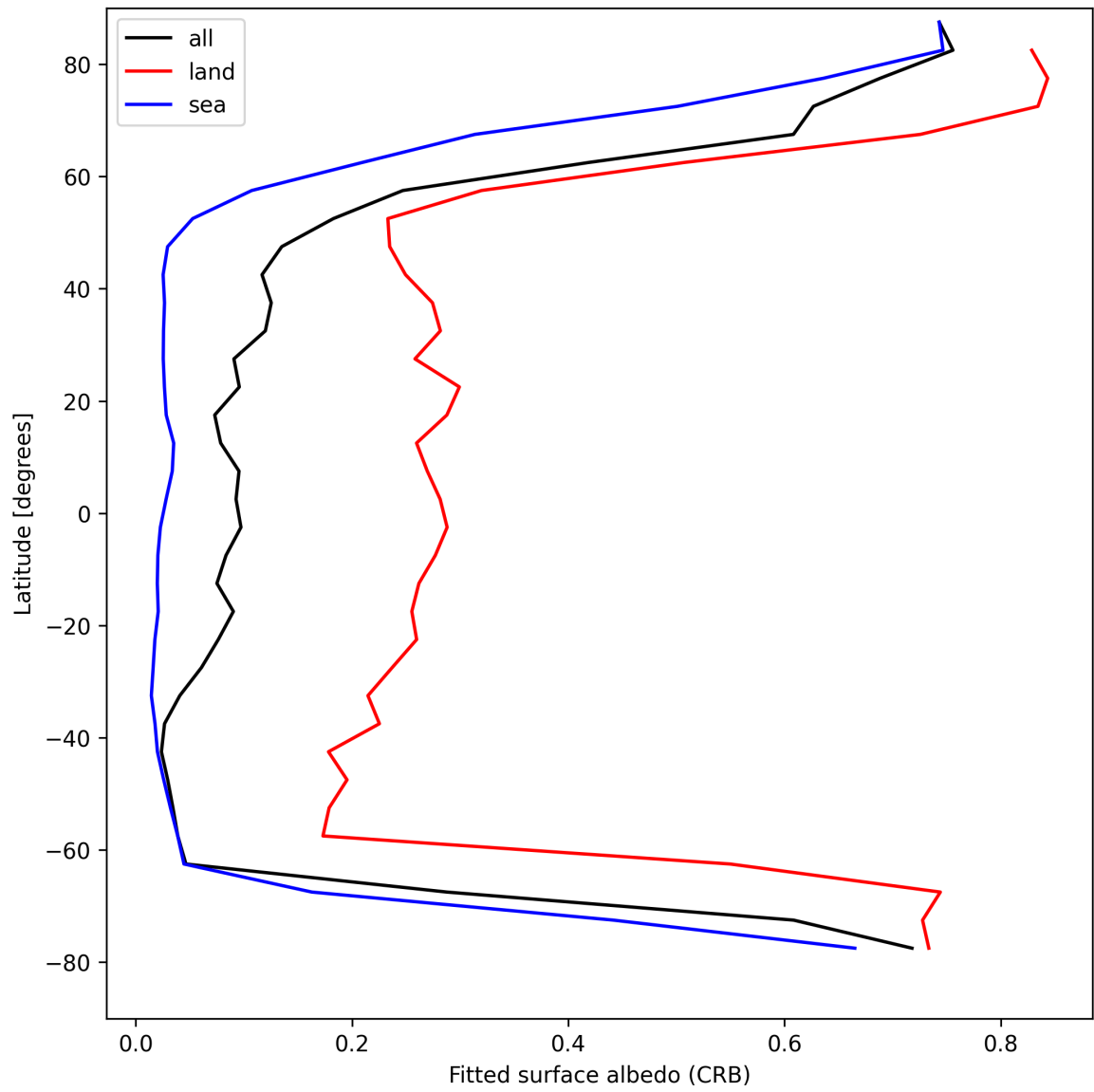
Figure 28: Zonal average of “Fitted surface albedo (CRB)” for 2025-04-19 to 2025-04-20.
