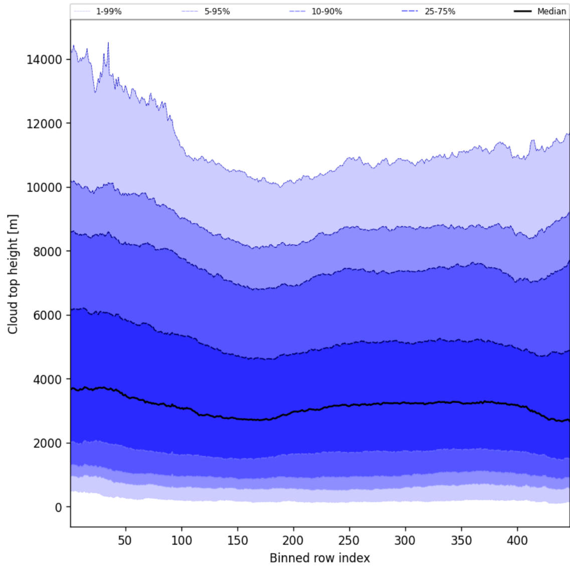
Figure 54: Along track statistics of “Cloud top height” for 2025-04-19 to 2025-04-20
