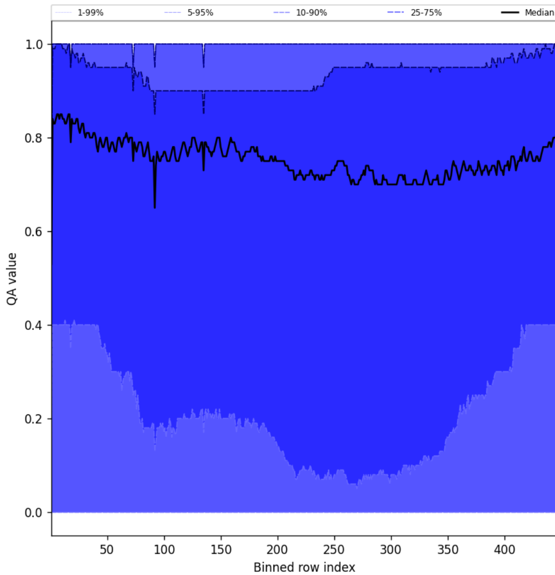
Figure 52: Along track statistics of “QA value” for 2025-04-19 to 2025-04-20
