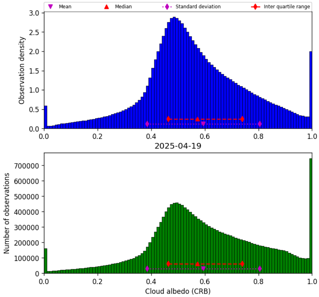
Figure 42: Histogram of “Cloud albedo (CRB)” for 2025-04-19 to 2025-04-20
