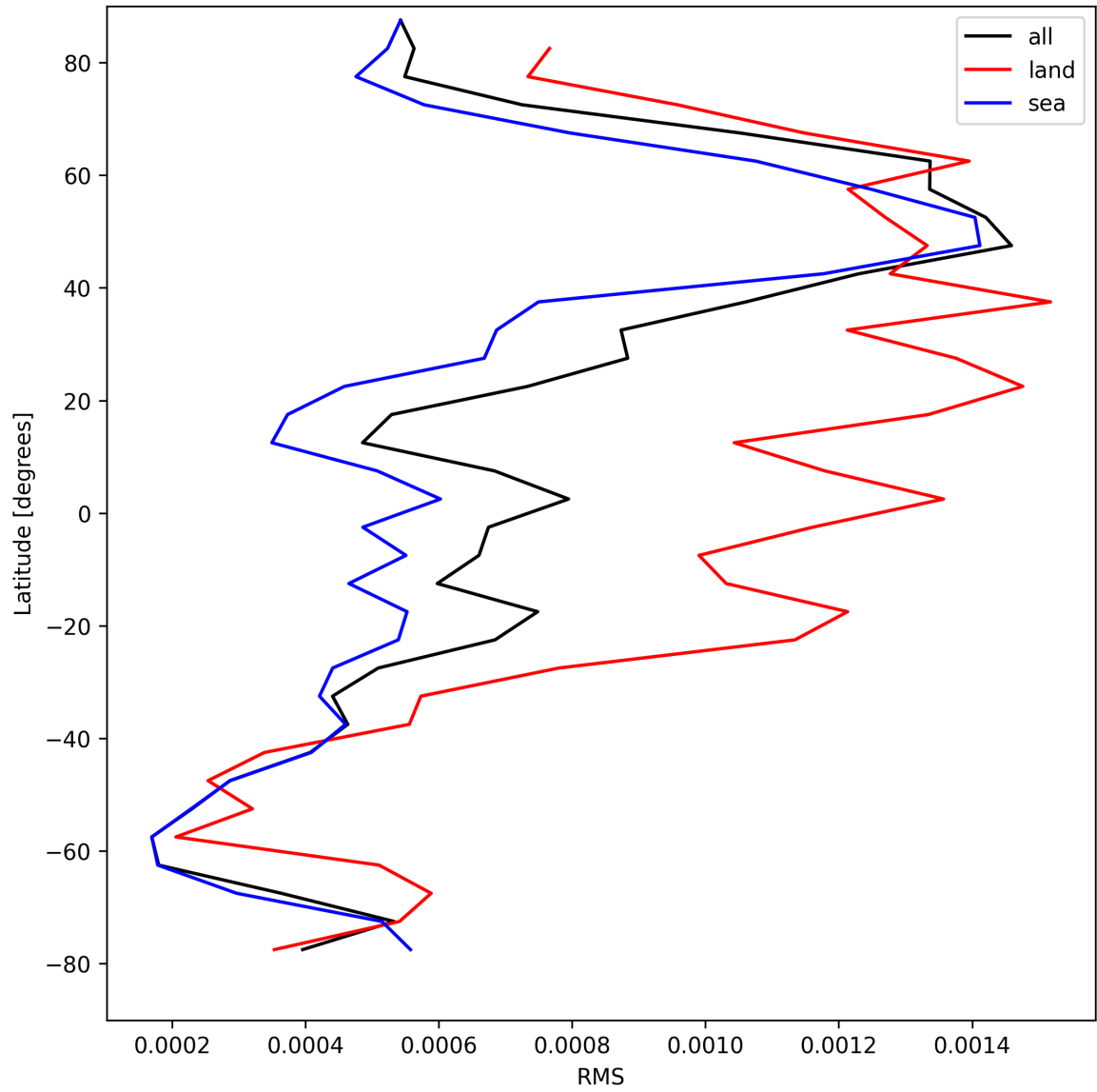
Figure 29: Zonal average of “RMS” for 2025-04-19 to 2025-04-20.
