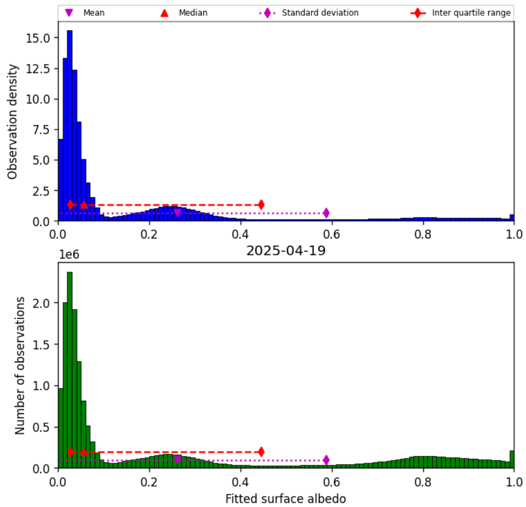
Figure 43: Histogram of “Fitted surface albedo” for 2025-04-19 to 2025-04-20
