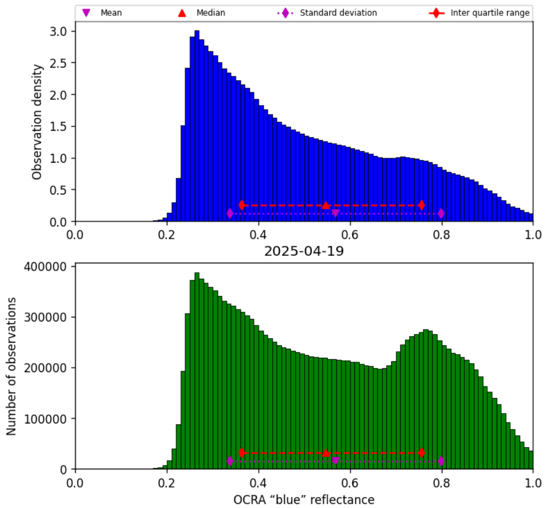
Figure 49: Histogram of “OCRA “blue” reflectance” for 2025-04-19 to 2025-04-20
