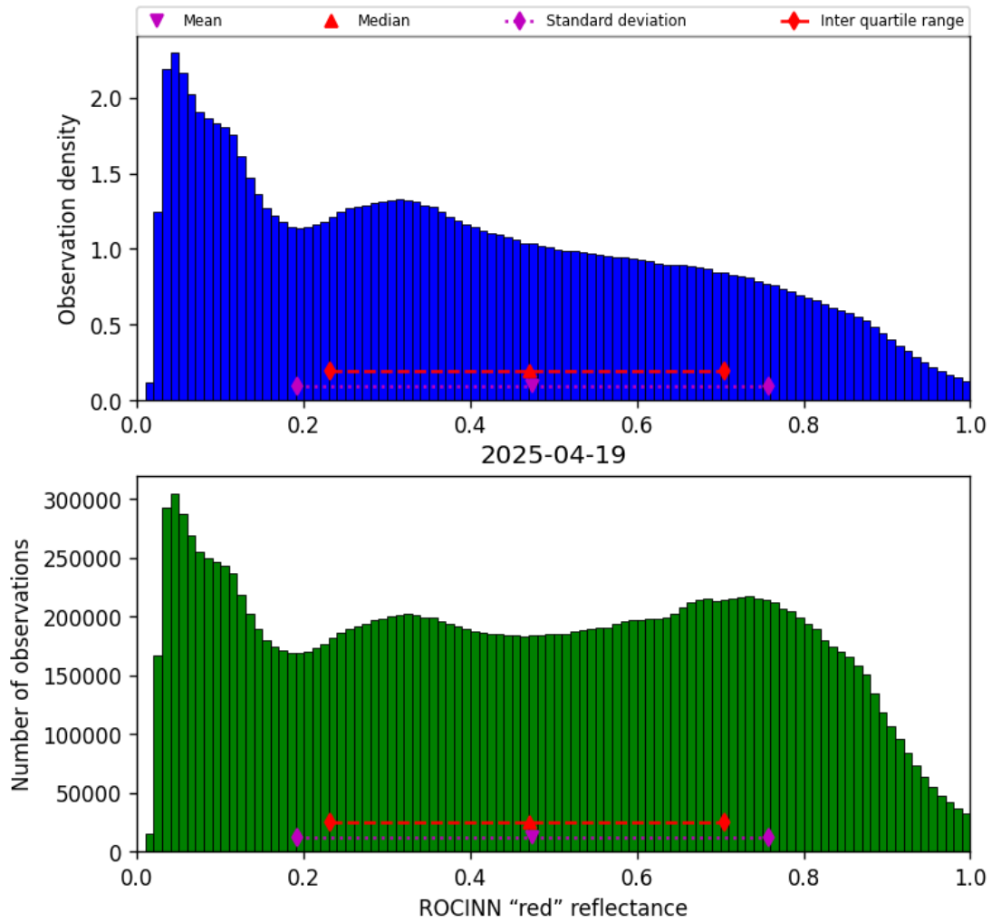
Figure 51: Histogram of “ROCINN “red” reflectance” for 2025-04-19 to 2025-04-20
