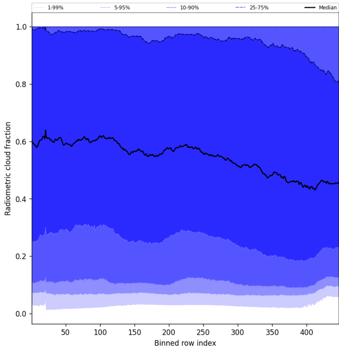
Figure 53: Along track statistics of “Radiometric cloud fraction” for 2025-04-19 to 2025-04-20
