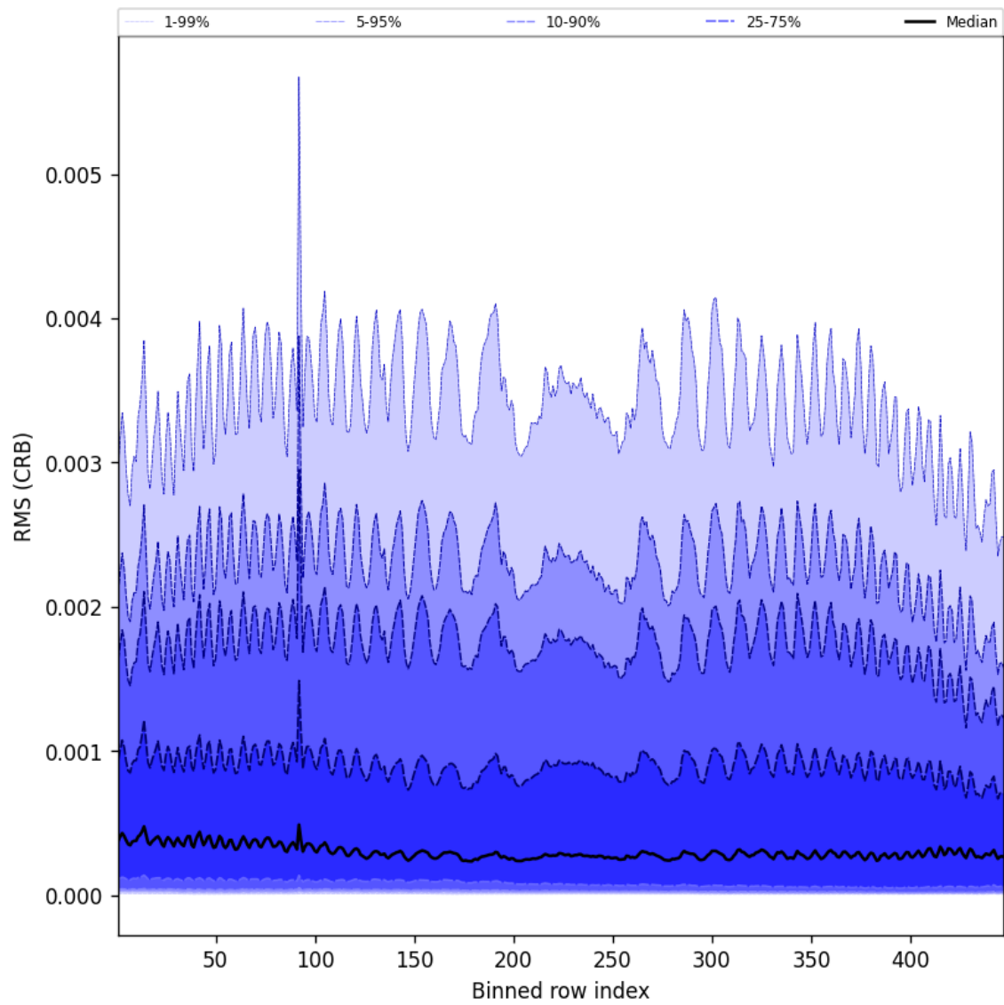
Figure 62: Along track statistics of “RMS (CRB)” for 2025-04-19 to 2025-04-20
