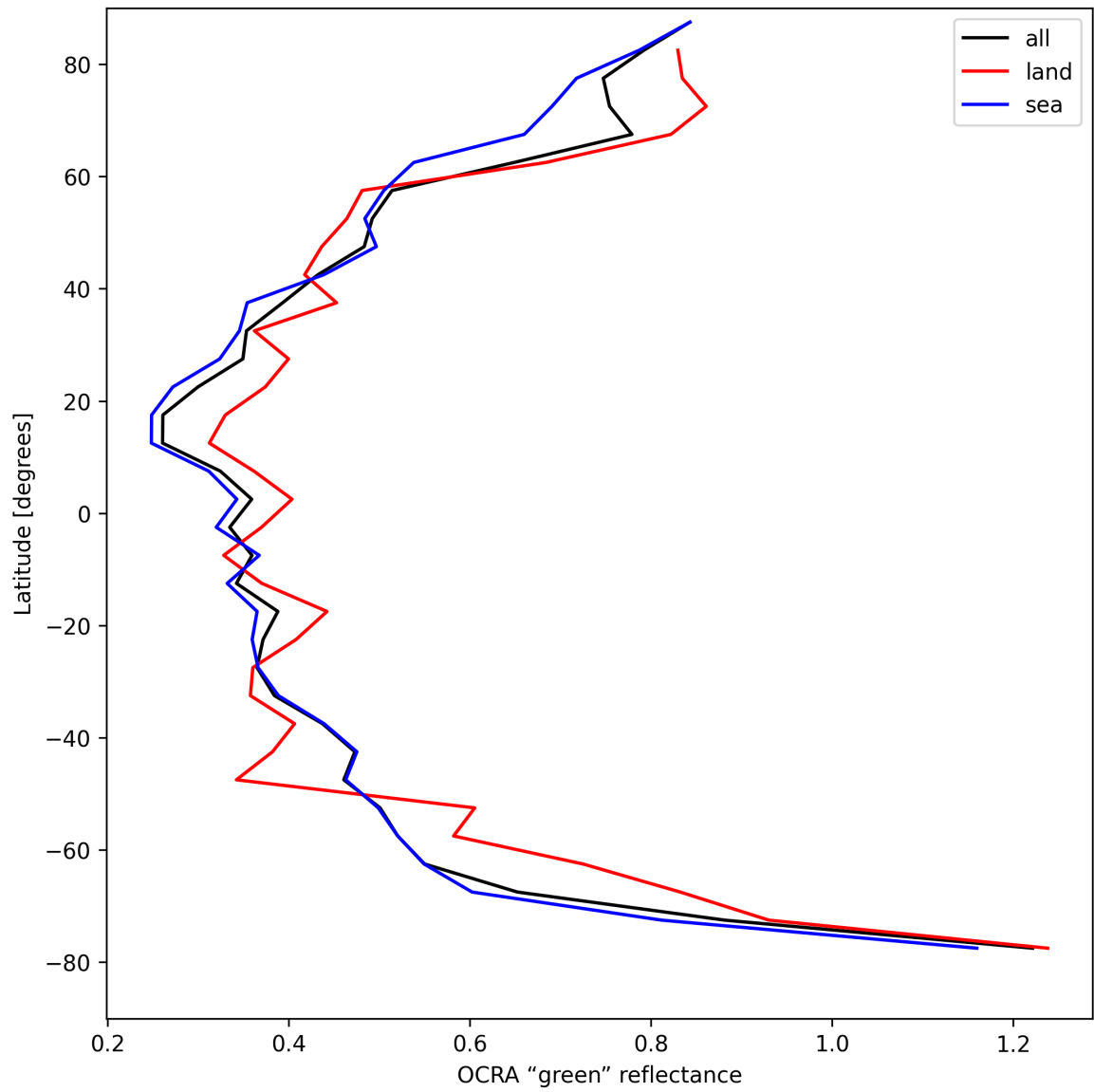
Figure 34: Zonal average of “OCRA “green” reflectance” for 2025-04-19 to 2025-04-20.
