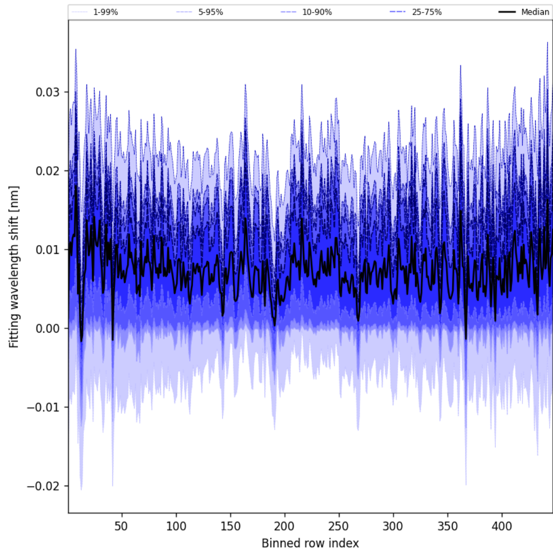
Figure 63: Along track statistics of “Fitting wavelength shift” for 2025-04-19 to 2025-04-20
