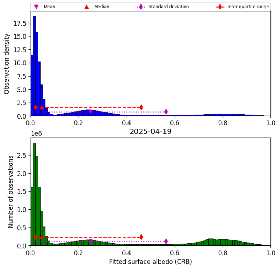
Figure 44: Histogram of “Fitted surface albedo (CRB)” for 2025-04-19 to 2025-04-20
