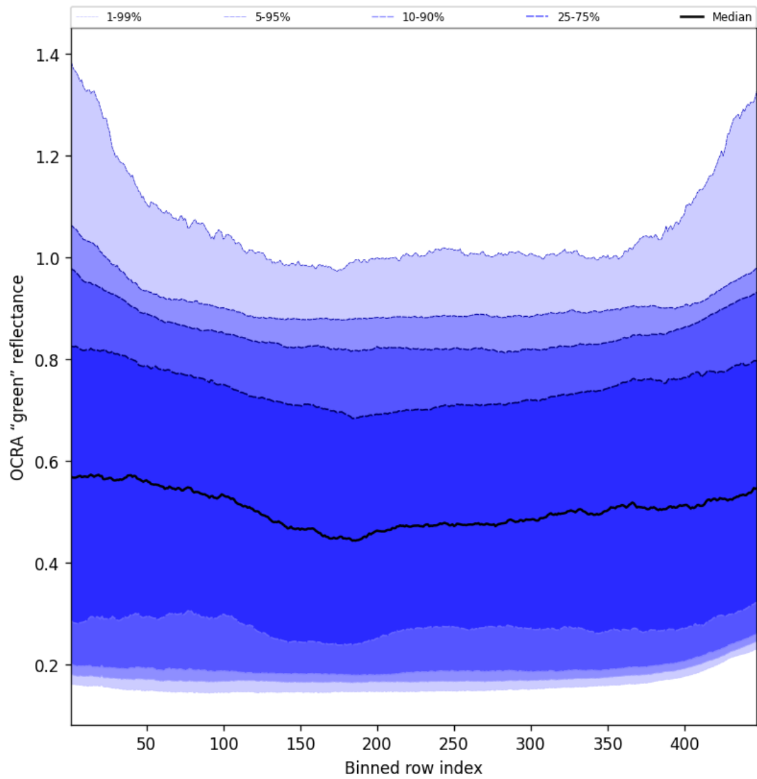
Figure 66: Along track statistics of “OCRA “green” reflectance” for 2025-04-19 to 2025-04-20
