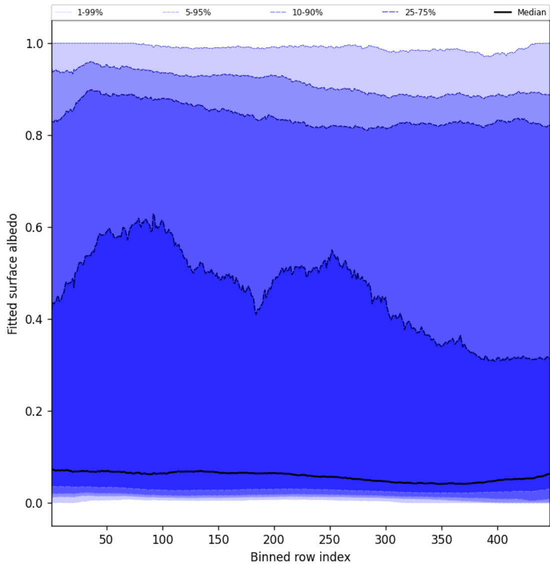
Figure 59: Along track statistics of “Fitted surface albedo” for 2025-04-19 to 2025-04-20
