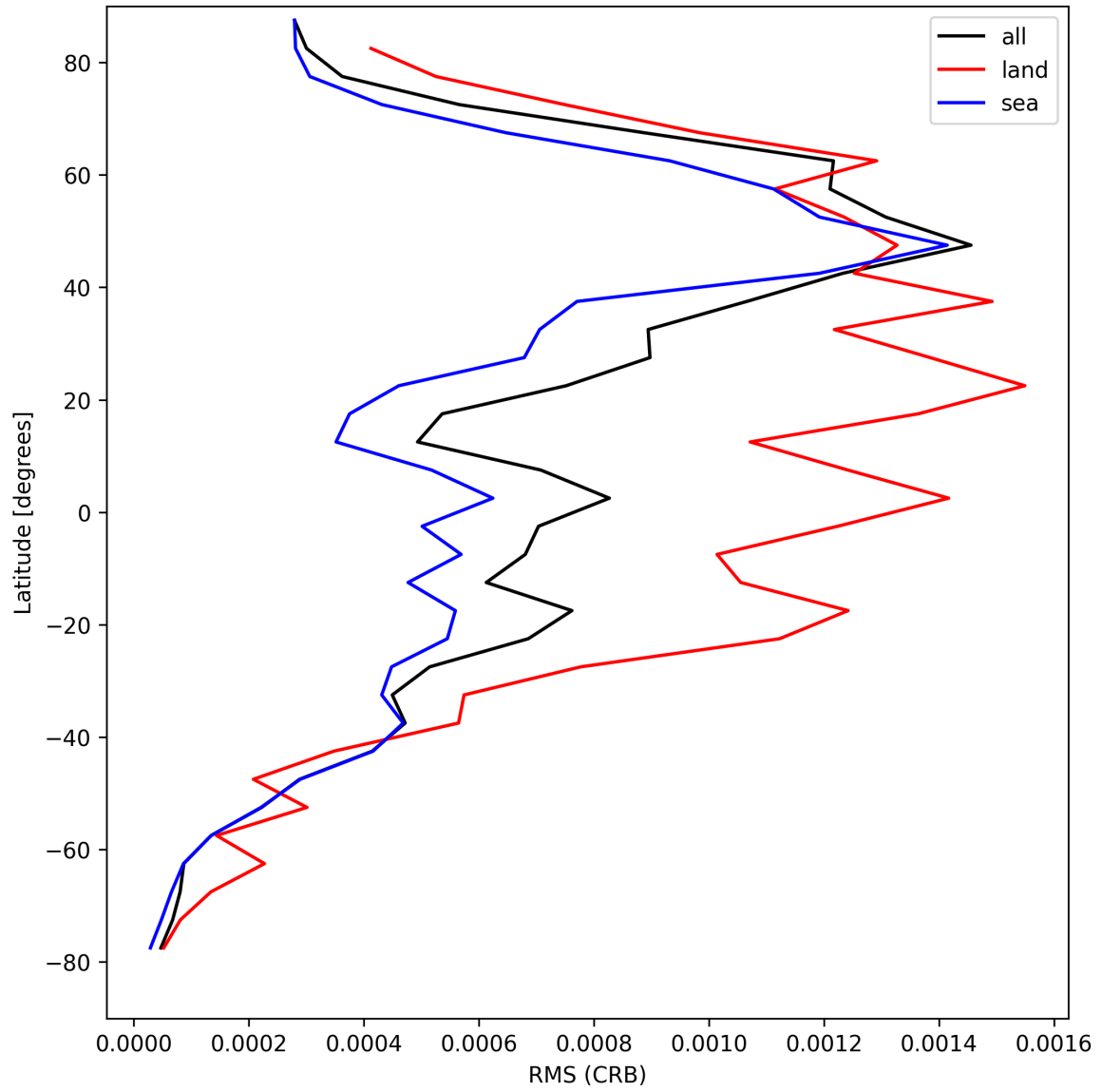
Figure 30: Zonal average of “RMS (CRB)” for 2025-04-19 to 2025-04-20.
