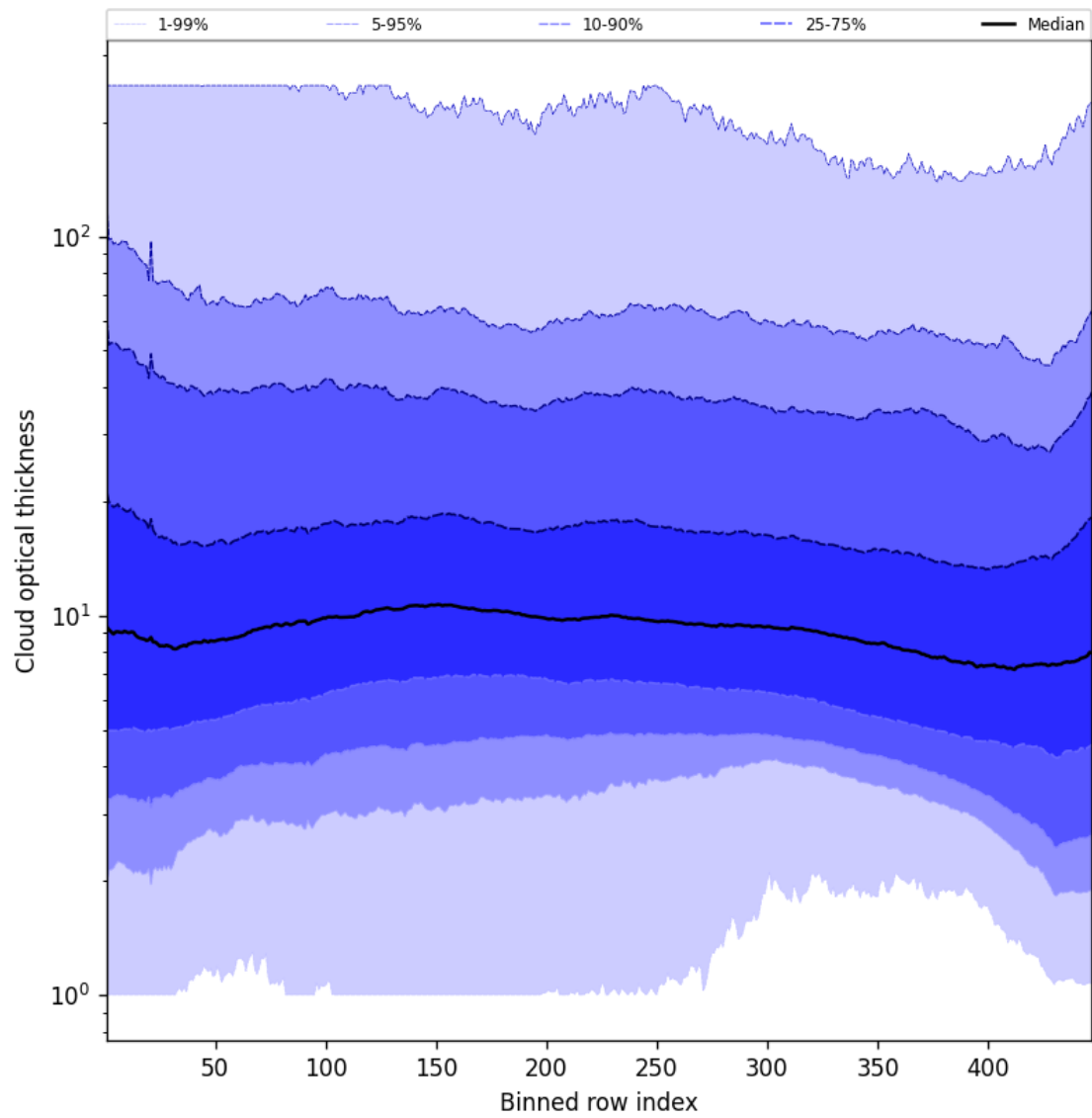
Figure 55: Along track statistics of “Cloud optical thickness” for 2025-04-19 to 2025-04-20
