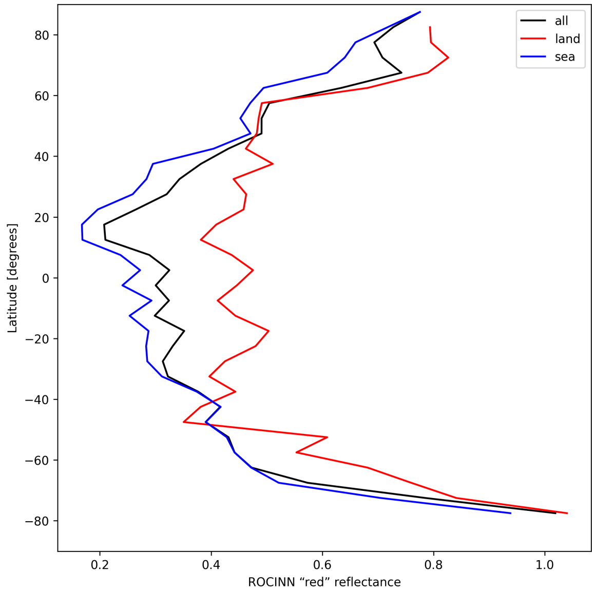
Figure 35: Zonal average of “ROCINN “red” reflectance” for 2025-04-19 to 2025-04-20.
