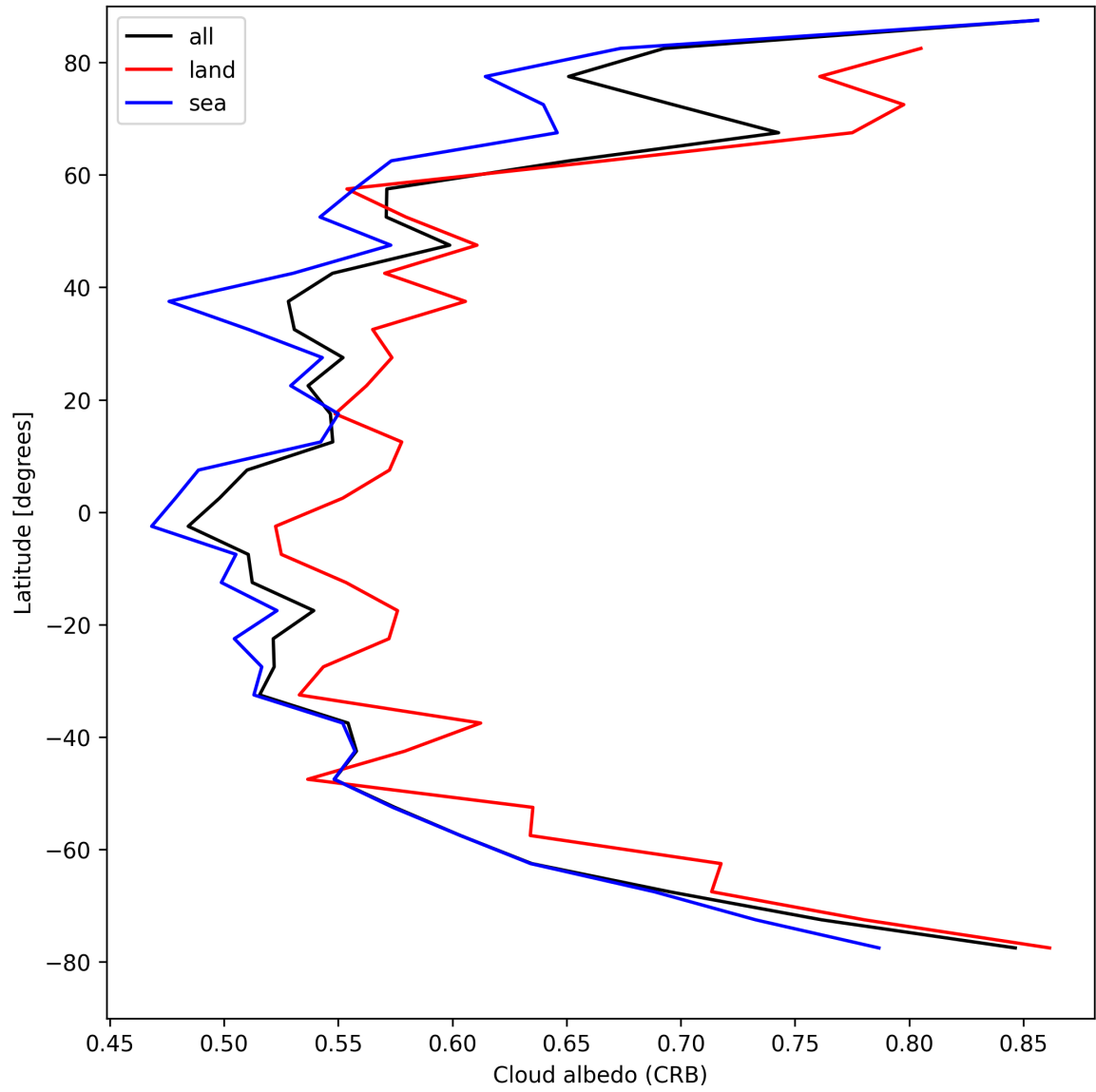
Figure 26: Zonal average of “Cloud albedo (CRB)” for 2025-04-19 to 2025-04-20.
