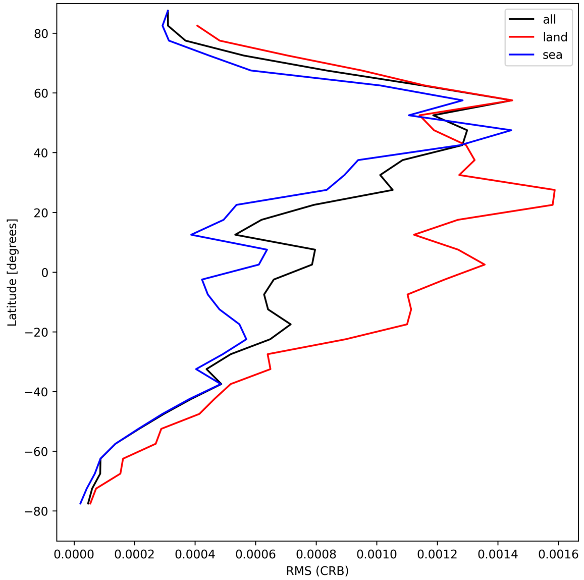
Figure 30: Zonal average of “RMS (CRB)” for 2025-04-20 to 2025-04-21.
