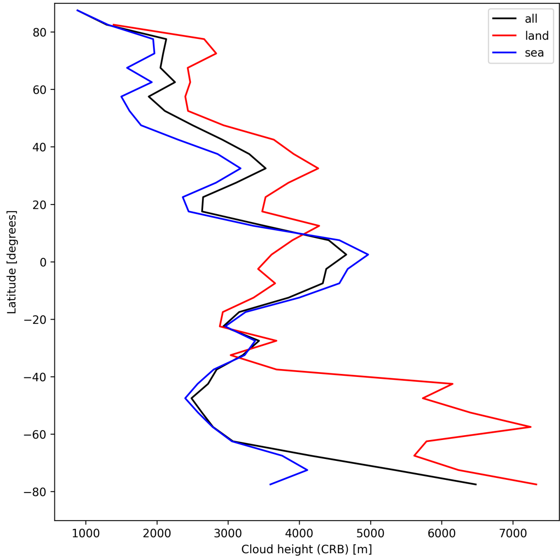
Figure 25: Zonal average of “Cloud height (CRB)” for 2025-04-20 to 2025-04-21.
