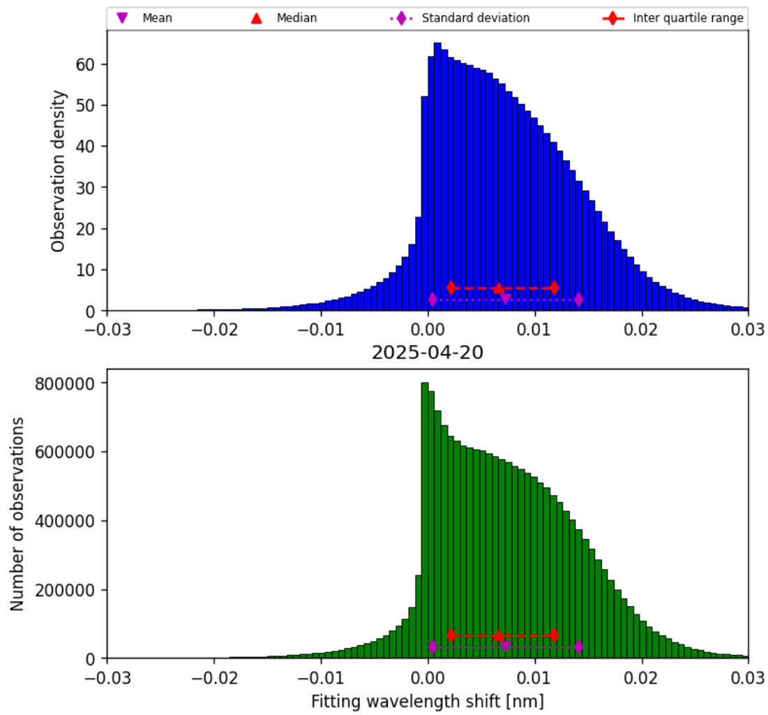
Figure 47: Histogram of “Fitting wavelength shift” for 2025-04-20 to 2025-04-21
