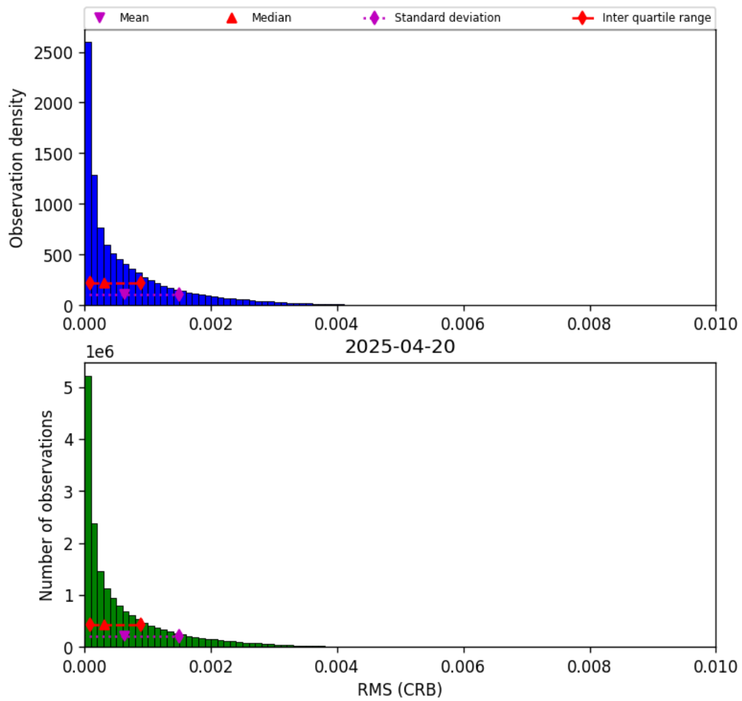
Figure 46: Histogram of “RMS (CRB)” for 2025-04-20 to 2025-04-21
