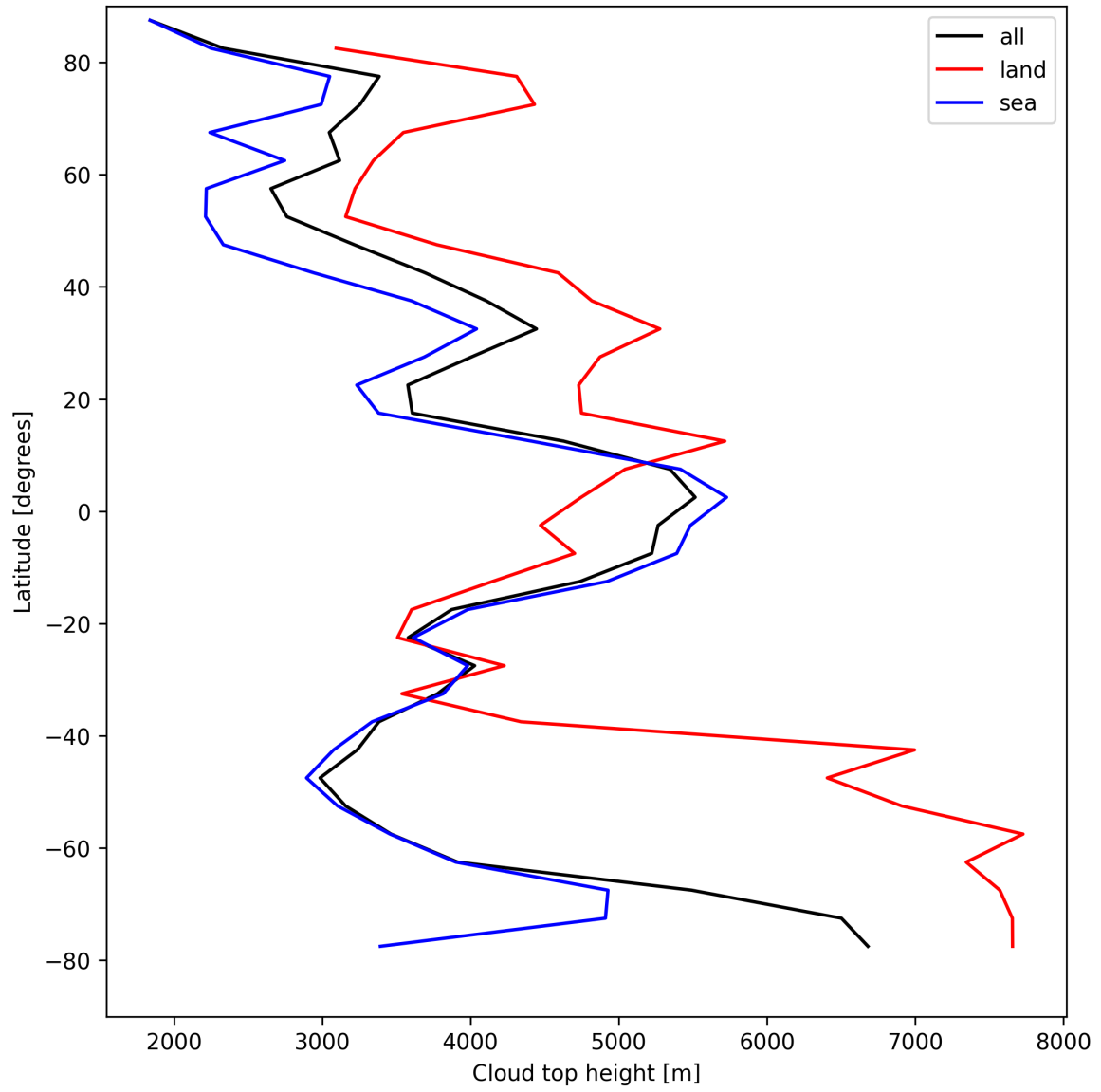
Figure 22: Zonal average of “Cloud top height” for 2025-04-20 to 2025-04-21.
