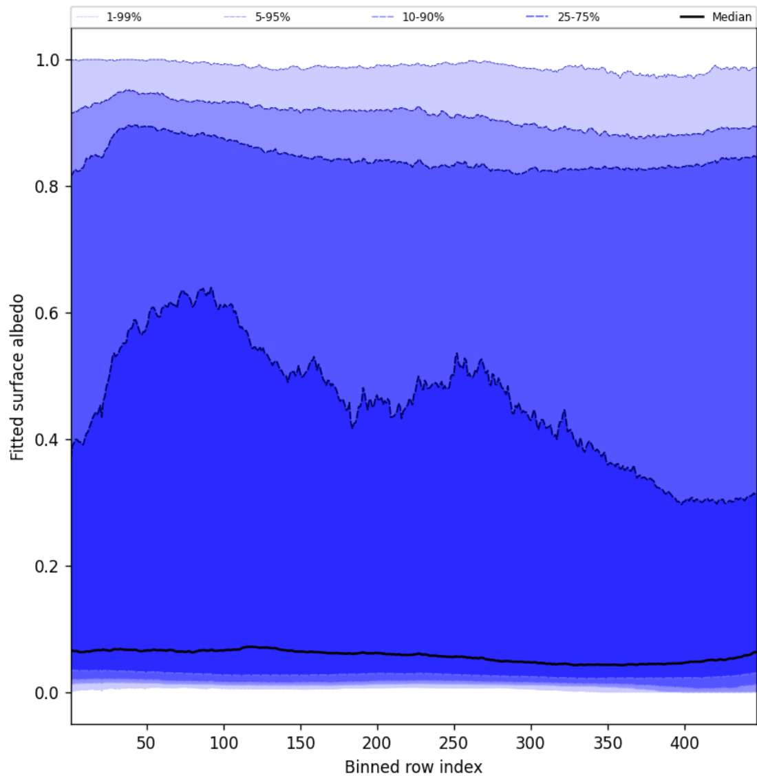
Figure 59: Along track statistics of “Fitted surface albedo” for 2025-04-20 to 2025-04-21
