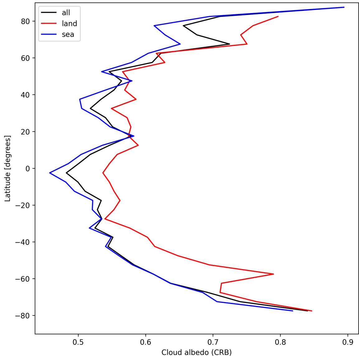
Figure 26: Zonal average of “Cloud albedo (CRB)” for 2025-04-20 to 2025-04-21.
