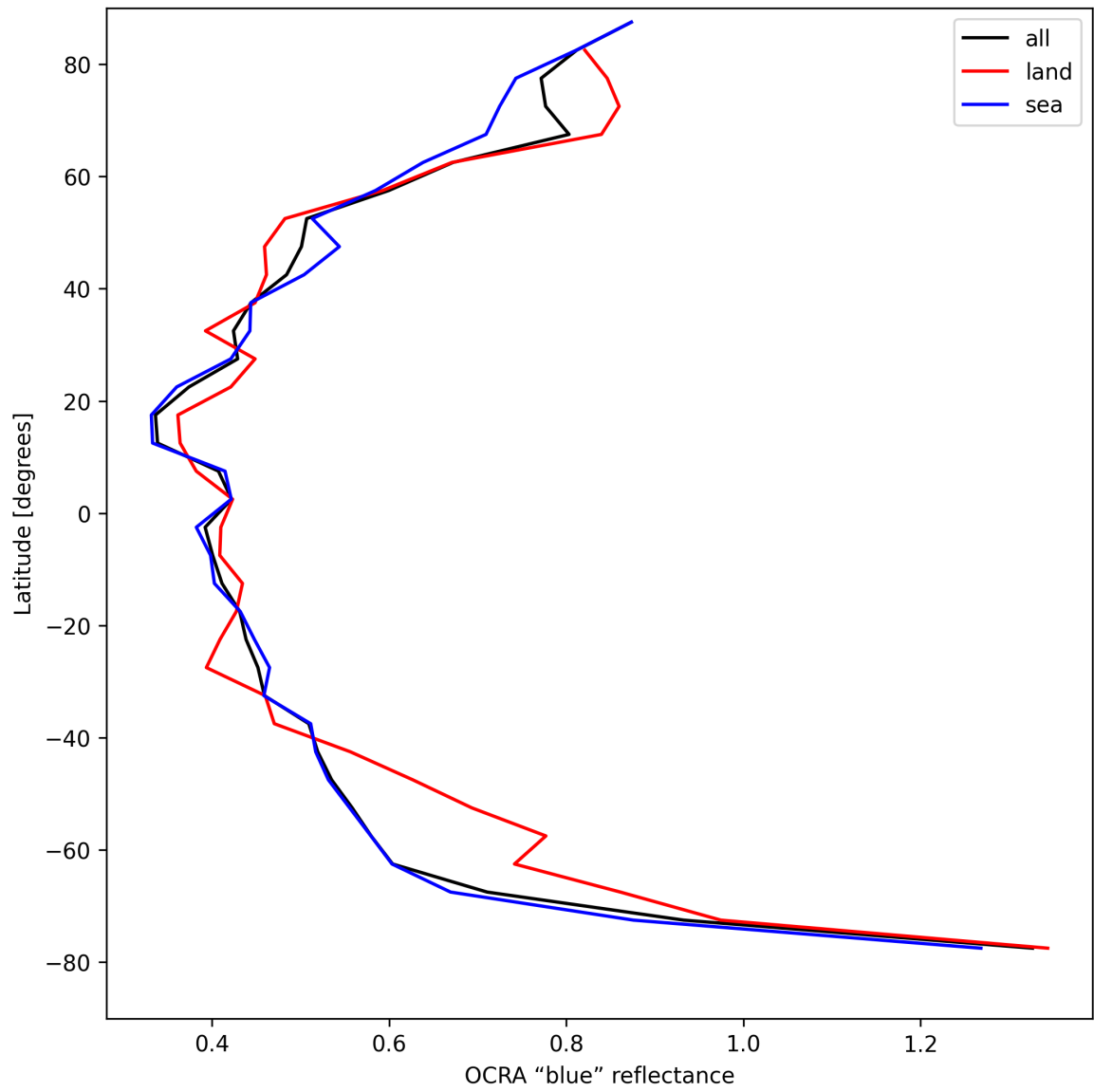
Figure 33: Zonal average of “OCRA “blue” reflectance” for 2025-04-20 to 2025-04-21.
