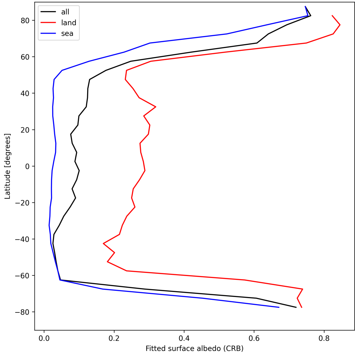
Figure 28: Zonal average of “Fitted surface albedo (CRB)” for 2025-04-20 to 2025-04-21.
