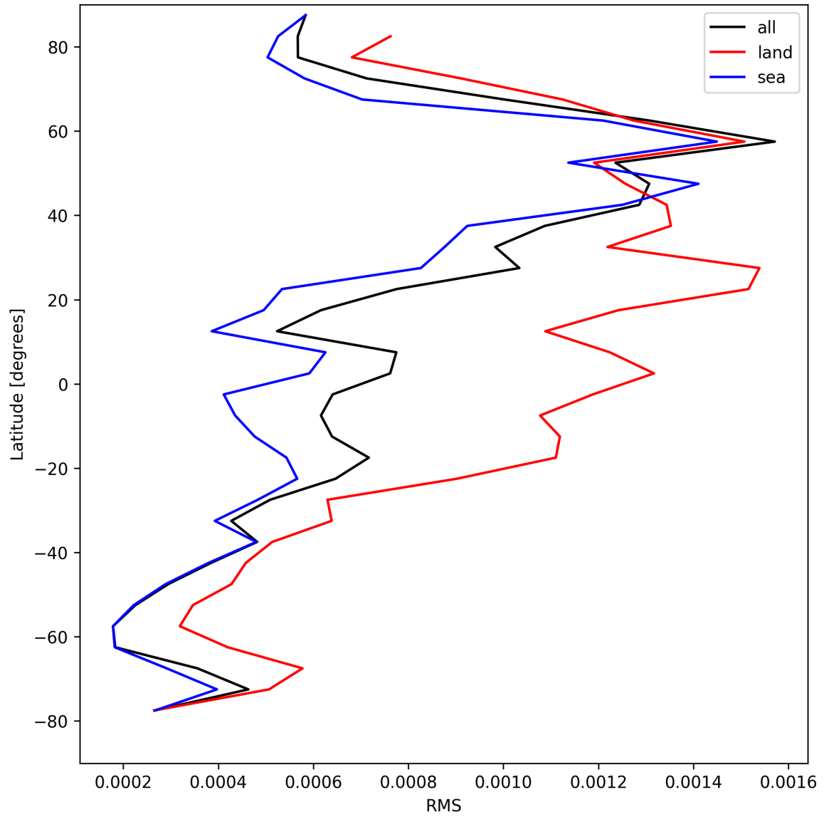
Figure 29: Zonal average of “RMS” for 2025-04-20 to 2025-04-21.
