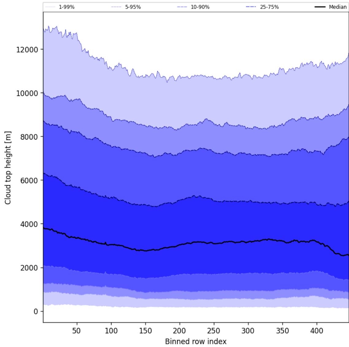
Figure 54: Along track statistics of “Cloud top height” for 2025-04-20 to 2025-04-21
