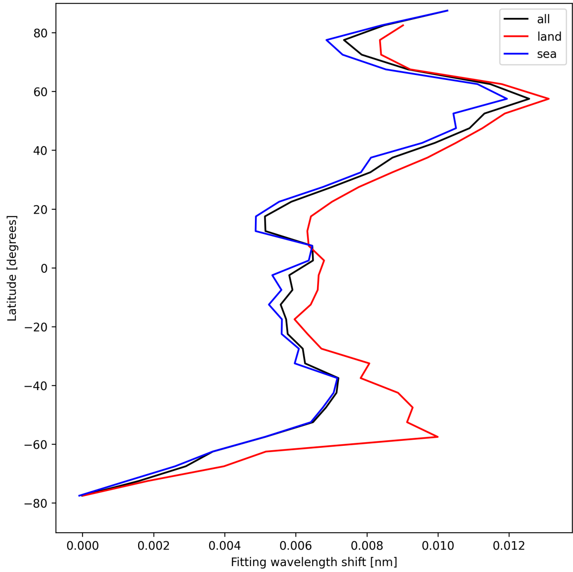
Figure 31: Zonal average of “Fitting wavelength shift” for 2025-04-20 to 2025-04-21.
