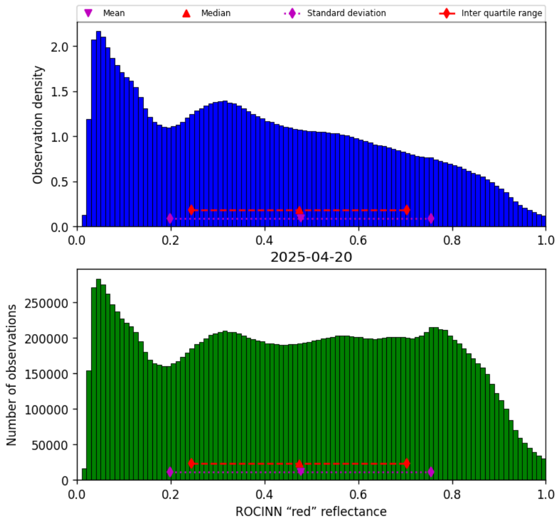
Figure 51: Histogram of “ROCINN “red” reflectance” for 2025-04-20 to 2025-04-21
