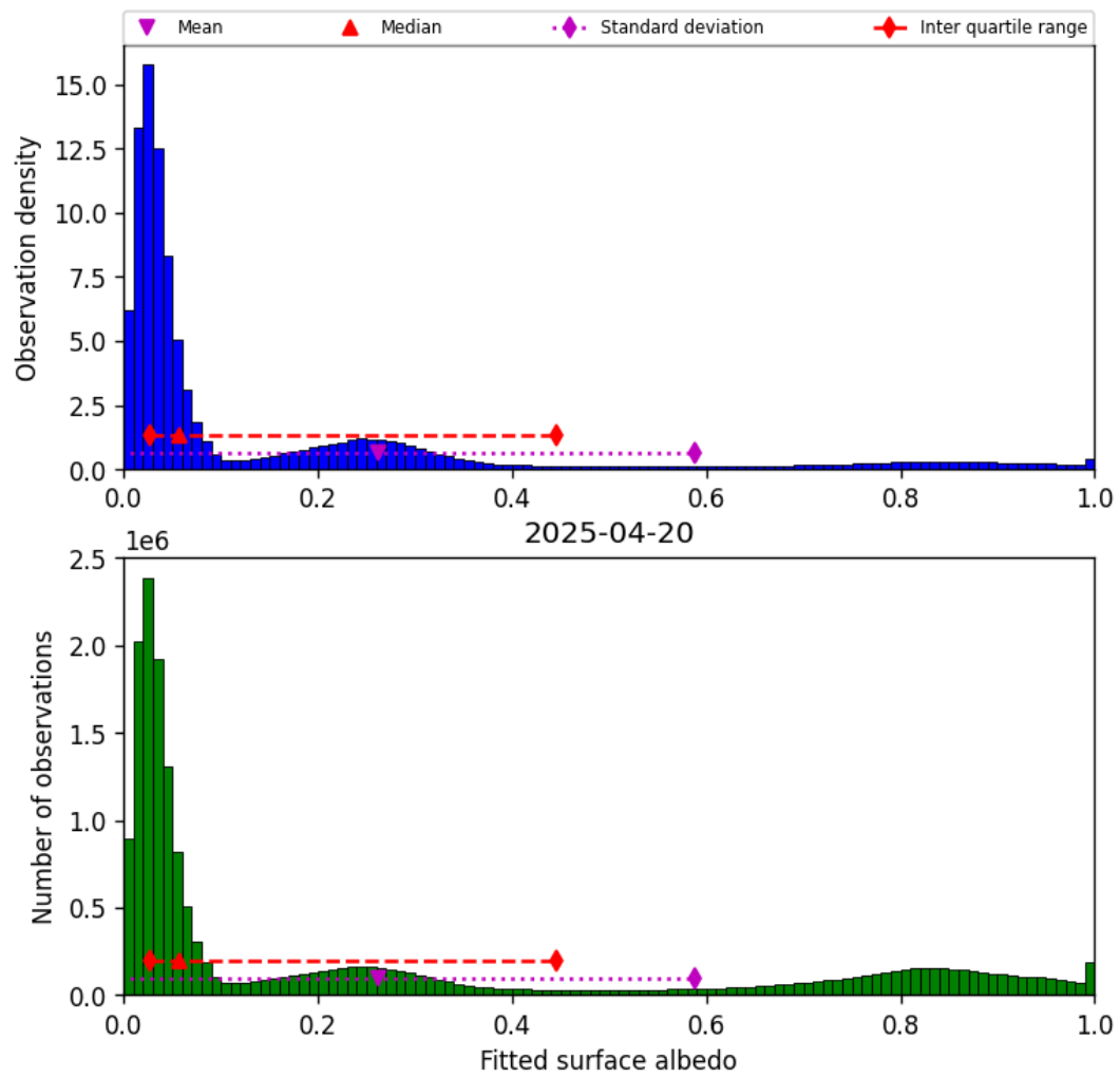
Figure 43: Histogram of “Fitted surface albedo” for 2025-04-20 to 2025-04-21
