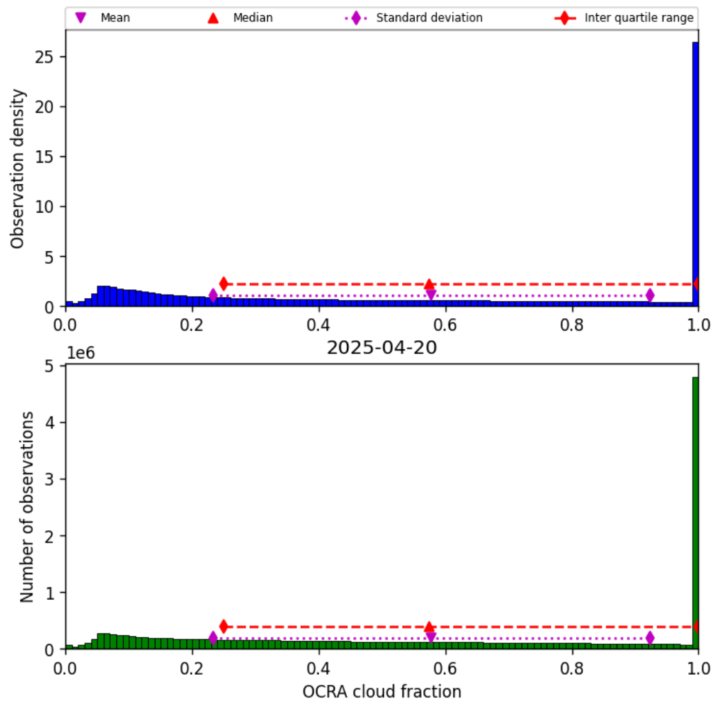
Figure 48: Histogram of “OCRA cloud fraction” for 2025-04-20 to 2025-04-21
