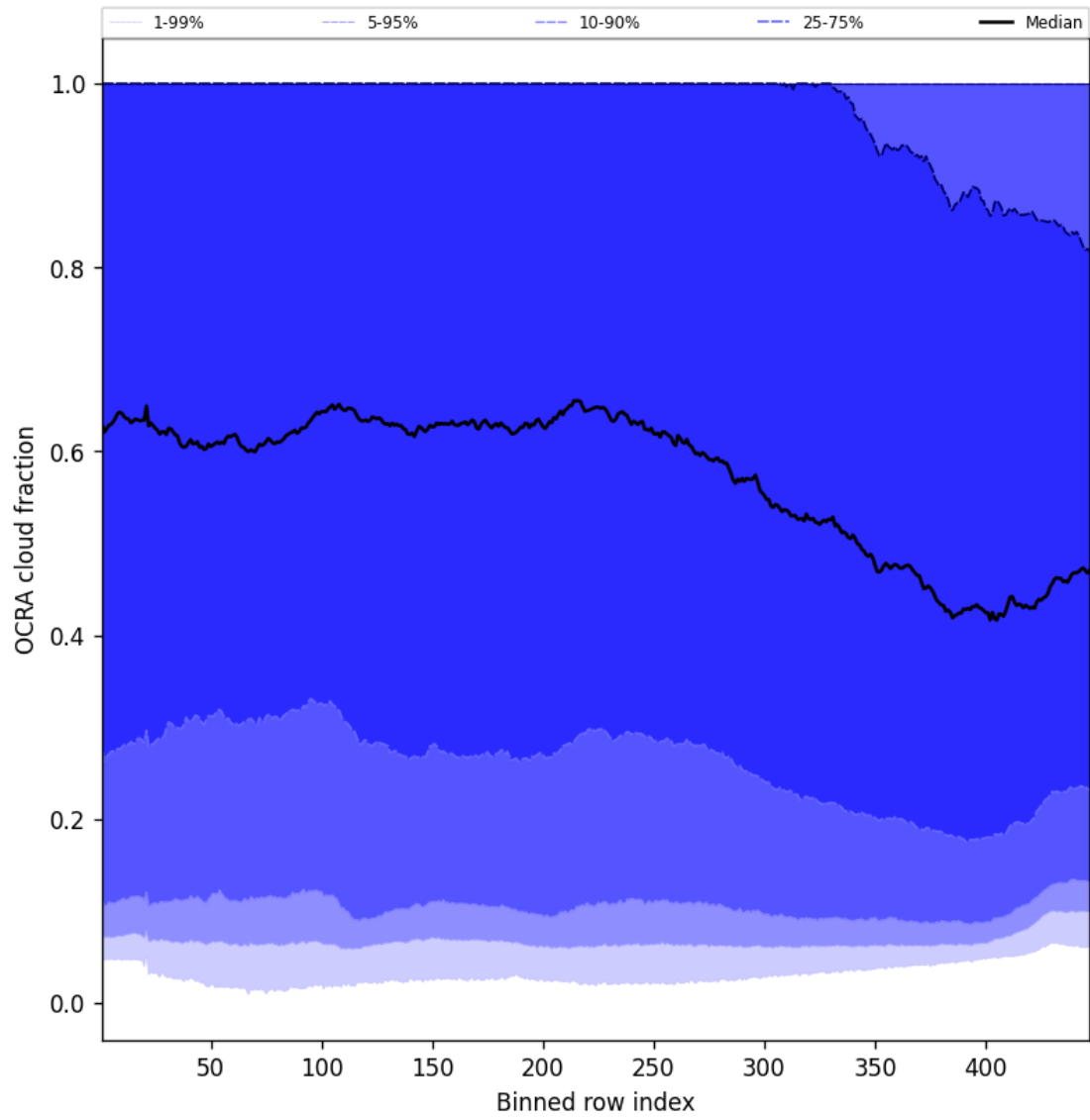
Figure 64: Along track statistics of “OCRA cloud fraction” for 2025-04-20 to 2025-04-21
