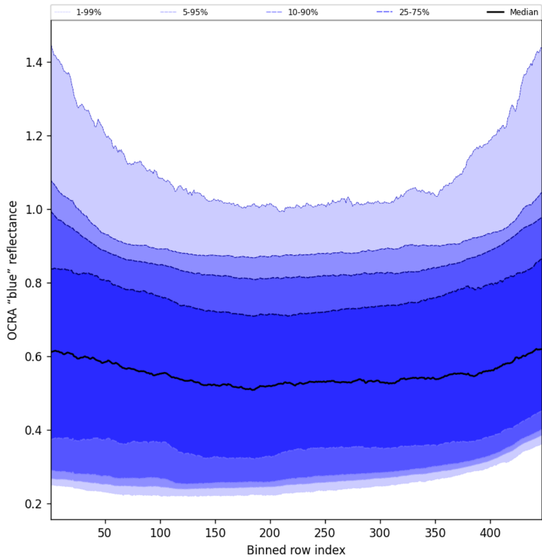
Figure 65: Along track statistics of “OCRA “blue” reflectance” for 2025-04-20 to 2025-04-21
