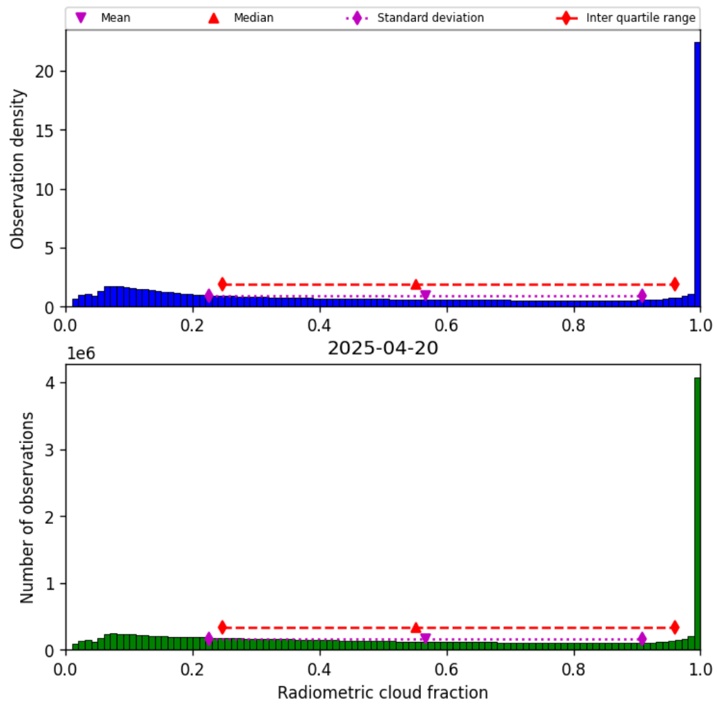
Figure 37: Histogram of “Radiometric cloud fraction” for 2025-04-20 to 2025-04-21
