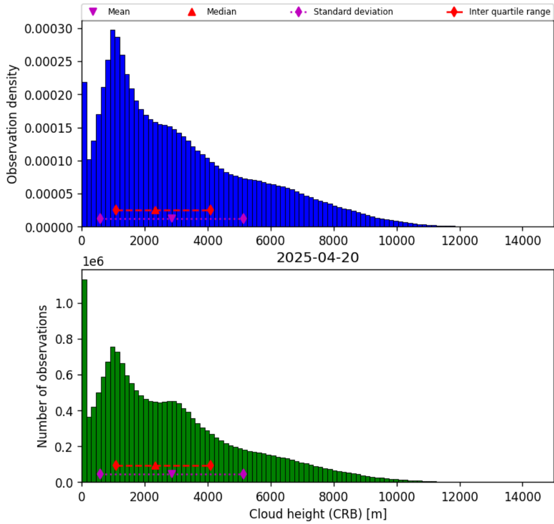
Figure 41: Histogram of “Cloud height (CRB)” for 2025-04-20 to 2025-04-21
