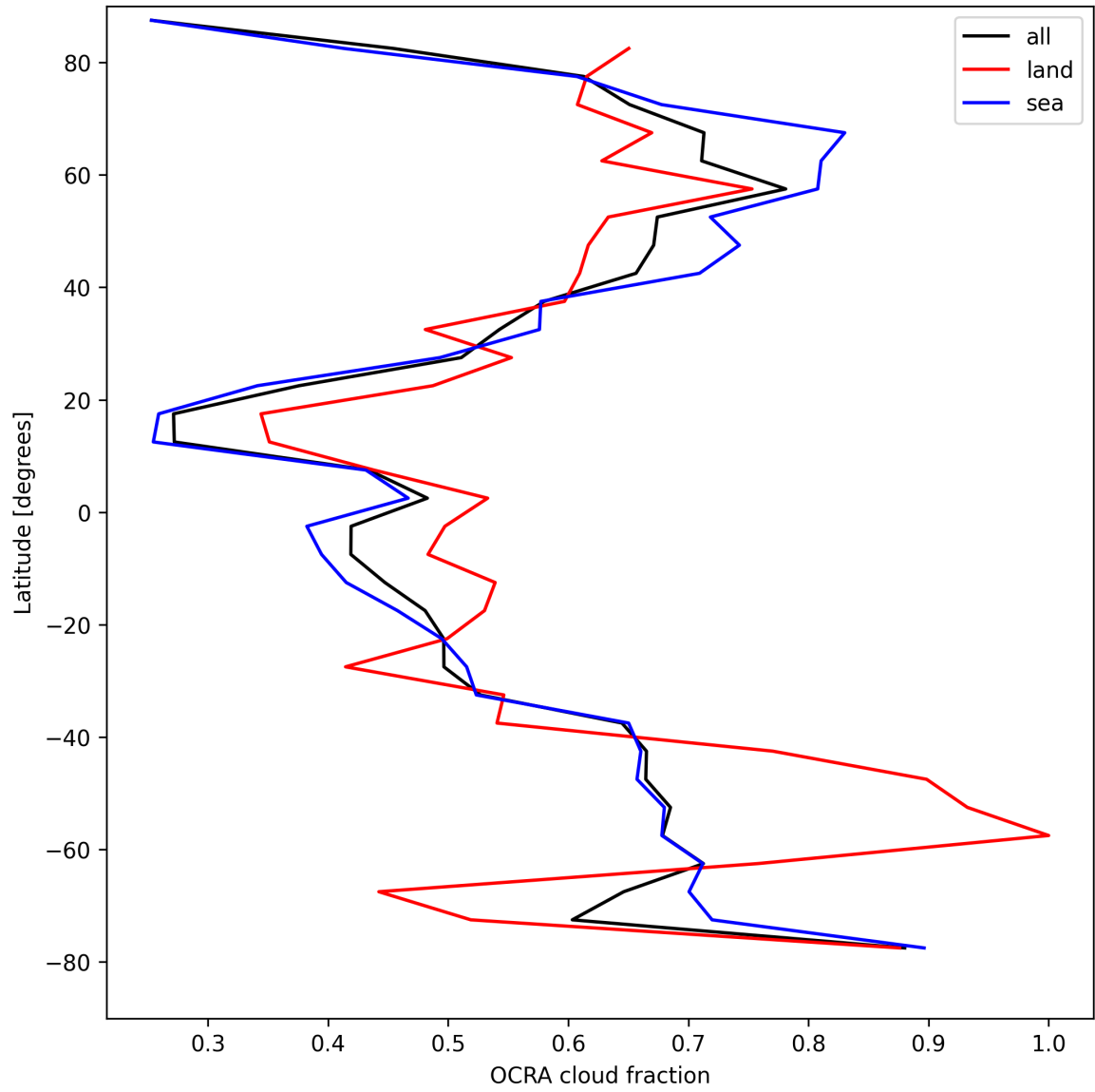
Figure 32: Zonal average of “OCRA cloud fraction” for 2025-04-20 to 2025-04-21.
