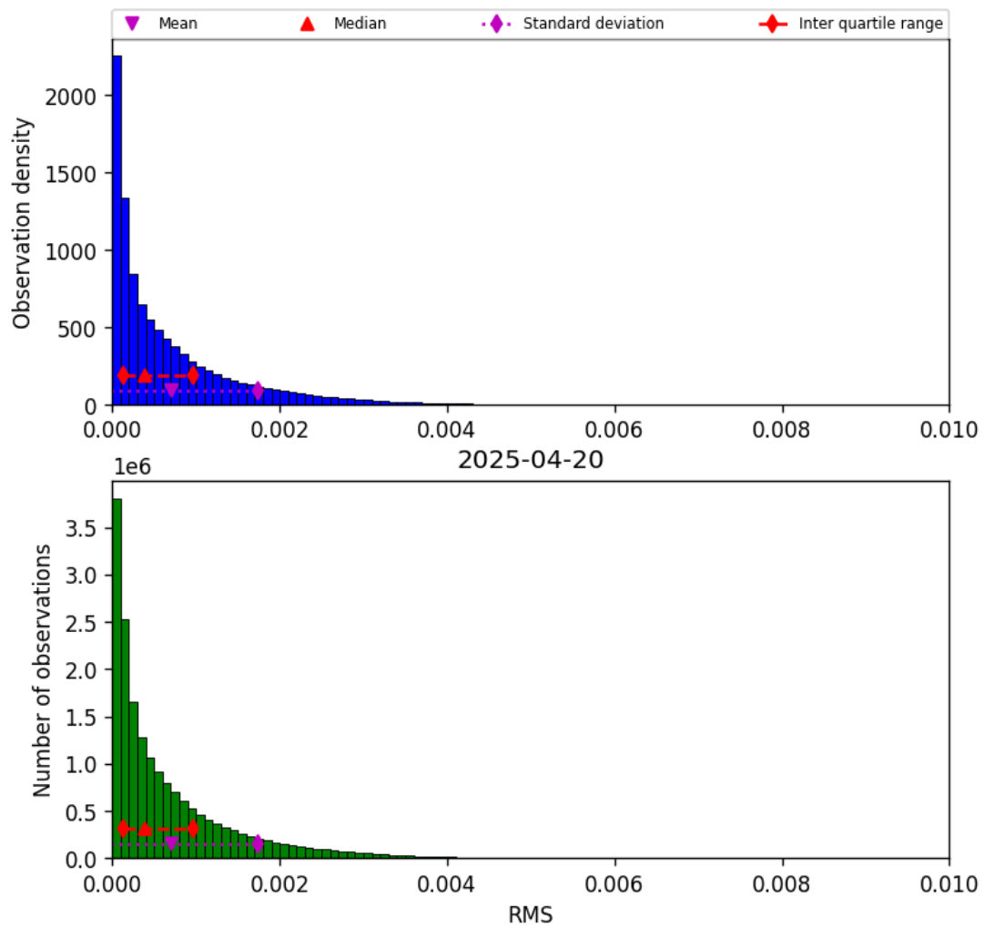
Figure 45: Histogram of “RMS” for 2025-04-20 to 2025-04-21
