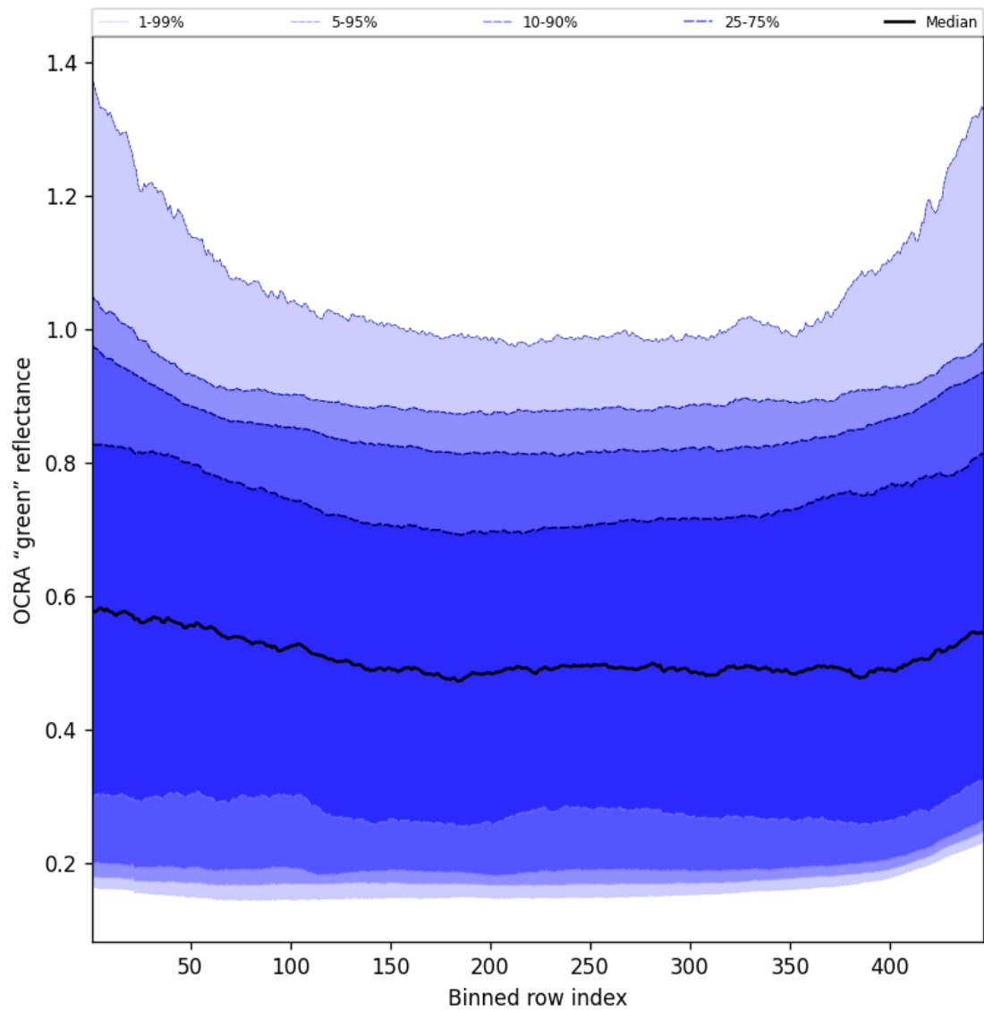
Figure 66: Along track statistics of "OCRA "green" reflectance" for 2025-04-20 to 2025-04-21
