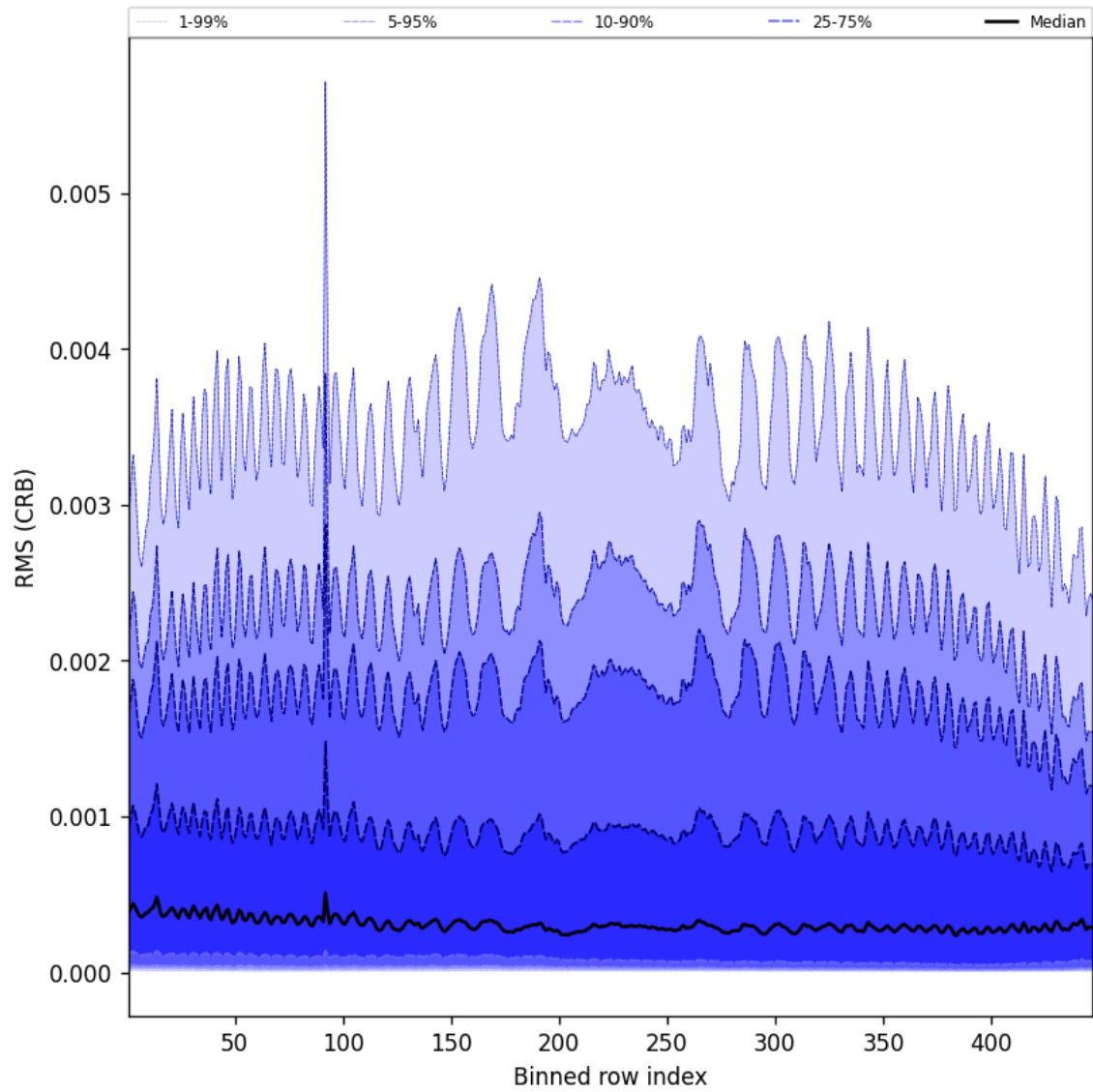
Figure 62: Along track statistics of “RMS (CRB)” for 2025-04-20 to 2025-04-21
