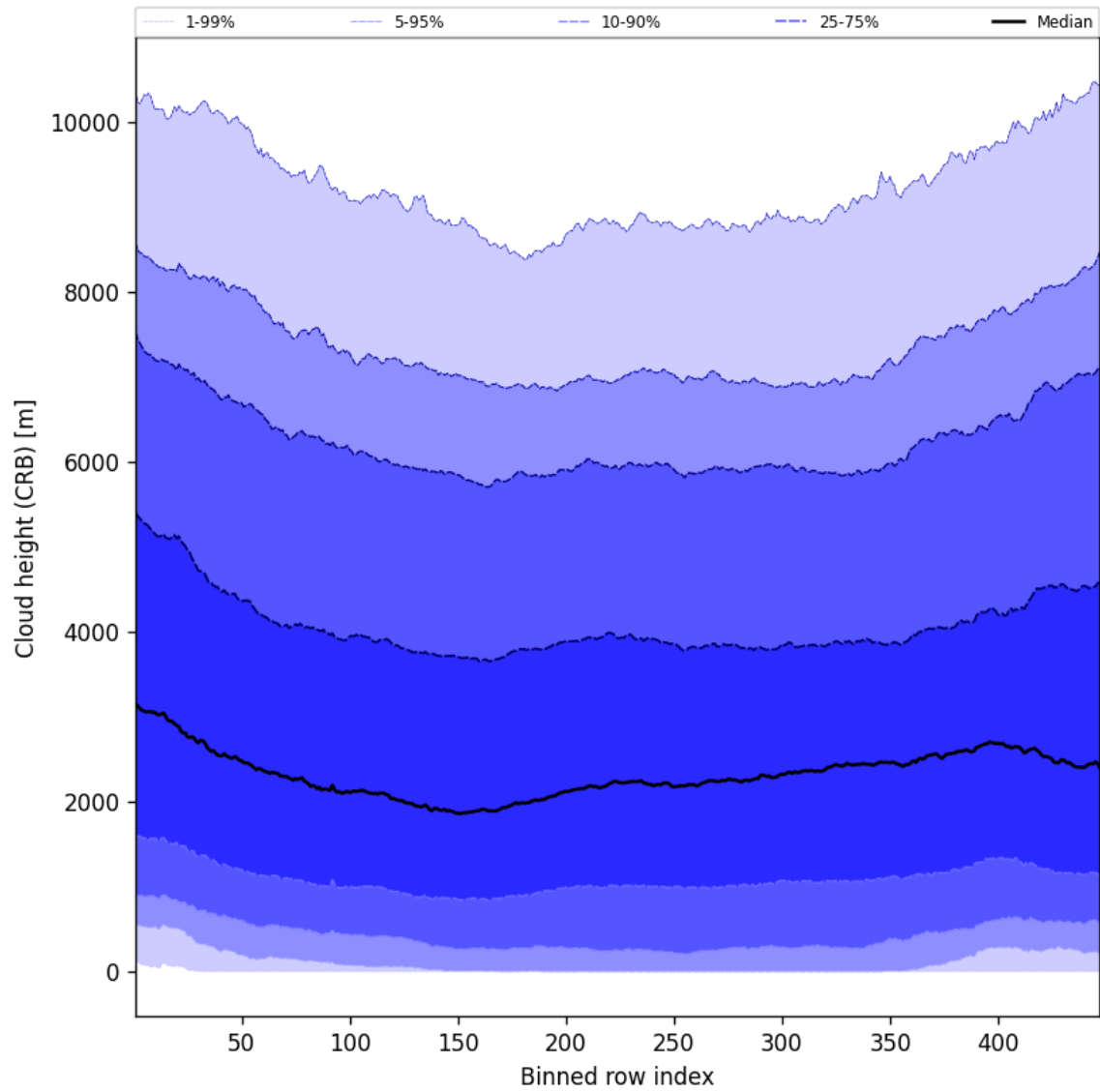
Figure 57: Along track statistics of “Cloud height (CRB)” for 2025-04-20 to 2025-04-21
