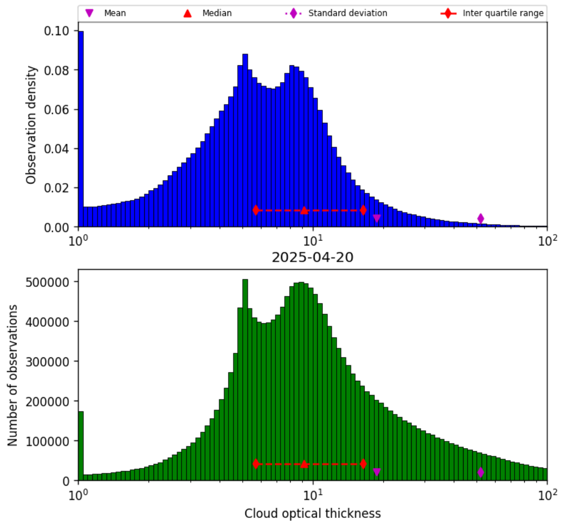
Figure 39: Histogram of “Cloud optical thickness” for 2025-04-20 to 2025-04-21
