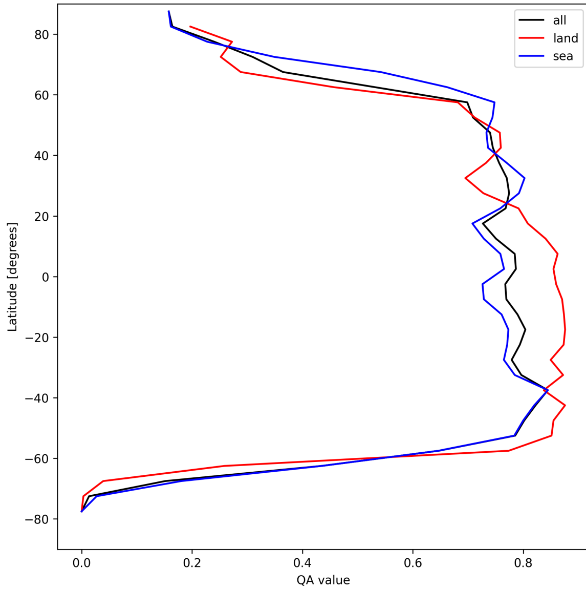
Figure 20: Zonal average of “QA value” for 2025-04-20 to 2025-04-21.
