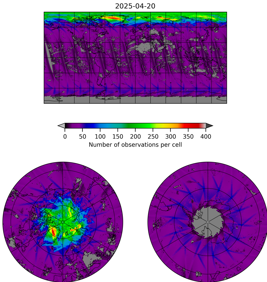
Figure 19: Map of the number of observations for 2025-04-20 to 2025-04-21
