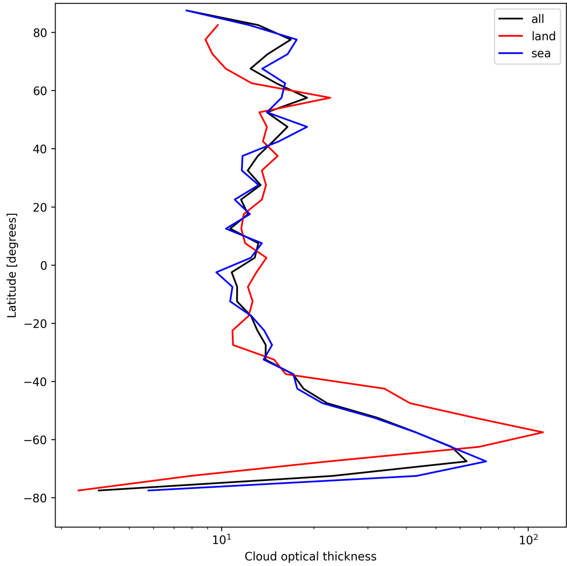
Figure 23: Zonal average of “Cloud optical thickness” for 2025-04-20 to 2025-04-21.
