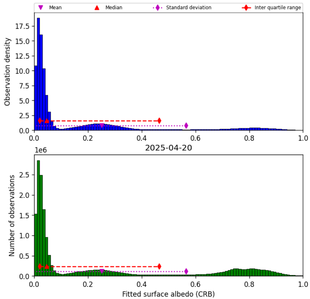
Figure 44: Histogram of “Fitted surface albedo (CRB)” for 2025-04-20 to 2025-04-21
