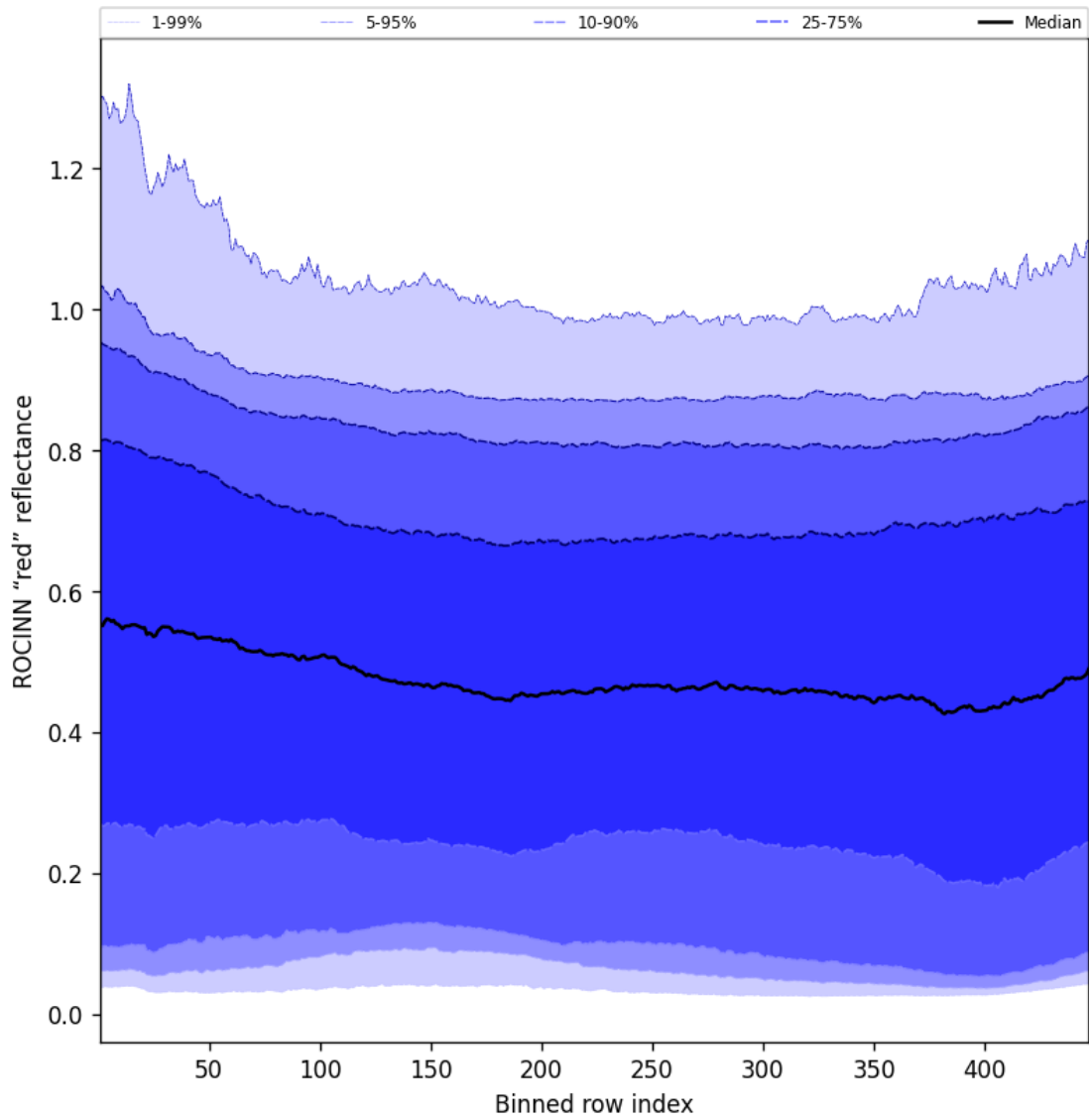
Figure 67: Along track statistics of "ROCINN "red" reflectance" for 2025-04-20 to 2025-04-21
