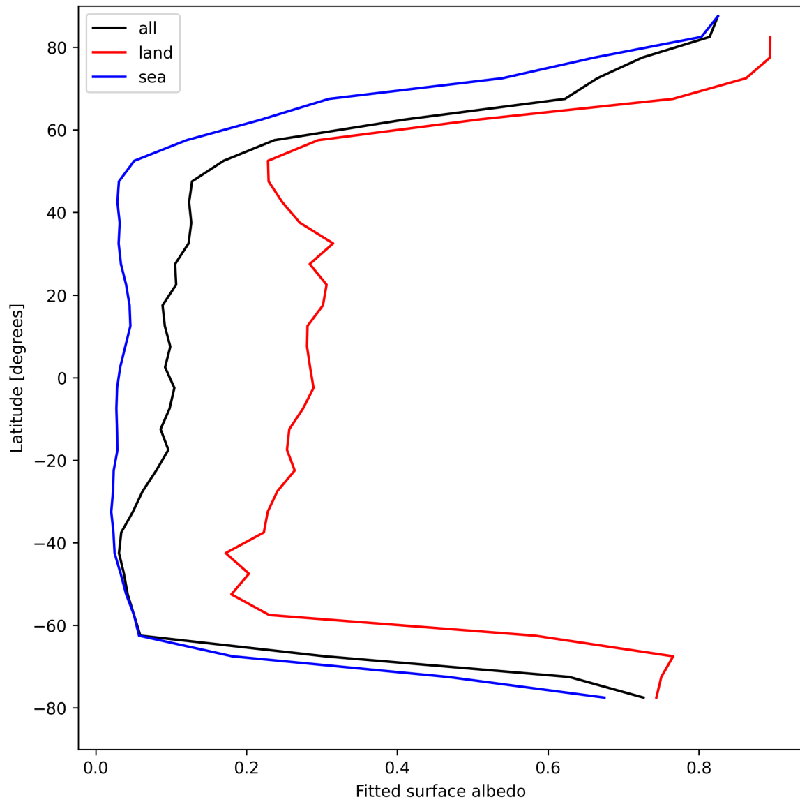
Figure 27: Zonal average of “Fitted surface albedo” for 2025-04-20 to 2025-04-21.
