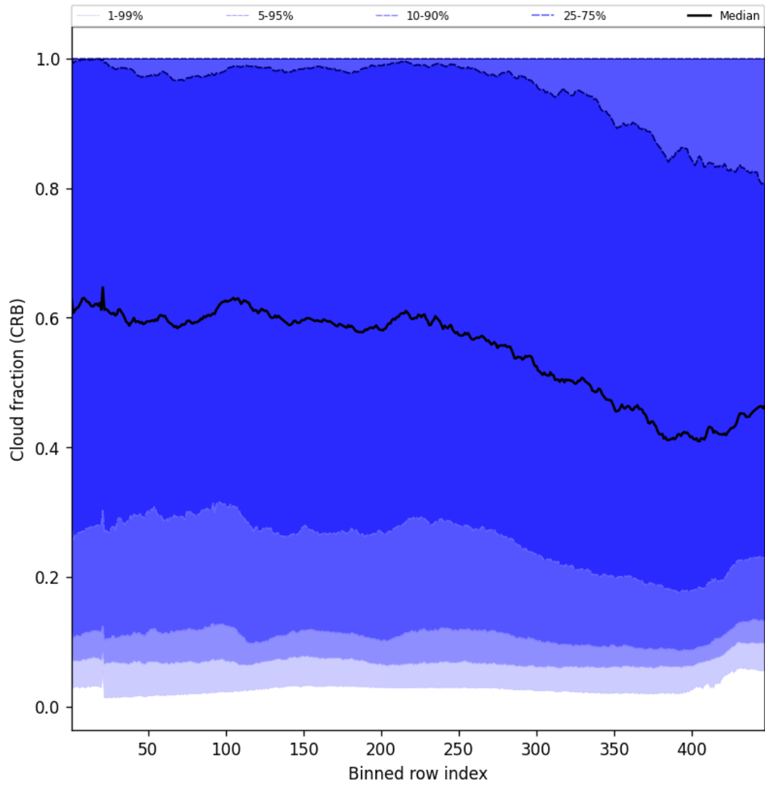
Figure 56: Along track statistics of “Cloud fraction (CRB)” for 2025-04-20 to 2025-04-21
