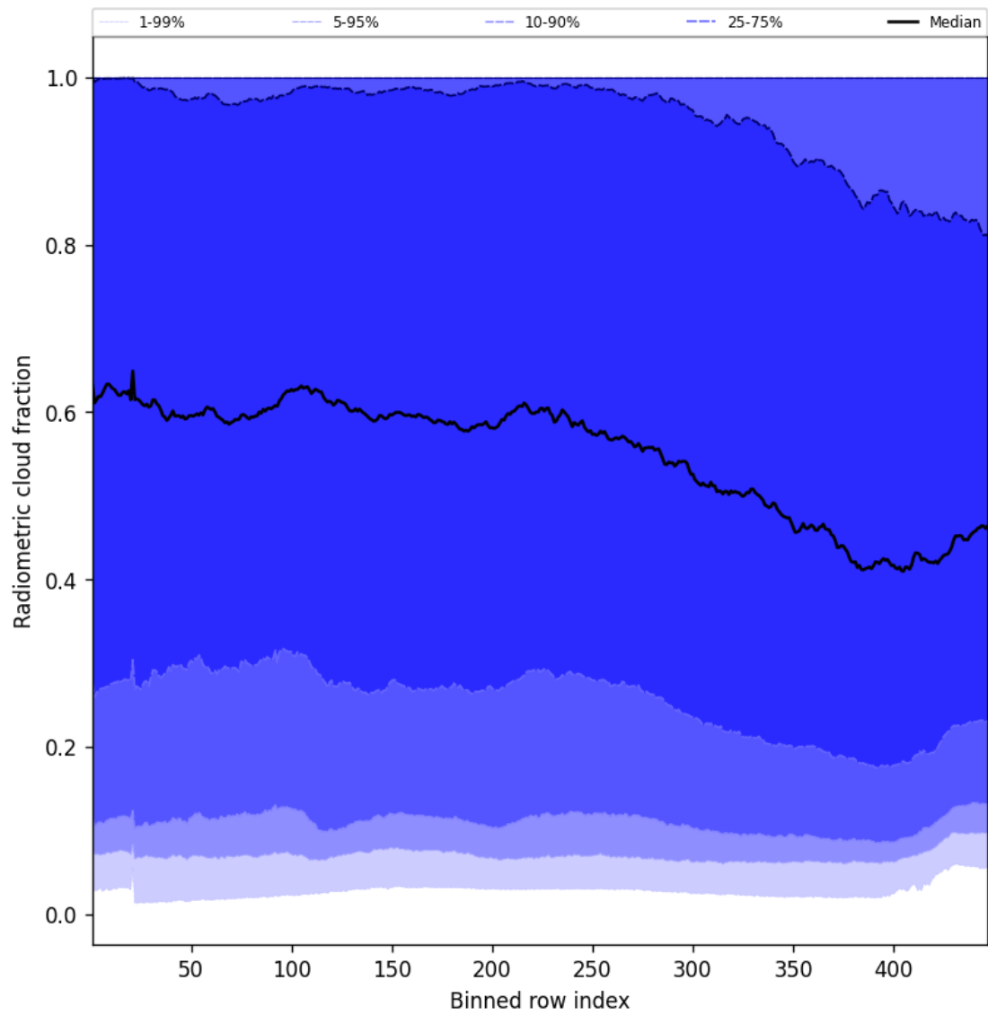
Figure 53: Along track statistics of “Radiometric cloud fraction” for 2025-04-20 to 2025-04-21
