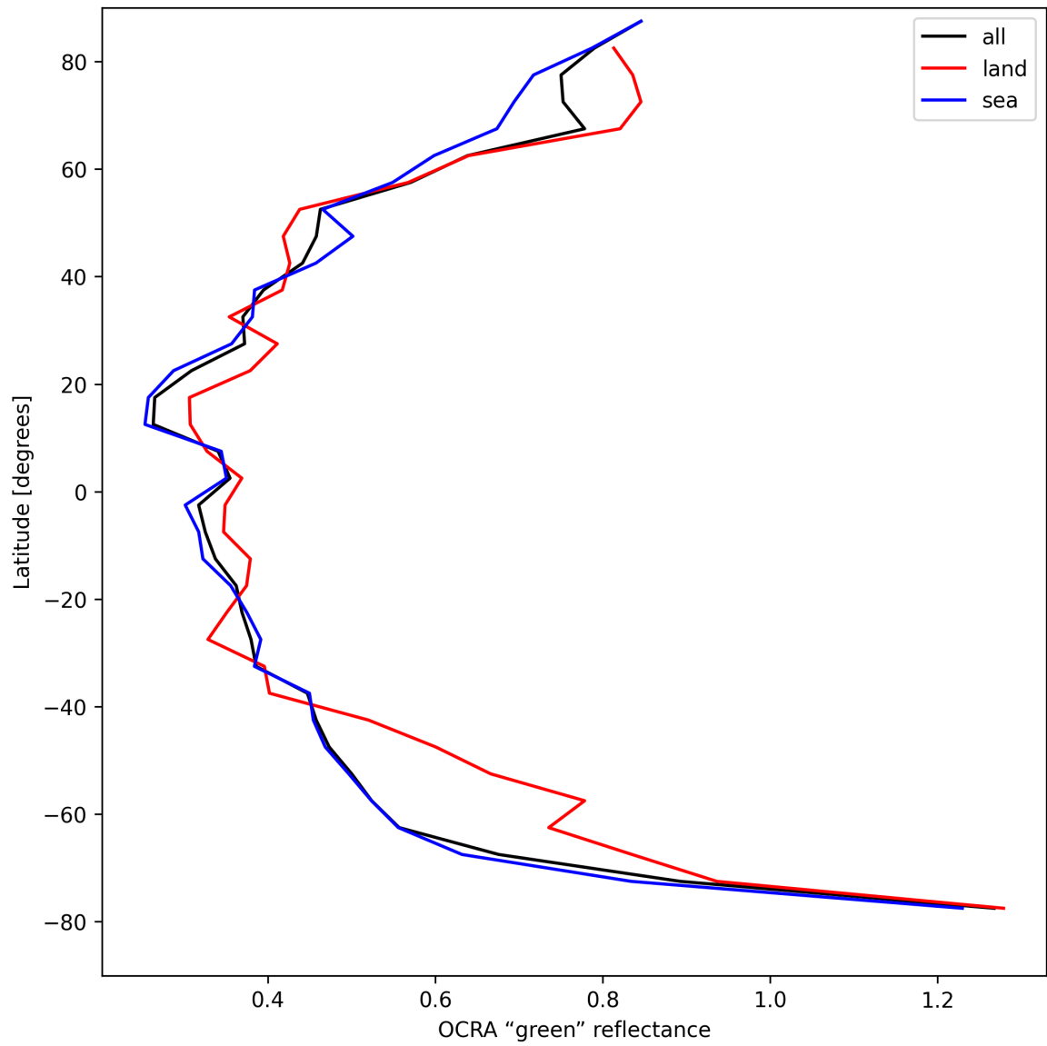
Figure 34: Zonal average of “OCRA “green” reflectance” for 2025-04-20 to 2025-04-21.
