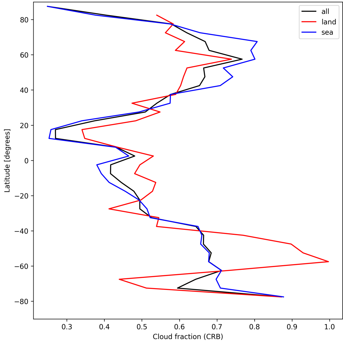
Figure 24: Zonal average of “Cloud fraction (CRB)” for 2025-04-20 to 2025-04-21.
