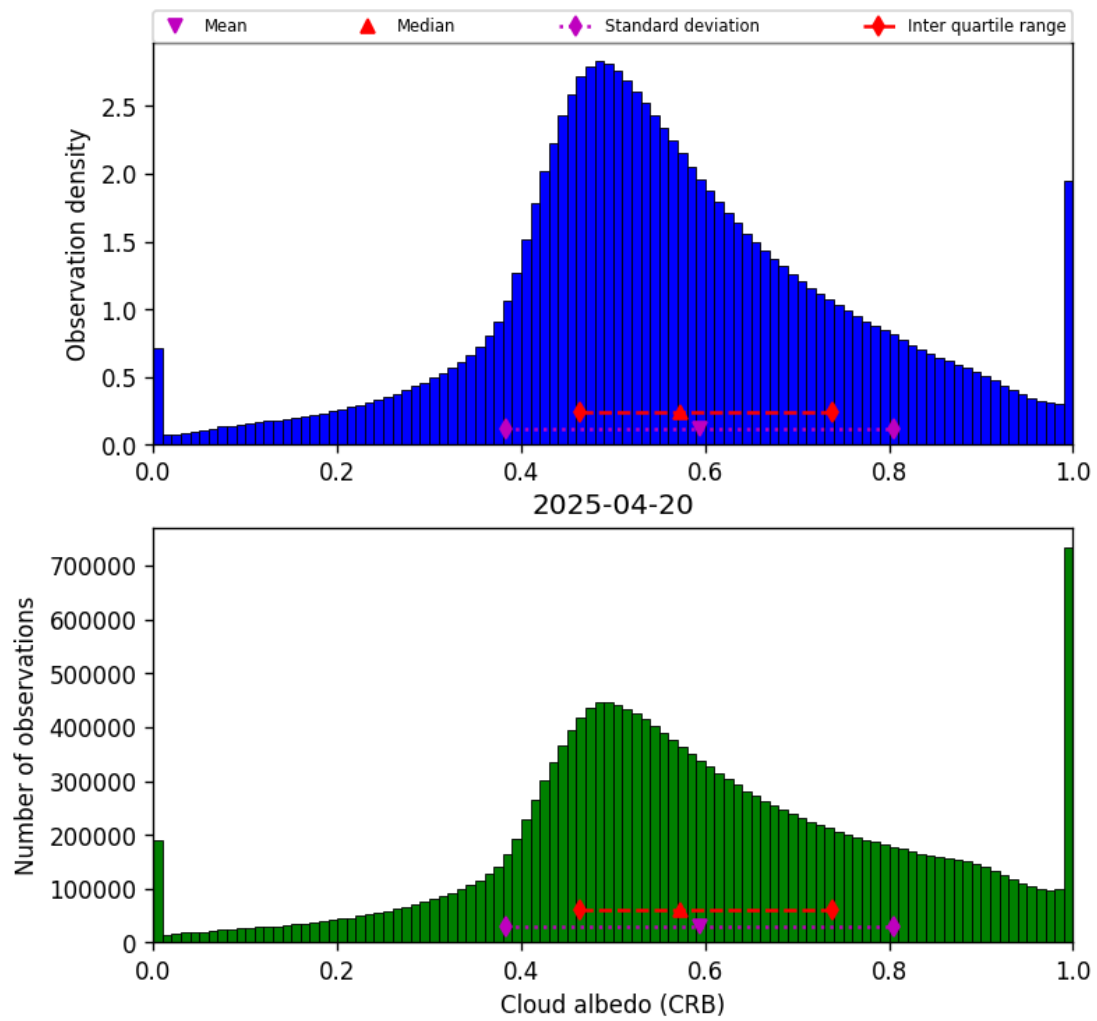
Figure 42: Histogram of “Cloud albedo (CRB)” for 2025-04-20 to 2025-04-21
