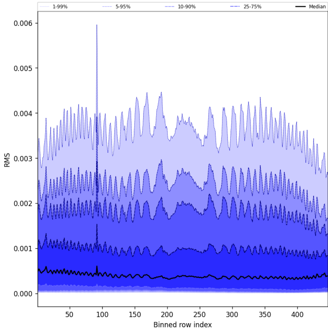
Figure 61: Along track statistics of “RMS” for 2025-04-20 to 2025-04-21
