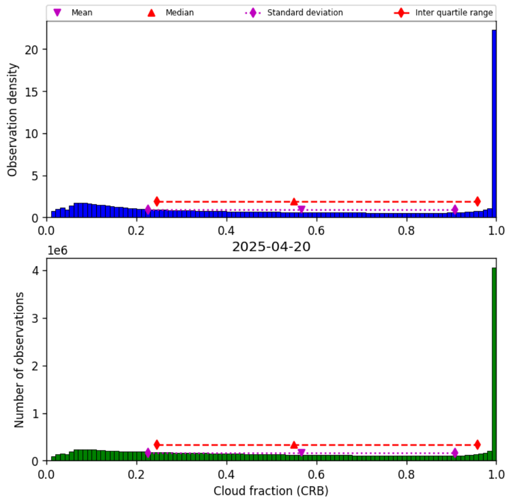
Figure 40: Histogram of “Cloud fraction (CRB)” for 2025-04-20 to 2025-04-21
