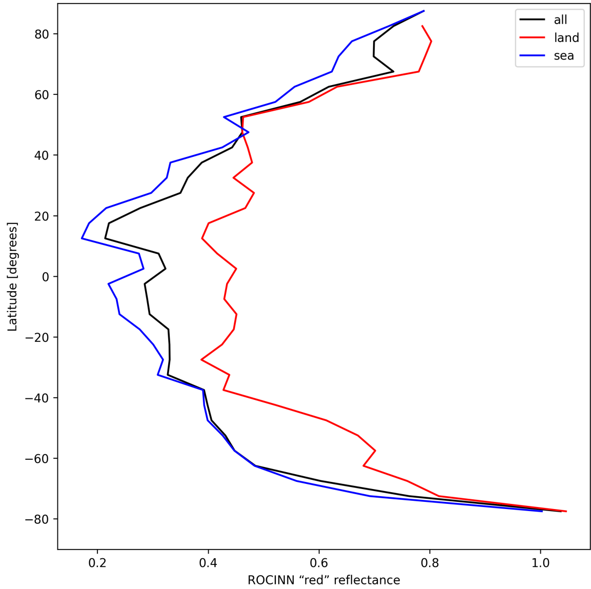
Figure 35: Zonal average of “ROCINN “red” reflectance” for 2025-04-20 to 2025-04-21.
