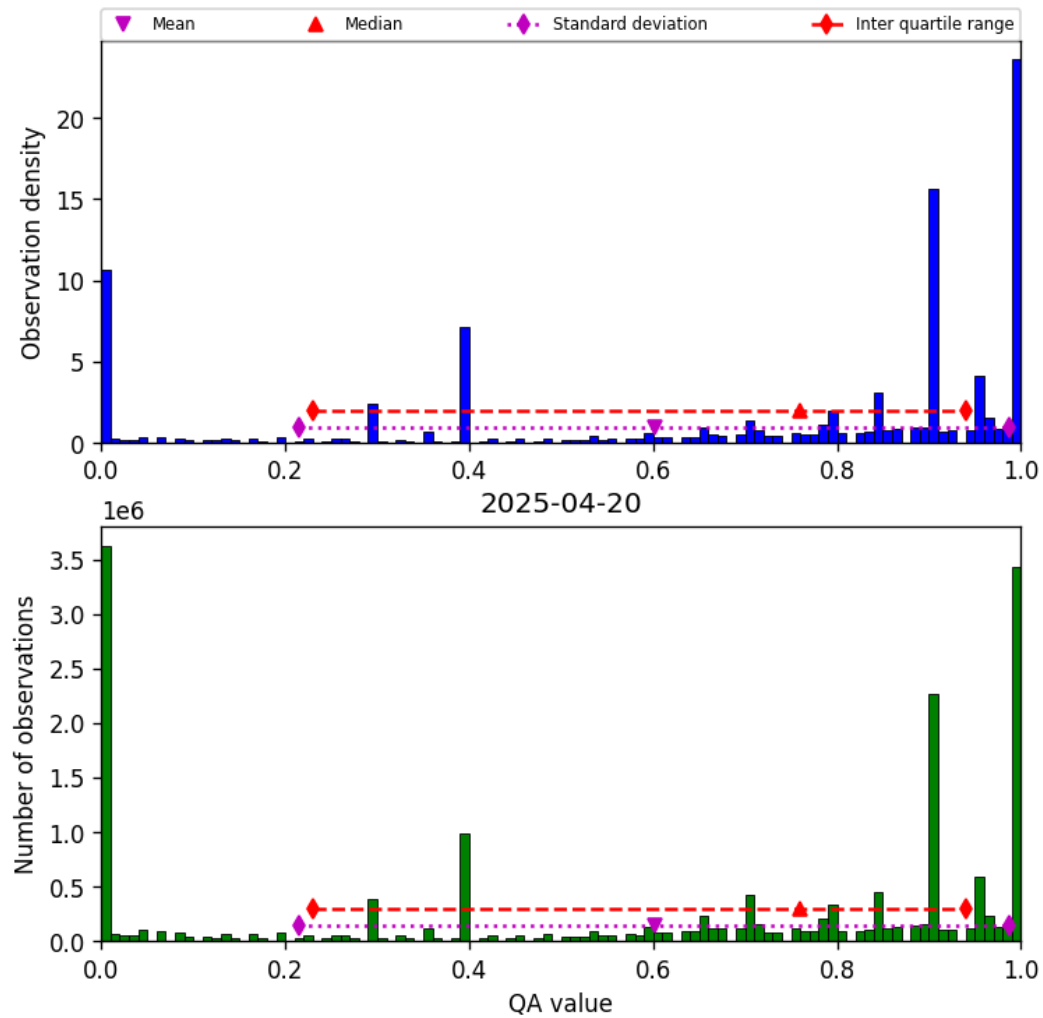
Figure 36: Histogram of “QA value” for 2025-04-20 to 2025-04-21
