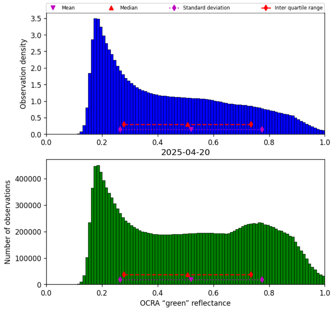
Figure 50: Histogram of “OCRA “green” reflectance” for 2025-04-20 to 2025-04-21
