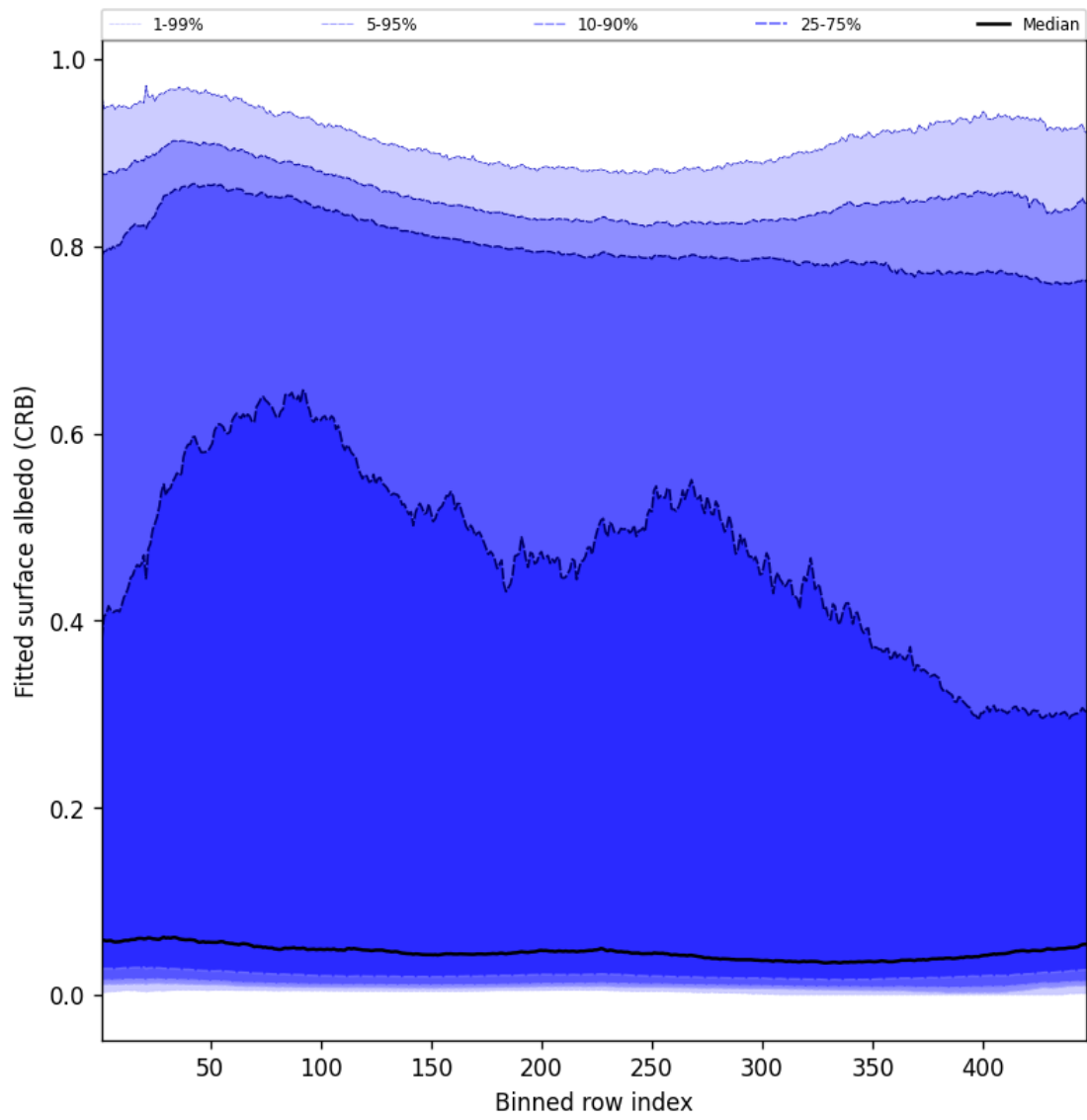
Figure 60: Along track statistics of “Fitted surface albedo (CRB)” for 2025-04-20 to 2025-04-21
