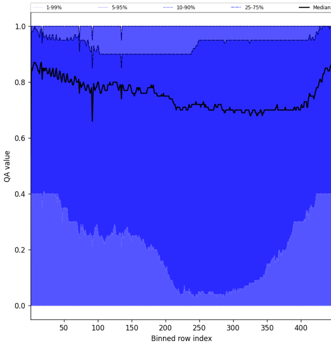
Figure 52: Along track statistics of “QA value” for 2025-04-20 to 2025-04-21
