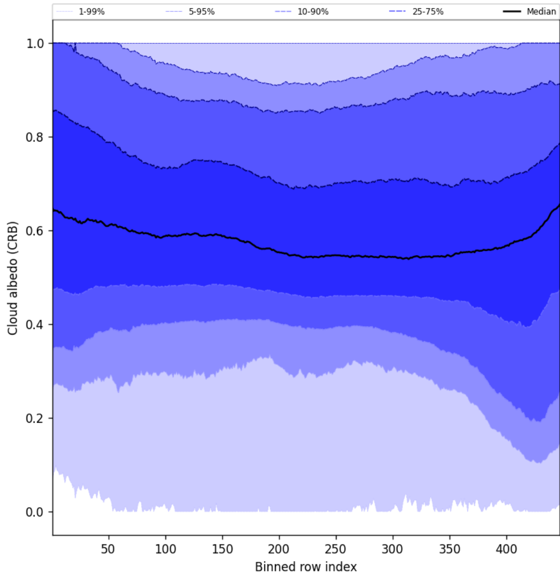
Figure 58: Along track statistics of “Cloud albedo (CRB)” for 2025-04-20 to 2025-04-21
