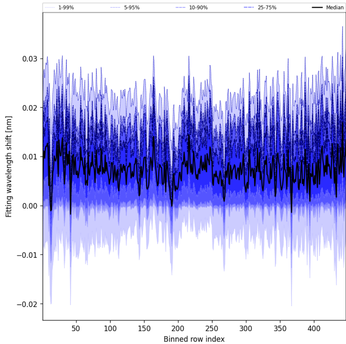
Figure 63: Along track statistics of “Fitting wavelength shift” for 2025-04-20 to 2025-04-21
