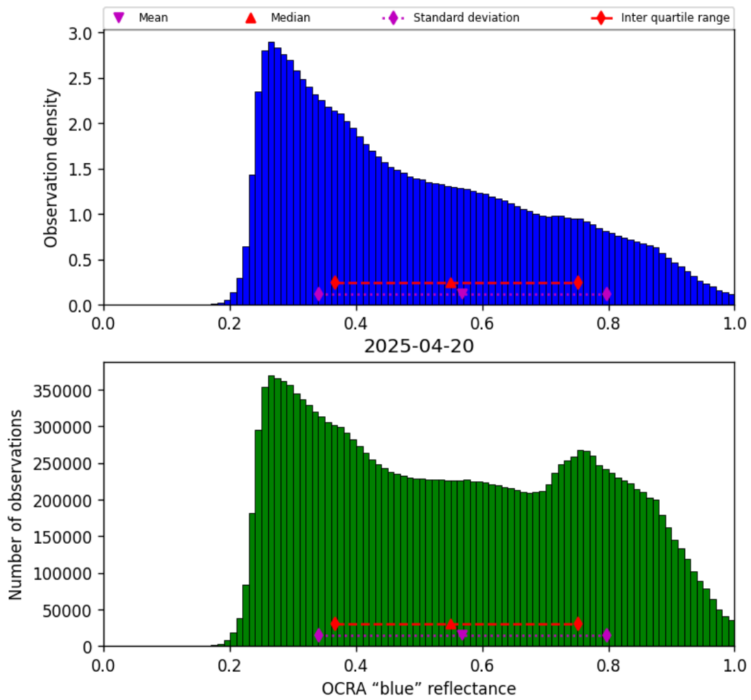
Figure 49: Histogram of "OCRA "blue" reflectance" for 2025-04-20 to 2025-04-21
