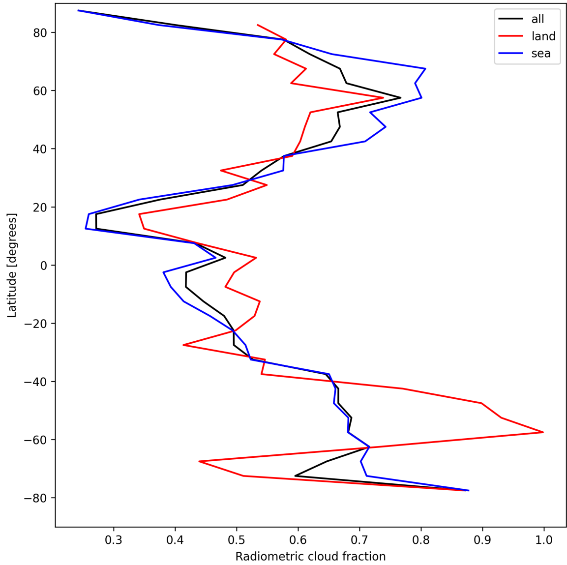
Figure 21: Zonal average of “Radiometric cloud fraction” for 2025-04-20 to 2025-04-21.
