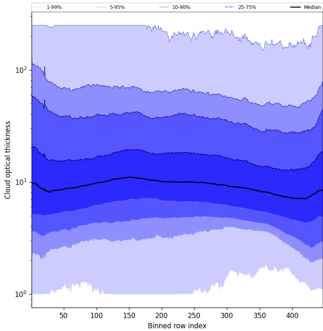
Figure 55: Along track statistics of “Cloud optical thickness” for 2025-04-20 to 2025-04-21
