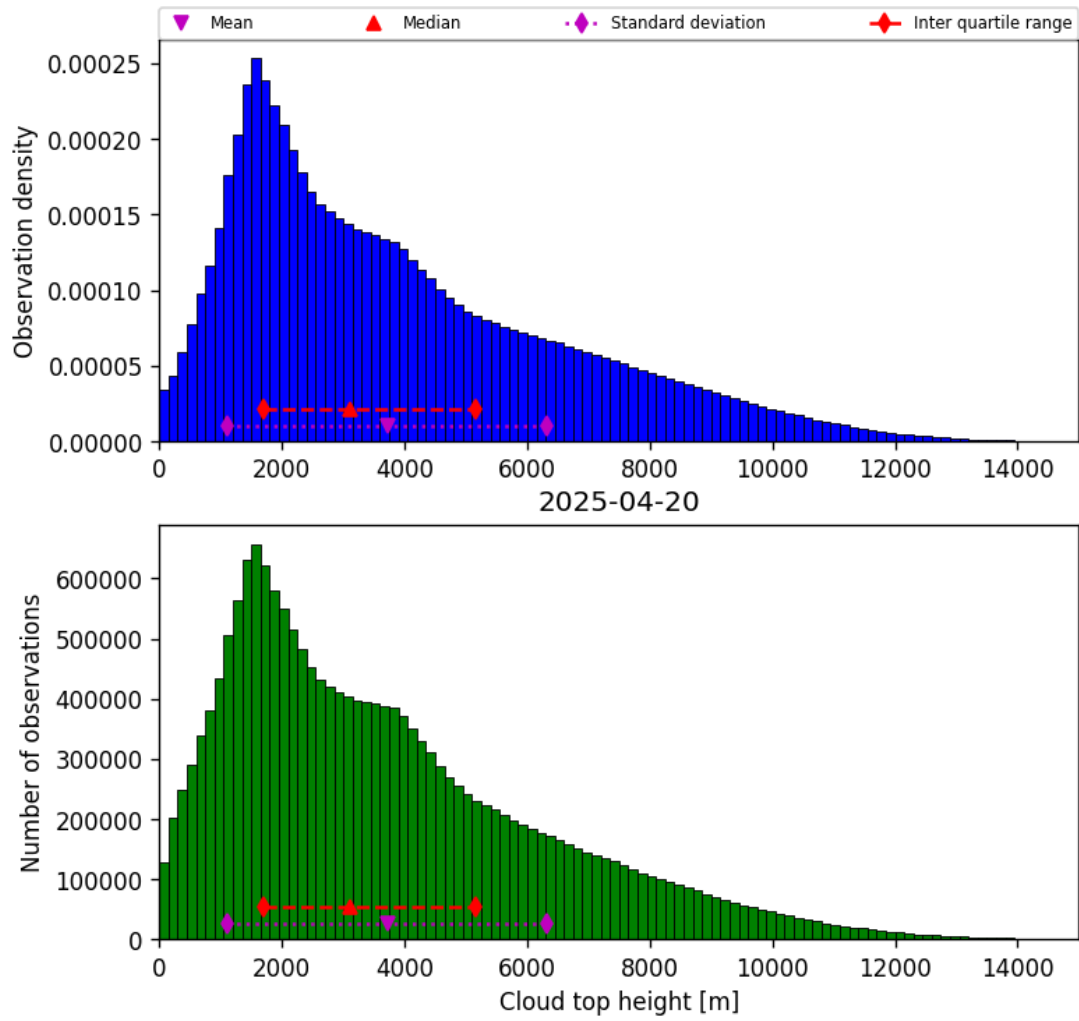
Figure 38: Histogram of “Cloud top height” for 2025-04-20 to 2025-04-21
