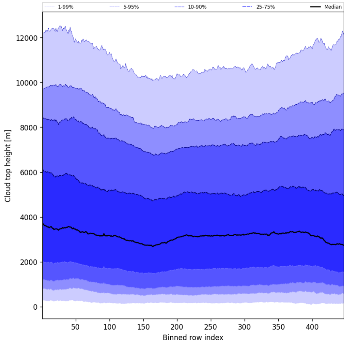
Figure 54: Along track statistics of “Cloud top height” for 2025-04-21 to 2025-04-22
