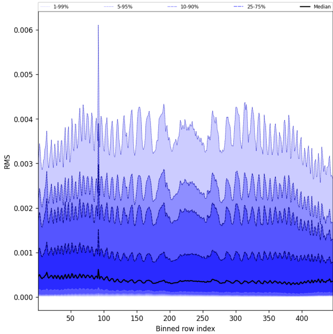
Figure 61: Along track statistics of “RMS” for 2025-04-21 to 2025-04-22
