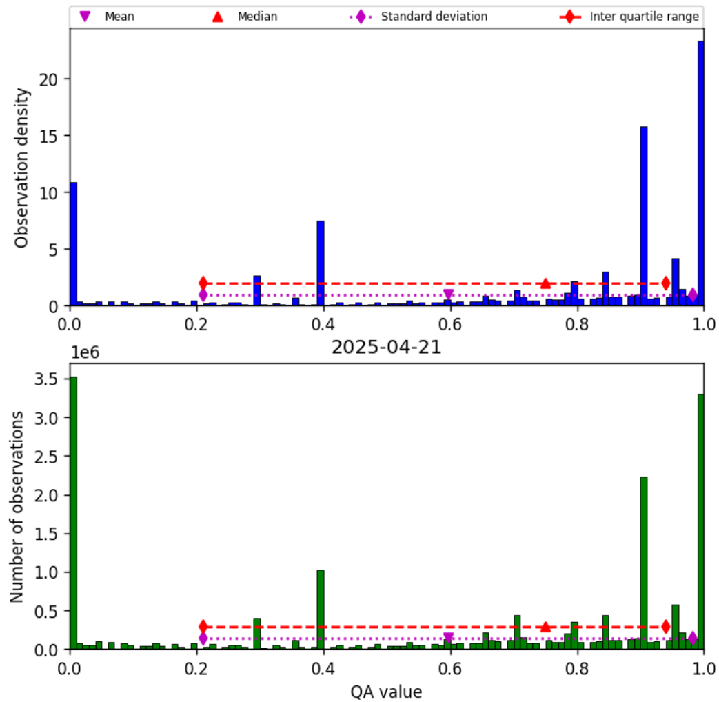
Figure 36: Histogram of “QA value” for 2025-04-21 to 2025-04-22
