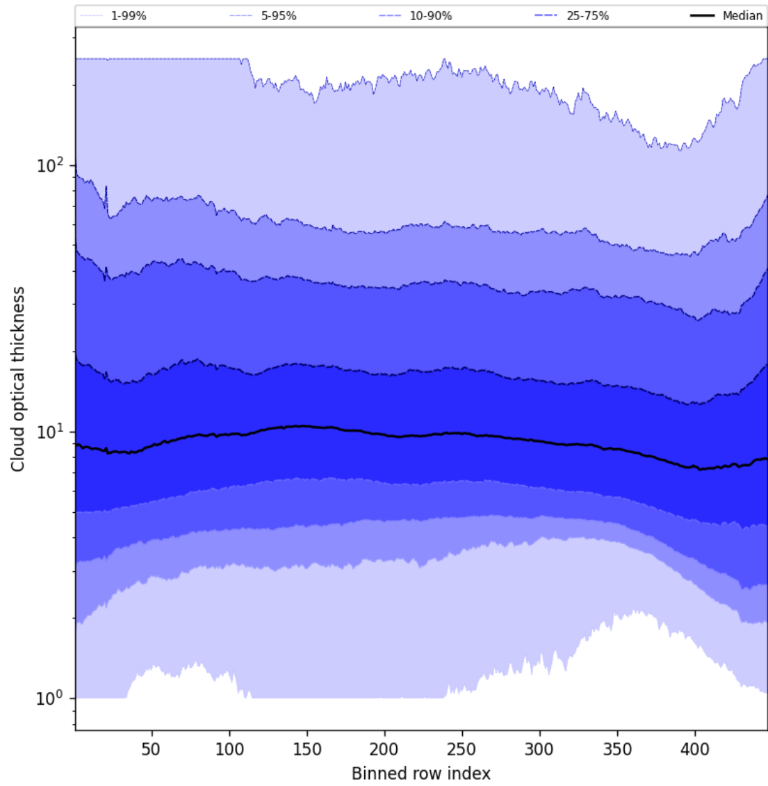
Figure 55: Along track statistics of “Cloud optical thickness” for 2025-04-21 to 2025-04-22
