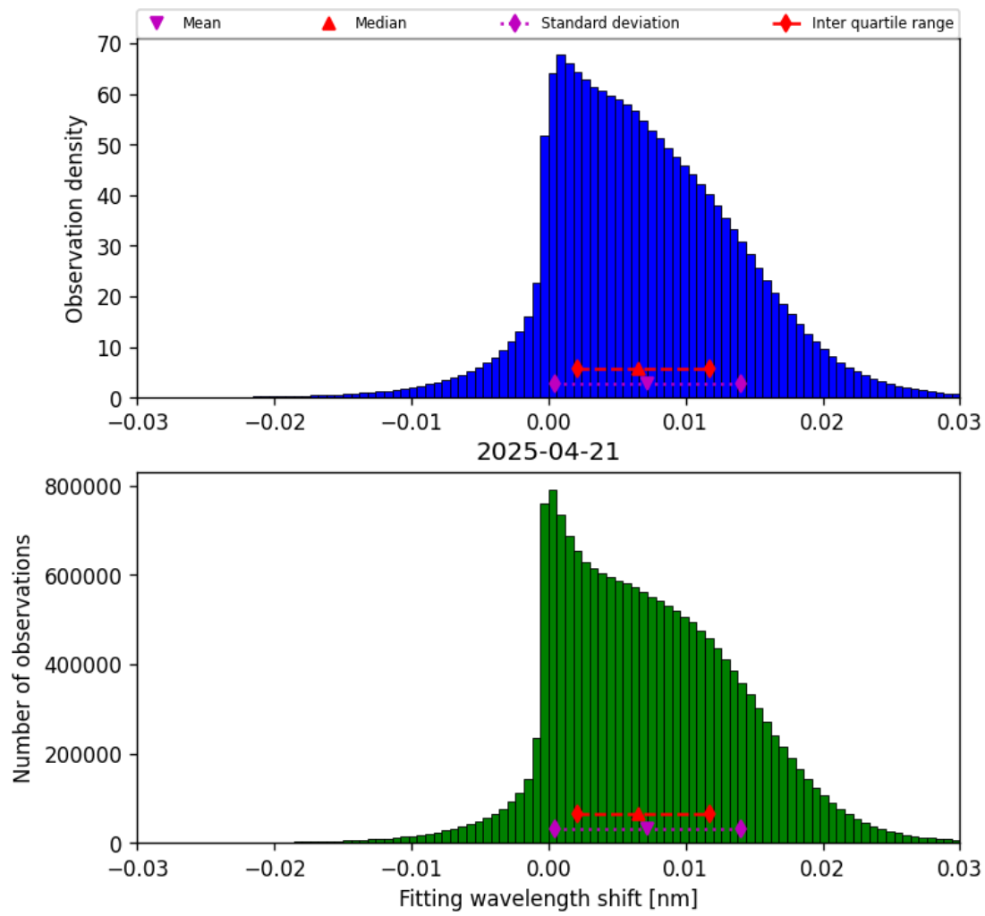
Figure 47: Histogram of “Fitting wavelength shift” for 2025-04-21 to 2025-04-22
