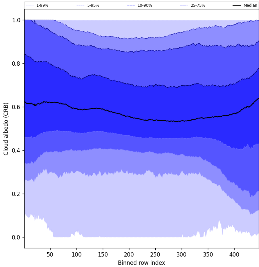
Figure 58: Along track statistics of “Cloud albedo (CRB)” for 2025-04-21 to 2025-04-22
