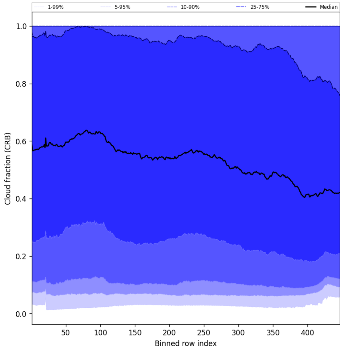
Figure 56: Along track statistics of “Cloud fraction (CRB)” for 2025-04-21 to 2025-04-22
