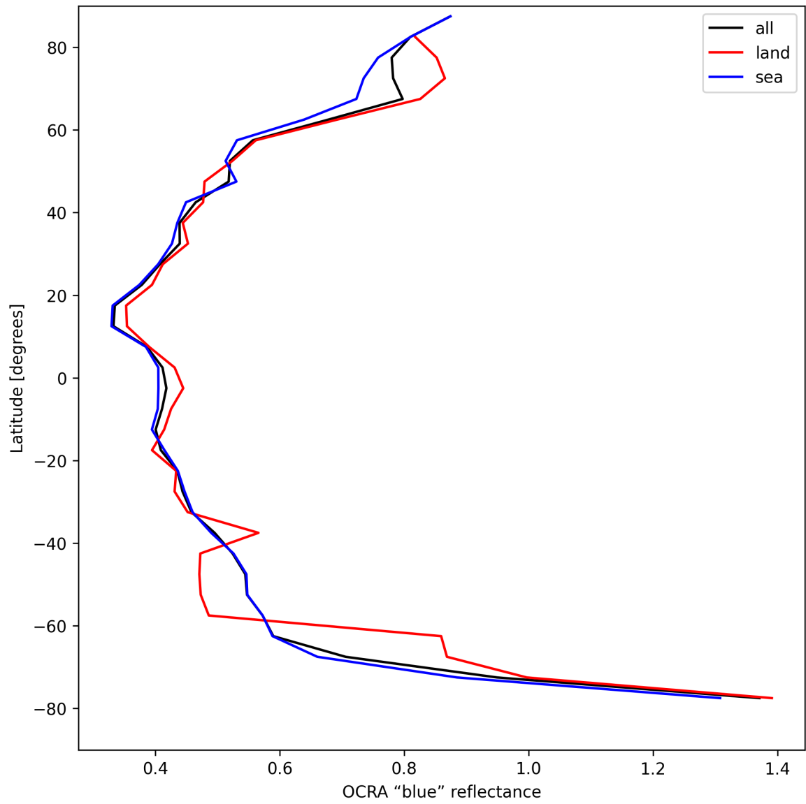
Figure 33: Zonal average of "OCRA "blue" reflectance" for 2025-04-21 to 2025-04-22.
