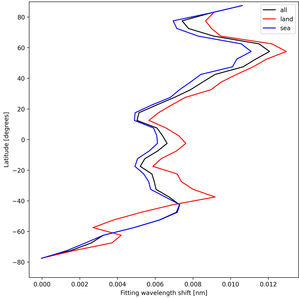
Figure 31: Zonal average of “Fitting wavelength shift” for 2025-04-21 to 2025-04-22.
