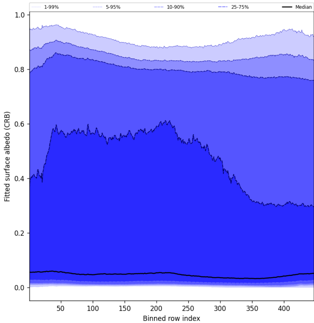
Figure 60: Along track statistics of “Fitted surface albedo (CRB)” for 2025-04-21 to 2025-04-22
