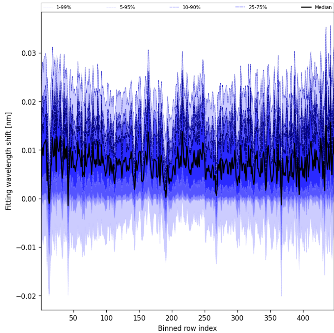
Figure 63: Along track statistics of “Fitting wavelength shift” for 2025-04-21 to 2025-04-22
