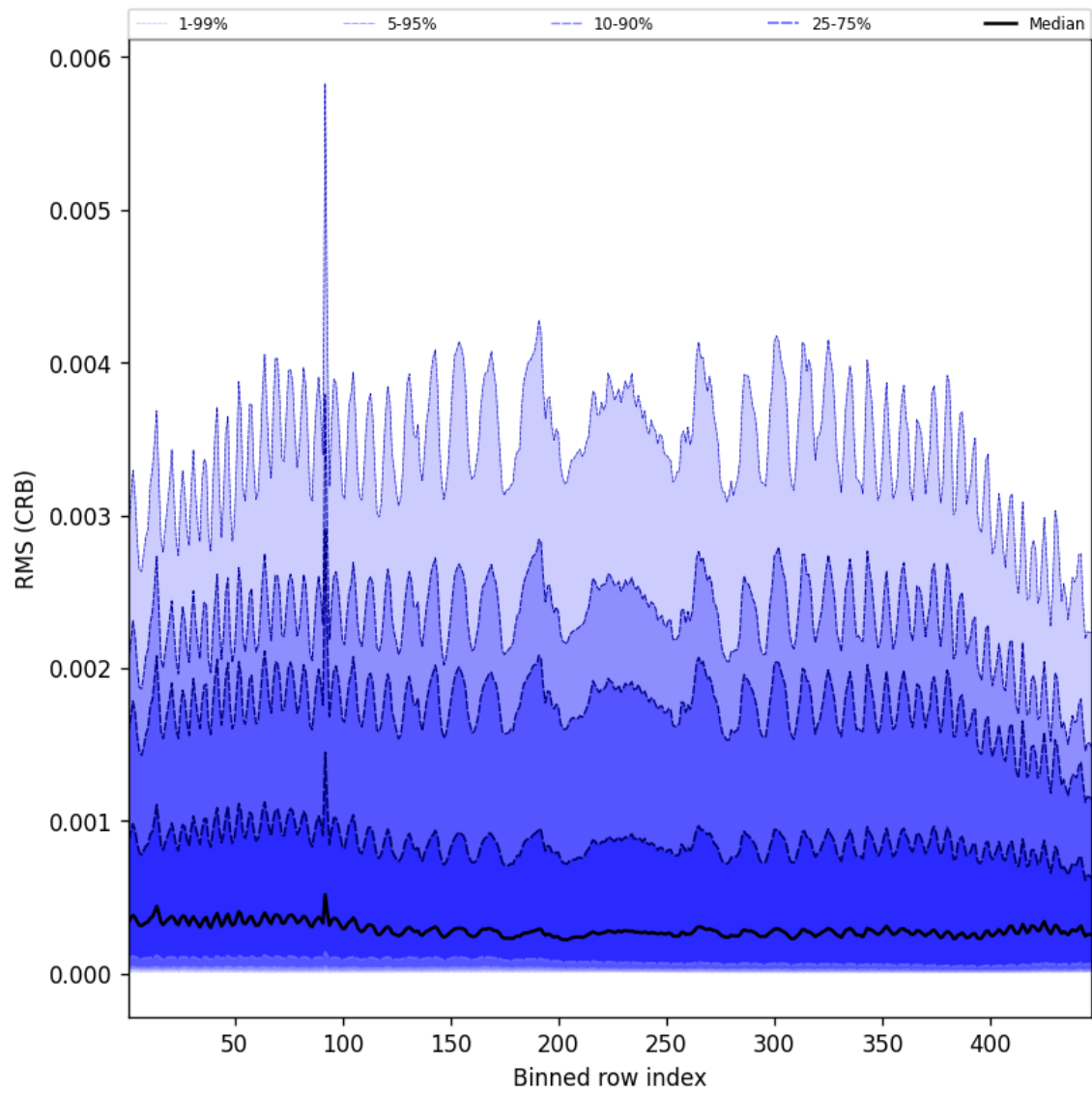
Figure 62: Along track statistics of “RMS (CRB)” for 2025-04-21 to 2025-04-22
