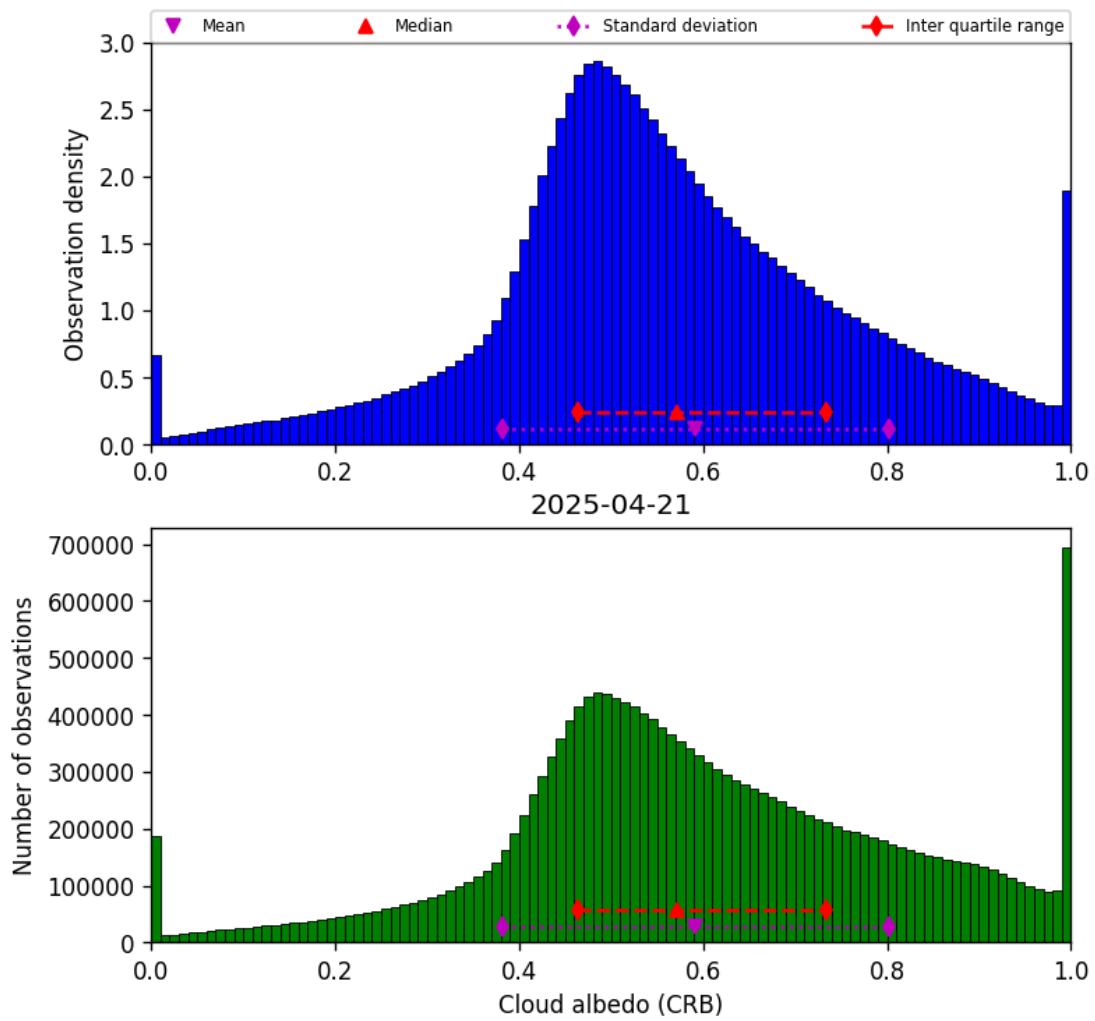
Figure 42: Histogram of “Cloud albedo (CRB)” for 2025-04-21 to 2025-04-22
