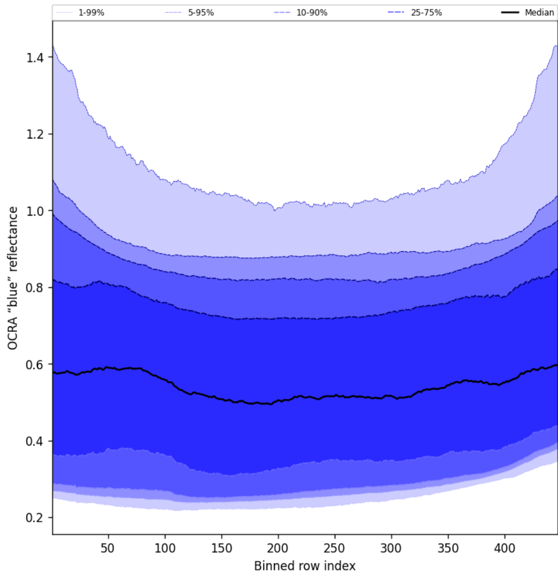
Figure 65: Along track statistics of “OCRA “blue” reflectance” for 2025-04-21 to 2025-04-22
