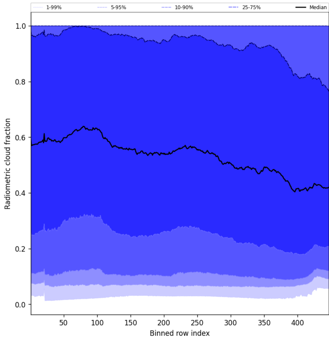
Figure 53: Along track statistics of “Radiometric cloud fraction” for 2025-04-21 to 2025-04-22
