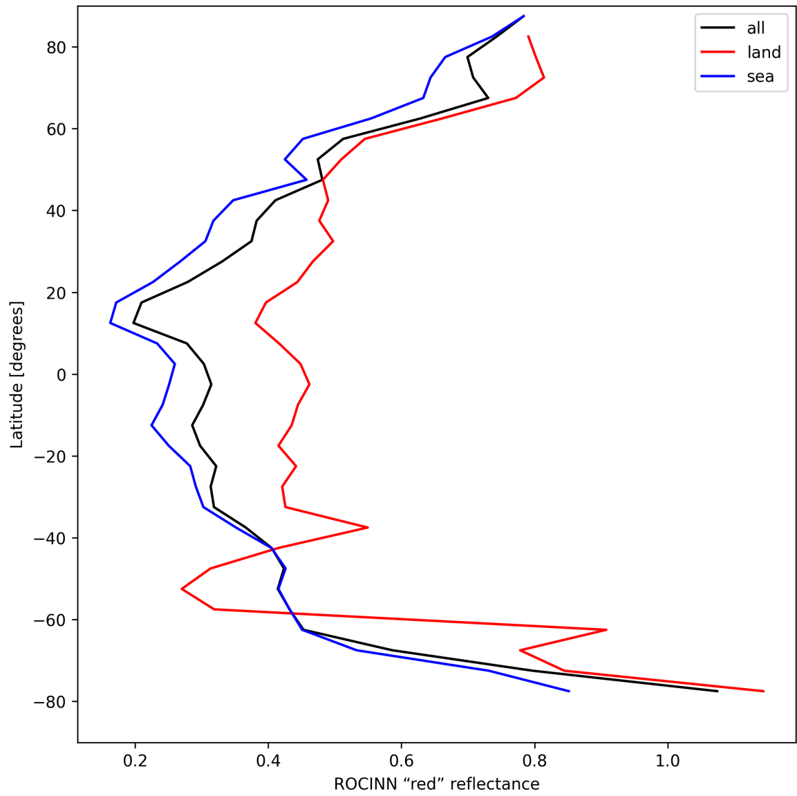
Figure 35: Zonal average of “ROCINN “red” reflectance” for 2025-04-21 to 2025-04-22.
