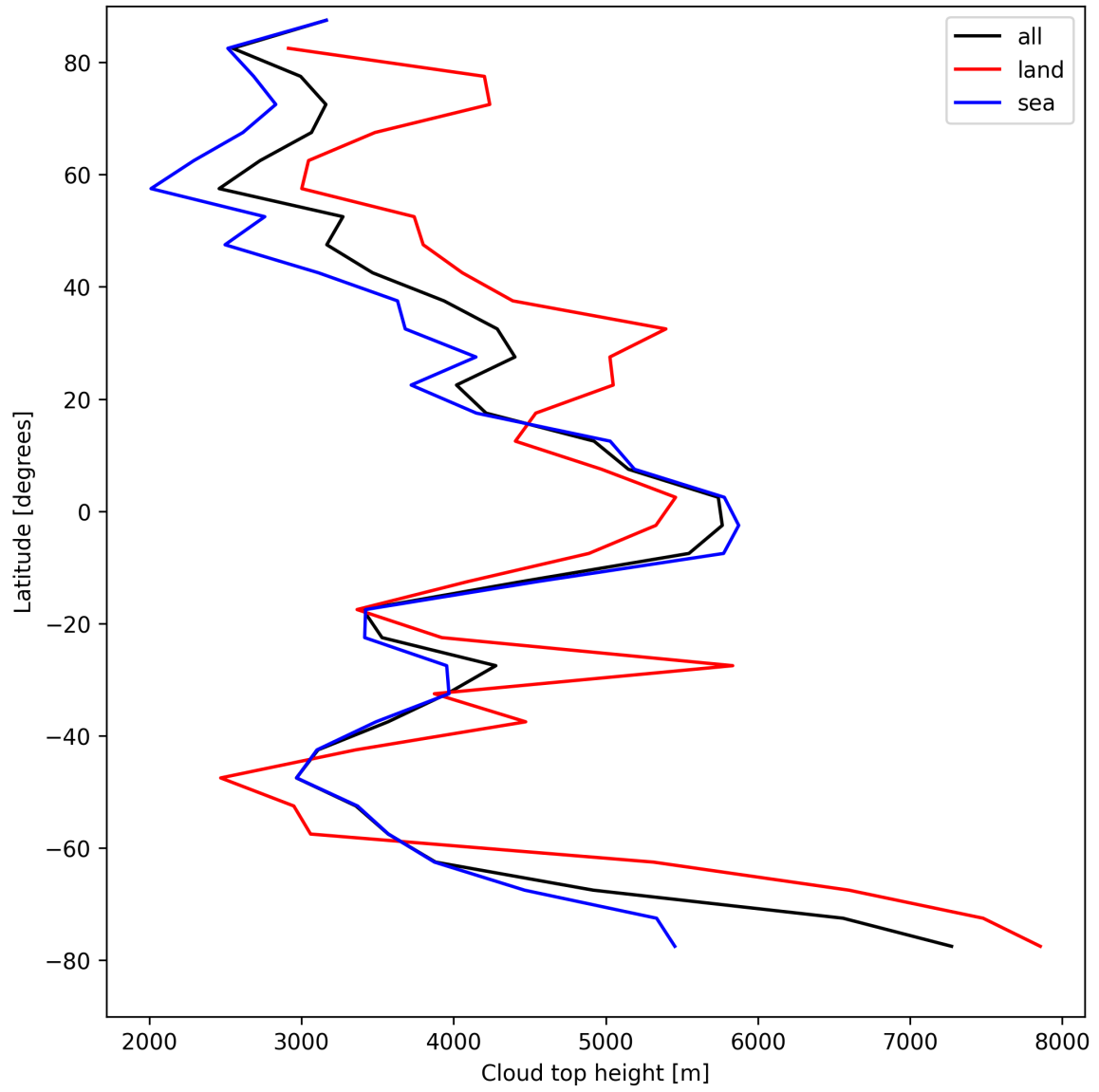
Figure 22: Zonal average of “Cloud top height” for 2025-04-21 to 2025-04-22.
