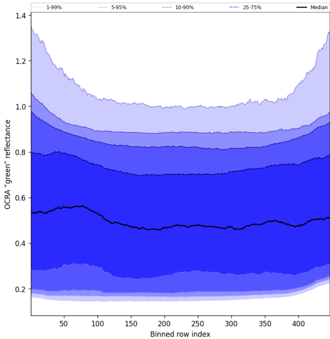
Figure 66: Along track statistics of “OCRA “green” reflectance” for 2025-04-21 to 2025-04-22
