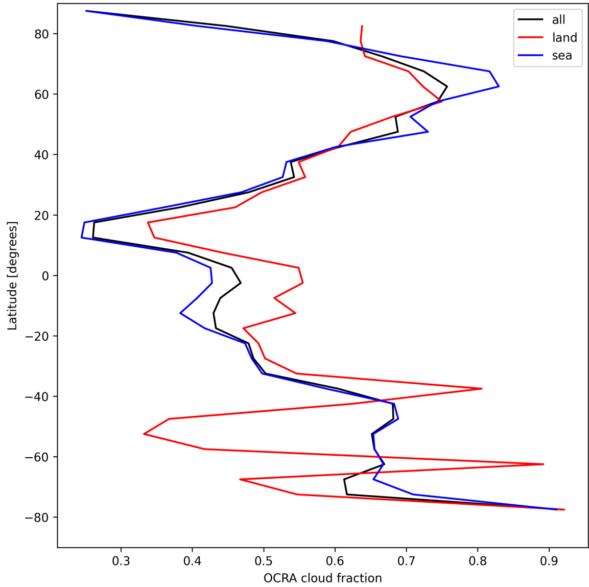
Figure 32: Zonal average of “OCRA cloud fraction” for 2025-04-21 to 2025-04-22.
