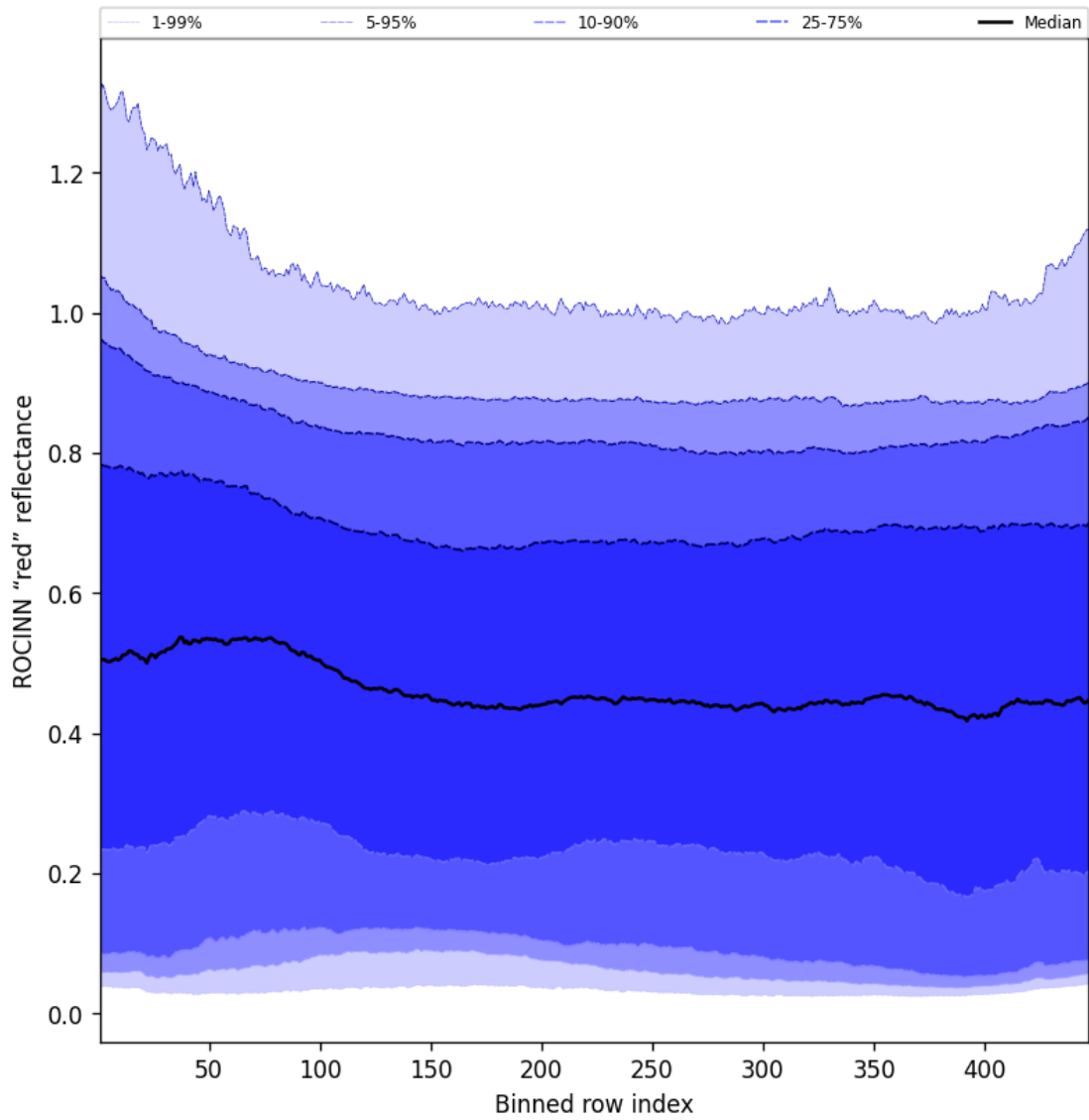
Figure 67: Along track statistics of “ROCINN “red” reflectance” for 2025-04-21 to 2025-04-22
