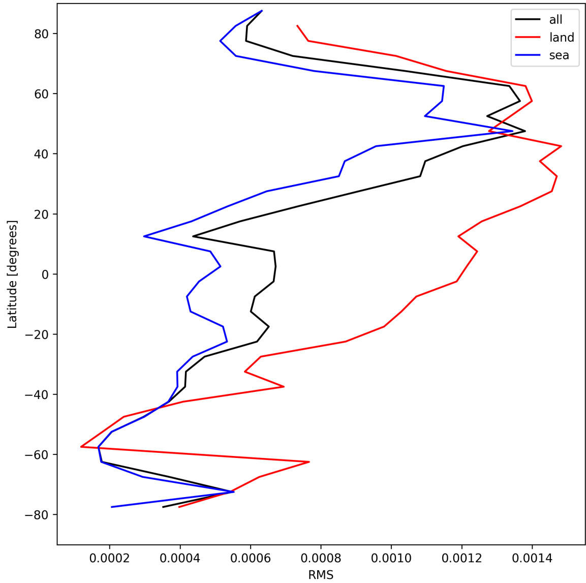
Figure 29: Zonal average of “RMS” for 2025-04-21 to 2025-04-22.
