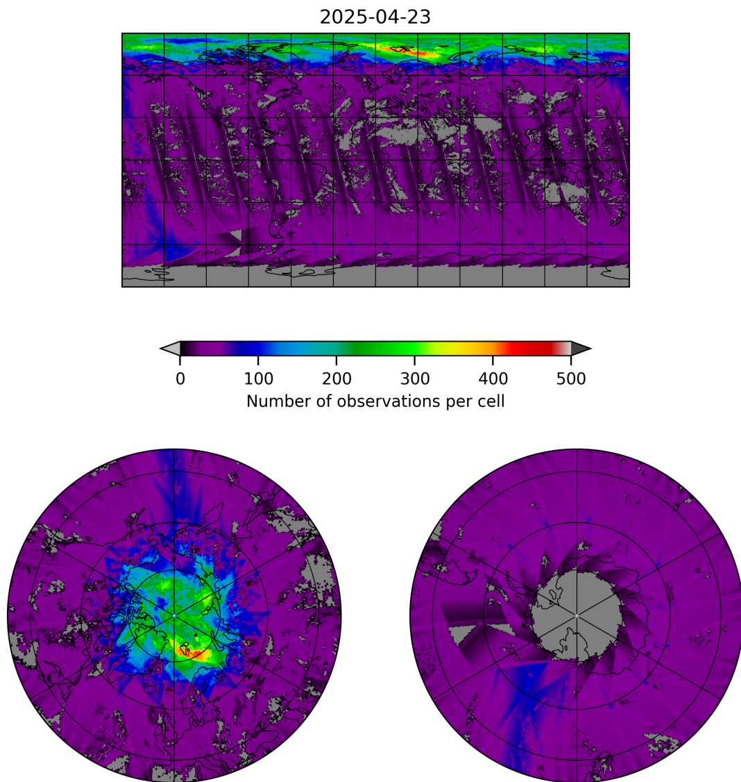
Figure 19: Map of the number of observations for 2025-04-23 to 2025-04-24
