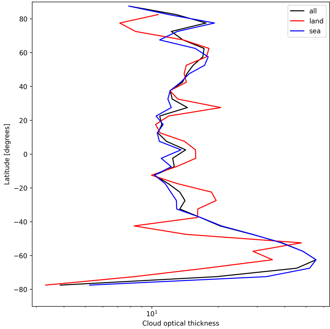
Figure 23: Zonal average of “Cloud optical thickness” for 2025-04-23 to 2025-04-24.
