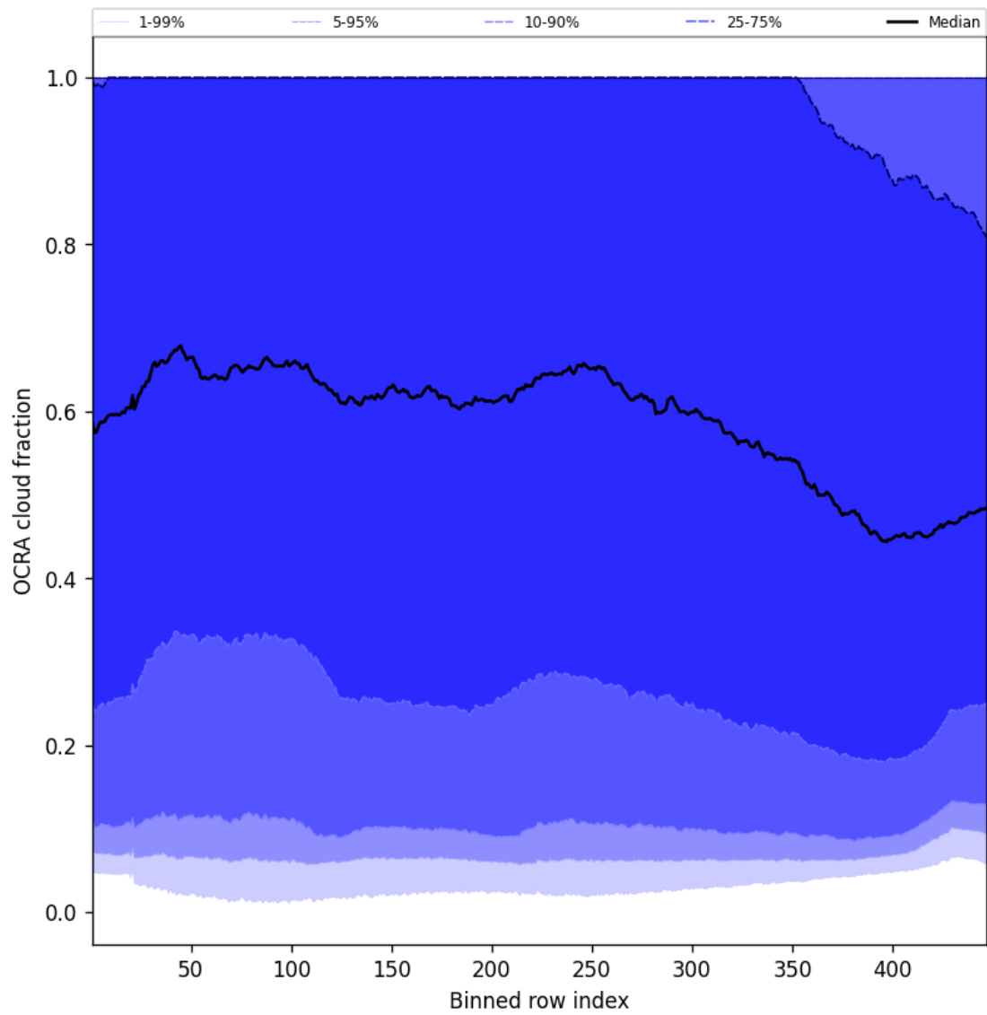
Figure 64: Along track statistics of “OCRA cloud fraction” for 2025-04-23 to 2025-04-24
