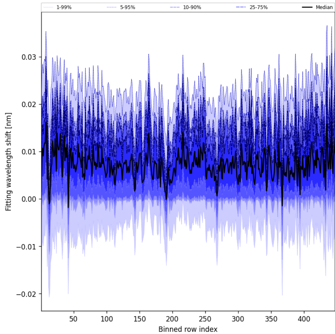
Figure 63: Along track statistics of “Fitting wavelength shift” for 2025-04-23 to 2025-04-24
