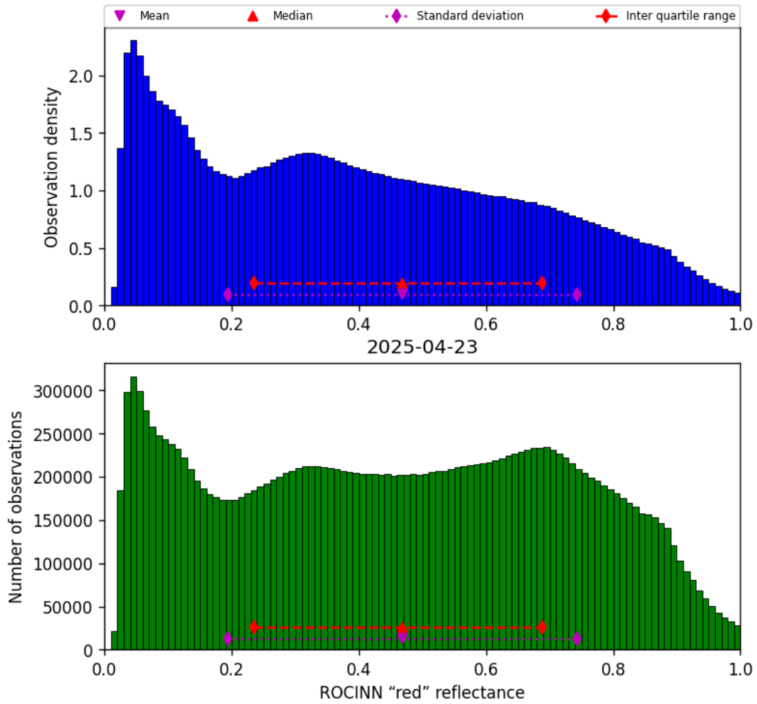
Figure 51: Histogram of “ROCINN “red” reflectance” for 2025-04-23 to 2025-04-24
