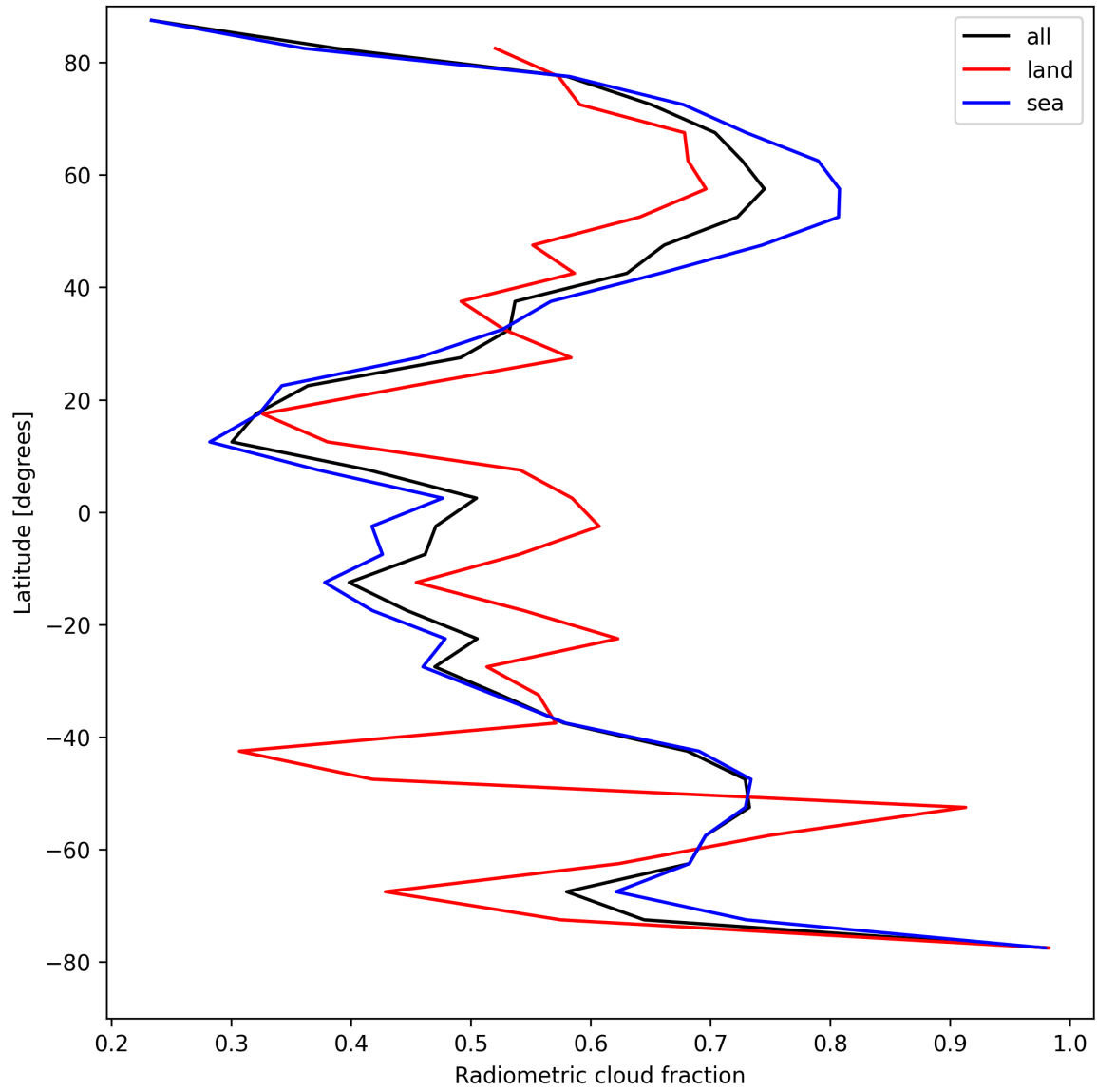
Figure 21: Zonal average of “Radiometric cloud fraction” for 2025-04-23 to 2025-04-24.
