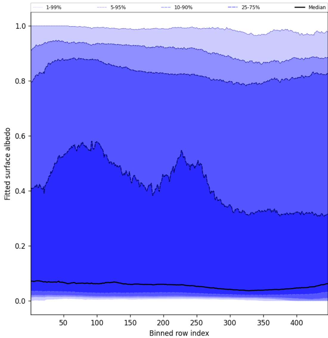
Figure 59: Along track statistics of “Fitted surface albedo” for 2025-04-23 to 2025-04-24
