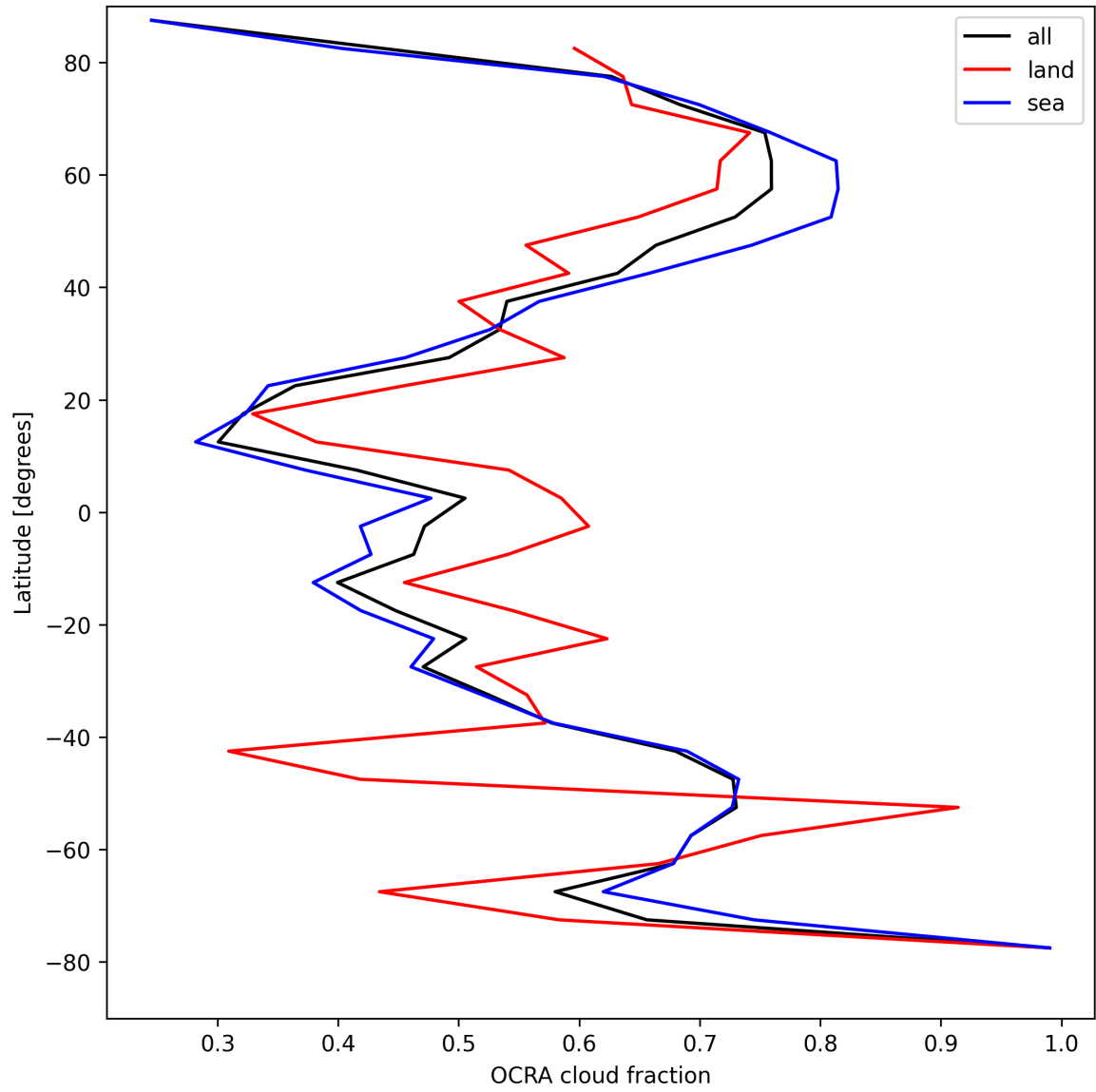
Figure 32: Zonal average of “OCRA cloud fraction” for 2025-04-23 to 2025-04-24.
