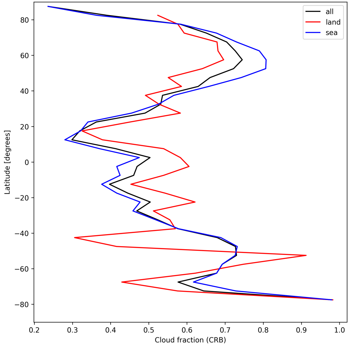
Figure 24: Zonal average of “Cloud fraction (CRB)” for 2025-04-23 to 2025-04-24.
