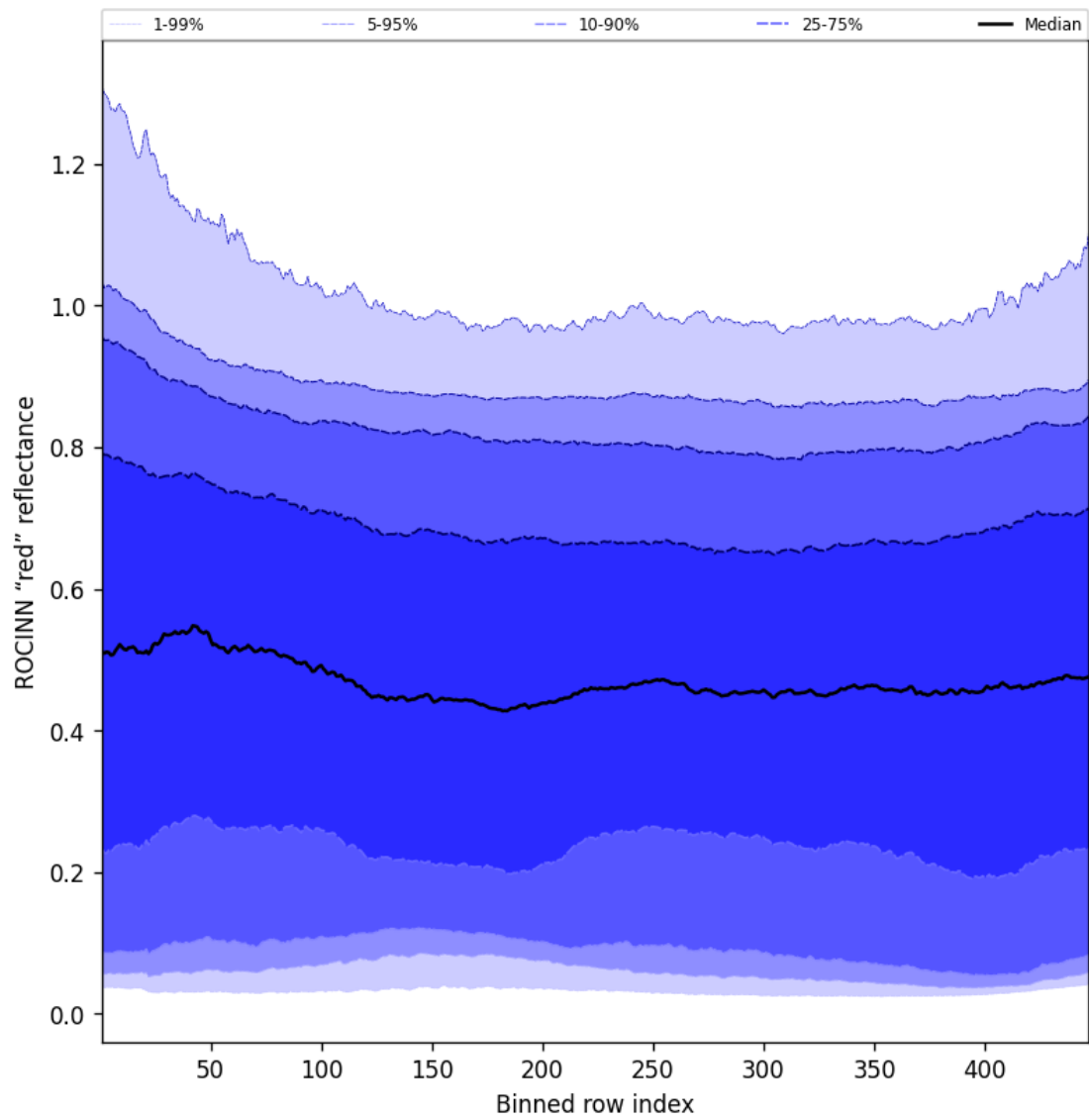
Figure 67: Along track statistics of "ROCINN "red" reflectance" for 2025-04-23 to 2025-04-24
