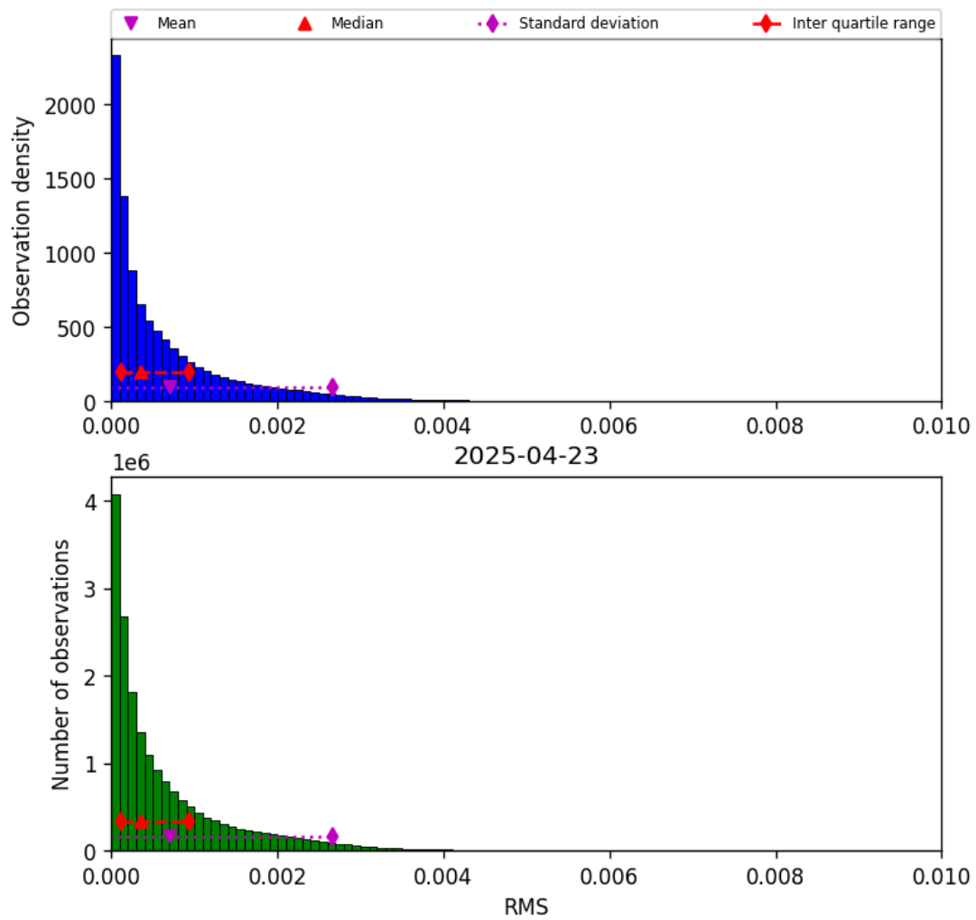
Figure 45: Histogram of “RMS” for 2025-04-23 to 2025-04-24
