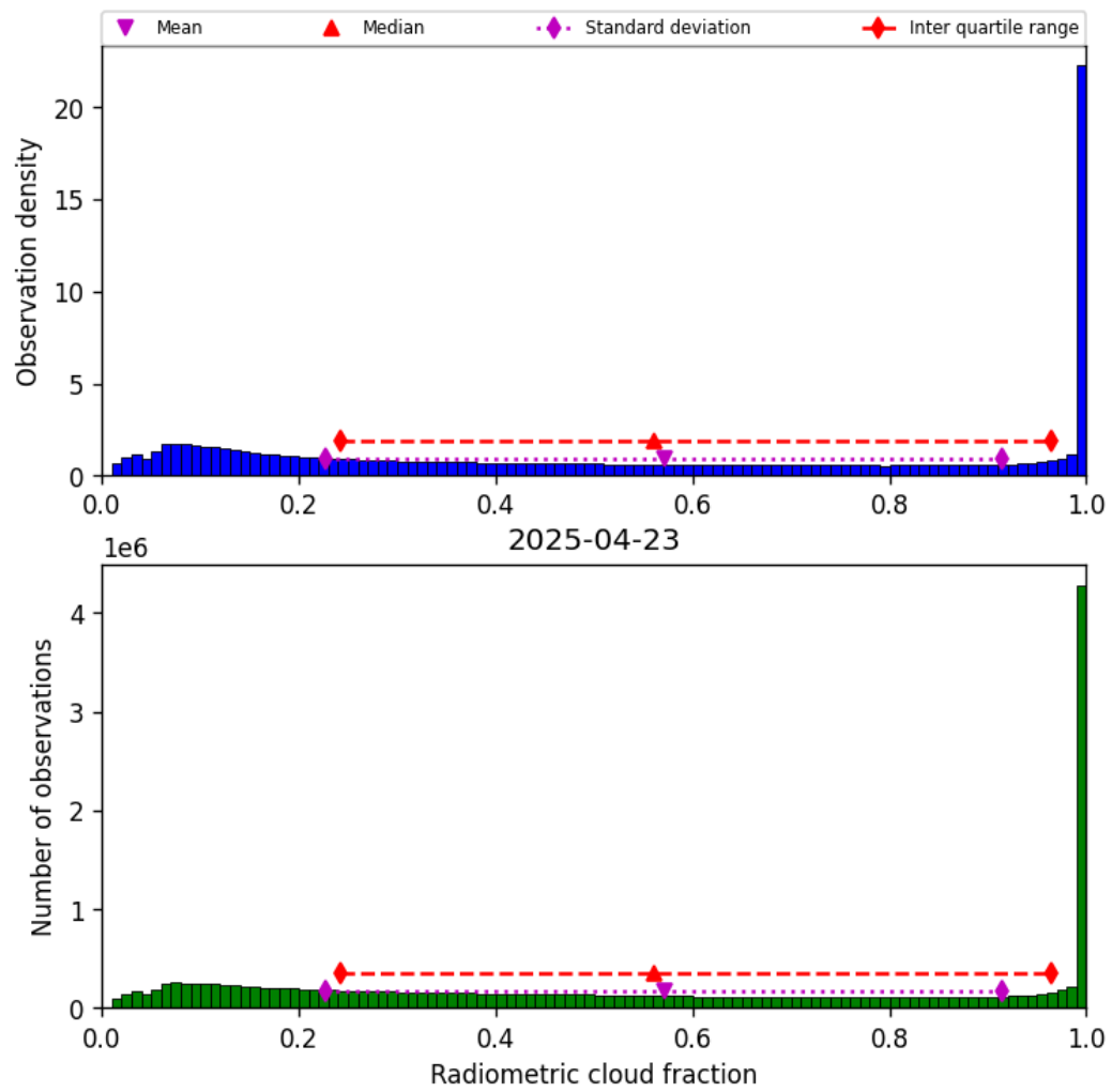
Figure 37: Histogram of “Radiometric cloud fraction” for 2025-04-23 to 2025-04-24
