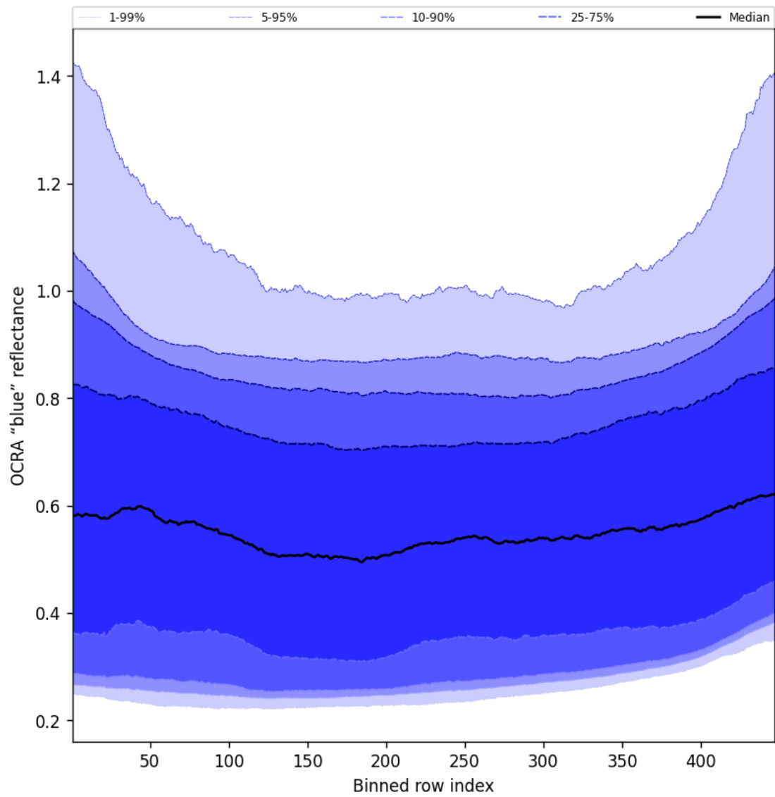
Figure 65: Along track statistics of “OCRA “blue” reflectance” for 2025-04-23 to 2025-04-24
