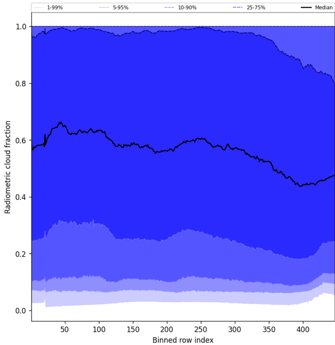
Figure 53: Along track statistics of “Radiometric cloud fraction” for 2025-04-23 to 2025-04-24
