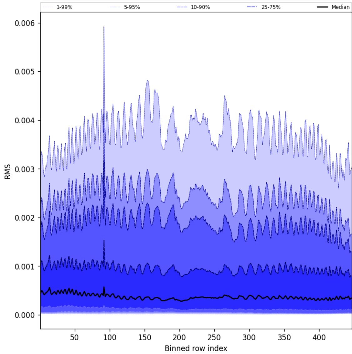
Figure 61: Along track statistics of “RMS” for 2025-04-23 to 2025-04-24
