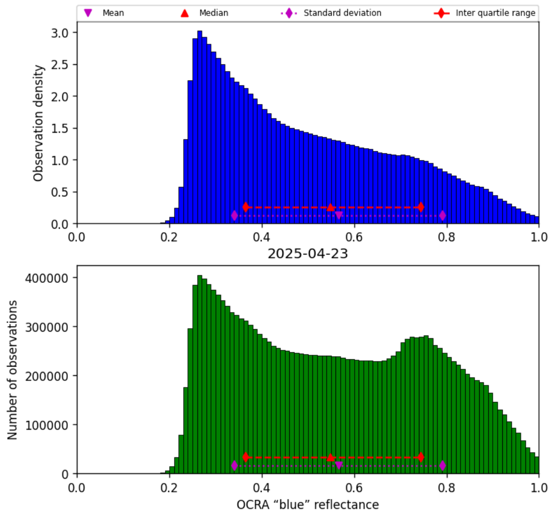
Figure 49: Histogram of “OCRA “blue” reflectance” for 2025-04-23 to 2025-04-24
