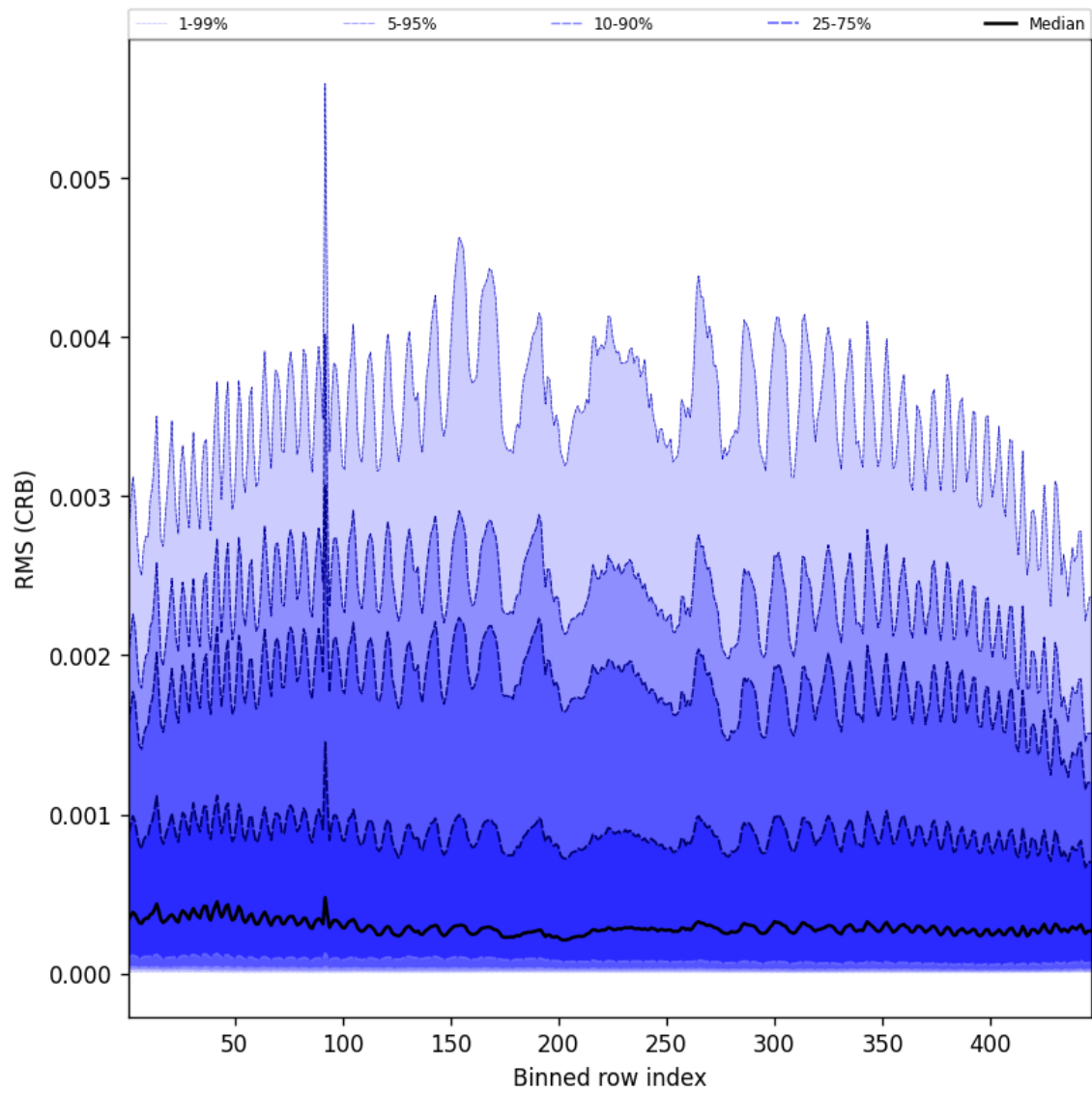
Figure 62: Along track statistics of “RMS (CRB)” for 2025-04-23 to 2025-04-24
