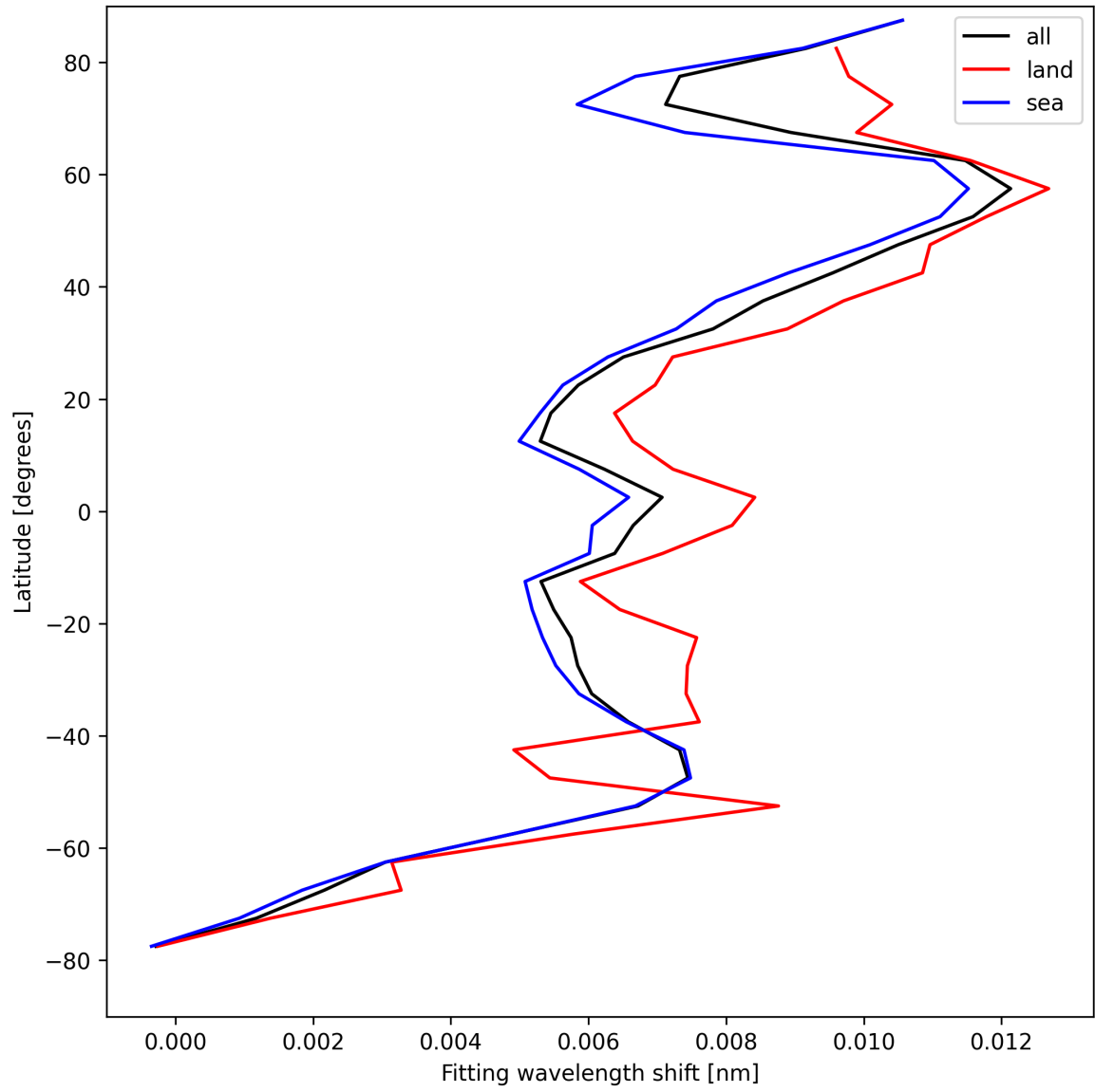
Figure 31: Zonal average of “Fitting wavelength shift” for 2025-04-23 to 2025-04-24.
