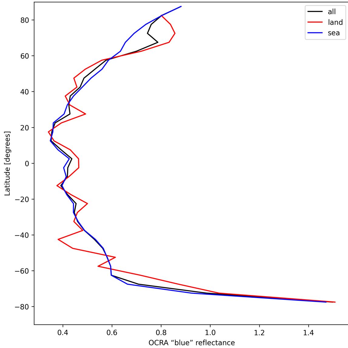
Figure 33: Zonal average of “OCRA “blue” reflectance” for 2025-04-23 to 2025-04-24.
