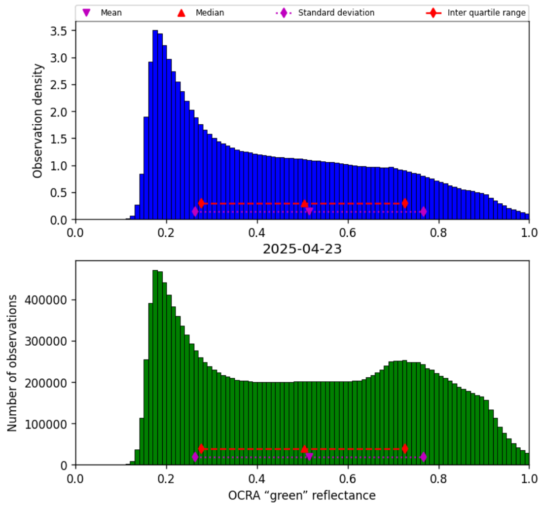
Figure 50: Histogram of “OCRA “green” reflectance” for 2025-04-23 to 2025-04-24
