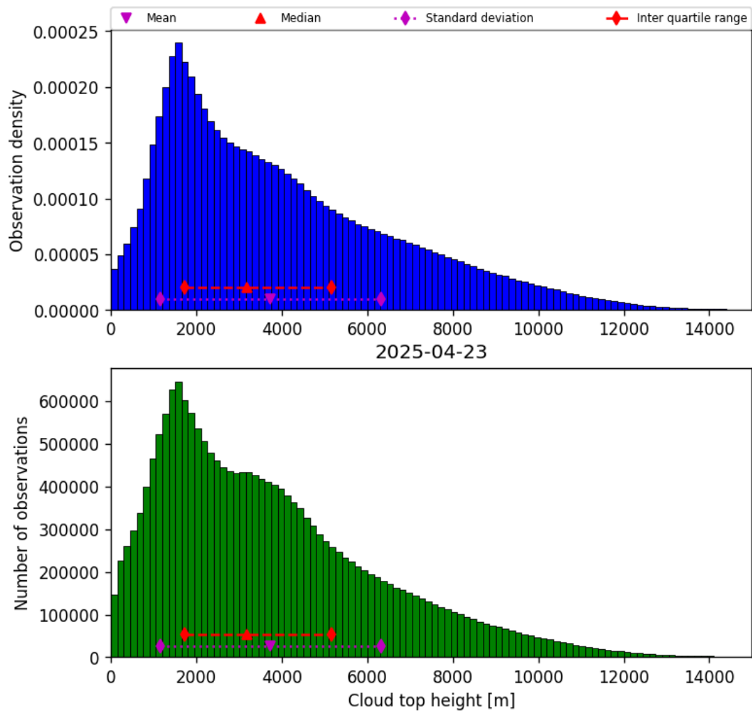
Figure 38: Histogram of “Cloud top height” for 2025-04-23 to 2025-04-24
