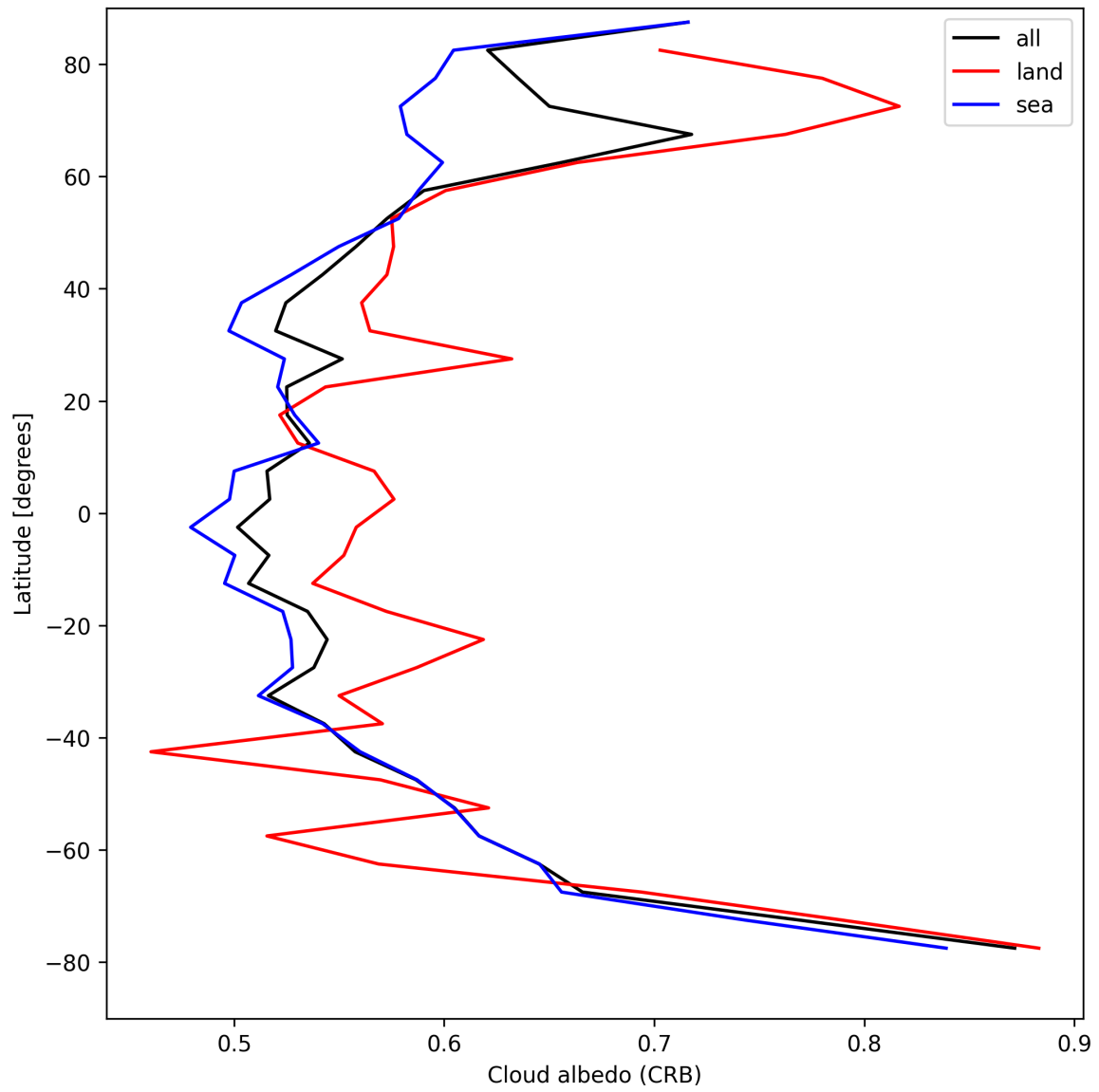
Figure 26: Zonal average of “Cloud albedo (CRB)” for 2025-04-23 to 2025-04-24.
