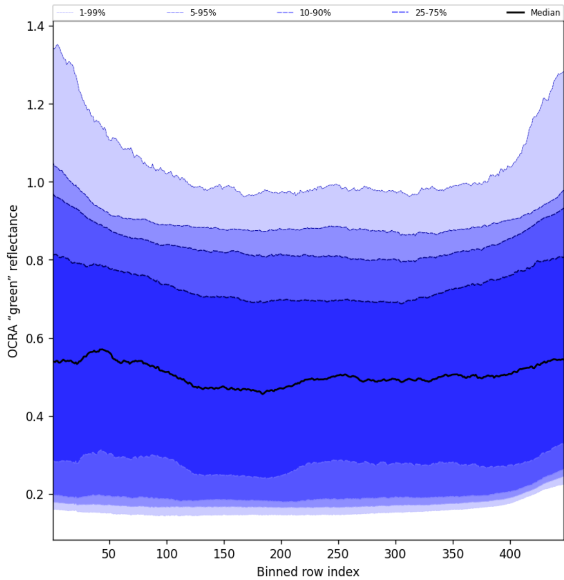
Figure 66: Along track statistics of “OCRA “green” reflectance” for 2025-04-23 to 2025-04-24
