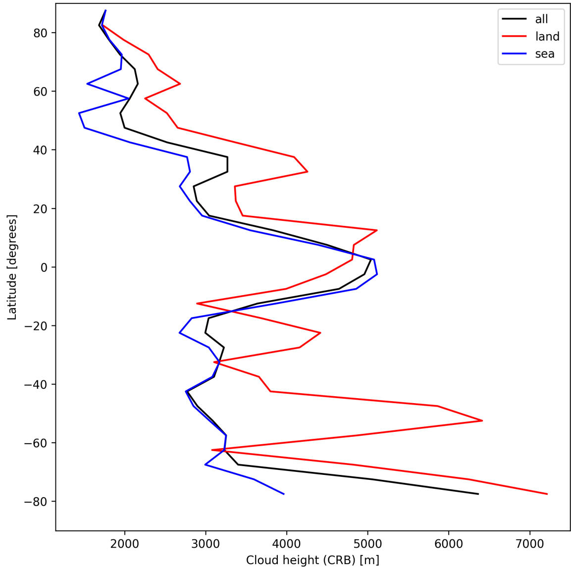
Figure 25: Zonal average of “Cloud height (CRB)” for 2025-04-23 to 2025-04-24.
