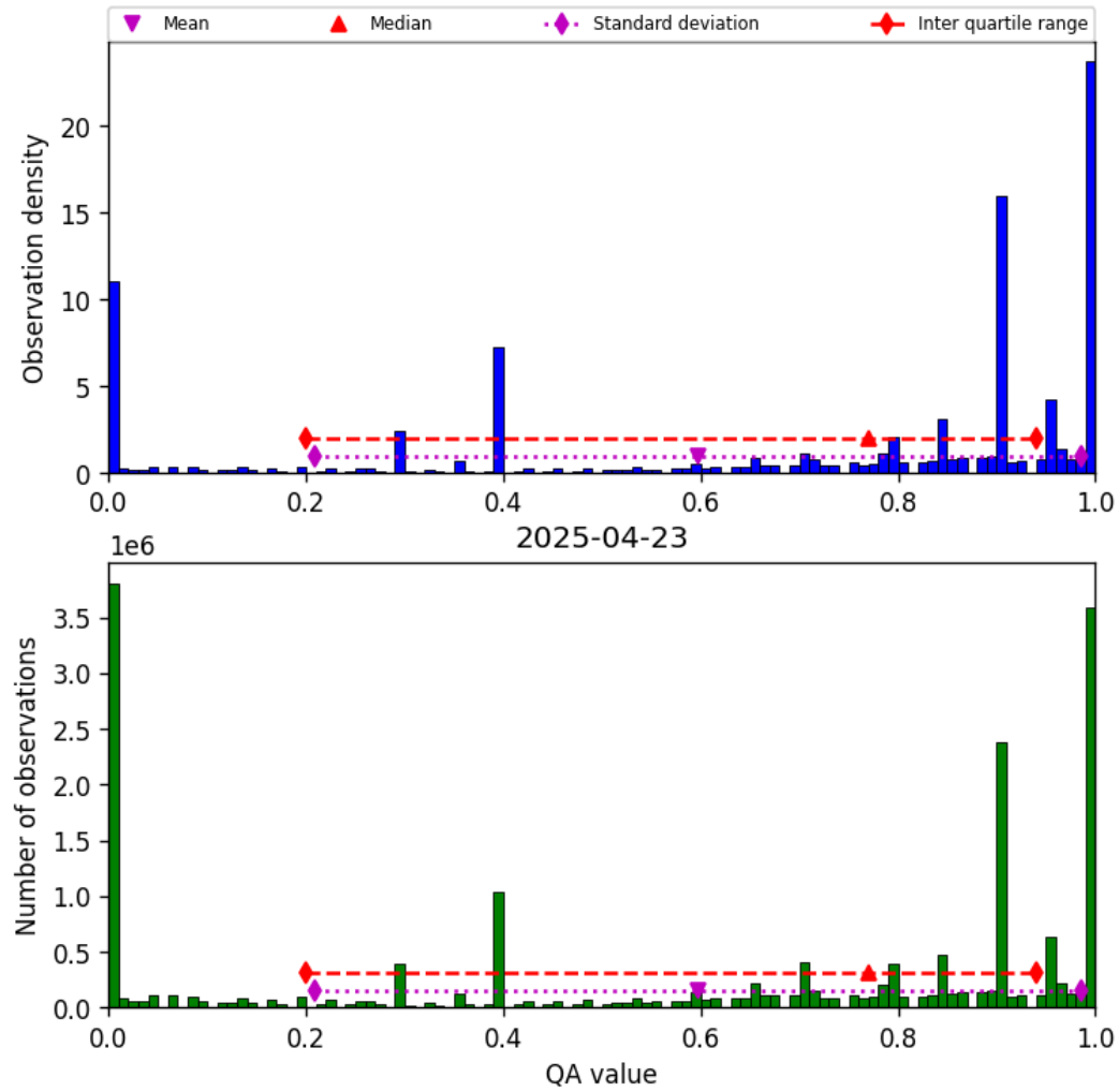
Figure 36: Histogram of “QA value” for 2025-04-23 to 2025-04-24
