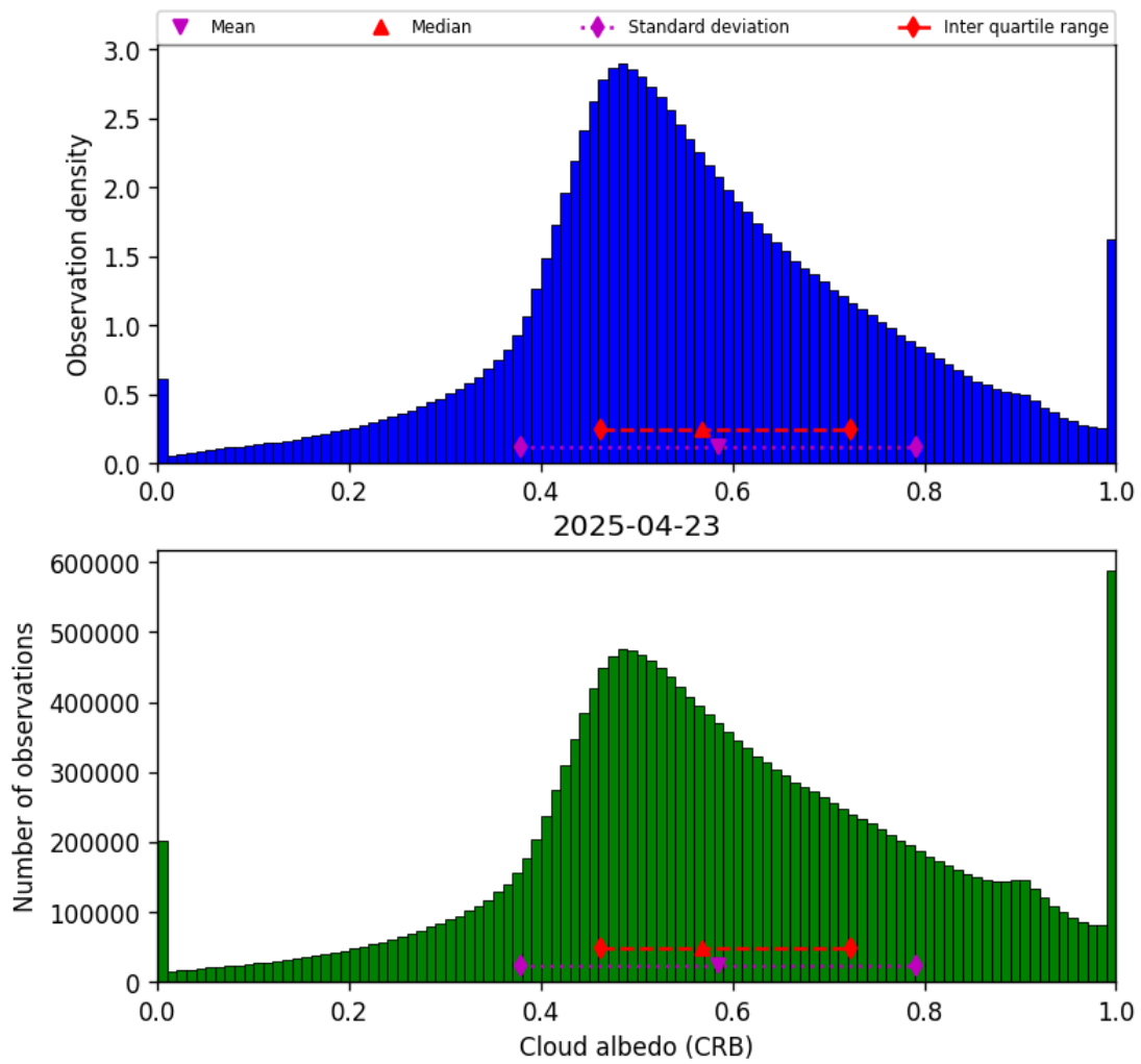
Figure 42: Histogram of “Cloud albedo (CRB)” for 2025-04-23 to 2025-04-24
