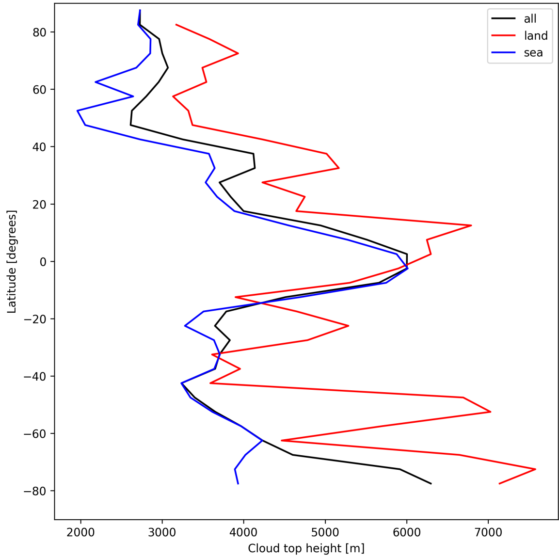
Figure 22: Zonal average of “Cloud top height” for 2025-04-23 to 2025-04-24.
