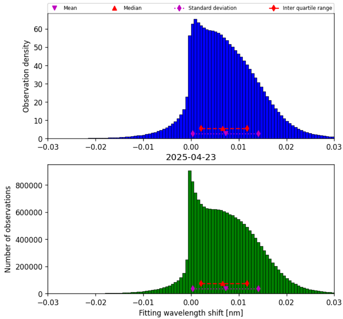
Figure 47: Histogram of “Fitting wavelength shift” for 2025-04-23 to 2025-04-24
