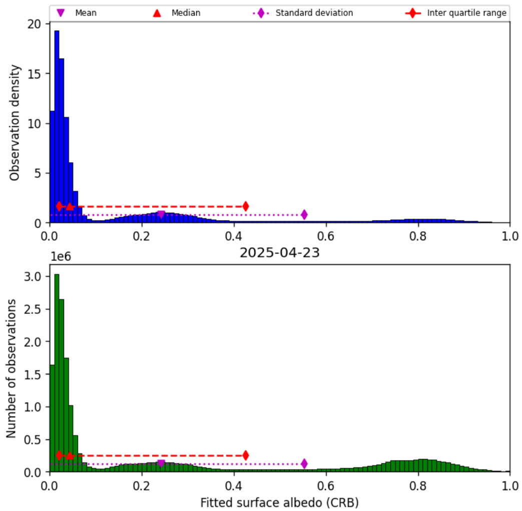
Figure 44: Histogram of “Fitted surface albedo (CRB)” for 2025-04-23 to 2025-04-24
