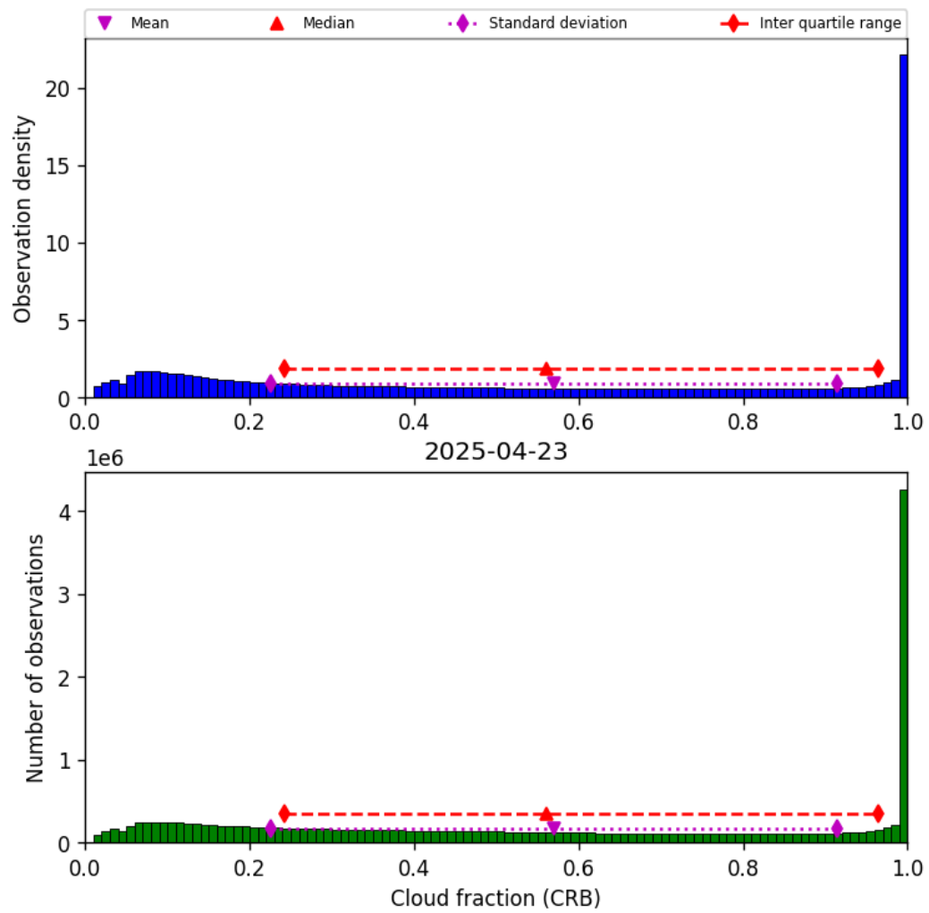
Figure 40: Histogram of “Cloud fraction (CRB)” for 2025-04-23 to 2025-04-24
