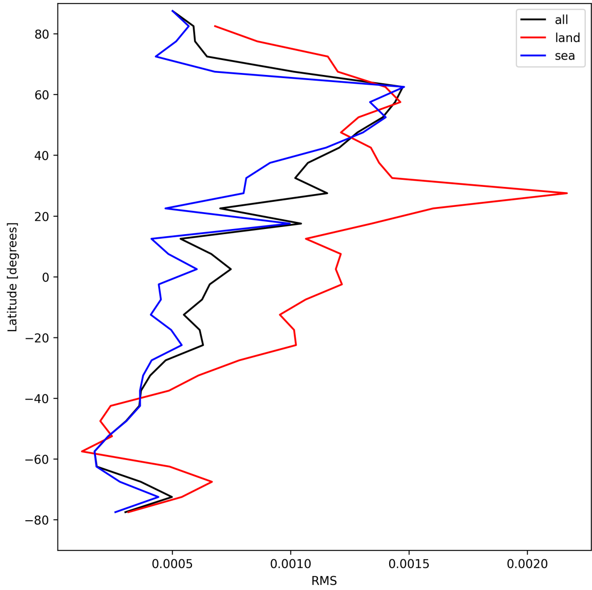
Figure 29: Zonal average of “RMS” for 2025-04-23 to 2025-04-24.
