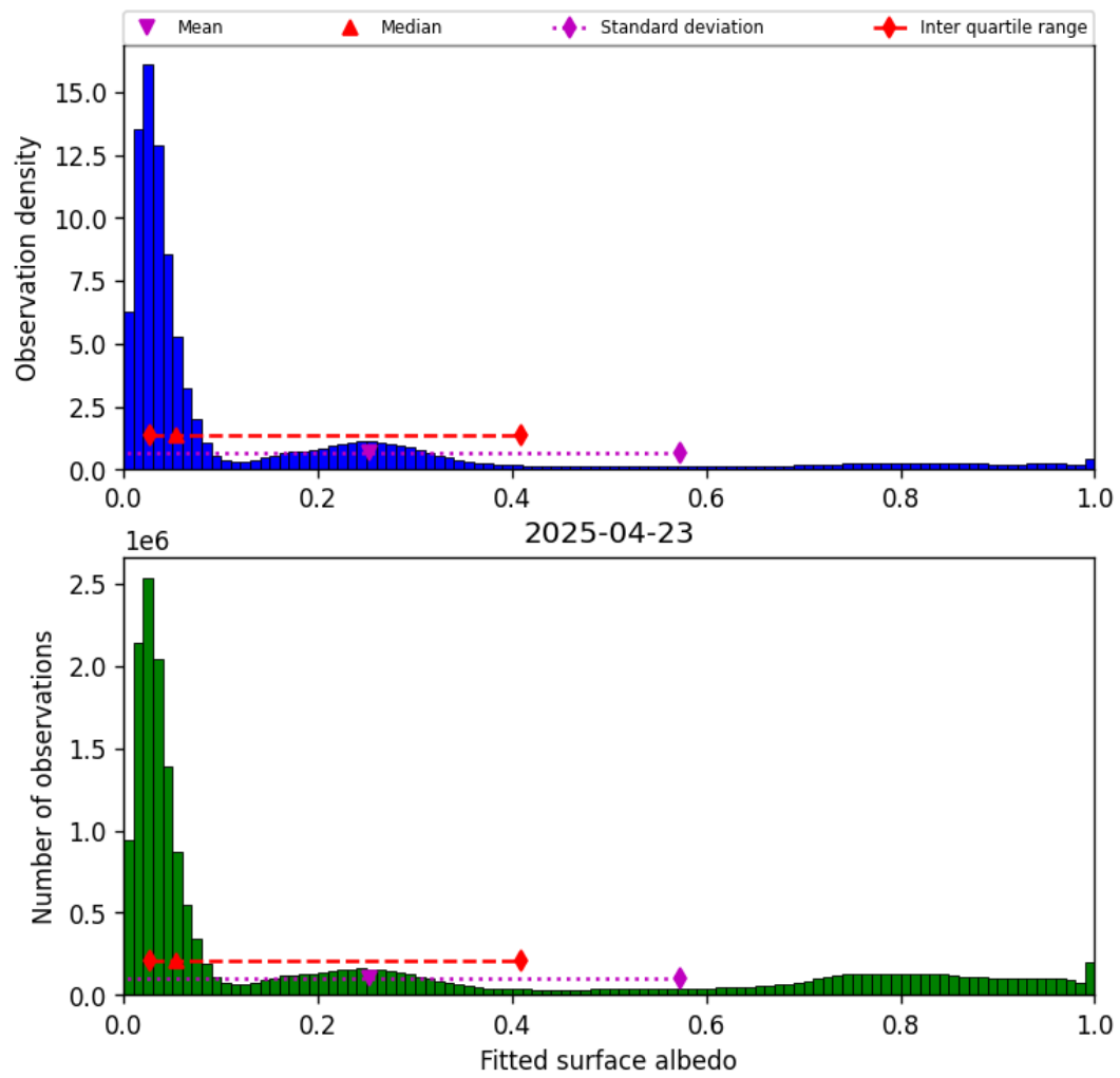
Figure 43: Histogram of “Fitted surface albedo” for 2025-04-23 to 2025-04-24
