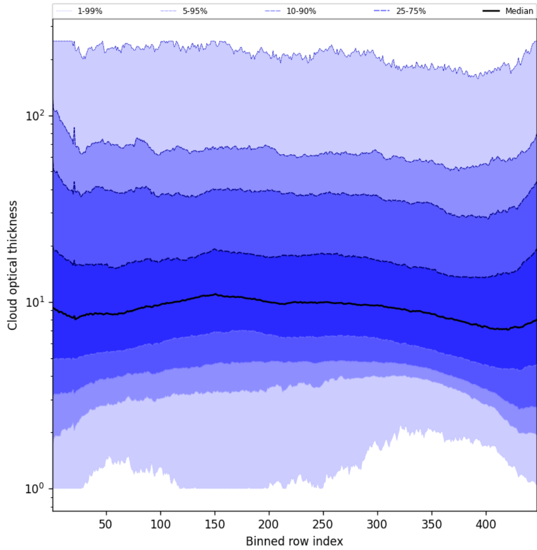
Figure 55: Along track statistics of “Cloud optical thickness” for 2025-04-23 to 2025-04-24
