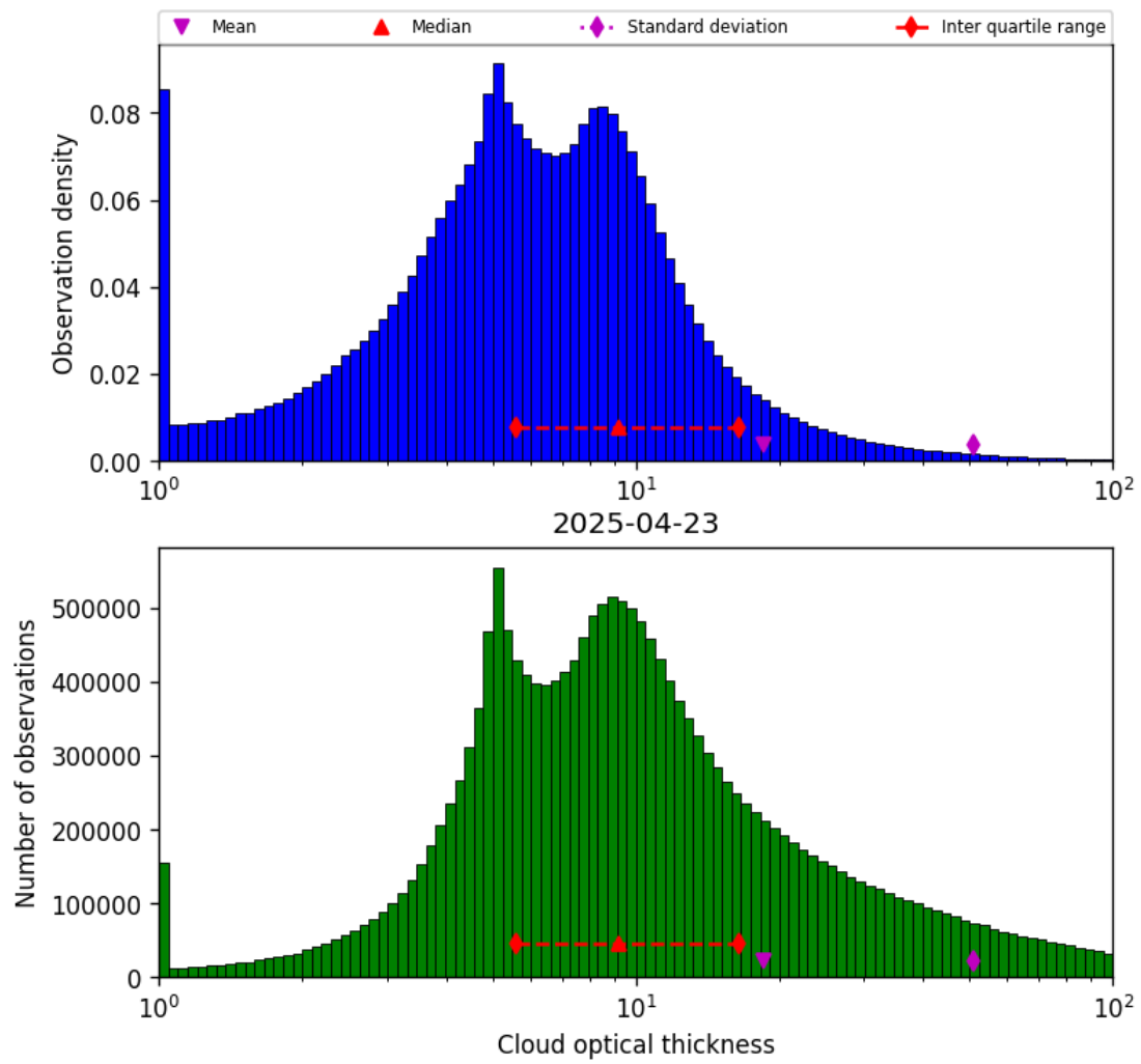
Figure 39: Histogram of “Cloud optical thickness” for 2025-04-23 to 2025-04-24
