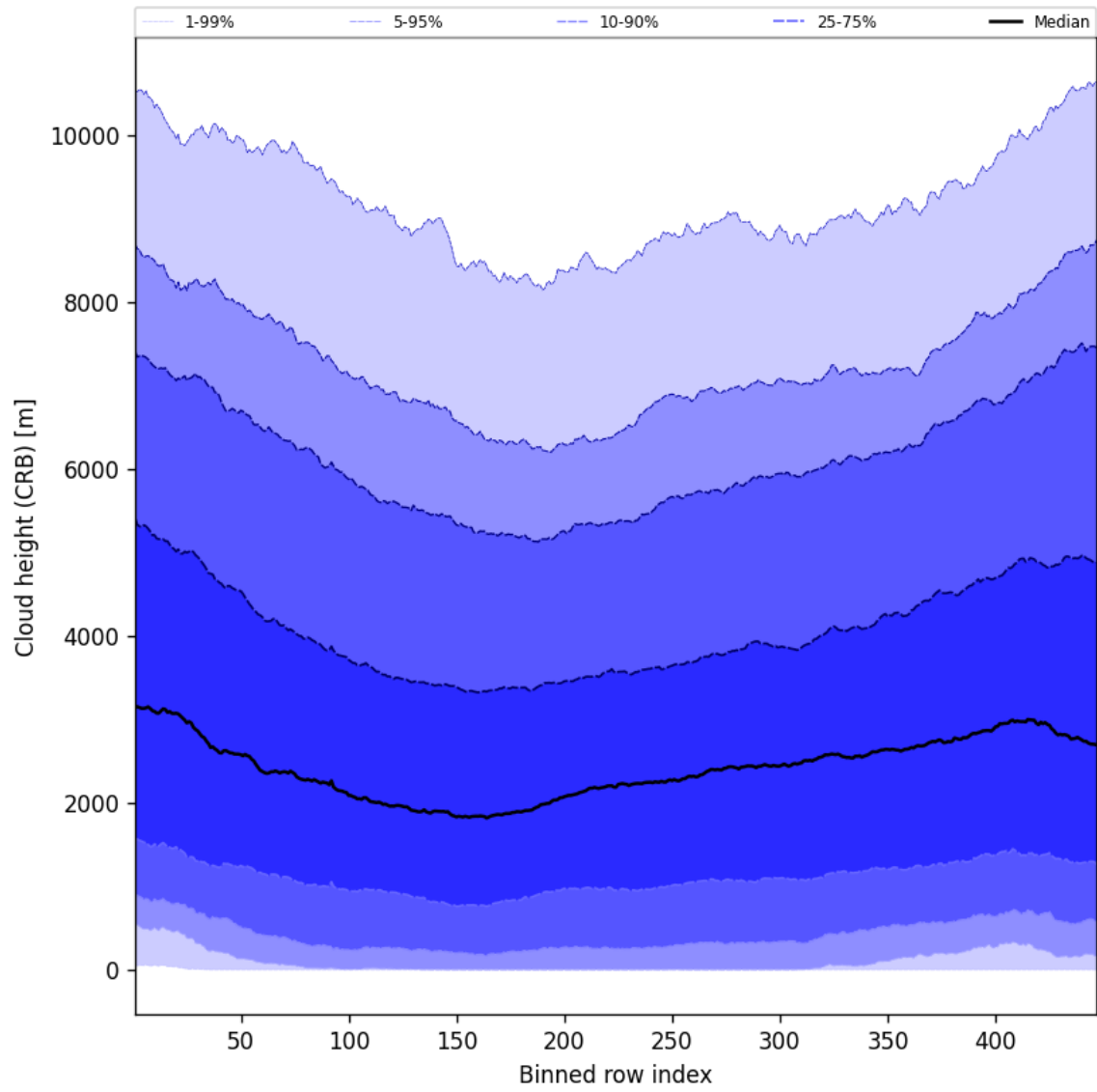
Figure 57: Along track statistics of “Cloud height (CRB)” for 2025-04-23 to 2025-04-24
