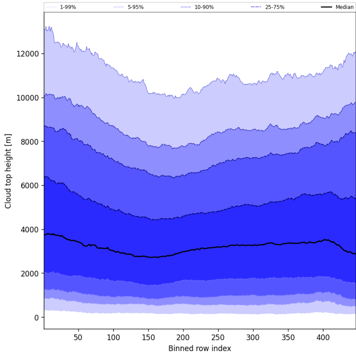
Figure 54: Along track statistics of “Cloud top height” for 2025-04-23 to 2025-04-24
