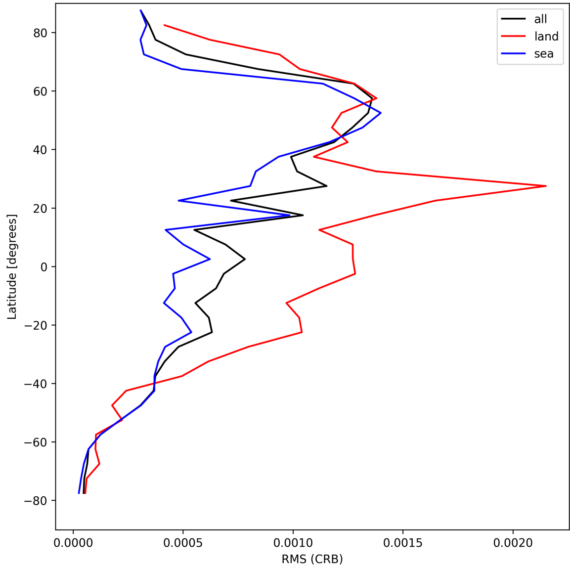
Figure 30: Zonal average of “RMS (CRB)” for 2025-04-23 to 2025-04-24.
