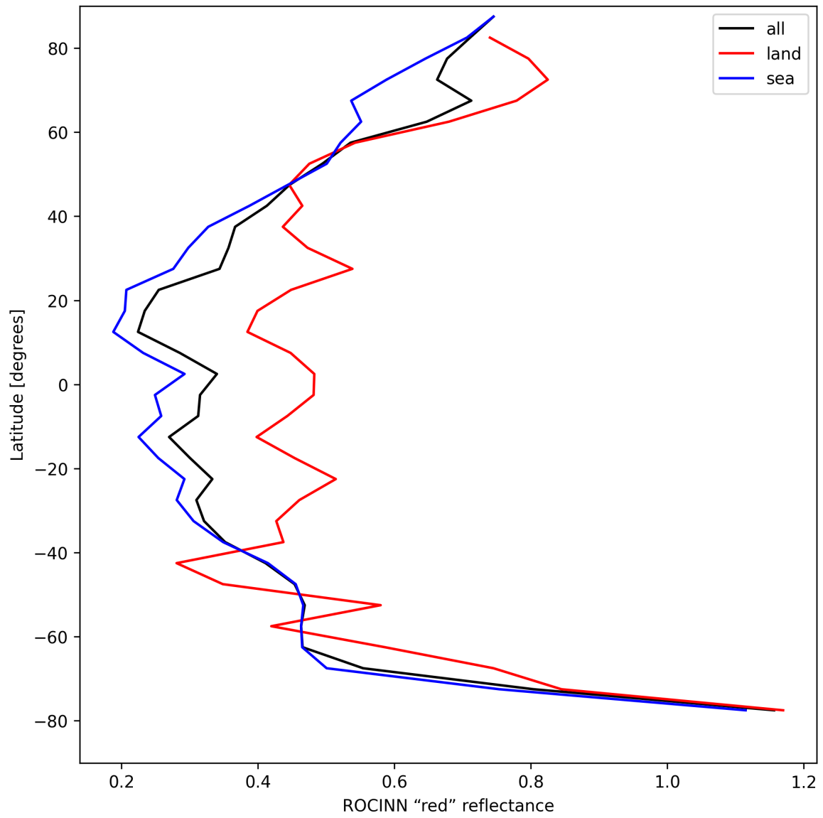
Figure 35: Zonal average of “ROCINN “red” reflectance” for 2025-04-23 to 2025-04-24.
