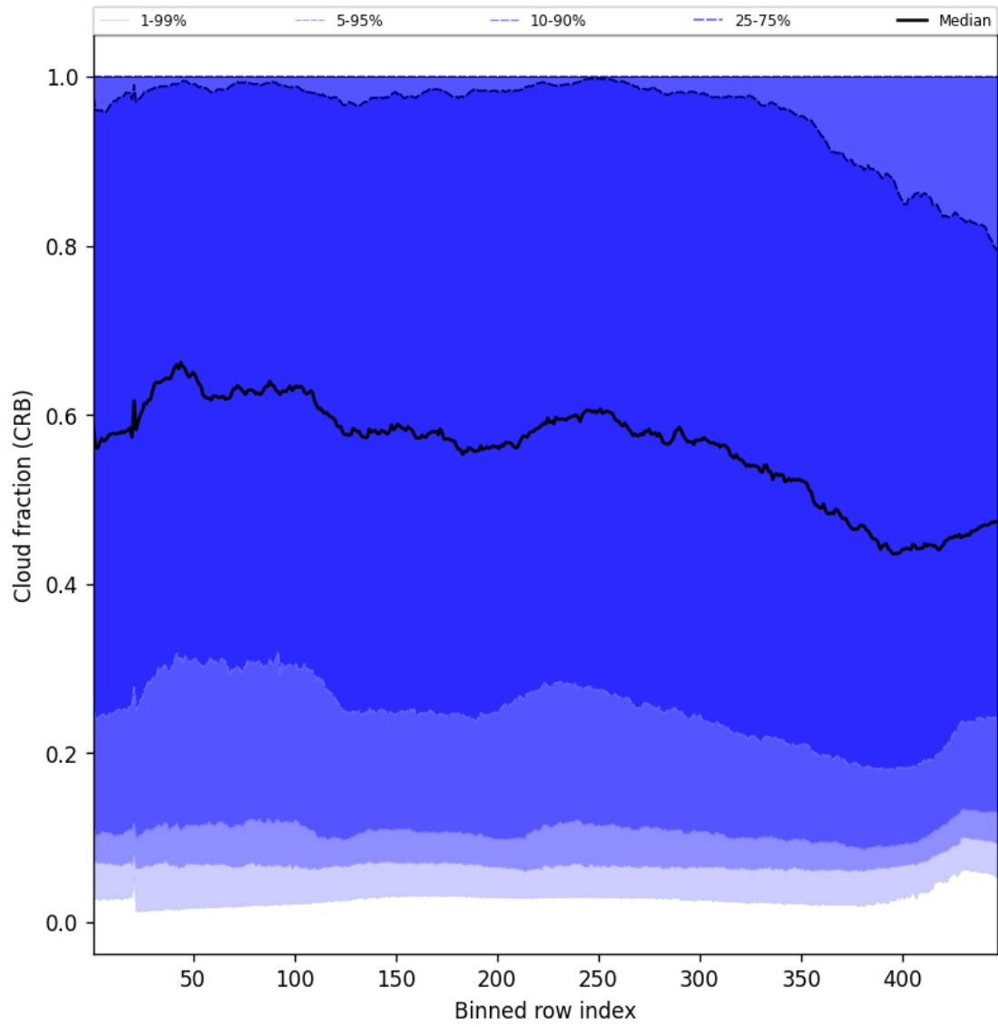
Figure 56: Along track statistics of “Cloud fraction (CRB)” for 2025-04-23 to 2025-04-24
