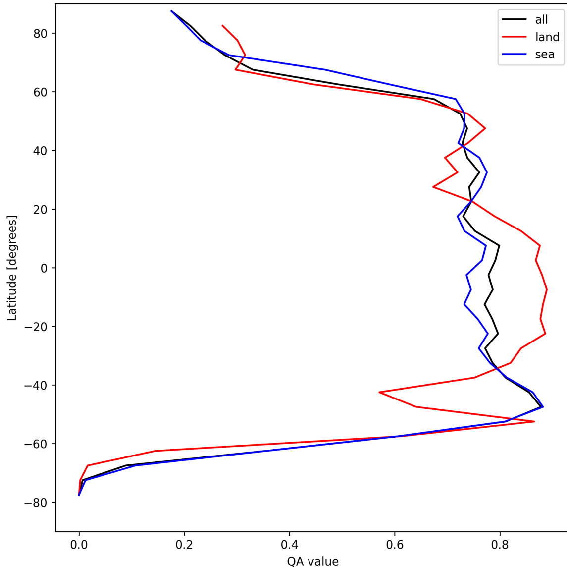
Figure 20: Zonal average of “QA value” for 2025-04-23 to 2025-04-24.
