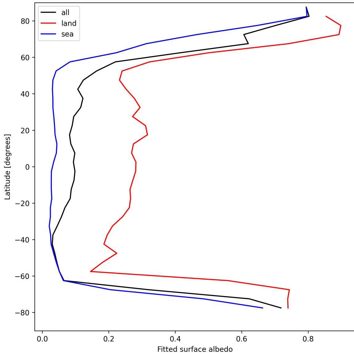
Figure 27: Zonal average of “Fitted surface albedo” for 2025-04-23 to 2025-04-24.
