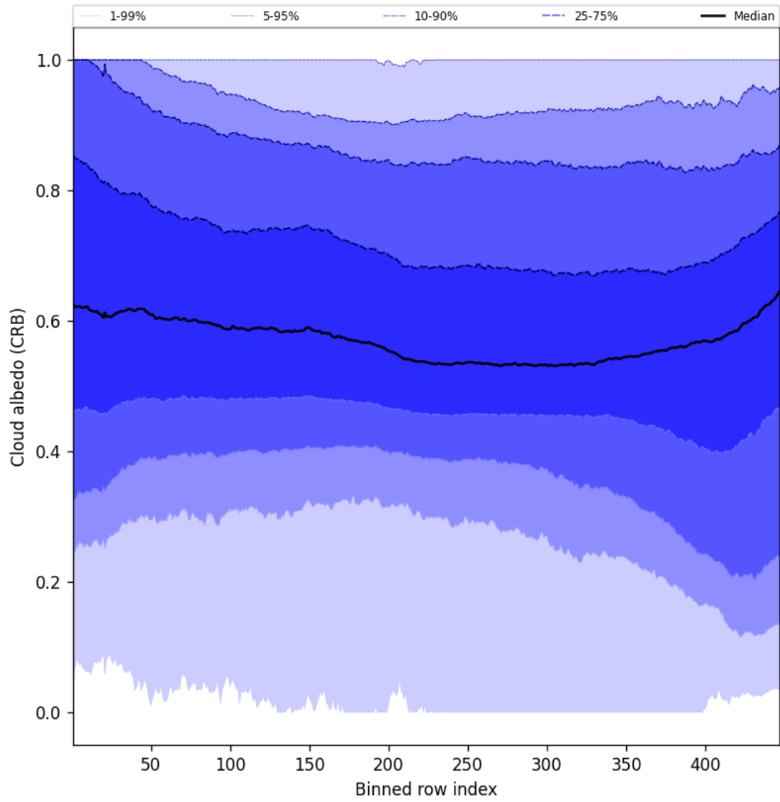
Figure 58: Along track statistics of “Cloud albedo (CRB)” for 2025-04-23 to 2025-04-24
