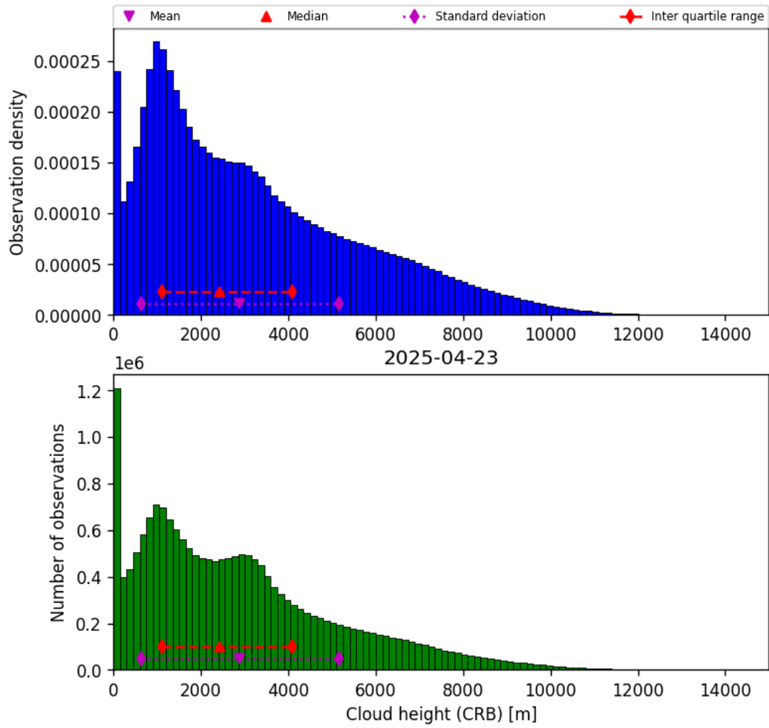
Figure 41: Histogram of “Cloud height (CRB)” for 2025-04-23 to 2025-04-24
