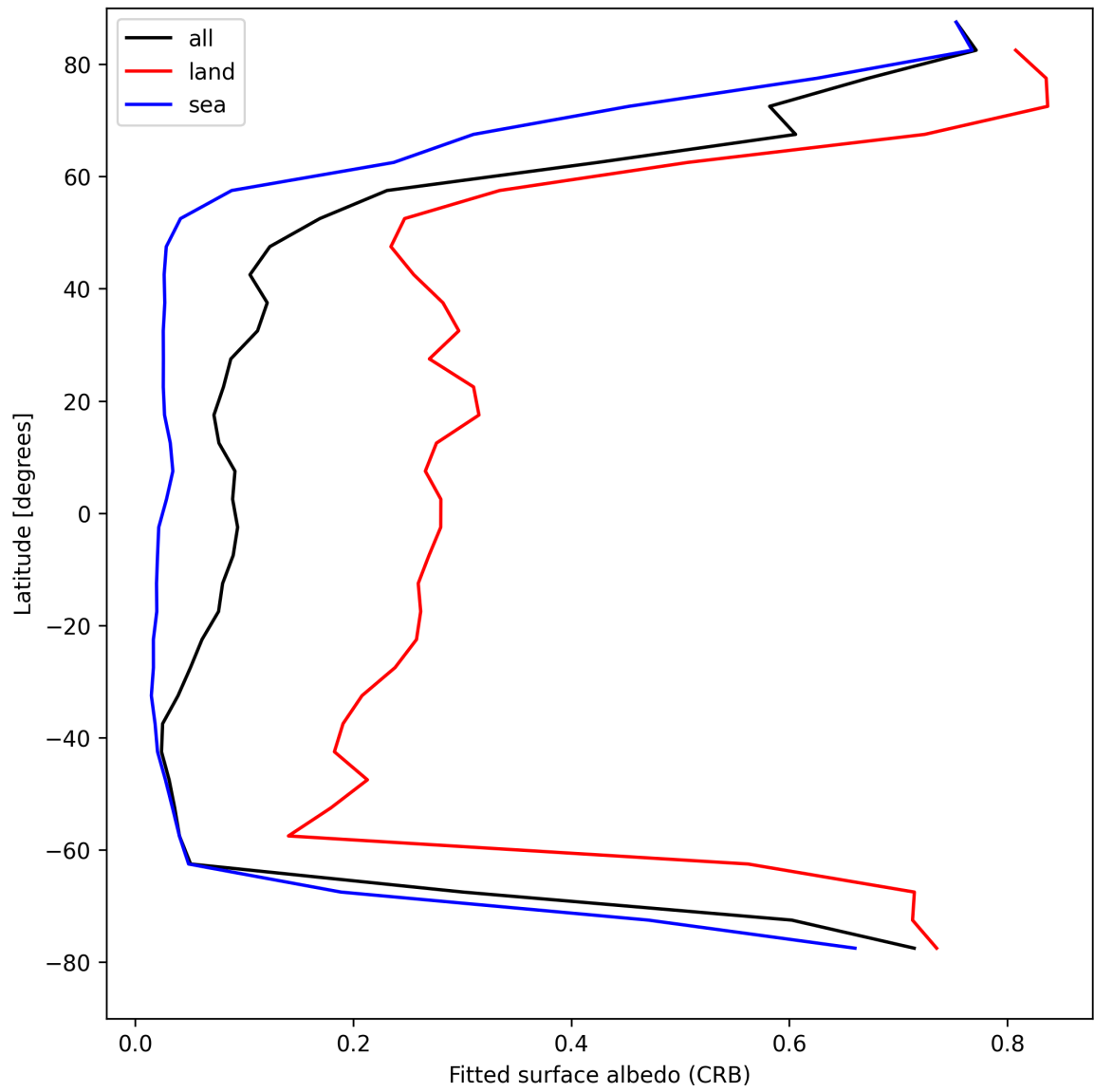
Figure 28: Zonal average of “Fitted surface albedo (CRB)” for 2025-04-23 to 2025-04-24.
