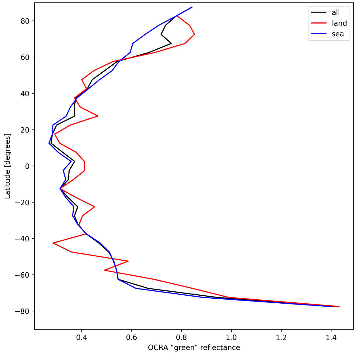
Figure 34: Zonal average of “OCRA “green” reflectance” for 2025-04-23 to 2025-04-24.
