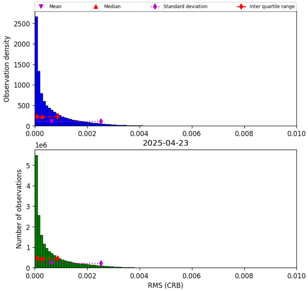
Figure 46: Histogram of “RMS (CRB)” for 2025-04-23 to 2025-04-24
