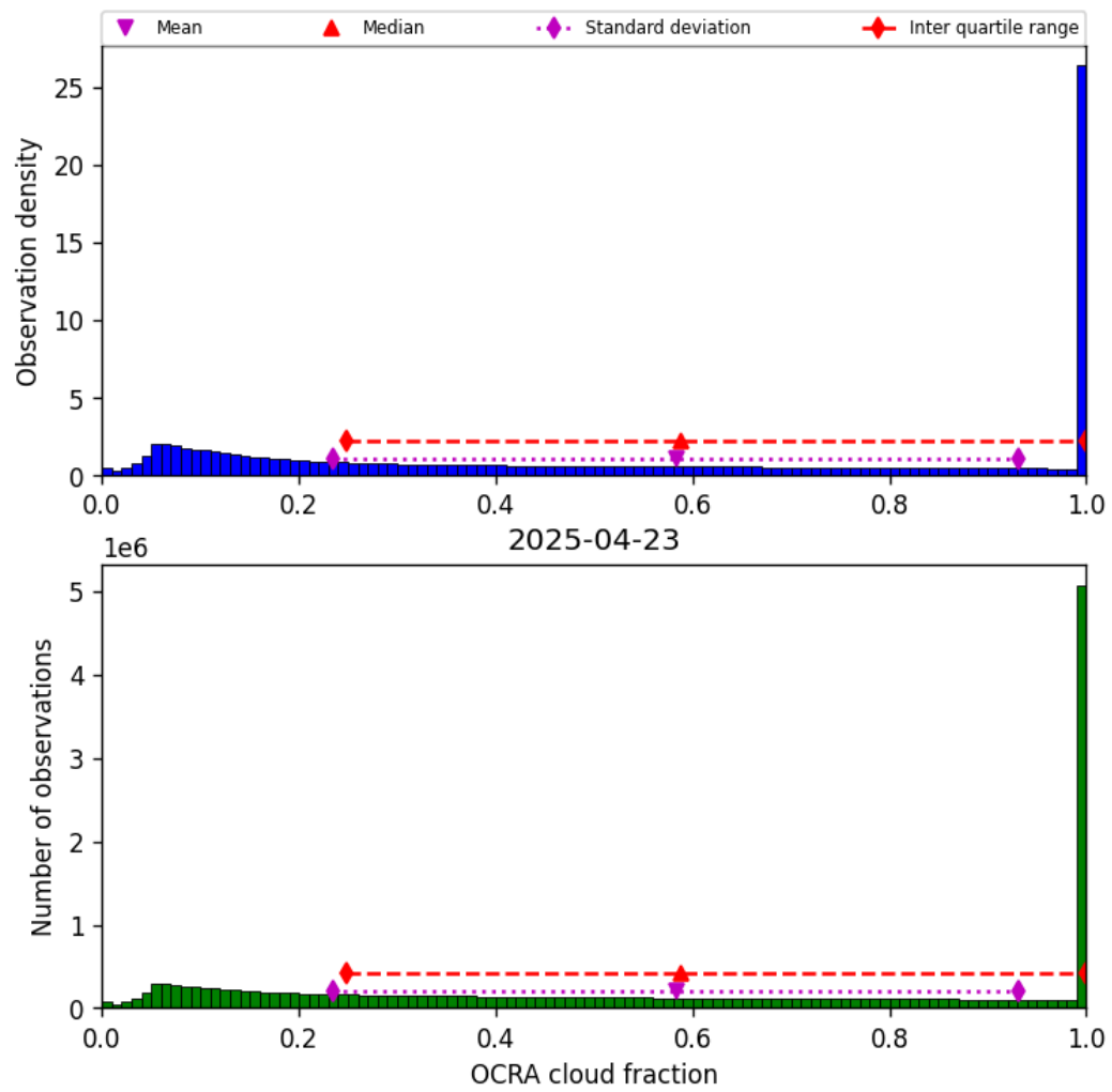
Figure 48: Histogram of “OCRA cloud fraction” for 2025-04-23 to 2025-04-24
