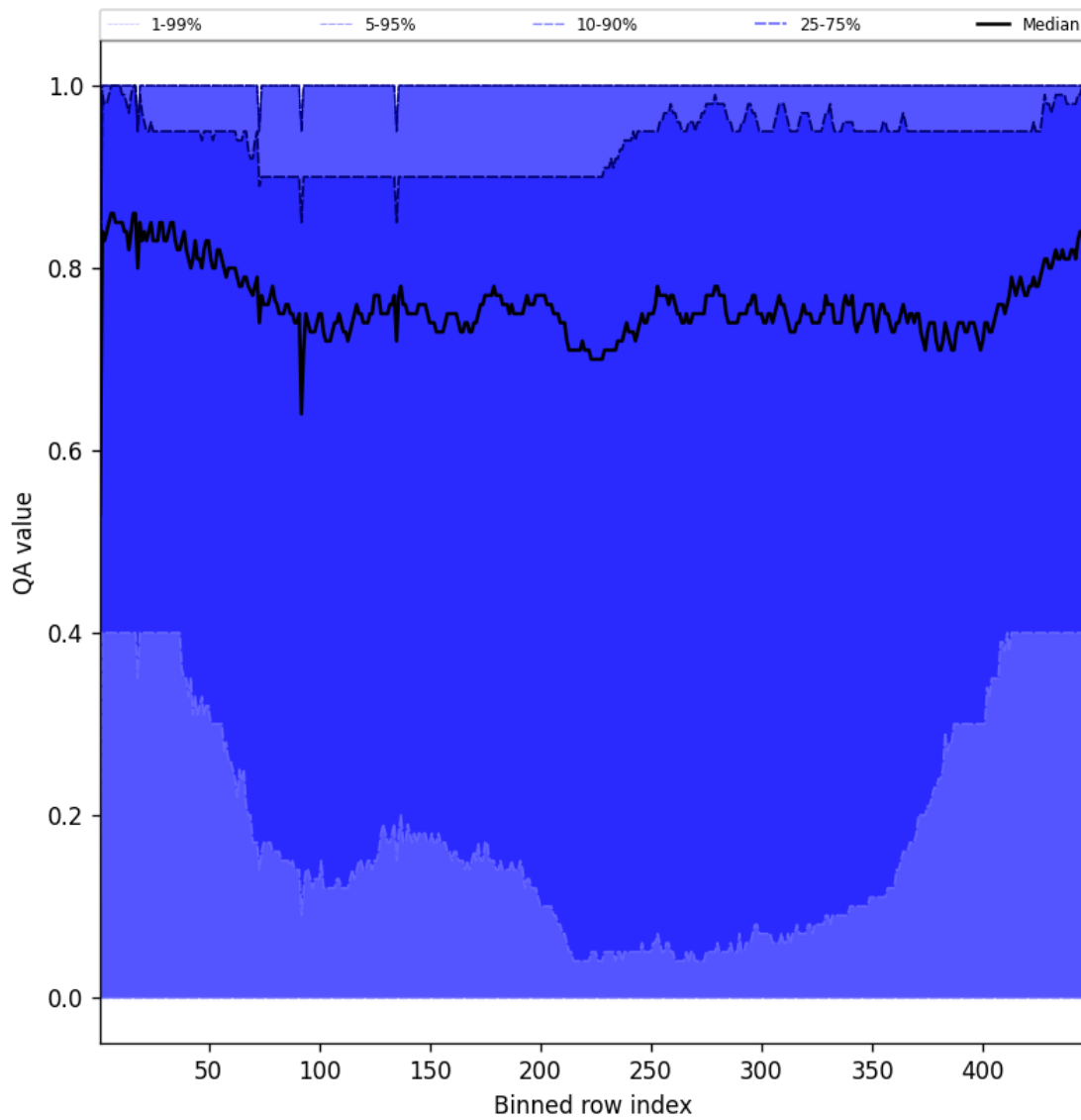
Figure 52: Along track statistics of “QA value” for 2025-04-23 to 2025-04-24
