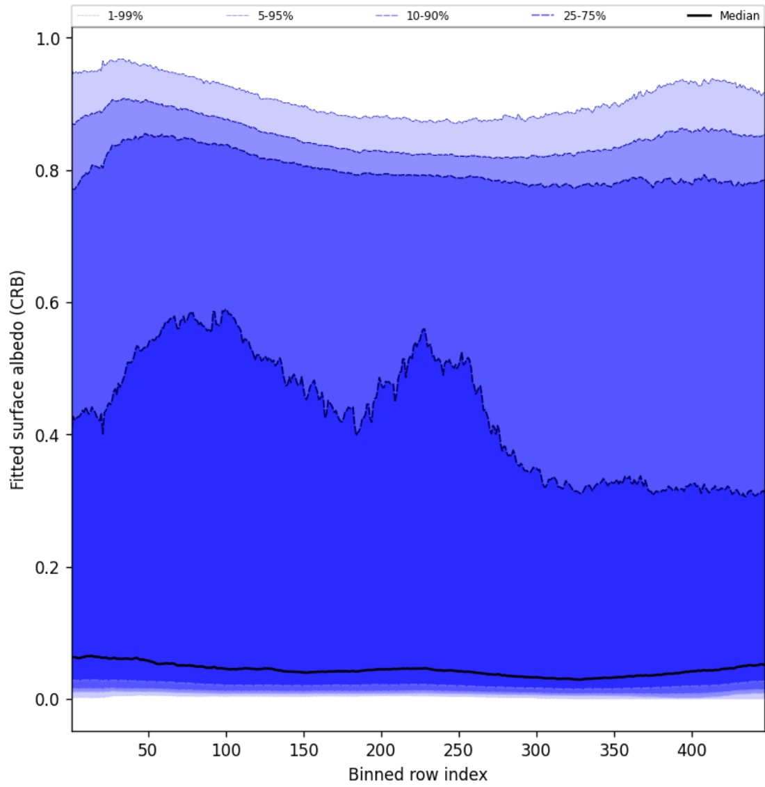
Figure 60: Along track statistics of “Fitted surface albedo (CRB)” for 2025-04-23 to 2025-04-24
