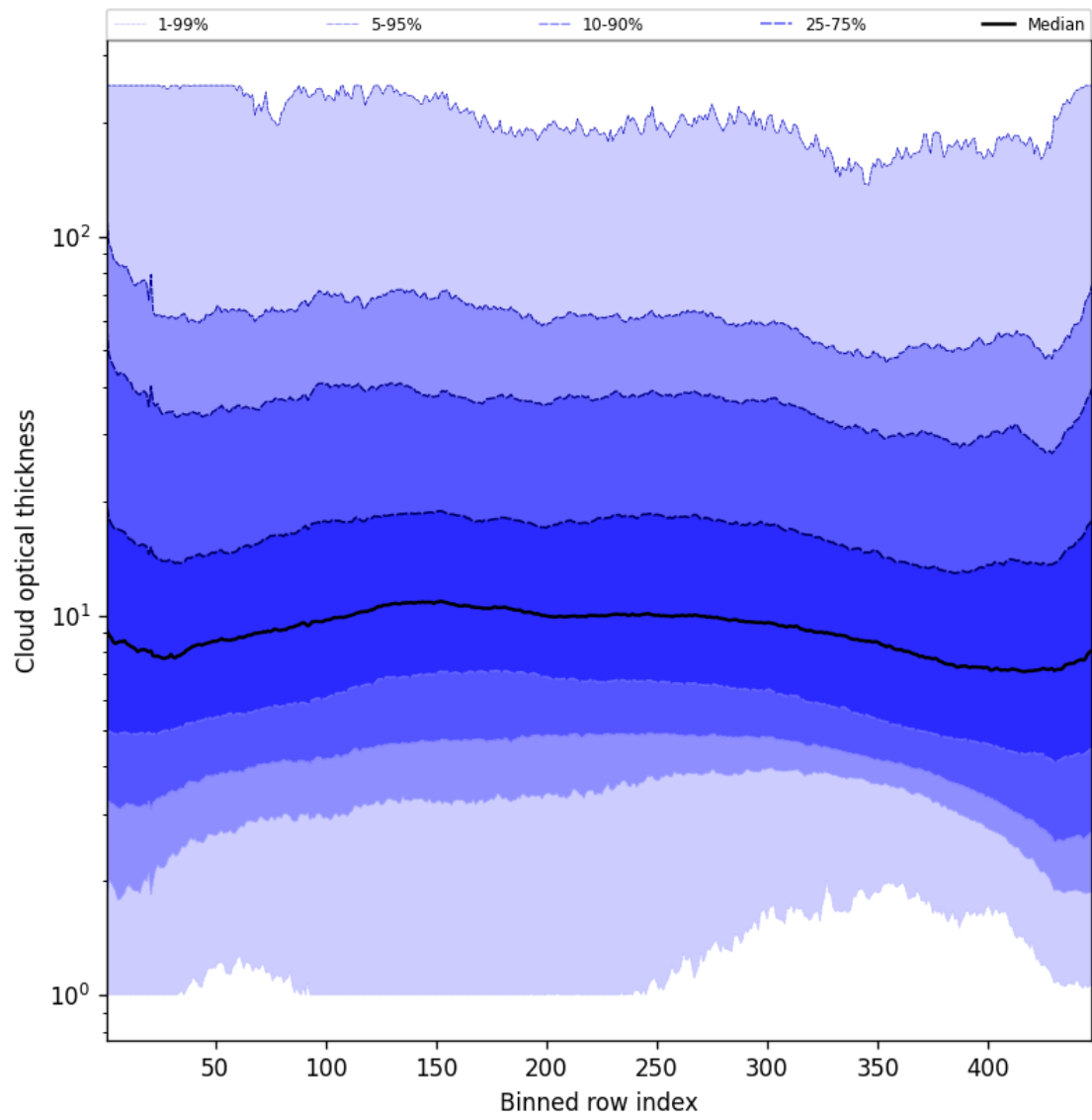
Figure 55: Along track statistics of “Cloud optical thickness” for 2025-04-24 to 2025-04-25
