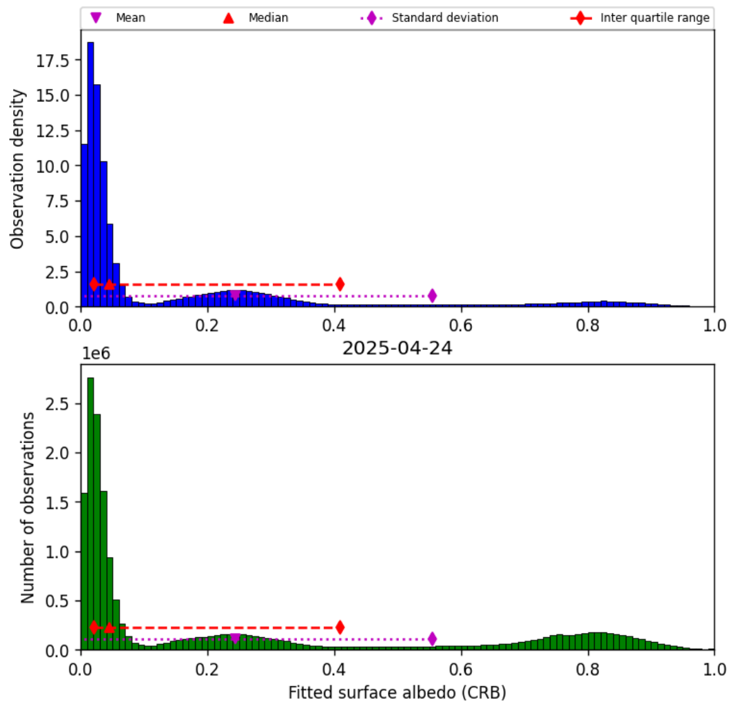
Figure 44: Histogram of “Fitted surface albedo (CRB)” for 2025-04-24 to 2025-04-25
