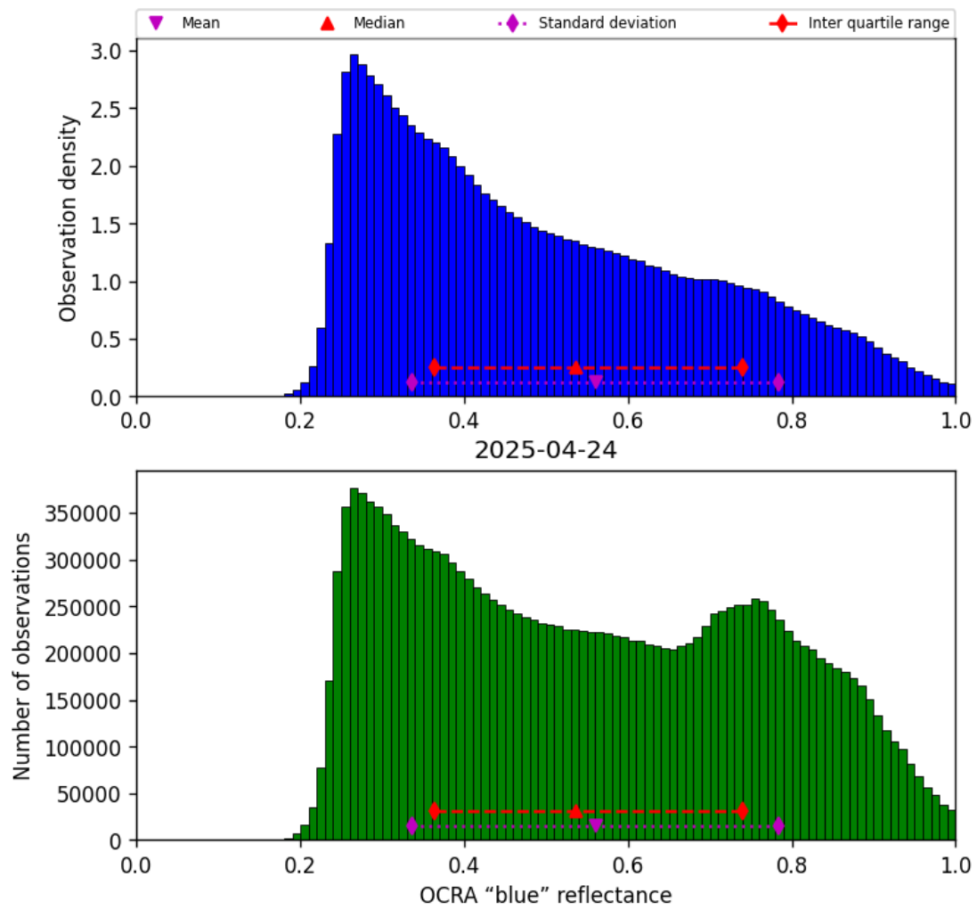
Figure 49: Histogram of “OCRA “blue” reflectance” for 2025-04-24 to 2025-04-25
