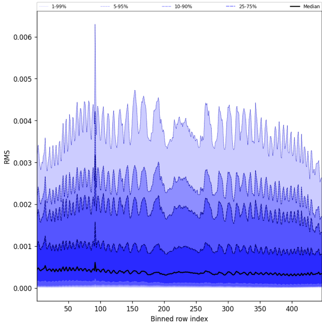
Figure 61: Along track statistics of “RMS” for 2025-04-24 to 2025-04-25
