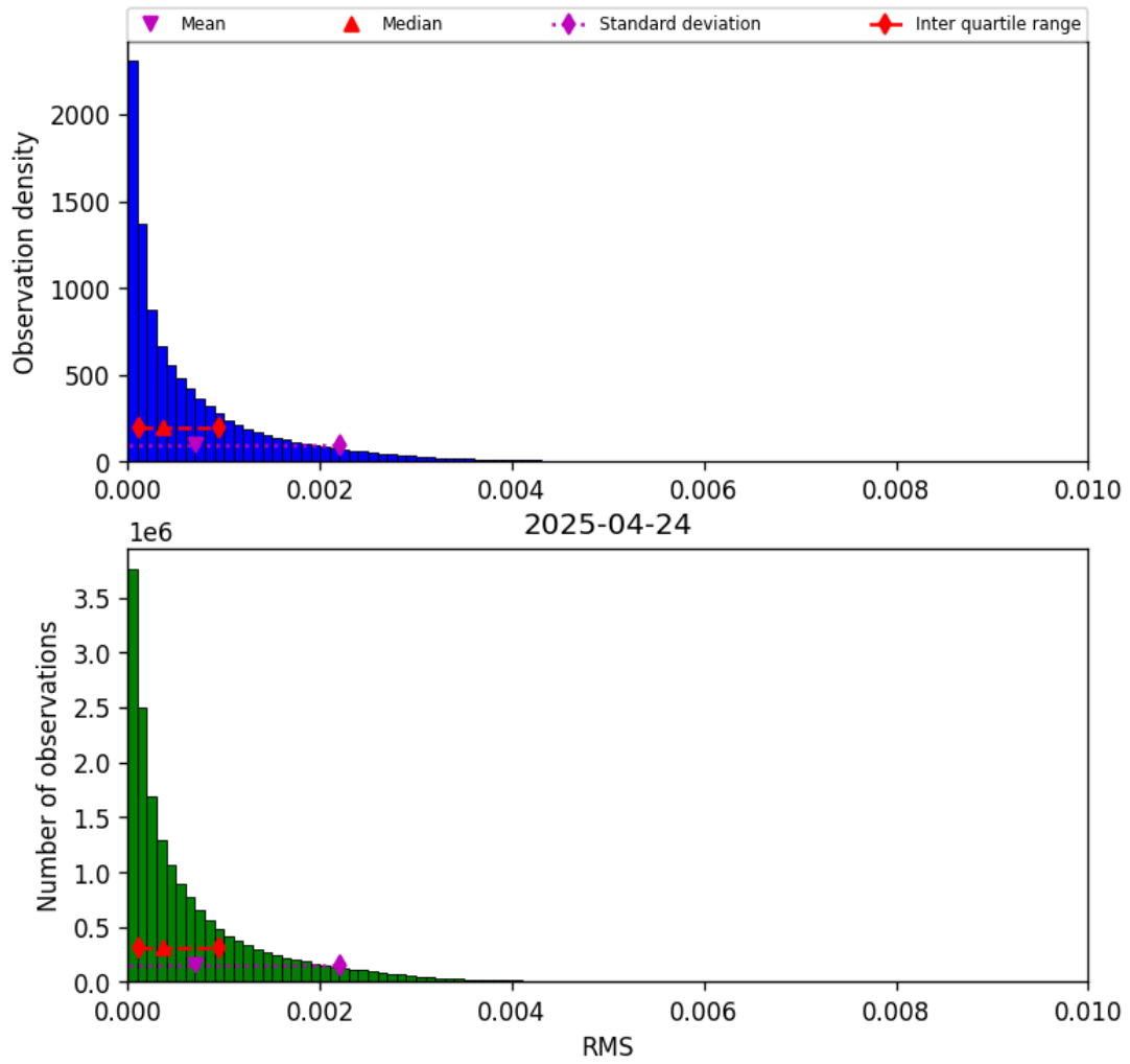
Figure 45: Histogram of “RMS” for 2025-04-24 to 2025-04-25
