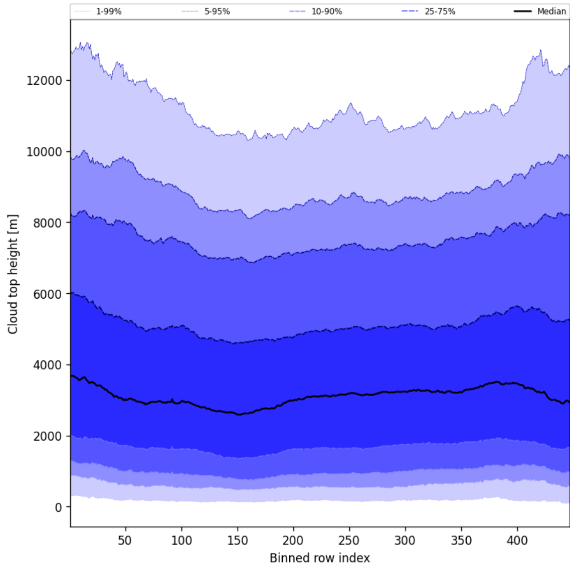
Figure 54: Along track statistics of “Cloud top height” for 2025-04-24 to 2025-04-25
