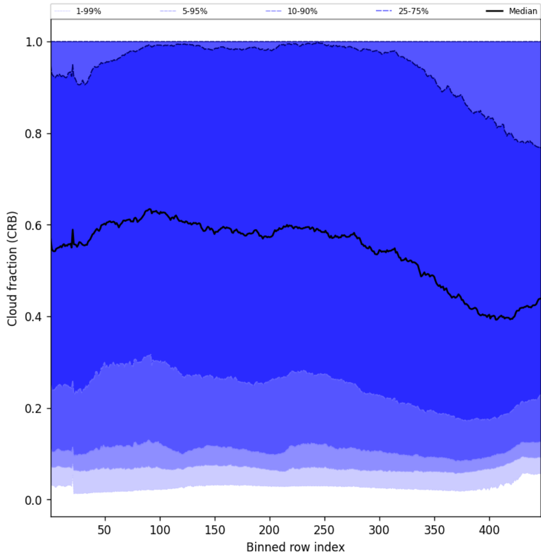
Figure 56: Along track statistics of “Cloud fraction (CRB)” for 2025-04-24 to 2025-04-25
