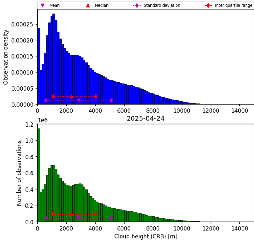
Figure 41: Histogram of “Cloud height (CRB)” for 2025-04-24 to 2025-04-25
