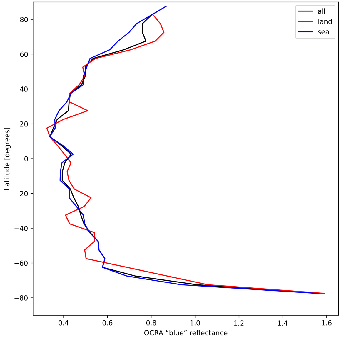
Figure 33: Zonal average of “OCRA “blue” reflectance” for 2025-04-24 to 2025-04-25.
