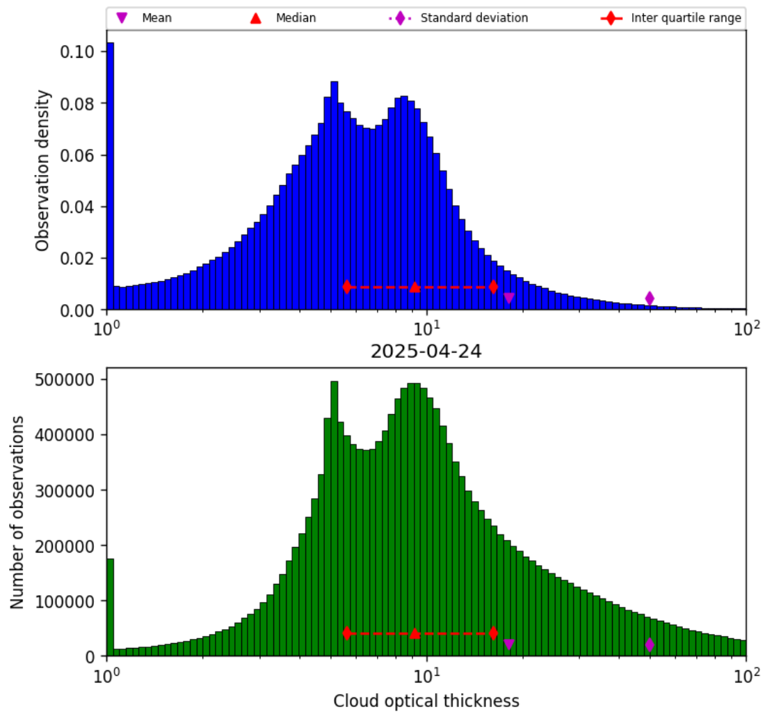
Figure 39: Histogram of “Cloud optical thickness” for 2025-04-24 to 2025-04-25
