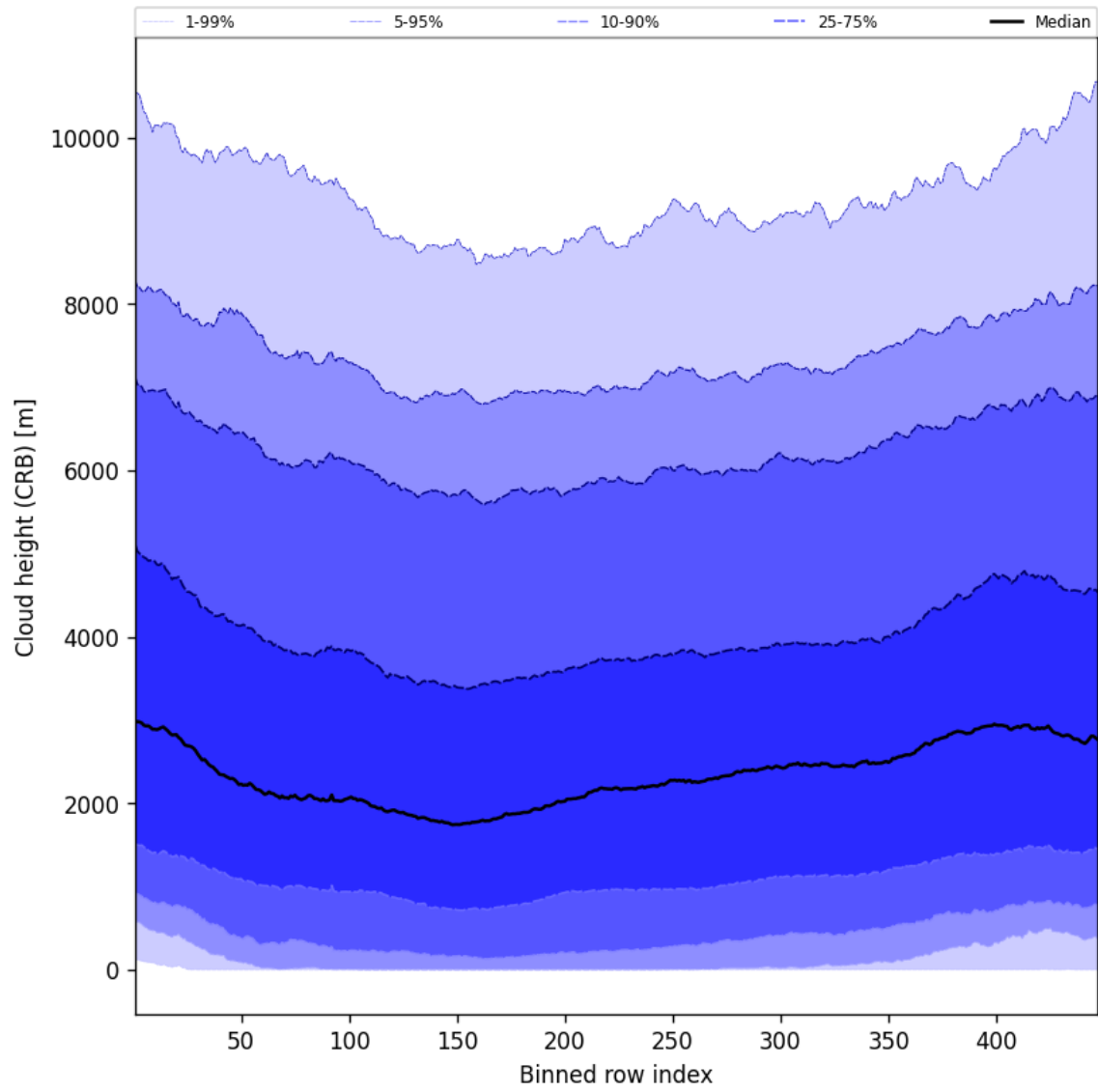
Figure 57: Along track statistics of “Cloud height (CRB)” for 2025-04-24 to 2025-04-25
