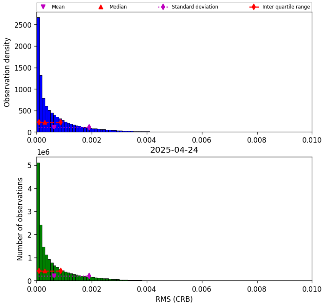
Figure 46: Histogram of “RMS (CRB)” for 2025-04-24 to 2025-04-25
