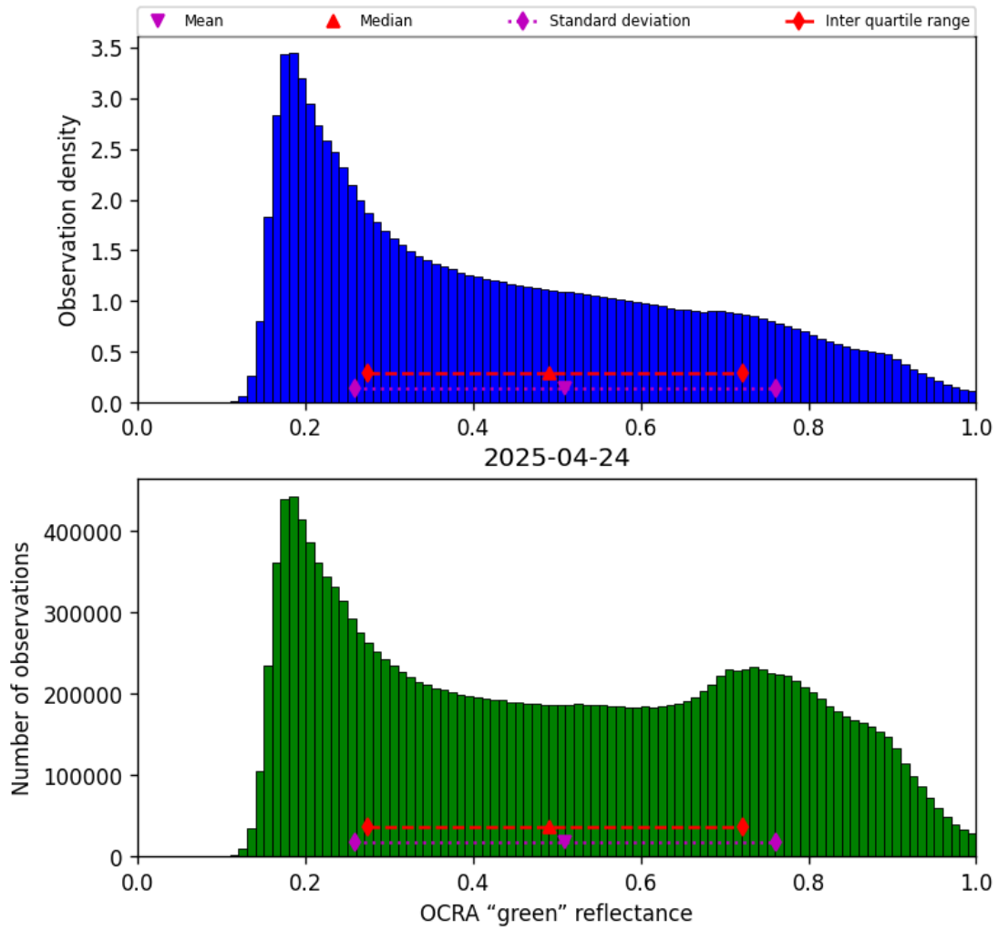
Figure 50: Histogram of “OCRA “green” reflectance” for 2025-04-24 to 2025-04-25
