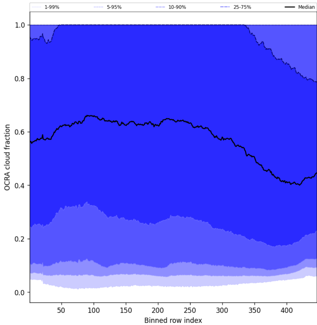
Figure 64: Along track statistics of “OCRA cloud fraction” for 2025-04-24 to 2025-04-25
