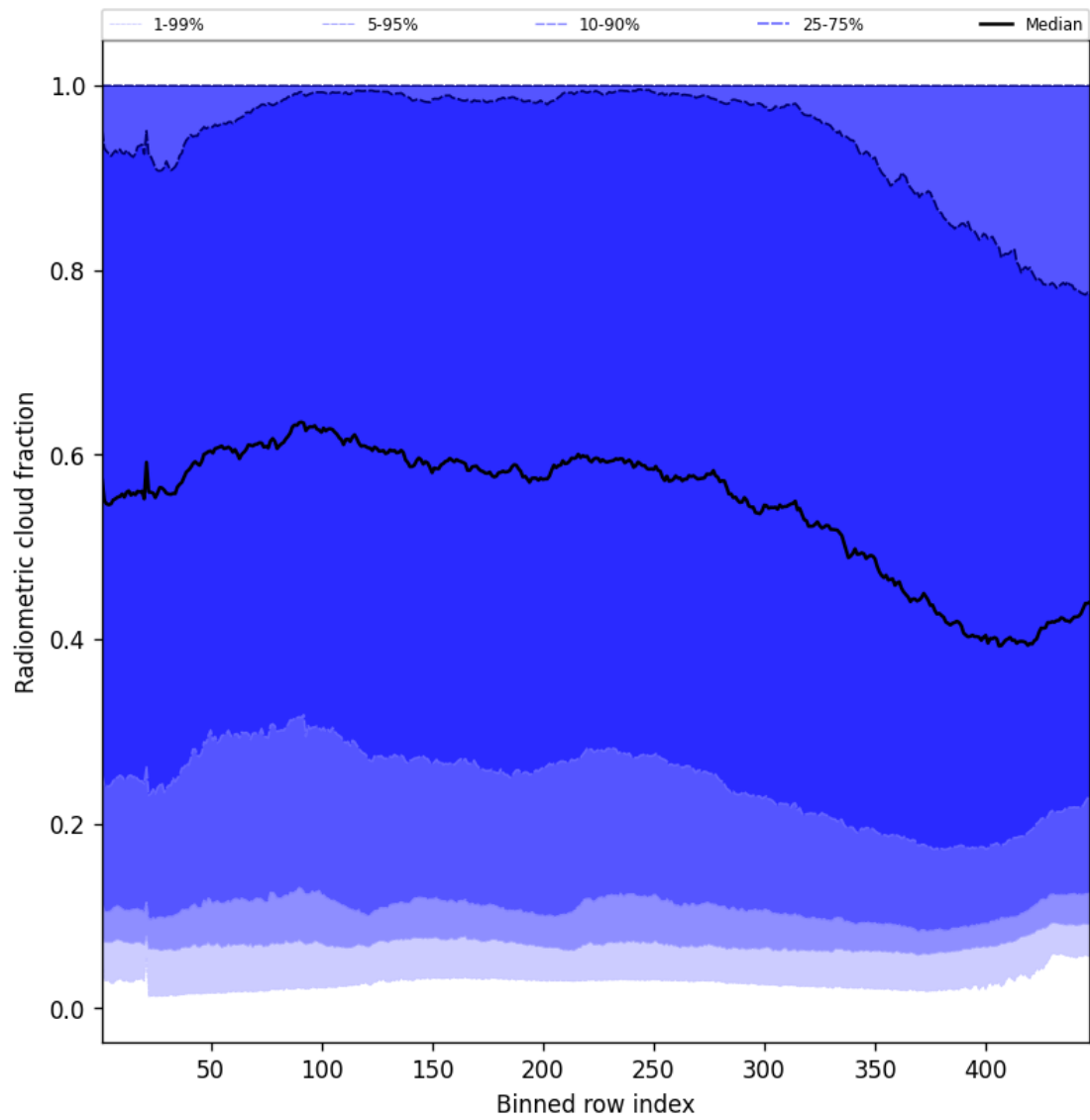
Figure 53: Along track statistics of “Radiometric cloud fraction” for 2025-04-24 to 2025-04-25
