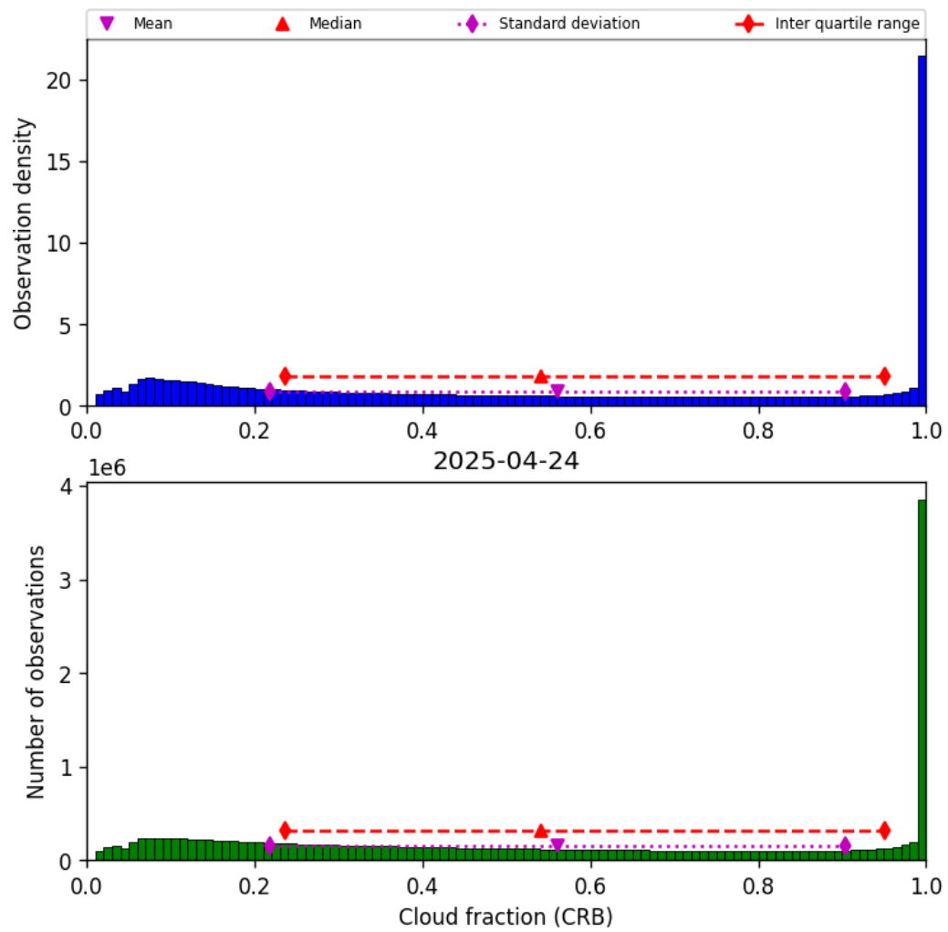
Figure 40: Histogram of “Cloud fraction (CRB)” for 2025-04-24 to 2025-04-25
