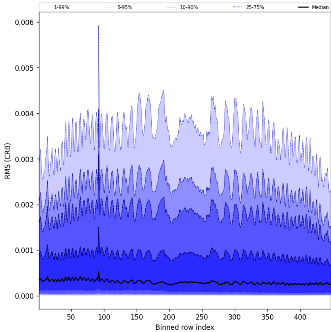
Figure 62: Along track statistics of “RMS (CRB)” for 2025-04-24 to 2025-04-25
