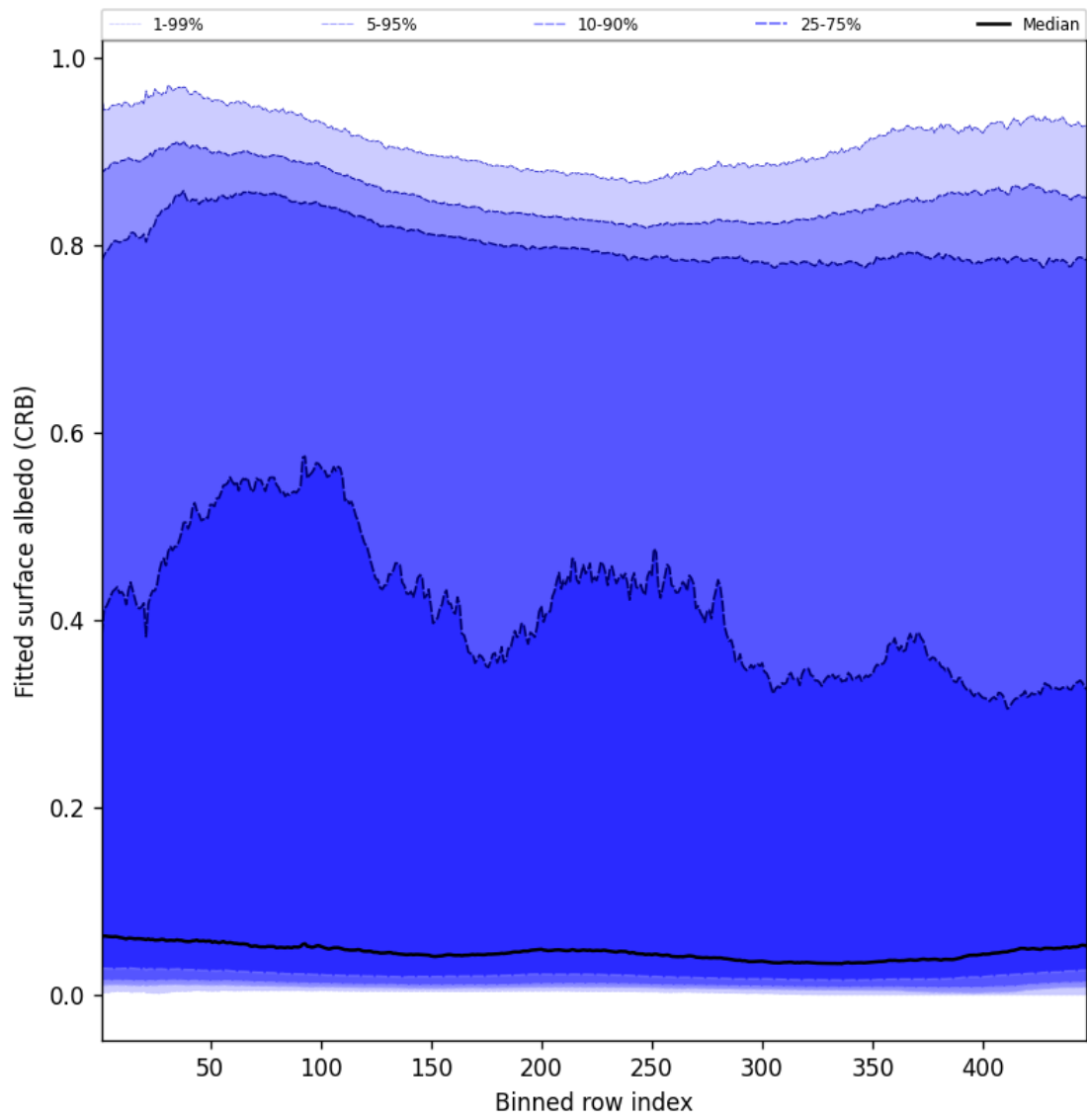
Figure 60: Along track statistics of “Fitted surface albedo (CRB)” for 2025-04-24 to 2025-04-25
