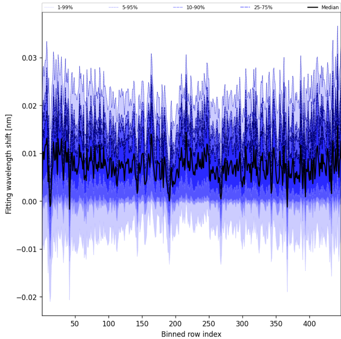
Figure 63: Along track statistics of “Fitting wavelength shift” for 2025-04-24 to 2025-04-25
