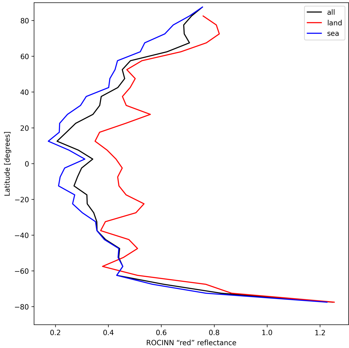
Figure 35: Zonal average of “ROCINN “red” reflectance” for 2025-04-24 to 2025-04-25.
