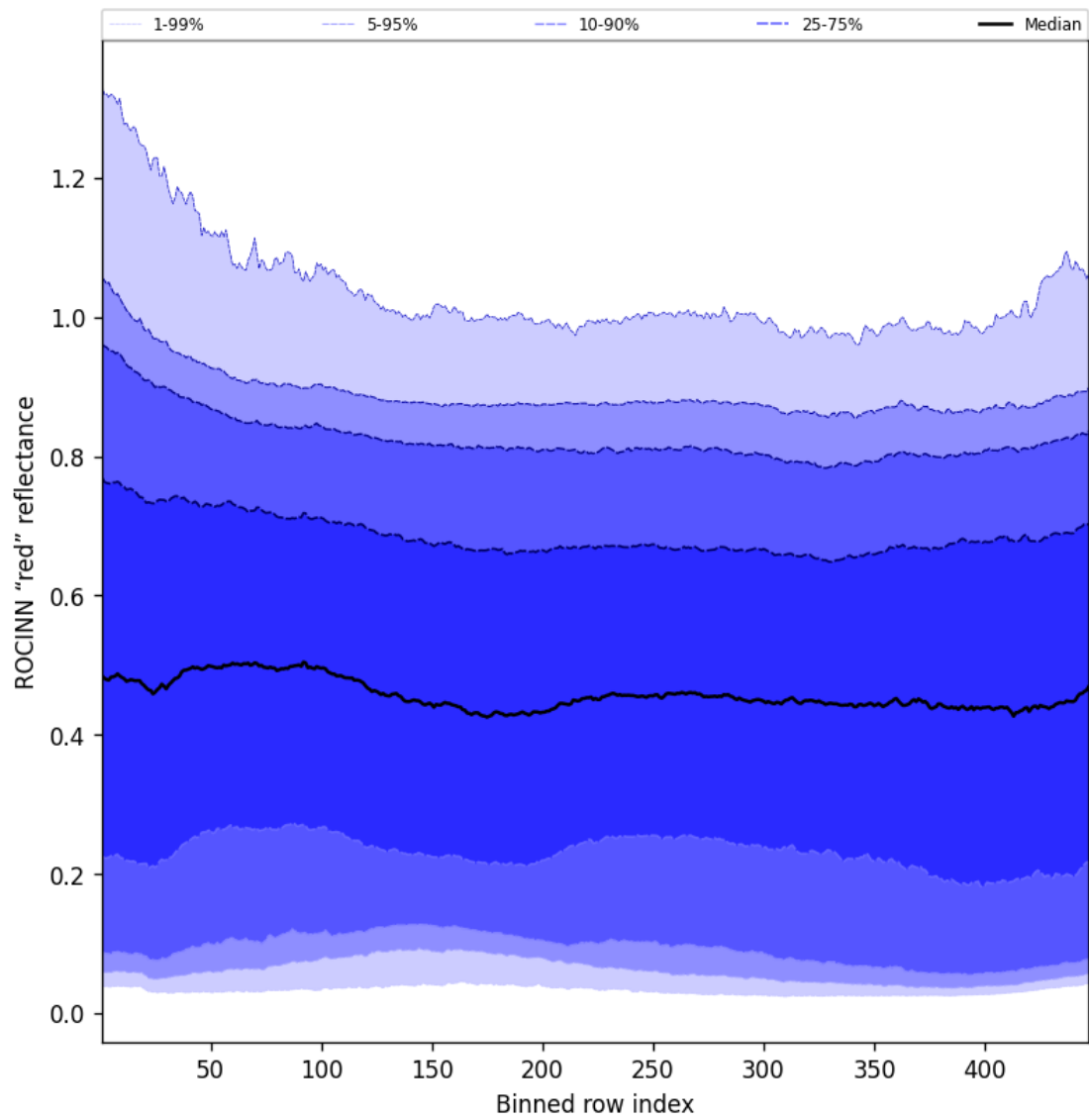
Figure 67: Along track statistics of “ROCINN “red” reflectance” for 2025-04-24 to 2025-04-25
