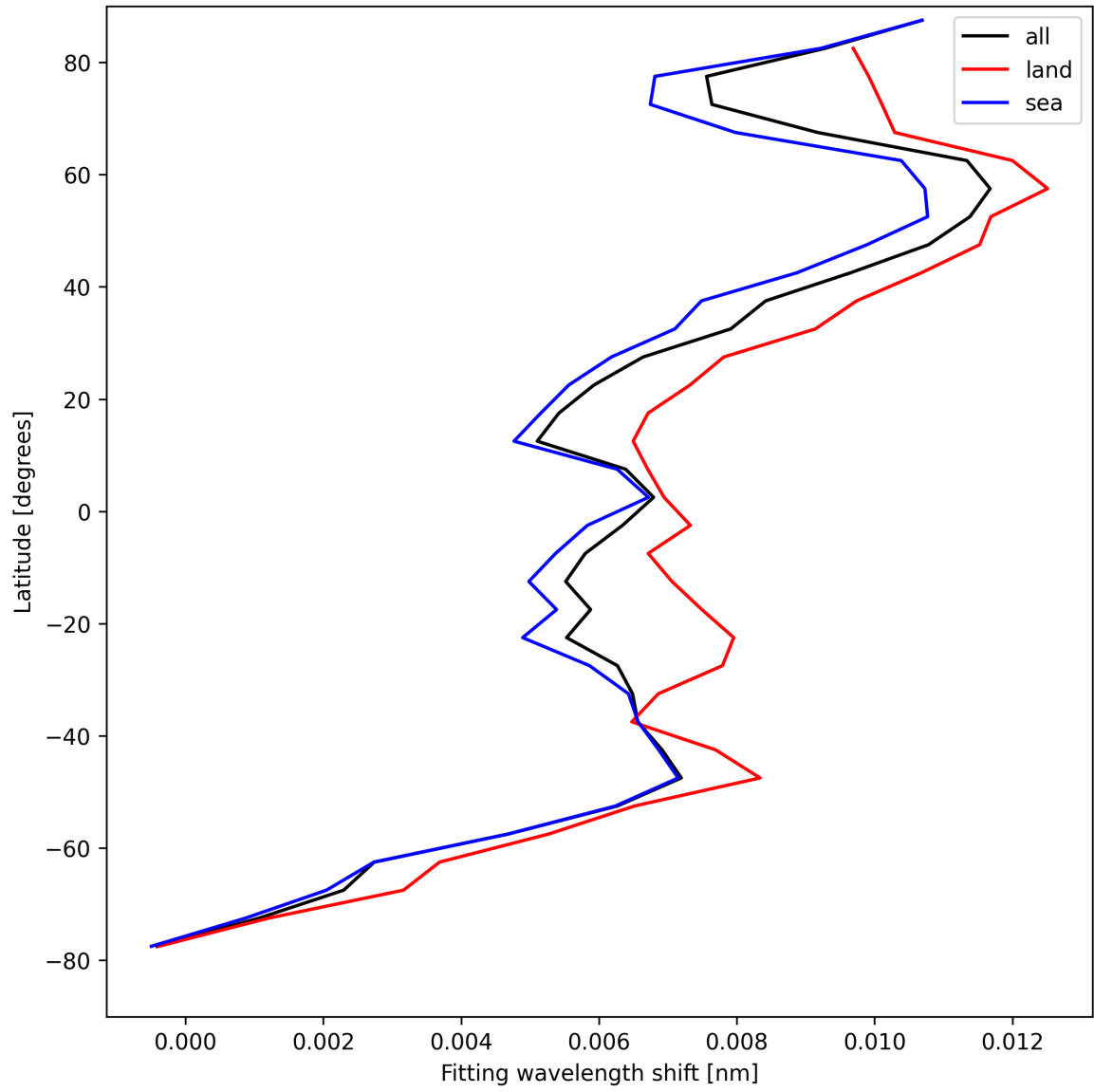
Figure 31: Zonal average of “Fitting wavelength shift” for 2025-04-24 to 2025-04-25.
