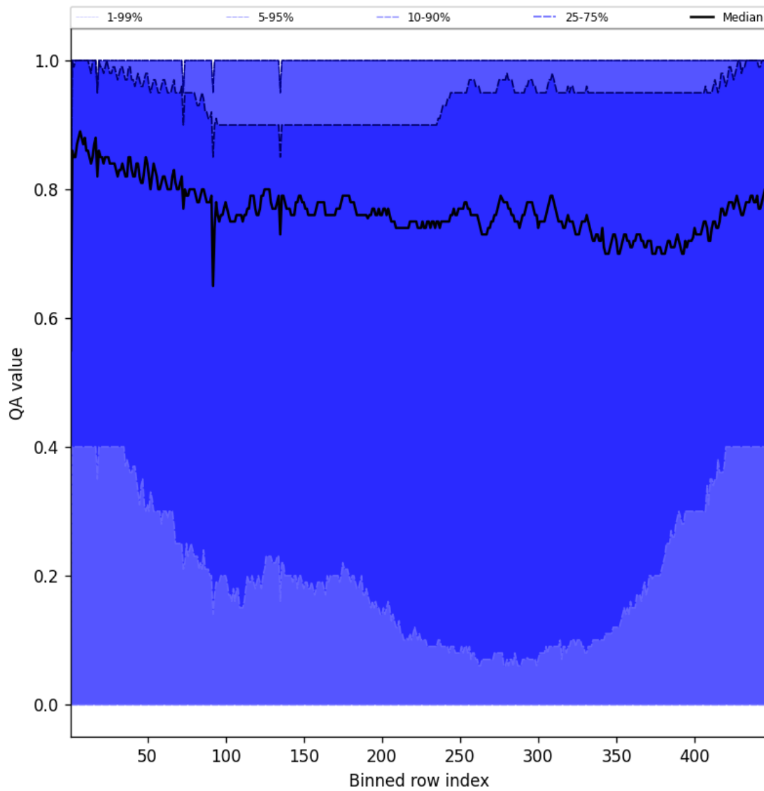
Figure 52: Along track statistics of “QA value” for 2025-04-24 to 2025-04-25
