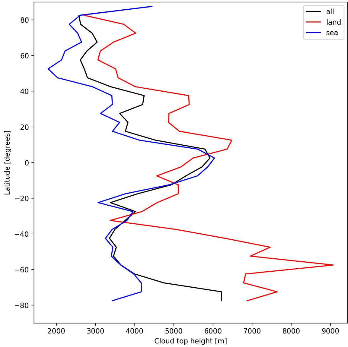
Figure 22: Zonal average of “Cloud top height” for 2025-04-24 to 2025-04-25.
