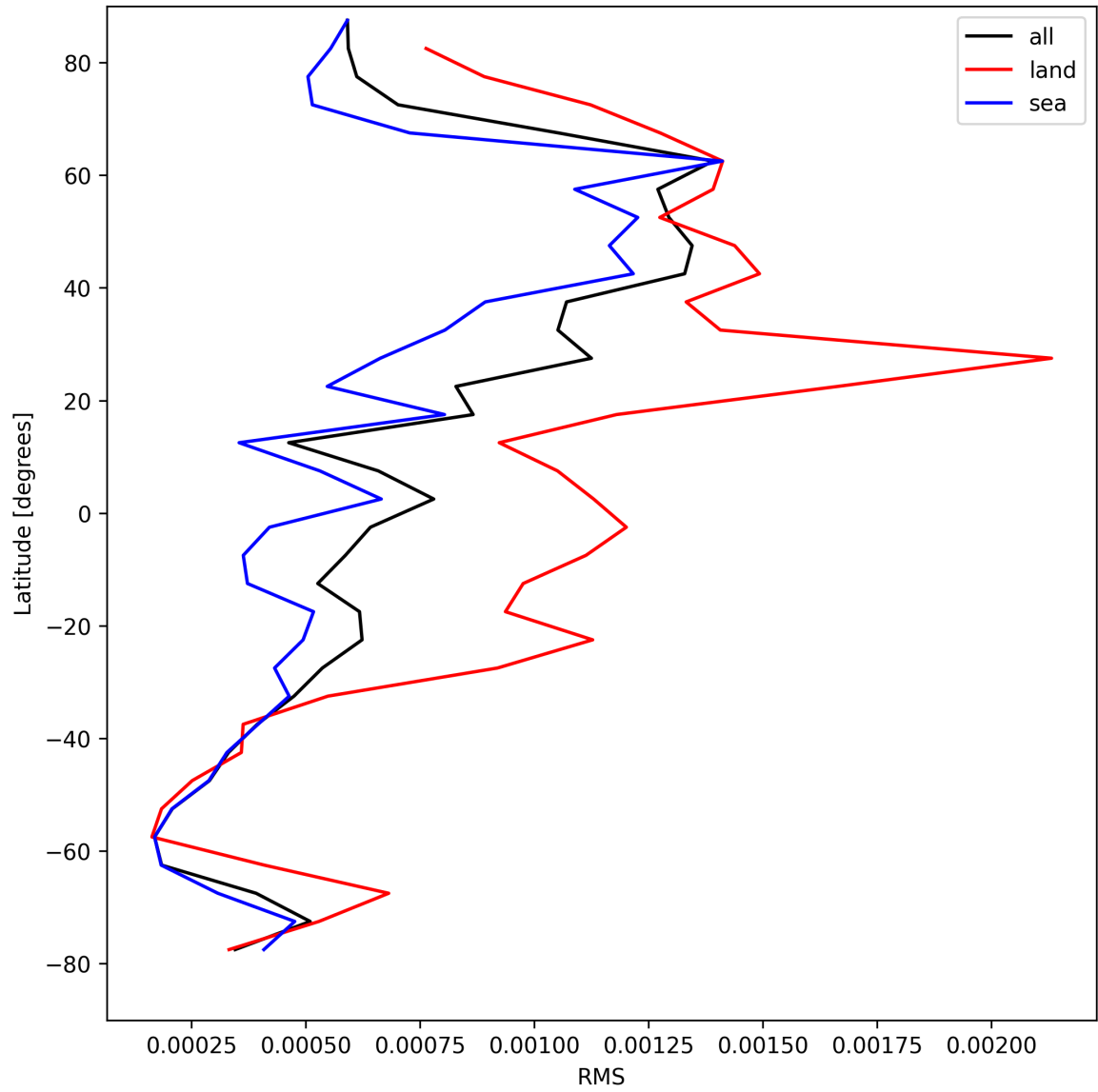
Figure 29: Zonal average of “RMS” for 2025-04-24 to 2025-04-25.
