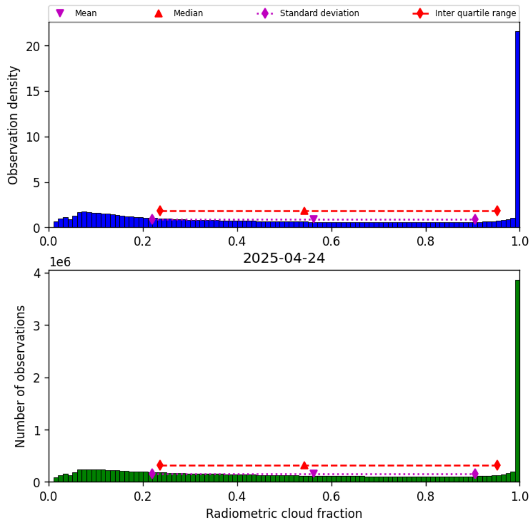
Figure 37: Histogram of “Radiometric cloud fraction” for 2025-04-24 to 2025-04-25
