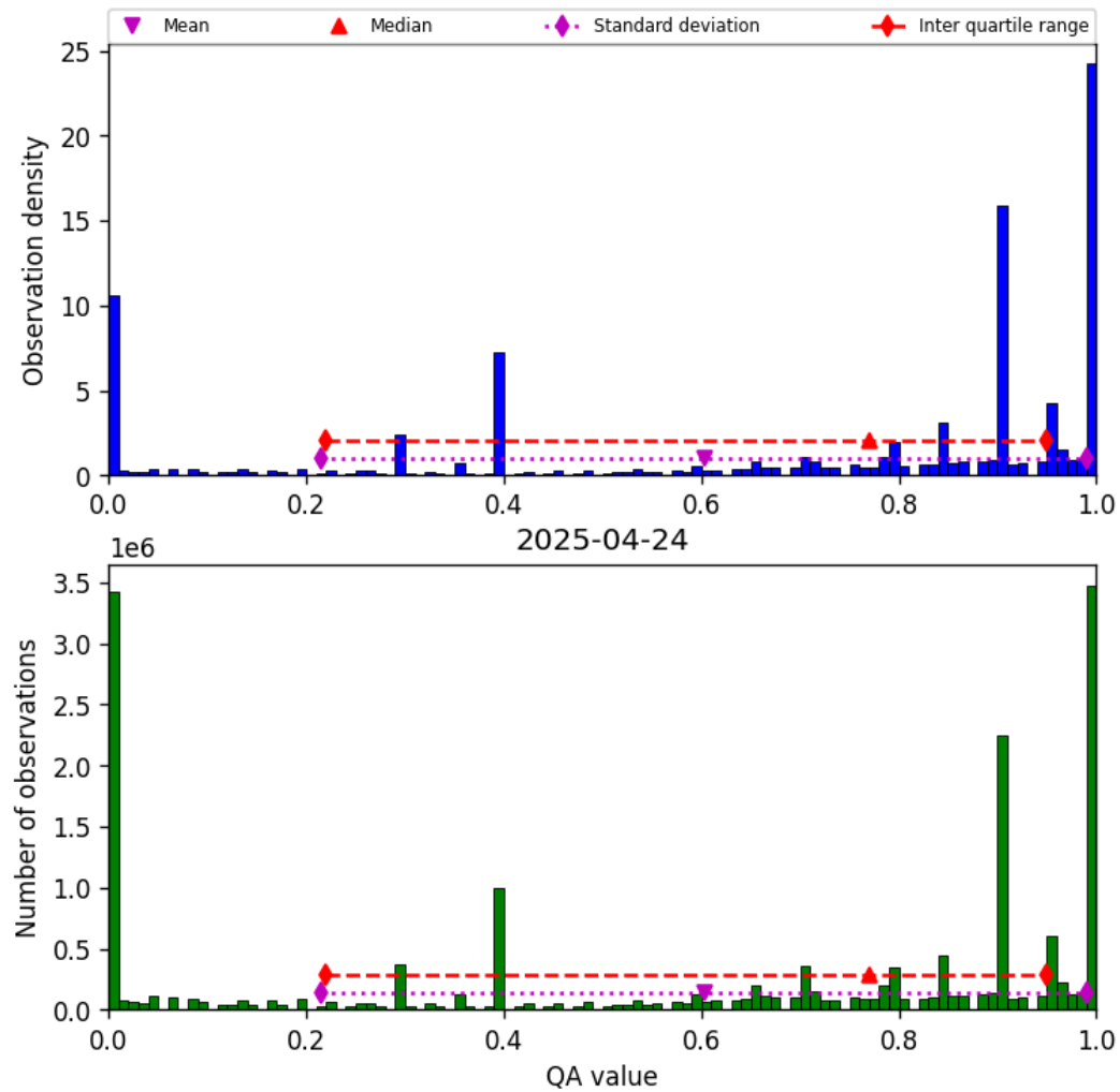
Figure 36: Histogram of “QA value” for 2025-04-24 to 2025-04-25
