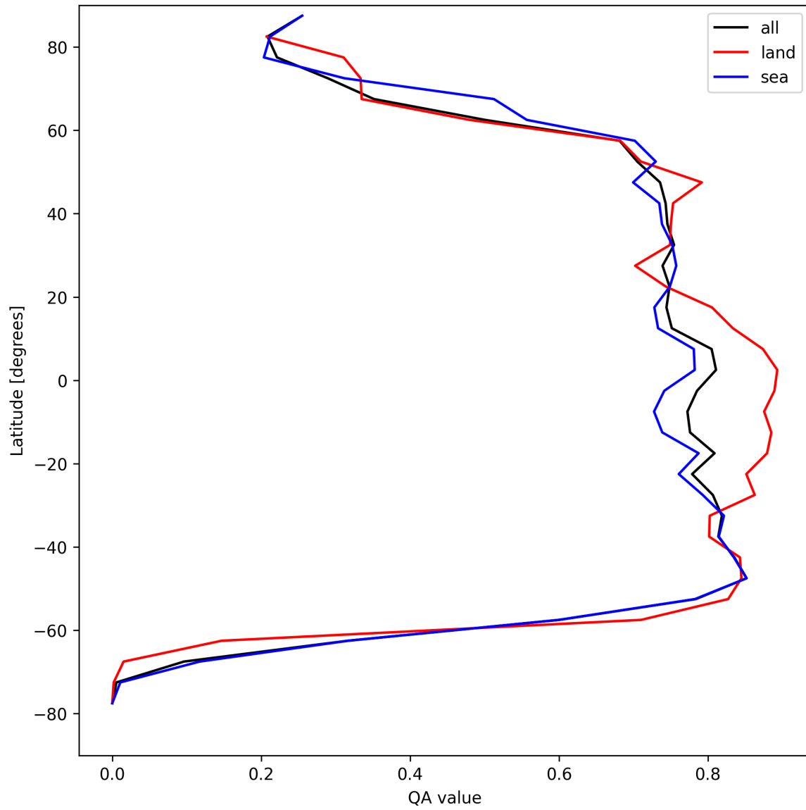
Figure 20: Zonal average of “QA value” for 2025-04-24 to 2025-04-25.
