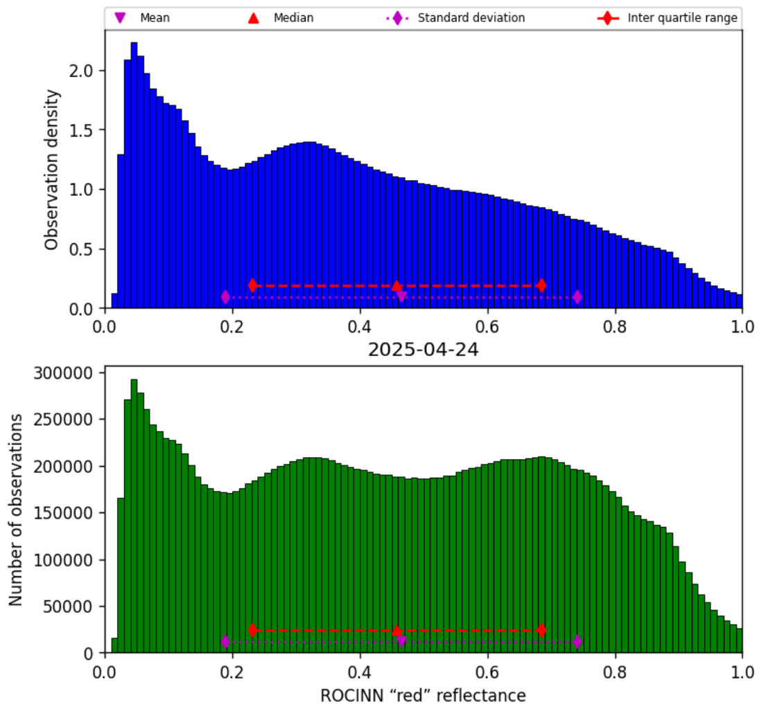
Figure 51: Histogram of “ROCINN “red” reflectance” for 2025-04-24 to 2025-04-25
