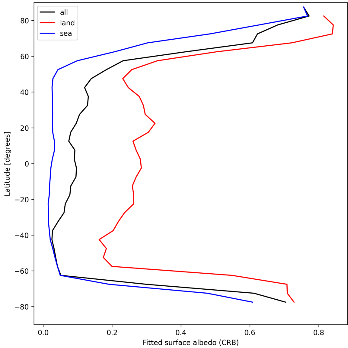
Figure 28: Zonal average of “Fitted surface albedo (CRB)” for 2025-04-24 to 2025-04-25.
