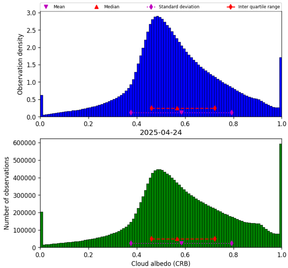
Figure 42: Histogram of “Cloud albedo (CRB)” for 2025-04-24 to 2025-04-25
