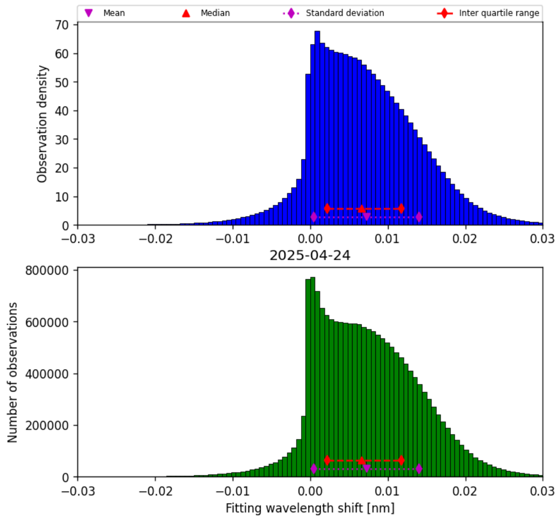
Figure 47: Histogram of “Fitting wavelength shift” for 2025-04-24 to 2025-04-25
