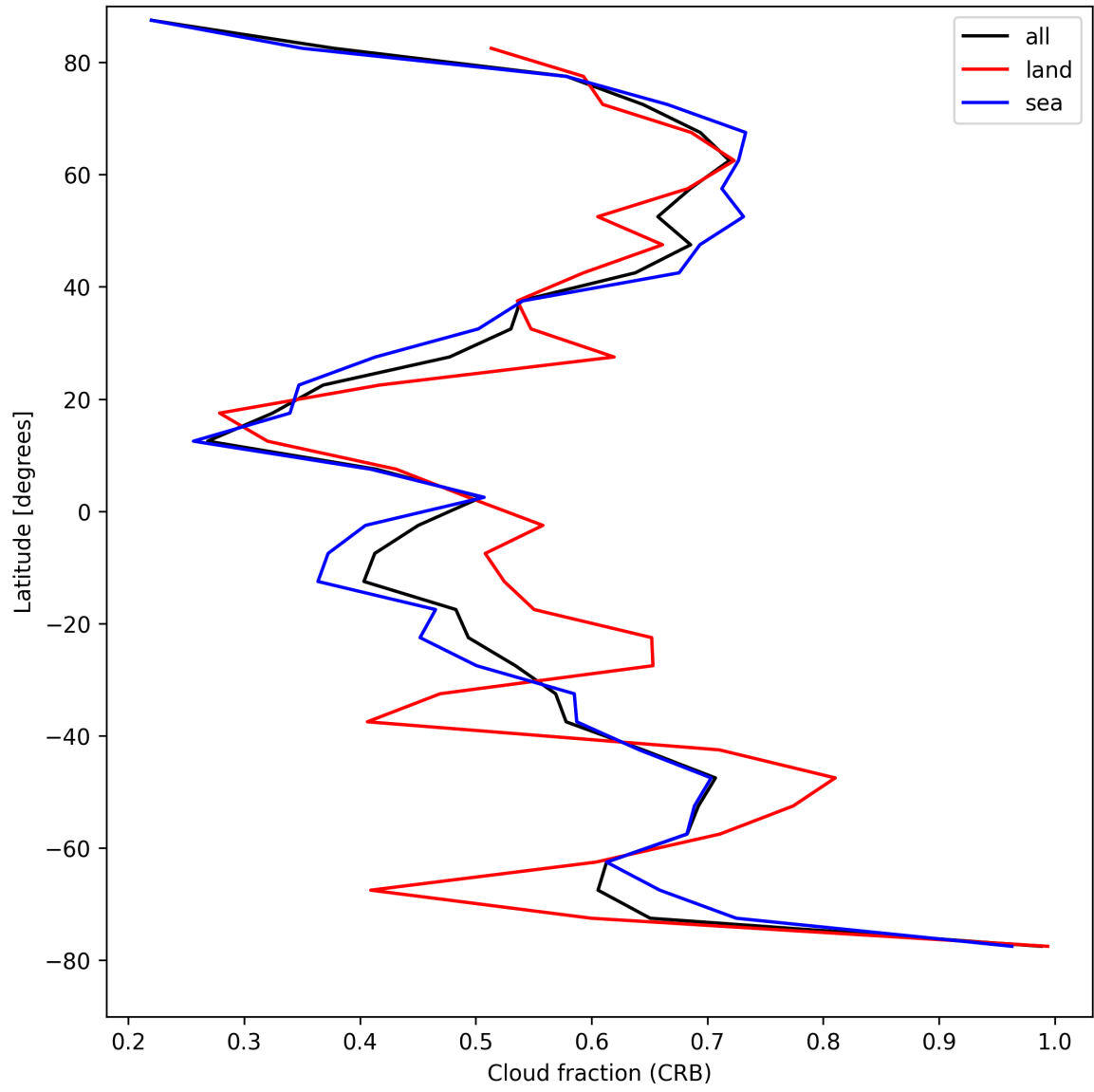
Figure 24: Zonal average of “Cloud fraction (CRB)” for 2025-04-24 to 2025-04-25.
