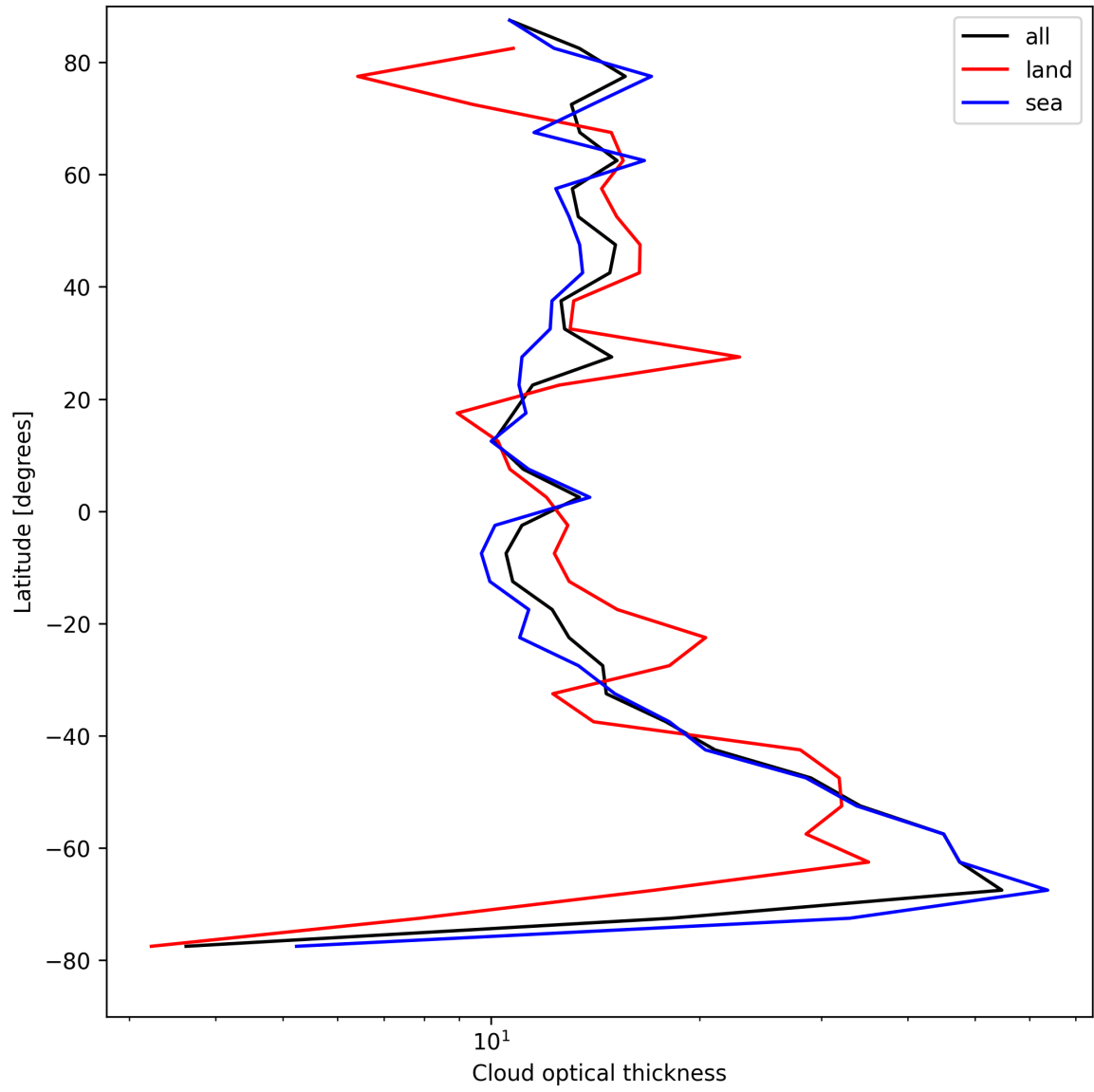
Figure 23: Zonal average of “Cloud optical thickness” for 2025-04-24 to 2025-04-25.
