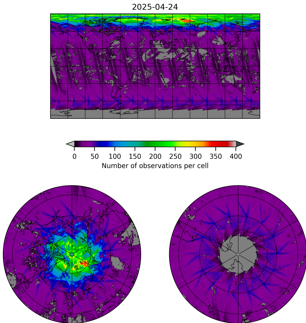
Figure 19: Map of the number of observations for 2025-04-24 to 2025-04-25
