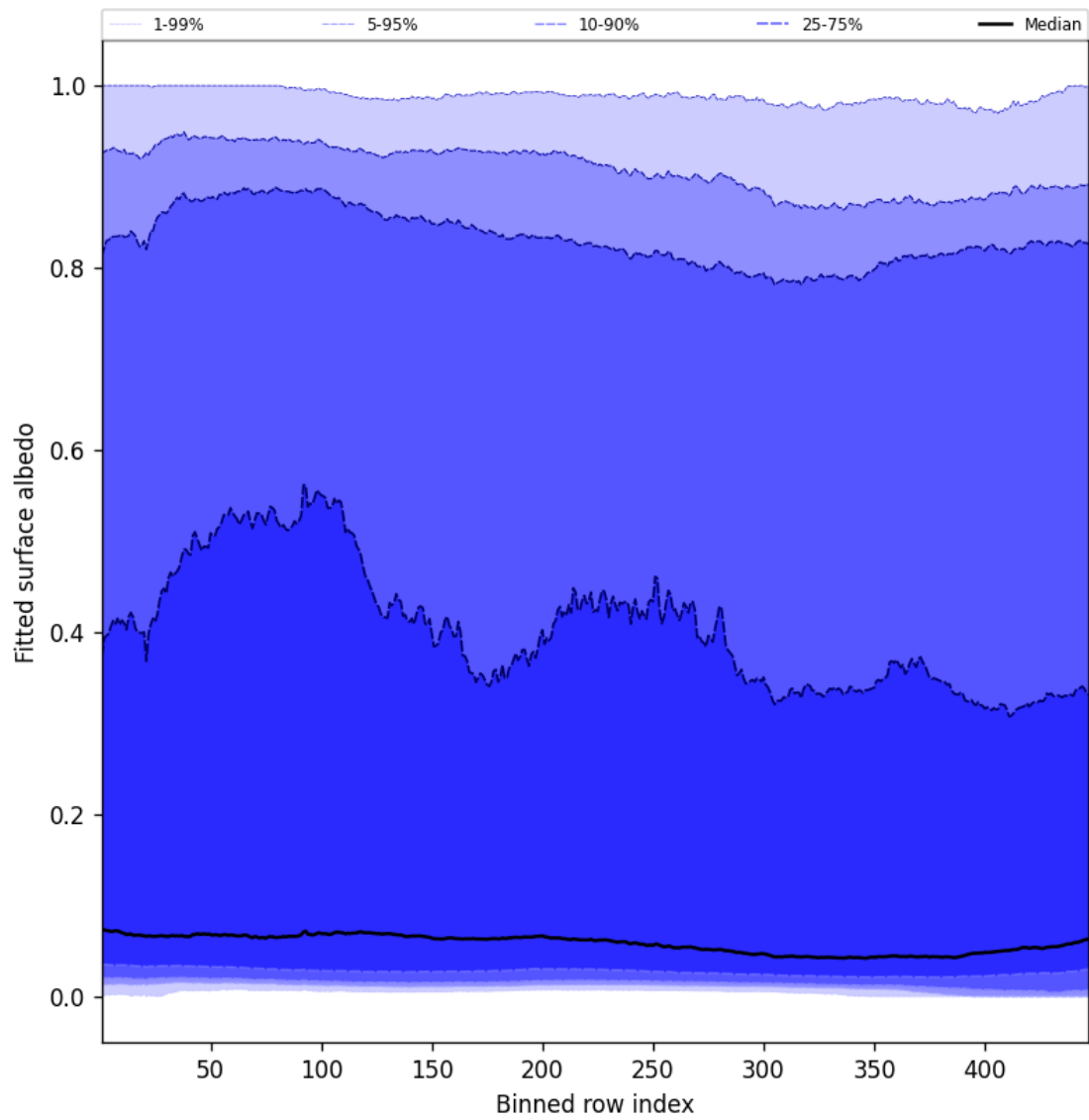
Figure 59: Along track statistics of “Fitted surface albedo” for 2025-04-24 to 2025-04-25
