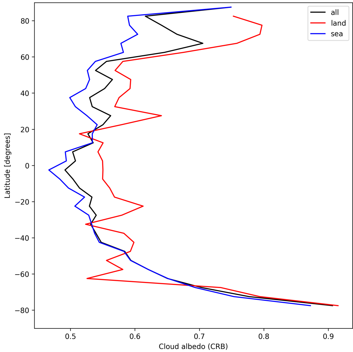
Figure 26: Zonal average of “Cloud albedo (CRB)” for 2025-04-24 to 2025-04-25.
