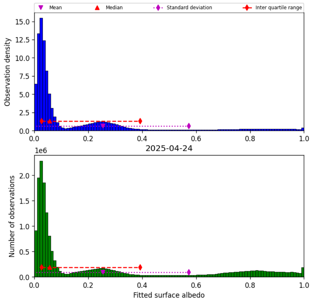
Figure 43: Histogram of “Fitted surface albedo” for 2025-04-24 to 2025-04-25
