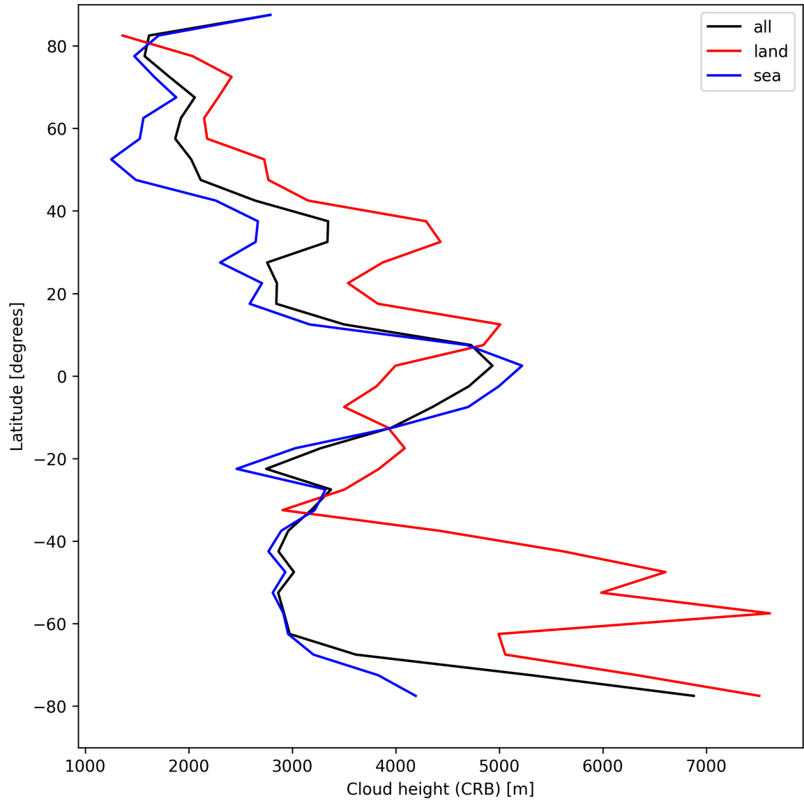
Figure 25: Zonal average of “Cloud height (CRB)” for 2025-04-24 to 2025-04-25.
