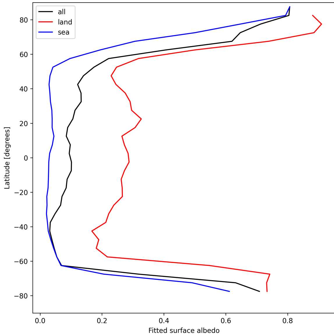
Figure 27: Zonal average of “Fitted surface albedo” for 2025-04-24 to 2025-04-25.
