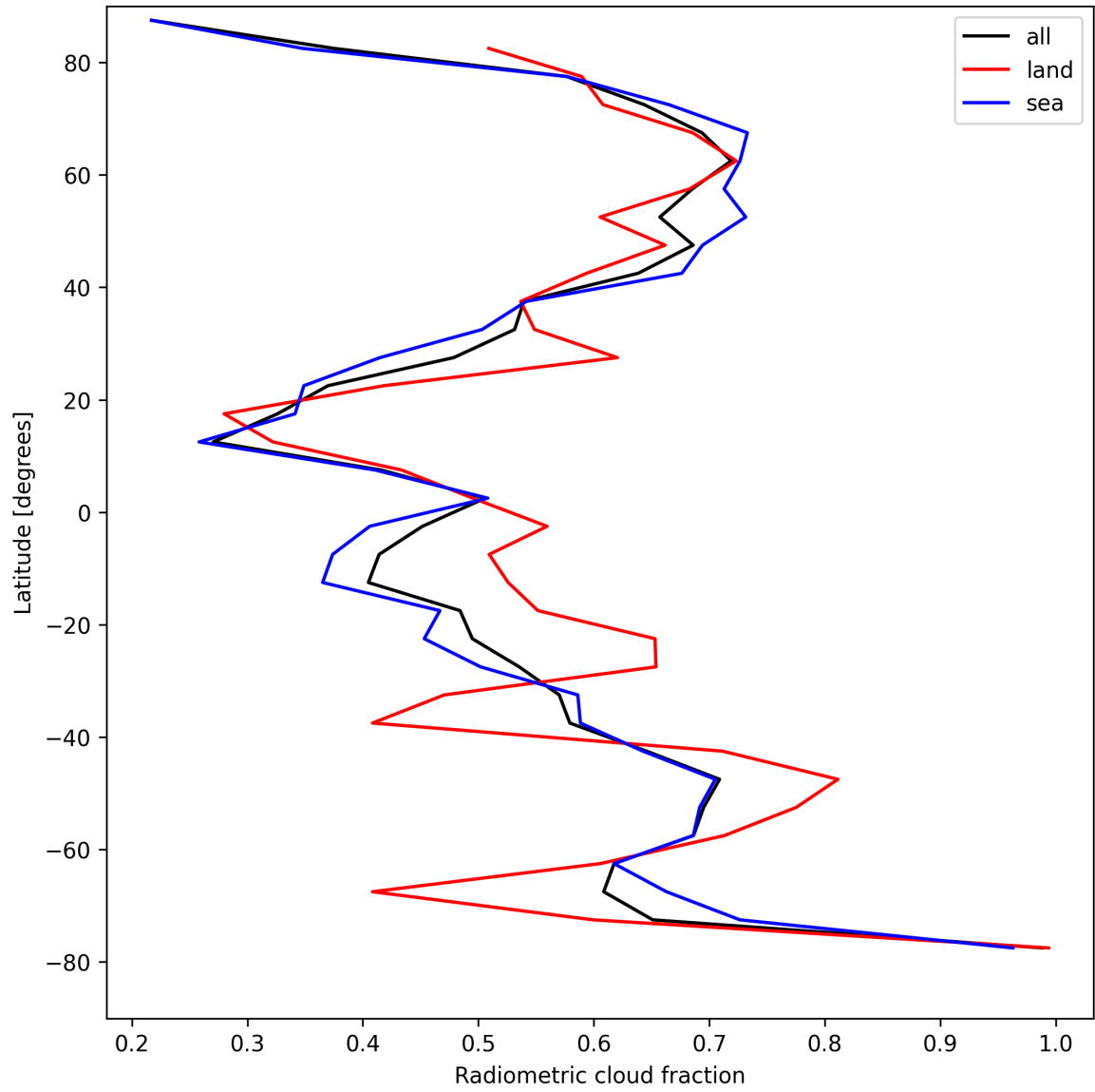
Figure 21: Zonal average of “Radiometric cloud fraction” for 2025-04-24 to 2025-04-25.
