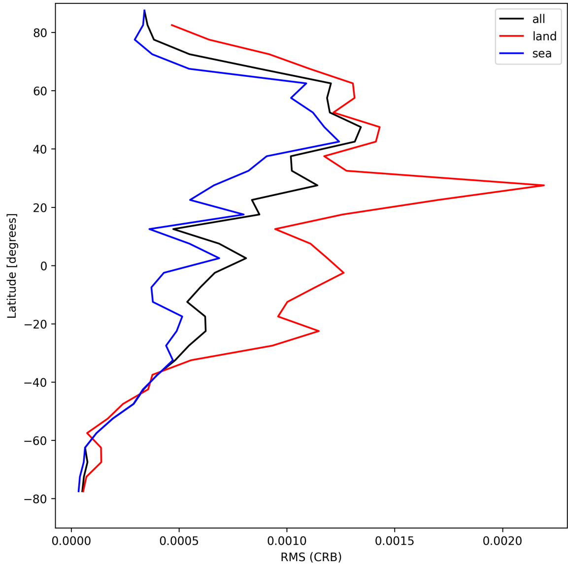
Figure 30: Zonal average of “RMS (CRB)” for 2025-04-24 to 2025-04-25.
