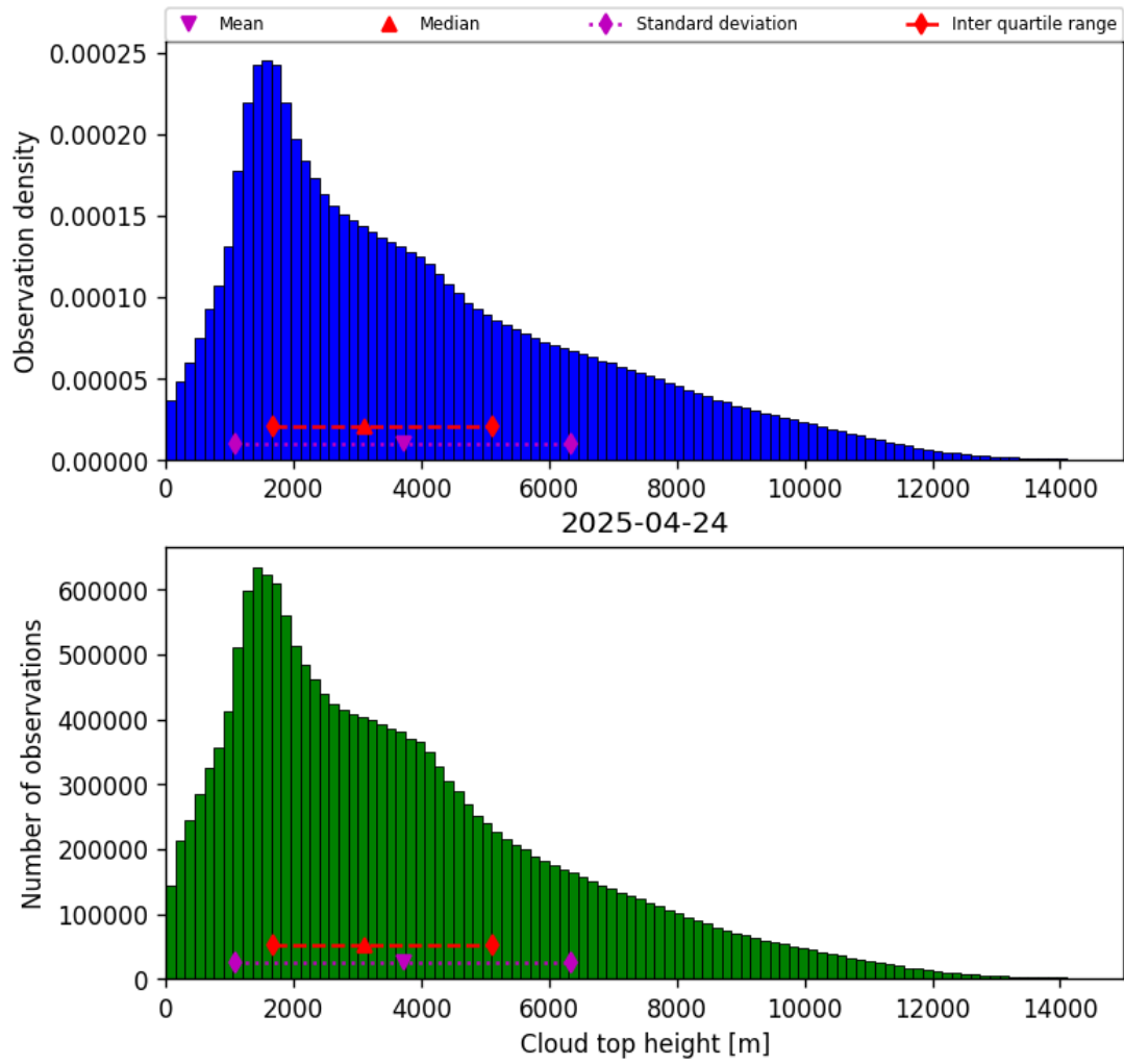
Figure 38: Histogram of “Cloud top height” for 2025-04-24 to 2025-04-25
