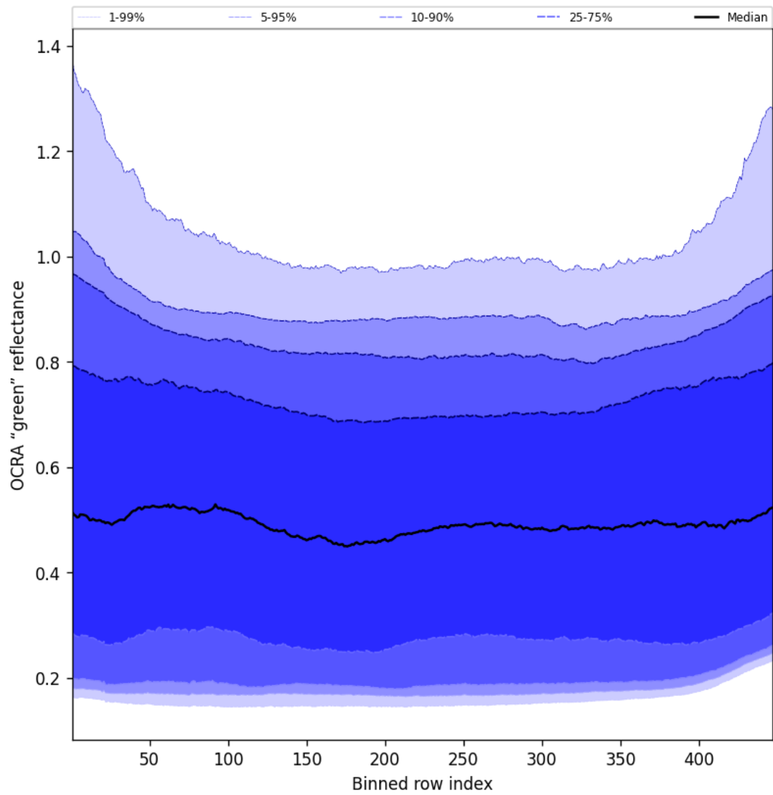
Figure 66: Along track statistics of “OCRA “green” reflectance” for 2025-04-24 to 2025-04-25
