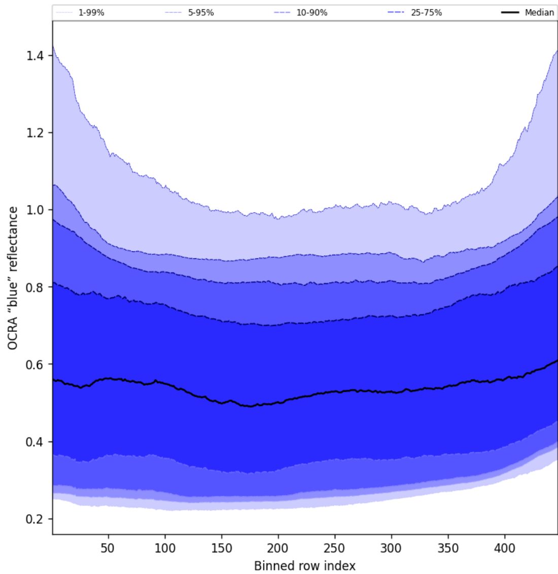
Figure 65: Along track statistics of “OCRA “blue” reflectance” for 2025-04-24 to 2025-04-25
