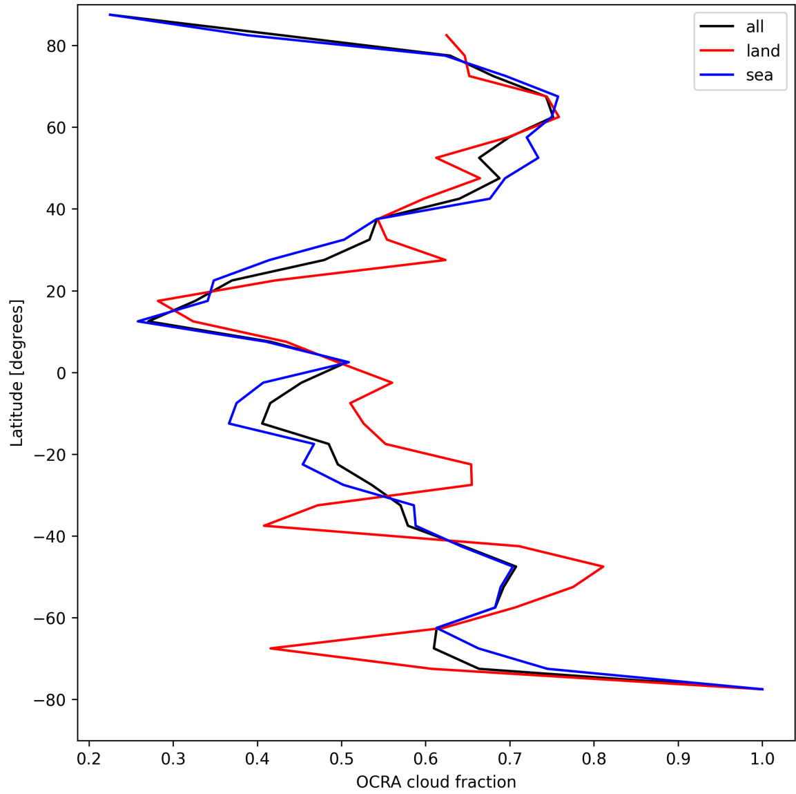
Figure 32: Zonal average of “OCRA cloud fraction” for 2025-04-24 to 2025-04-25.
