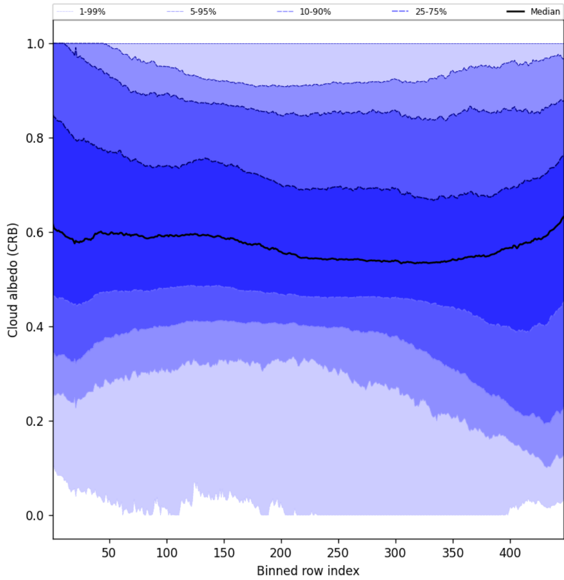
Figure 58: Along track statistics of “Cloud albedo (CRB)” for 2025-04-24 to 2025-04-25
