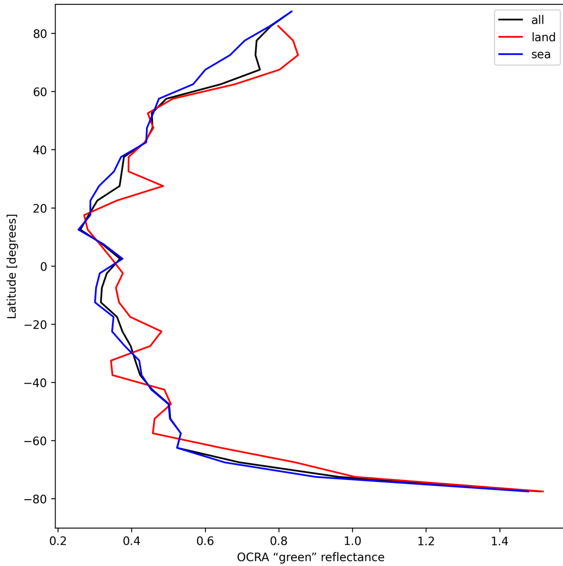
Figure 34: Zonal average of “OCRA “green” reflectance” for 2025-04-24 to 2025-04-25.
