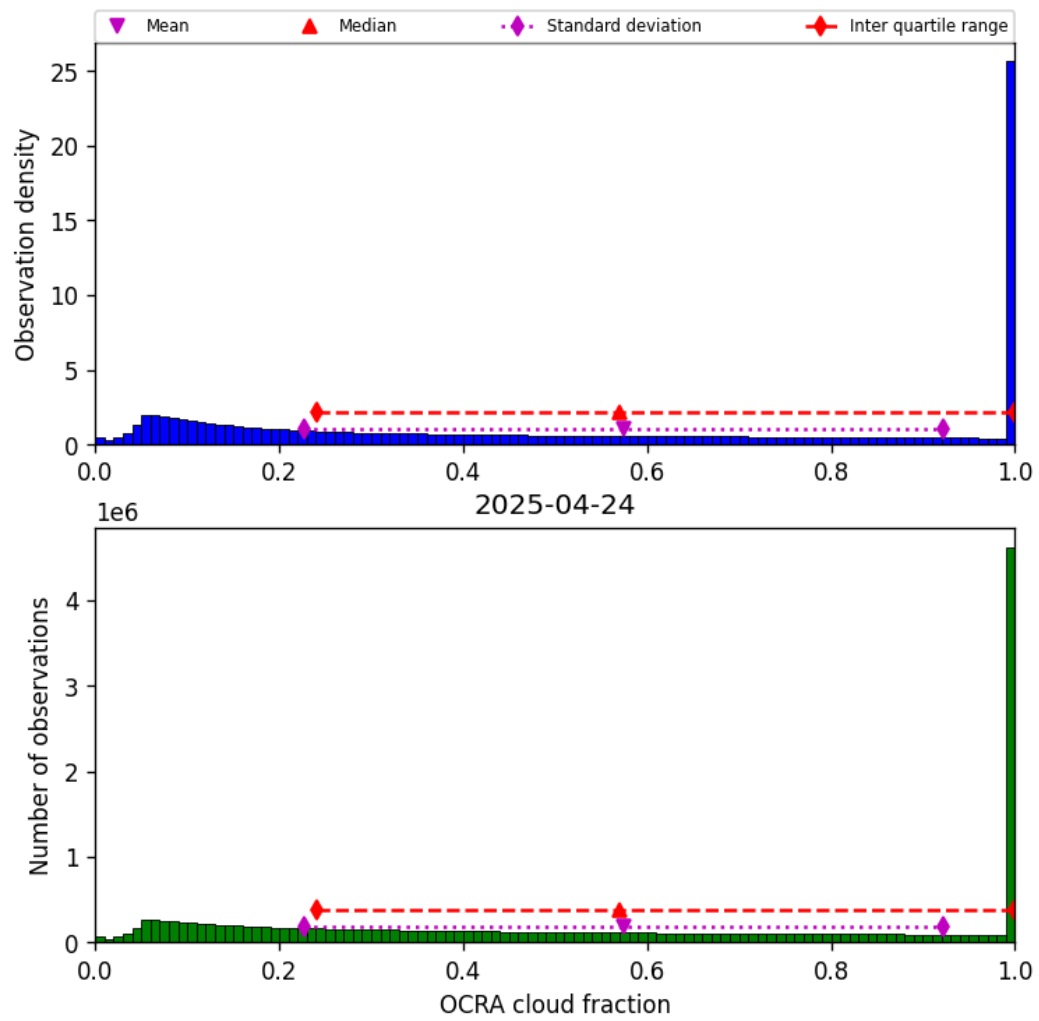
Figure 48: Histogram of “OCRA cloud fraction” for 2025-04-24 to 2025-04-25
