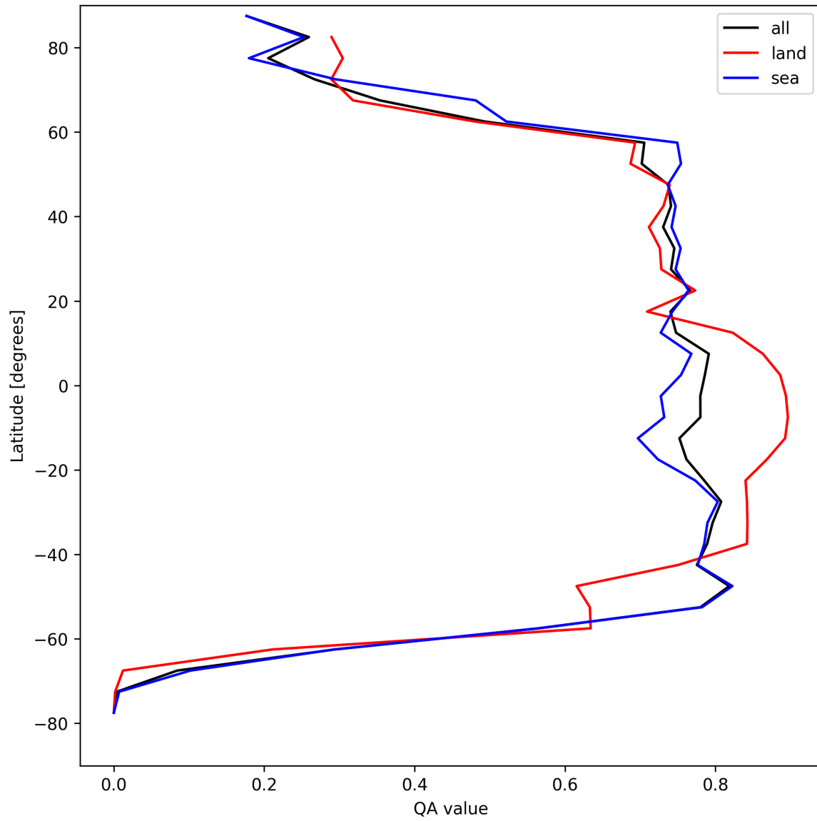
Figure 20: Zonal average of “QA value” for 2025-04-25 to 2025-04-26.
