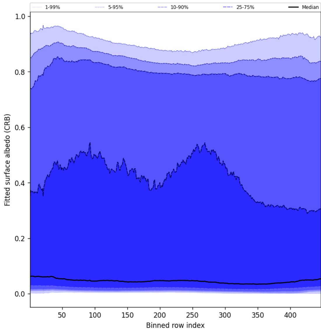
Figure 60: Along track statistics of “Fitted surface albedo (CRB)” for 2025-04-25 to 2025-04-26
