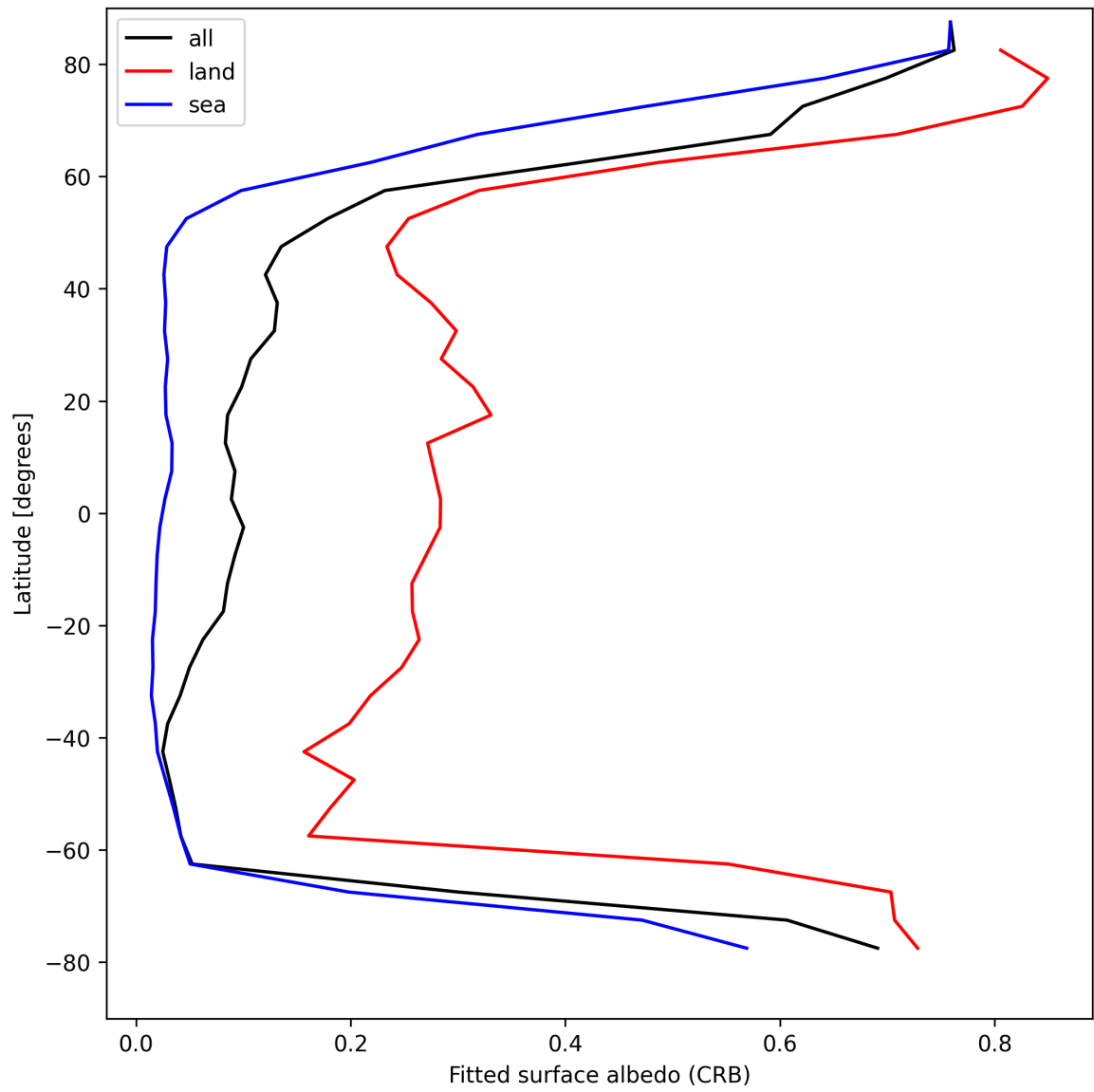
Figure 28: Zonal average of “Fitted surface albedo (CRB)” for 2025-04-25 to 2025-04-26.
