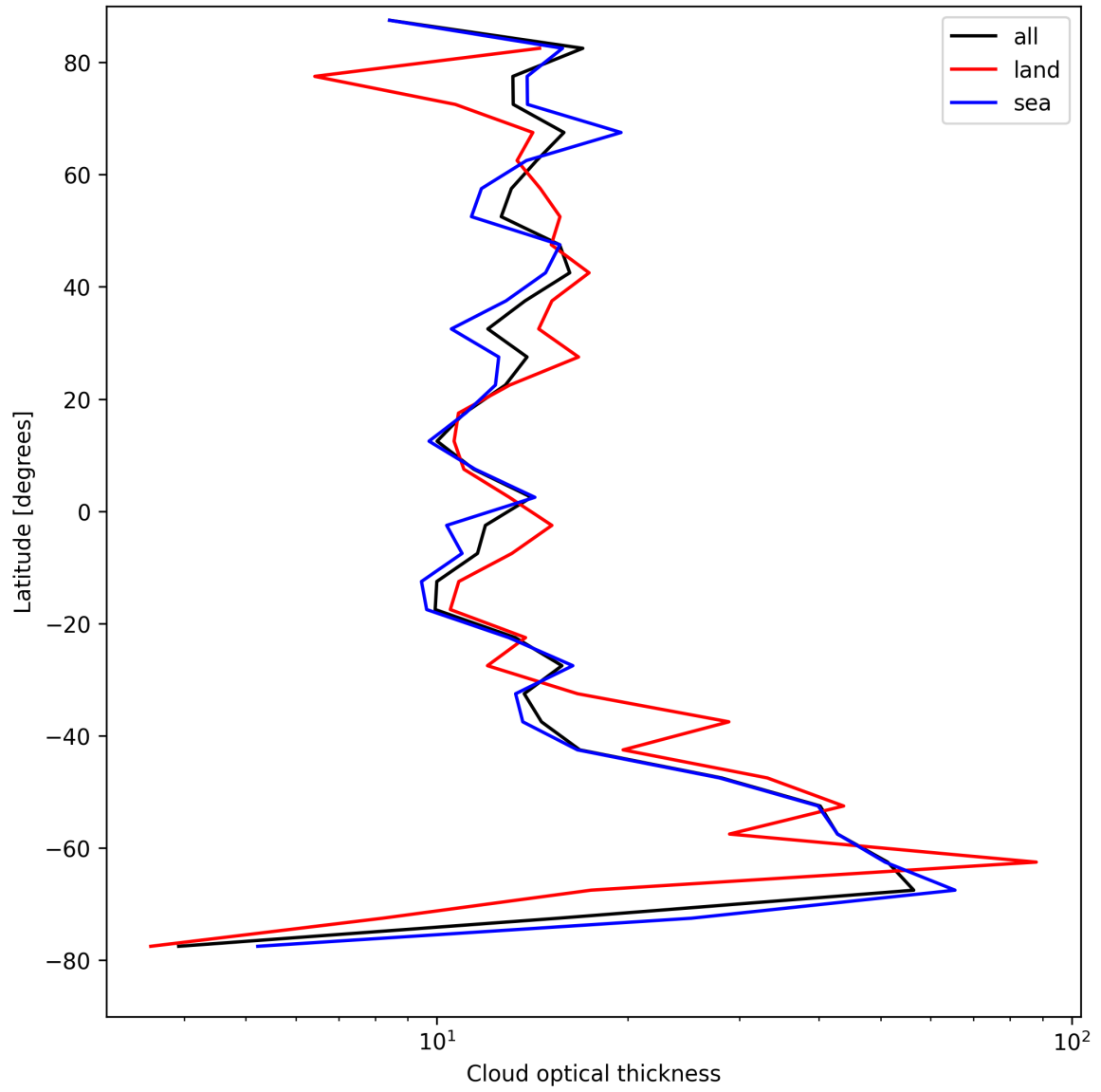
Figure 23: Zonal average of “Cloud optical thickness” for 2025-04-25 to 2025-04-26.
