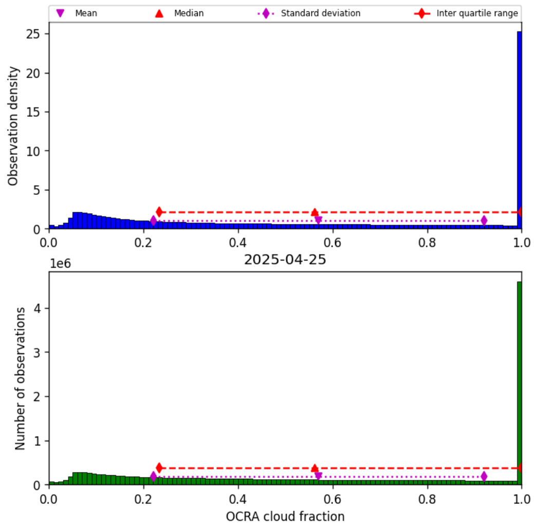
Figure 48: Histogram of “OCRA cloud fraction” for 2025-04-25 to 2025-04-26
