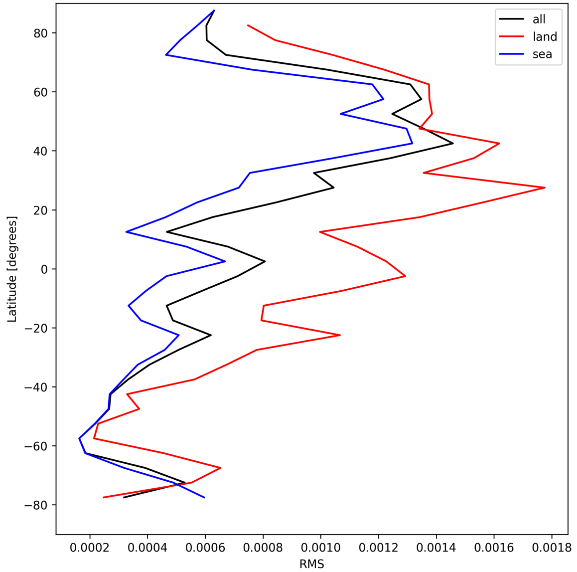
Figure 29: Zonal average of “RMS” for 2025-04-25 to 2025-04-26.
