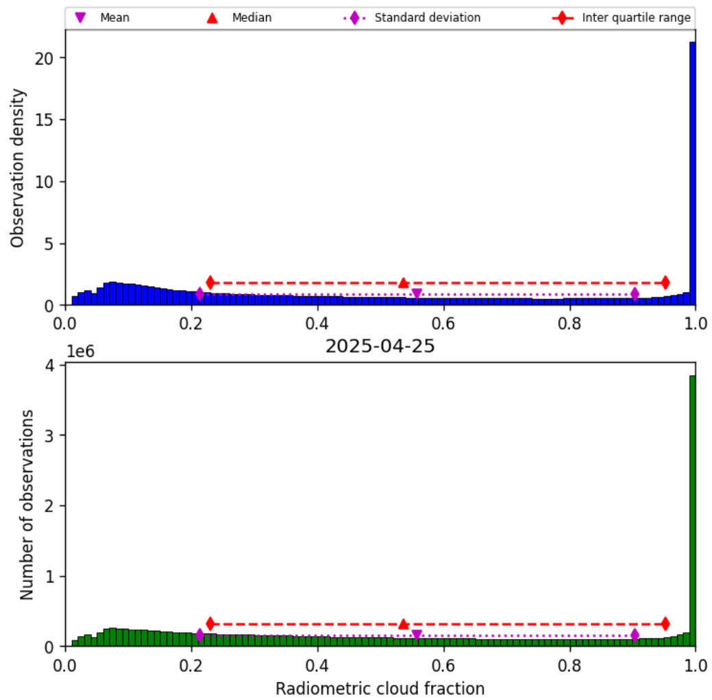
Figure 37: Histogram of “Radiometric cloud fraction” for 2025-04-25 to 2025-04-26
