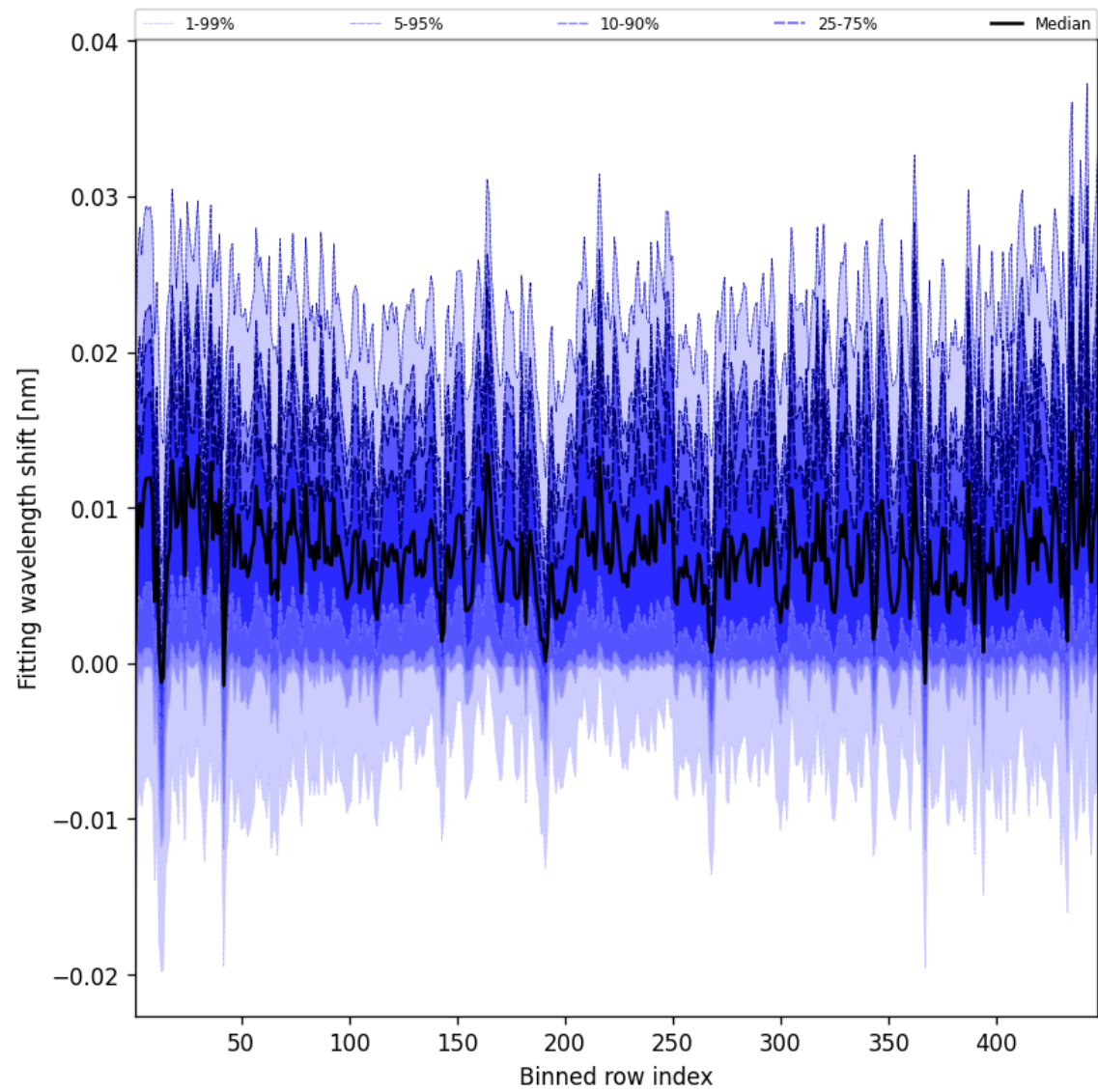
Figure 63: Along track statistics of “Fitting wavelength shift” for 2025-04-25 to 2025-04-26
