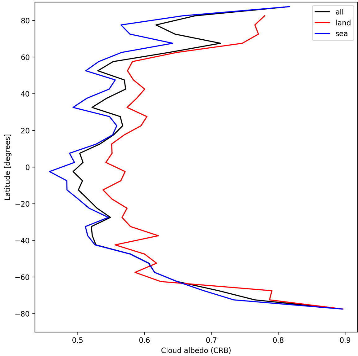
Figure 26: Zonal average of “Cloud albedo (CRB)” for 2025-04-25 to 2025-04-26.
