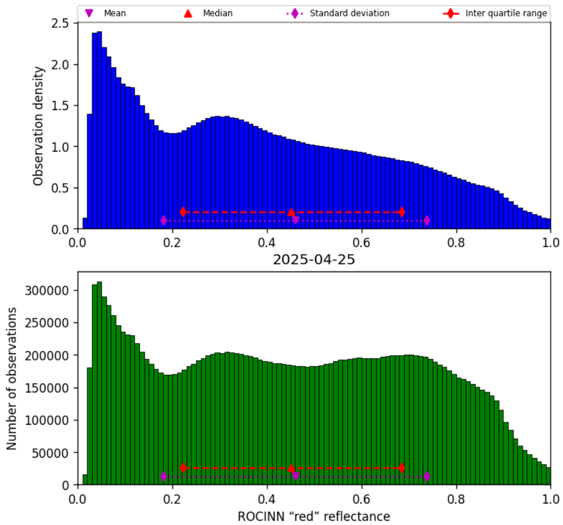
Figure 51: Histogram of “ROCINN “red” reflectance” for 2025-04-25 to 2025-04-26
