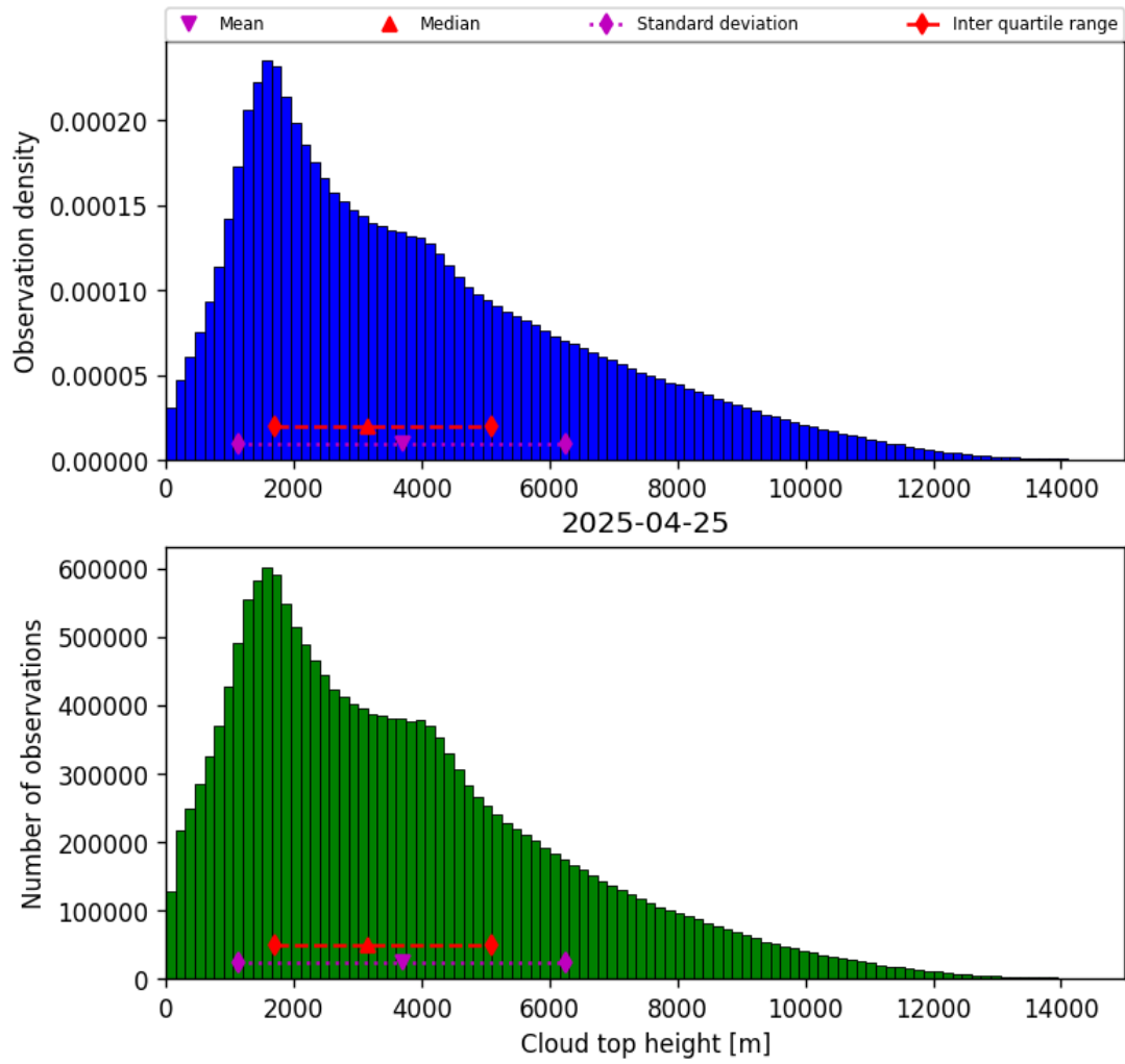
Figure 38: Histogram of “Cloud top height” for 2025-04-25 to 2025-04-26
