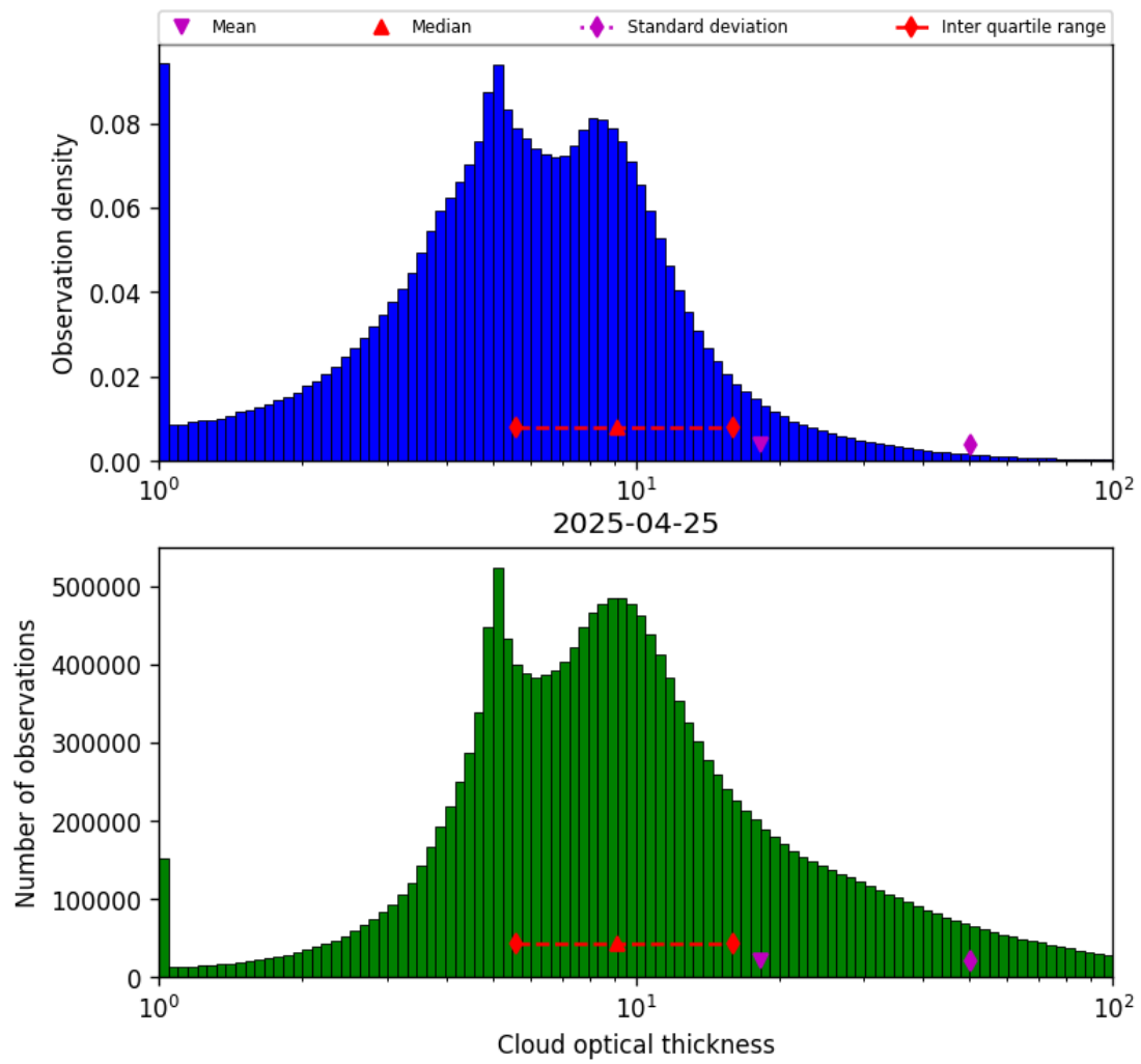
Figure 39: Histogram of “Cloud optical thickness” for 2025-04-25 to 2025-04-26
