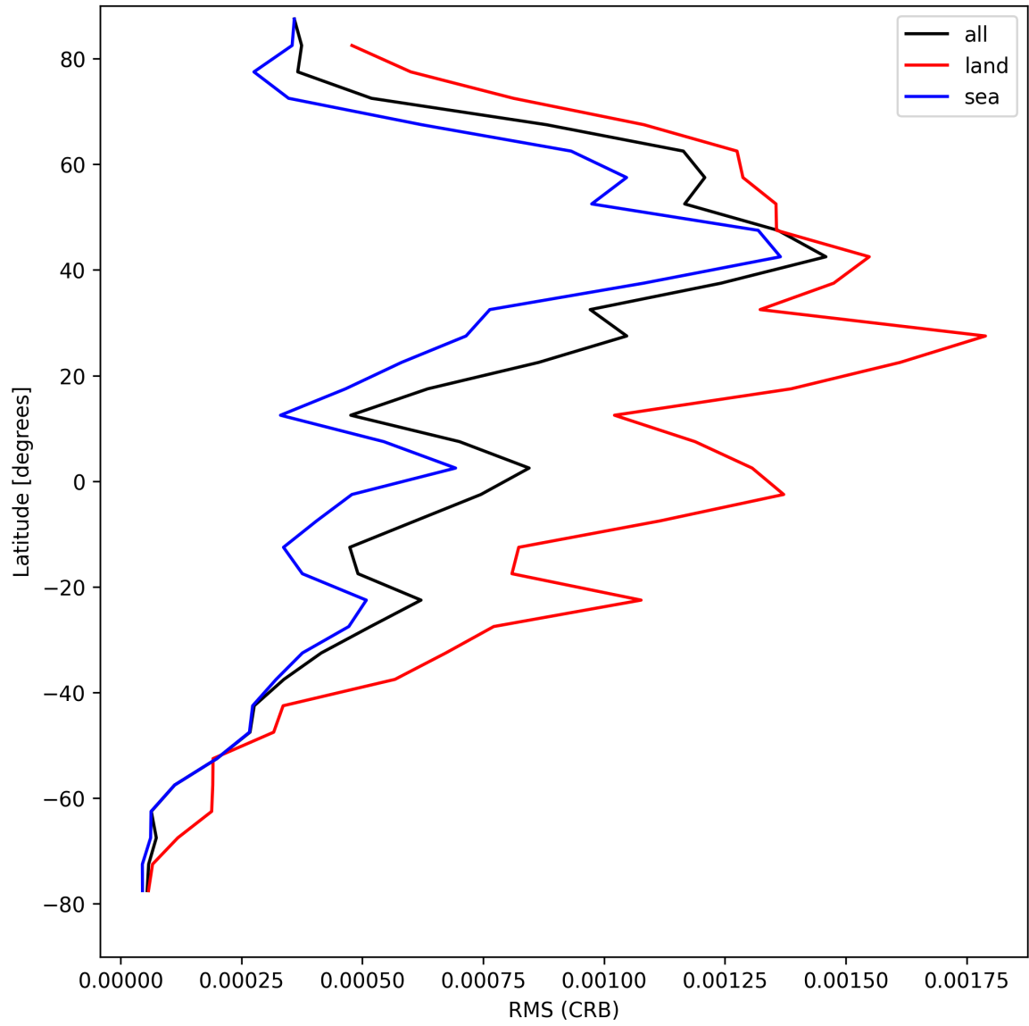
Figure 30: Zonal average of “RMS (CRB)” for 2025-04-25 to 2025-04-26.
