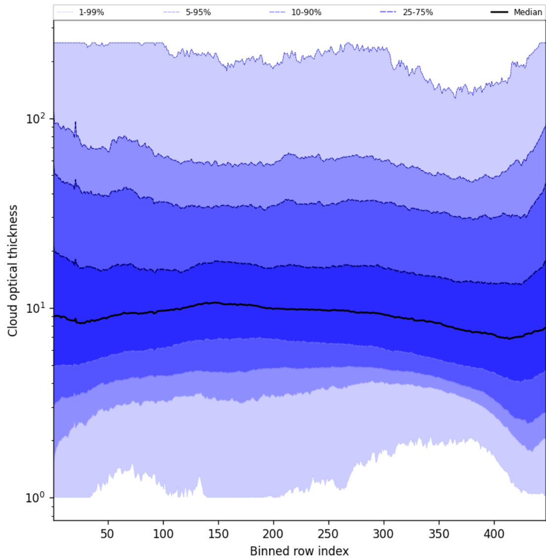
Figure 55: Along track statistics of “Cloud optical thickness” for 2025-04-25 to 2025-04-26
