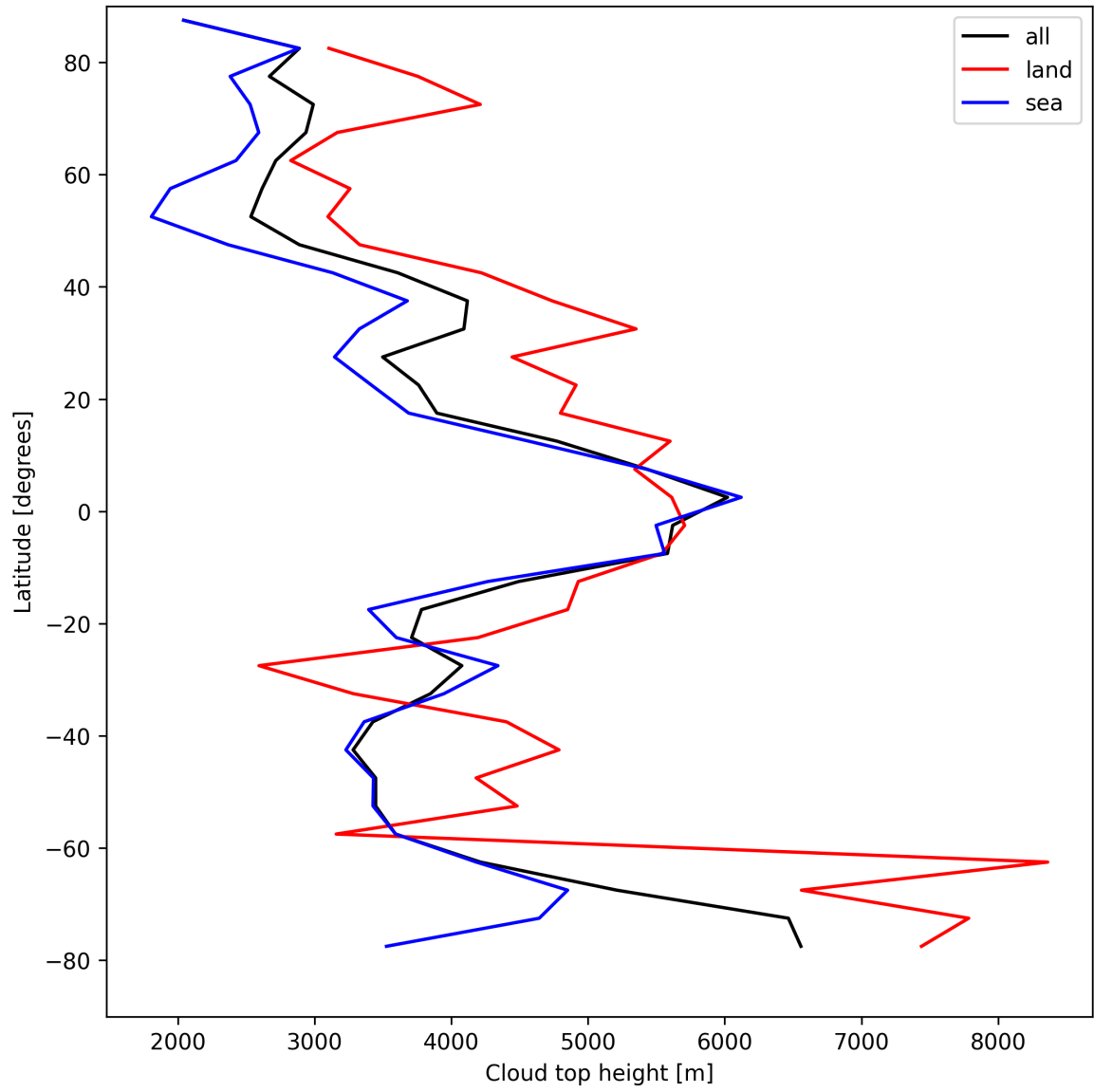
Figure 22: Zonal average of “Cloud top height” for 2025-04-25 to 2025-04-26.
