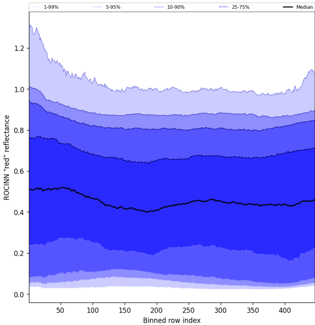
Figure 67: Along track statistics of "ROCINN "red" reflectance" for 2025-04-25 to 2025-04-26
