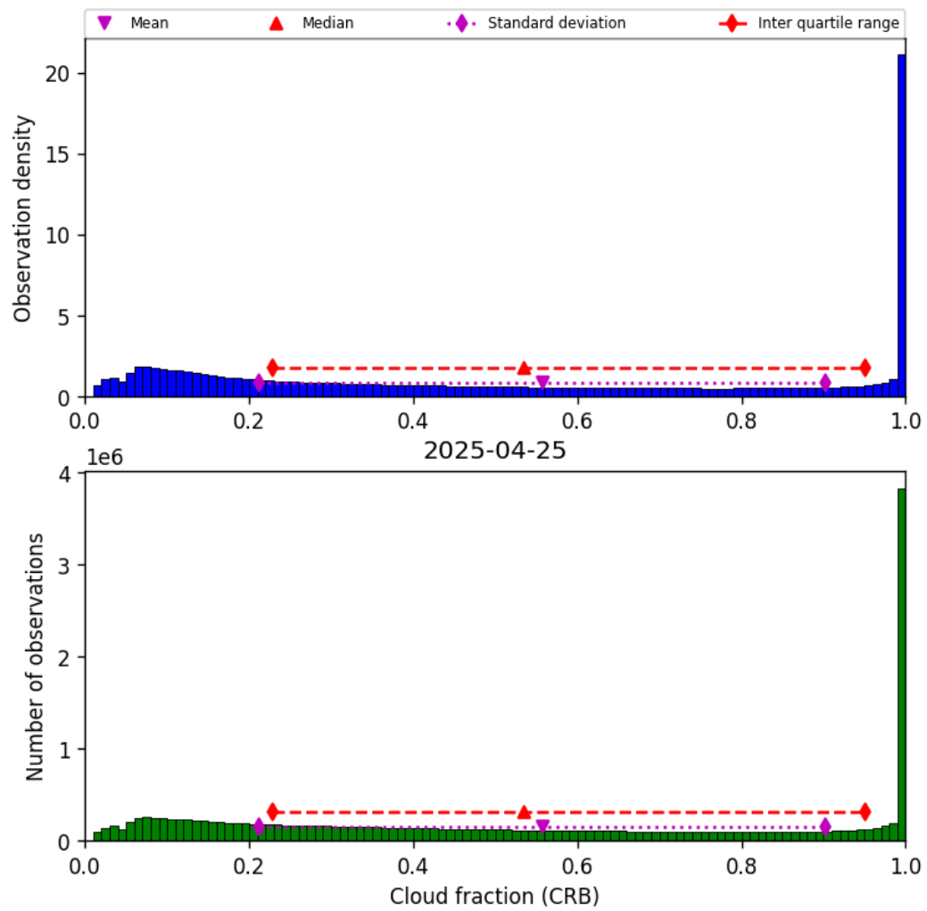
Figure 40: Histogram of “Cloud fraction (CRB)” for 2025-04-25 to 2025-04-26
