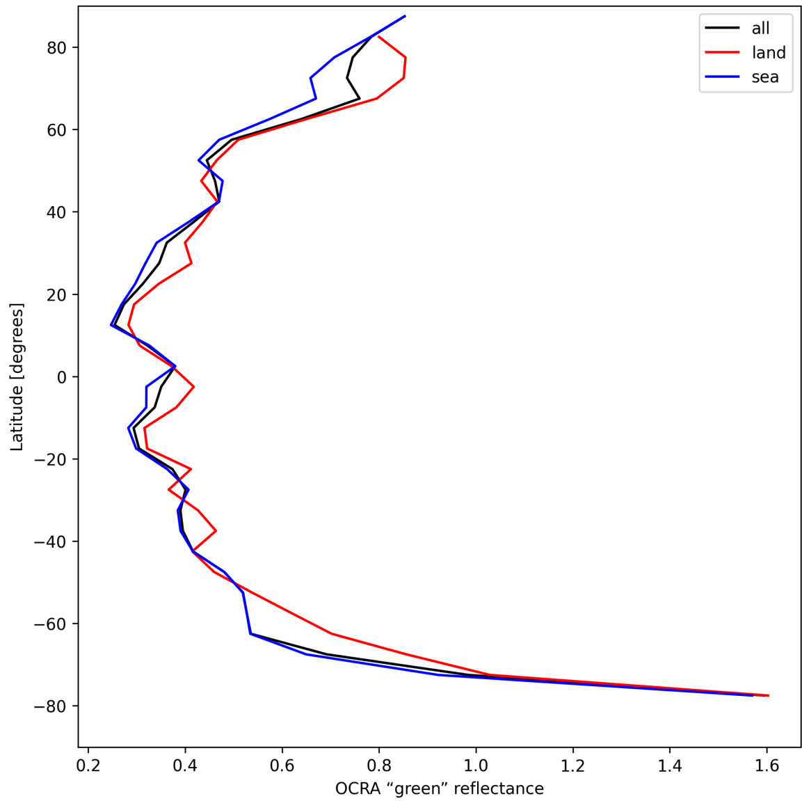
Figure 34: Zonal average of “OCRA “green” reflectance” for 2025-04-25 to 2025-04-26.
