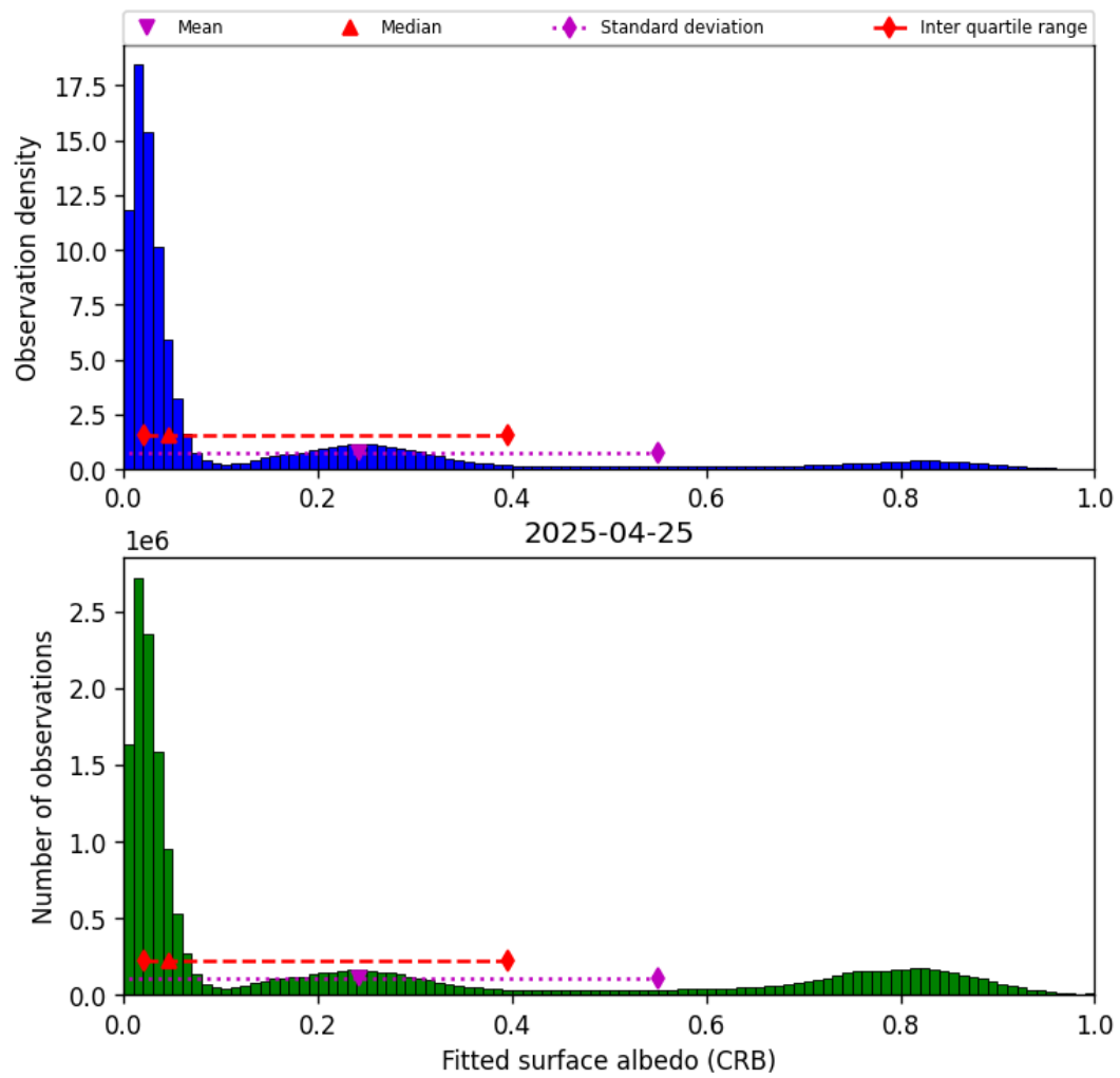
Figure 44: Histogram of “Fitted surface albedo (CRB)” for 2025-04-25 to 2025-04-26
