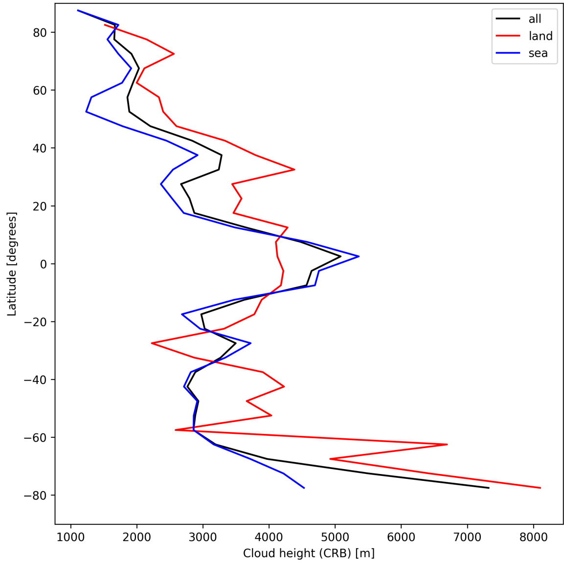
Figure 25: Zonal average of “Cloud height (CRB)” for 2025-04-25 to 2025-04-26.
