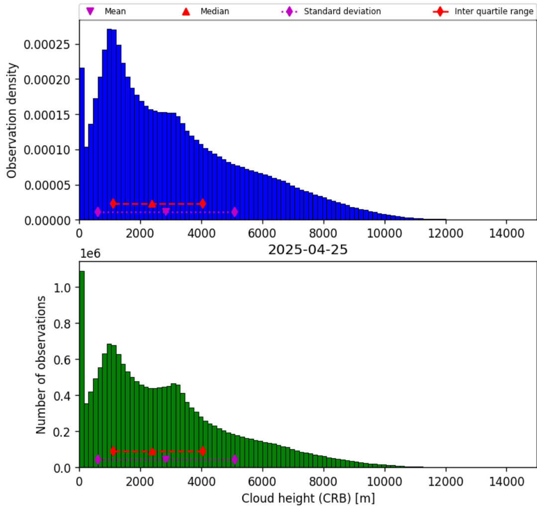
Figure 41: Histogram of “Cloud height (CRB)” for 2025-04-25 to 2025-04-26
