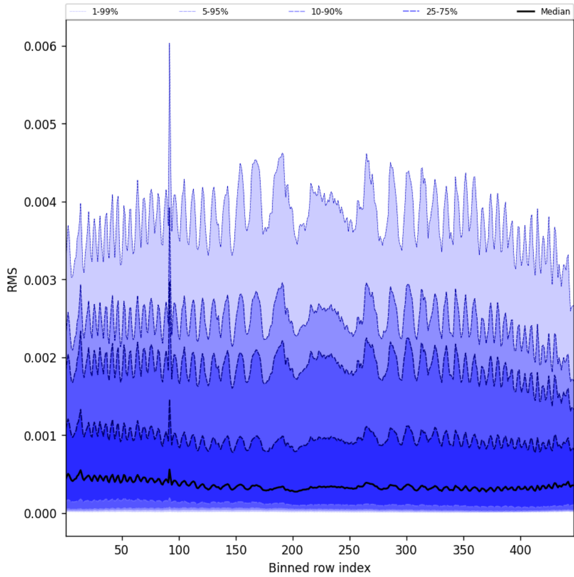
Figure 61: Along track statistics of “RMS” for 2025-04-25 to 2025-04-26
