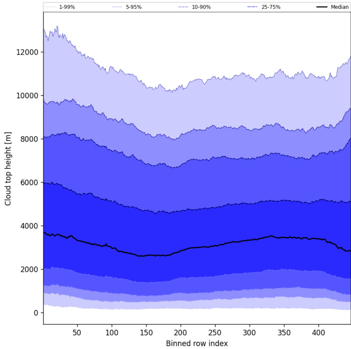
Figure 54: Along track statistics of “Cloud top height” for 2025-04-25 to 2025-04-26
