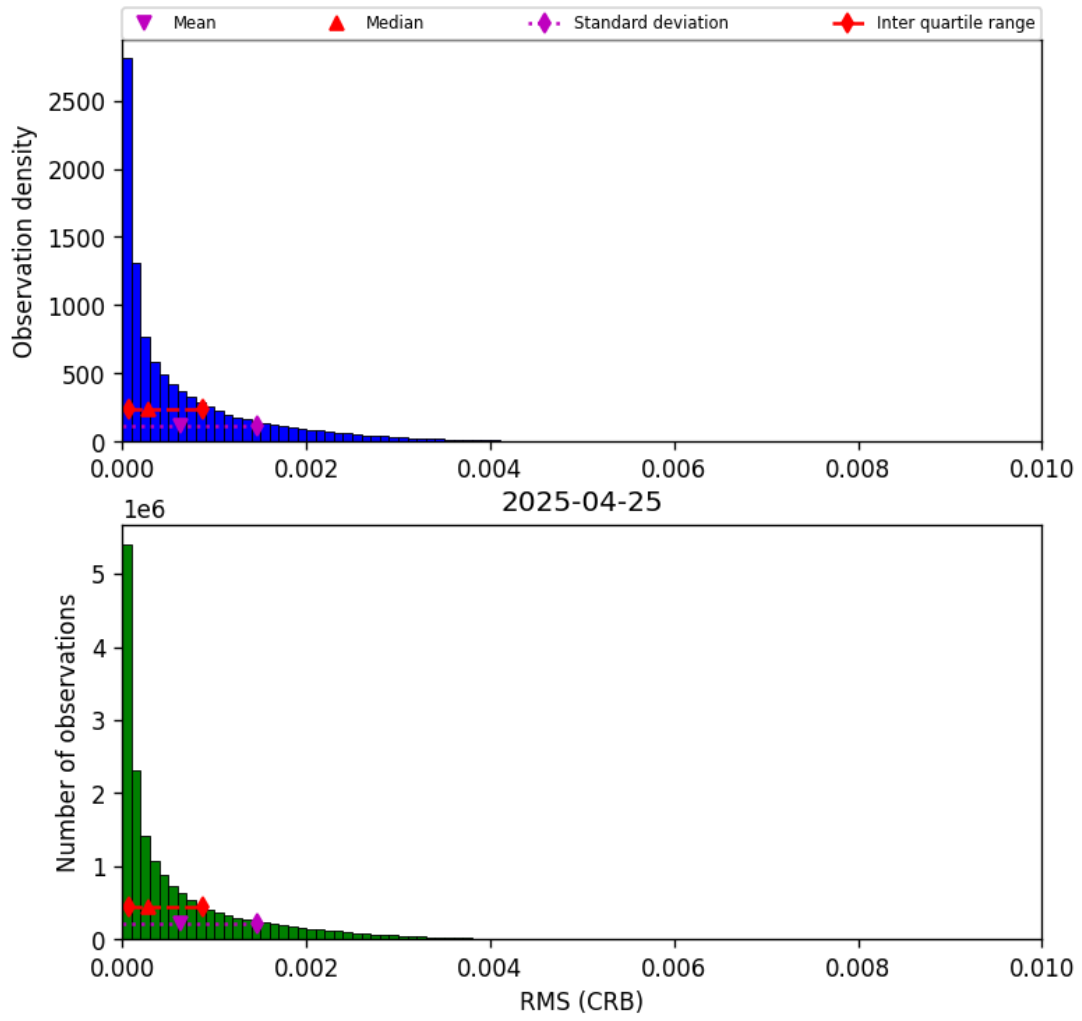
Figure 46: Histogram of “RMS (CRB)” for 2025-04-25 to 2025-04-26
