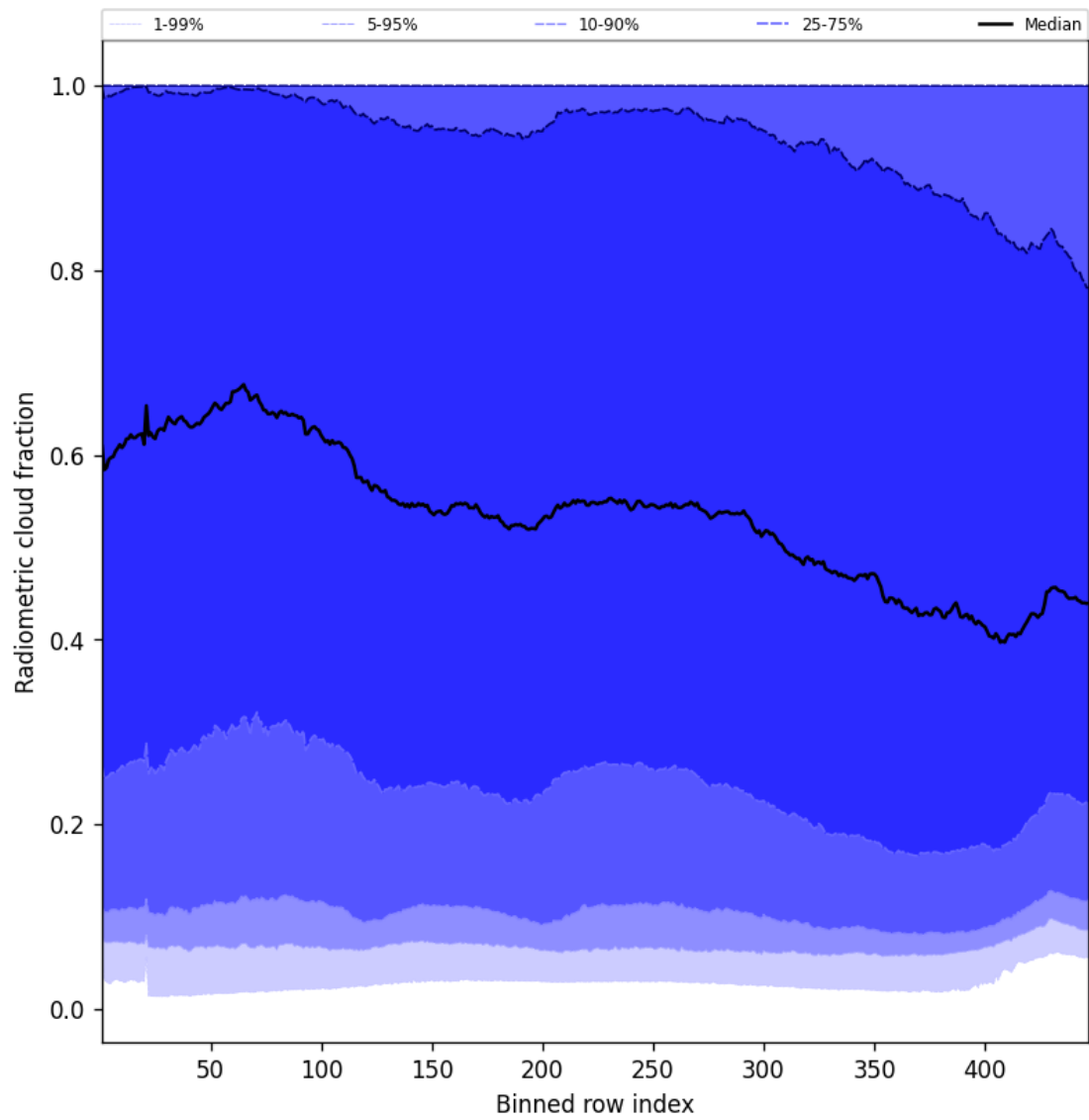
Figure 53: Along track statistics of “Radiometric cloud fraction” for 2025-04-25 to 2025-04-26
