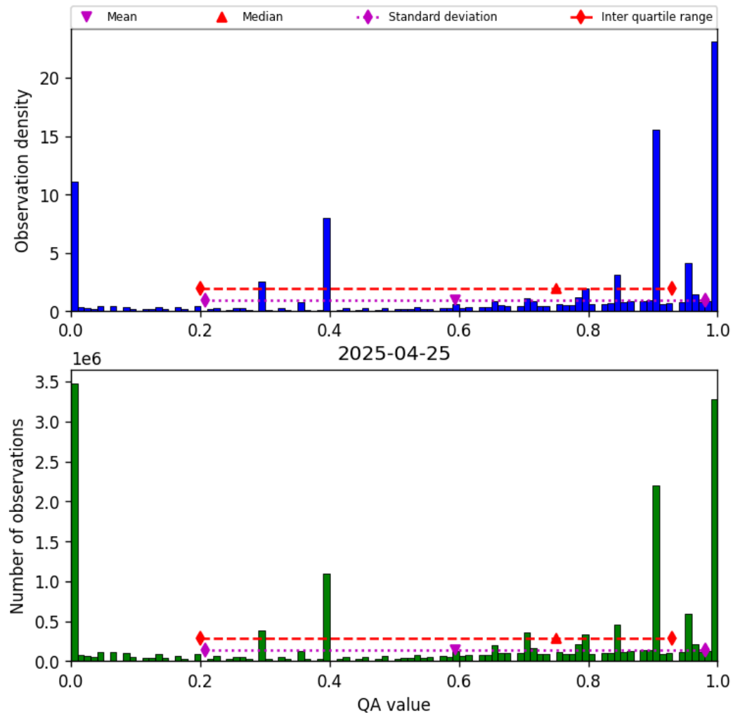
Figure 36: Histogram of “QA value” for 2025-04-25 to 2025-04-26
