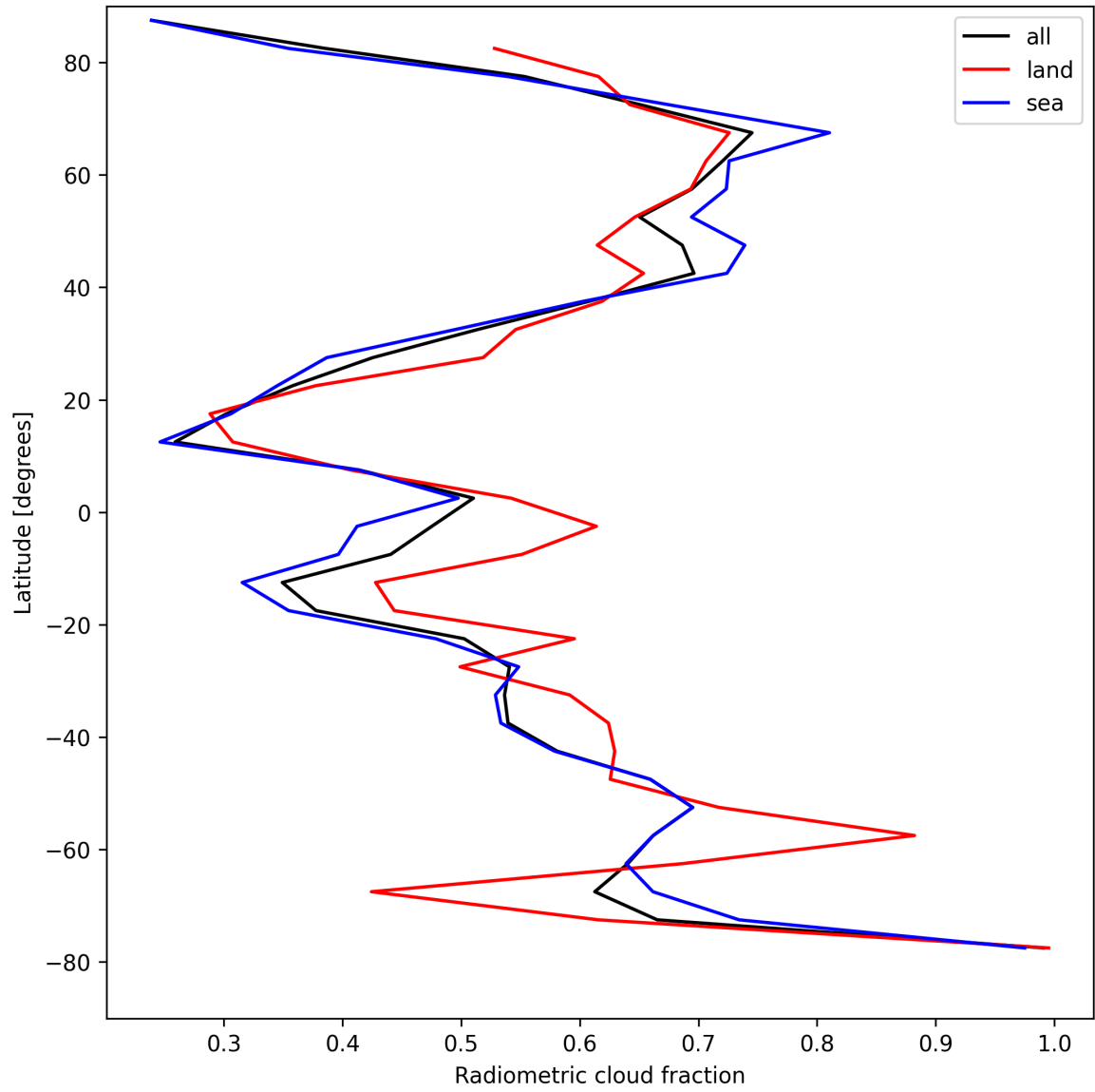
Figure 21: Zonal average of “Radiometric cloud fraction” for 2025-04-25 to 2025-04-26.
