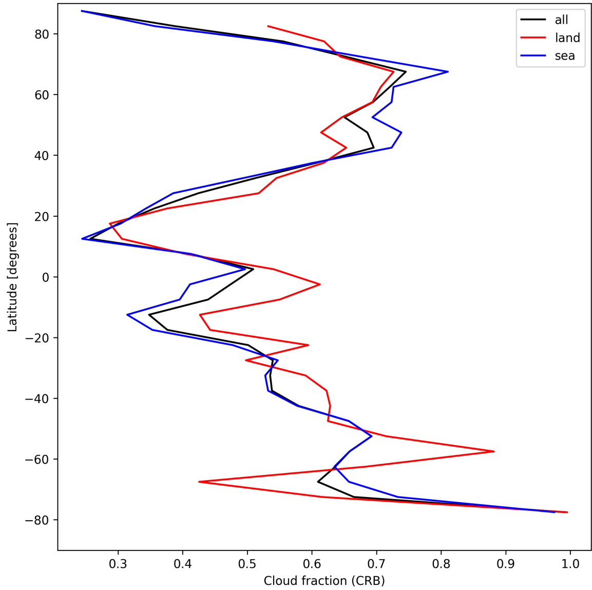
Figure 24: Zonal average of “Cloud fraction (CRB)” for 2025-04-25 to 2025-04-26.
