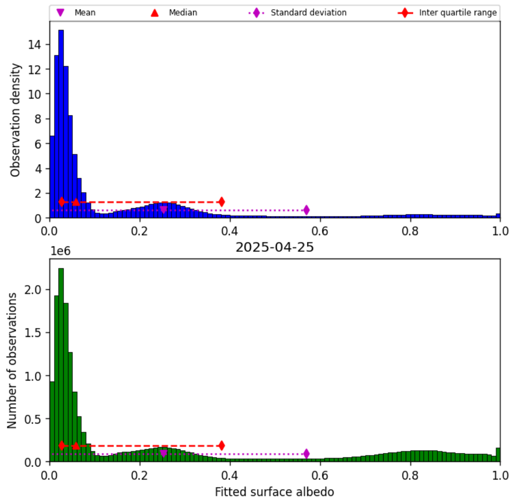
Figure 43: Histogram of “Fitted surface albedo” for 2025-04-25 to 2025-04-26
