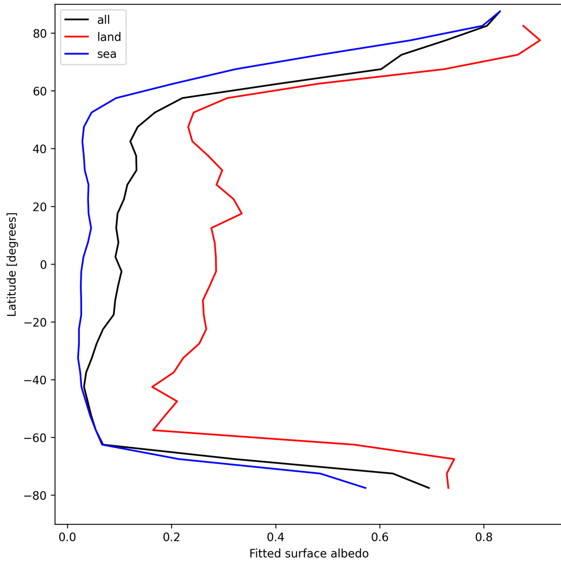
Figure 27: Zonal average of “Fitted surface albedo” for 2025-04-25 to 2025-04-26.
