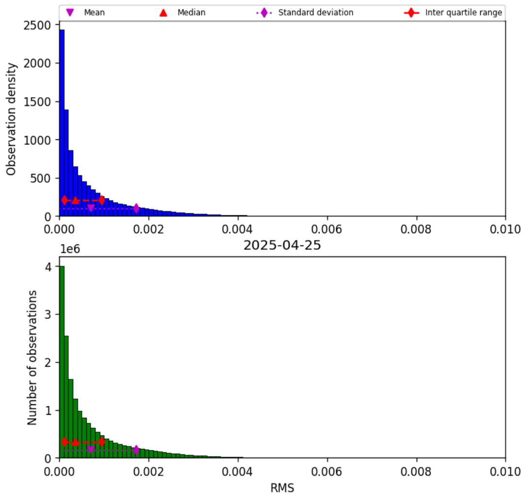
Figure 45: Histogram of “RMS” for 2025-04-25 to 2025-04-26
