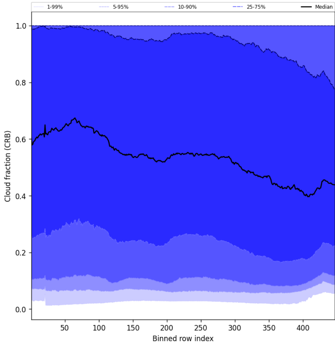
Figure 56: Along track statistics of “Cloud fraction (CRB)” for 2025-04-25 to 2025-04-26
