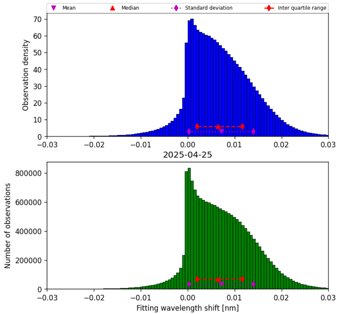
Figure 47: Histogram of “Fitting wavelength shift” for 2025-04-25 to 2025-04-26
