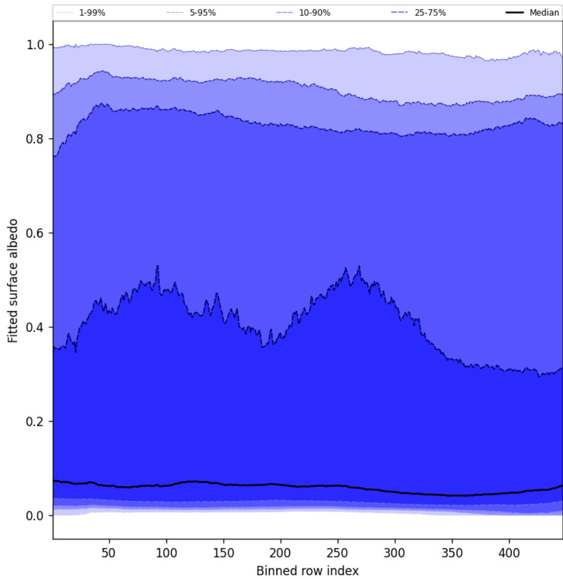
Figure 59: Along track statistics of “Fitted surface albedo” for 2025-04-25 to 2025-04-26
