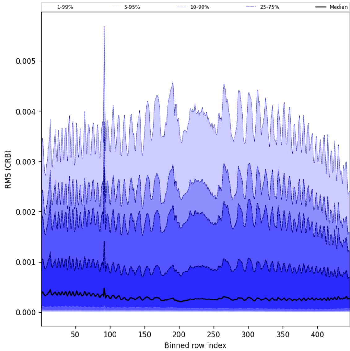
Figure 62: Along track statistics of “RMS (CRB)” for 2025-04-25 to 2025-04-26
