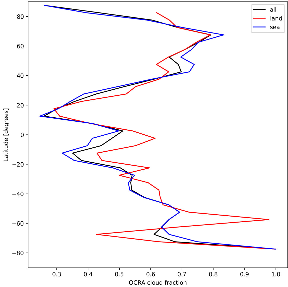
Figure 32: Zonal average of “OCRA cloud fraction” for 2025-04-25 to 2025-04-26.
