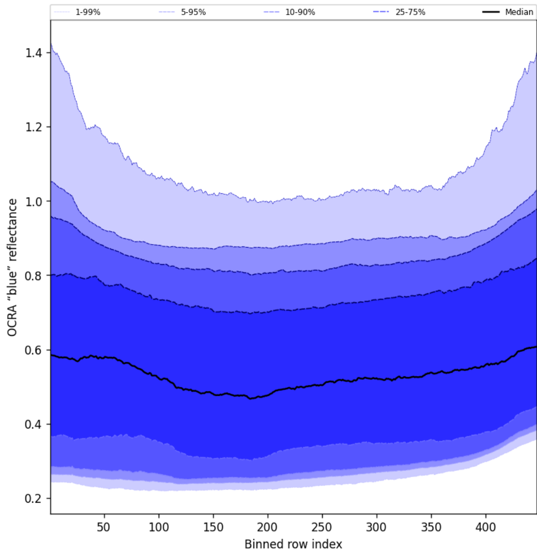
Figure 65: Along track statistics of “OCRA “blue” reflectance” for 2025-04-25 to 2025-04-26
