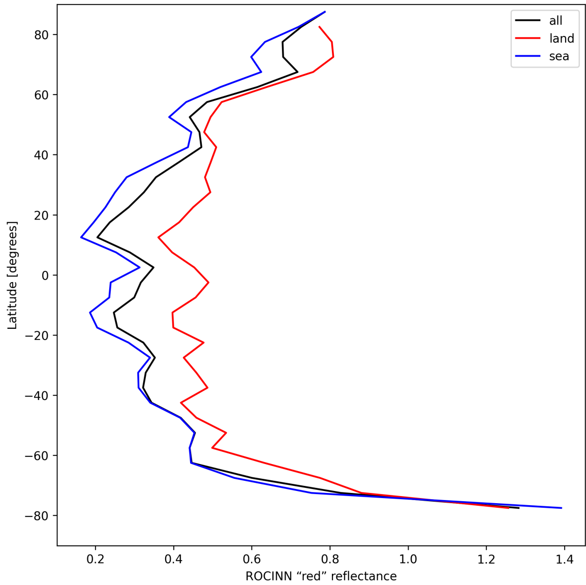
Figure 35: Zonal average of “ROCINN “red” reflectance” for 2025-04-25 to 2025-04-26.
