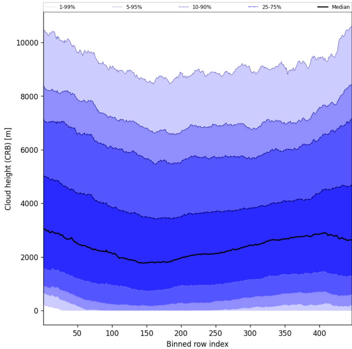
Figure 57: Along track statistics of “Cloud height (CRB)” for 2025-04-25 to 2025-04-26
