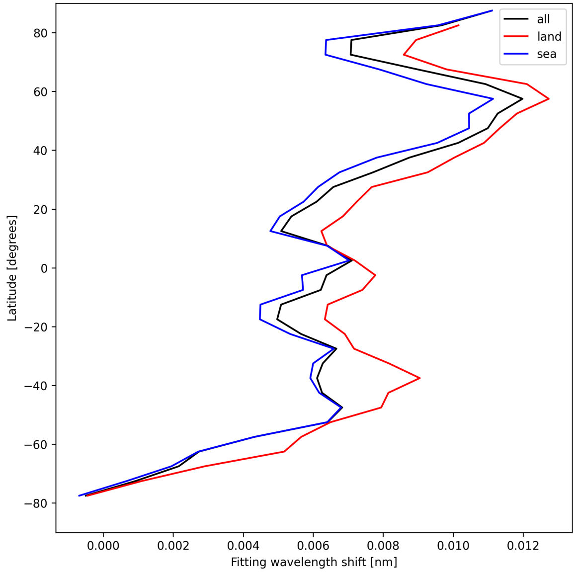
Figure 31: Zonal average of “Fitting wavelength shift” for 2025-04-25 to 2025-04-26.
