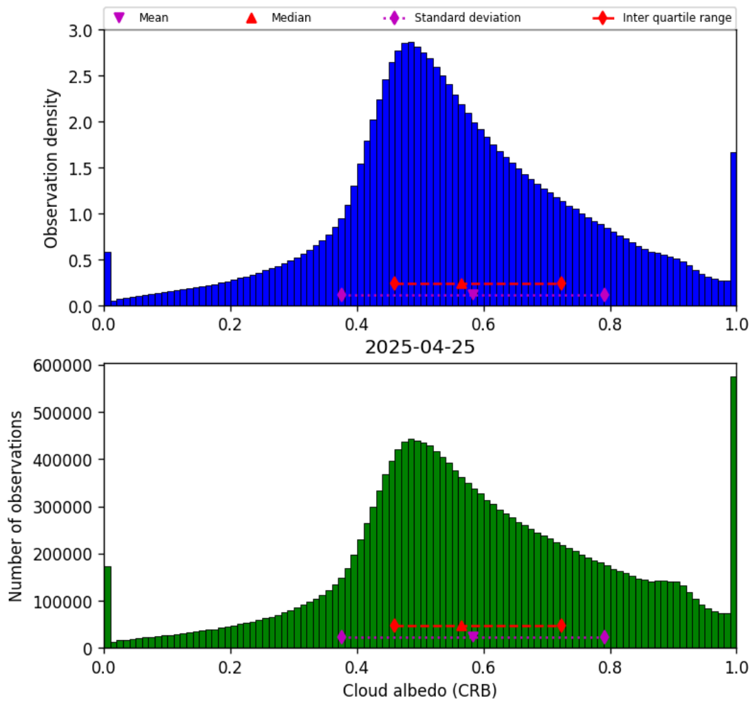
Figure 42: Histogram of “Cloud albedo (CRB)” for 2025-04-25 to 2025-04-26
