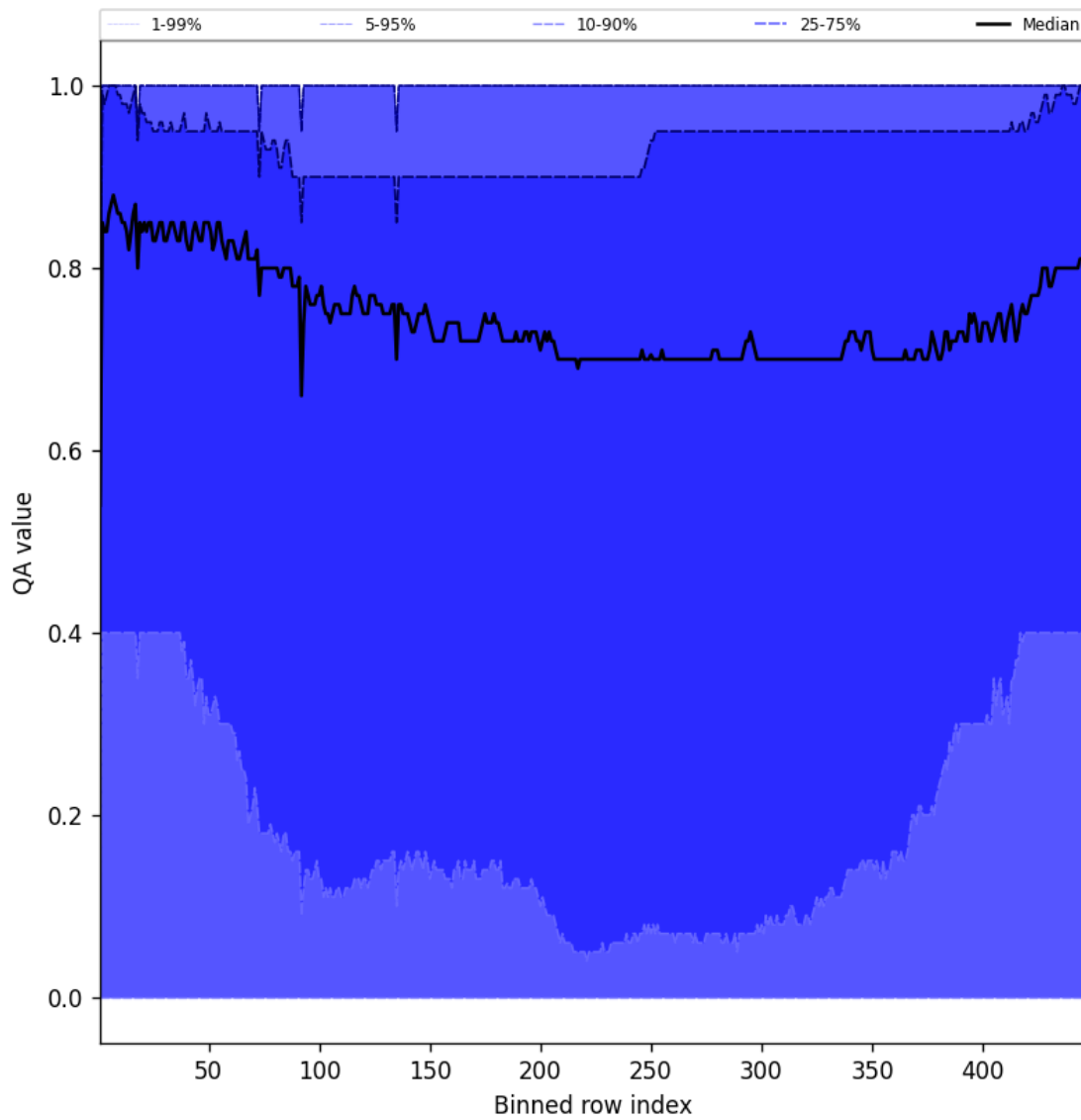
Figure 52: Along track statistics of "QA value" for 2025-04-25 to 2025-04-26
