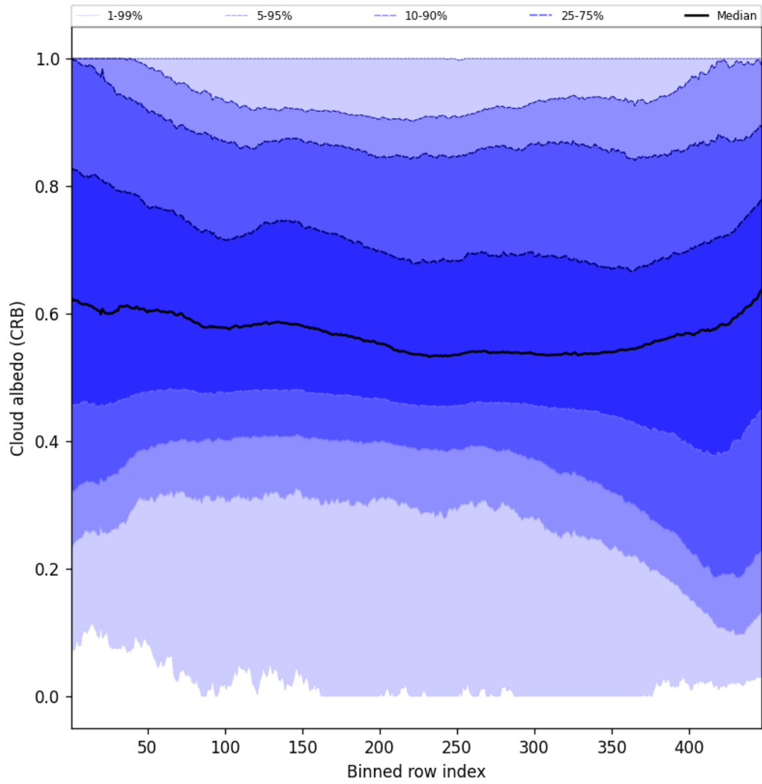
Figure 58: Along track statistics of “Cloud albedo (CRB)” for 2025-04-25 to 2025-04-26
