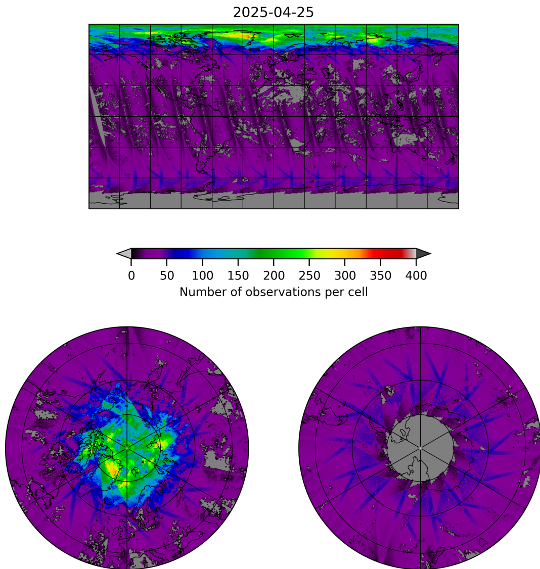
Figure 19: Map of the number of observations for 2025-04-25 to 2025-04-26
