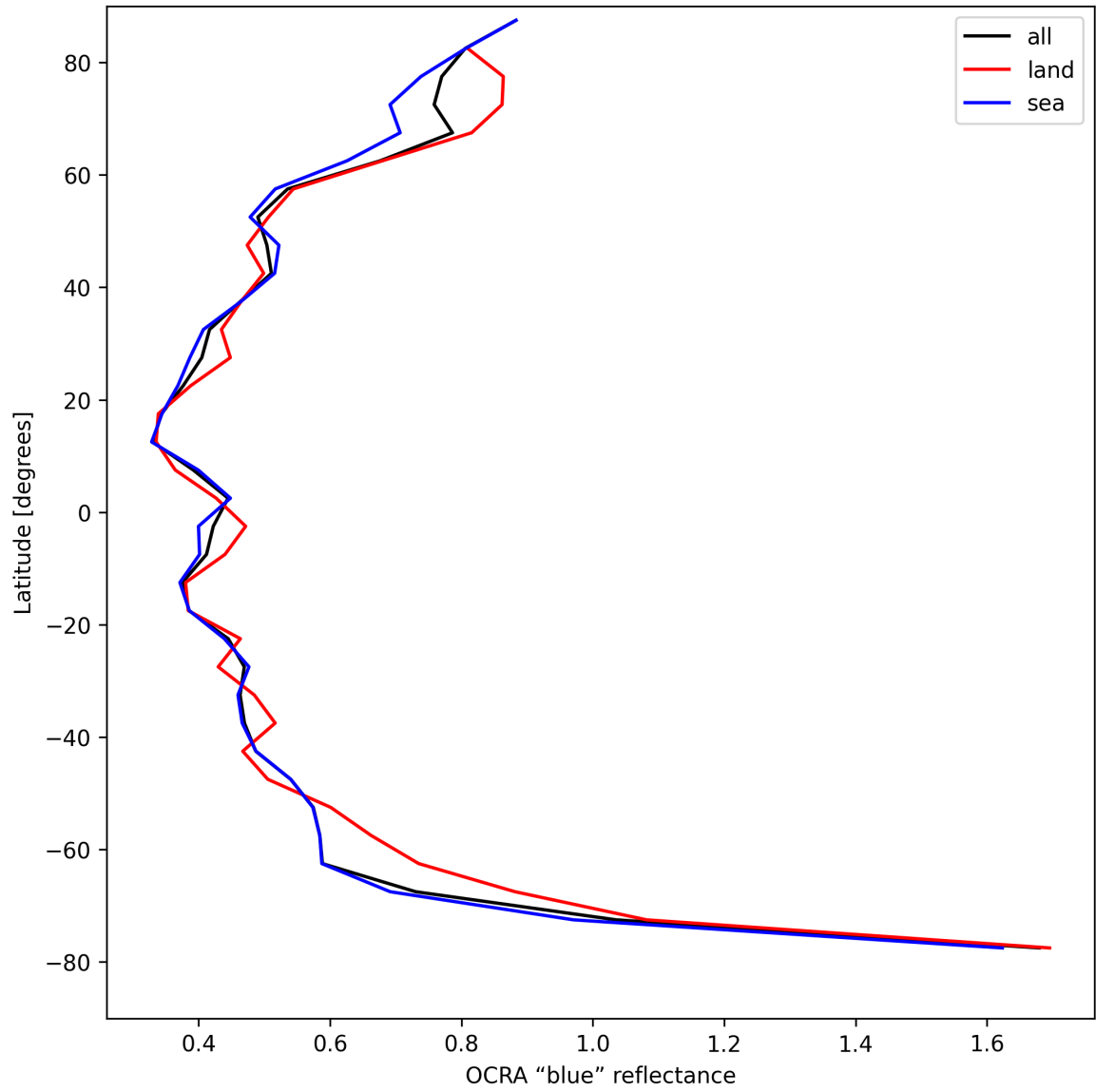
Figure 33: Zonal average of “OCRA “blue” reflectance” for 2025-04-25 to 2025-04-26.
