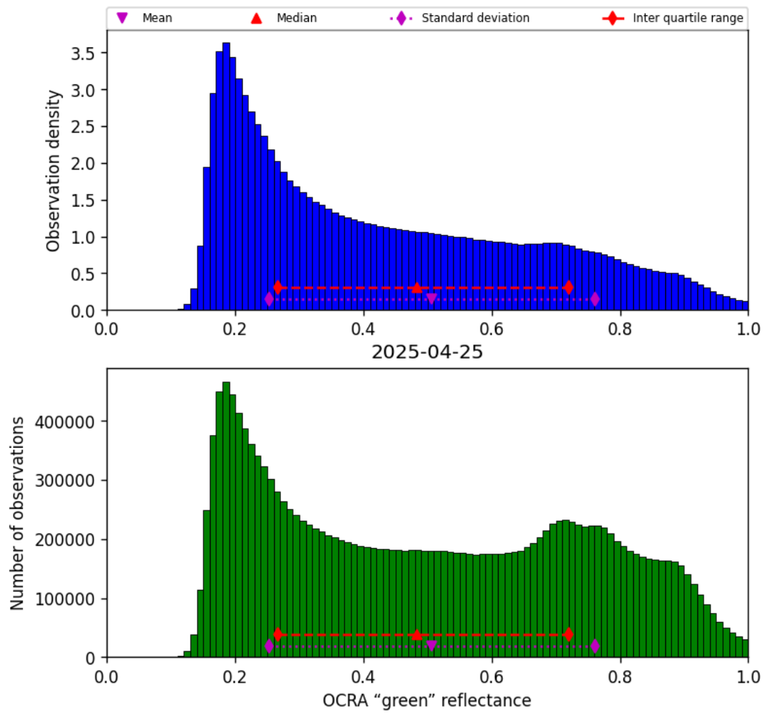
Figure 50: Histogram of “OCRA “green” reflectance” for 2025-04-25 to 2025-04-26
