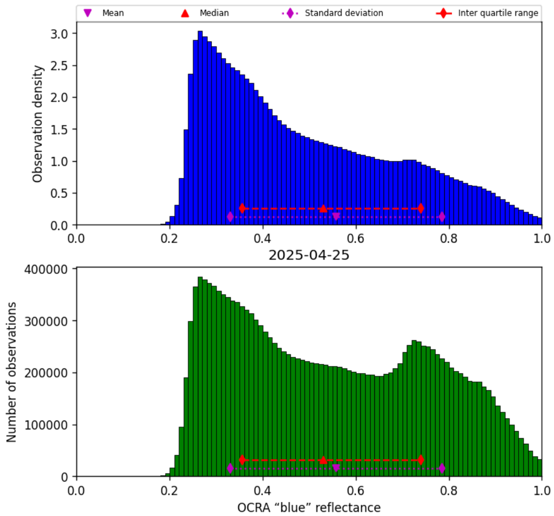
Figure 49: Histogram of “OCRA “blue” reflectance” for 2025-04-25 to 2025-04-26
