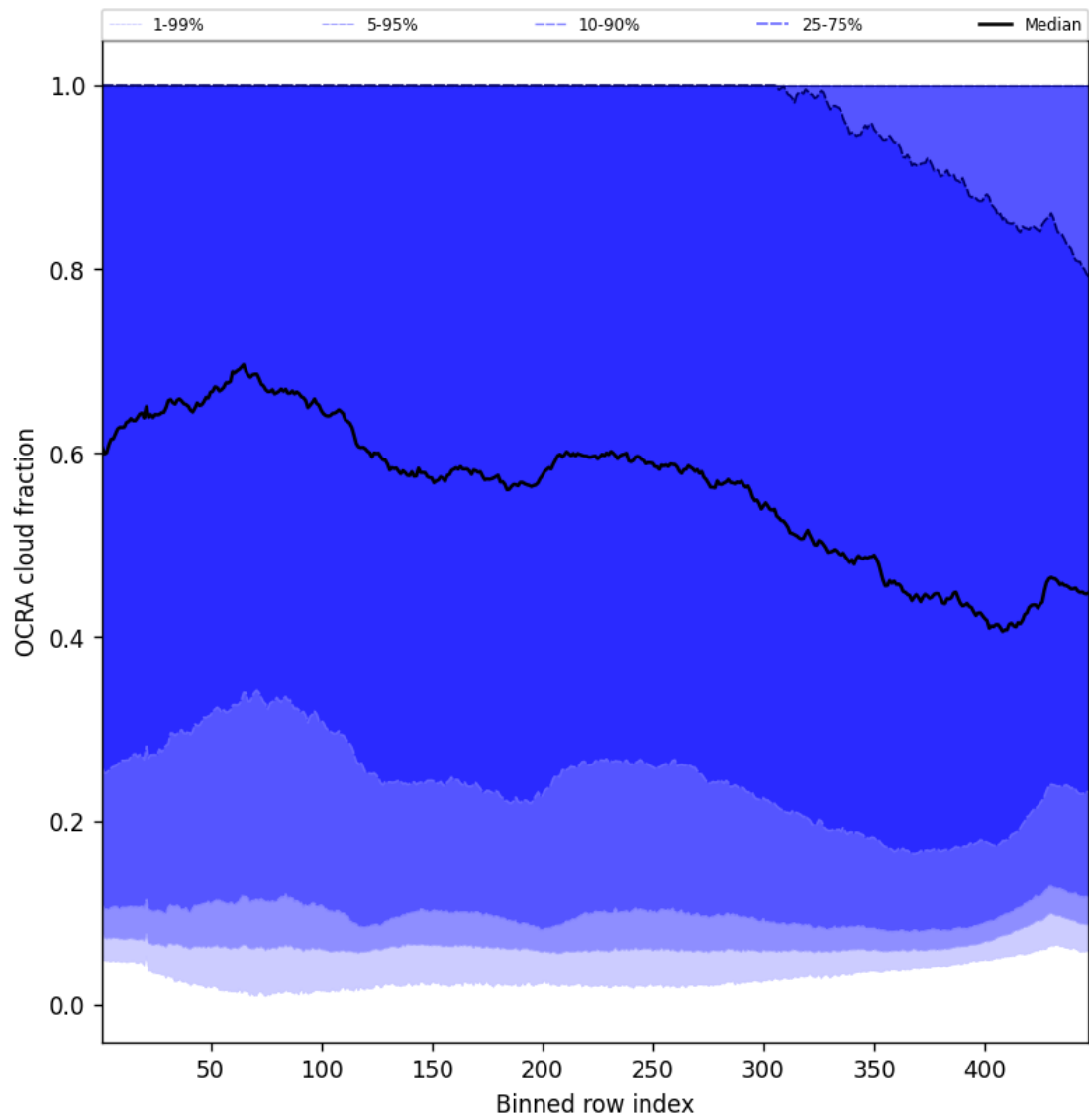
Figure 64: Along track statistics of “OCRA cloud fraction” for 2025-04-25 to 2025-04-26
