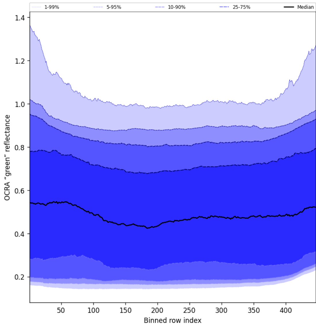
Figure 66: Along track statistics of "OCRA "green" reflectance" for 2025-04-25 to 2025-04-26
