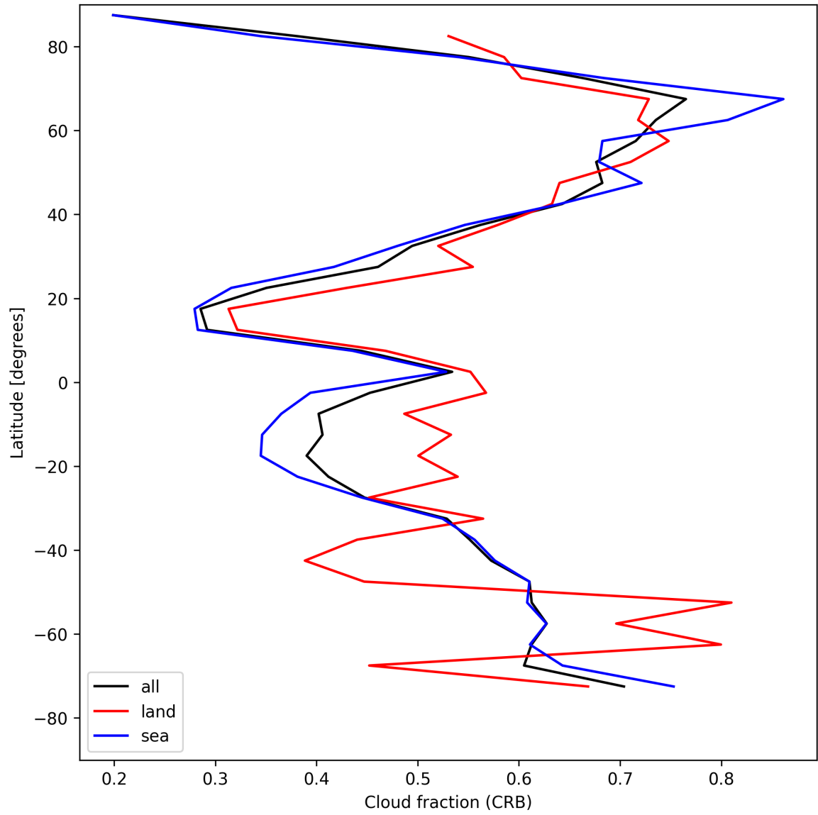
Figure 24: Zonal average of “Cloud fraction (CRB)” for 2025-04-27 to 2025-04-27.
