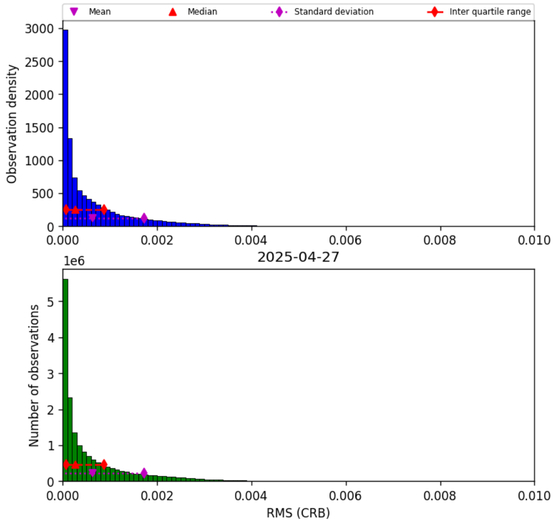
Figure 46: Histogram of “RMS (CRB)” for 2025-04-27 to 2025-04-27
