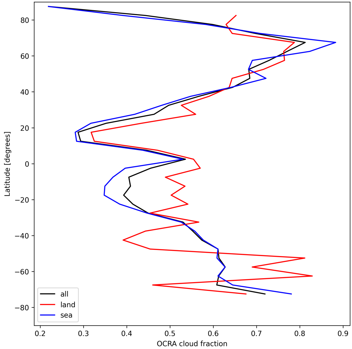
Figure 32: Zonal average of “OCRA cloud fraction” for 2025-04-27 to 2025-04-27.
