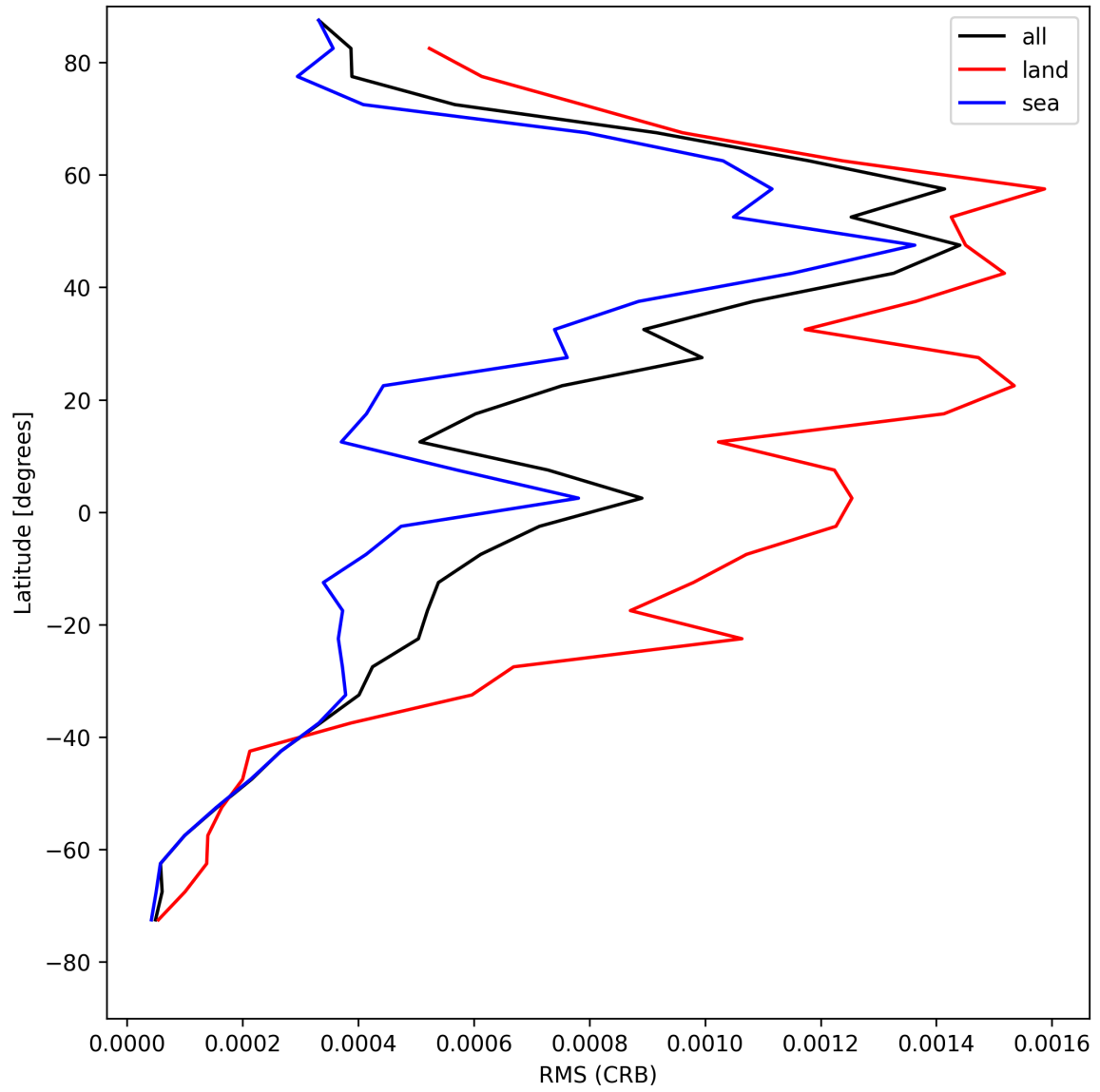
Figure 30: Zonal average of “RMS (CRB)” for 2025-04-27 to 2025-04-27.
