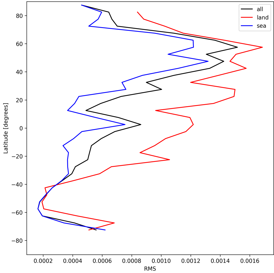
Figure 29: Zonal average of “RMS” for 2025-04-27 to 2025-04-27.
