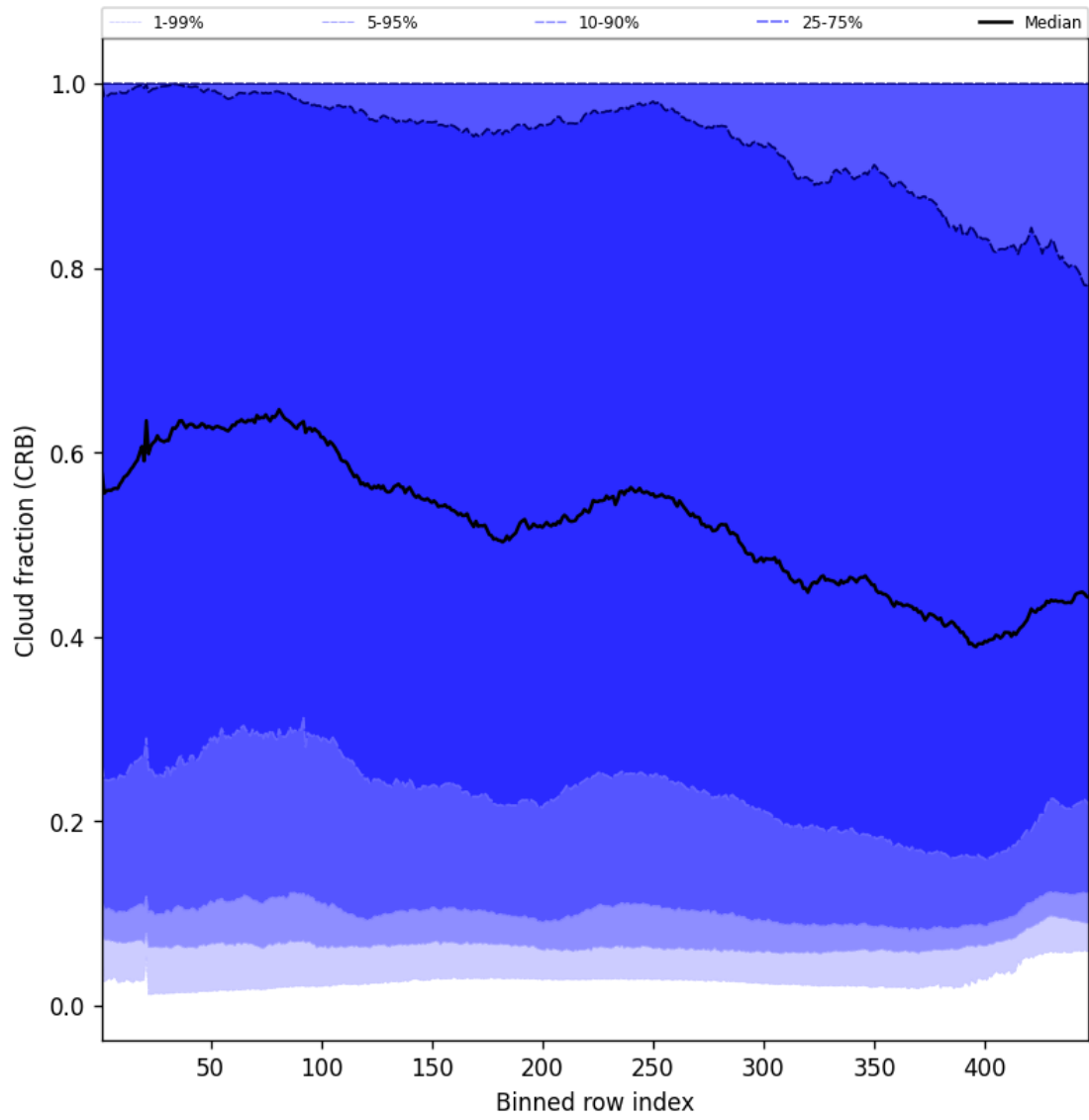
Figure 56: Along track statistics of “Cloud fraction (CRB)” for 2025-04-27 to 2025-04-27
