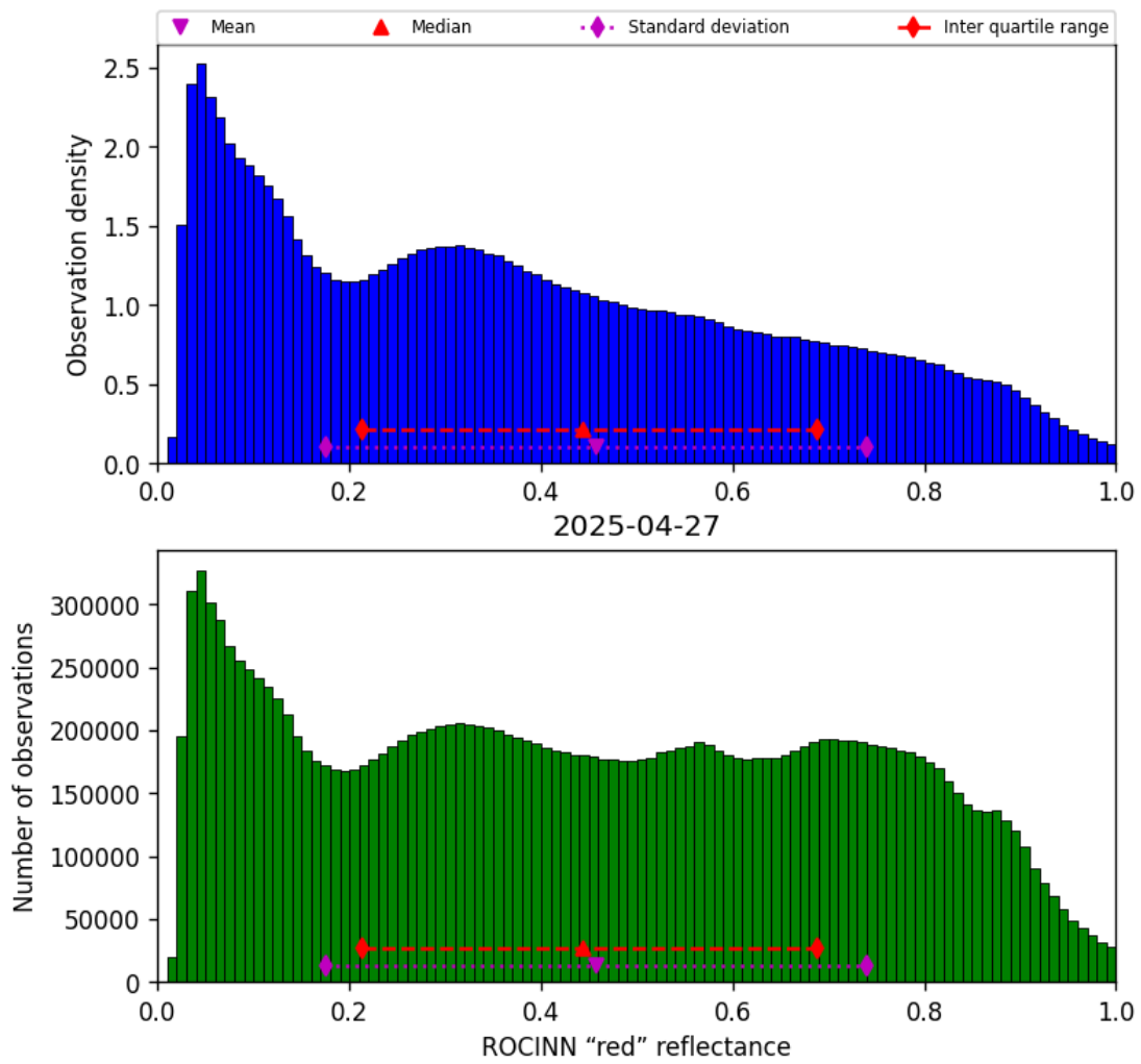
Figure 51: Histogram of “ROCINN “red” reflectance” for 2025-04-27 to 2025-04-27
