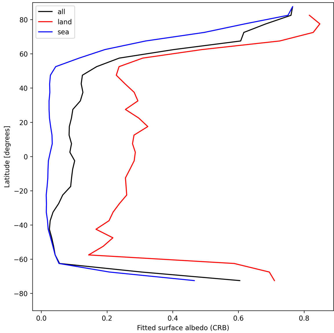
Figure 28: Zonal average of “Fitted surface albedo (CRB)” for 2025-04-27 to 2025-04-27.
