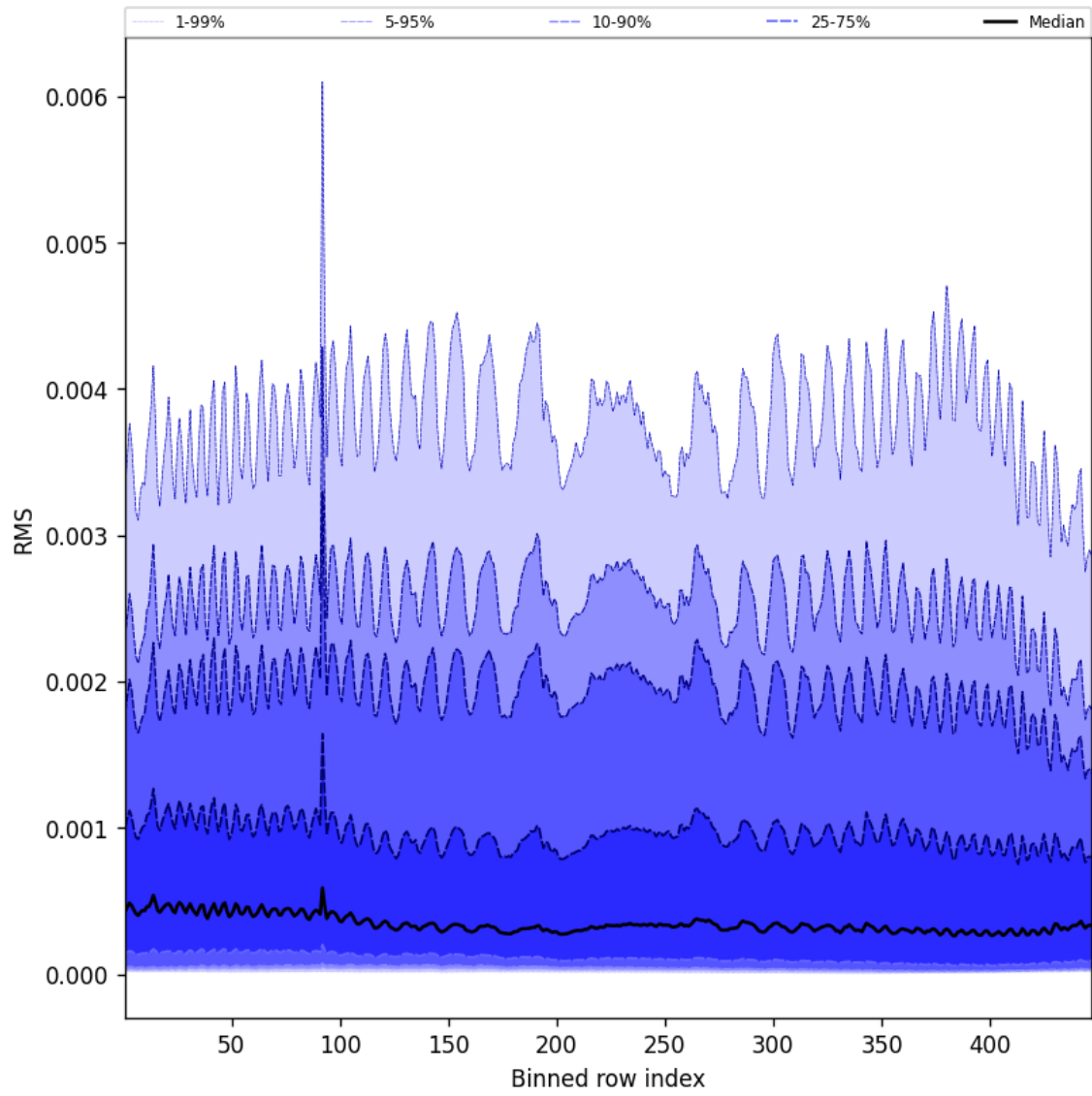
Figure 61: Along track statistics of “RMS” for 2025-04-27 to 2025-04-27
