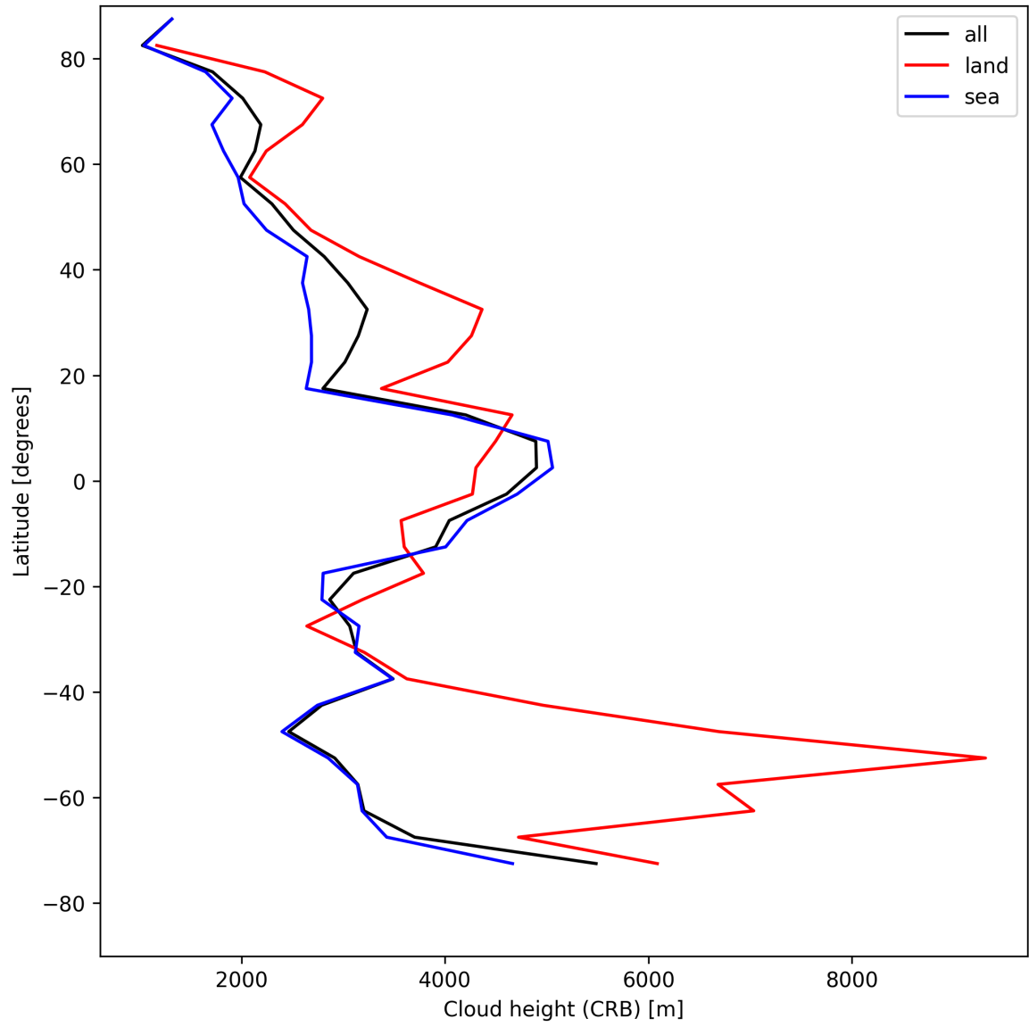
Figure 25: Zonal average of “Cloud height (CRB)” for 2025-04-27 to 2025-04-27.
