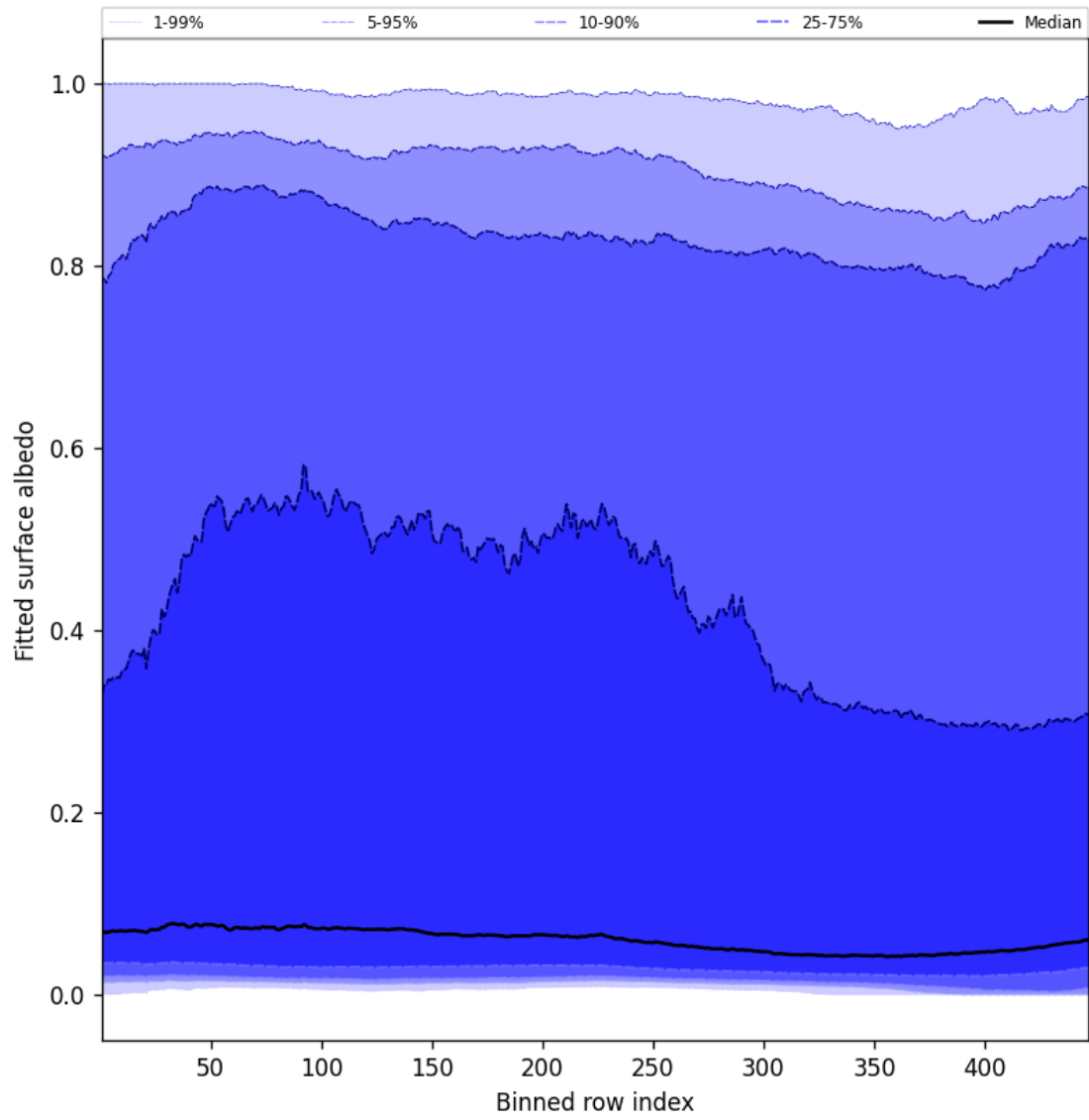
Figure 59: Along track statistics of “Fitted surface albedo” for 2025-04-27 to 2025-04-27
