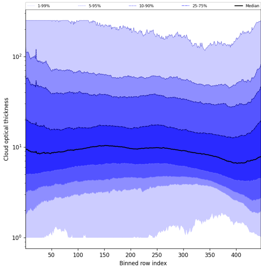
Figure 55: Along track statistics of “Cloud optical thickness” for 2025-04-27 to 2025-04-27
