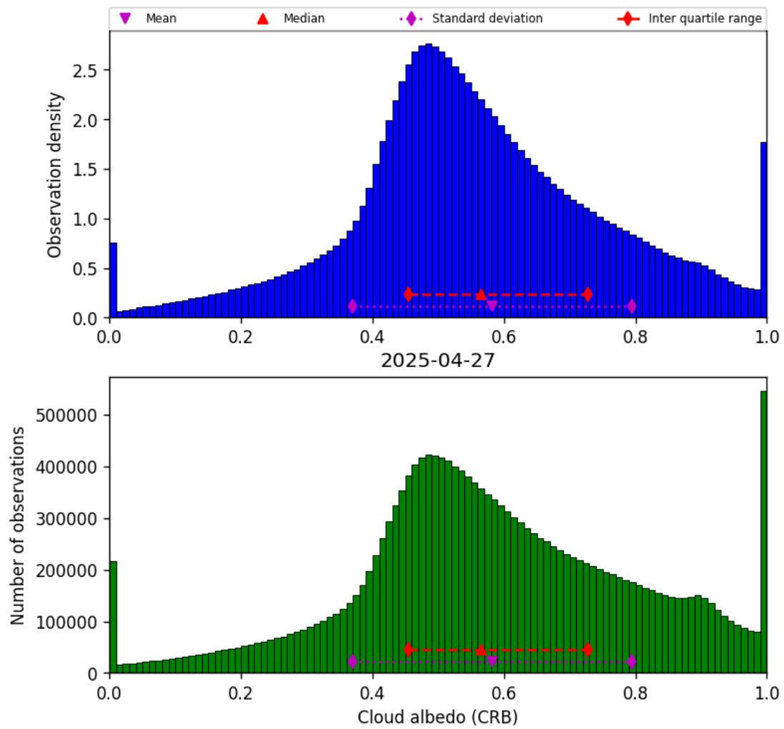
Figure 42: Histogram of “Cloud albedo (CRB)” for 2025-04-27 to 2025-04-27
