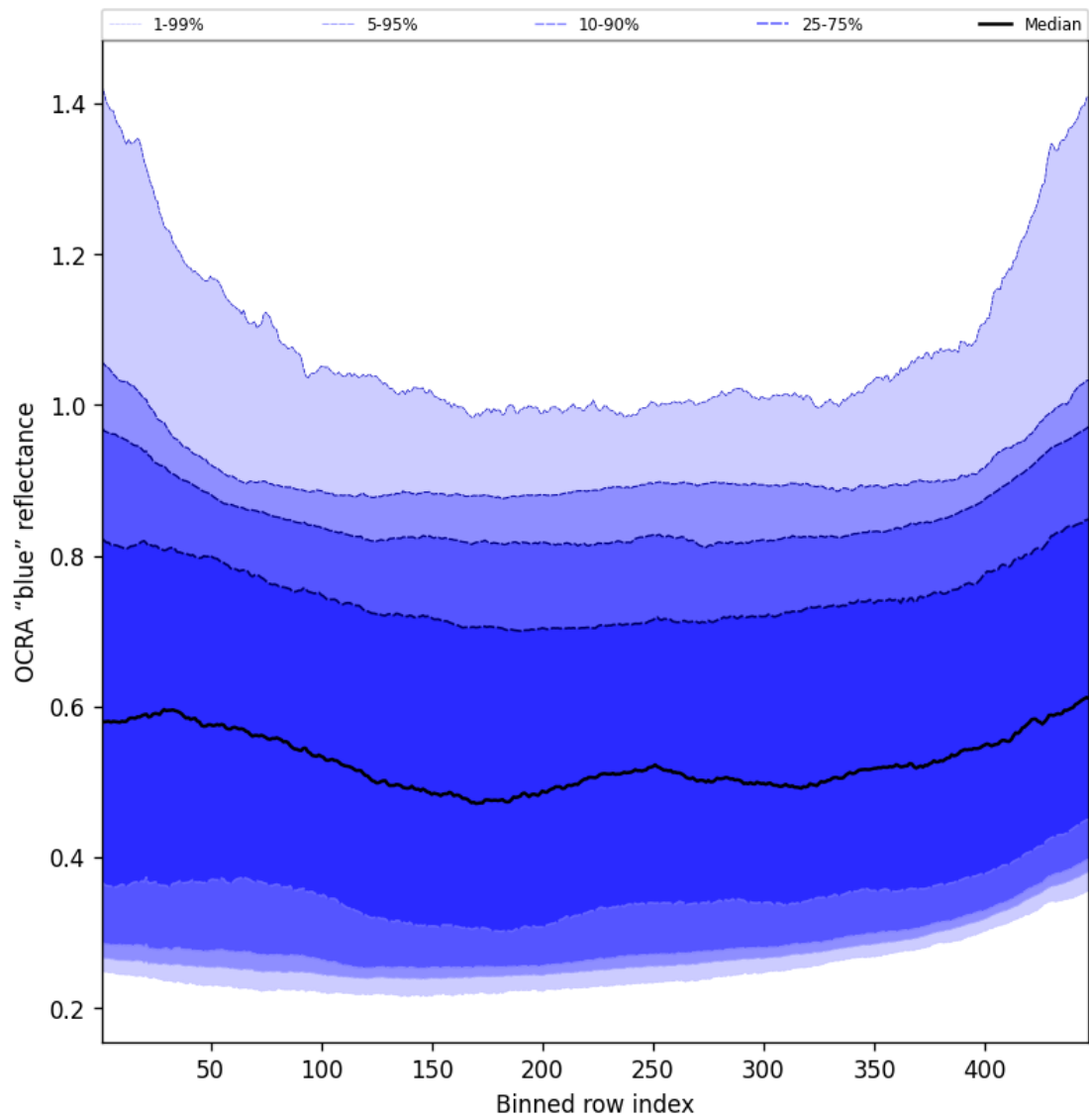
Figure 65: Along track statistics of “OCRA “blue” reflectance” for 2025-04-27 to 2025-04-27
