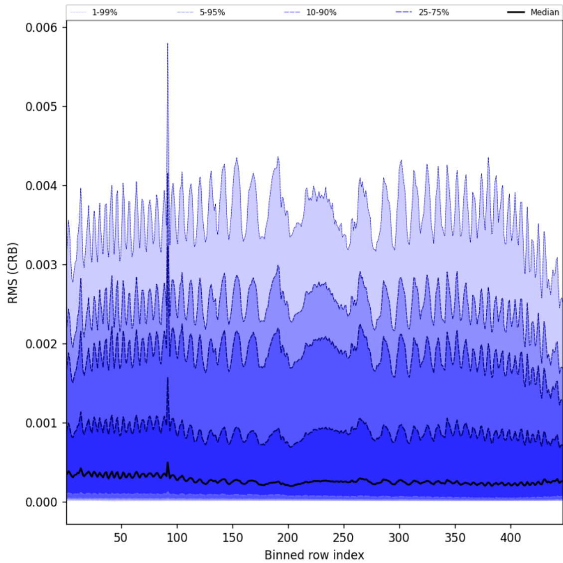
Figure 62: Along track statistics of “RMS (CRB)” for 2025-04-27 to 2025-04-27
