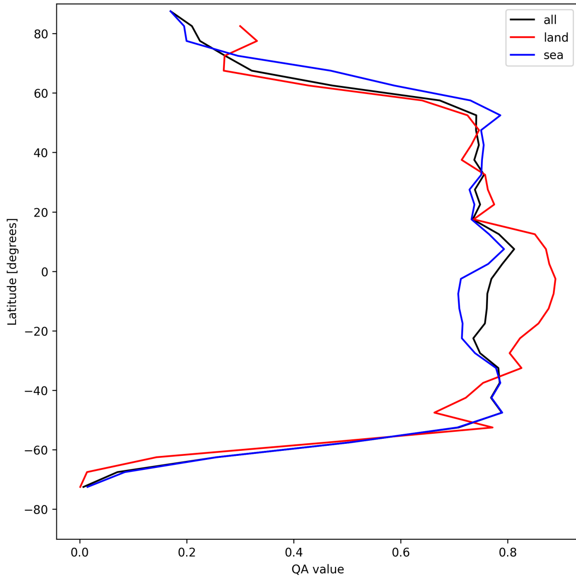
Figure 20: Zonal average of “QA value” for 2025-04-27 to 2025-04-27.
