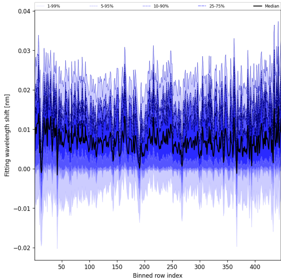
Figure 63: Along track statistics of “Fitting wavelength shift” for 2025-04-27 to 2025-04-27
