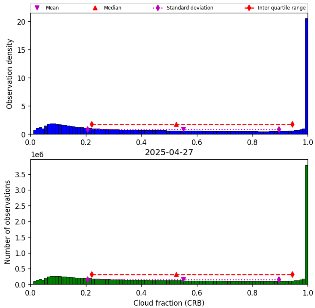
Figure 40: Histogram of “Cloud fraction (CRB)” for 2025-04-27 to 2025-04-27
