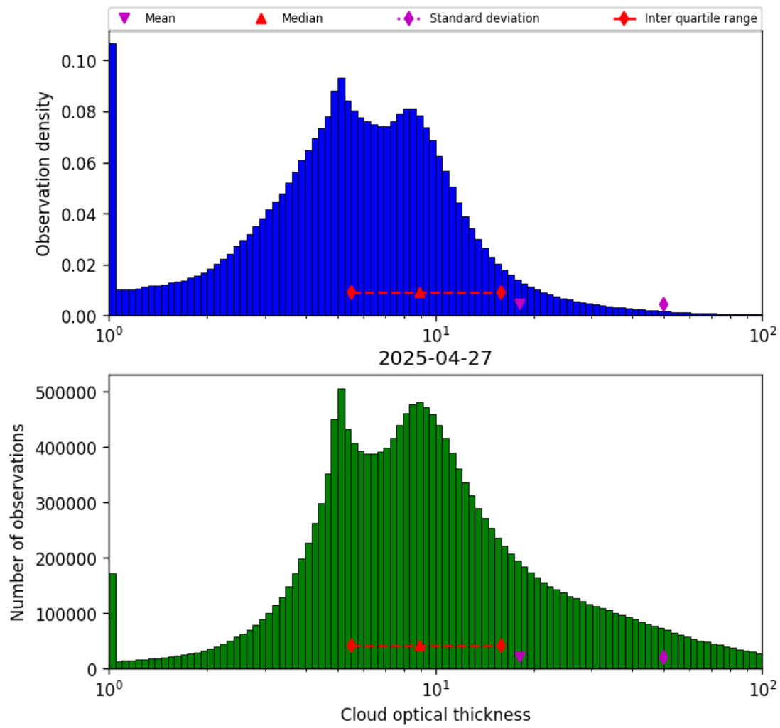
Figure 39: Histogram of “Cloud optical thickness” for 2025-04-27 to 2025-04-27
