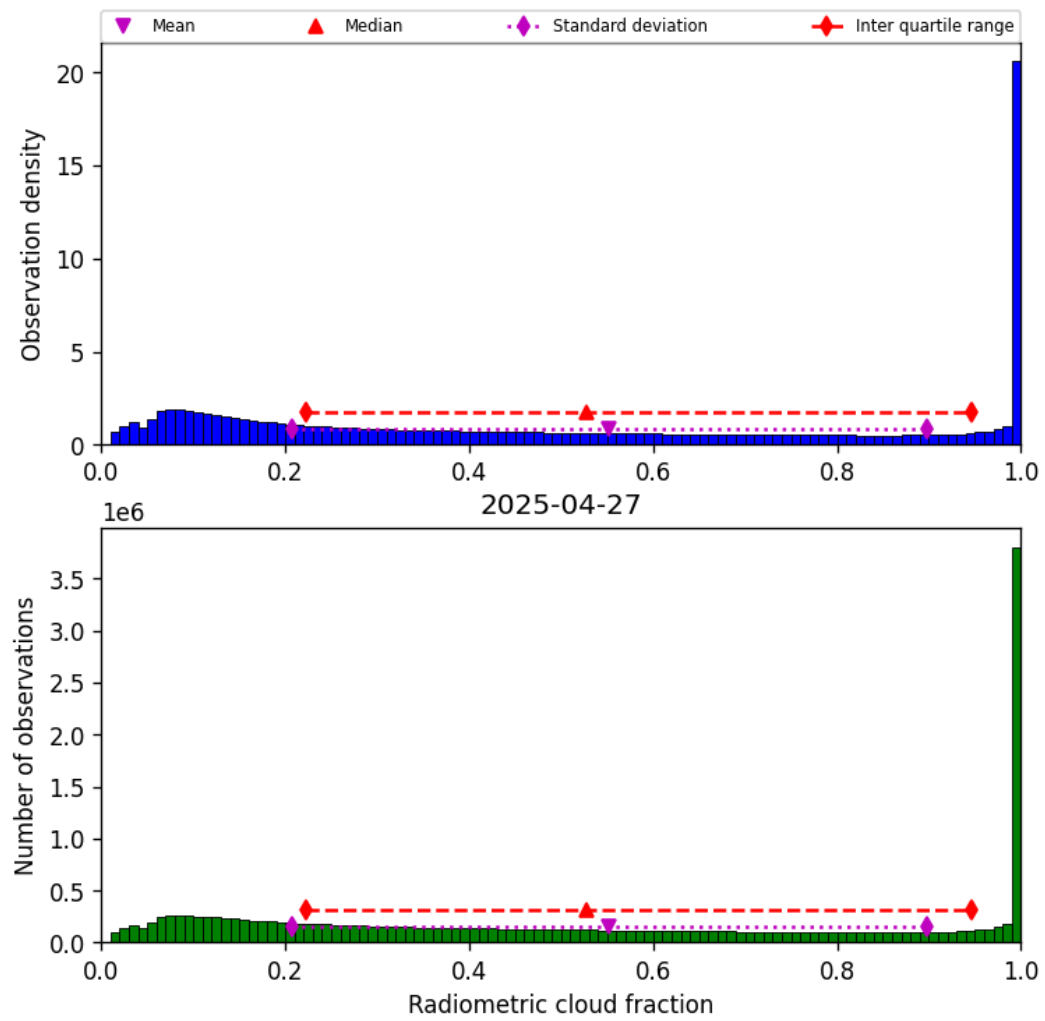
Figure 37: Histogram of “Radiometric cloud fraction” for 2025-04-27 to 2025-04-27
