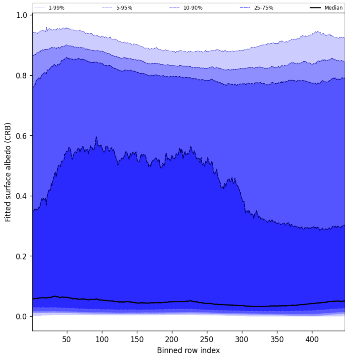
Figure 60: Along track statistics of “Fitted surface albedo (CRB)” for 2025-04-27 to 2025-04-27
