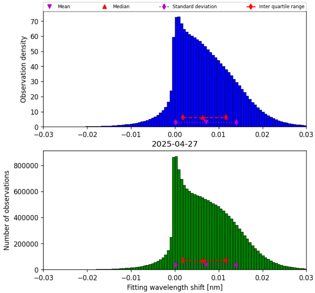
Figure 47: Histogram of “Fitting wavelength shift” for 2025-04-27 to 2025-04-27
