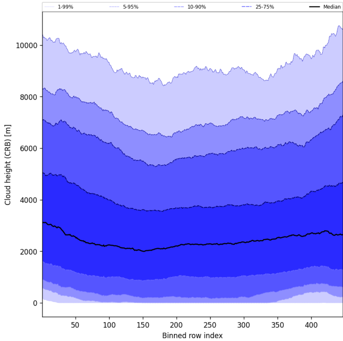
Figure 57: Along track statistics of “Cloud height (CRB)” for 2025-04-27 to 2025-04-27
