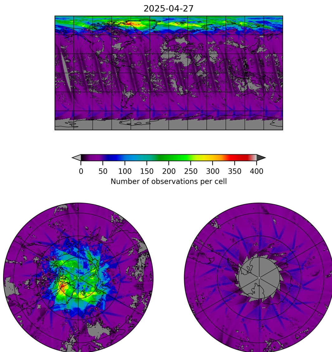
Figure 19: Map of the number of observations for 2025-04-27 to 2025-04-27
