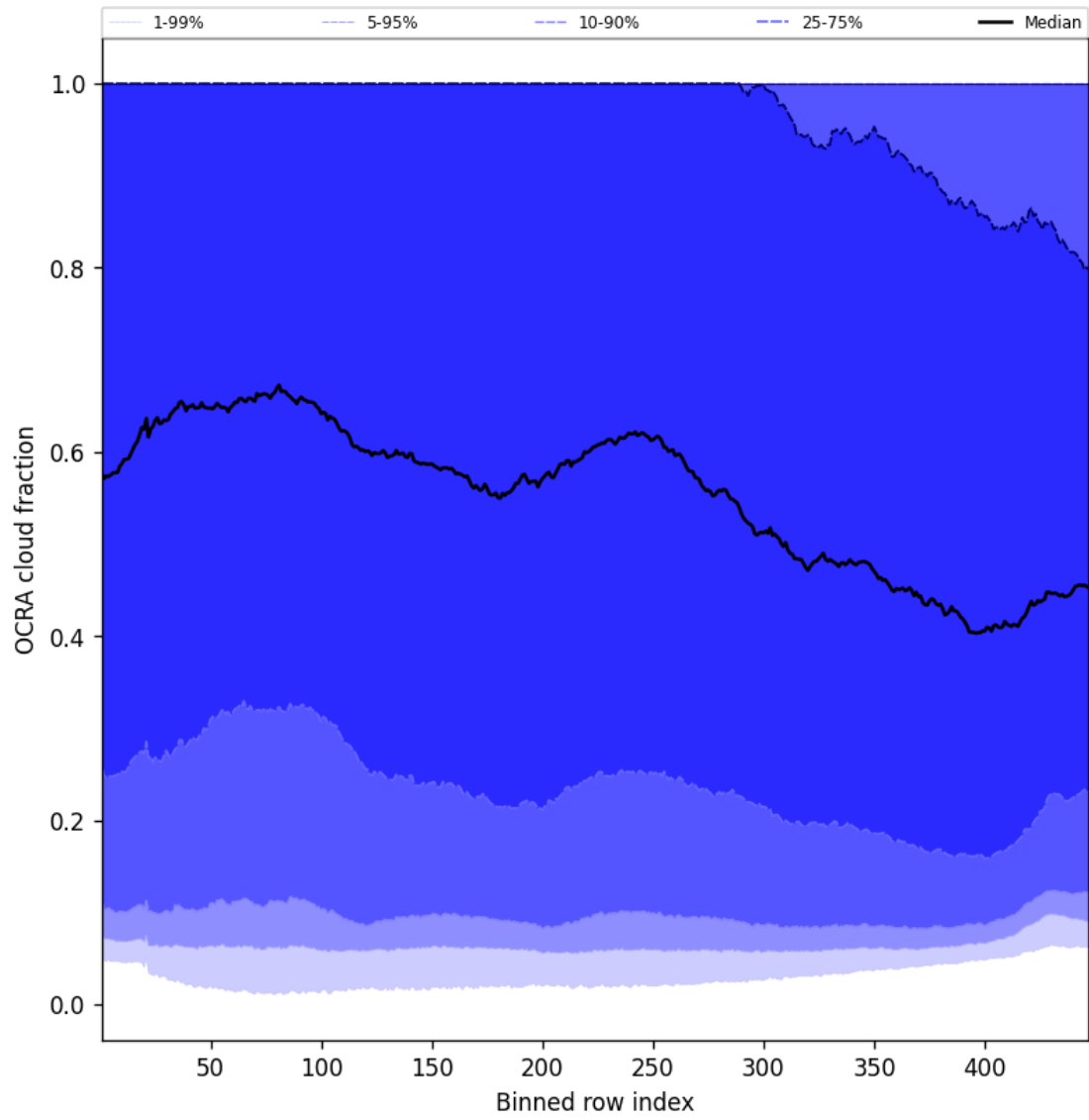
Figure 64: Along track statistics of “OCRA cloud fraction” for 2025-04-27 to 2025-04-27
