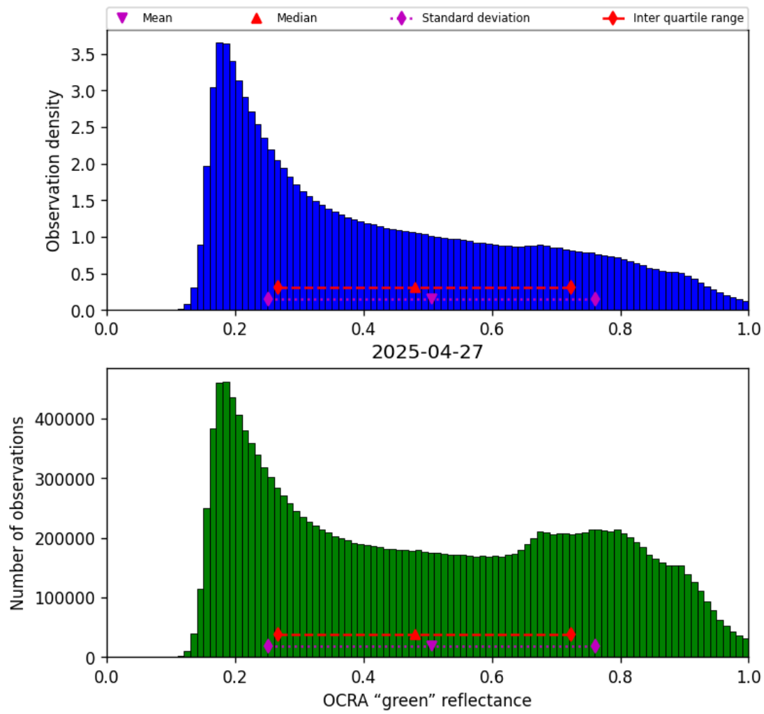
Figure 50: Histogram of “OCRA “green” reflectance” for 2025-04-27 to 2025-04-27
