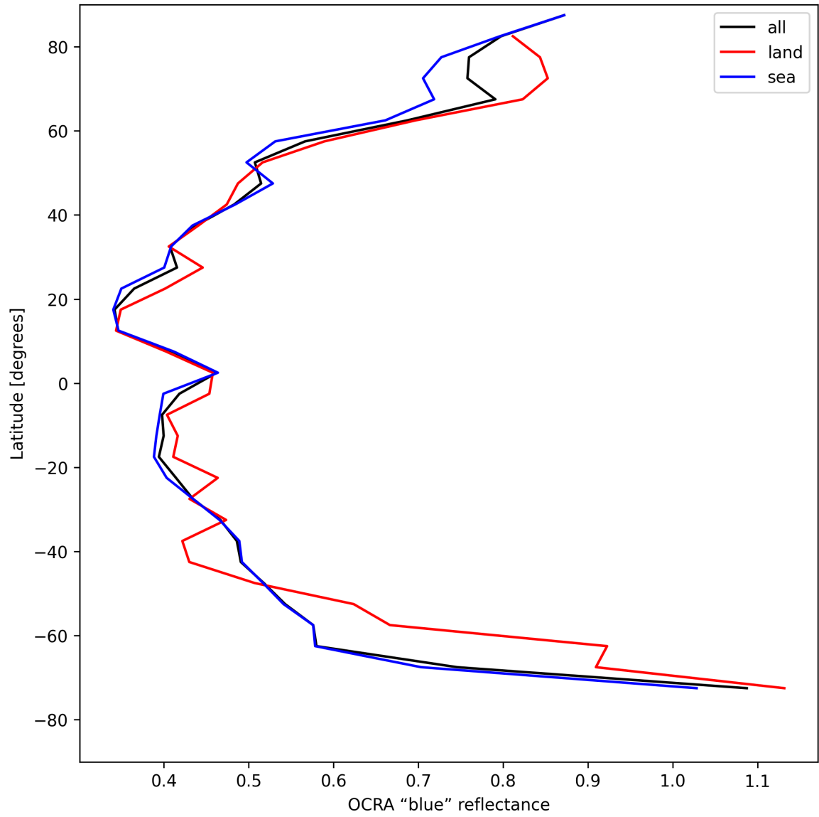
Figure 33: Zonal average of “OCRA “blue” reflectance” for 2025-04-27 to 2025-04-27.
