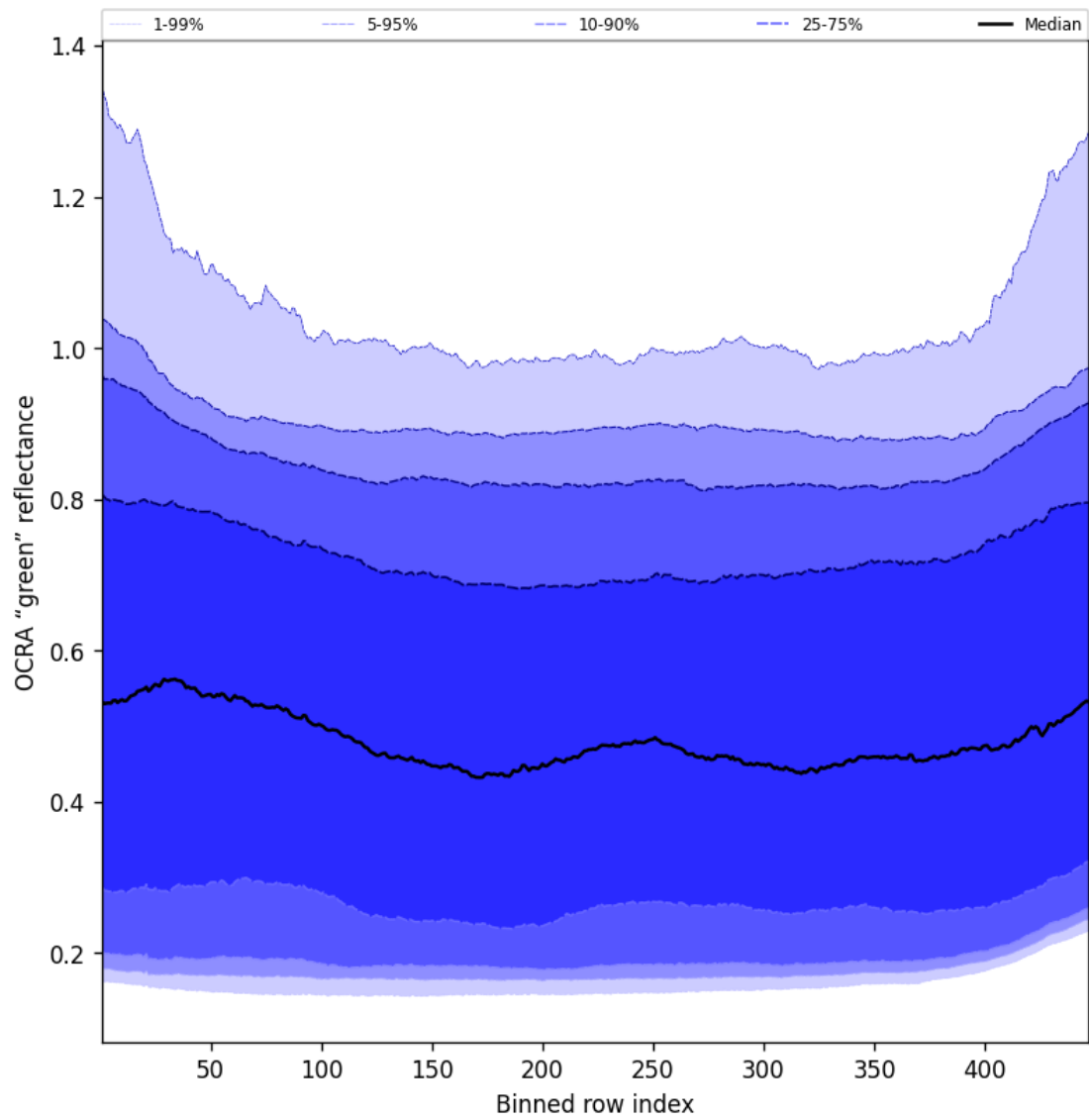
Figure 66: Along track statistics of “OCRA “green” reflectance” for 2025-04-27 to 2025-04-27
