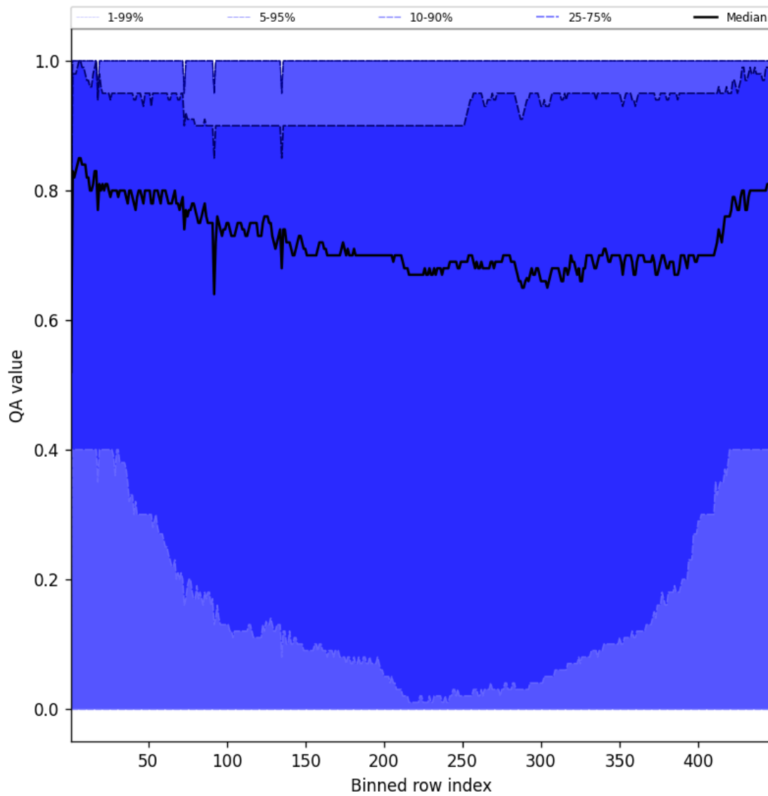
Figure 52: Along track statistics of “QA value” for 2025-04-27 to 2025-04-27
