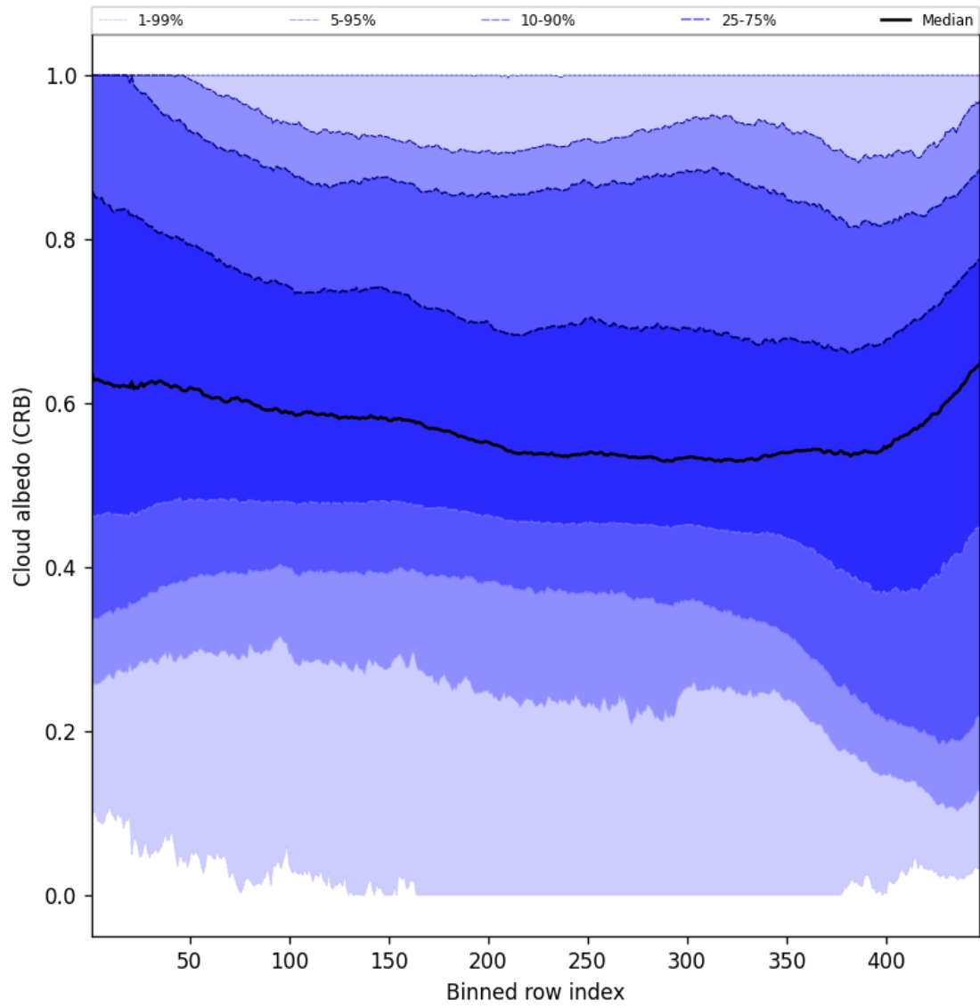
Figure 58: Along track statistics of “Cloud albedo (CRB)” for 2025-04-27 to 2025-04-27
