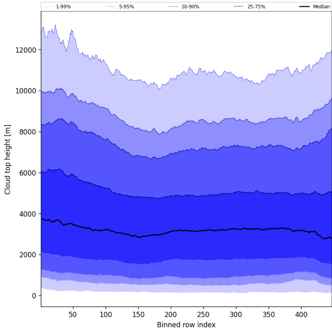
Figure 54: Along track statistics of “Cloud top height” for 2025-04-27 to 2025-04-27
