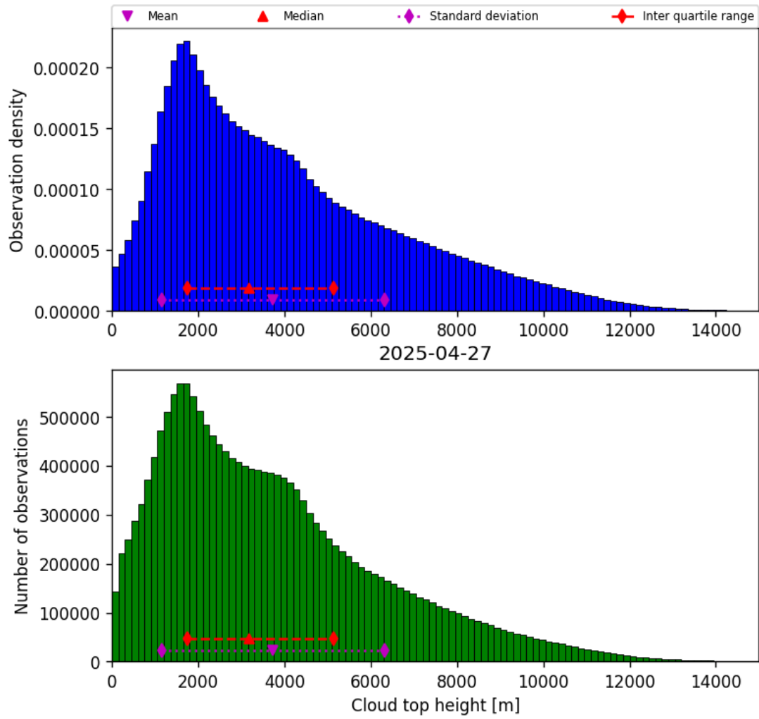
Figure 38: Histogram of “Cloud top height” for 2025-04-27 to 2025-04-27
