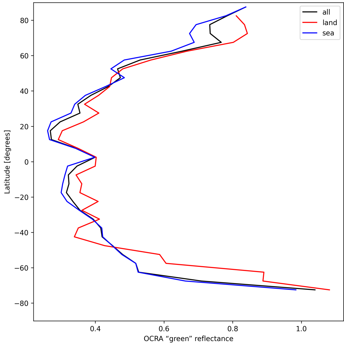
Figure 34: Zonal average of “OCRA “green” reflectance” for 2025-04-27 to 2025-04-27.
