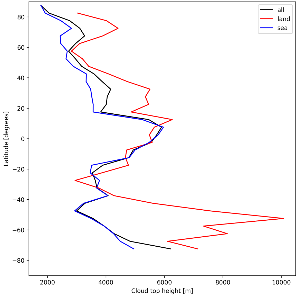
Figure 22: Zonal average of “Cloud top height” for 2025-04-27 to 2025-04-27.
