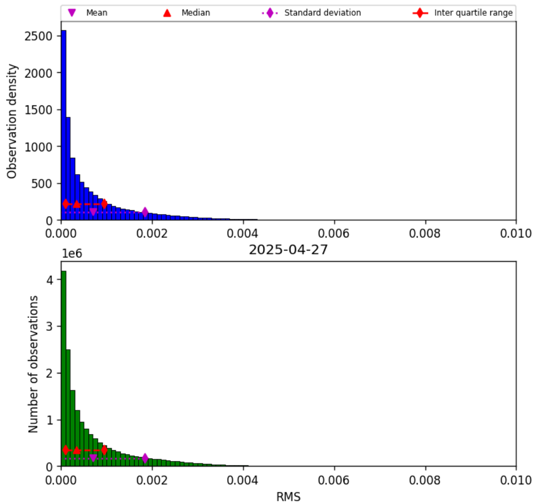
Figure 45: Histogram of “RMS” for 2025-04-27 to 2025-04-27
