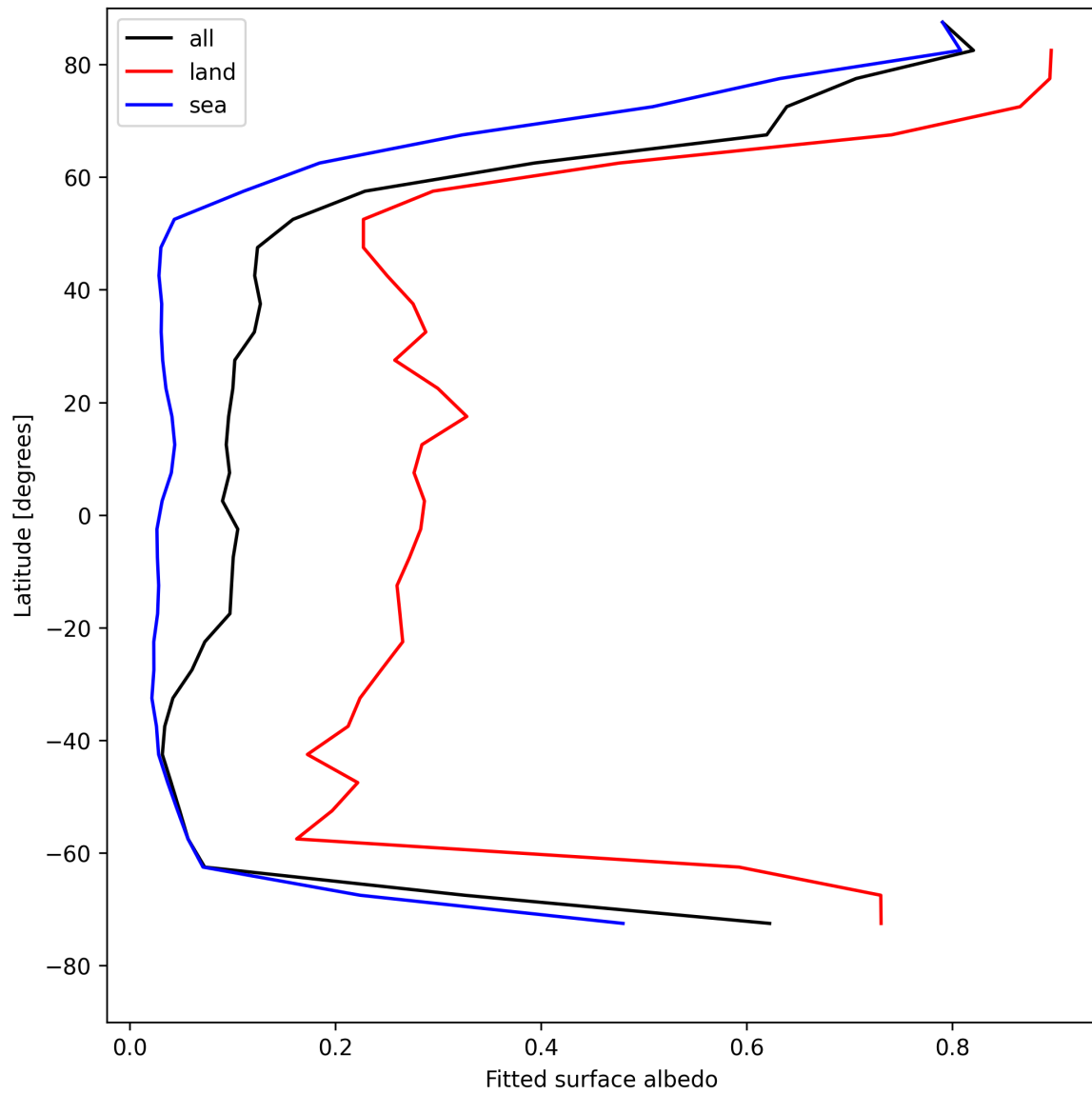
Figure 27: Zonal average of “Fitted surface albedo” for 2025-04-27 to 2025-04-27.
