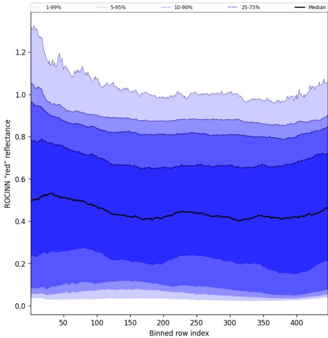
Figure 67: Along track statistics of "ROCINN "red" reflectance" for 2025-04-27 to 2025-04-27
