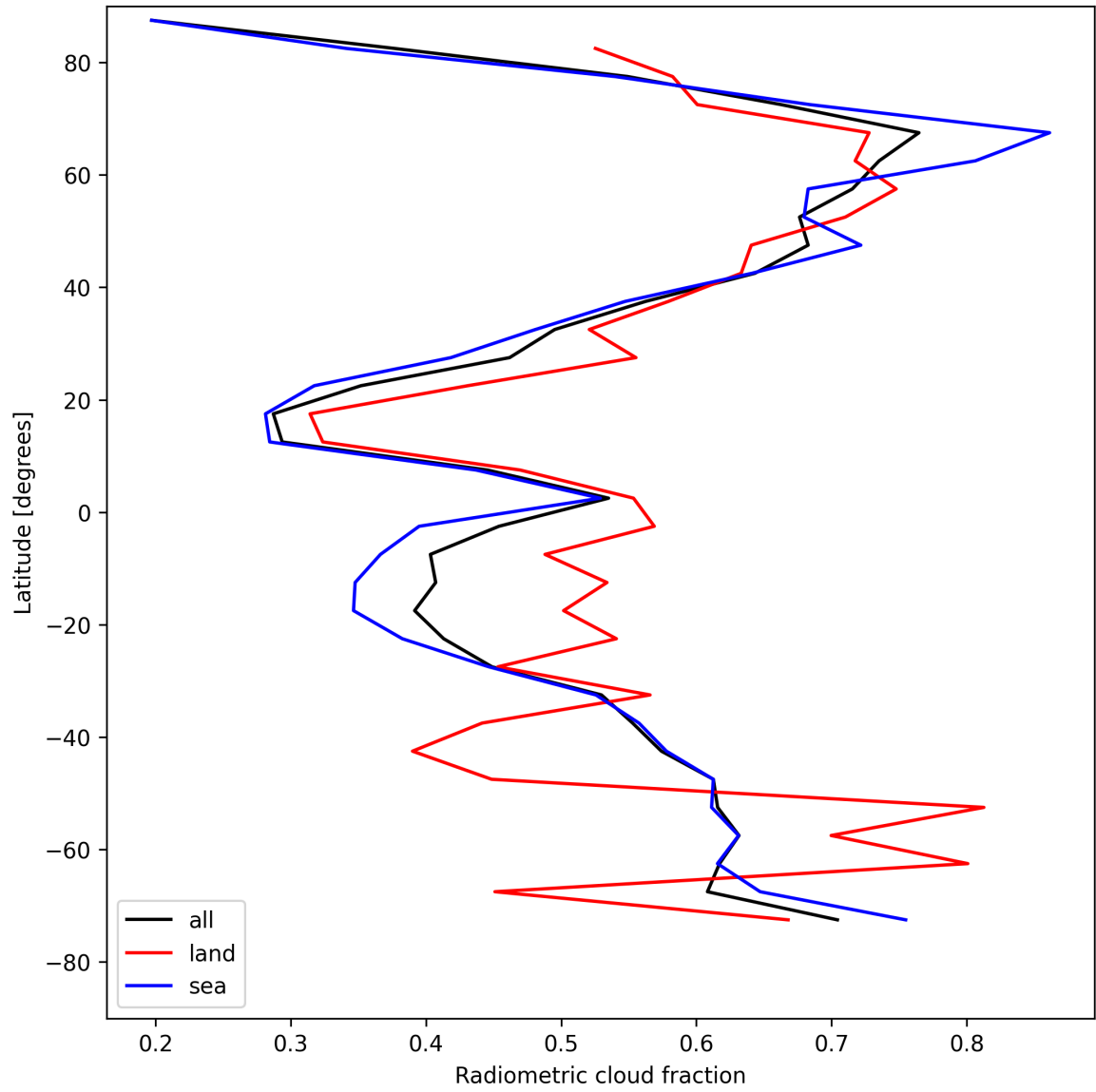
Figure 21: Zonal average of “Radiometric cloud fraction” for 2025-04-27 to 2025-04-27.
