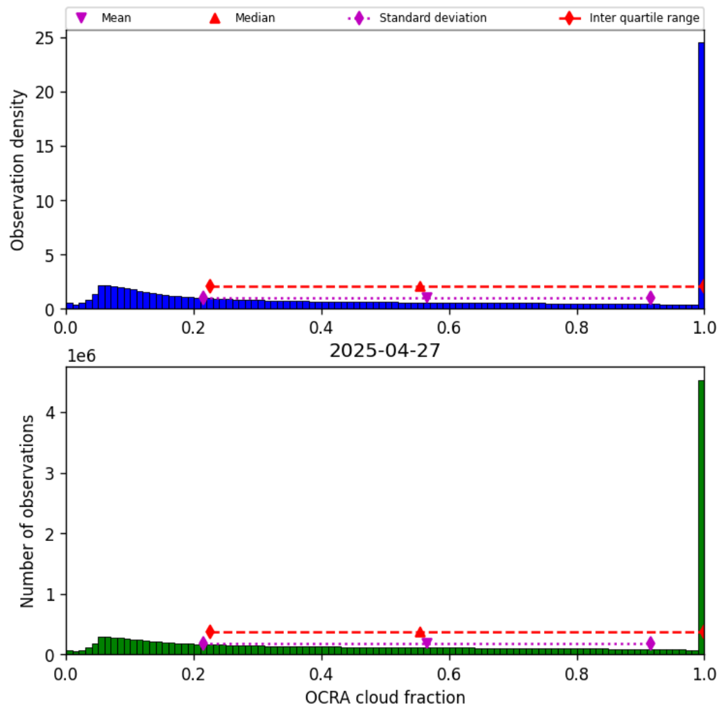
Figure 48: Histogram of “OCRA cloud fraction” for 2025-04-27 to 2025-04-27
