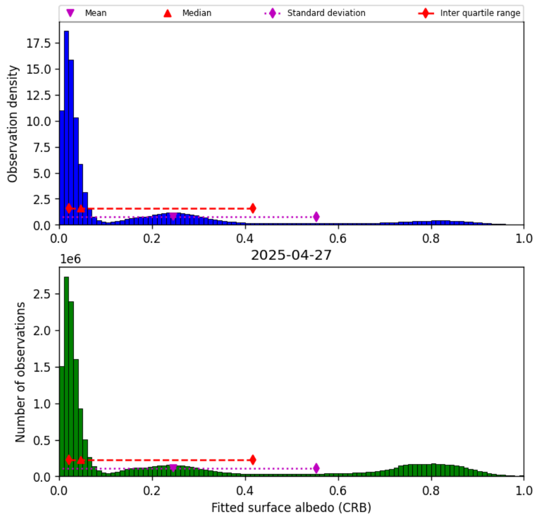
Figure 44: Histogram of “Fitted surface albedo (CRB)” for 2025-04-27 to 2025-04-27
