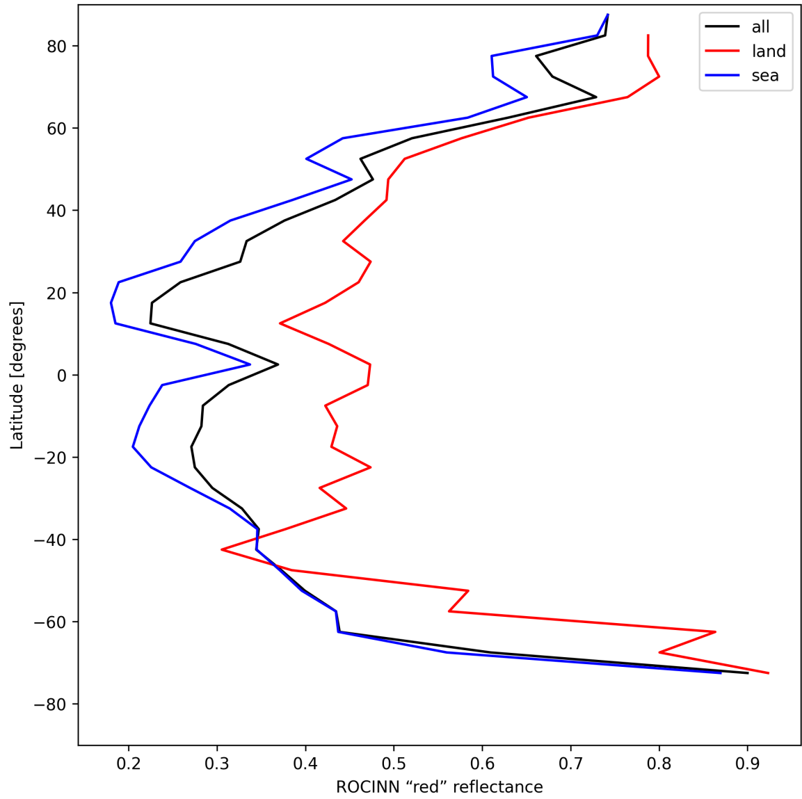
Figure 35: Zonal average of “ROCINN “red” reflectance” for 2025-04-27 to 2025-04-27.
