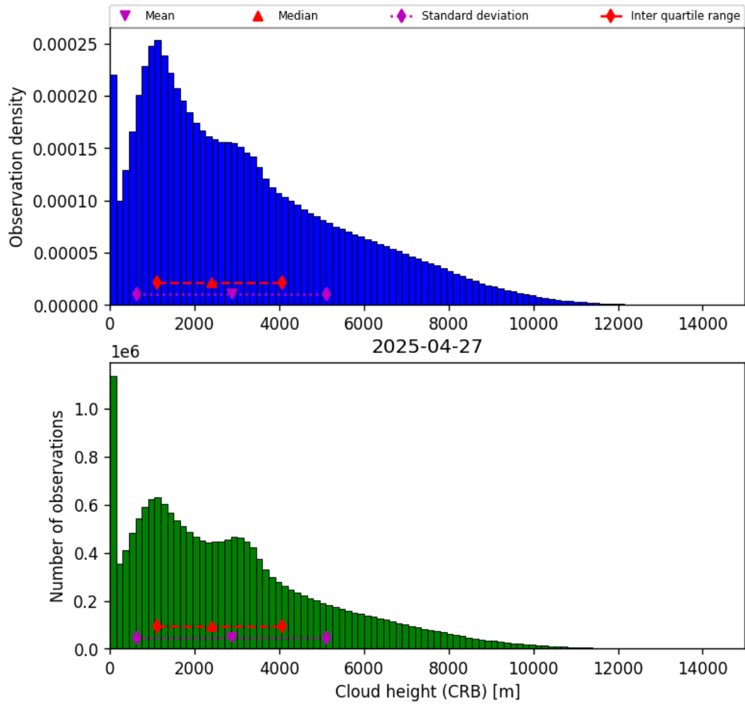
Figure 41: Histogram of “Cloud height (CRB)” for 2025-04-27 to 2025-04-27
