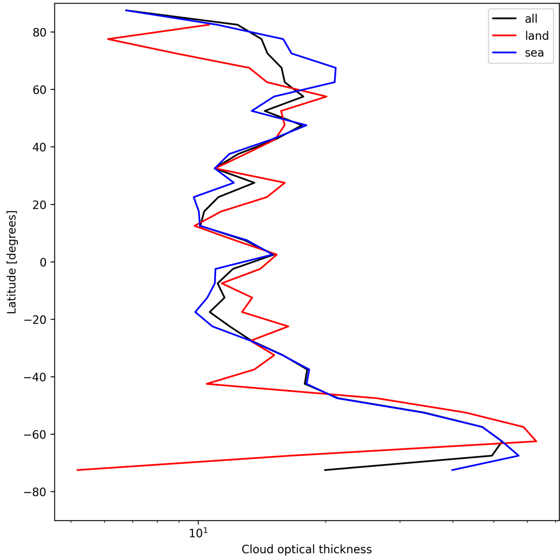
Figure 23: Zonal average of “Cloud optical thickness” for 2025-04-27 to 2025-04-27.
