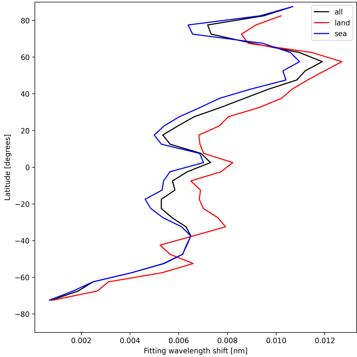
Figure 31: Zonal average of “Fitting wavelength shift” for 2025-04-27 to 2025-04-27.
