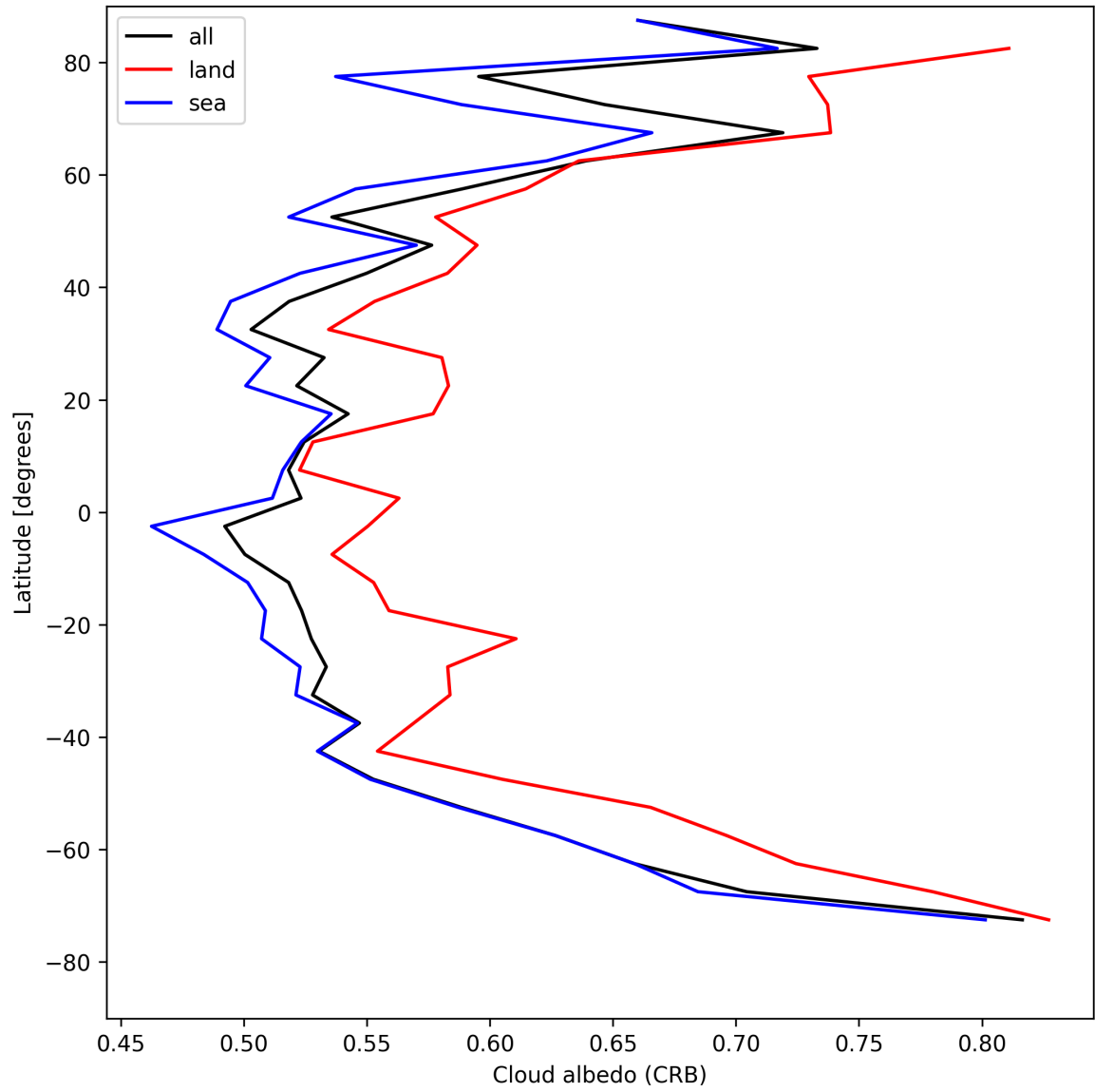
Figure 26: Zonal average of “Cloud albedo (CRB)” for 2025-04-27 to 2025-04-27.
