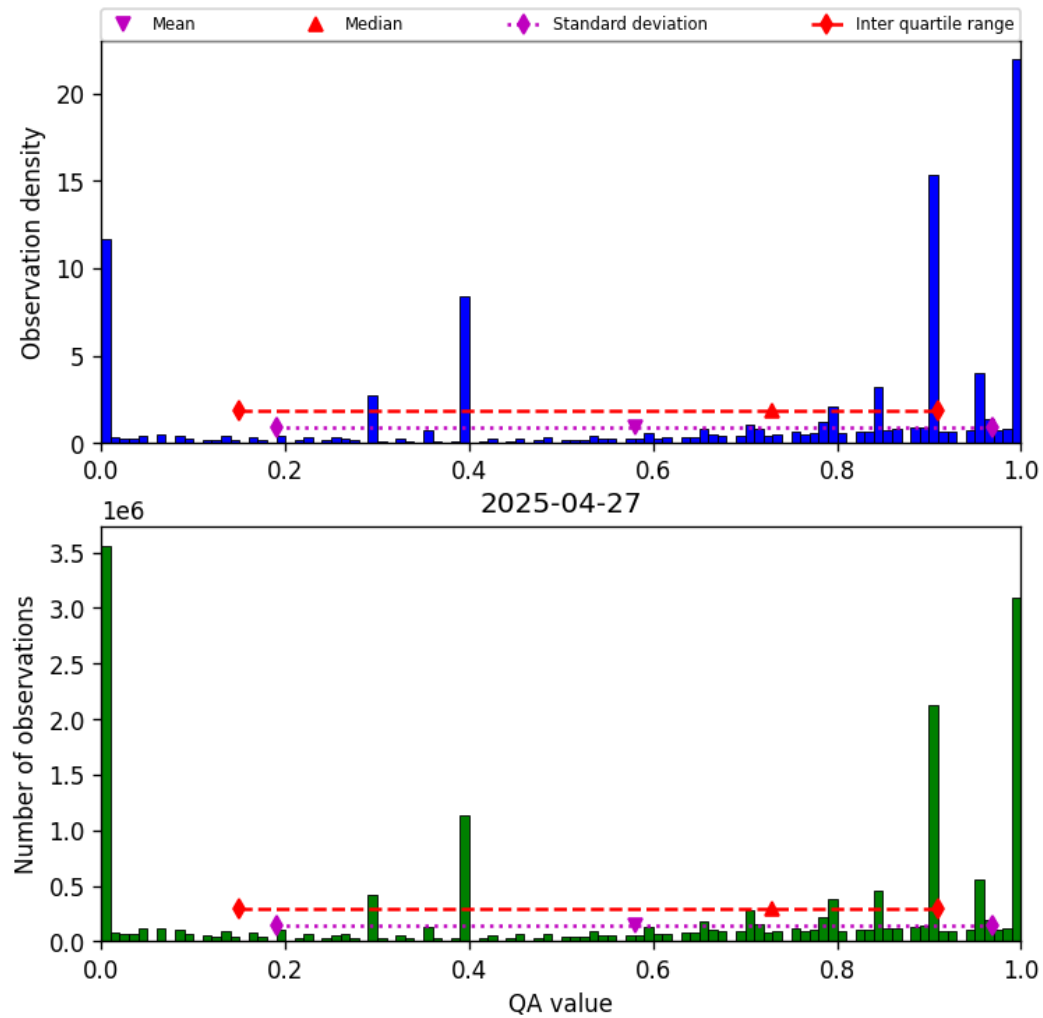
Figure 36: Histogram of “QA value” for 2025-04-27 to 2025-04-27
