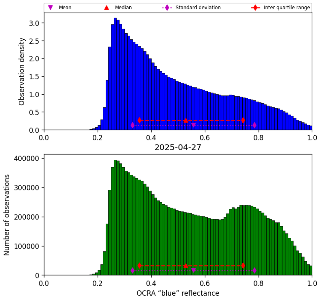
Figure 49: Histogram of “OCRA “blue” reflectance” for 2025-04-27 to 2025-04-27
