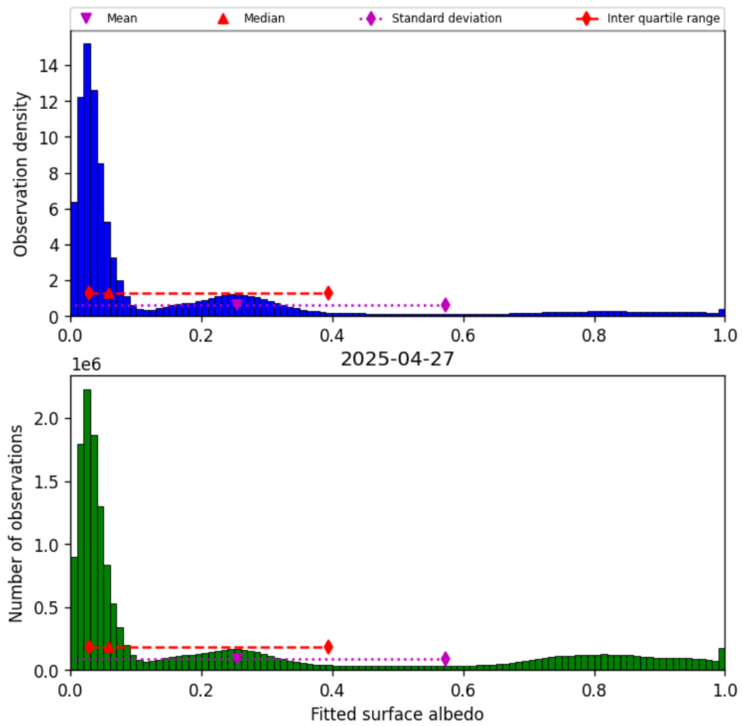
Figure 43: Histogram of “Fitted surface albedo” for 2025-04-27 to 2025-04-27
