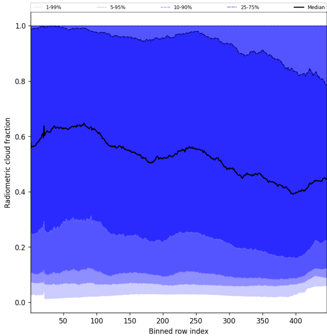
Figure 53: Along track statistics of “Radiometric cloud fraction” for 2025-04-27 to 2025-04-27
