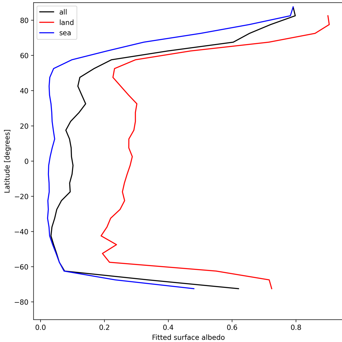
Figure 27: Zonal average of “Fitted surface albedo” for 2025-04-29 to 2025-04-30.
