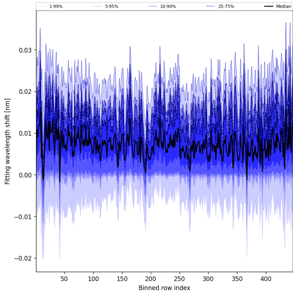
Figure 63: Along track statistics of “Fitting wavelength shift” for 2025-04-29 to 2025-04-30
