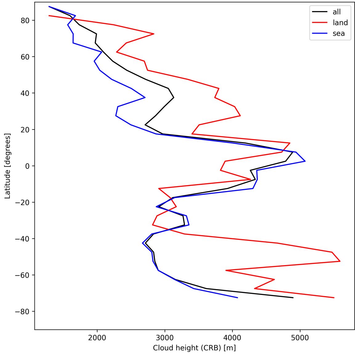
Figure 25: Zonal average of “Cloud height (CRB)” for 2025-04-29 to 2025-04-30.
