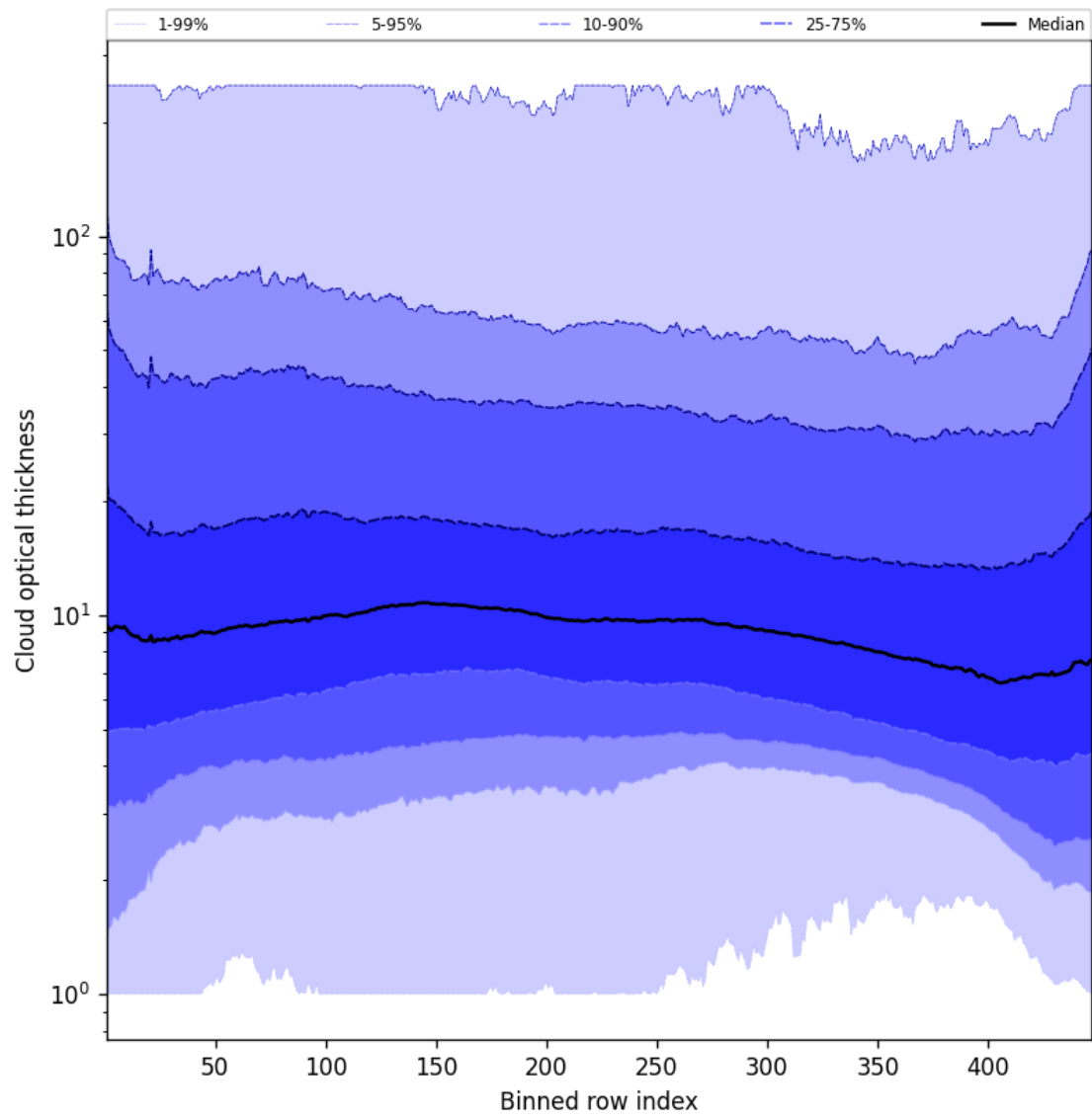
Figure 55: Along track statistics of “Cloud optical thickness” for 2025-04-29 to 2025-04-30
