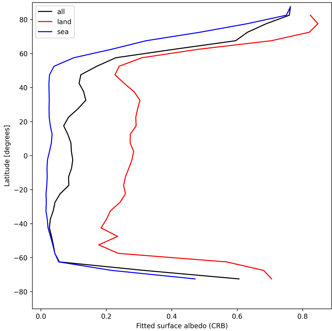
Figure 28: Zonal average of “Fitted surface albedo (CRB)” for 2025-04-29 to 2025-04-30.
