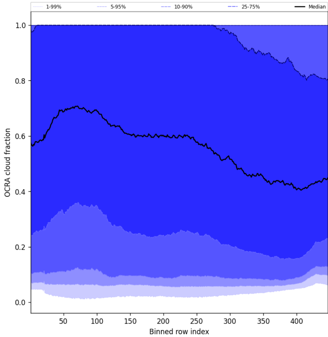
Figure 64: Along track statistics of “OCRA cloud fraction” for 2025-04-29 to 2025-04-30
