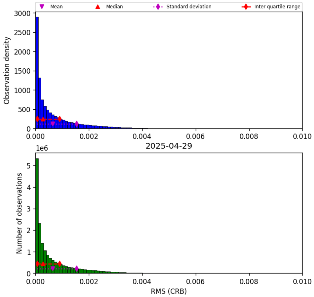
Figure 46: Histogram of “RMS (CRB)” for 2025-04-29 to 2025-04-30
