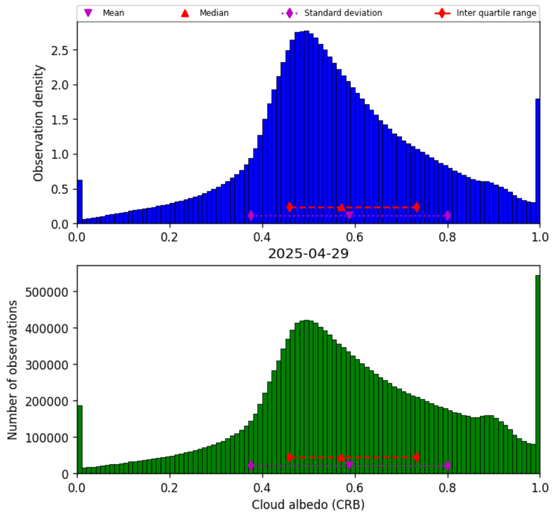
Figure 42: Histogram of “Cloud albedo (CRB)” for 2025-04-29 to 2025-04-30
