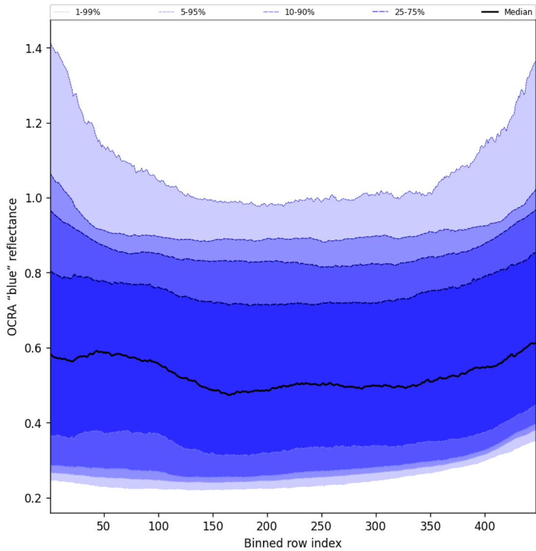
Figure 65: Along track statistics of “OCRA “blue” reflectance” for 2025-04-29 to 2025-04-30
