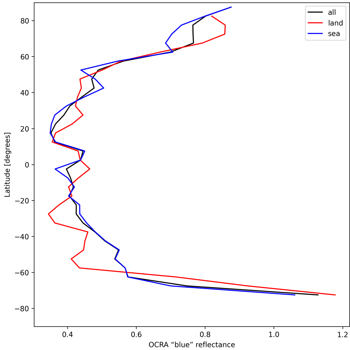
Figure 33: Zonal average of “OCRA “blue” reflectance” for 2025-04-29 to 2025-04-30.
