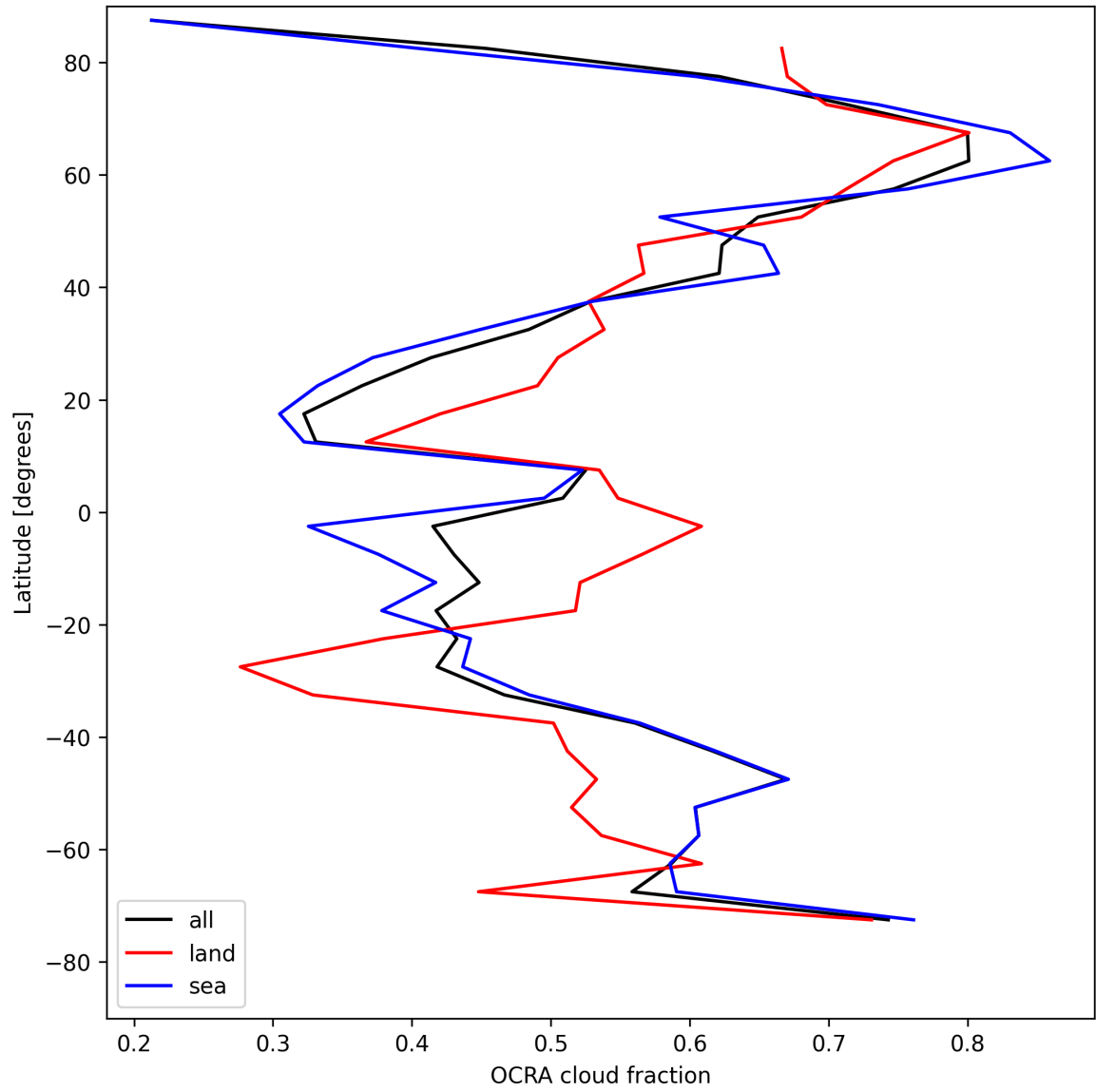
Figure 32: Zonal average of “OCRA cloud fraction” for 2025-04-29 to 2025-04-30.
