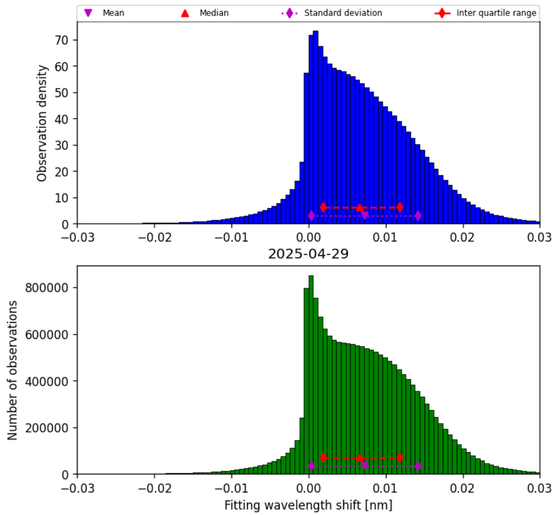
Figure 47: Histogram of “Fitting wavelength shift” for 2025-04-29 to 2025-04-30
