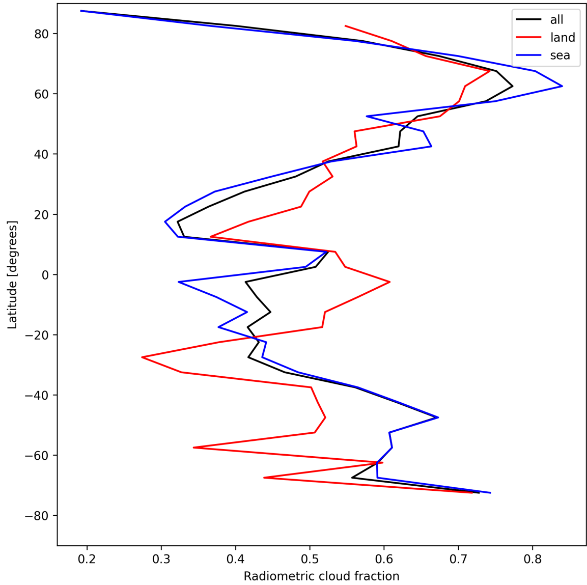
Figure 21: Zonal average of “Radiometric cloud fraction” for 2025-04-29 to 2025-04-30.
