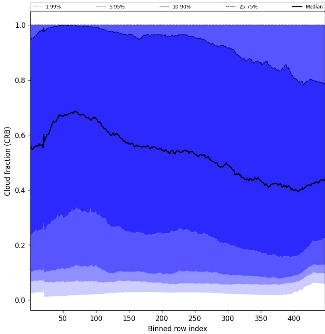
Figure 56: Along track statistics of “Cloud fraction (CRB)” for 2025-04-29 to 2025-04-30
