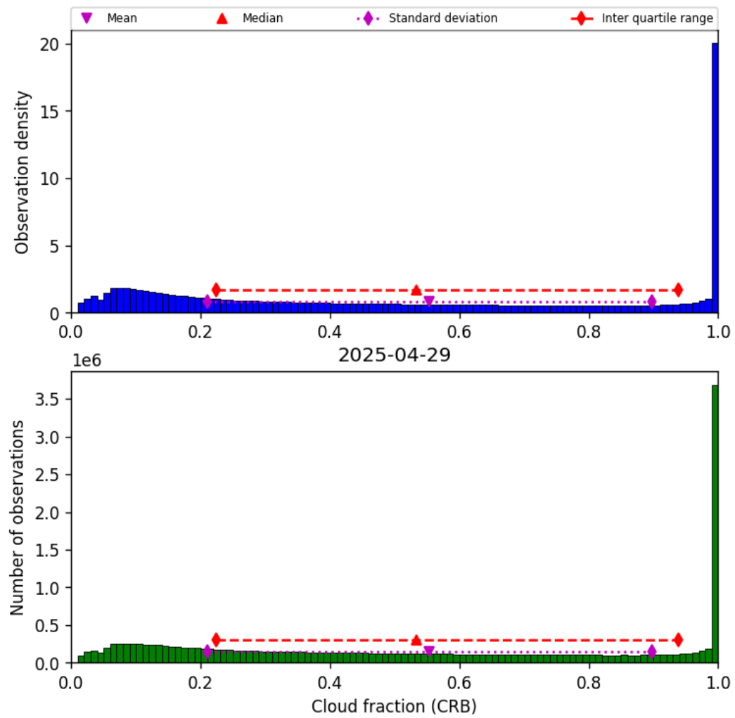
Figure 40: Histogram of “Cloud fraction (CRB)” for 2025-04-29 to 2025-04-30
