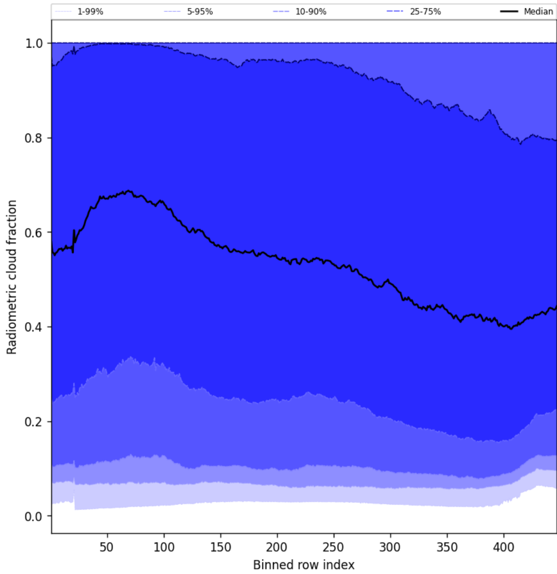
Figure 53: Along track statistics of “Radiometric cloud fraction” for 2025-04-29 to 2025-04-30
