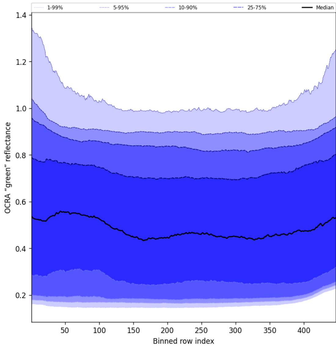
Figure 66: Along track statistics of "OCRA "green" reflectance" for 2025-04-29 to 2025-04-30
