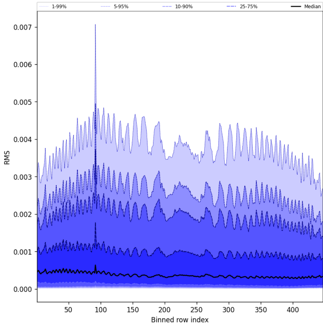
Figure 61: Along track statistics of “RMS” for 2025-04-29 to 2025-04-30
