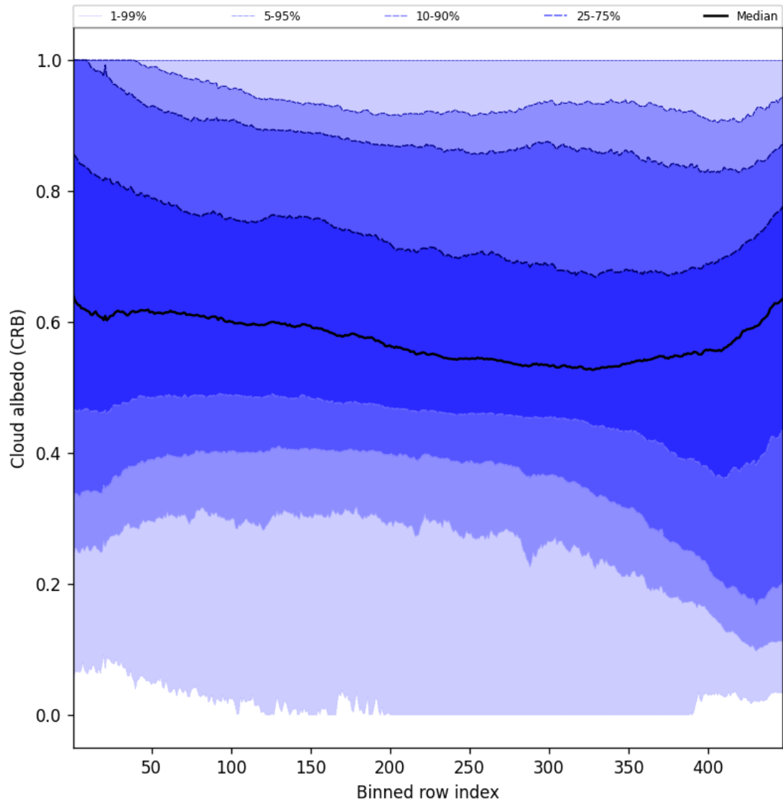
Figure 58: Along track statistics of “Cloud albedo (CRB)” for 2025-04-29 to 2025-04-30
