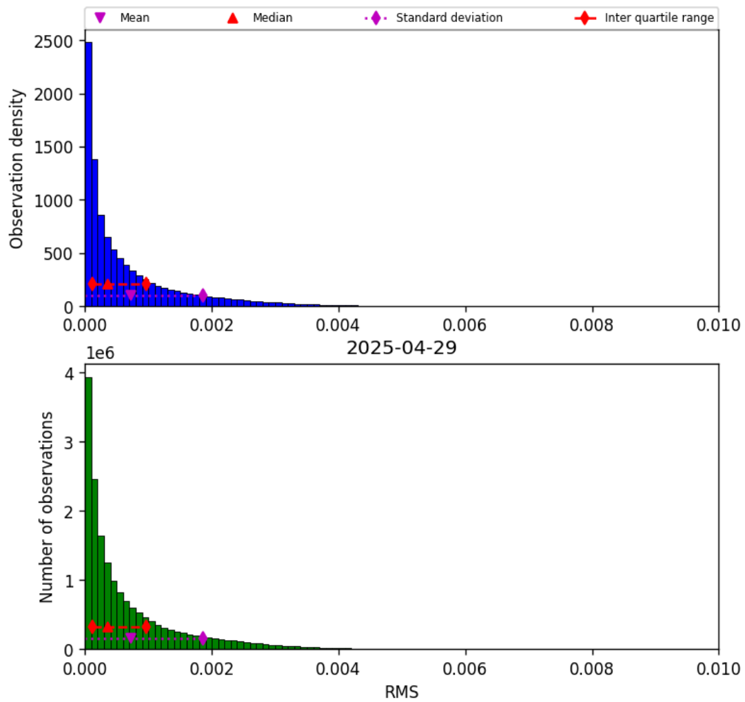
Figure 45: Histogram of “RMS” for 2025-04-29 to 2025-04-30
