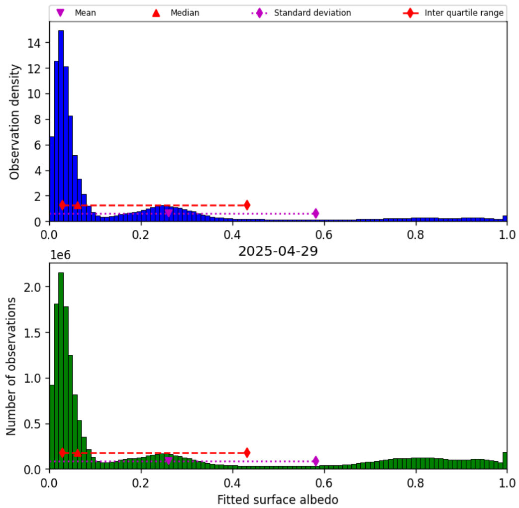
Figure 43: Histogram of “Fitted surface albedo” for 2025-04-29 to 2025-04-30
