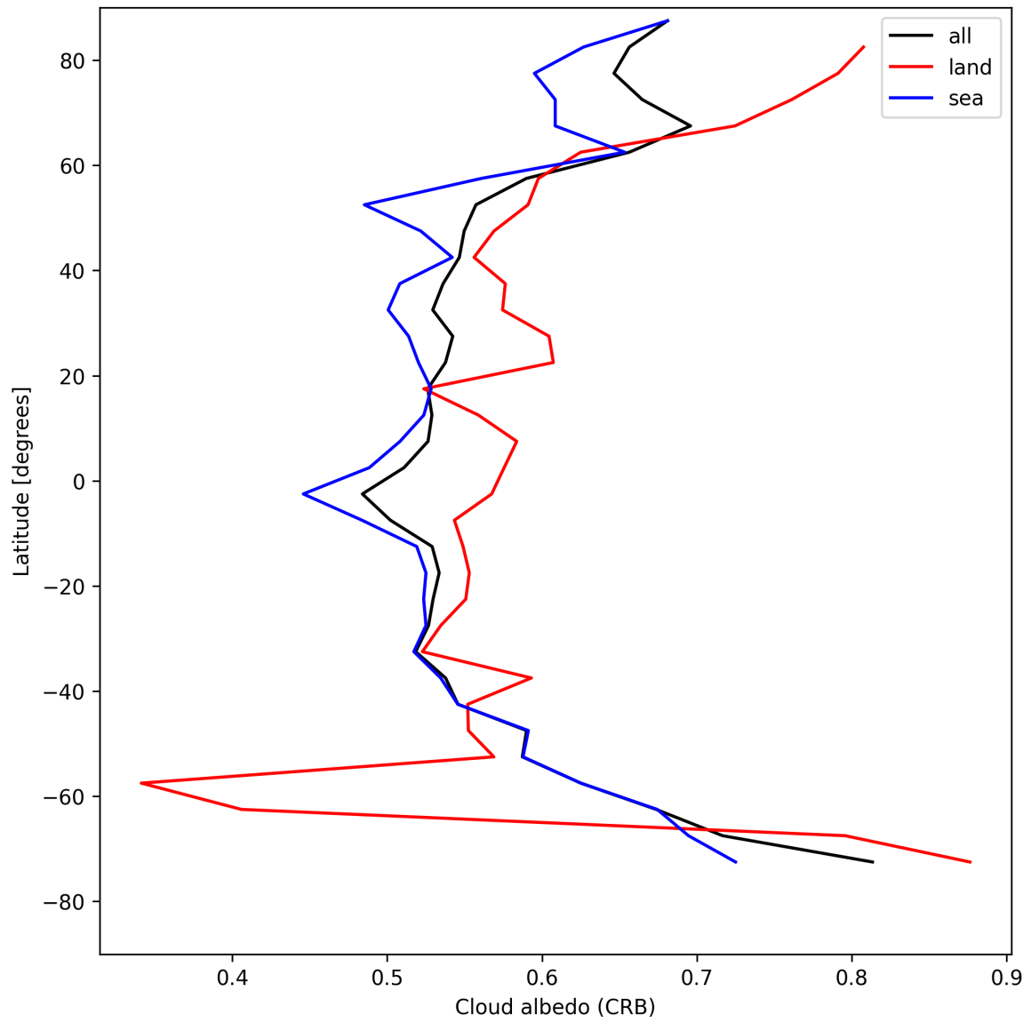
Figure 26: Zonal average of “Cloud albedo (CRB)” for 2025-04-29 to 2025-04-30.
