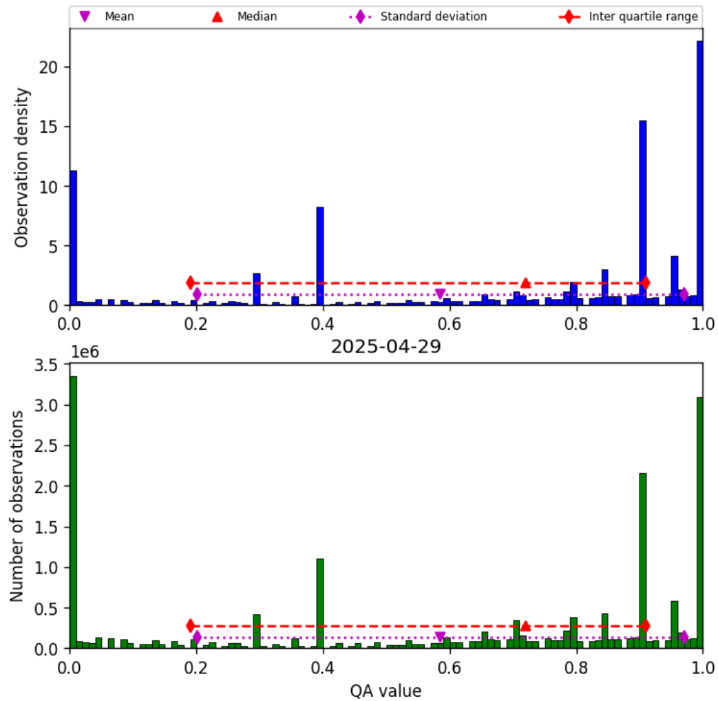
Figure 36: Histogram of “QA value” for 2025-04-29 to 2025-04-30
