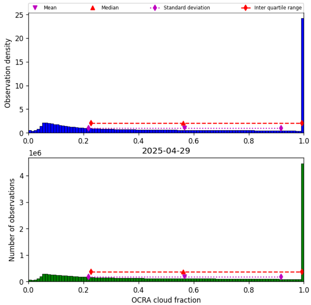
Figure 48: Histogram of “OCRA cloud fraction” for 2025-04-29 to 2025-04-30
