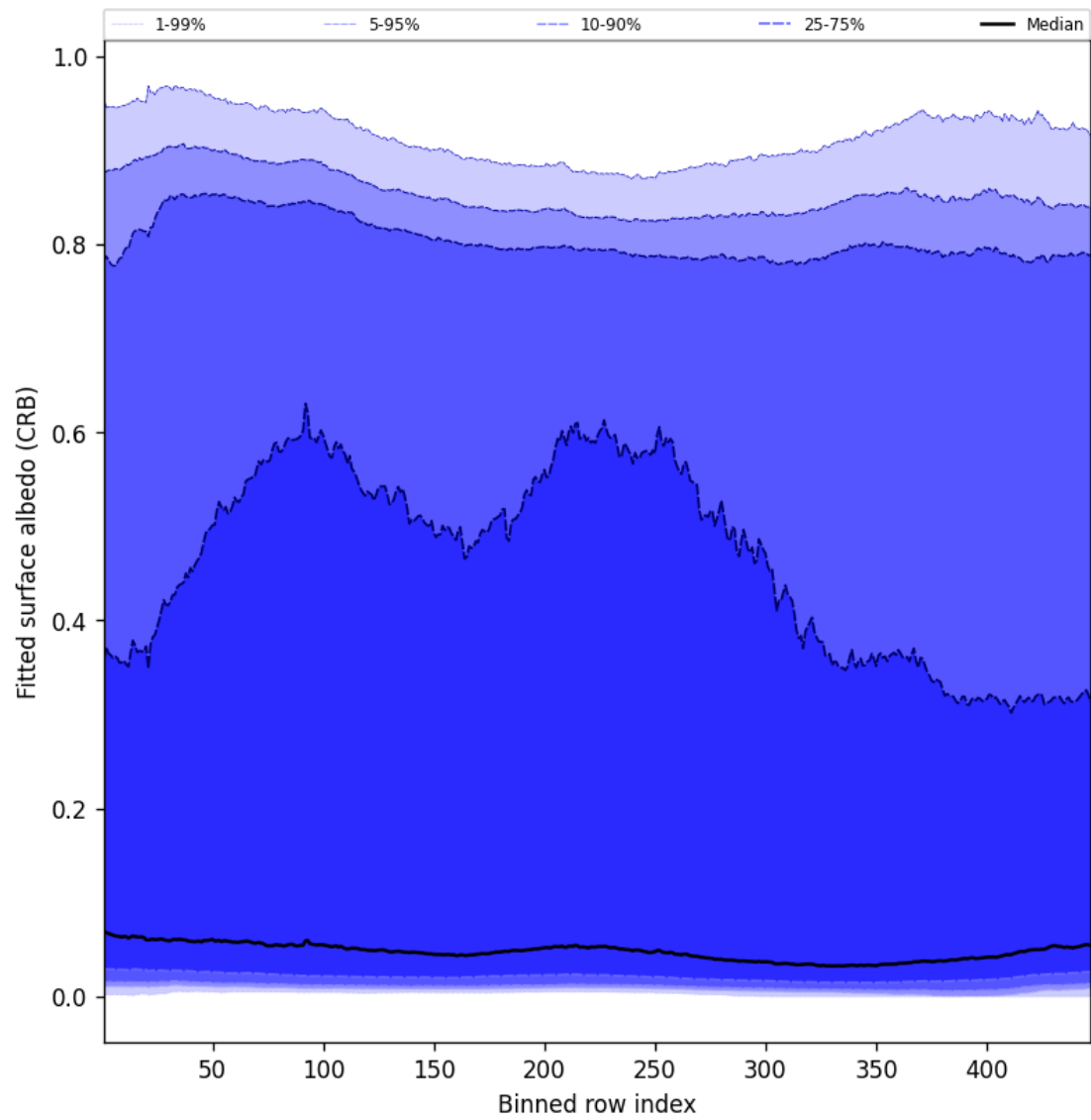
Figure 60: Along track statistics of “Fitted surface albedo (CRB)” for 2025-04-29 to 2025-04-30
