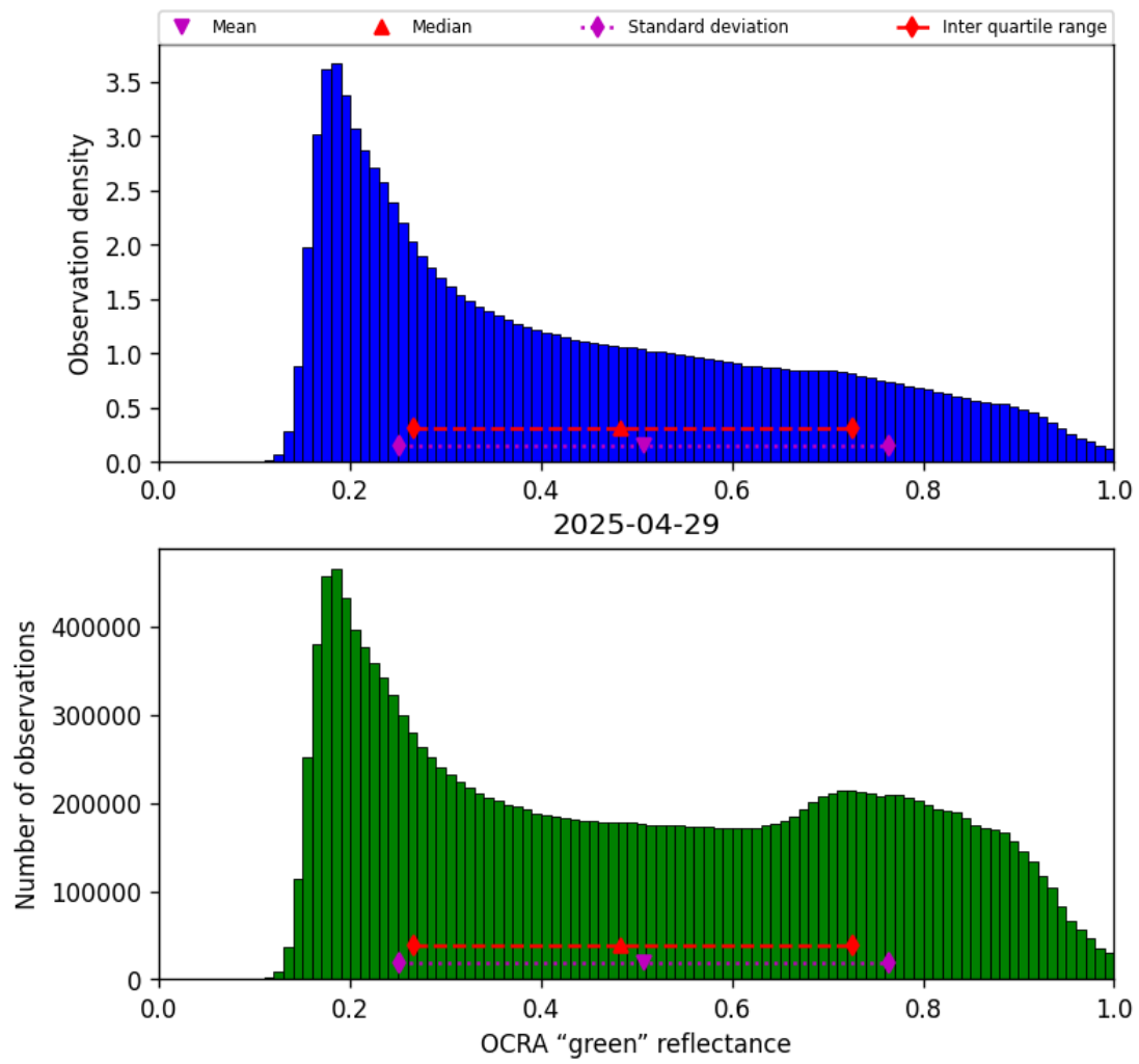
Figure 50: Histogram of “OCRA “green” reflectance” for 2025-04-29 to 2025-04-30
