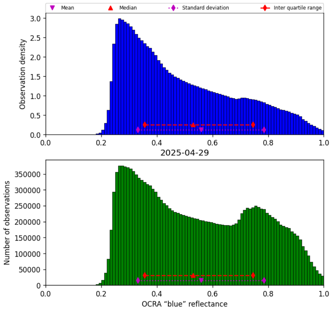
Figure 49: Histogram of “OCRA “blue” reflectance” for 2025-04-29 to 2025-04-30
