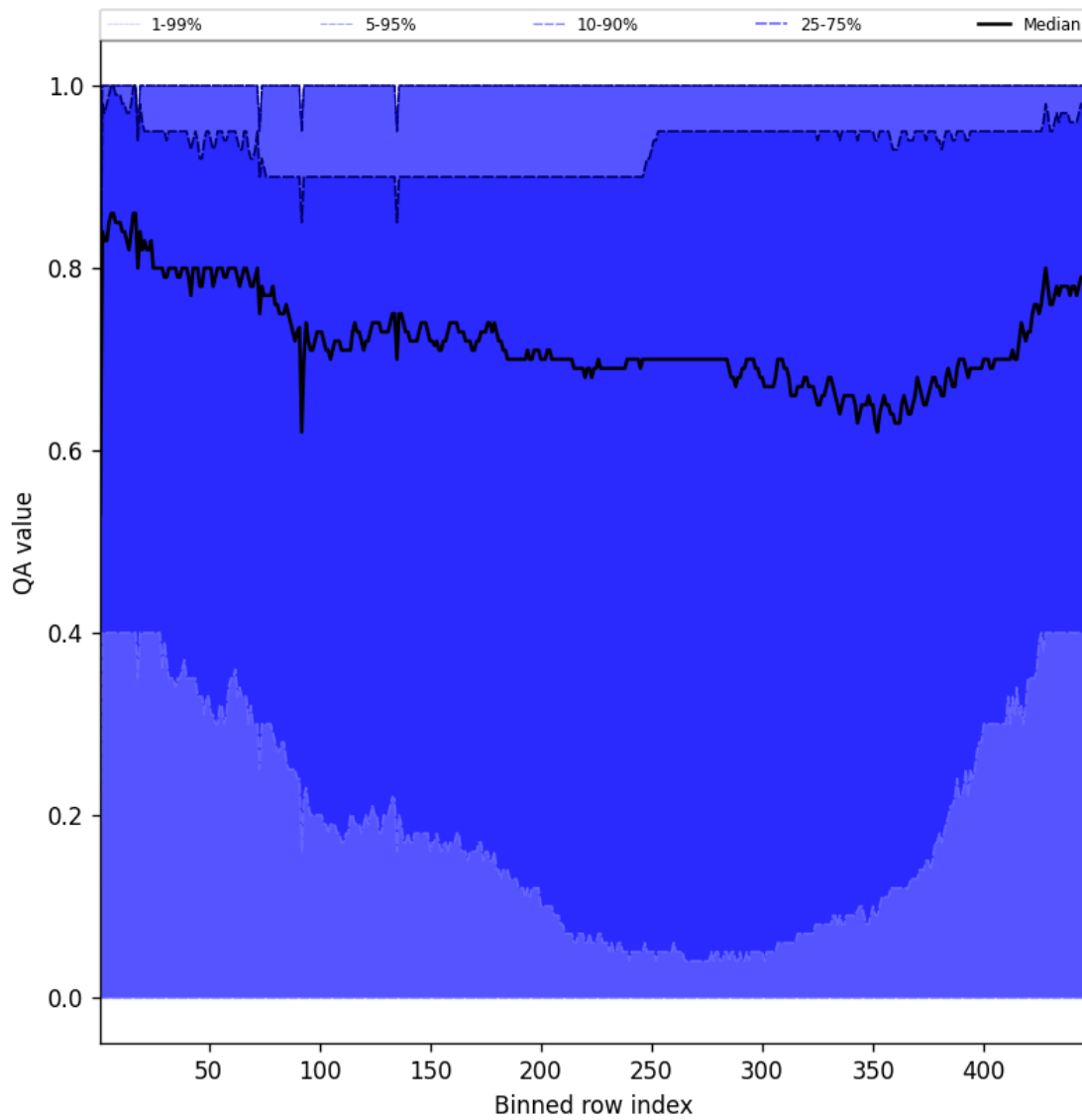
Figure 52: Along track statistics of “QA value” for 2025-04-29 to 2025-04-30
