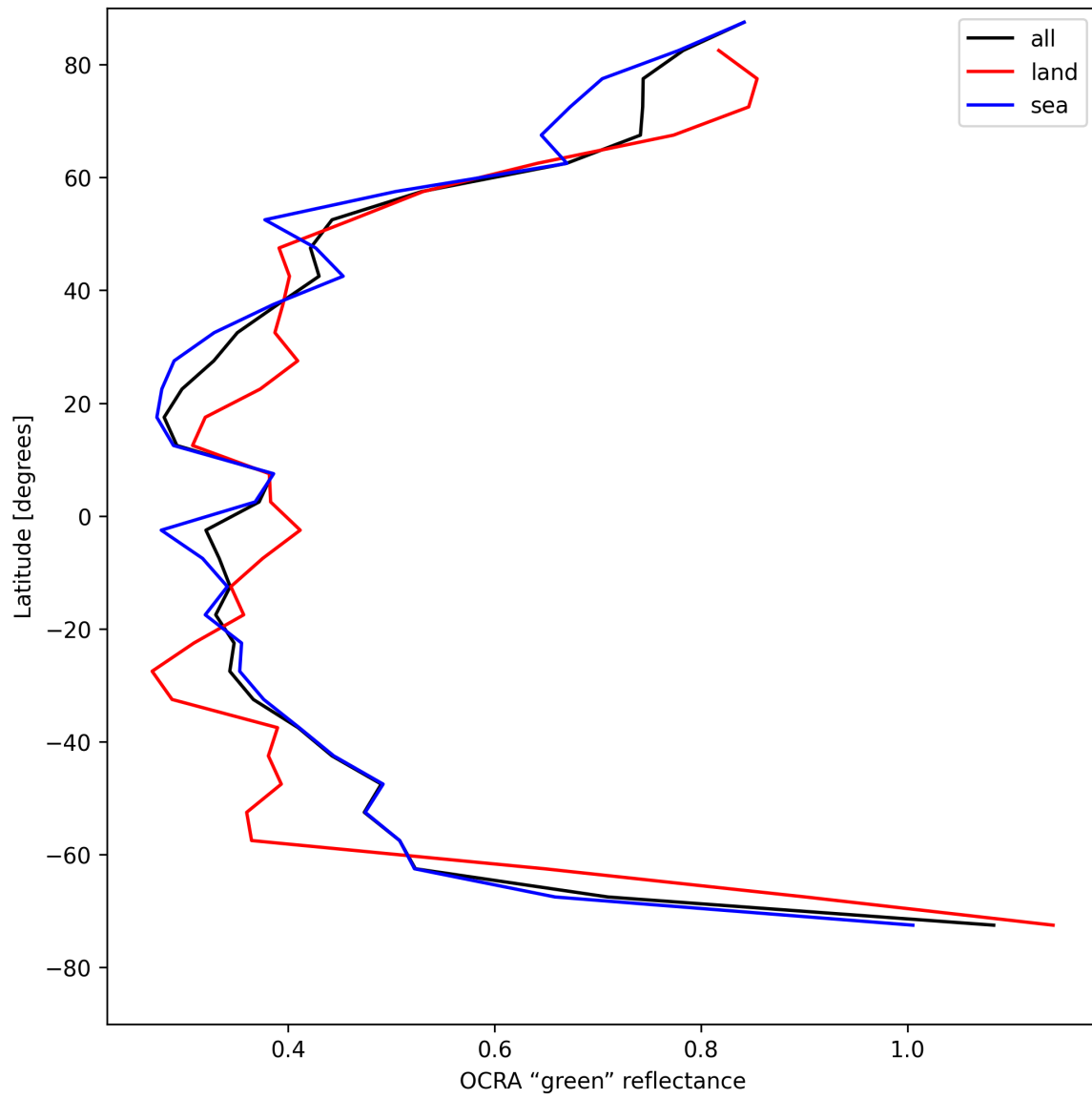
Figure 34: Zonal average of “OCRA “green” reflectance” for 2025-04-29 to 2025-04-30.
