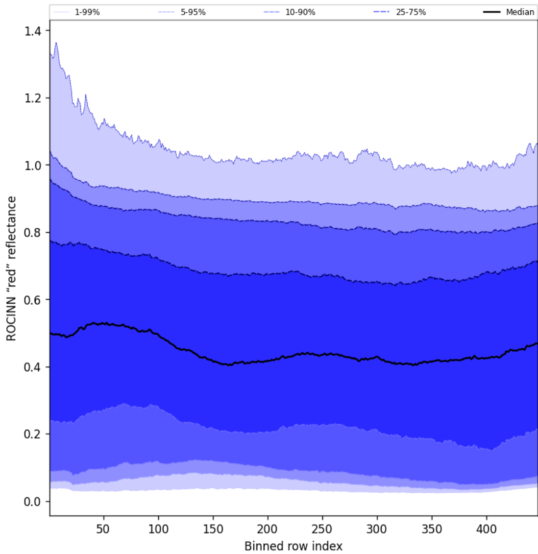
Figure 67: Along track statistics of "ROCINN "red" reflectance" for 2025-04-29 to 2025-04-30
