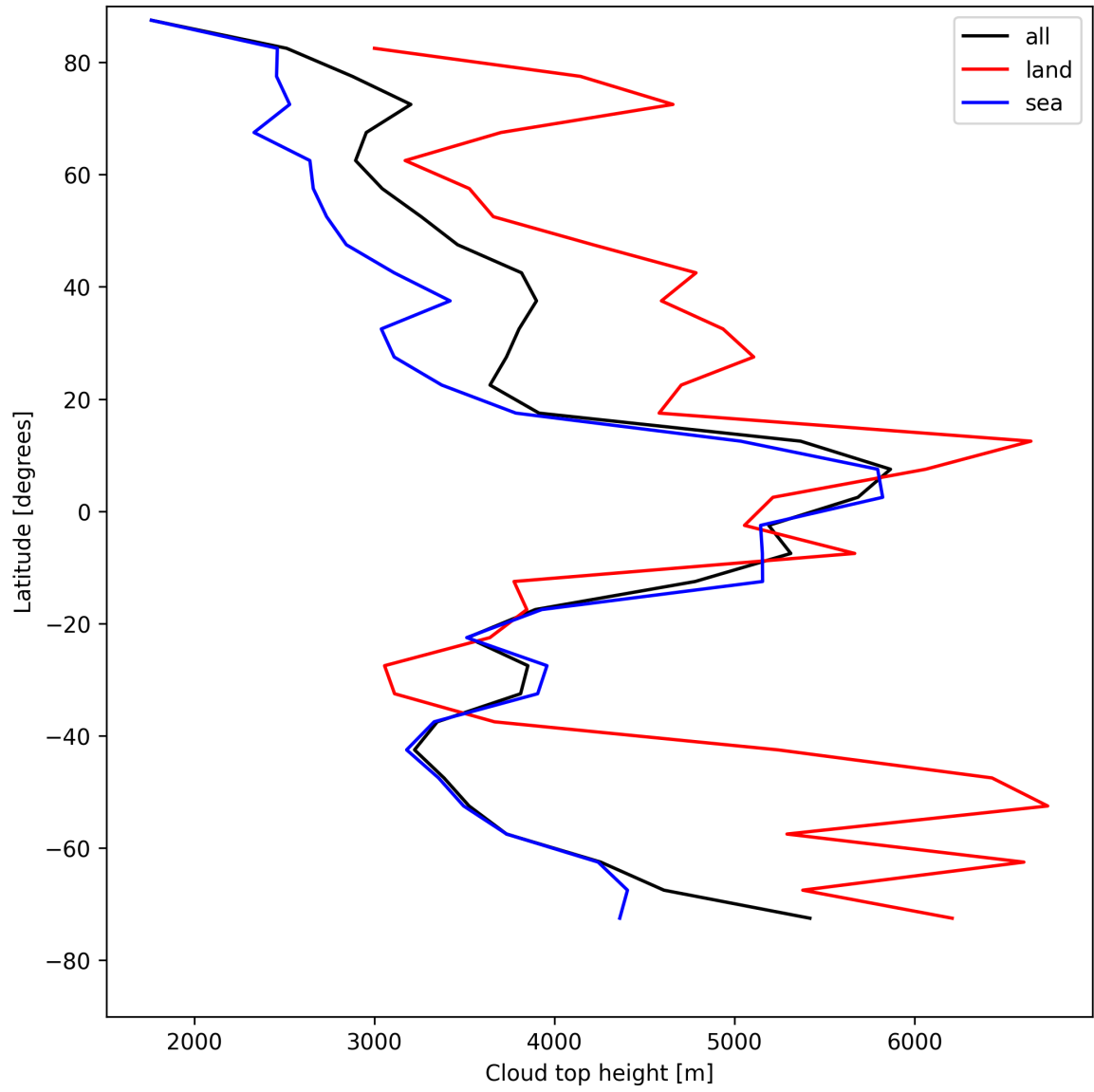
Figure 22: Zonal average of “Cloud top height” for 2025-04-29 to 2025-04-30.
