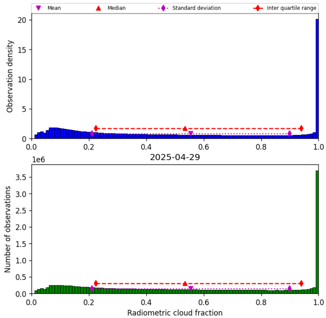
Figure 37: Histogram of “Radiometric cloud fraction” for 2025-04-29 to 2025-04-30
