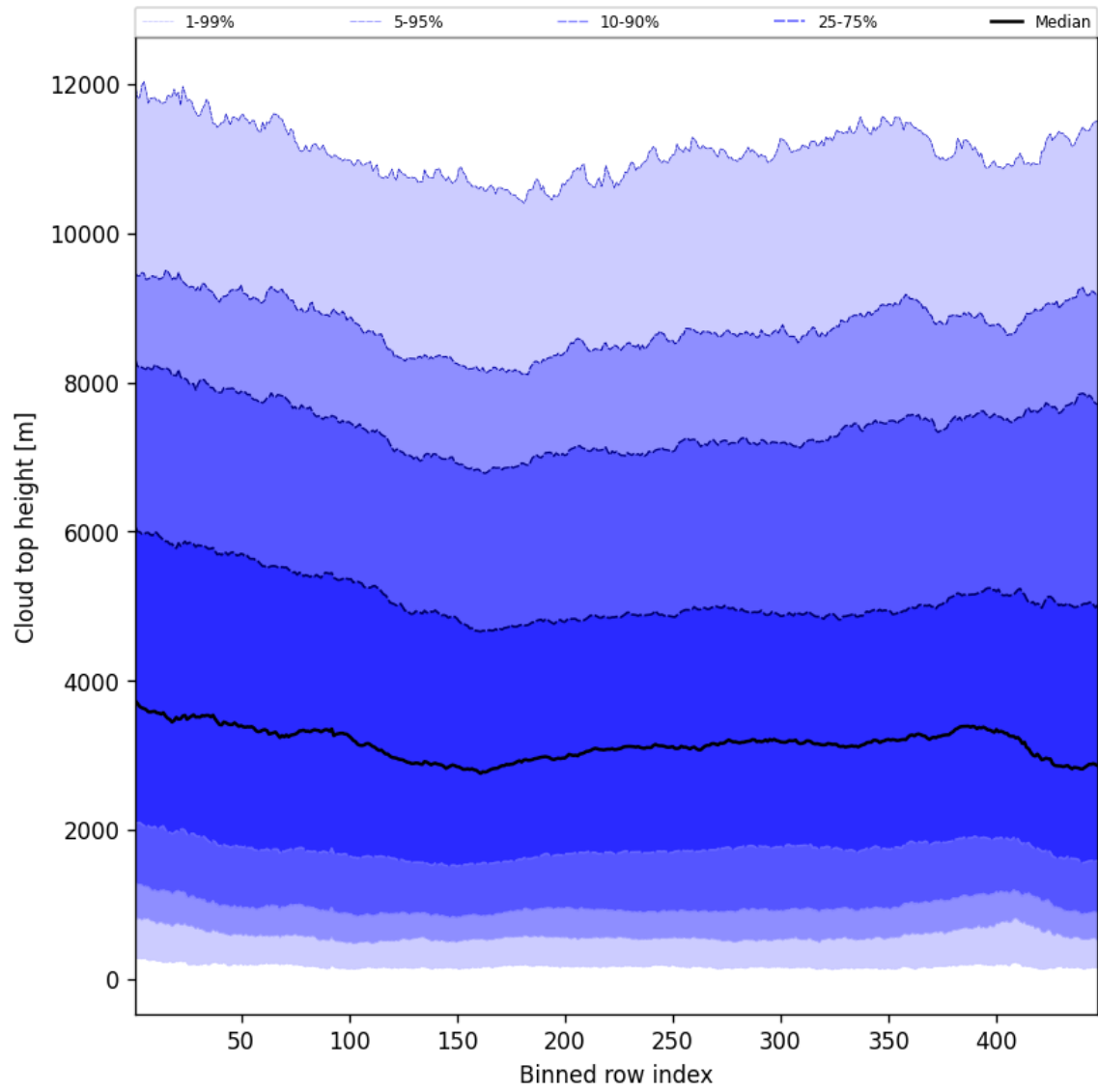
Figure 54: Along track statistics of “Cloud top height” for 2025-04-29 to 2025-04-30
