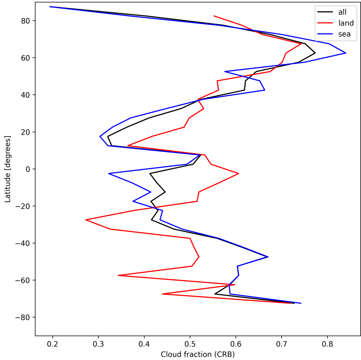
Figure 24: Zonal average of “Cloud fraction (CRB)” for 2025-04-29 to 2025-04-30.
