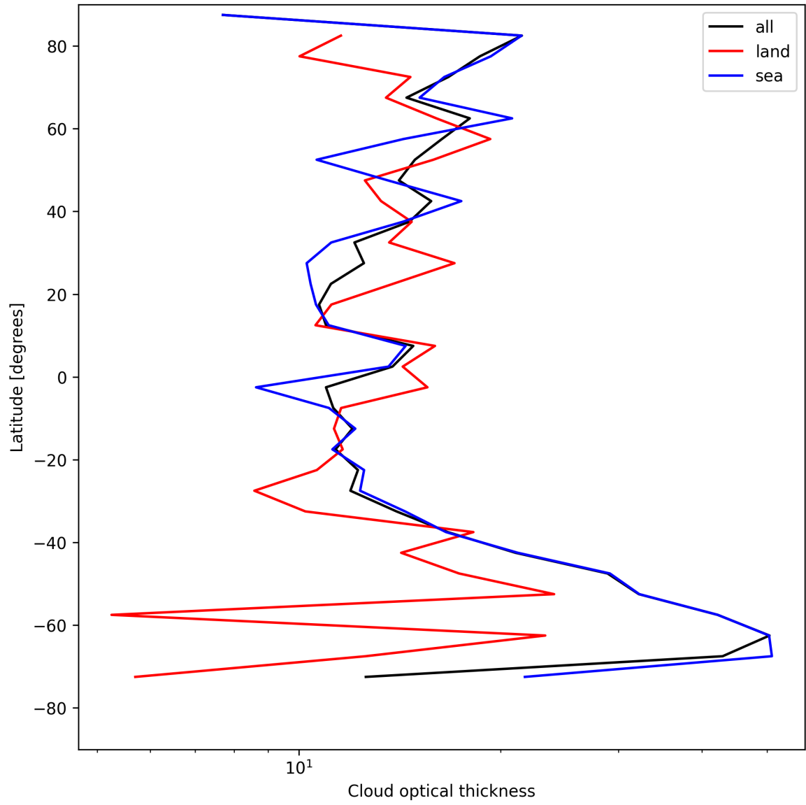
Figure 23: Zonal average of “Cloud optical thickness” for 2025-04-29 to 2025-04-30.
