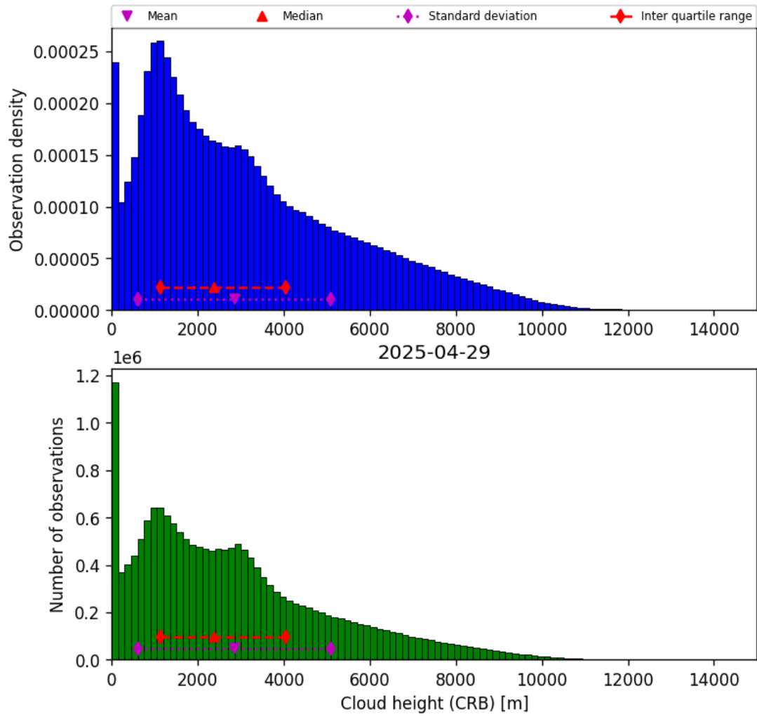
Figure 41: Histogram of “Cloud height (CRB)” for 2025-04-29 to 2025-04-30
