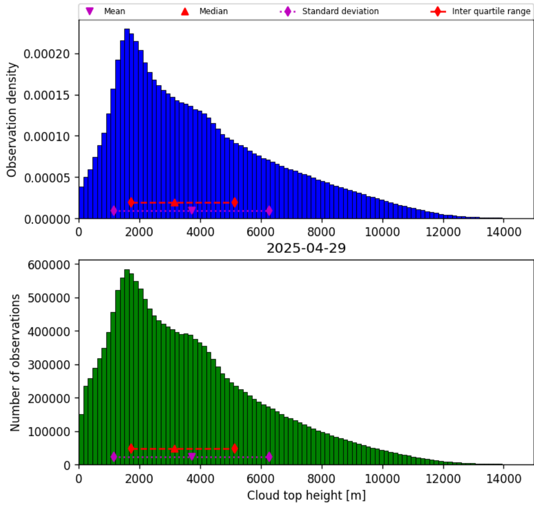
Figure 38: Histogram of “Cloud top height” for 2025-04-29 to 2025-04-30
