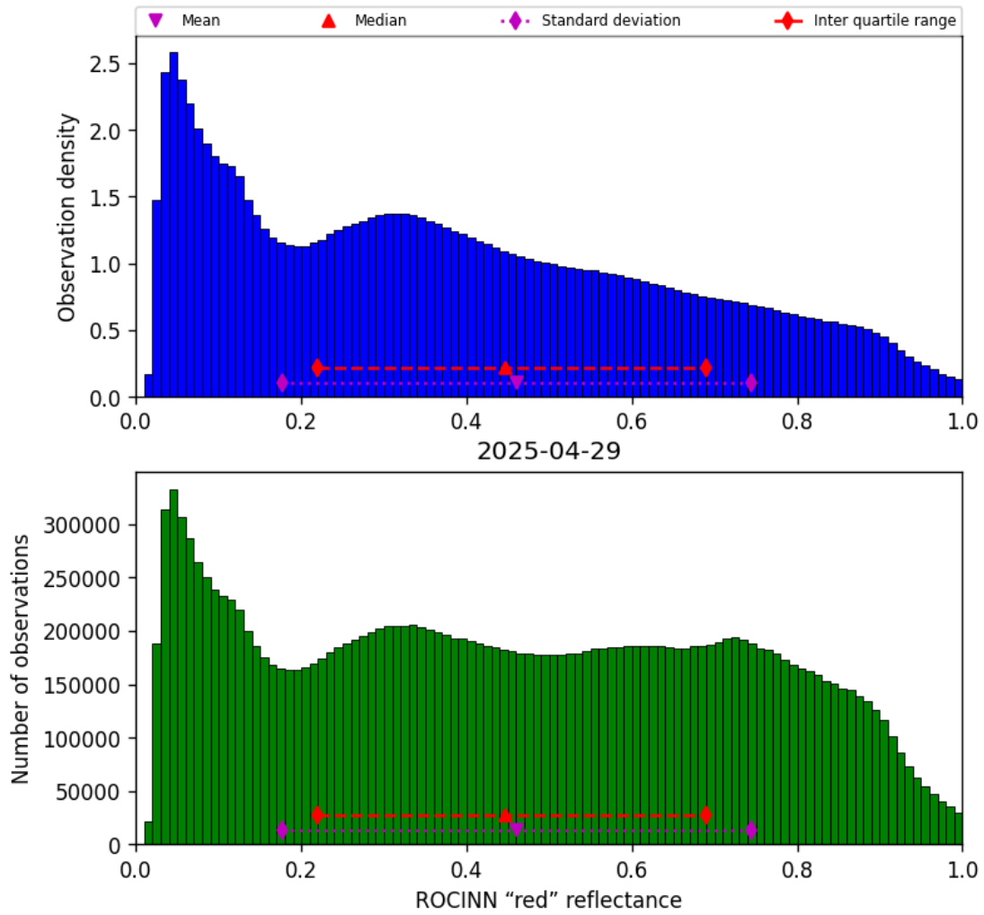
Figure 51: Histogram of “ROCINN “red” reflectance” for 2025-04-29 to 2025-04-30
