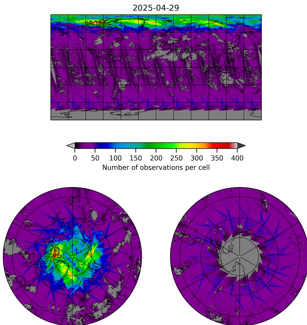
Figure 19: Map of the number of observations for 2025-04-29 to 2025-04-30
