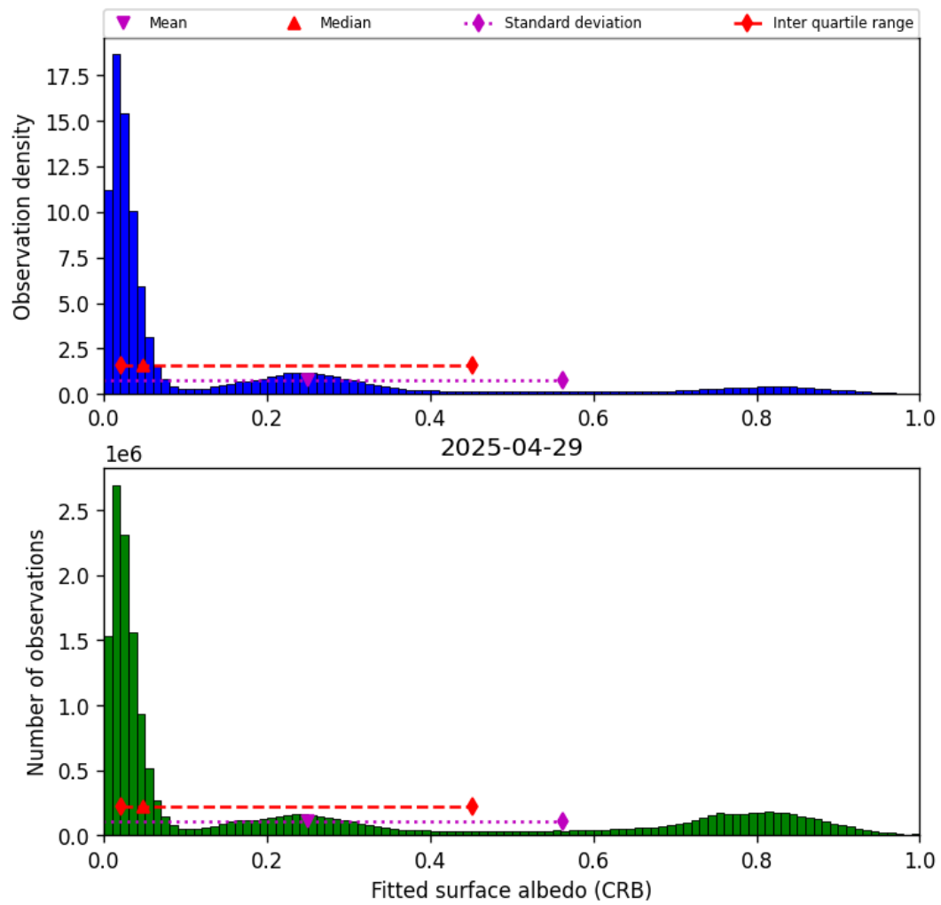
Figure 44: Histogram of “Fitted surface albedo (CRB)” for 2025-04-29 to 2025-04-30
