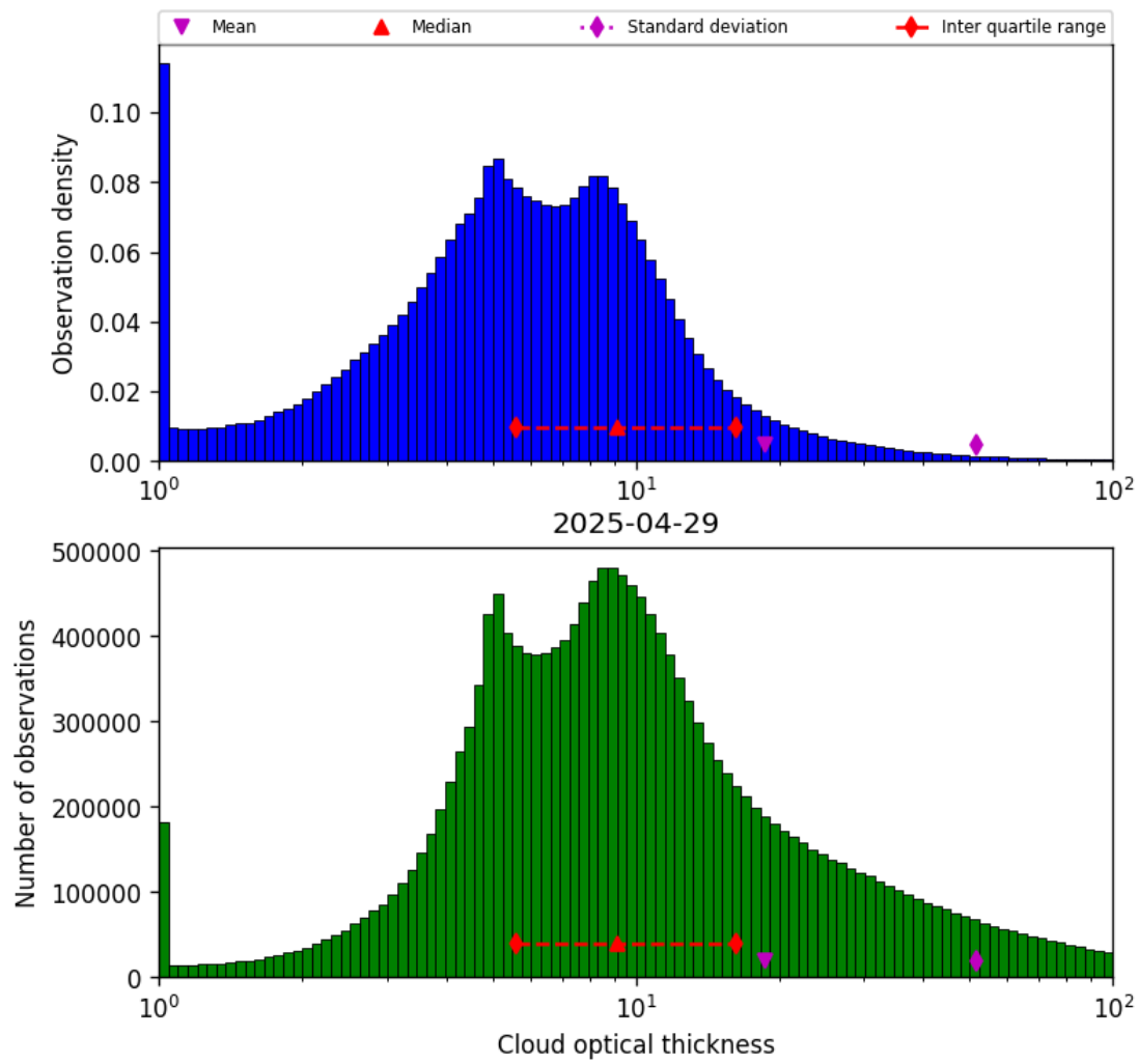
Figure 39: Histogram of “Cloud optical thickness” for 2025-04-29 to 2025-04-30
