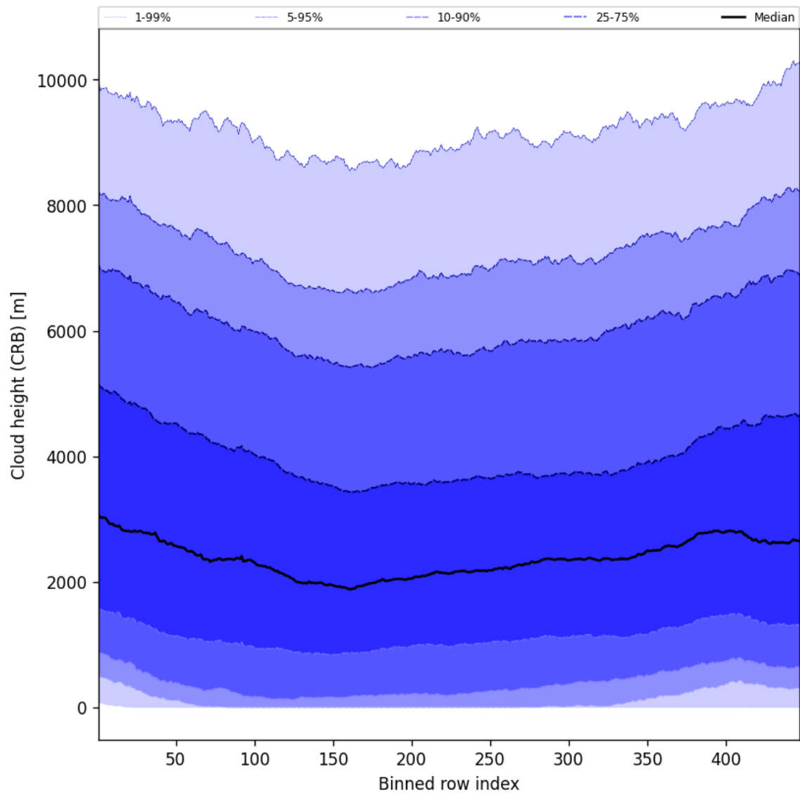
Figure 57: Along track statistics of “Cloud height (CRB)” for 2025-04-29 to 2025-04-30
