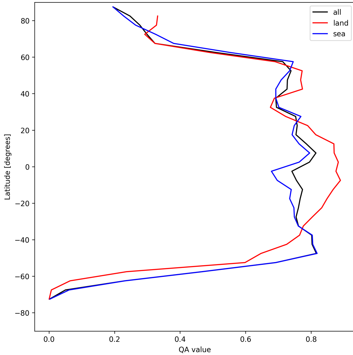
Figure 20: Zonal average of “QA value” for 2025-04-29 to 2025-04-30.
