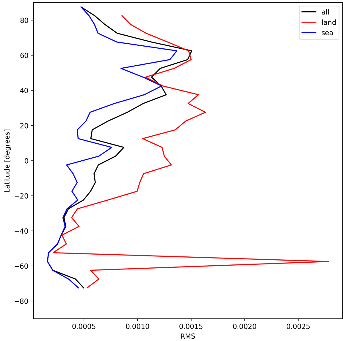
Figure 29: Zonal average of “RMS” for 2025-04-29 to 2025-04-30.
