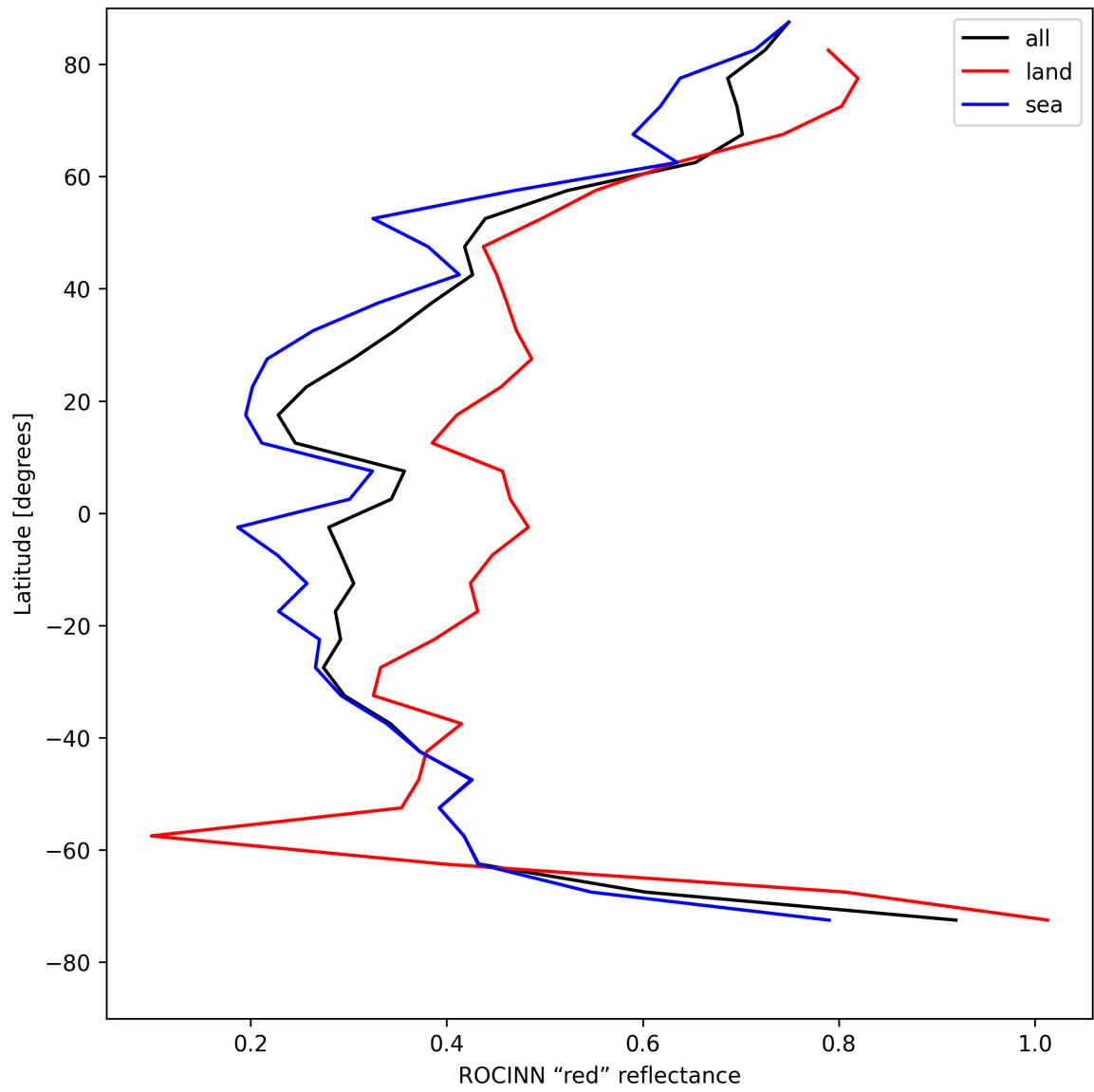
Figure 35: Zonal average of “ROCINN “red” reflectance” for 2025-04-29 to 2025-04-30.
