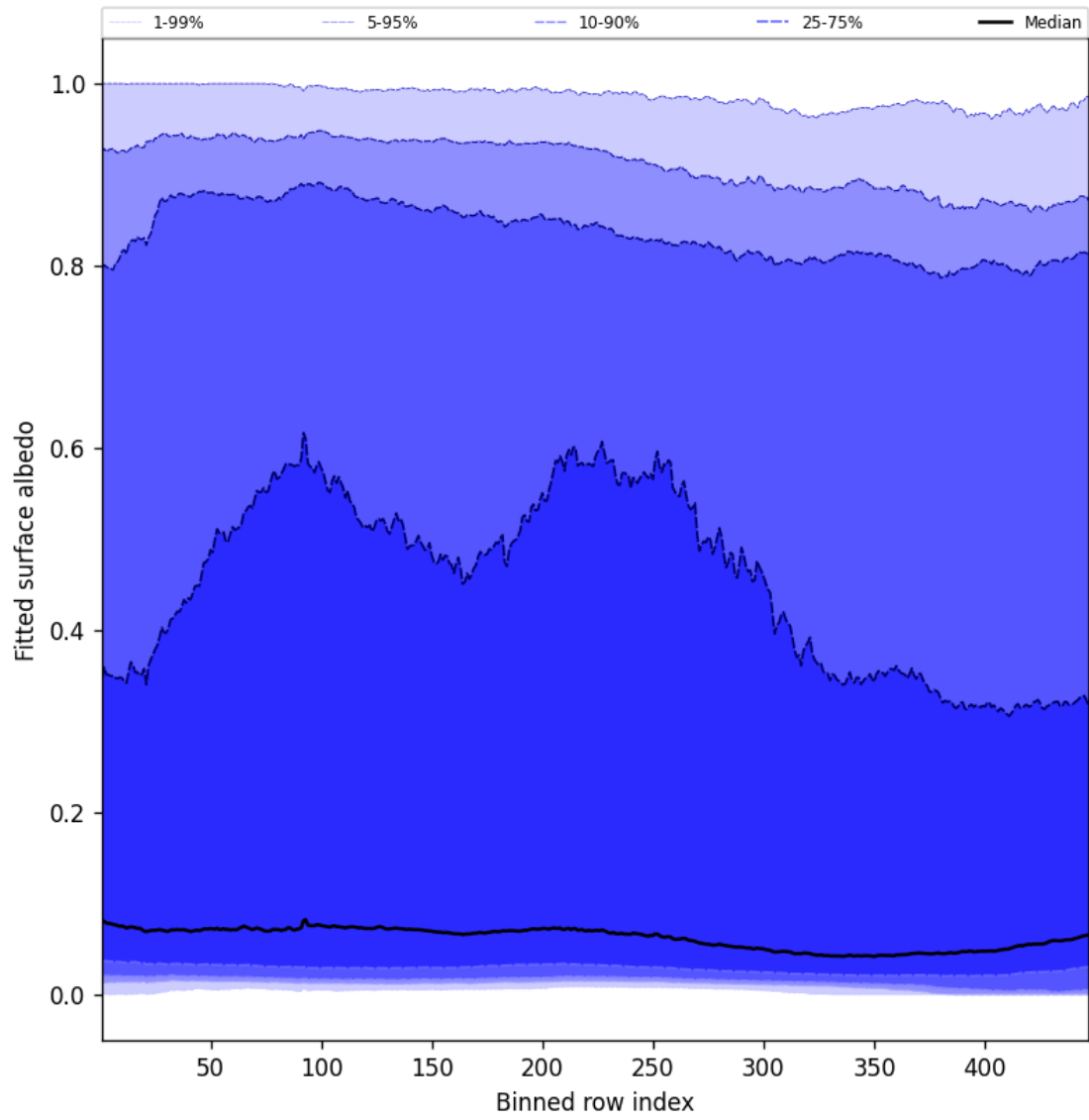
Figure 59: Along track statistics of “Fitted surface albedo” for 2025-04-29 to 2025-04-30
