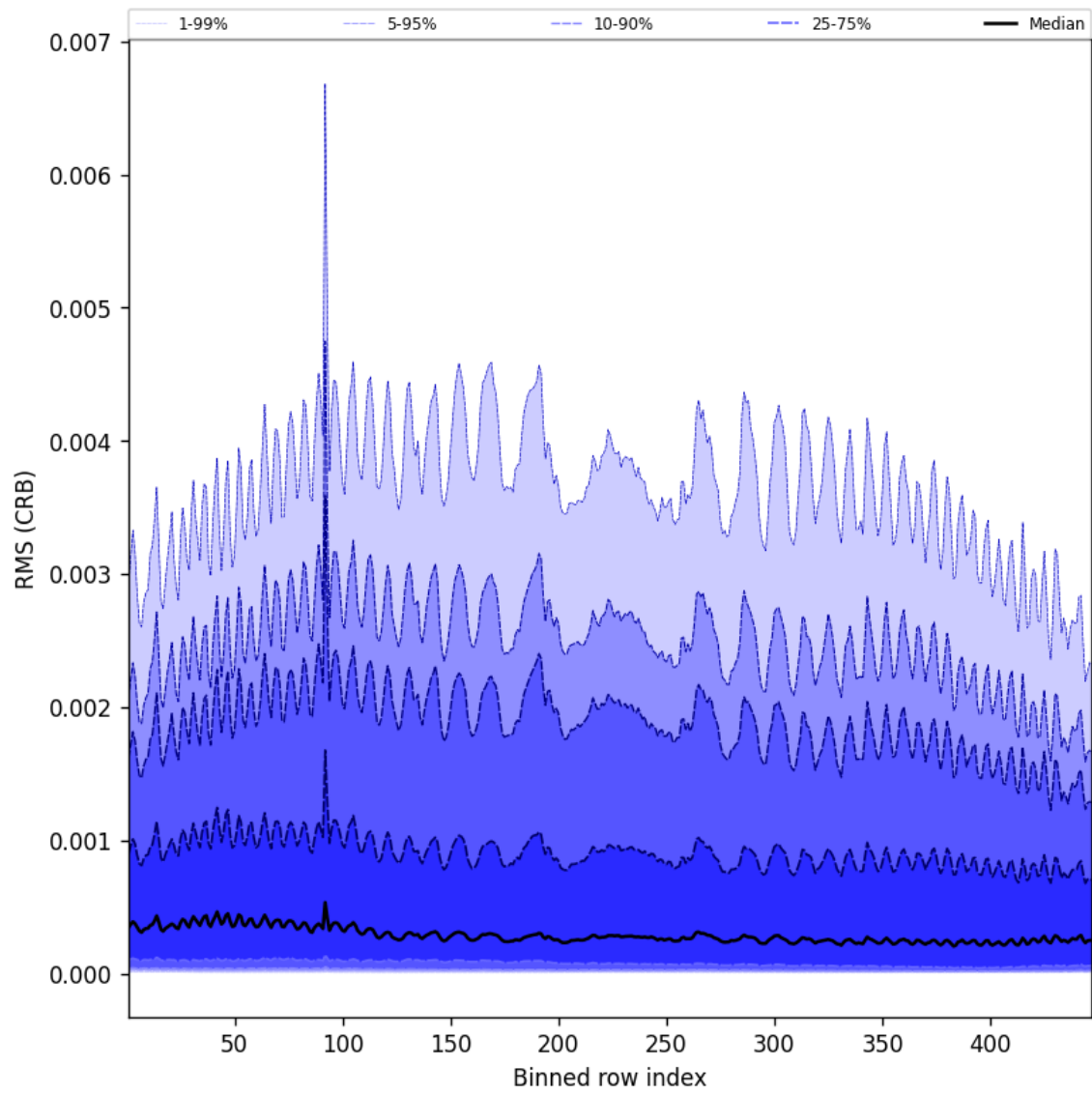
Figure 62: Along track statistics of “RMS (CRB)” for 2025-04-29 to 2025-04-30
