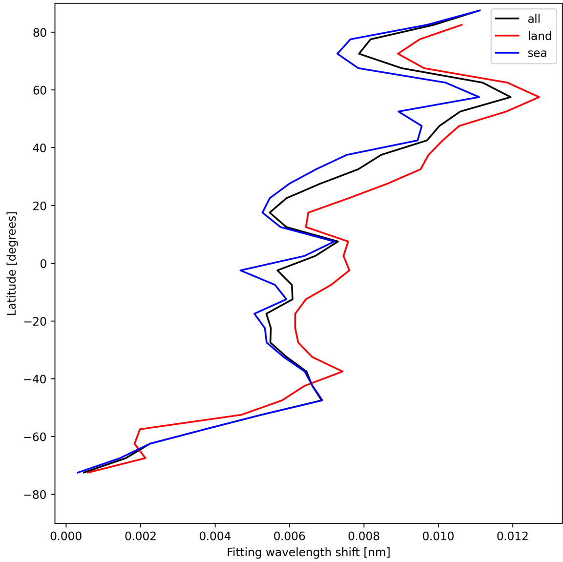
Figure 31: Zonal average of “Fitting wavelength shift” for 2025-04-29 to 2025-04-30.
