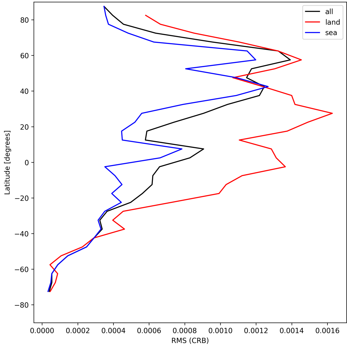
Figure 30: Zonal average of “RMS (CRB)” for 2025-04-29 to 2025-04-30.
