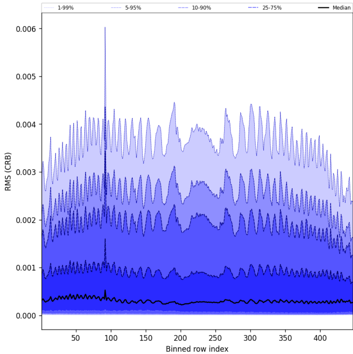
Figure 62: Along track statistics of “RMS (CRB)” for 2025-04-30 to 2025-05-01
