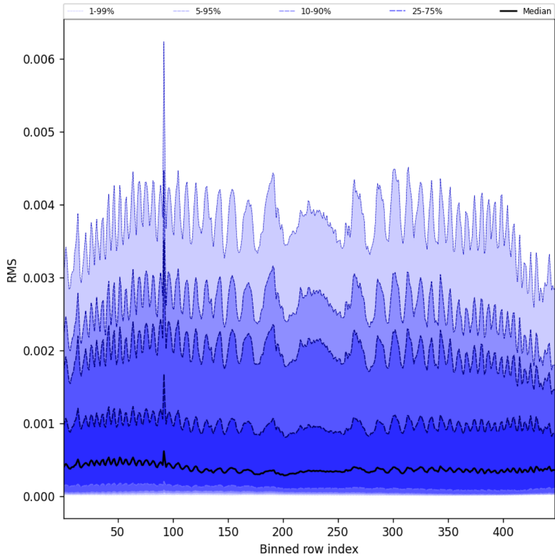
Figure 61: Along track statistics of “RMS” for 2025-04-30 to 2025-05-01
