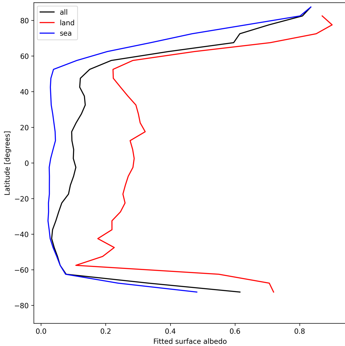
Figure 27: Zonal average of “Fitted surface albedo” for 2025-04-30 to 2025-05-01.
