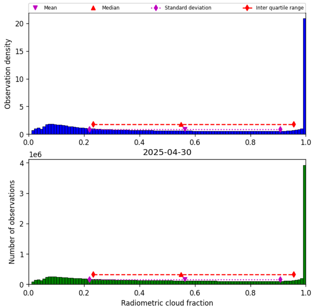
Figure 37: Histogram of “Radiometric cloud fraction” for 2025-04-30 to 2025-05-01
