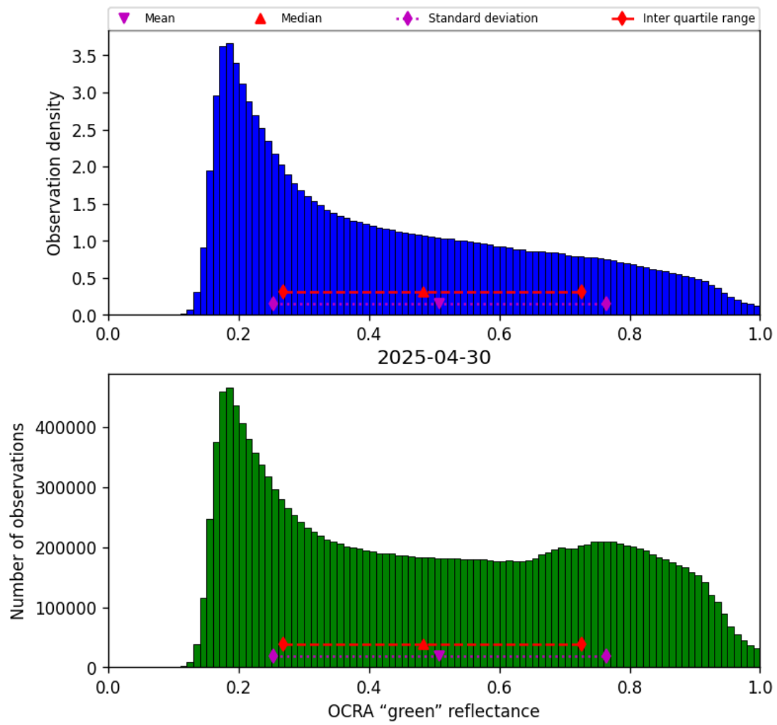
Figure 50: Histogram of “OCRA “green” reflectance” for 2025-04-30 to 2025-05-01
