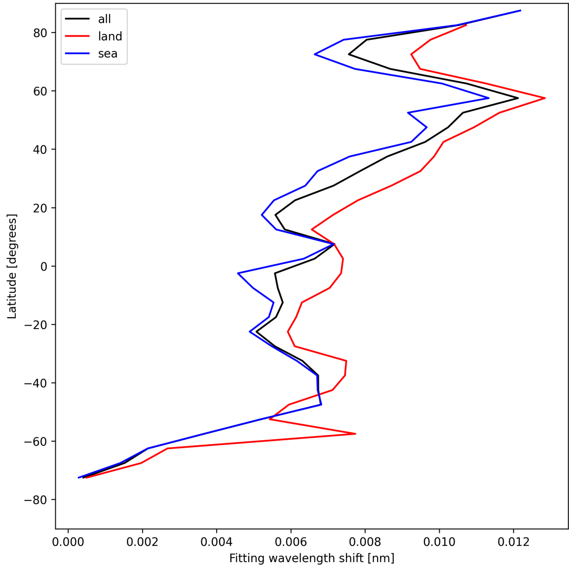
Figure 31: Zonal average of “Fitting wavelength shift” for 2025-04-30 to 2025-05-01.
