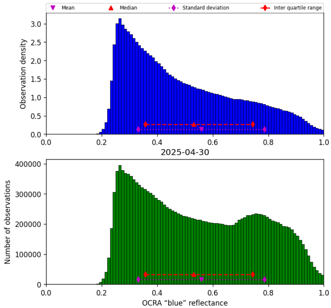
Figure 49: Histogram of “OCRA “blue” reflectance” for 2025-04-30 to 2025-05-01
