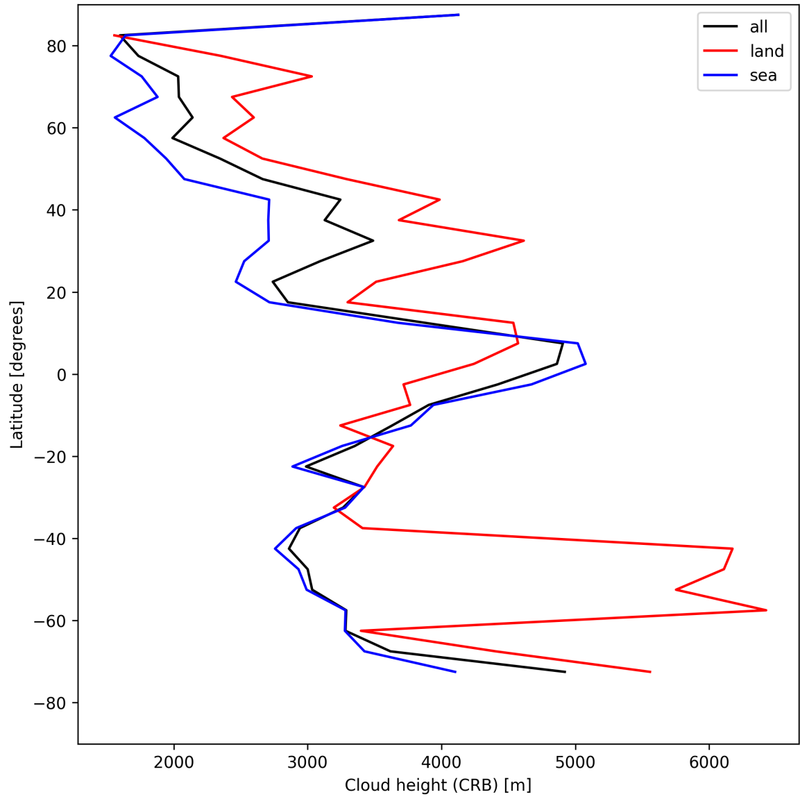
Figure 25: Zonal average of “Cloud height (CRB)” for 2025-04-30 to 2025-05-01.
