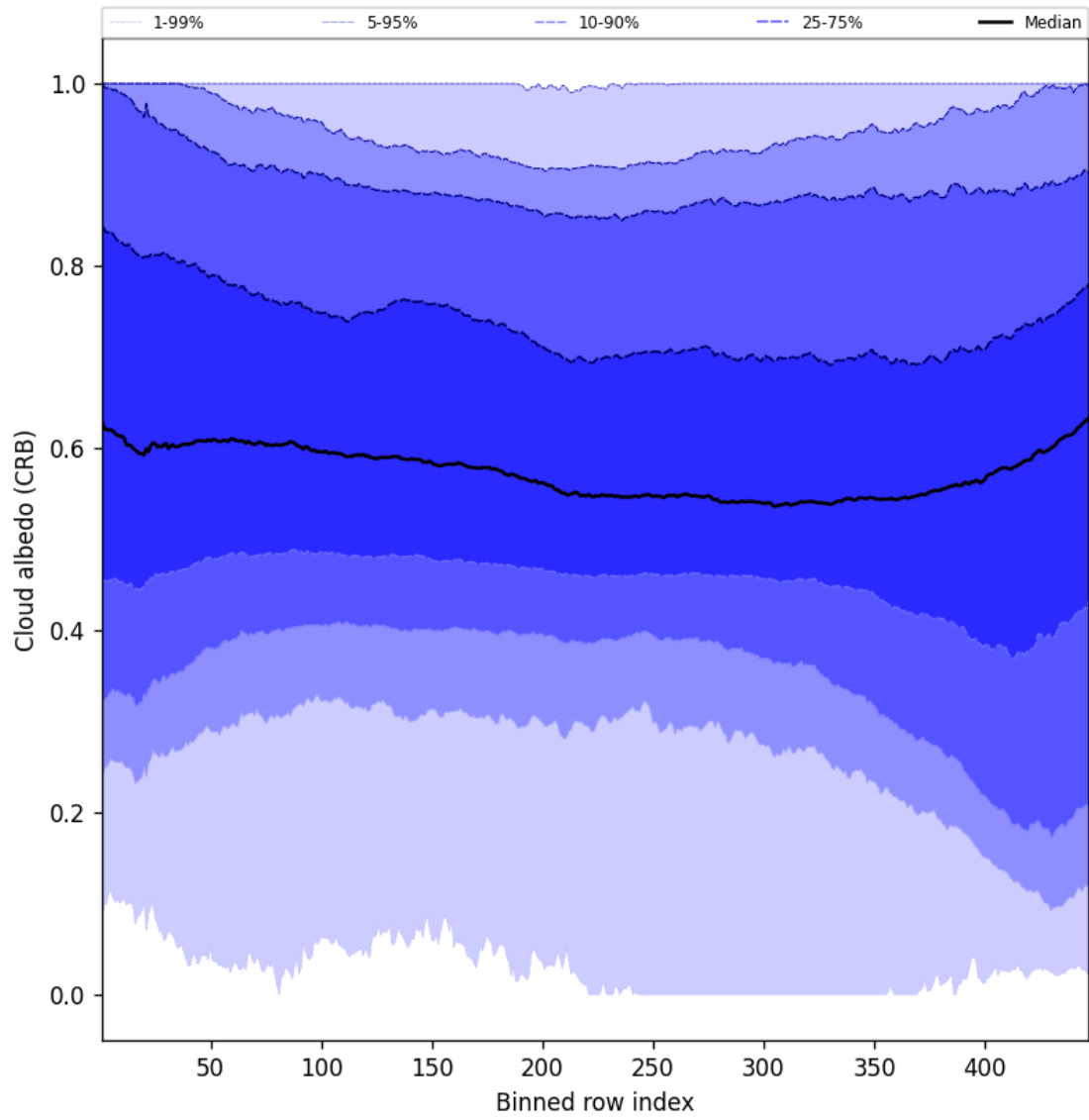
Figure 58: Along track statistics of “Cloud albedo (CRB)” for 2025-04-30 to 2025-05-01
