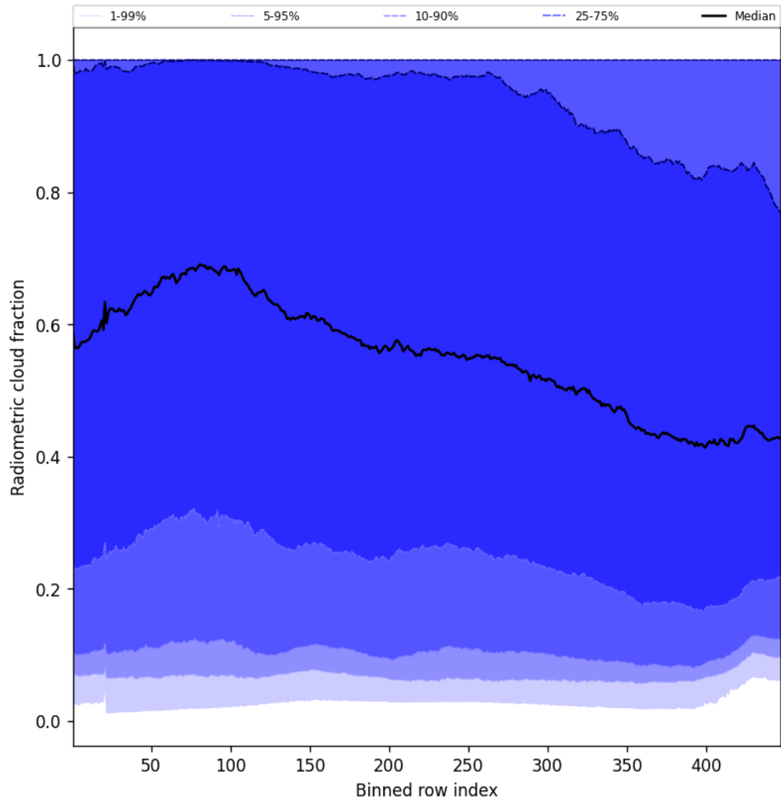
Figure 53: Along track statistics of “Radiometric cloud fraction” for 2025-04-30 to 2025-05-01
