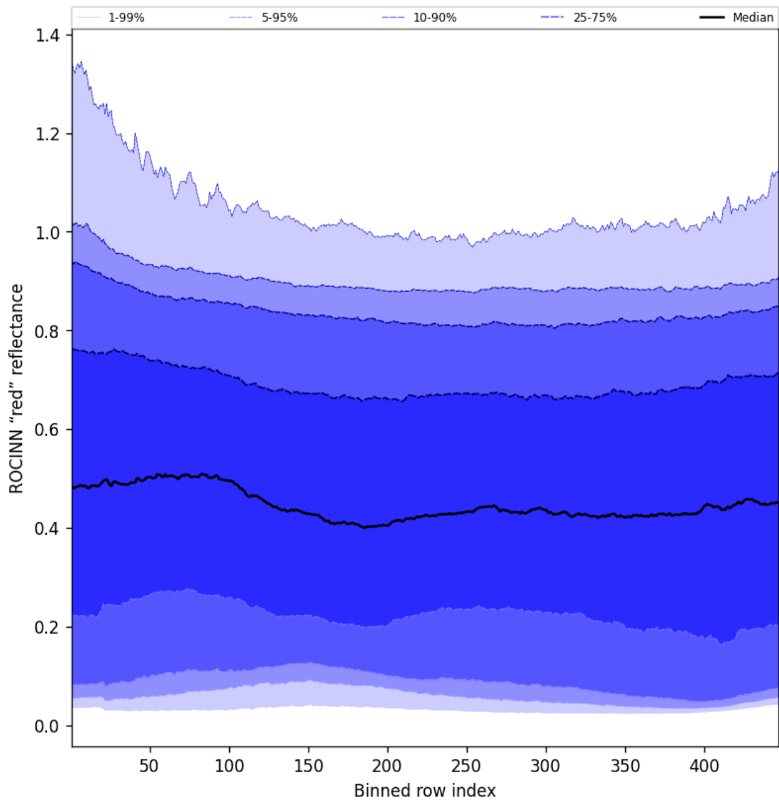
Figure 67: Along track statistics of "ROCINN "red" reflectance" for 2025-04-30 to 2025-05-01
