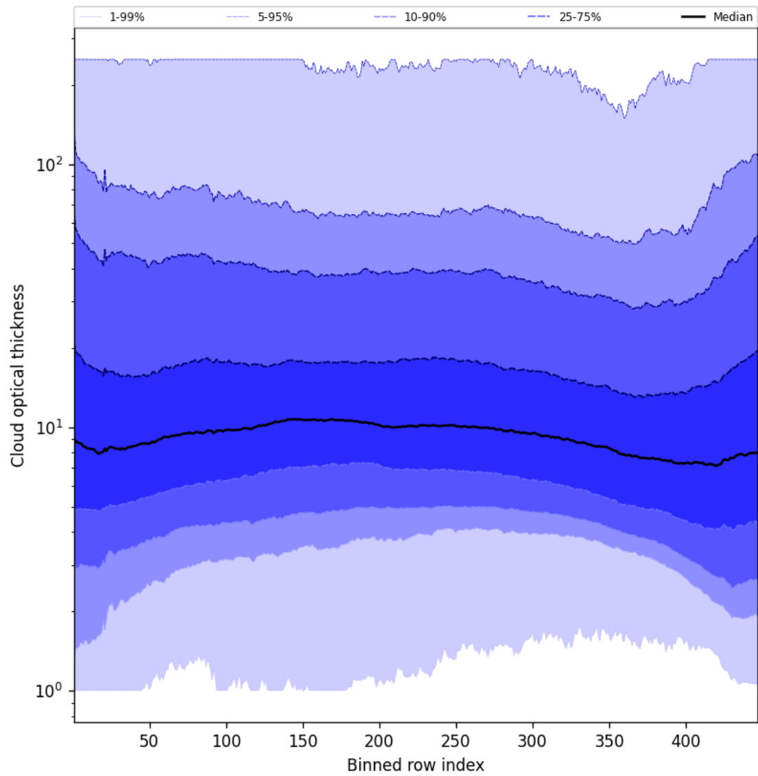
Figure 55: Along track statistics of “Cloud optical thickness” for 2025-04-30 to 2025-05-01
