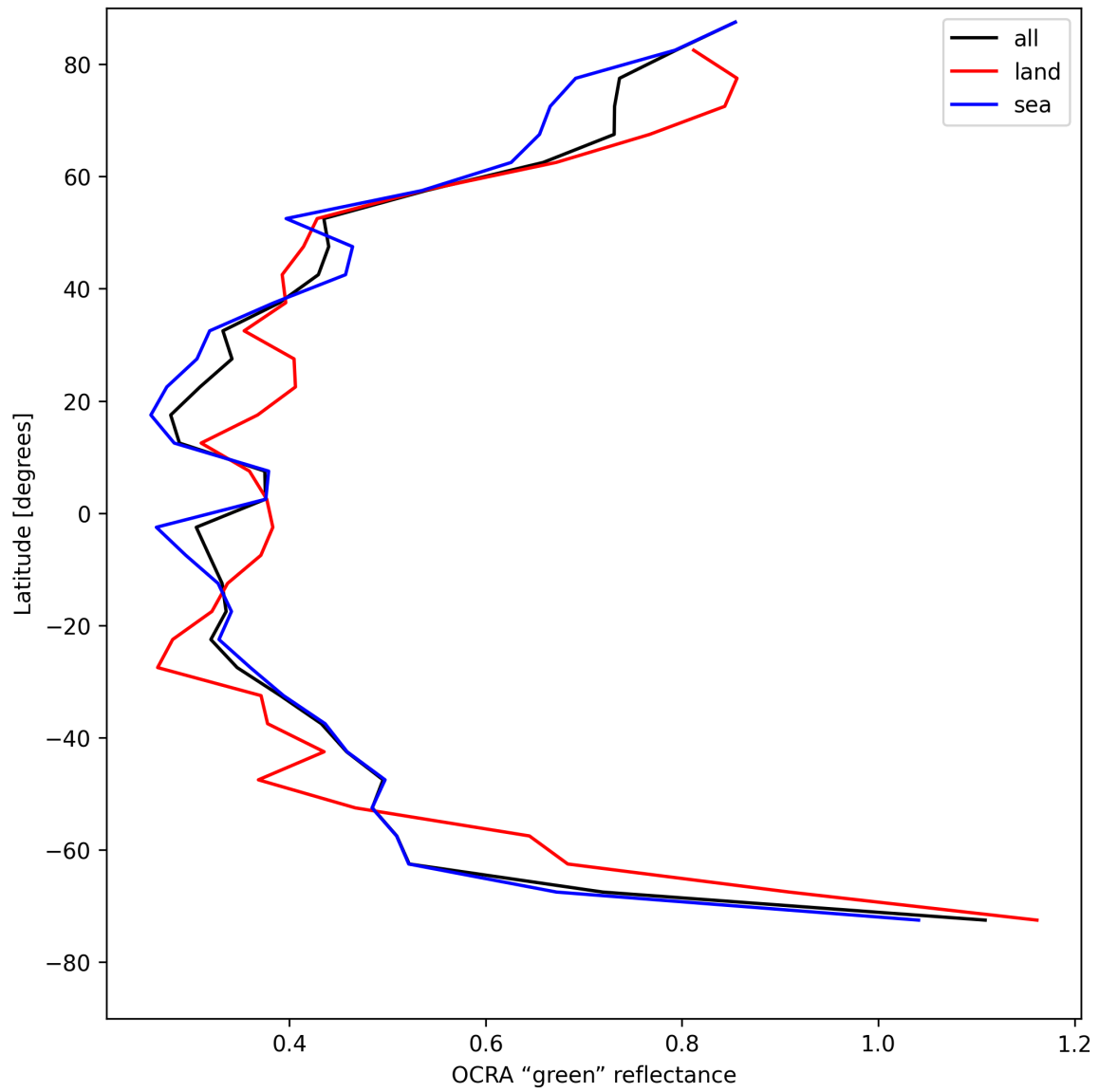
Figure 34: Zonal average of "OCRA "green" reflectance" for 2025-04-30 to 2025-05-01.
