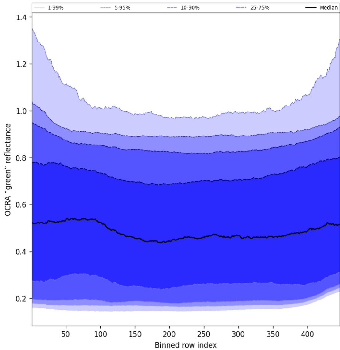
Figure 66: Along track statistics of “OCRA “green” reflectance” for 2025-04-30 to 2025-05-01
