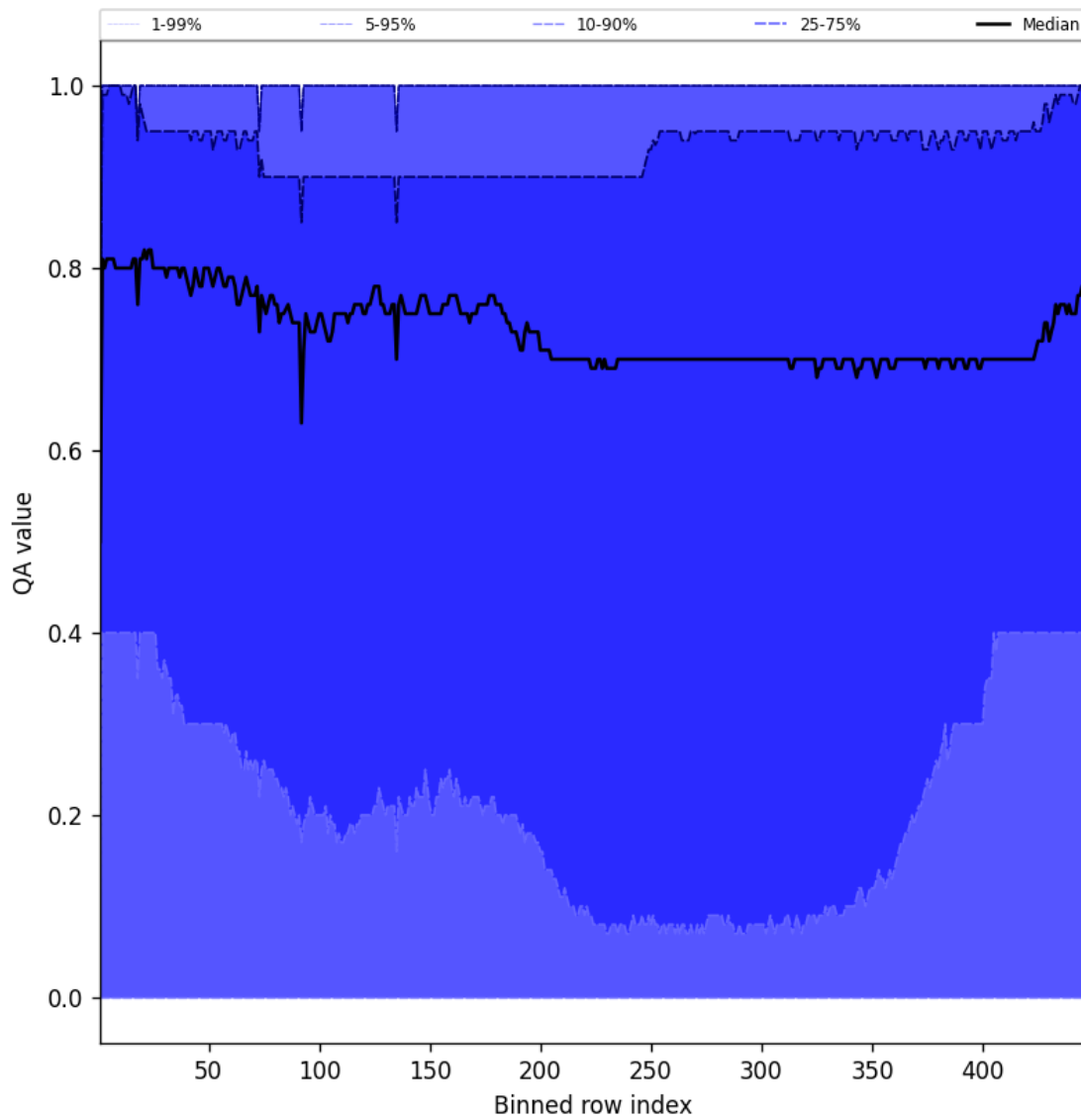
Figure 52: Along track statistics of “QA value” for 2025-04-30 to 2025-05-01
