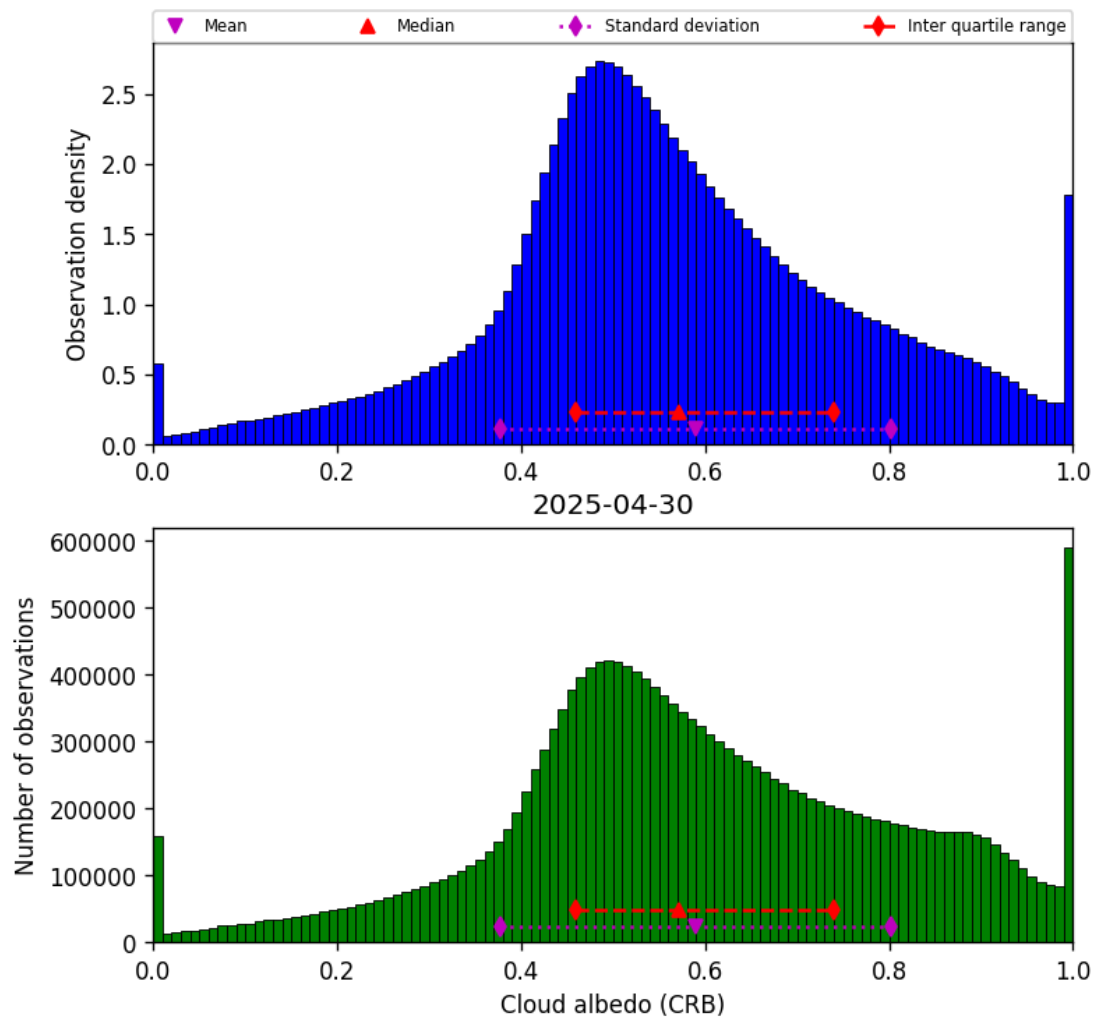
Figure 42: Histogram of “Cloud albedo (CRB)” for 2025-04-30 to 2025-05-01
