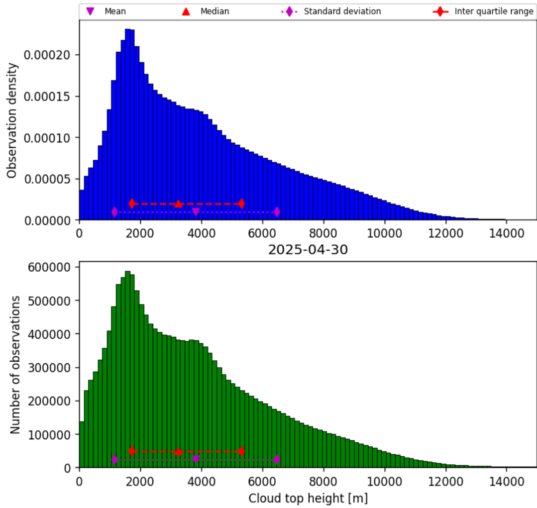
Figure 38: Histogram of “Cloud top height” for 2025-04-30 to 2025-05-01
