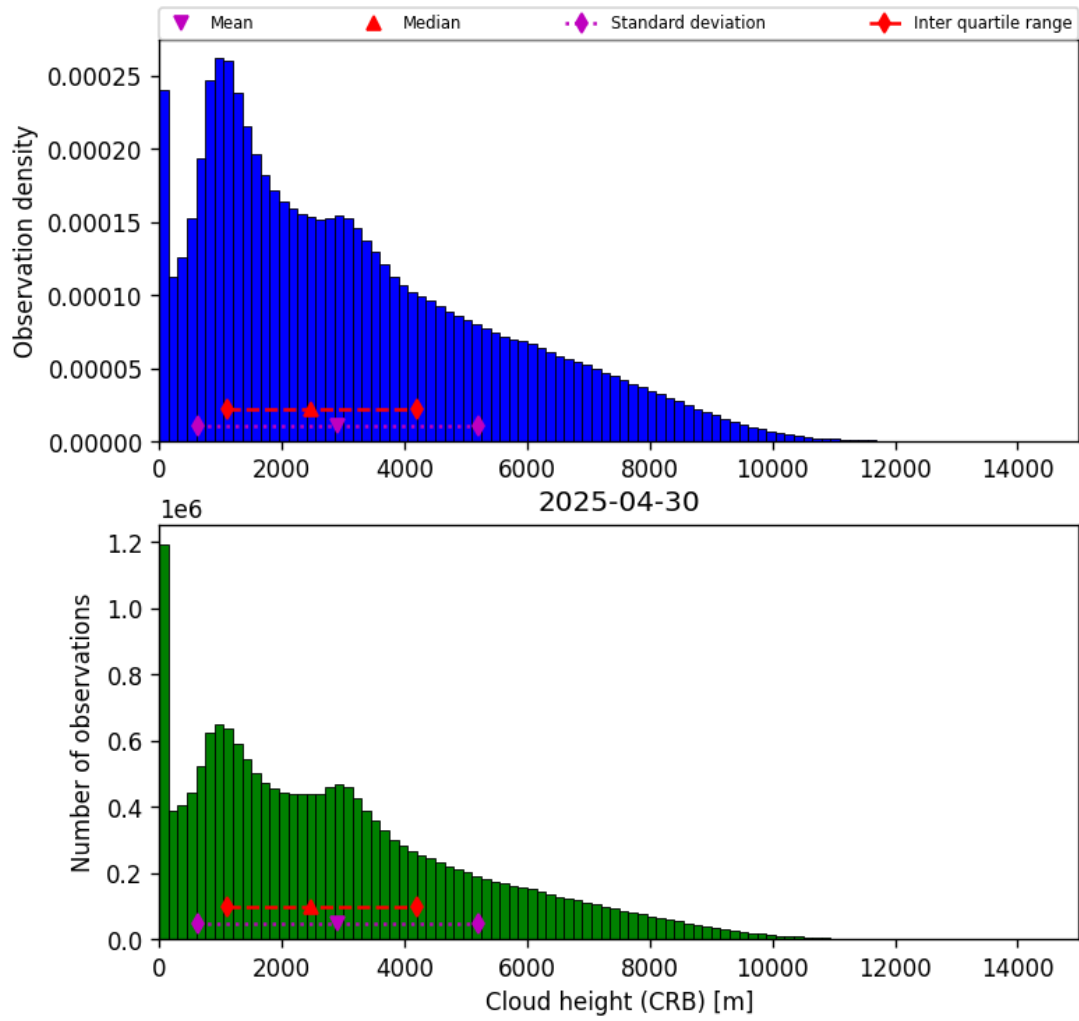
Figure 41: Histogram of “Cloud height (CRB)” for 2025-04-30 to 2025-05-01
