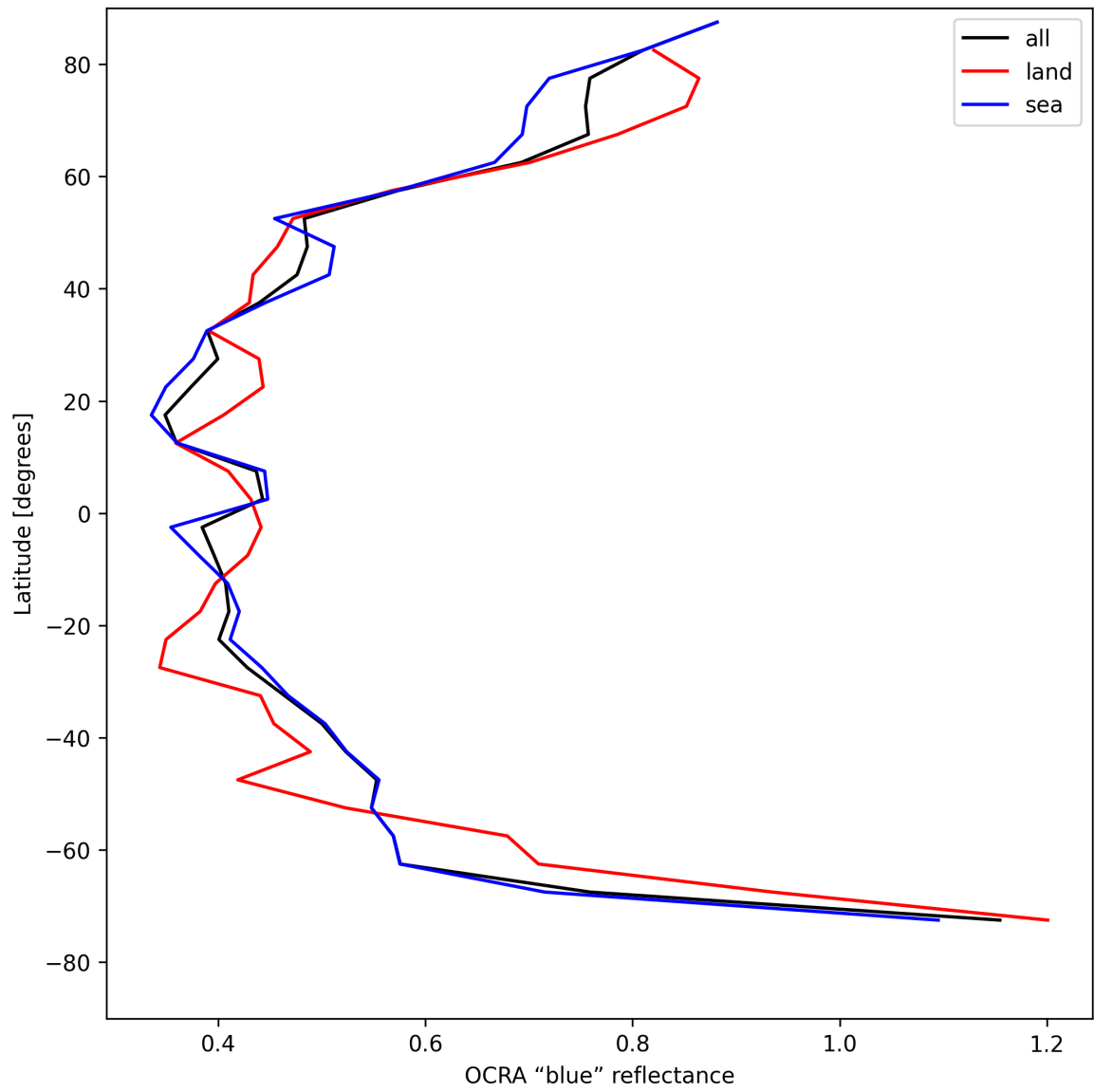
Figure 33: Zonal average of “OCRA “blue” reflectance” for 2025-04-30 to 2025-05-01.
