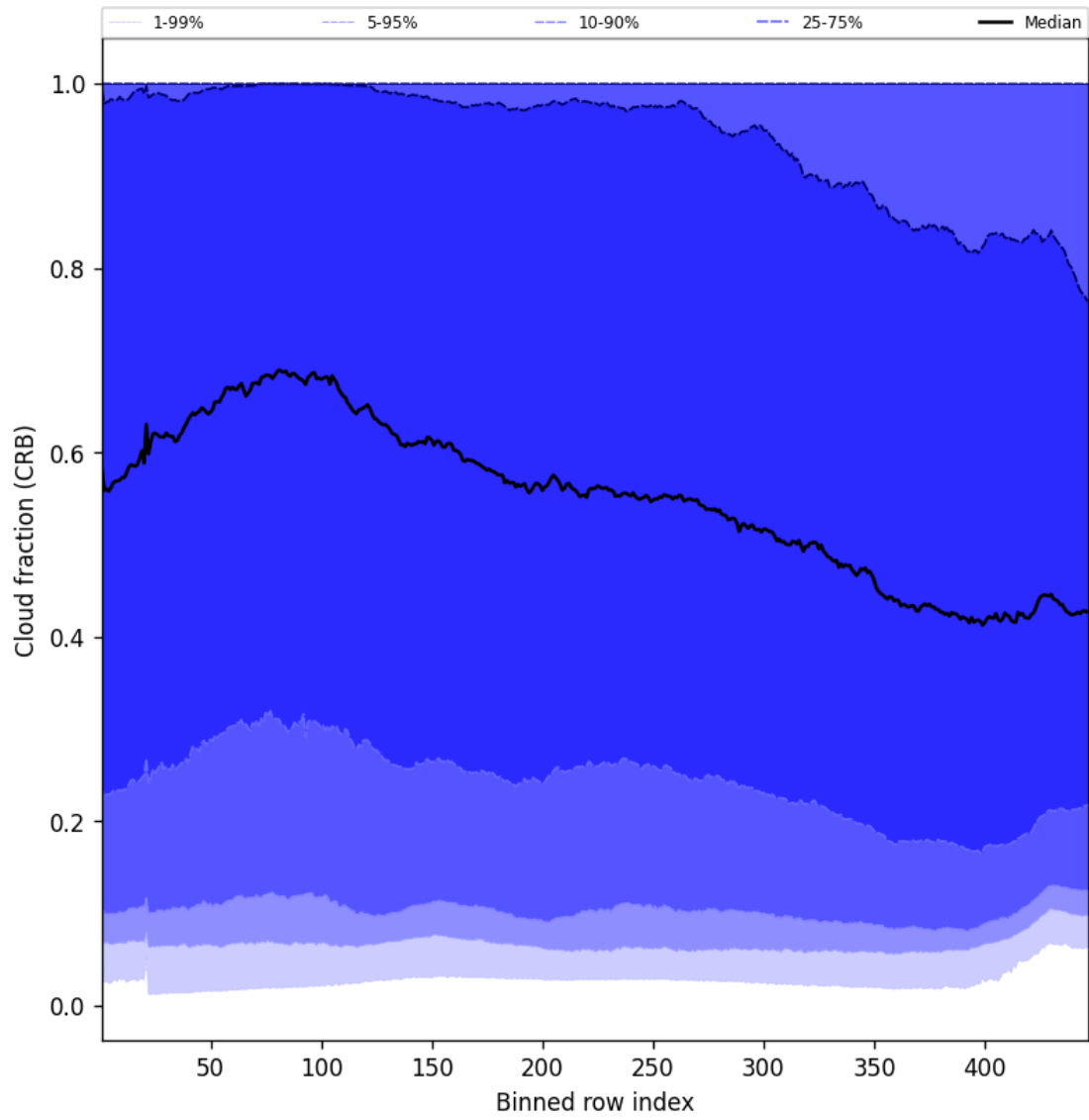
Figure 56: Along track statistics of “Cloud fraction (CRB)” for 2025-04-30 to 2025-05-01
