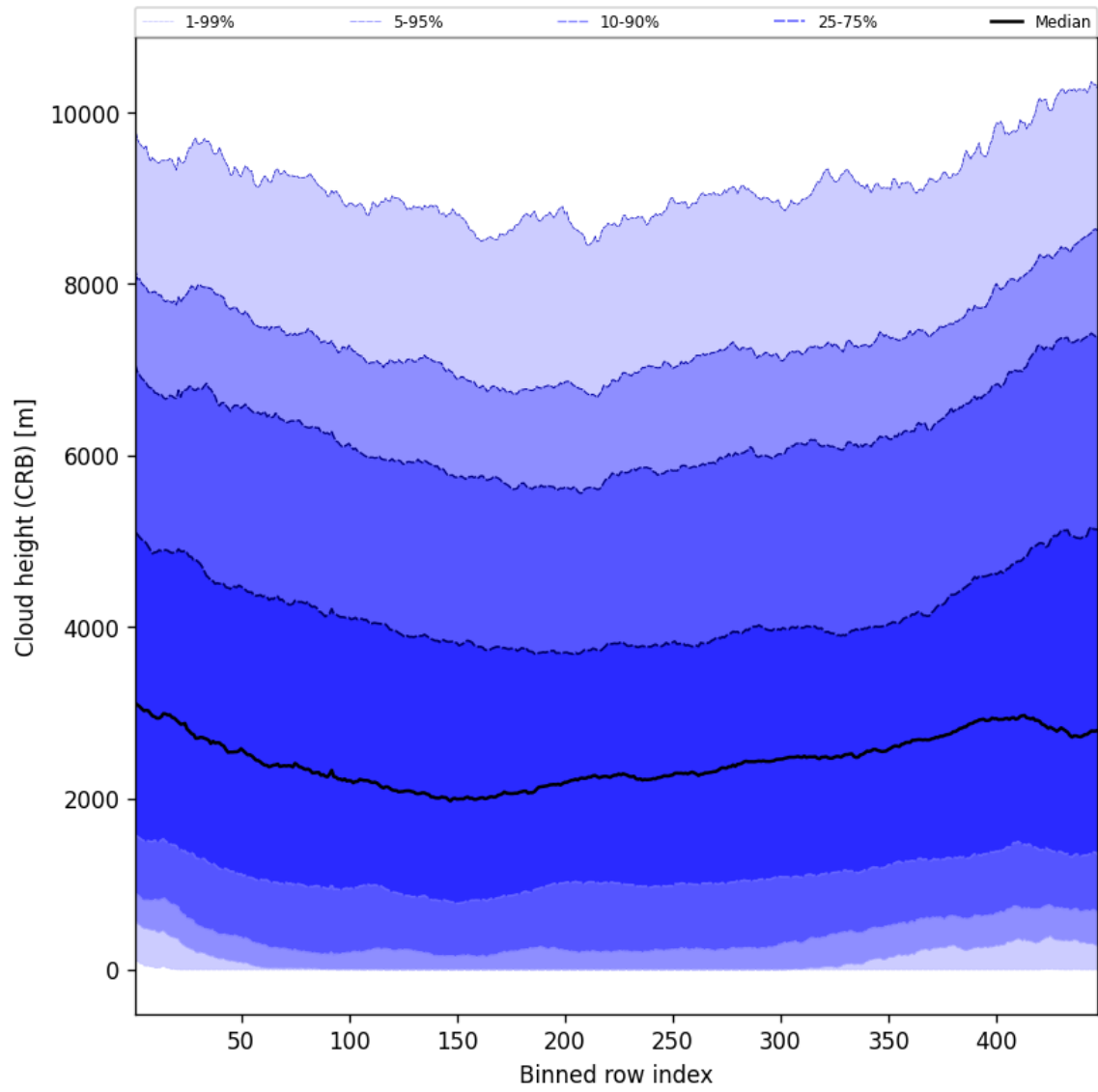
Figure 57: Along track statistics of “Cloud height (CRB)” for 2025-04-30 to 2025-05-01
