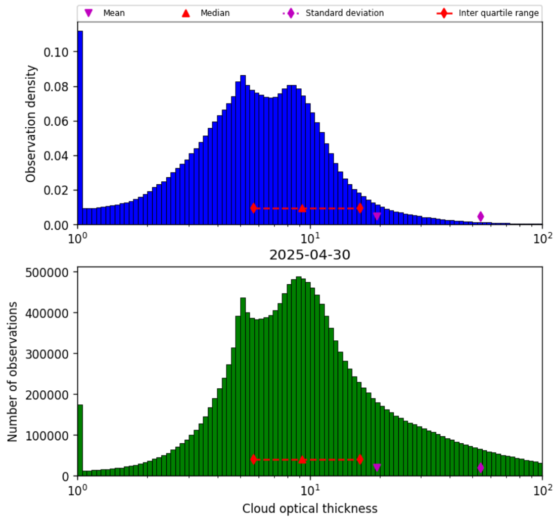
Figure 39: Histogram of “Cloud optical thickness” for 2025-04-30 to 2025-05-01
