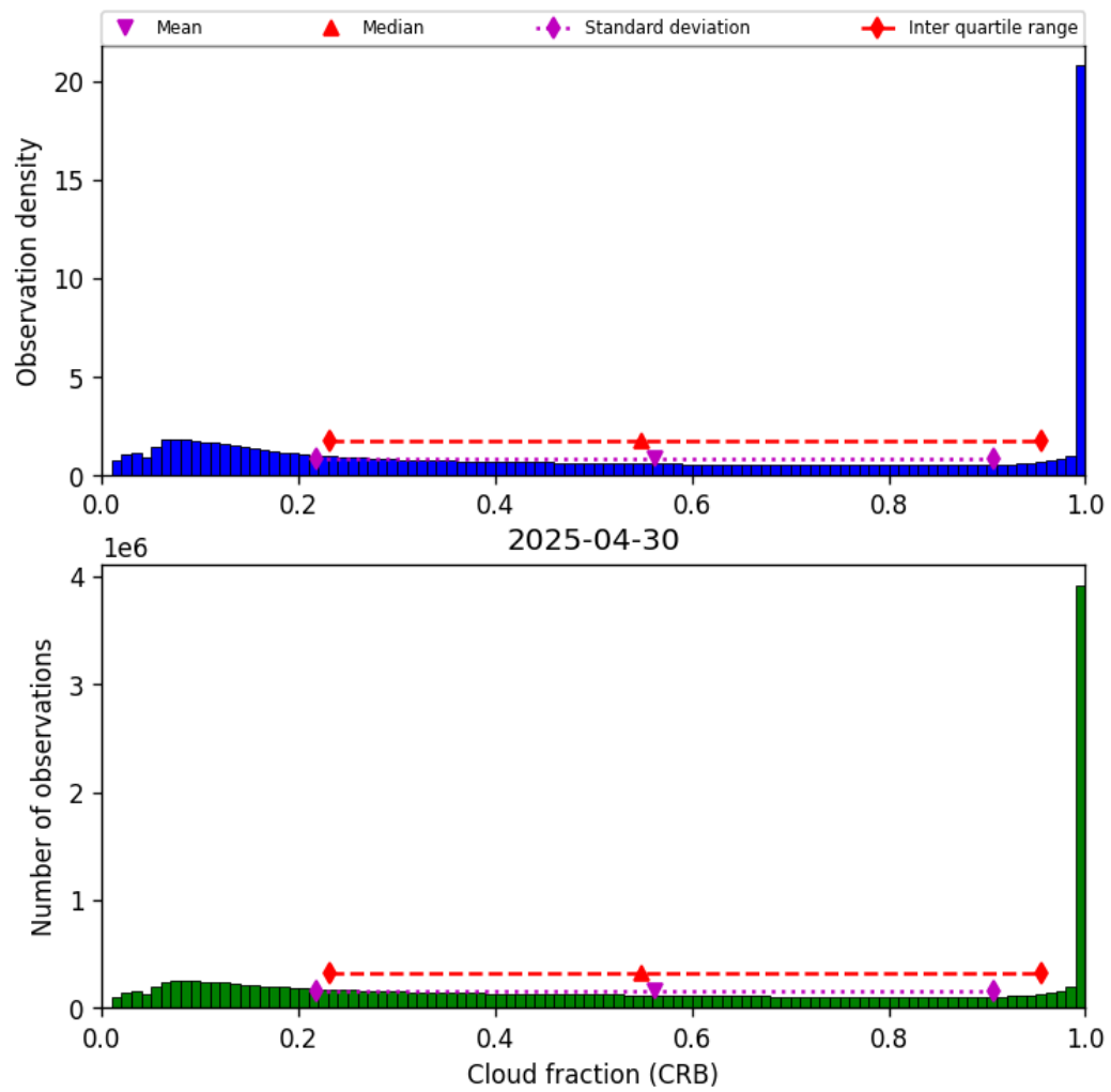
Figure 40: Histogram of “Cloud fraction (CRB)” for 2025-04-30 to 2025-05-01
