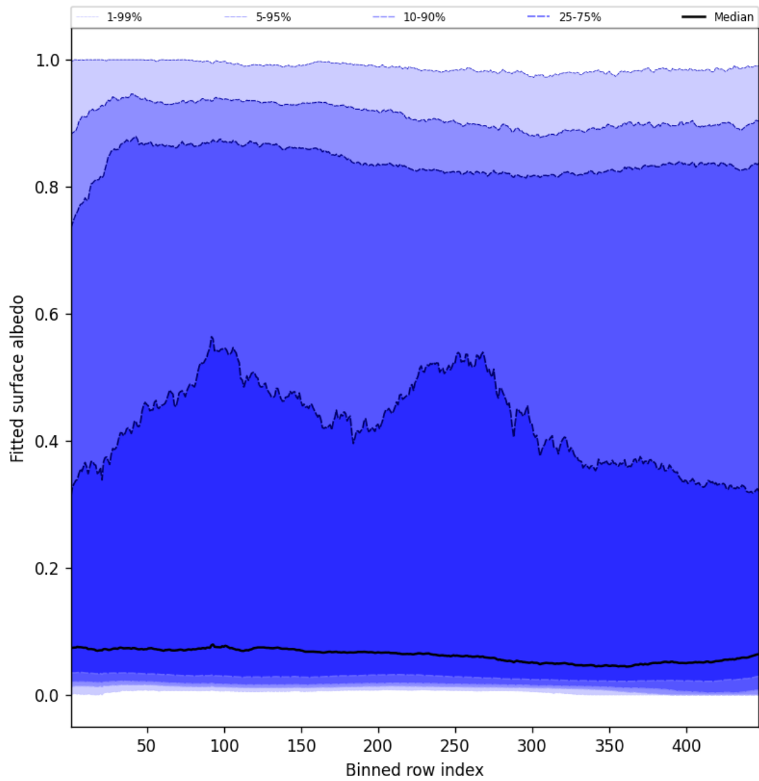
Figure 59: Along track statistics of “Fitted surface albedo” for 2025-04-30 to 2025-05-01
