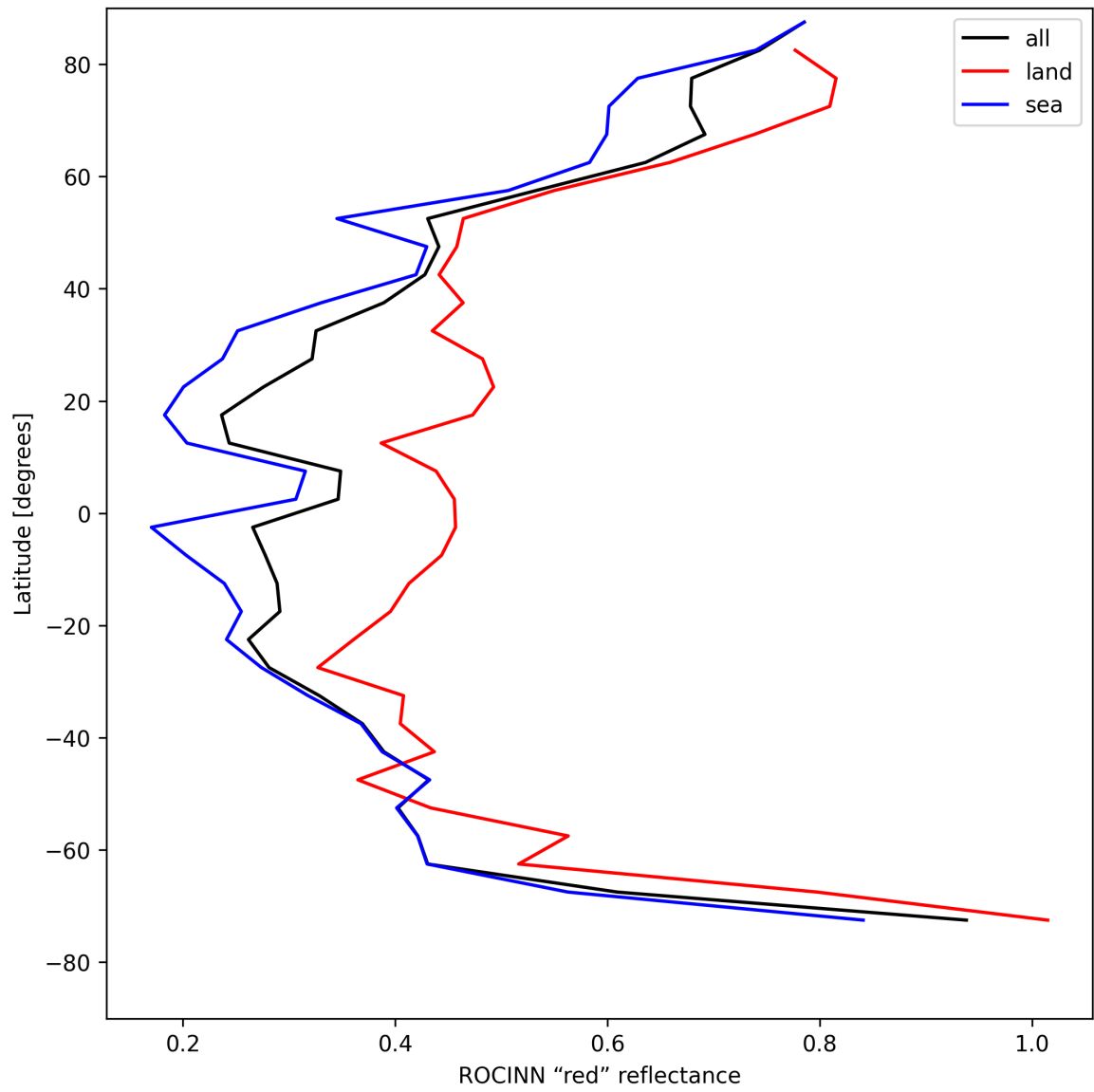
Figure 35: Zonal average of “ROCINN “red” reflectance” for 2025-04-30 to 2025-05-01.
