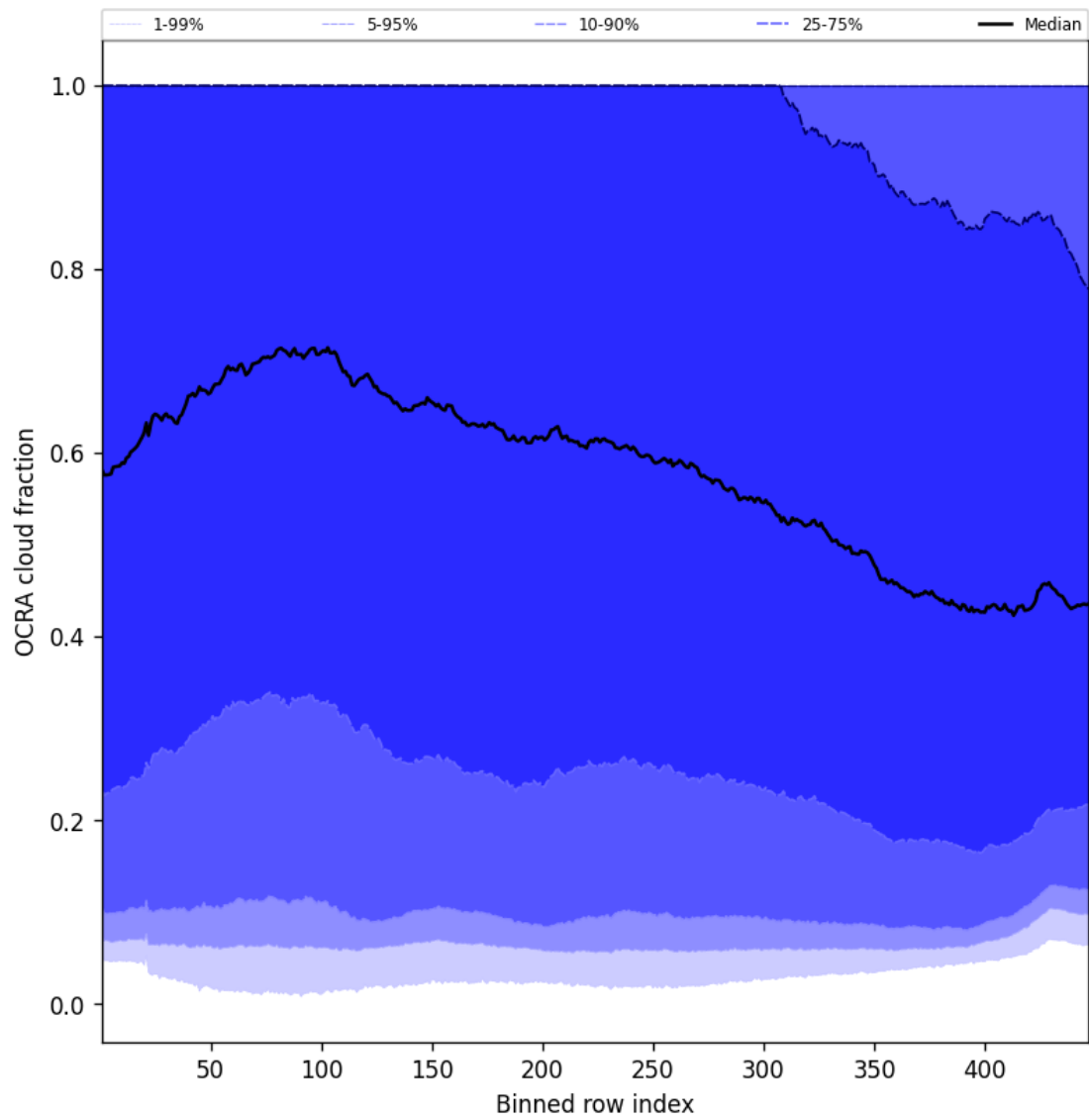
Figure 64: Along track statistics of “OCRA cloud fraction” for 2025-04-30 to 2025-05-01
