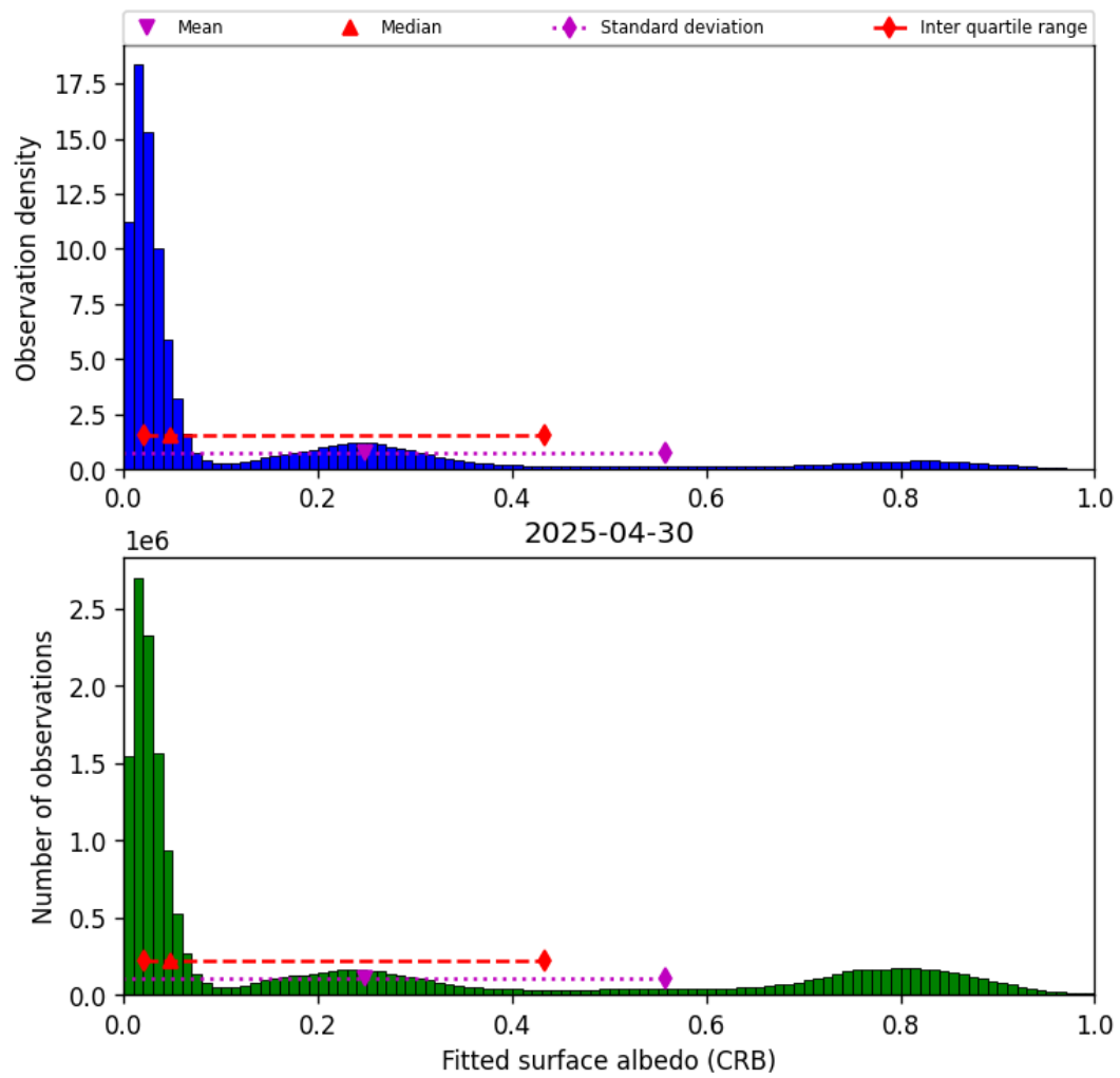
Figure 44: Histogram of “Fitted surface albedo (CRB)” for 2025-04-30 to 2025-05-01
