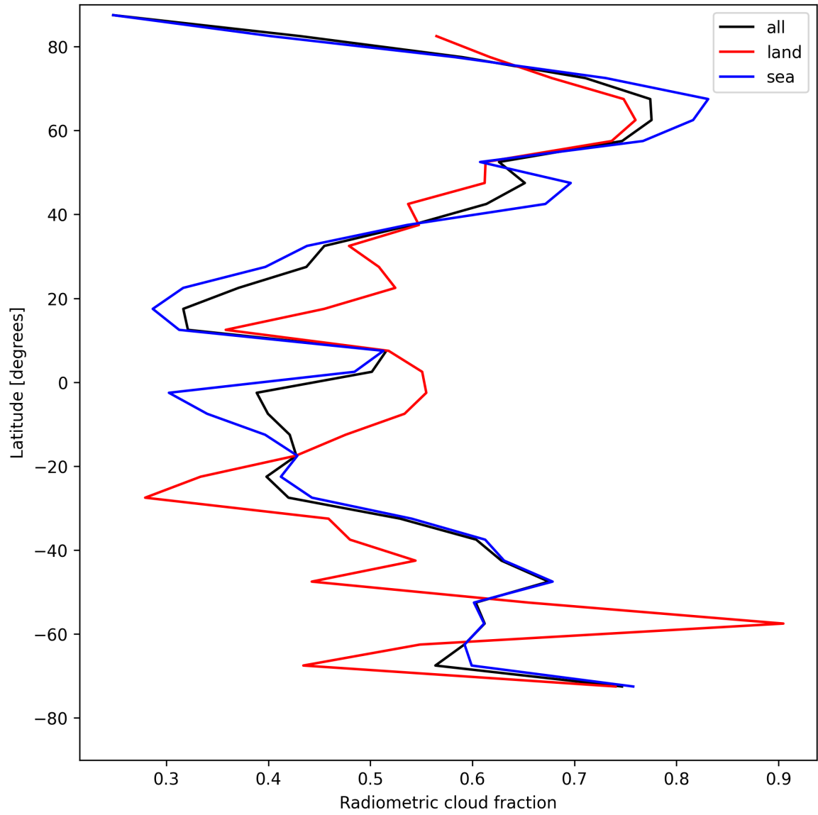
Figure 21: Zonal average of “Radiometric cloud fraction” for 2025-04-30 to 2025-05-01.
