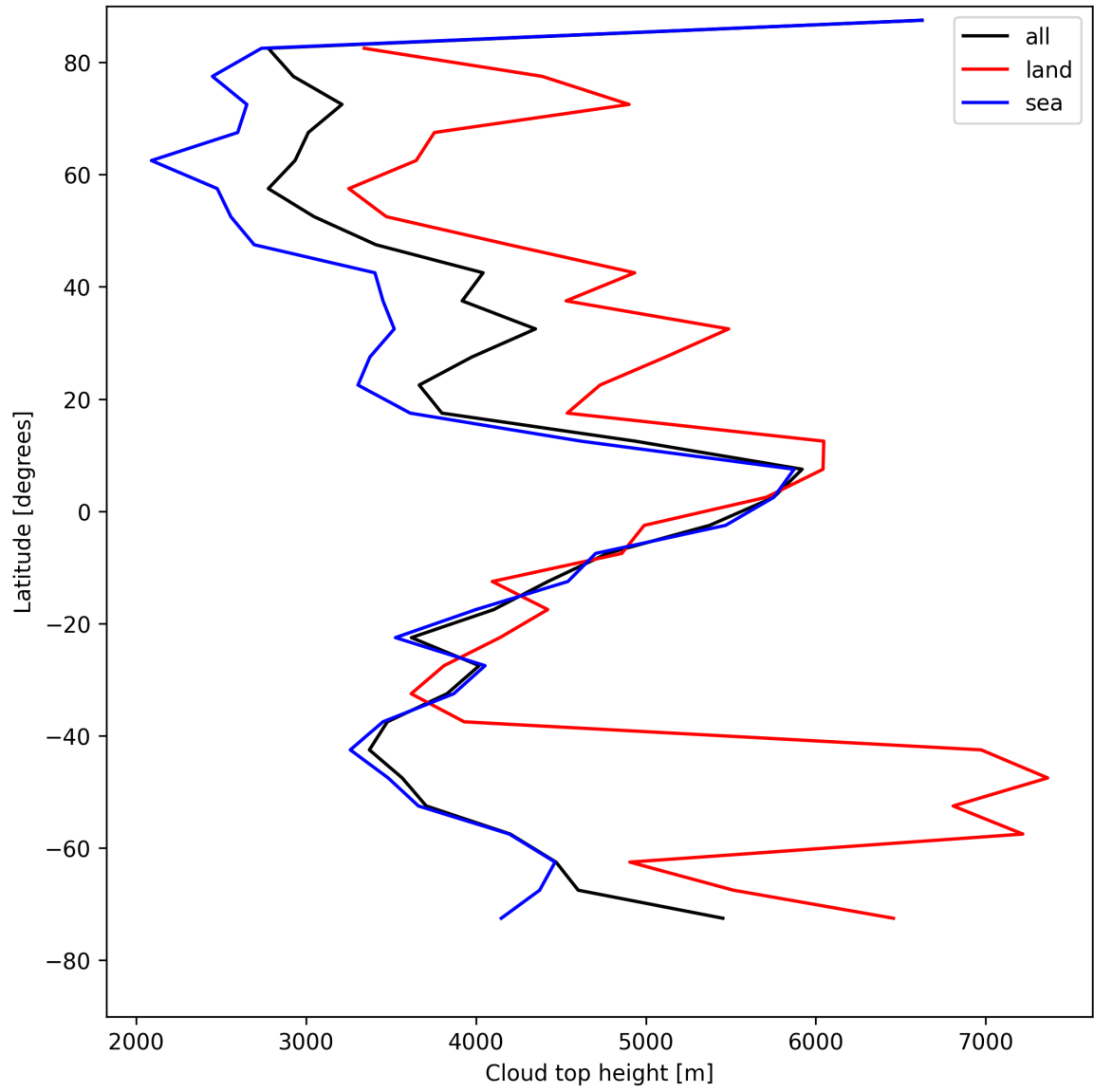
Figure 22: Zonal average of “Cloud top height” for 2025-04-30 to 2025-05-01.
