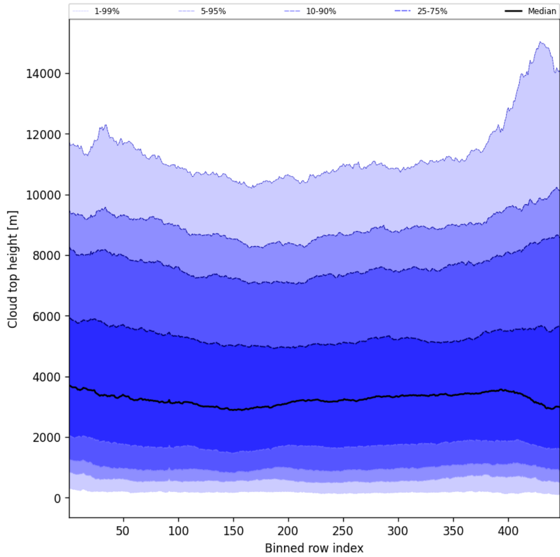
Figure 54: Along track statistics of “Cloud top height” for 2025-04-30 to 2025-05-01
