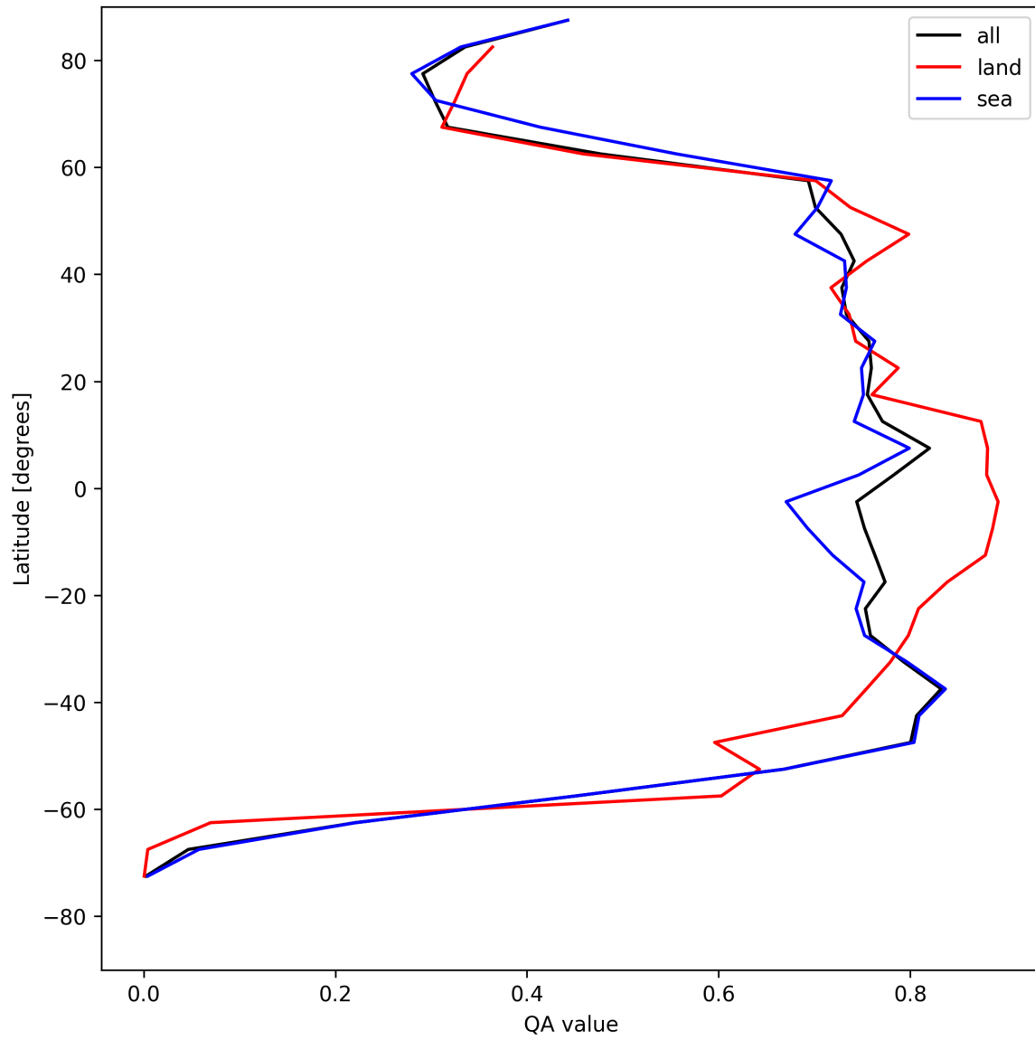
Figure 20: Zonal average of “QA value” for 2025-04-30 to 2025-05-01.
