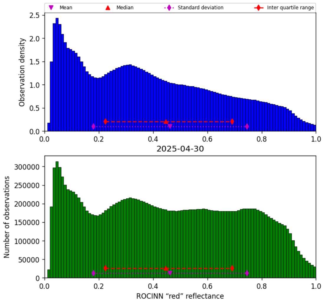
Figure 51: Histogram of “ROCINN “red” reflectance” for 2025-04-30 to 2025-05-01
