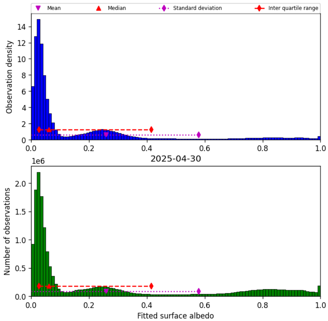
Figure 43: Histogram of “Fitted surface albedo” for 2025-04-30 to 2025-05-01
