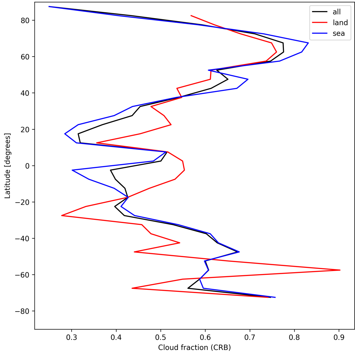
Figure 24: Zonal average of “Cloud fraction (CRB)” for 2025-04-30 to 2025-05-01.
