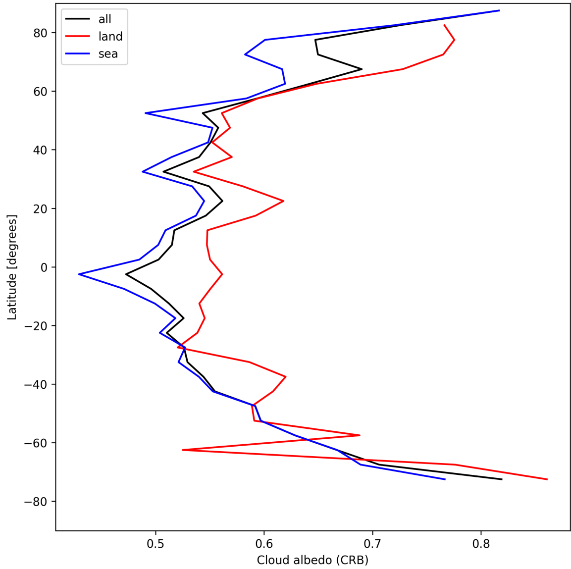
Figure 26: Zonal average of “Cloud albedo (CRB)” for 2025-04-30 to 2025-05-01.
