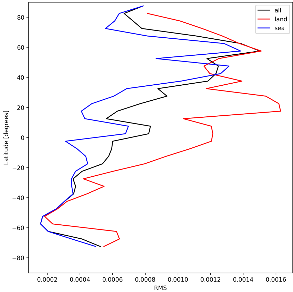
Figure 29: Zonal average of “RMS” for 2025-04-30 to 2025-05-01.
