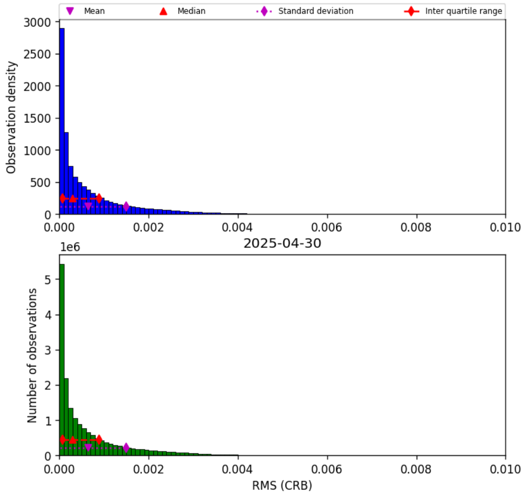
Figure 46: Histogram of “RMS (CRB)” for 2025-04-30 to 2025-05-01
