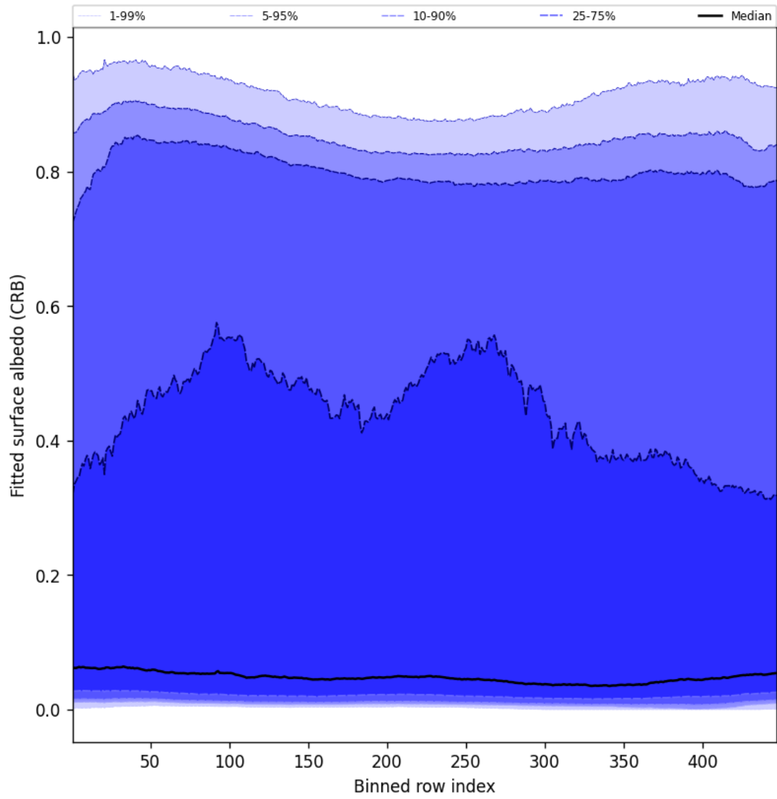
Figure 60: Along track statistics of “Fitted surface albedo (CRB)” for 2025-04-30 to 2025-05-01
