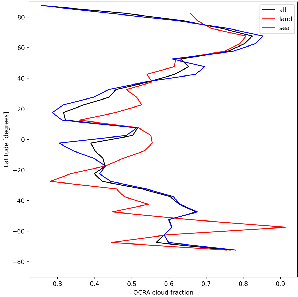
Figure 32: Zonal average of “OCRA cloud fraction” for 2025-04-30 to 2025-05-01.
