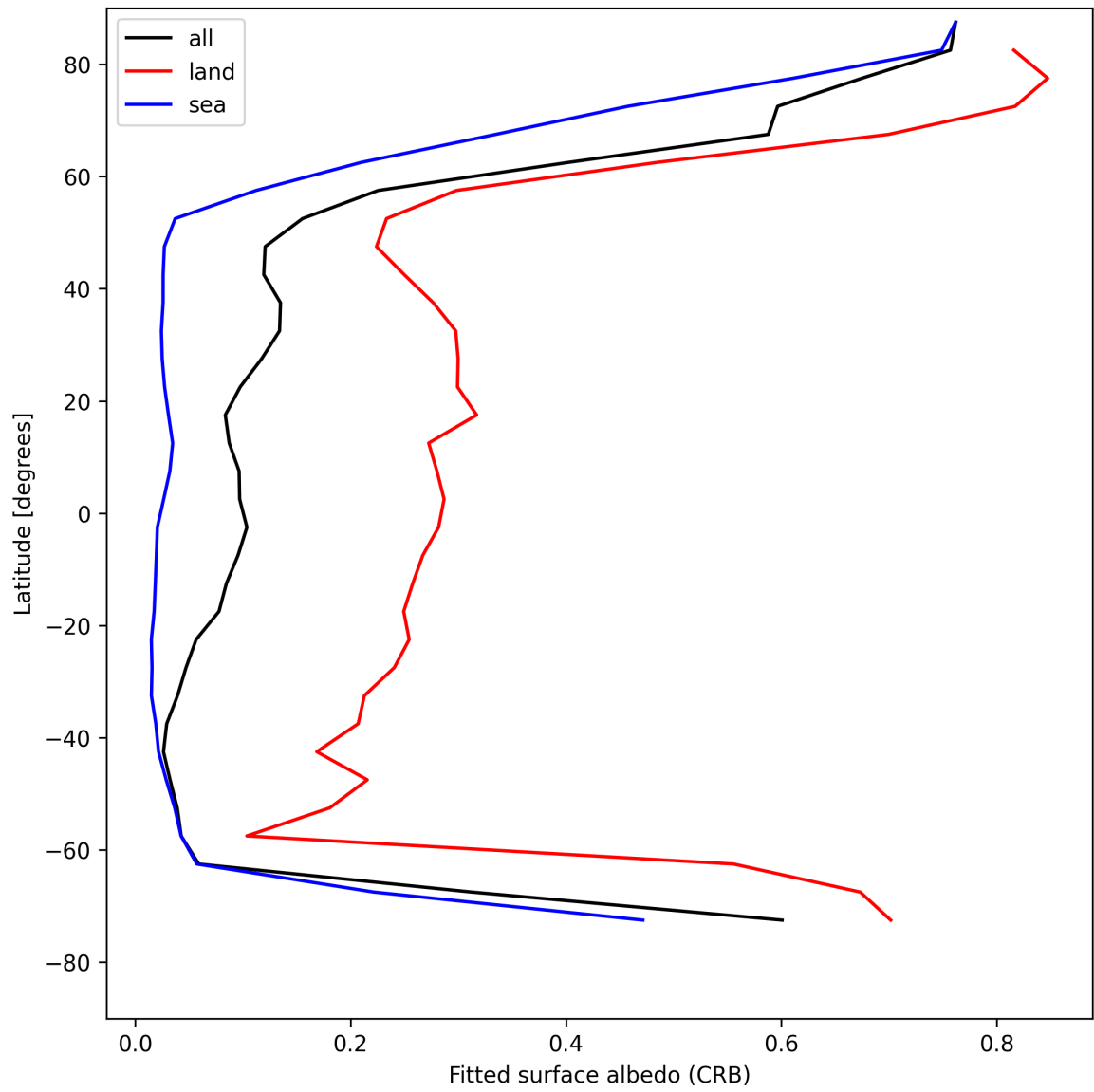
Figure 28: Zonal average of “Fitted surface albedo (CRB)” for 2025-04-30 to 2025-05-01.
