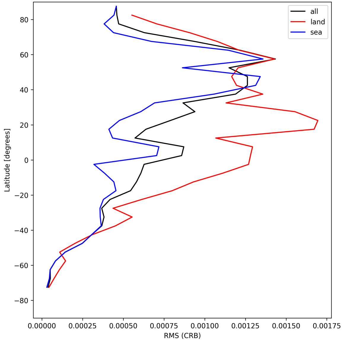
Figure 30: Zonal average of “RMS (CRB)” for 2025-04-30 to 2025-05-01.
