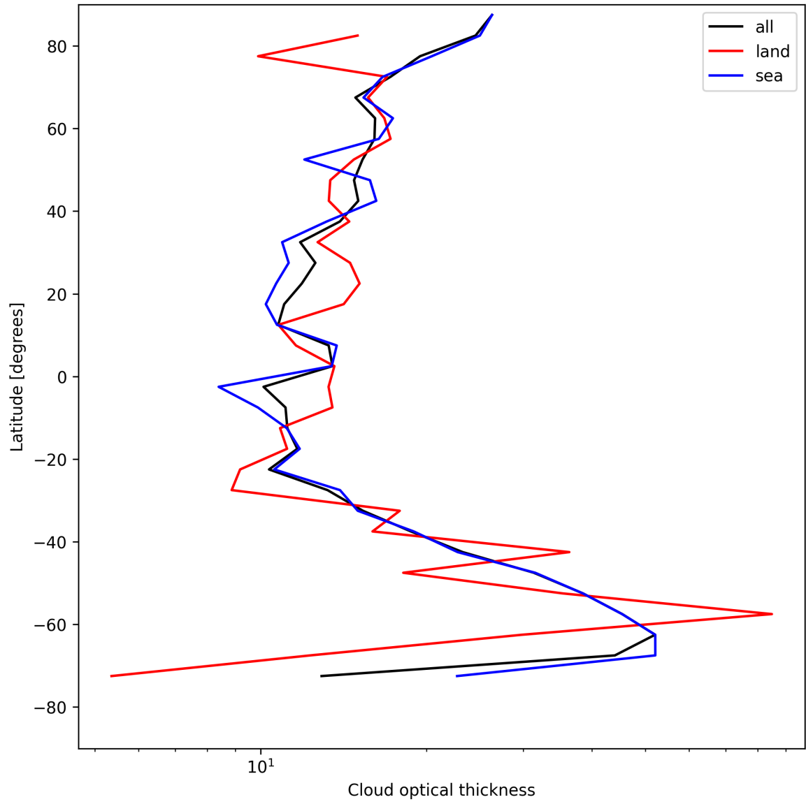
Figure 23: Zonal average of “Cloud optical thickness” for 2025-04-30 to 2025-05-01.
