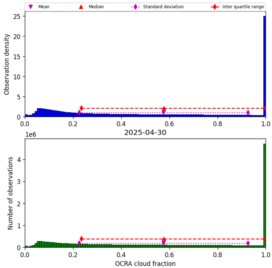
Figure 48: Histogram of “OCRA cloud fraction” for 2025-04-30 to 2025-05-01
