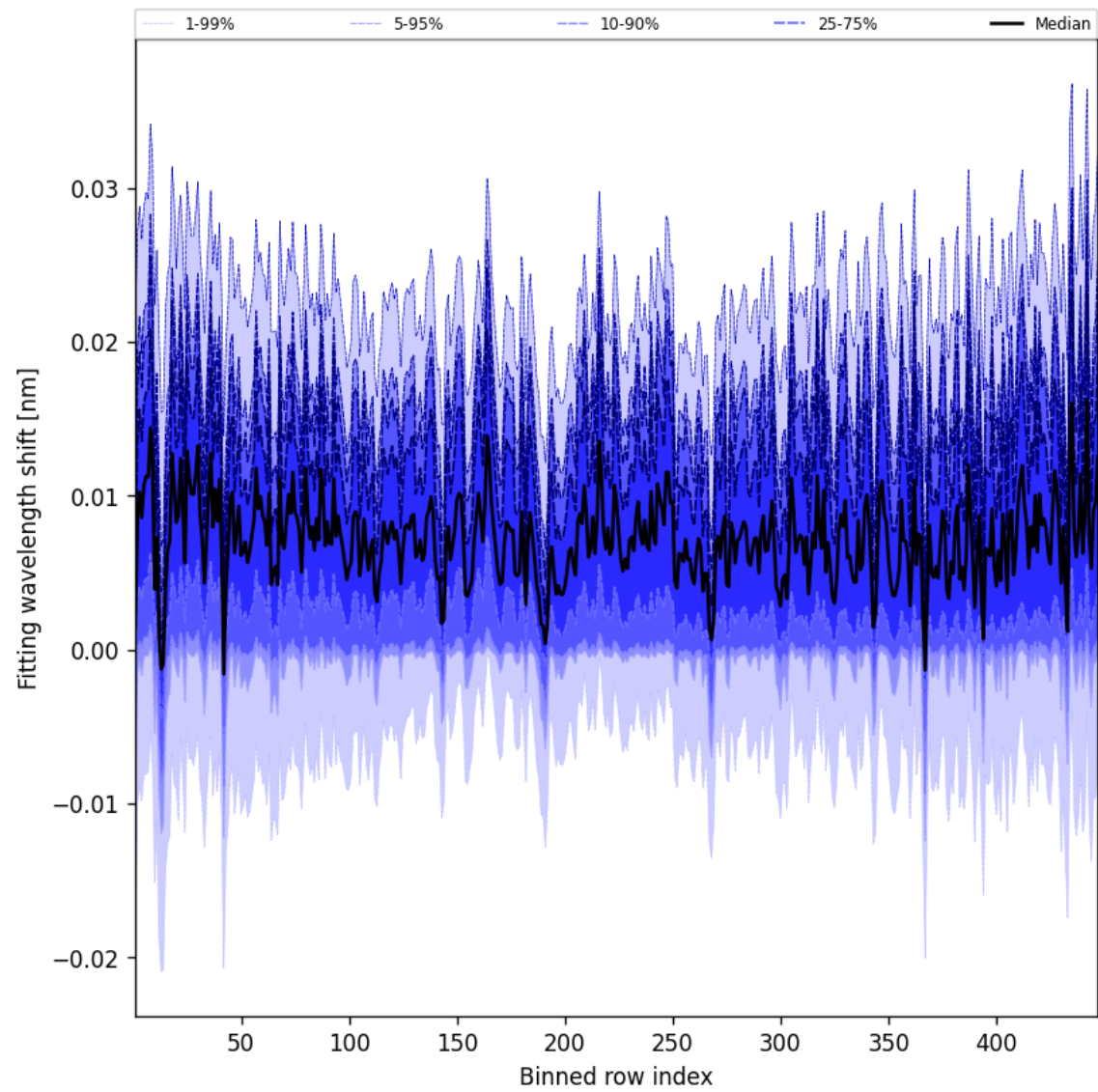
Figure 63: Along track statistics of “Fitting wavelength shift” for 2025-04-30 to 2025-05-01
