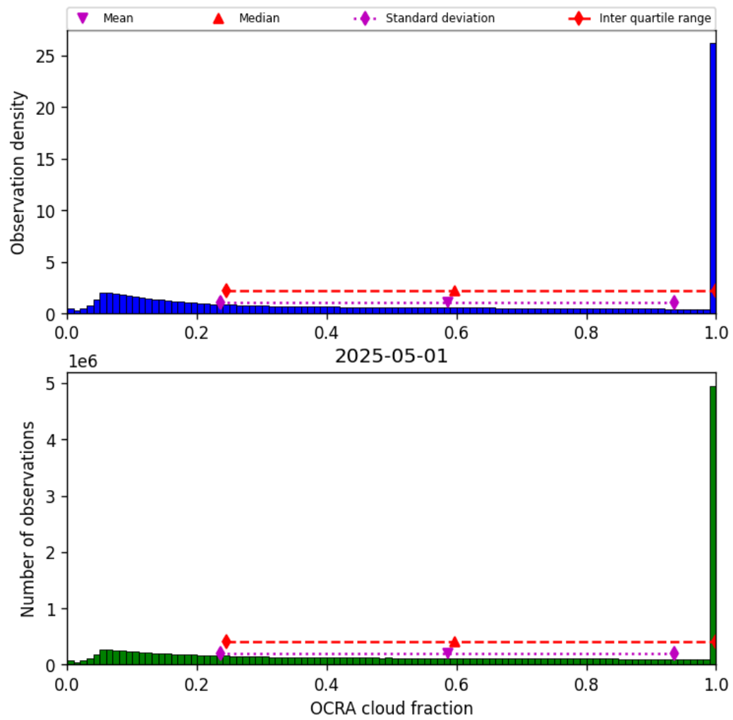
Figure 48: Histogram of “OCRA cloud fraction” for 2025-05-01 to 2025-05-02
