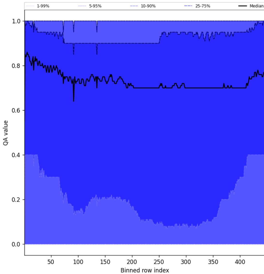
Figure 52: Along track statistics of “QA value” for 2025-05-01 to 2025-05-02
