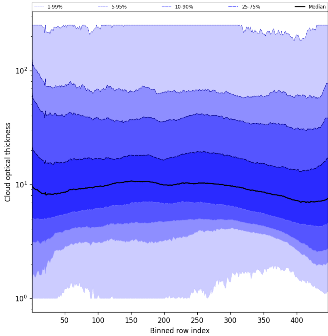
Figure 55: Along track statistics of “Cloud optical thickness” for 2025-05-01 to 2025-05-02
