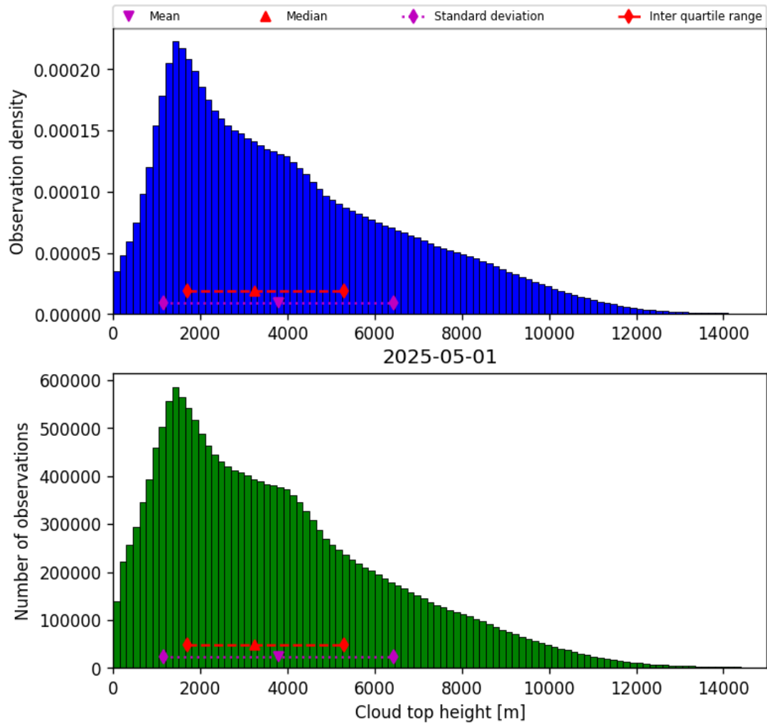
Figure 38: Histogram of “Cloud top height” for 2025-05-01 to 2025-05-02
