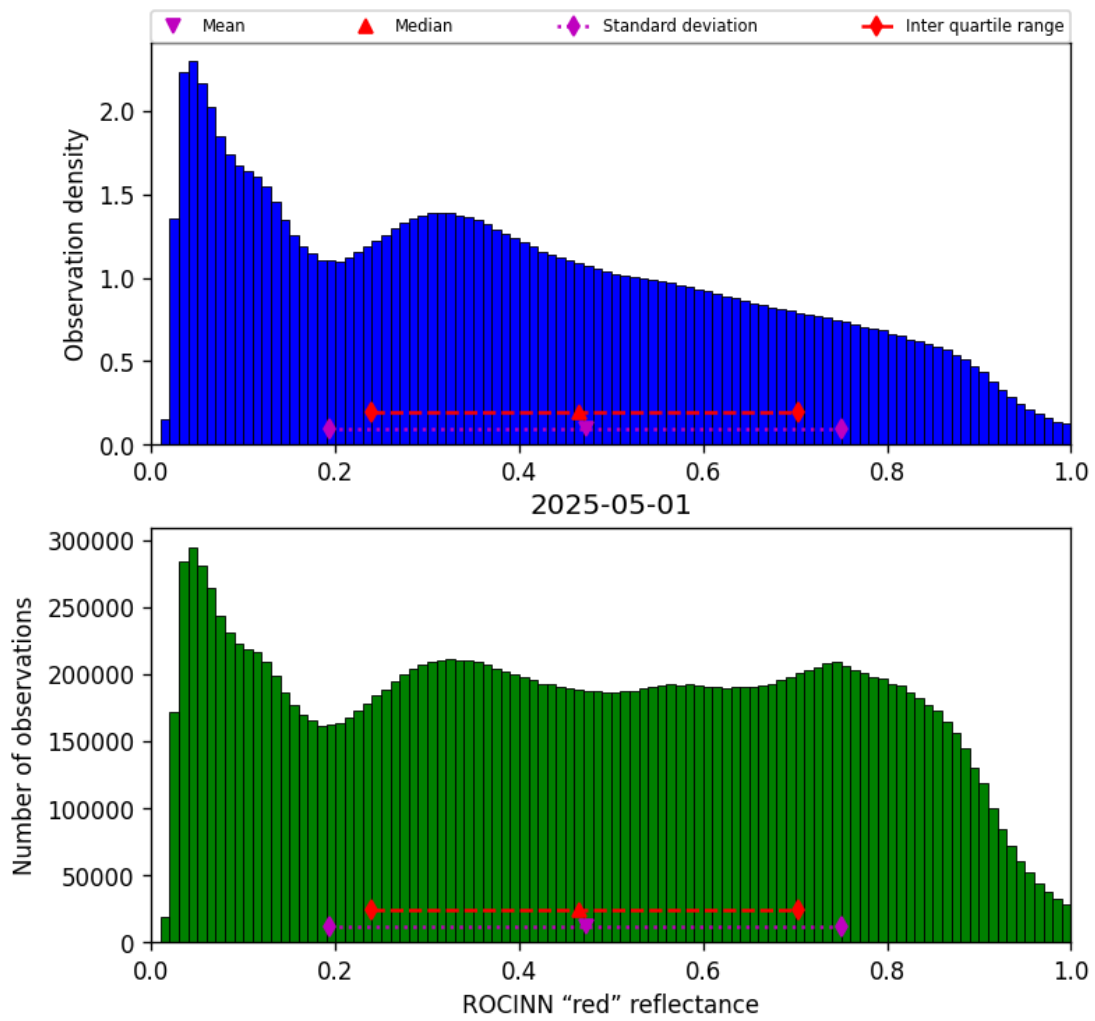
Figure 51: Histogram of “ROCINN “red” reflectance” for 2025-05-01 to 2025-05-02
