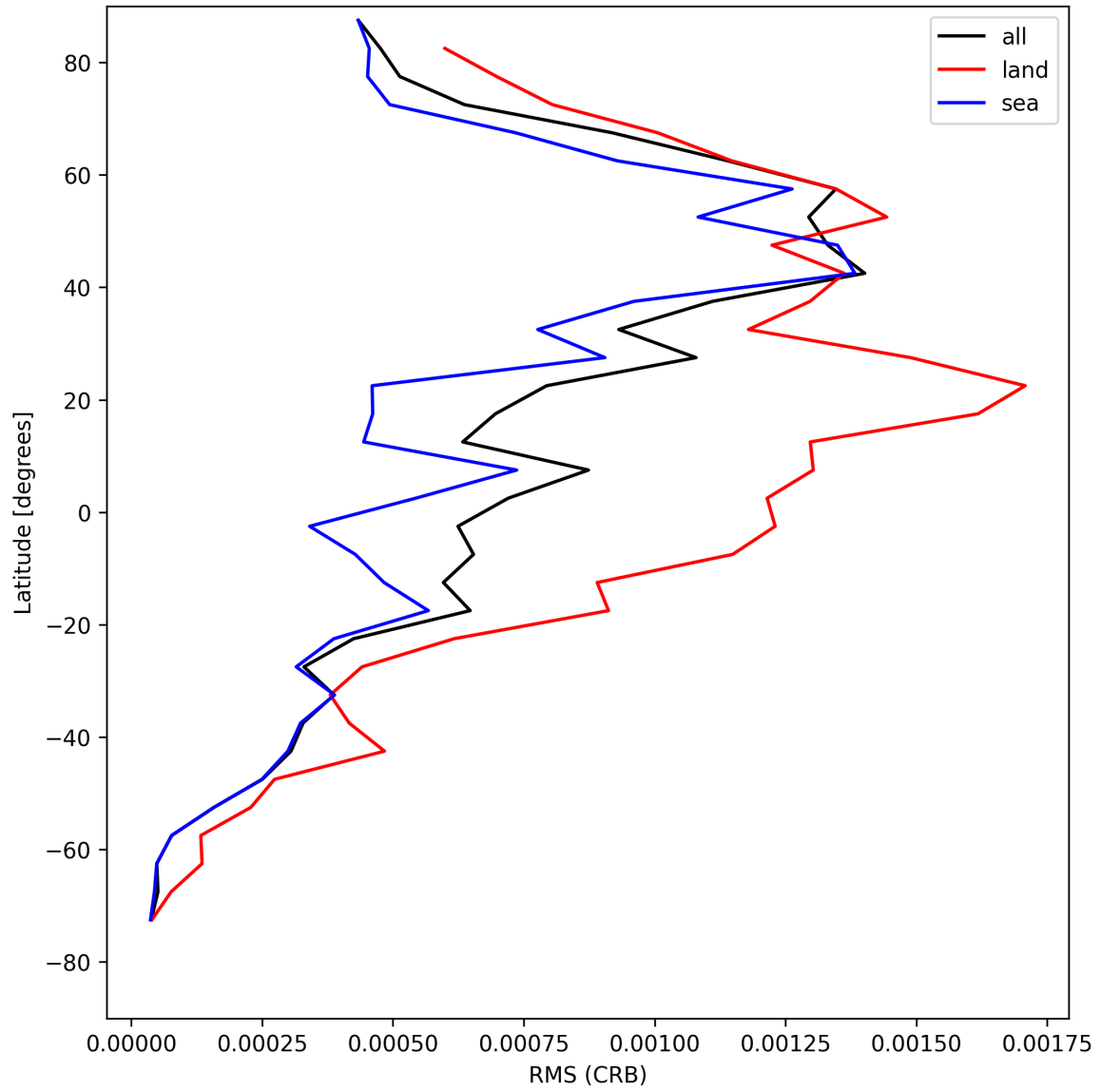
Figure 30: Zonal average of “RMS (CRB)” for 2025-05-01 to 2025-05-02.
