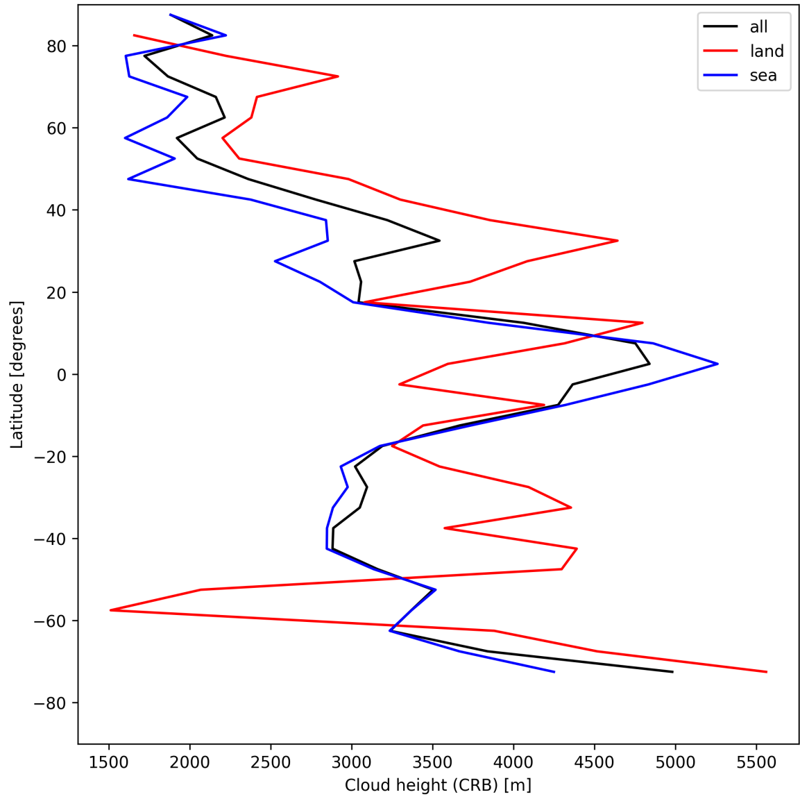
Figure 25: Zonal average of “Cloud height (CRB)” for 2025-05-01 to 2025-05-02.
