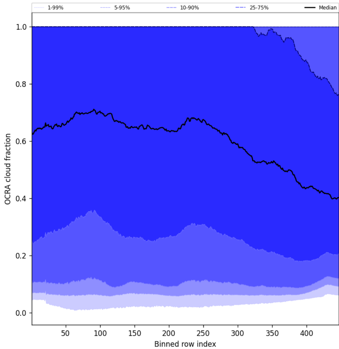
Figure 64: Along track statistics of “OCRA cloud fraction” for 2025-05-01 to 2025-05-02
