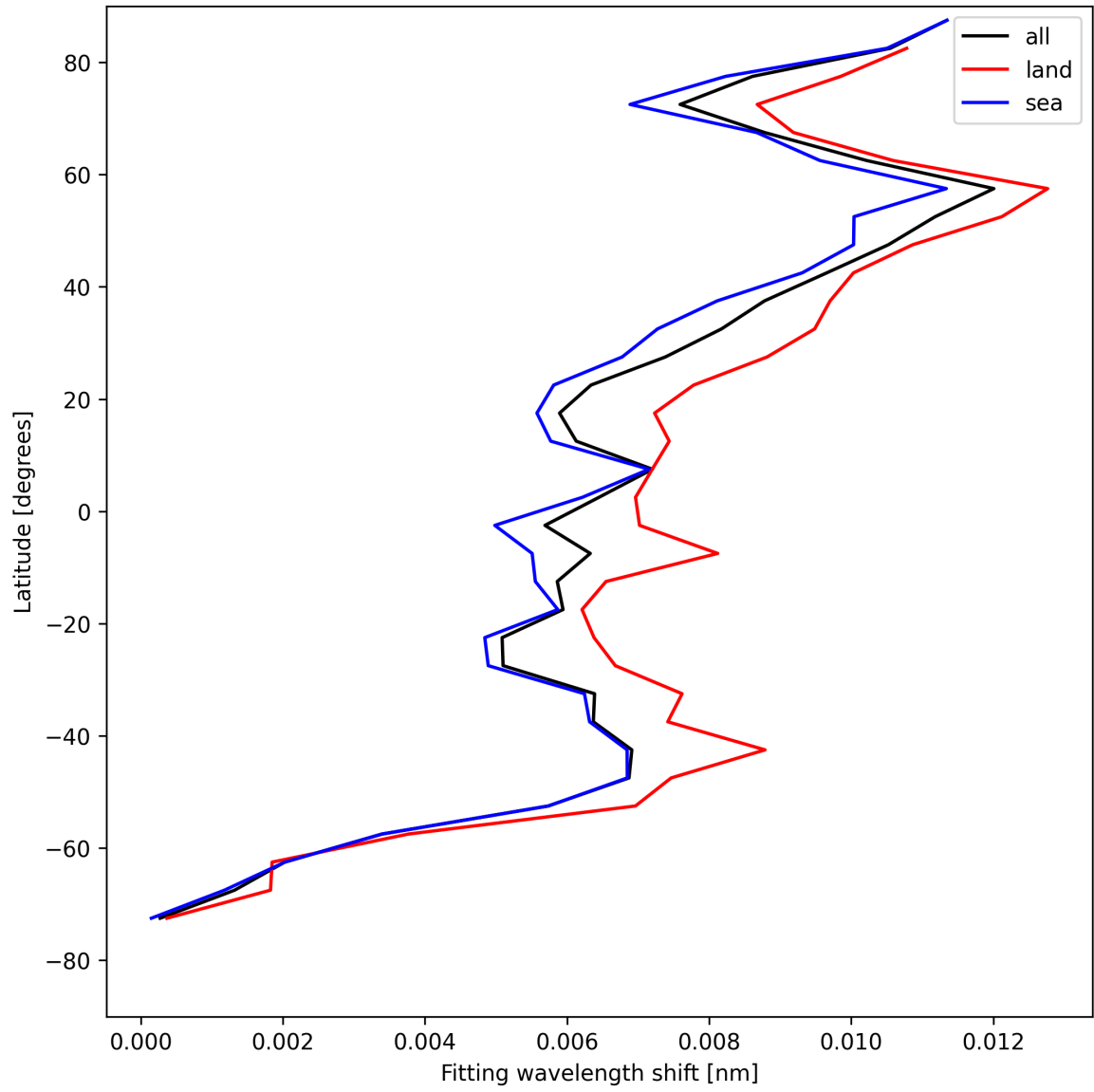
Figure 31: Zonal average of “Fitting wavelength shift” for 2025-05-01 to 2025-05-02.
