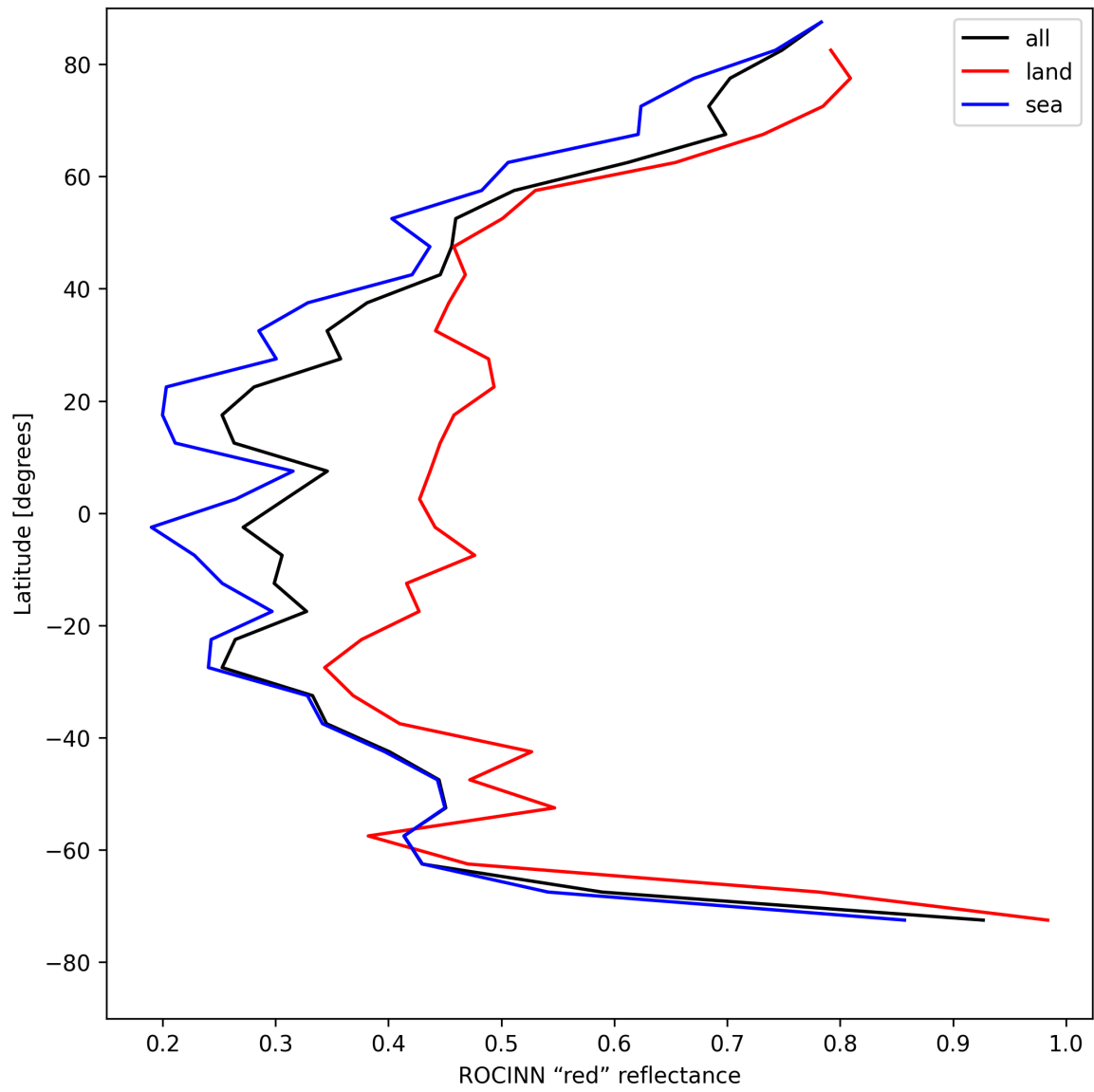
Figure 35: Zonal average of “ROCINN “red” reflectance” for 2025-05-01 to 2025-05-02.
