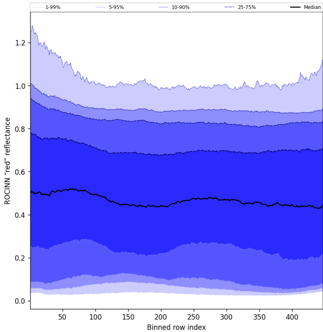
Figure 67: Along track statistics of “ROCINN “red” reflectance” for 2025-05-01 to 2025-05-02
