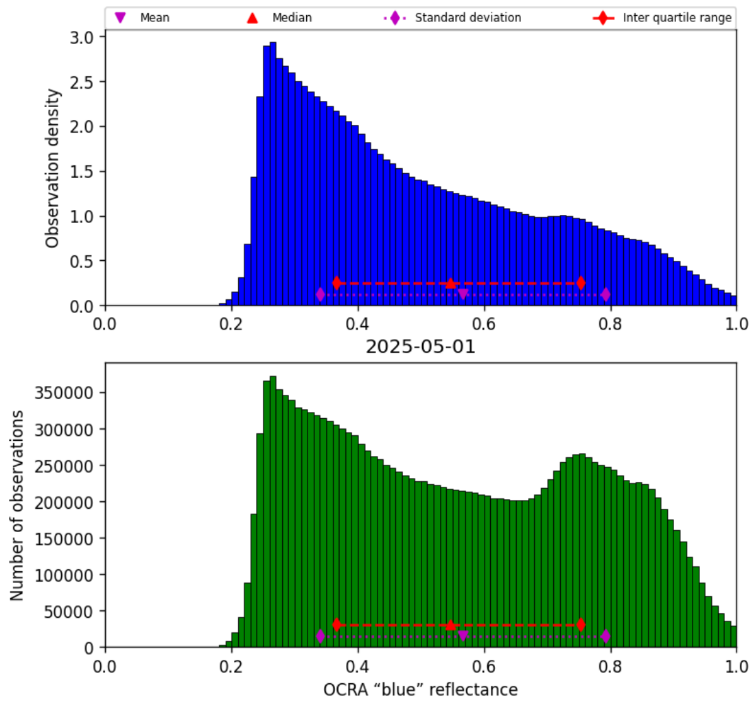
Figure 49: Histogram of “OCRA “blue” reflectance” for 2025-05-01 to 2025-05-02
