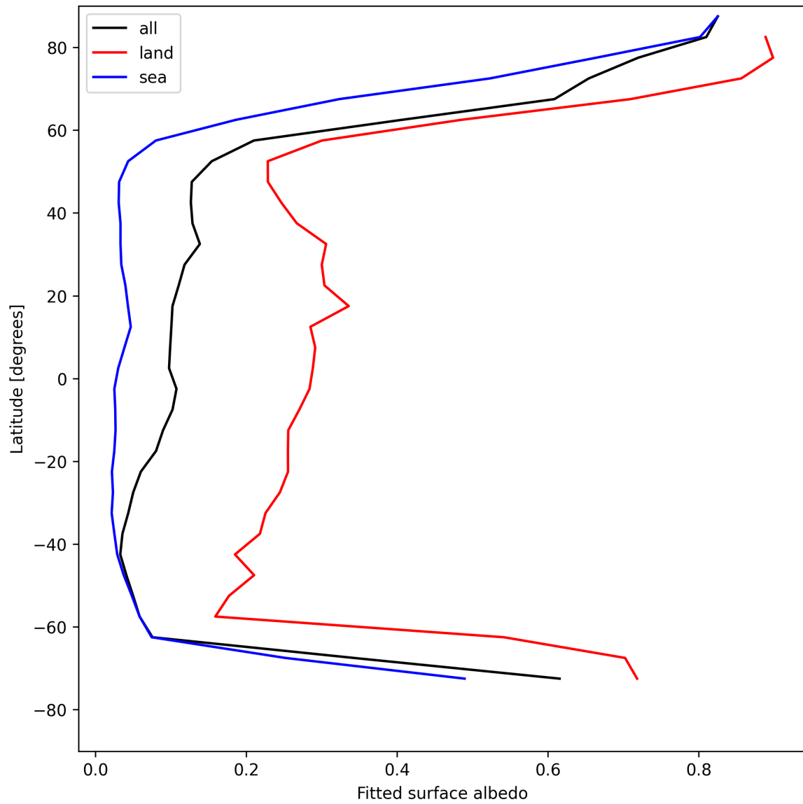
Figure 27: Zonal average of “Fitted surface albedo” for 2025-05-01 to 2025-05-02.
