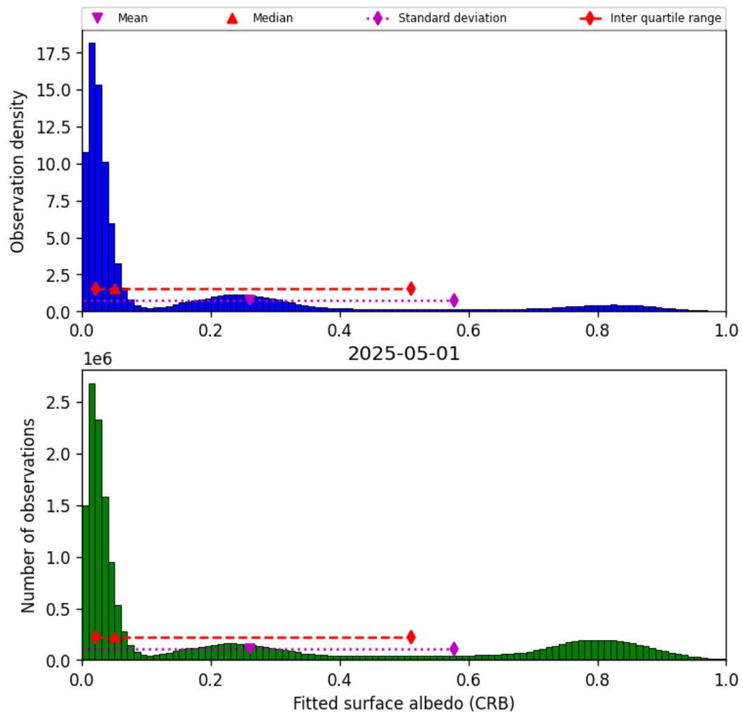
Figure 44: Histogram of “Fitted surface albedo (CRB)” for 2025-05-01 to 2025-05-02
