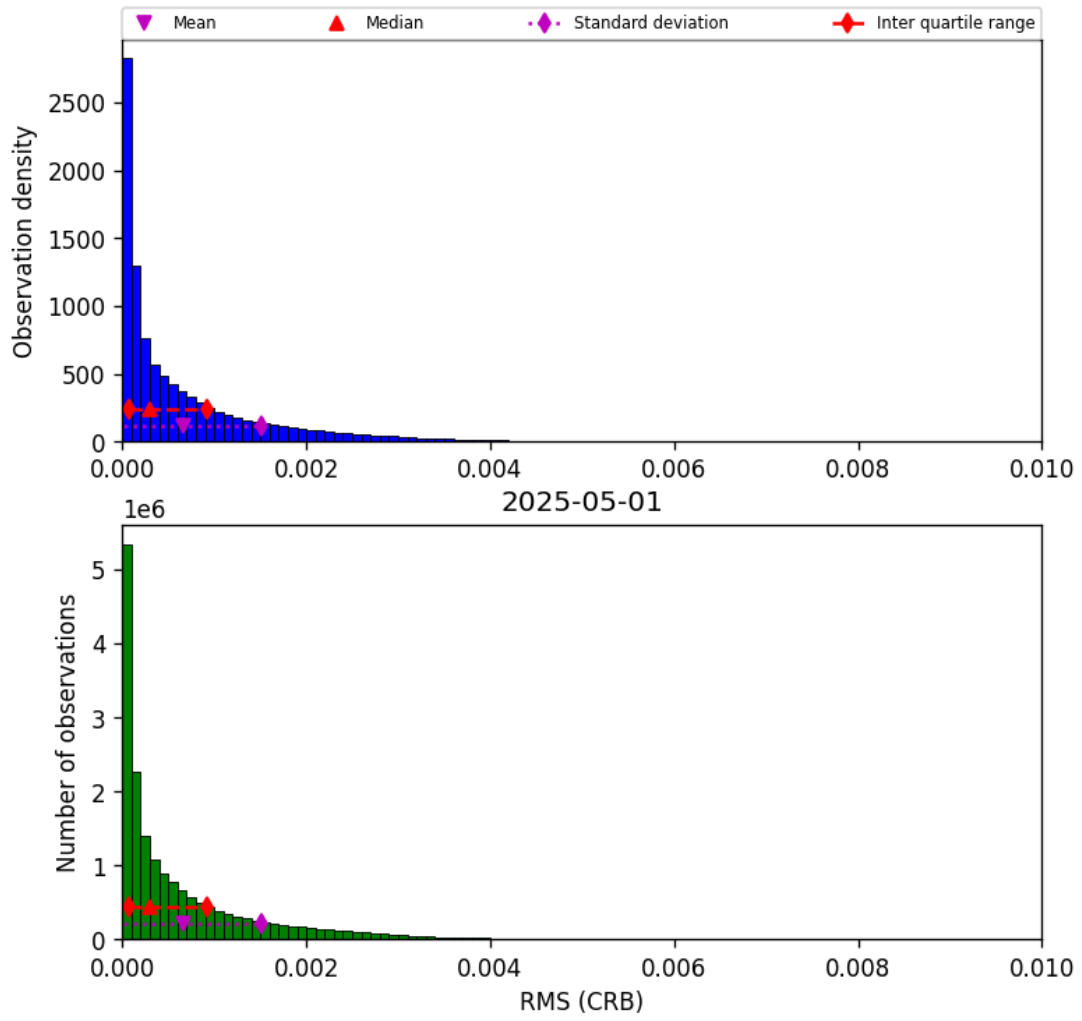
Figure 46: Histogram of “RMS (CRB)” for 2025-05-01 to 2025-05-02
