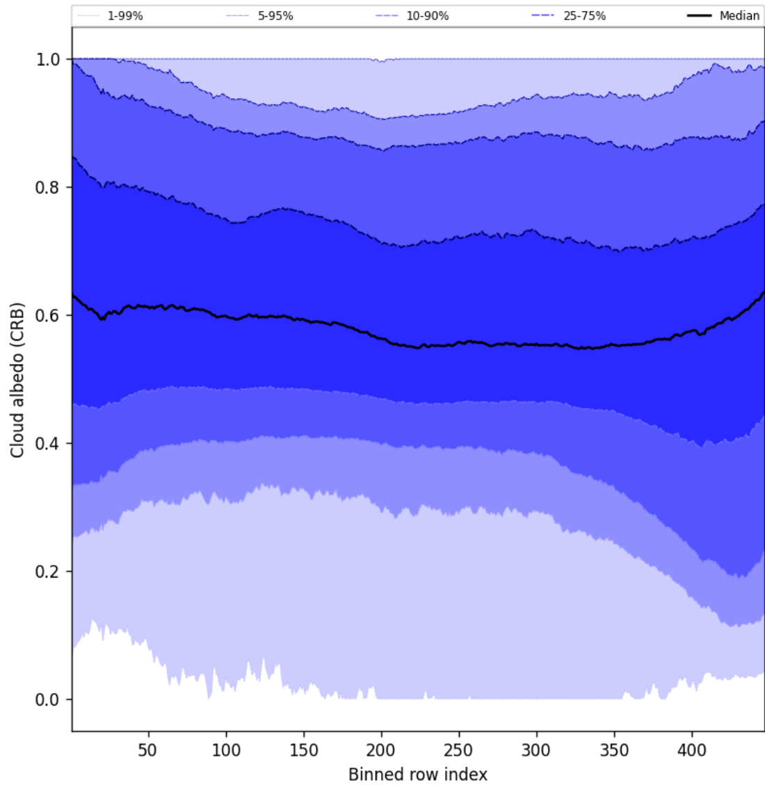
Figure 58: Along track statistics of “Cloud albedo (CRB)” for 2025-05-01 to 2025-05-02
