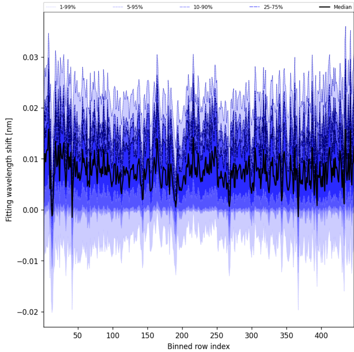
Figure 63: Along track statistics of “Fitting wavelength shift” for 2025-05-01 to 2025-05-02
