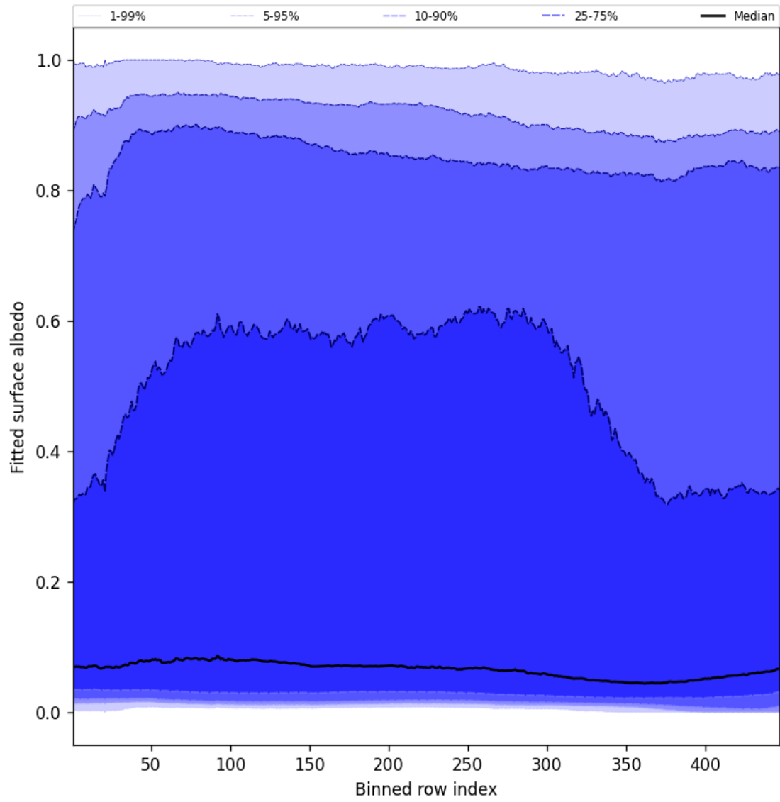
Figure 59: Along track statistics of “Fitted surface albedo” for 2025-05-01 to 2025-05-02
