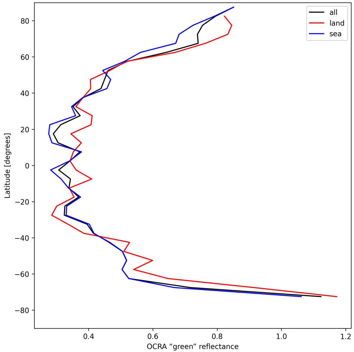
Figure 34: Zonal average of “OCRA “green” reflectance” for 2025-05-01 to 2025-05-02.
