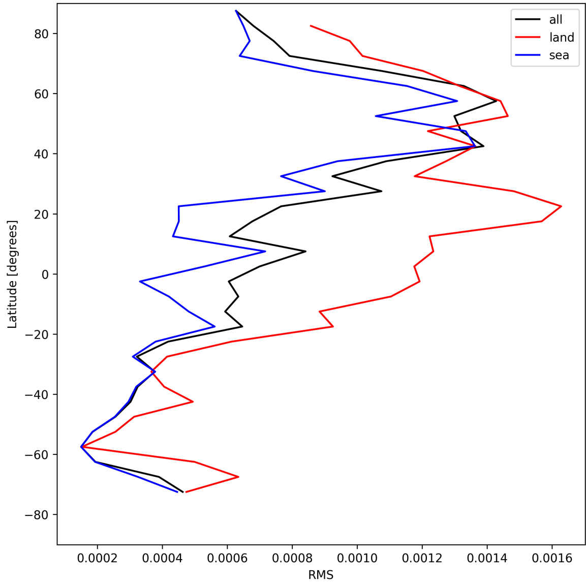
Figure 29: Zonal average of “RMS” for 2025-05-01 to 2025-05-02.
