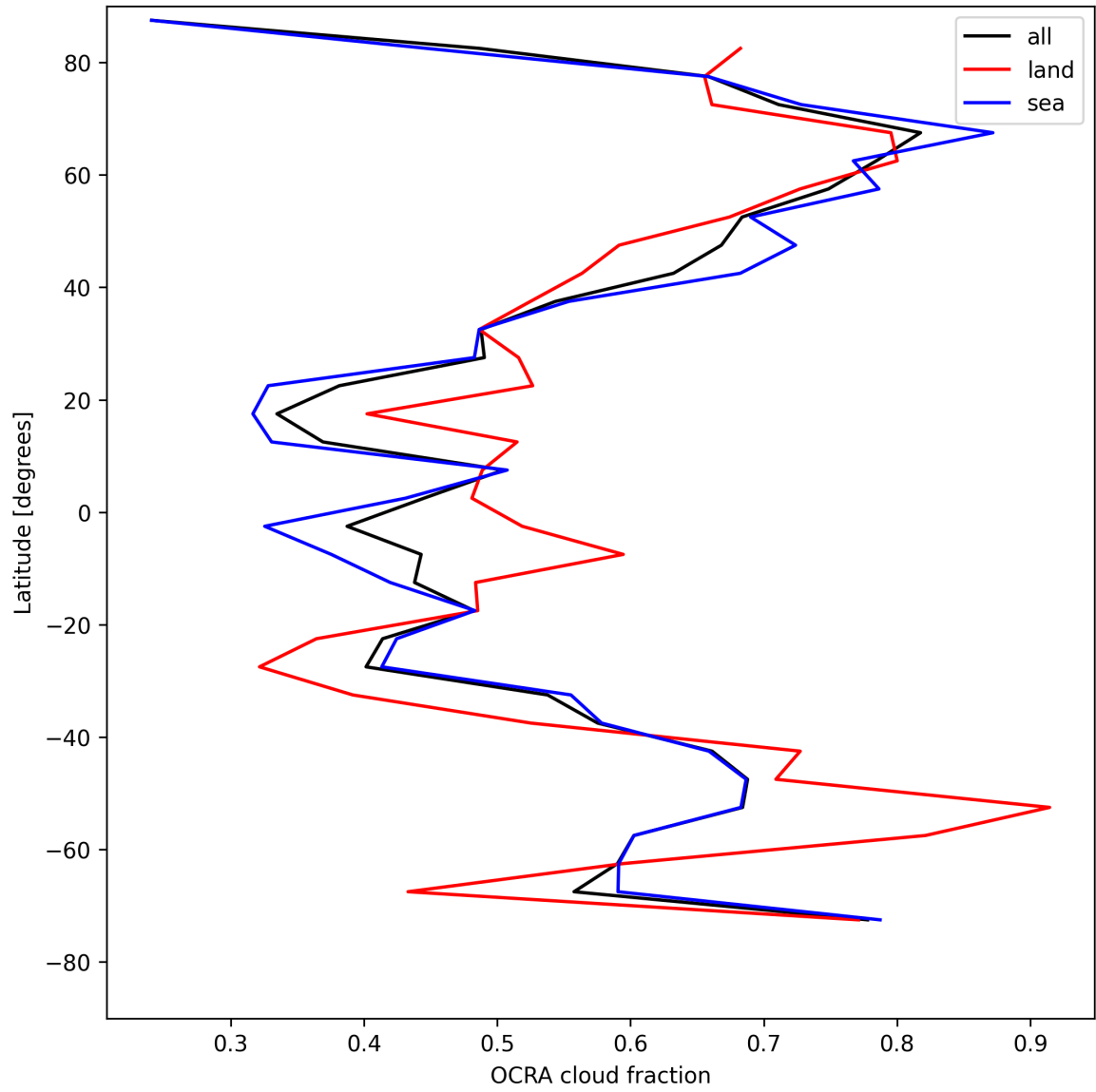
Figure 32: Zonal average of “OCRA cloud fraction” for 2025-05-01 to 2025-05-02.
