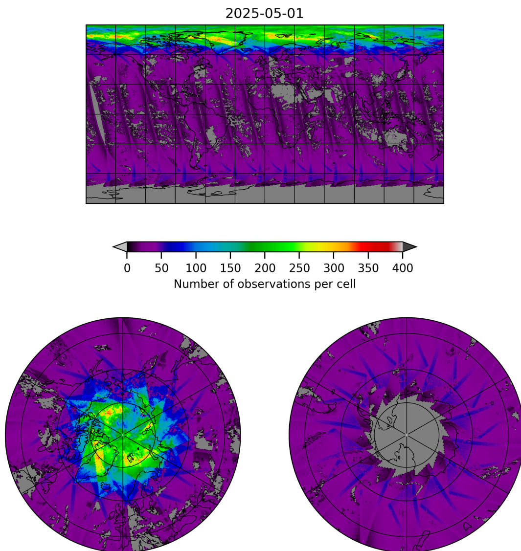
Figure 19: Map of the number of observations for 2025-05-01 to 2025-05-02
