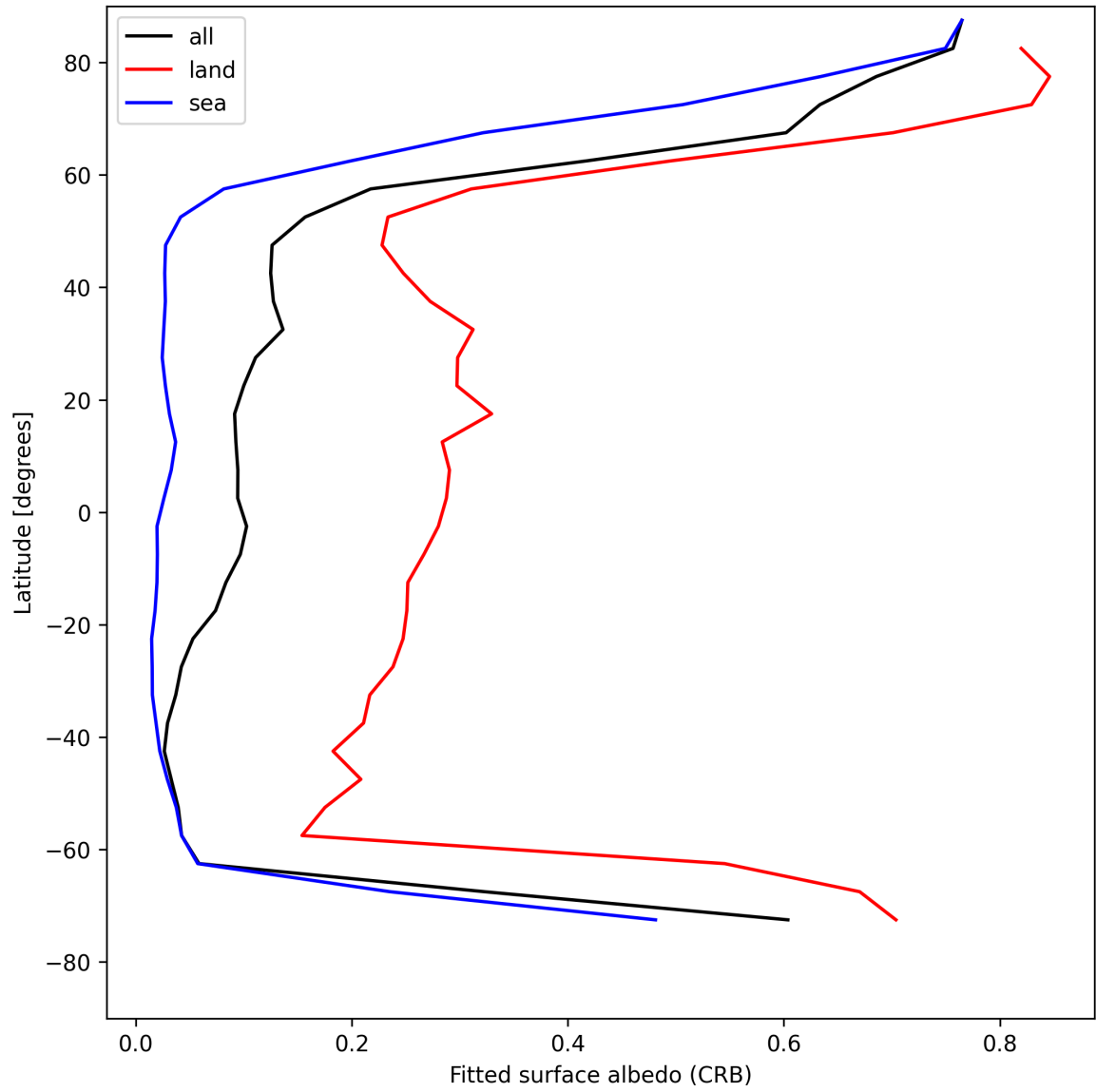
Figure 28: Zonal average of “Fitted surface albedo (CRB)” for 2025-05-01 to 2025-05-02.
