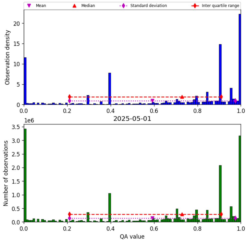
Figure 36: Histogram of “QA value” for 2025-05-01 to 2025-05-02
