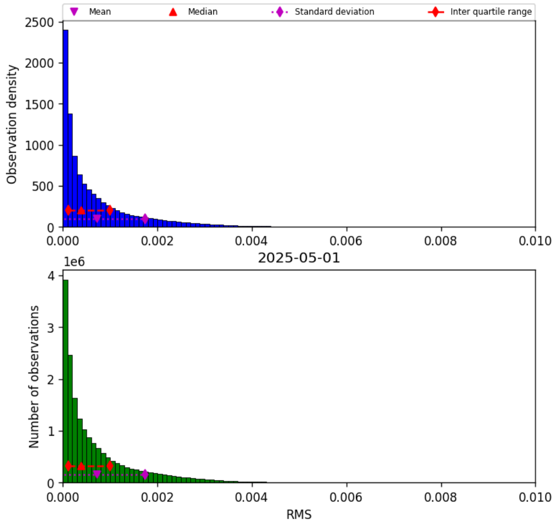
Figure 45: Histogram of “RMS” for 2025-05-01 to 2025-05-02
