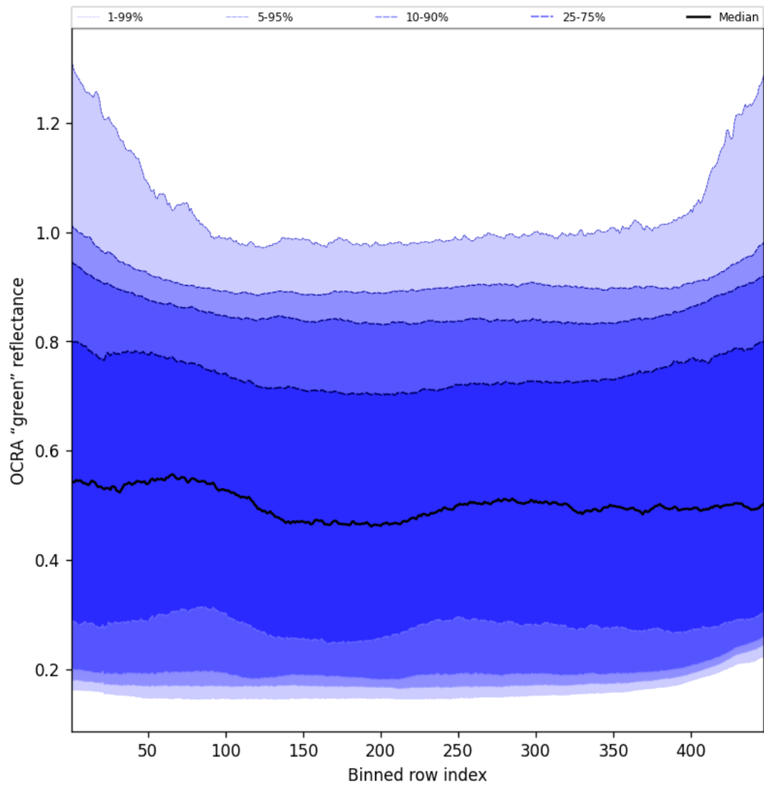
Figure 66: Along track statistics of “OCRA “green” reflectance” for 2025-05-01 to 2025-05-02
