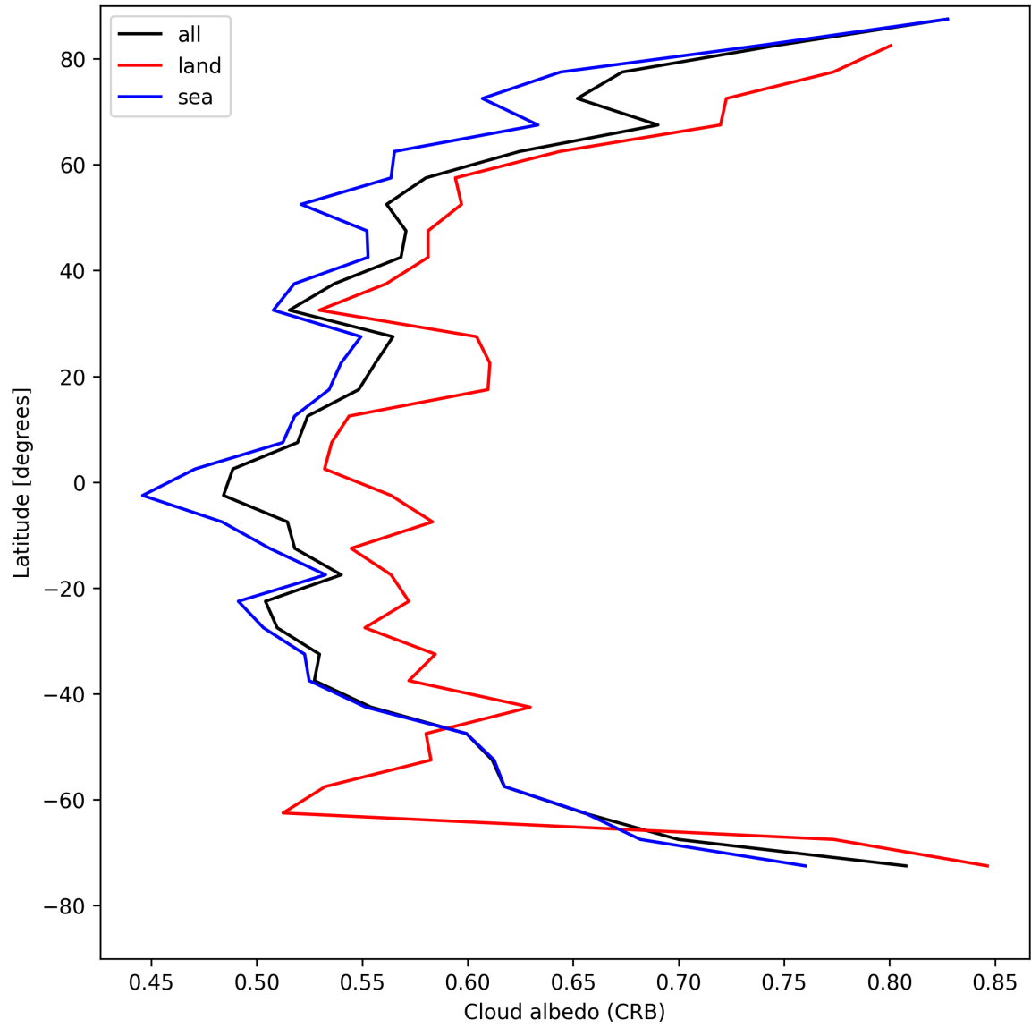
Figure 26: Zonal average of “Cloud albedo (CRB)” for 2025-05-01 to 2025-05-02.
