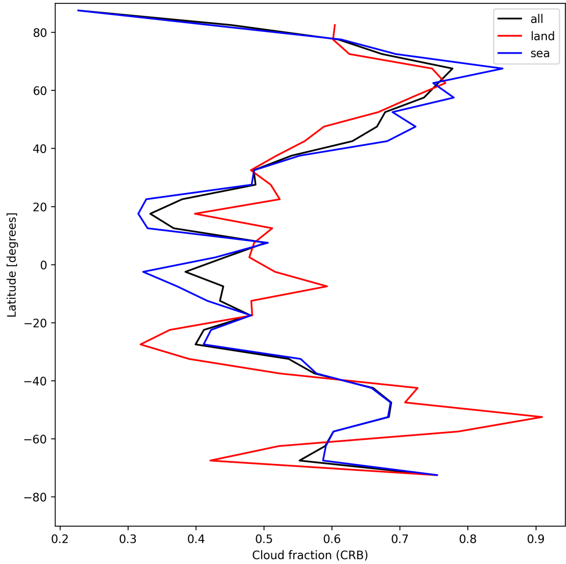
Figure 24: Zonal average of “Cloud fraction (CRB)” for 2025-05-01 to 2025-05-02.
