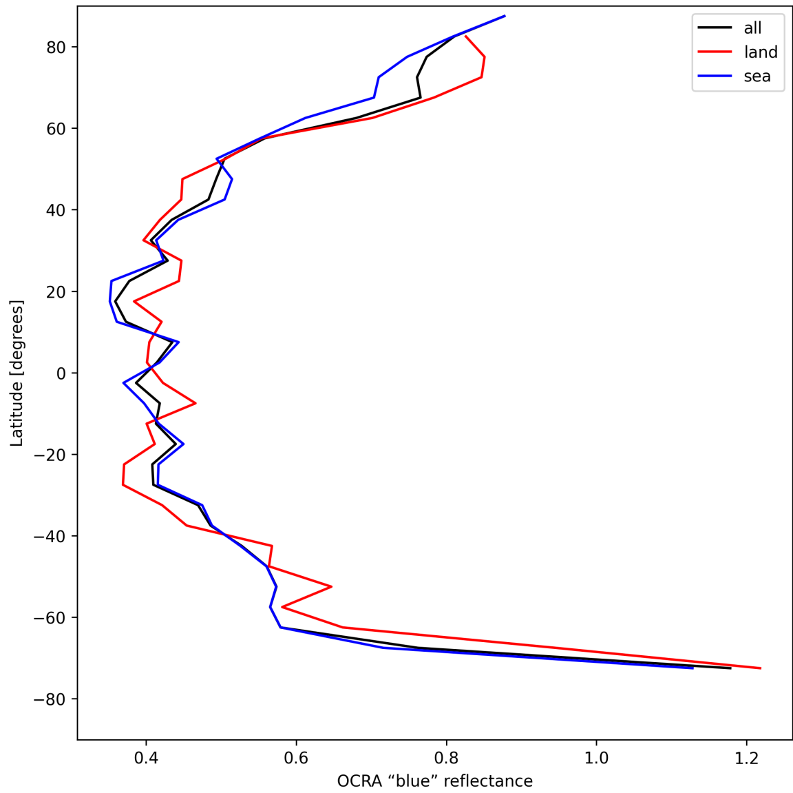
Figure 33: Zonal average of "OCRA "blue" reflectance" for 2025-05-01 to 2025-05-02.
