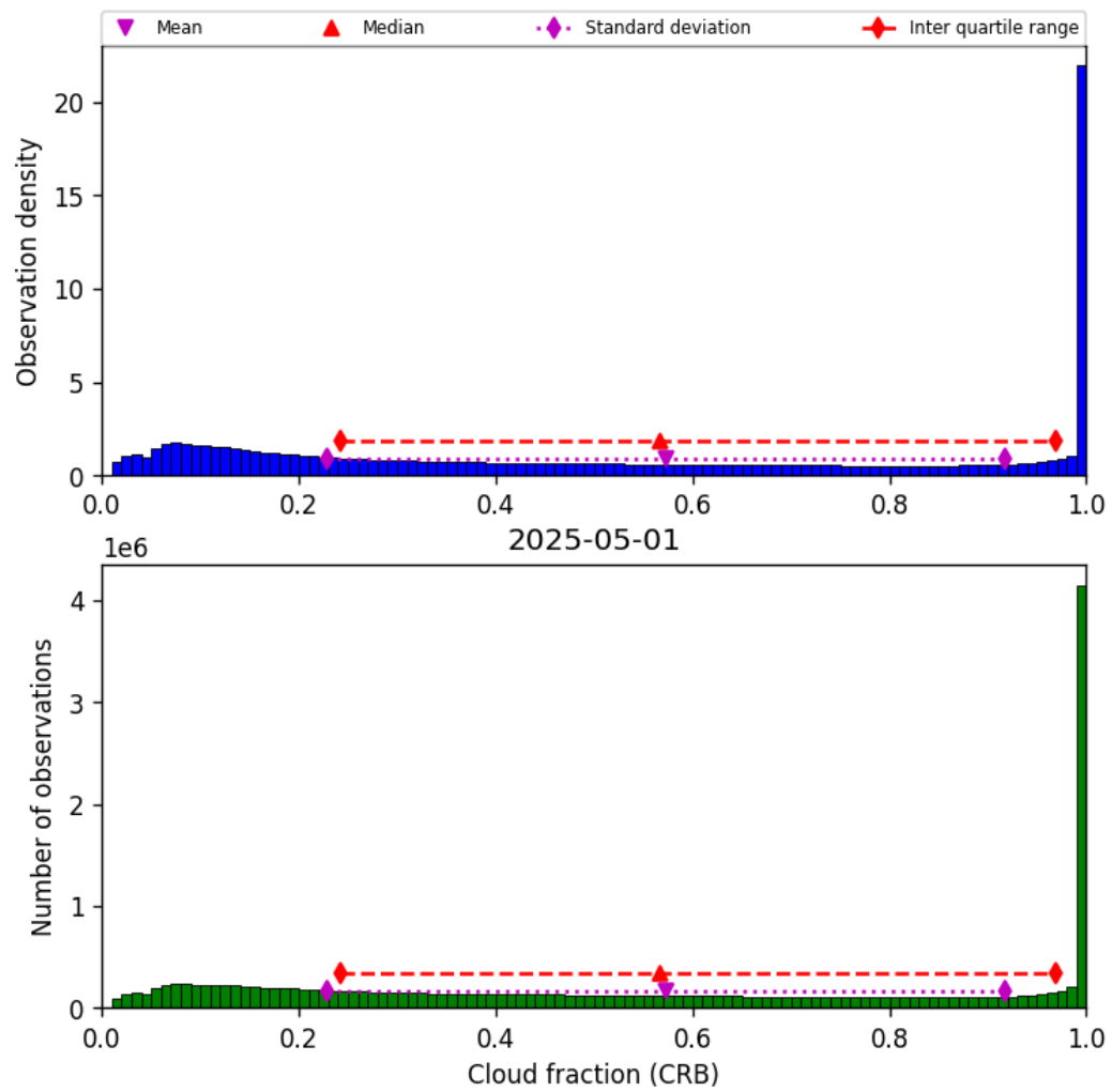
Figure 40: Histogram of “Cloud fraction (CRB)” for 2025-05-01 to 2025-05-02
