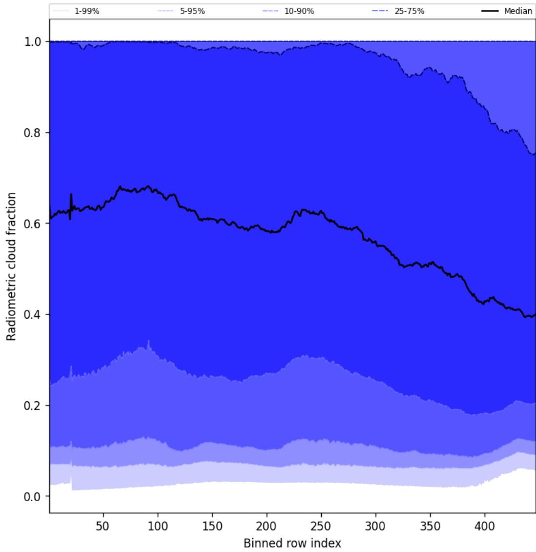
Figure 53: Along track statistics of “Radiometric cloud fraction” for 2025-05-01 to 2025-05-02
