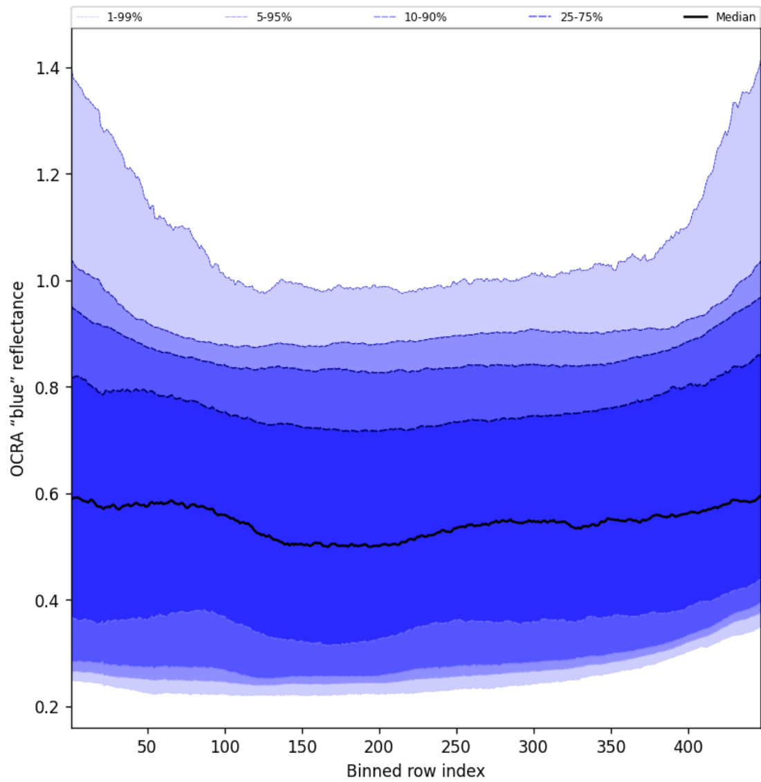
Figure 65: Along track statistics of “OCRA “blue” reflectance” for 2025-05-01 to 2025-05-02
