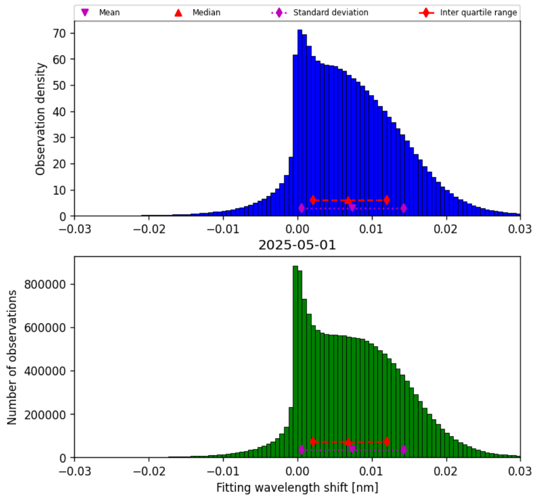
Figure 47: Histogram of “Fitting wavelength shift” for 2025-05-01 to 2025-05-02
