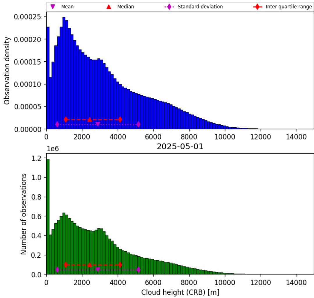
Figure 41: Histogram of “Cloud height (CRB)” for 2025-05-01 to 2025-05-02
