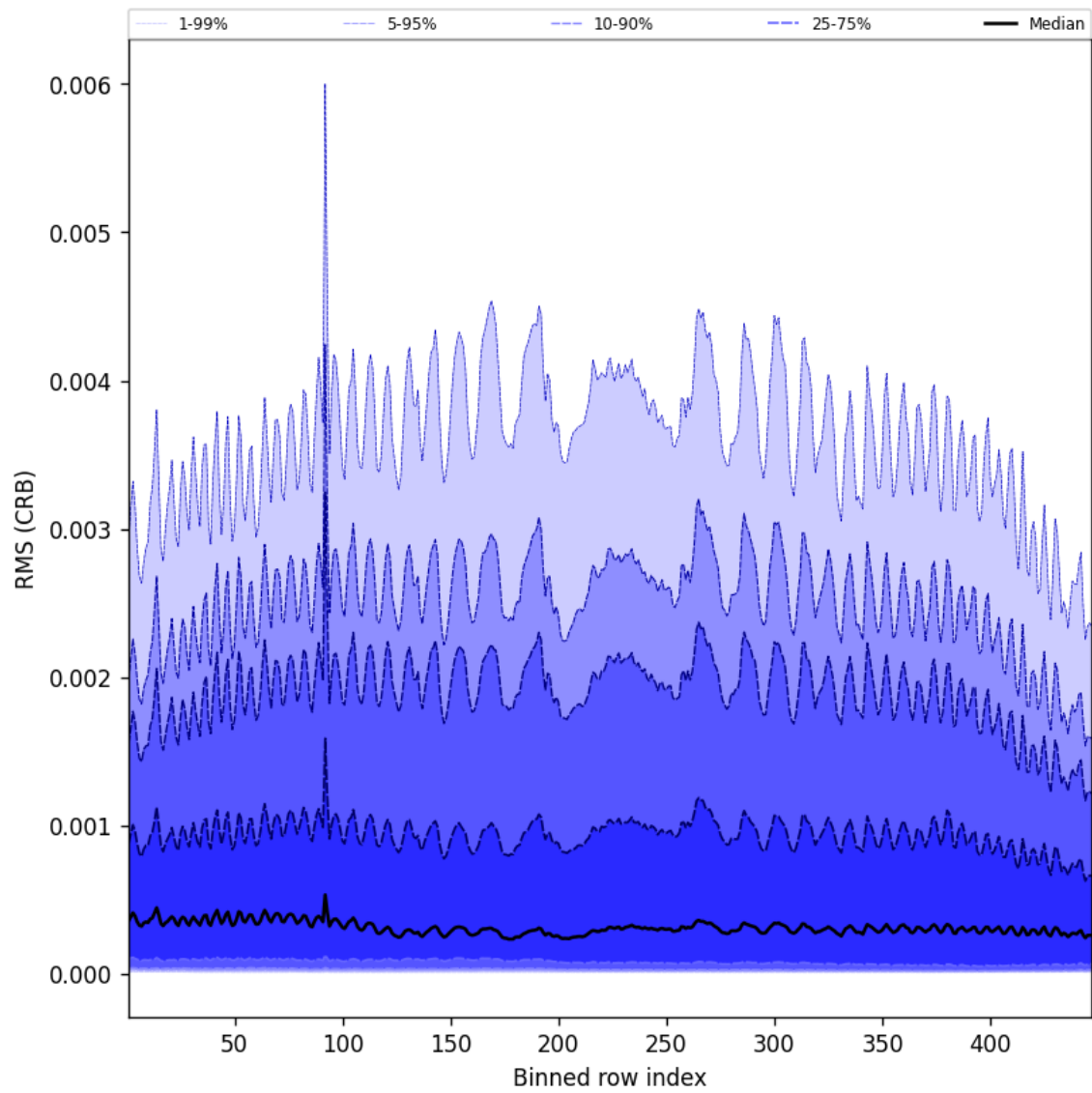
Figure 62: Along track statistics of “RMS (CRB)” for 2025-05-01 to 2025-05-02
