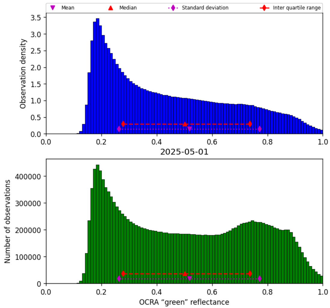
Figure 50: Histogram of “OCRA “green” reflectance” for 2025-05-01 to 2025-05-02
