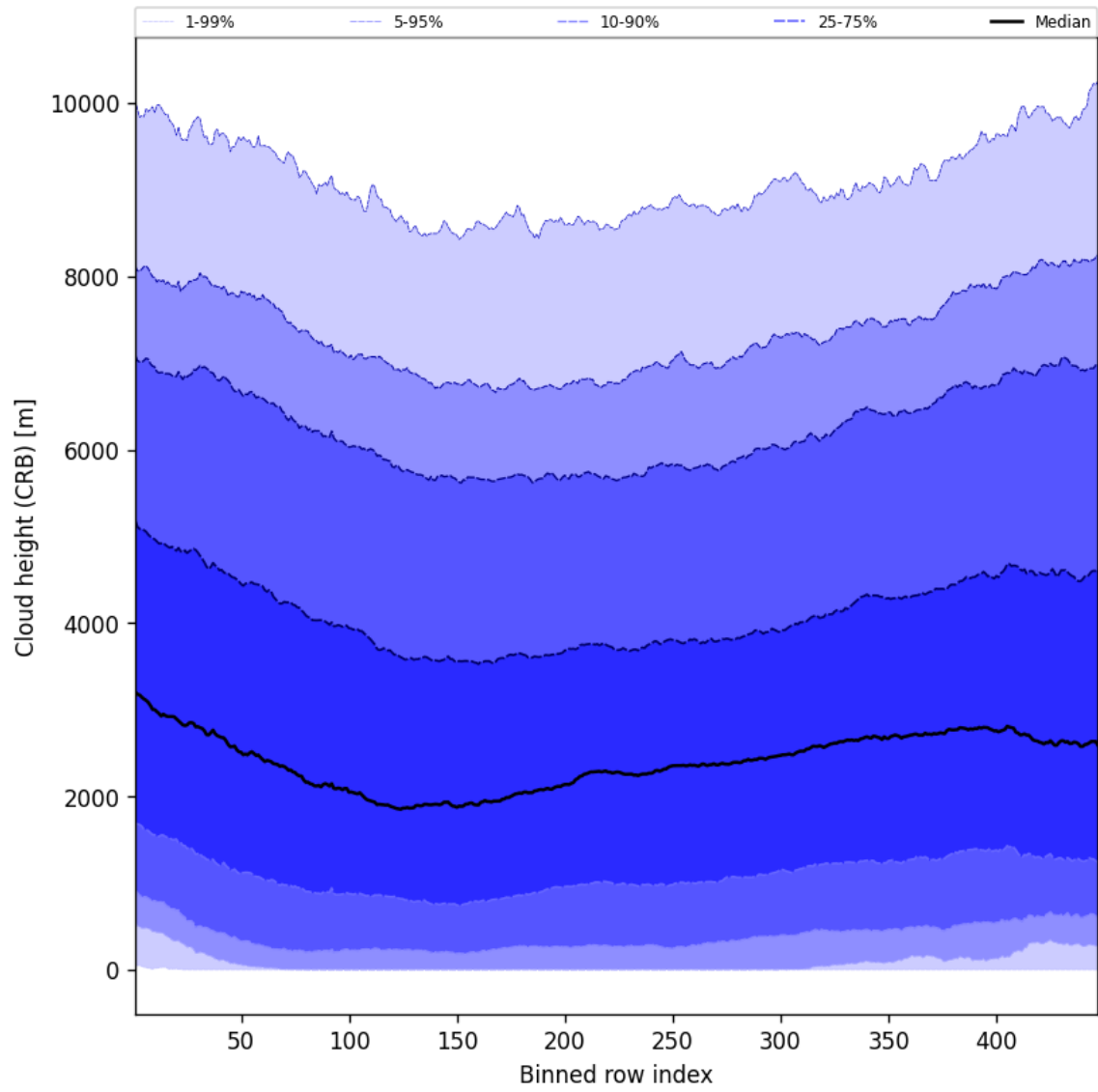
Figure 57: Along track statistics of “Cloud height (CRB)” for 2025-05-01 to 2025-05-02
