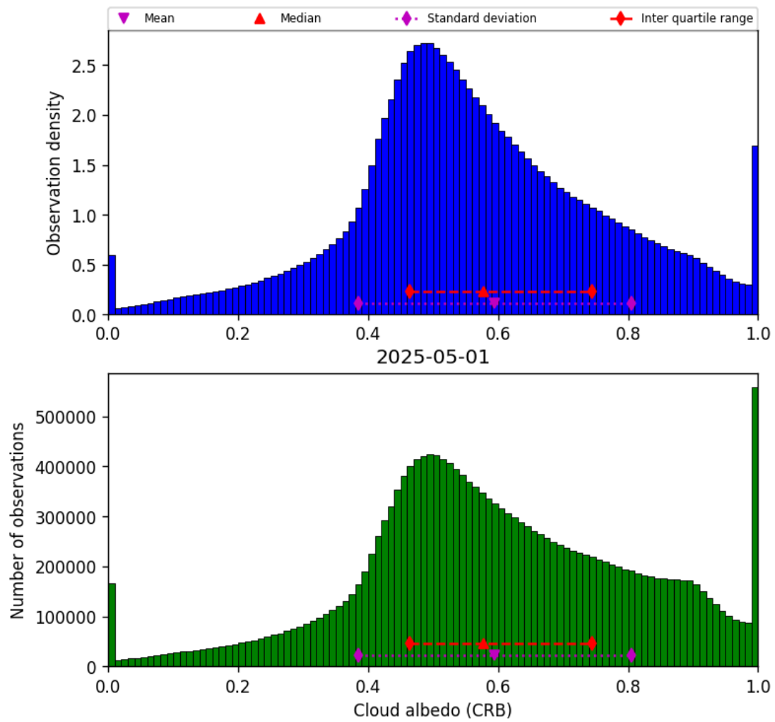
Figure 42: Histogram of “Cloud albedo (CRB)” for 2025-05-01 to 2025-05-02
