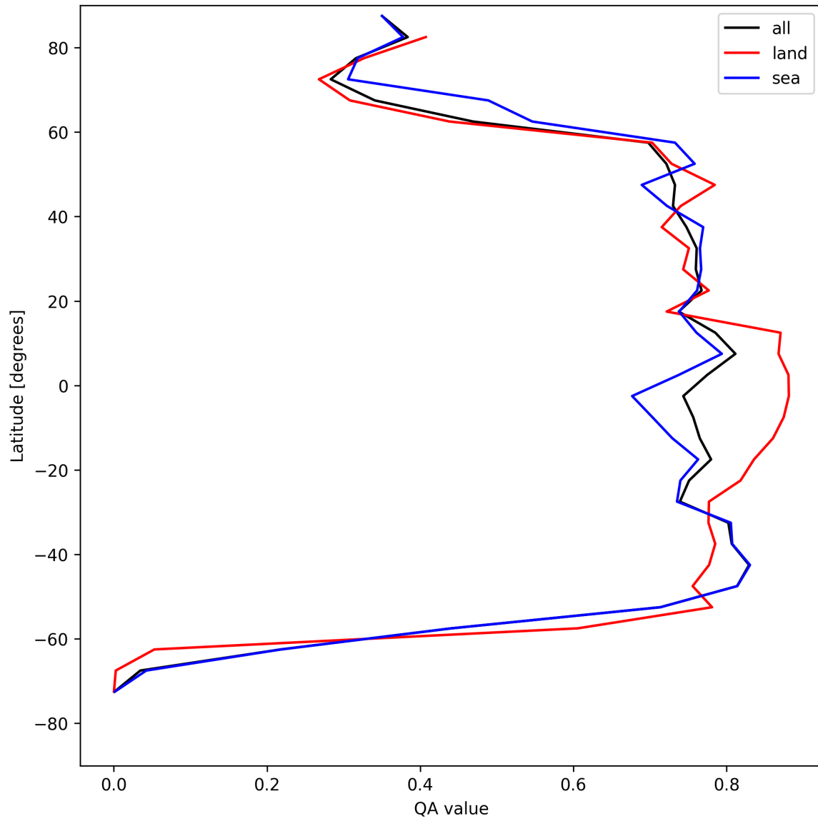
Figure 20: Zonal average of “QA value” for 2025-05-01 to 2025-05-02.
