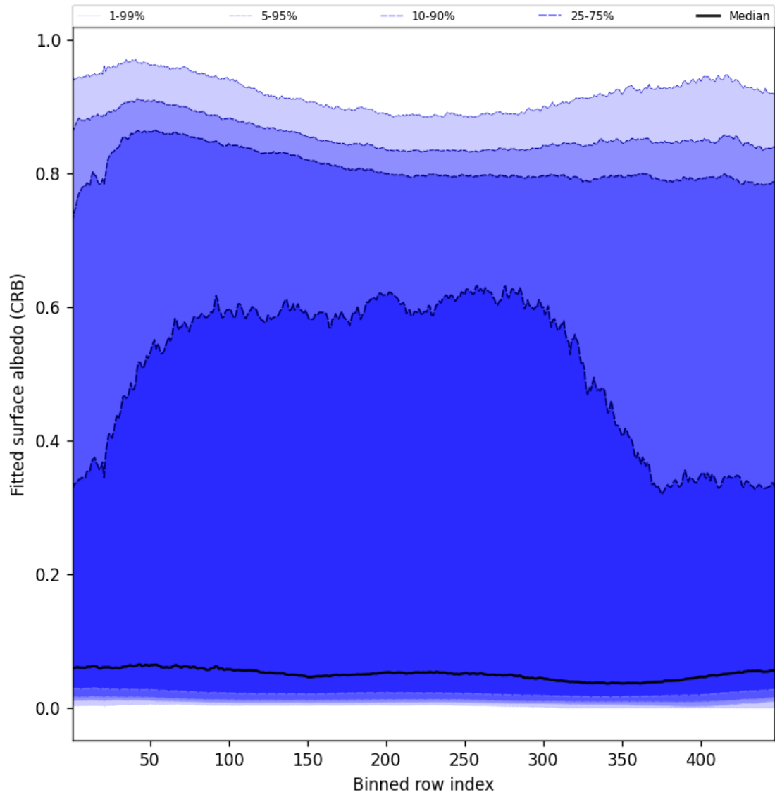
Figure 60: Along track statistics of “Fitted surface albedo (CRB)” for 2025-05-01 to 2025-05-02
