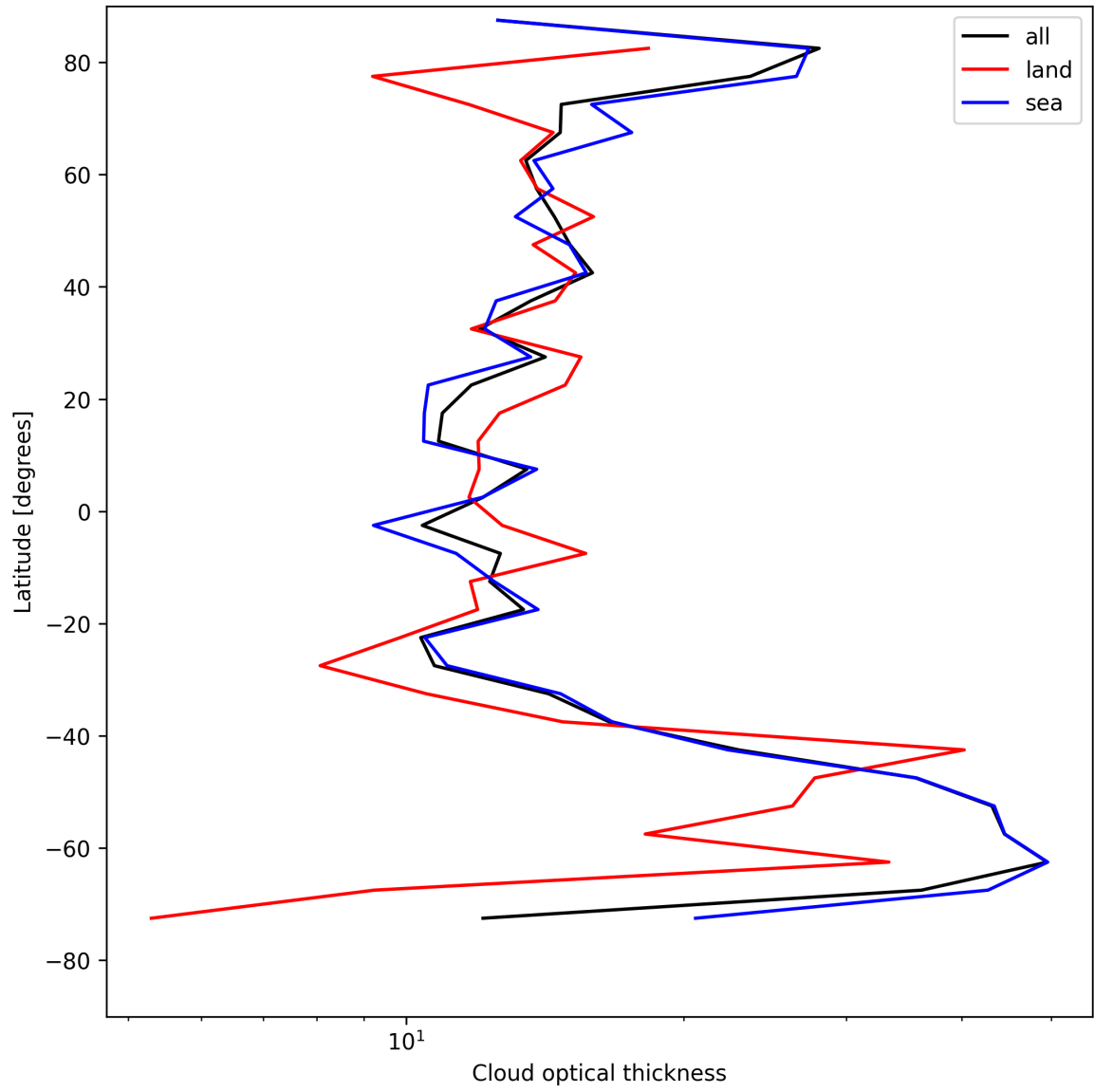
Figure 23: Zonal average of “Cloud optical thickness” for 2025-05-01 to 2025-05-02.
