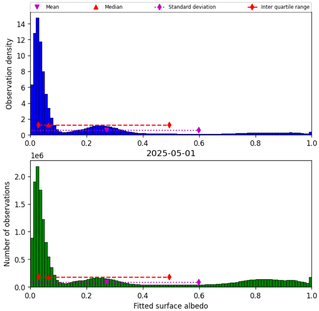
Figure 43: Histogram of “Fitted surface albedo” for 2025-05-01 to 2025-05-02
