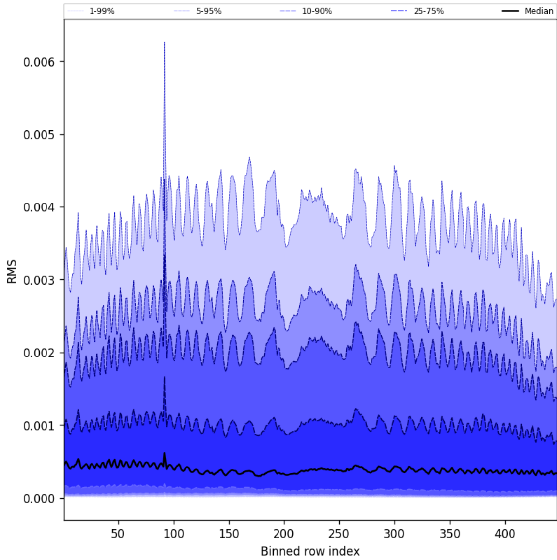
Figure 61: Along track statistics of “RMS” for 2025-05-01 to 2025-05-02
