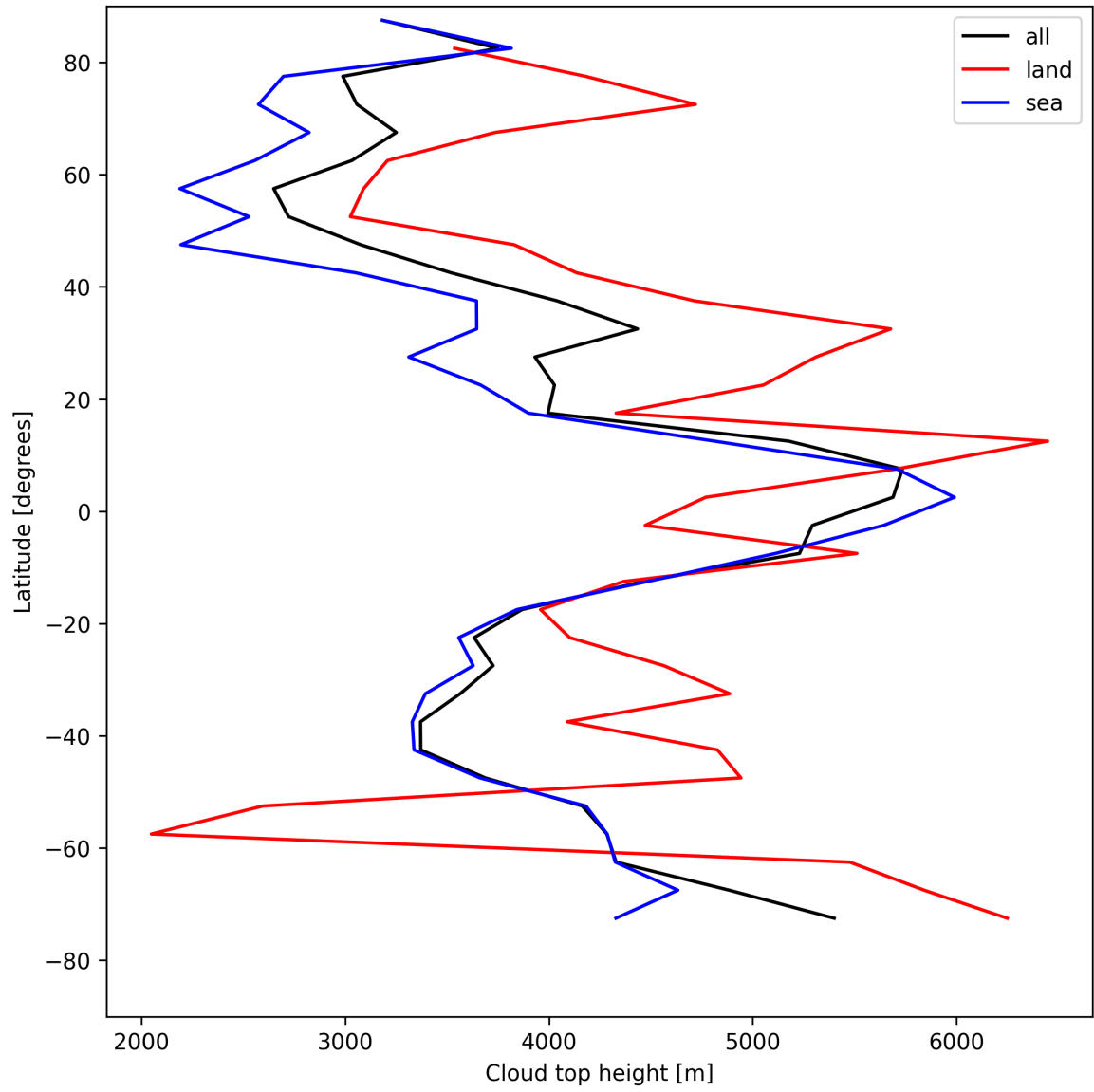
Figure 22: Zonal average of “Cloud top height” for 2025-05-01 to 2025-05-02.
