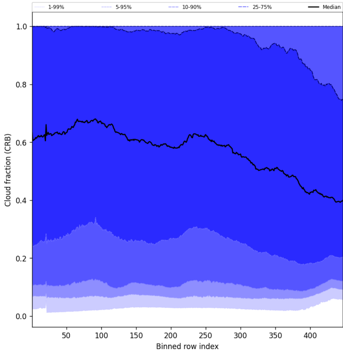
Figure 56: Along track statistics of “Cloud fraction (CRB)” for 2025-05-01 to 2025-05-02
