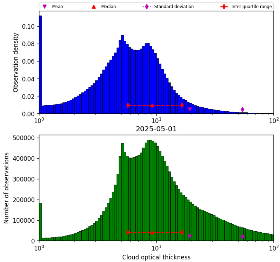
Figure 39: Histogram of “Cloud optical thickness” for 2025-05-01 to 2025-05-02
