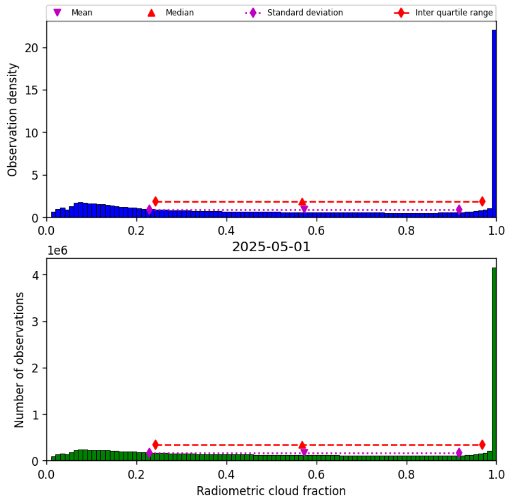
Figure 37: Histogram of “Radiometric cloud fraction” for 2025-05-01 to 2025-05-02
