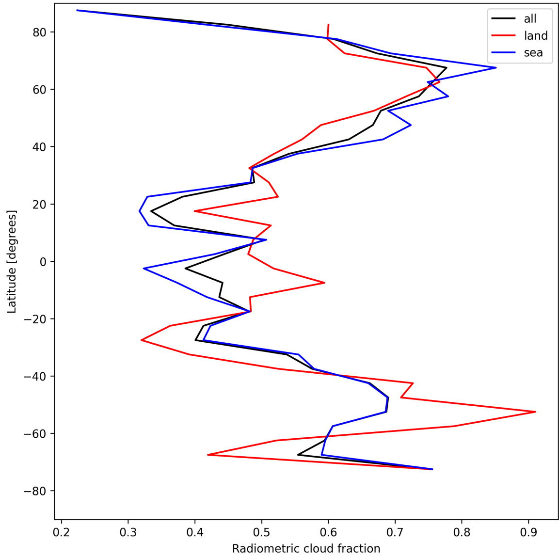
Figure 21: Zonal average of “Radiometric cloud fraction” for 2025-05-01 to 2025-05-02.
