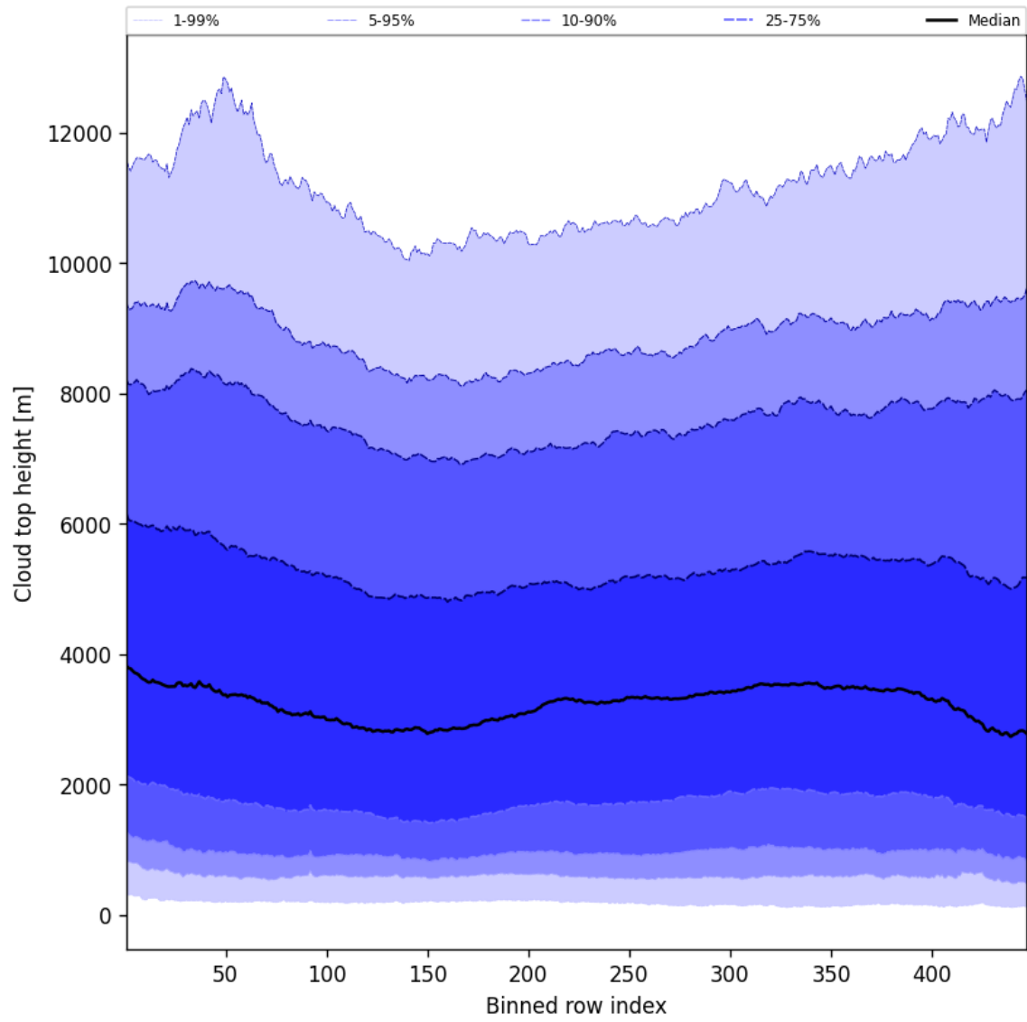
Figure 54: Along track statistics of “Cloud top height” for 2025-05-01 to 2025-05-02
