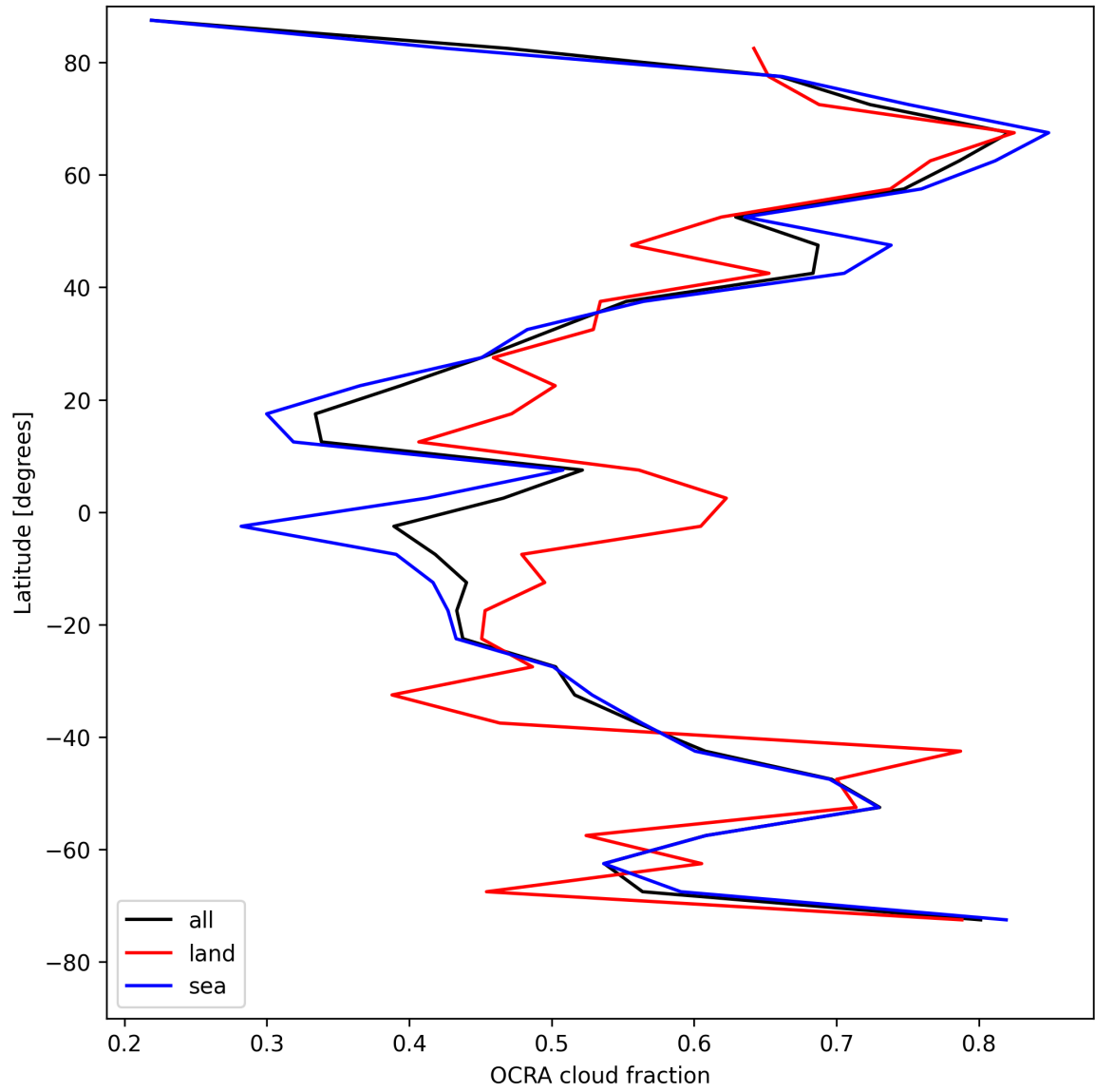
Figure 32: Zonal average of “OCRA cloud fraction” for 2025-05-02 to 2025-05-02.
