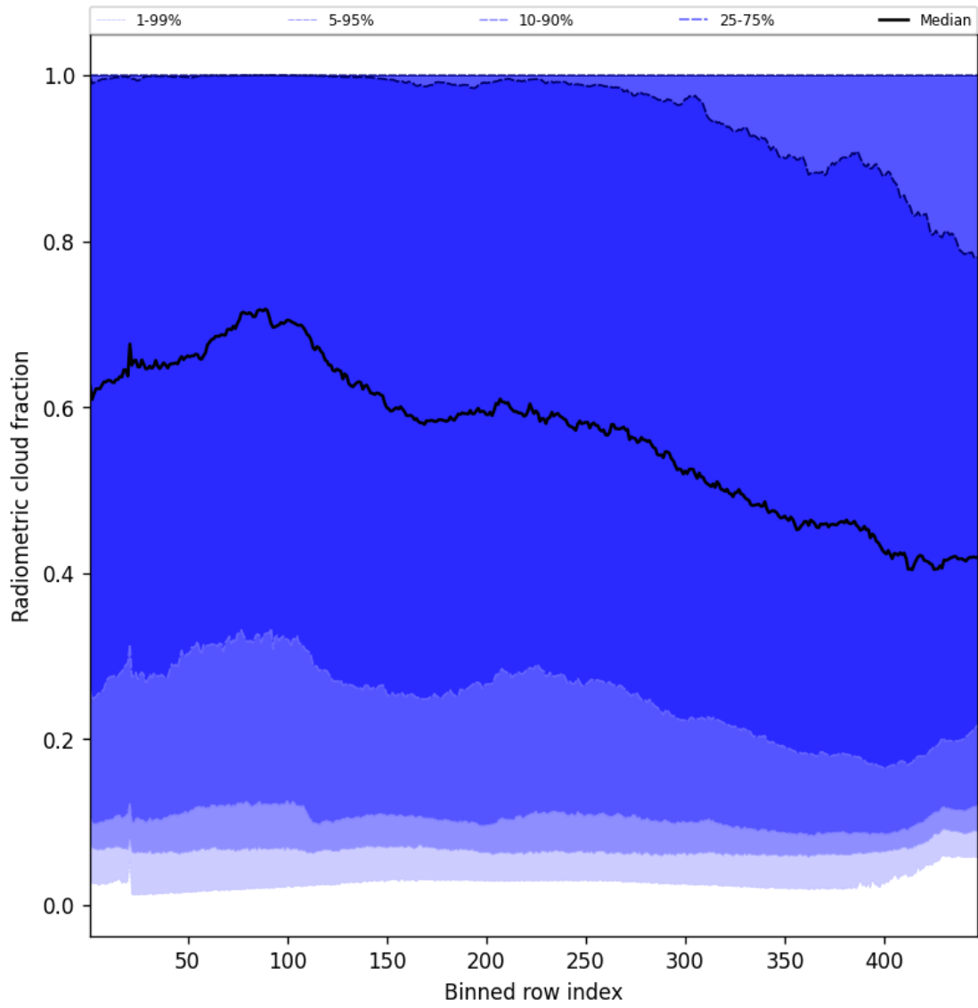
Figure 53: Along track statistics of “Radiometric cloud fraction” for 2025-05-02 to 2025-05-02
