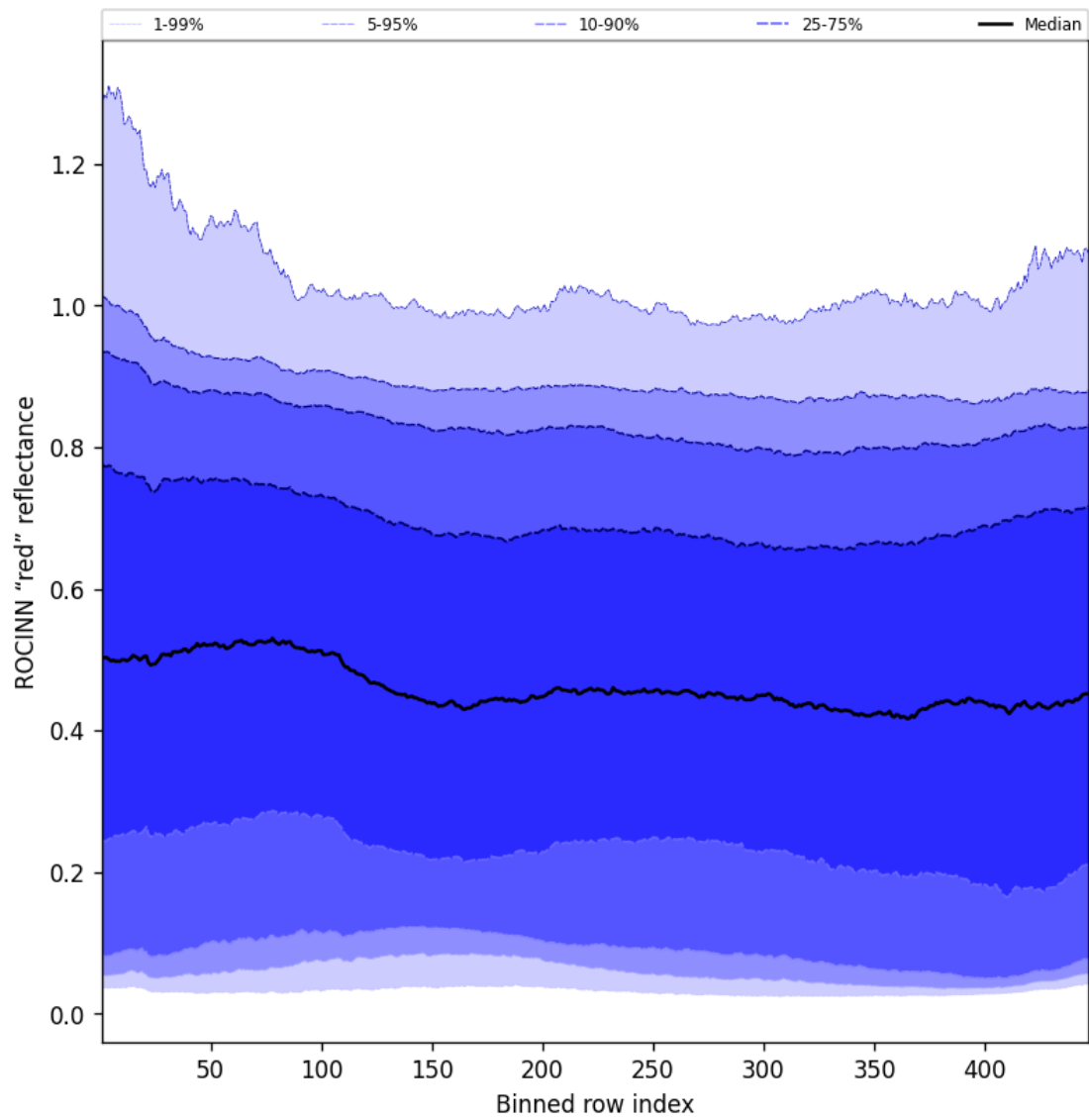
Figure 67: Along track statistics of “ROCINN “red” reflectance” for 2025-05-02 to 2025-05-02
