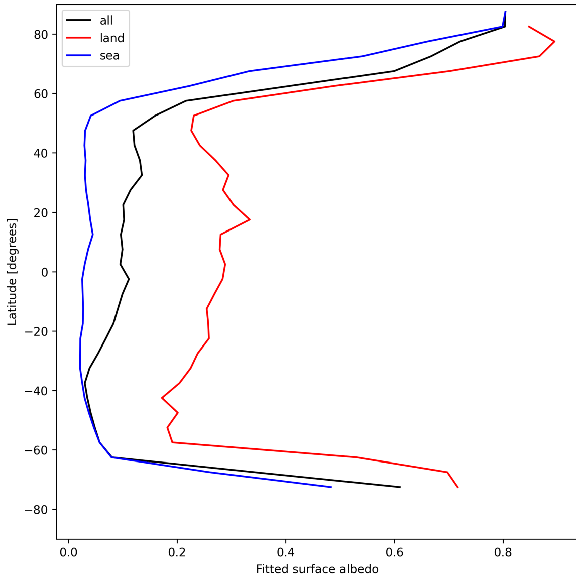
Figure 27: Zonal average of “Fitted surface albedo” for 2025-05-02 to 2025-05-02.
