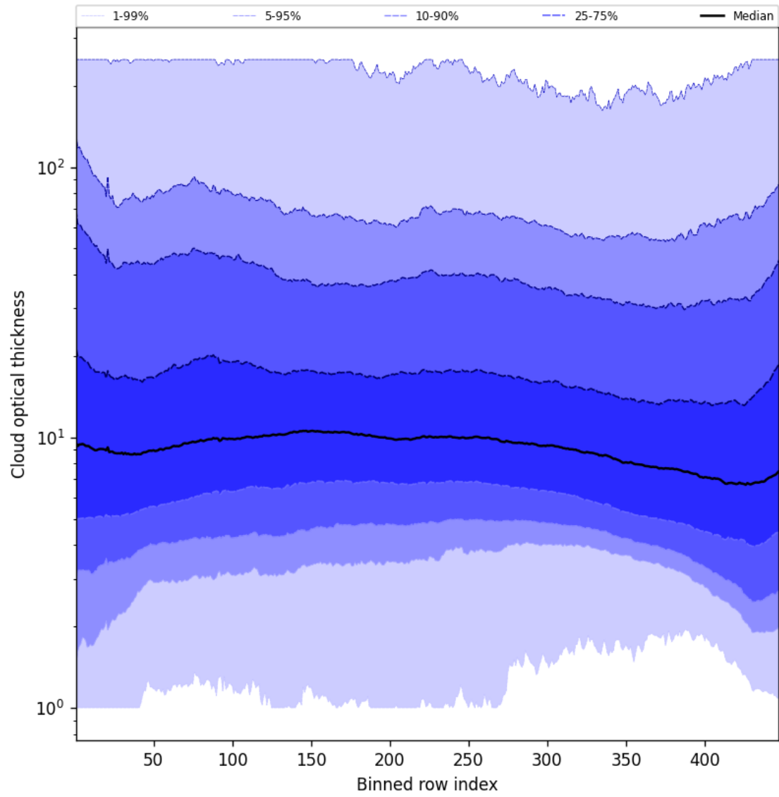
Figure 55: Along track statistics of “Cloud optical thickness” for 2025-05-02 to 2025-05-02
