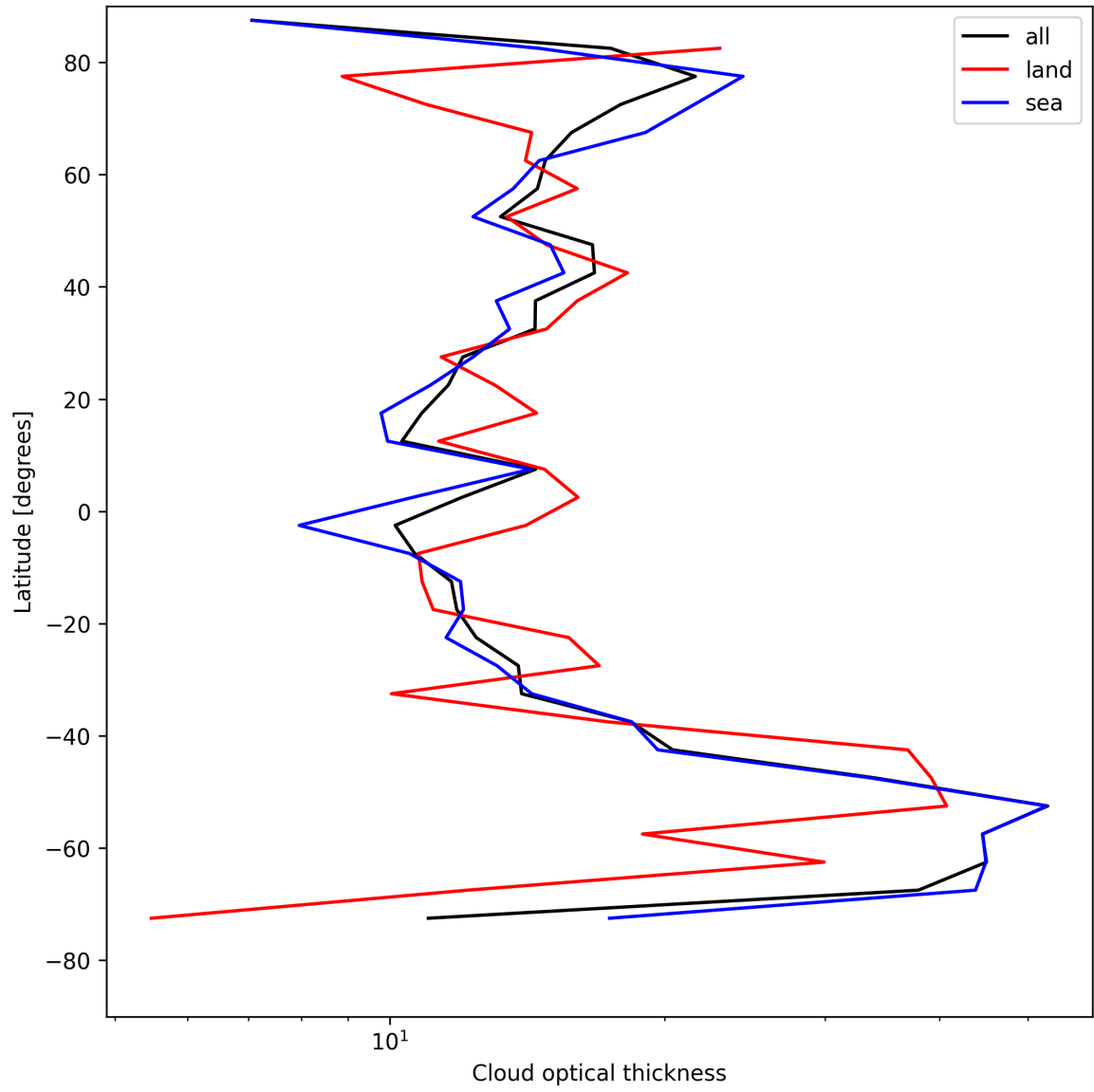
Figure 23: Zonal average of “Cloud optical thickness” for 2025-05-02 to 2025-05-02.
