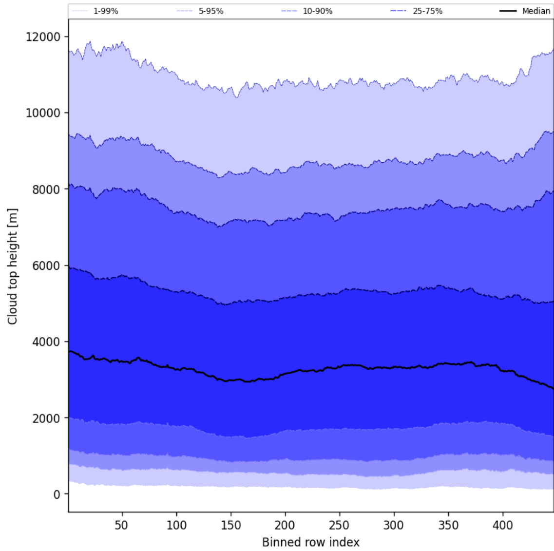
Figure 54: Along track statistics of “Cloud top height” for 2025-05-02 to 2025-05-02
