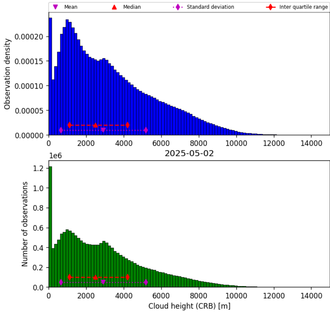
Figure 41: Histogram of “Cloud height (CRB)” for 2025-05-02 to 2025-05-02
