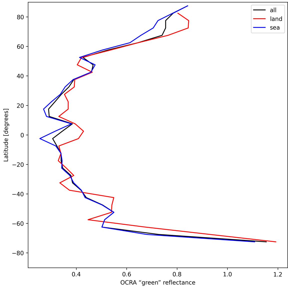
Figure 34: Zonal average of “OCRA “green” reflectance” for 2025-05-02 to 2025-05-02.
