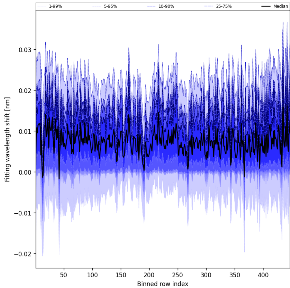
Figure 63: Along track statistics of “Fitting wavelength shift” for 2025-05-02 to 2025-05-02
