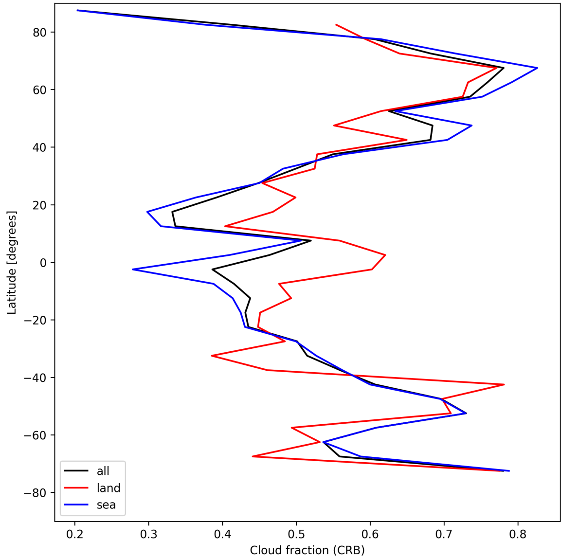
Figure 24: Zonal average of “Cloud fraction (CRB)” for 2025-05-02 to 2025-05-02.
