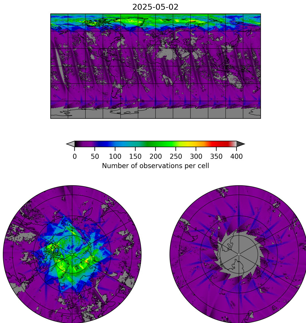
Figure 19: Map of the number of observations for 2025-05-02 to 2025-05-02
