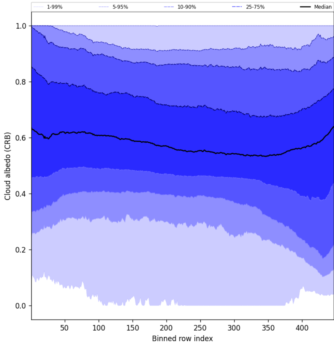
Figure 58: Along track statistics of “Cloud albedo (CRB)” for 2025-05-02 to 2025-05-02
