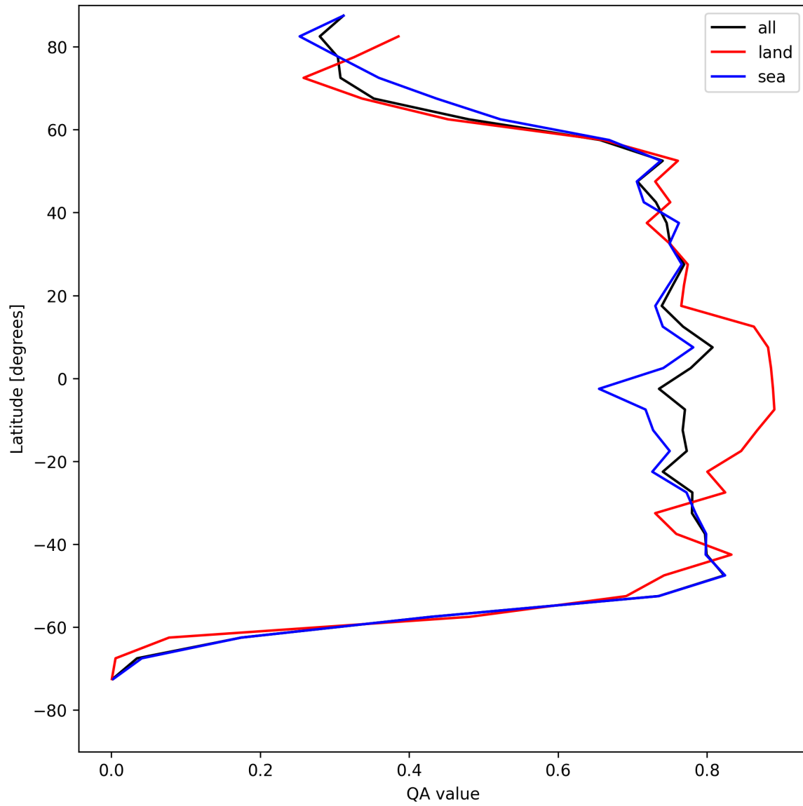
Figure 20: Zonal average of “QA value” for 2025-05-02 to 2025-05-02.
