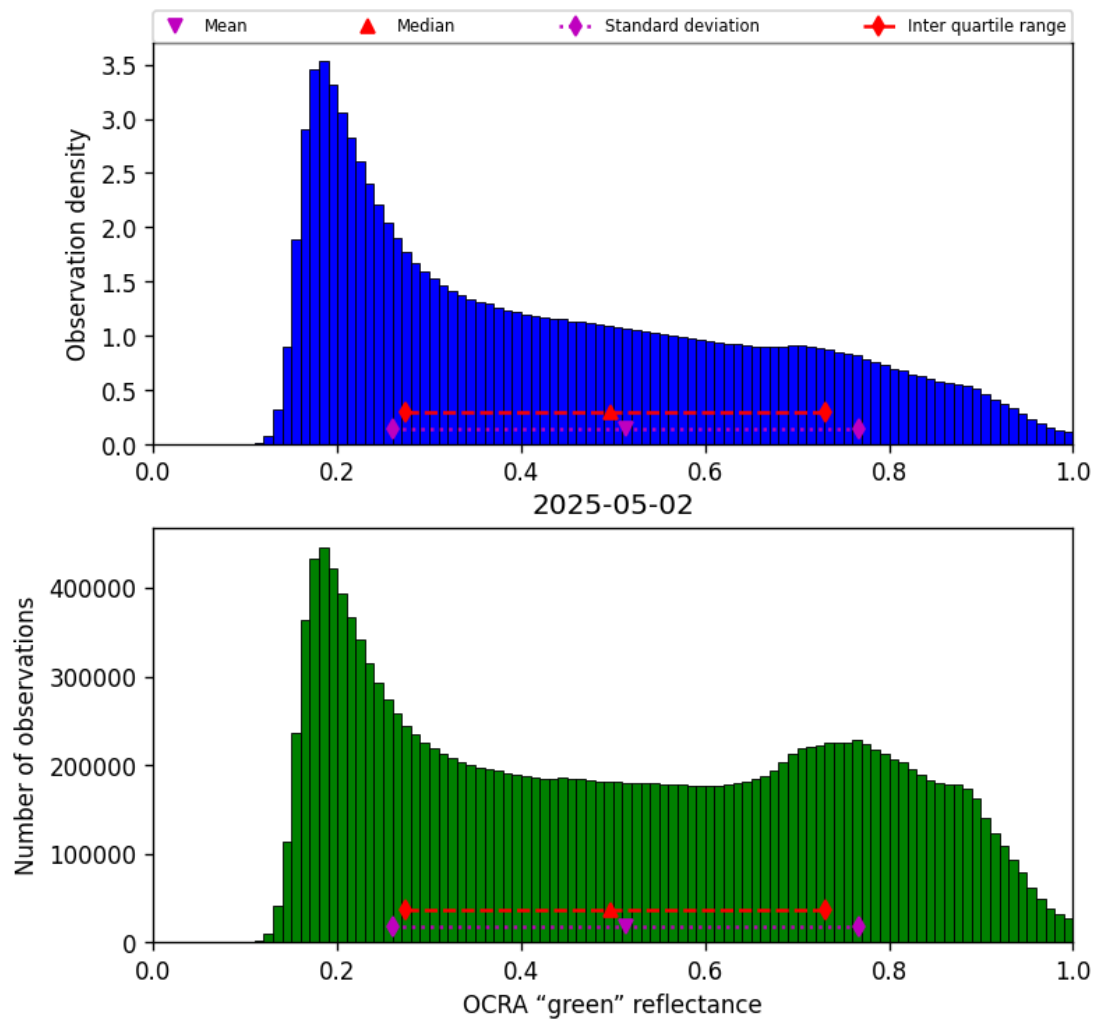
Figure 50: Histogram of “OCRA “green” reflectance” for 2025-05-02 to 2025-05-02
