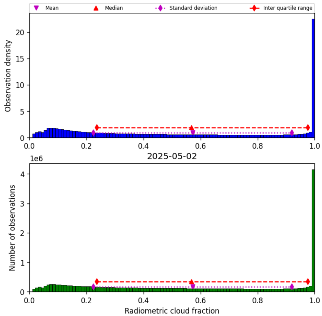
Figure 37: Histogram of “Radiometric cloud fraction” for 2025-05-02 to 2025-05-02
