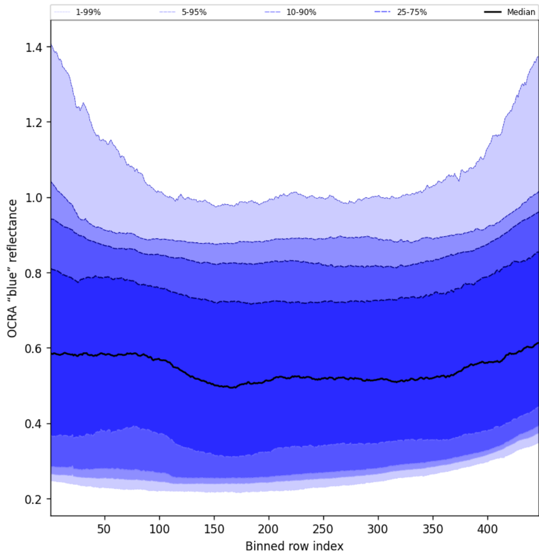
Figure 65: Along track statistics of “OCRA “blue” reflectance” for 2025-05-02 to 2025-05-02
