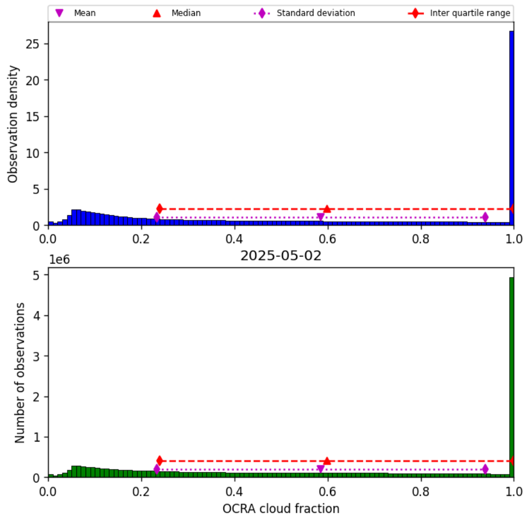
Figure 48: Histogram of “OCRA cloud fraction” for 2025-05-02 to 2025-05-02
