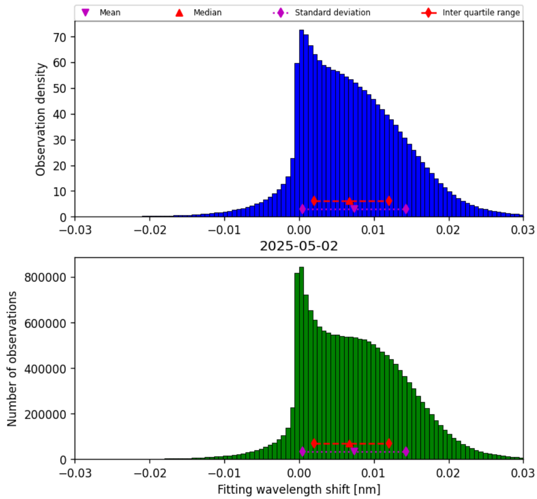
Figure 47: Histogram of “Fitting wavelength shift” for 2025-05-02 to 2025-05-02
