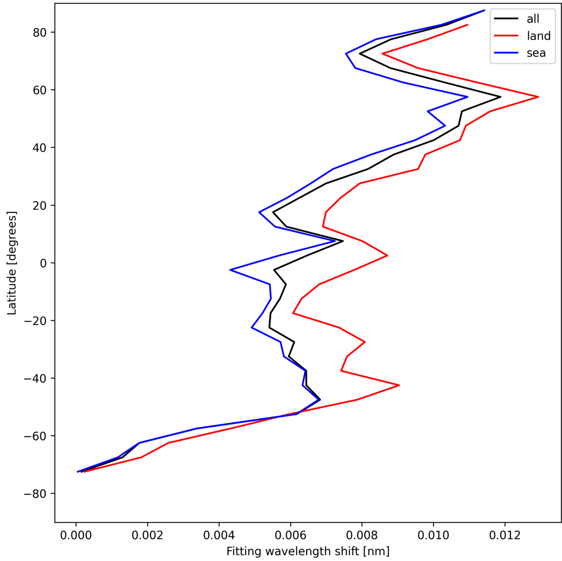
Figure 31: Zonal average of “Fitting wavelength shift” for 2025-05-02 to 2025-05-02.
