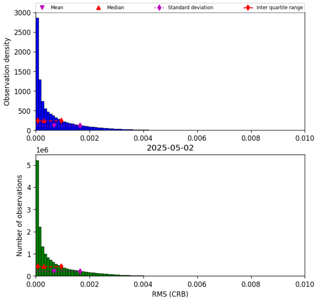
Figure 46: Histogram of “RMS (CRB)” for 2025-05-02 to 2025-05-02
