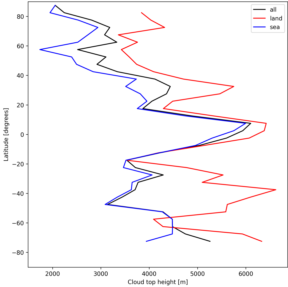
Figure 22: Zonal average of “Cloud top height” for 2025-05-02 to 2025-05-02.
