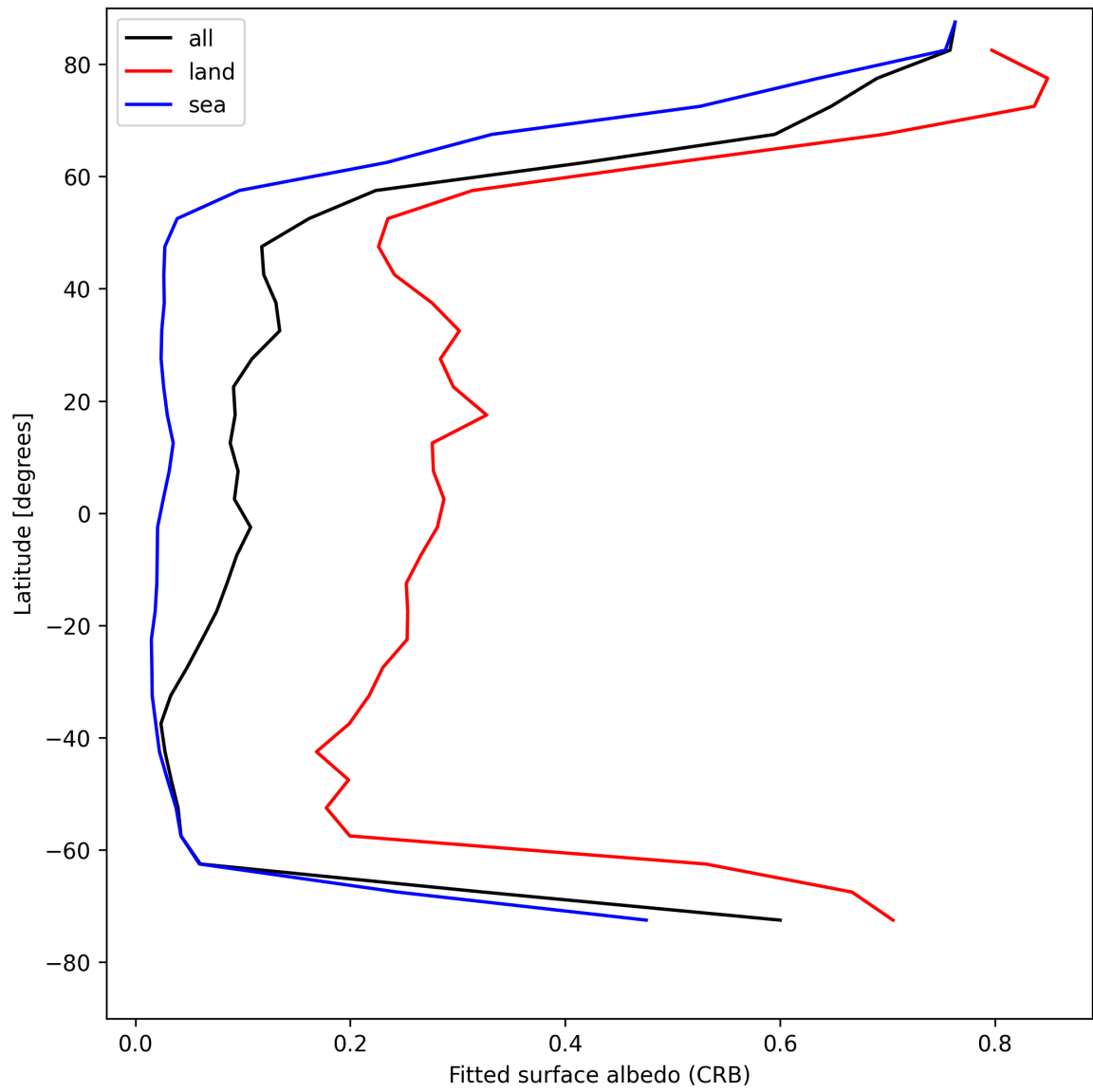
Figure 28: Zonal average of “Fitted surface albedo (CRB)” for 2025-05-02 to 2025-05-02.
