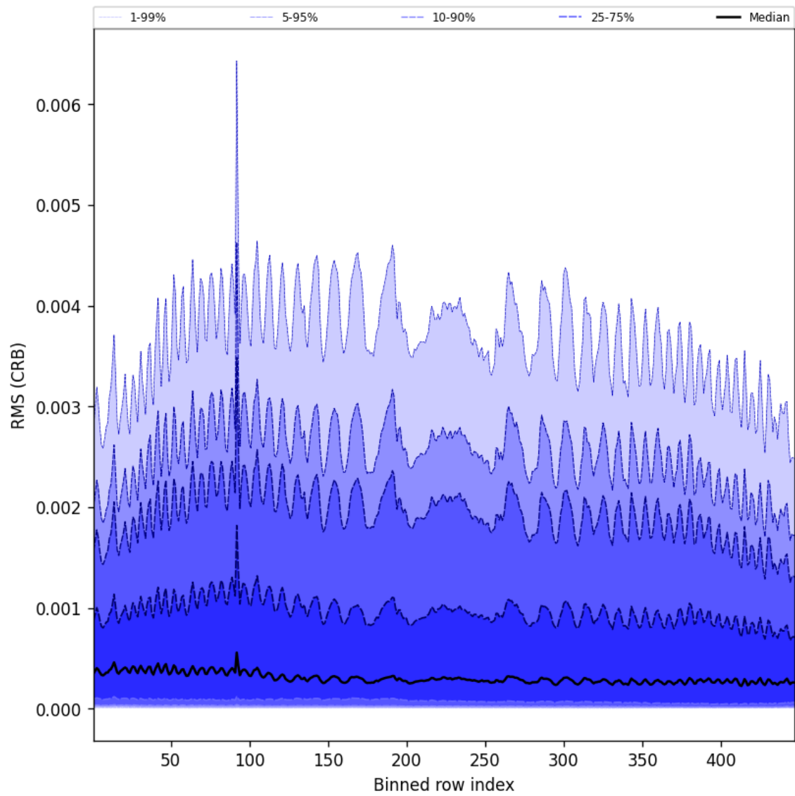
Figure 62: Along track statistics of “RMS (CRB)” for 2025-05-02 to 2025-05-02
