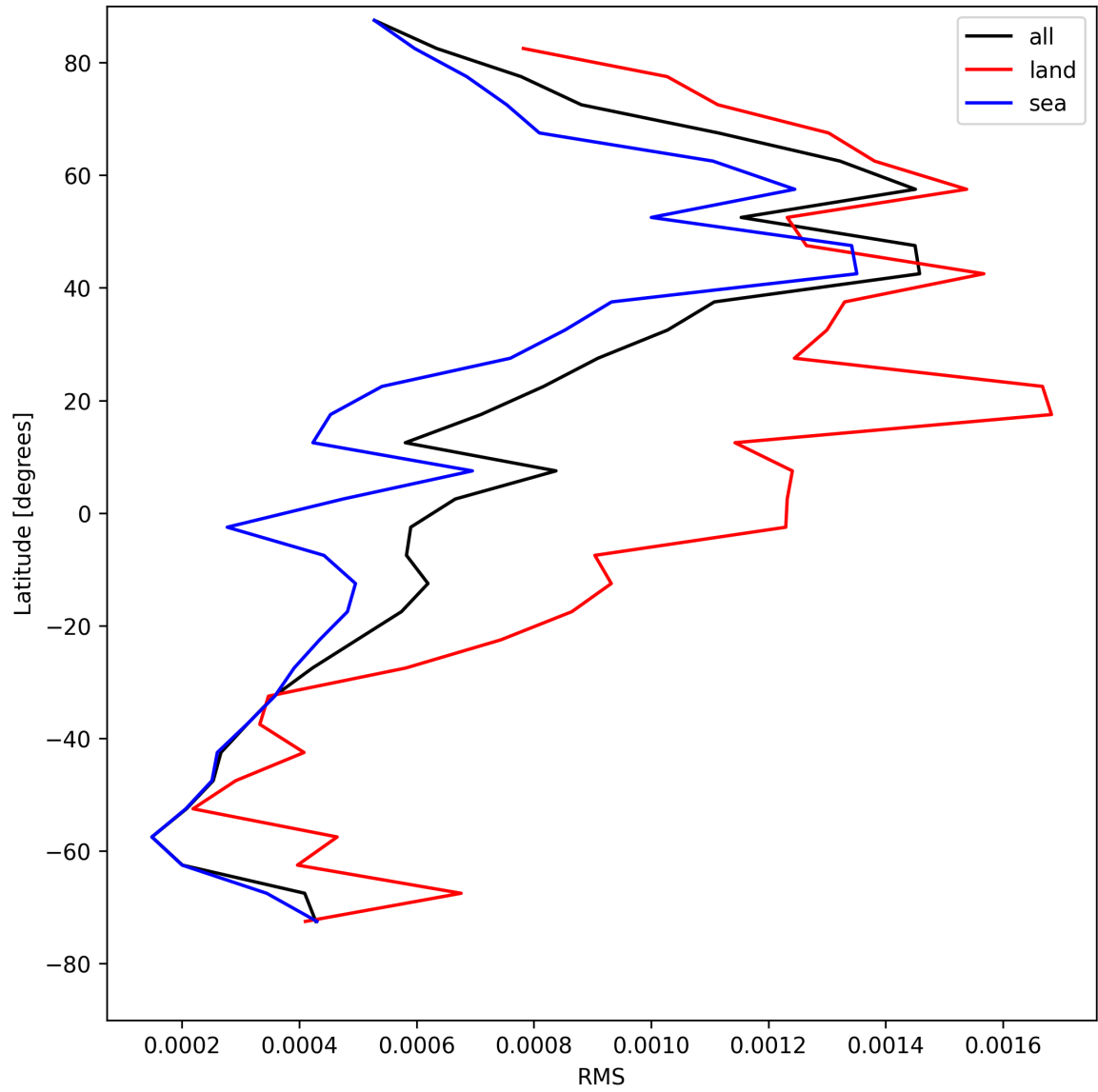
Figure 29: Zonal average of “RMS” for 2025-05-02 to 2025-05-02.
