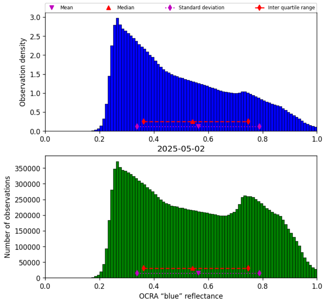
Figure 49: Histogram of “OCRA “blue” reflectance” for 2025-05-02 to 2025-05-02
