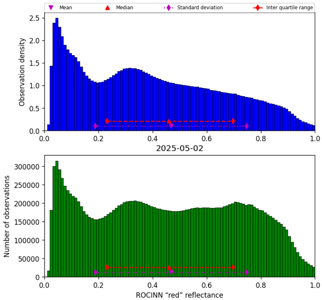
Figure 51: Histogram of “ROCINN “red” reflectance” for 2025-05-02 to 2025-05-02
