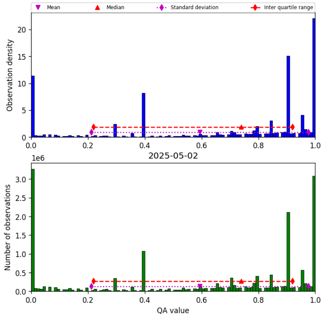
Figure 36: Histogram of “QA value” for 2025-05-02 to 2025-05-02
