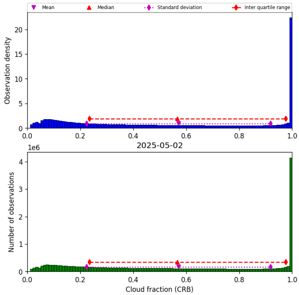
Figure 40: Histogram of “Cloud fraction (CRB)” for 2025-05-02 to 2025-05-02
