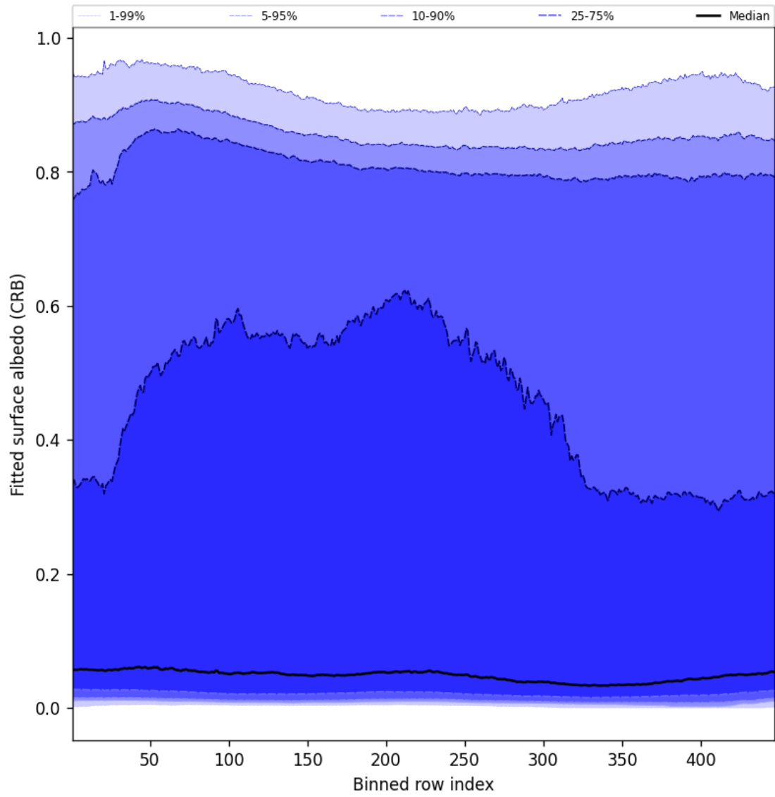
Figure 60: Along track statistics of “Fitted surface albedo (CRB)” for 2025-05-02 to 2025-05-02
