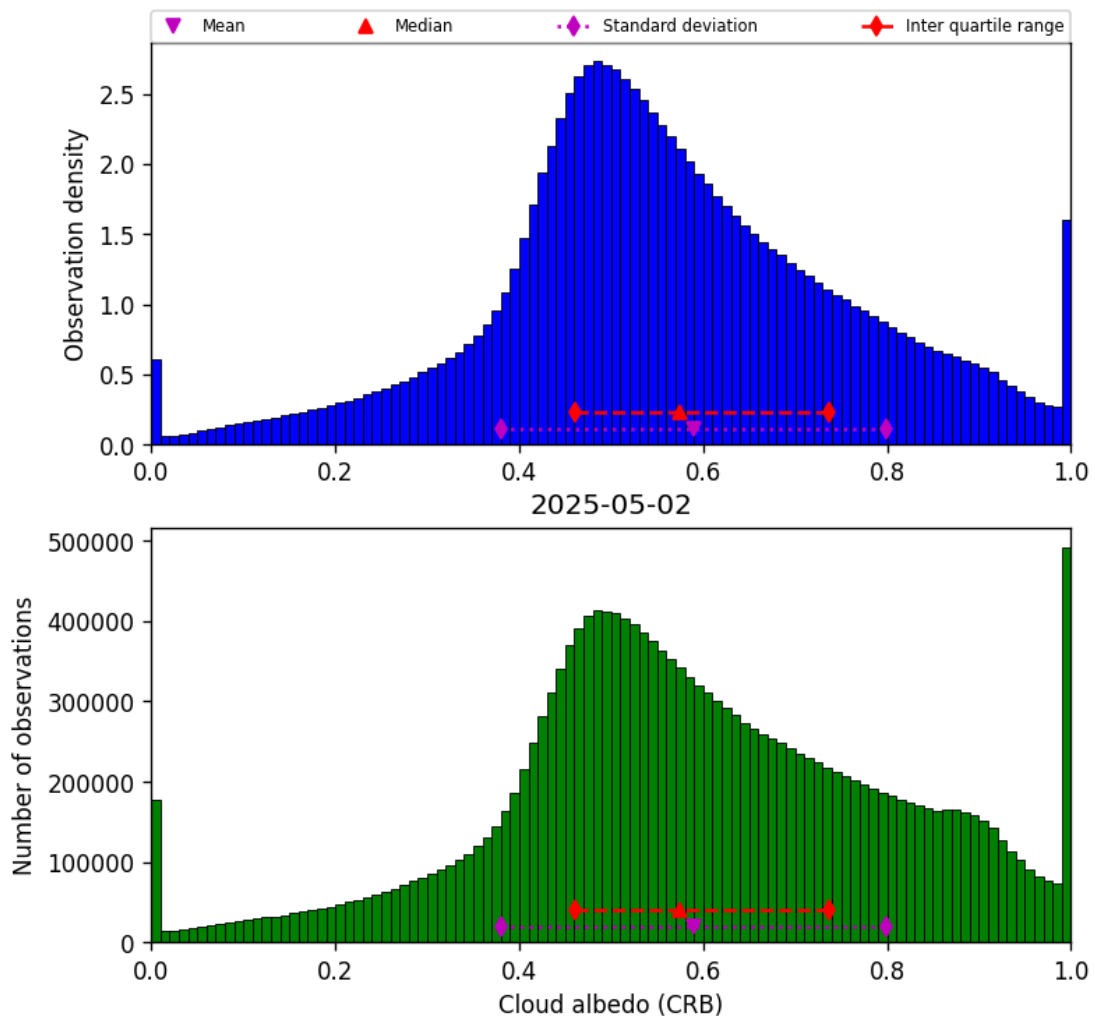
Figure 42: Histogram of “Cloud albedo (CRB)” for 2025-05-02 to 2025-05-02
