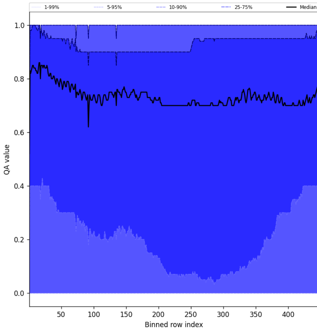
Figure 52: Along track statistics of “QA value” for 2025-05-02 to 2025-05-02
