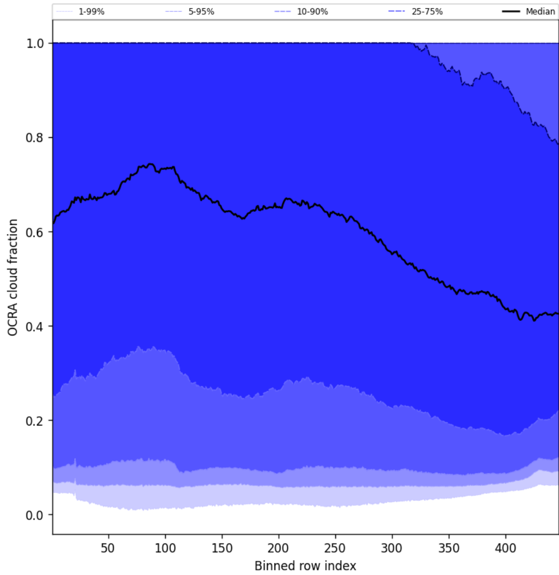
Figure 64: Along track statistics of “OCRA cloud fraction” for 2025-05-02 to 2025-05-02
