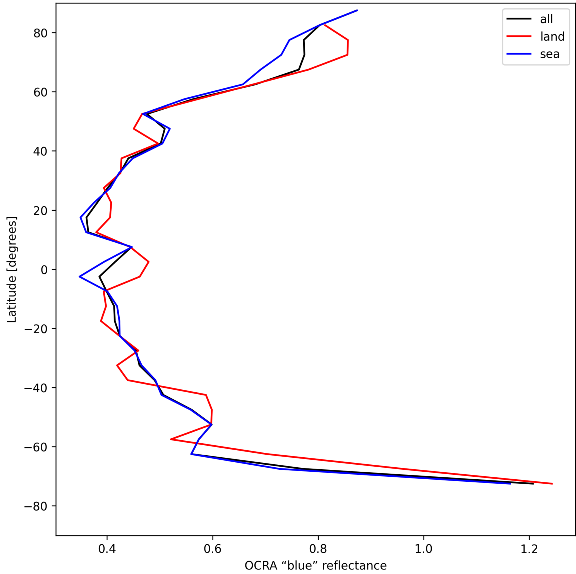
Figure 33: Zonal average of “OCRA “blue” reflectance” for 2025-05-02 to 2025-05-02.
