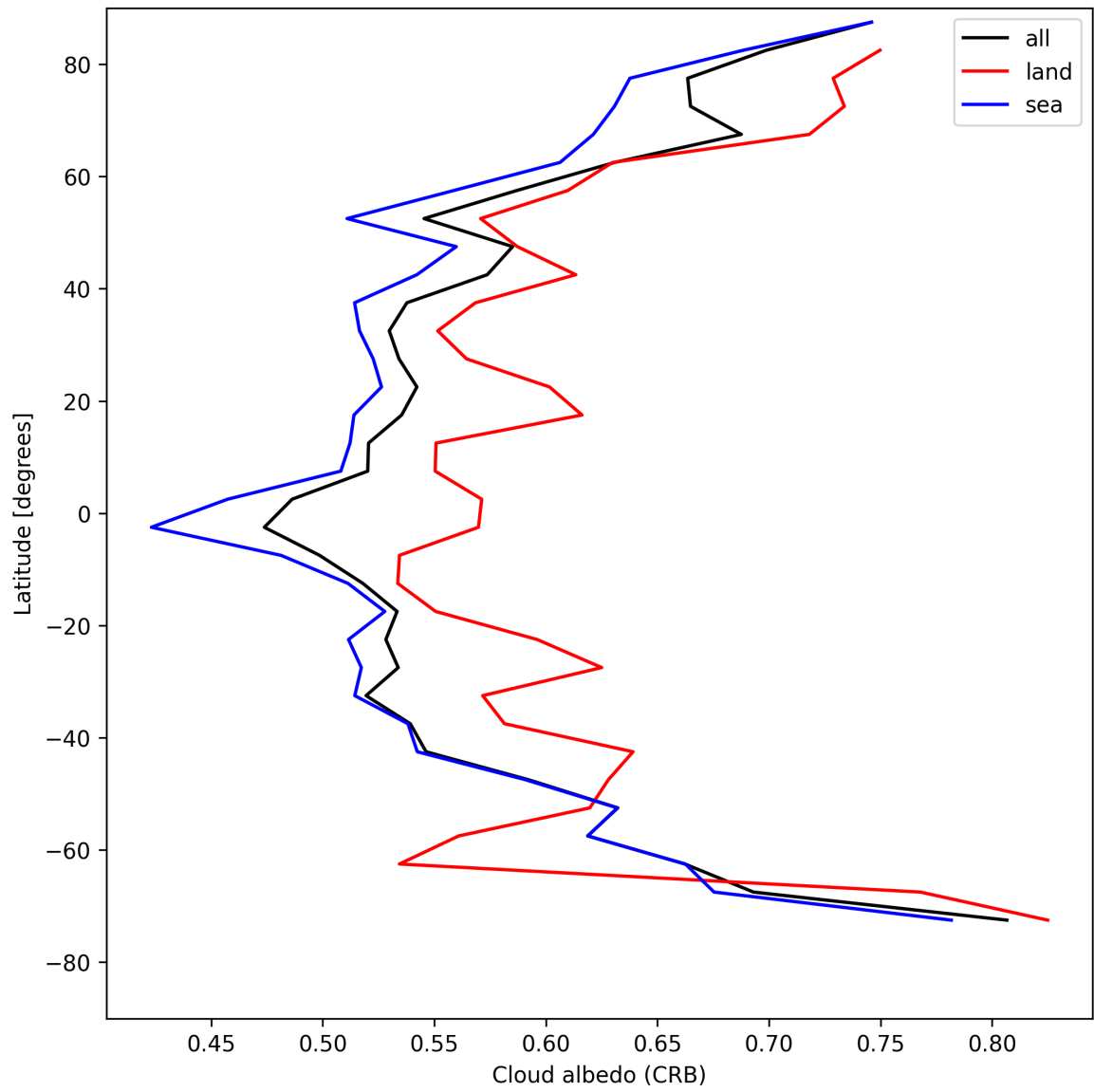
Figure 26: Zonal average of “Cloud albedo (CRB)” for 2025-05-02 to 2025-05-02.
