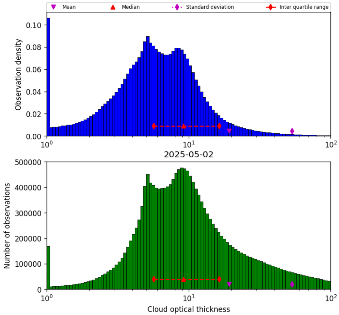
Figure 39: Histogram of “Cloud optical thickness” for 2025-05-02 to 2025-05-02
