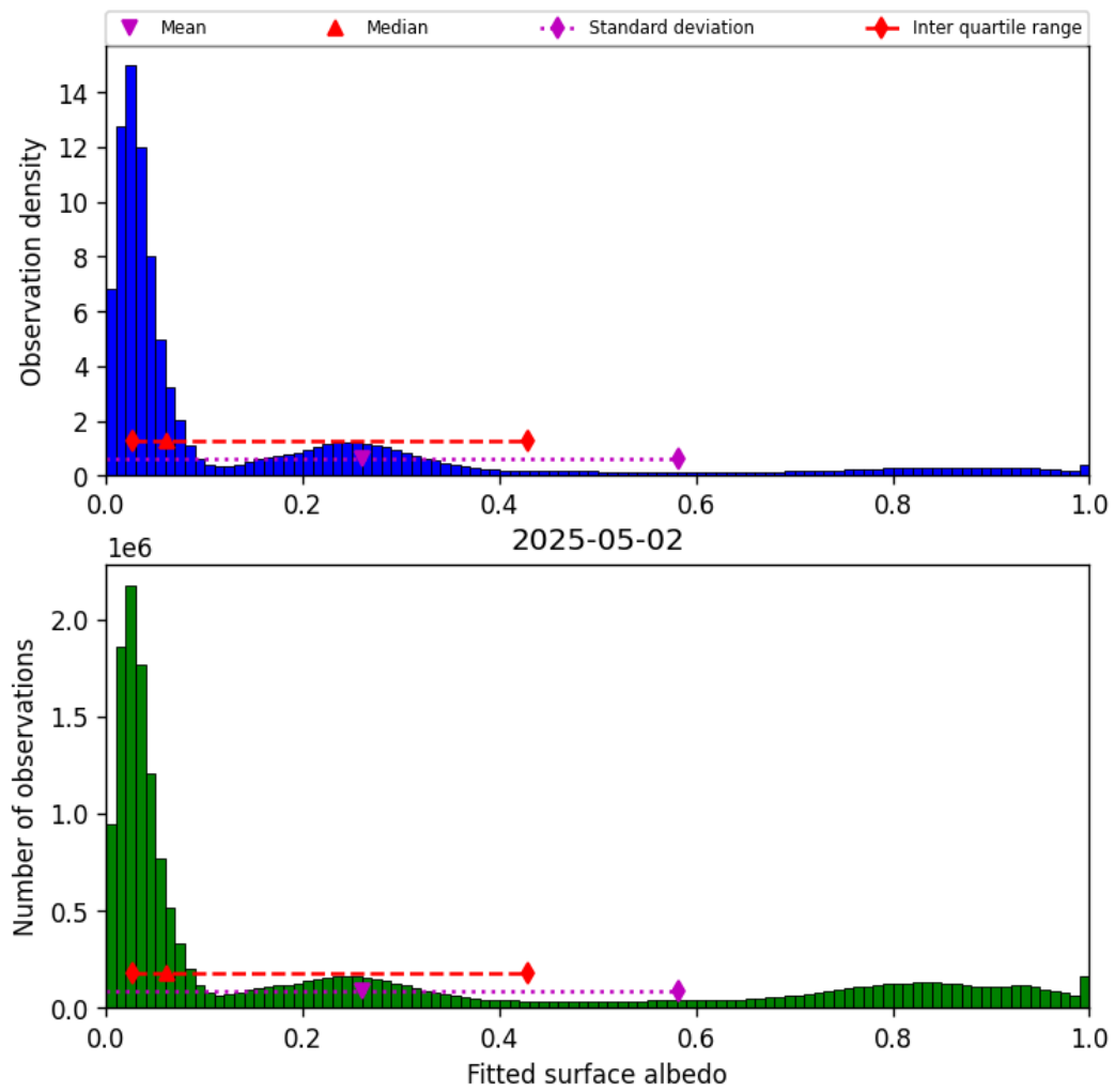
Figure 43: Histogram of “Fitted surface albedo” for 2025-05-02 to 2025-05-02
