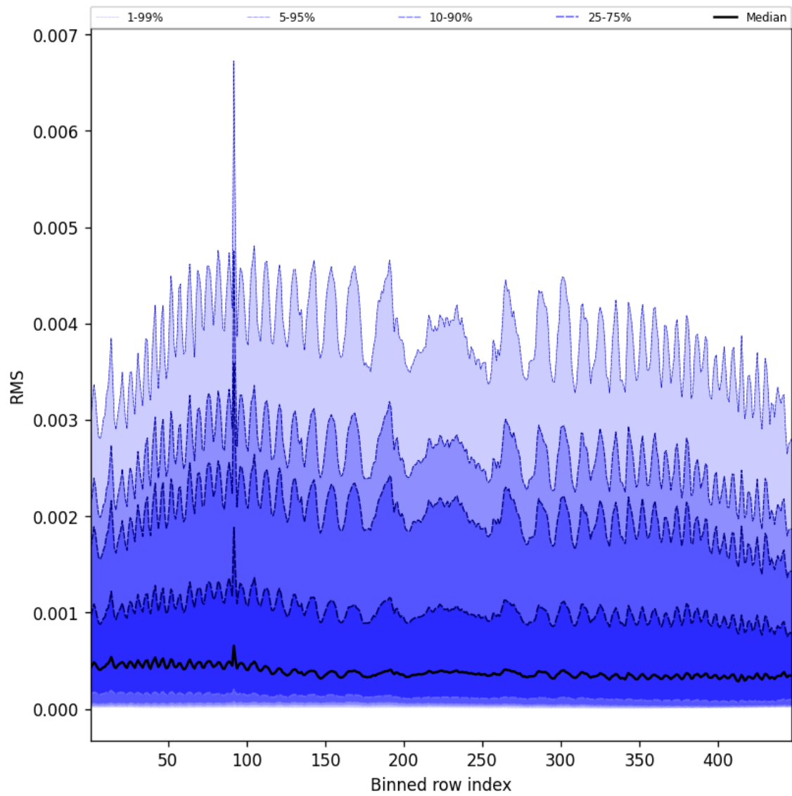
Figure 61: Along track statistics of “RMS” for 2025-05-02 to 2025-05-02
