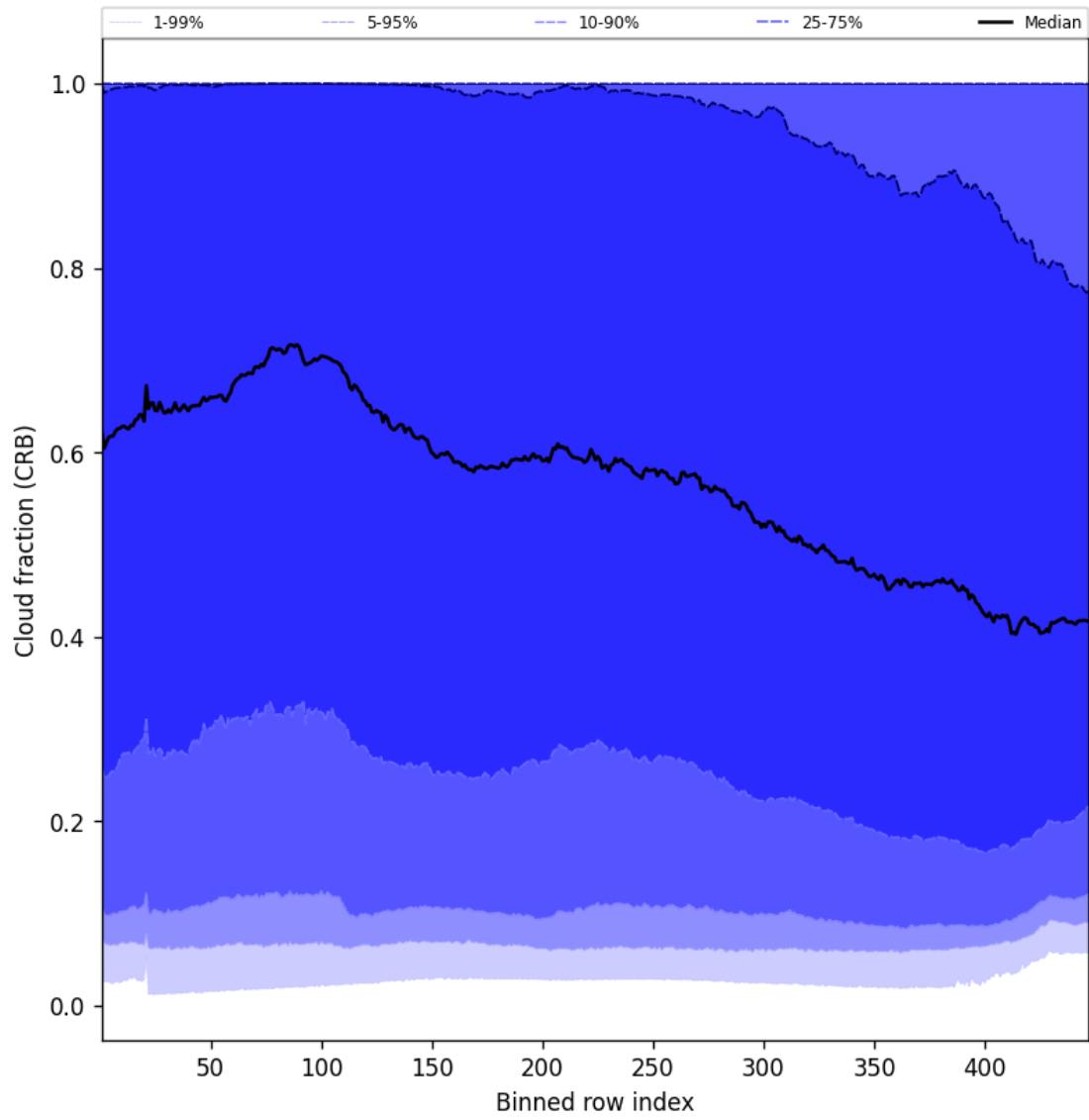
Figure 56: Along track statistics of “Cloud fraction (CRB)” for 2025-05-02 to 2025-05-02
