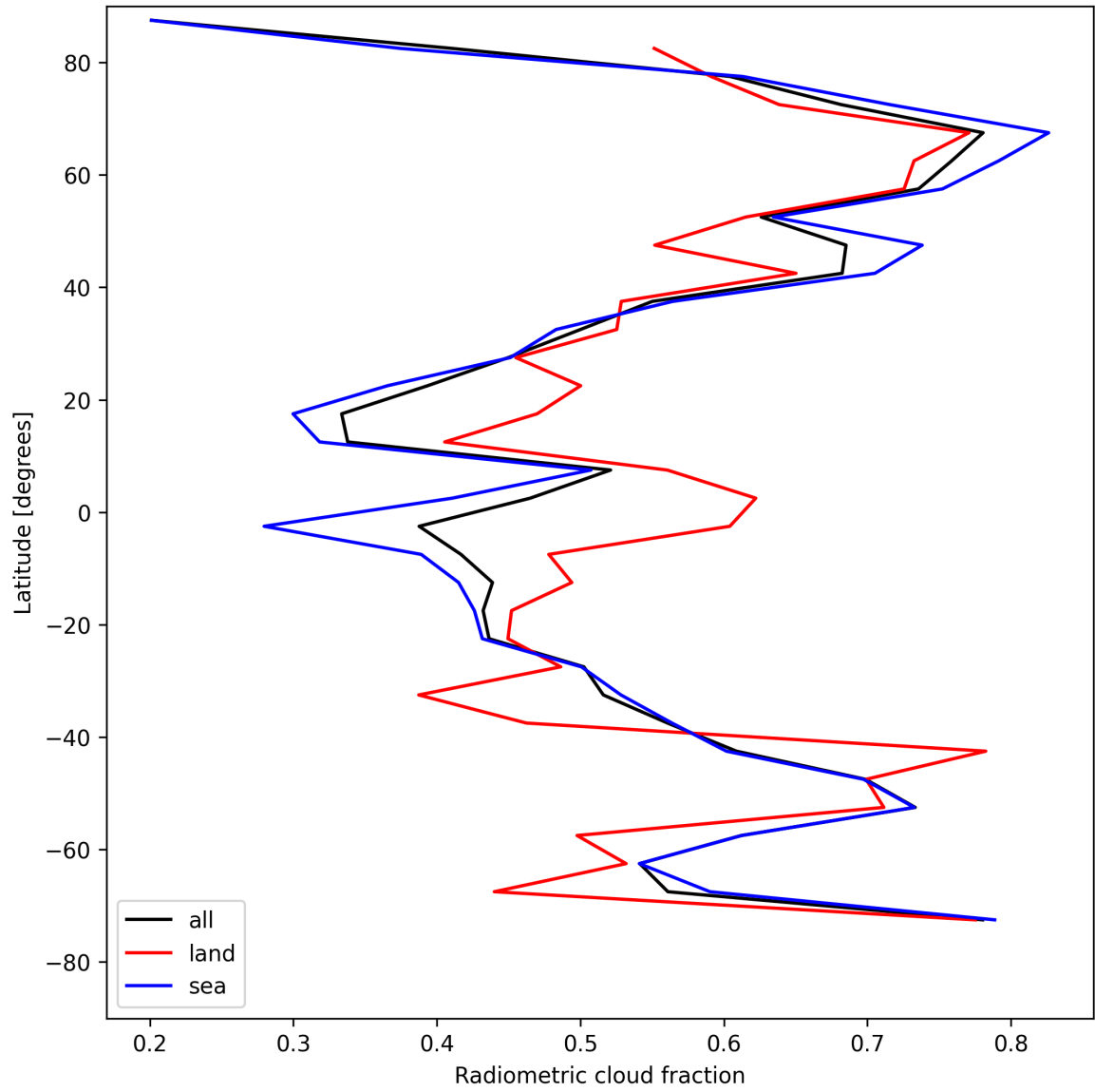
Figure 21: Zonal average of “Radiometric cloud fraction” for 2025-05-02 to 2025-05-02.
