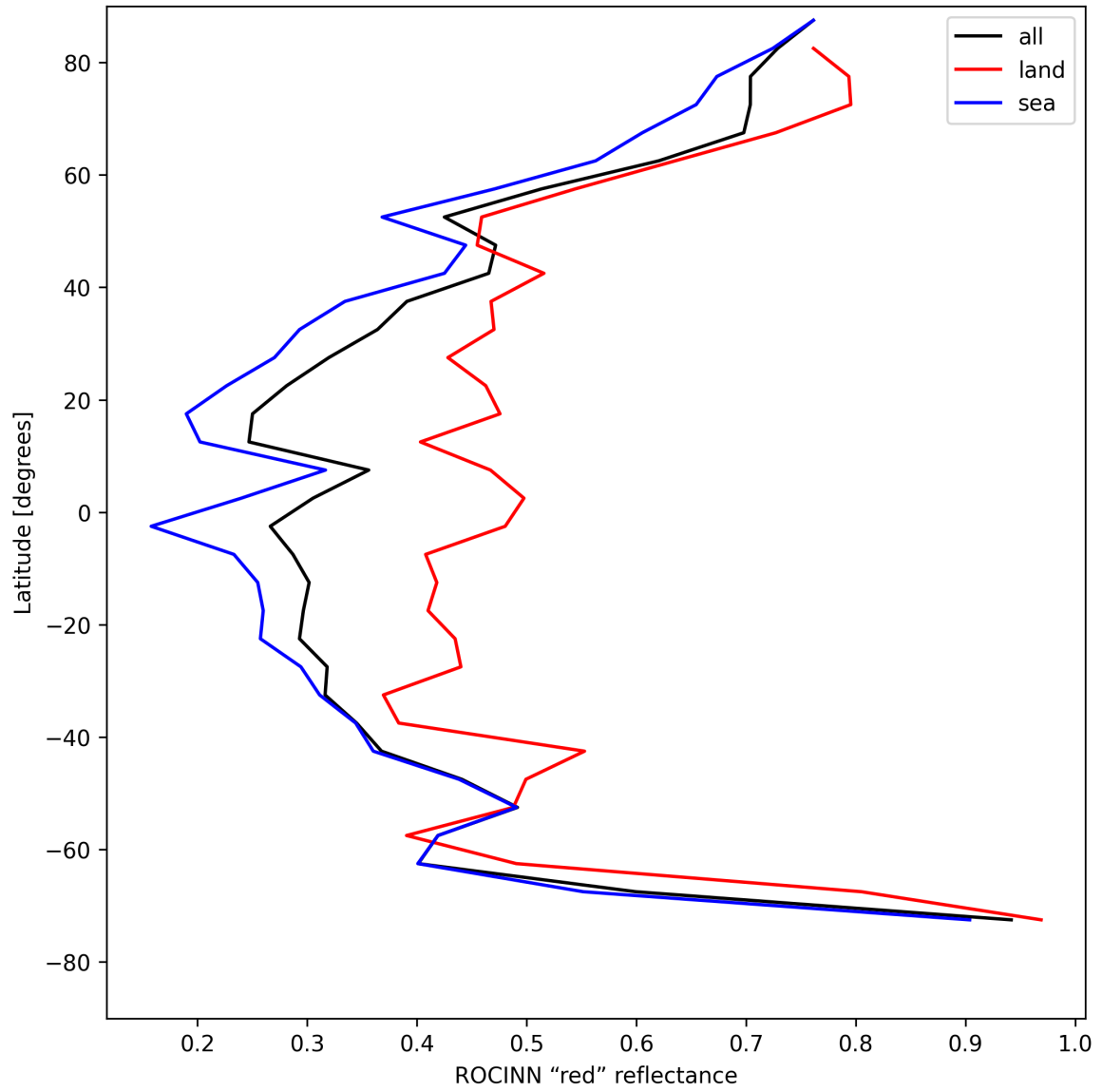
Figure 35: Zonal average of “ROCINN “red” reflectance” for 2025-05-02 to 2025-05-02.
