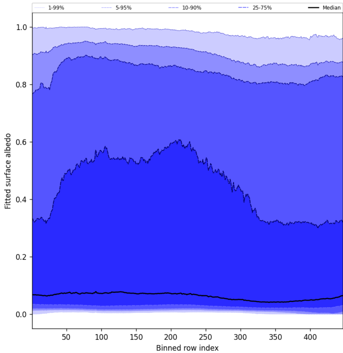
Figure 59: Along track statistics of “Fitted surface albedo” for 2025-05-02 to 2025-05-02
