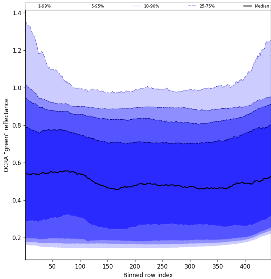
Figure 66: Along track statistics of “OCRA “green” reflectance” for 2025-05-02 to 2025-05-02
