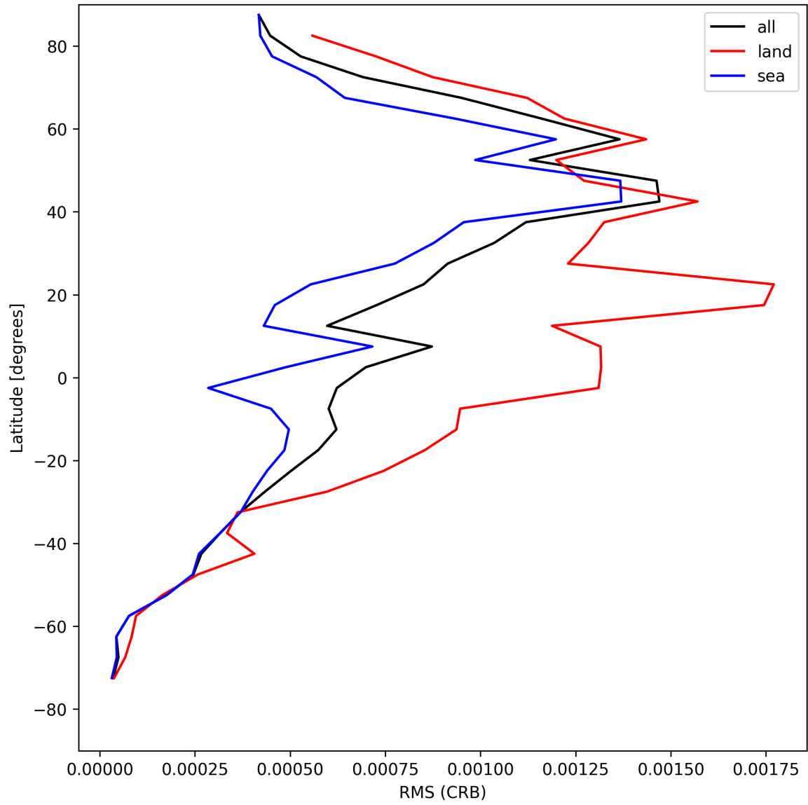
Figure 30: Zonal average of “RMS (CRB)” for 2025-05-02 to 2025-05-02.
