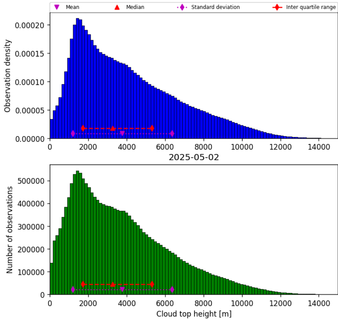
Figure 38: Histogram of “Cloud top height” for 2025-05-02 to 2025-05-02
