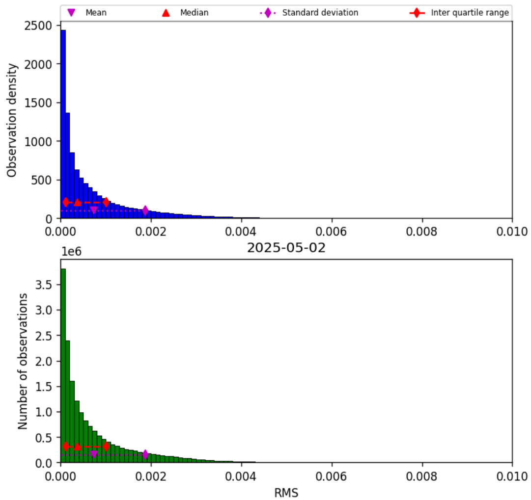
Figure 45: Histogram of “RMS” for 2025-05-02 to 2025-05-02
