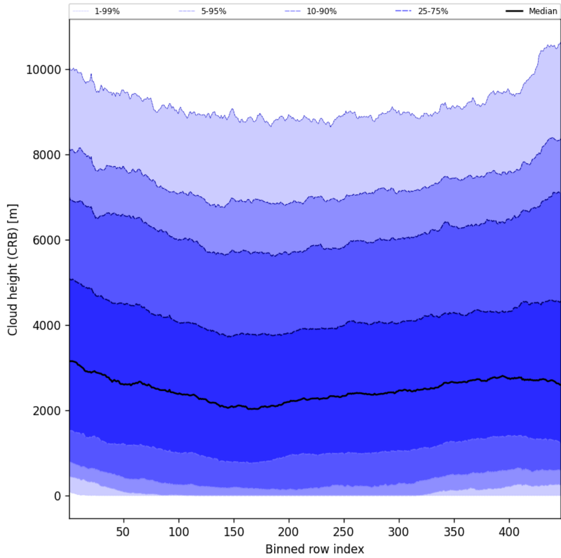
Figure 57: Along track statistics of “Cloud height (CRB)” for 2025-05-02 to 2025-05-02
