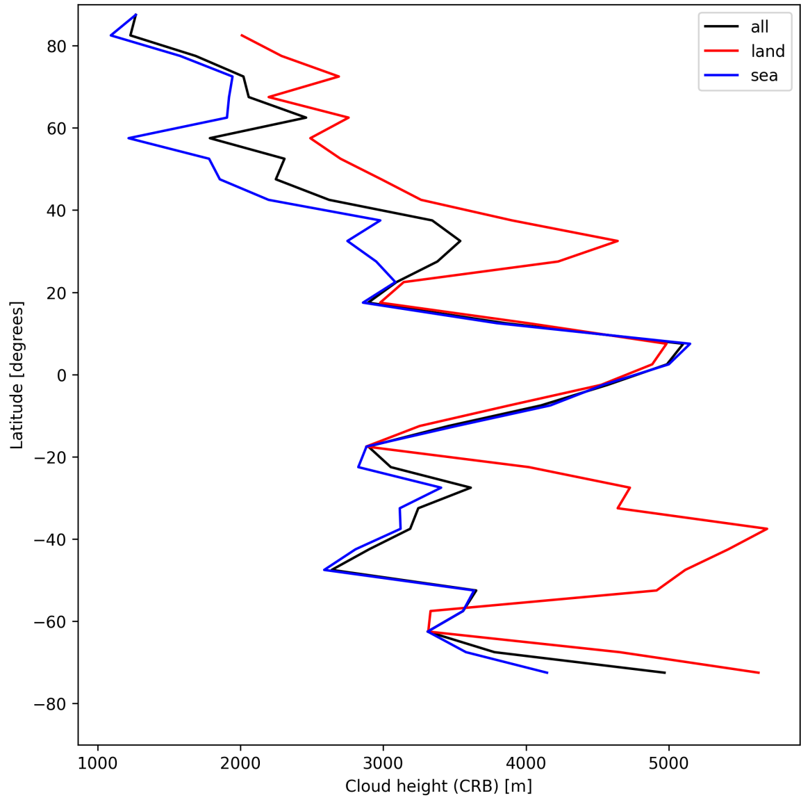
Figure 25: Zonal average of “Cloud height (CRB)” for 2025-05-02 to 2025-05-02.
