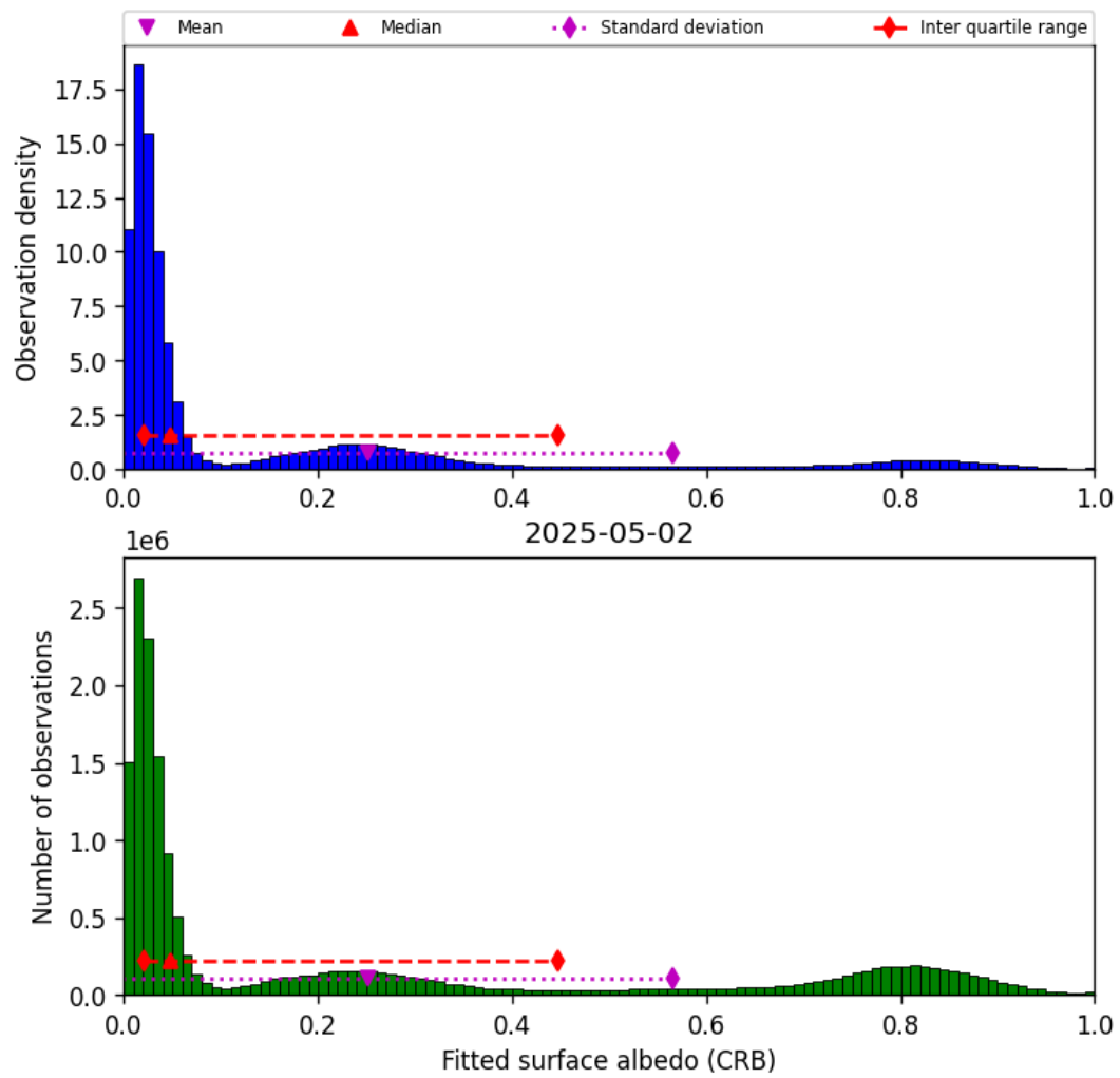
Figure 44: Histogram of “Fitted surface albedo (CRB)” for 2025-05-02 to 2025-05-02
