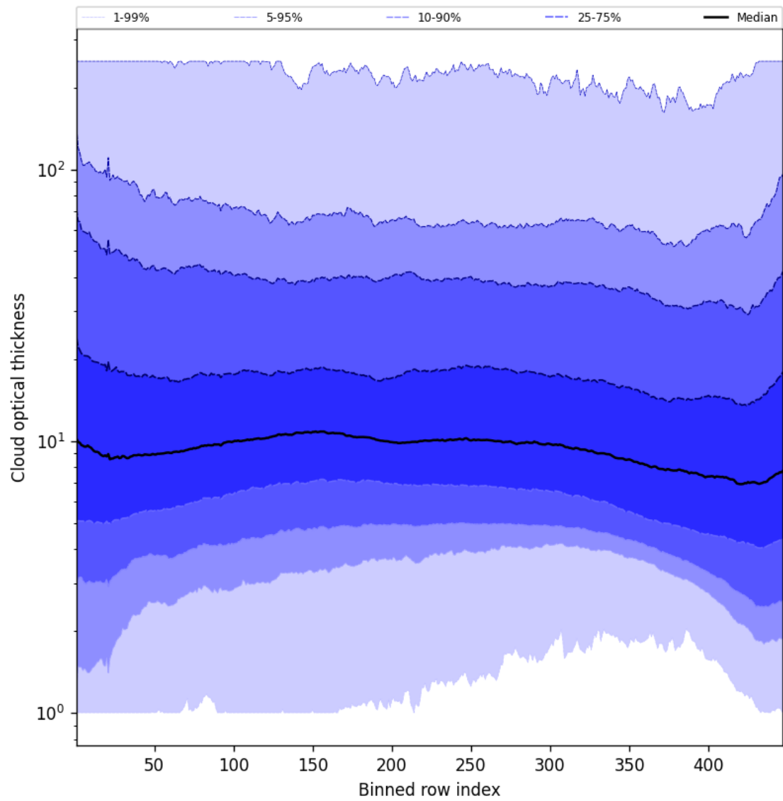
Figure 55: Along track statistics of “Cloud optical thickness” for 2025-05-04 to 2025-05-05
