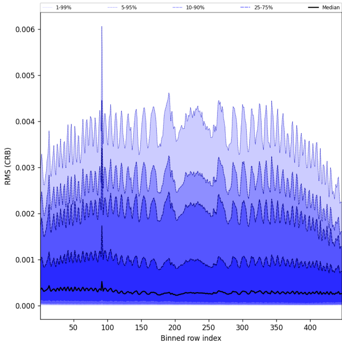
Figure 62: Along track statistics of “RMS (CRB)” for 2025-05-04 to 2025-05-05
