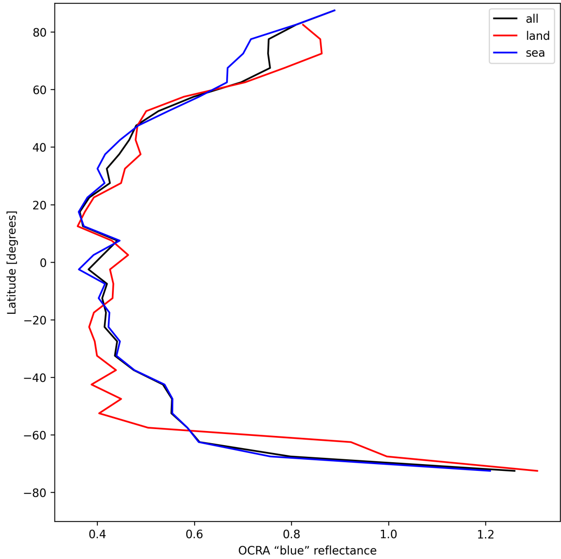
Figure 33: Zonal average of “OCRA “blue” reflectance” for 2025-05-04 to 2025-05-05.
