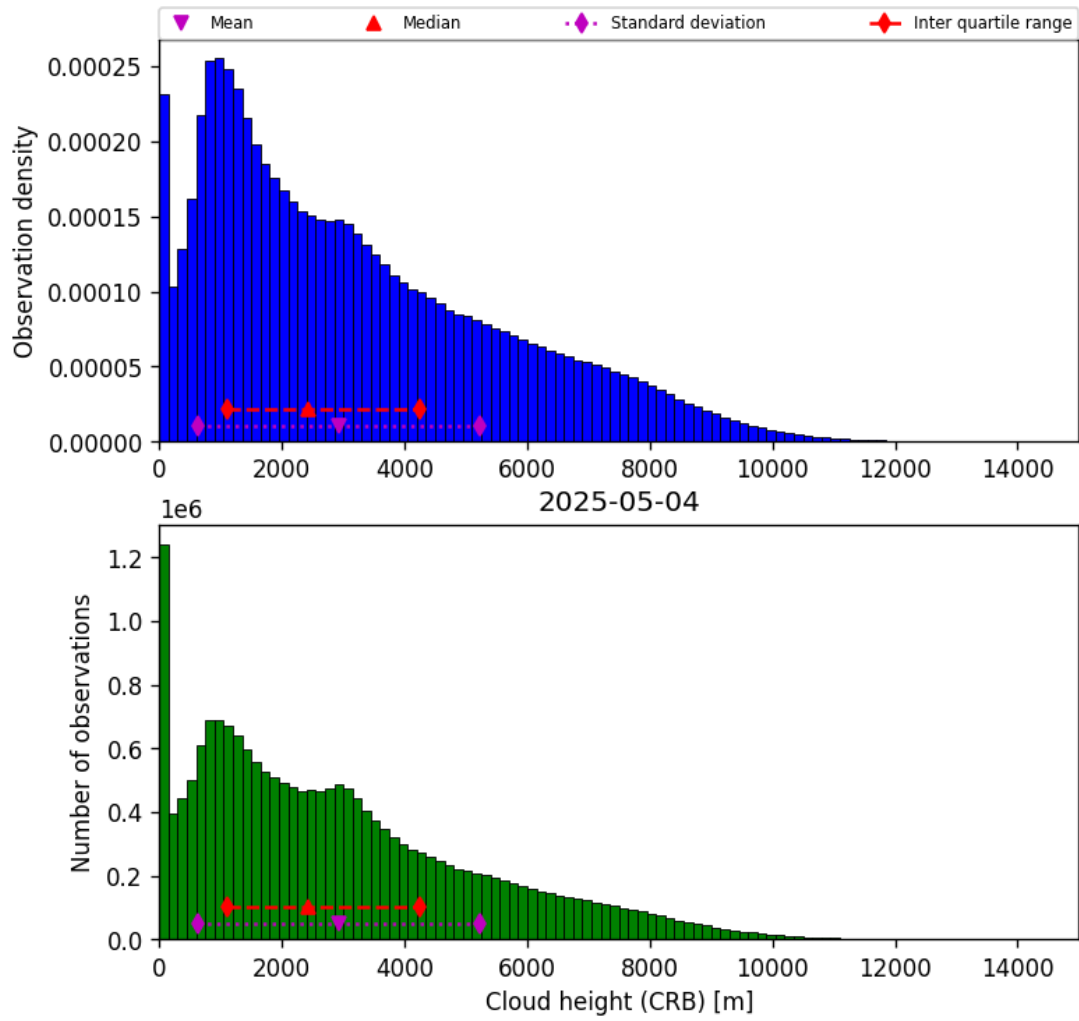
Figure 41: Histogram of “Cloud height (CRB)” for 2025-05-04 to 2025-05-05
