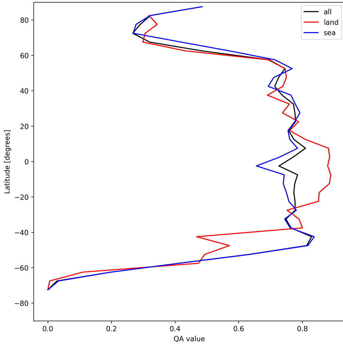
Figure 20: Zonal average of “QA value” for 2025-05-04 to 2025-05-05.
