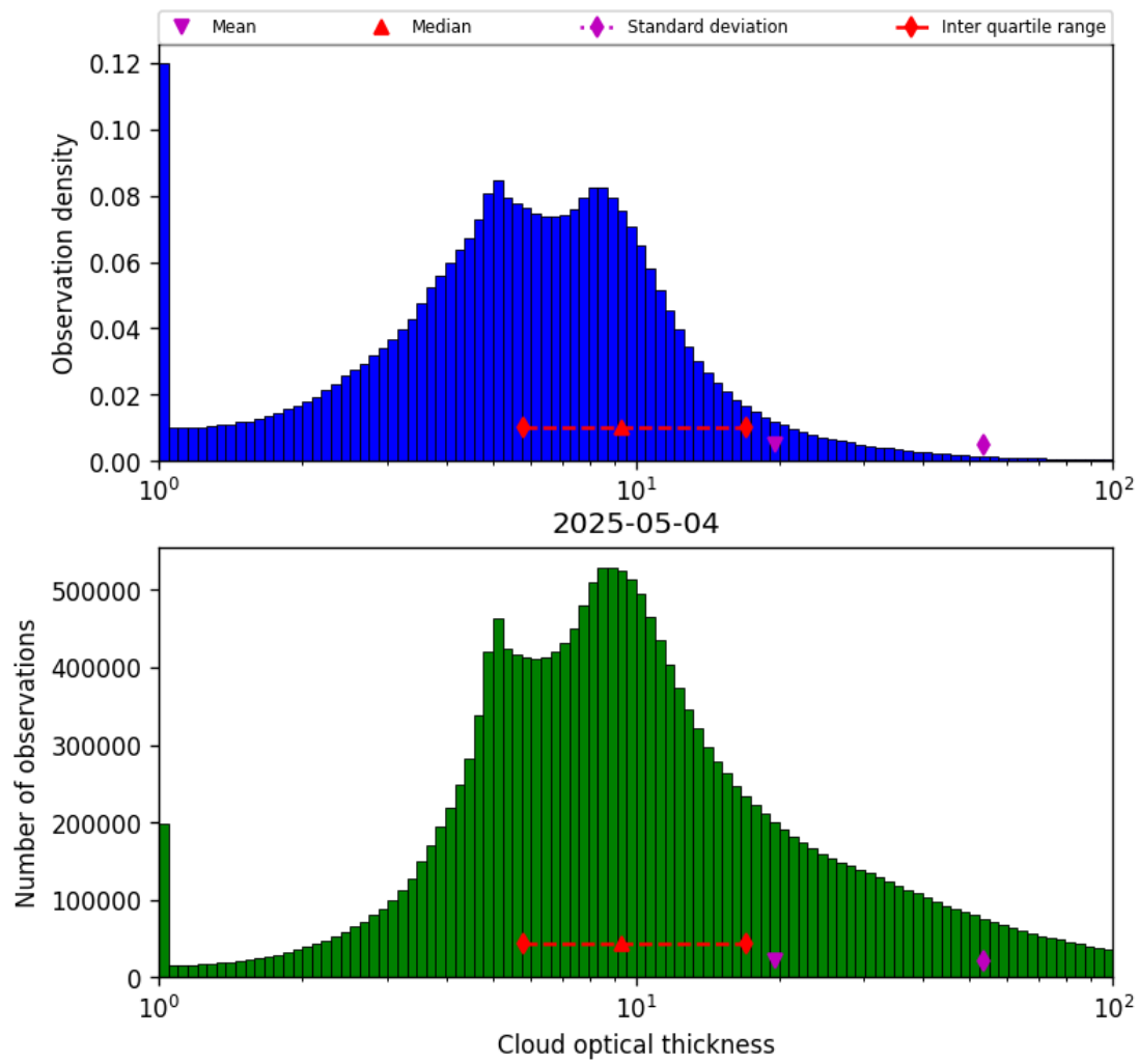
Figure 39: Histogram of “Cloud optical thickness” for 2025-05-04 to 2025-05-05
