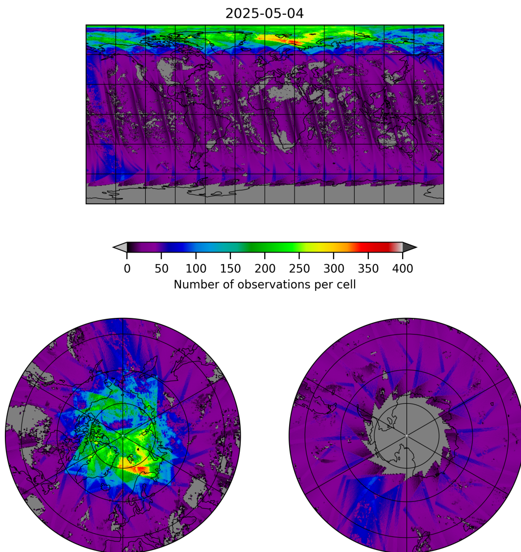
Figure 19: Map of the number of observations for 2025-05-04 to 2025-05-05
