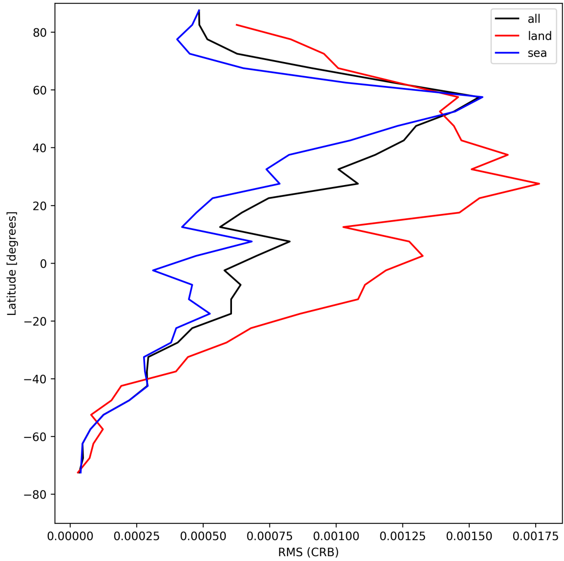
Figure 30: Zonal average of “RMS (CRB)” for 2025-05-04 to 2025-05-05.
