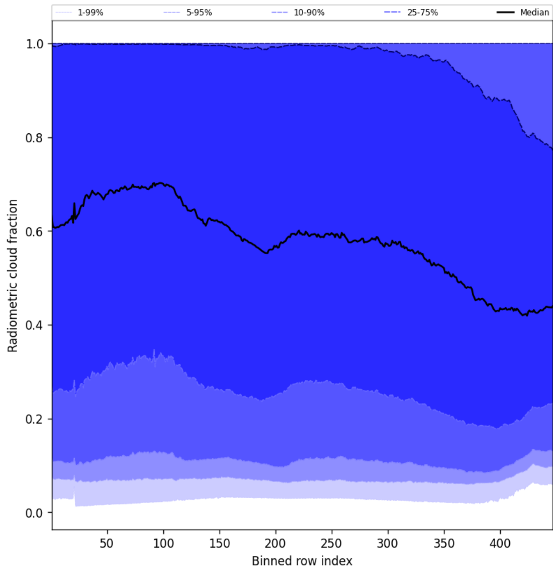
Figure 53: Along track statistics of “Radiometric cloud fraction” for 2025-05-04 to 2025-05-05
