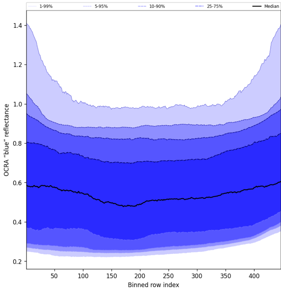
Figure 65: Along track statistics of “OCRA “blue” reflectance” for 2025-05-04 to 2025-05-05
