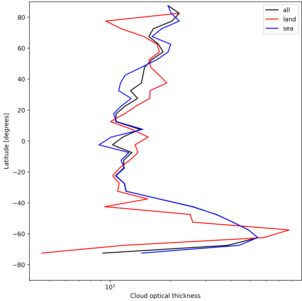
Figure 23: Zonal average of “Cloud optical thickness” for 2025-05-04 to 2025-05-05.
