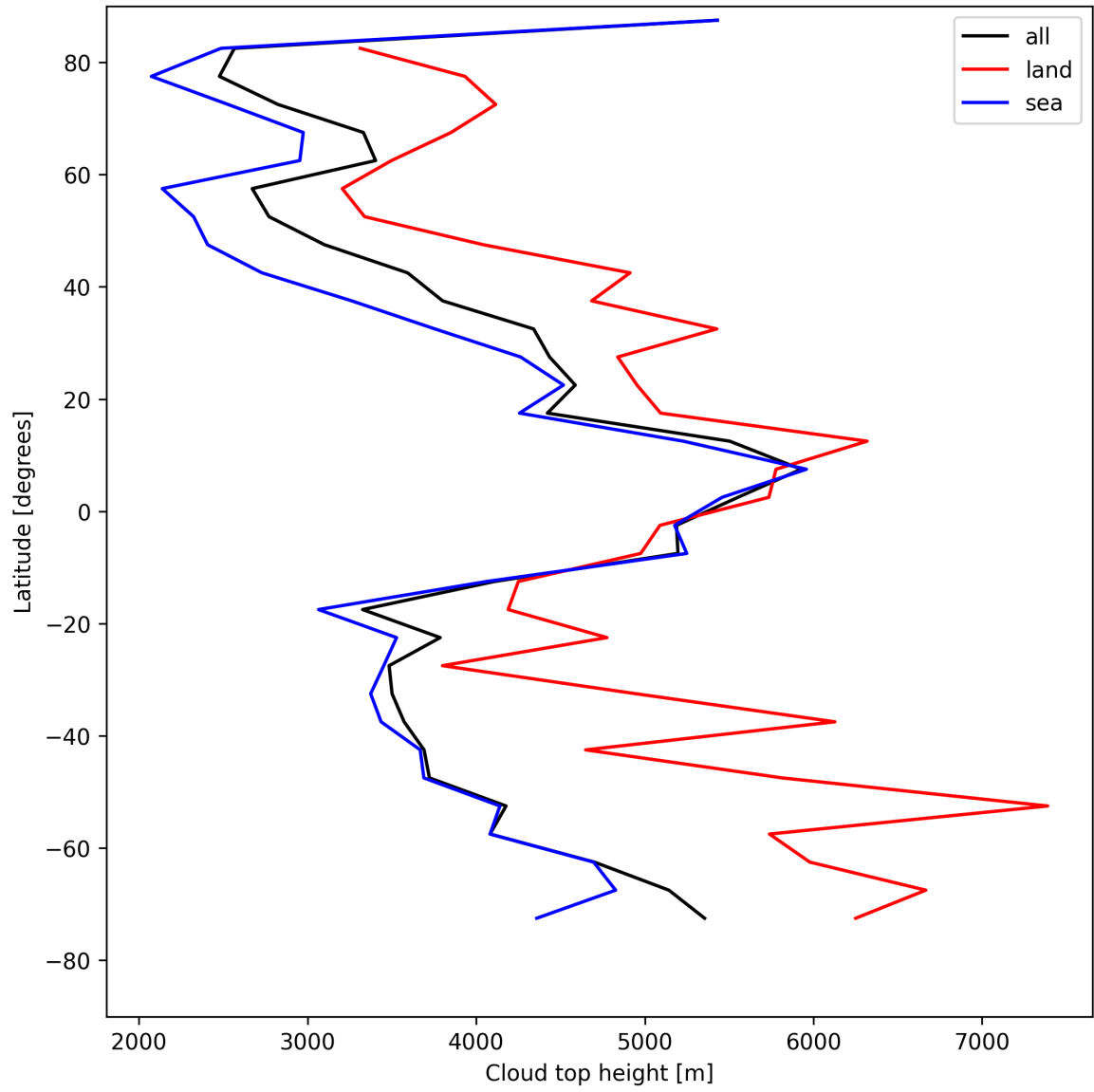
Figure 22: Zonal average of “Cloud top height” for 2025-05-04 to 2025-05-05.
