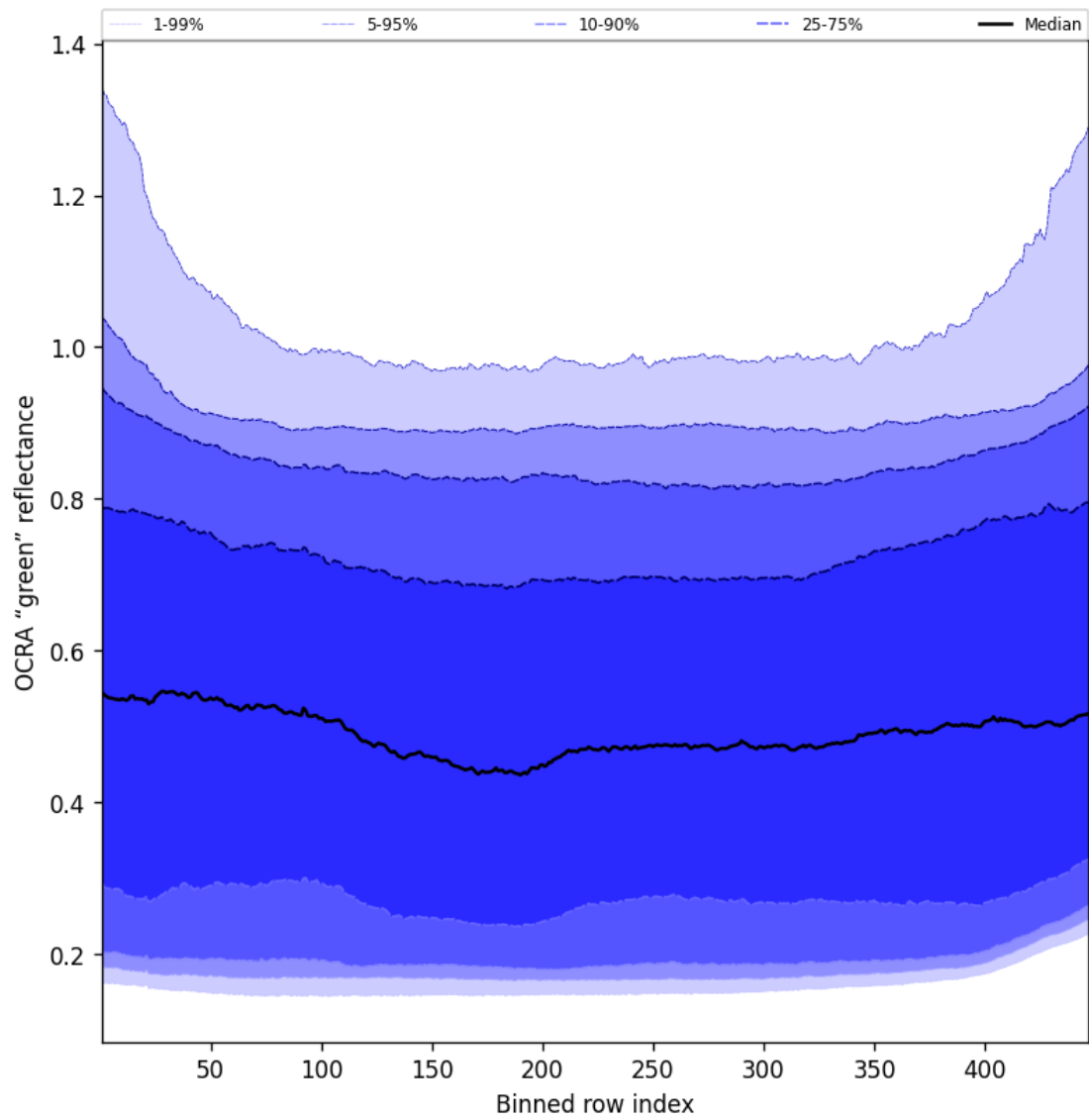
Figure 66: Along track statistics of “OCRA “green” reflectance” for 2025-05-04 to 2025-05-05
