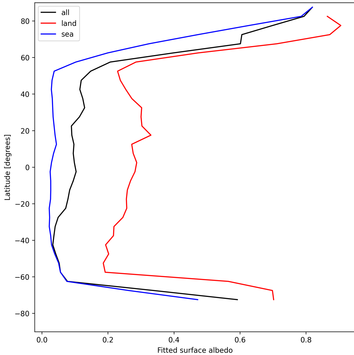
Figure 27: Zonal average of “Fitted surface albedo” for 2025-05-04 to 2025-05-05.
