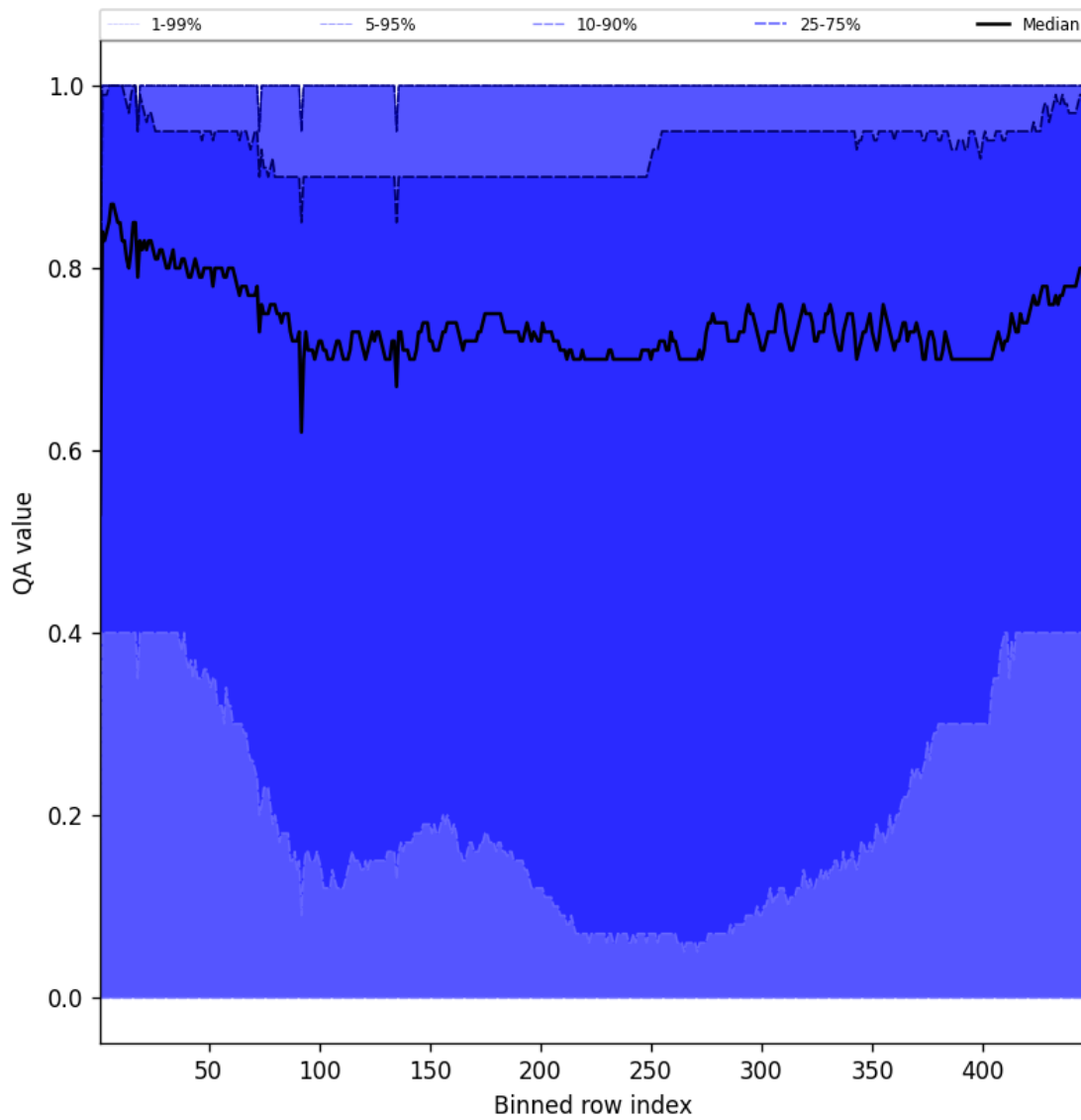
Figure 52: Along track statistics of “QA value” for 2025-05-04 to 2025-05-05
