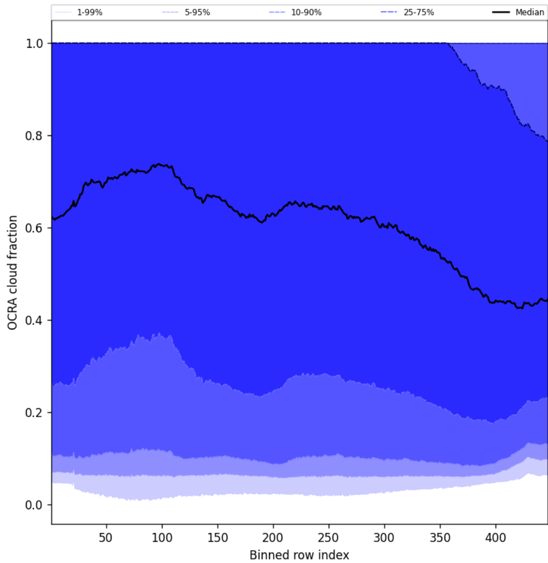
Figure 64: Along track statistics of “OCRA cloud fraction” for 2025-05-04 to 2025-05-05
