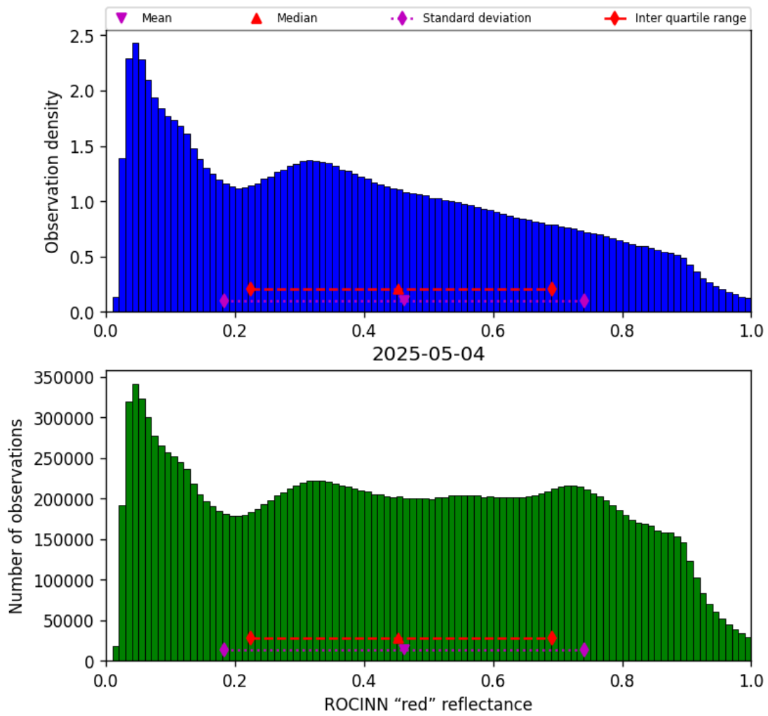
Figure 51: Histogram of “ROCINN “red” reflectance” for 2025-05-04 to 2025-05-05
