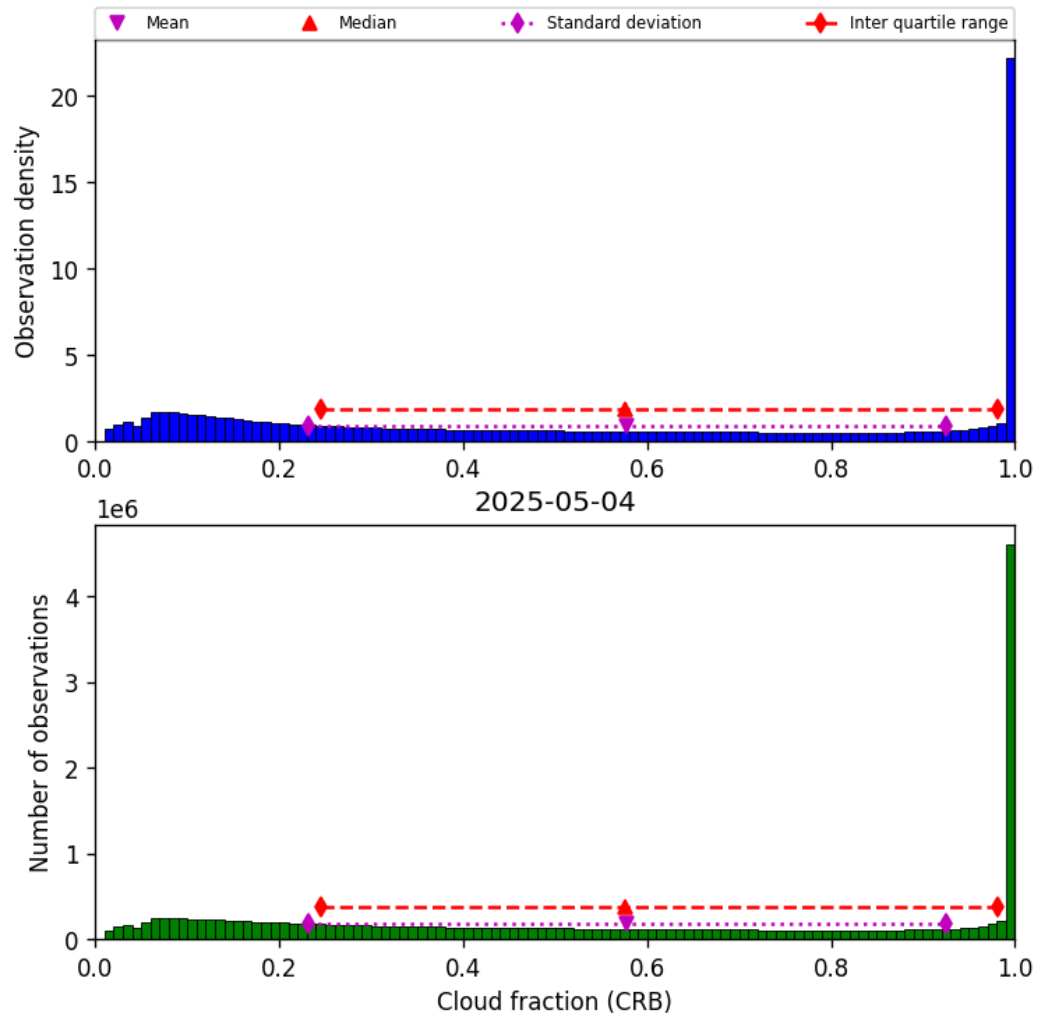
Figure 40: Histogram of “Cloud fraction (CRB)” for 2025-05-04 to 2025-05-05
