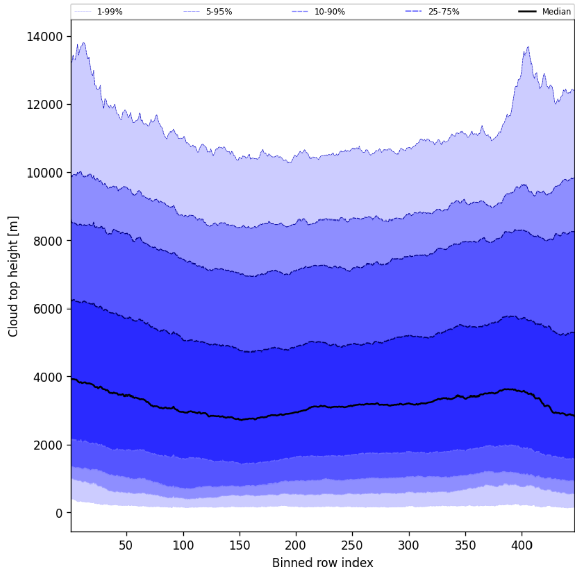
Figure 54: Along track statistics of “Cloud top height” for 2025-05-04 to 2025-05-05
