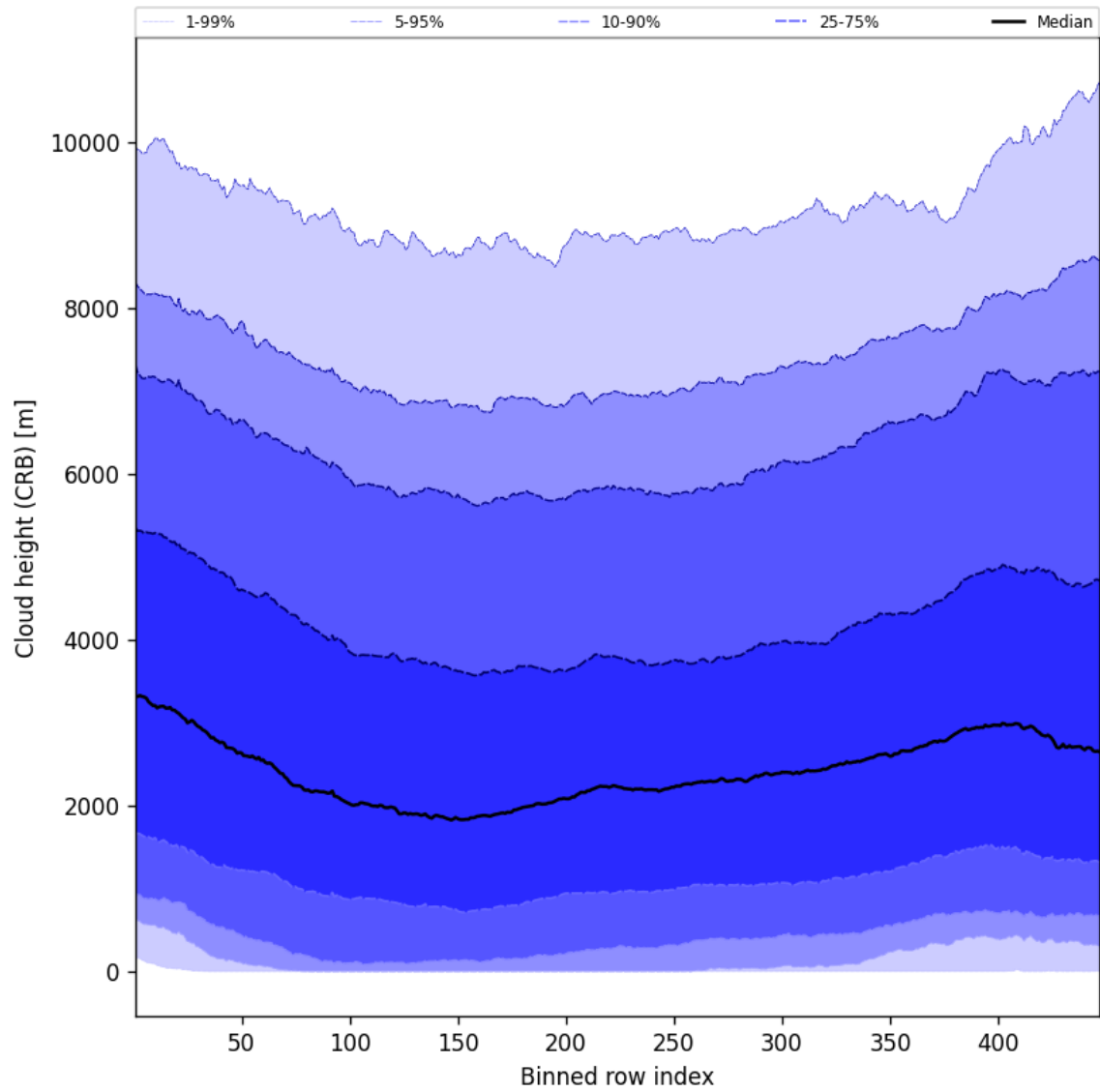
Figure 57: Along track statistics of “Cloud height (CRB)” for 2025-05-04 to 2025-05-05
