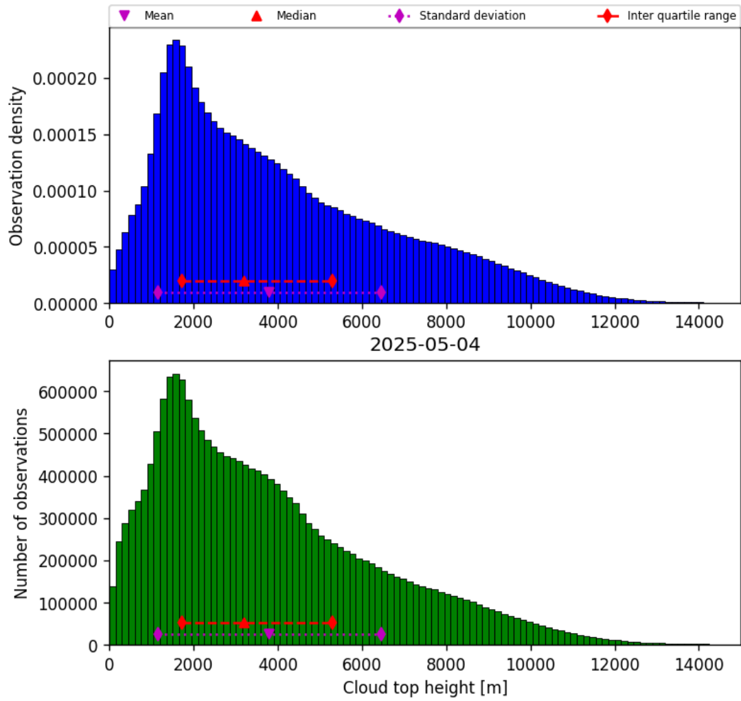
Figure 38: Histogram of “Cloud top height” for 2025-05-04 to 2025-05-05
