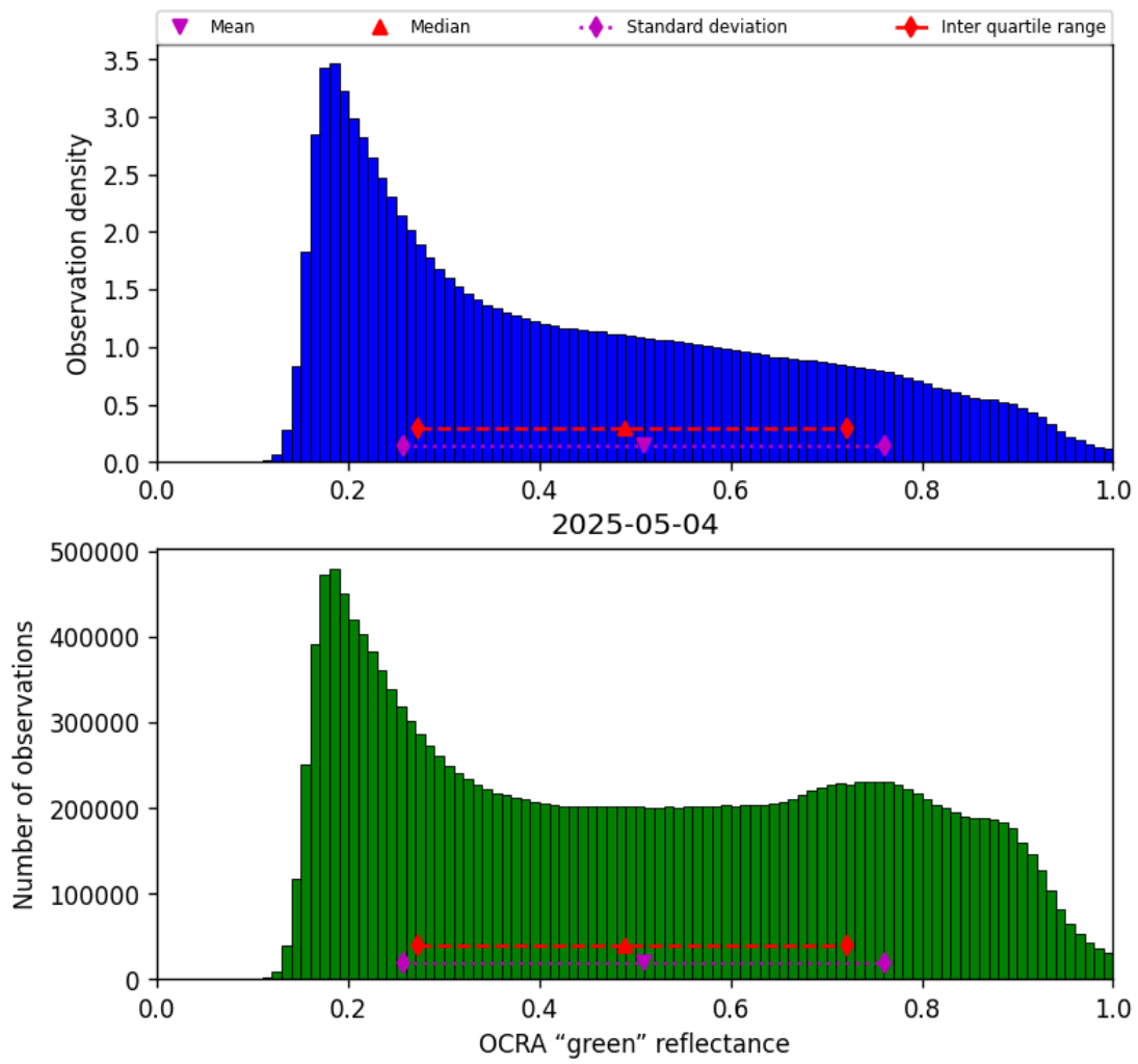
Figure 50: Histogram of “OCRA “green” reflectance” for 2025-05-04 to 2025-05-05
