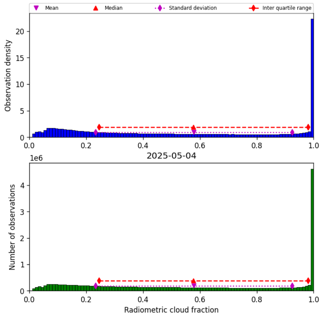
Figure 37: Histogram of “Radiometric cloud fraction” for 2025-05-04 to 2025-05-05
