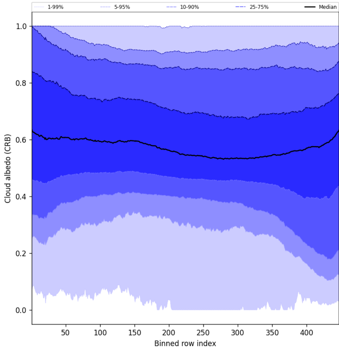
Figure 58: Along track statistics of “Cloud albedo (CRB)” for 2025-05-04 to 2025-05-05
