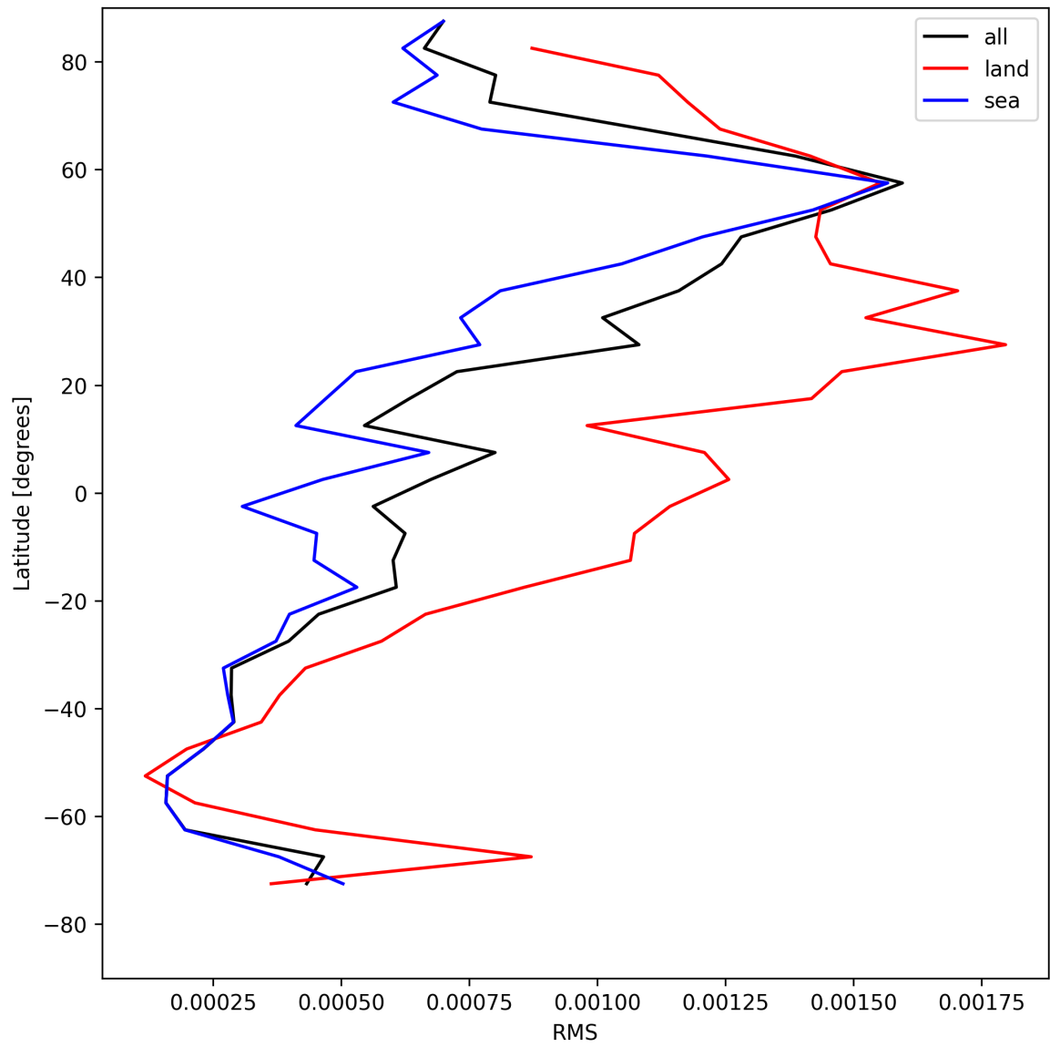
Figure 29: Zonal average of “RMS” for 2025-05-04 to 2025-05-05.
