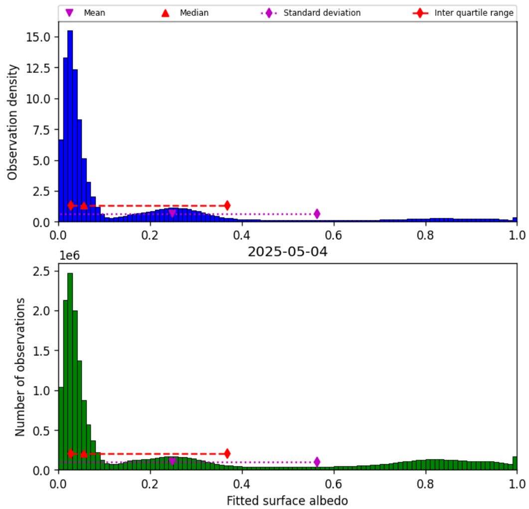
Figure 43: Histogram of “Fitted surface albedo” for 2025-05-04 to 2025-05-05
