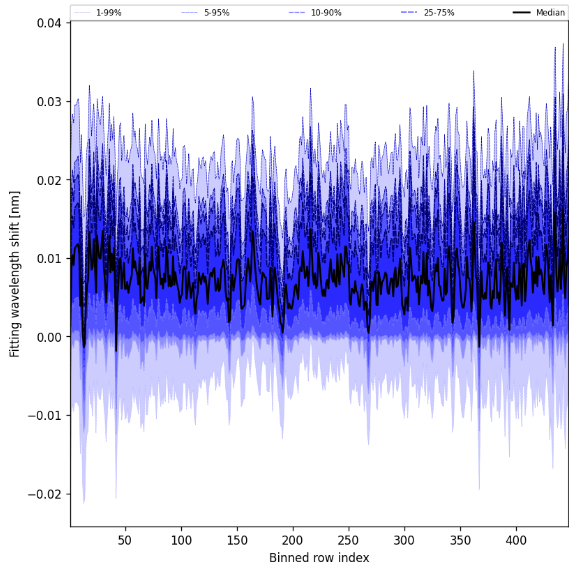
Figure 63: Along track statistics of “Fitting wavelength shift” for 2025-05-04 to 2025-05-05
