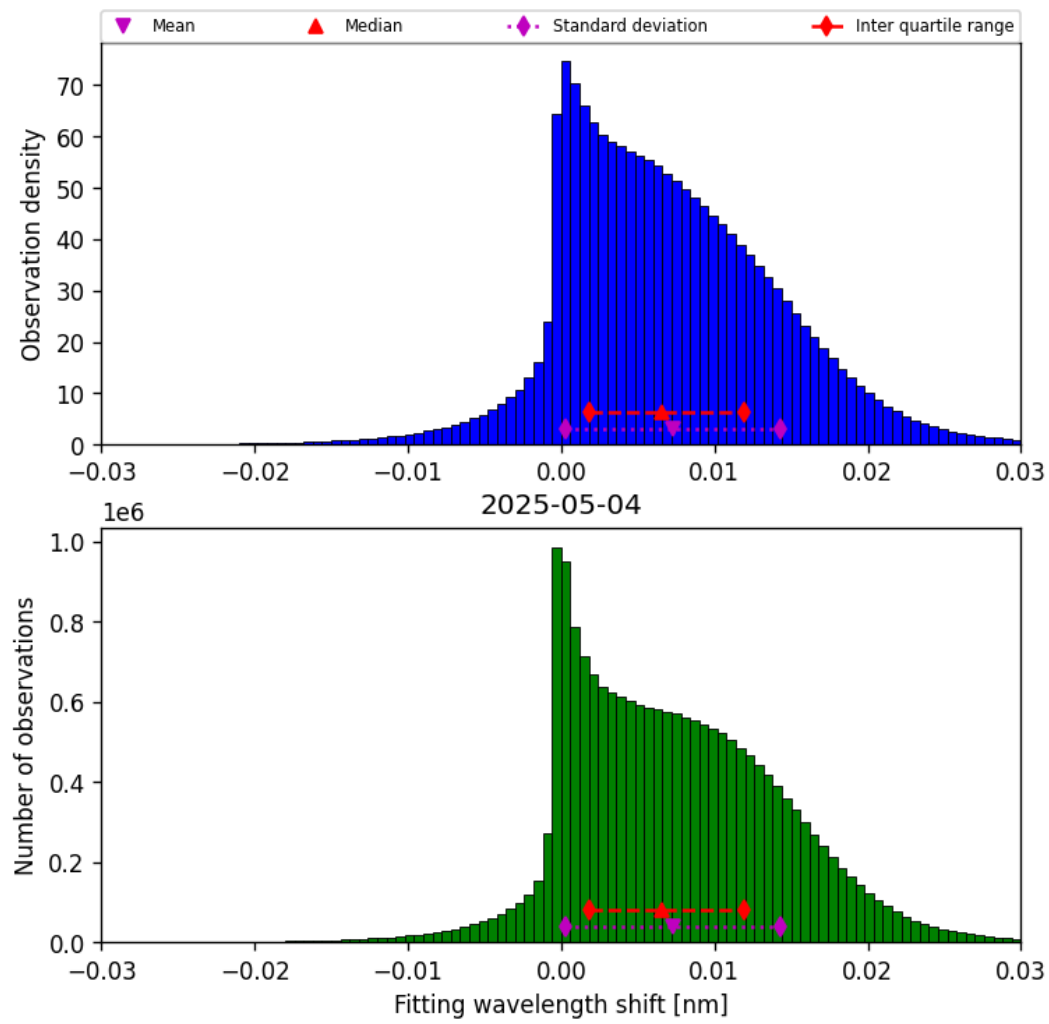
Figure 47: Histogram of “Fitting wavelength shift” for 2025-05-04 to 2025-05-05
