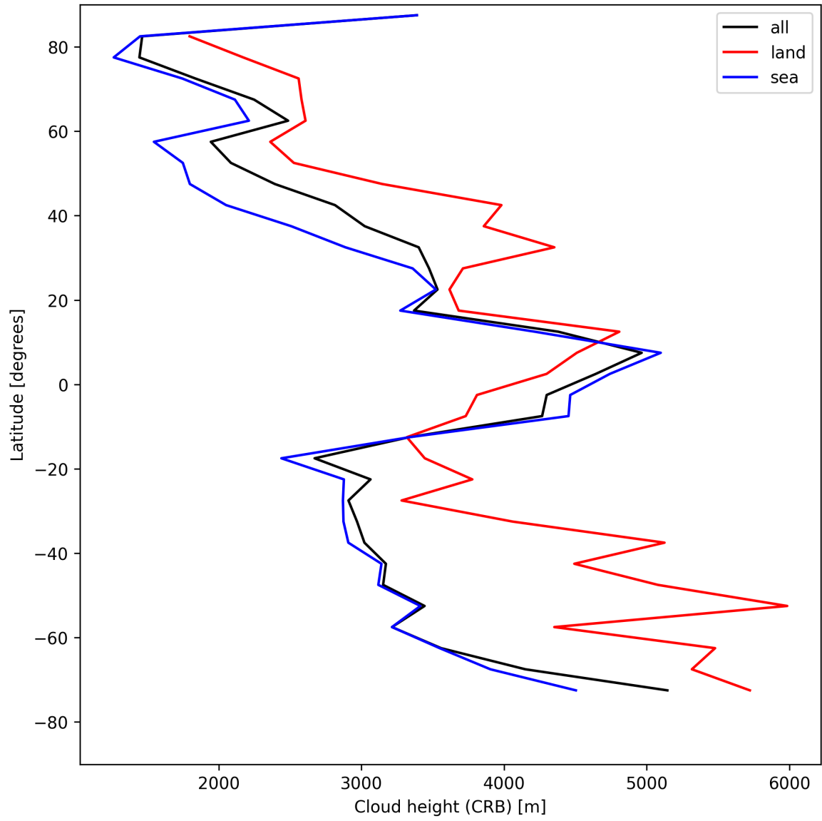
Figure 25: Zonal average of “Cloud height (CRB)” for 2025-05-04 to 2025-05-05.
