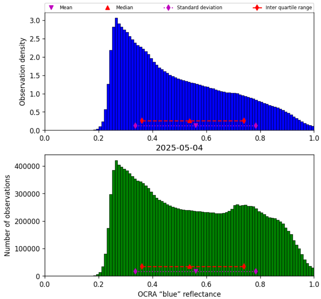
Figure 49: Histogram of “OCRA “blue” reflectance” for 2025-05-04 to 2025-05-05
