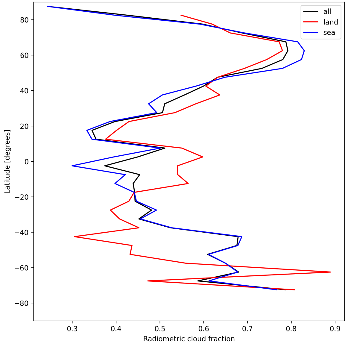
Figure 21: Zonal average of “Radiometric cloud fraction” for 2025-05-04 to 2025-05-05.
