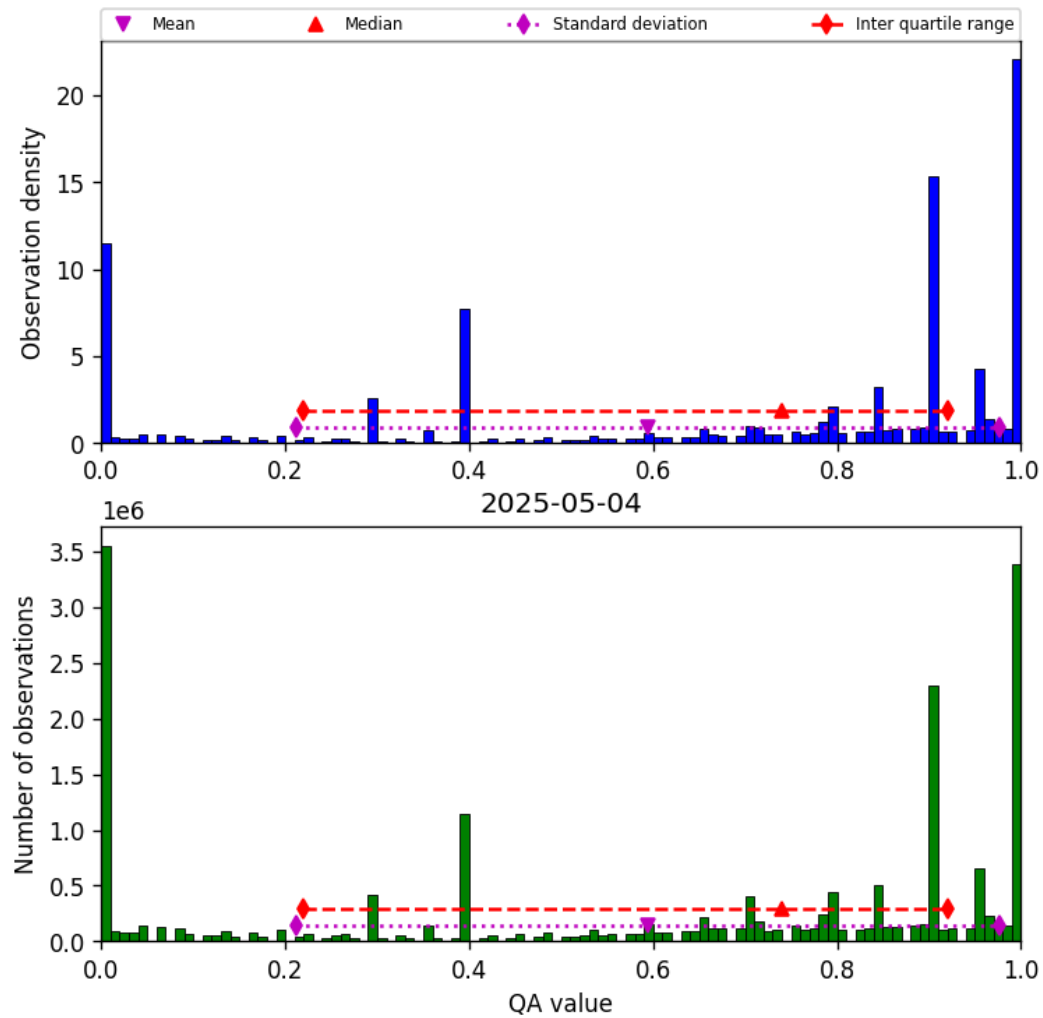
Figure 36: Histogram of “QA value” for 2025-05-04 to 2025-05-05
