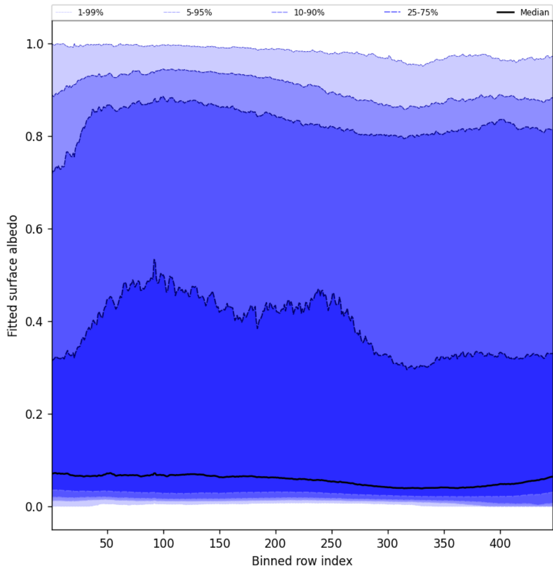
Figure 59: Along track statistics of “Fitted surface albedo” for 2025-05-04 to 2025-05-05
