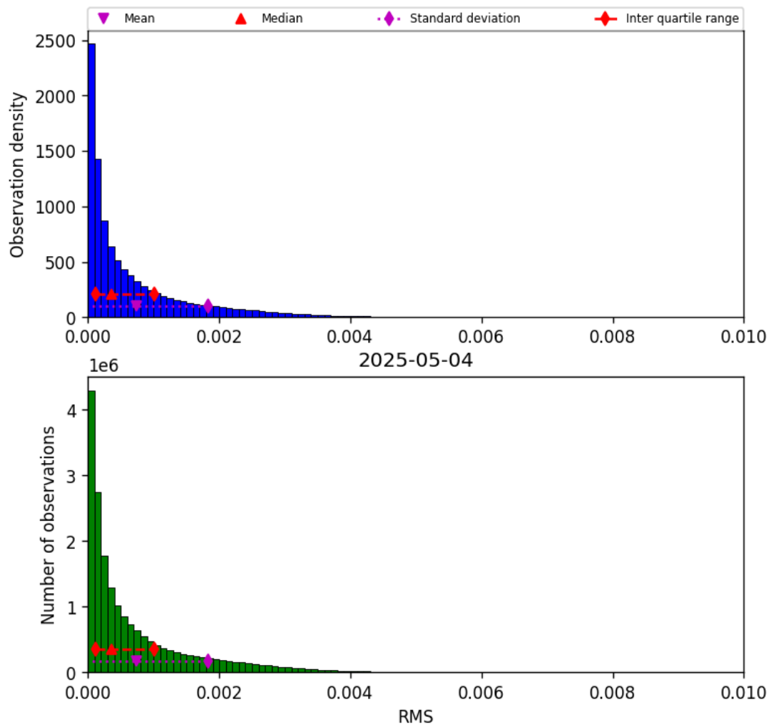
Figure 45: Histogram of “RMS” for 2025-05-04 to 2025-05-05
