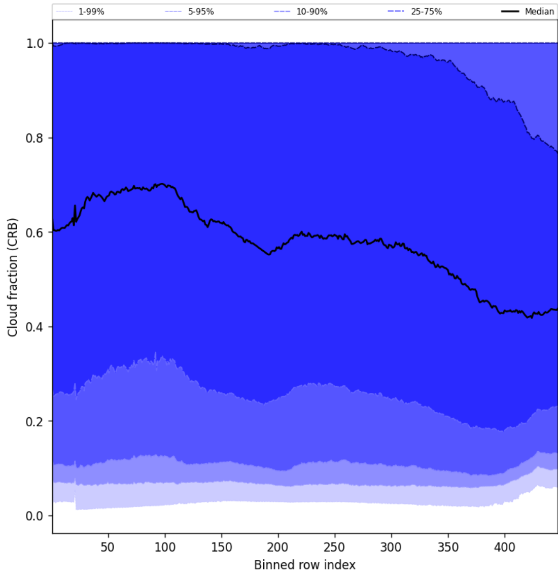
Figure 56: Along track statistics of “Cloud fraction (CRB)” for 2025-05-04 to 2025-05-05
