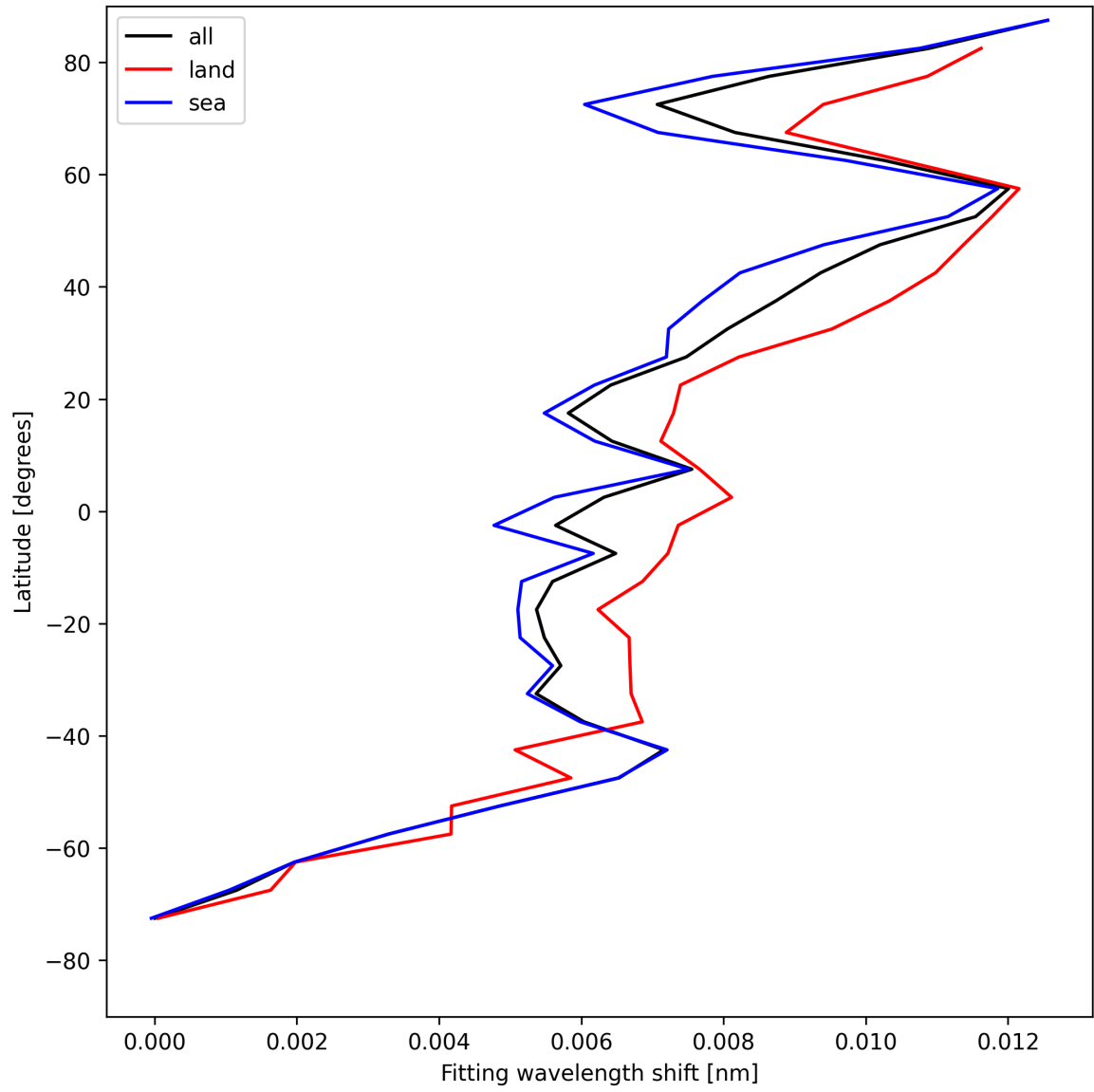
Figure 31: Zonal average of “Fitting wavelength shift” for 2025-05-04 to 2025-05-05.
