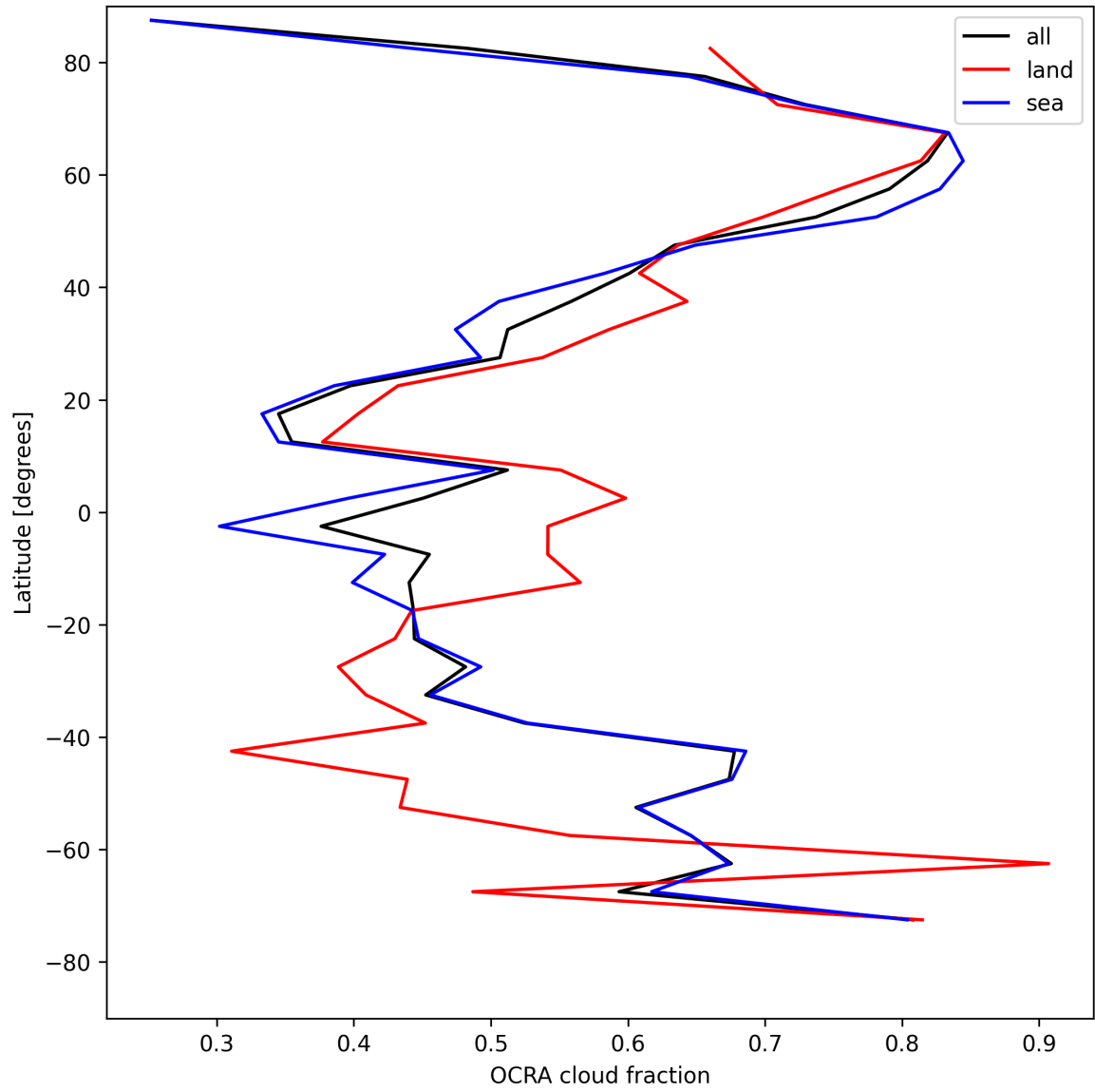
Figure 32: Zonal average of “OCRA cloud fraction” for 2025-05-04 to 2025-05-05.
