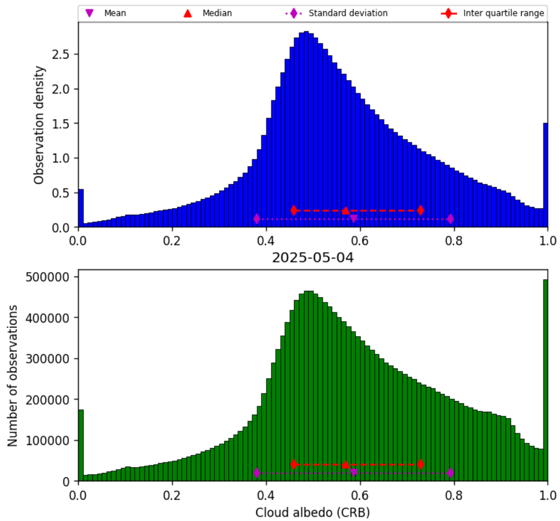
Figure 42: Histogram of “Cloud albedo (CRB)” for 2025-05-04 to 2025-05-05
