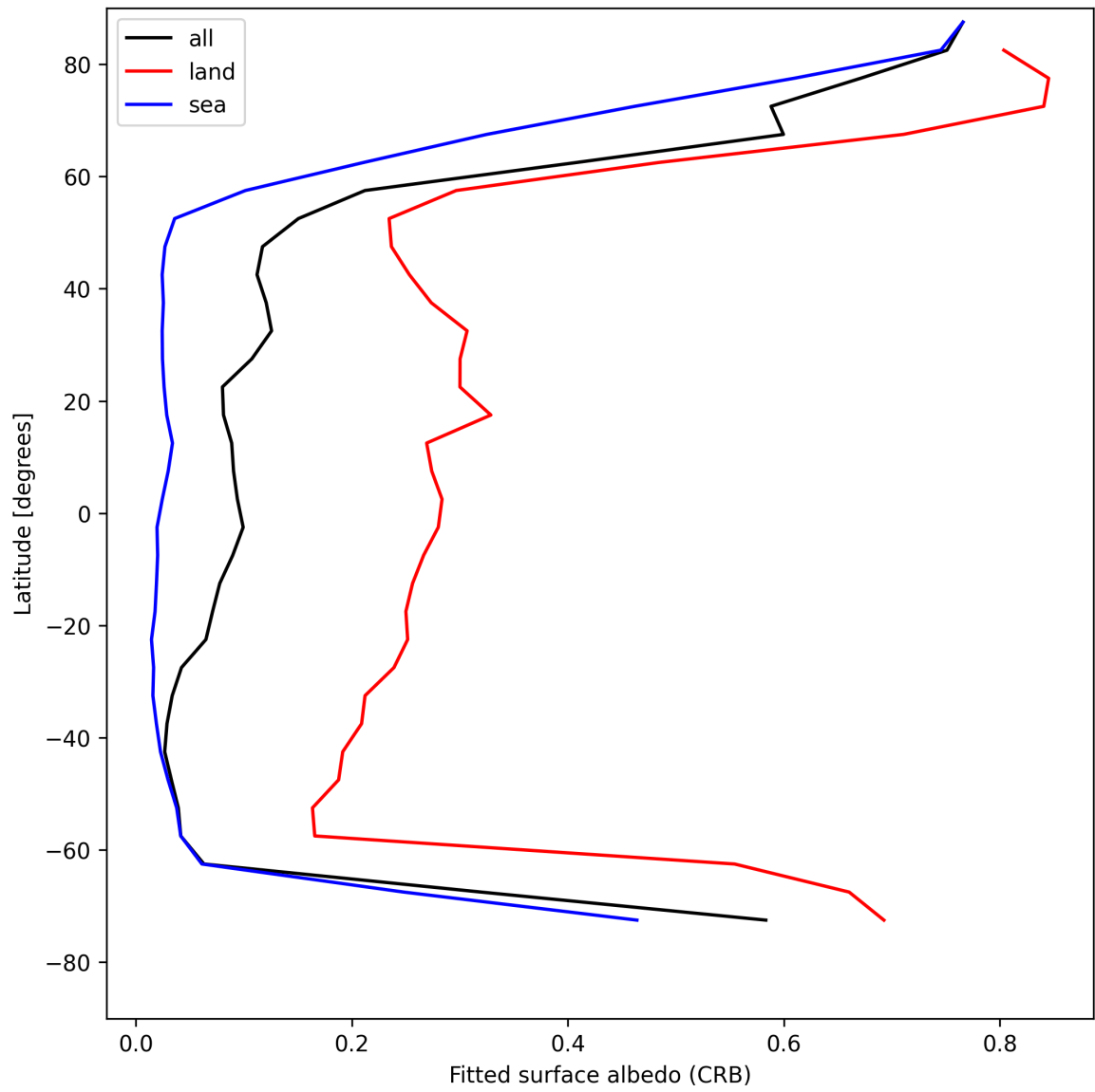
Figure 28: Zonal average of “Fitted surface albedo (CRB)” for 2025-05-04 to 2025-05-05.
