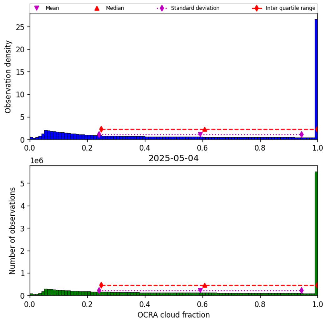
Figure 48: Histogram of “OCRA cloud fraction” for 2025-05-04 to 2025-05-05
