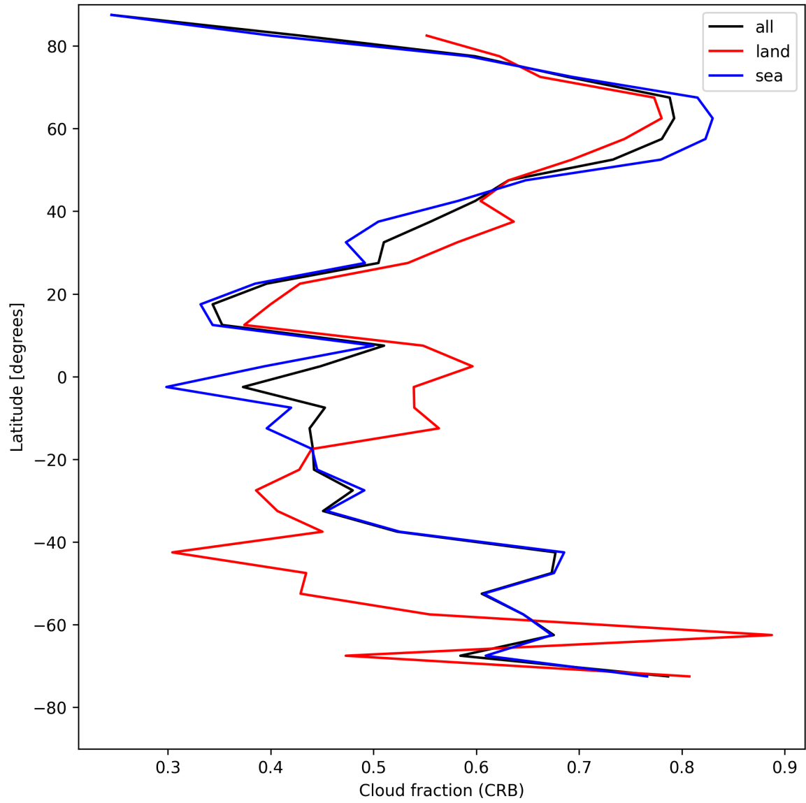
Figure 24: Zonal average of “Cloud fraction (CRB)” for 2025-05-04 to 2025-05-05.
