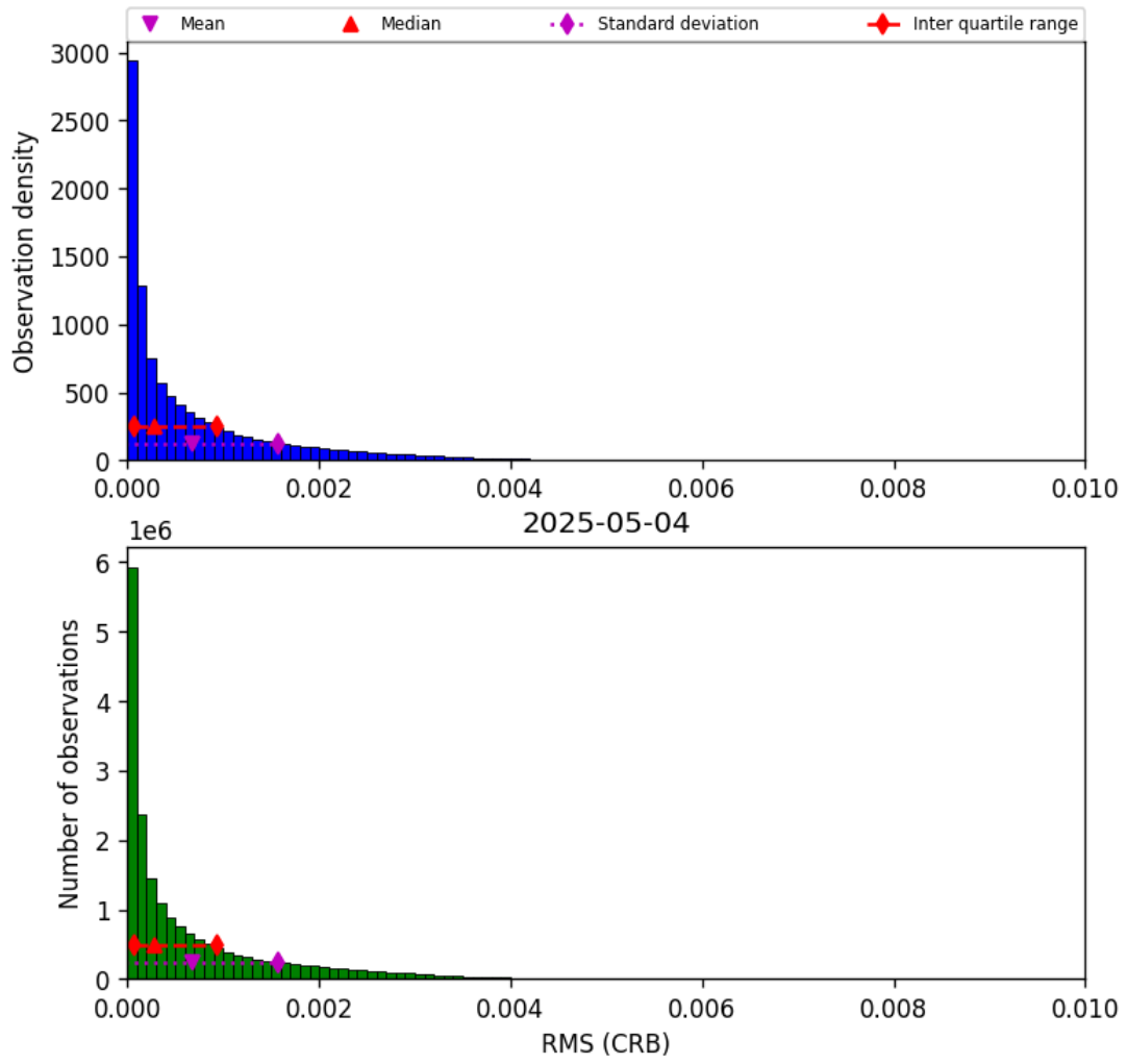
Figure 46: Histogram of “RMS (CRB)” for 2025-05-04 to 2025-05-05
