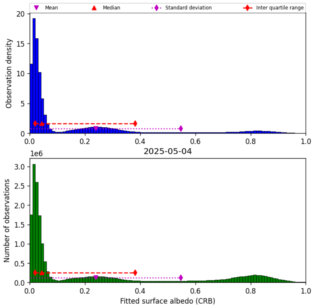
Figure 44: Histogram of “Fitted surface albedo (CRB)” for 2025-05-04 to 2025-05-05
