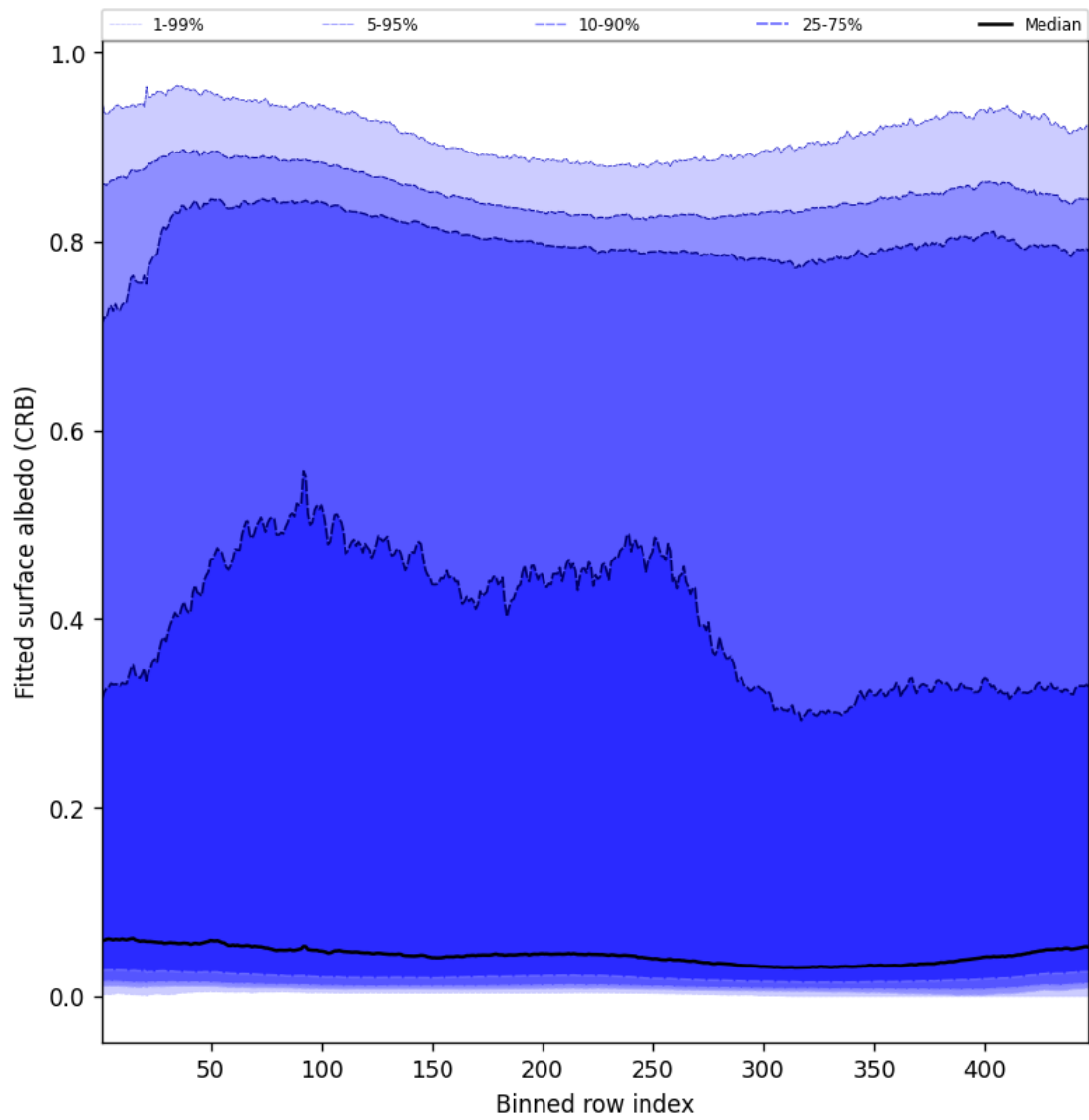
Figure 60: Along track statistics of “Fitted surface albedo (CRB)” for 2025-05-04 to 2025-05-05
