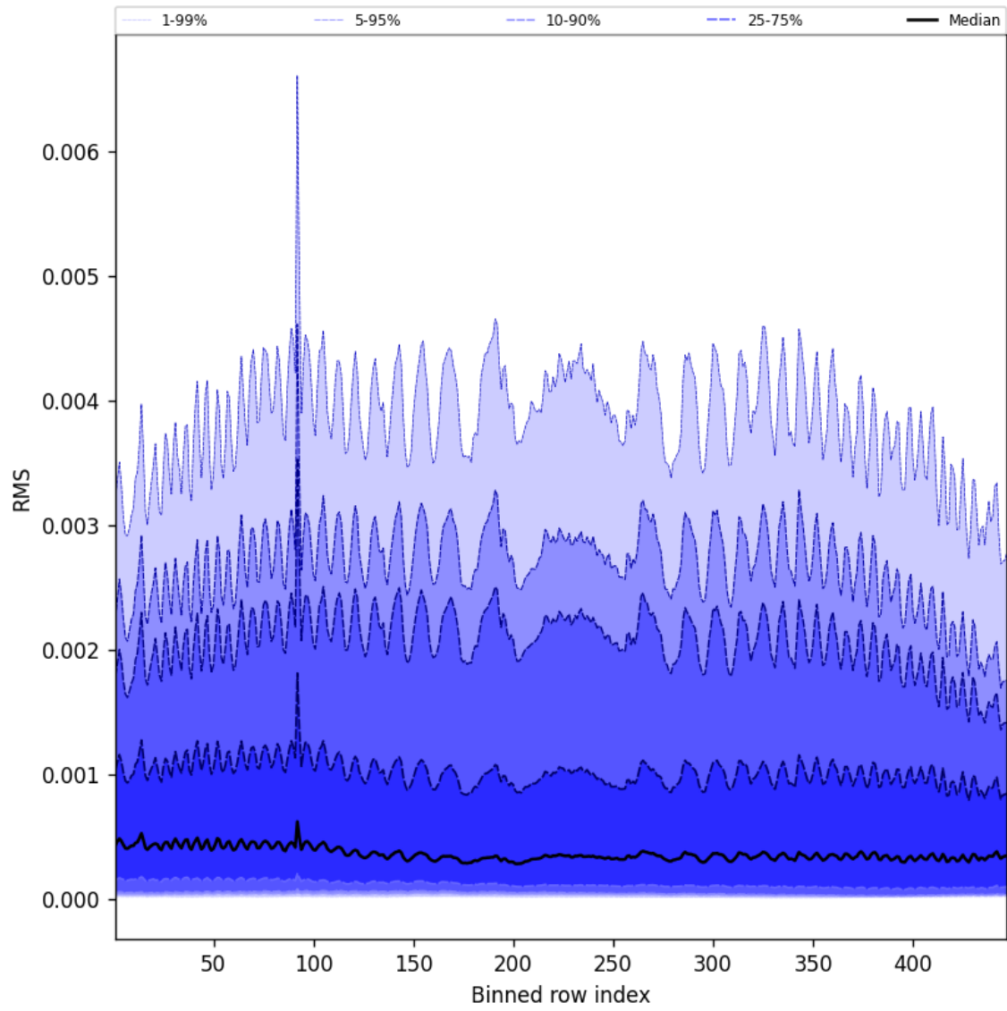
Figure 61: Along track statistics of “RMS” for 2025-05-04 to 2025-05-05
