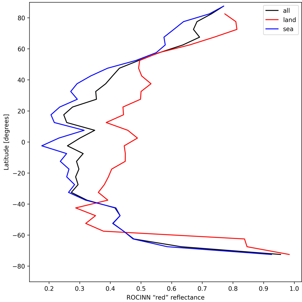
Figure 35: Zonal average of “ROCINN “red” reflectance” for 2025-05-04 to 2025-05-05.
