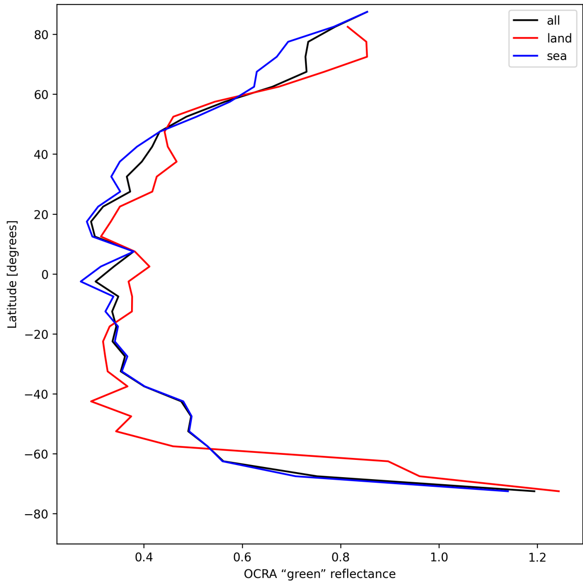
Figure 34: Zonal average of “OCRA “green” reflectance” for 2025-05-04 to 2025-05-05.
