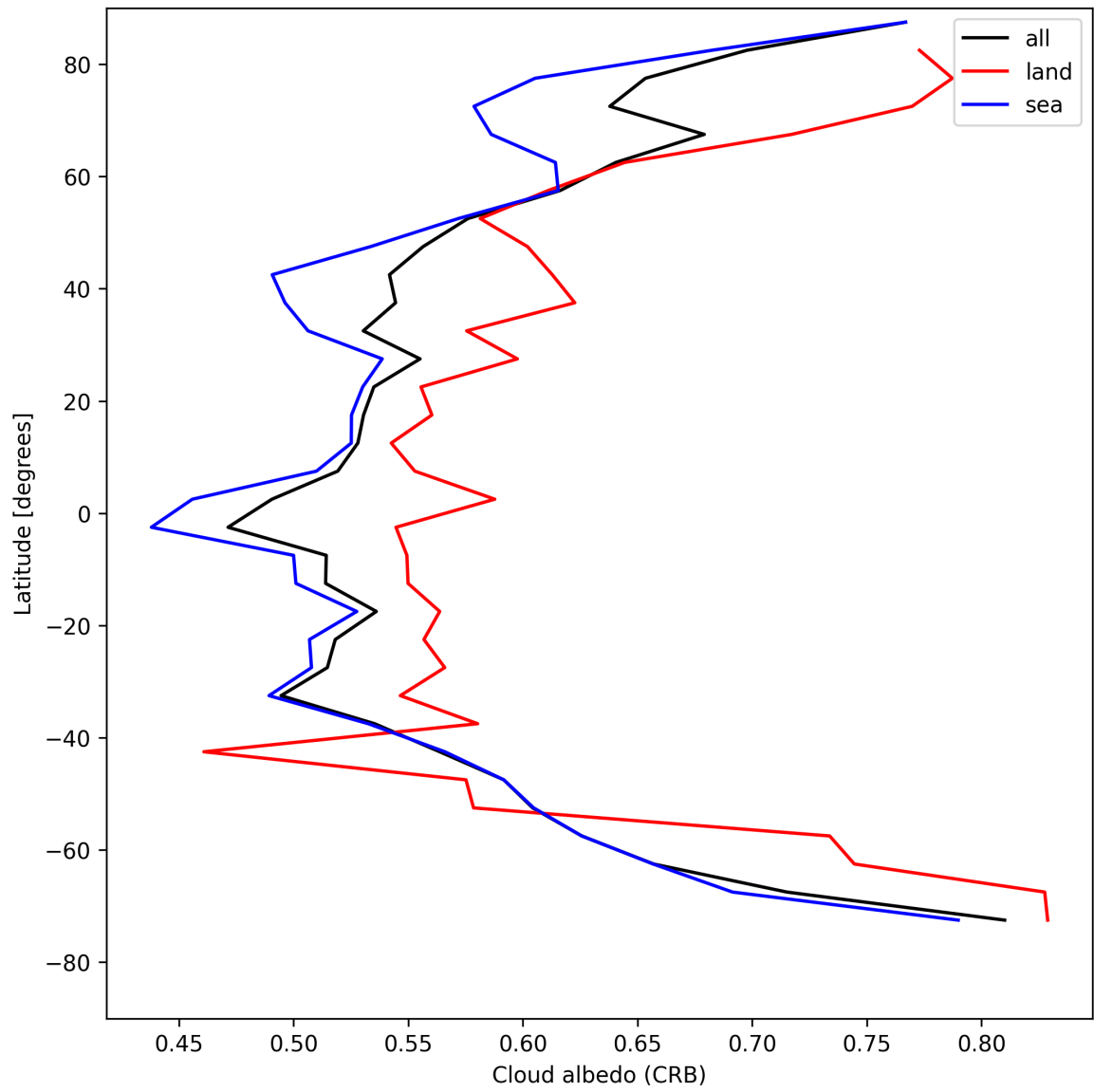
Figure 26: Zonal average of “Cloud albedo (CRB)” for 2025-05-04 to 2025-05-05.
