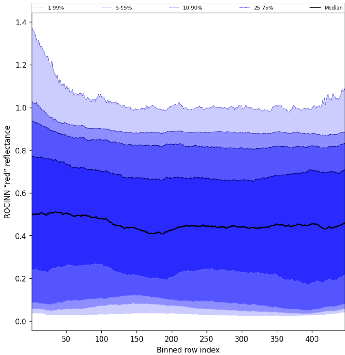
Figure 67: Along track statistics of “ROCINN “red” reflectance” for 2025-05-04 to 2025-05-05
