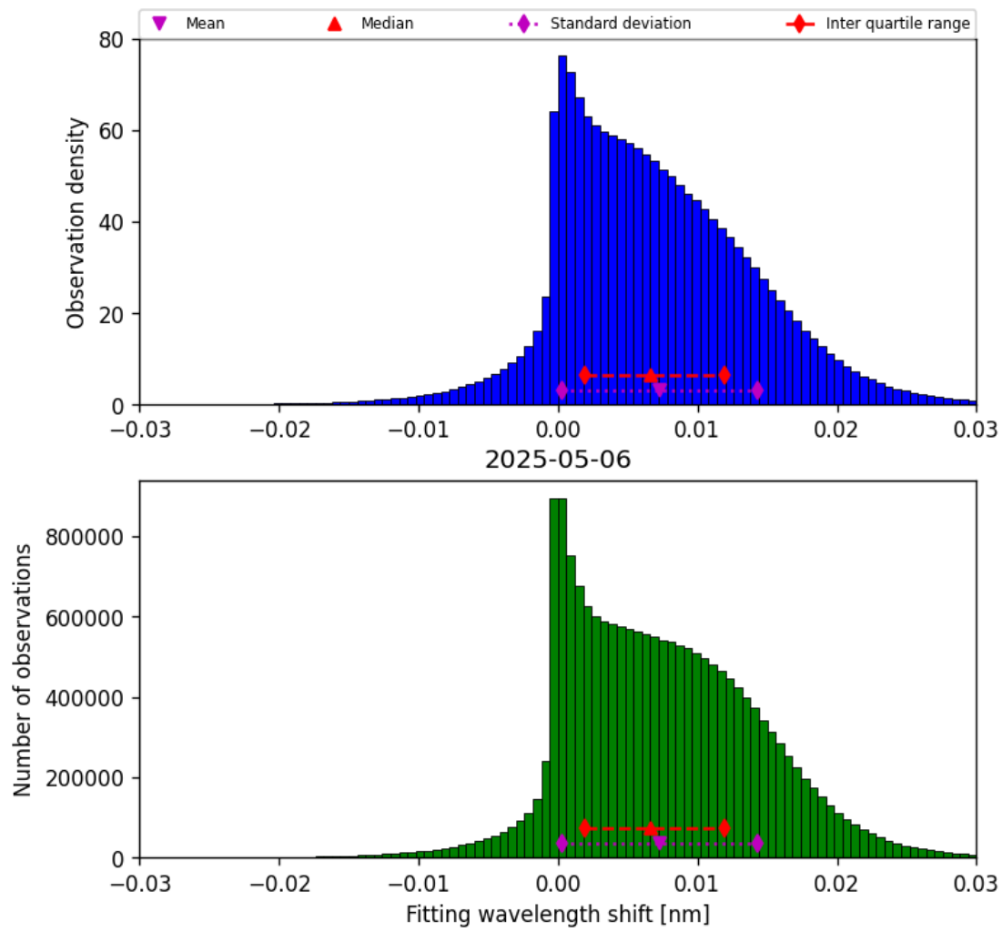
Figure 47: Histogram of “Fitting wavelength shift” for 2025-05-06 to 2025-05-07
