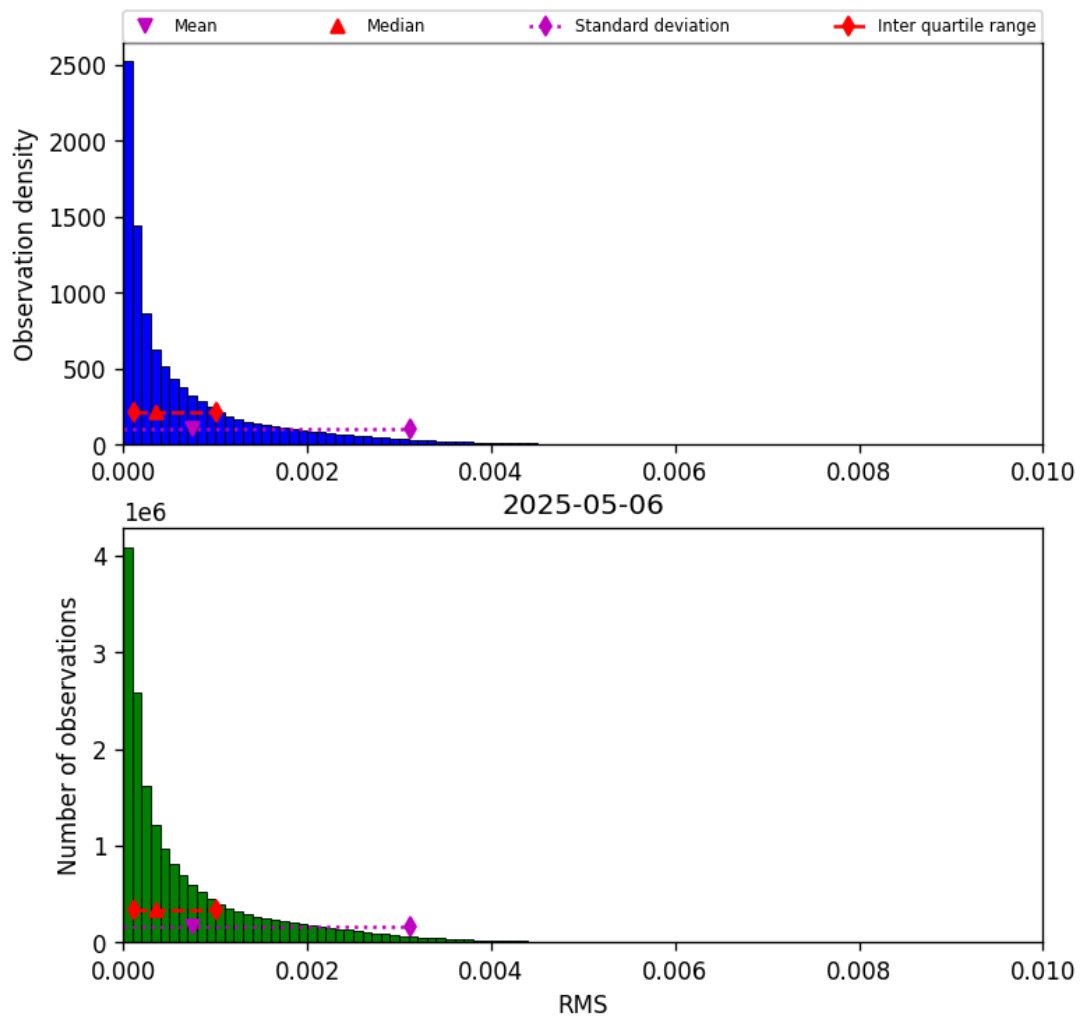
Figure 45: Histogram of “RMS” for 2025-05-06 to 2025-05-07
