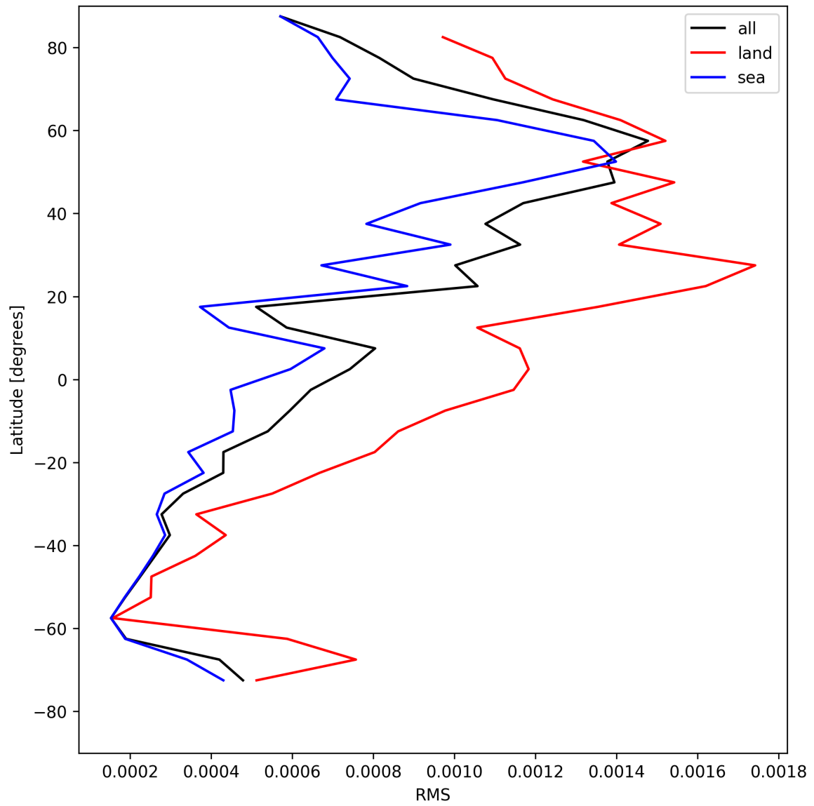
Figure 29: Zonal average of “RMS” for 2025-05-06 to 2025-05-07.
