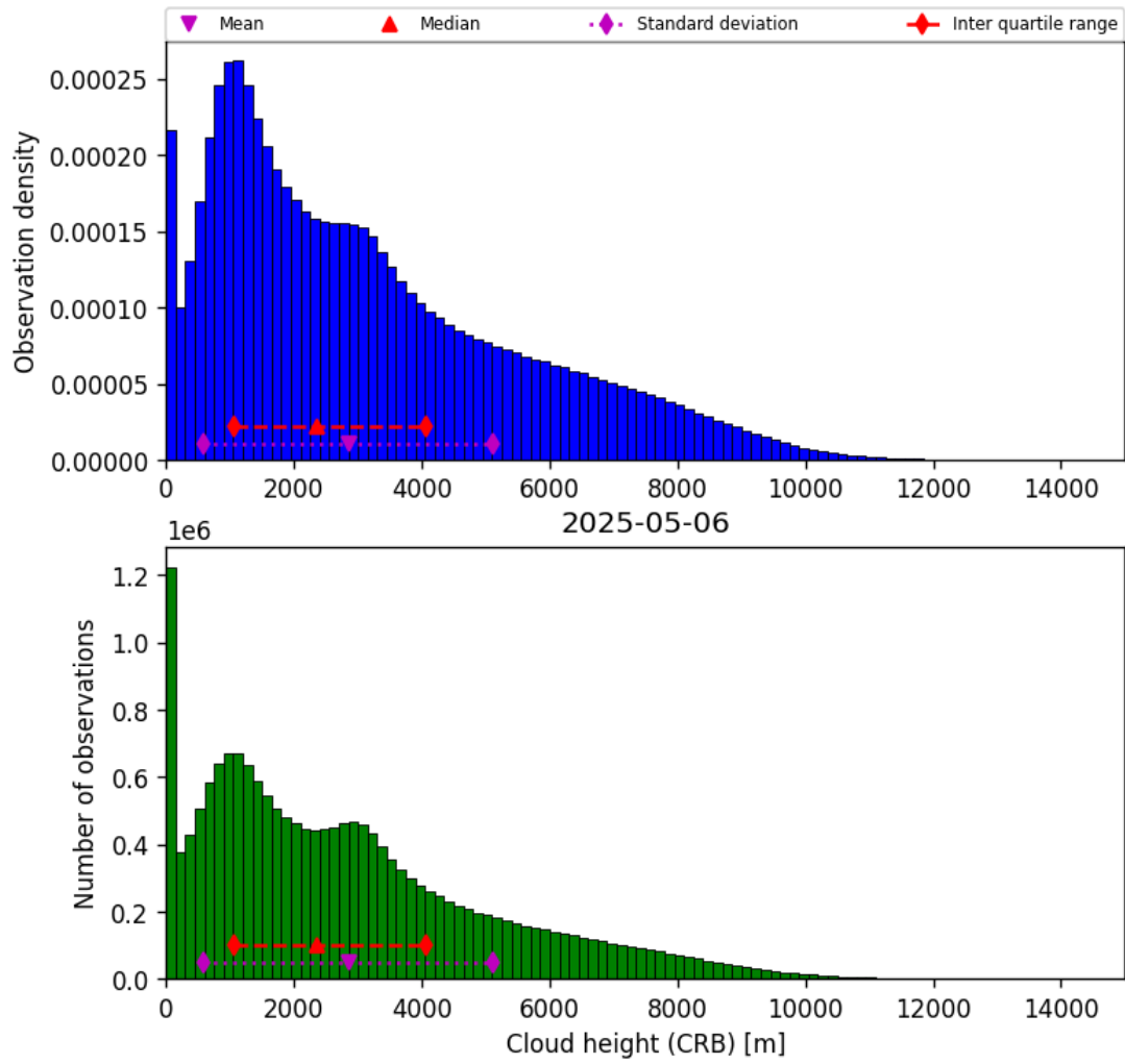
Figure 41: Histogram of “Cloud height (CRB)” for 2025-05-06 to 2025-05-07
