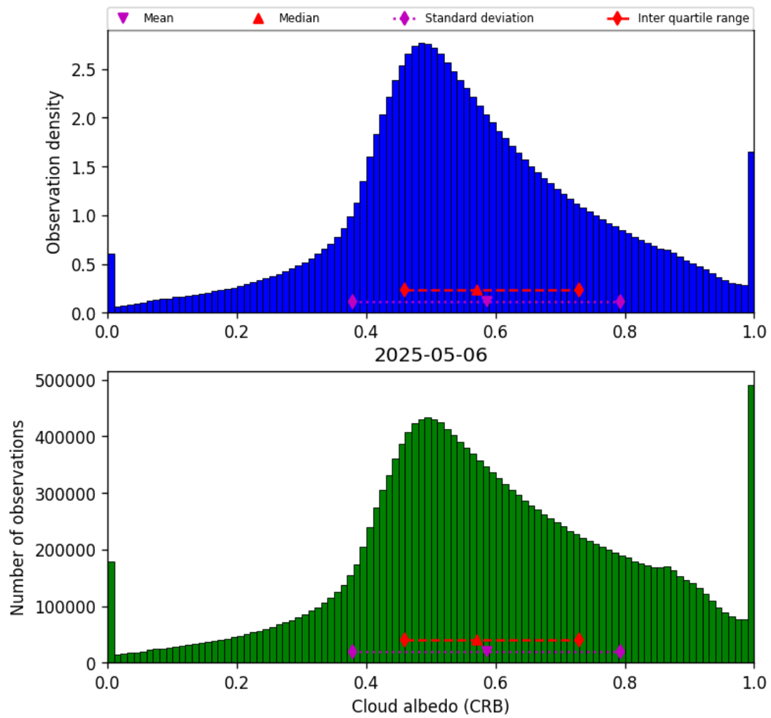
Figure 42: Histogram of “Cloud albedo (CRB)” for 2025-05-06 to 2025-05-07
