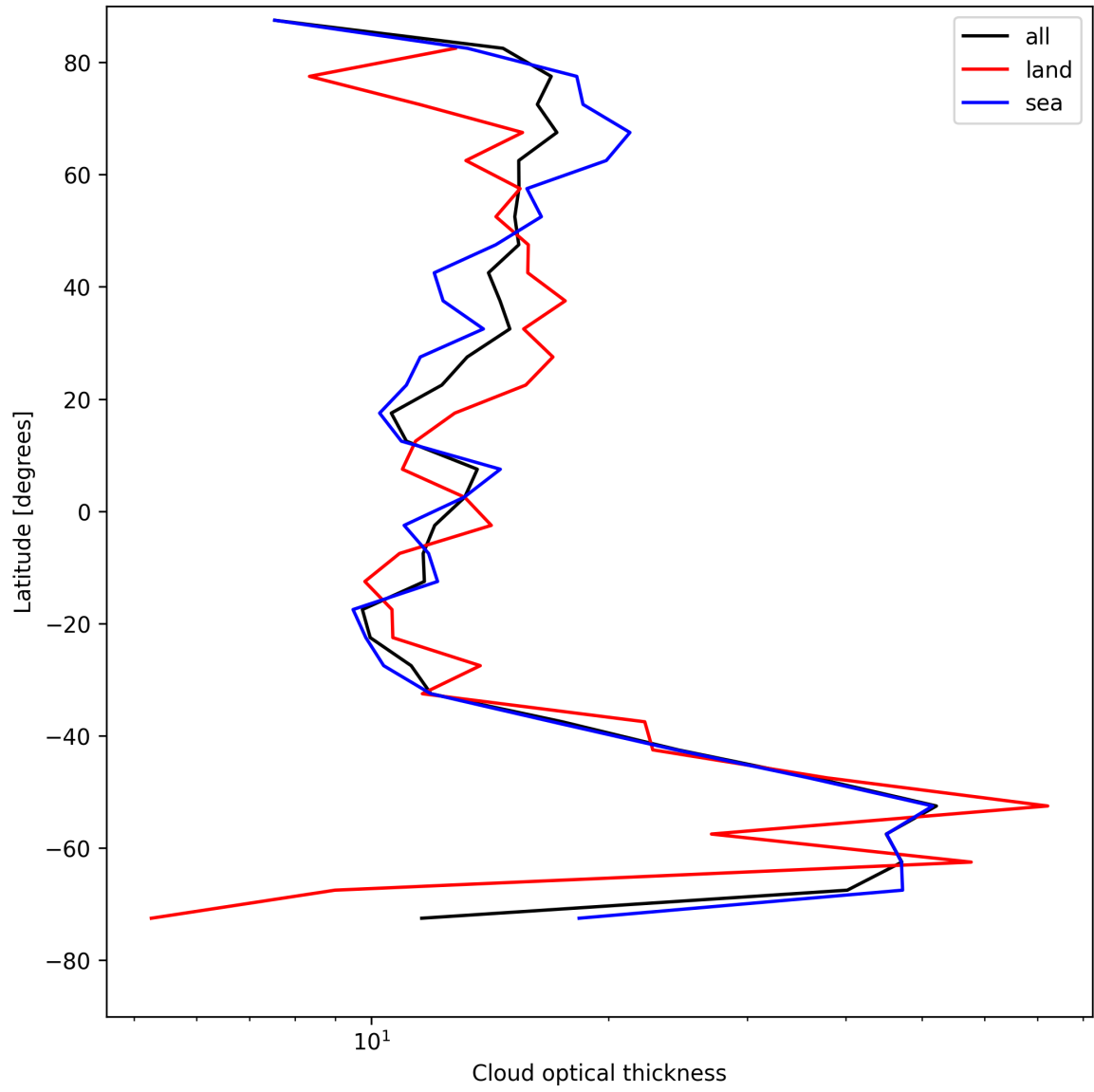
Figure 23: Zonal average of “Cloud optical thickness” for 2025-05-06 to 2025-05-07.
