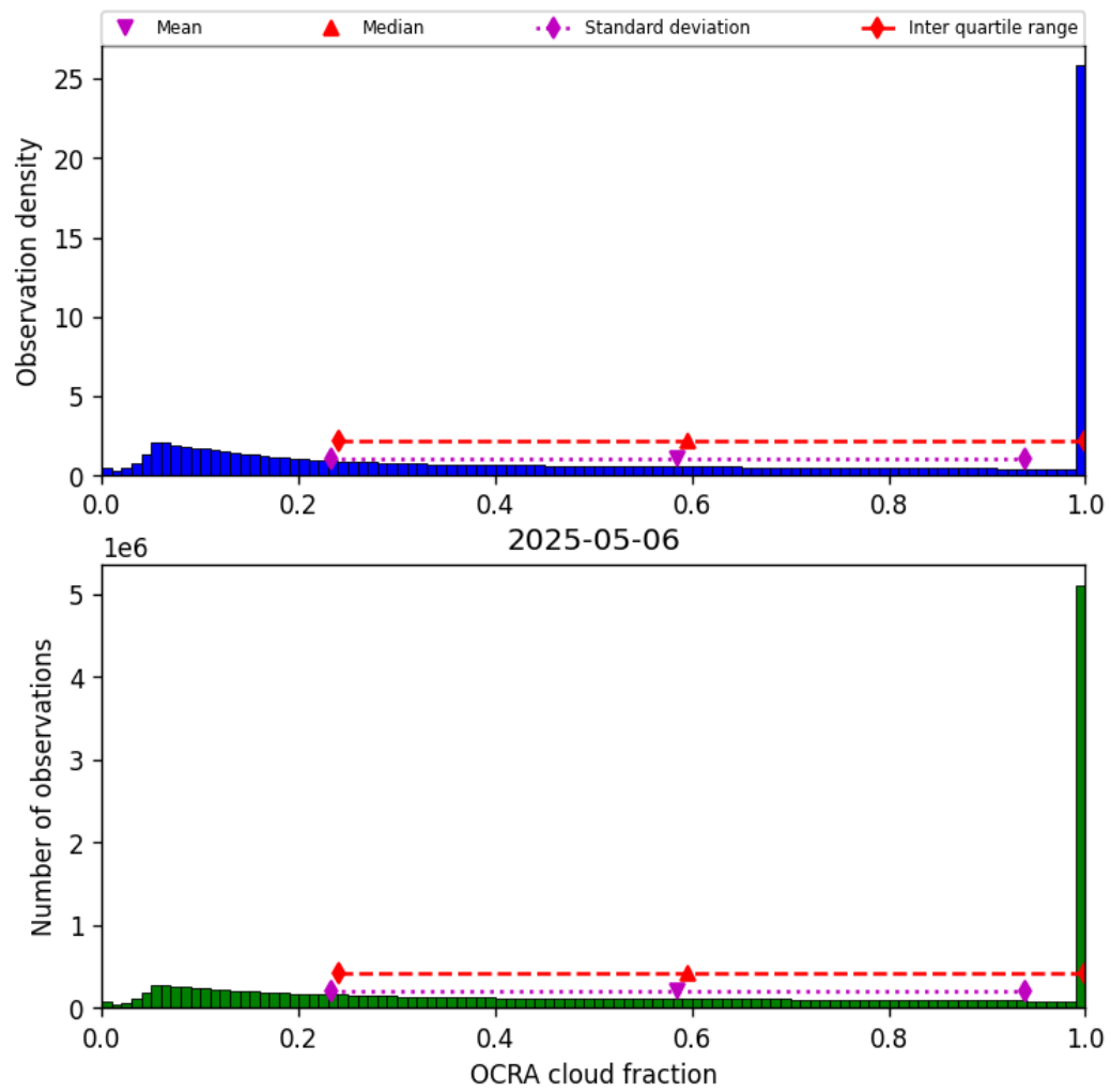
Figure 48: Histogram of “OCRA cloud fraction” for 2025-05-06 to 2025-05-07
