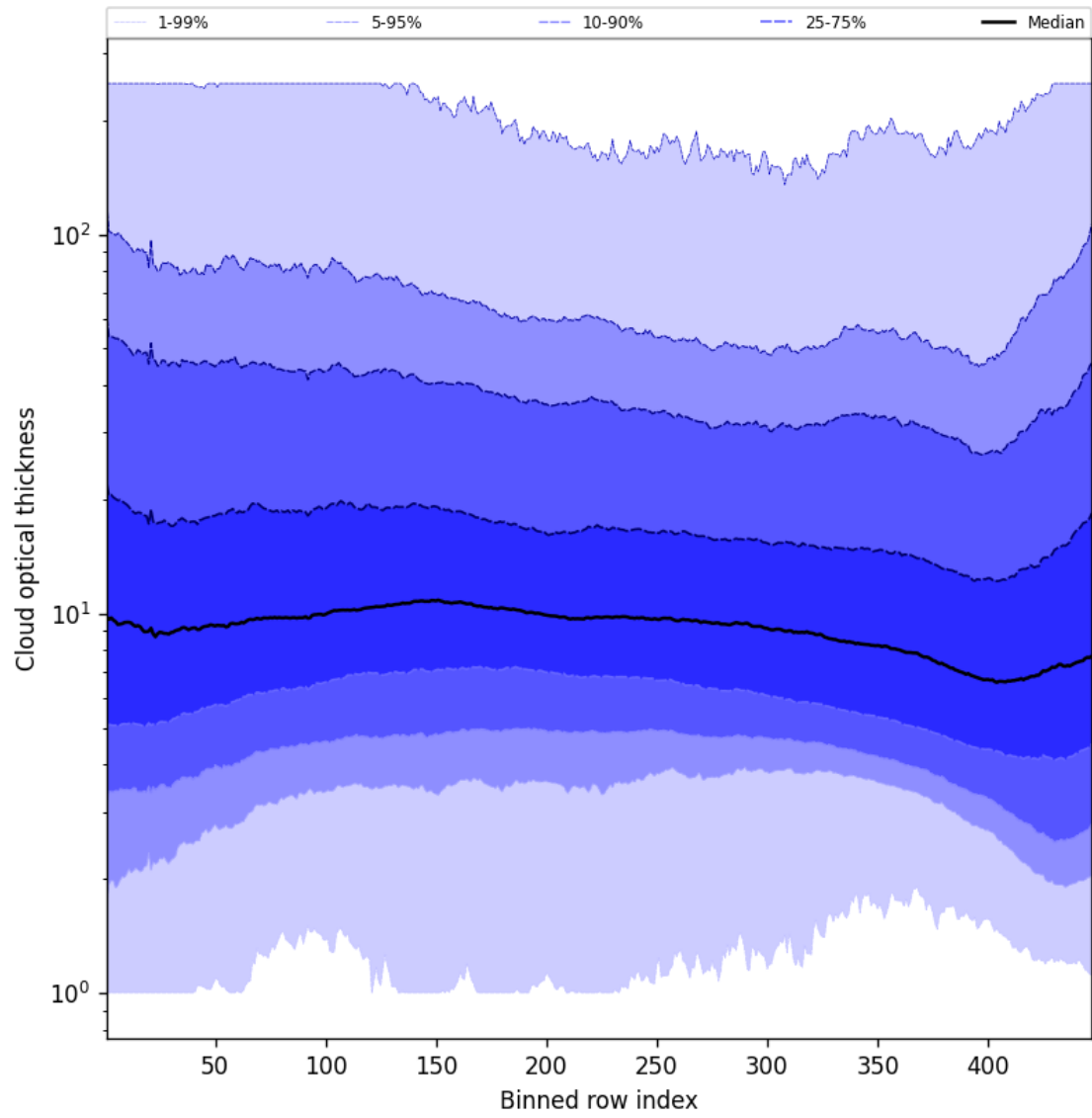
Figure 55: Along track statistics of “Cloud optical thickness” for 2025-05-06 to 2025-05-07
