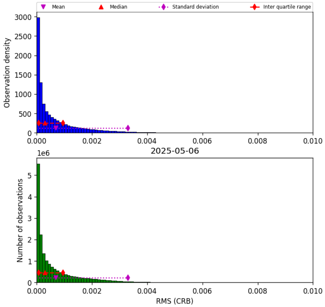
Figure 46: Histogram of “RMS (CRB)” for 2025-05-06 to 2025-05-07
