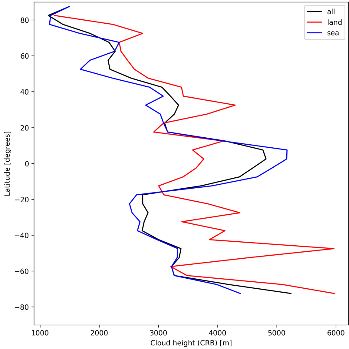
Figure 25: Zonal average of “Cloud height (CRB)” for 2025-05-06 to 2025-05-07.
