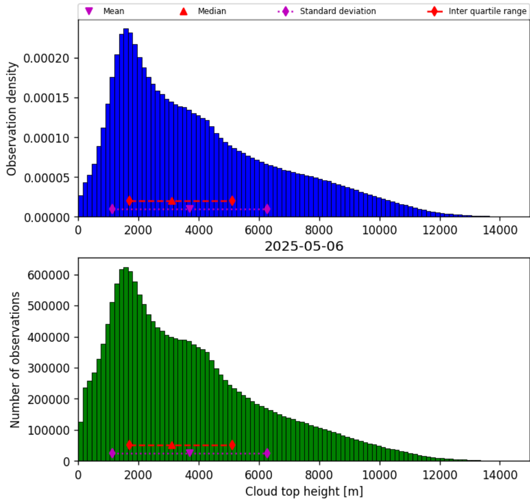
Figure 38: Histogram of “Cloud top height” for 2025-05-06 to 2025-05-07
